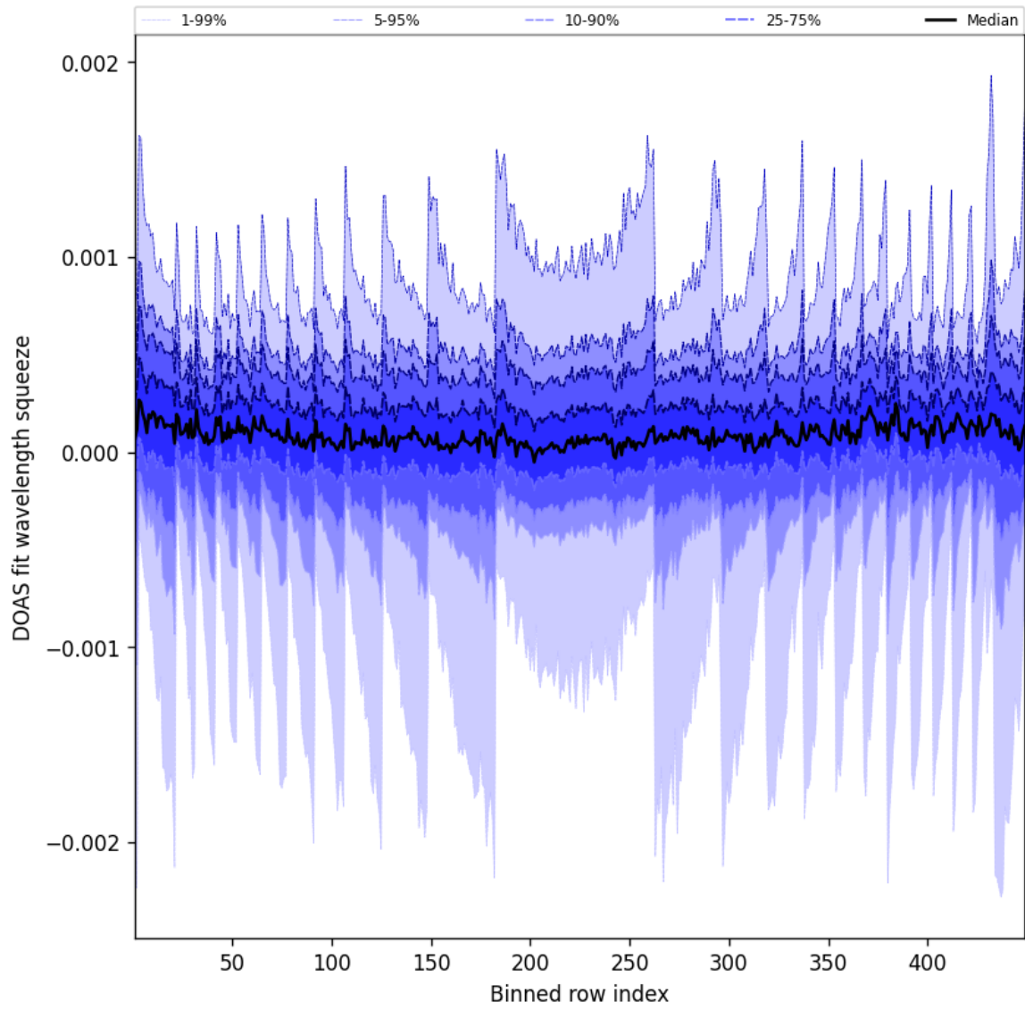
Figure 48: Along track statistics of “DOAS fit wavelength squeeze” for 2025-07-28 to 2025-07-29
