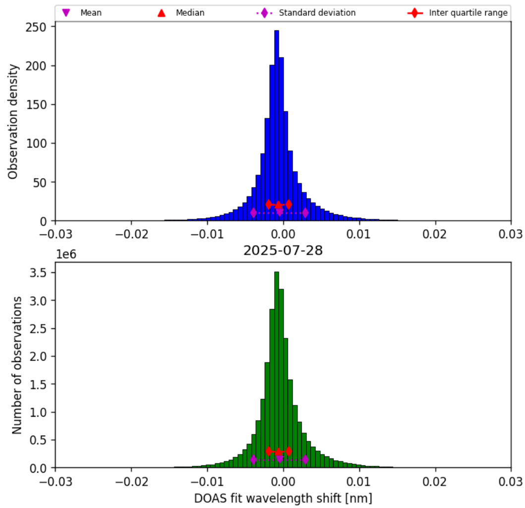
Figure 35: Histogram of “DOAS fit wavelength shift” for 2025-07-28 to 2025-07-29
