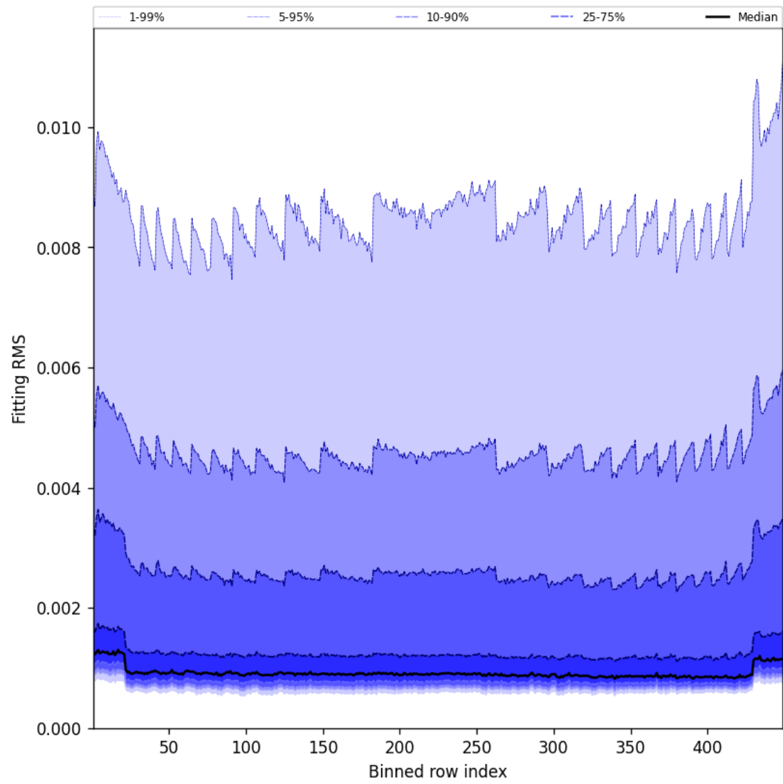
Figure 46: Along track statistics of “Fitting RMS” for 2025-07-28 to 2025-07-29
