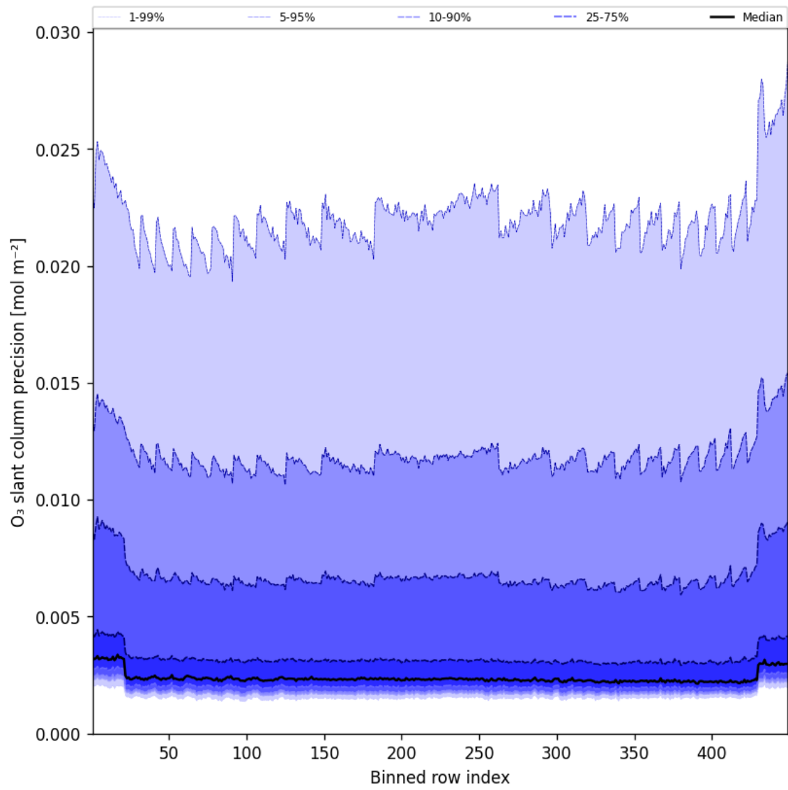
Figure 44: Along track statistics of “O 3 slant column precision” for 2025-07-28 to 2025-07-29
