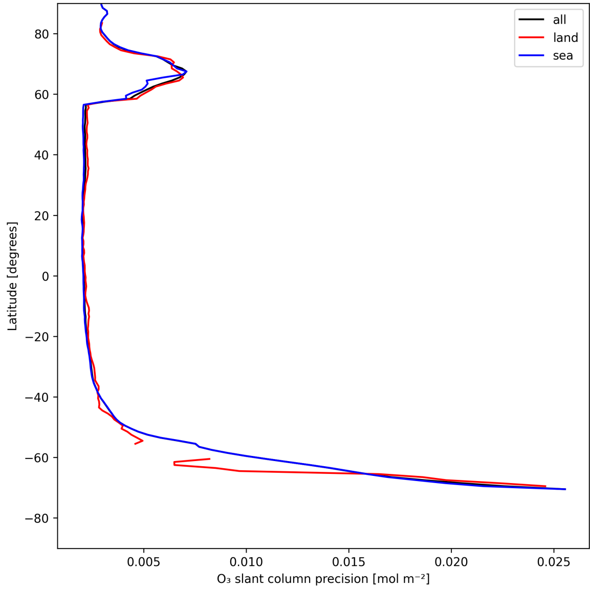
Figure 20: Zonal average of "O 3 slant column precision" for 2025-07-28 to 2025-07-29.
