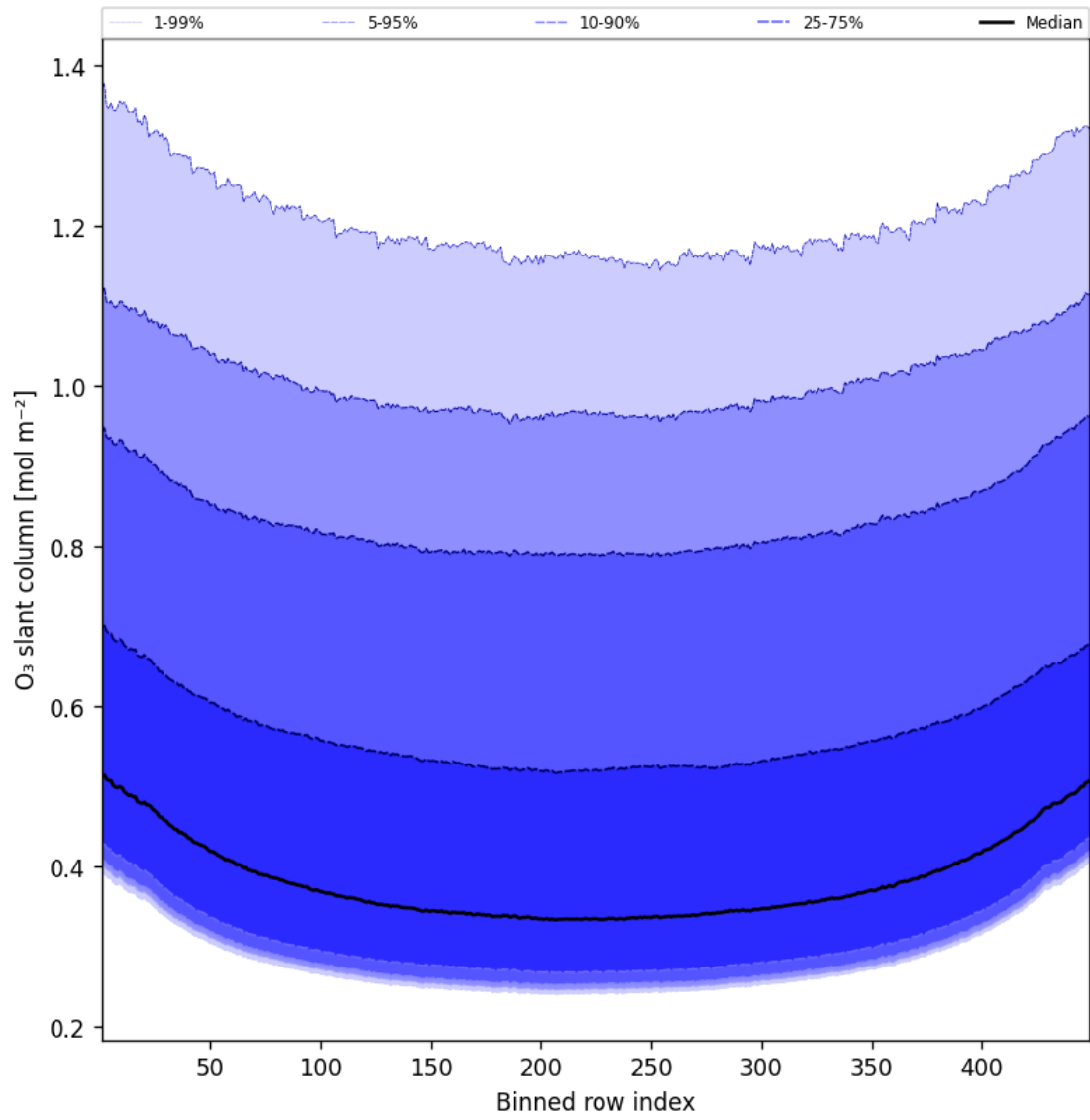
Figure 43: Along track statistics of “O 3 slant column” for 2025-07-28 to 2025-07-29
