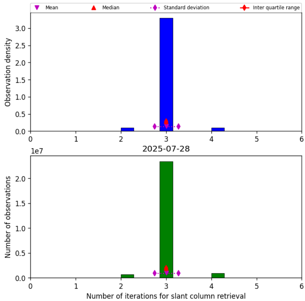
Figure 33: Histogram of “Number of iterations for slant column retrieval” for 2025-07-28 to 2025-07-29
