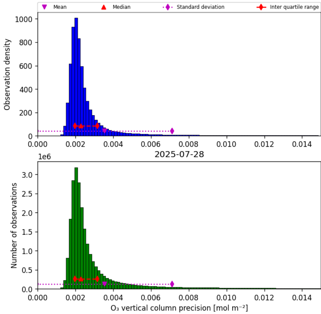
Figure 30: Histogram of “O 3 vertical column precision” for 2025-07-28 to 2025-07-29
