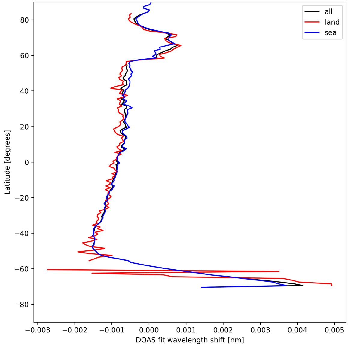
Figure 23: Zonal average of "DOAS fit wavelength shift" for 2025-07-28 to 2025-07-29.
