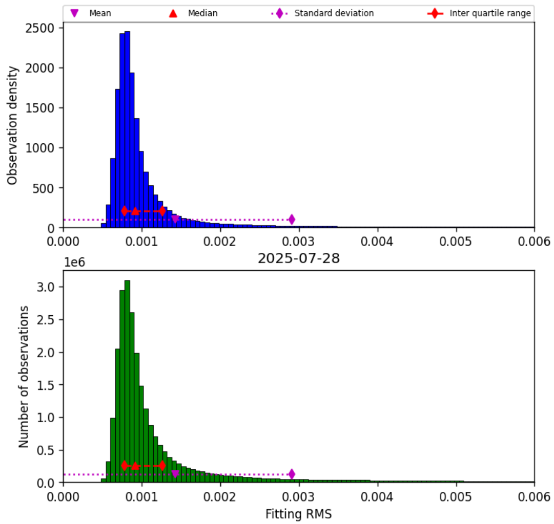
Figure 34: Histogram of “Fitting RMS” for 2025-07-28 to 2025-07-29
