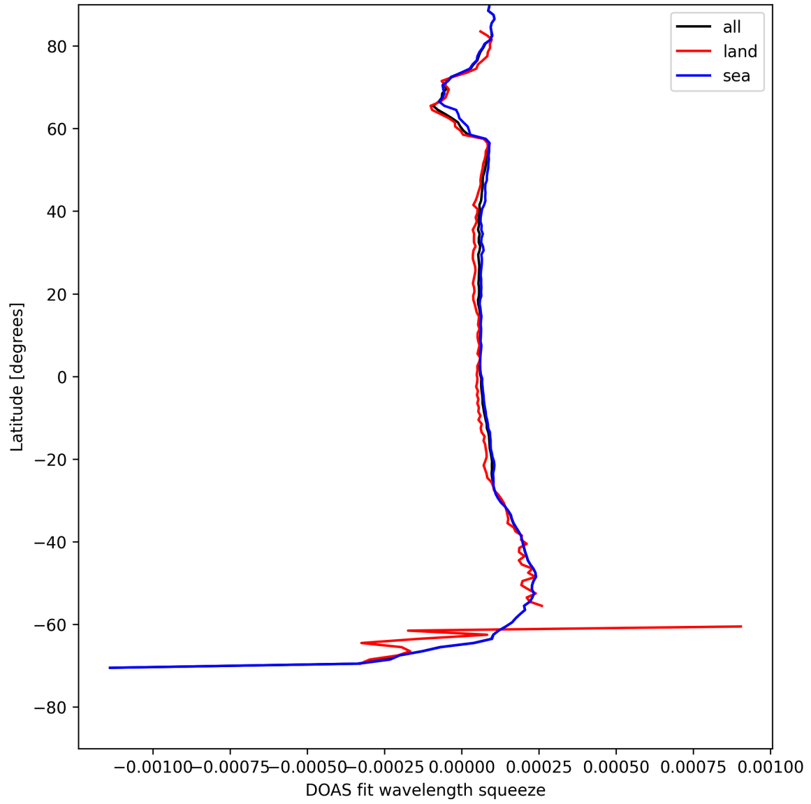
Figure 24: Zonal average of “DOAS fit wavelength squeeze” for 2025-07-28 to 2025-07-29.
