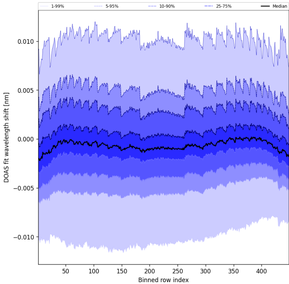
Figure 47: Along track statistics of “DOAS fit wavelength shift” for 2025-07-28 to 2025-07-29
