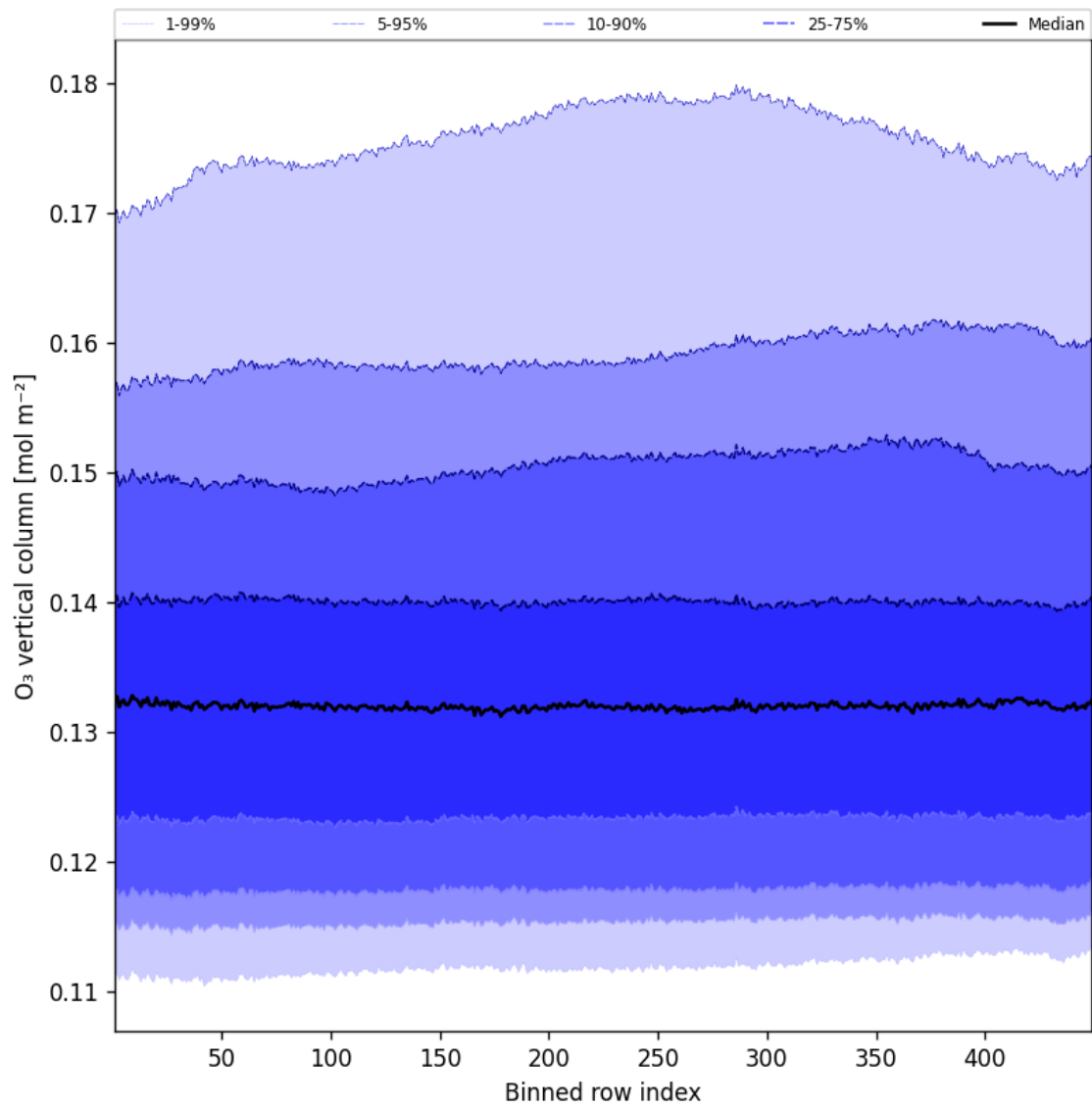
Figure 41: Along track statistics of “O 3 vertical column” for 2025-07-28 to 2025-07-29
