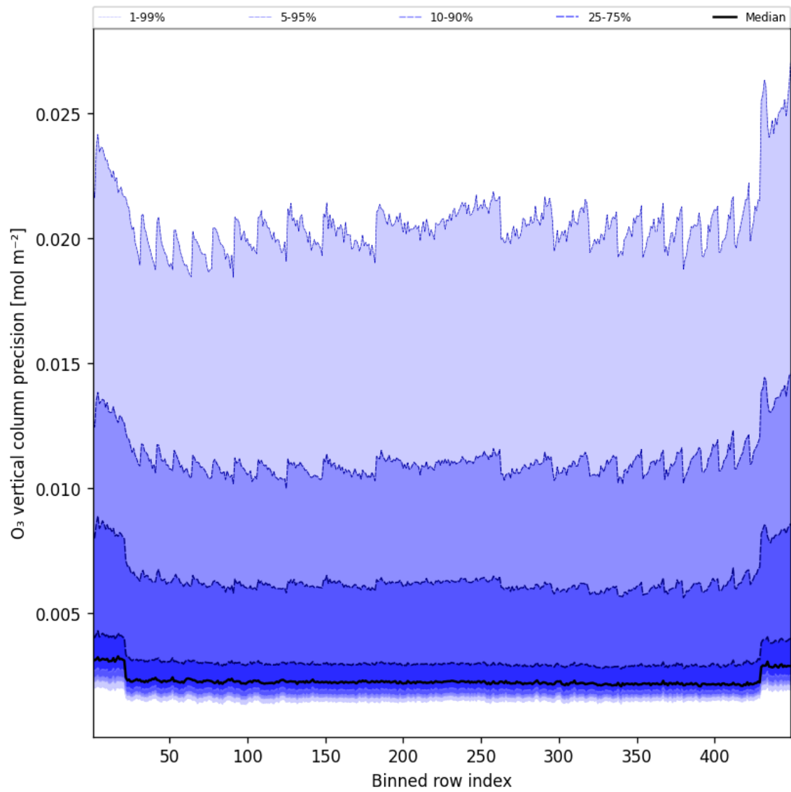
Figure 42: Along track statistics of “O 3 vertical column precision” for 2025-07-28 to 2025-07-29
