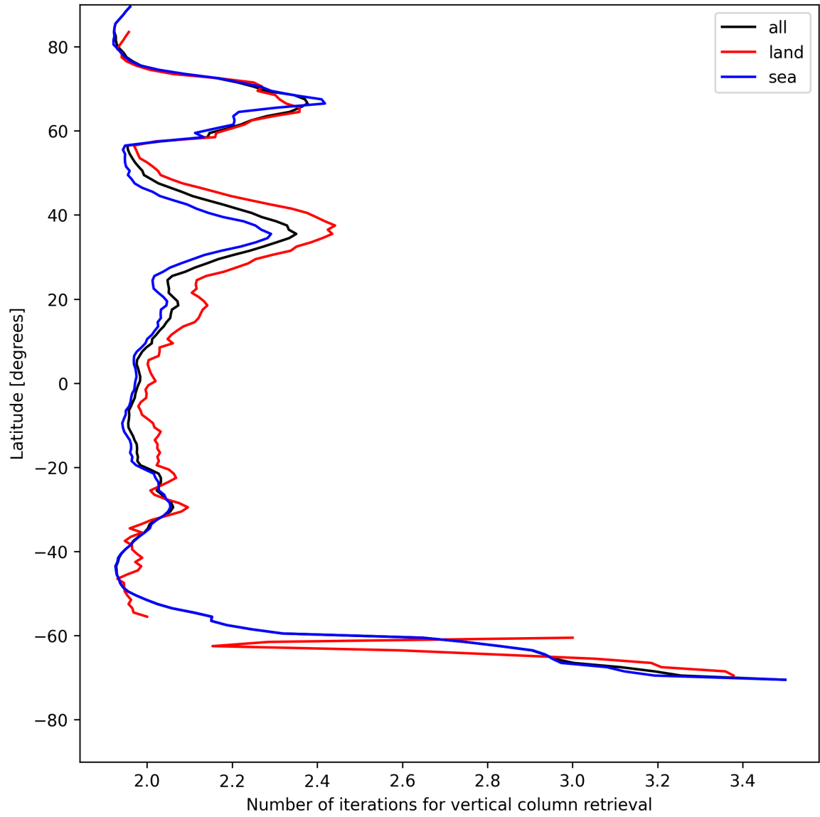
Figure 27: Zonal average of “Number of iterations for vertical column retrieval” for 2025-07-28 to 2025-07-29.
