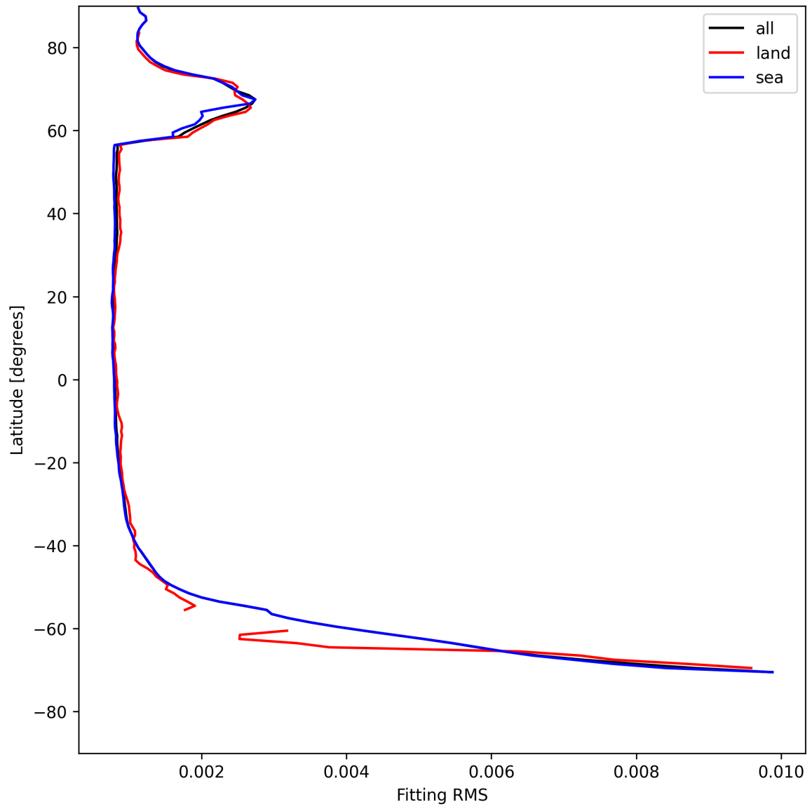
Figure 22: Zonal average of “Fitting RMS” for 2025-07-28 to 2025-07-29.
