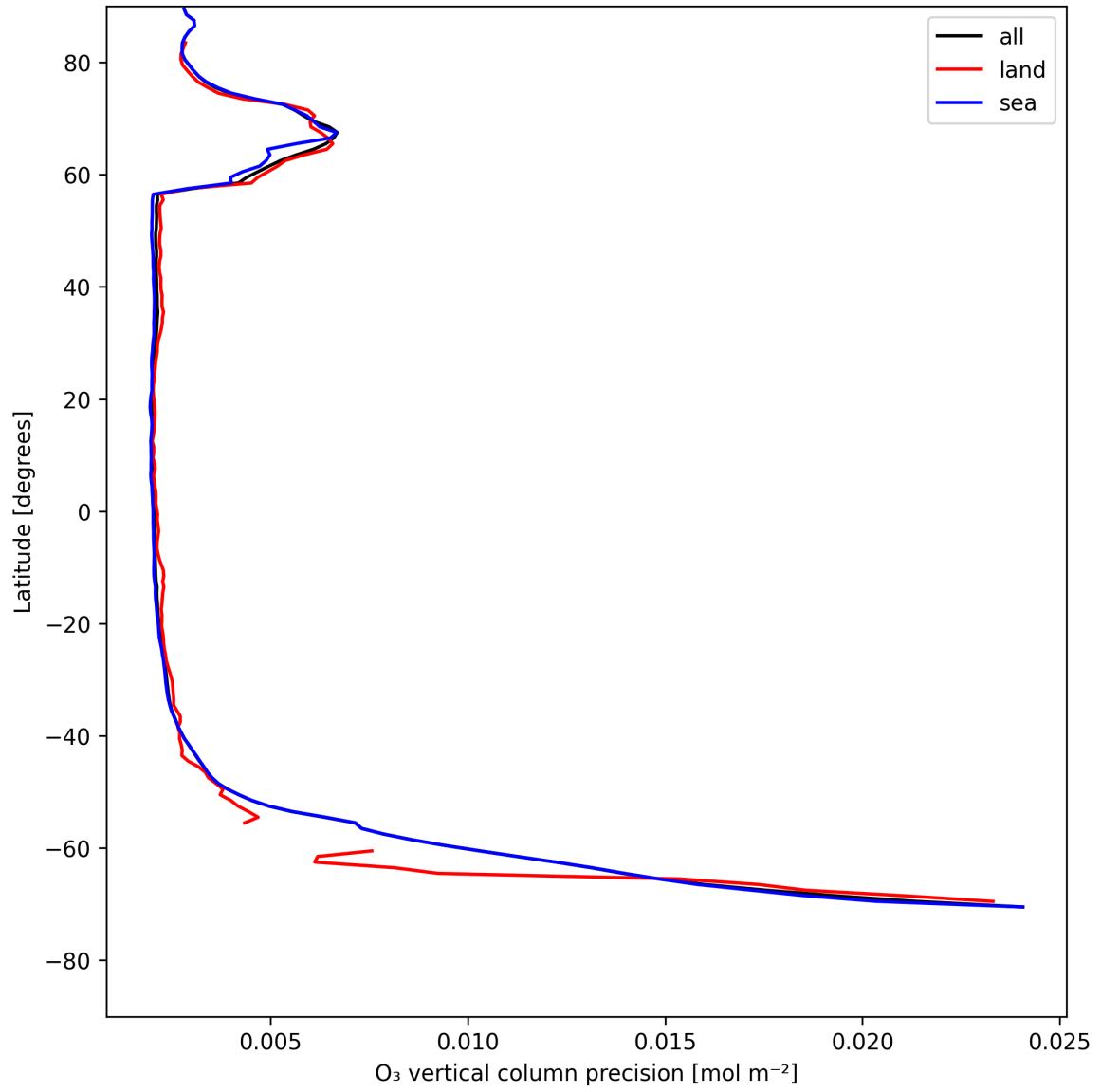
Figure 18: Zonal average of “O 3 vertical column precision” for 2025-07-28 to 2025-07-29.
