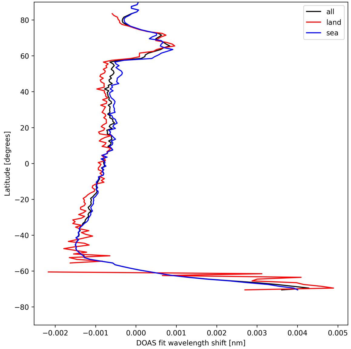
Figure 23: Zonal average of “DOAS fit wavelength shift” for 2025-07-29 to 2025-07-30.
