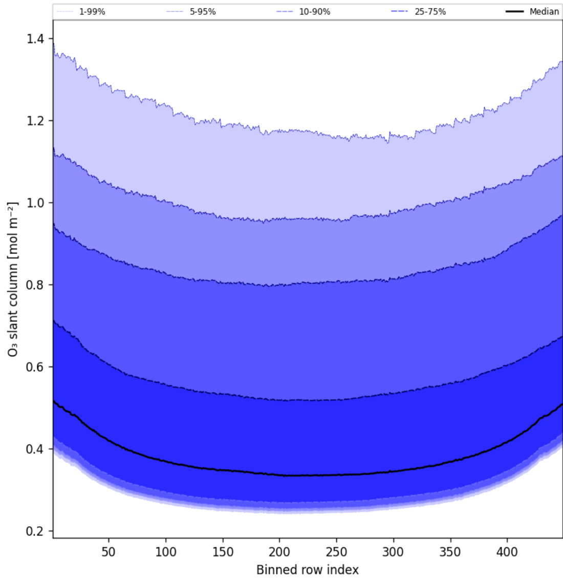
Figure 43: Along track statistics of “O 3 slant column” for 2025-07-29 to 2025-07-30
