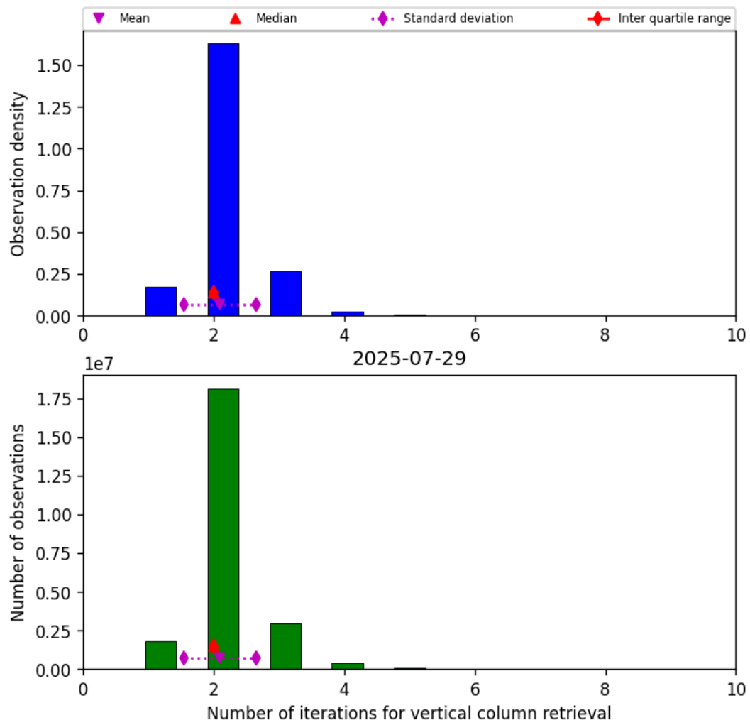
Figure 39: Histogram of “Number of iterations for vertical column retrieval” for 2025-07-29 to 2025-07-30
