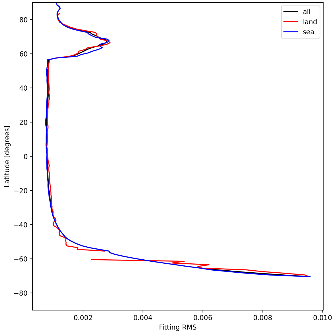
Figure 22: Zonal average of “Fitting RMS” for 2025-07-29 to 2025-07-30.
