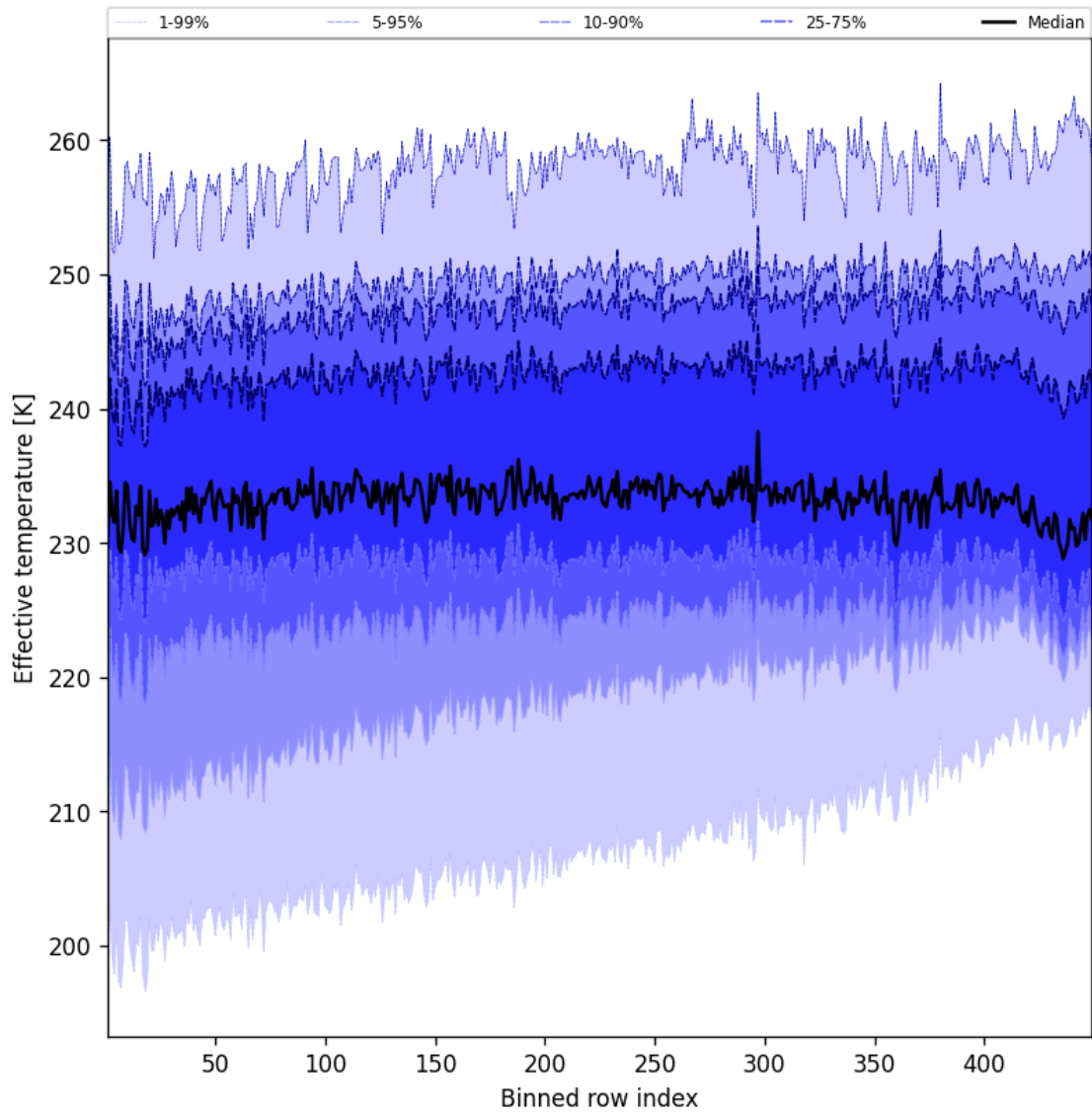
Figure 50: Along track statistics of “Effective temperature” for 2025-07-29 to 2025-07-30
