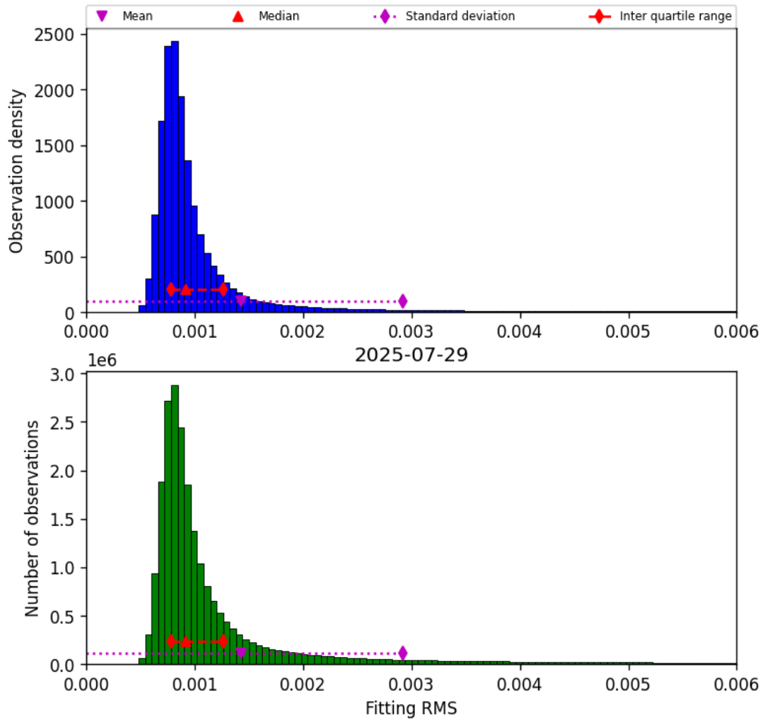
Figure 34: Histogram of “Fitting RMS” for 2025-07-29 to 2025-07-30
