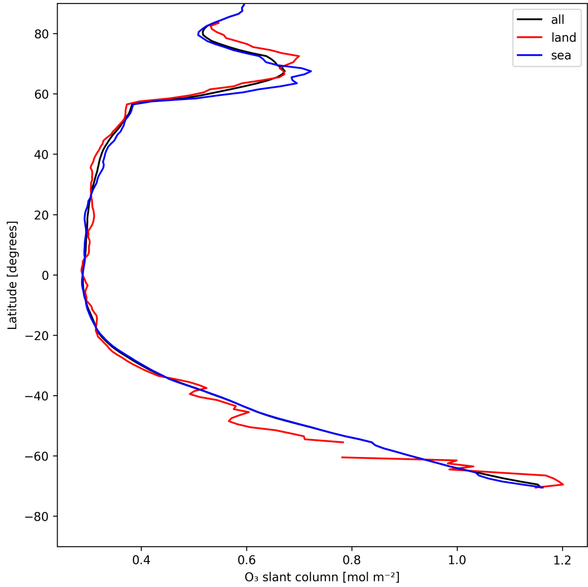
Figure 19: Zonal average of “O 3 slant column” for 2025-07-29 to 2025-07-30.
