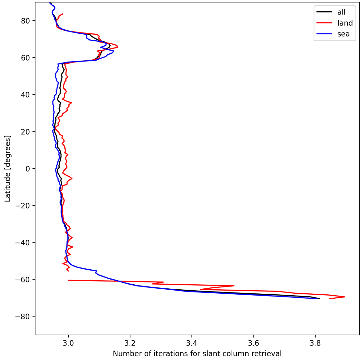
Figure 21: Zonal average of “Number of iterations for slant column retrieval” for 2025-07-29 to 2025-07-30.
