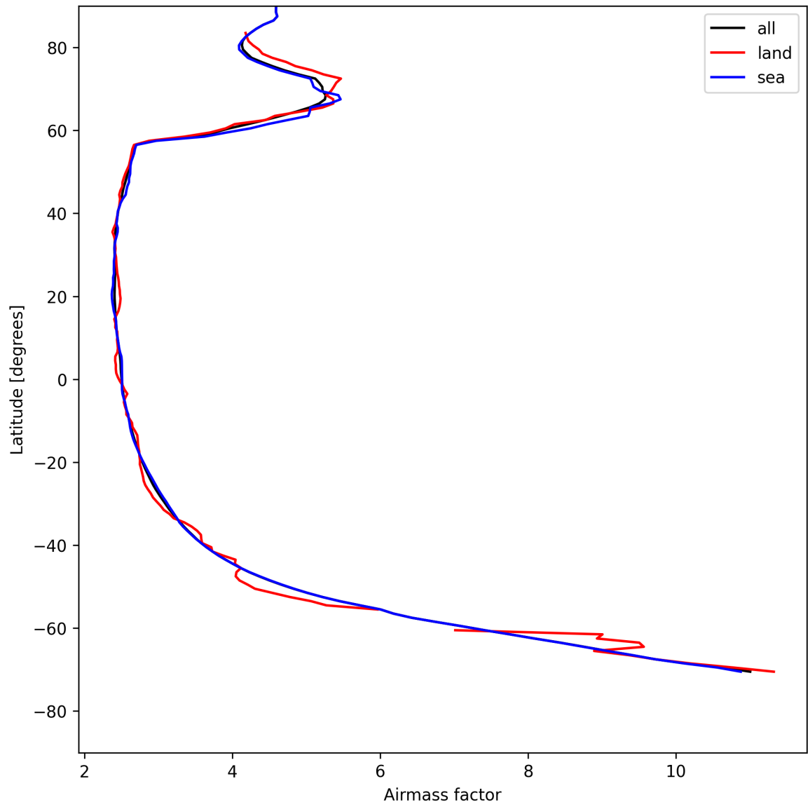
Figure 25: Zonal average of “Airmass factor” for 2025-07-29 to 2025-07-30.
