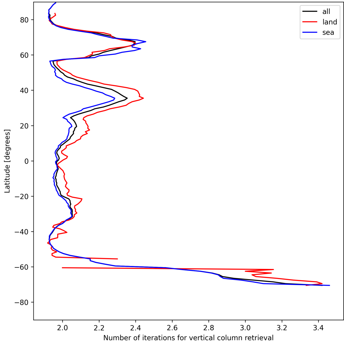
Figure 27: Zonal average of “Number of iterations for vertical column retrieval” for 2025-07-29 to 2025-07-30.
