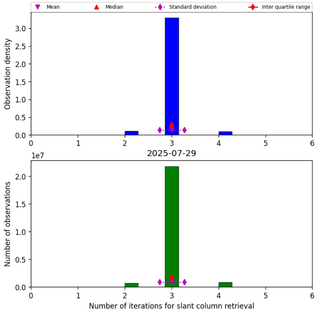
Figure 33: Histogram of “Number of iterations for slant column retrieval” for 2025-07-29 to 2025-07-30
