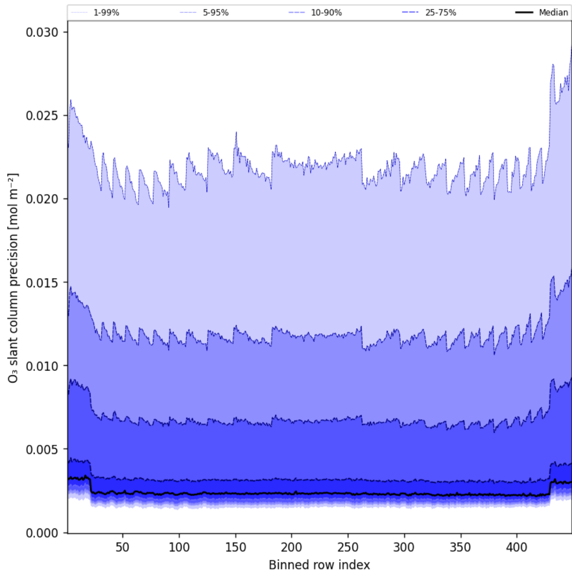
Figure 44: Along track statistics of “O 3 slant column precision” for 2025-07-29 to 2025-07-30
