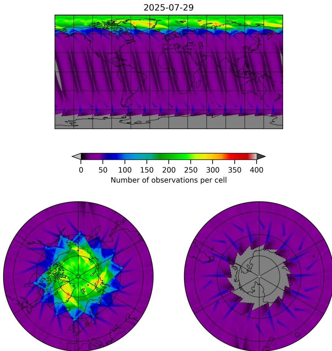
Figure 15: Map of the number of observations for 2025-07-29 to 2025-07-30
