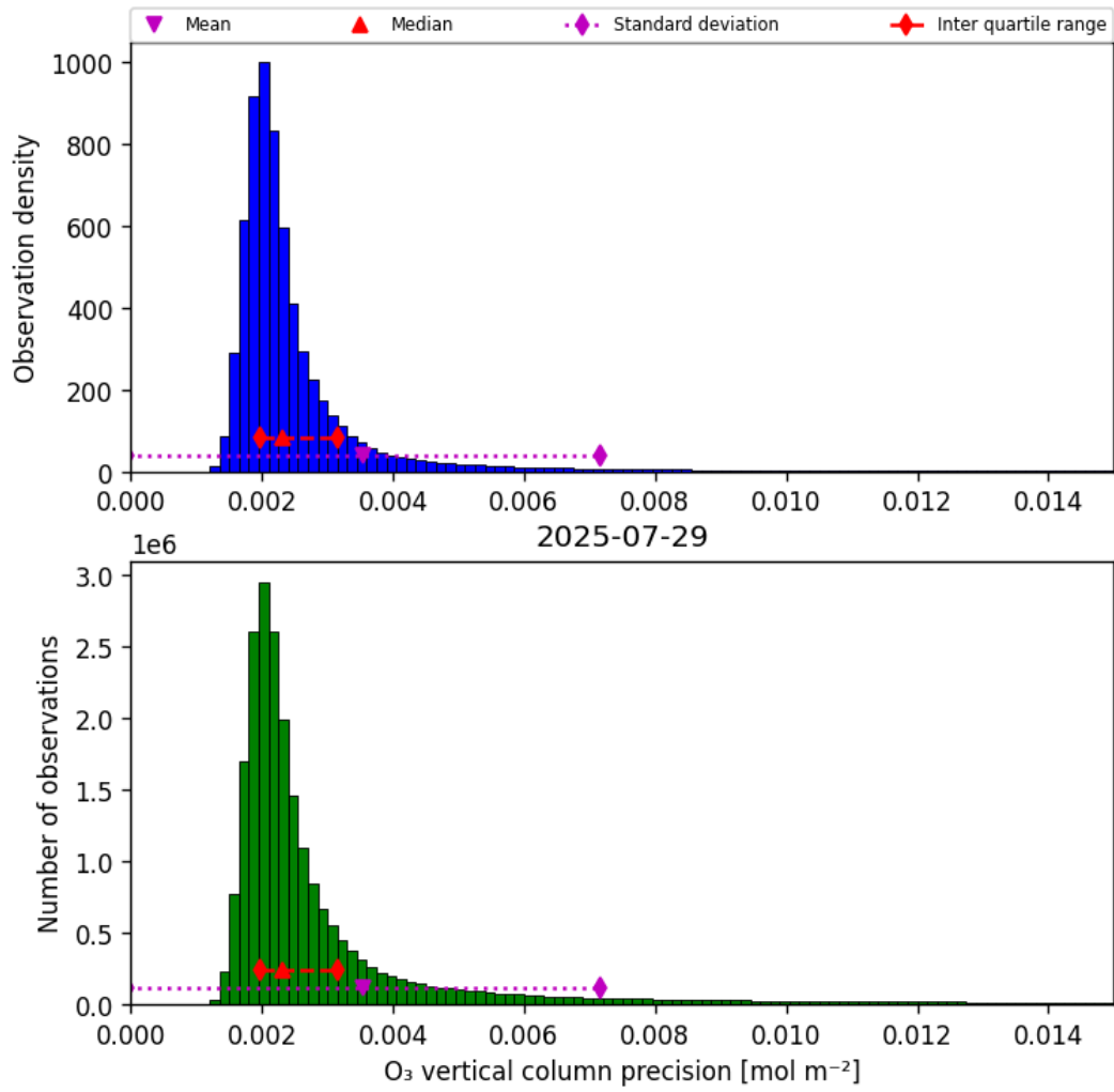
Figure 30: Histogram of “O 3 vertical column precision” for 2025-07-29 to 2025-07-30
