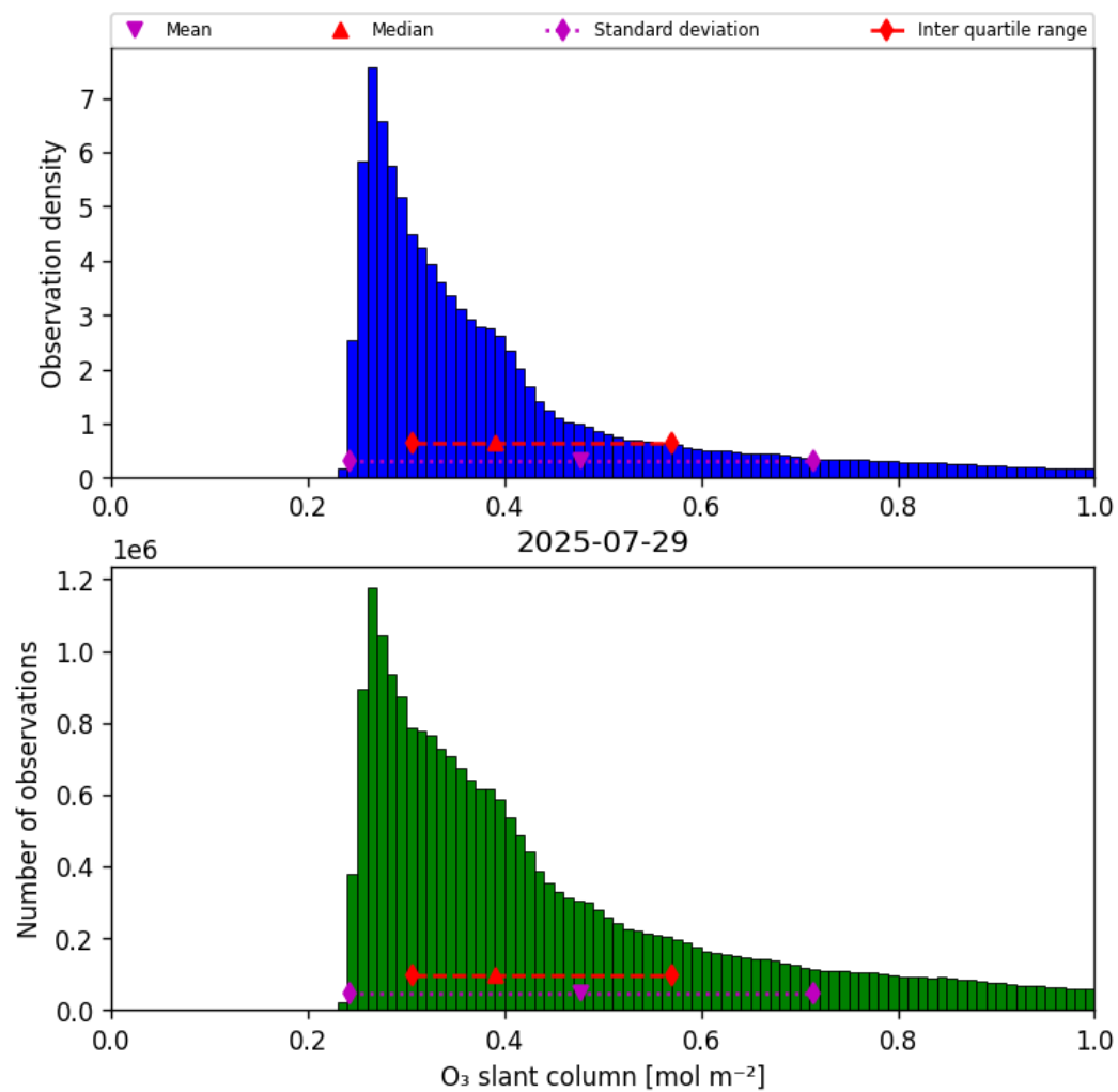
Figure 31: Histogram of “O 3 slant column” for 2025-07-29 to 2025-07-30
