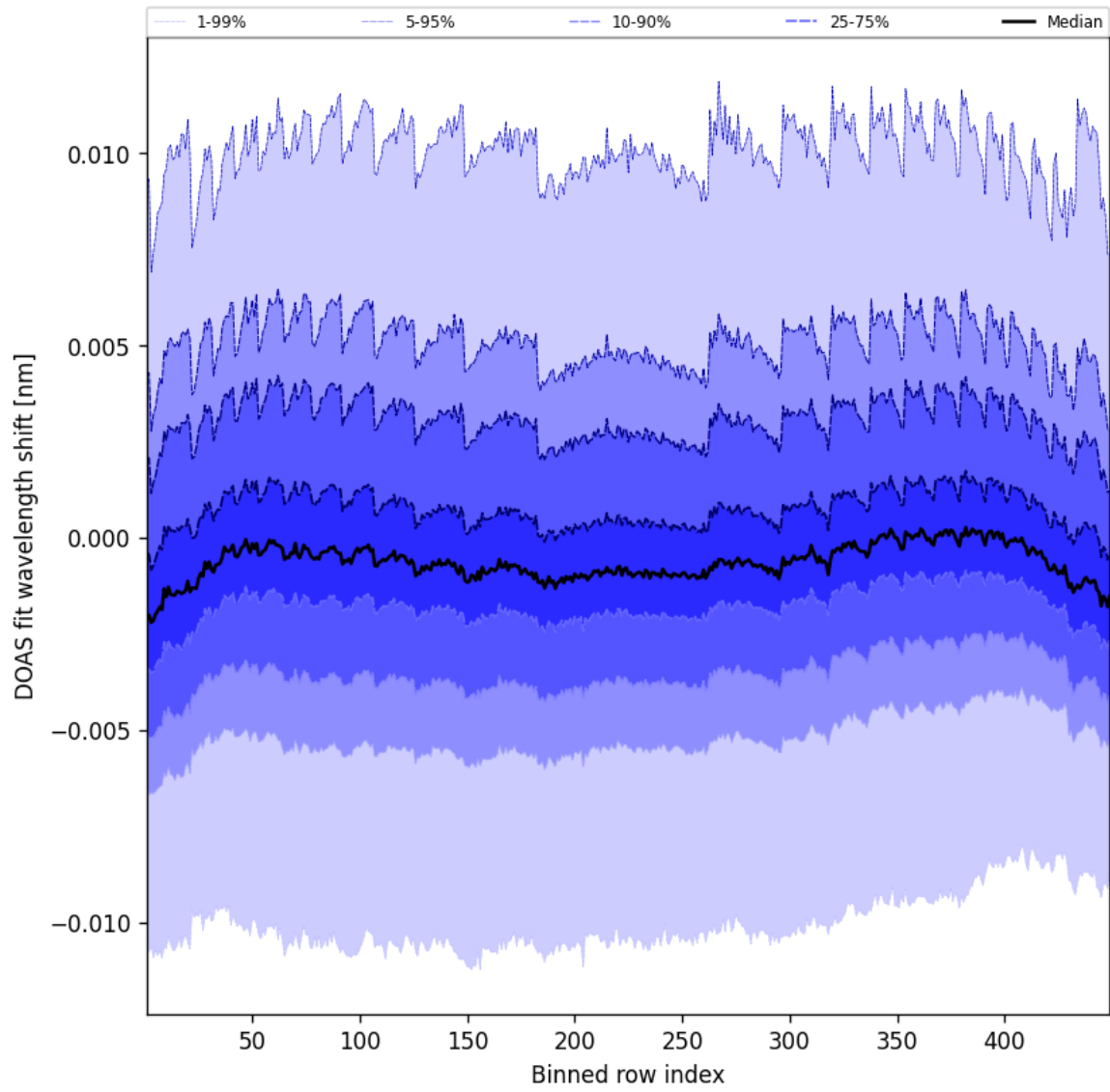
Figure 47: Along track statistics of “DOAS fit wavelength shift” for 2025-07-29 to 2025-07-30
