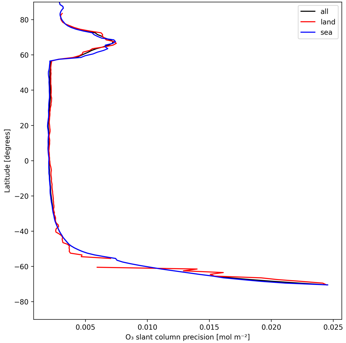
Figure 20: Zonal average of “O 3 slant column precision” for 2025-07-29 to 2025-07-30.
