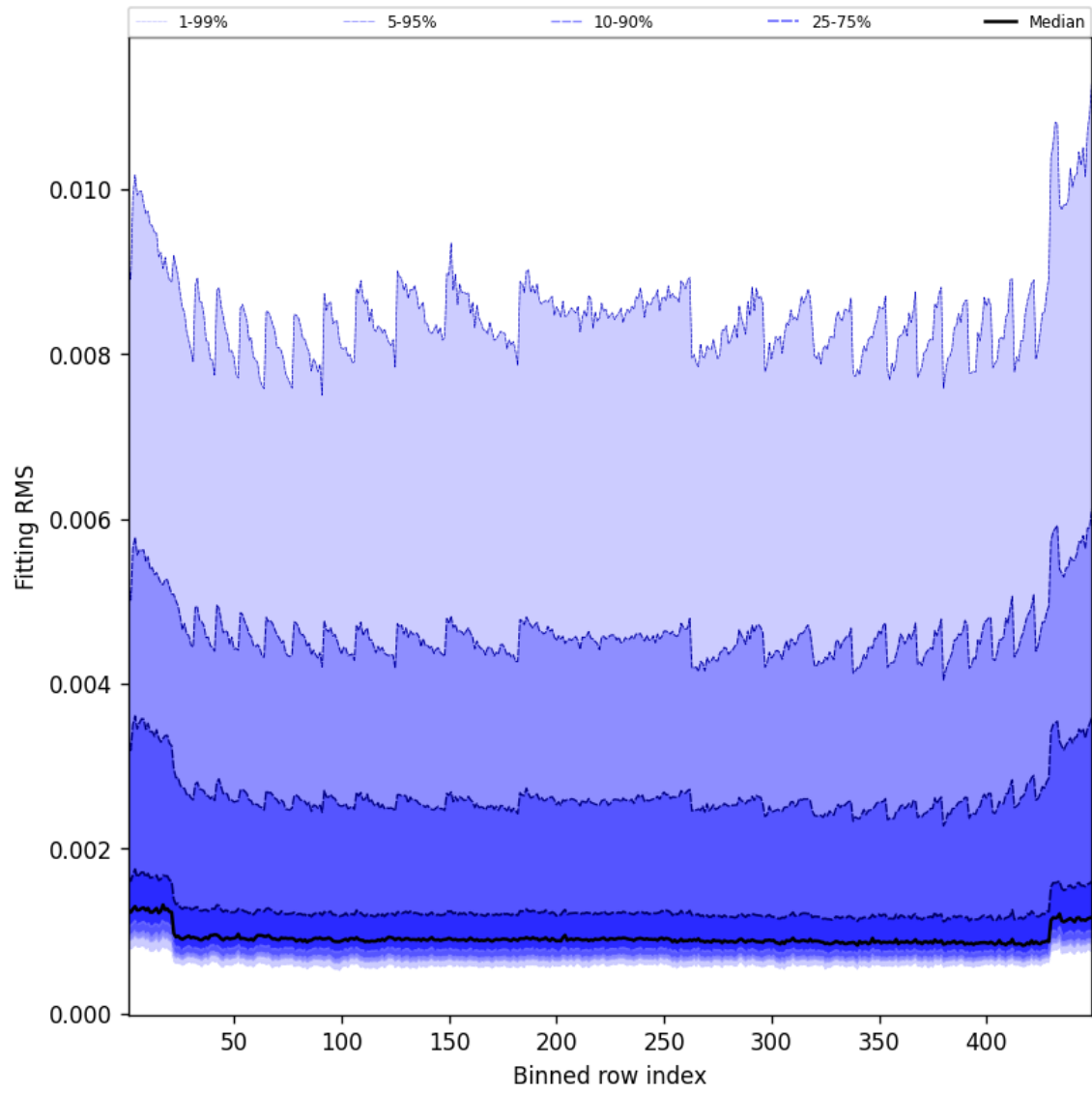
Figure 46: Along track statistics of “Fitting RMS” for 2025-07-29 to 2025-07-30
