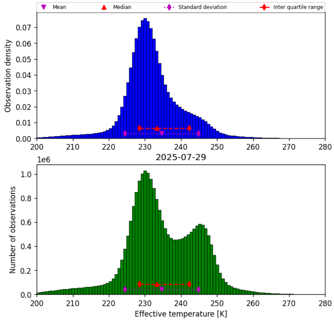
Figure 38: Histogram of “Effective temperature” for 2025-07-29 to 2025-07-30
