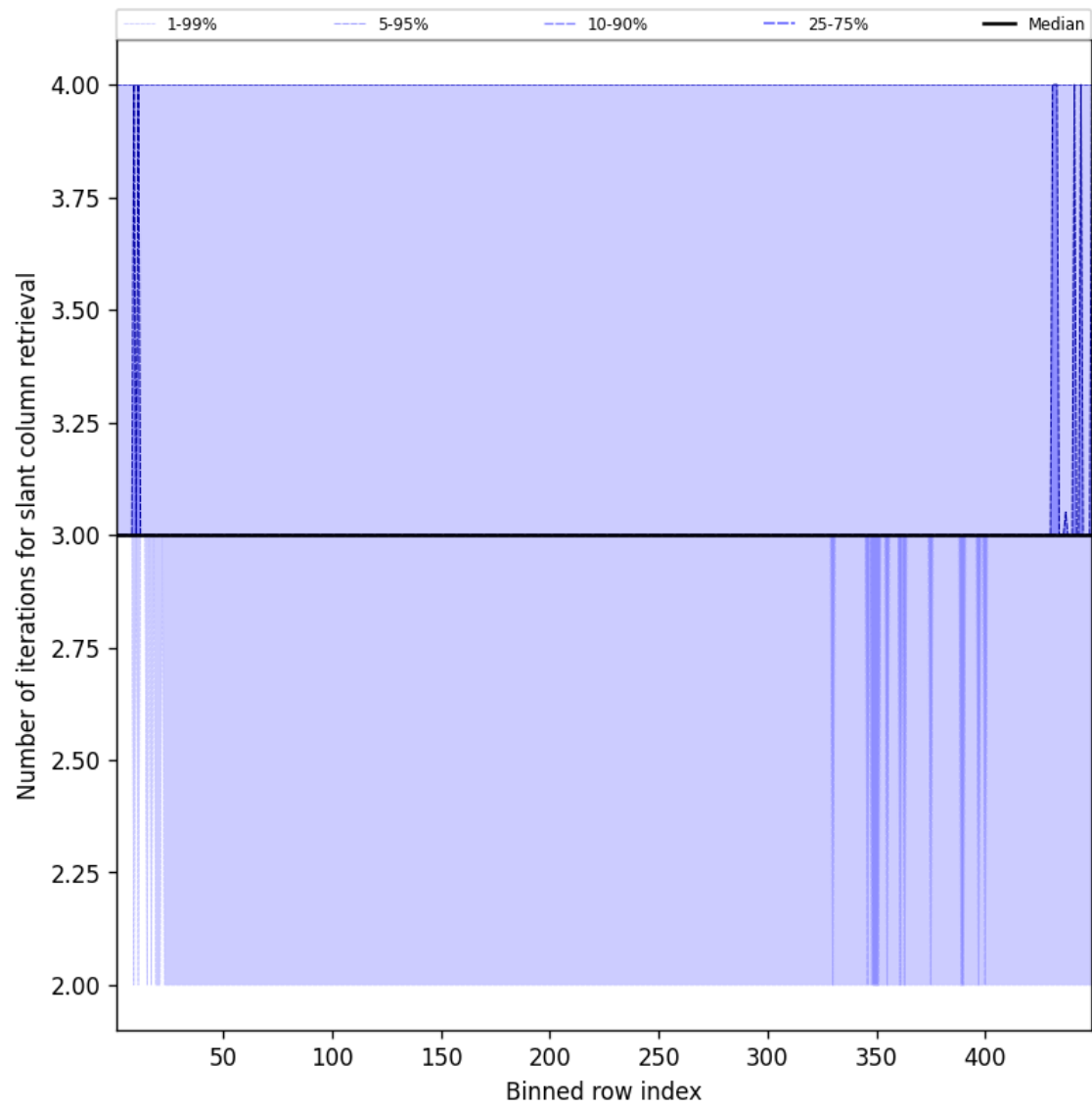
Figure 45: Along track statistics of “Number of iterations for slant column retrieval” for 2025-07-29 to 2025-07-30
