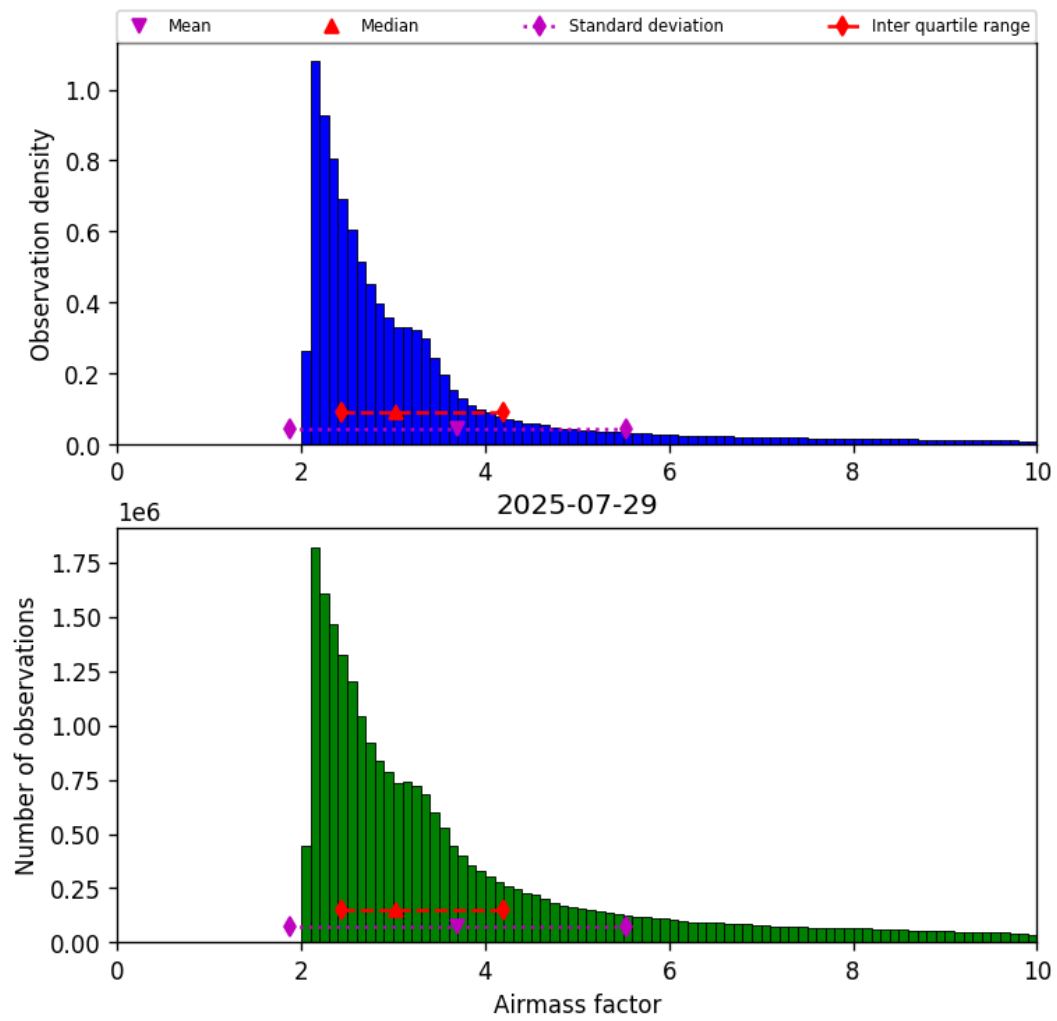
Figure 37: Histogram of “Airmass factor” for 2025-07-29 to 2025-07-30
