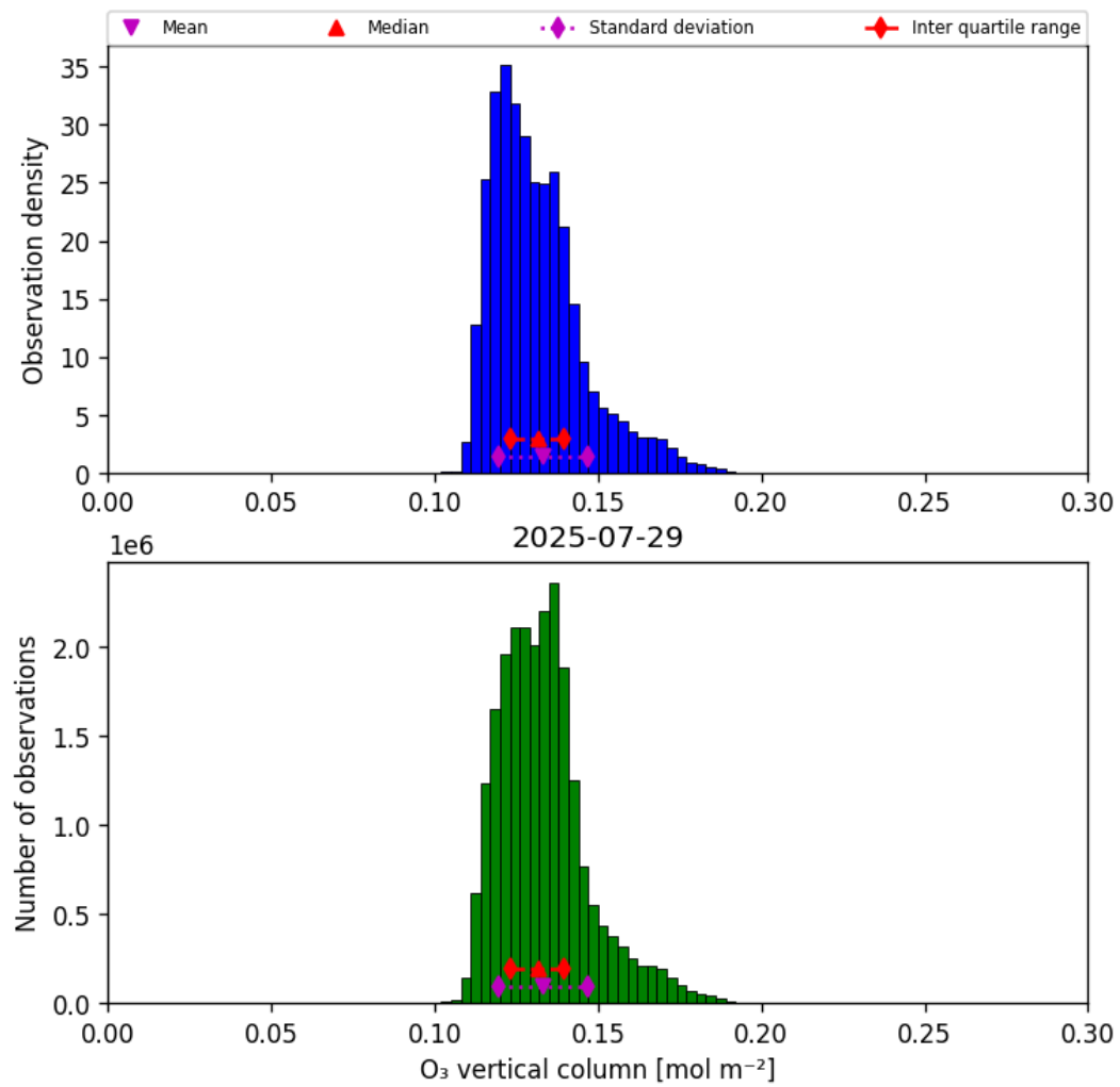
Figure 29: Histogram of “O 3 vertical column” for 2025-07-29 to 2025-07-30
