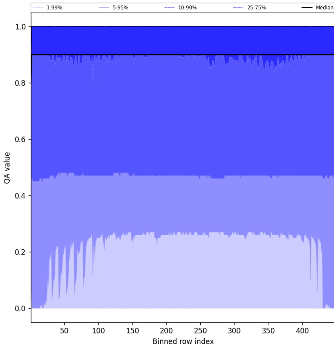
Figure 40: Along track statistics of “QA value” for 2025-07-29 to 2025-07-30
