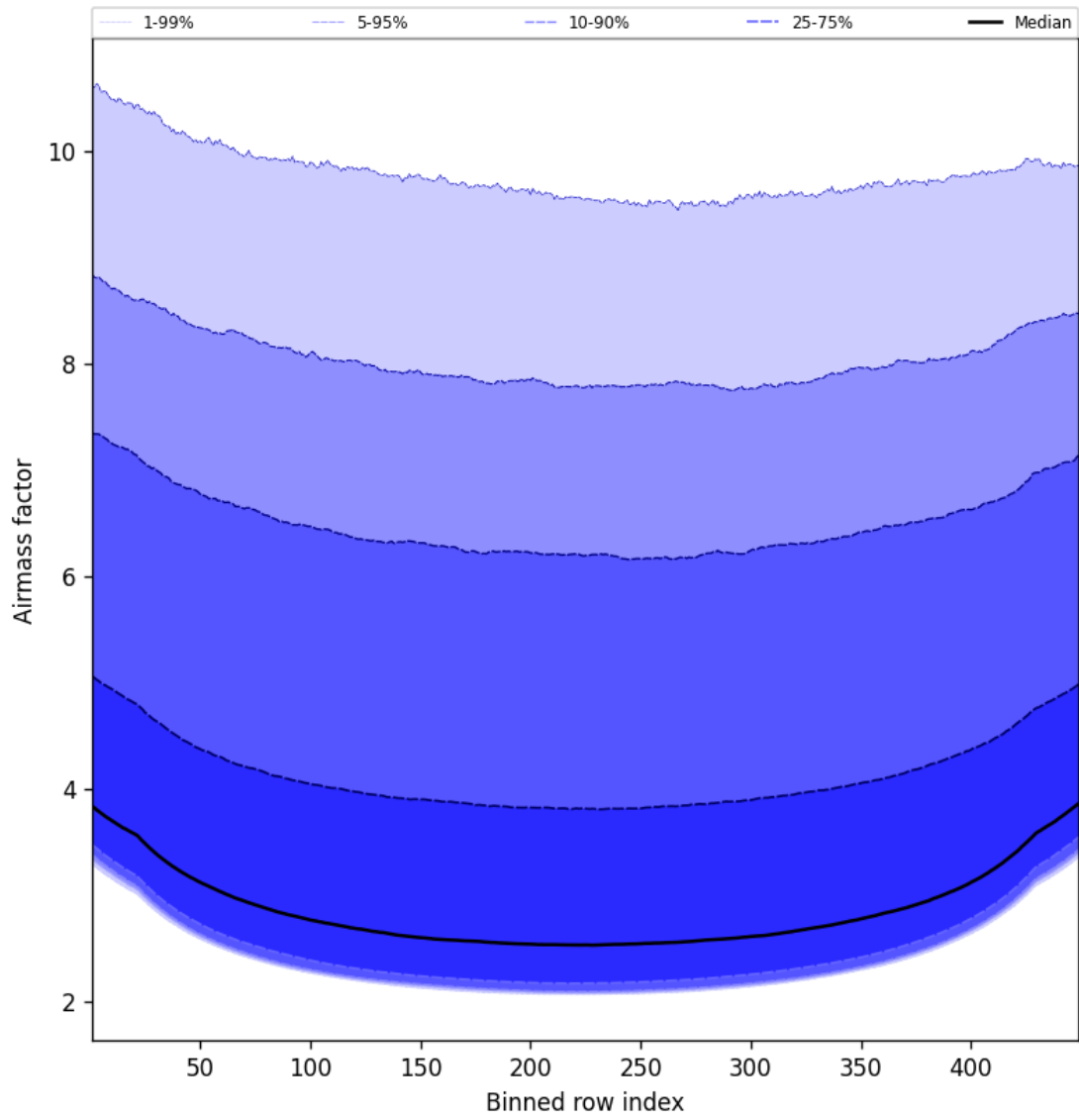
Figure 49: Along track statistics of “Airmass factor” for 2025-07-29 to 2025-07-30
