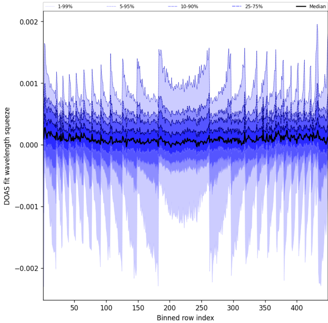
Figure 48: Along track statistics of “DOAS fit wavelength squeeze” for 2025-07-29 to 2025-07-30
