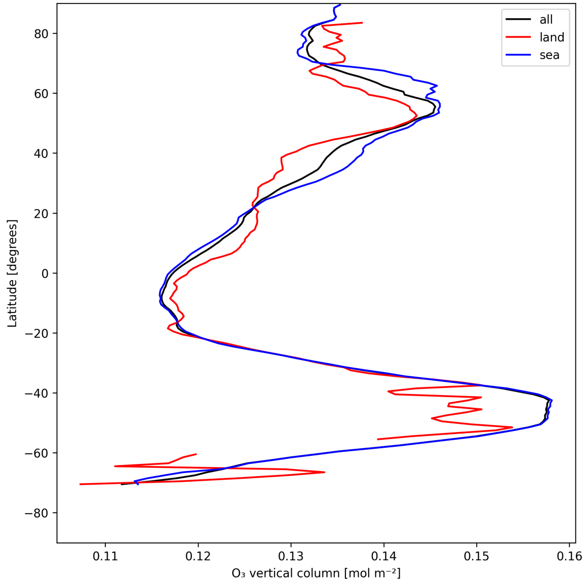
Figure 17: Zonal average of “O 3 vertical column” for 2025-07-29 to 2025-07-30.
