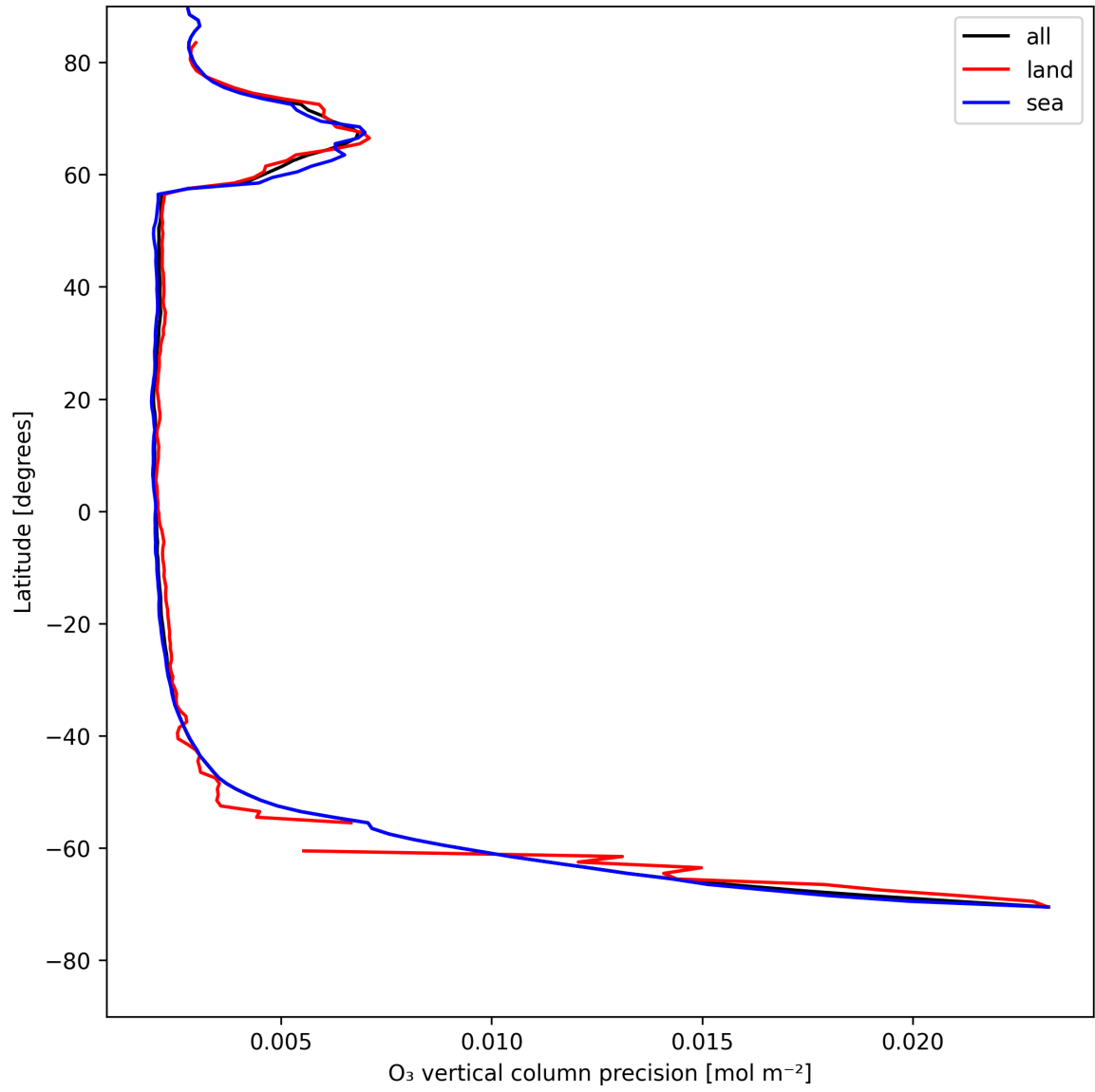
Figure 18: Zonal average of “O 3 vertical column precision” for 2025-07-29 to 2025-07-30.
