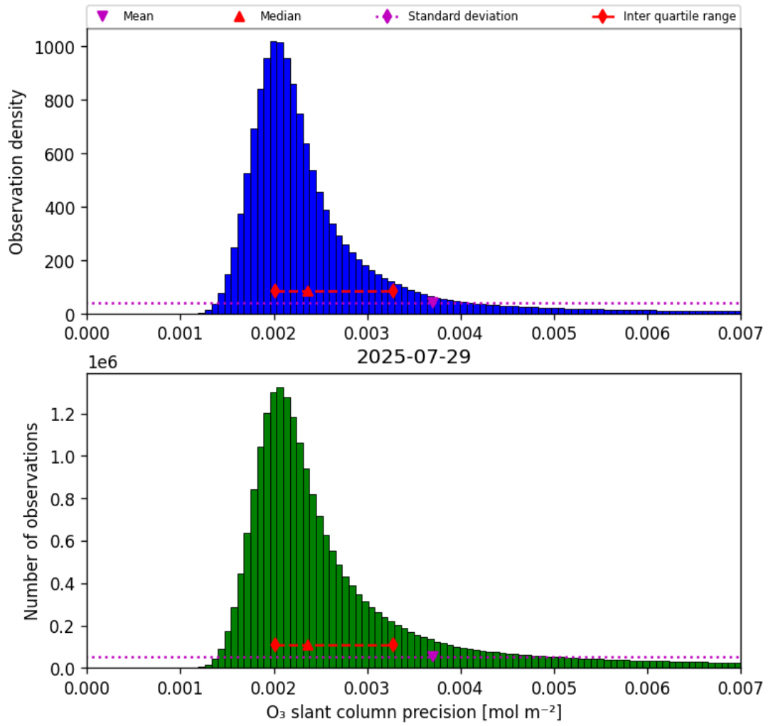
Figure 32: Histogram of “O 3 slant column precision” for 2025-07-29 to 2025-07-30
