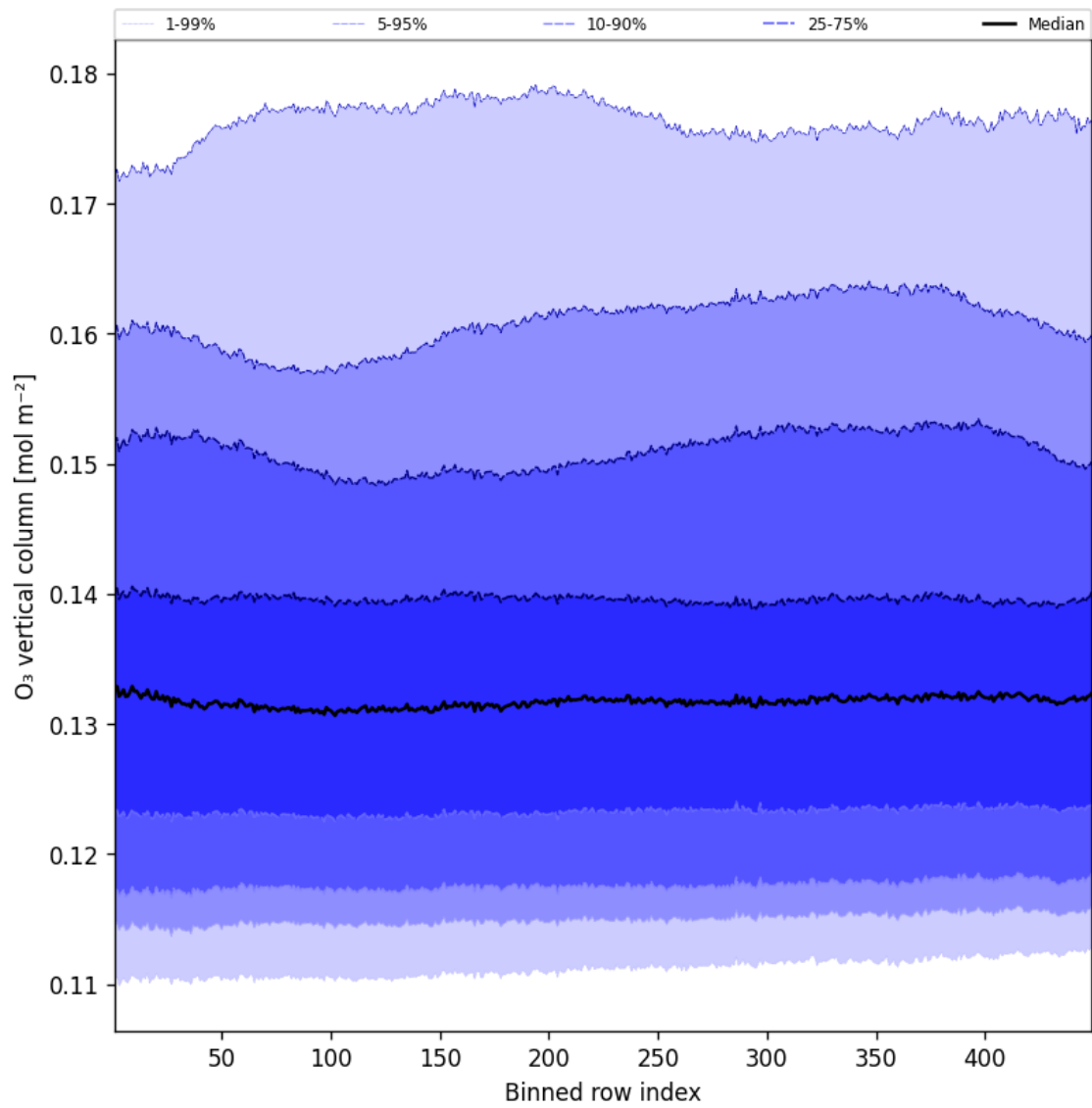
Figure 41: Along track statistics of “O 3 vertical column” for 2025-07-29 to 2025-07-30
