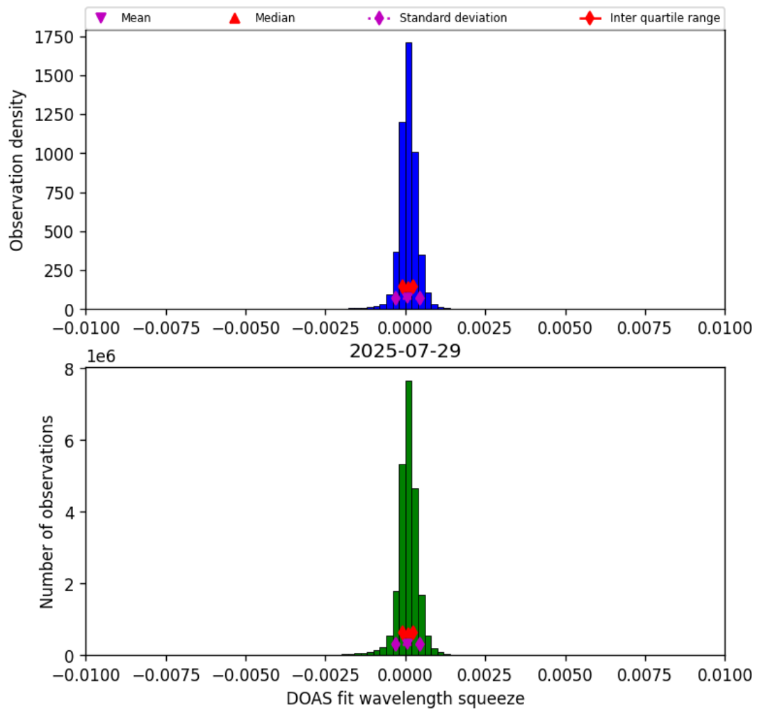
Figure 36: Histogram of “DOAS fit wavelength squeeze” for 2025-07-29 to 2025-07-30
