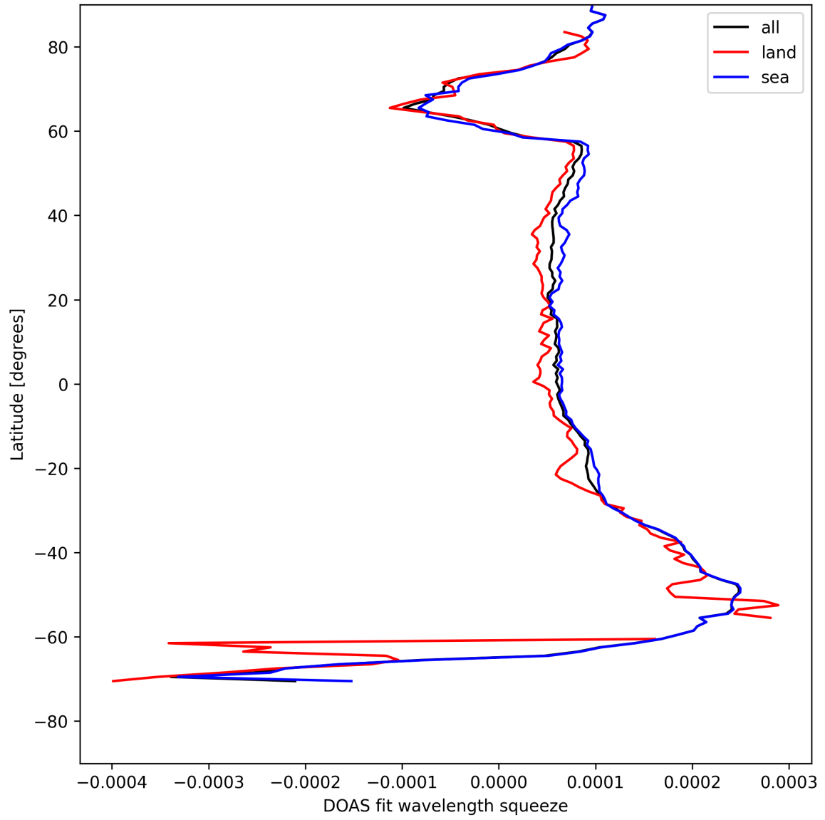
Figure 24: Zonal average of “DOAS fit wavelength squeeze” for 2025-07-29 to 2025-07-30.
