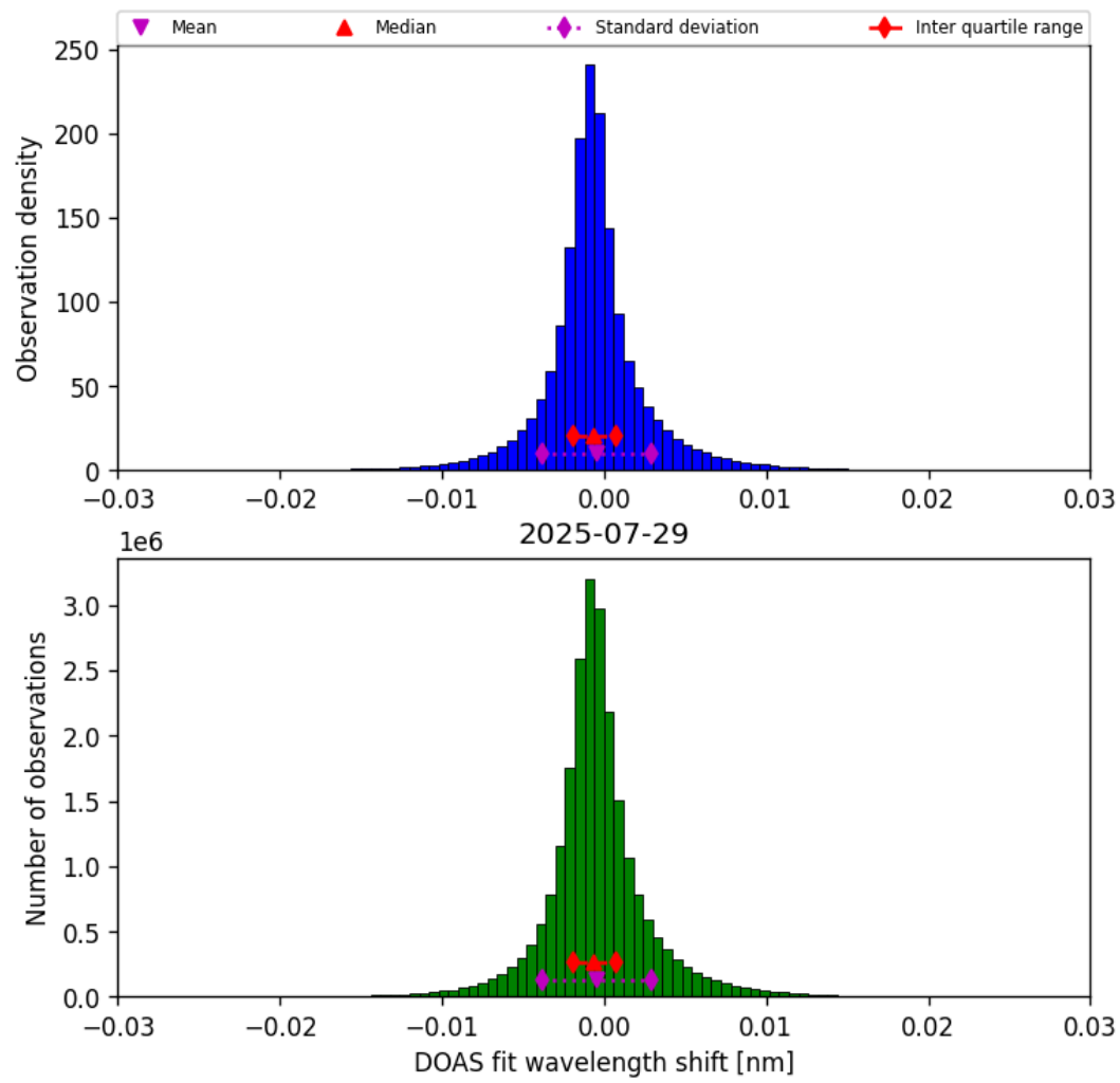
Figure 35: Histogram of “DOAS fit wavelength shift” for 2025-07-29 to 2025-07-30
