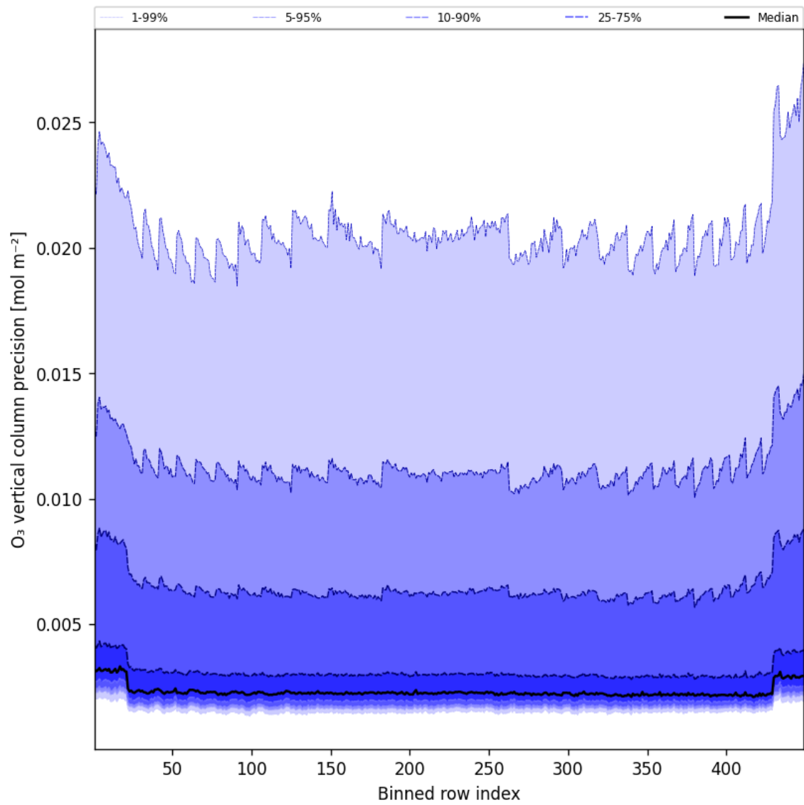
Figure 42: Along track statistics of “O 3 vertical column precision” for 2025-07-29 to 2025-07-30
