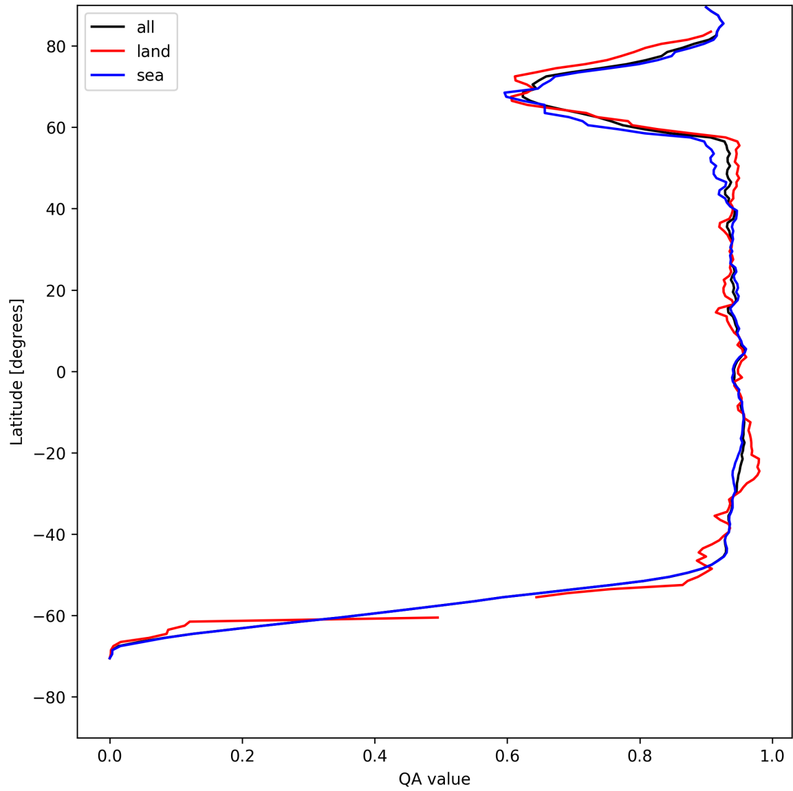
Figure 16: Zonal average of “QA value” for 2025-07-29 to 2025-07-30.
