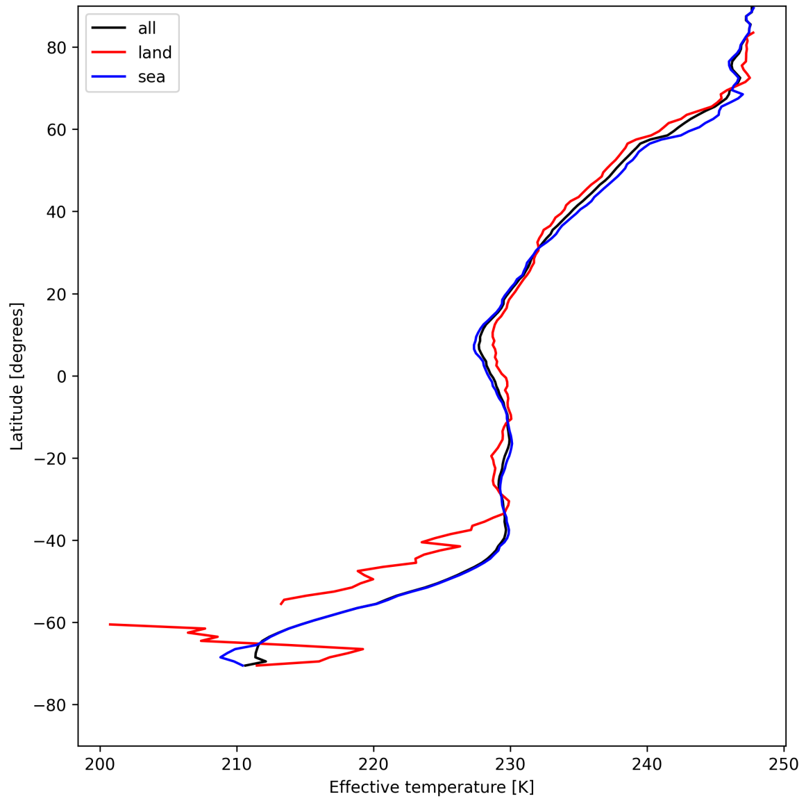
Figure 26: Zonal average of “Effective temperature” for 2025-07-29 to 2025-07-30.
