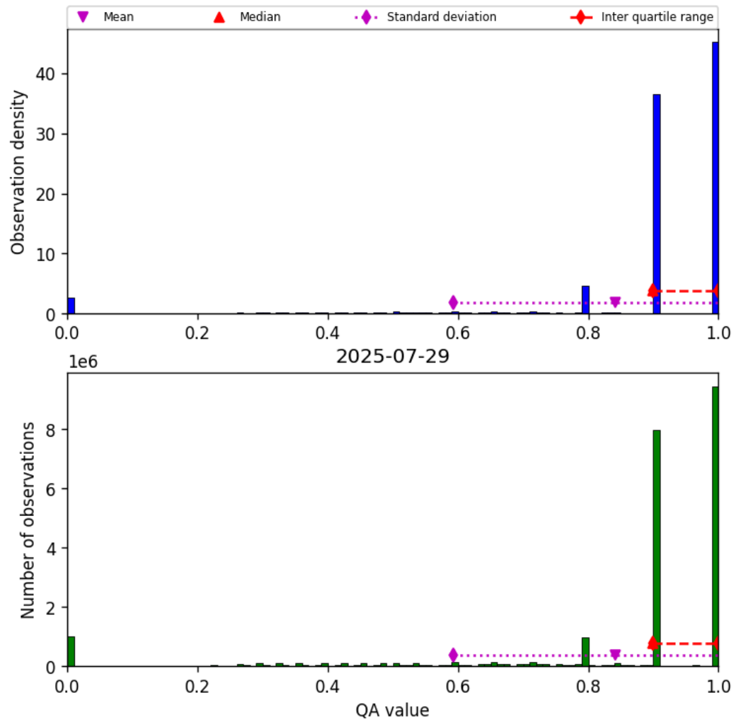
Figure 28: Histogram of “QA value” for 2025-07-29 to 2025-07-30
