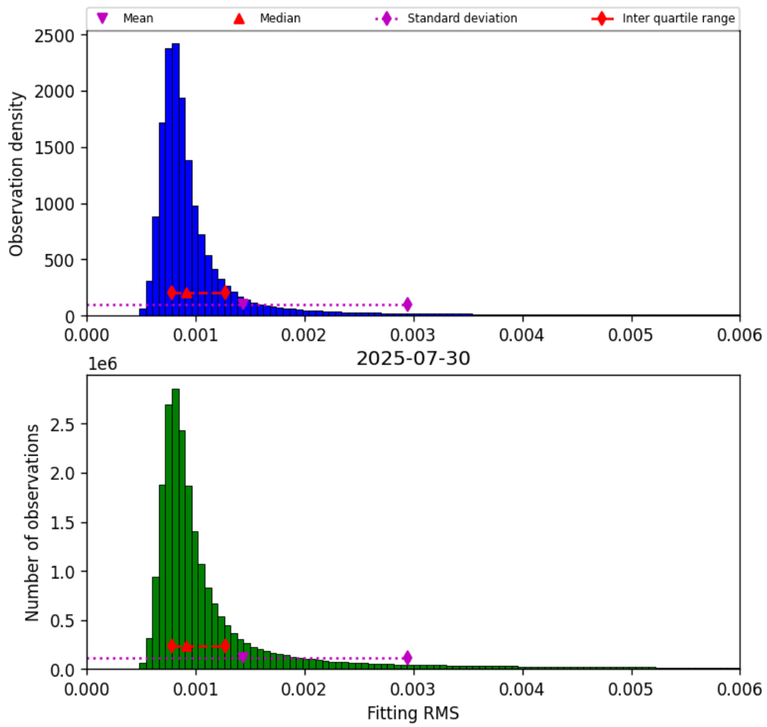
Figure 34: Histogram of “Fitting RMS” for 2025-07-30 to 2025-07-31
