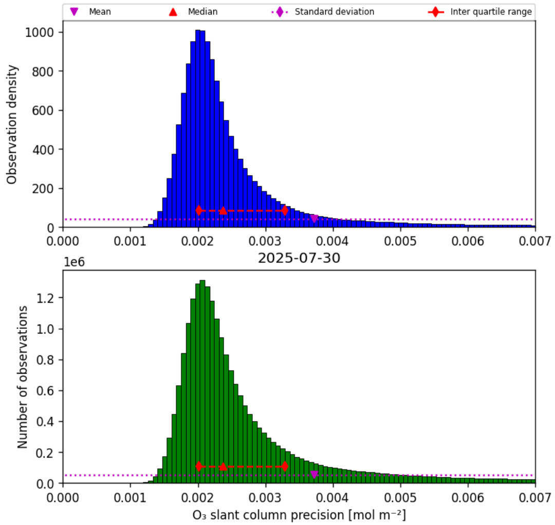
Figure 32: Histogram of “O 3 slant column precision” for 2025-07-30 to 2025-07-31
