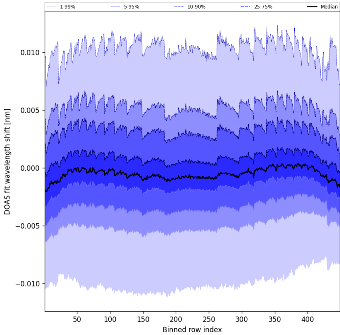
Figure 47: Along track statistics of “DOAS fit wavelength shift” for 2025-07-30 to 2025-07-31
