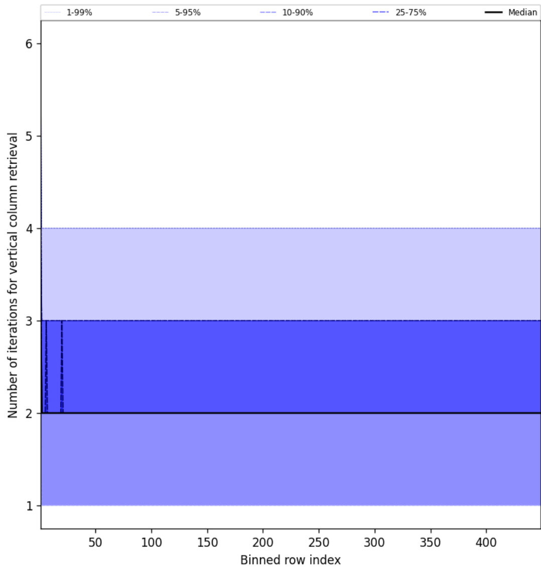
Figure 51: Along track statistics of “Number of iterations for vertical column retrieval” for 2025-07-30 to 2025-07-31
