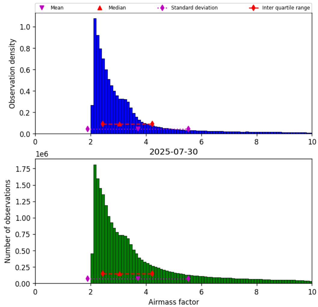
Figure 37: Histogram of “Airmass factor” for 2025-07-30 to 2025-07-31
