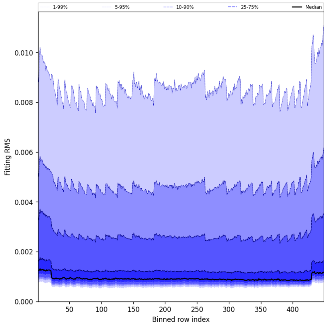
Figure 46: Along track statistics of “Fitting RMS” for 2025-07-30 to 2025-07-31
