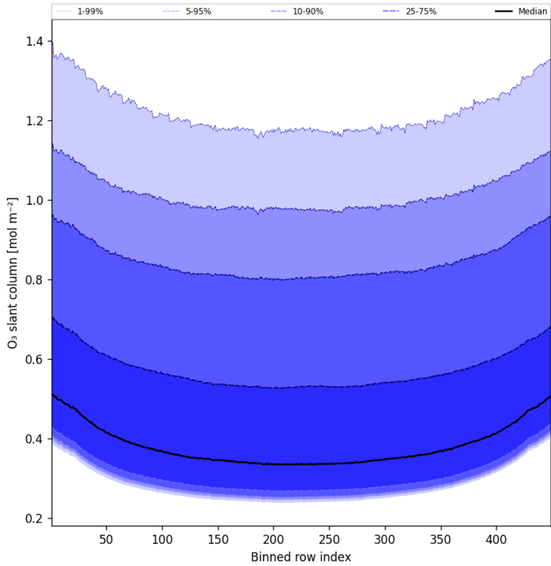
Figure 43: Along track statistics of “O 3 slant column” for 2025-07-30 to 2025-07-31
