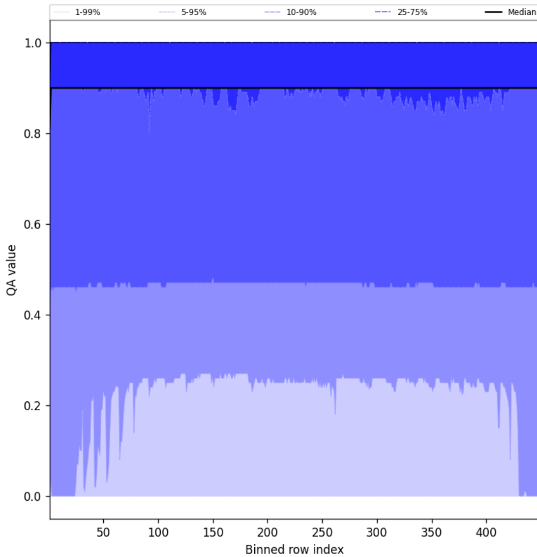
Figure 40: Along track statistics of “QA value” for 2025-07-30 to 2025-07-31
