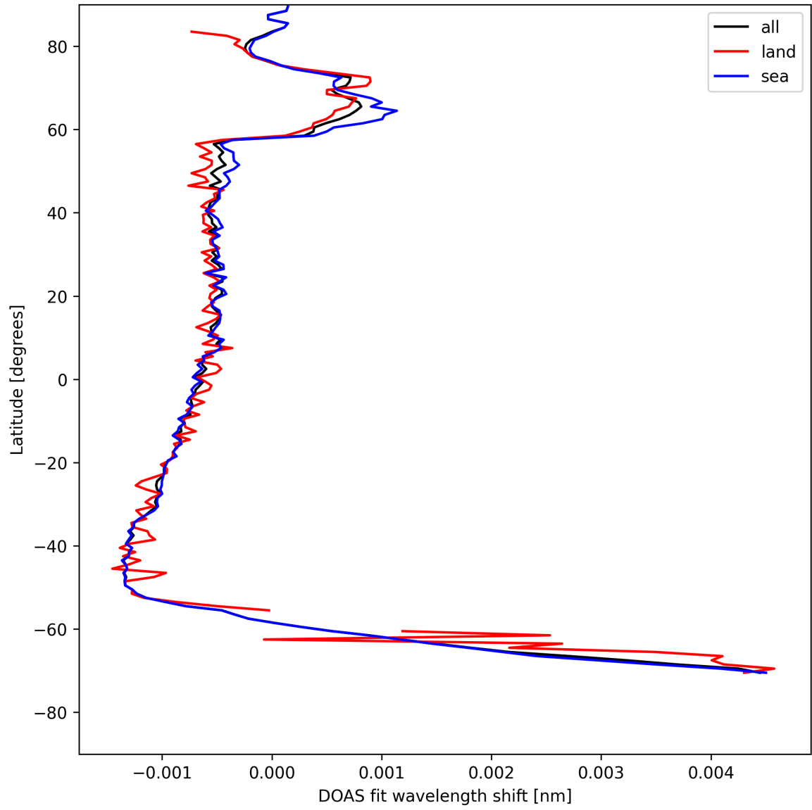
Figure 23: Zonal average of “DOAS fit wavelength shift” for 2025-07-30 to 2025-07-31.
