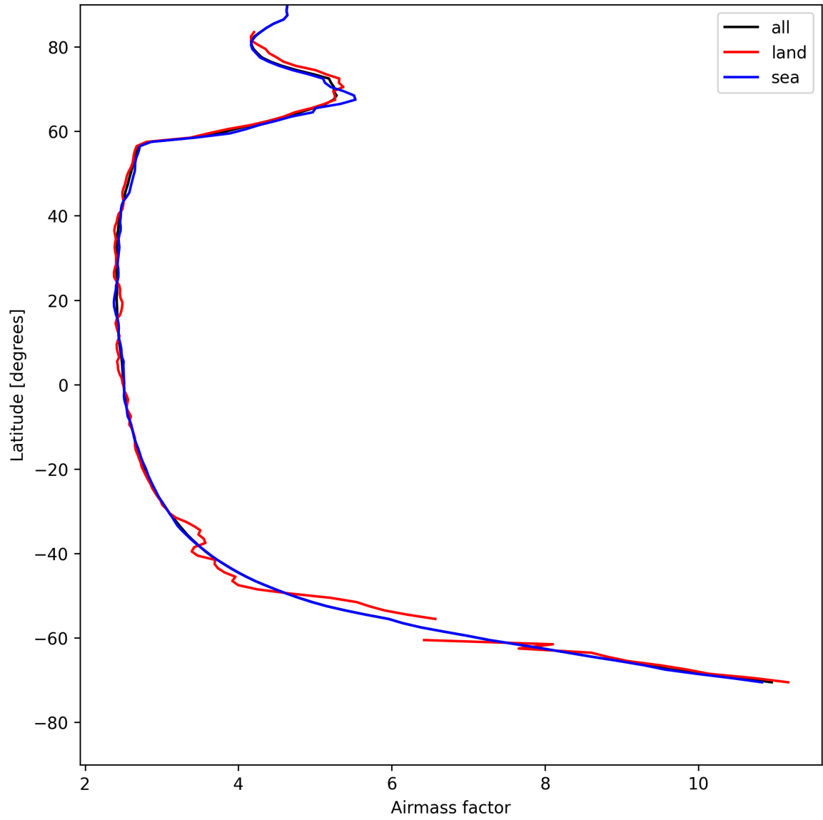
Figure 25: Zonal average of “Airmass factor” for 2025-07-30 to 2025-07-31.
