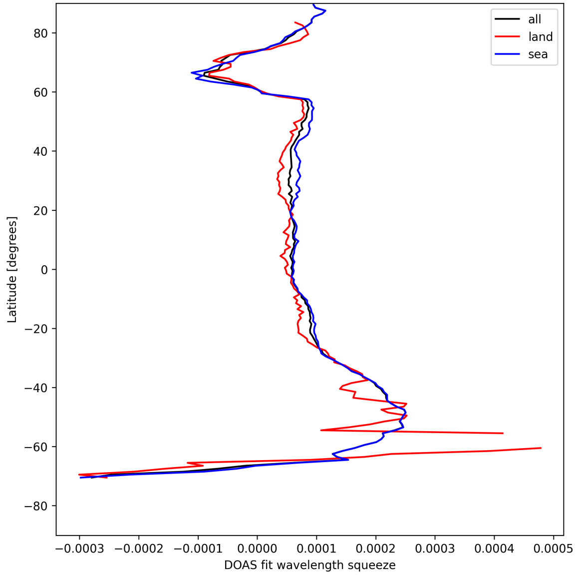
Figure 24: Zonal average of "DOAS fit wavelength squeeze" for 2025-07-30 to 2025-07-31.
