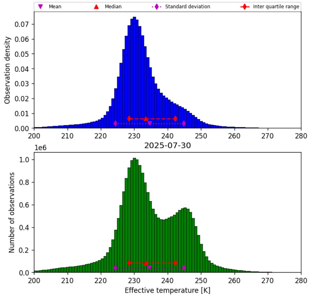
Figure 38: Histogram of “Effective temperature” for 2025-07-30 to 2025-07-31
