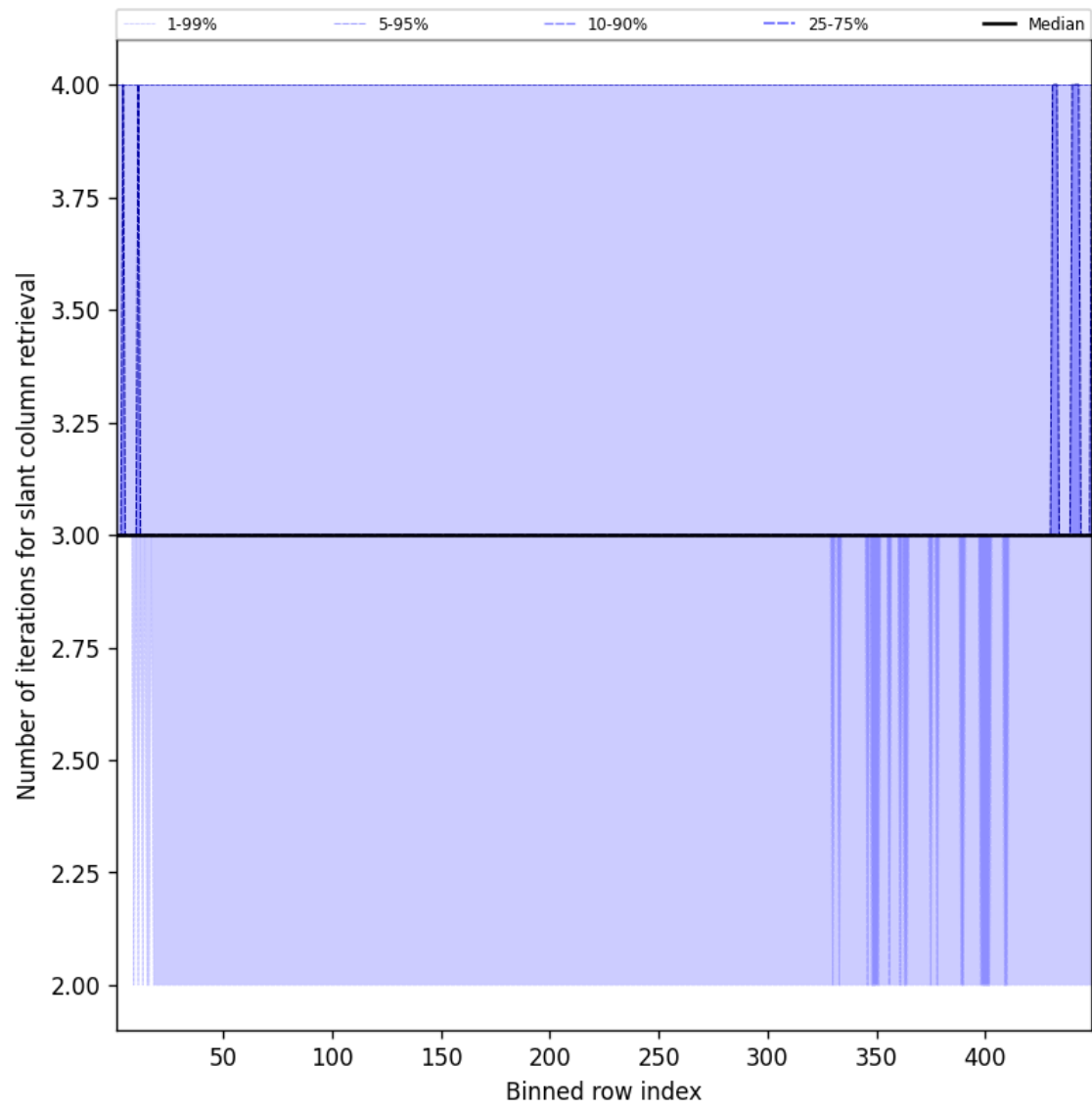
Figure 45: Along track statistics of “Number of iterations for slant column retrieval” for 2025-07-30 to 2025-07-31
