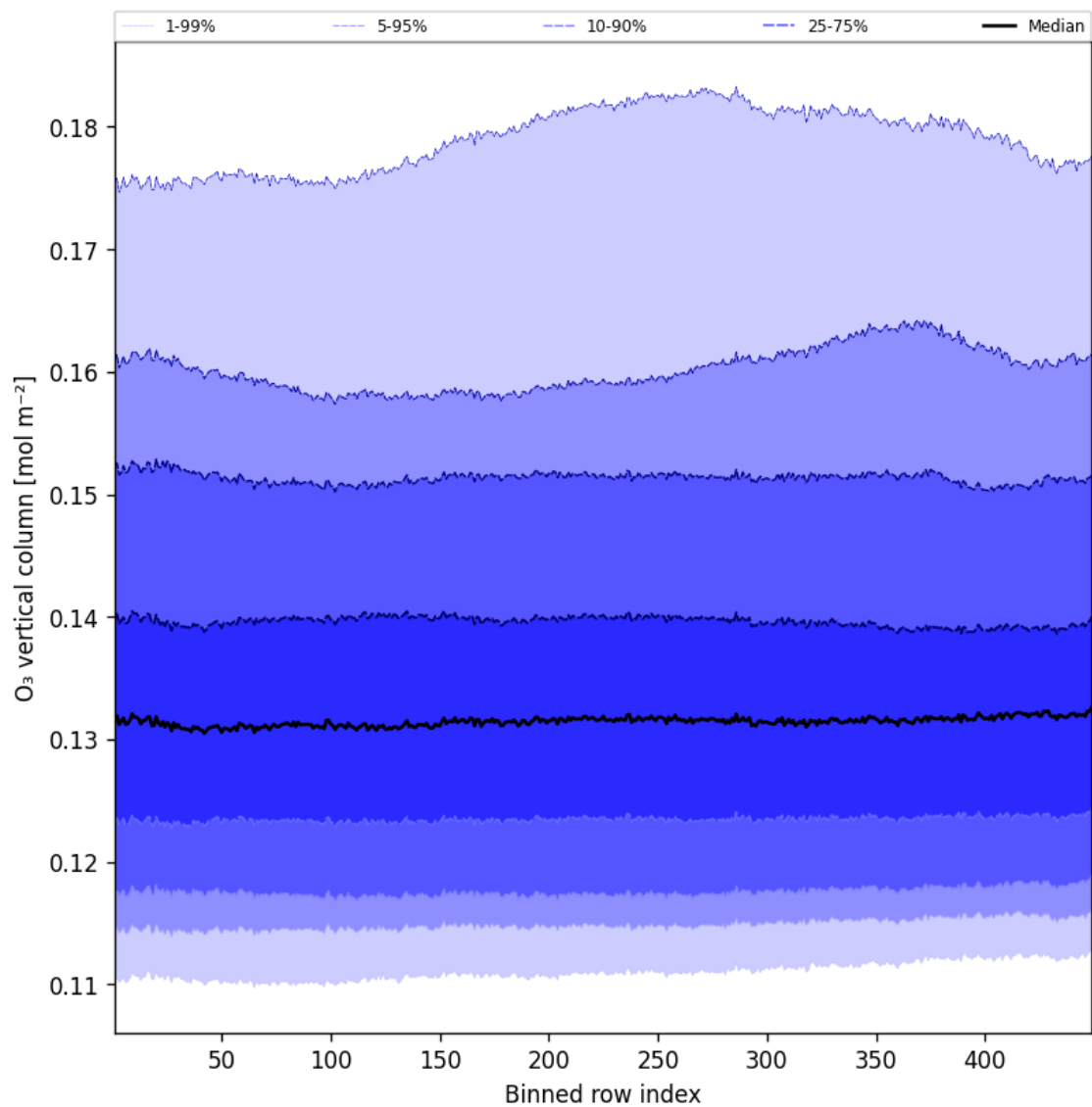
Figure 41: Along track statistics of “O 3 vertical column” for 2025-07-30 to 2025-07-31
