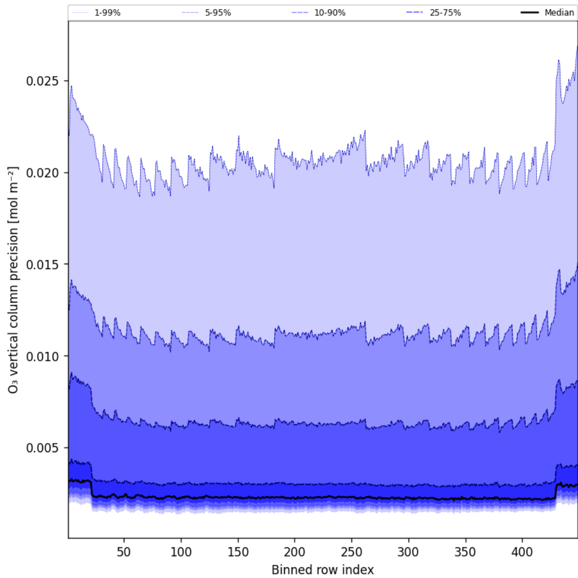
Figure 42: Along track statistics of “O 3 vertical column precision” for 2025-07-30 to 2025-07-31
