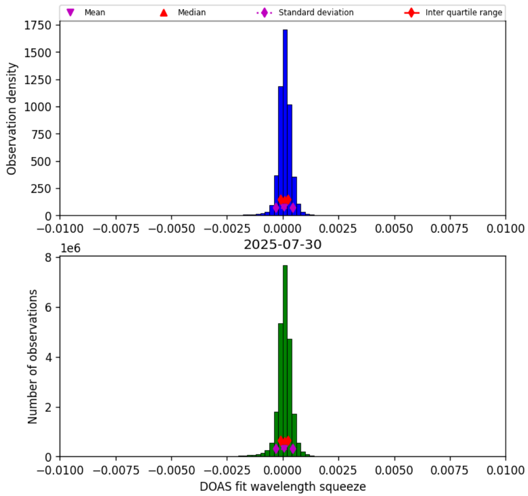
Figure 36: Histogram of “DOAS fit wavelength squeeze” for 2025-07-30 to 2025-07-31
