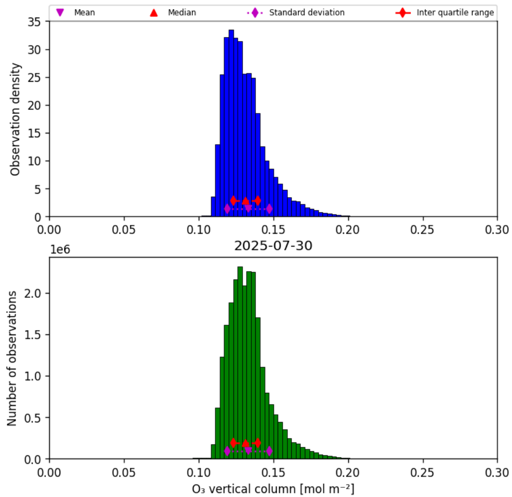
Figure 29: Histogram of “O 3 vertical column” for 2025-07-30 to 2025-07-31
