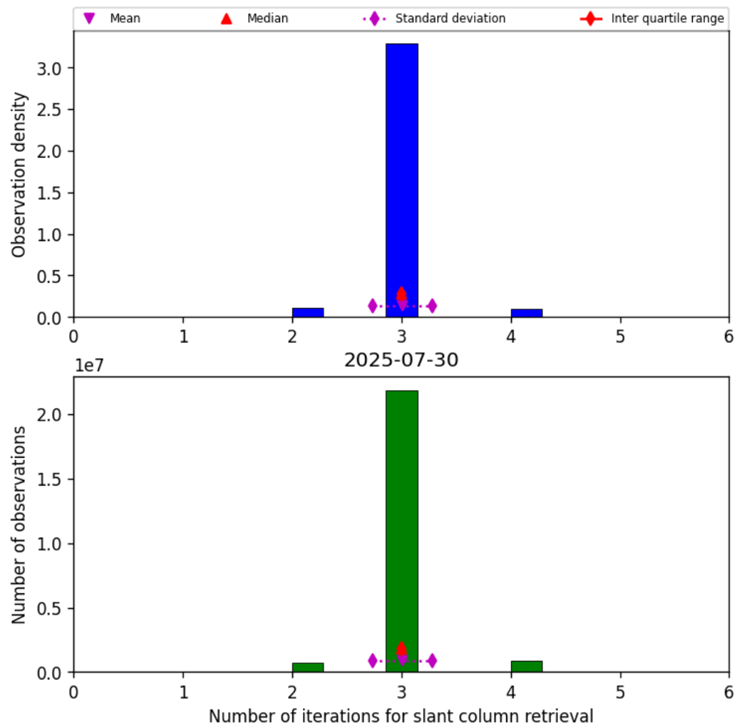
Figure 33: Histogram of “Number of iterations for slant column retrieval” for 2025-07-30 to 2025-07-31
