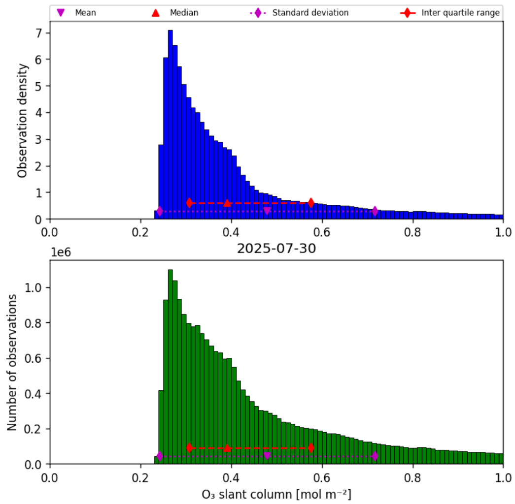
Figure 31: Histogram of “O 3 slant column” for 2025-07-30 to 2025-07-31
