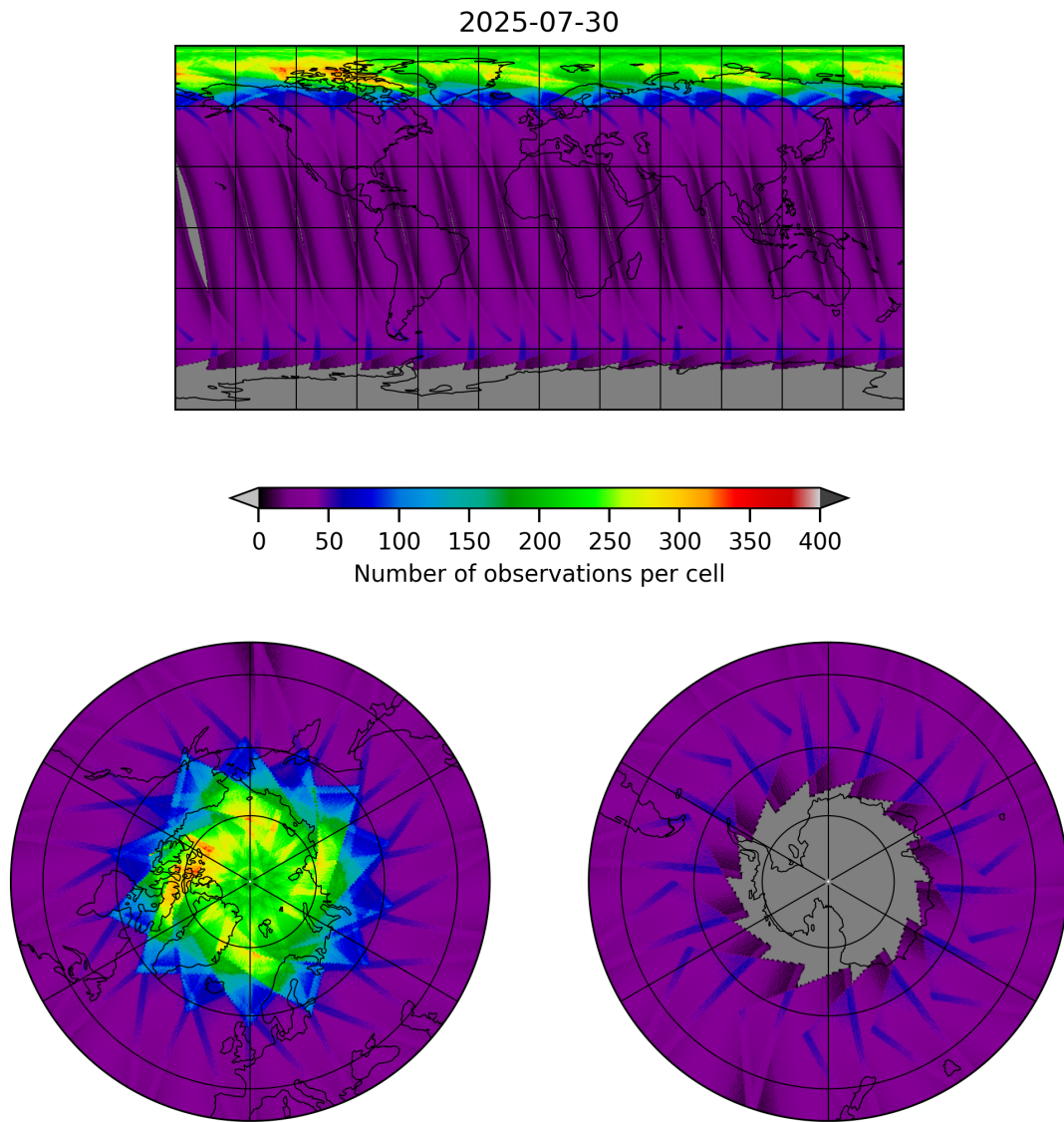
Figure 15: Map of the number of observations for 2025-07-30 to 2025-07-31
