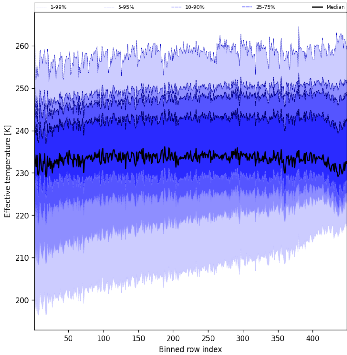
Figure 50: Along track statistics of “Effective temperature” for 2025-07-30 to 2025-07-31
