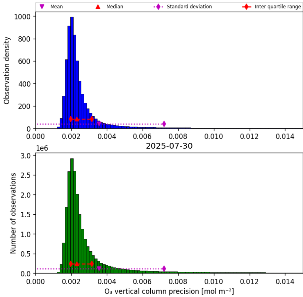
Figure 30: Histogram of “O 3 vertical column precision” for 2025-07-30 to 2025-07-31
