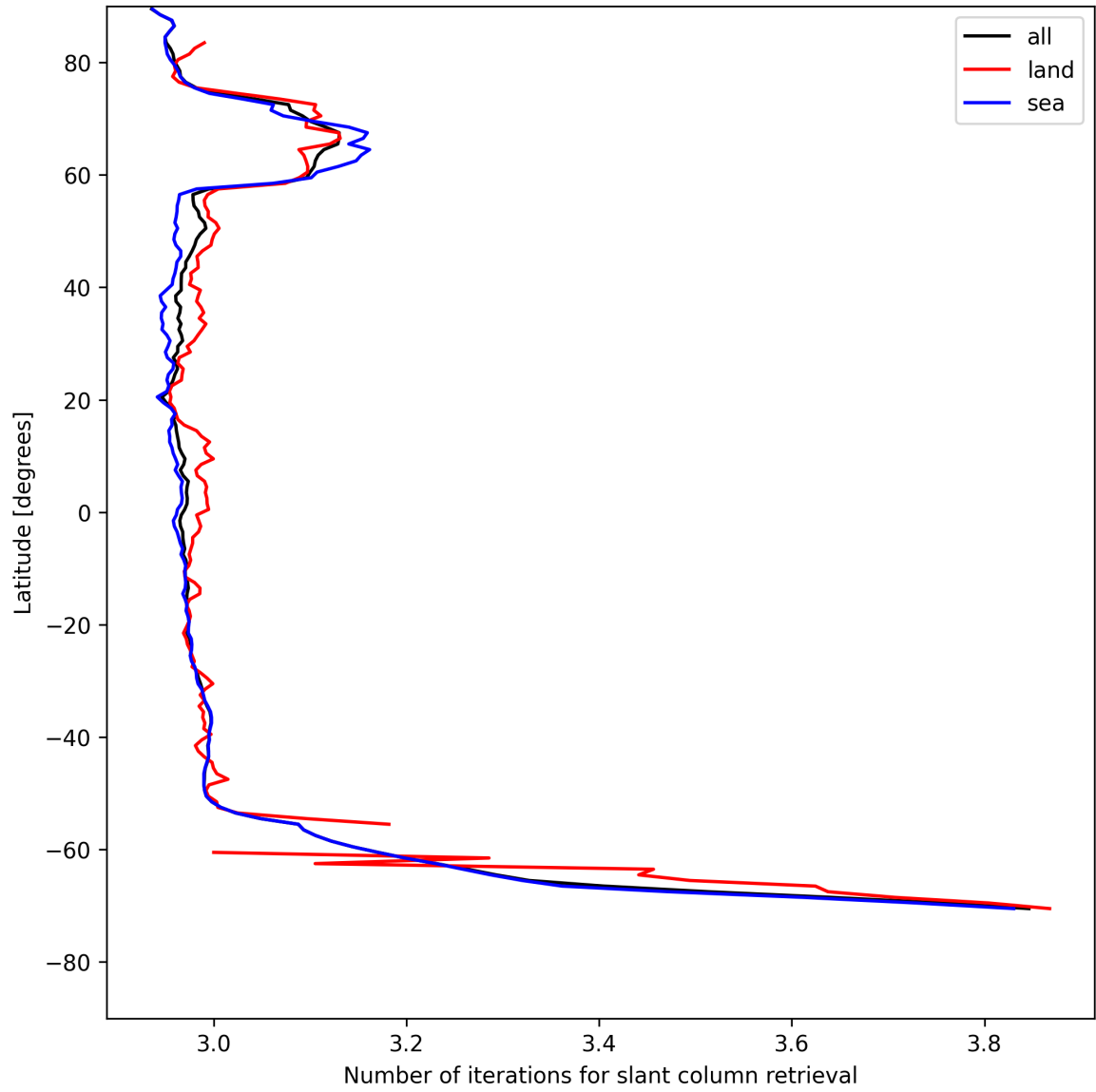
Figure 21: Zonal average of “Number of iterations for slant column retrieval” for 2025-07-30 to 2025-07-31.
