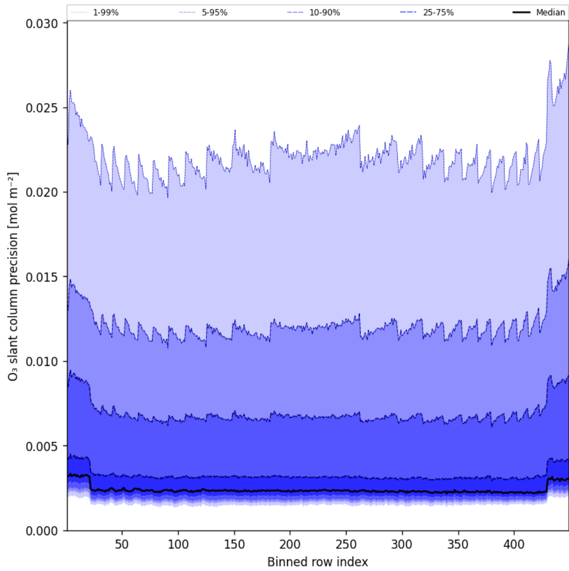
Figure 44: Along track statistics of “O 3 slant column precision” for 2025-07-30 to 2025-07-31
