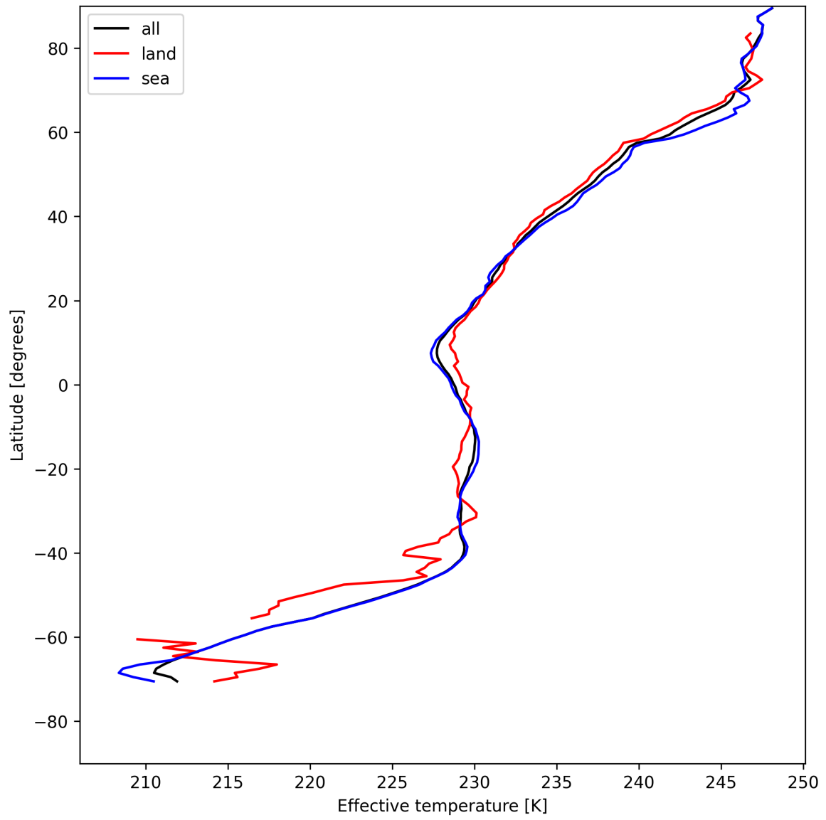
Figure 26: Zonal average of “Effective temperature” for 2025-07-30 to 2025-07-31.
