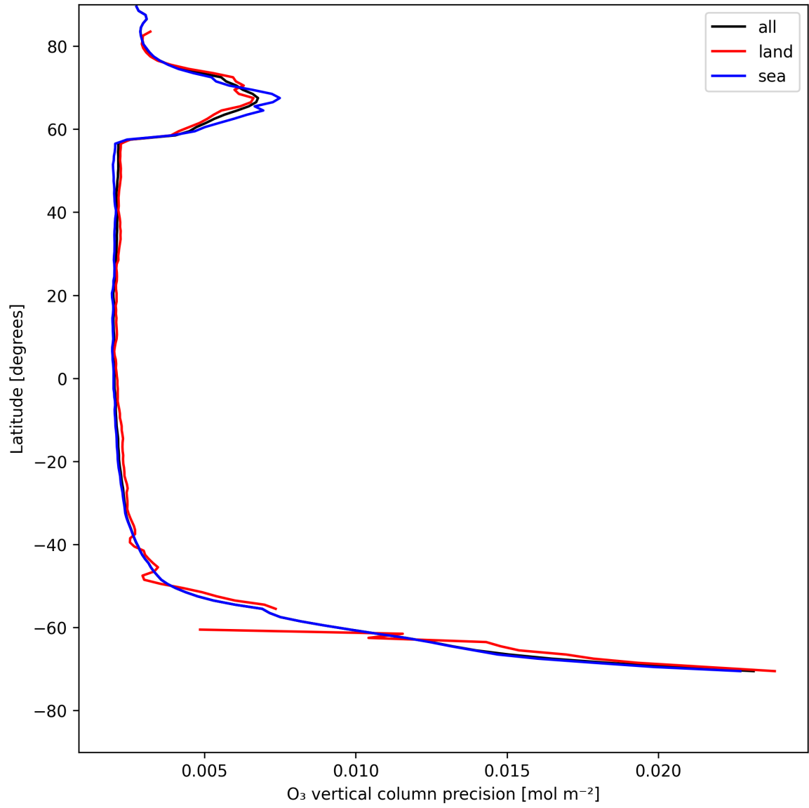
Figure 18: Zonal average of “O 3 vertical column precision” for 2025-07-30 to 2025-07-31.
