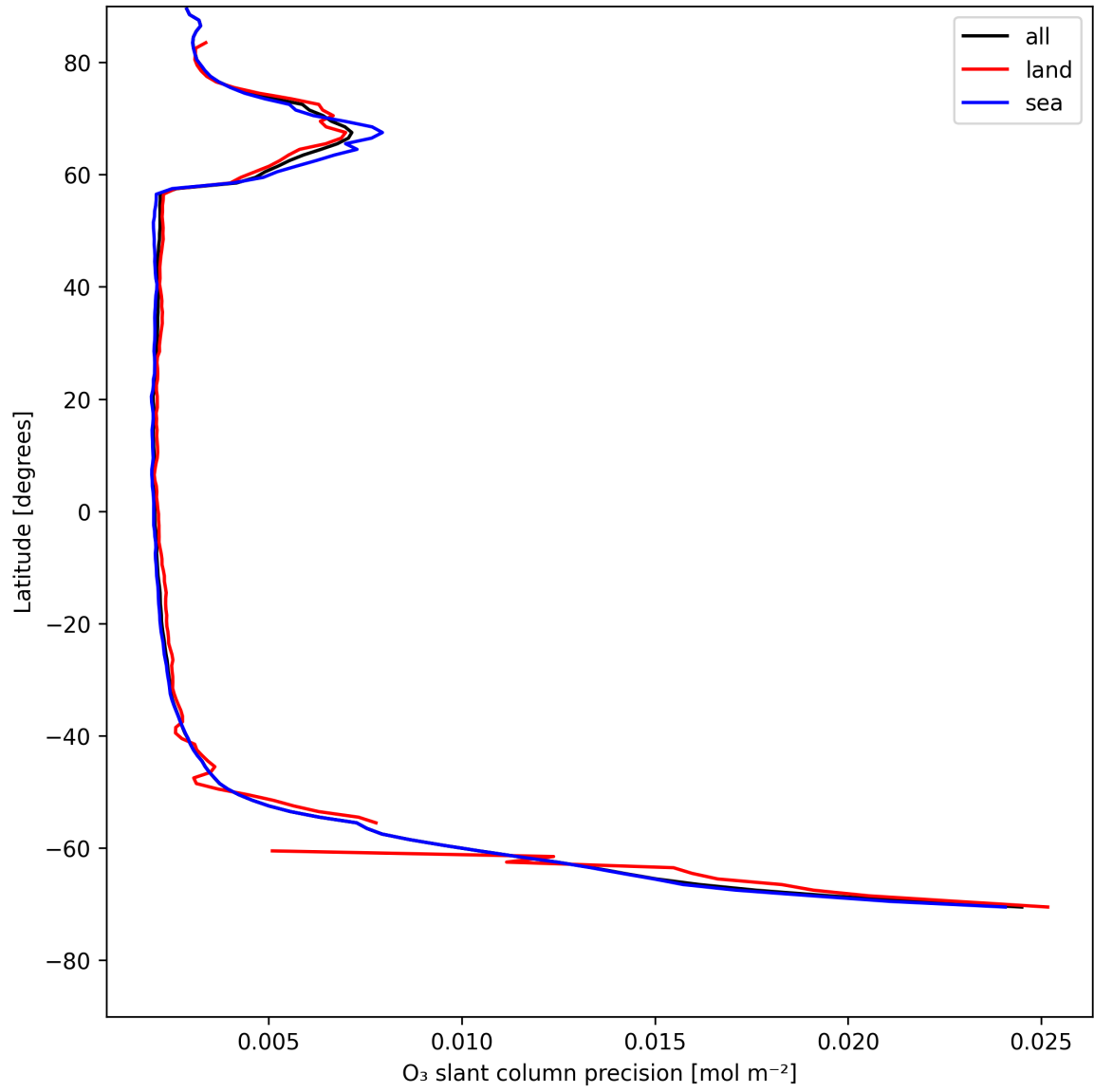
Figure 20: Zonal average of "O 3 slant column precision" for 2025-07-30 to 2025-07-31.
