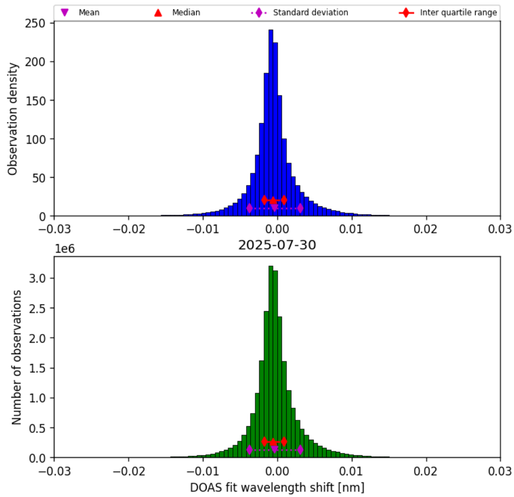
Figure 35: Histogram of “DOAS fit wavelength shift” for 2025-07-30 to 2025-07-31
