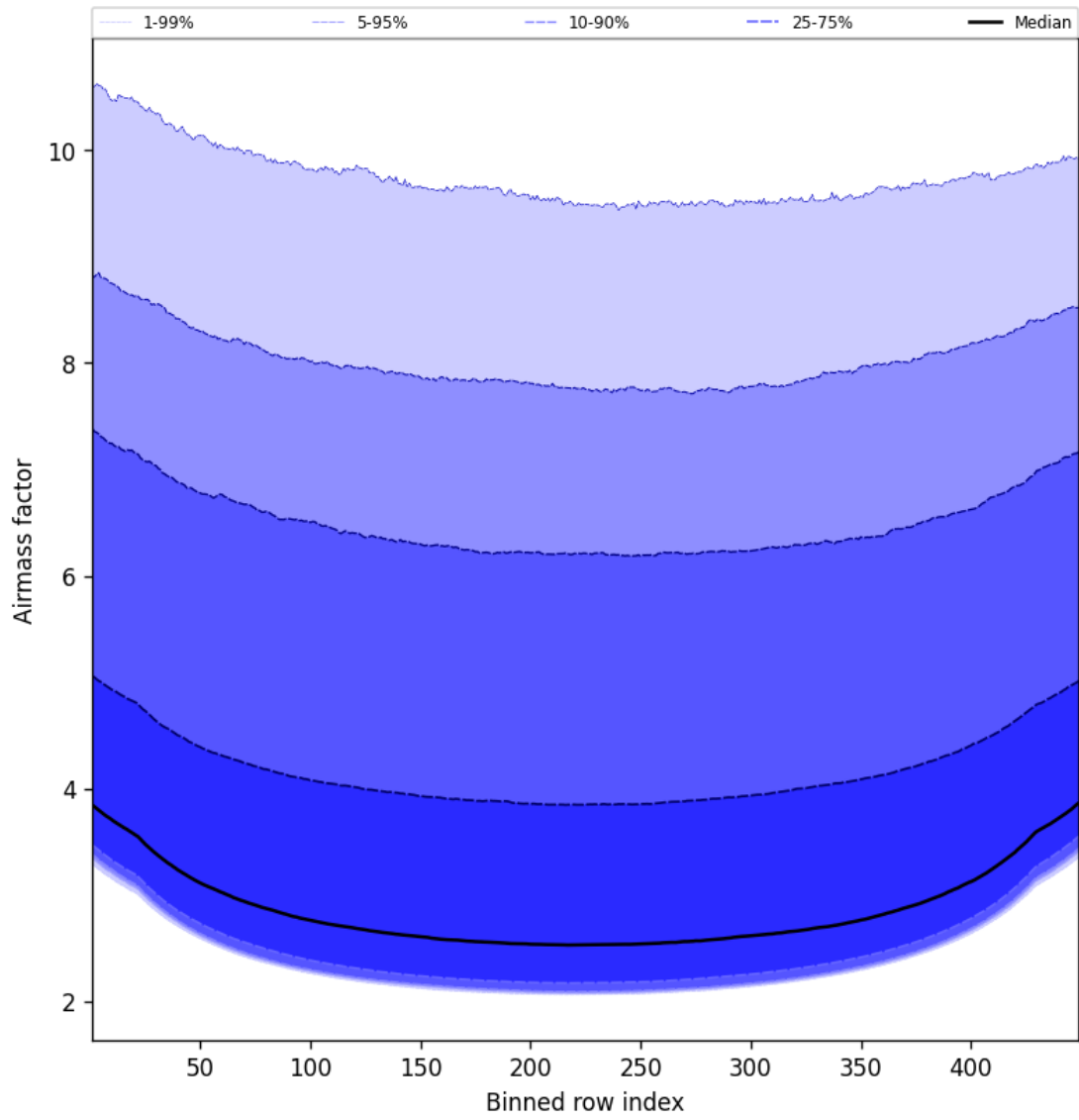
Figure 49: Along track statistics of “Airmass factor” for 2025-07-30 to 2025-07-31
