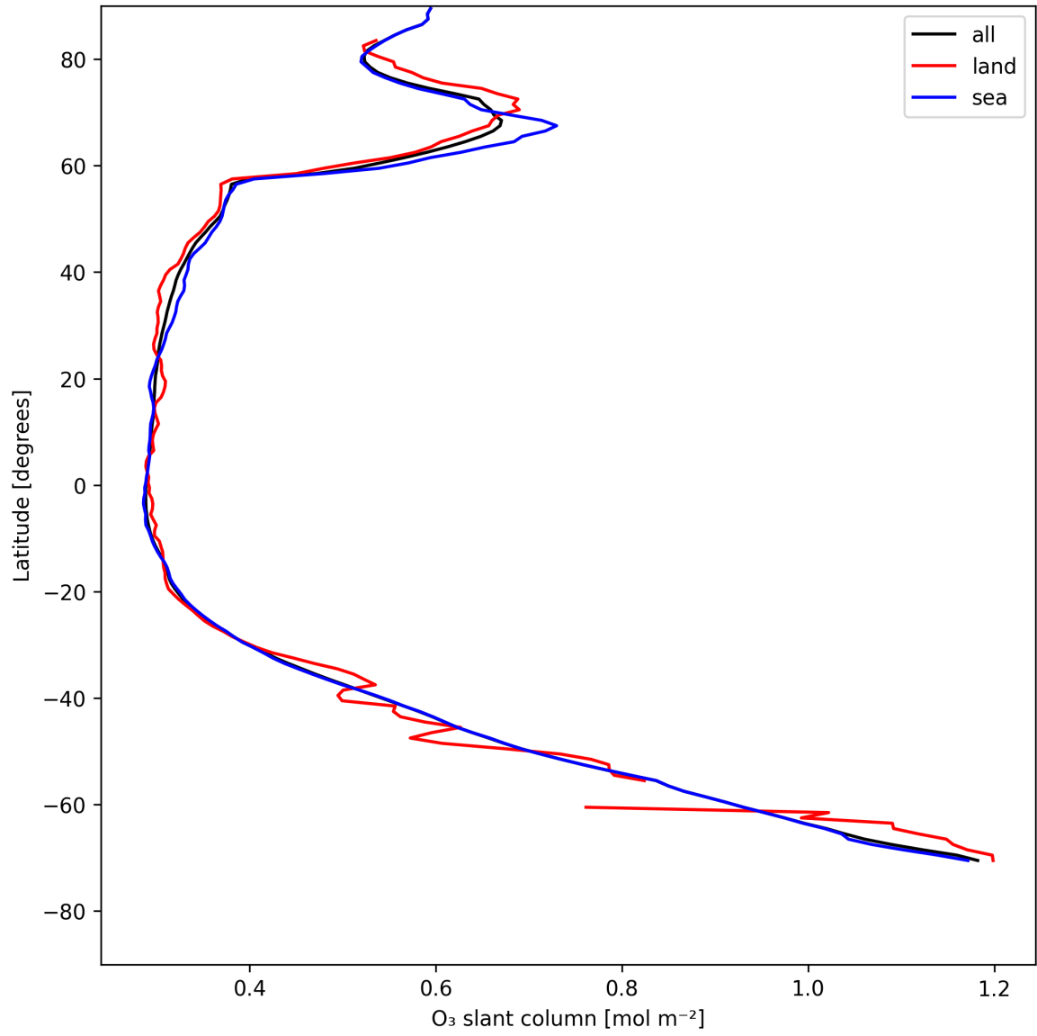
Figure 19: Zonal average of “O 3 slant column” for 2025-07-30 to 2025-07-31.
