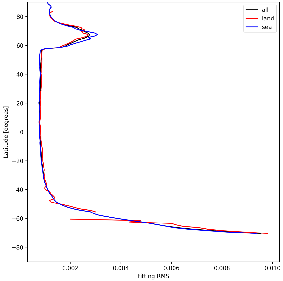
Figure 22: Zonal average of “Fitting RMS” for 2025-07-30 to 2025-07-31.
