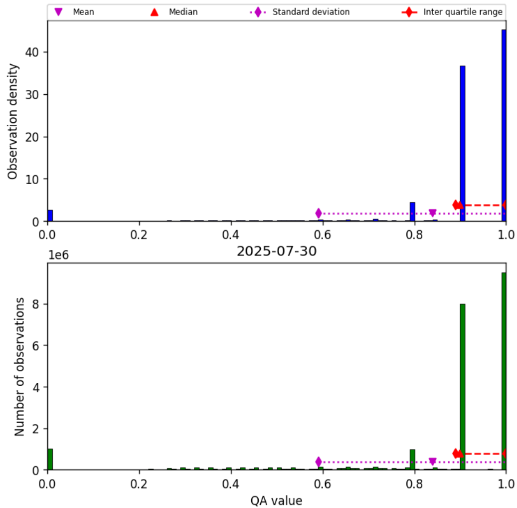
Figure 28: Histogram of “QA value” for 2025-07-30 to 2025-07-31
