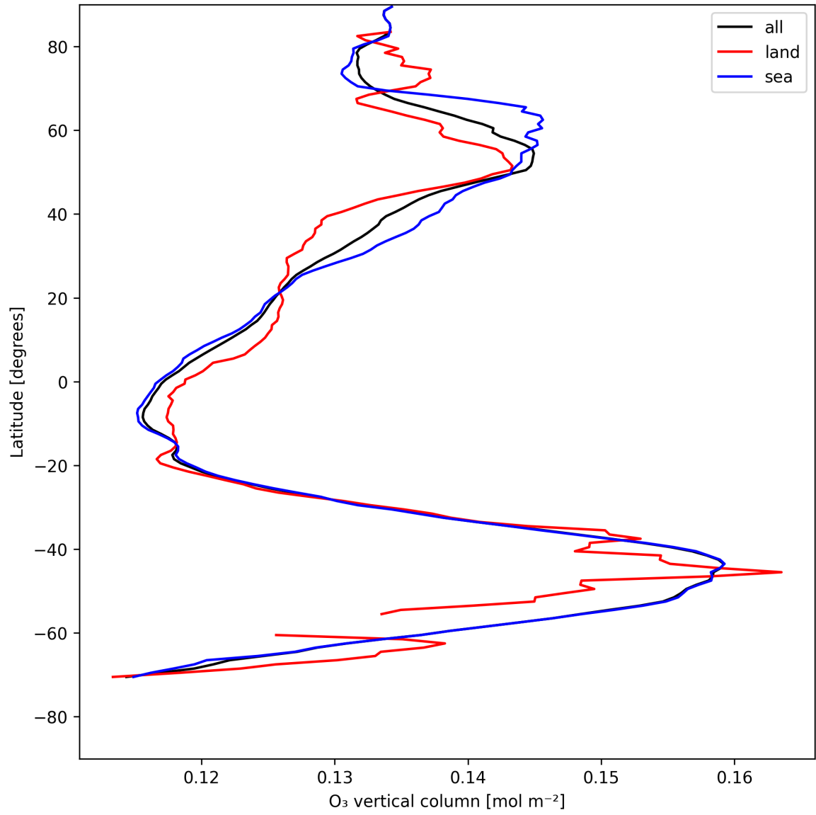
Figure 17: Zonal average of “O 3 vertical column” for 2025-07-30 to 2025-07-31.
