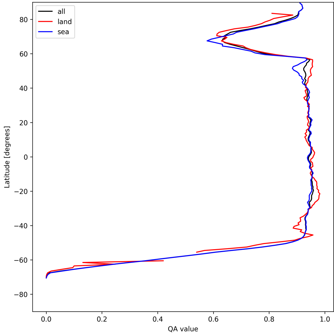
Figure 16: Zonal average of “QA value” for 2025-07-30 to 2025-07-31.
