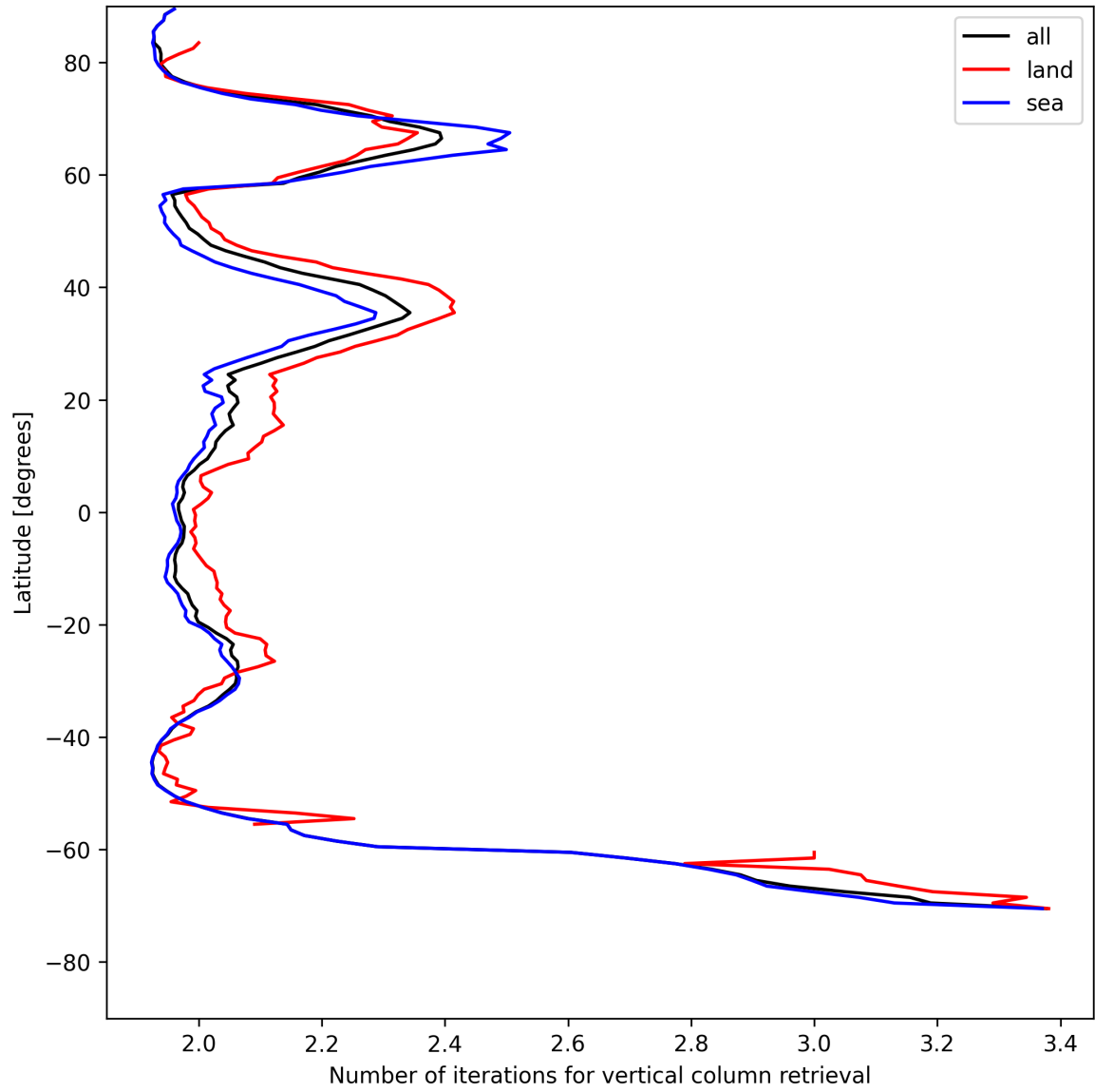
Figure 27: Zonal average of “Number of iterations for vertical column retrieval” for 2025-07-30 to 2025-07-31.
