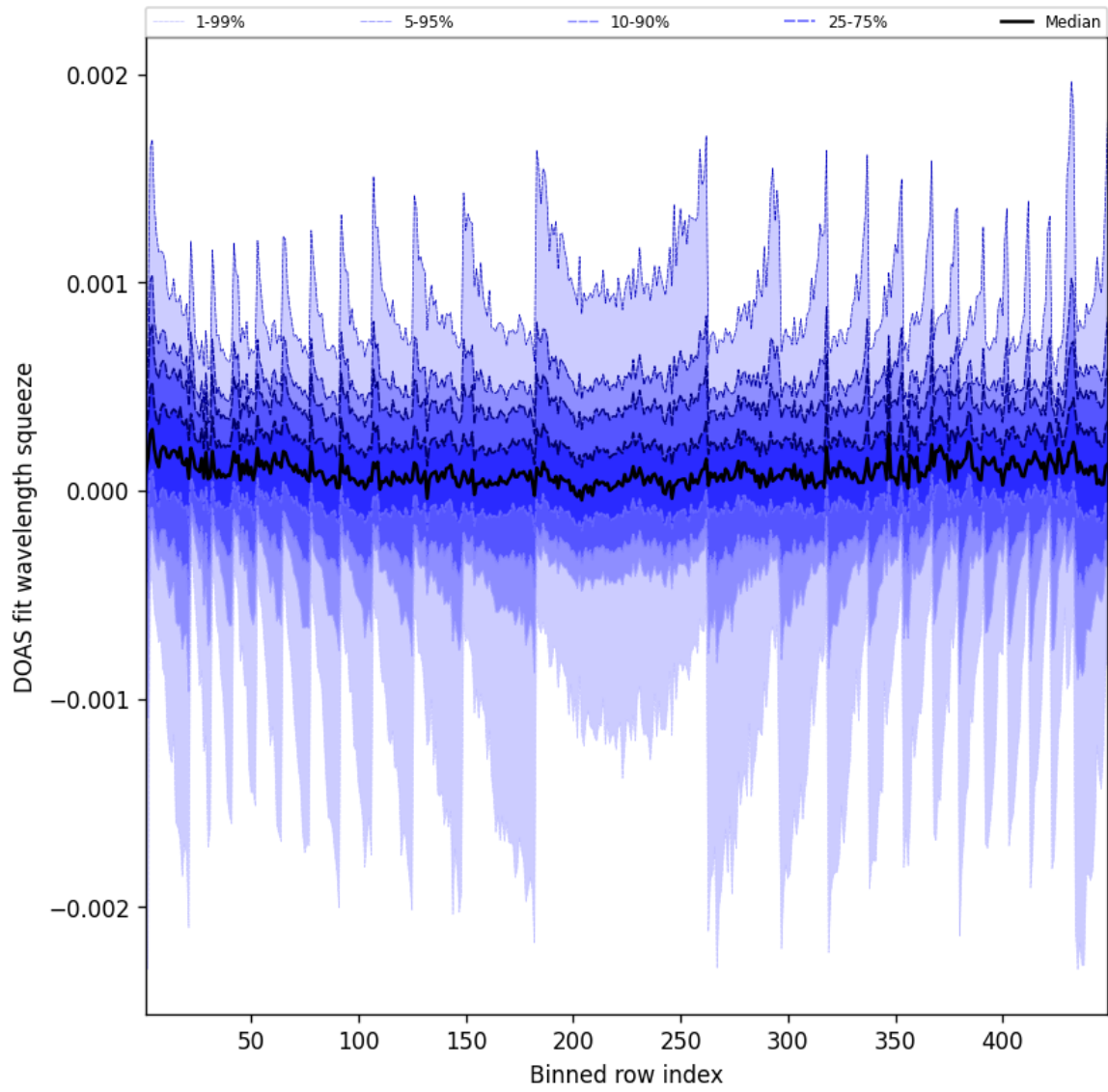
Figure 48: Along track statistics of “DOAS fit wavelength squeeze” for 2025-07-30 to 2025-07-31
