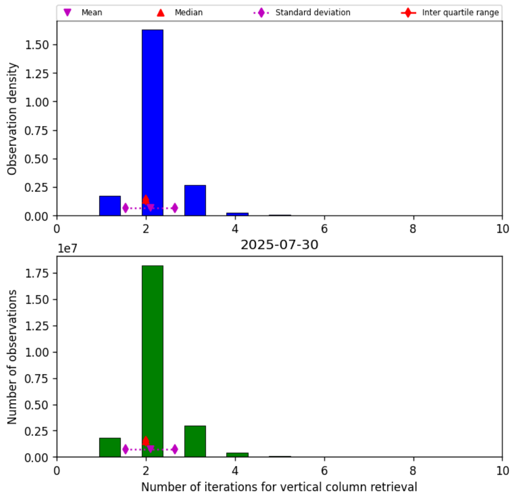
Figure 39: Histogram of “Number of iterations for vertical column retrieval” for 2025-07-30 to 2025-07-31
