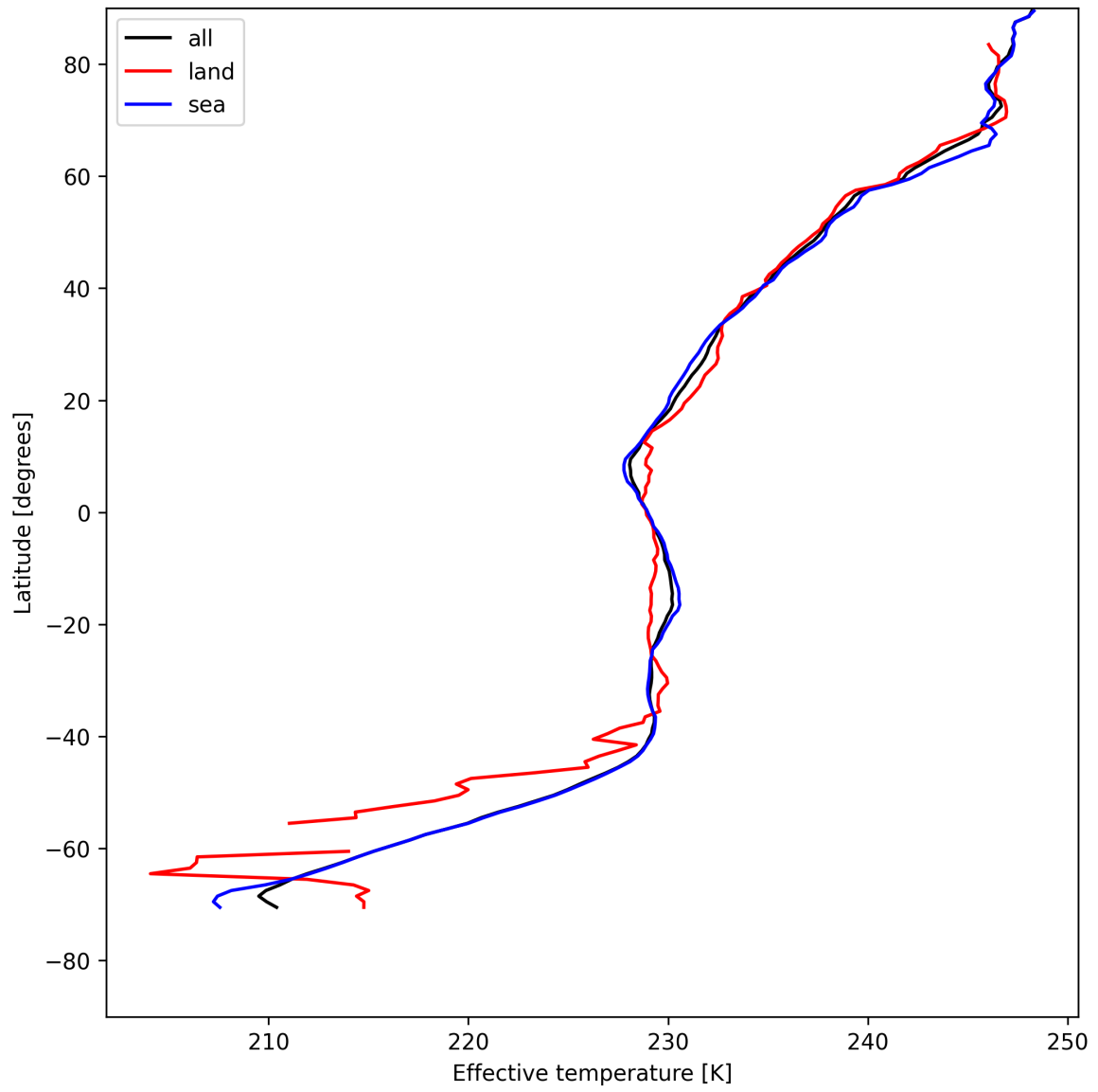
Figure 26: Zonal average of "Effective temperature" for 2025-07-31 to 2025-08-01.
