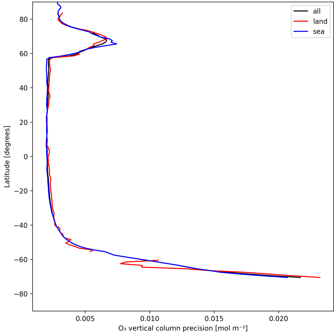
Figure 18: Zonal average of “O 3 vertical column precision” for 2025-07-31 to 2025-08-01.
