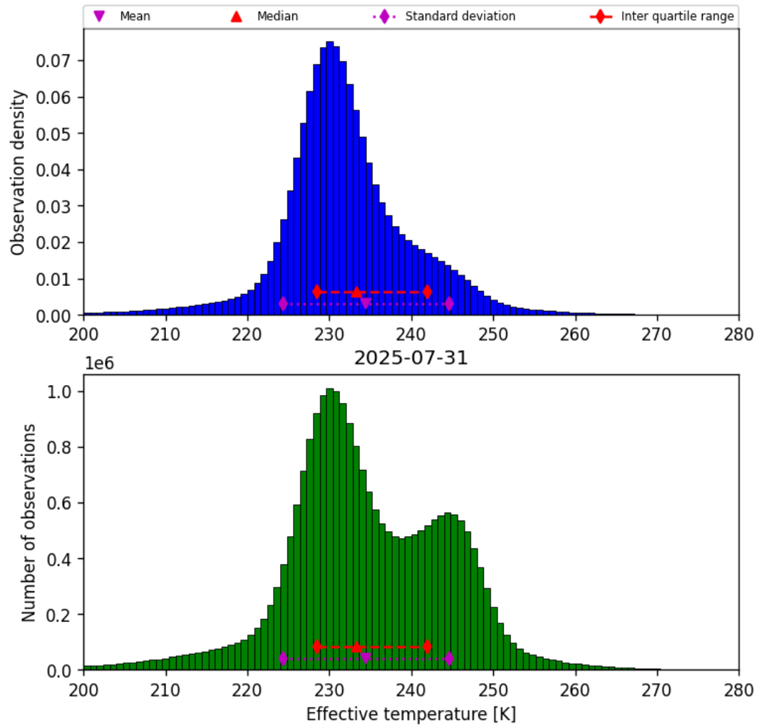
Figure 38: Histogram of “Effective temperature” for 2025-07-31 to 2025-08-01
