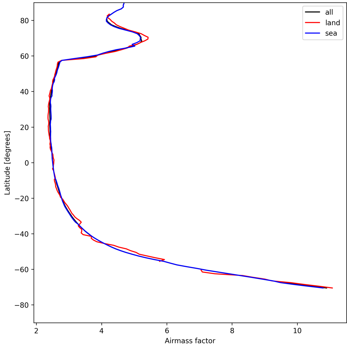
Figure 25: Zonal average of “Airmass factor” for 2025-07-31 to 2025-08-01.
