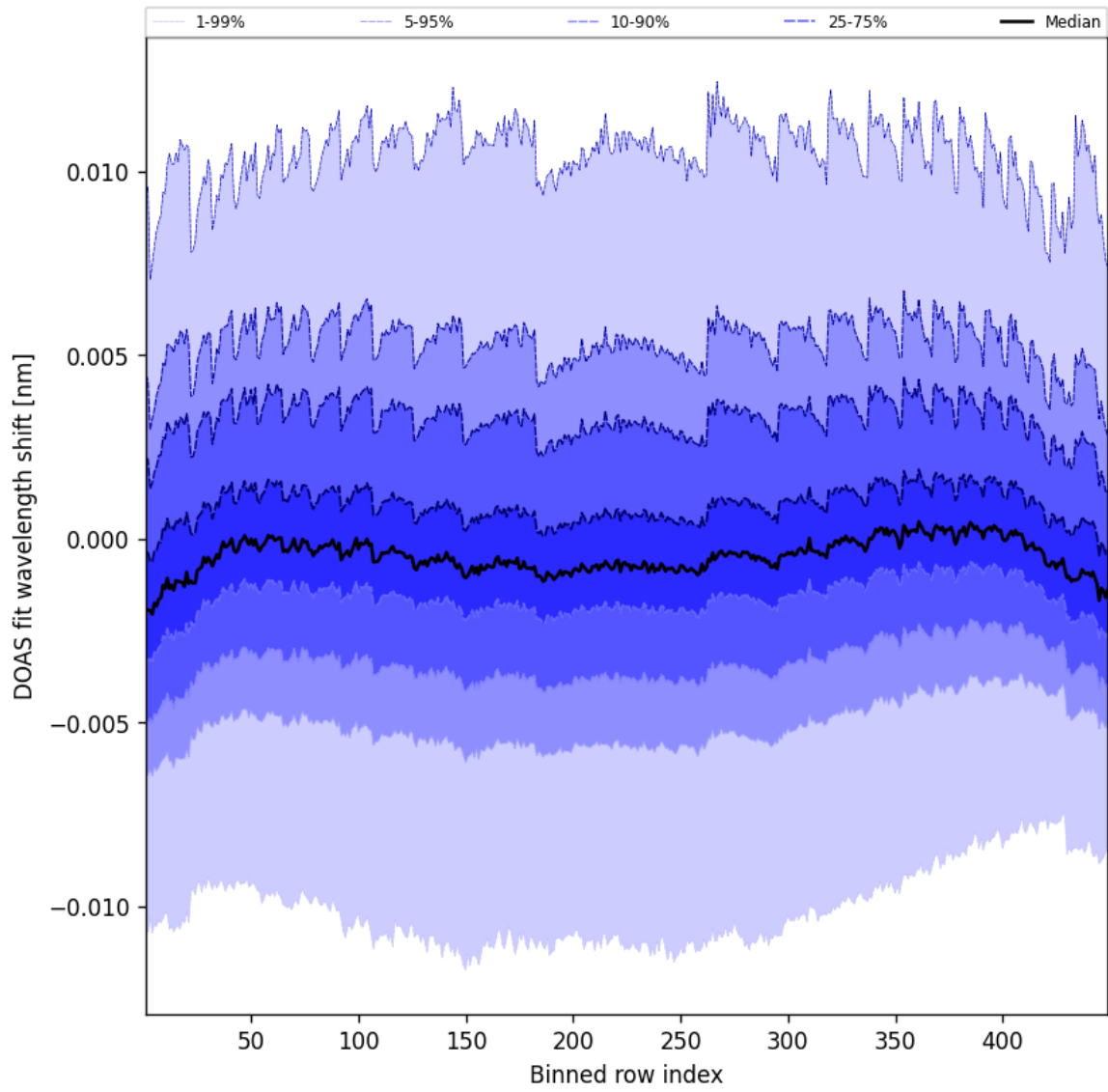
Figure 47: Along track statistics of “DOAS fit wavelength shift” for 2025-07-31 to 2025-08-01
