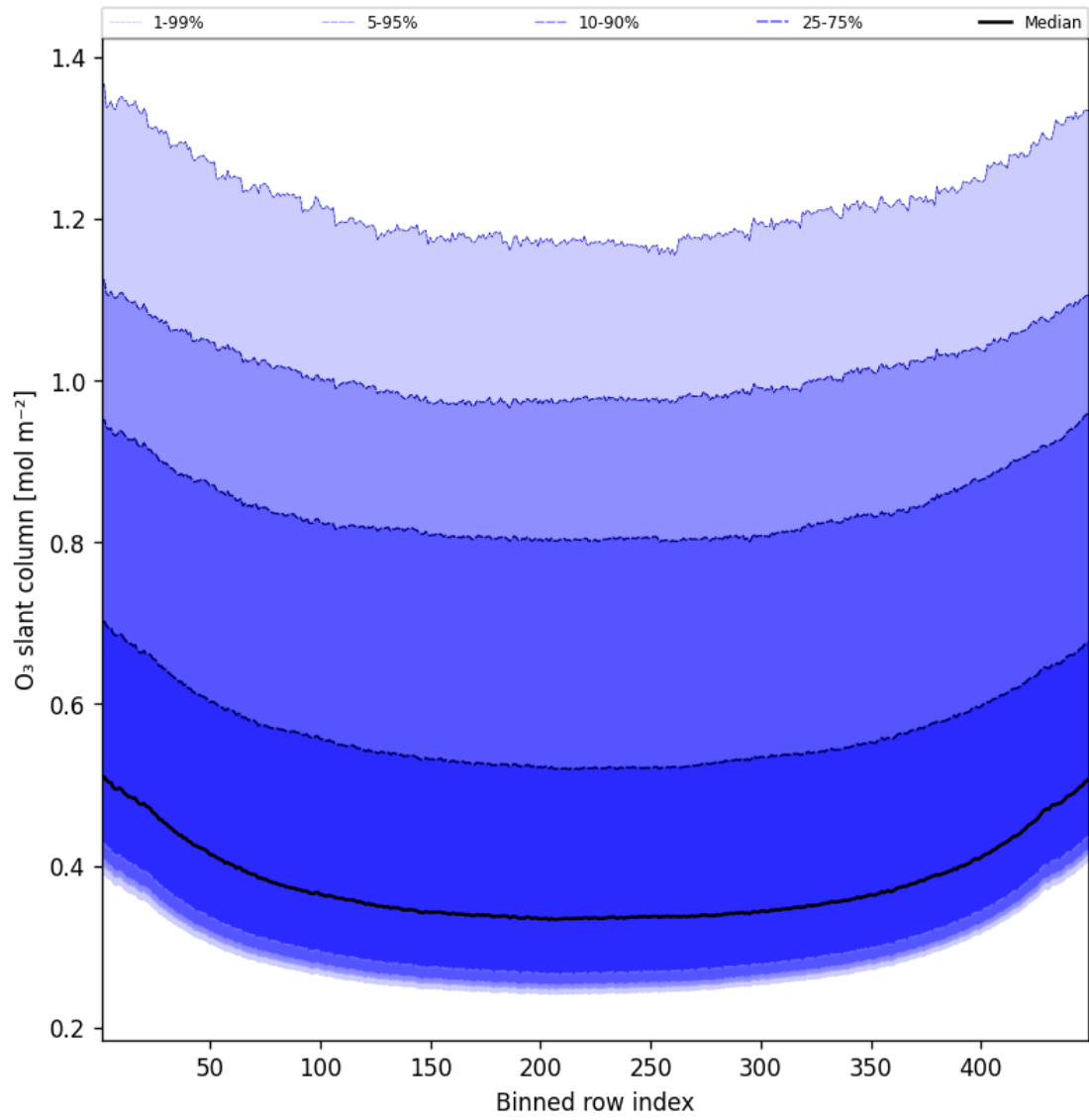
Figure 43: Along track statistics of “O 3 slant column” for 2025-07-31 to 2025-08-01
