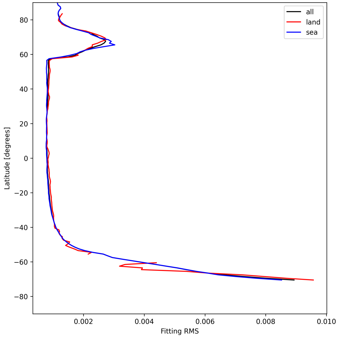
Figure 22: Zonal average of “Fitting RMS” for 2025-07-31 to 2025-08-01.
