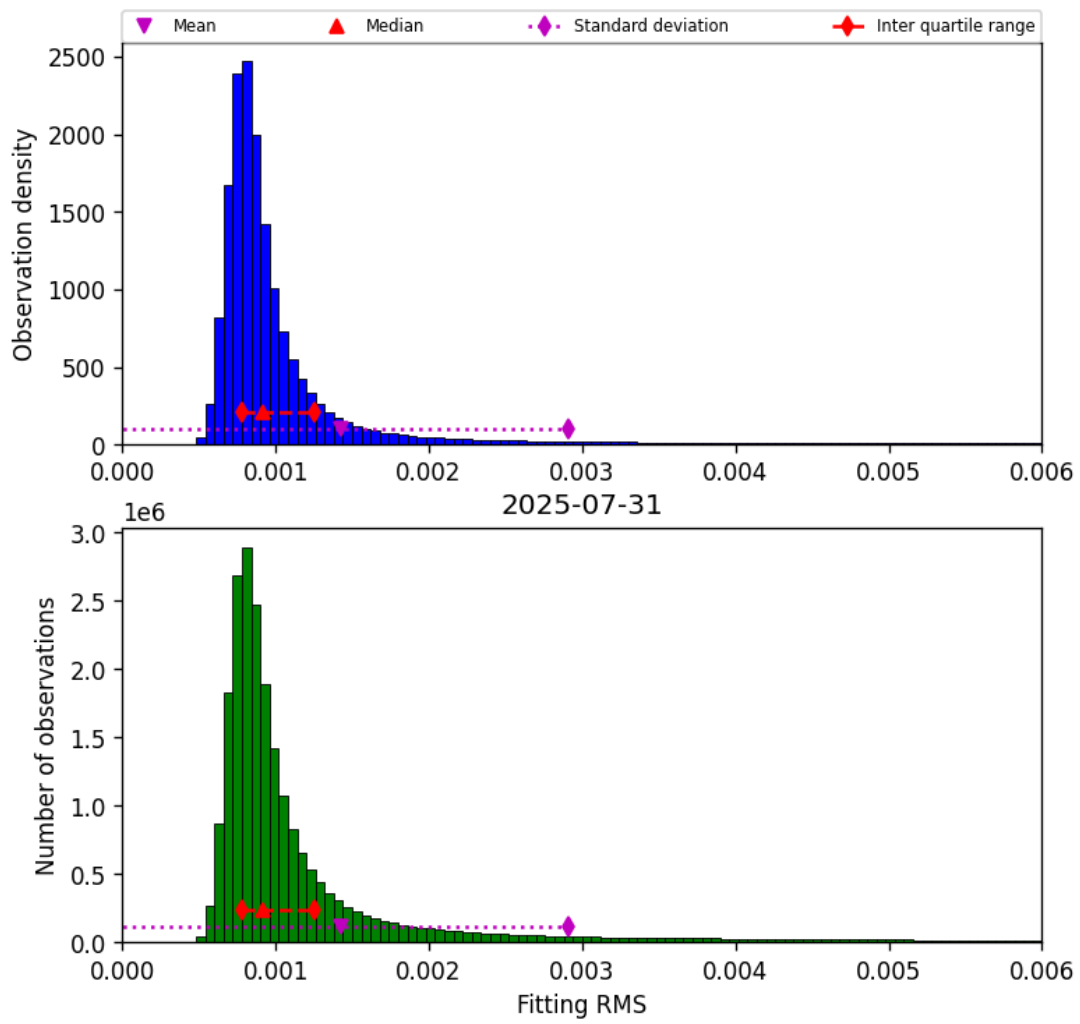
Figure 34: Histogram of “Fitting RMS” for 2025-07-31 to 2025-08-01
