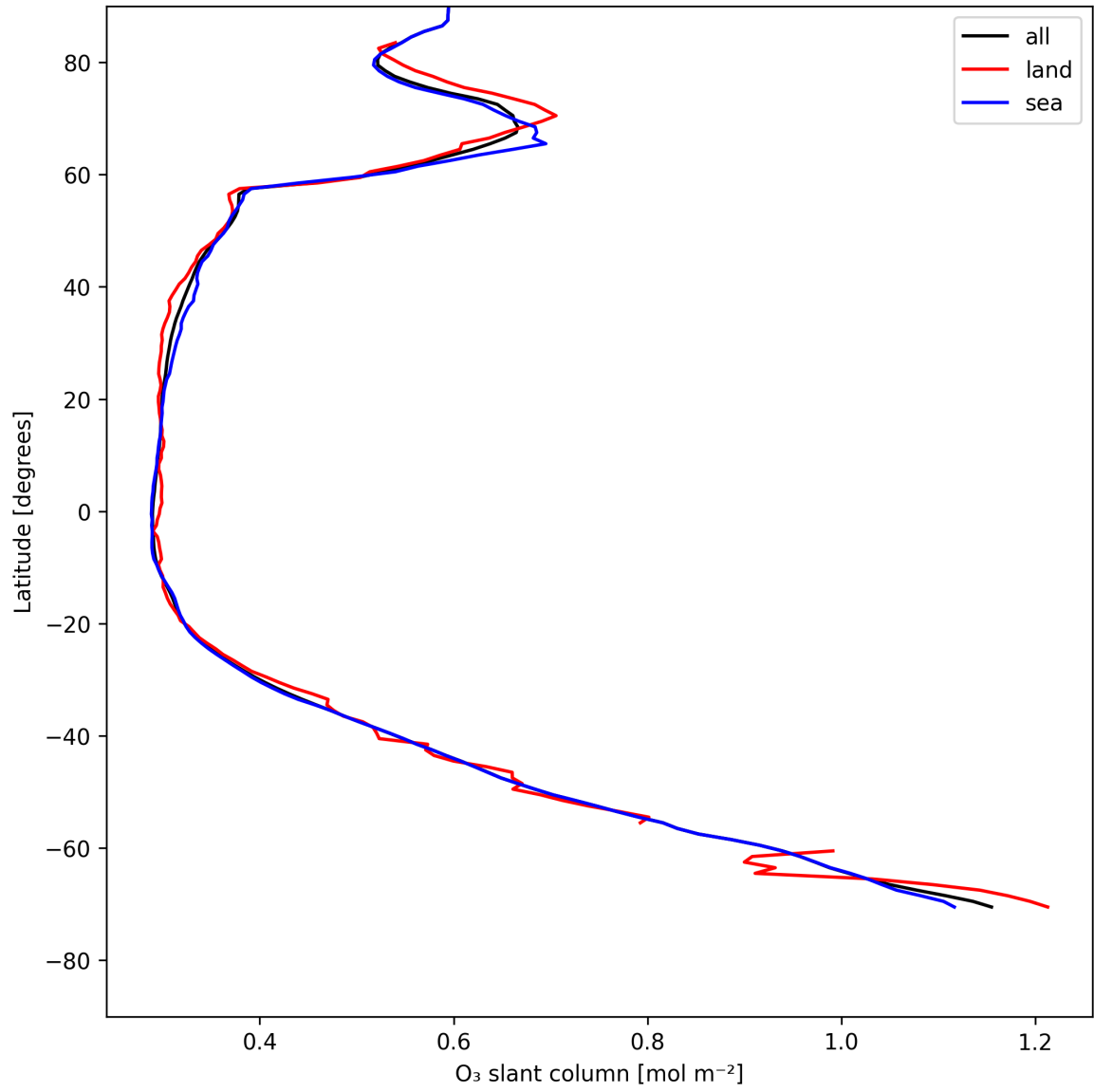
Figure 19: Zonal average of “O 3 slant column” for 2025-07-31 to 2025-08-01.
