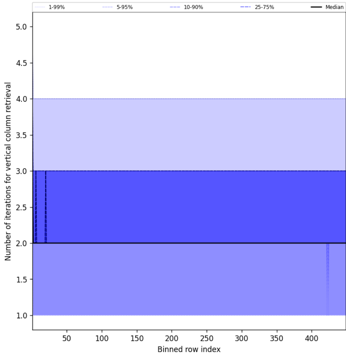
Figure 51: Along track statistics of “Number of iterations for vertical column retrieval” for 2025-07-31 to 2025-08-01
