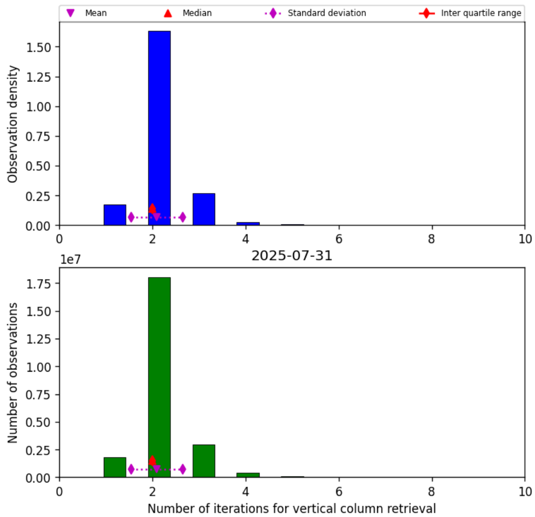
Figure 39: Histogram of “Number of iterations for vertical column retrieval” for 2025-07-31 to 2025-08-01
