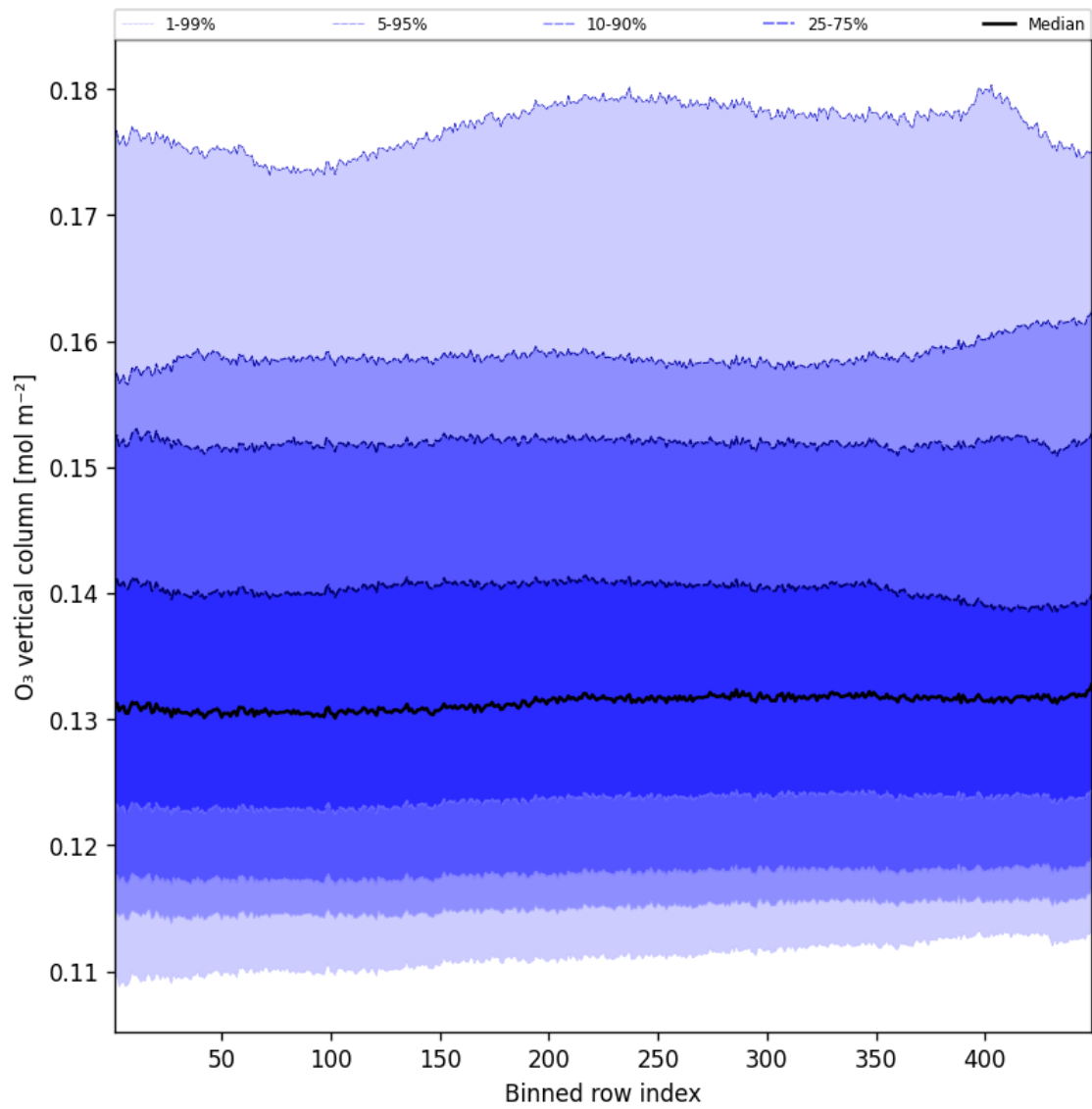
Figure 41: Along track statistics of “O 3 vertical column” for 2025-07-31 to 2025-08-01
