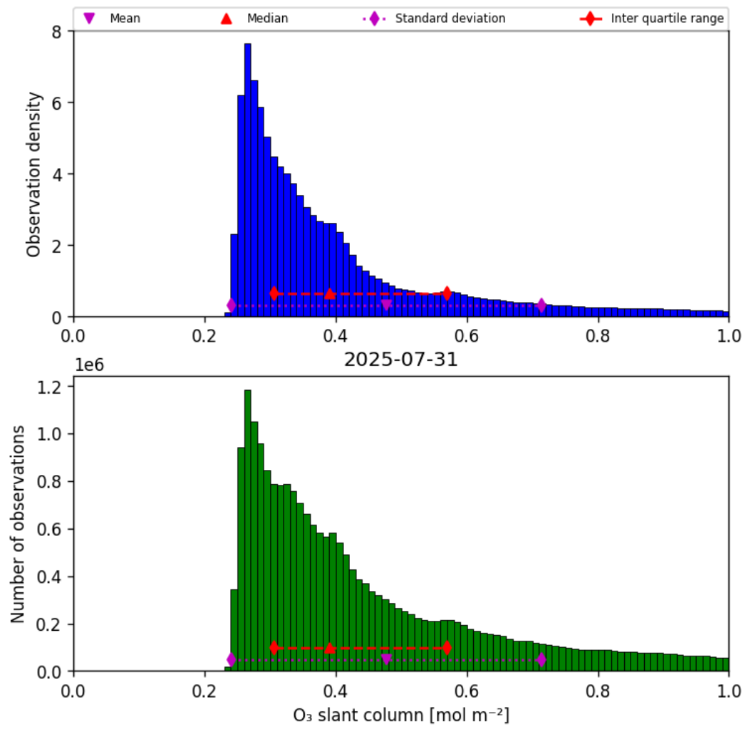
Figure 31: Histogram of “O 3 slant column” for 2025-07-31 to 2025-08-01
