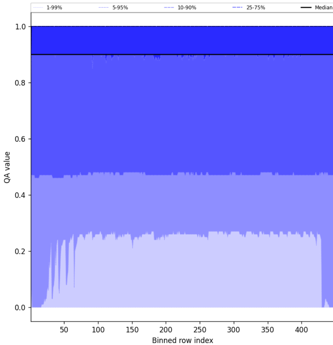
Figure 40: Along track statistics of “QA value” for 2025-07-31 to 2025-08-01
