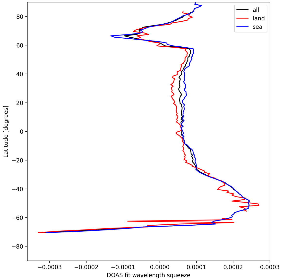
Figure 24: Zonal average of “DOAS fit wavelength squeeze” for 2025-07-31 to 2025-08-01.
