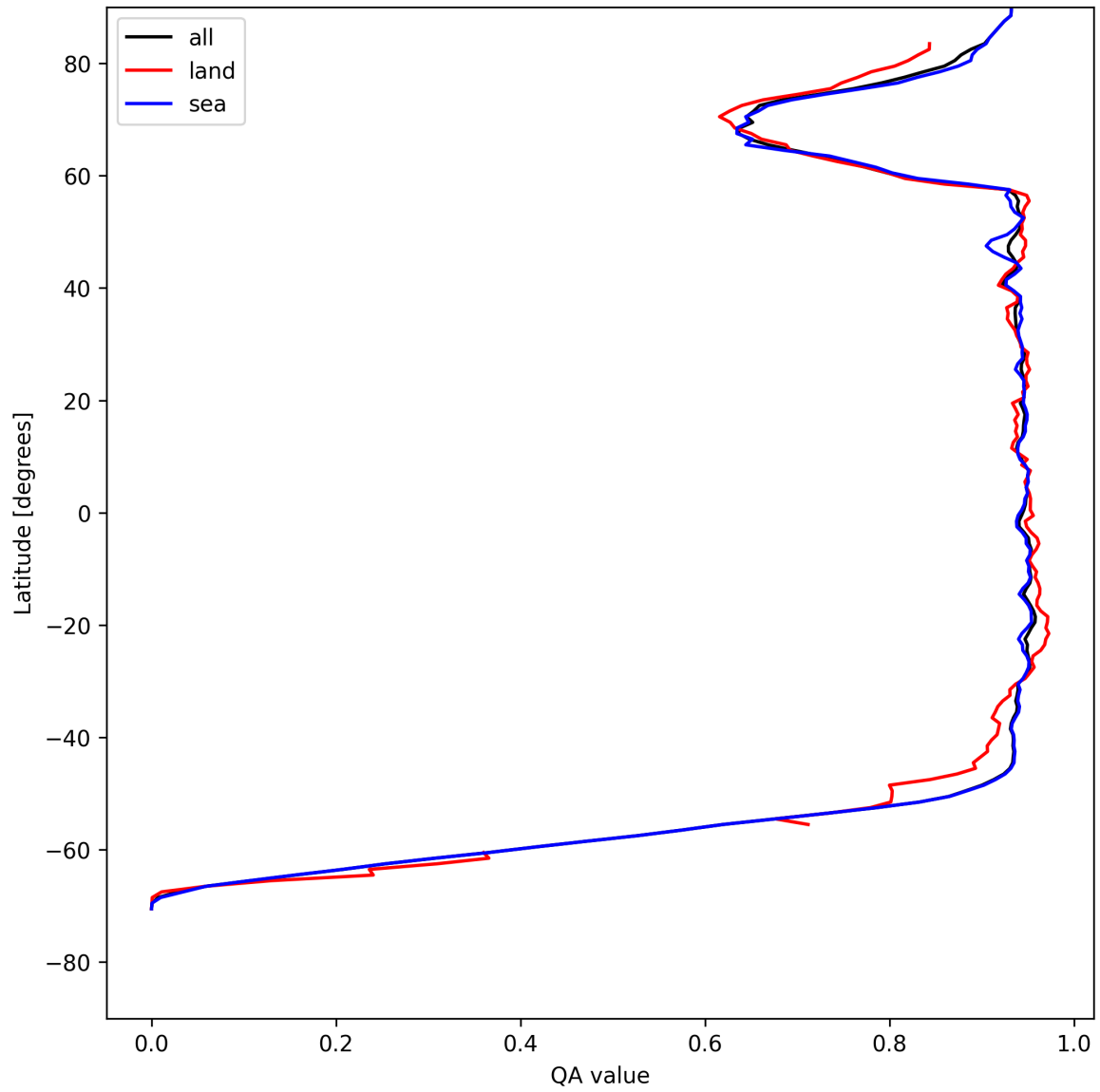
Figure 16: Zonal average of “QA value” for 2025-07-31 to 2025-08-01.
