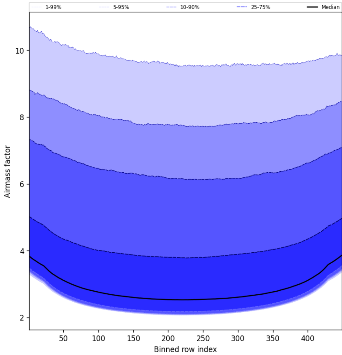
Figure 49: Along track statistics of “Airmass factor” for 2025-07-31 to 2025-08-01
