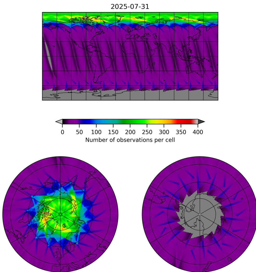
Figure 15: Map of the number of observations for 2025-07-31 to 2025-08-01
