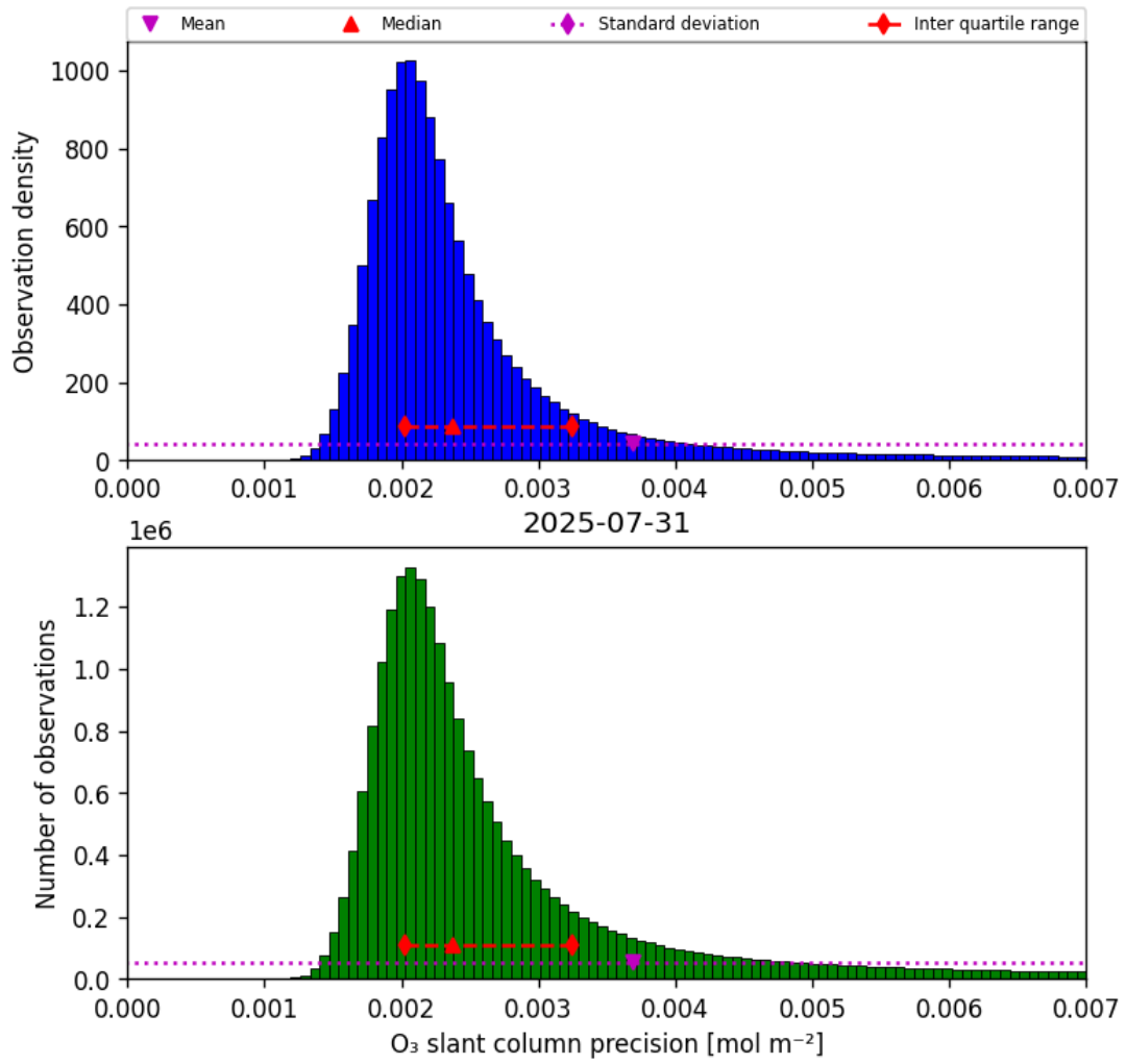
Figure 32: Histogram of “O 3 slant column precision” for 2025-07-31 to 2025-08-01
