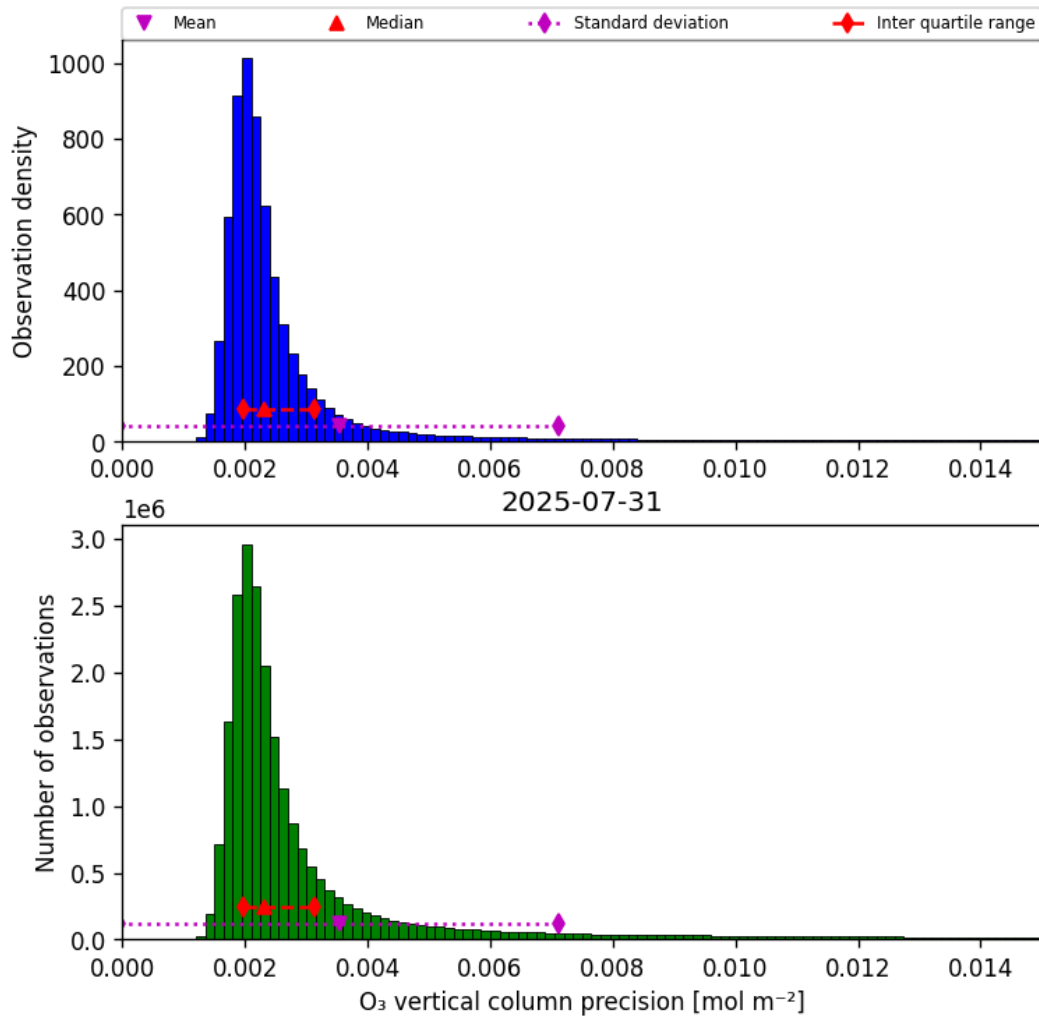
Figure 30: Histogram of “O 3 vertical column precision” for 2025-07-31 to 2025-08-01
