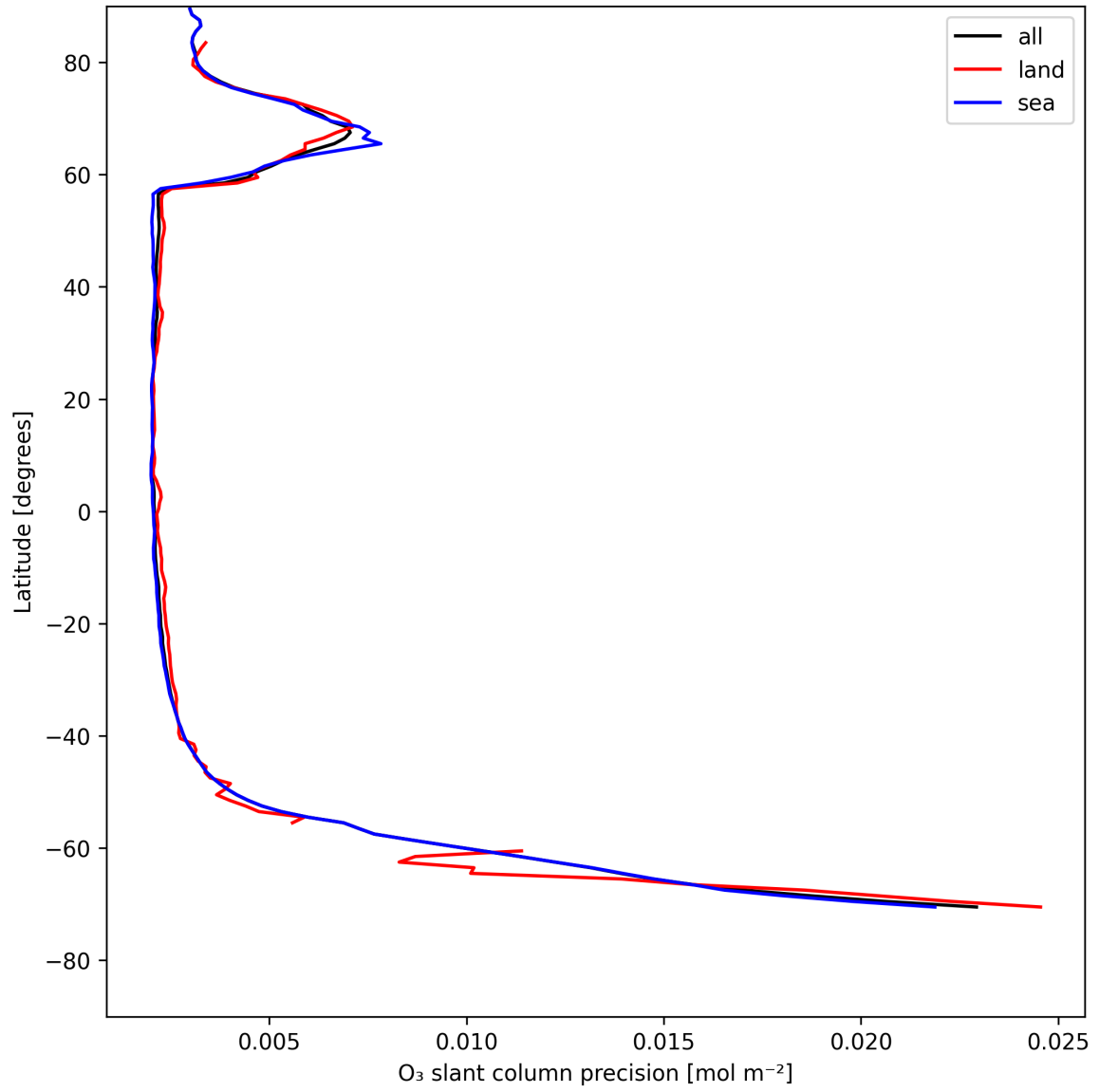
Figure 20: Zonal average of “O 3 slant column precision” for 2025-07-31 to 2025-08-01.
