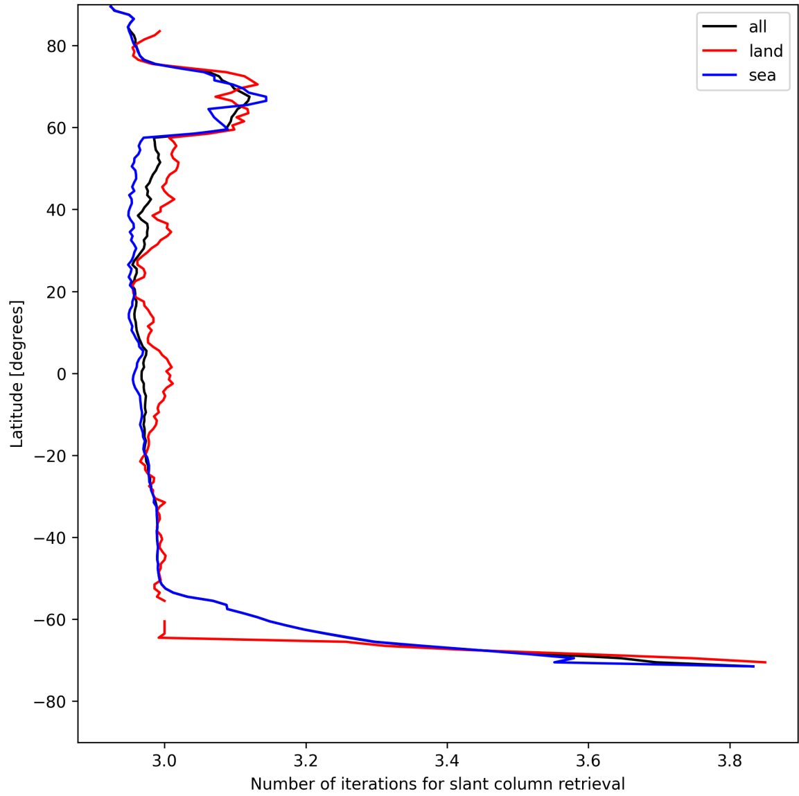
Figure 21: Zonal average of “Number of iterations for slant column retrieval” for 2025-08-01 to 2025-08-01.
