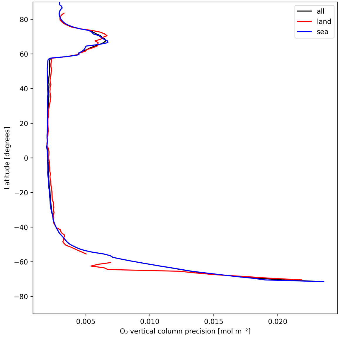
Figure 18: Zonal average of “O 3 vertical column precision” for 2025-08-01 to 2025-08-01.
