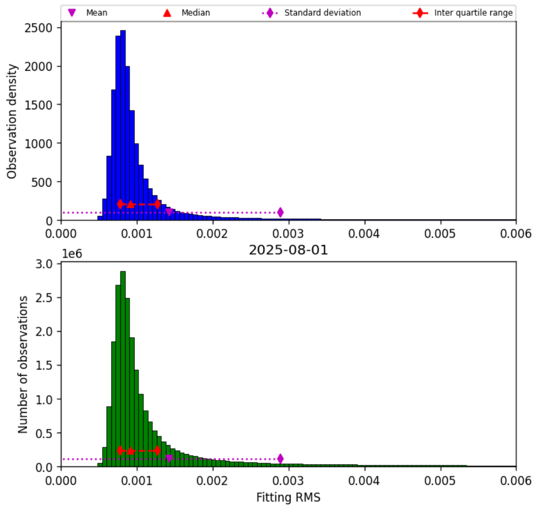
Figure 34: Histogram of “Fitting RMS” for 2025-08-01 to 2025-08-01
