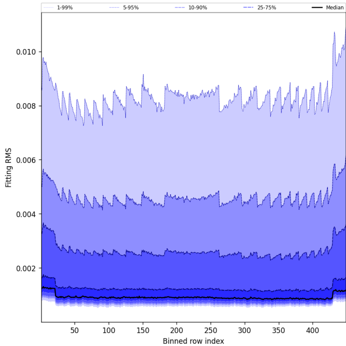
Figure 46: Along track statistics of “Fitting RMS” for 2025-08-01 to 2025-08-01
