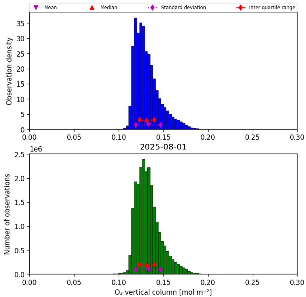
Figure 29: Histogram of “O 3 vertical column” for 2025-08-01 to 2025-08-01
