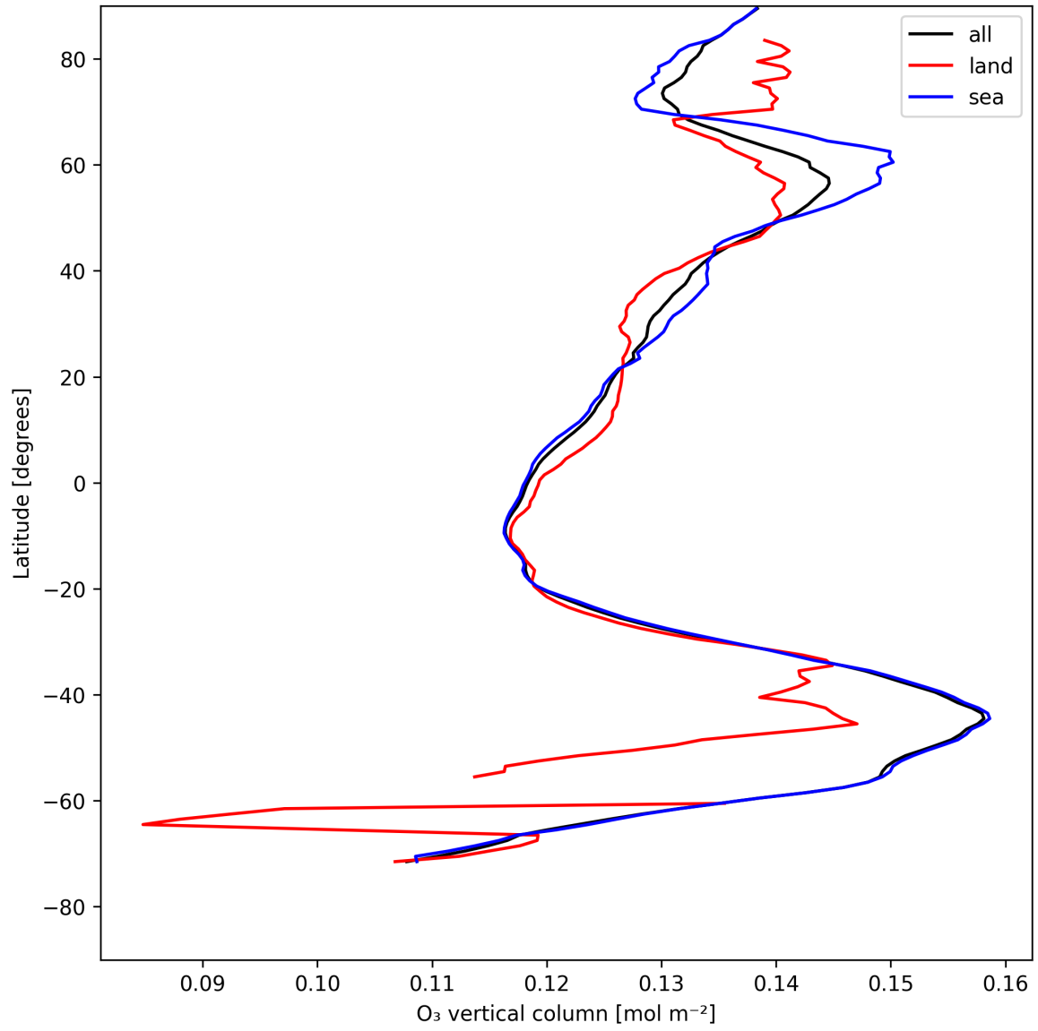
Figure 17: Zonal average of “O 3 vertical column” for 2025-08-03 to 2025-08-04.
