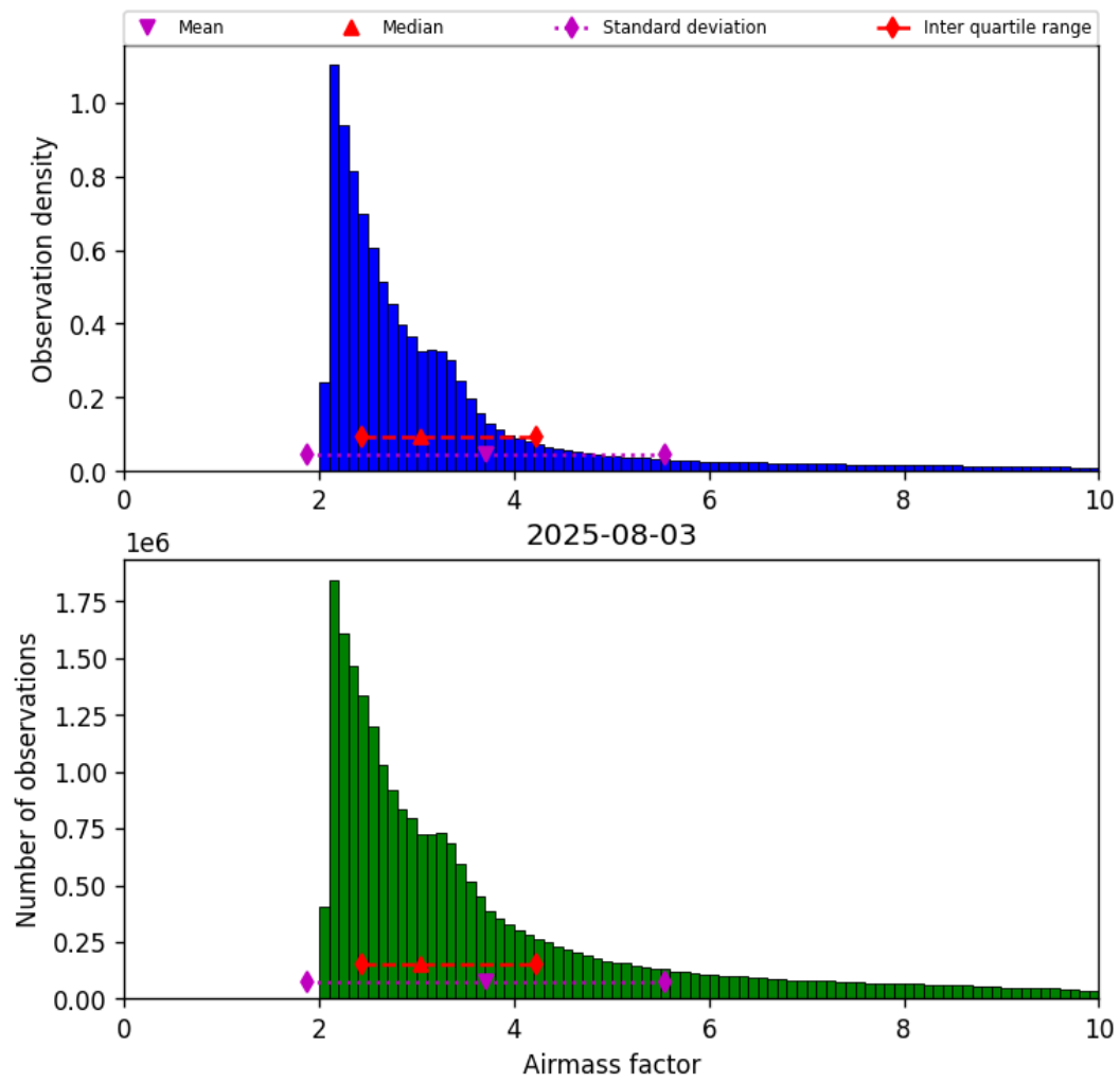
Figure 37: Histogram of “Airmass factor” for 2025-08-03 to 2025-08-04
