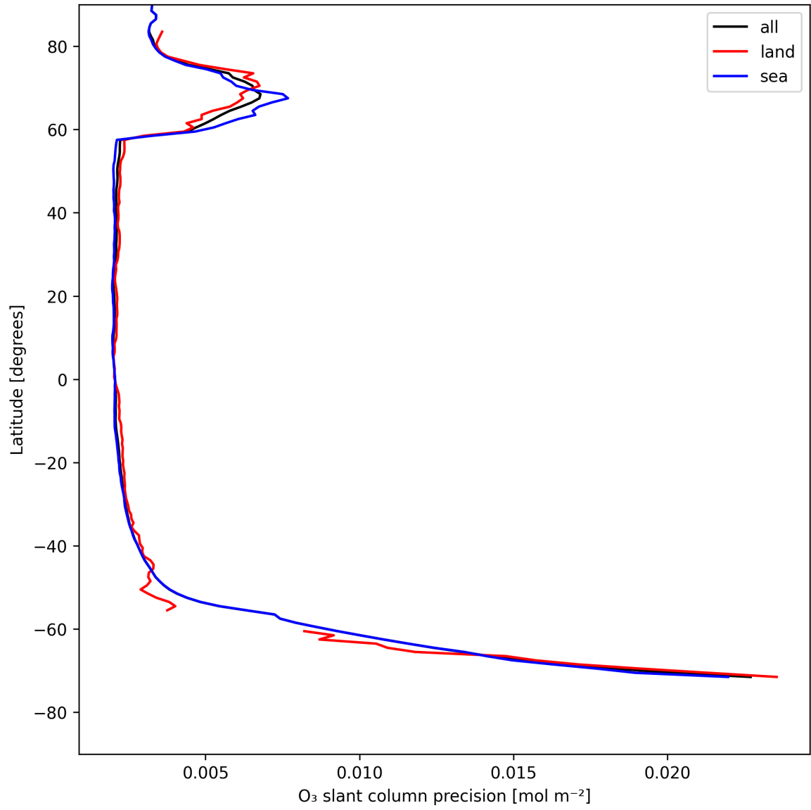
Figure 20: Zonal average of “O 3 slant column precision” for 2025-08-03 to 2025-08-04.
