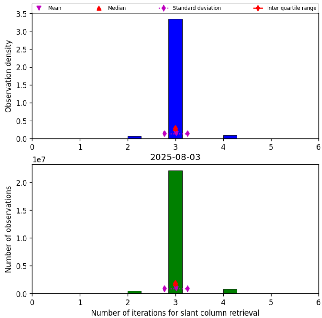
Figure 33: Histogram of "Number of iterations for slant column retrieval" for 2025-08-03 to 2025-08-04
