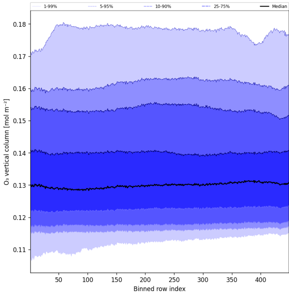
Figure 41: Along track statistics of “O 3 vertical column” for 2025-08-03 to 2025-08-04
