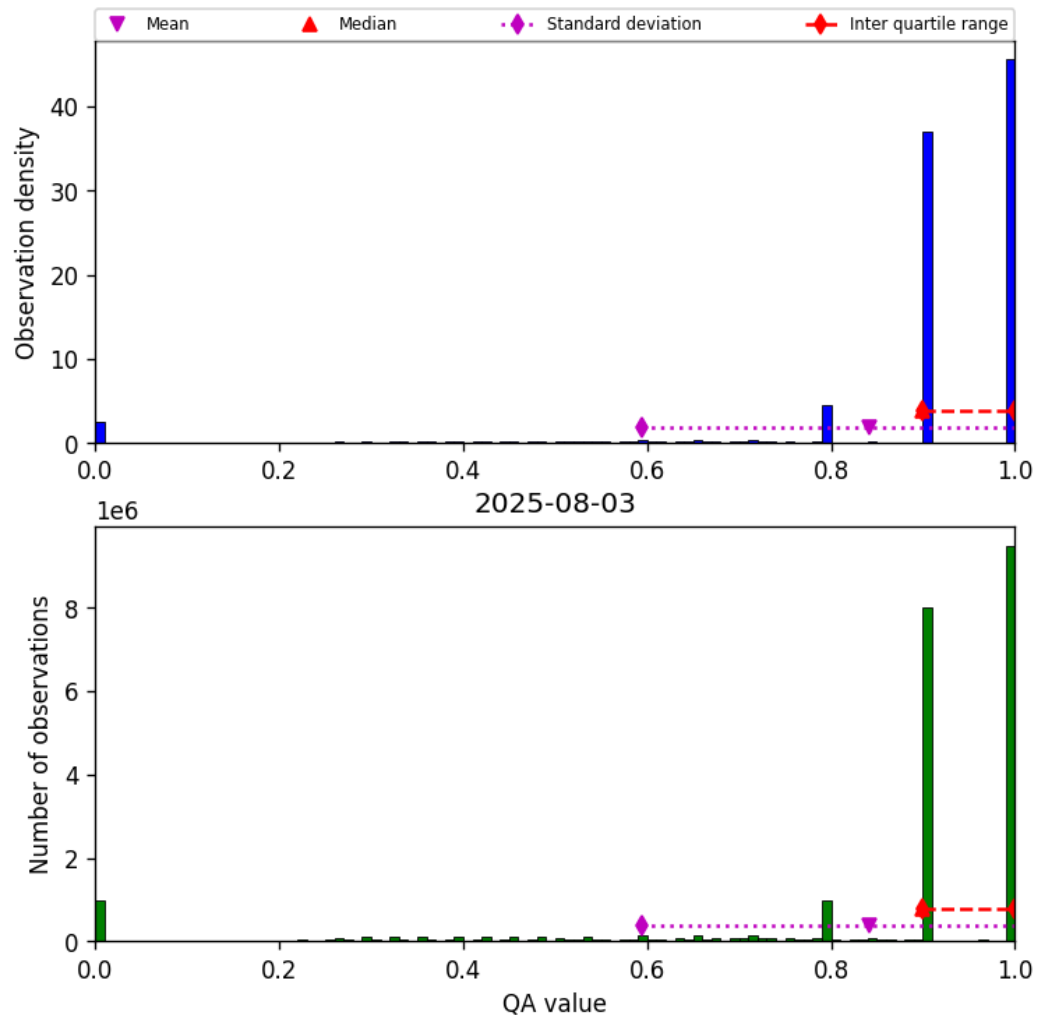
Figure 28: Histogram of “QA value” for 2025-08-03 to 2025-08-04
