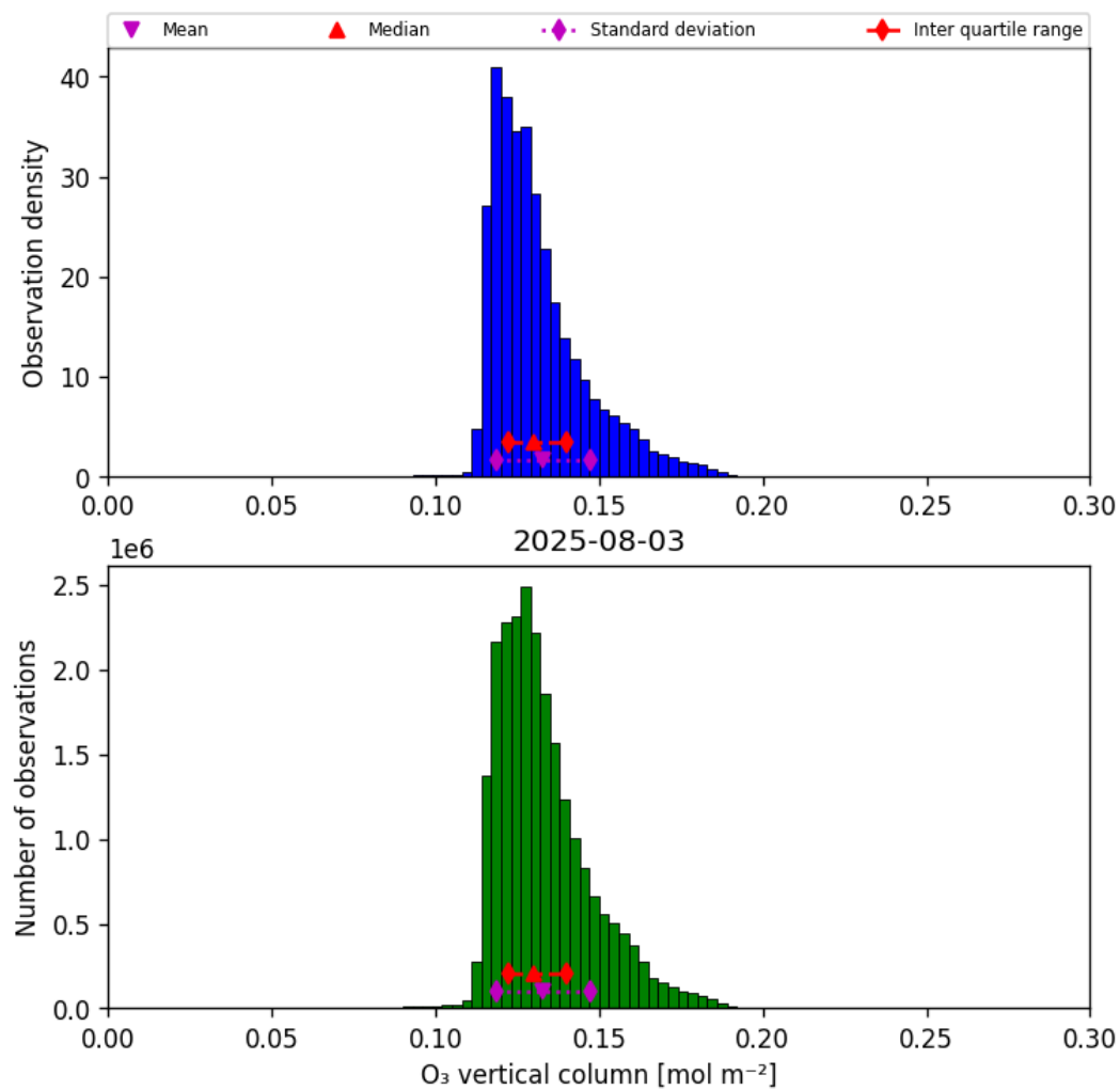
Figure 29: Histogram of “O 3 vertical column” for 2025-08-03 to 2025-08-04
