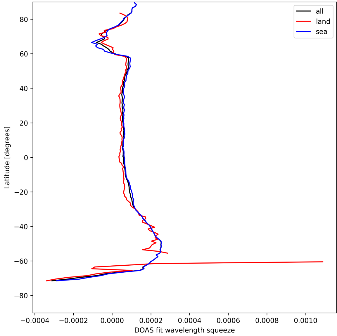
Figure 24: Zonal average of “DOAS fit wavelength squeeze” for 2025-08-03 to 2025-08-04.
