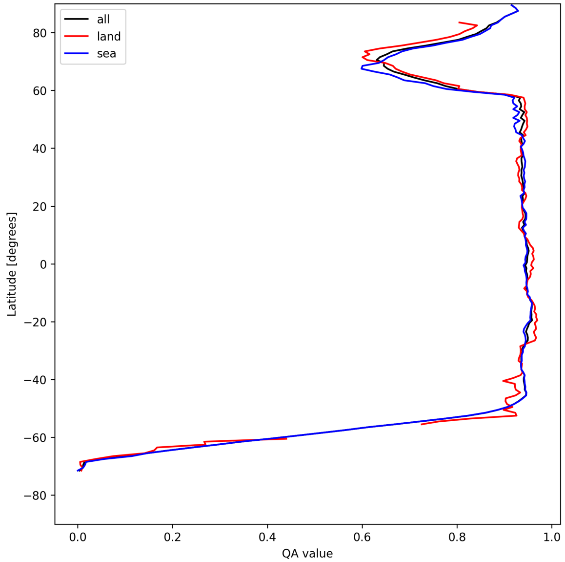
Figure 16: Zonal average of “QA value” for 2025-08-03 to 2025-08-04.
