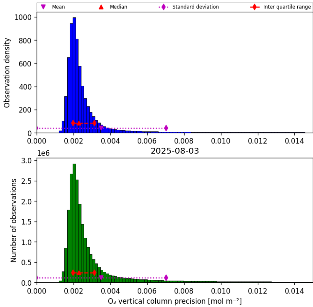
Figure 30: Histogram of “O 3 vertical column precision” for 2025-08-03 to 2025-08-04
