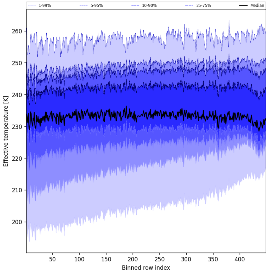
Figure 50: Along track statistics of “Effective temperature” for 2025-08-03 to 2025-08-04
