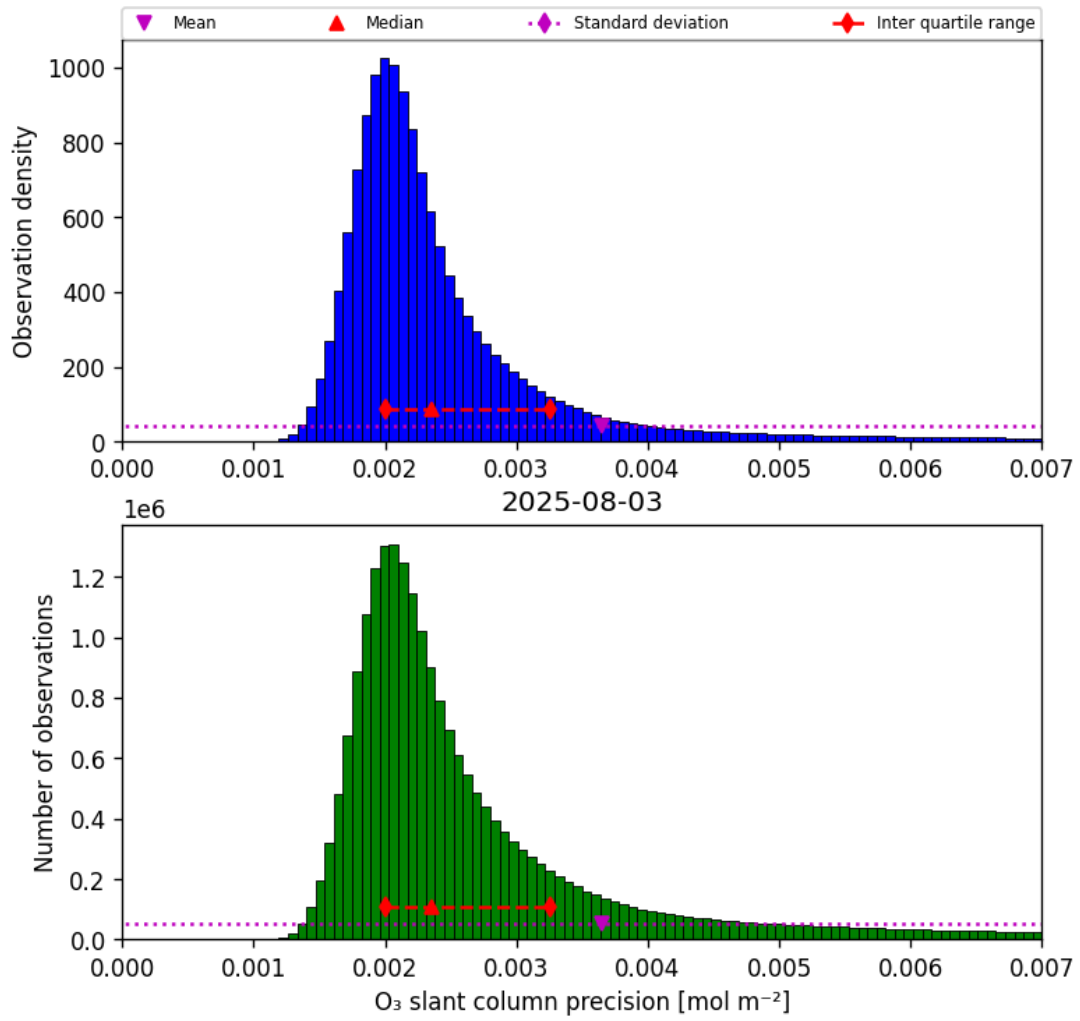
Figure 32: Histogram of “O 3 slant column precision” for 2025-08-03 to 2025-08-04
