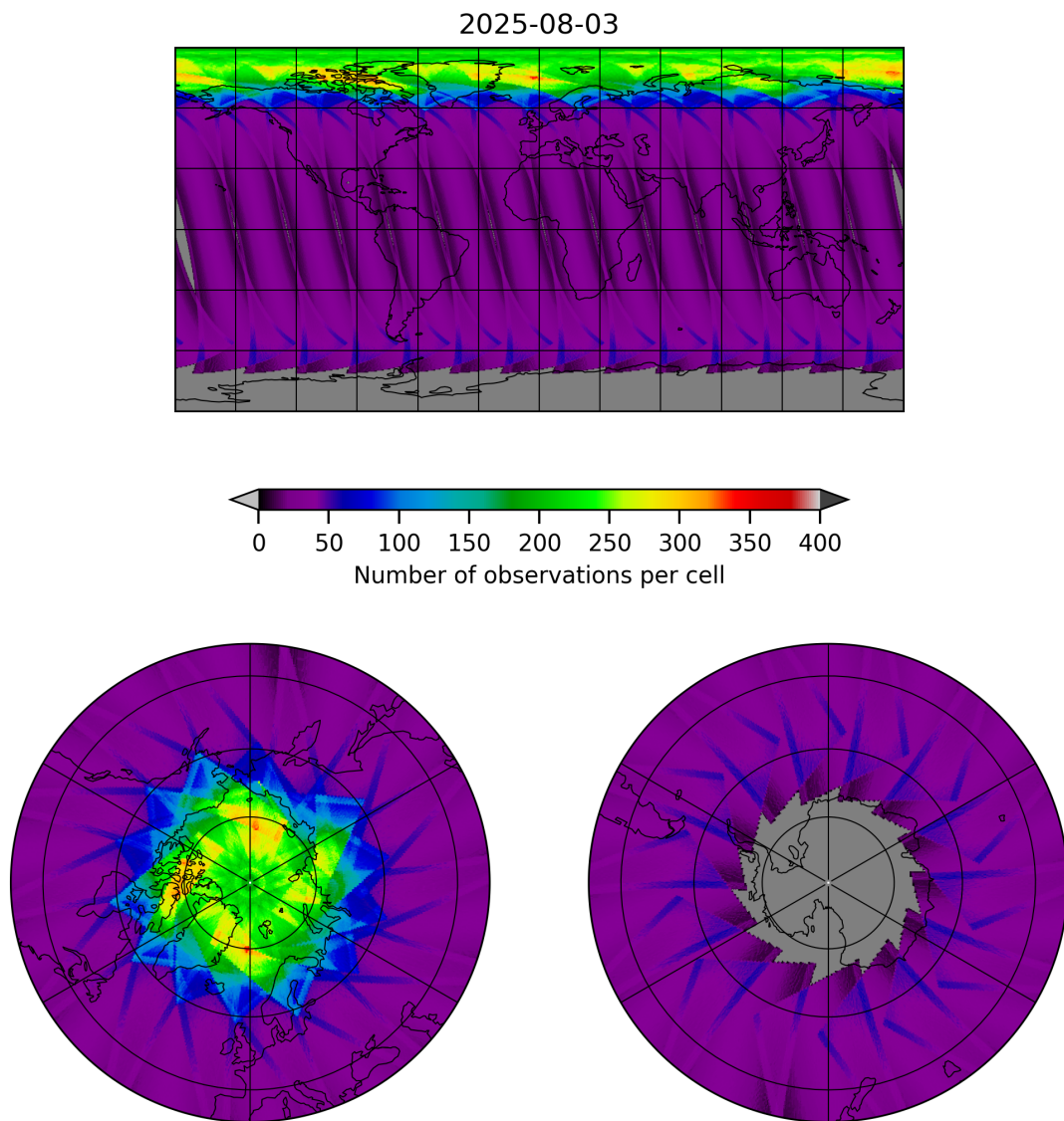
Figure 15: Map of the number of observations for 2025-08-03 to 2025-08-04
