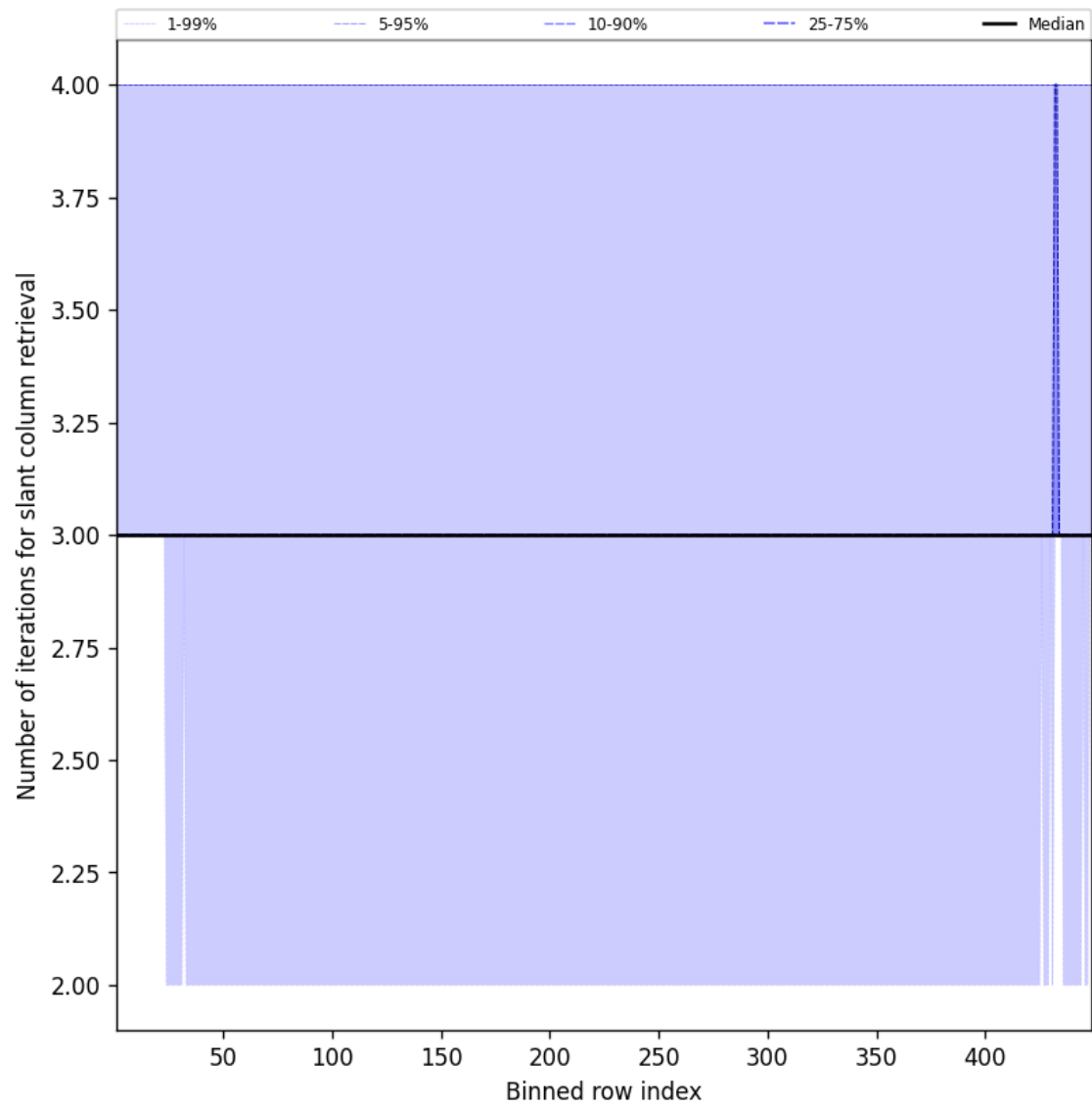
Figure 45: Along track statistics of “Number of iterations for slant column retrieval” for 2025-08-03 to 2025-08-04
