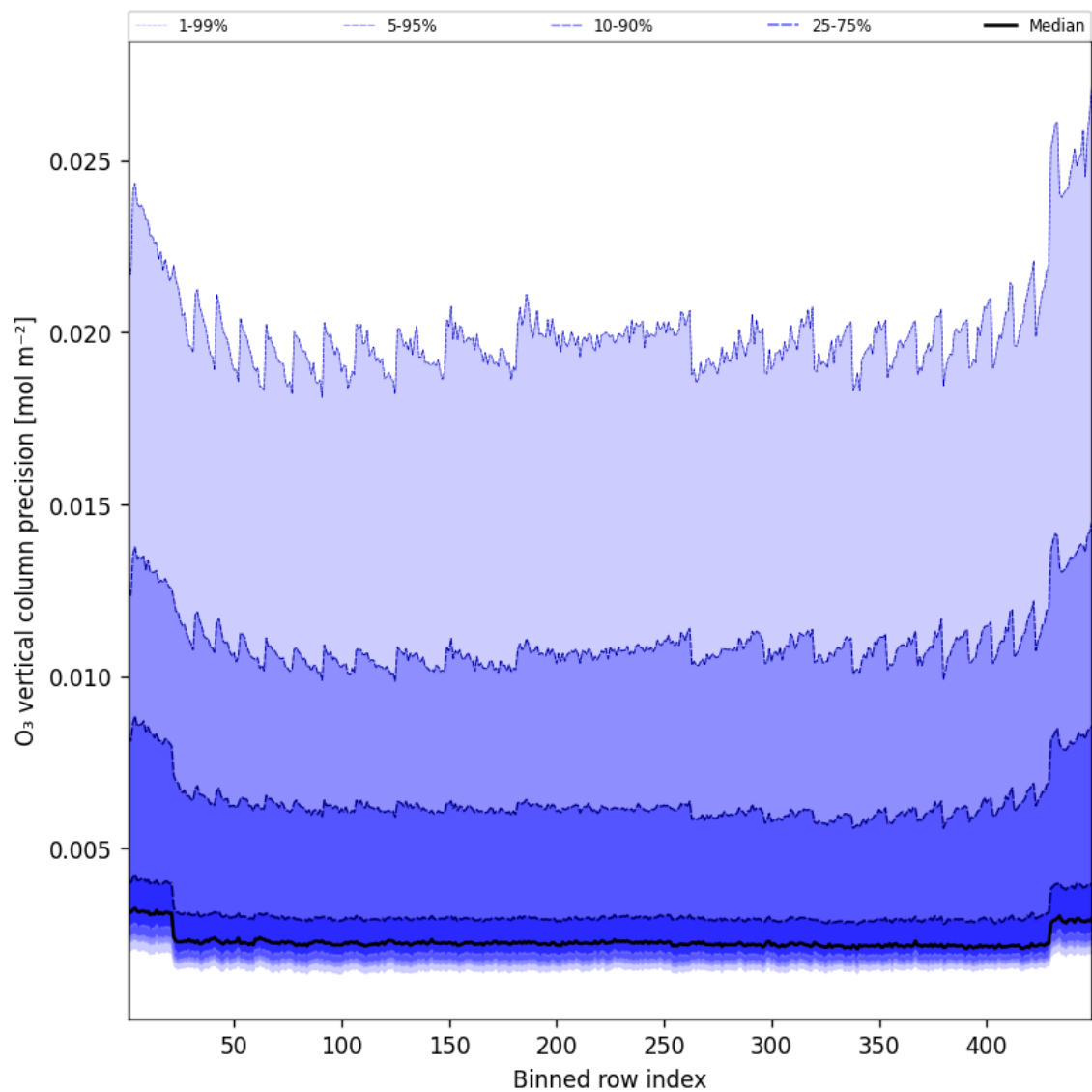
Figure 42: Along track statistics of “O 3 vertical column precision” for 2025-08-03 to 2025-08-04
