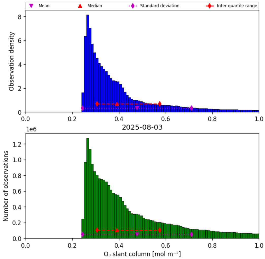
Figure 31: Histogram of “O 3 slant column” for 2025-08-03 to 2025-08-04
