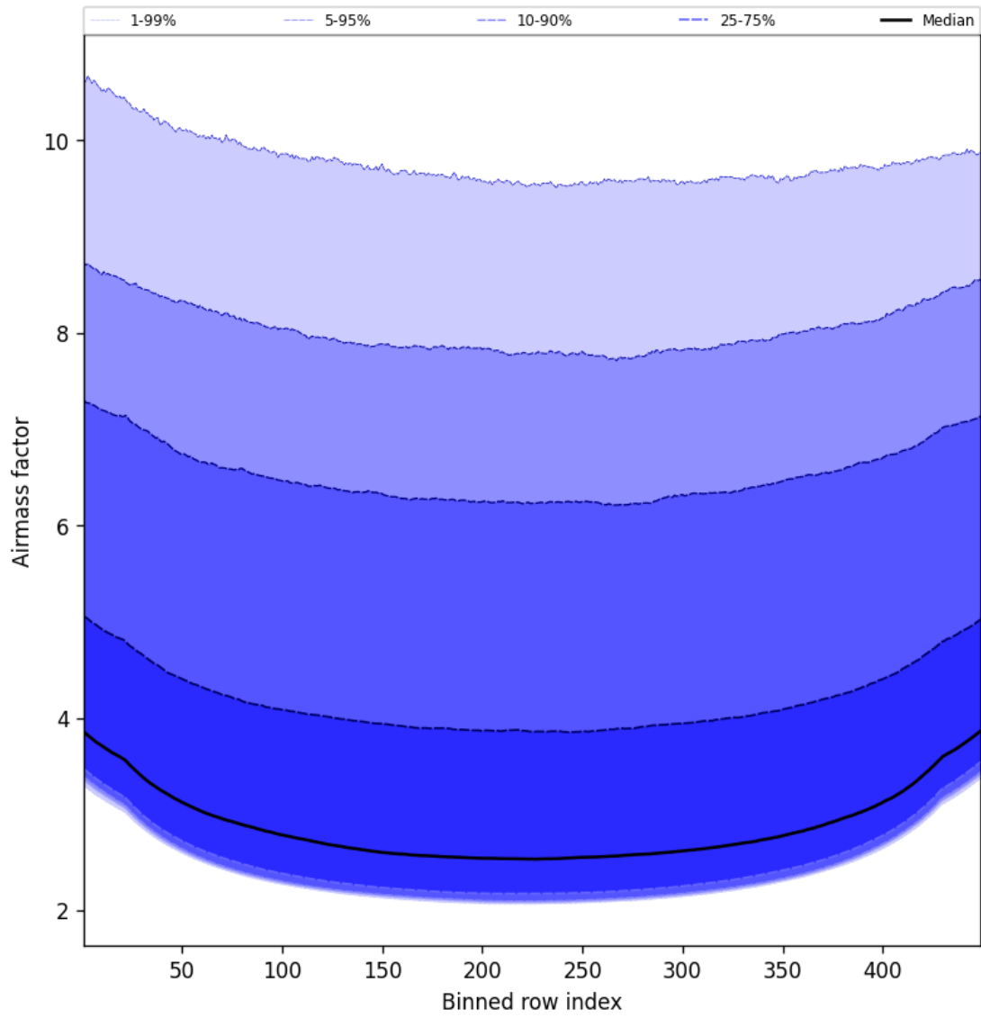
Figure 49: Along track statistics of “Airmass factor” for 2025-08-03 to 2025-08-04
