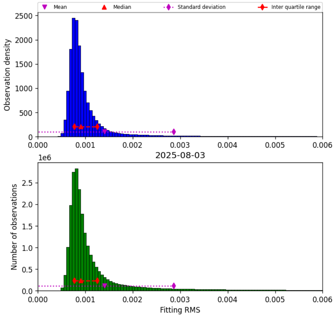
Figure 34: Histogram of “Fitting RMS” for 2025-08-03 to 2025-08-04
