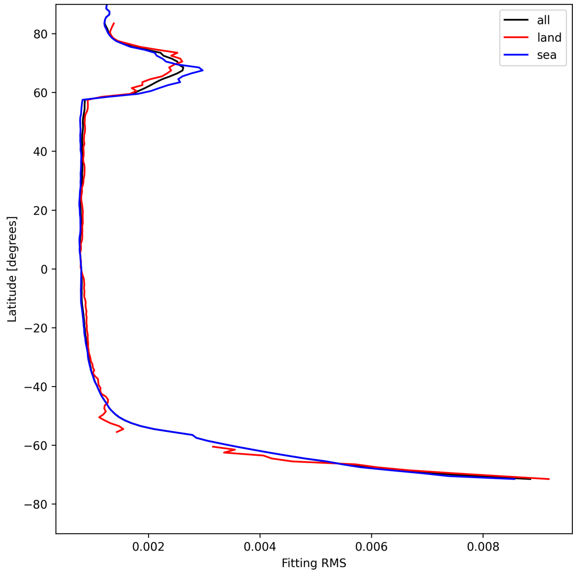
Figure 22: Zonal average of “Fitting RMS” for 2025-08-03 to 2025-08-04.
