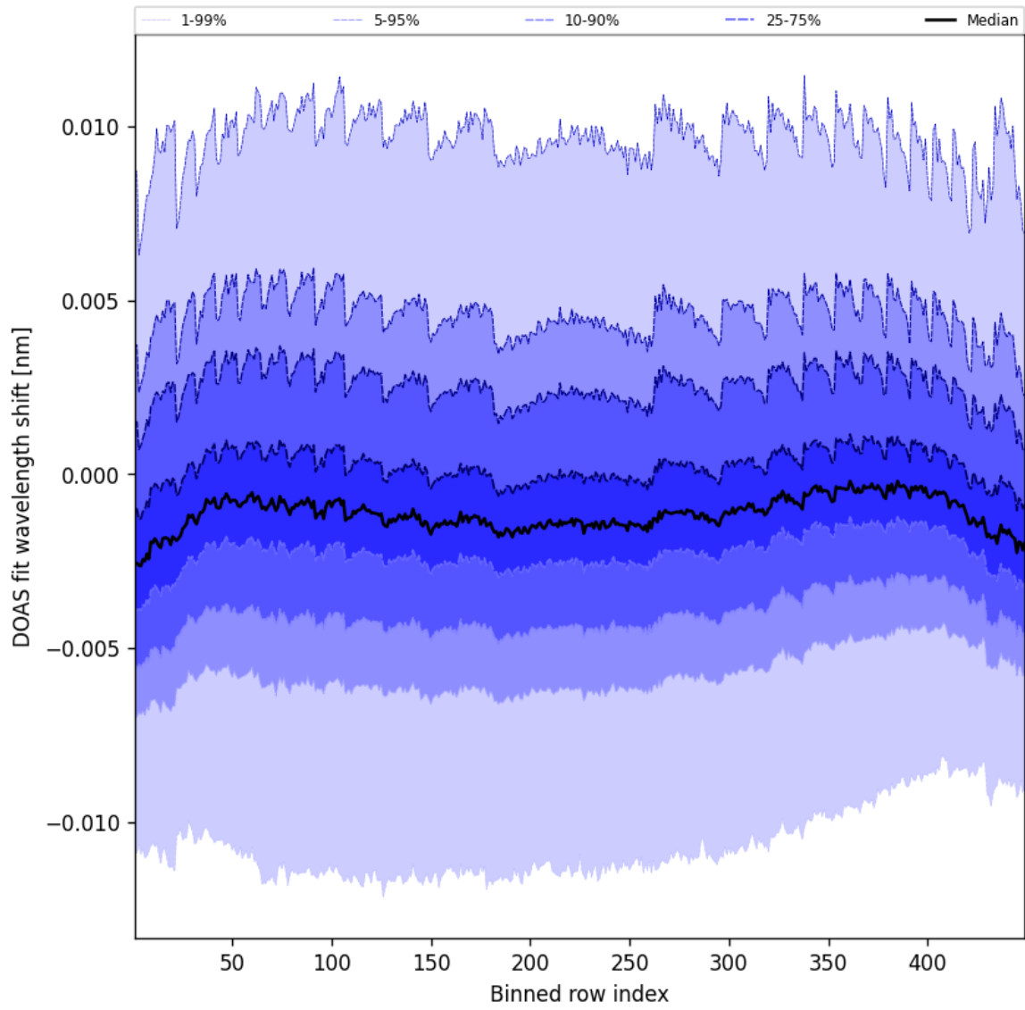
Figure 47: Along track statistics of “DOAS fit wavelength shift” for 2025-08-03 to 2025-08-04
