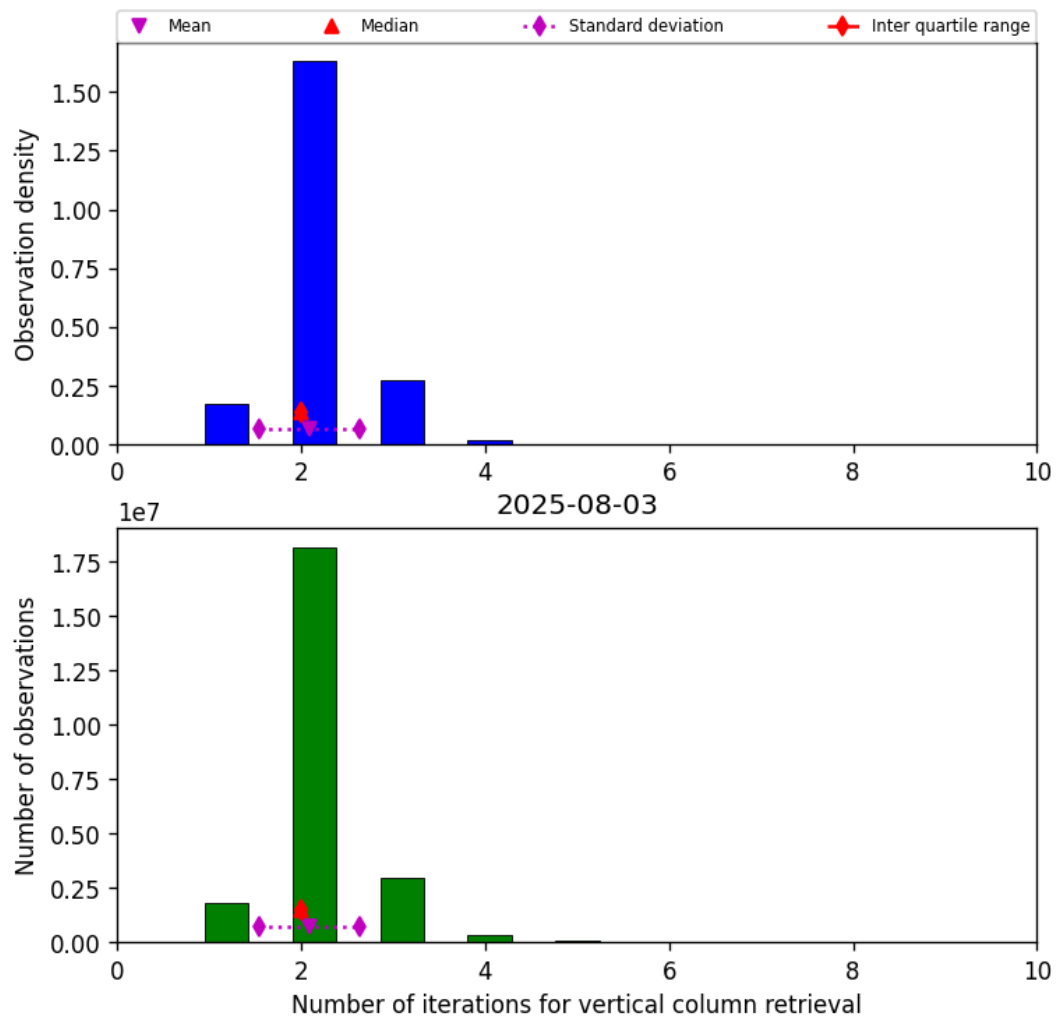
Figure 39: Histogram of “Number of iterations for vertical column retrieval” for 2025-08-03 to 2025-08-04
