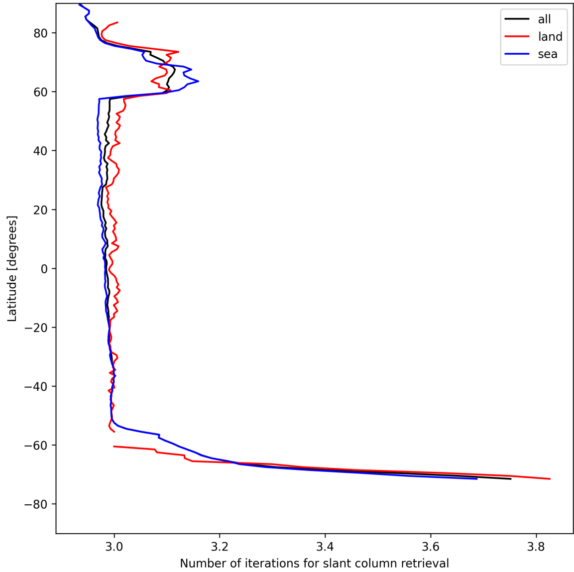
Figure 21: Zonal average of “Number of iterations for slant column retrieval” for 2025-08-03 to 2025-08-04.
