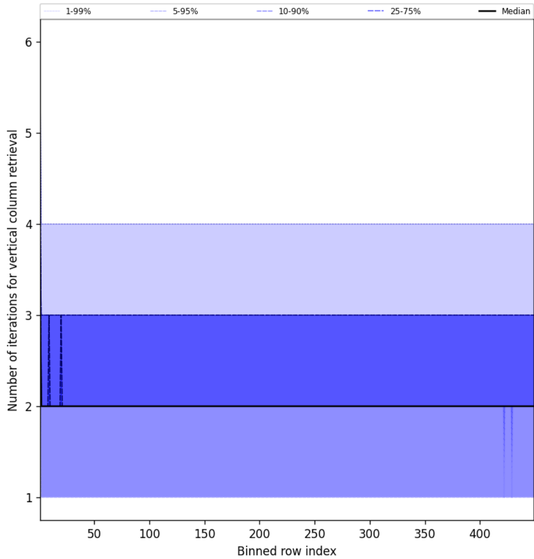
Figure 51: Along track statistics of “Number of iterations for vertical column retrieval” for 2025-08-03 to 2025-08-04
