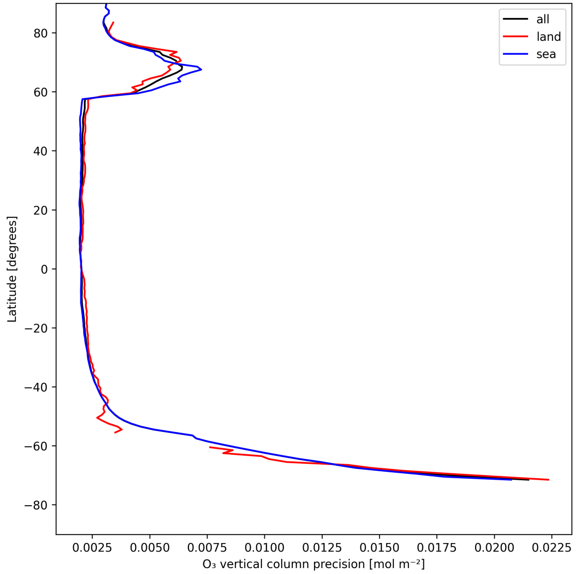
Figure 18: Zonal average of “O 3 vertical column precision” for 2025-08-03 to 2025-08-04.
