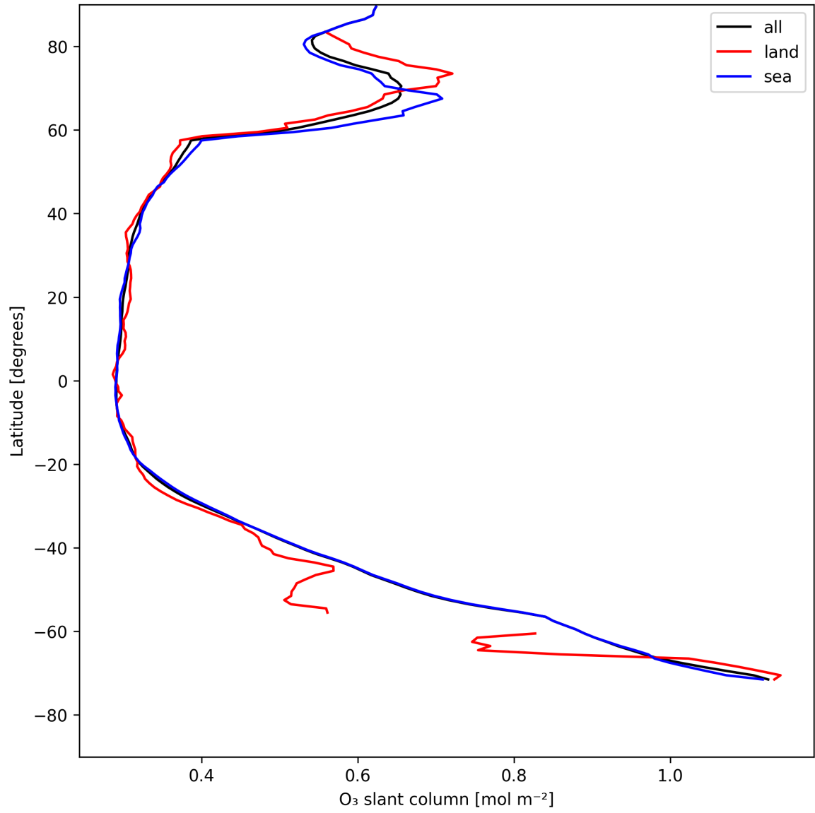
Figure 19: Zonal average of “O 3 slant column” for 2025-08-03 to 2025-08-04.
