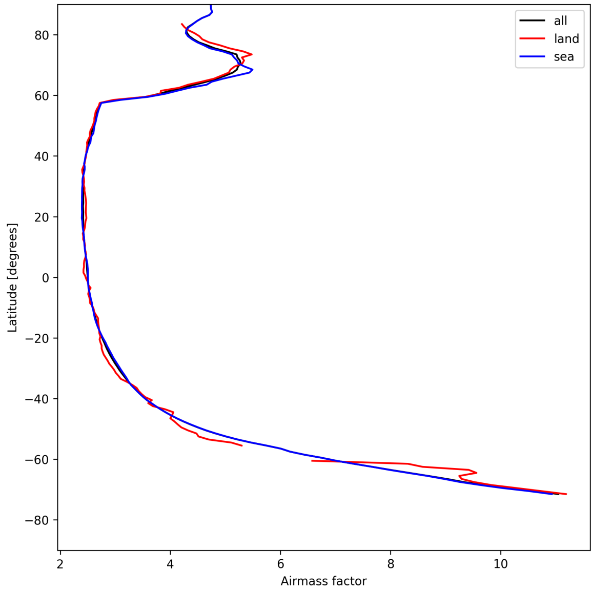
Figure 25: Zonal average of “Airmass factor” for 2025-08-03 to 2025-08-04.
