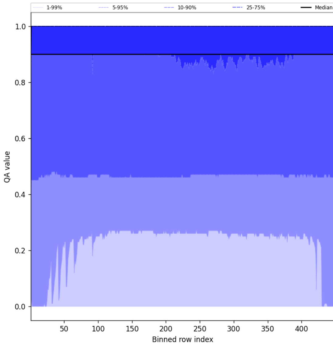
Figure 40: Along track statistics of “QA value” for 2025-08-03 to 2025-08-04
