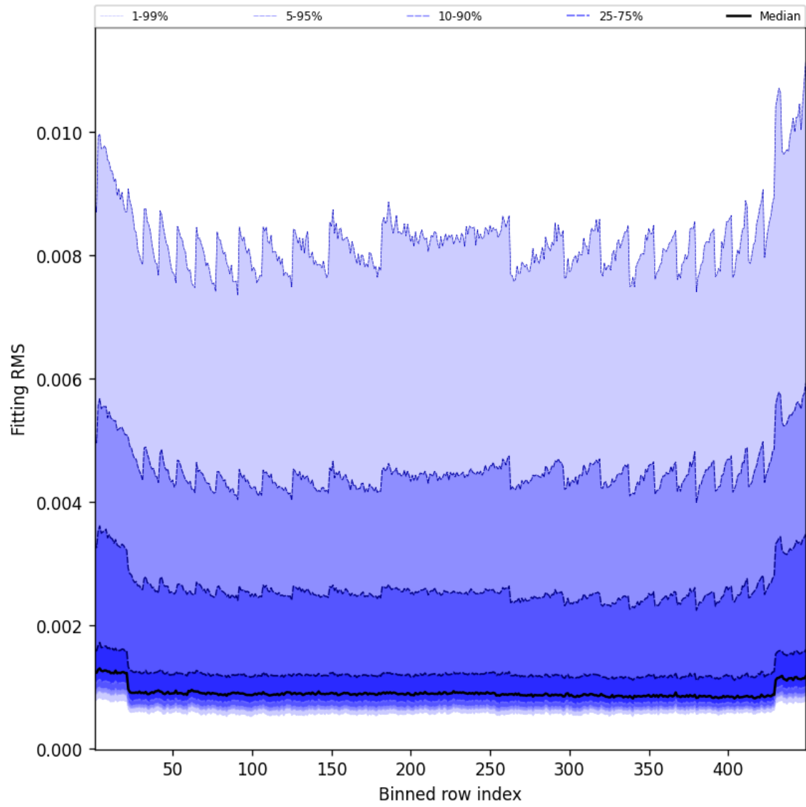
Figure 46: Along track statistics of “Fitting RMS” for 2025-08-03 to 2025-08-04
