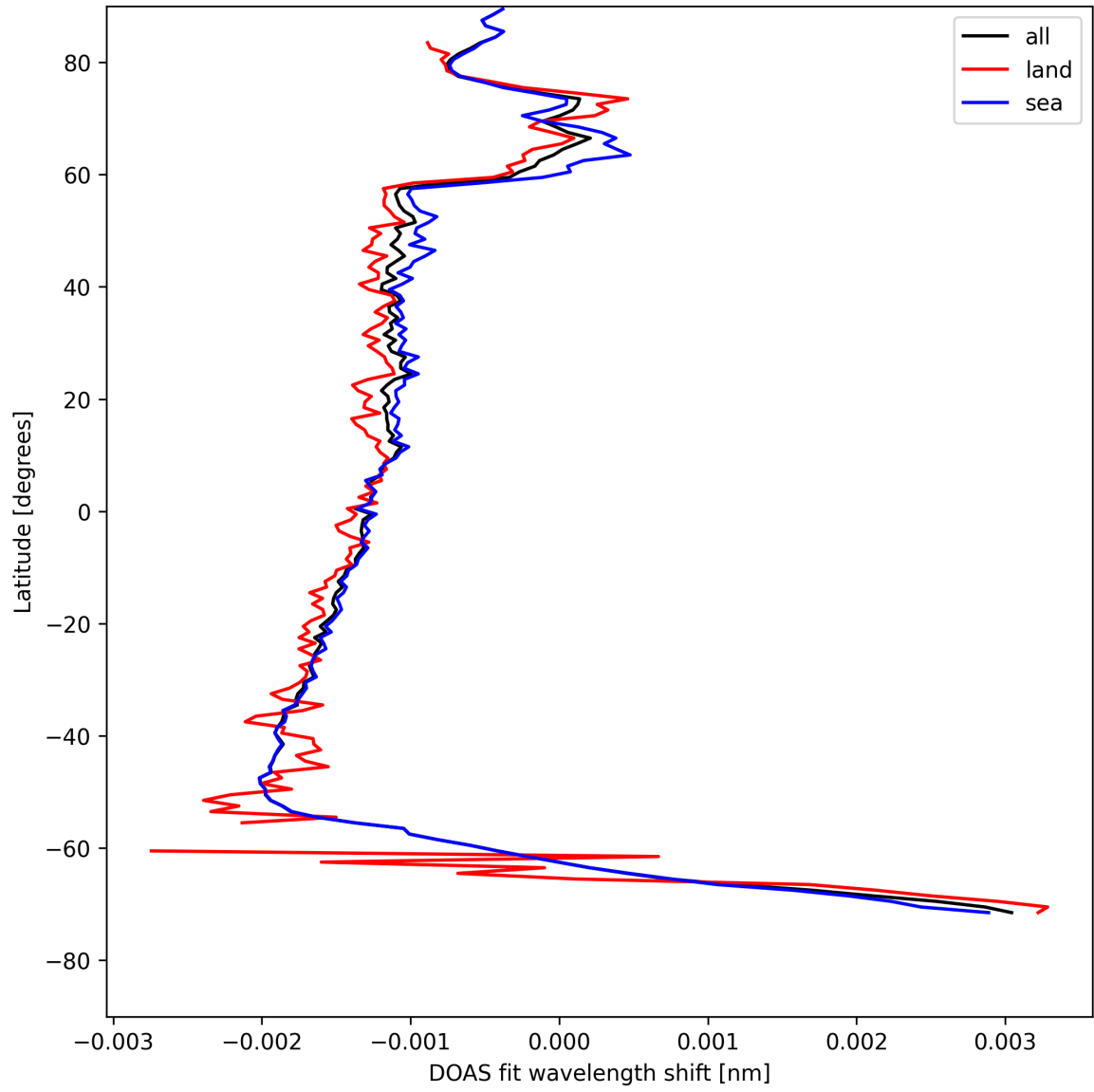
Figure 23: Zonal average of “DOAS fit wavelength shift” for 2025-08-03 to 2025-08-04.
