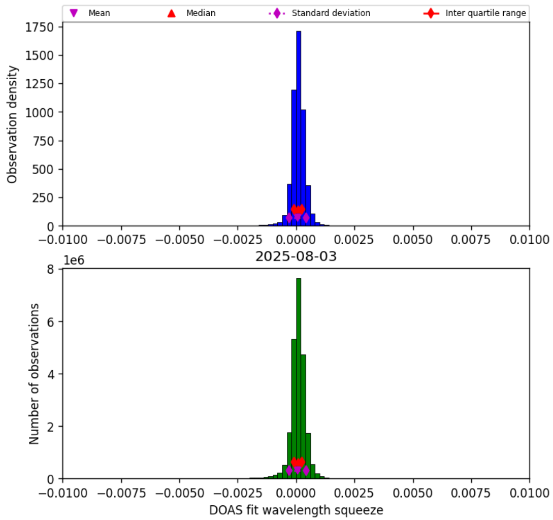
Figure 36: Histogram of “DOAS fit wavelength squeeze” for 2025-08-03 to 2025-08-04
