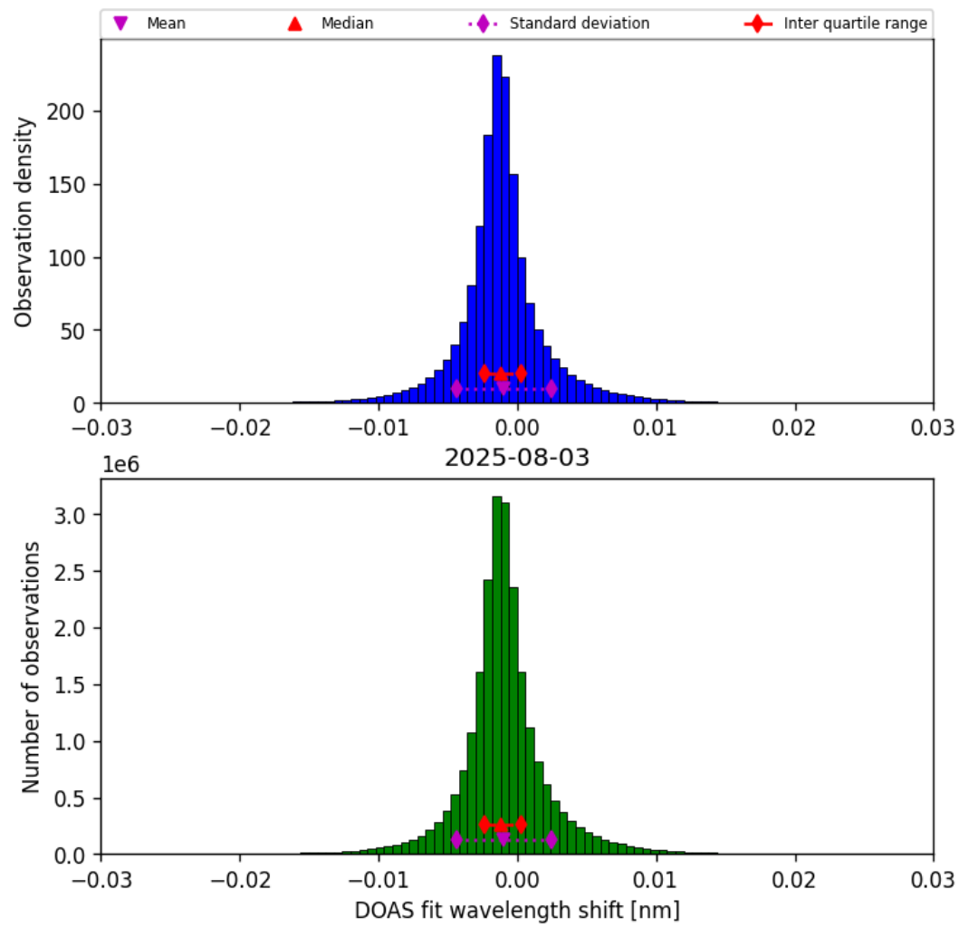
Figure 35: Histogram of “DOAS fit wavelength shift” for 2025-08-03 to 2025-08-04
