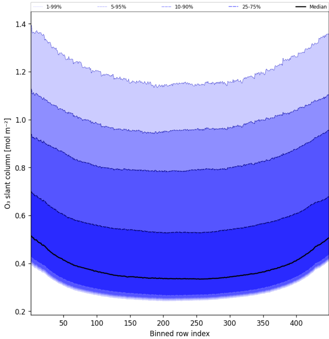
Figure 43: Along track statistics of “O 3 slant column” for 2025-08-03 to 2025-08-04
