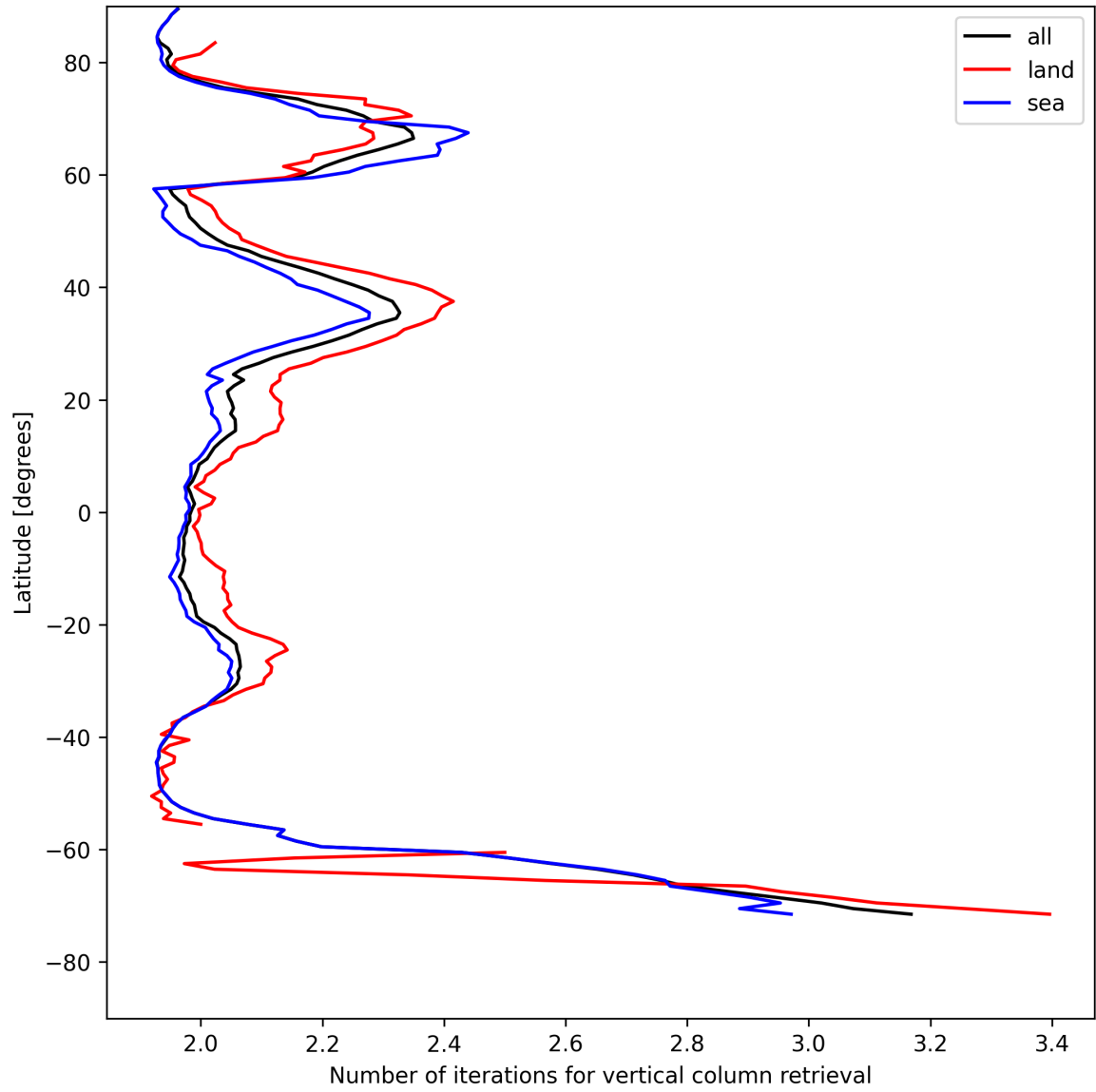
Figure 27: Zonal average of “Number of iterations for vertical column retrieval” for 2025-08-03 to 2025-08-04.
