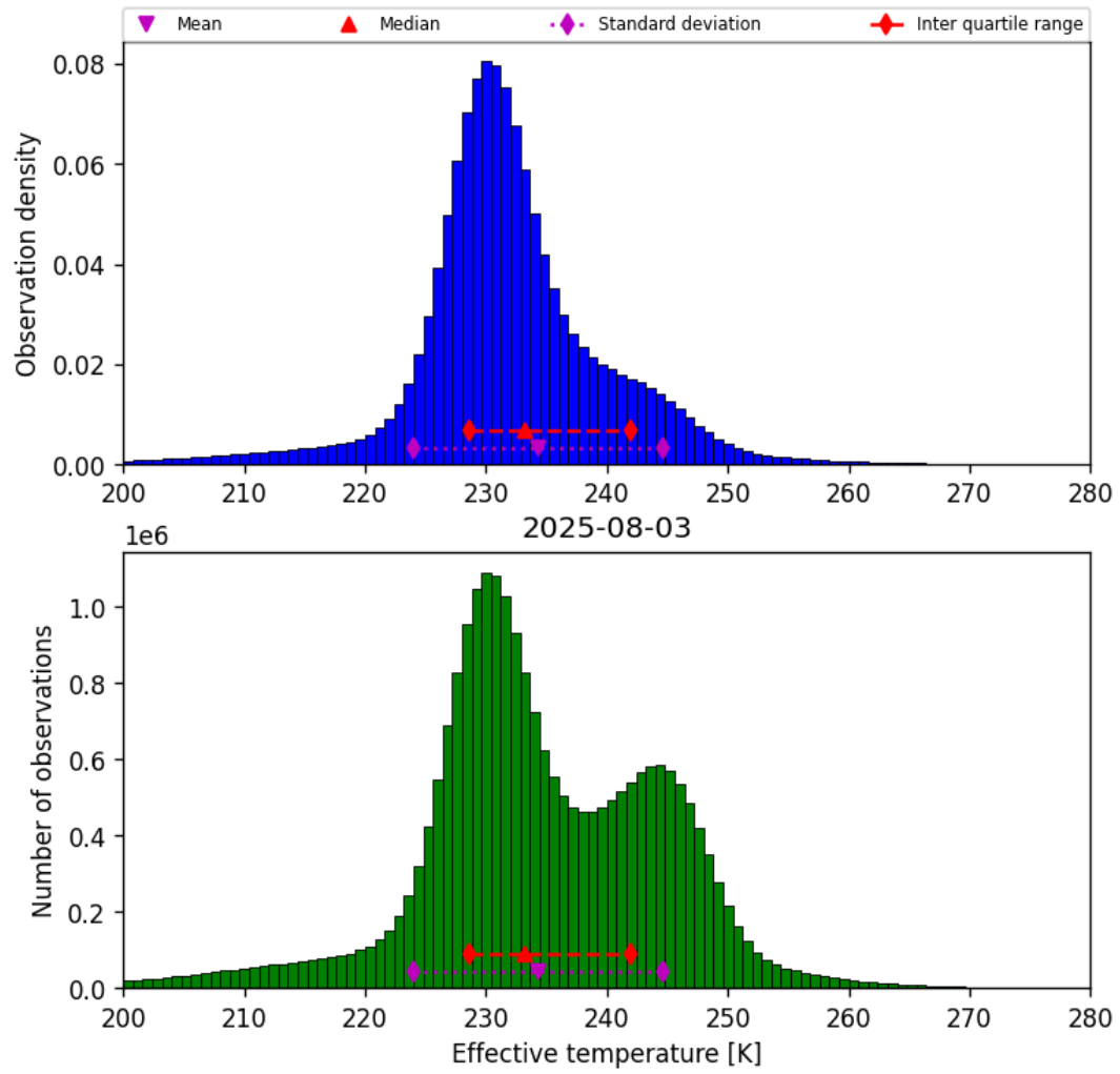
Figure 38: Histogram of “Effective temperature” for 2025-08-03 to 2025-08-04
