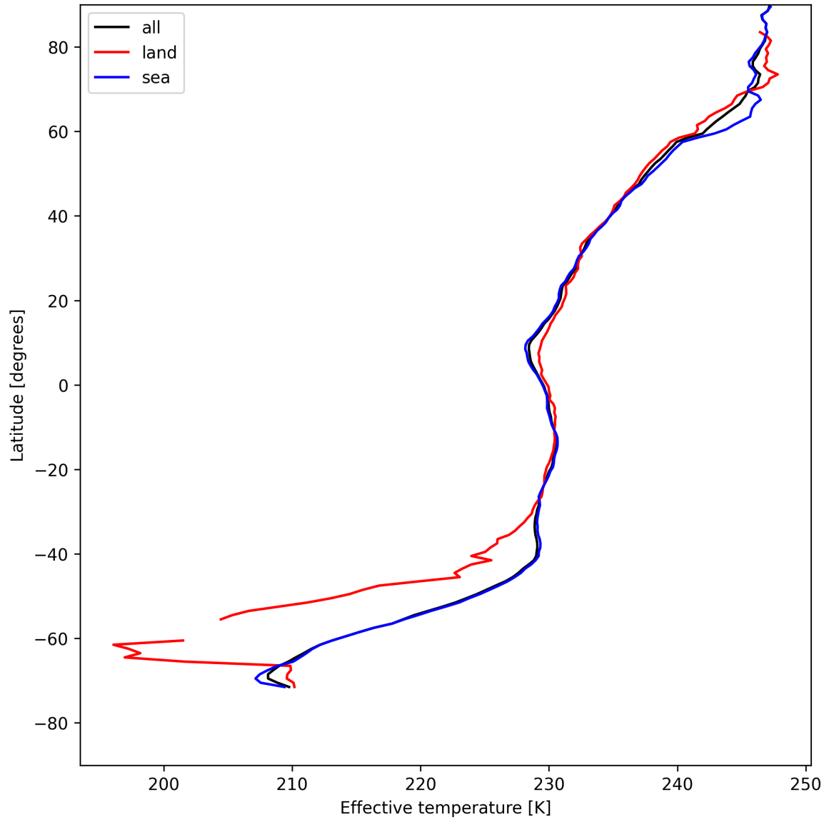
Figure 26: Zonal average of “Effective temperature” for 2025-08-03 to 2025-08-04.
