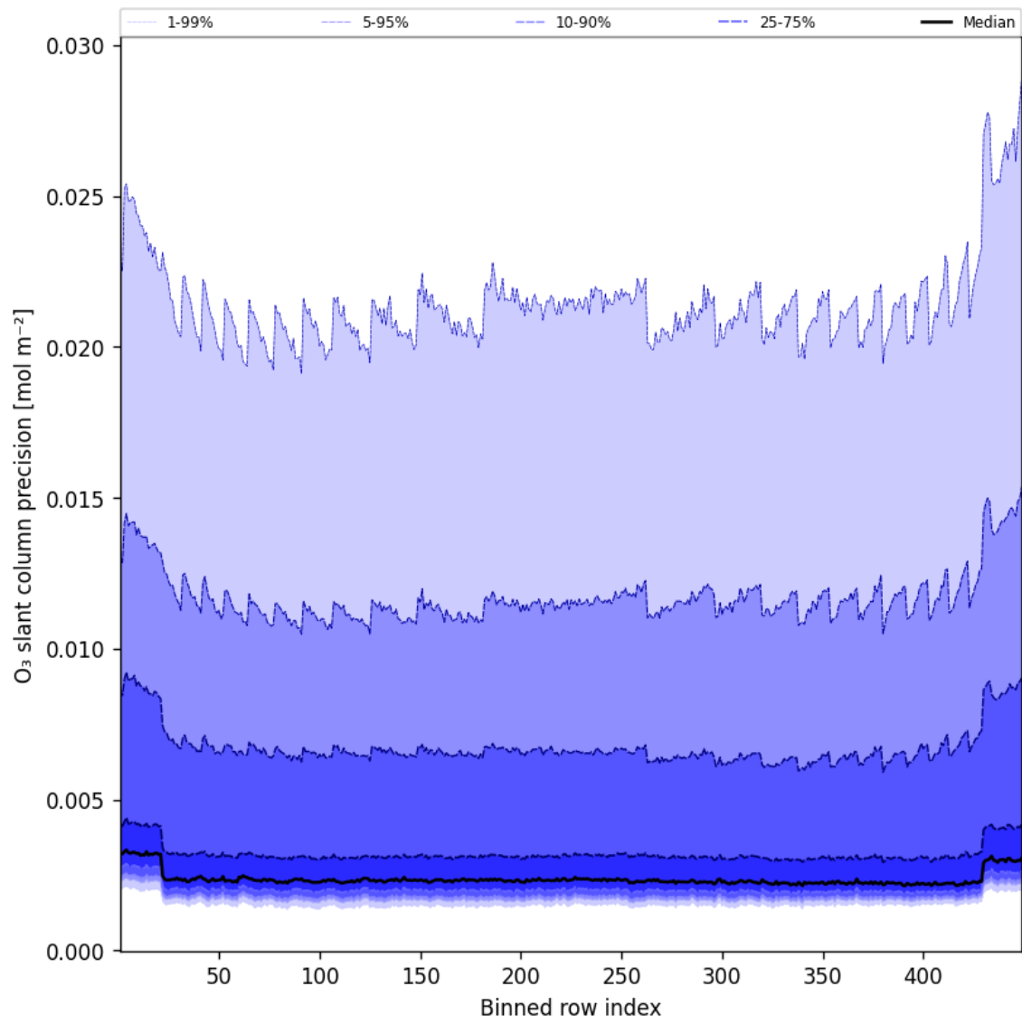
Figure 44: Along track statistics of “O 3 slant column precision” for 2025-08-03 to 2025-08-04
