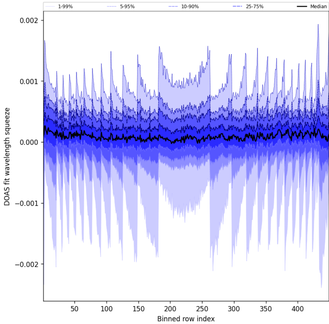
Figure 48: Along track statistics of “DOAS fit wavelength squeeze” for 2025-08-03 to 2025-08-04
