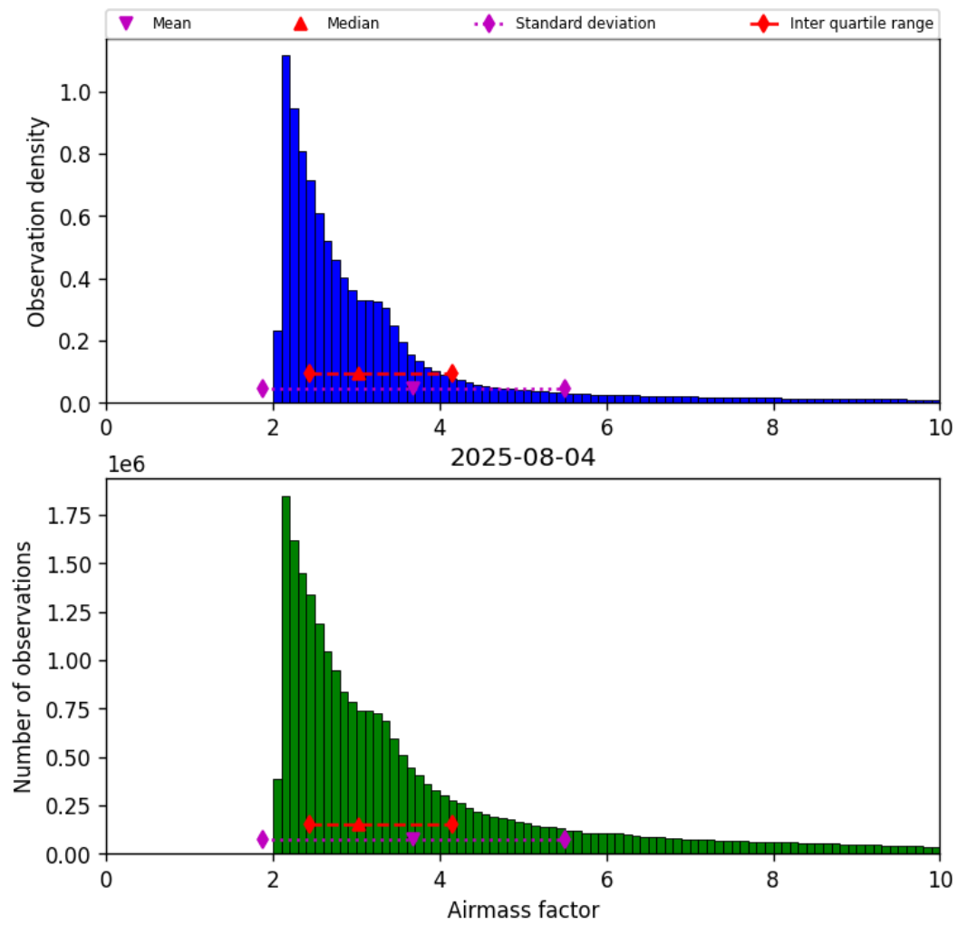
Figure 37: Histogram of “Airmass factor” for 2025-08-04 to 2025-08-05
