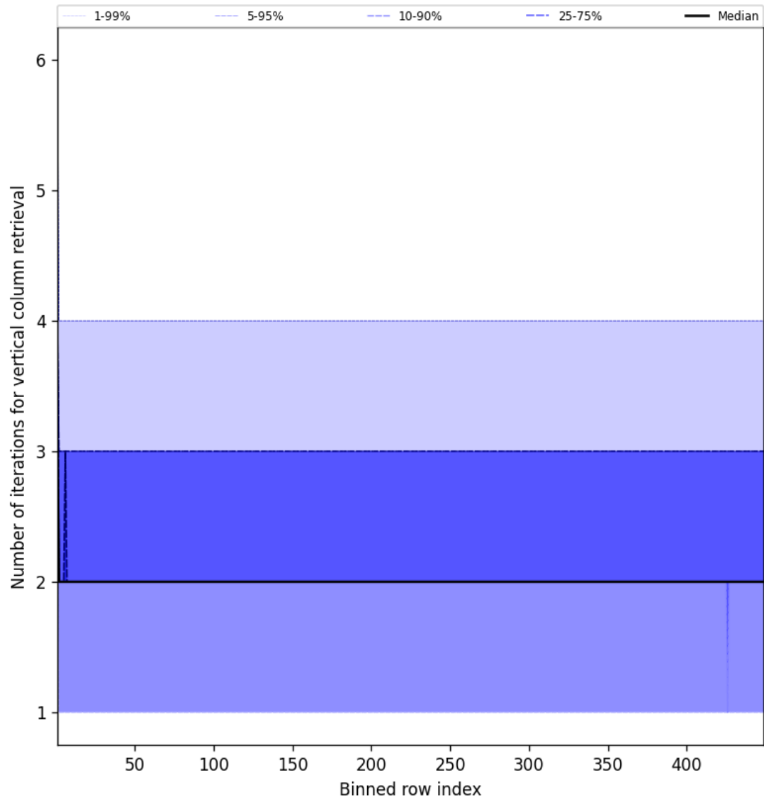
Figure 51: Along track statistics of “Number of iterations for vertical column retrieval” for 2025-08-04 to 2025-08-05
