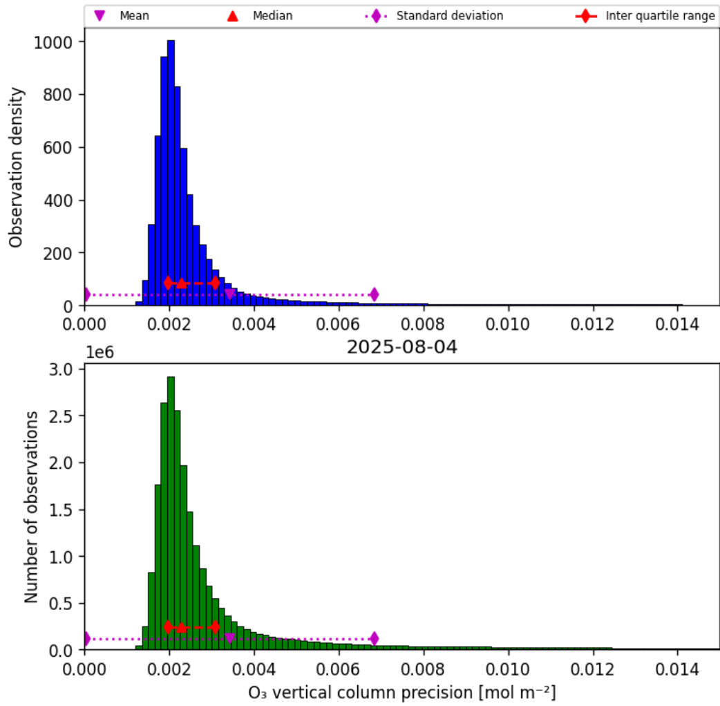
Figure 30: Histogram of “O 3 vertical column precision” for 2025-08-04 to 2025-08-05
