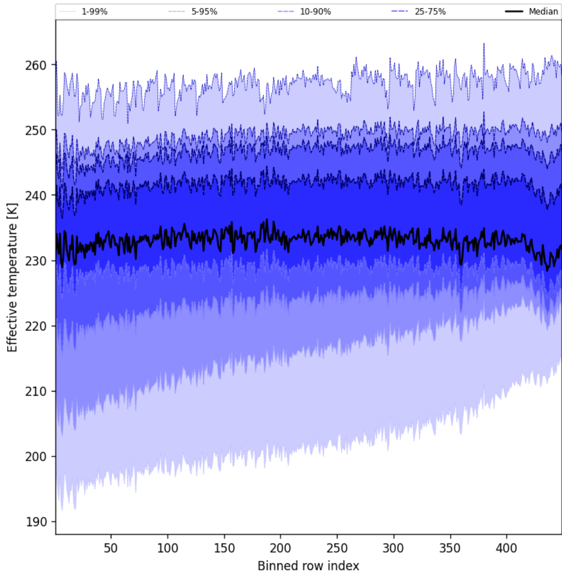
Figure 50: Along track statistics of “Effective temperature” for 2025-08-04 to 2025-08-05
