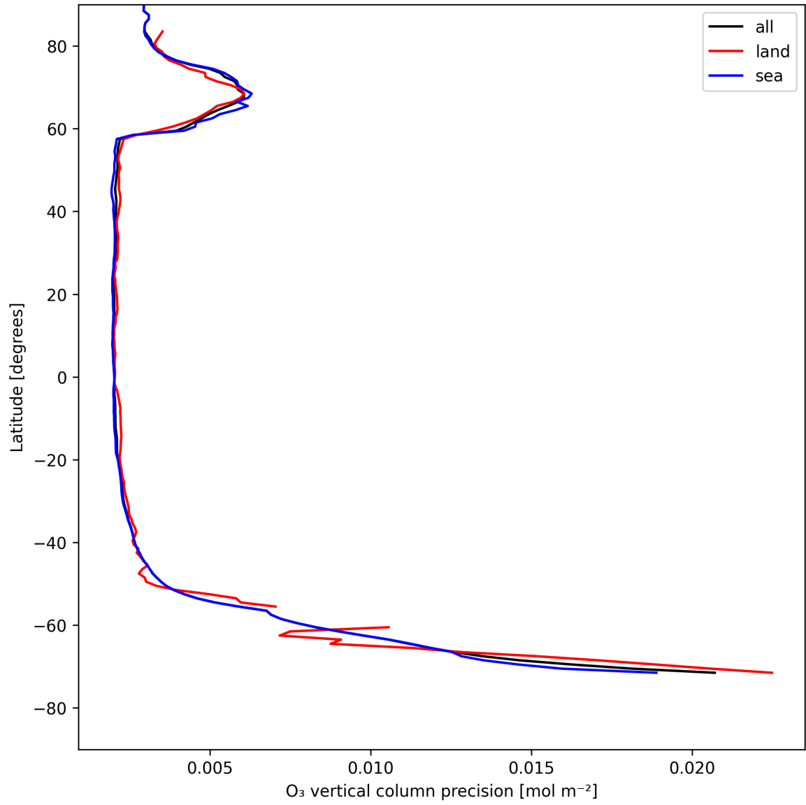
Figure 18: Zonal average of “O 3 vertical column precision” for 2025-08-04 to 2025-08-05.
