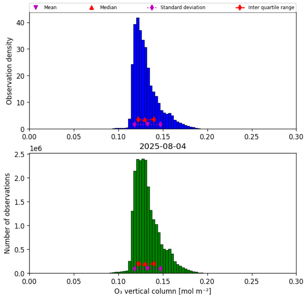
Figure 29: Histogram of “O 3 vertical column” for 2025-08-04 to 2025-08-05
