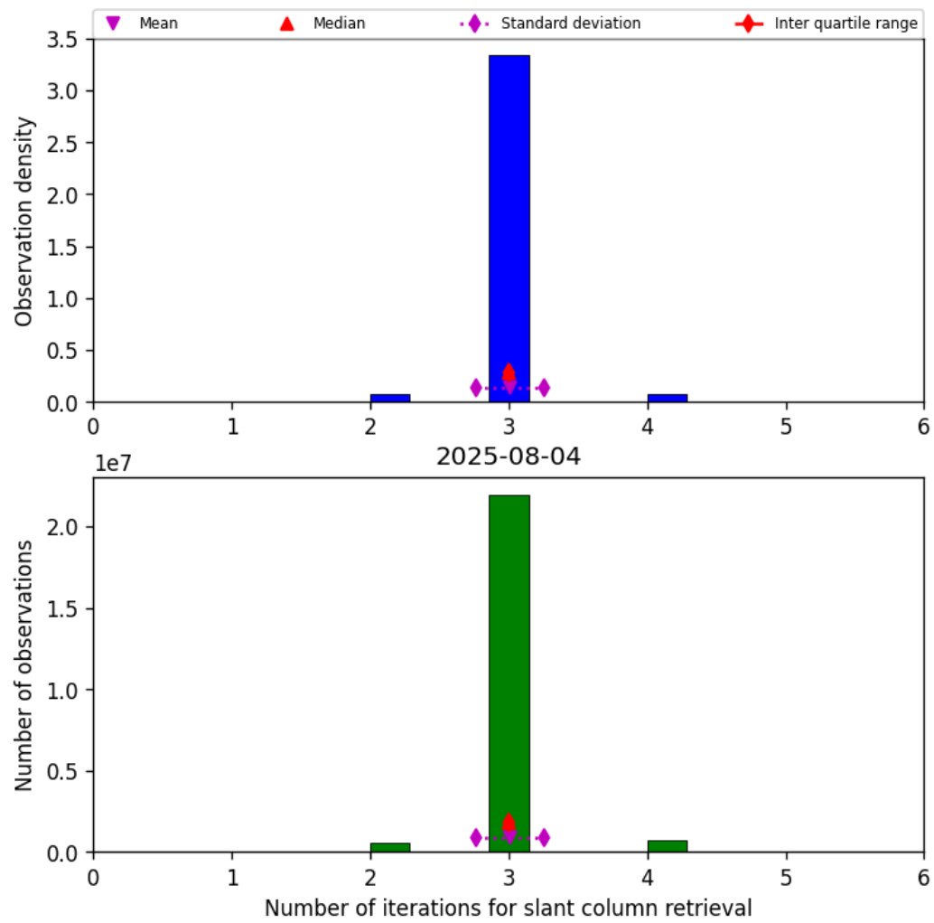
Figure 33: Histogram of “Number of iterations for slant column retrieval” for 2025-08-04 to 2025-08-05
