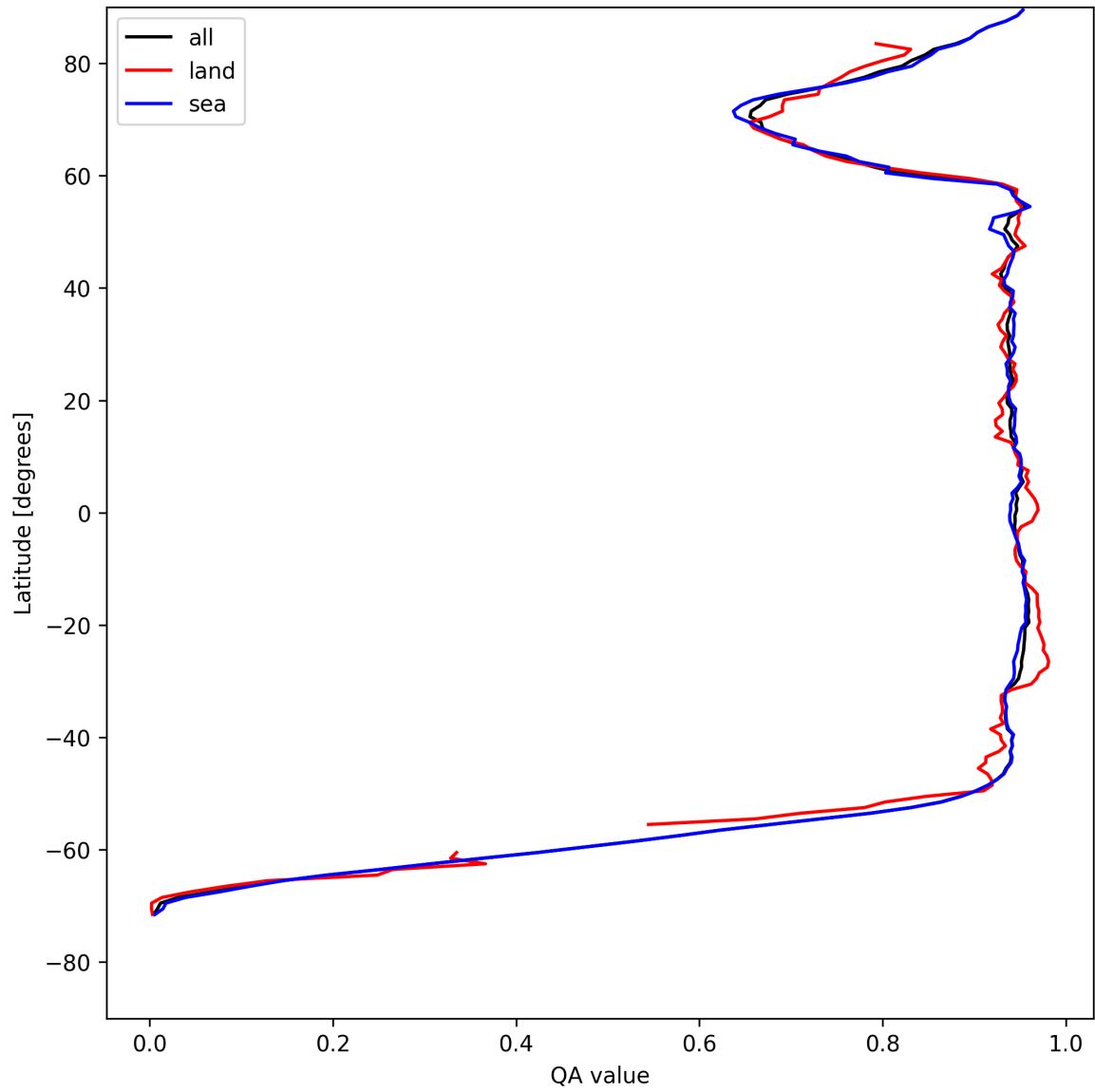
Figure 16: Zonal average of “QA value” for 2025-08-04 to 2025-08-05.
