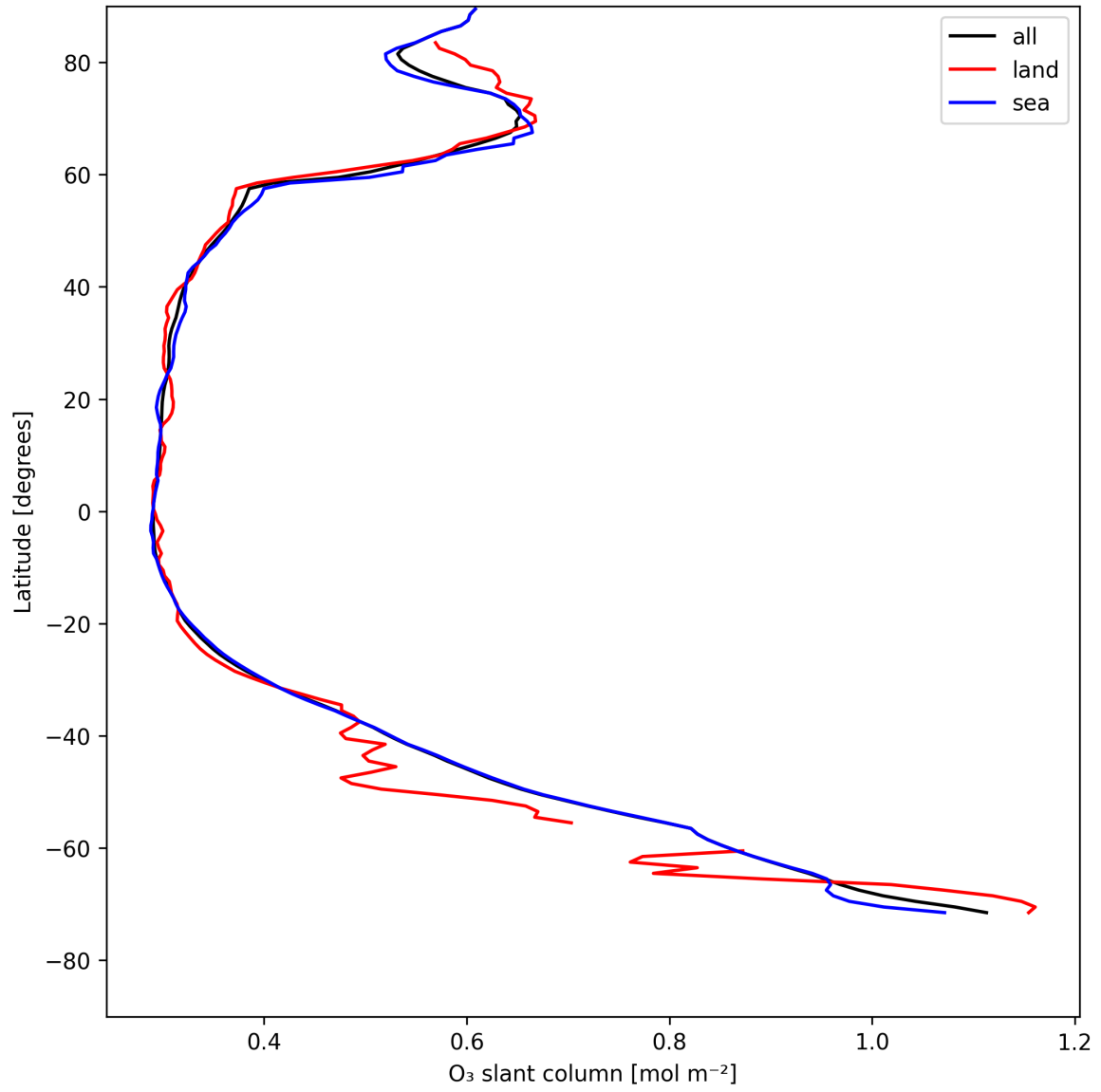
Figure 19: Zonal average of “O 3 slant column” for 2025-08-04 to 2025-08-05.
