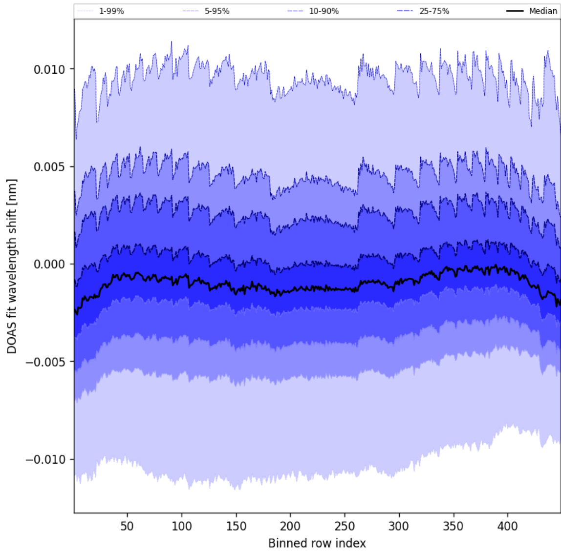
Figure 47: Along track statistics of “DOAS fit wavelength shift” for 2025-08-04 to 2025-08-05
