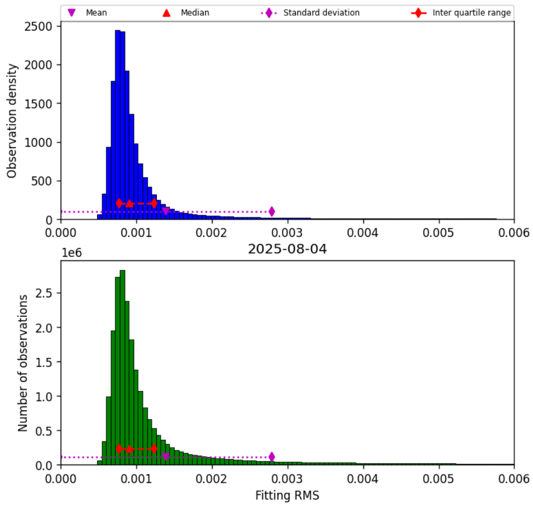
Figure 34: Histogram of “Fitting RMS” for 2025-08-04 to 2025-08-05
