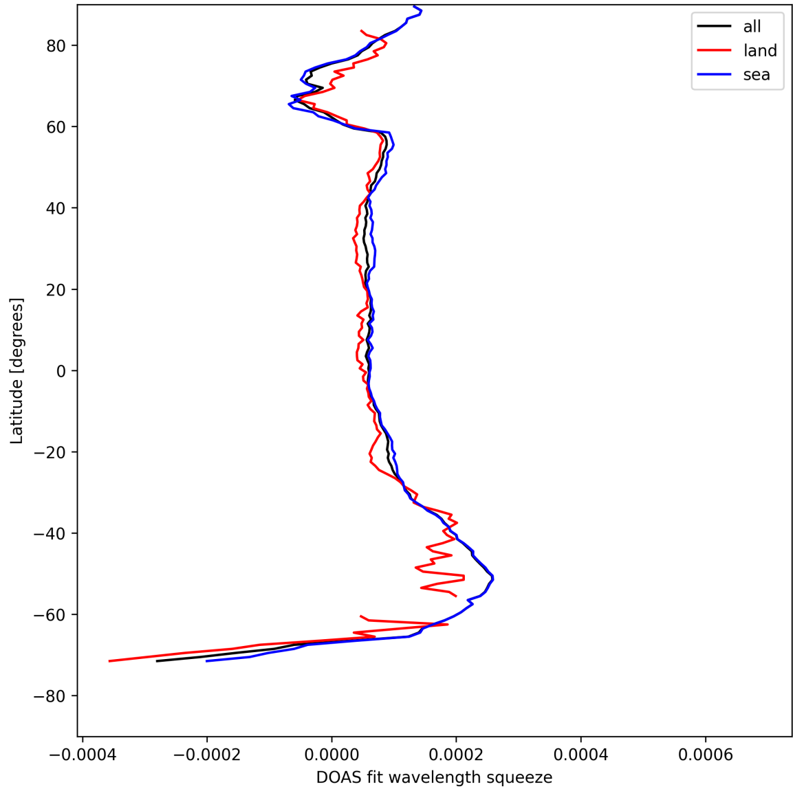
Figure 24: Zonal average of “DOAS fit wavelength squeeze” for 2025-08-04 to 2025-08-05.
