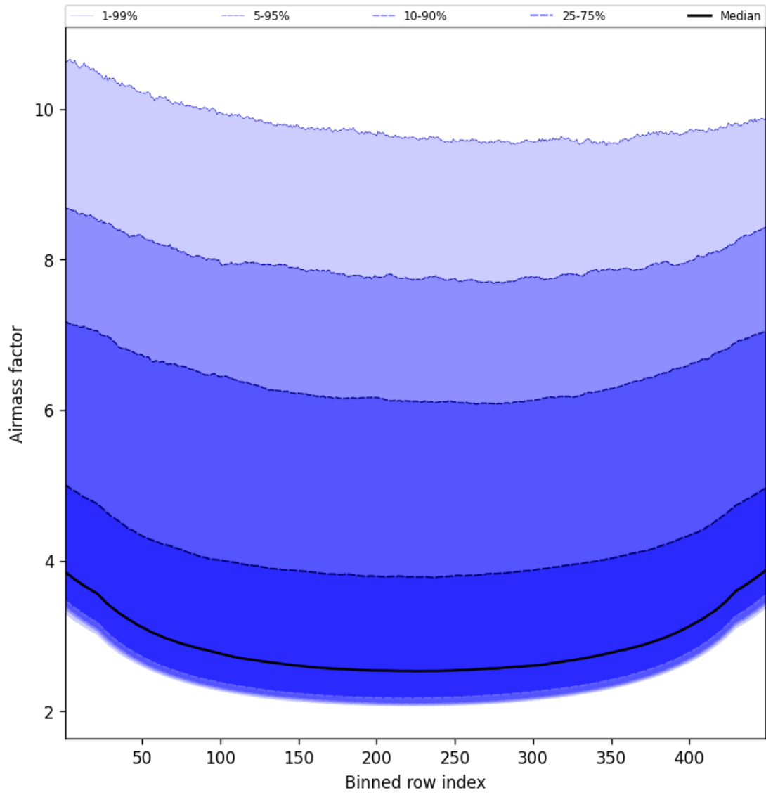
Figure 49: Along track statistics of “Airmass factor” for 2025-08-04 to 2025-08-05
