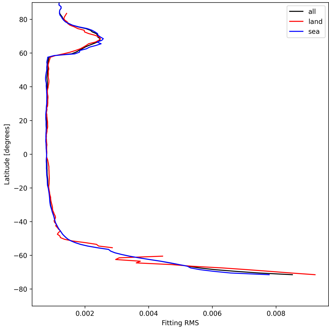
Figure 22: Zonal average of “Fitting RMS” for 2025-08-04 to 2025-08-05.
