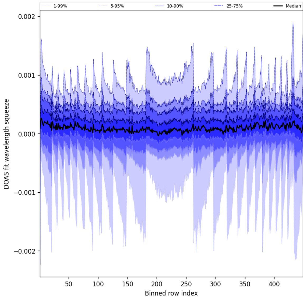
Figure 48: Along track statistics of “DOAS fit wavelength squeeze” for 2025-08-04 to 2025-08-05
