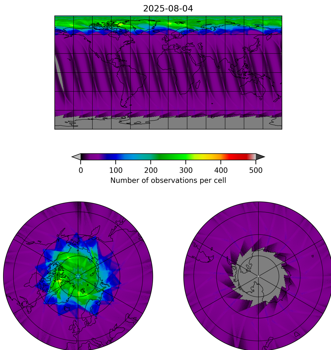
Figure 15: Map of the number of observations for 2025-08-04 to 2025-08-05
