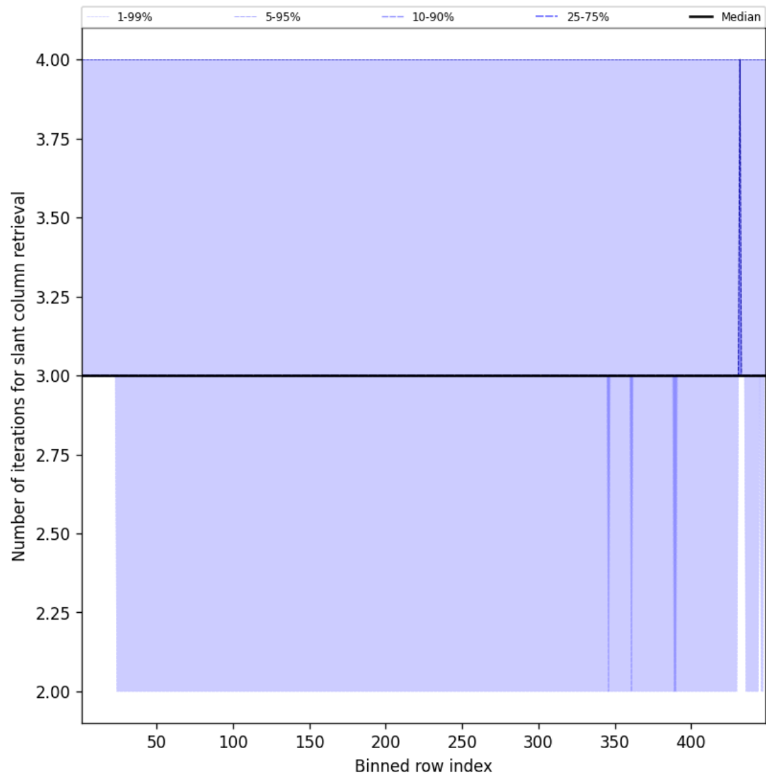
Figure 45: Along track statistics of “Number of iterations for slant column retrieval” for 2025-08-04 to 2025-08-05
