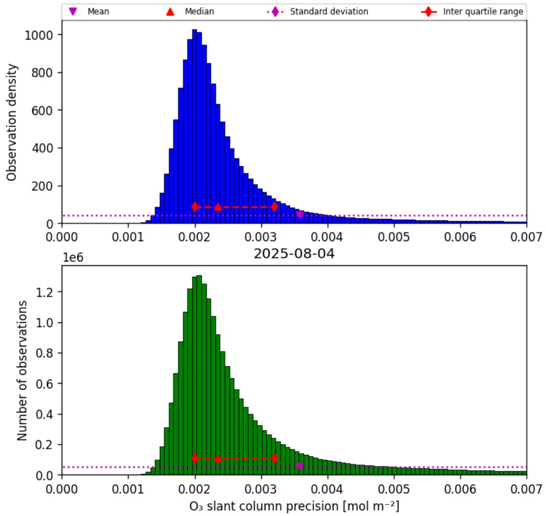
Figure 32: Histogram of “O 3 slant column precision” for 2025-08-04 to 2025-08-05
