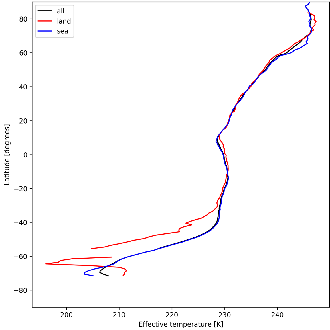
Figure 26: Zonal average of “Effective temperature” for 2025-08-04 to 2025-08-05.
