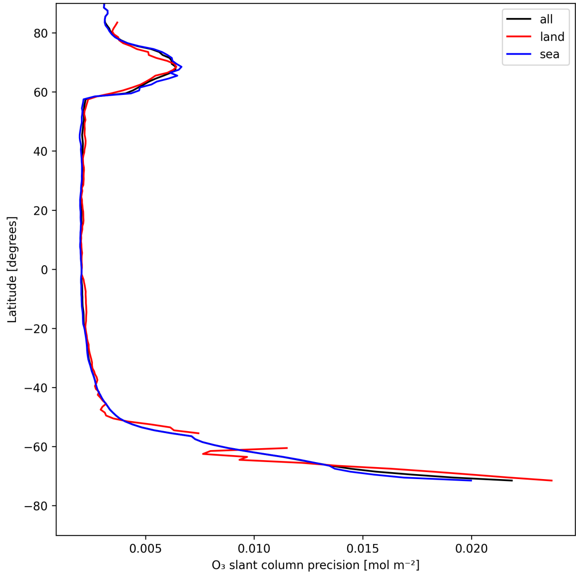
Figure 20: Zonal average of “O 3 slant column precision” for 2025-08-04 to 2025-08-05.
