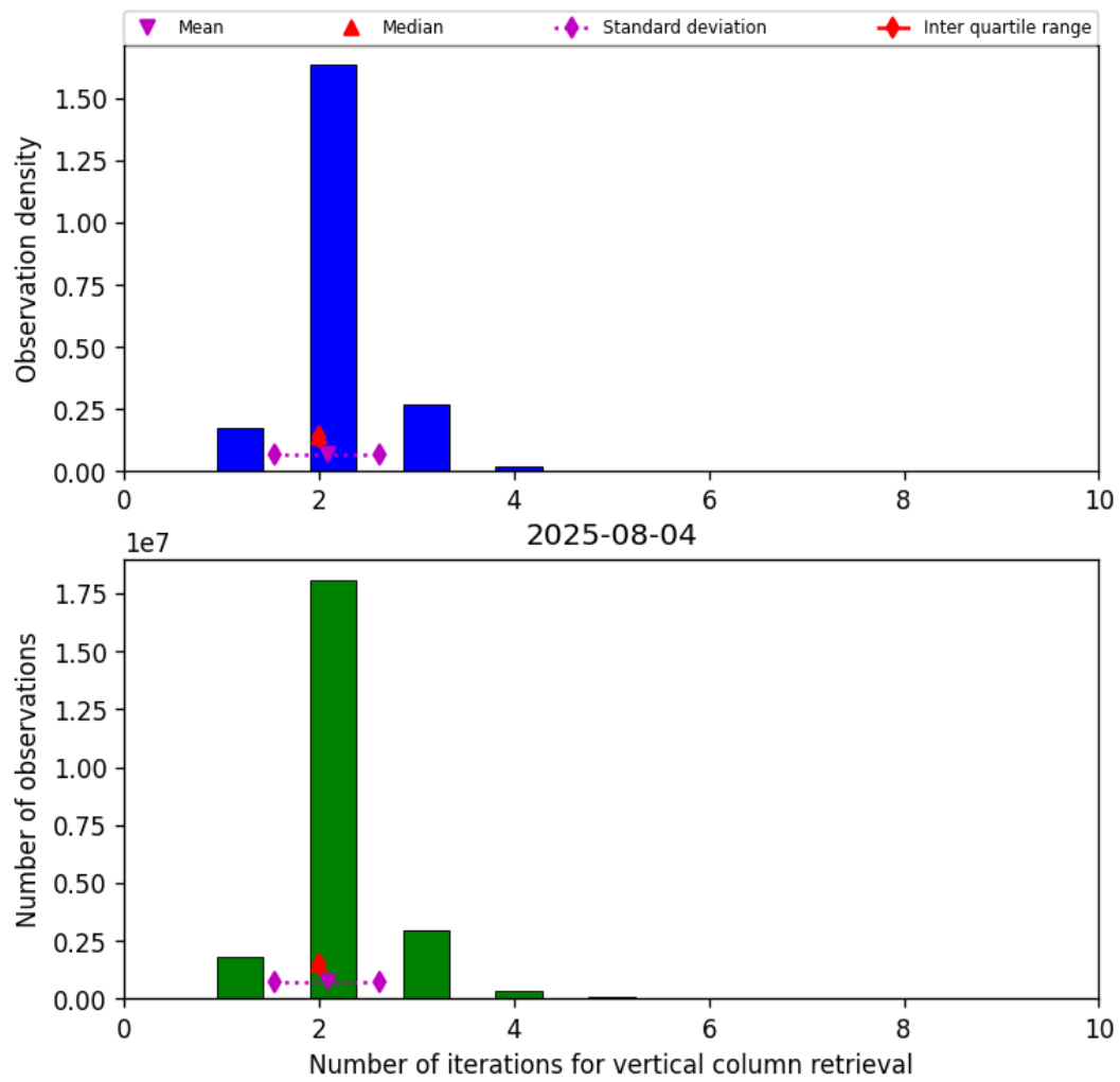
Figure 39: Histogram of “Number of iterations for vertical column retrieval” for 2025-08-04 to 2025-08-05
