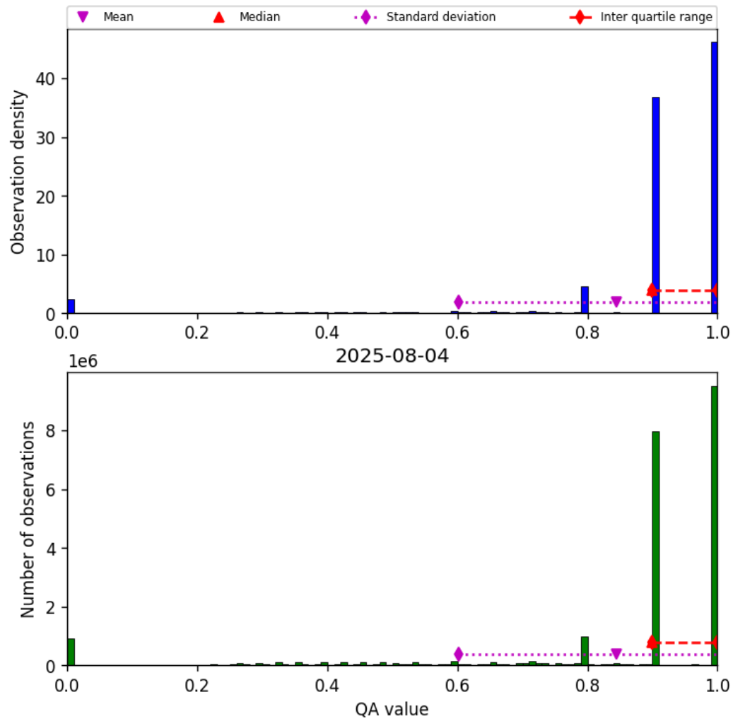
Figure 28: Histogram of “QA value” for 2025-08-04 to 2025-08-05
