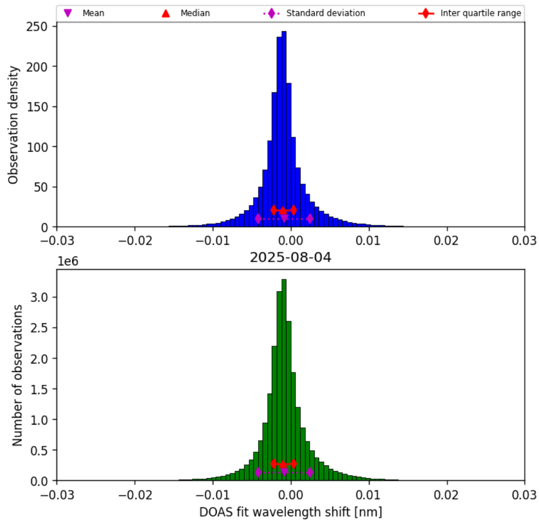
Figure 35: Histogram of “DOAS fit wavelength shift” for 2025-08-04 to 2025-08-05
