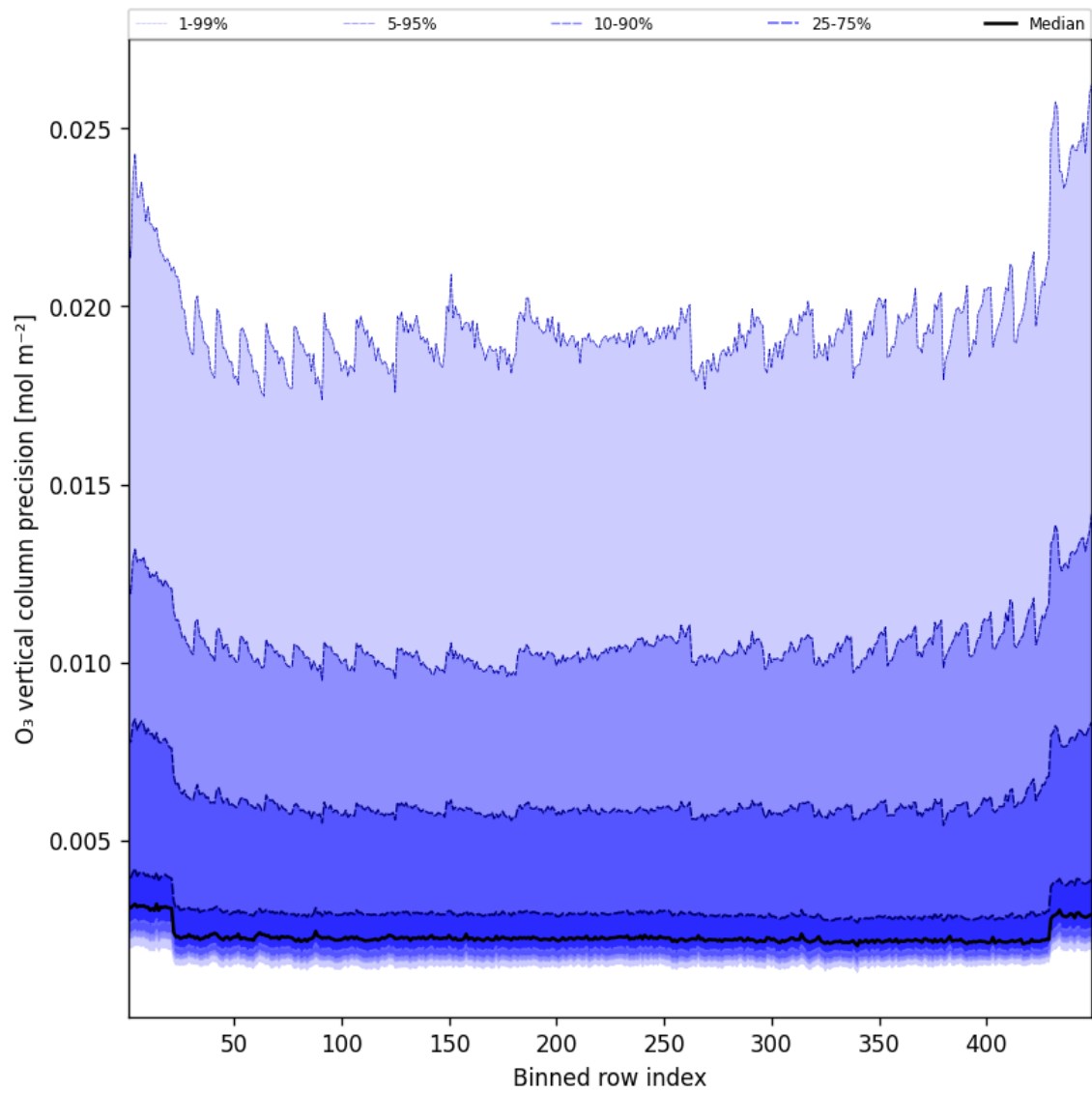
Figure 42: Along track statistics of “O 3 vertical column precision” for 2025-08-04 to 2025-08-05
