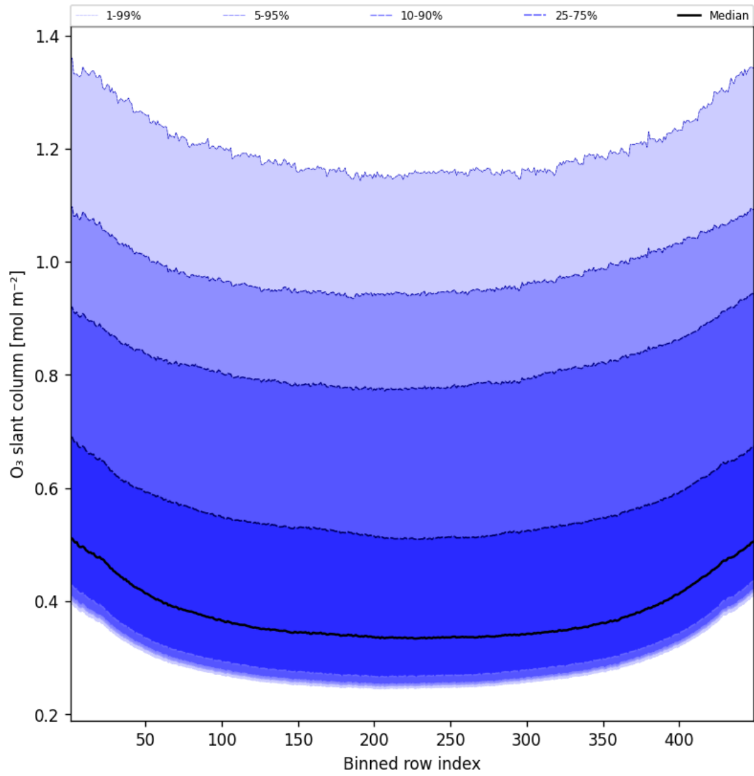
Figure 43: Along track statistics of “O 3 slant column” for 2025-08-04 to 2025-08-05
