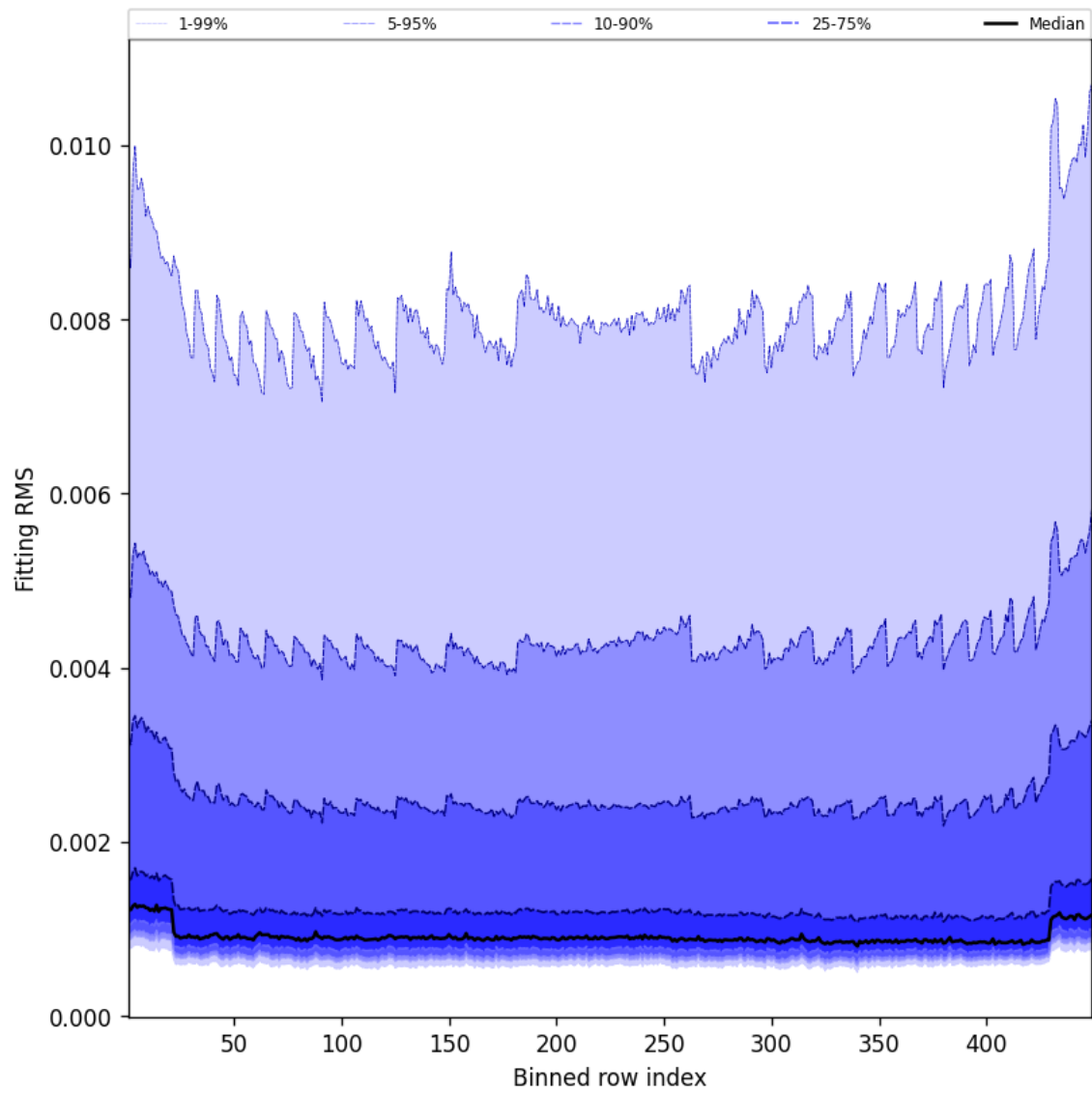
Figure 46: Along track statistics of “Fitting RMS” for 2025-08-04 to 2025-08-05
