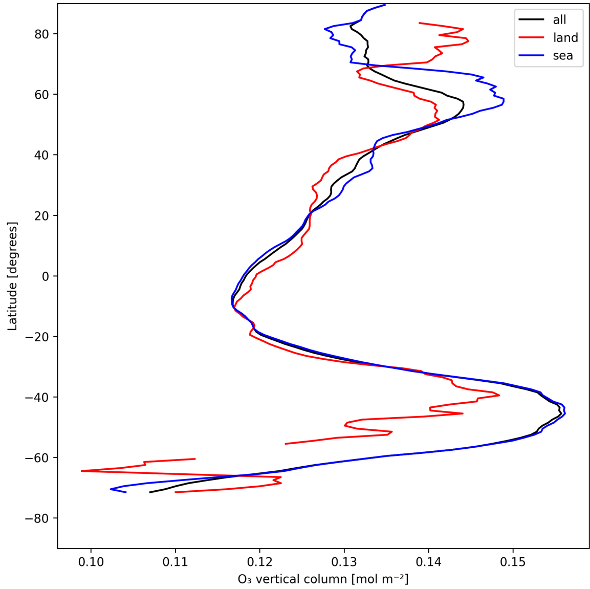
Figure 17: Zonal average of “O 3 vertical column” for 2025-08-04 to 2025-08-05.
