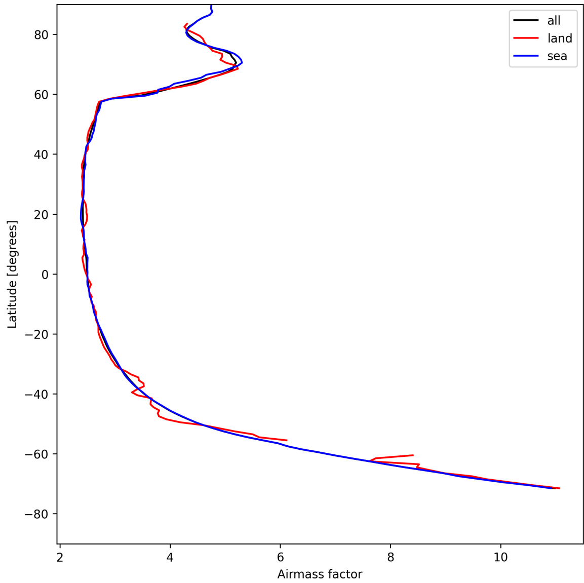
Figure 25: Zonal average of “Airmass factor” for 2025-08-04 to 2025-08-05.
