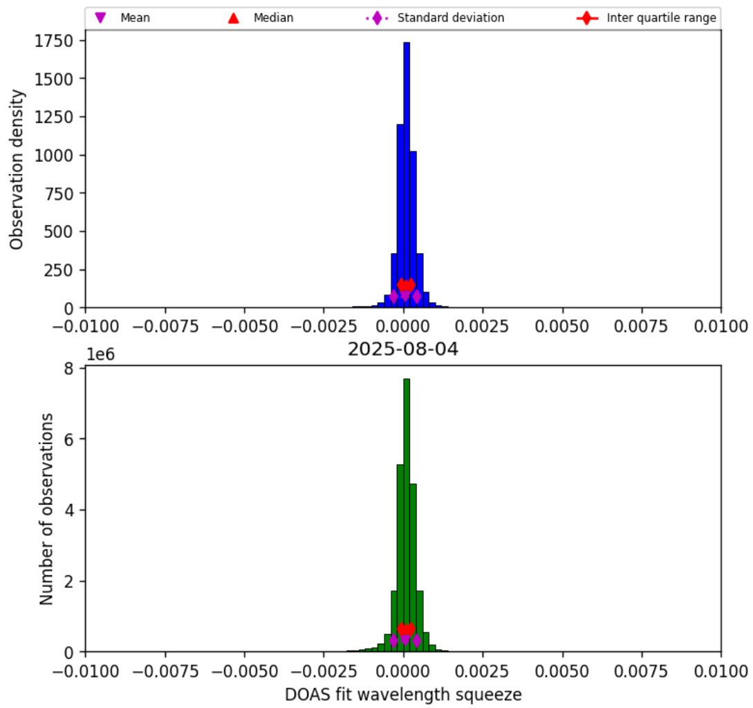
Figure 36: Histogram of “DOAS fit wavelength squeeze” for 2025-08-04 to 2025-08-05
