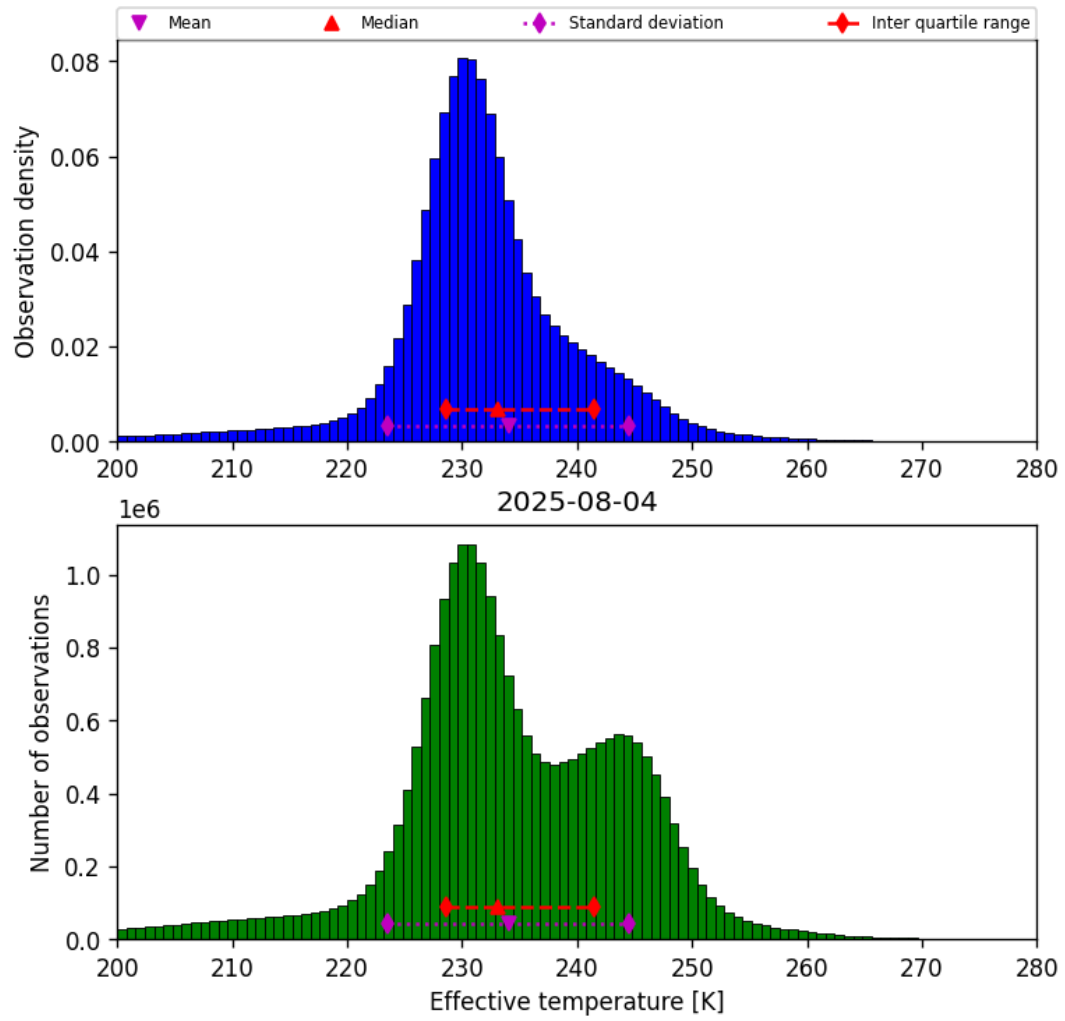
Figure 38: Histogram of “Effective temperature” for 2025-08-04 to 2025-08-05
