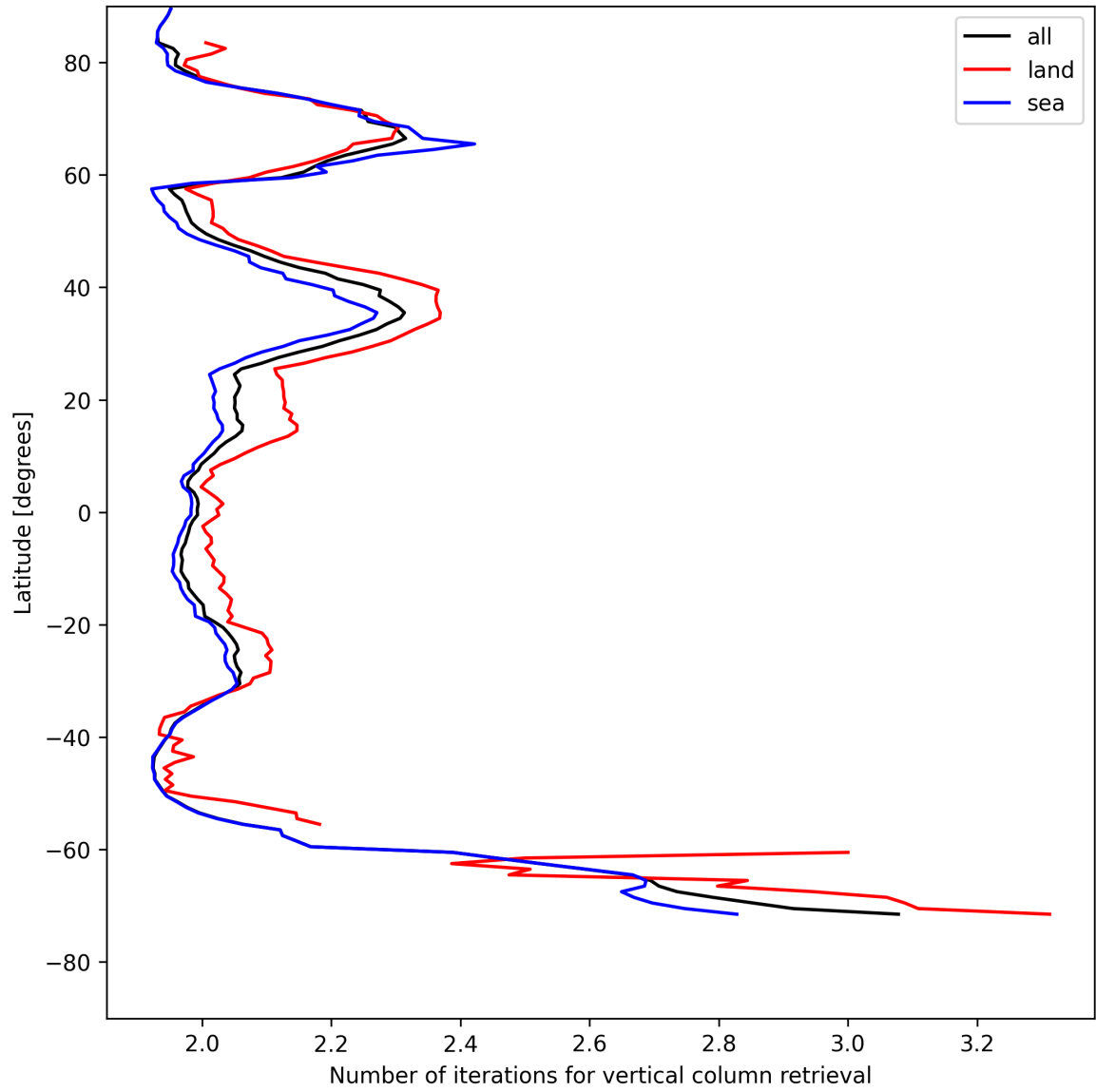
Figure 27: Zonal average of “Number of iterations for vertical column retrieval” for 2025-08-04 to 2025-08-05.
