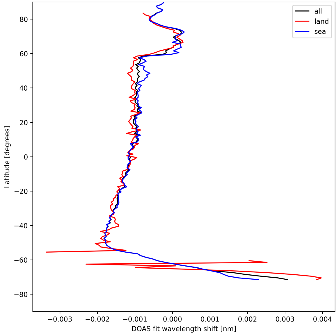
Figure 23: Zonal average of “DOAS fit wavelength shift” for 2025-08-04 to 2025-08-05.
