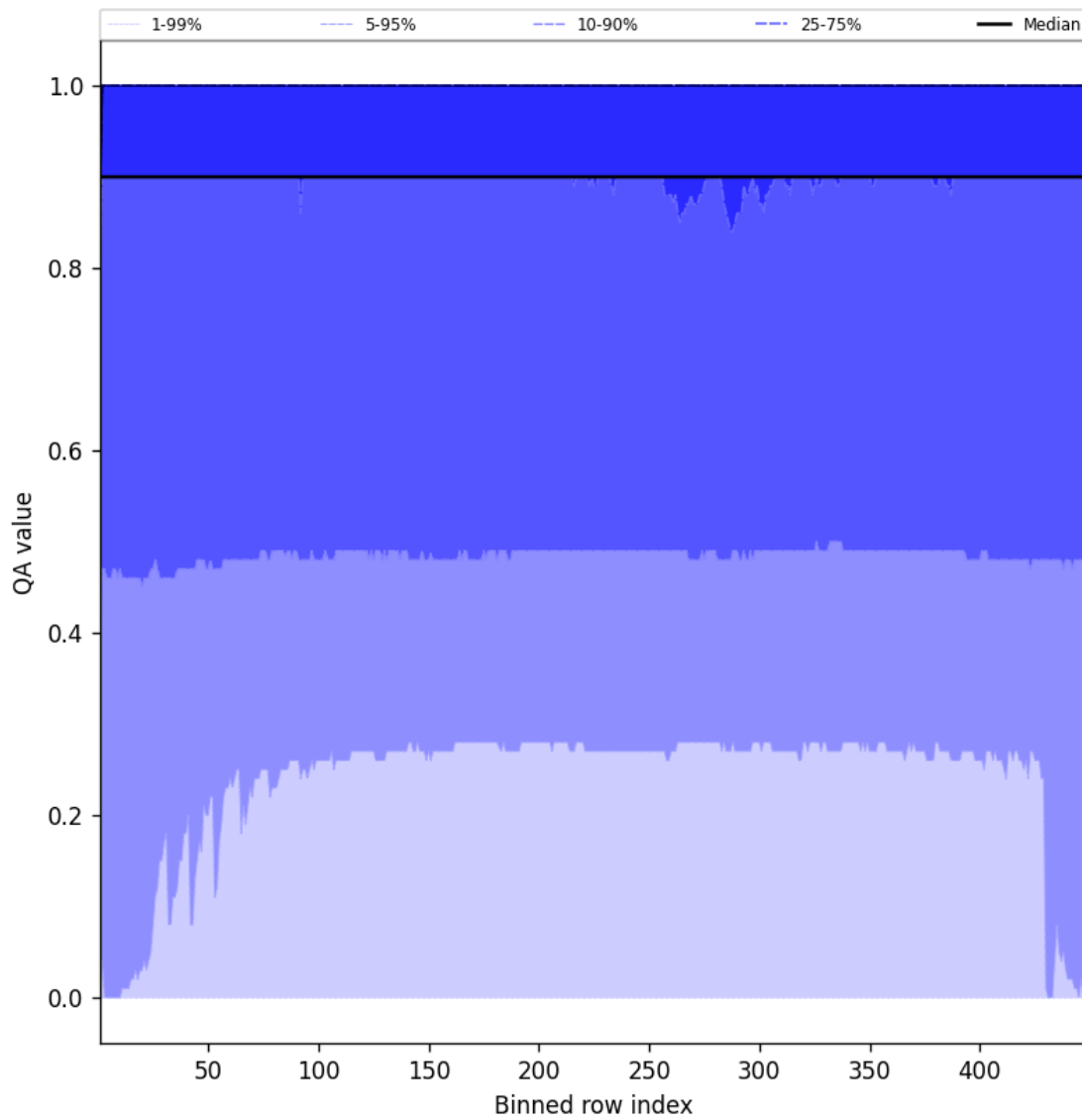
Figure 40: Along track statistics of “QA value” for 2025-08-04 to 2025-08-05
