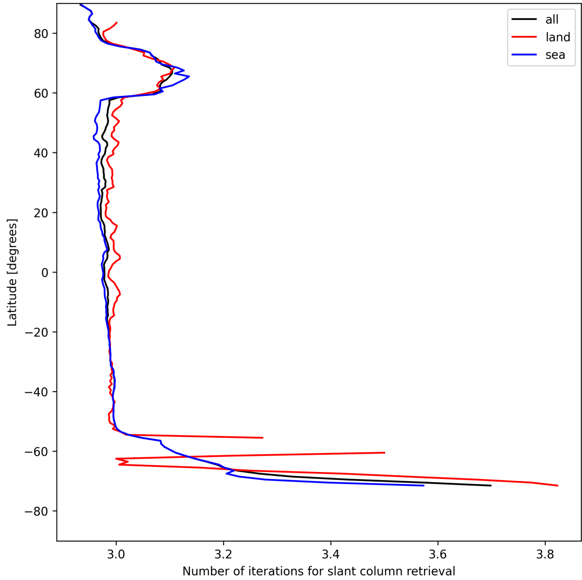
Figure 21: Zonal average of “Number of iterations for slant column retrieval” for 2025-08-04 to 2025-08-05.
