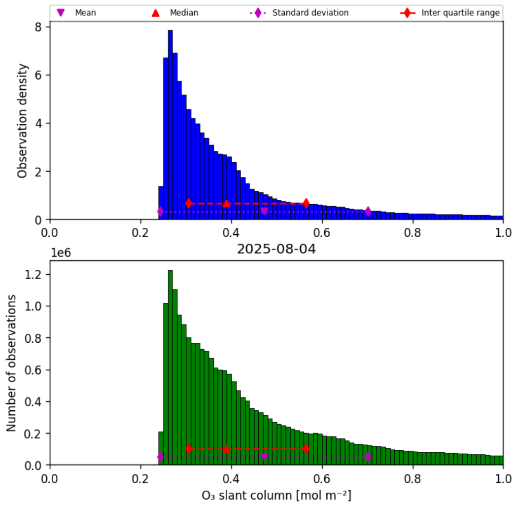
Figure 31: Histogram of “O 3 slant column” for 2025-08-04 to 2025-08-05
