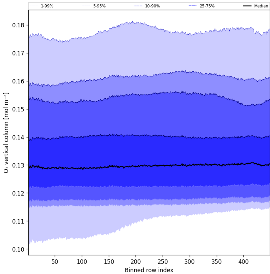
Figure 41: Along track statistics of “O 3 vertical column” for 2025-08-04 to 2025-08-05
