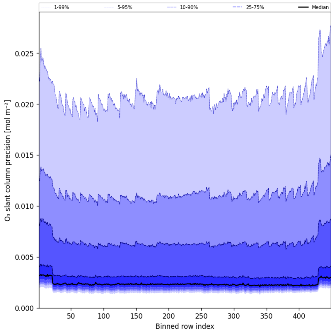
Figure 44: Along track statistics of “O 3 slant column precision” for 2025-08-04 to 2025-08-05
