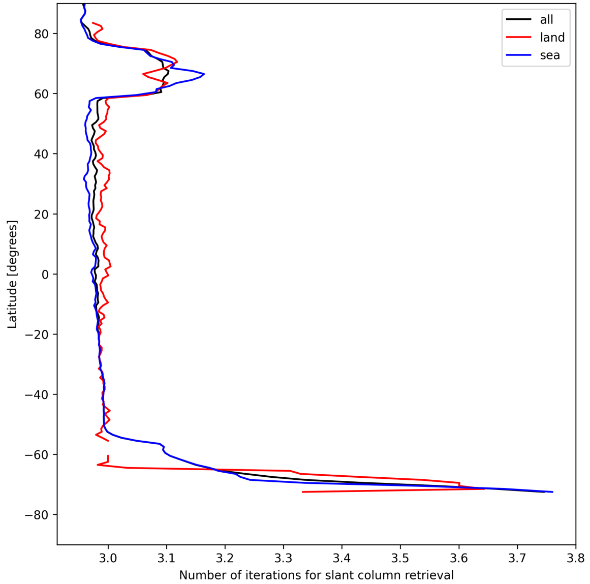
Figure 21: Zonal average of “Number of iterations for slant column retrieval” for 2025-08-05 to 2025-08-06.
