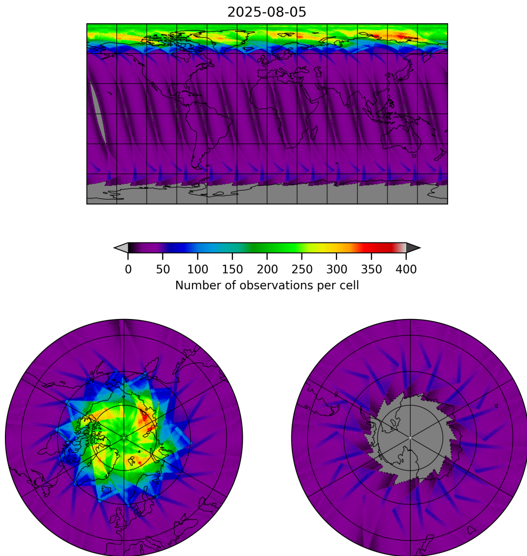
Figure 15: Map of the number of observations for 2025-08-05 to 2025-08-06
