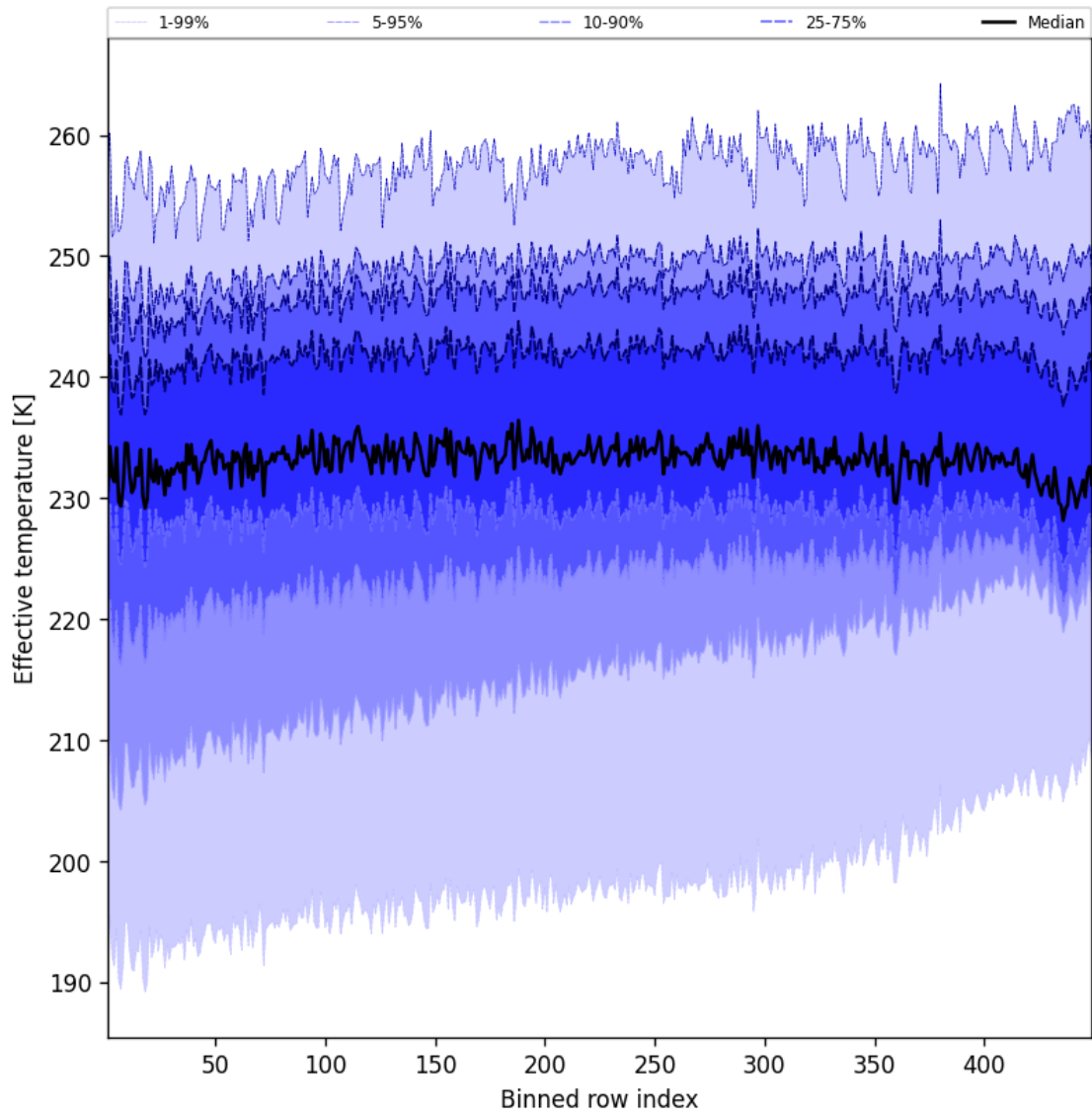
Figure 50: Along track statistics of “Effective temperature” for 2025-08-05 to 2025-08-06
