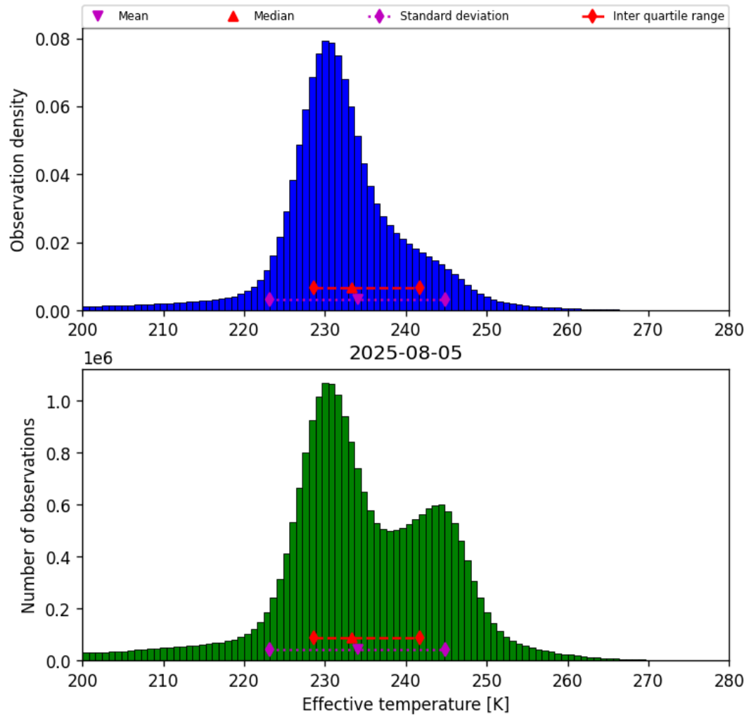
Figure 38: Histogram of “Effective temperature” for 2025-08-05 to 2025-08-06
