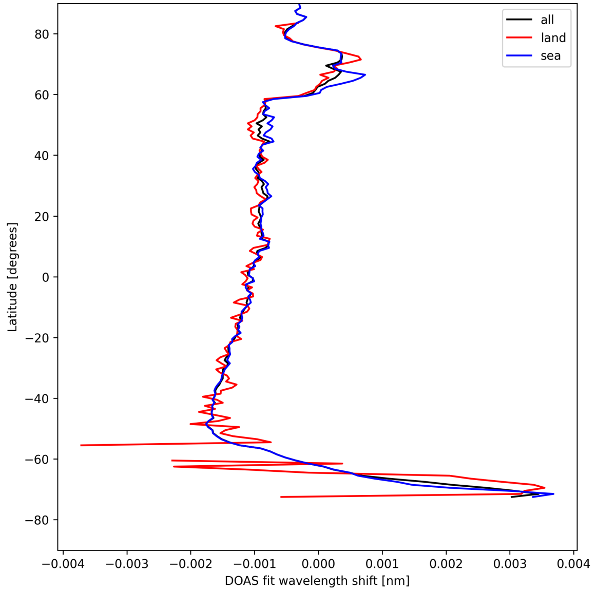
Figure 23: Zonal average of "DOAS fit wavelength shift" for 2025-08-05 to 2025-08-06.
