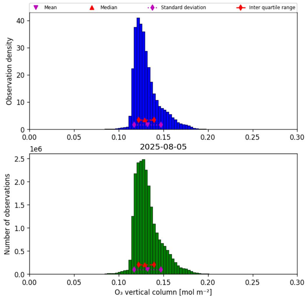
Figure 29: Histogram of “O 3 vertical column” for 2025-08-05 to 2025-08-06
