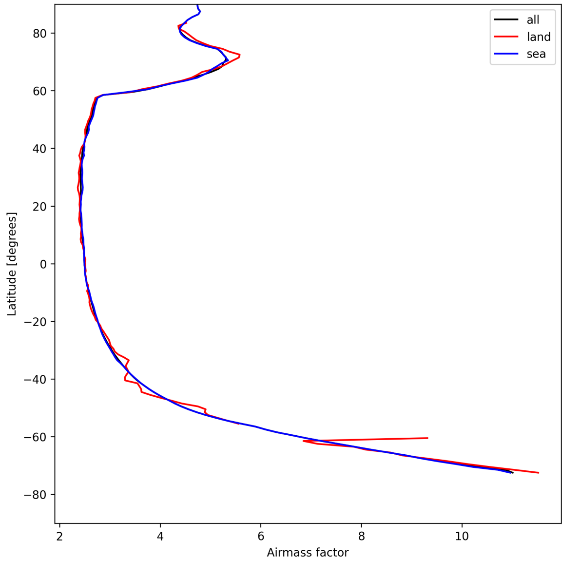
Figure 25: Zonal average of “Airmass factor” for 2025-08-05 to 2025-08-06.
