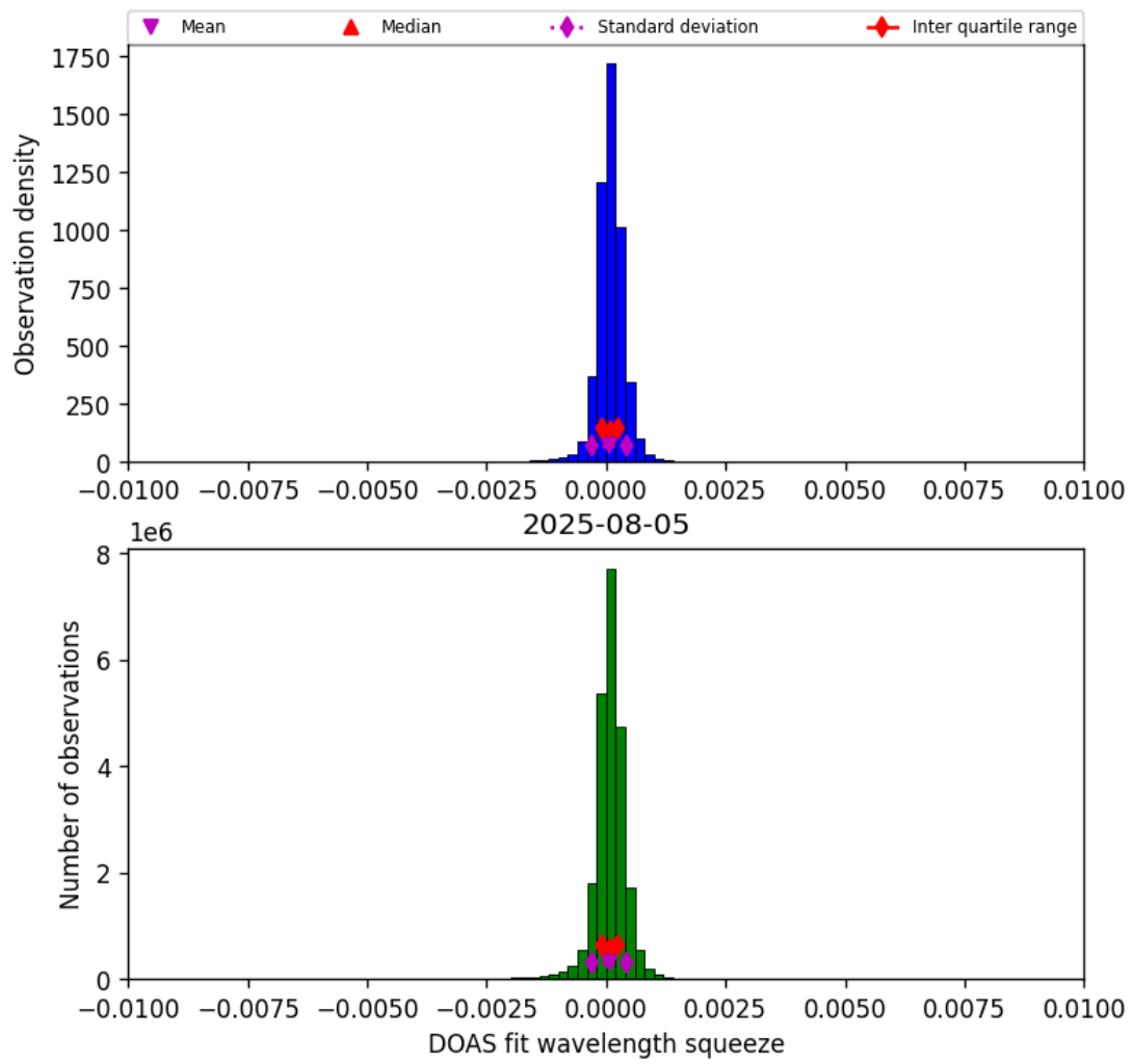
Figure 36: Histogram of “DOAS fit wavelength squeeze” for 2025-08-05 to 2025-08-06
