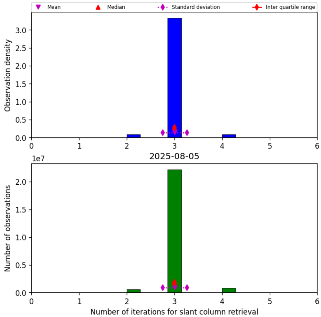
Figure 33: Histogram of “Number of iterations for slant column retrieval” for 2025-08-05 to 2025-08-06
