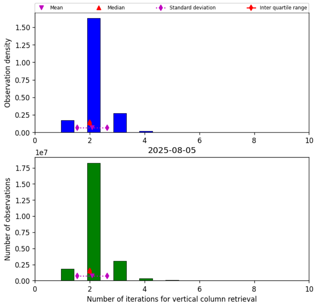
Figure 39: Histogram of “Number of iterations for vertical column retrieval” for 2025-08-05 to 2025-08-06
