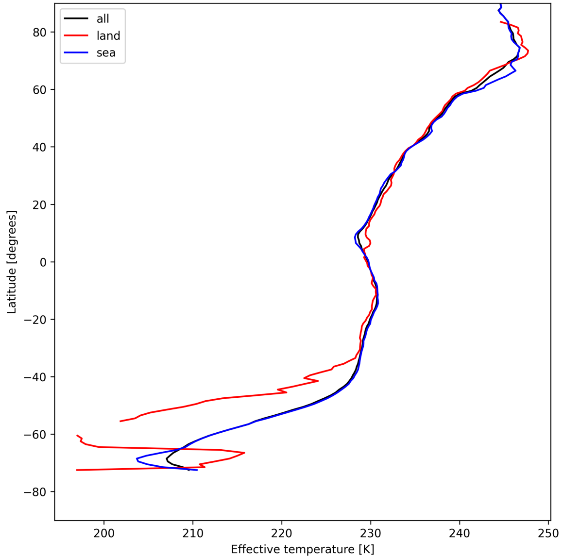
Figure 26: Zonal average of “Effective temperature” for 2025-08-05 to 2025-08-06.
