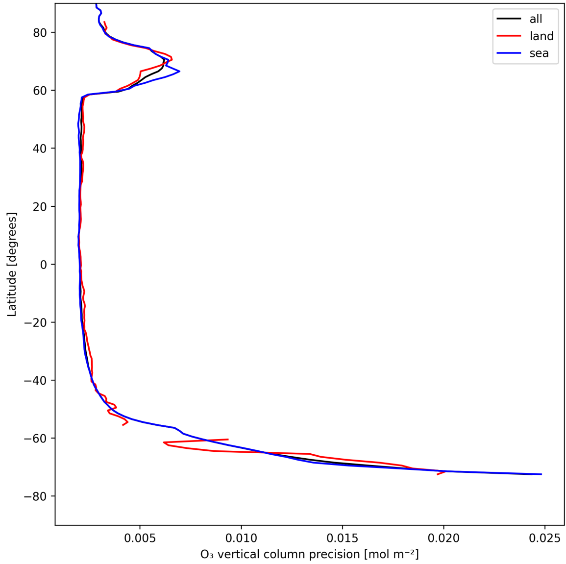
Figure 18: Zonal average of “O 3 vertical column precision” for 2025-08-05 to 2025-08-06.
