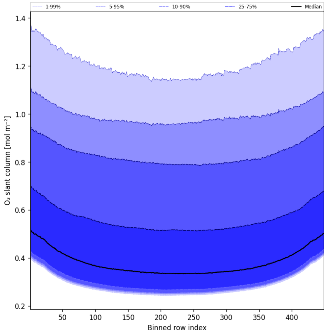
Figure 43: Along track statistics of “O 3 slant column” for 2025-08-05 to 2025-08-06
