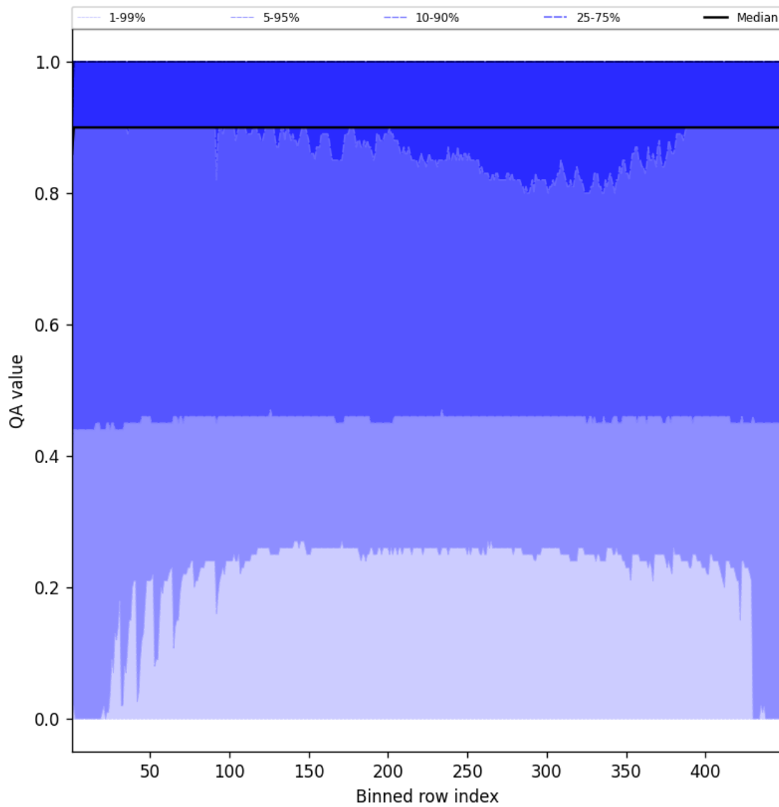
Figure 40: Along track statistics of “QA value” for 2025-08-05 to 2025-08-06
