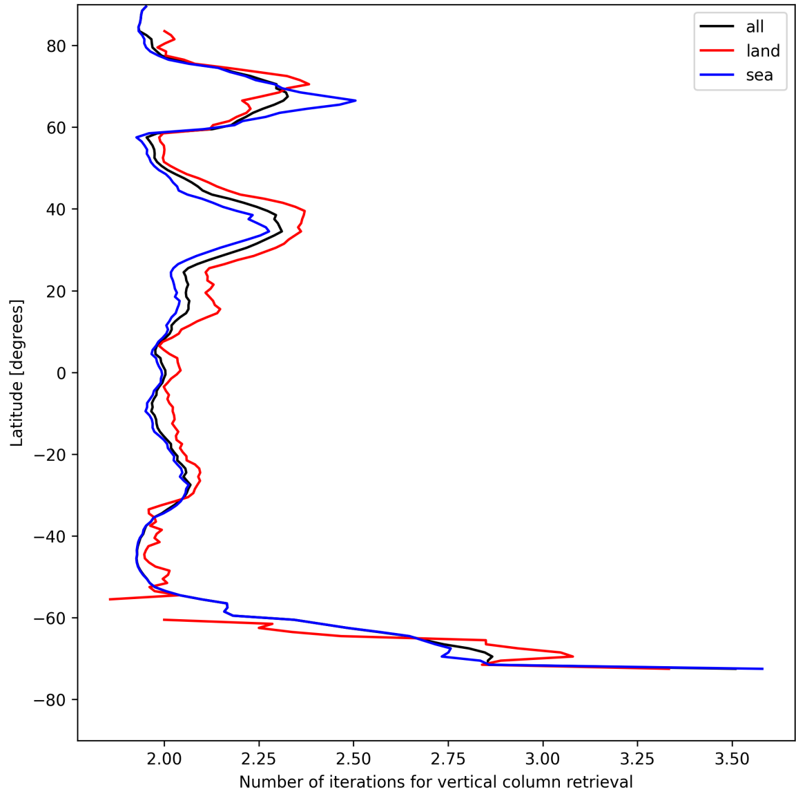
Figure 27: Zonal average of “Number of iterations for vertical column retrieval” for 2025-08-05 to 2025-08-06.
