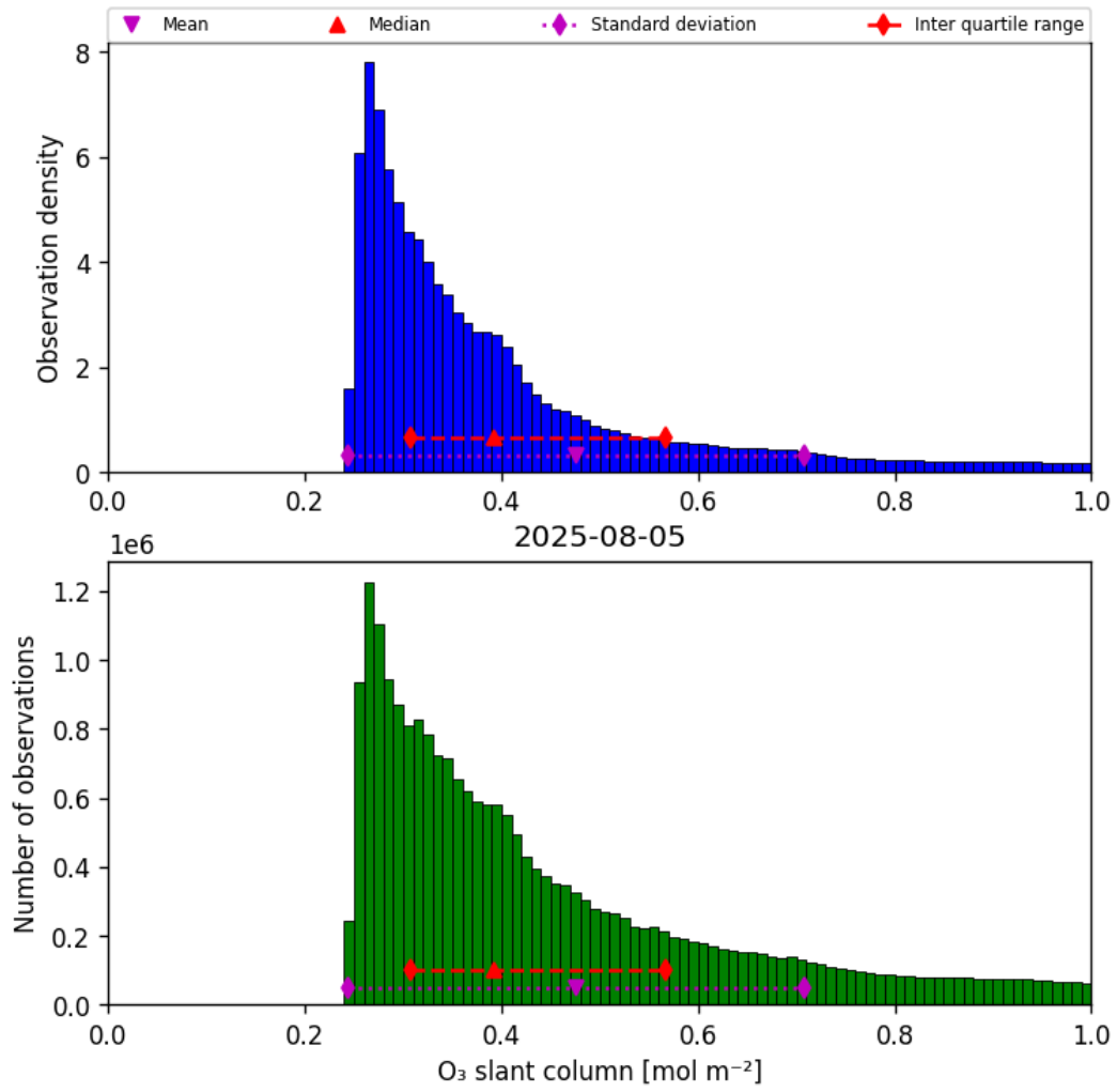
Figure 31: Histogram of “O 3 slant column” for 2025-08-05 to 2025-08-06
