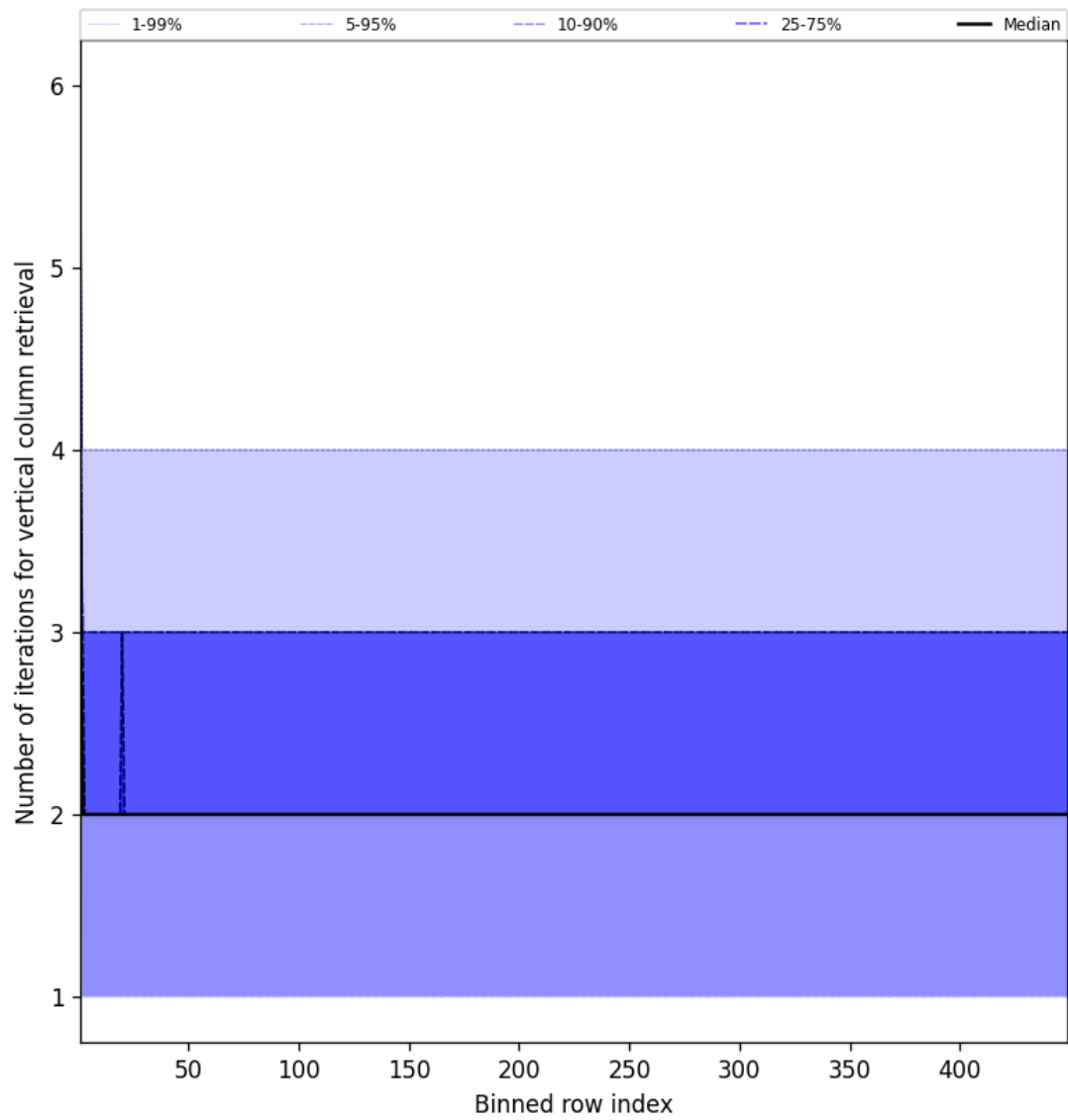
Figure 51: Along track statistics of “Number of iterations for vertical column retrieval” for 2025-08-05 to 2025-08-06
