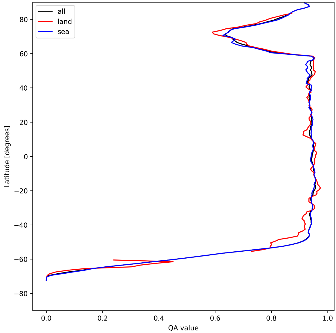
Figure 16: Zonal average of “QA value” for 2025-08-05 to 2025-08-06.
