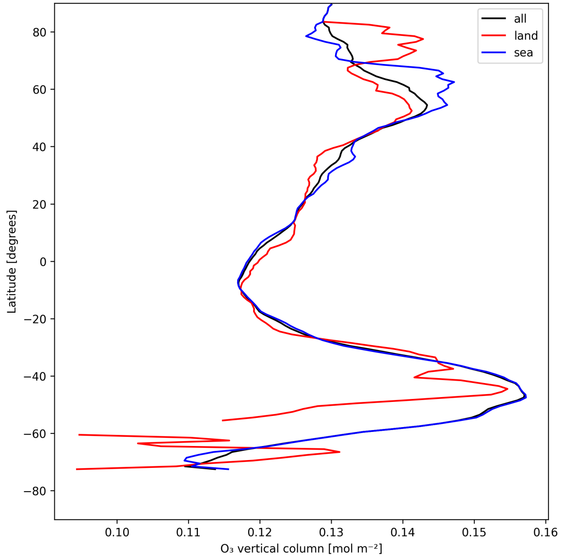
Figure 17: Zonal average of “O 3 vertical column” for 2025-08-05 to 2025-08-06.
