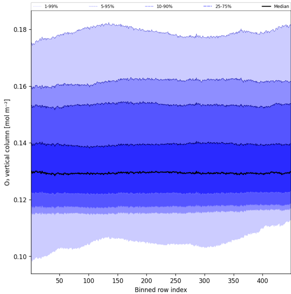
Figure 41: Along track statistics of “O 3 vertical column” for 2025-08-05 to 2025-08-06
