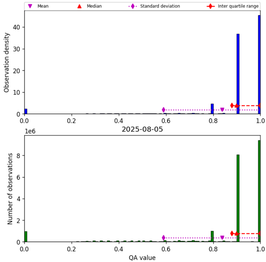
Figure 28: Histogram of “QA value” for 2025-08-05 to 2025-08-06
