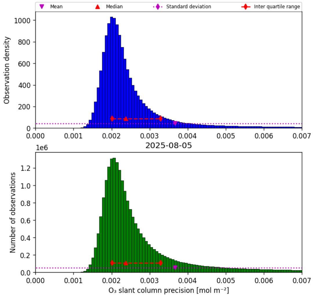
Figure 32: Histogram of “O 3 slant column precision” for 2025-08-05 to 2025-08-06
