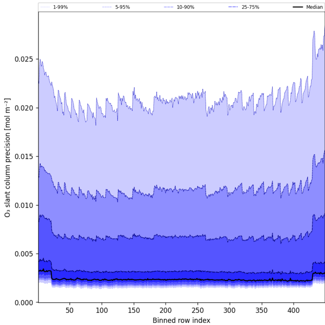
Figure 44: Along track statistics of “O 3 slant column precision” for 2025-08-05 to 2025-08-06
