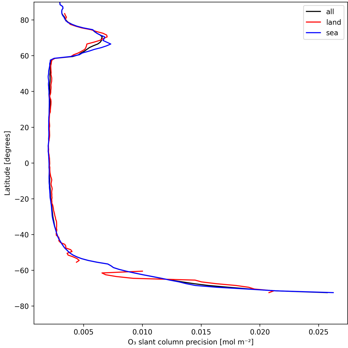
Figure 20: Zonal average of “O 3 slant column precision” for 2025-08-05 to 2025-08-06.
