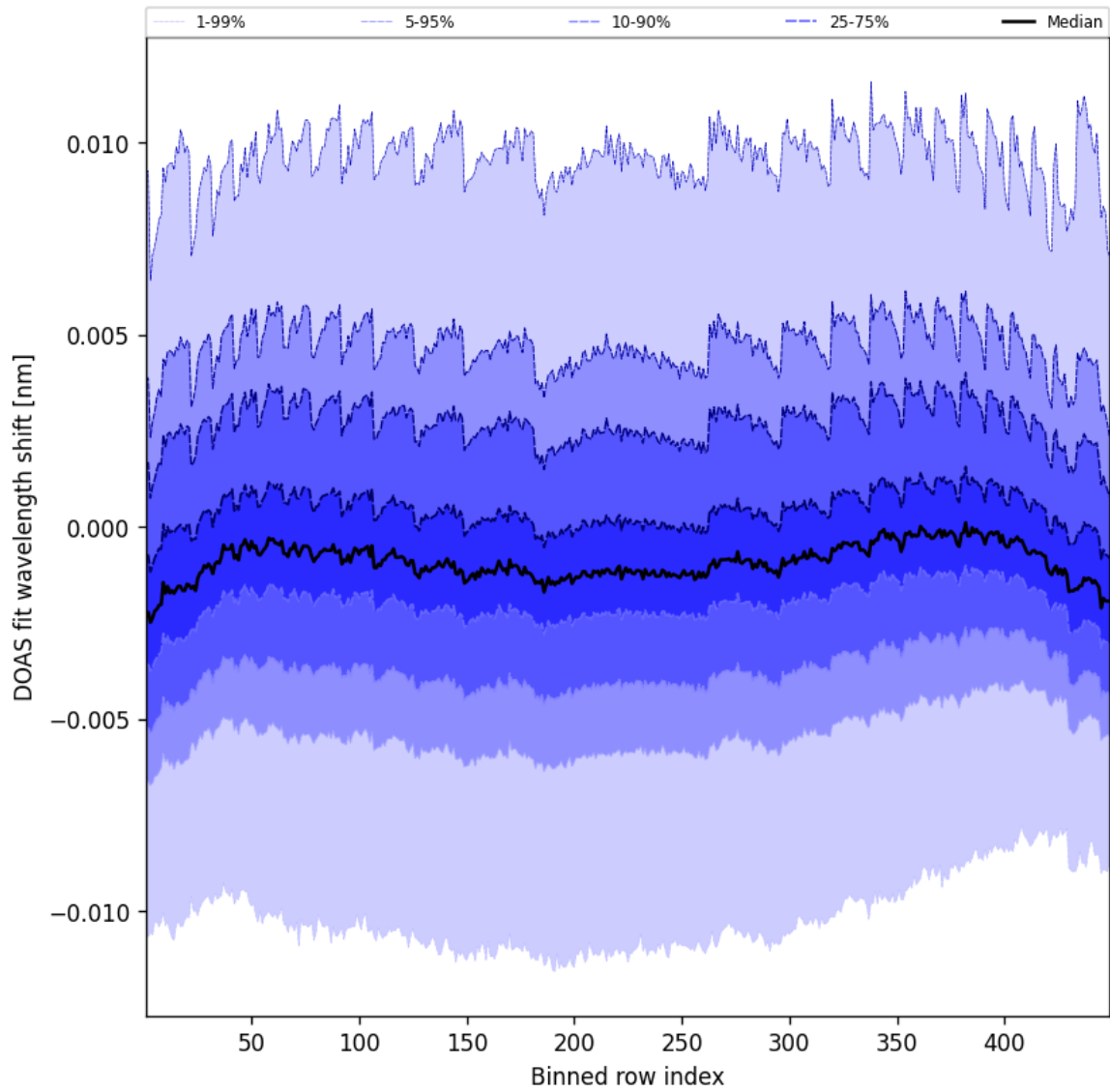
Figure 47: Along track statistics of “DOAS fit wavelength shift” for 2025-08-05 to 2025-08-06
