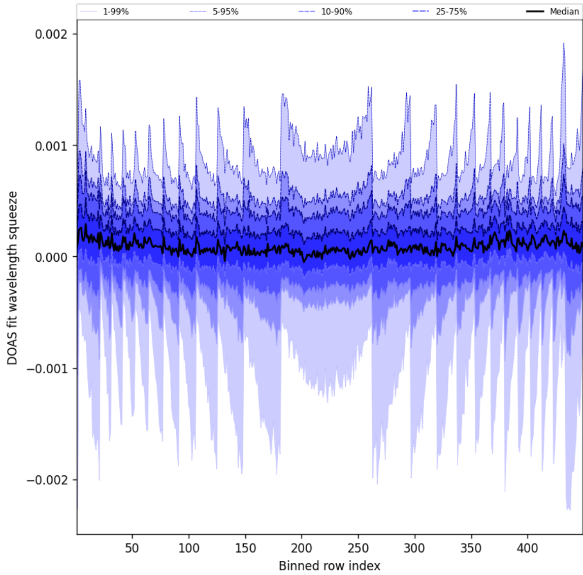
Figure 48: Along track statistics of “DOAS fit wavelength squeeze” for 2025-08-05 to 2025-08-06
