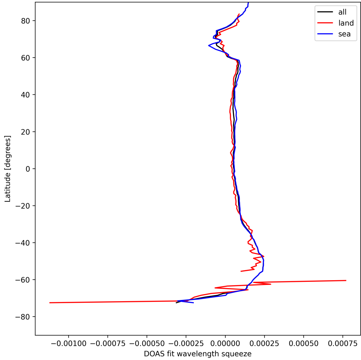
Figure 24: Zonal average of “DOAS fit wavelength squeeze” for 2025-08-05 to 2025-08-06.
