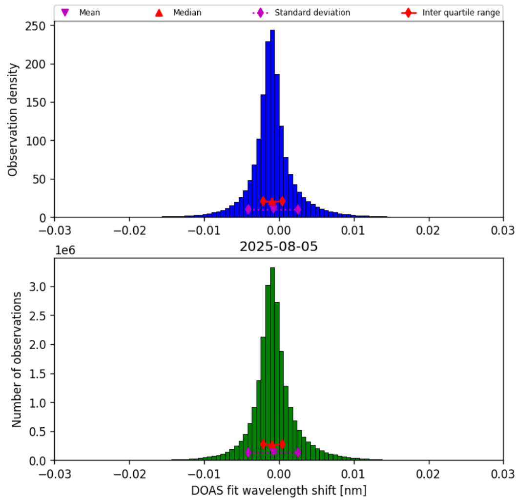
Figure 35: Histogram of “DOAS fit wavelength shift” for 2025-08-05 to 2025-08-06
