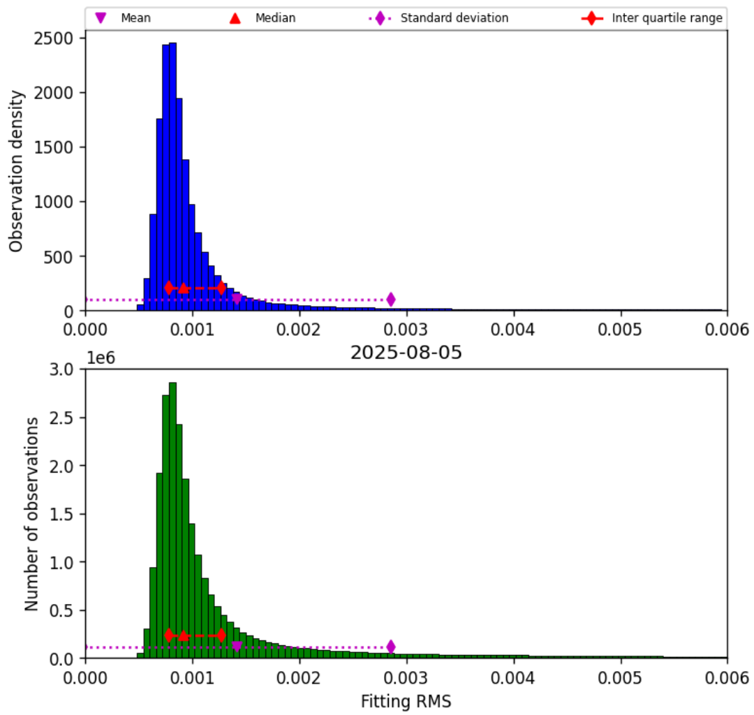
Figure 34: Histogram of “Fitting RMS” for 2025-08-05 to 2025-08-06
