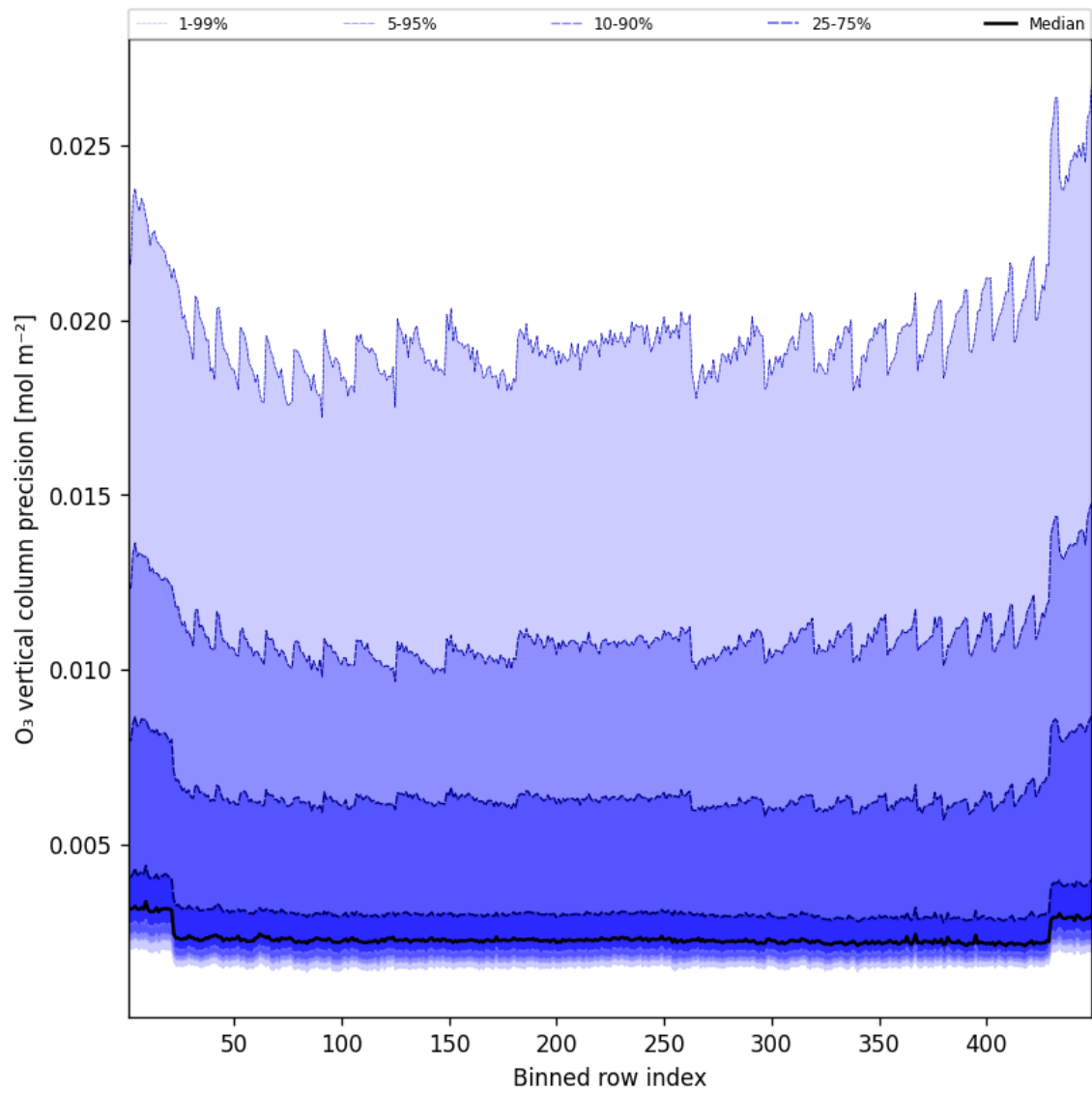
Figure 42: Along track statistics of “O 3 vertical column precision” for 2025-08-05 to 2025-08-06
