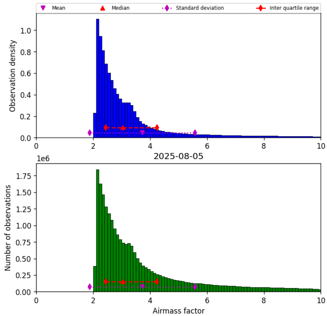
Figure 37: Histogram of “Airmass factor” for 2025-08-05 to 2025-08-06
