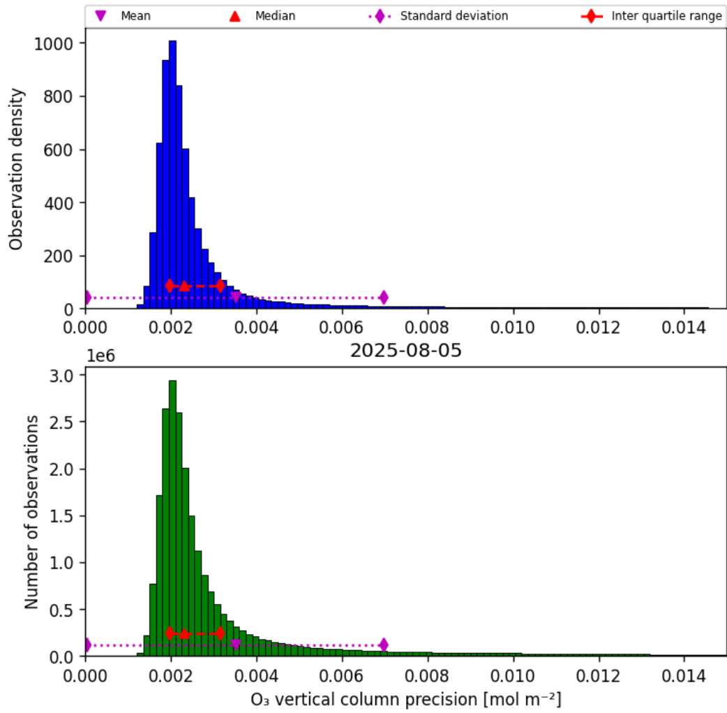
Figure 30: Histogram of “O 3 vertical column precision” for 2025-08-05 to 2025-08-06
