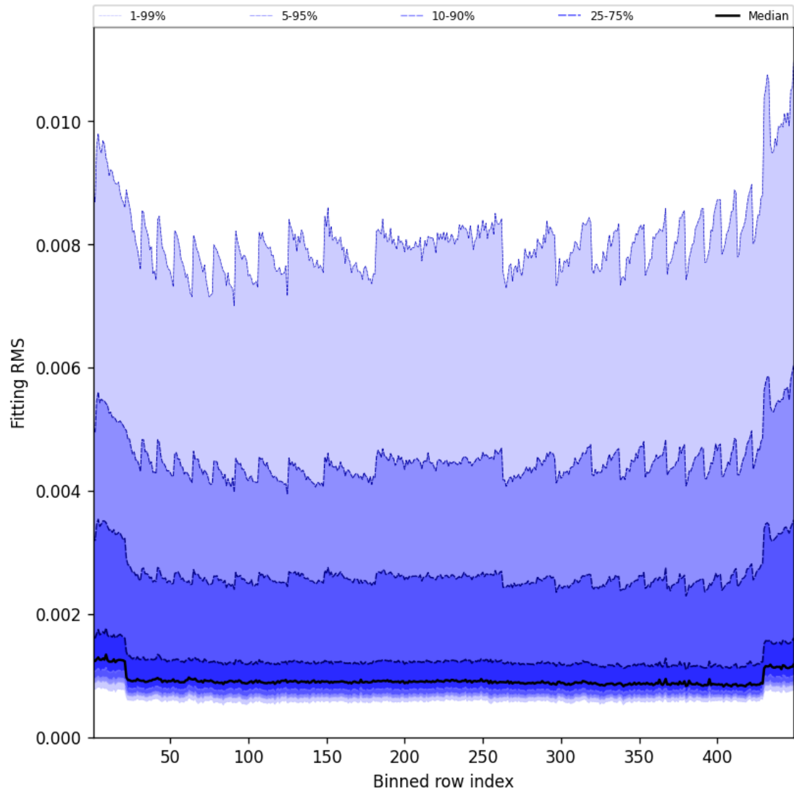
Figure 46: Along track statistics of “Fitting RMS” for 2025-08-05 to 2025-08-06
