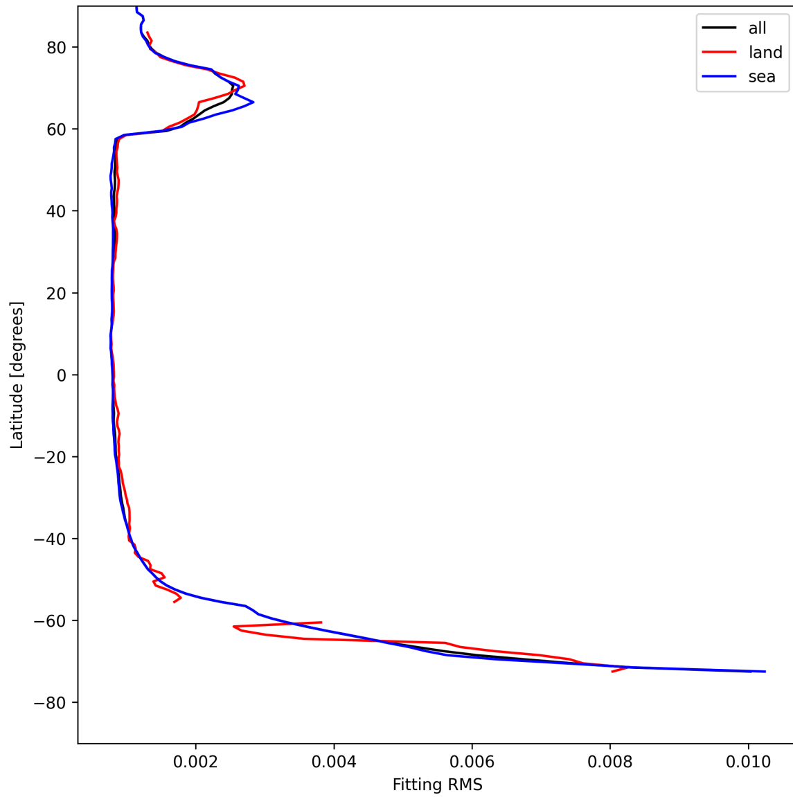
Figure 22: Zonal average of “Fitting RMS” for 2025-08-05 to 2025-08-06.
