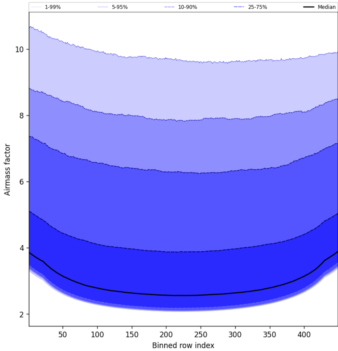
Figure 49: Along track statistics of “Airmass factor” for 2025-08-05 to 2025-08-06
