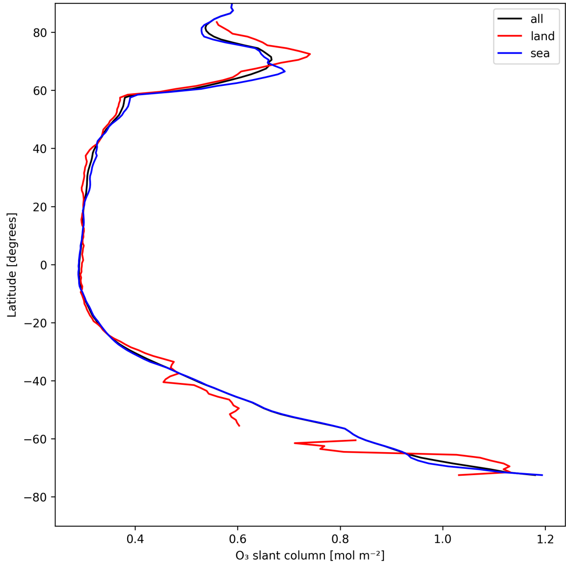
Figure 19: Zonal average of “O 3 slant column” for 2025-08-05 to 2025-08-06.
