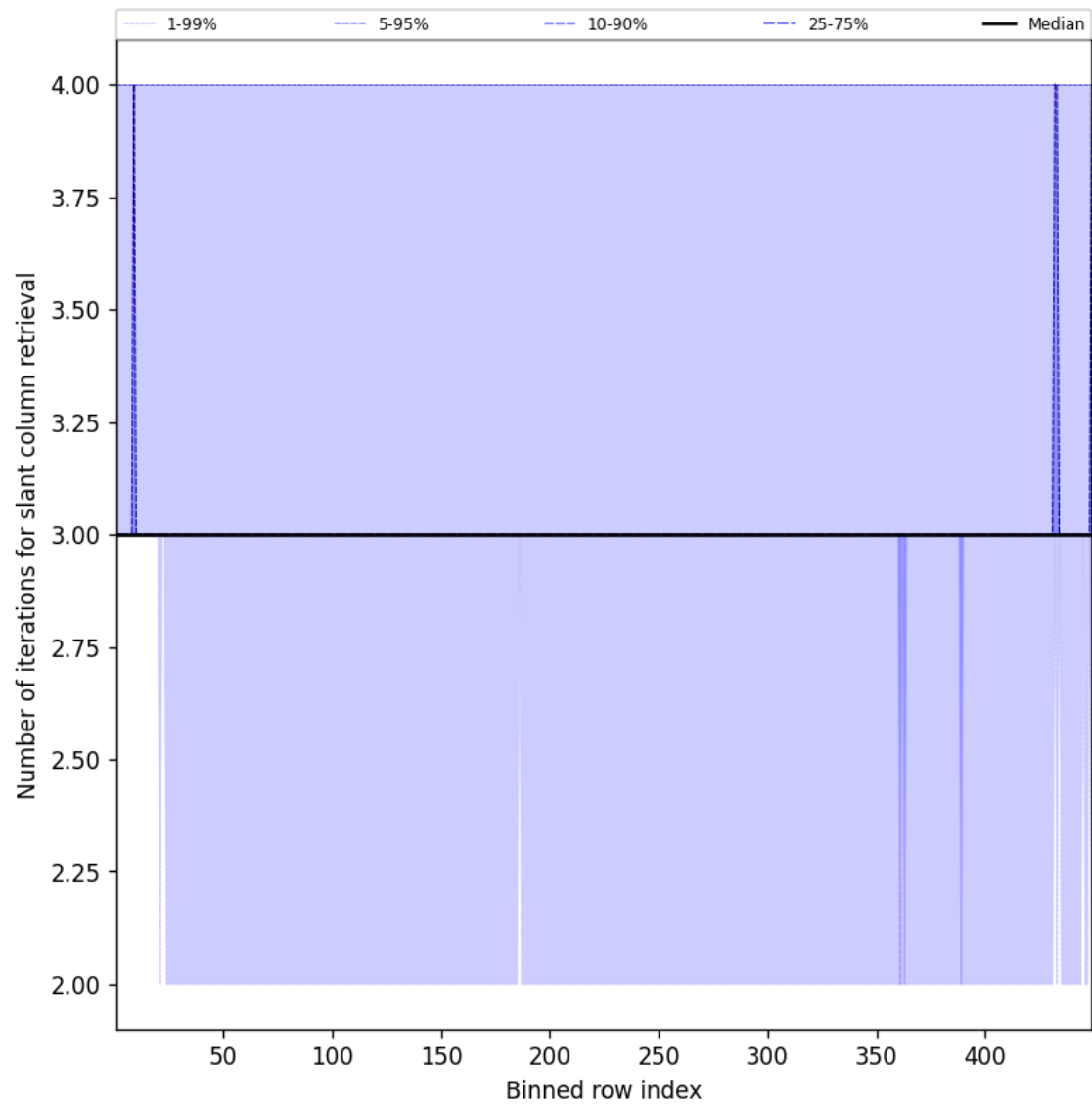
Figure 45: Along track statistics of “Number of iterations for slant column retrieval” for 2025-08-05 to 2025-08-06
