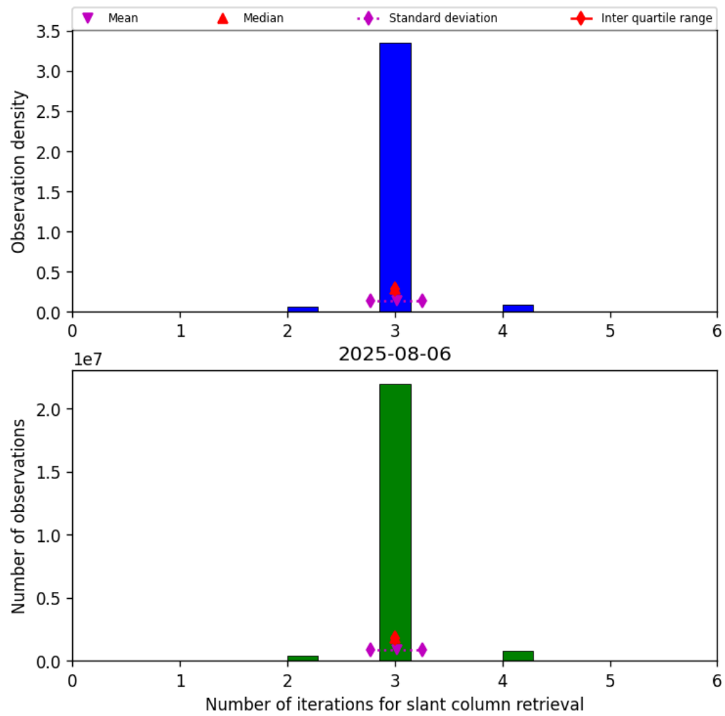
Figure 33: Histogram of “Number of iterations for slant column retrieval” for 2025-08-06 to 2025-08-07
