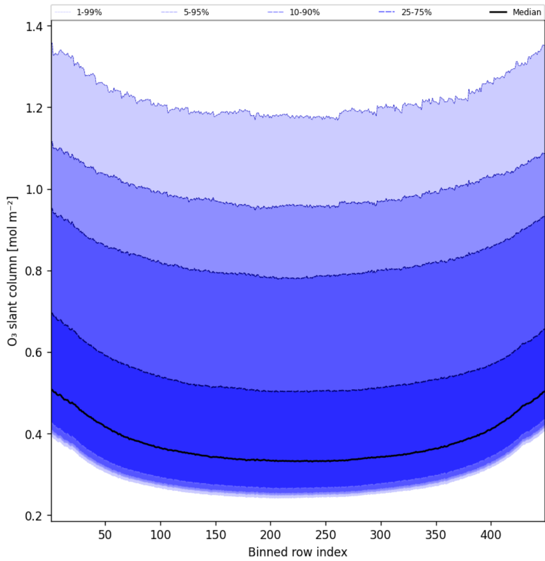
Figure 43: Along track statistics of “O 3 slant column” for 2025-08-06 to 2025-08-07
