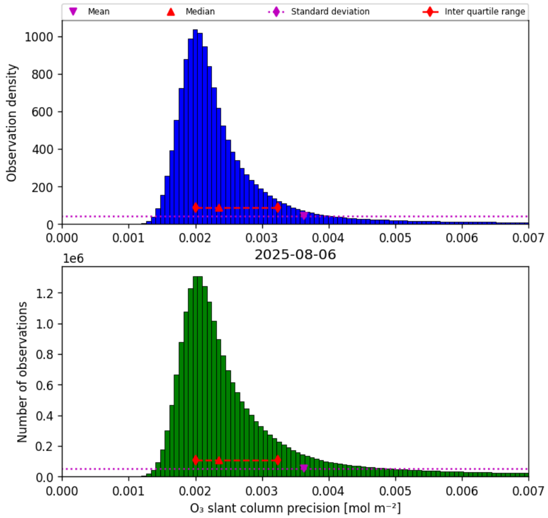
Figure 32: Histogram of “O 3 slant column precision” for 2025-08-06 to 2025-08-07
