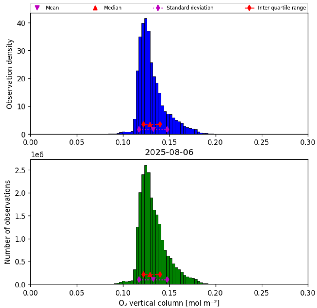
Figure 29: Histogram of “O 3 vertical column” for 2025-08-06 to 2025-08-07
