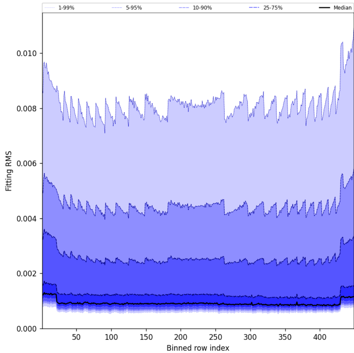
Figure 46: Along track statistics of “Fitting RMS” for 2025-08-06 to 2025-08-07
