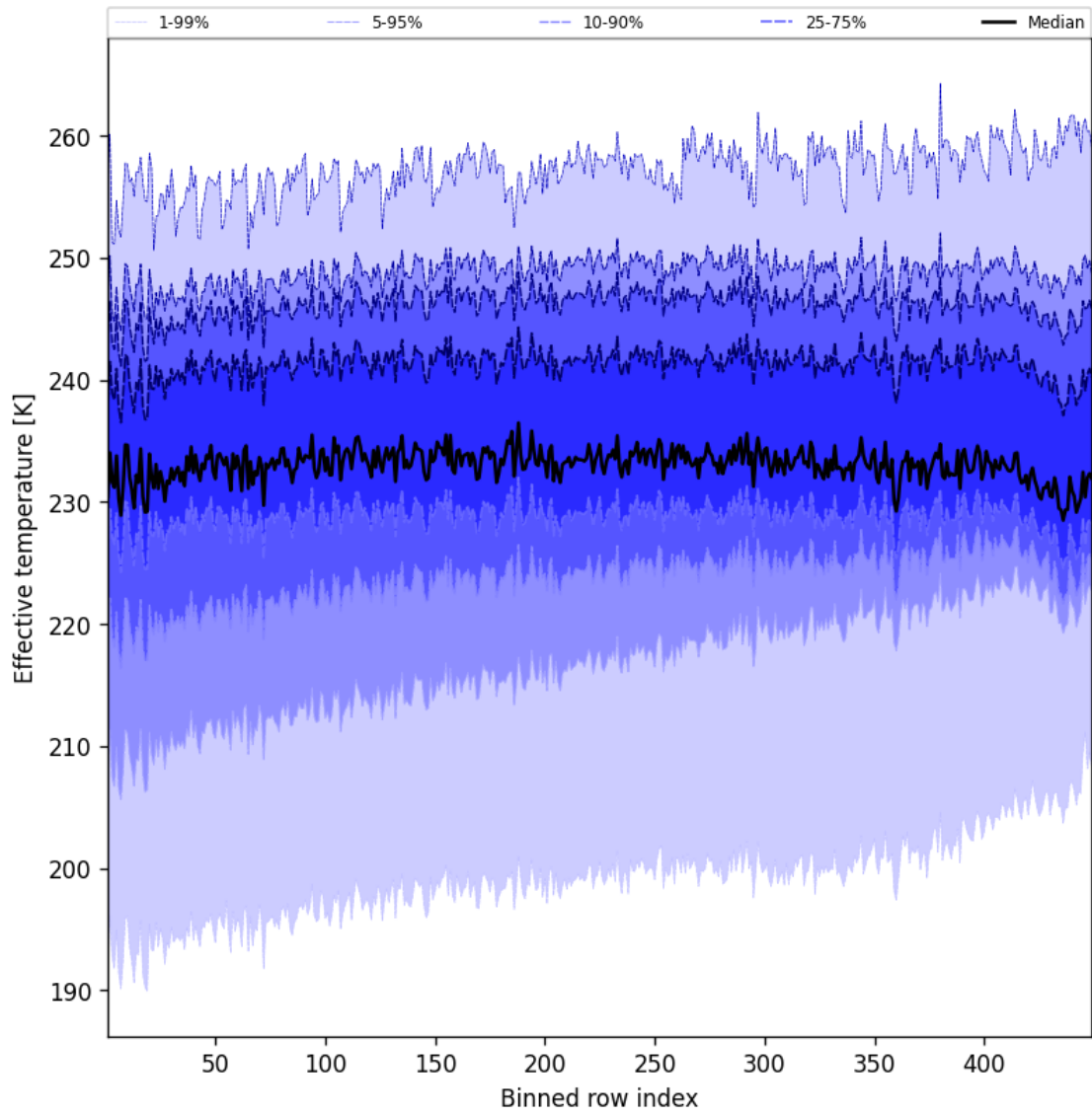
Figure 50: Along track statistics of “Effective temperature” for 2025-08-06 to 2025-08-07
