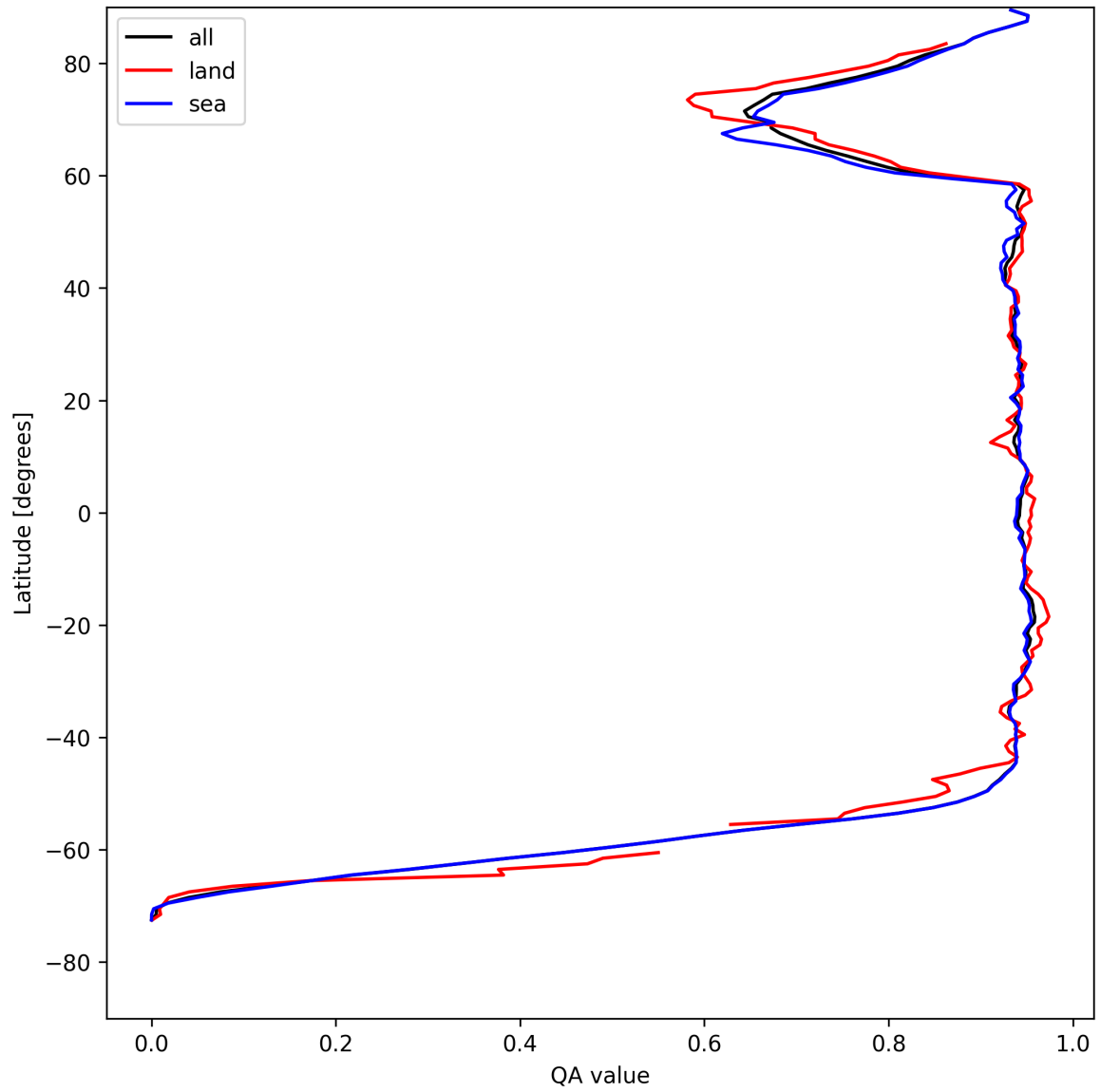
Figure 16: Zonal average of “QA value” for 2025-08-06 to 2025-08-07.
