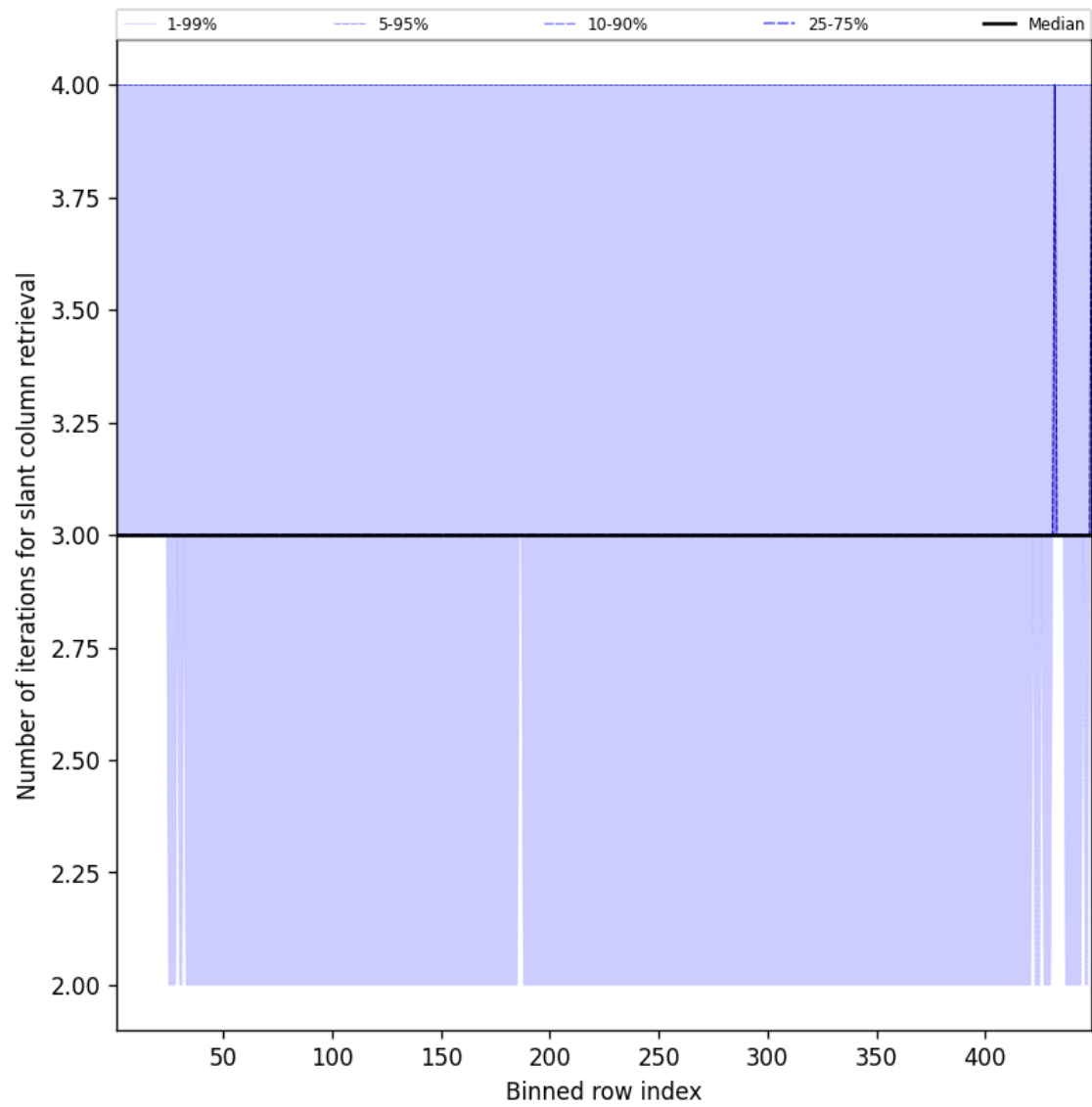
Figure 45: Along track statistics of “Number of iterations for slant column retrieval” for 2025-08-06 to 2025-08-07
