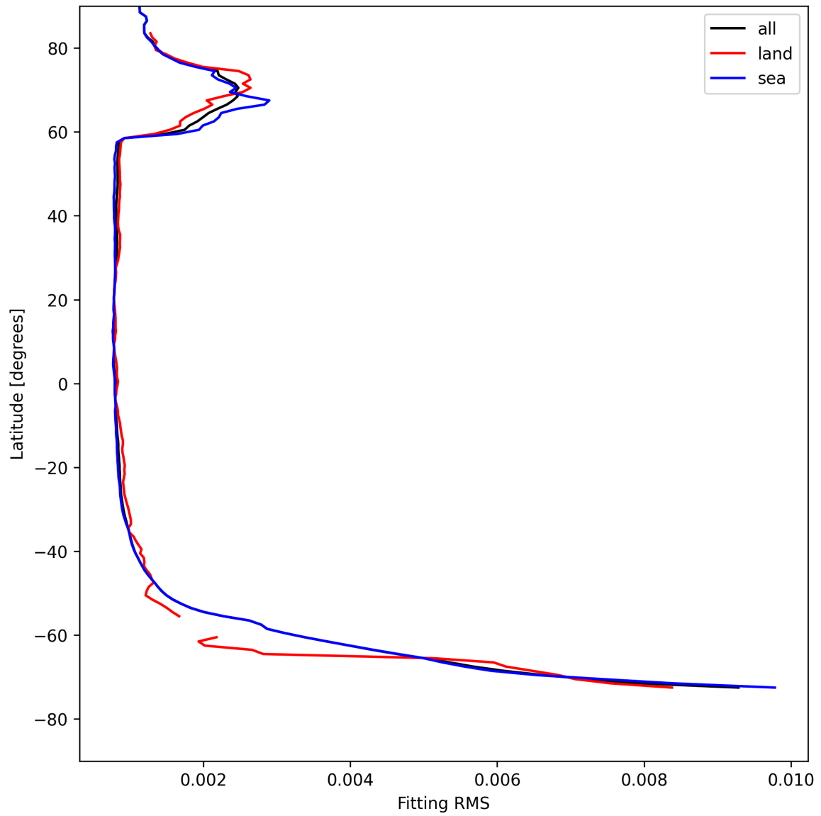
Figure 22: Zonal average of “Fitting RMS” for 2025-08-06 to 2025-08-07.
