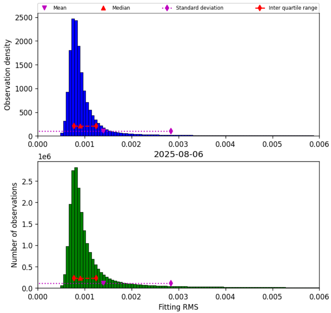
Figure 34: Histogram of “Fitting RMS” for 2025-08-06 to 2025-08-07
