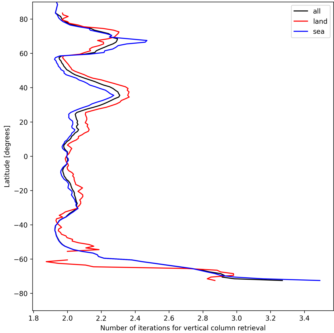
Figure 27: Zonal average of “Number of iterations for vertical column retrieval” for 2025-08-06 to 2025-08-07.
