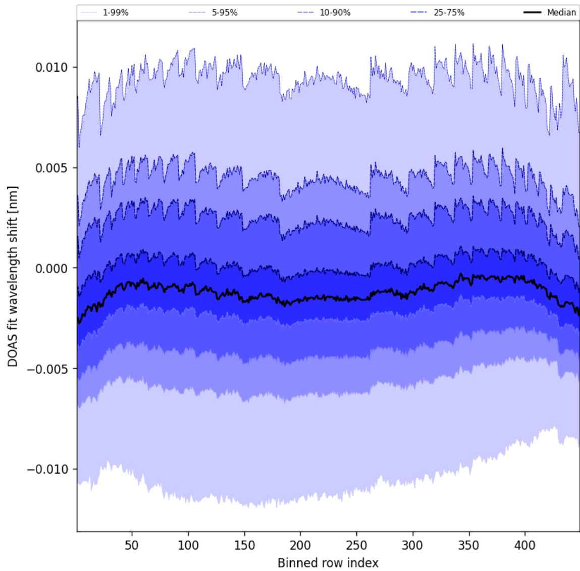
Figure 47: Along track statistics of “DOAS fit wavelength shift” for 2025-08-06 to 2025-08-07
