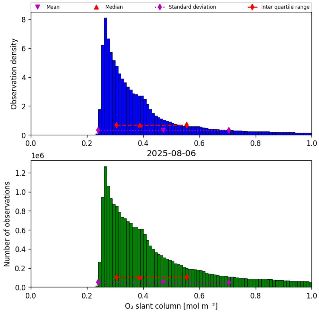
Figure 31: Histogram of “O 3 slant column” for 2025-08-06 to 2025-08-07
