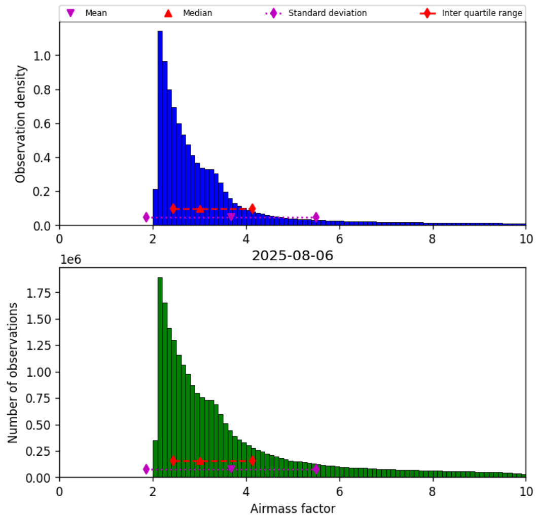
Figure 37: Histogram of “Airmass factor” for 2025-08-06 to 2025-08-07
