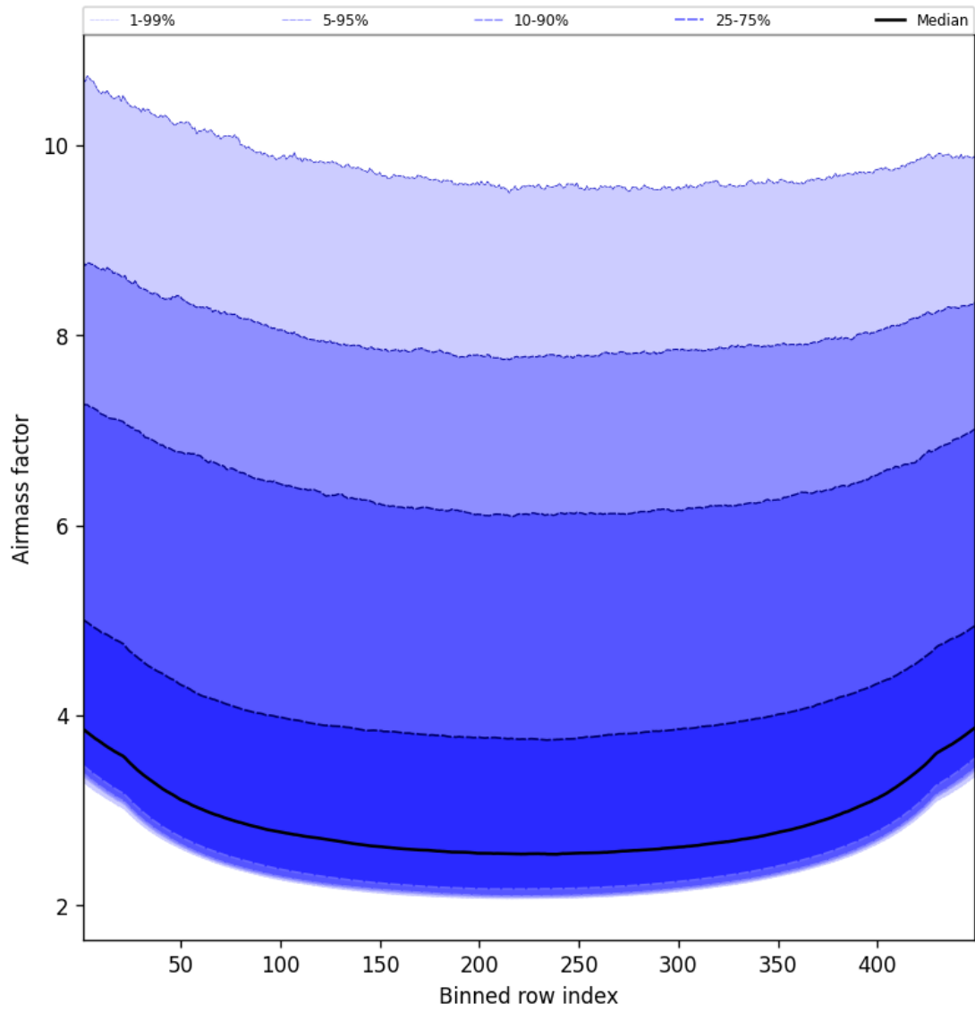
Figure 49: Along track statistics of “Airmass factor” for 2025-08-06 to 2025-08-07
