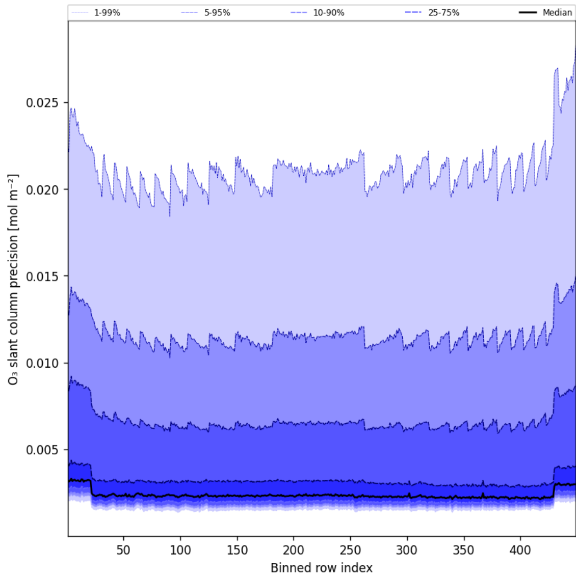
Figure 44: Along track statistics of “O 3 slant column precision” for 2025-08-06 to 2025-08-07
