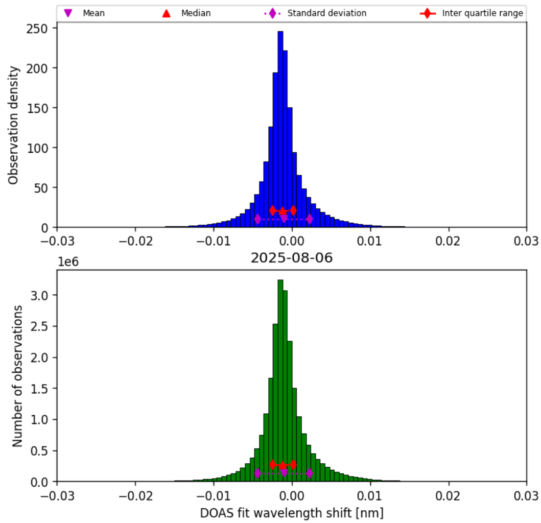
Figure 35: Histogram of “DOAS fit wavelength shift” for 2025-08-06 to 2025-08-07
