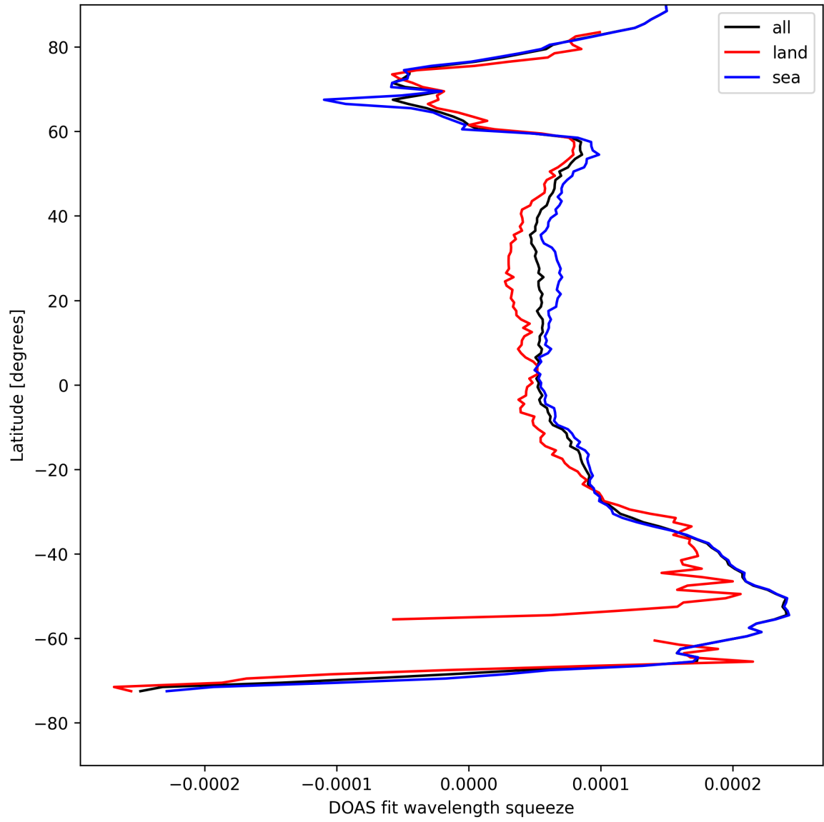
Figure 24: Zonal average of “DOAS fit wavelength squeeze” for 2025-08-06 to 2025-08-07.
