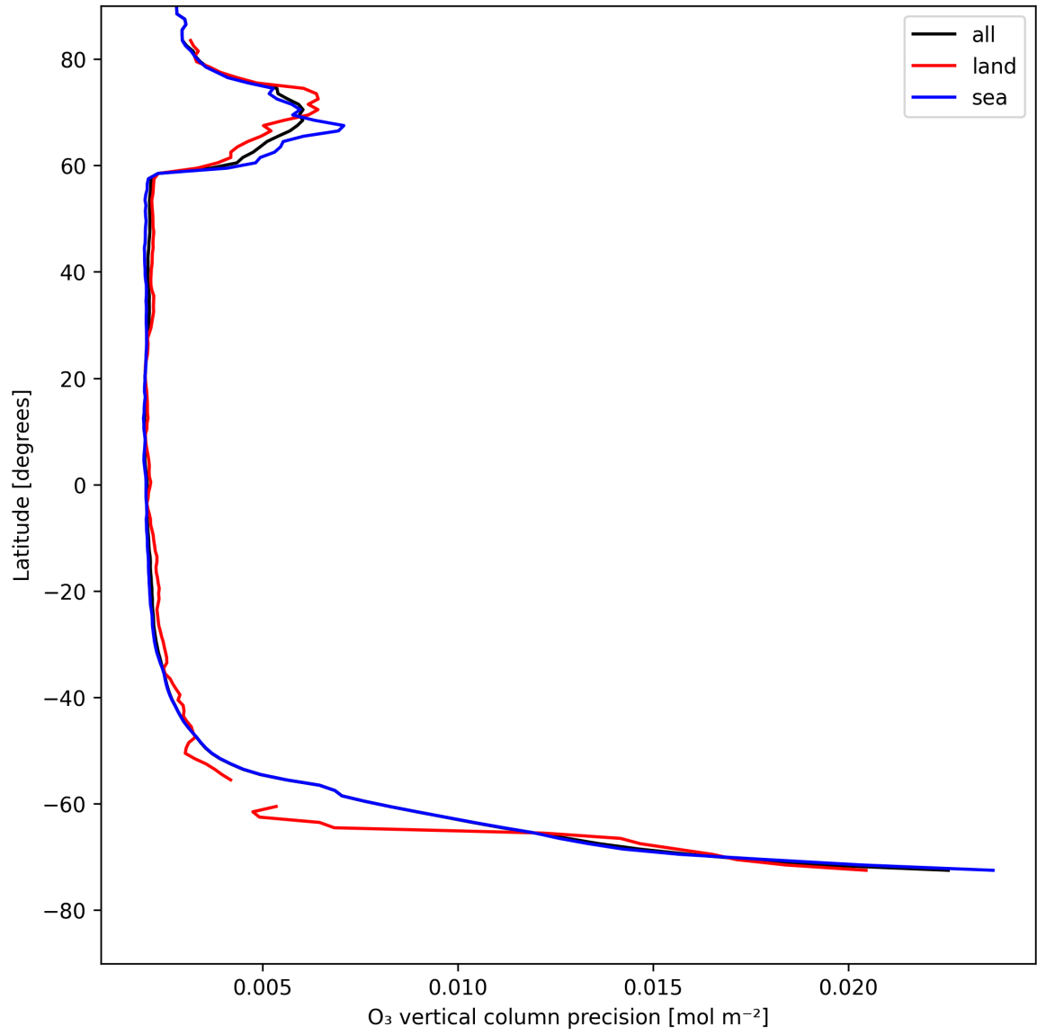
Figure 18: Zonal average of “O 3 vertical column precision” for 2025-08-06 to 2025-08-07.
