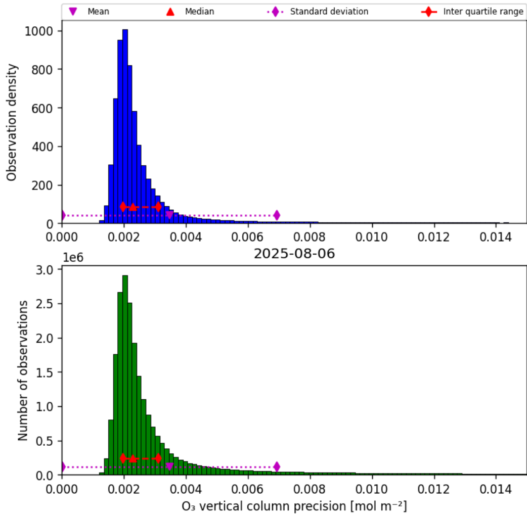
Figure 30: Histogram of “O 3 vertical column precision” for 2025-08-06 to 2025-08-07
