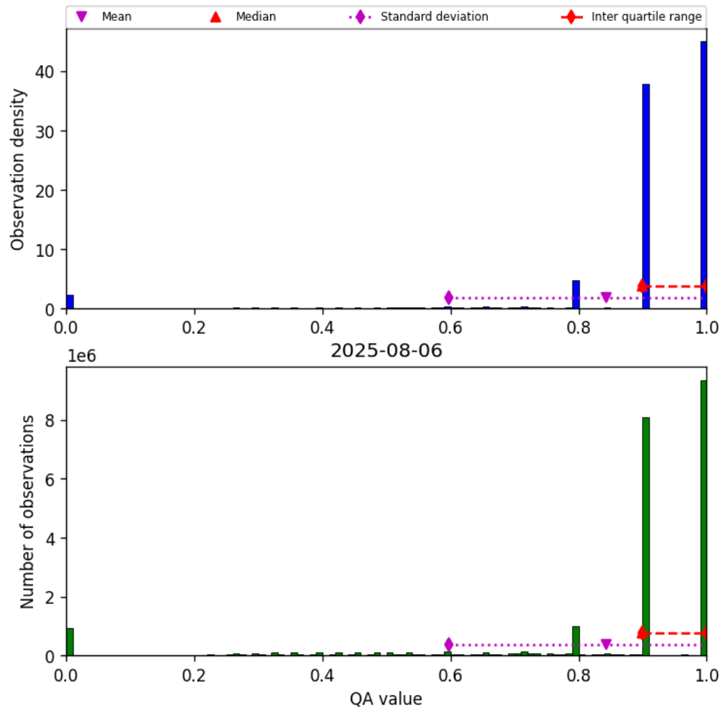
Figure 28: Histogram of “QA value” for 2025-08-06 to 2025-08-07
