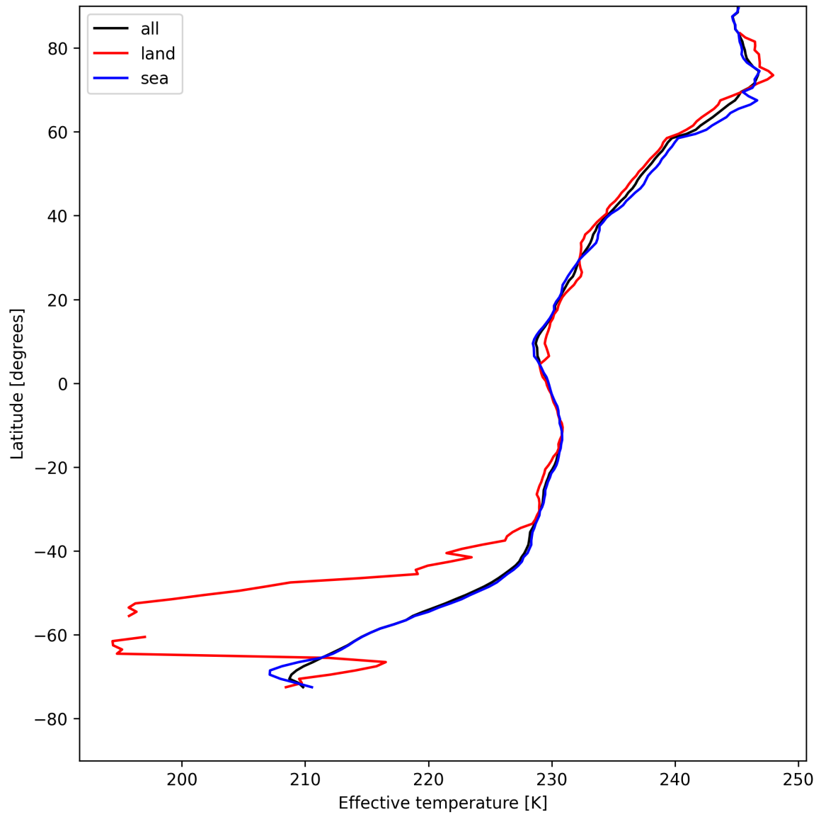
Figure 26: Zonal average of "Effective temperature" for 2025-08-06 to 2025-08-07.
