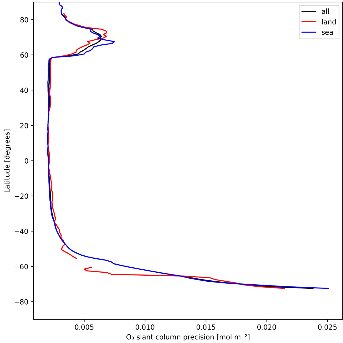
Figure 20: Zonal average of “O 3 slant column precision” for 2025-08-06 to 2025-08-07.
