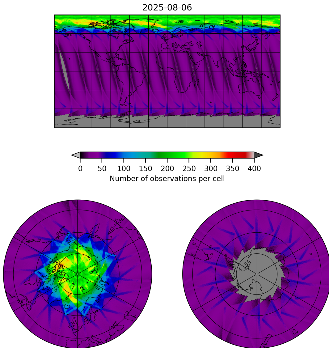
Figure 15: Map of the number of observations for 2025-08-06 to 2025-08-07
