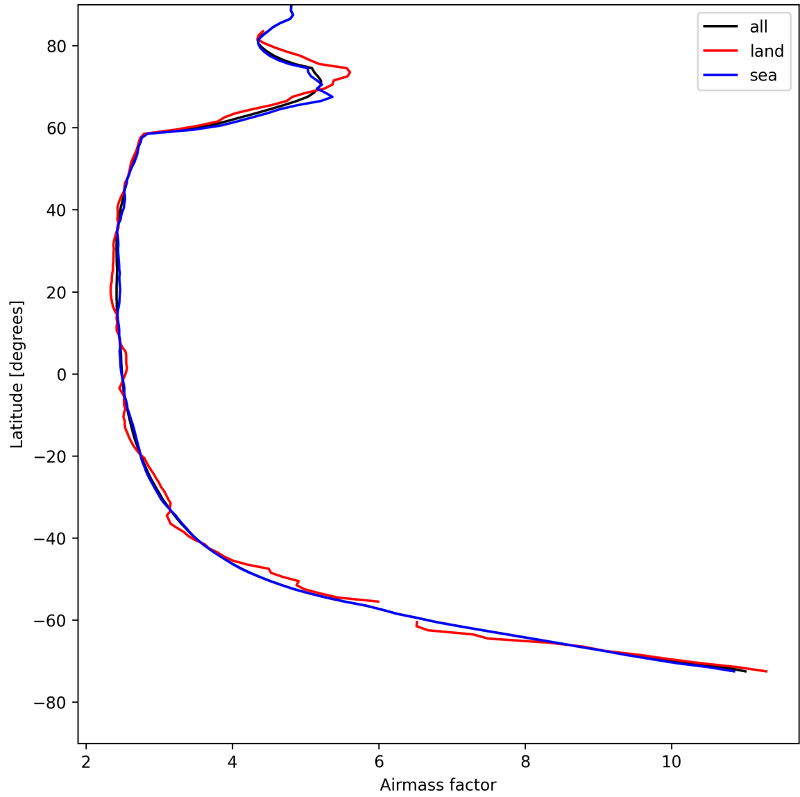
Figure 25: Zonal average of “Airmass factor” for 2025-08-06 to 2025-08-07.
