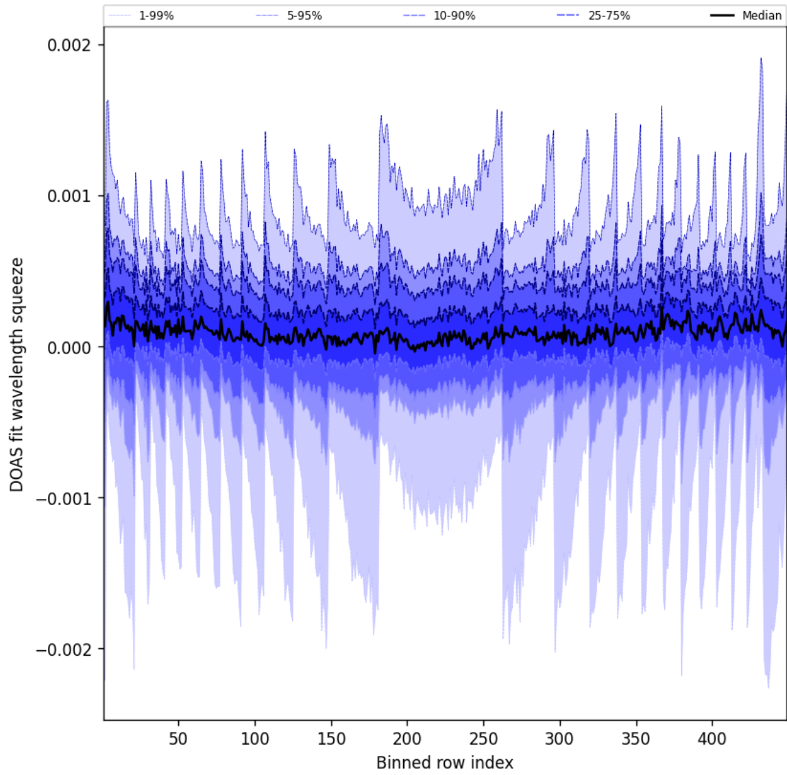
Figure 48: Along track statistics of “DOAS fit wavelength squeeze” for 2025-08-06 to 2025-08-07
