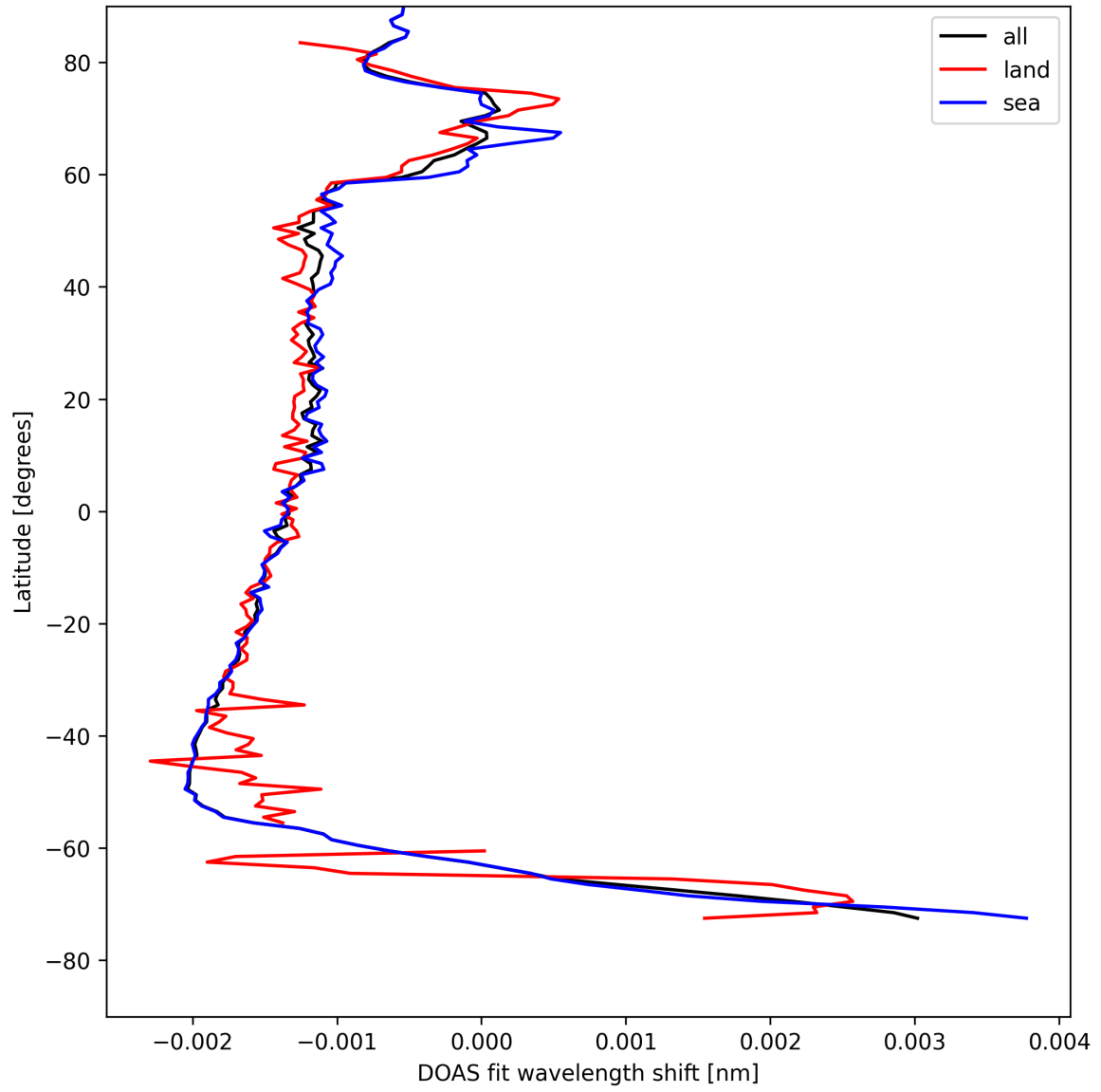
Figure 23: Zonal average of “DOAS fit wavelength shift” for 2025-08-06 to 2025-08-07.
