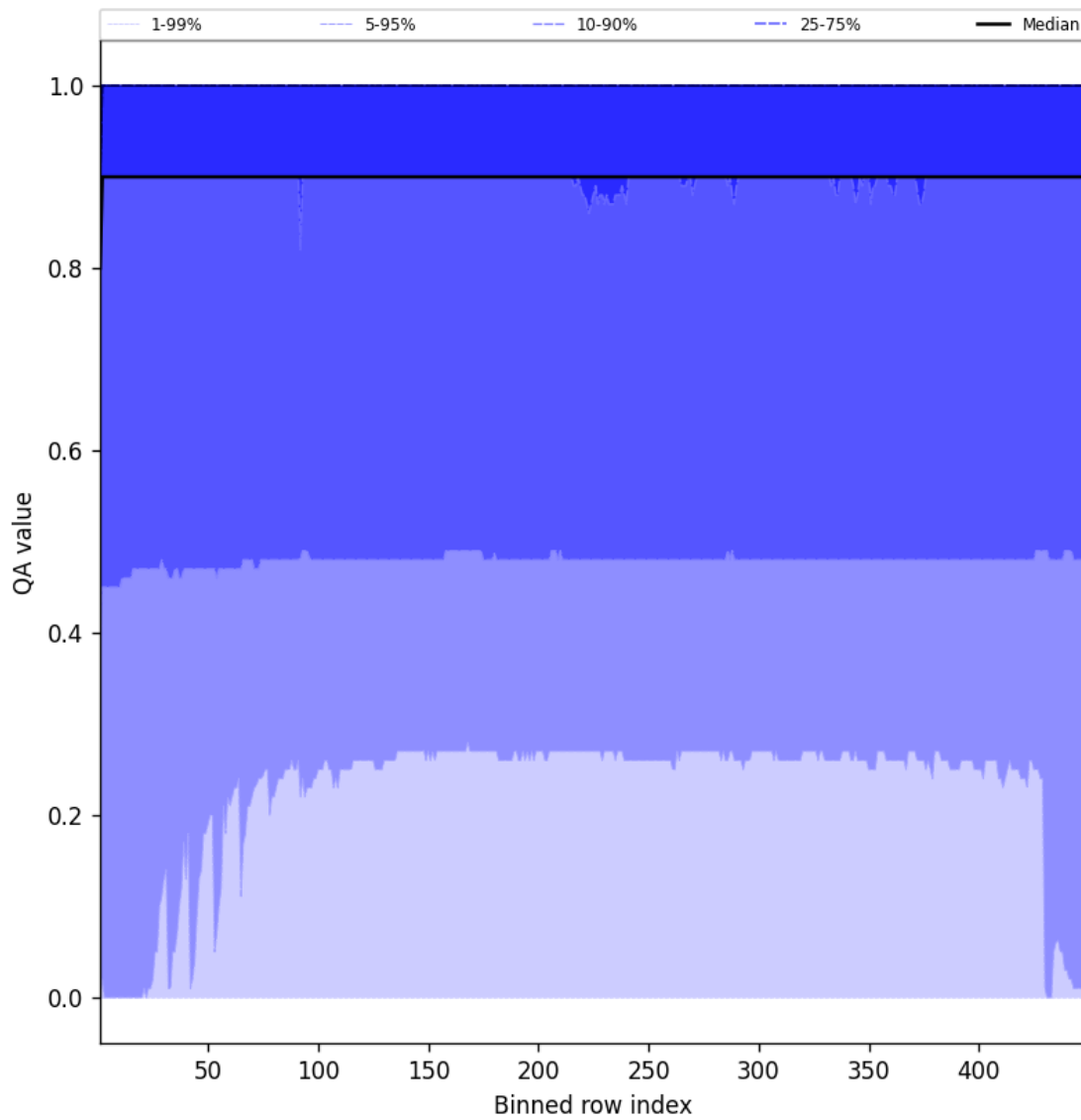
Figure 40: Along track statistics of “QA value” for 2025-08-06 to 2025-08-07
