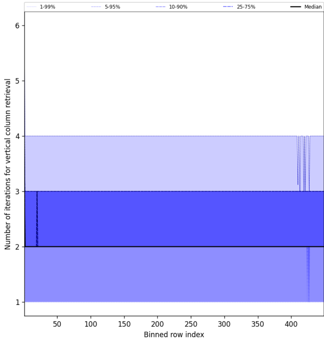
Figure 51: Along track statistics of “Number of iterations for vertical column retrieval” for 2025-08-06 to 2025-08-07
