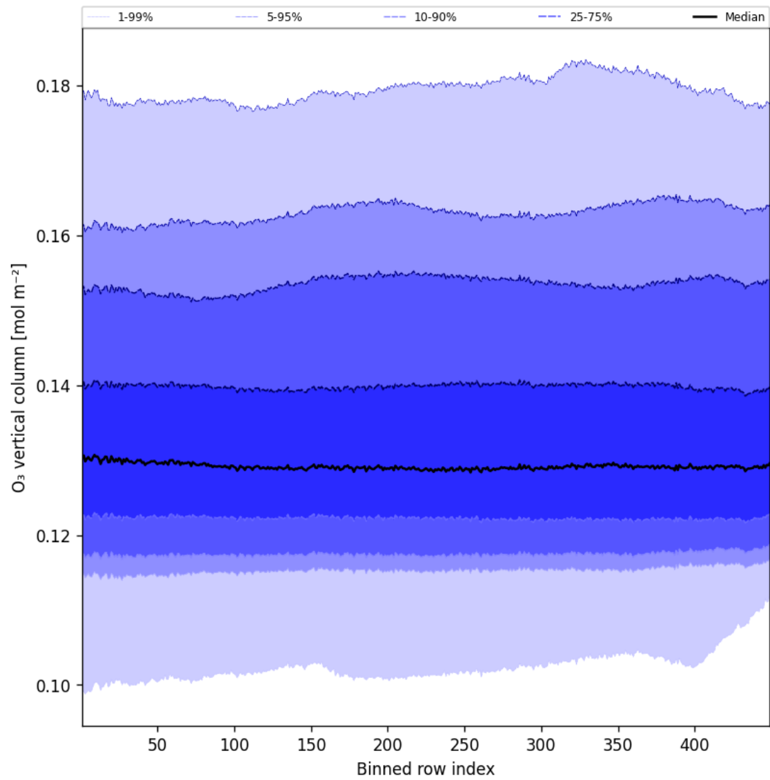
Figure 41: Along track statistics of “O 3 vertical column” for 2025-08-06 to 2025-08-07
