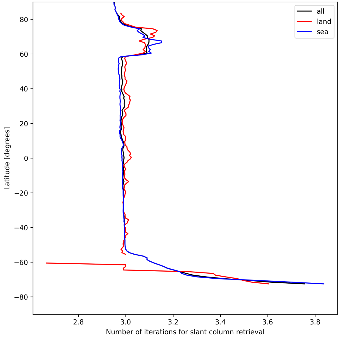
Figure 21: Zonal average of “Number of iterations for slant column retrieval” for 2025-08-06 to 2025-08-07.
