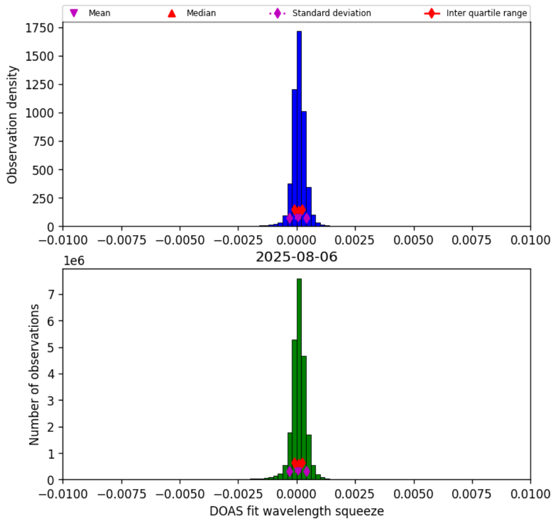
Figure 36: Histogram of “DOAS fit wavelength squeeze” for 2025-08-06 to 2025-08-07
