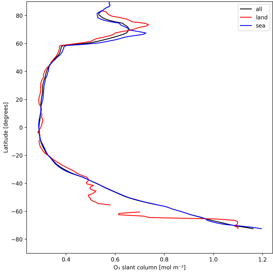
Figure 19: Zonal average of “O 3 slant column” for 2025-08-06 to 2025-08-07.
