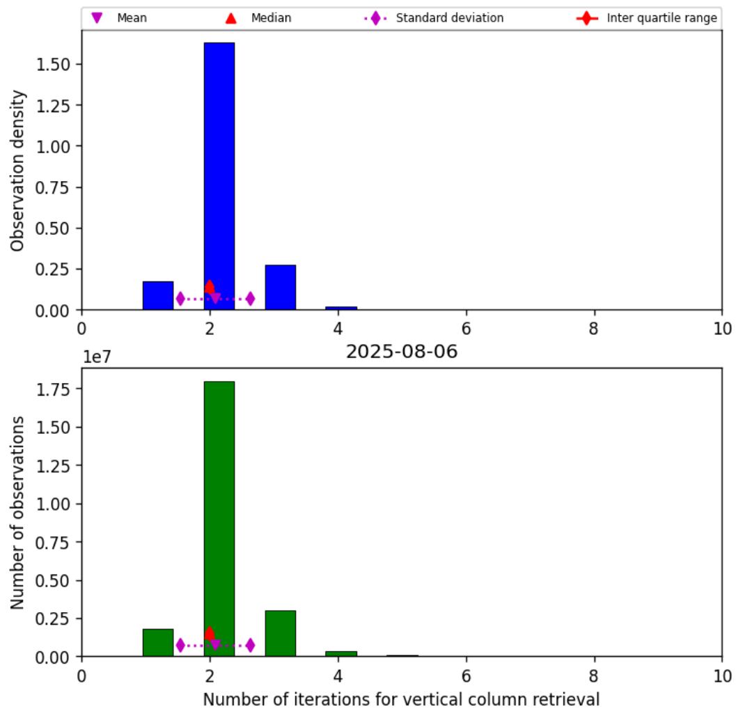
Figure 39: Histogram of “Number of iterations for vertical column retrieval” for 2025-08-06 to 2025-08-07
