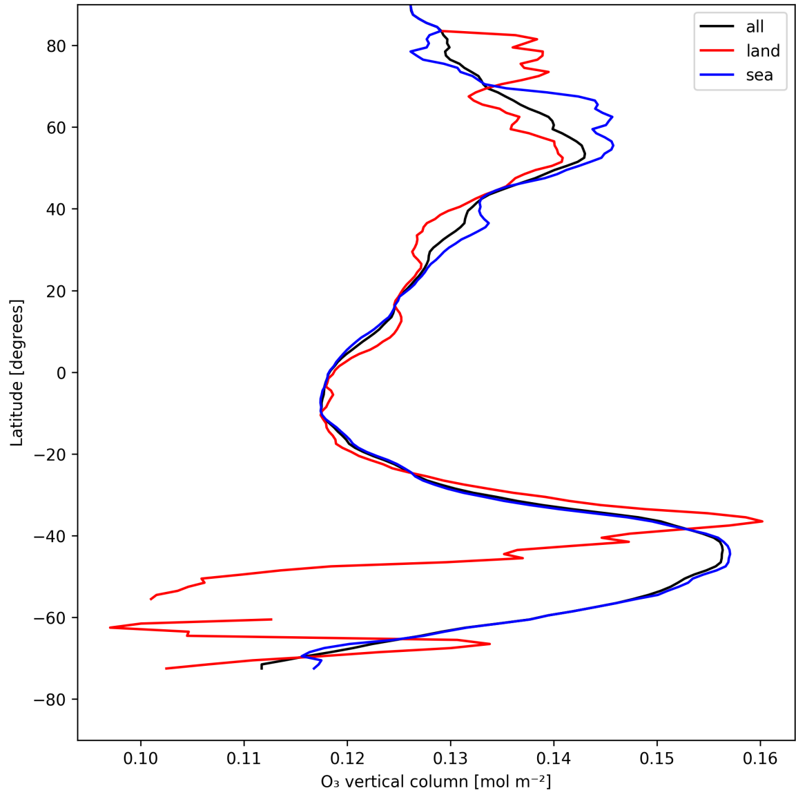
Figure 17: Zonal average of “O 3 vertical column” for 2025-08-06 to 2025-08-07.
