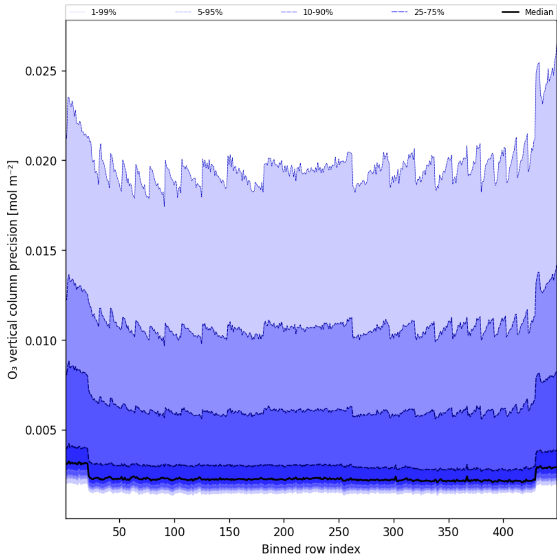
Figure 42: Along track statistics of “O 3 vertical column precision” for 2025-08-06 to 2025-08-07
