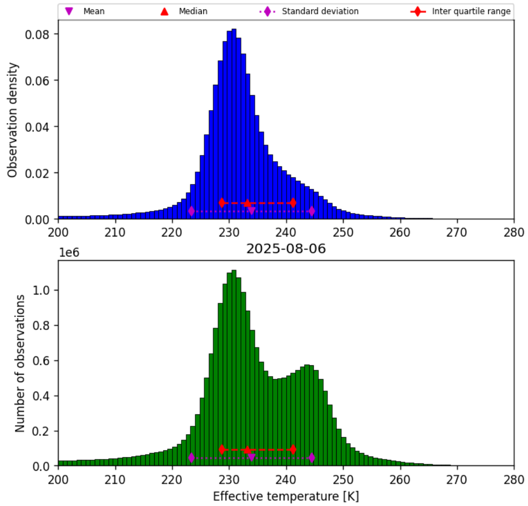
Figure 38: Histogram of “Effective temperature” for 2025-08-06 to 2025-08-07
