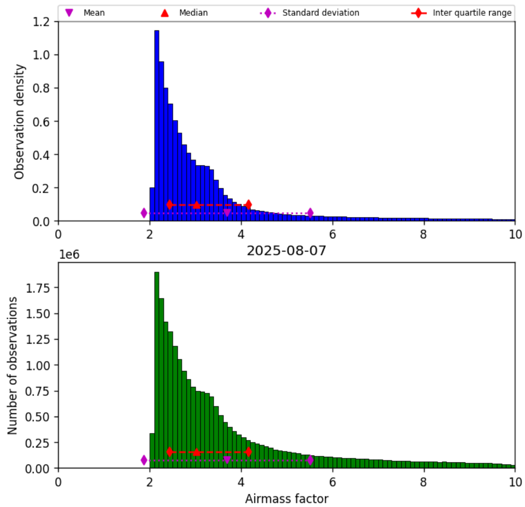
Figure 37: Histogram of “Airmass factor” for 2025-08-07 to 2025-08-07
