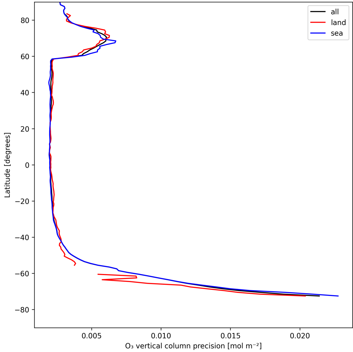
Figure 18: Zonal average of “O 3 vertical column precision” for 2025-08-07 to 2025-08-07.
