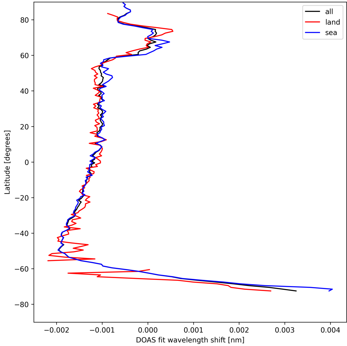
Figure 23: Zonal average of "DOAS fit wavelength shift" for 2025-08-07 to 2025-08-07.
