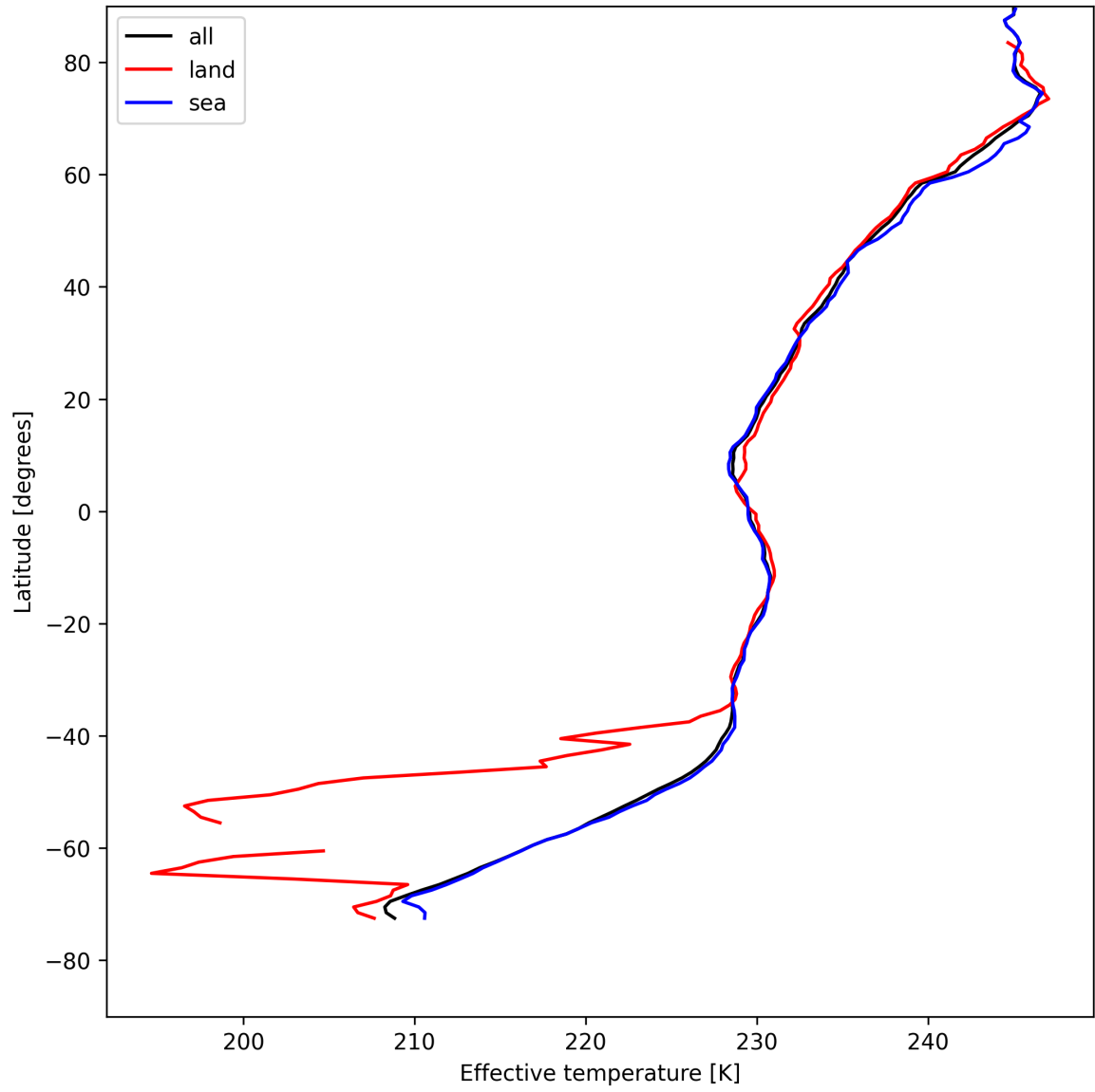
Figure 26: Zonal average of “Effective temperature” for 2025-08-07 to 2025-08-07.
