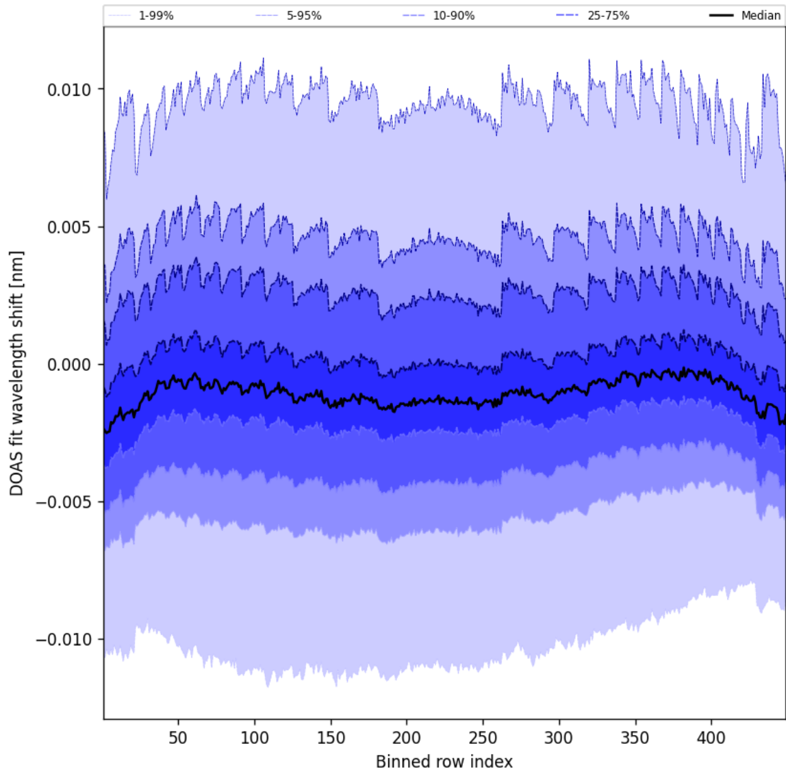
Figure 47: Along track statistics of "DOAS fit wavelength shift" for 2025-08-07 to 2025-08-07
