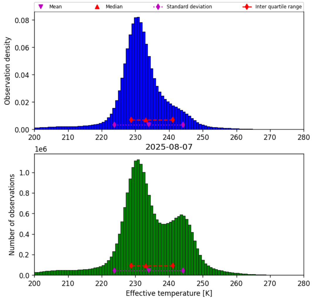
Figure 38: Histogram of “Effective temperature” for 2025-08-07 to 2025-08-07
