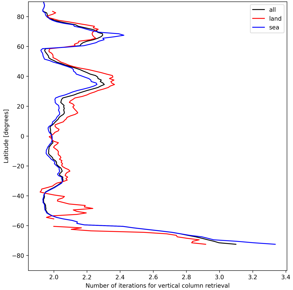
Figure 27: Zonal average of “Number of iterations for vertical column retrieval” for 2025-08-07 to 2025-08-07.
