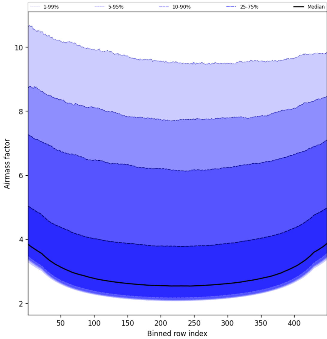
Figure 49: Along track statistics of “Airmass factor” for 2025-08-07 to 2025-08-07
