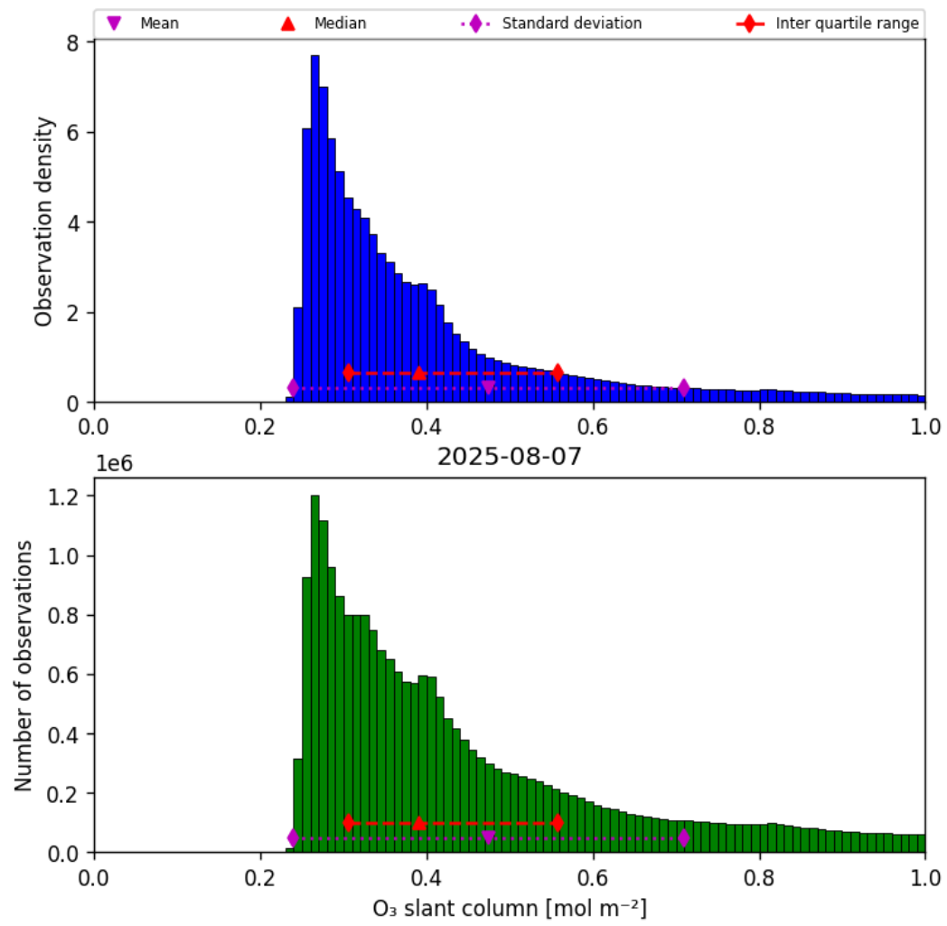
Figure 31: Histogram of “O 3 slant column” for 2025-08-07 to 2025-08-07
