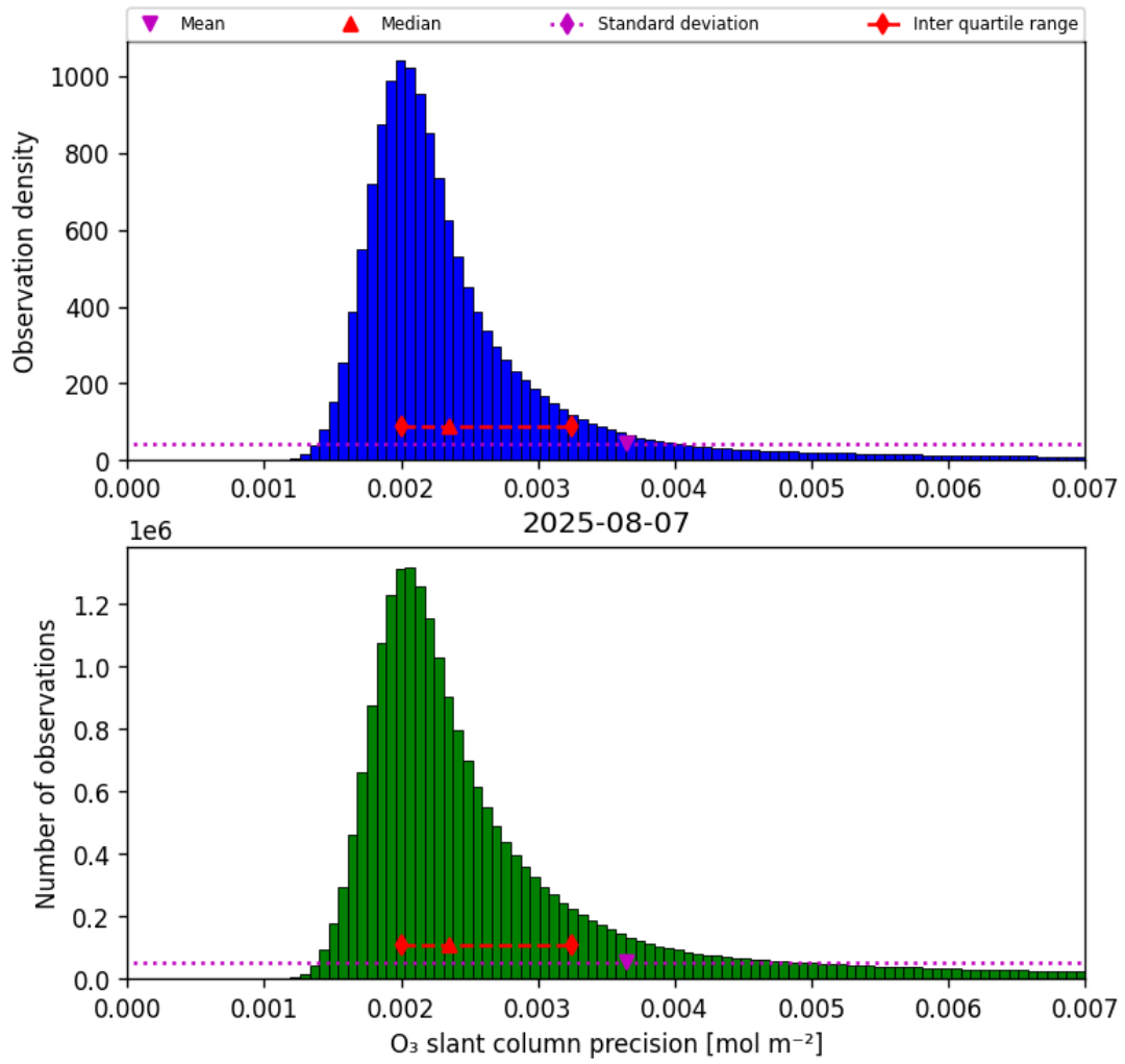
Figure 32: Histogram of “O 3 slant column precision” for 2025-08-07 to 2025-08-07
