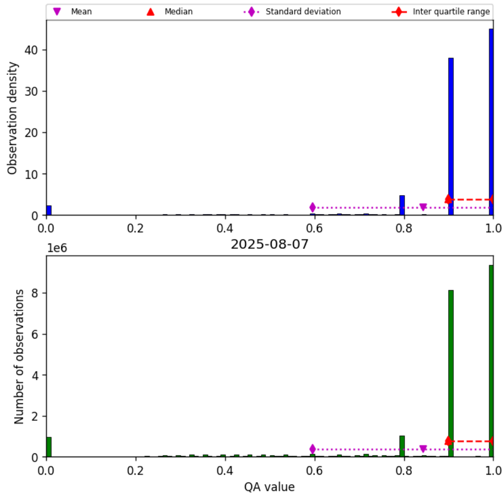
Figure 28: Histogram of “QA value” for 2025-08-07 to 2025-08-07
