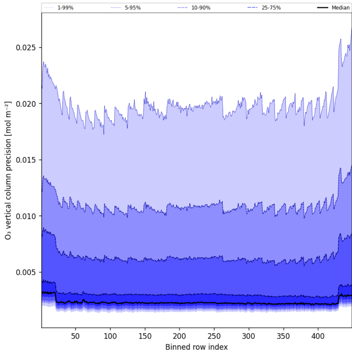
Figure 42: Along track statistics of “O 3 vertical column precision” for 2025-08-07 to 2025-08-07
