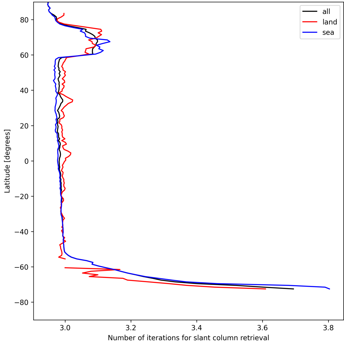
Figure 21: Zonal average of “Number of iterations for slant column retrieval” for 2025-08-07 to 2025-08-07.
