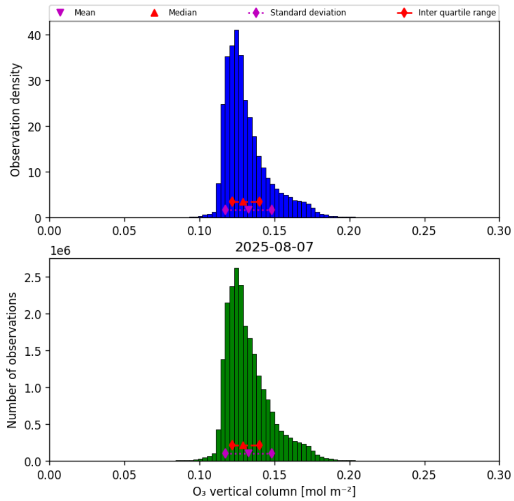
Figure 29: Histogram of “O 3 vertical column” for 2025-08-07 to 2025-08-07
