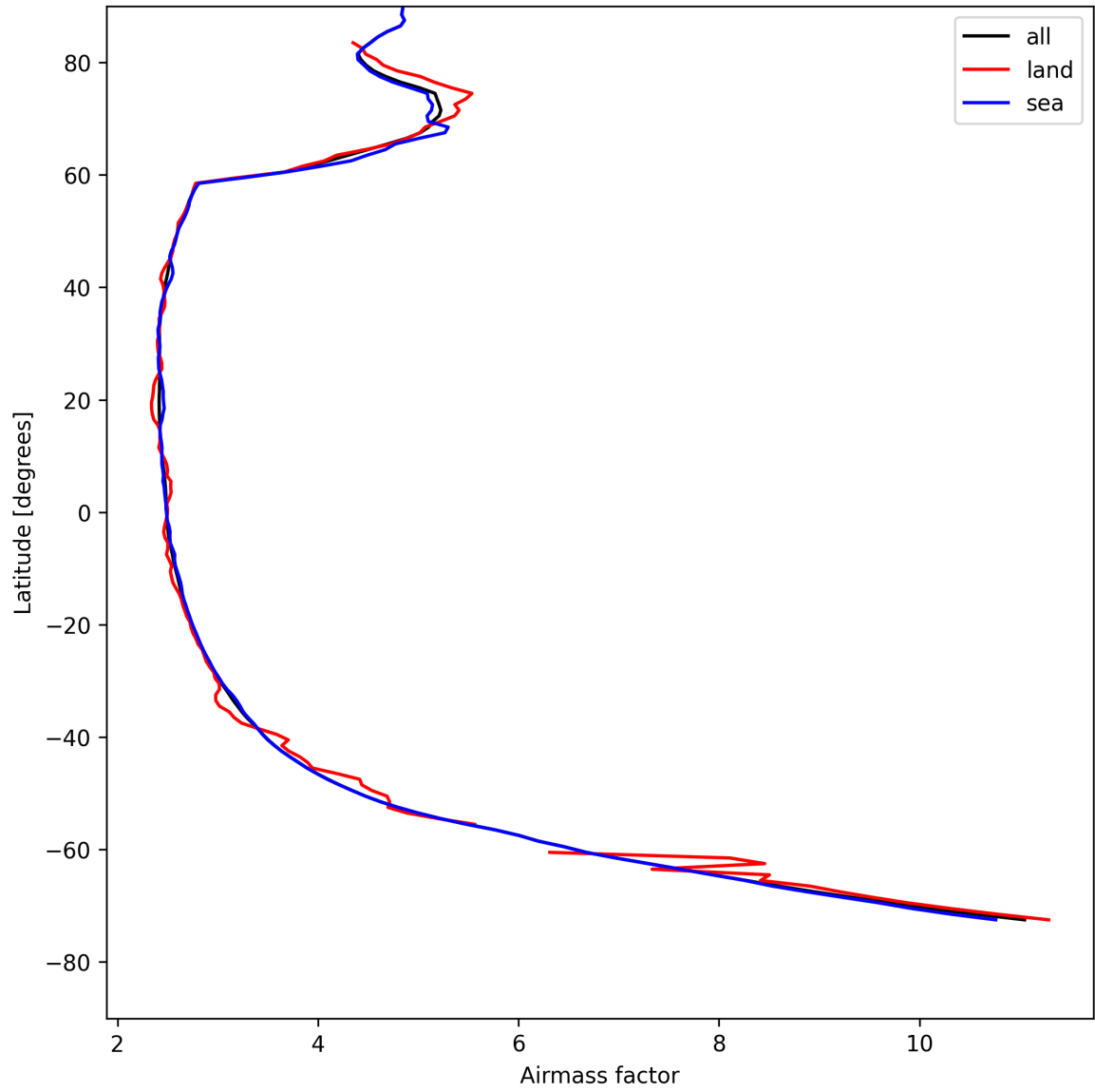
Figure 25: Zonal average of “Airmass factor” for 2025-08-07 to 2025-08-07.
