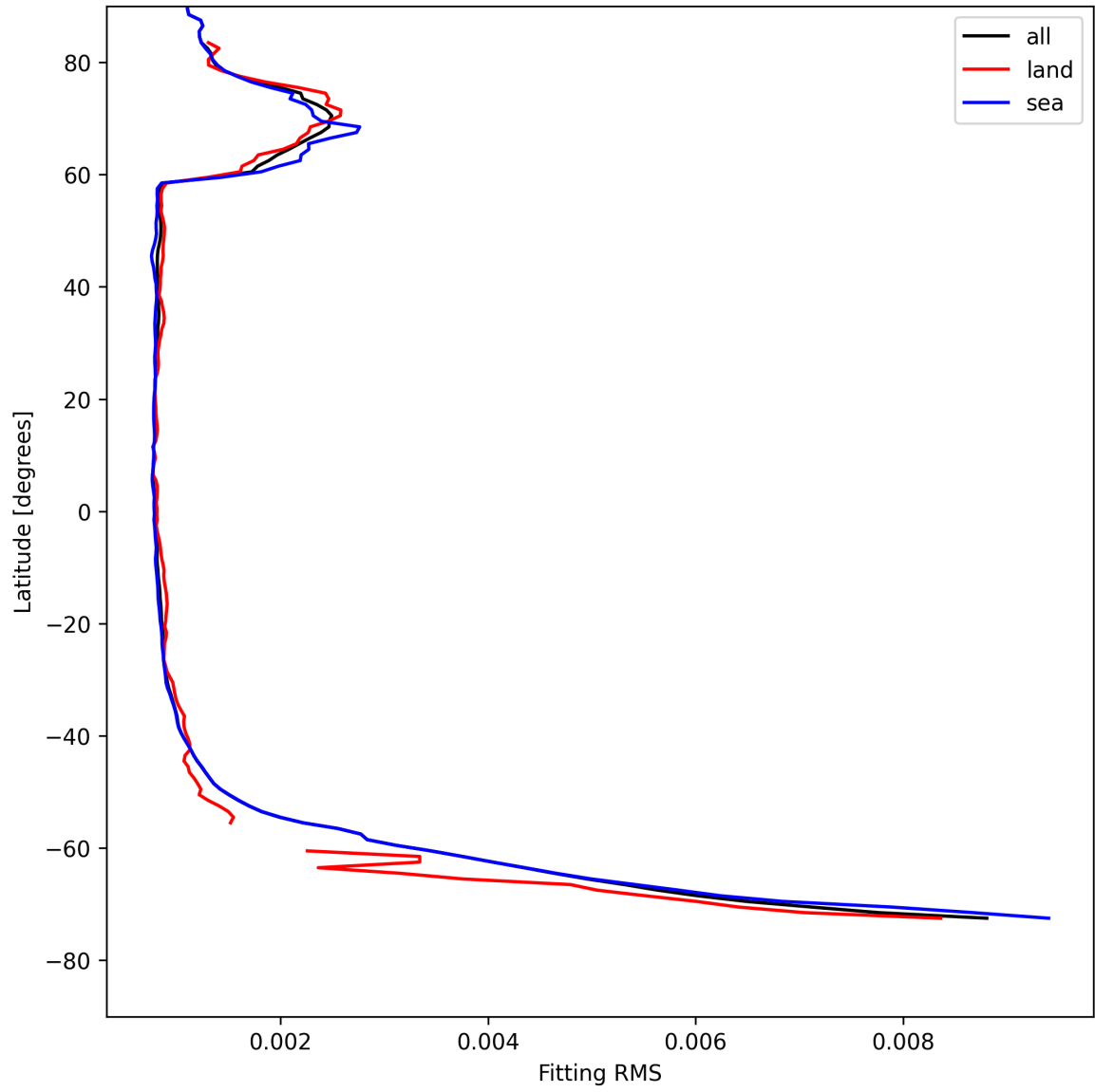
Figure 22: Zonal average of “Fitting RMS” for 2025-08-07 to 2025-08-07.
