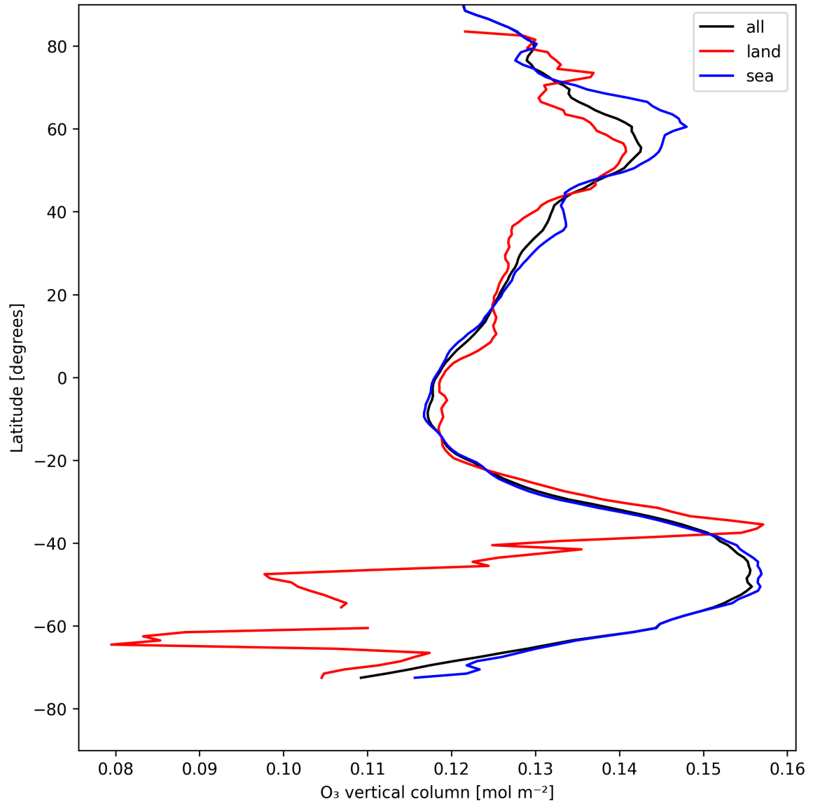
Figure 17: Zonal average of “O 3 vertical column” for 2025-08-07 to 2025-08-07.
