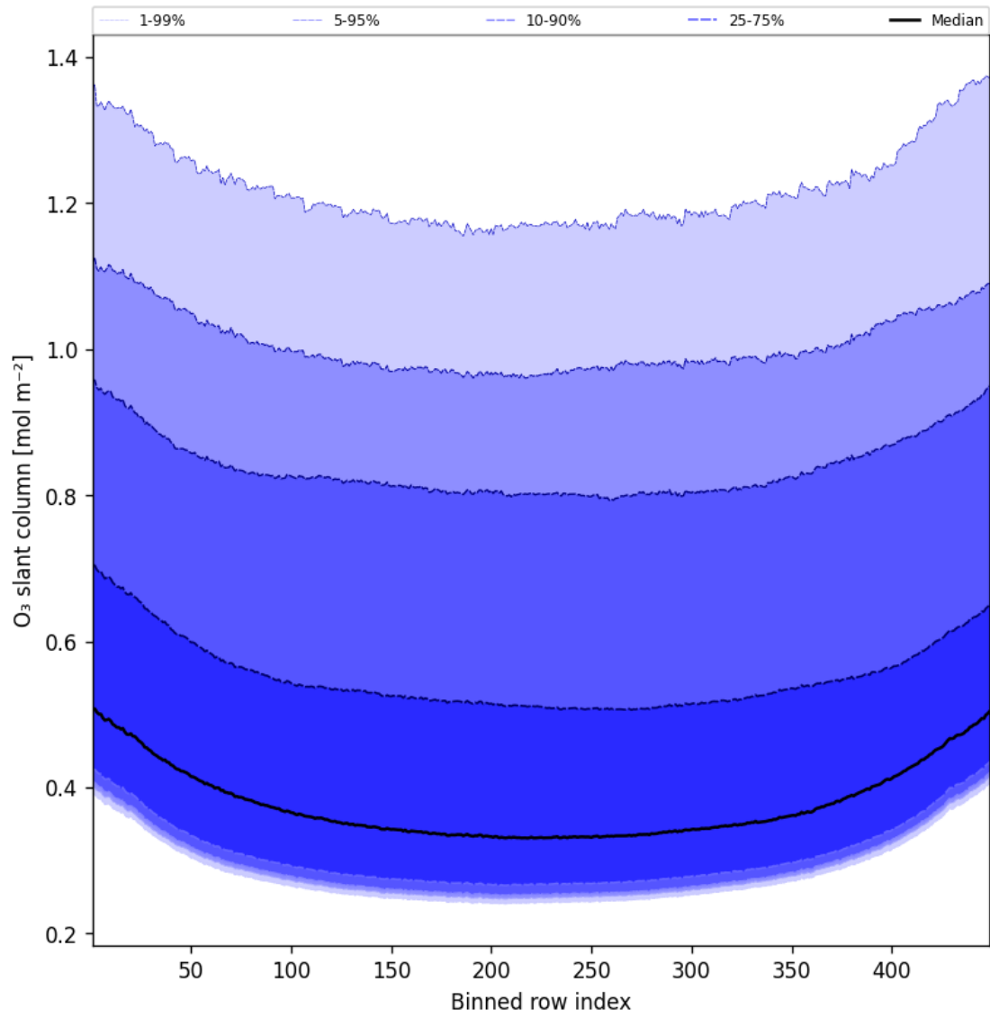
Figure 43: Along track statistics of “O 3 slant column” for 2025-08-07 to 2025-08-07
