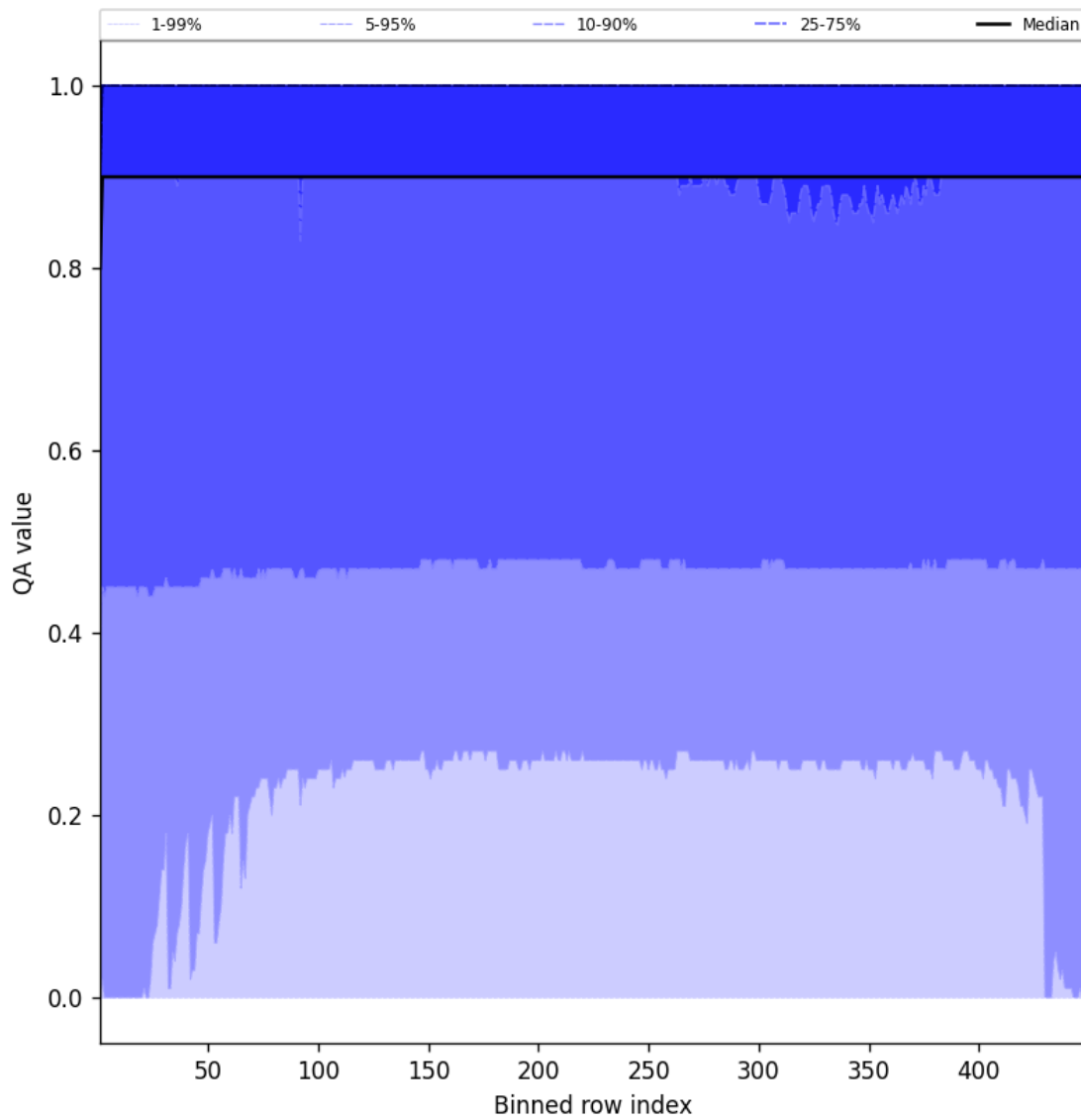
Figure 40: Along track statistics of “QA value” for 2025-08-07 to 2025-08-07
