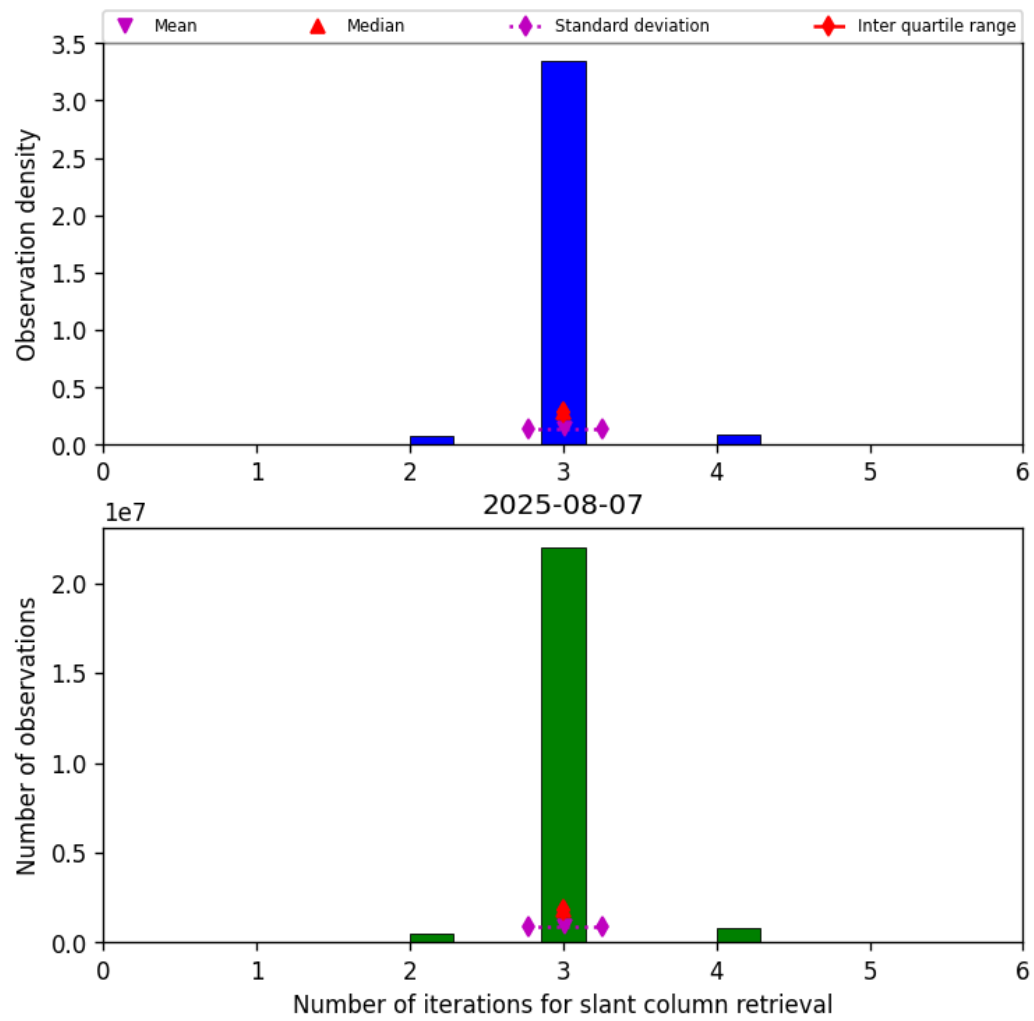
Figure 33: Histogram of “Number of iterations for slant column retrieval” for 2025-08-07 to 2025-08-07
