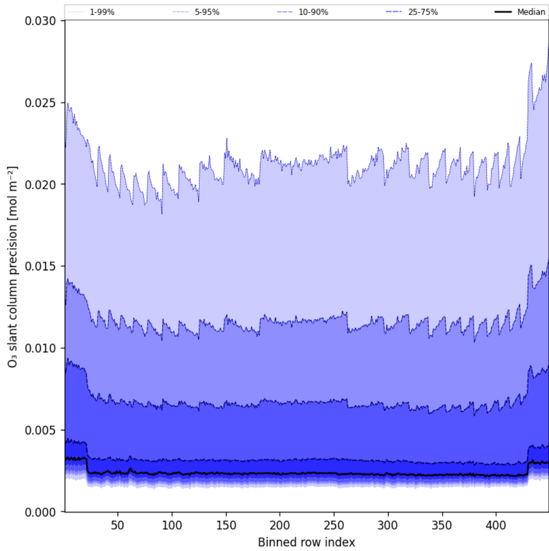
Figure 44: Along track statistics of “O 3 slant column precision” for 2025-08-07 to 2025-08-07
