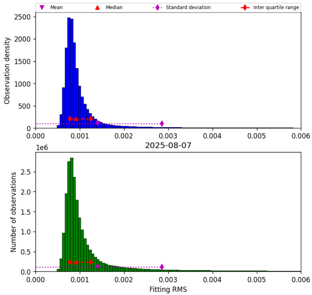
Figure 34: Histogram of “Fitting RMS” for 2025-08-07 to 2025-08-07
