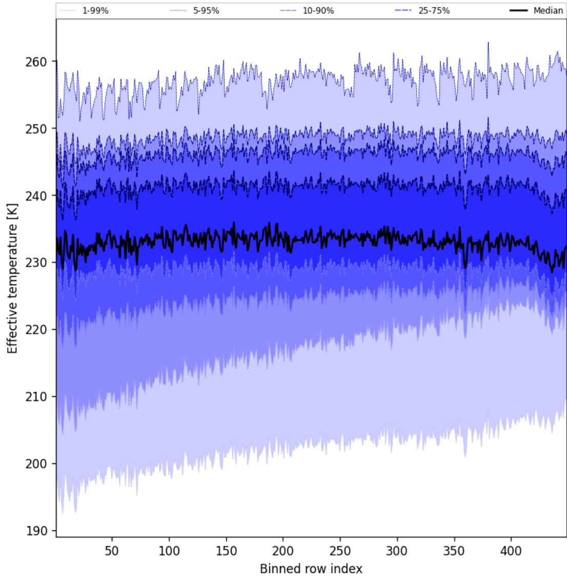
Figure 50: Along track statistics of "Effective temperature" for 2025-08-07 to 2025-08-07
