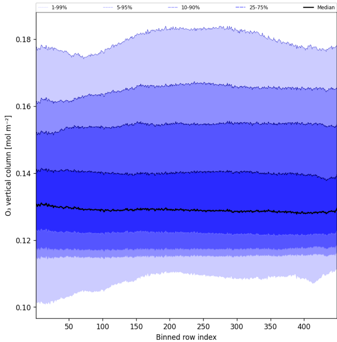
Figure 41: Along track statistics of “O 3 vertical column” for 2025-08-07 to 2025-08-07
