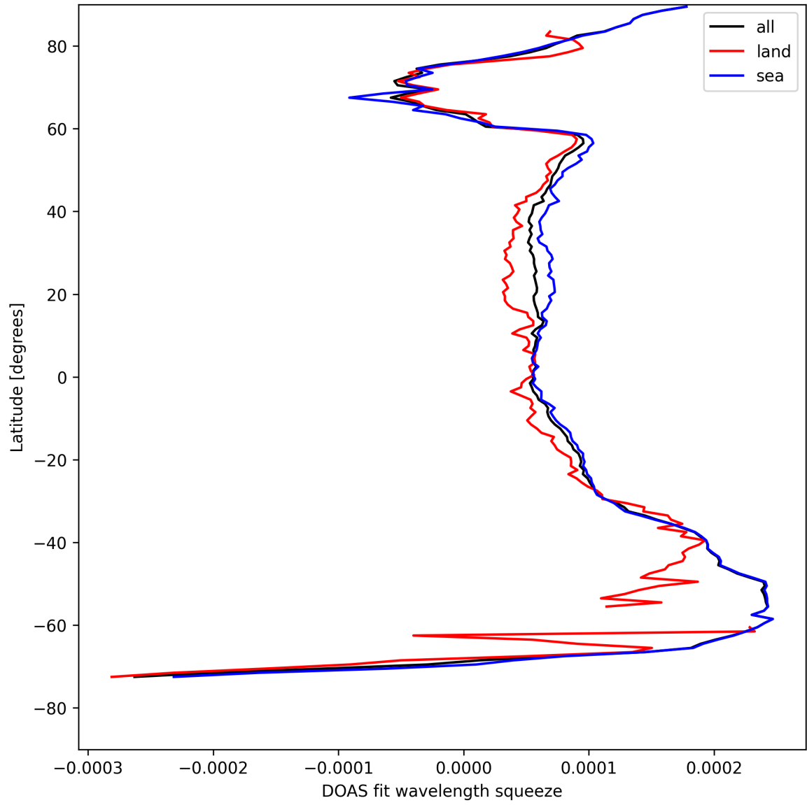
Figure 24: Zonal average of “DOAS fit wavelength squeeze” for 2025-08-07 to 2025-08-07.
