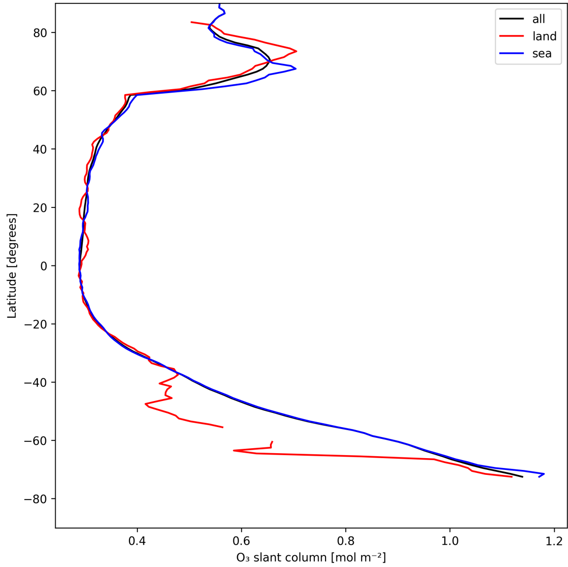
Figure 19: Zonal average of “O 3 slant column” for 2025-08-07 to 2025-08-07.
