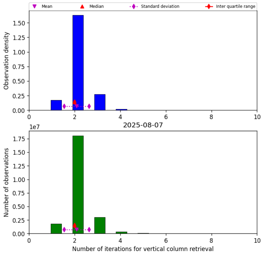
Figure 39: Histogram of “Number of iterations for vertical column retrieval” for 2025-08-07 to 2025-08-07
