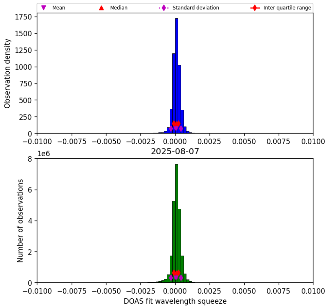
Figure 36: Histogram of “DOAS fit wavelength squeeze” for 2025-08-07 to 2025-08-07
