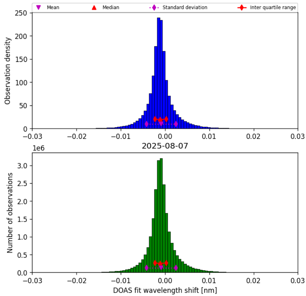
Figure 35: Histogram of “DOAS fit wavelength shift” for 2025-08-07 to 2025-08-07
