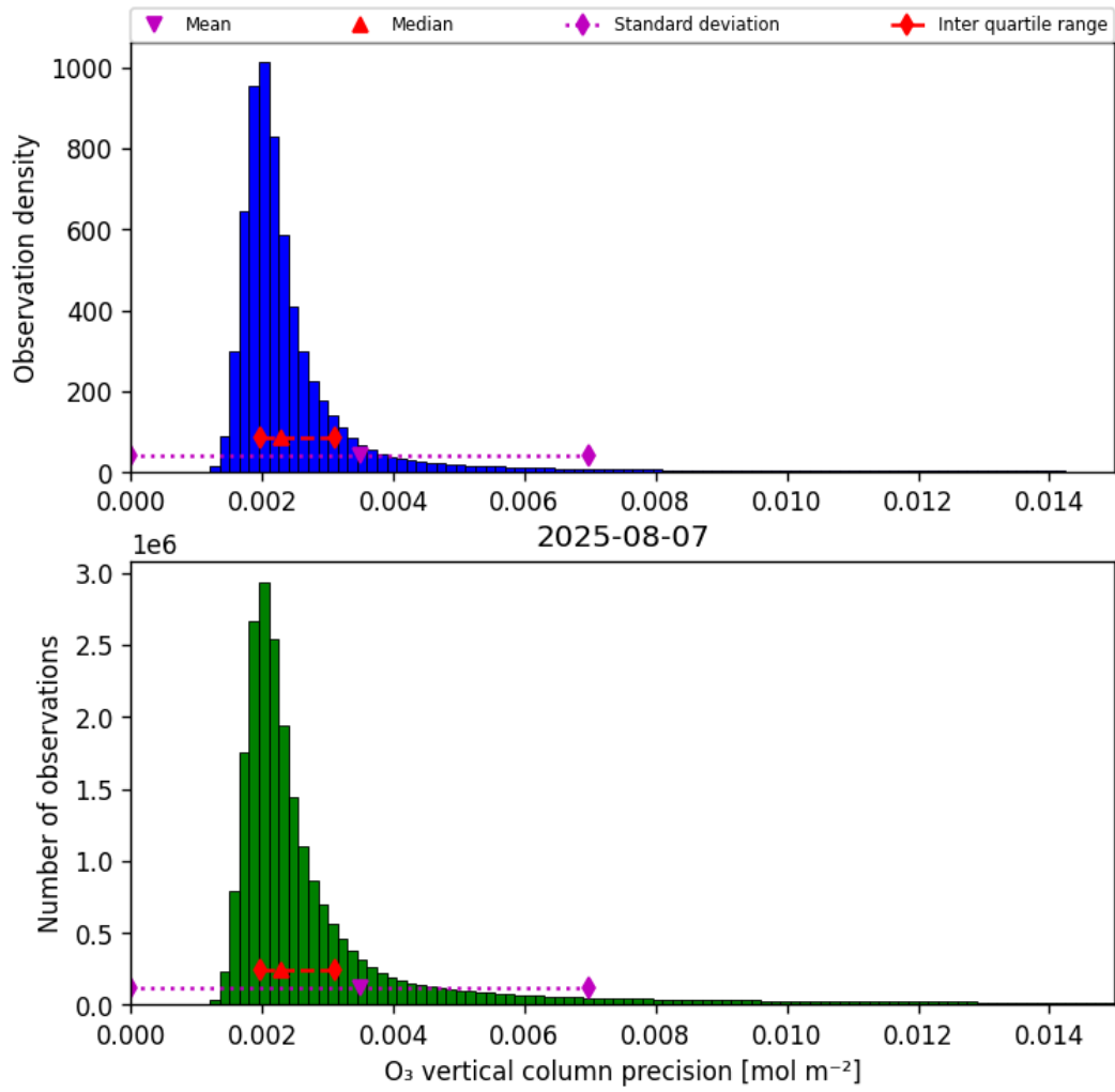
Figure 30: Histogram of “O 3 vertical column precision” for 2025-08-07 to 2025-08-07
