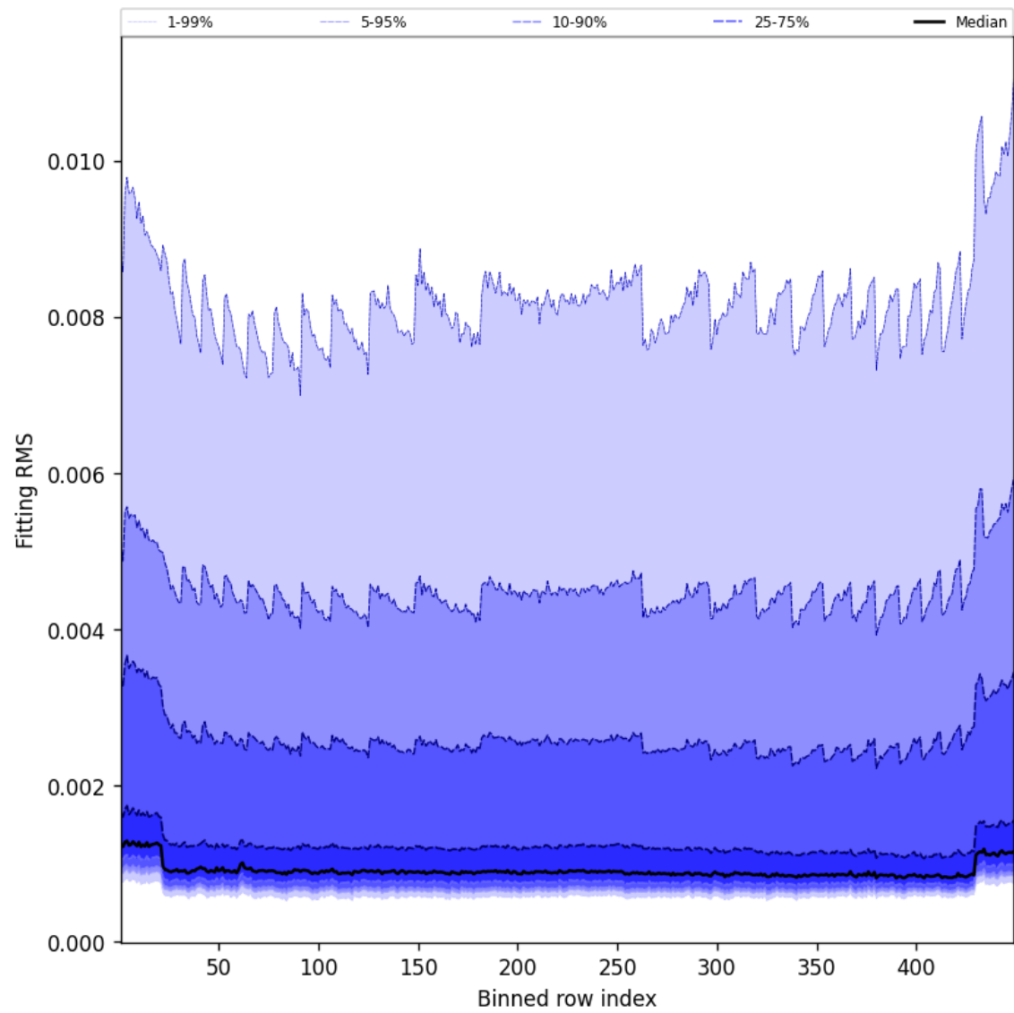
Figure 46: Along track statistics of “Fitting RMS” for 2025-08-07 to 2025-08-07
