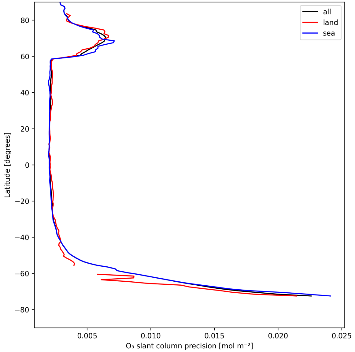
Figure 20: Zonal average of “O 3 slant column precision” for 2025-08-07 to 2025-08-07.
