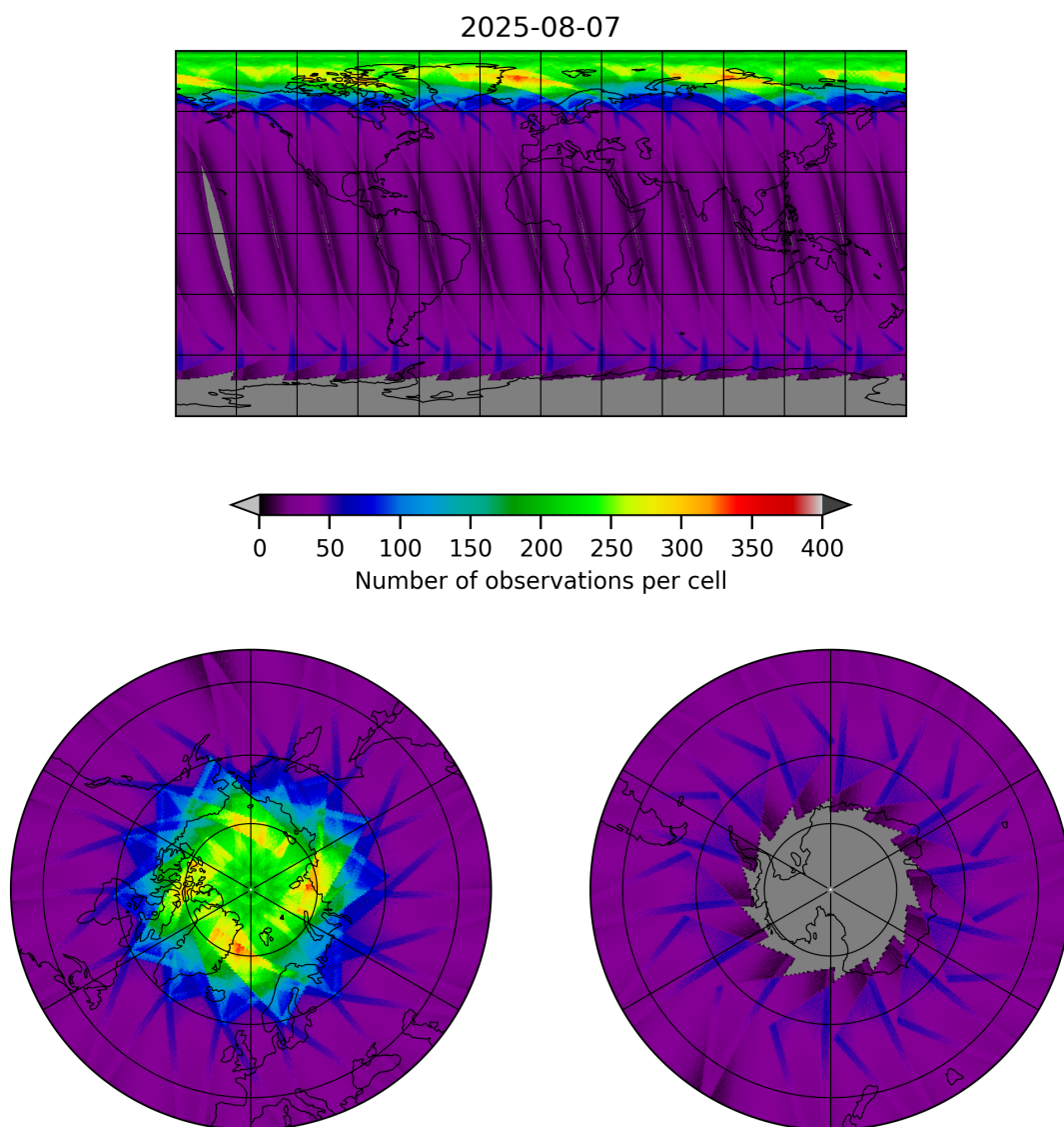
Figure 15: Map of the number of observations for 2025-08-07 to 2025-08-07
