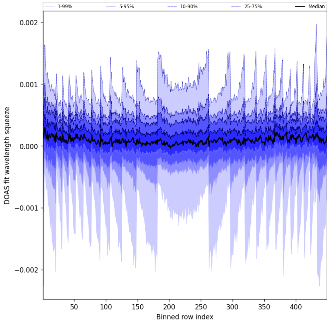
Figure 48: Along track statistics of “DOAS fit wavelength squeeze” for 2025-08-07 to 2025-08-07
