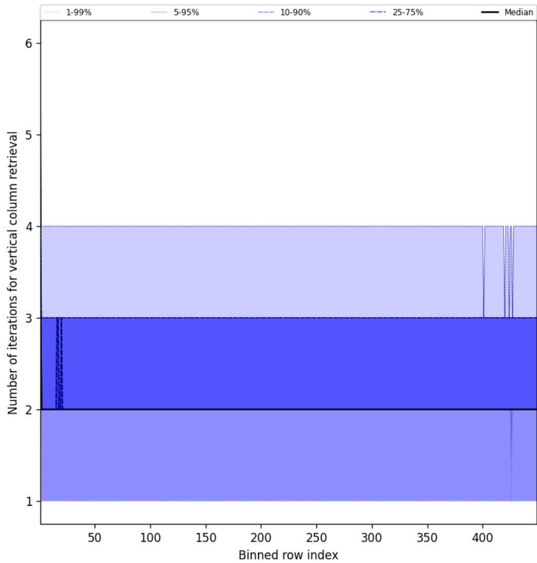
Figure 51: Along track statistics of “Number of iterations for vertical column retrieval” for 2025-08-07 to 2025-08-07
