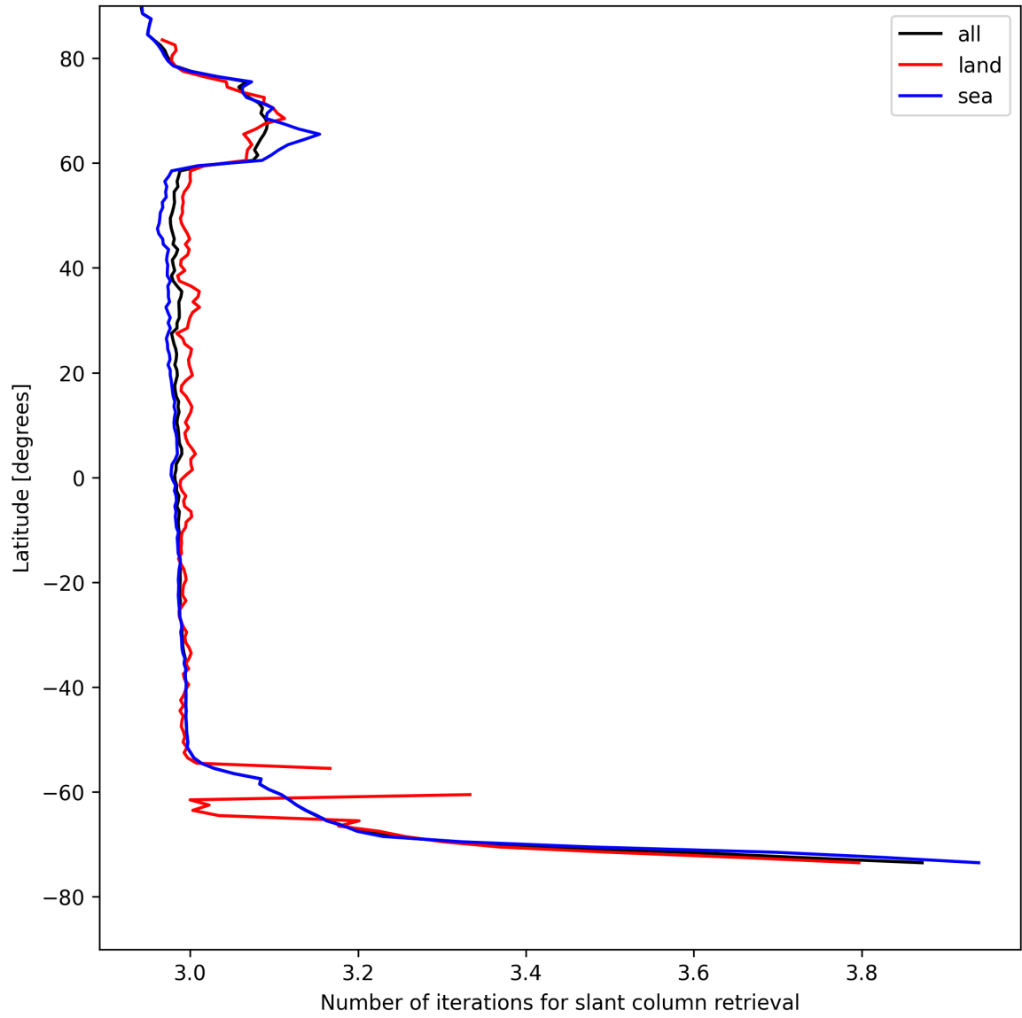
Figure 21: Zonal average of “Number of iterations for slant column retrieval” for 2025-08-09 to 2025-08-10.
