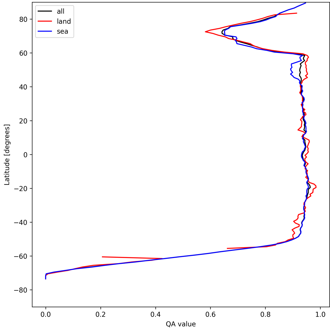
Figure 16: Zonal average of “QA value” for 2025-08-09 to 2025-08-10.
