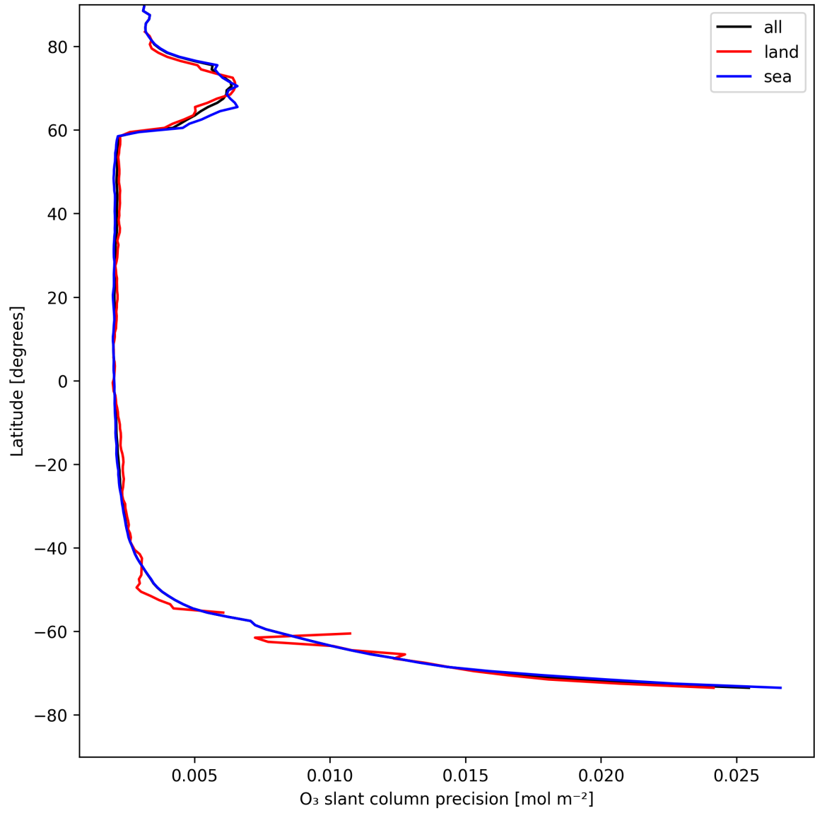
Figure 20: Zonal average of "O 3 slant column precision" for 2025-08-09 to 2025-08-10.
