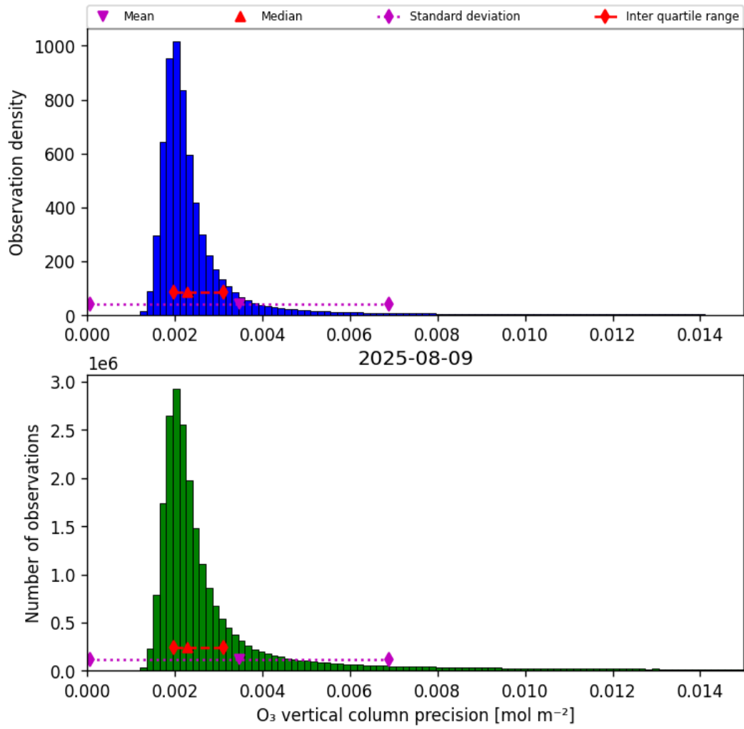
Figure 30: Histogram of “O 3 vertical column precision” for 2025-08-09 to 2025-08-10
