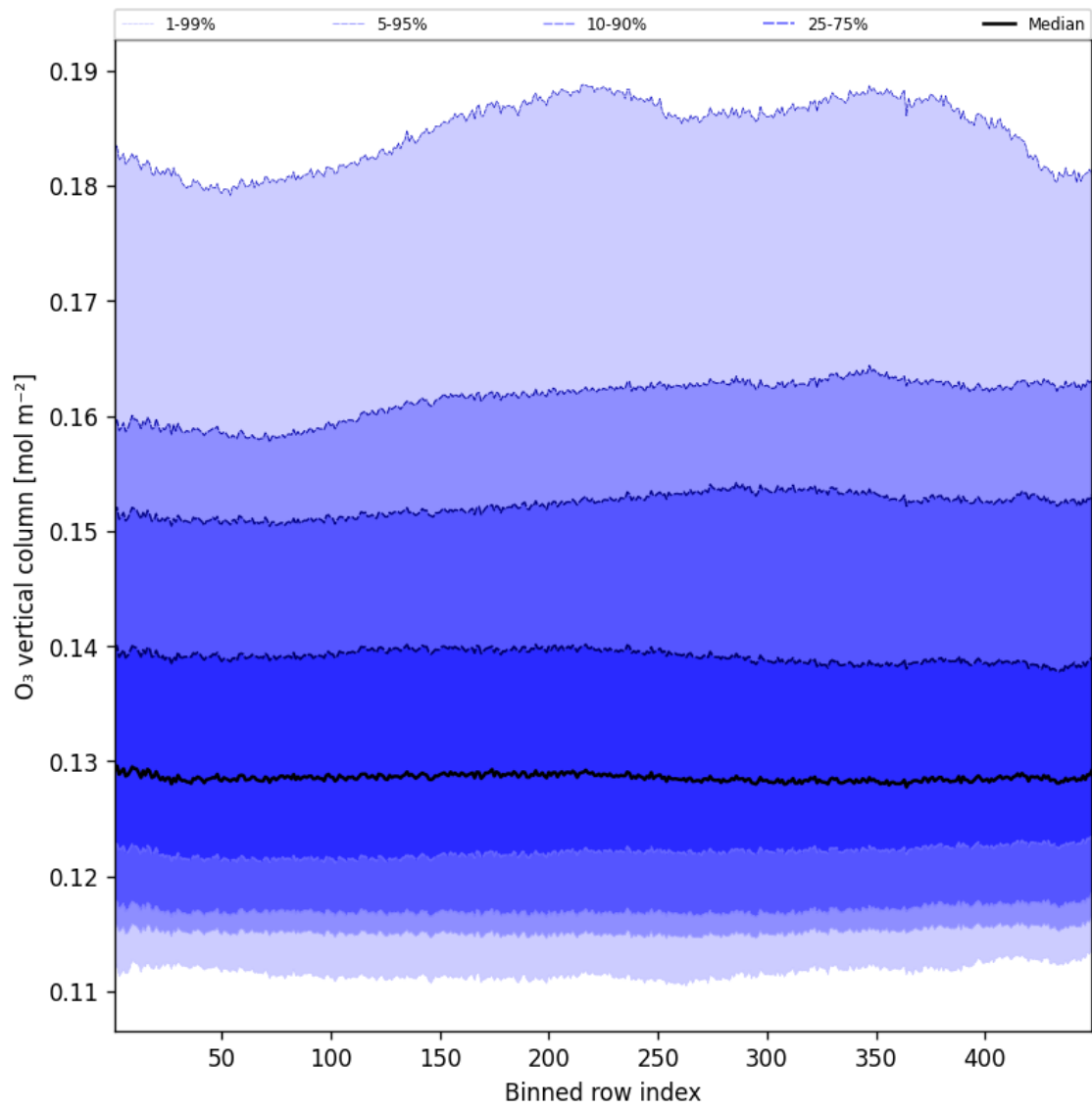
Figure 41: Along track statistics of “O 3 vertical column” for 2025-08-09 to 2025-08-10
