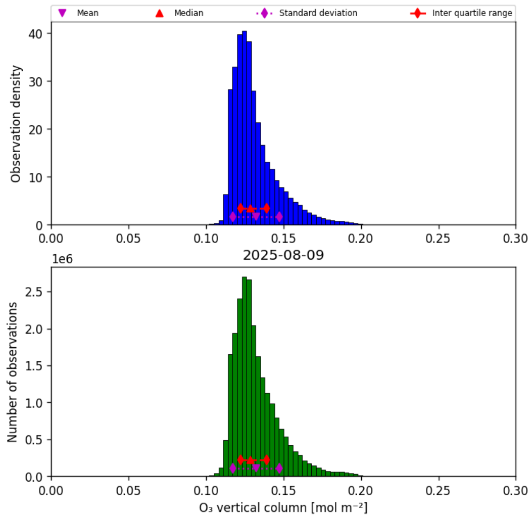
Figure 29: Histogram of “O 3 vertical column” for 2025-08-09 to 2025-08-10
