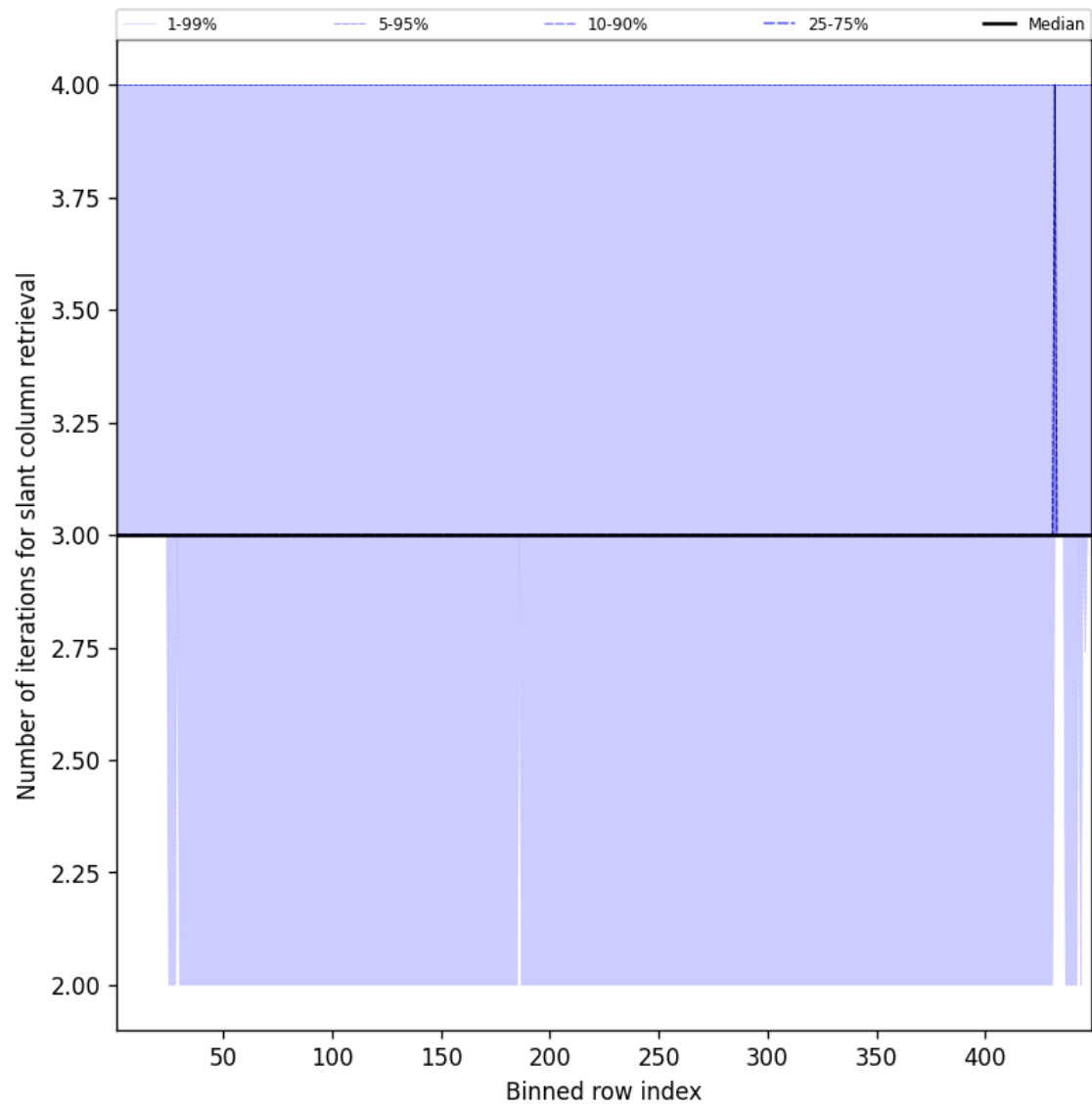
Figure 45: Along track statistics of “Number of iterations for slant column retrieval” for 2025-08-09 to 2025-08-10
