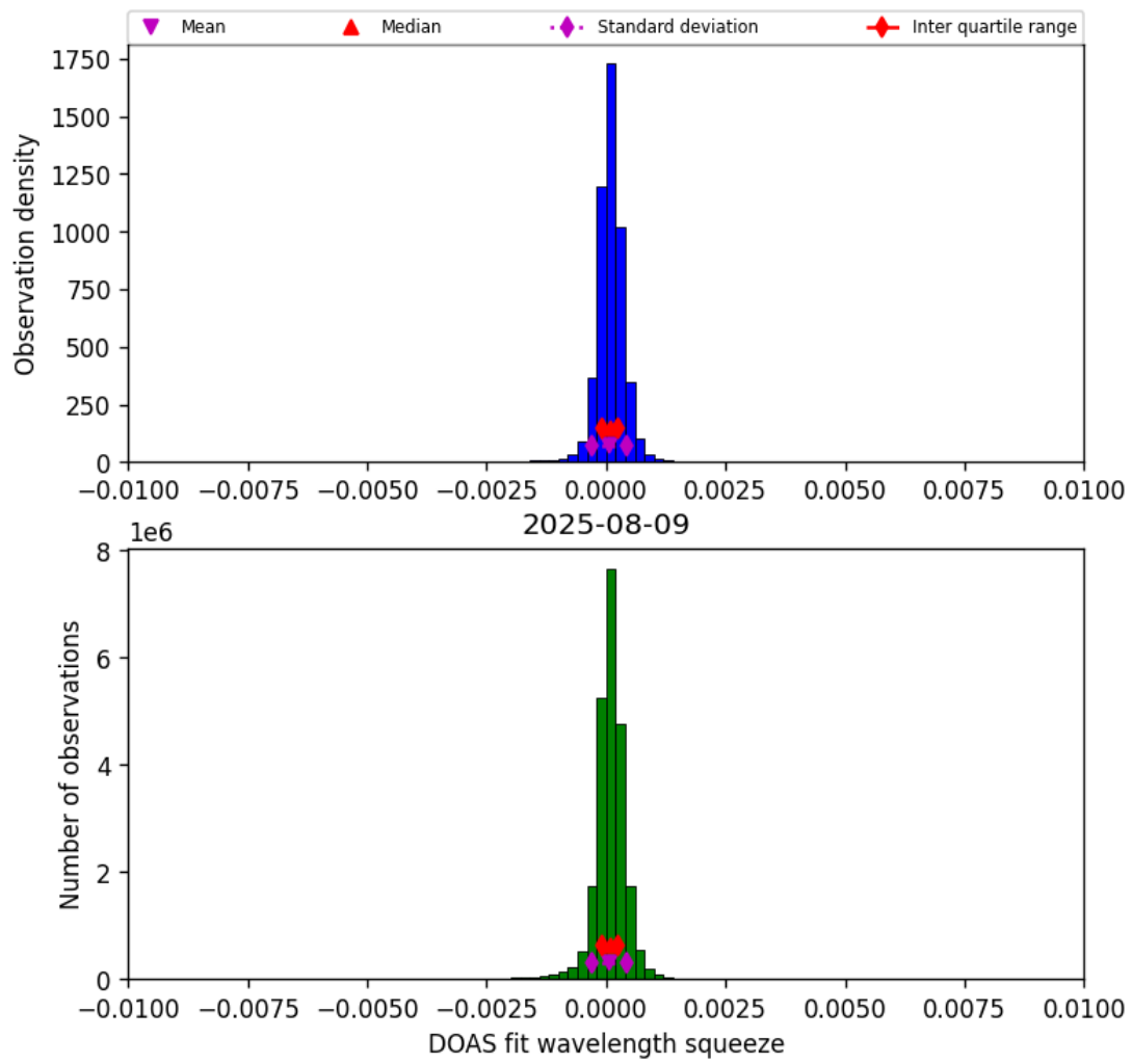
Figure 36: Histogram of “DOAS fit wavelength squeeze” for 2025-08-09 to 2025-08-10
