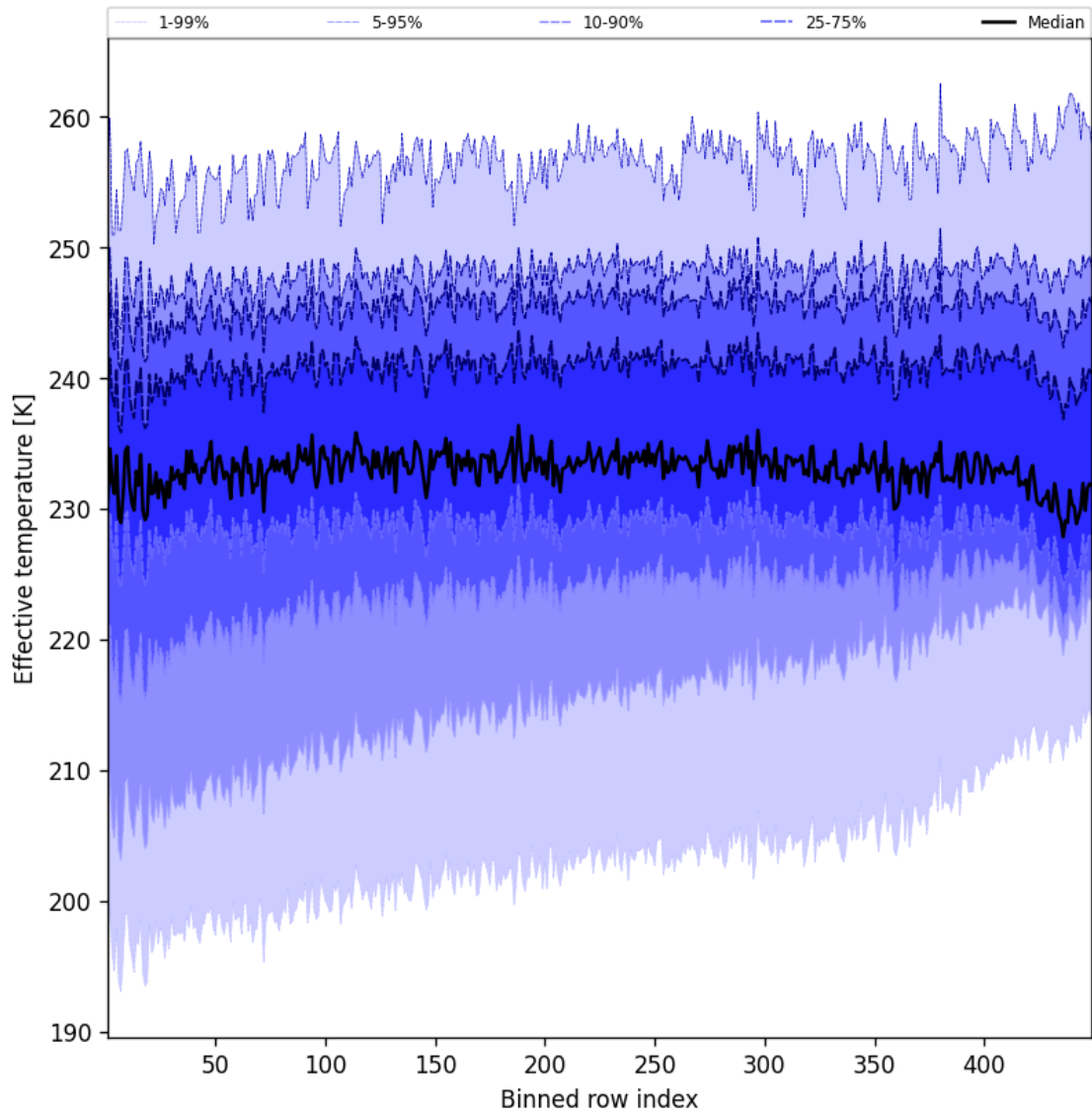
Figure 50: Along track statistics of “Effective temperature” for 2025-08-09 to 2025-08-10
