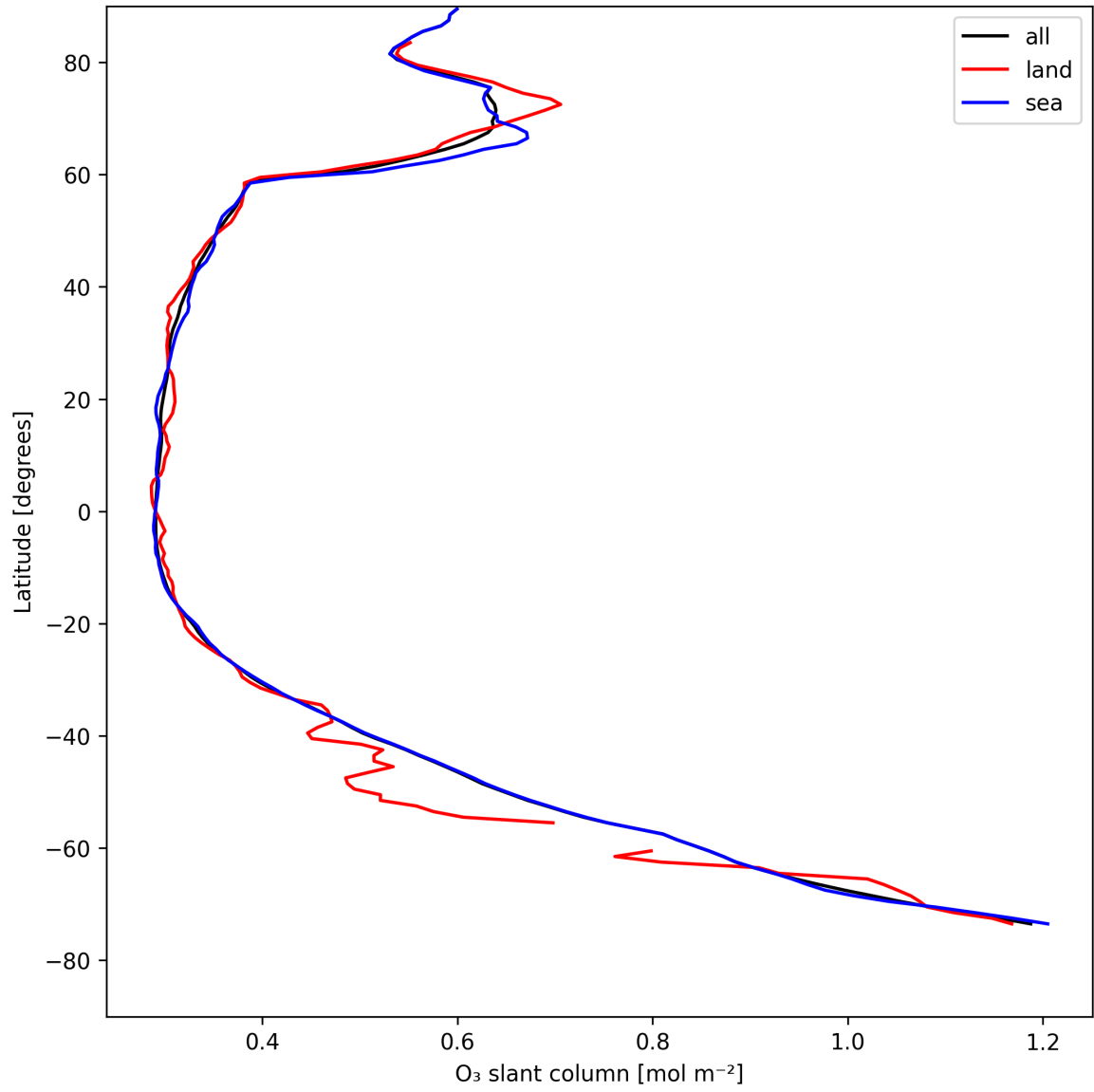
Figure 19: Zonal average of “O 3 slant column” for 2025-08-09 to 2025-08-10.
