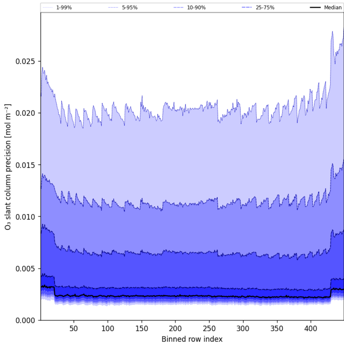
Figure 44: Along track statistics of “O 3 slant column precision” for 2025-08-09 to 2025-08-10
