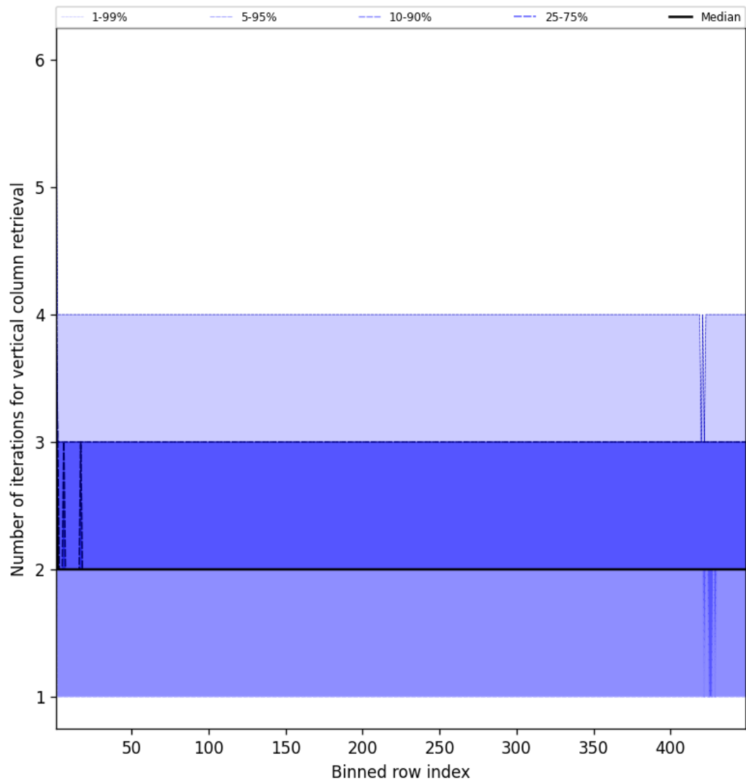
Figure 51: Along track statistics of “Number of iterations for vertical column retrieval” for 2025-08-09 to 2025-08-10
