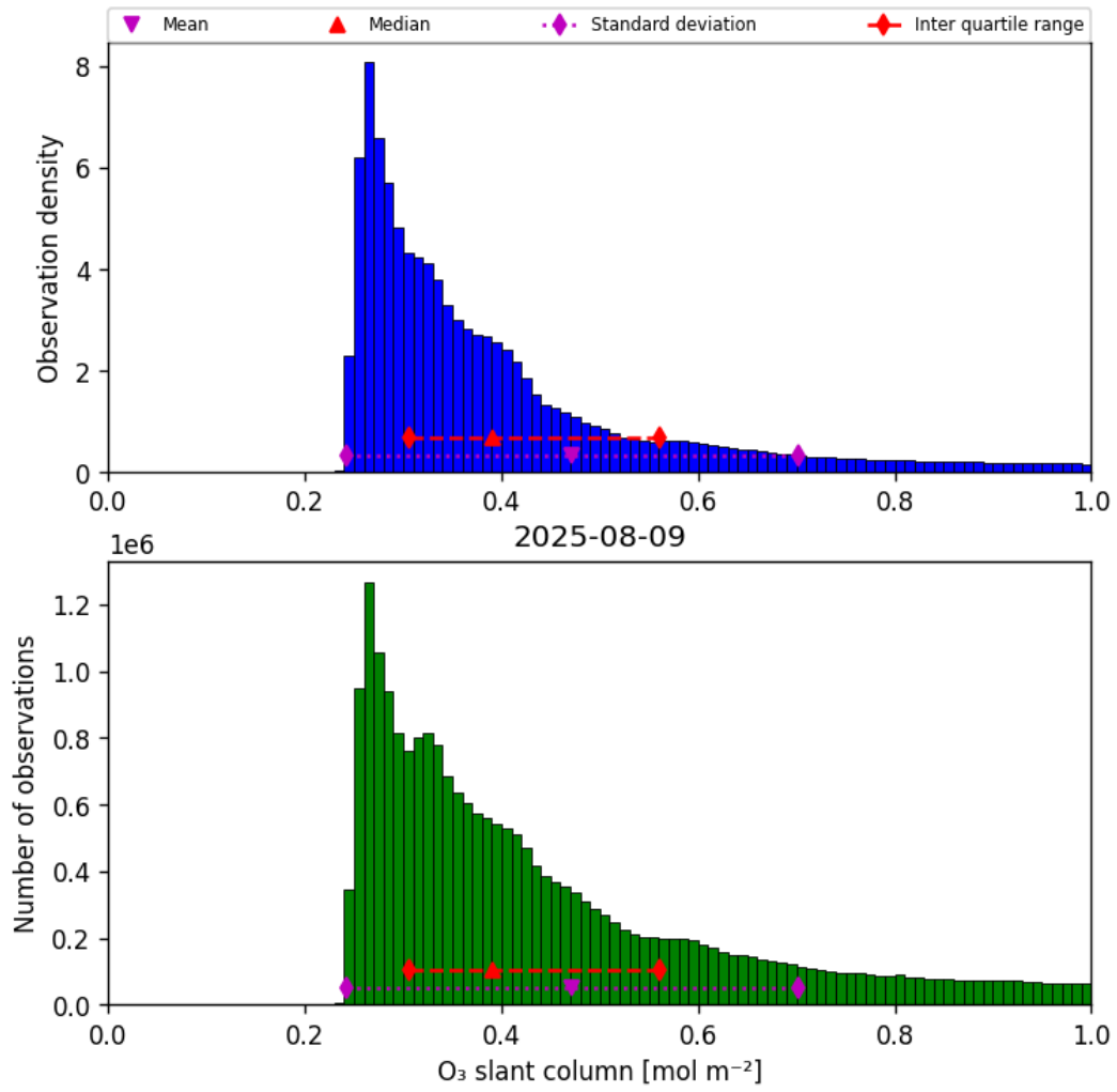
Figure 31: Histogram of “O 3 slant column” for 2025-08-09 to 2025-08-10
