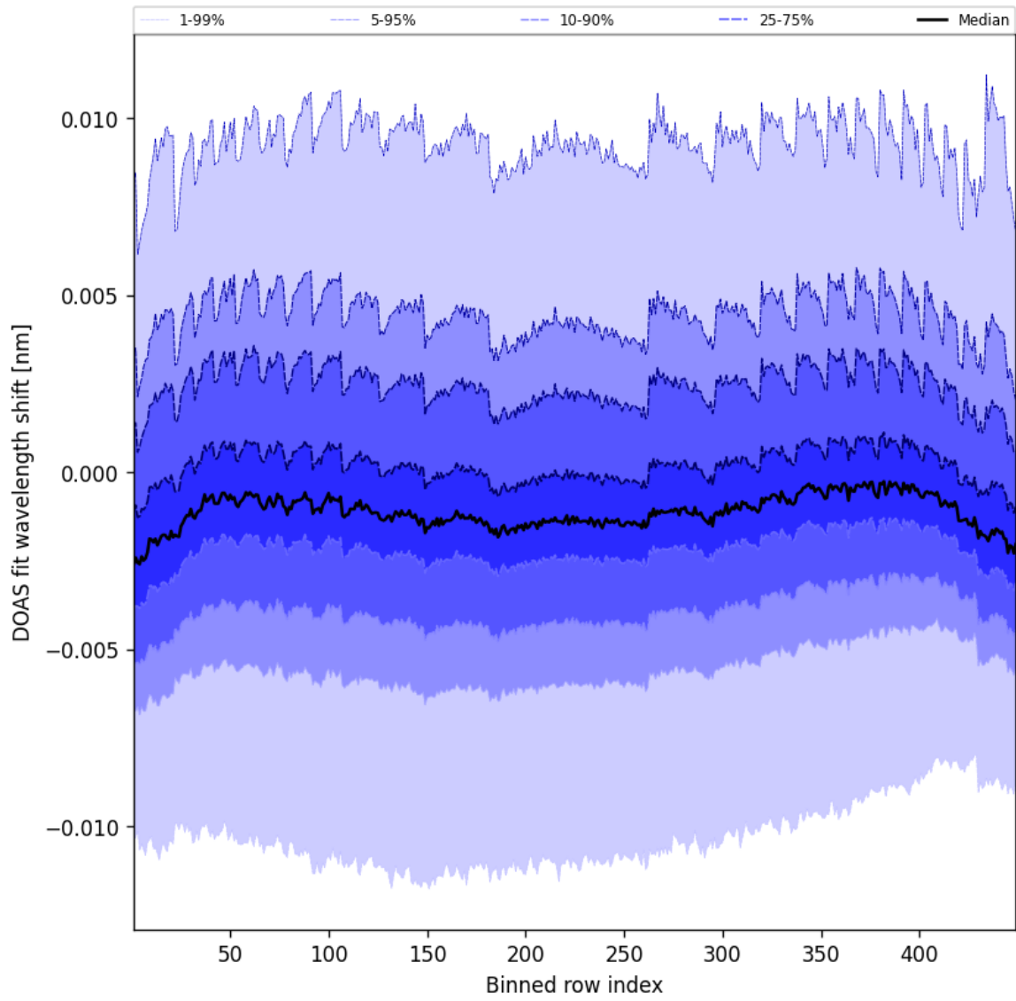
Figure 47: Along track statistics of “DOAS fit wavelength shift” for 2025-08-09 to 2025-08-10
