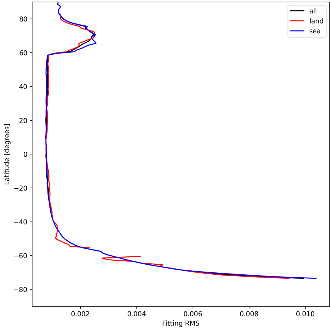
Figure 22: Zonal average of “Fitting RMS” for 2025-08-09 to 2025-08-10.
