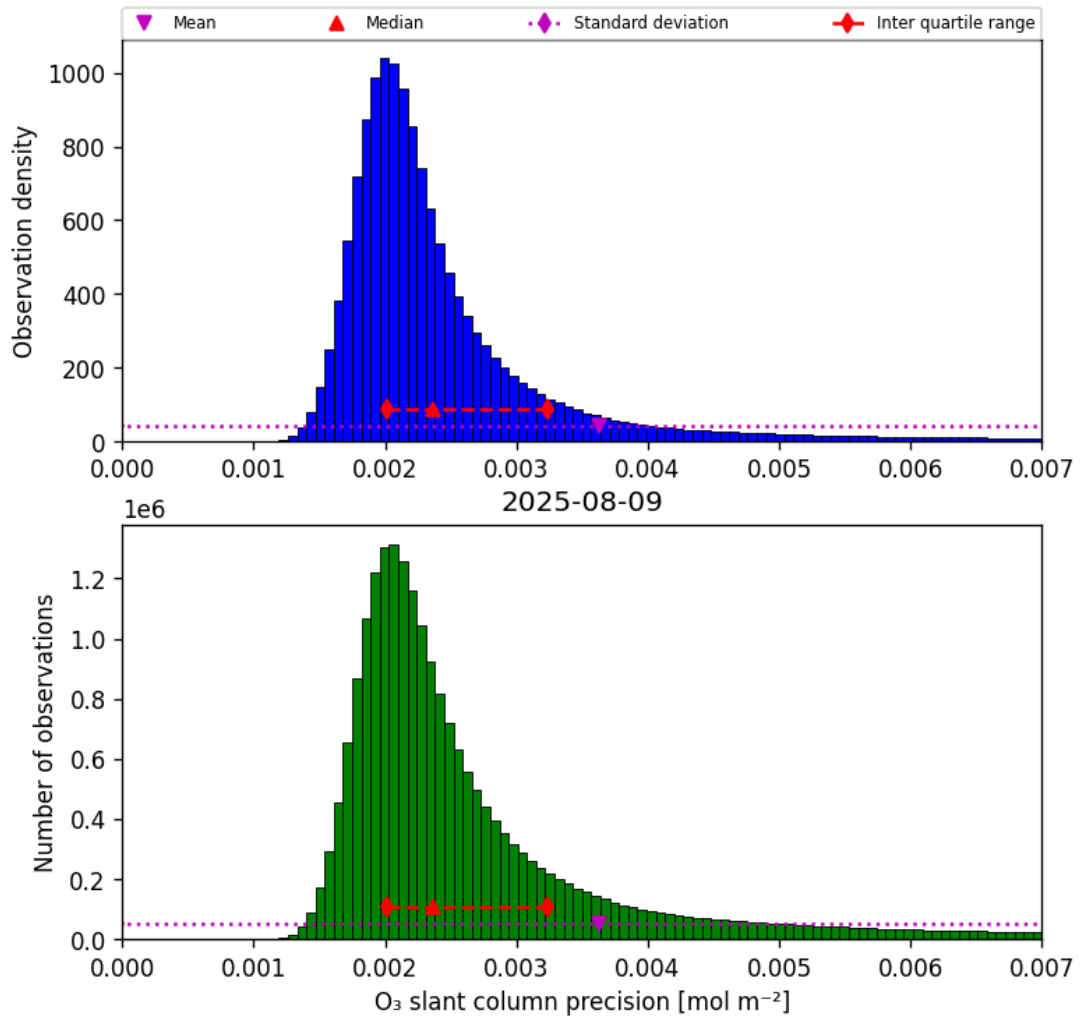
Figure 32: Histogram of "O 3 slant column precision" for 2025-08-09 to 2025-08-10
