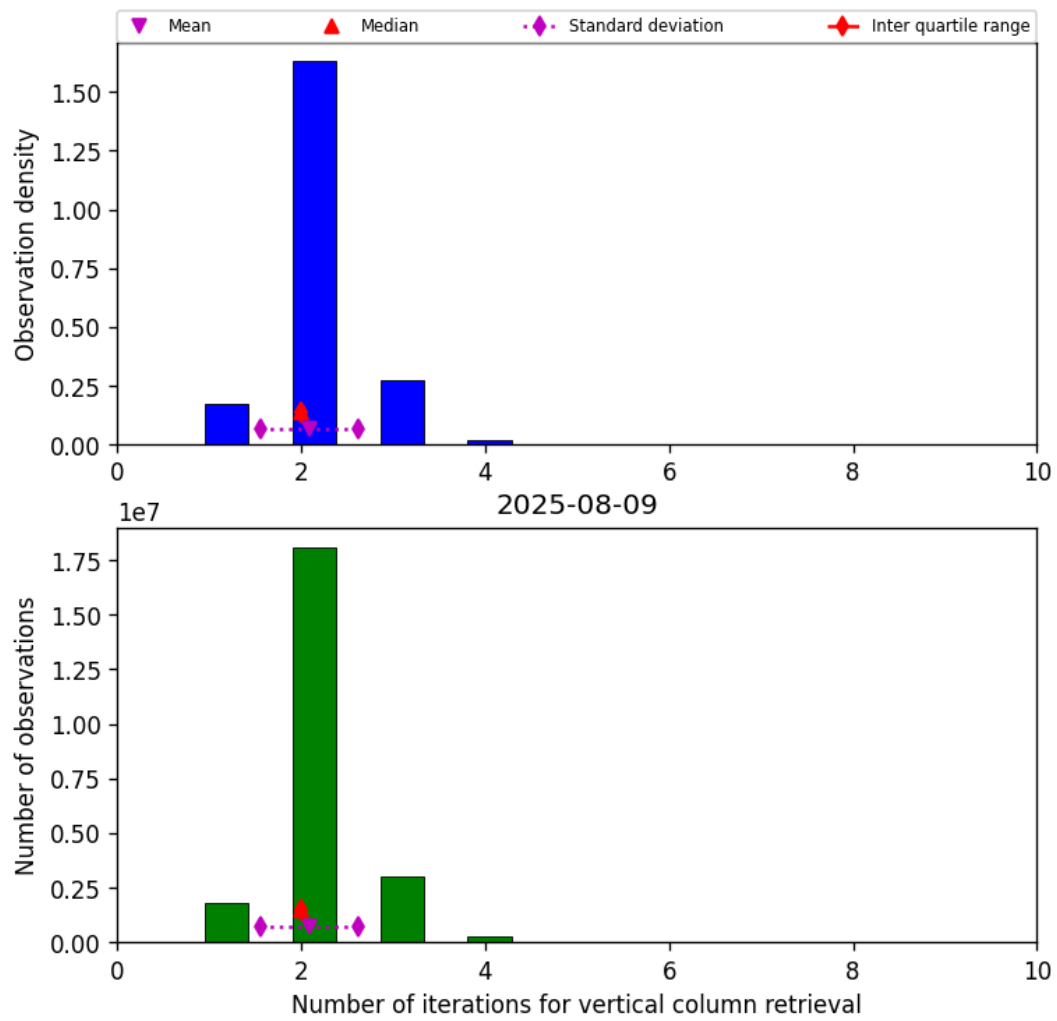
Figure 39: Histogram of “Number of iterations for vertical column retrieval” for 2025-08-09 to 2025-08-10
