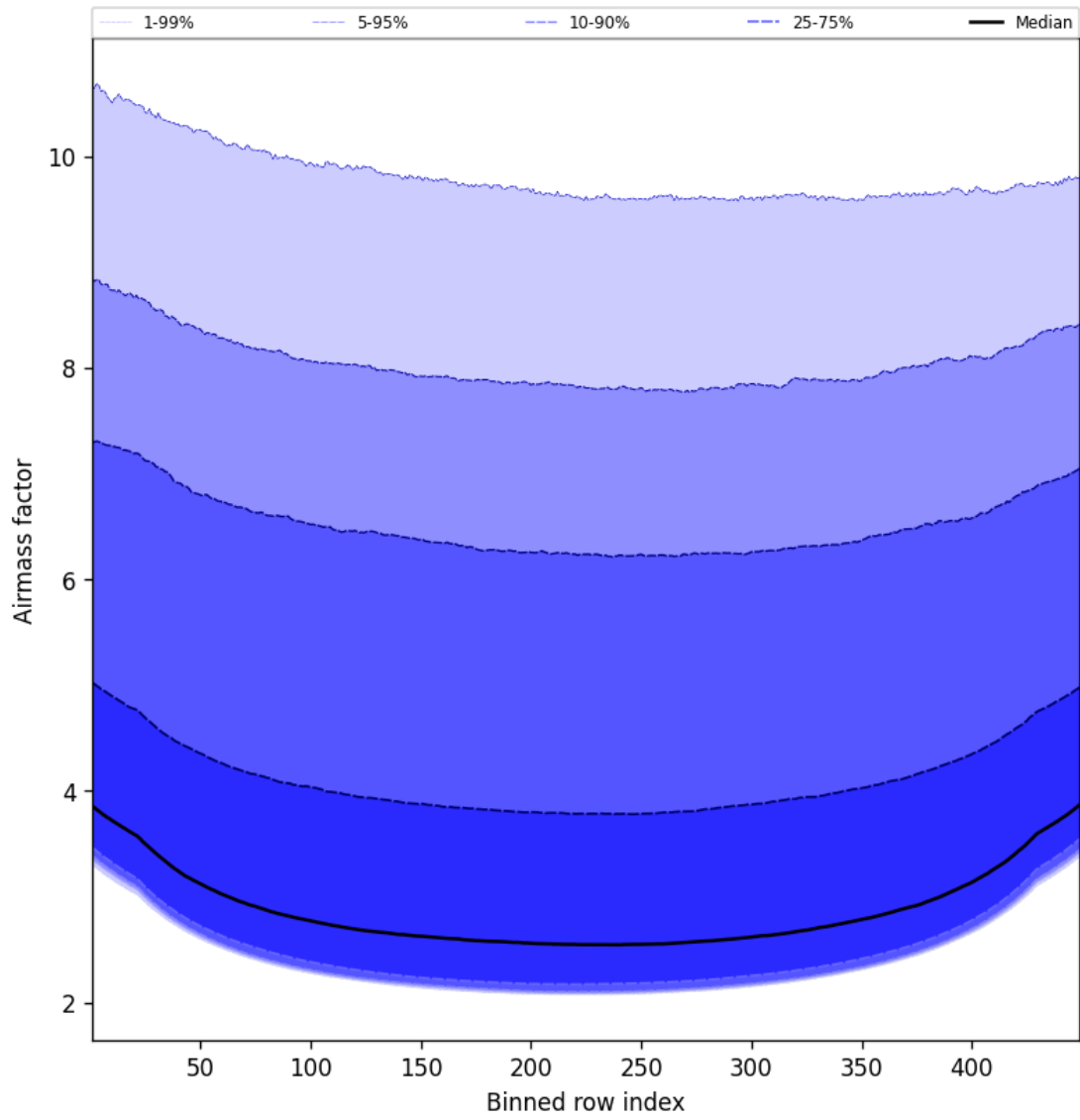
Figure 49: Along track statistics of “Airmass factor” for 2025-08-09 to 2025-08-10
