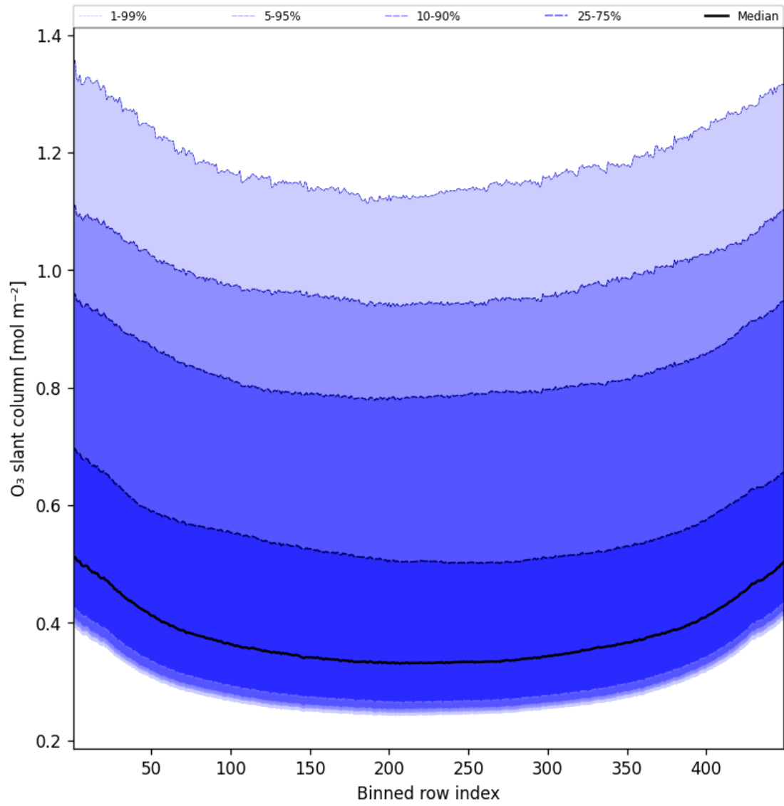
Figure 43: Along track statistics of "O 3 slant column" for 2025-08-09 to 2025-08-10
