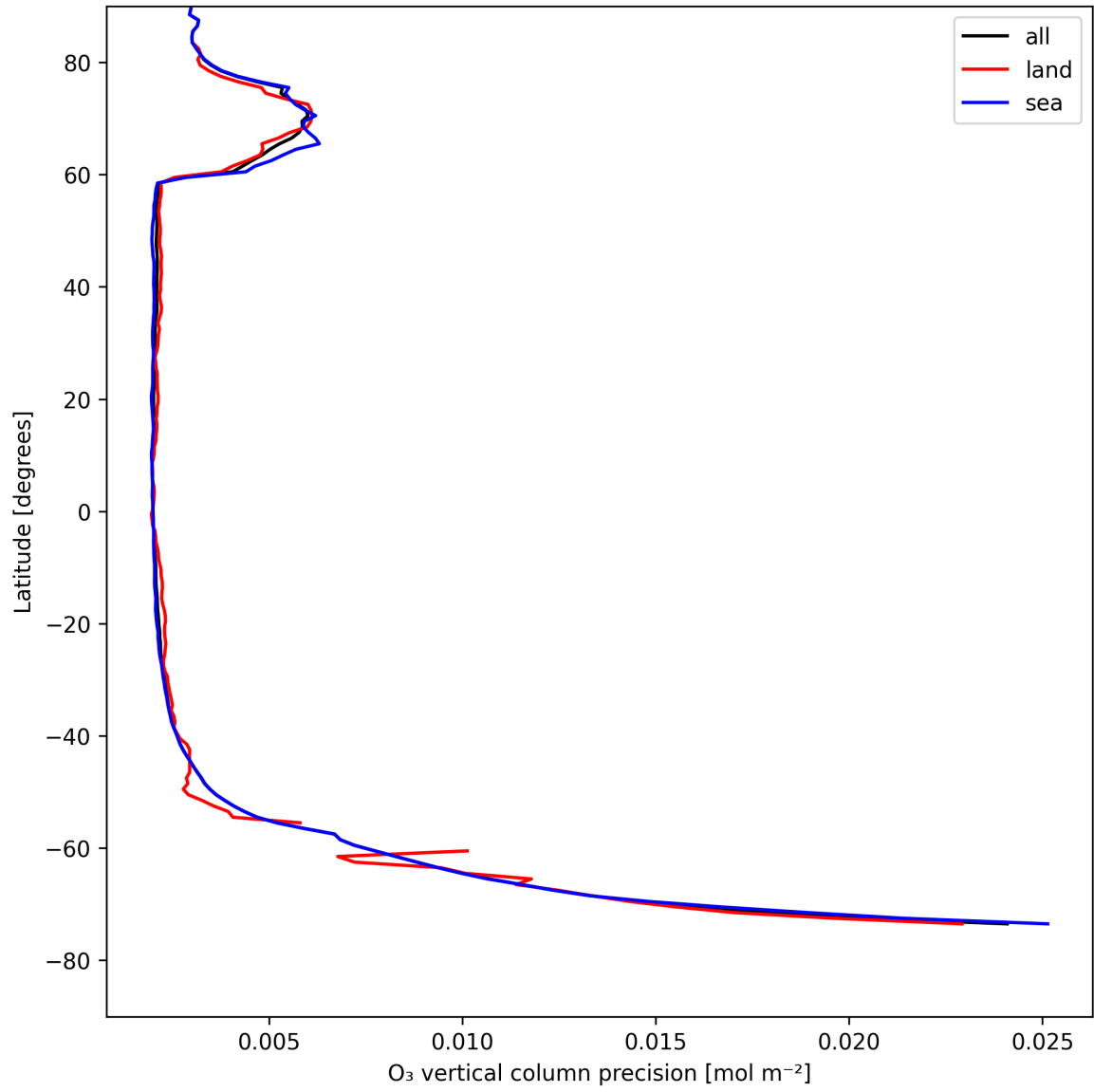
Figure 18: Zonal average of “O 3 vertical column precision” for 2025-08-09 to 2025-08-10.
