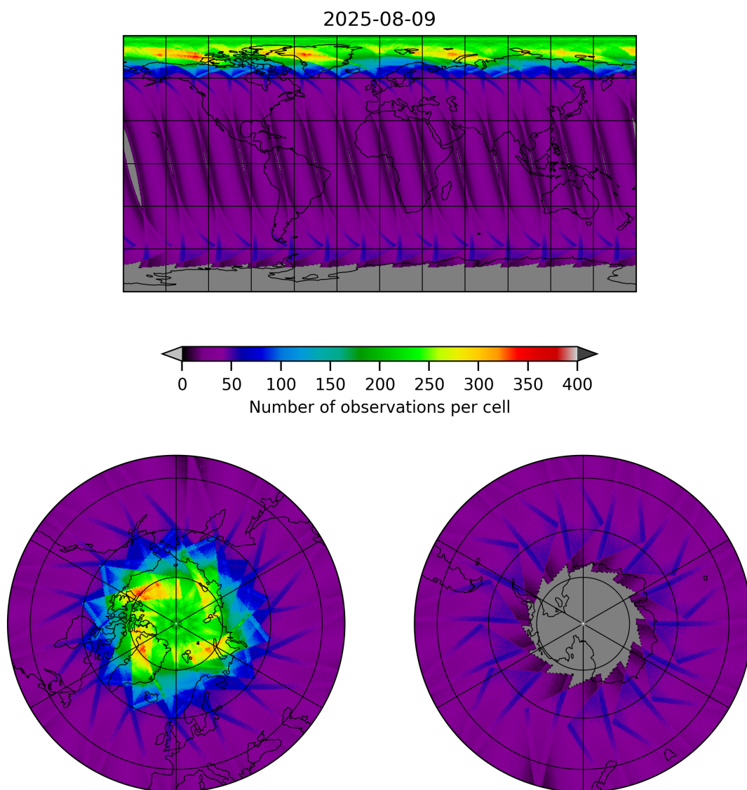
Figure 15: Map of the number of observations for 2025-08-09 to 2025-08-10
