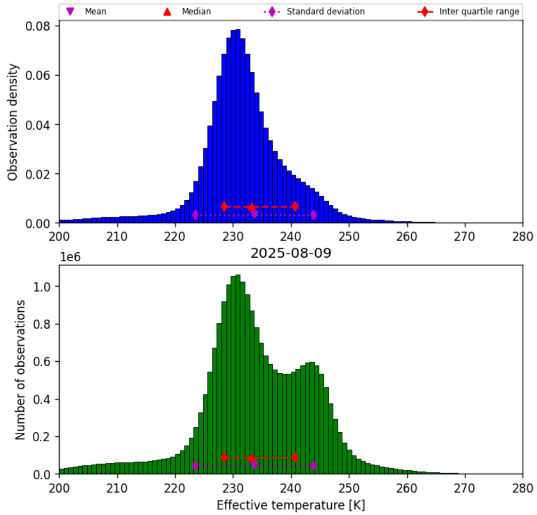
Figure 38: Histogram of “Effective temperature” for 2025-08-09 to 2025-08-10
