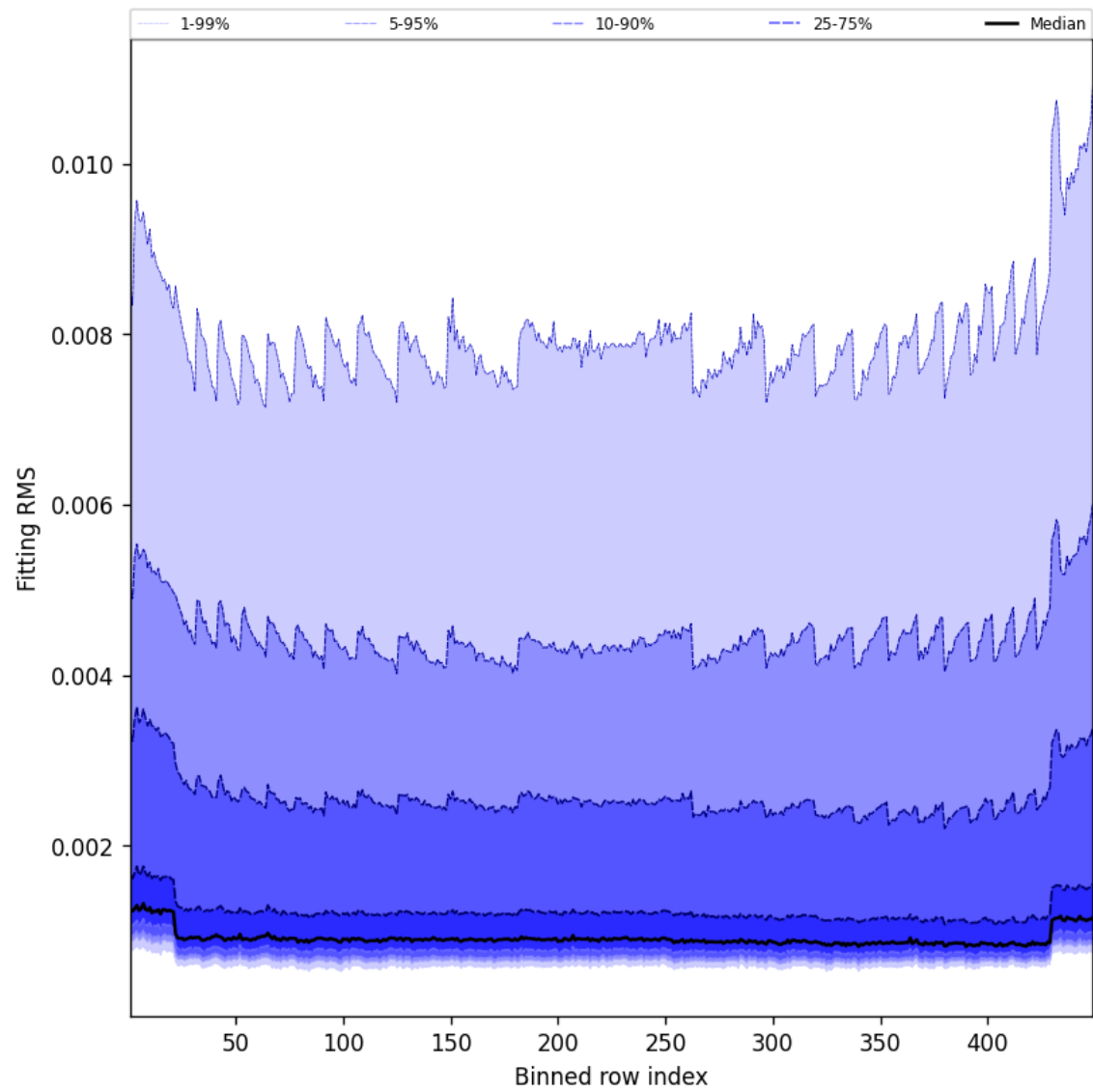
Figure 46: Along track statistics of “Fitting RMS” for 2025-08-09 to 2025-08-10
