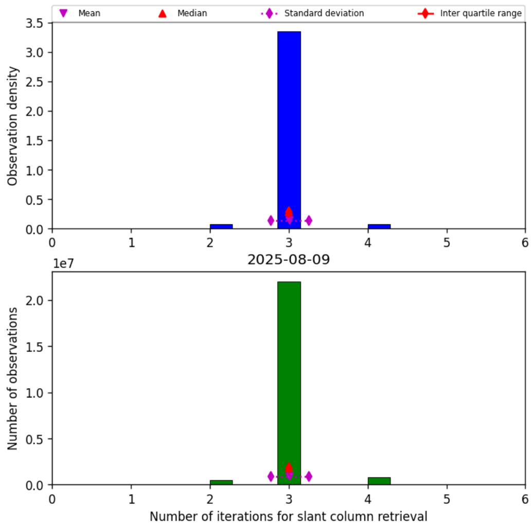
Figure 33: Histogram of “Number of iterations for slant column retrieval” for 2025-08-09 to 2025-08-10
