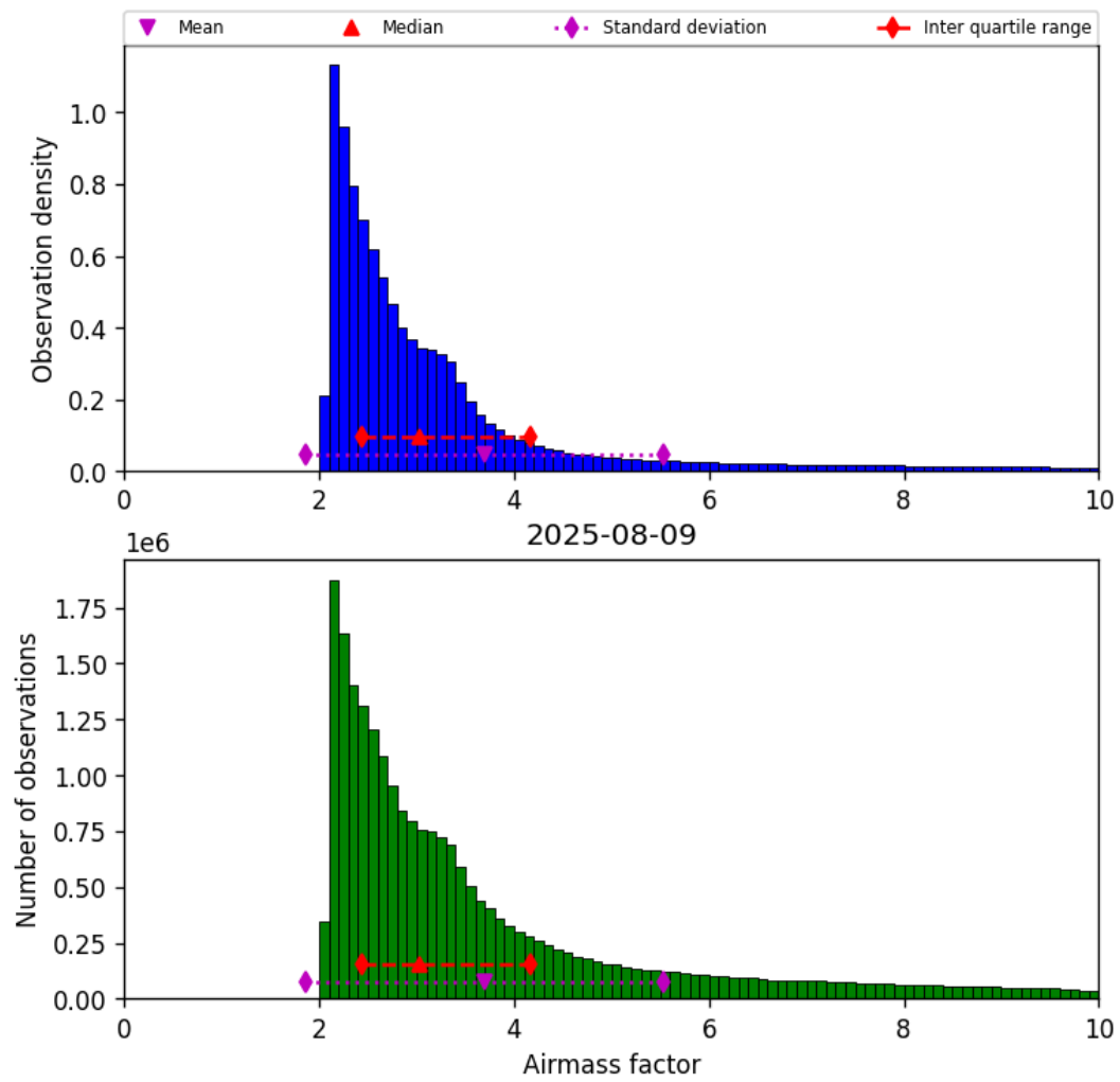
Figure 37: Histogram of “Airmass factor” for 2025-08-09 to 2025-08-10
