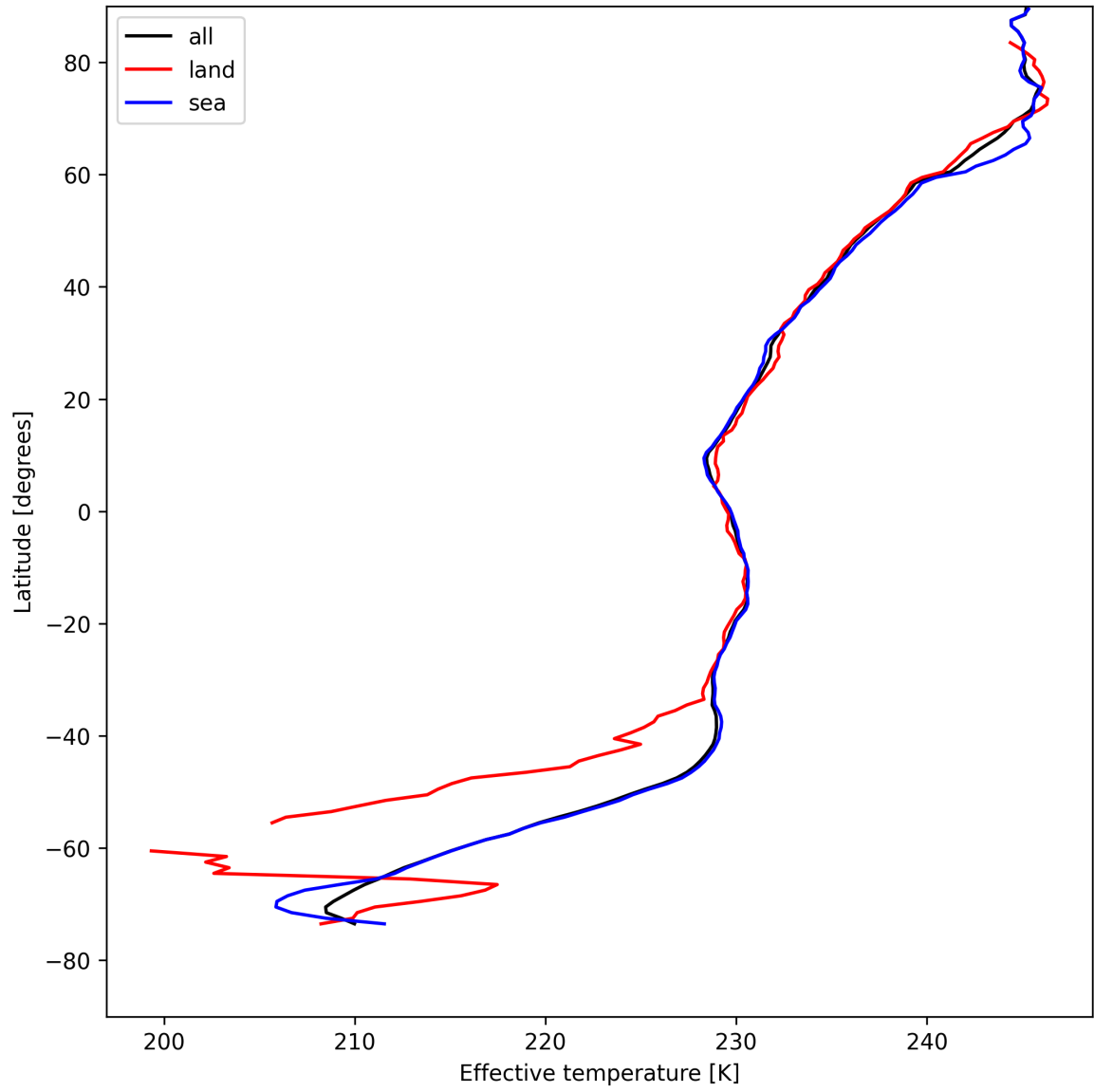
Figure 26: Zonal average of "Effective temperature" for 2025-08-09 to 2025-08-10.
