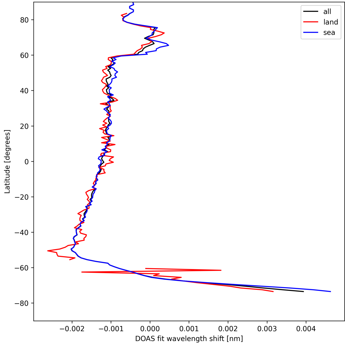
Figure 23: Zonal average of "DOAS fit wavelength shift" for 2025-08-09 to 2025-08-10.
