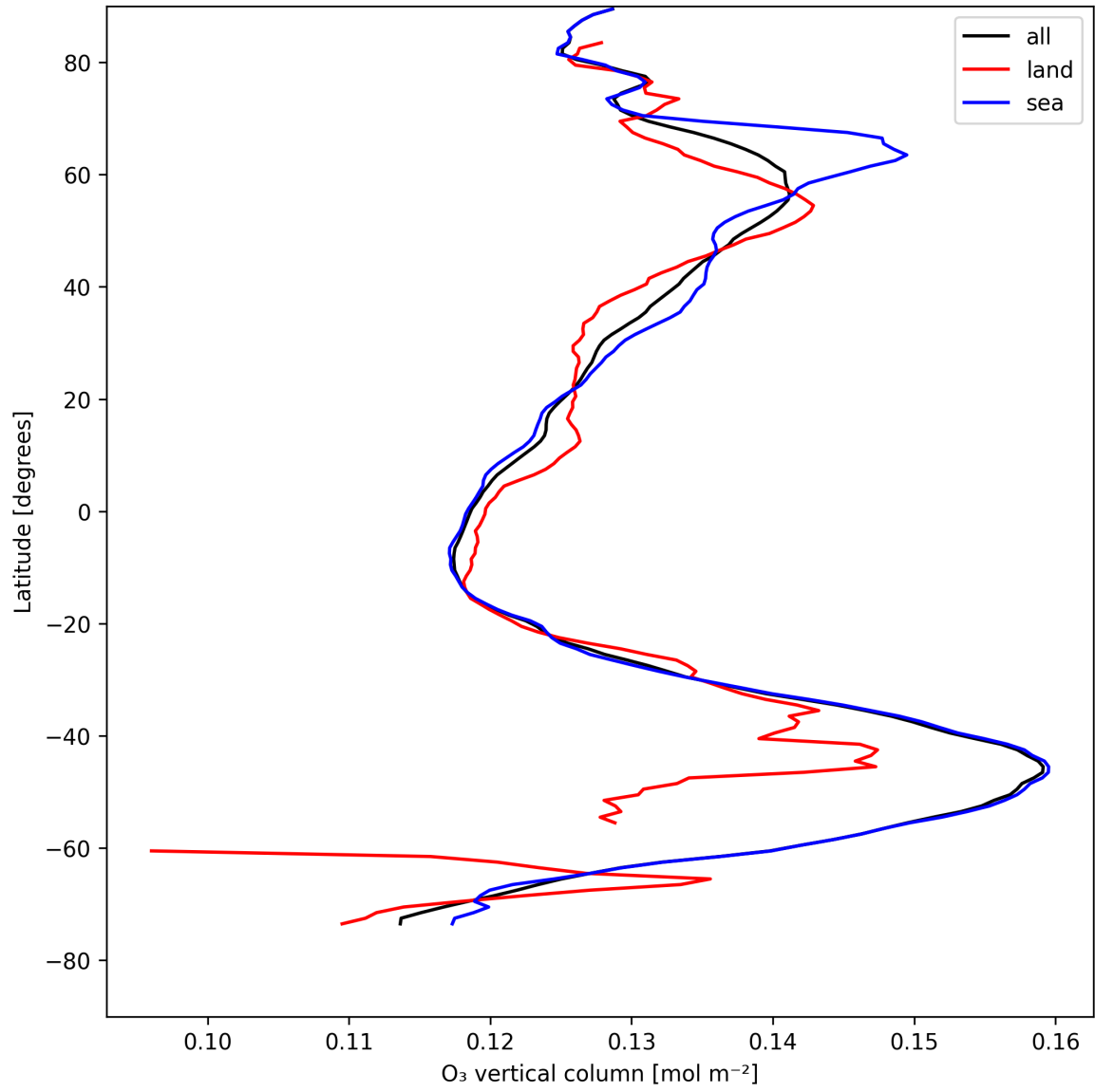
Figure 17: Zonal average of “O 3 vertical column” for 2025-08-09 to 2025-08-10.
