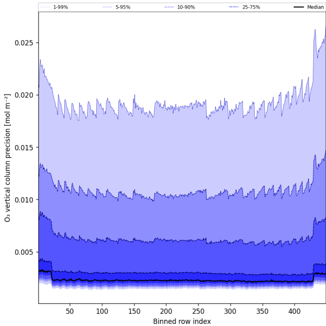
Figure 42: Along track statistics of “O 3 vertical column precision” for 2025-08-09 to 2025-08-10
