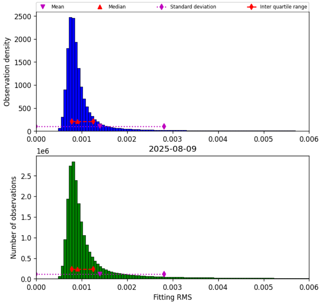
Figure 34: Histogram of “Fitting RMS” for 2025-08-09 to 2025-08-10
