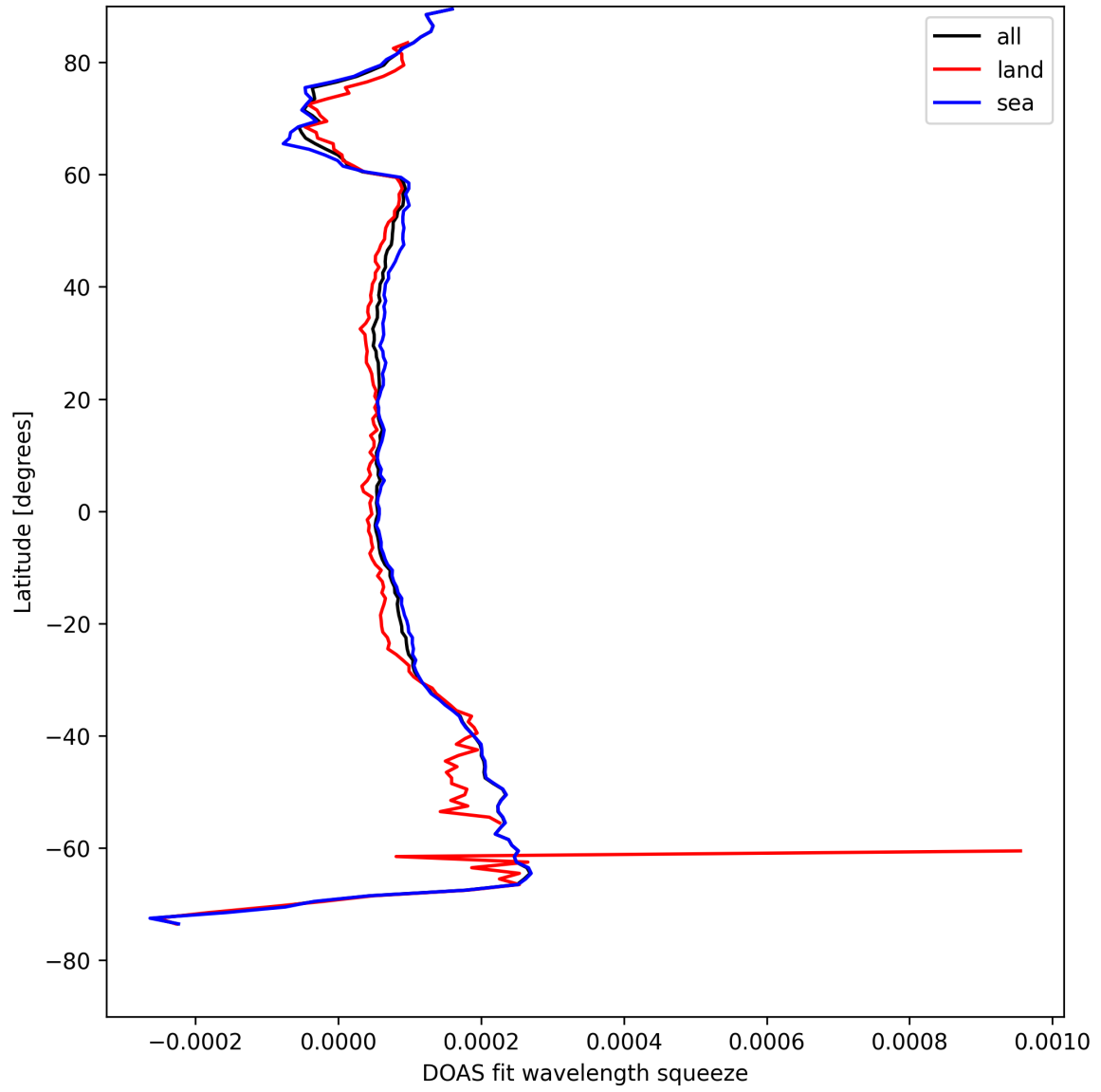
Figure 24: Zonal average of “DOAS fit wavelength squeeze” for 2025-08-09 to 2025-08-10.
