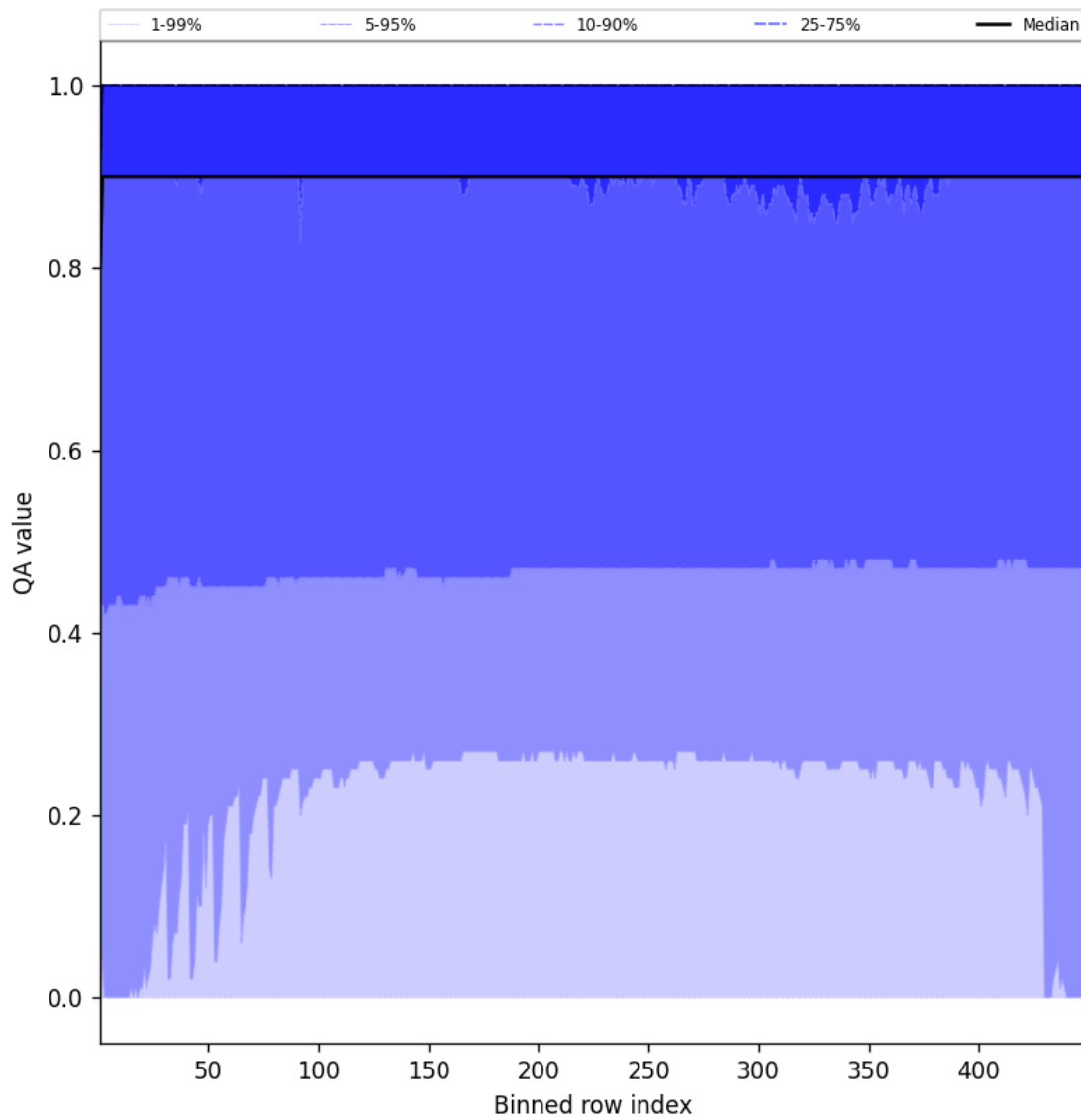
Figure 40: Along track statistics of “QA value” for 2025-08-09 to 2025-08-10
