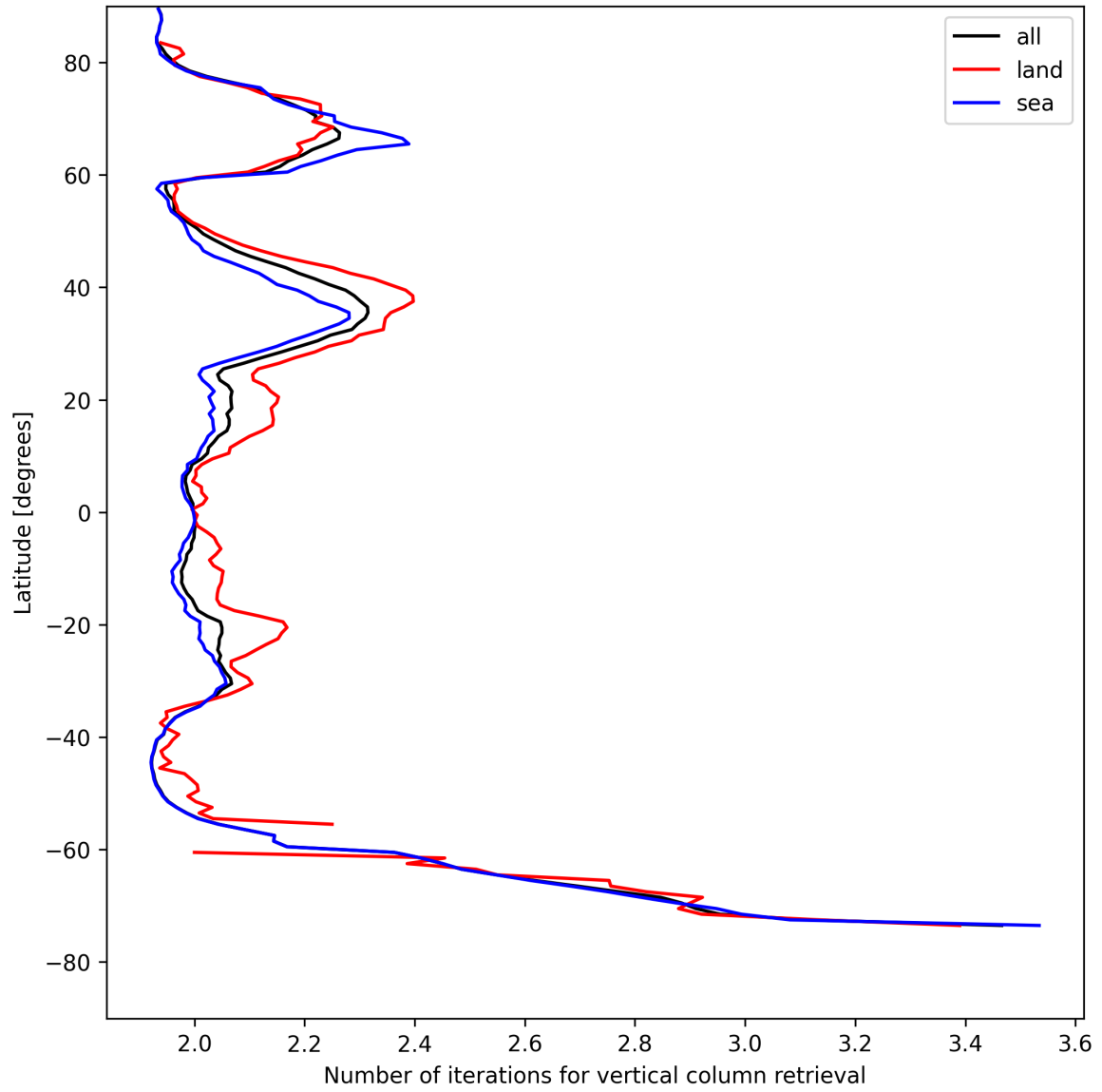
Figure 27: Zonal average of “Number of iterations for vertical column retrieval” for 2025-08-09 to 2025-08-10.
