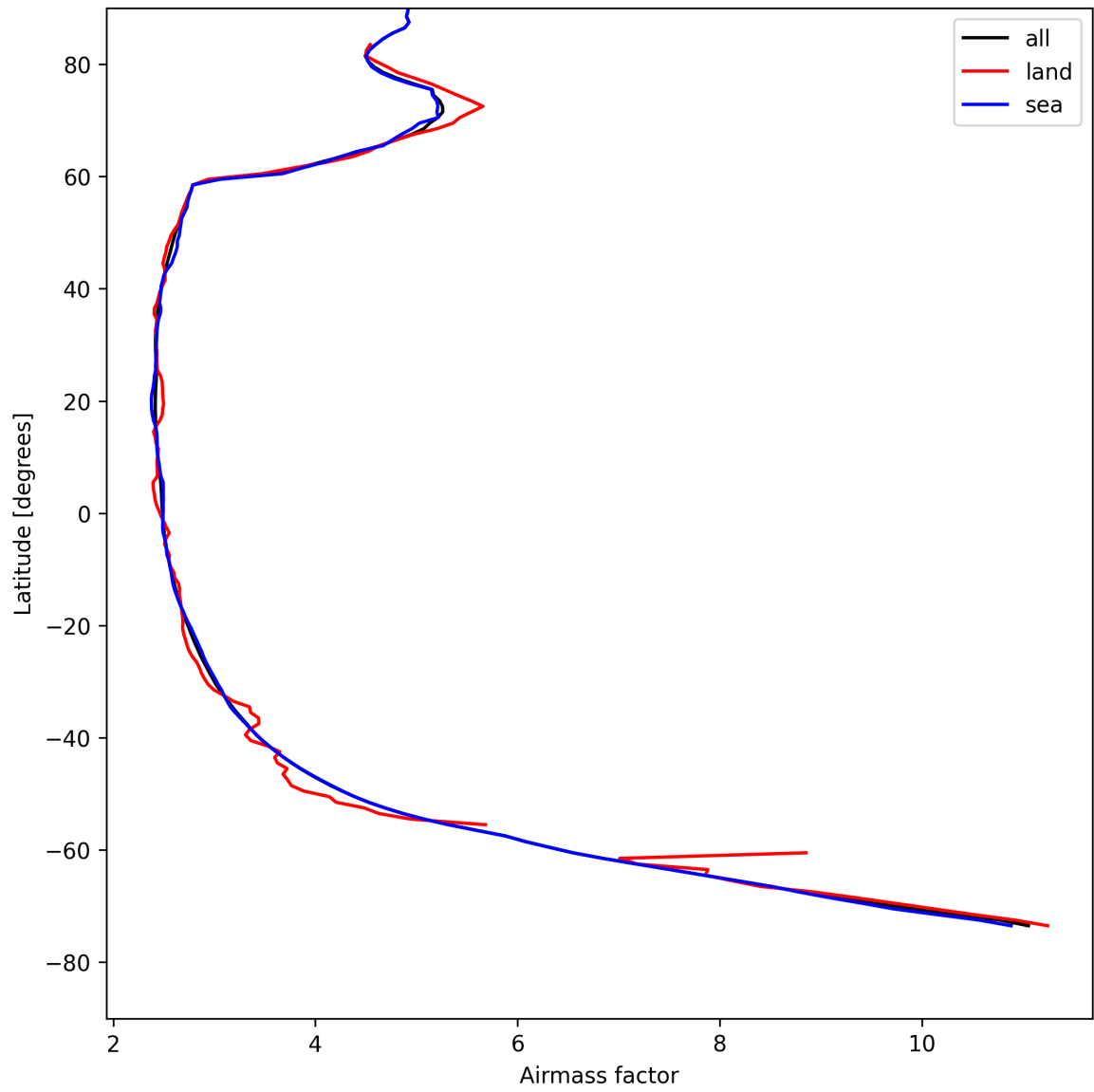
Figure 25: Zonal average of “Airmass factor” for 2025-08-09 to 2025-08-10.
