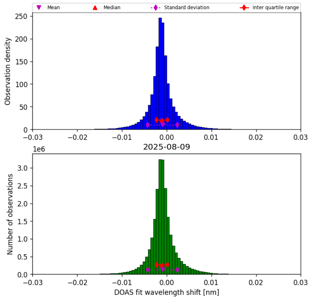
Figure 35: Histogram of “DOAS fit wavelength shift” for 2025-08-09 to 2025-08-10
