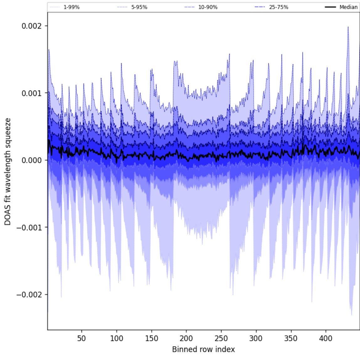
Figure 48: Along track statistics of “DOAS fit wavelength squeeze” for 2025-08-09 to 2025-08-10
