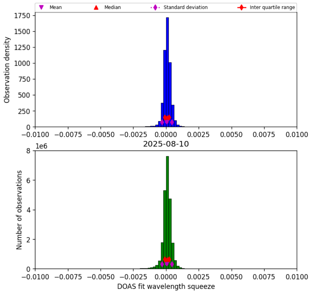
Figure 36: Histogram of “DOAS fit wavelength squeeze” for 2025-08-10 to 2025-08-11
