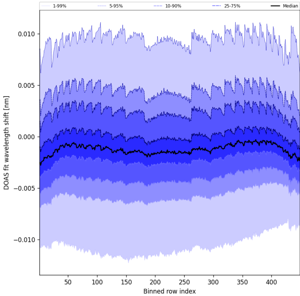
Figure 47: Along track statistics of “DOAS fit wavelength shift” for 2025-08-10 to 2025-08-11
