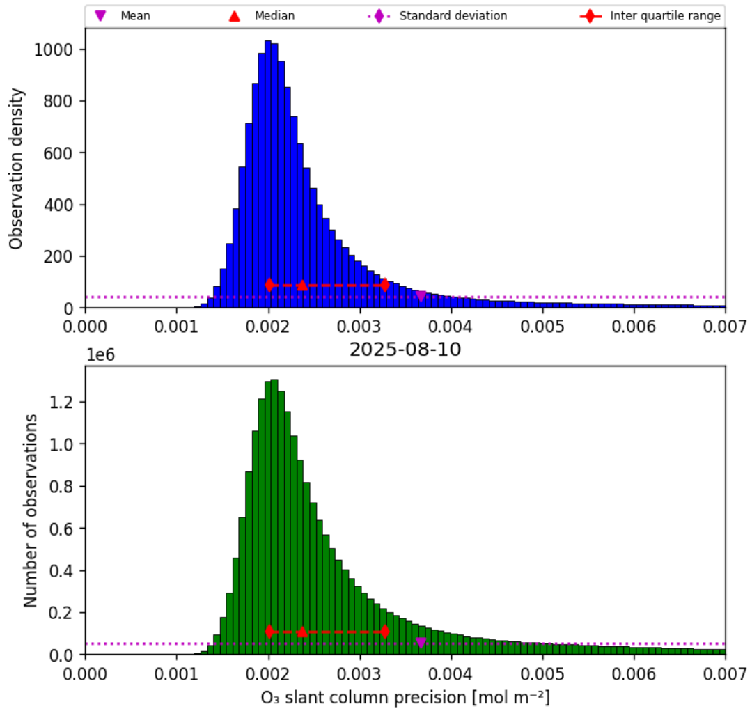
Figure 32: Histogram of “O 3 slant column precision” for 2025-08-10 to 2025-08-11
