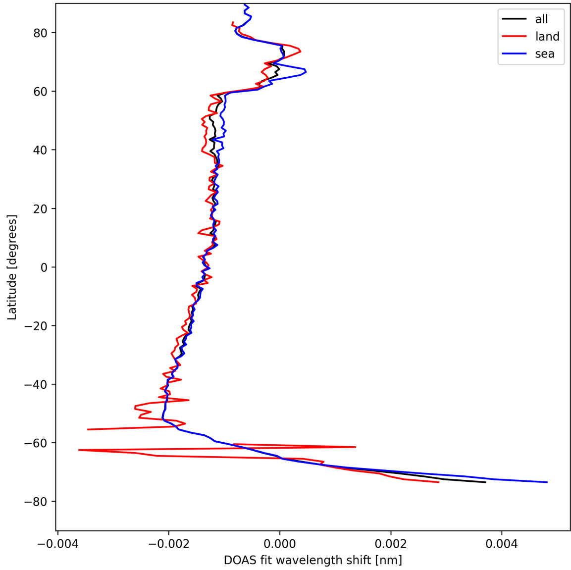
Figure 23: Zonal average of "DOAS fit wavelength shift" for 2025-08-10 to 2025-08-11.
