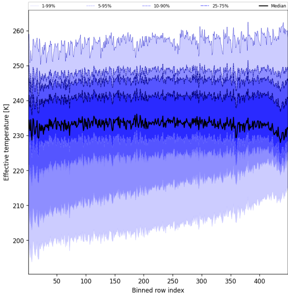
Figure 50: Along track statistics of “Effective temperature” for 2025-08-10 to 2025-08-11
