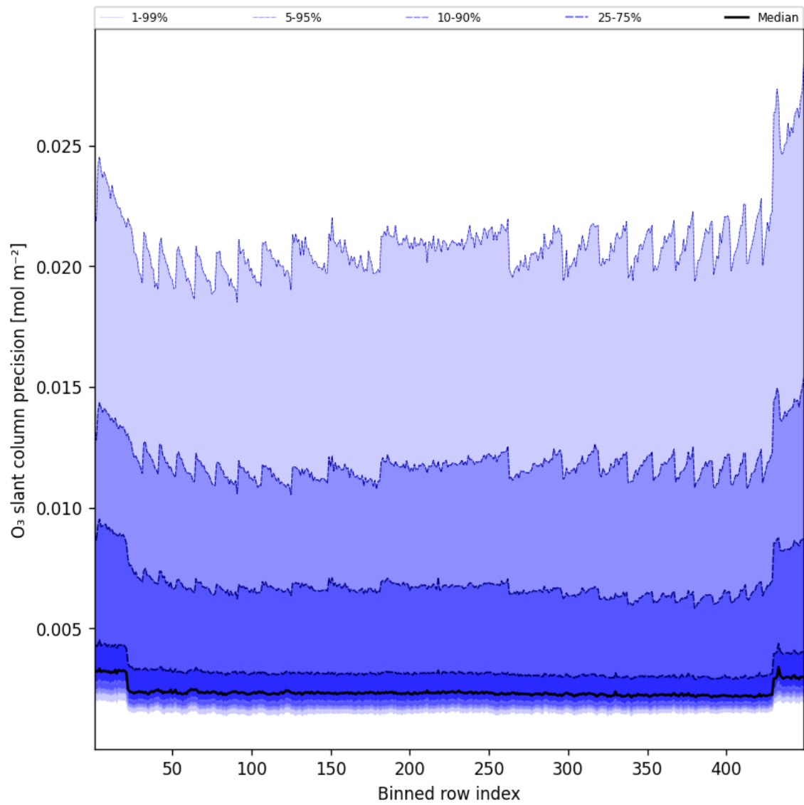
Figure 44: Along track statistics of “O 3 slant column precision” for 2025-08-10 to 2025-08-11
