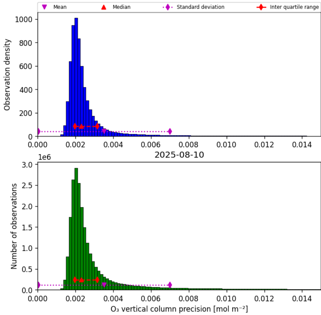
Figure 30: Histogram of “O 3 vertical column precision” for 2025-08-10 to 2025-08-11
