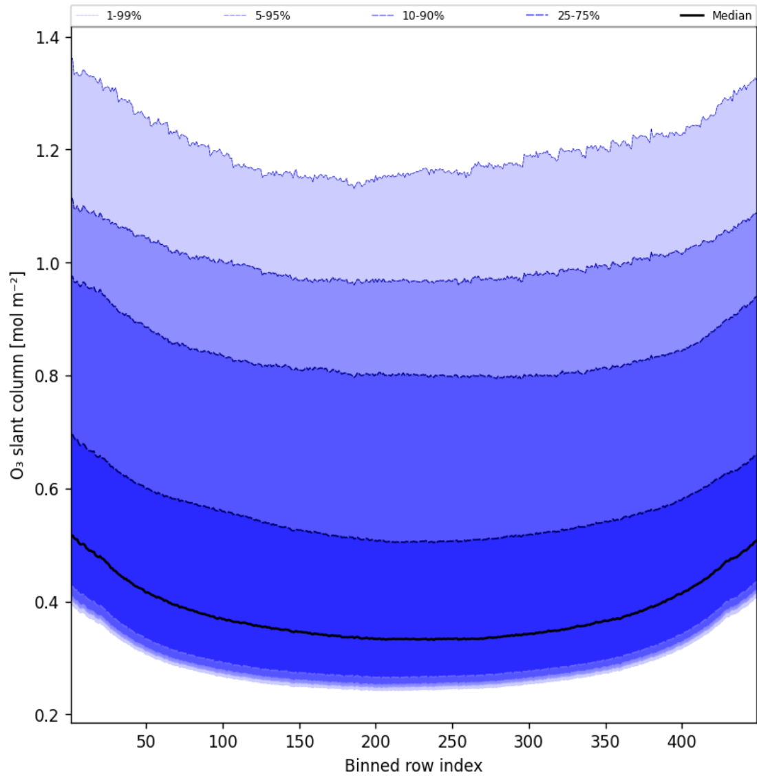
Figure 43: Along track statistics of “O 3 slant column” for 2025-08-10 to 2025-08-11
