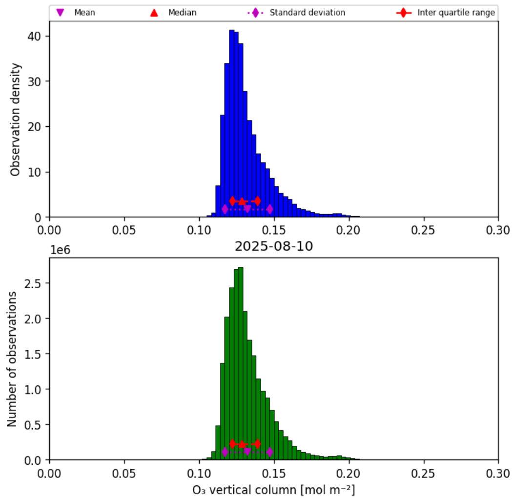
Figure 29: Histogram of “O 3 vertical column” for 2025-08-10 to 2025-08-11
