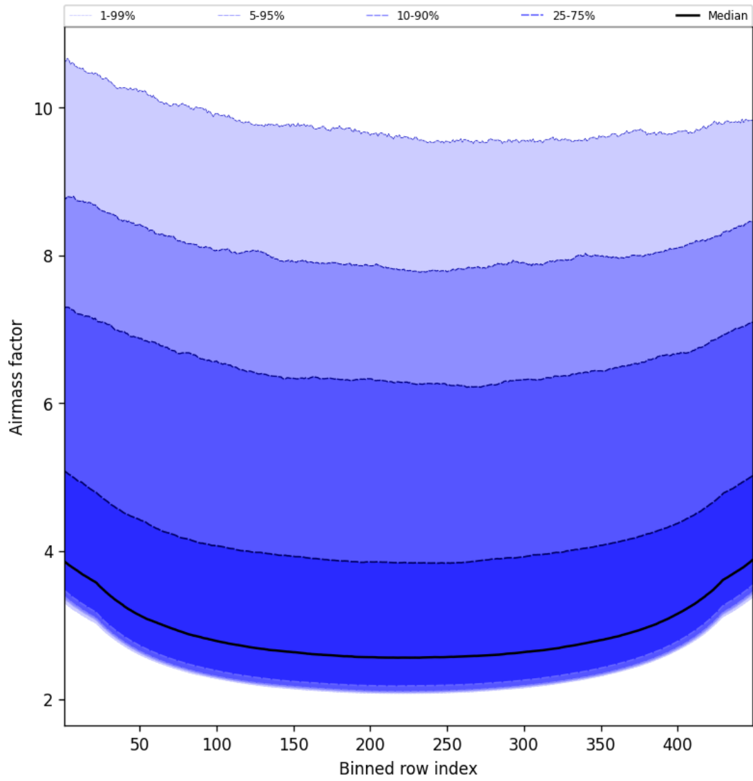
Figure 49: Along track statistics of “Airmass factor” for 2025-08-10 to 2025-08-11
