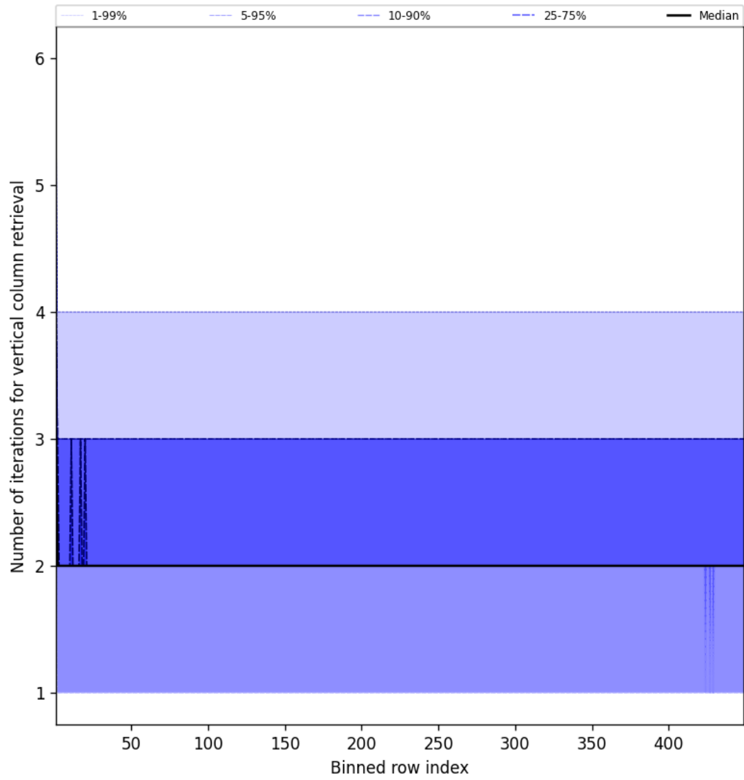
Figure 51: Along track statistics of “Number of iterations for vertical column retrieval” for 2025-08-10 to 2025-08-11
