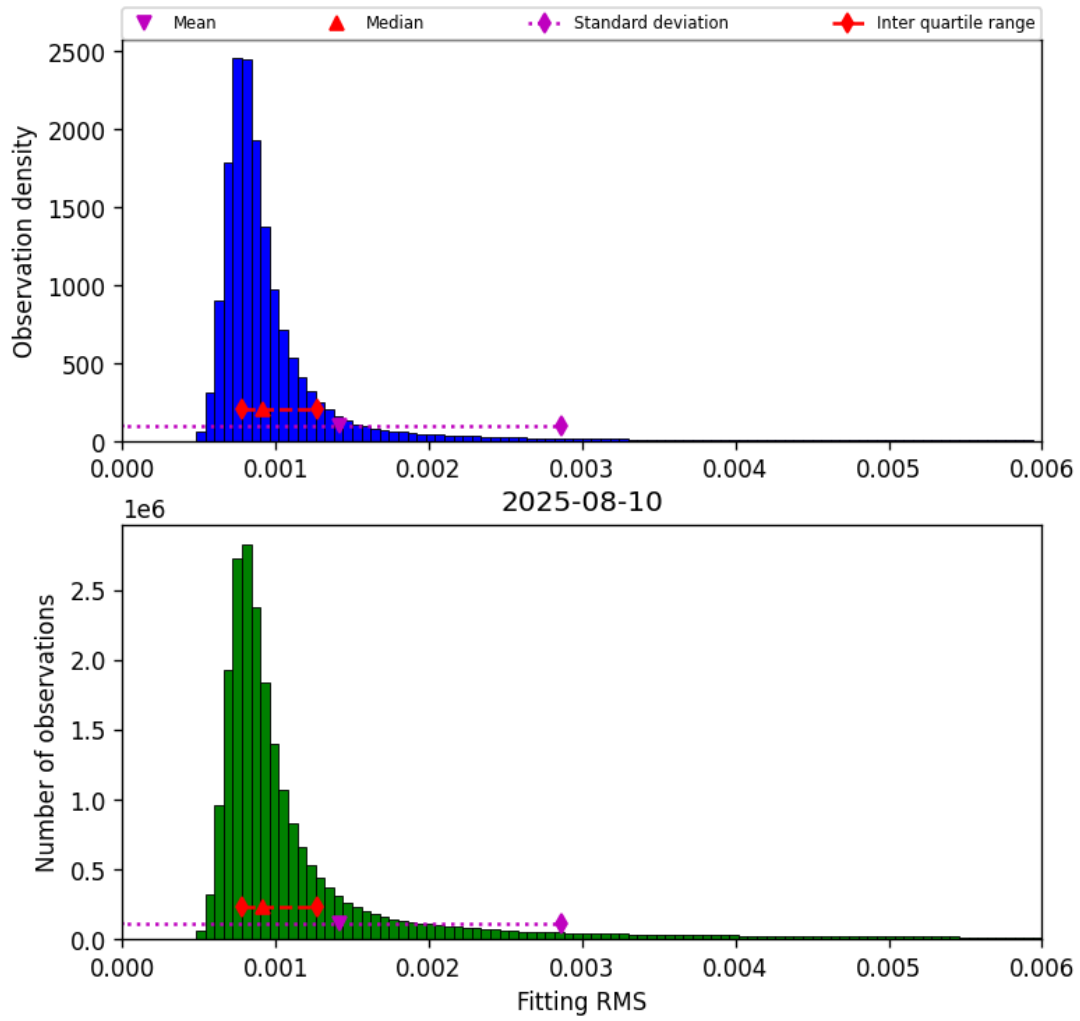
Figure 34: Histogram of “Fitting RMS” for 2025-08-10 to 2025-08-11
