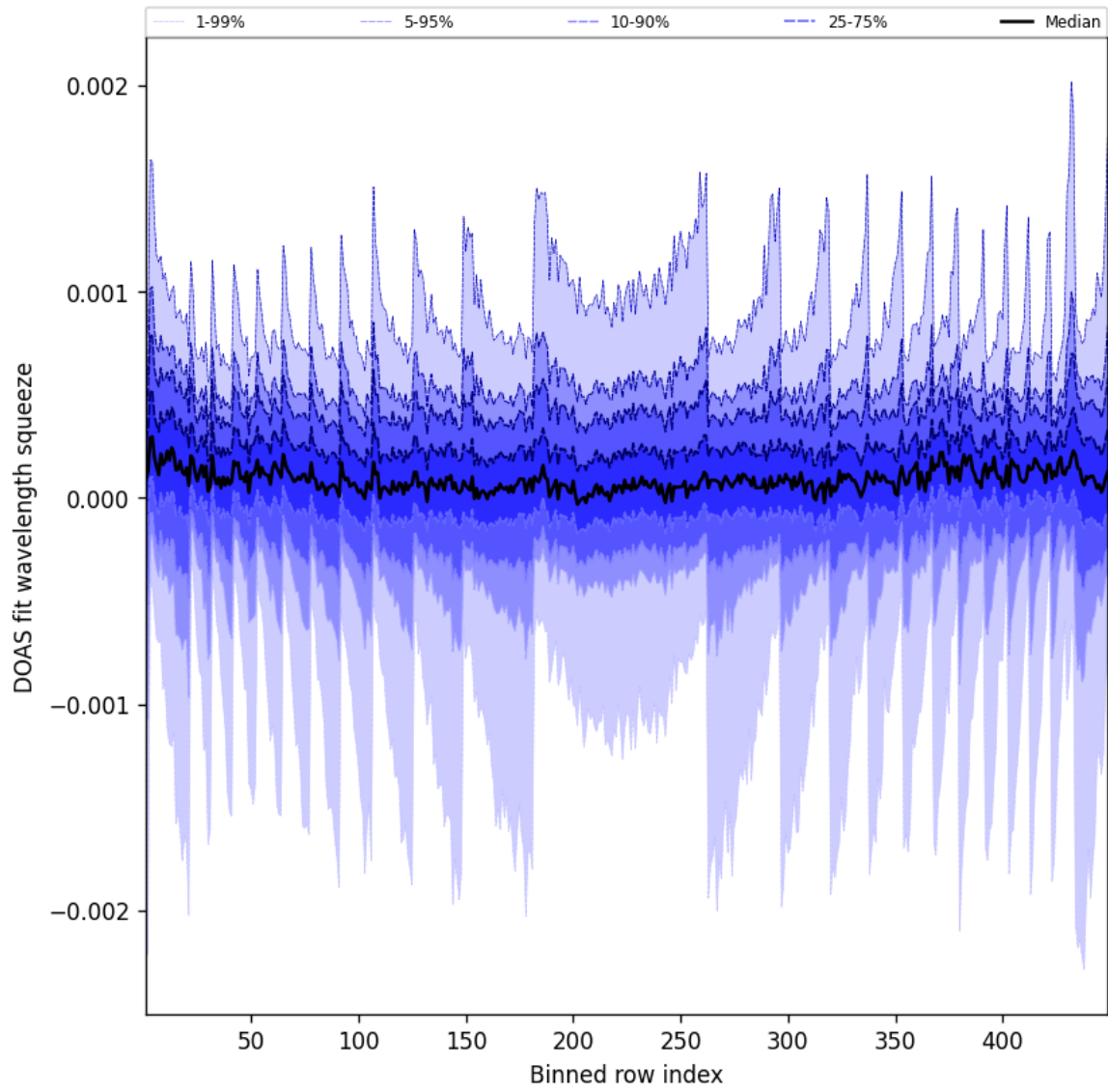
Figure 48: Along track statistics of “DOAS fit wavelength squeeze” for 2025-08-10 to 2025-08-11
