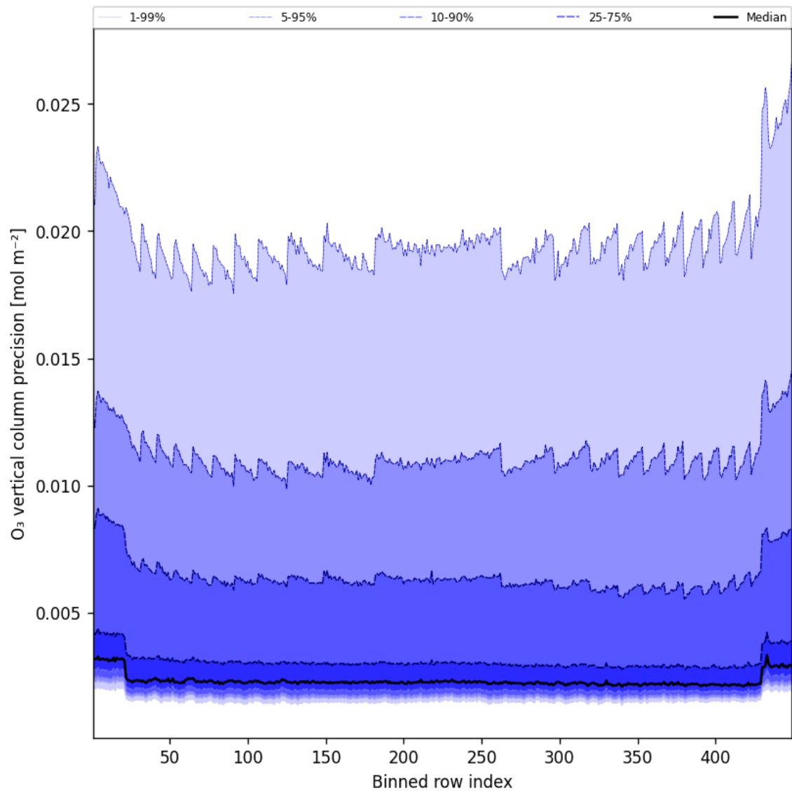
Figure 42: Along track statistics of “O 3 vertical column precision” for 2025-08-10 to 2025-08-11
