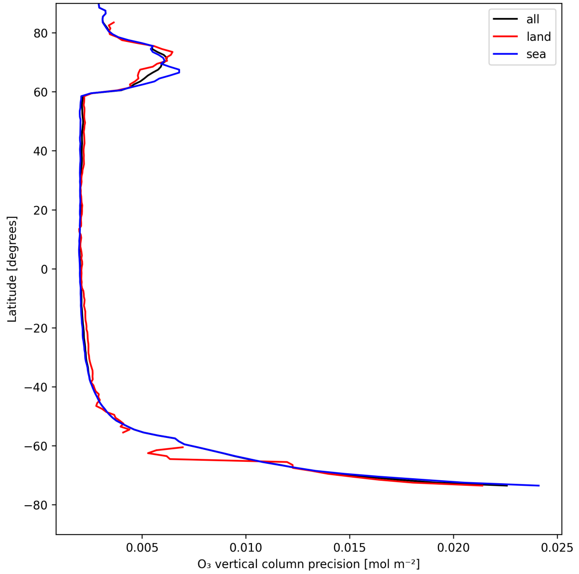
Figure 18: Zonal average of “O 3 vertical column precision” for 2025-08-10 to 2025-08-11.
