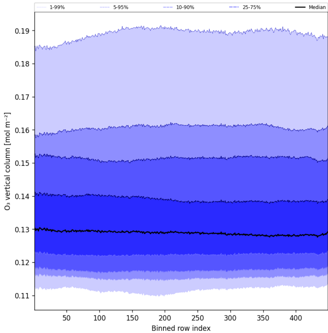
Figure 41: Along track statistics of “O 3 vertical column” for 2025-08-10 to 2025-08-11
