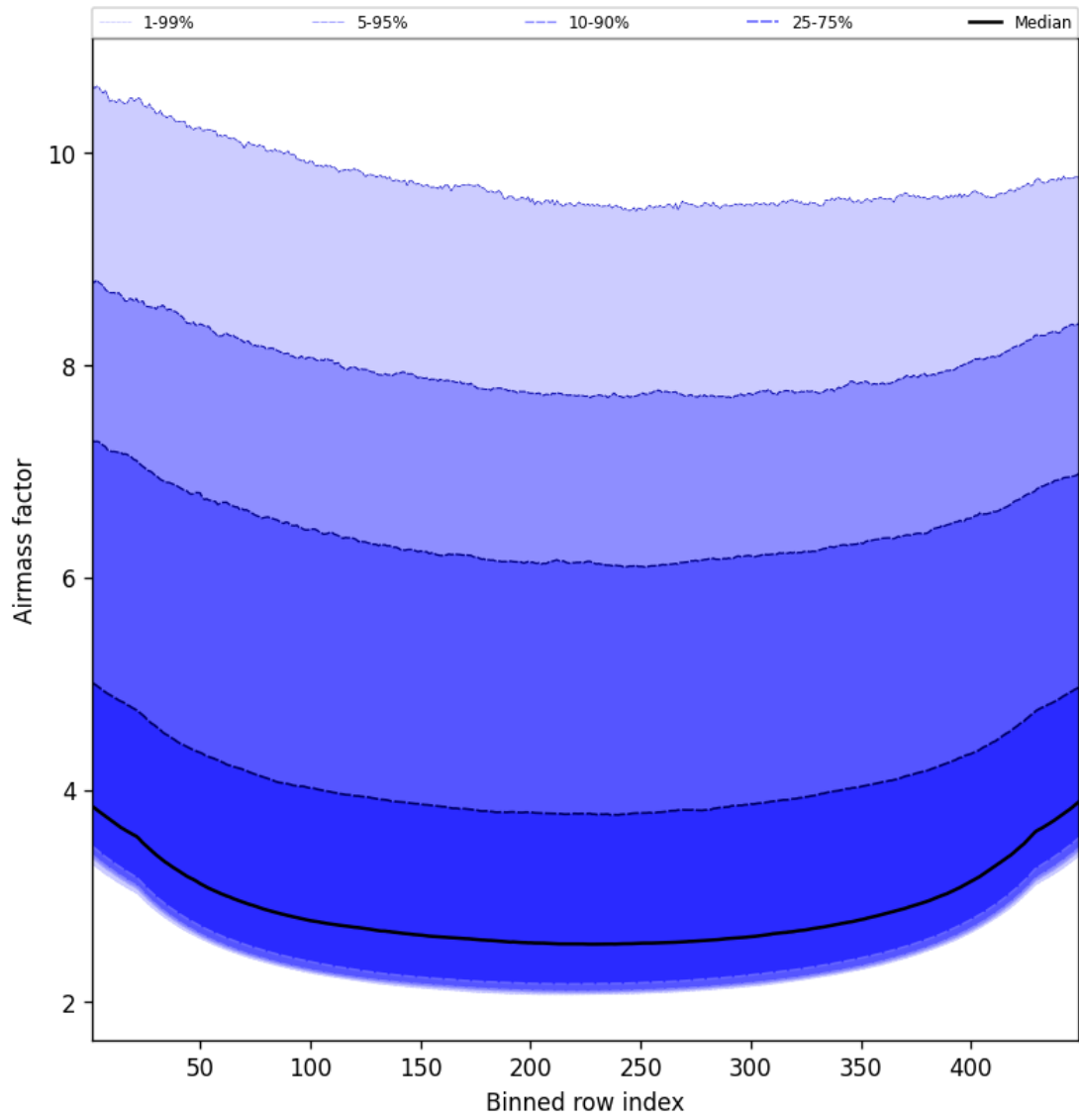
Figure 49: Along track statistics of “Airmass factor” for 2025-08-11 to 2025-08-12
