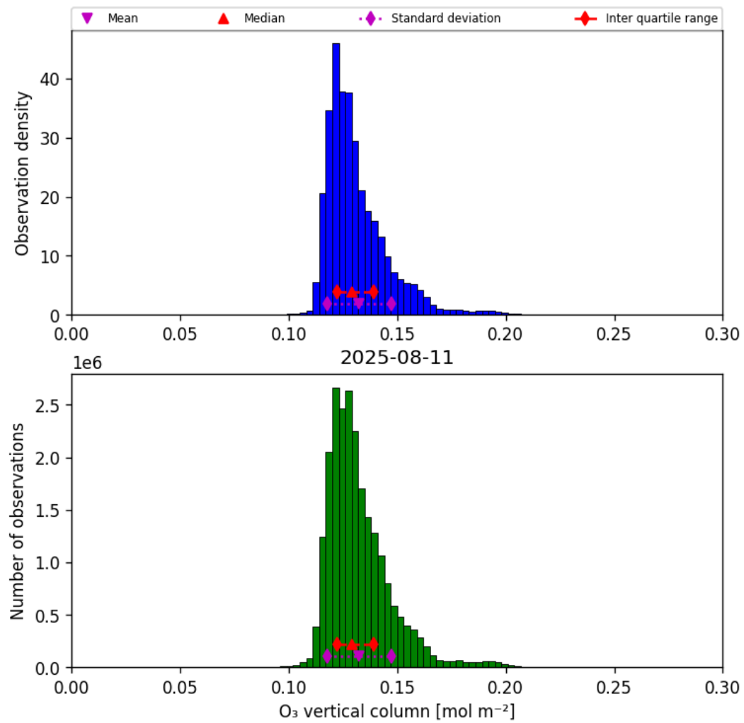
Figure 29: Histogram of “O 3 vertical column” for 2025-08-11 to 2025-08-12
