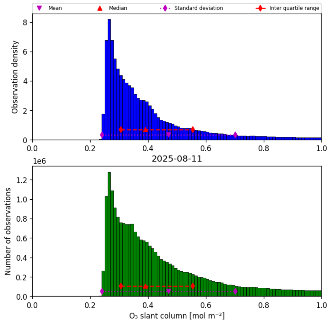
Figure 31: Histogram of “O 3 slant column” for 2025-08-11 to 2025-08-12
