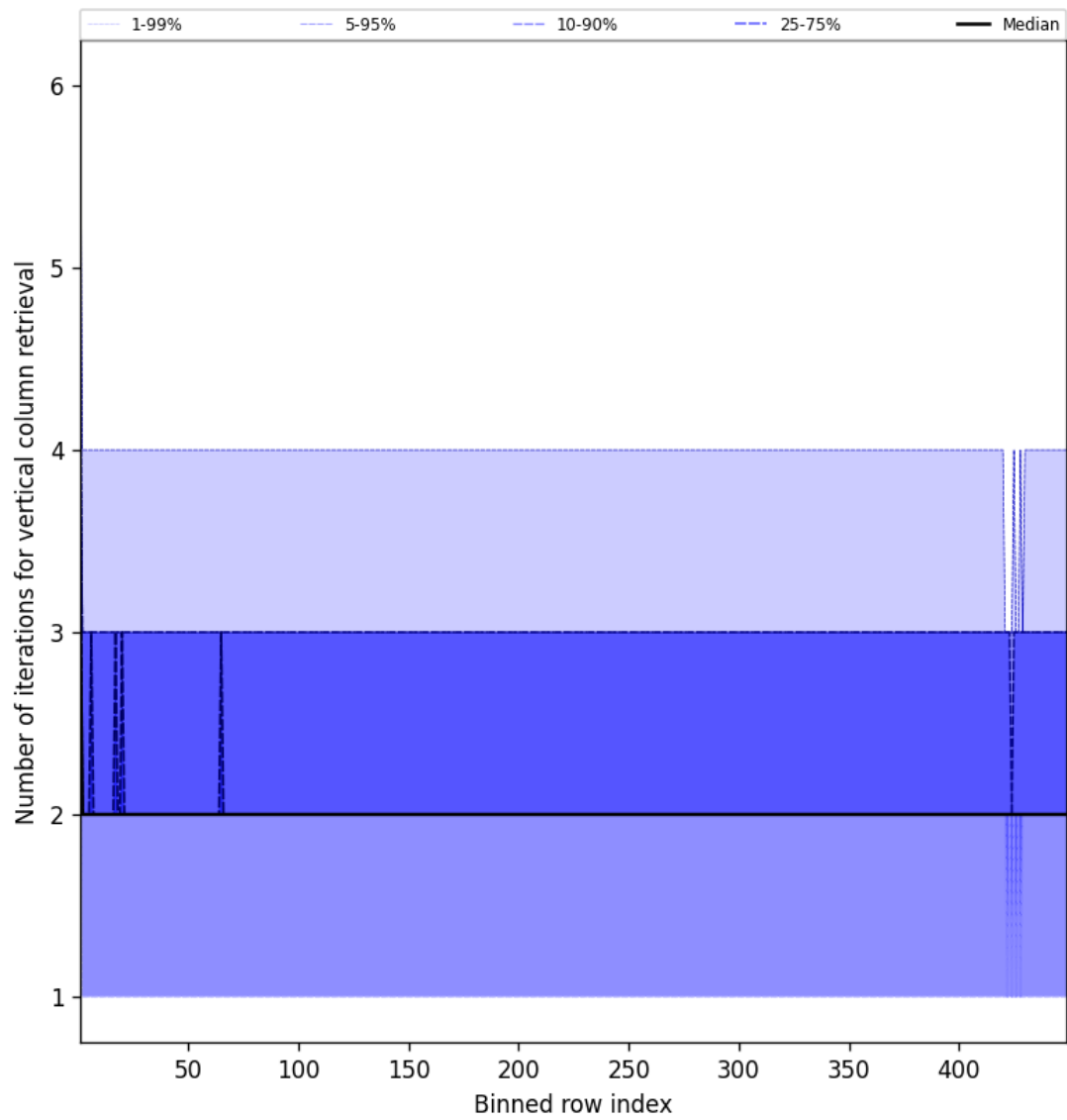
Figure 51: Along track statistics of “Number of iterations for vertical column retrieval” for 2025-08-11 to 2025-08-12
