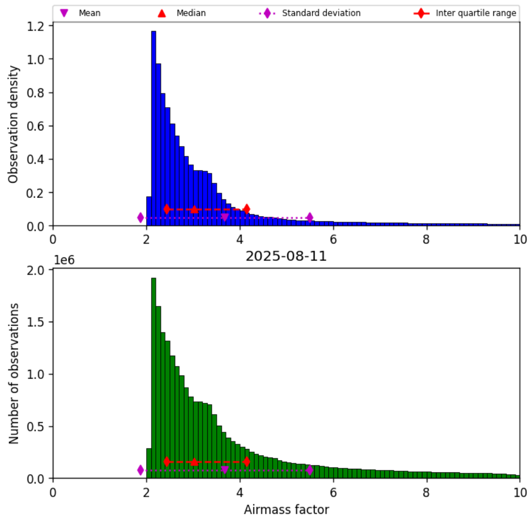
Figure 37: Histogram of “Airmass factor” for 2025-08-11 to 2025-08-12
