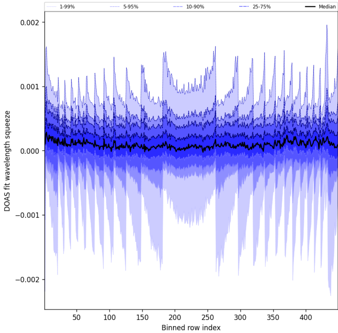
Figure 48: Along track statistics of “DOAS fit wavelength squeeze” for 2025-08-11 to 2025-08-12
