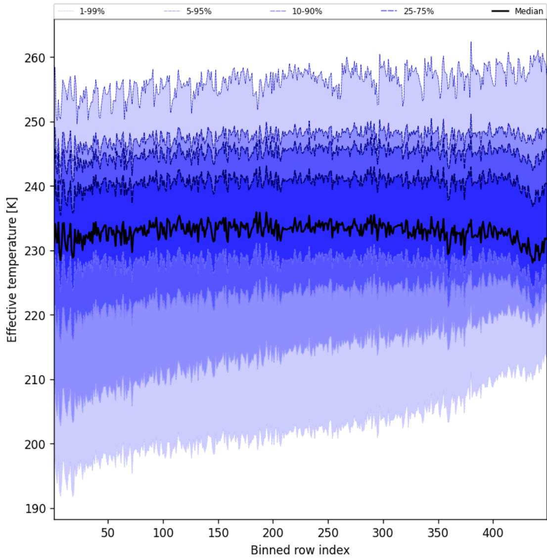
Figure 50: Along track statistics of “Effective temperature” for 2025-08-11 to 2025-08-12
