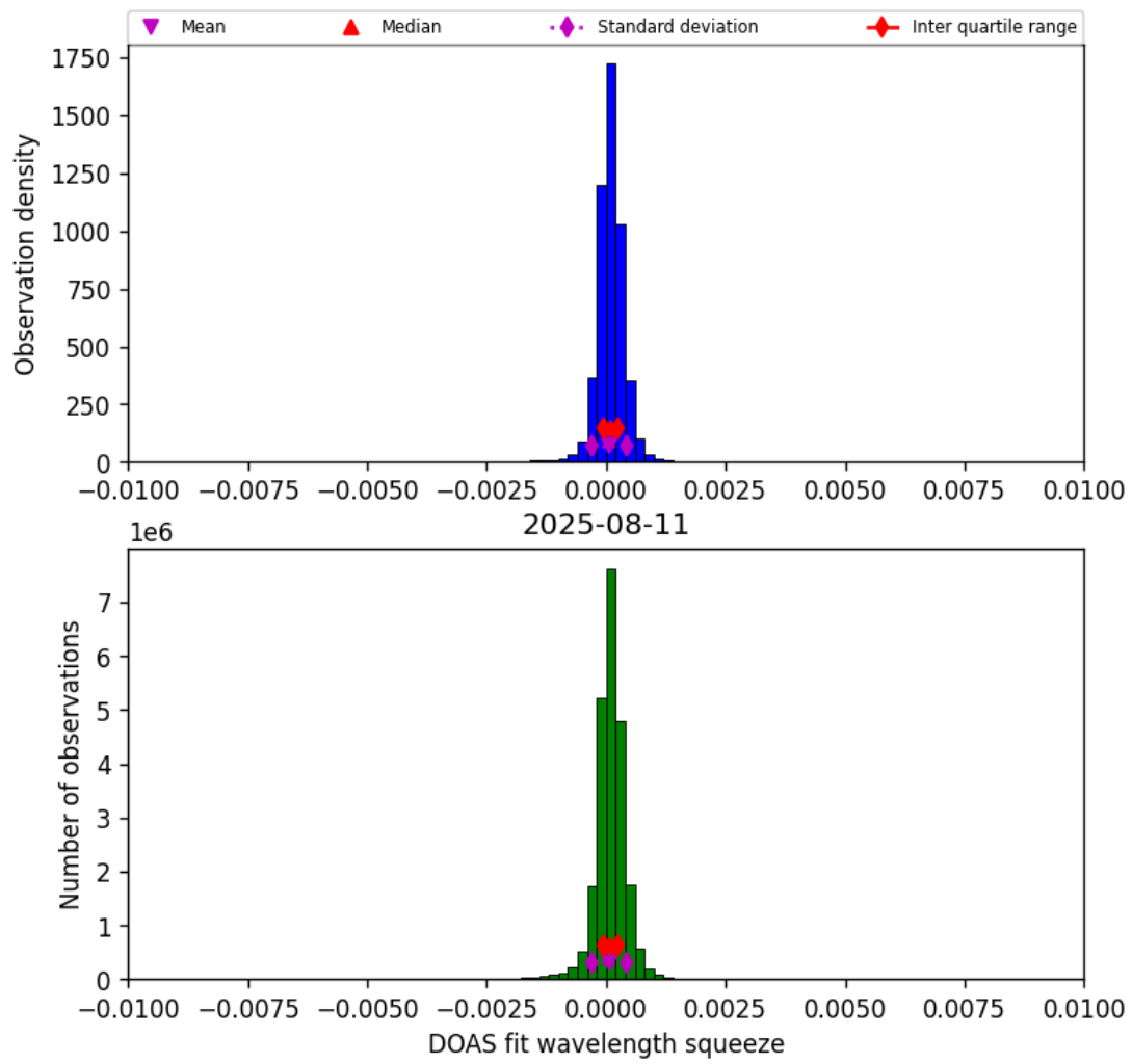
Figure 36: Histogram of “DOAS fit wavelength squeeze” for 2025-08-11 to 2025-08-12
