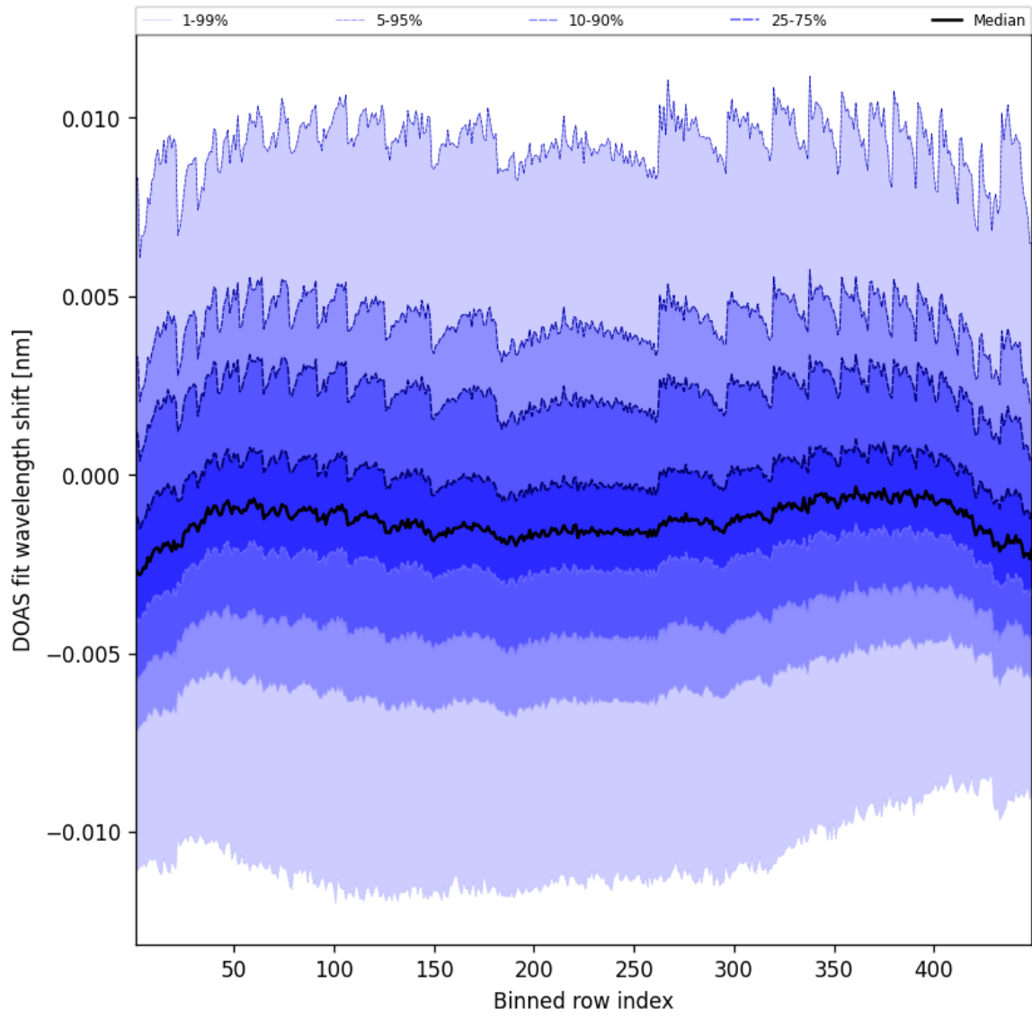
Figure 47: Along track statistics of “DOAS fit wavelength shift” for 2025-08-11 to 2025-08-12
