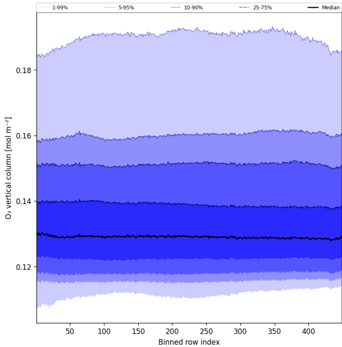
Figure 41: Along track statistics of “ \text{O}_3 vertical column” for 2025-08-11 to 2025-08-12
