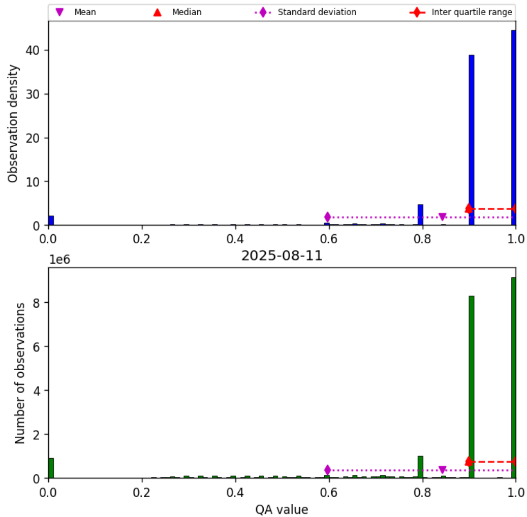
Figure 28: Histogram of “QA value” for 2025-08-11 to 2025-08-12
