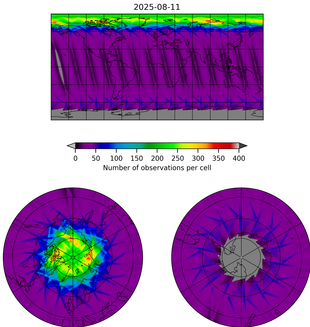
Figure 15: Map of the number of observations for 2025-08-11 to 2025-08-12
