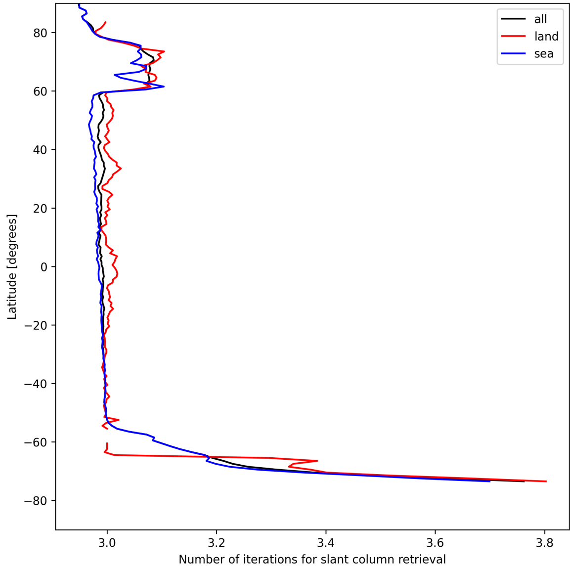
Figure 21: Zonal average of “Number of iterations for slant column retrieval” for 2025-08-11 to 2025-08-12.
