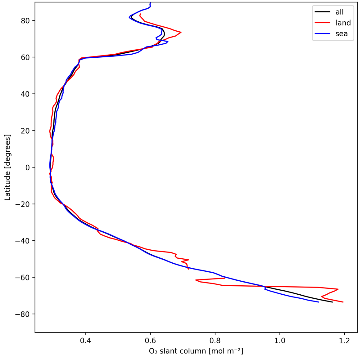
Figure 19: Zonal average of “O 3 slant column” for 2025-08-11 to 2025-08-12.
