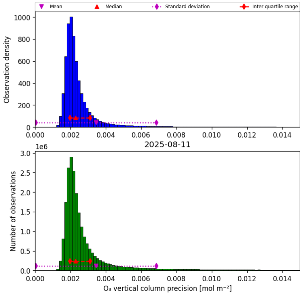
Figure 30: Histogram of “O 3 vertical column precision” for 2025-08-11 to 2025-08-12
