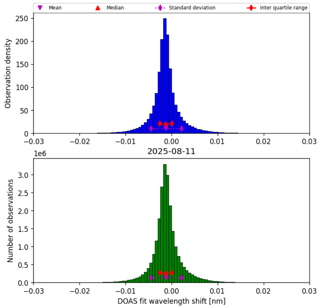
Figure 35: Histogram of “DOAS fit wavelength shift” for 2025-08-11 to 2025-08-12
