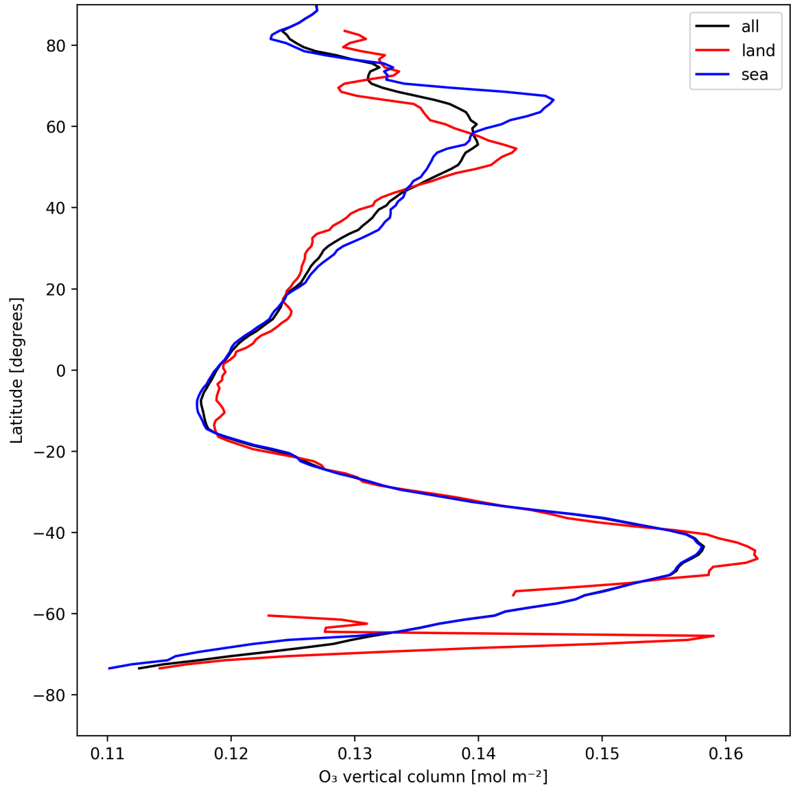
Figure 17: Zonal average of “O 3 vertical column” for 2025-08-11 to 2025-08-12.
