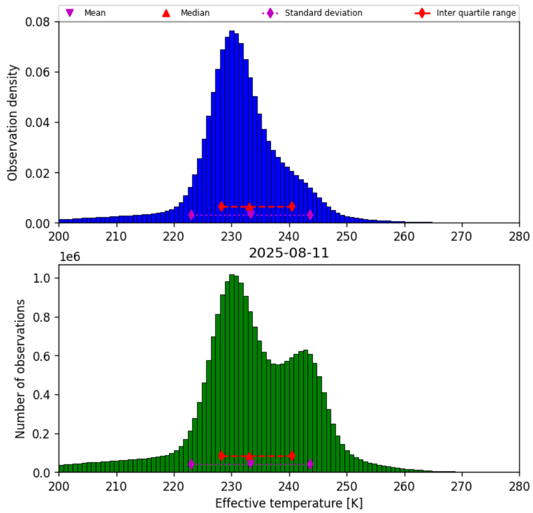
Figure 38: Histogram of “Effective temperature” for 2025-08-11 to 2025-08-12
