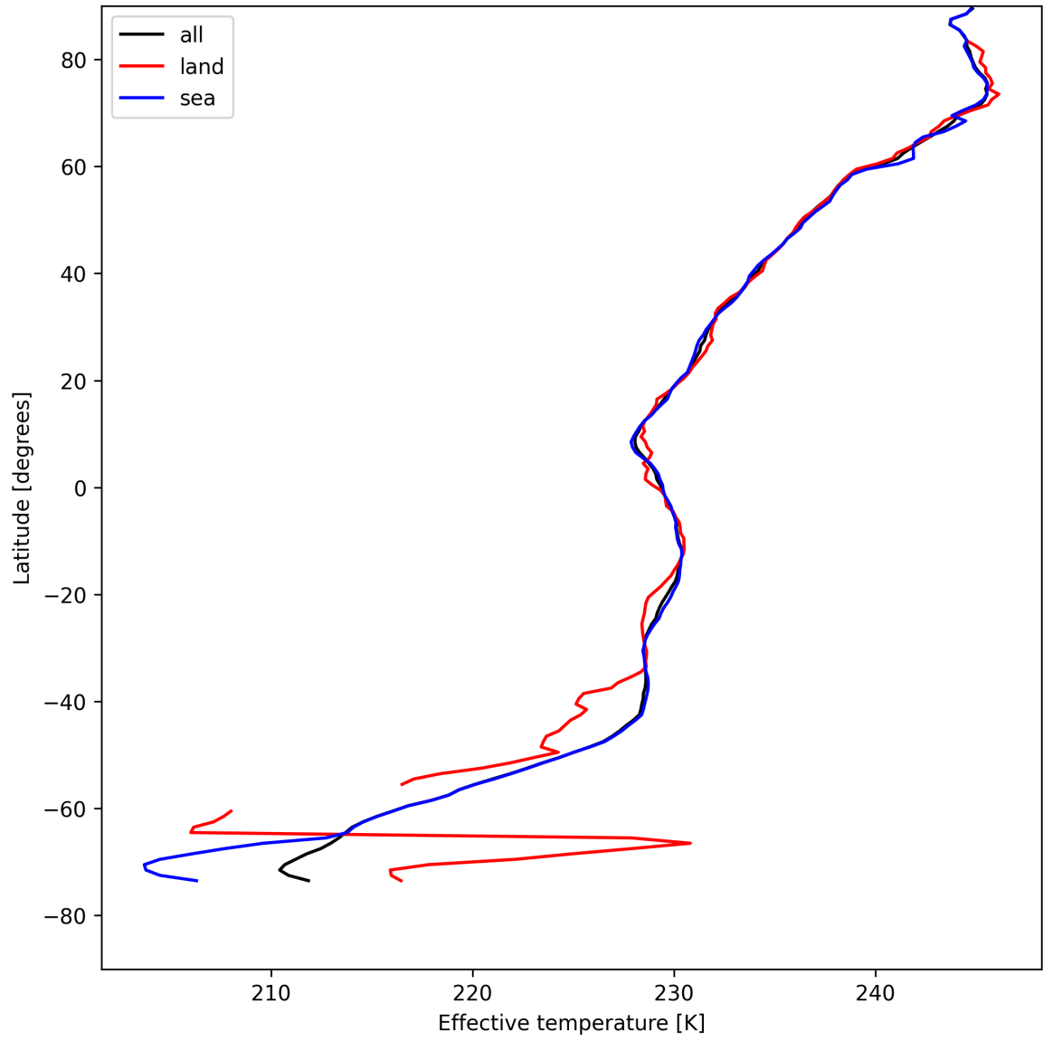
Figure 26: Zonal average of "Effective temperature" for 2025-08-11 to 2025-08-12.
