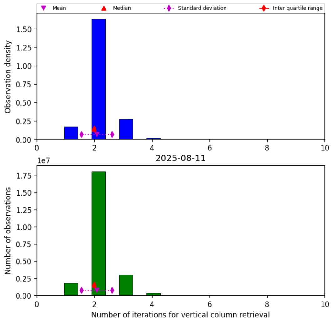
Figure 39: Histogram of “Number of iterations for vertical column retrieval” for 2025-08-11 to 2025-08-12
