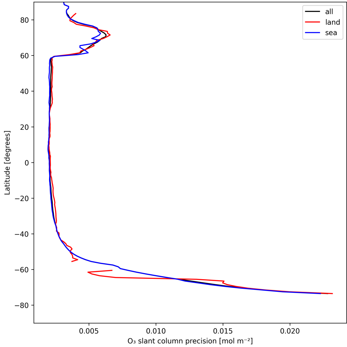
Figure 20: Zonal average of “O 3 slant column precision” for 2025-08-11 to 2025-08-12.
