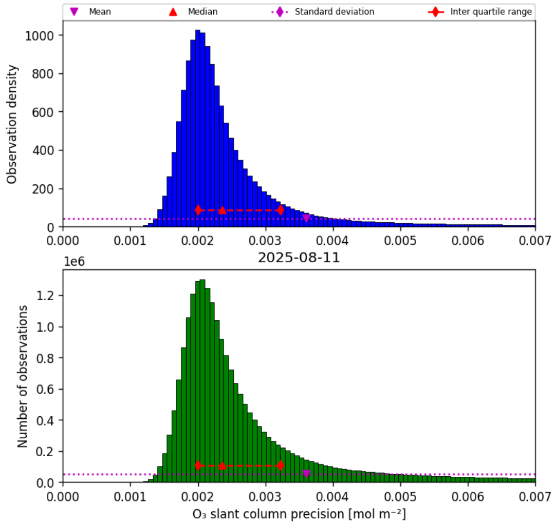
Figure 32: Histogram of “O 3 slant column precision” for 2025-08-11 to 2025-08-12
