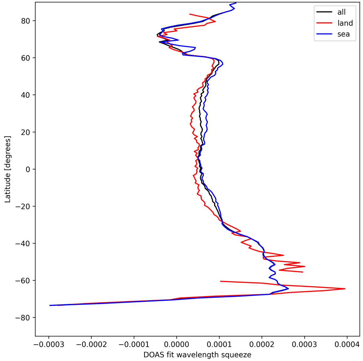
Figure 24: Zonal average of “DOAS fit wavelength squeeze” for 2025-08-11 to 2025-08-12.
