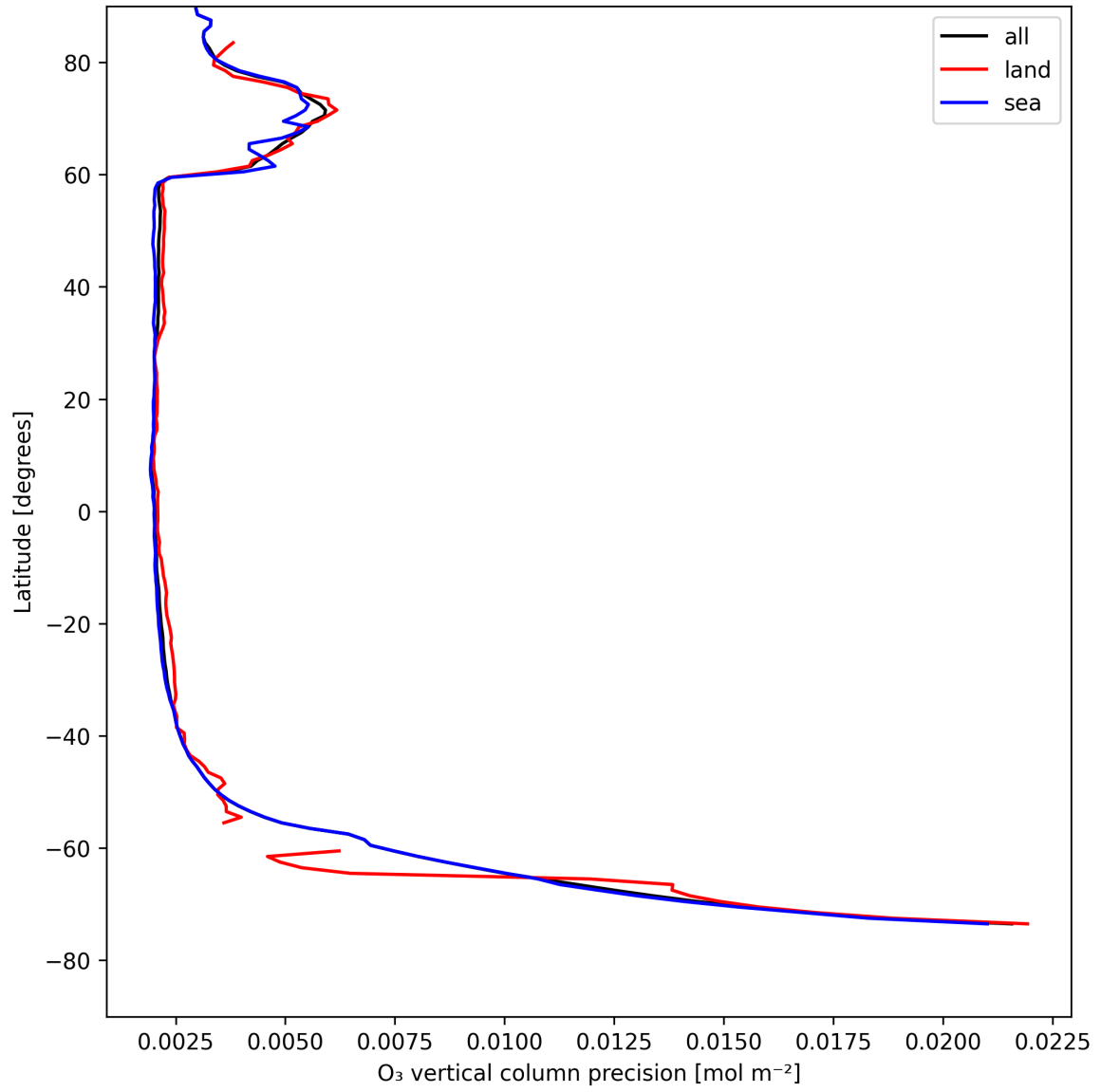
Figure 18: Zonal average of "O 3 vertical column precision" for 2025-08-11 to 2025-08-12.
