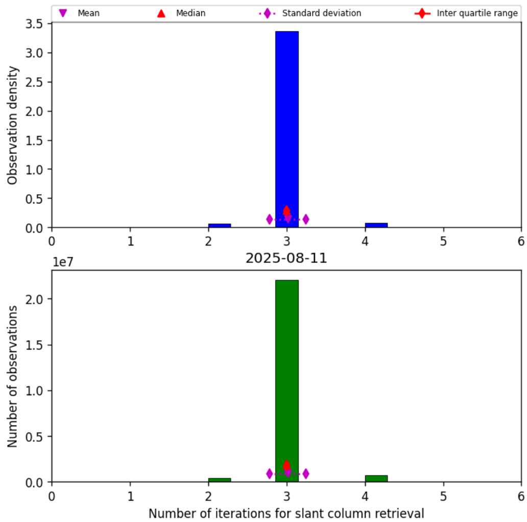
Figure 33: Histogram of "Number of iterations for slant column retrieval" for 2025-08-11 to 2025-08-12
