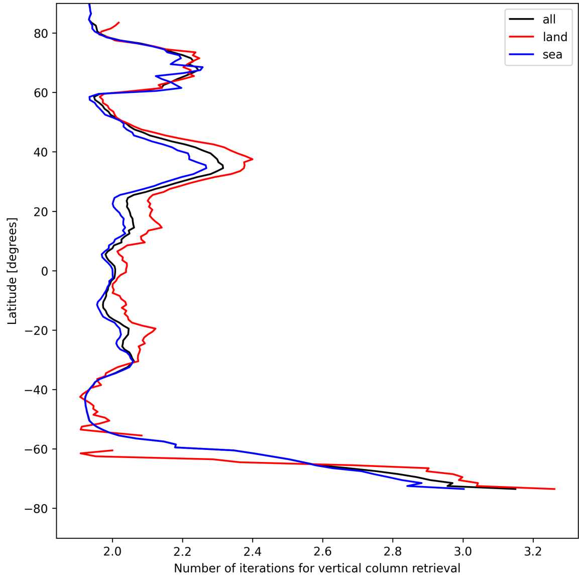
Figure 27: Zonal average of “Number of iterations for vertical column retrieval” for 2025-08-11 to 2025-08-12.
