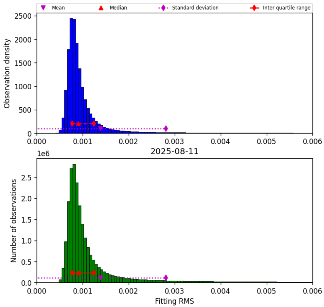
Figure 34: Histogram of “Fitting RMS” for 2025-08-11 to 2025-08-12
