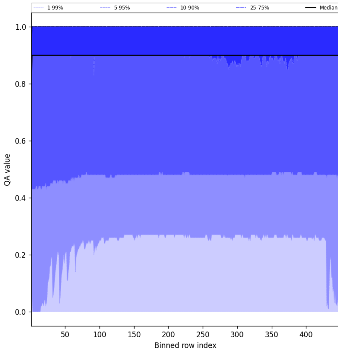
Figure 40: Along track statistics of “QA value” for 2025-08-11 to 2025-08-12
