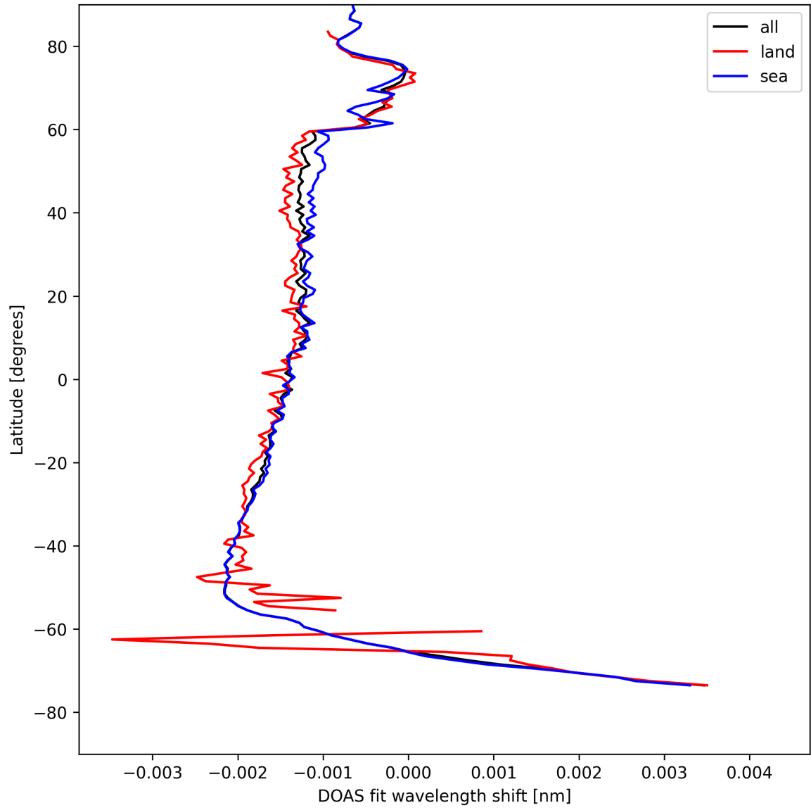
Figure 23: Zonal average of “DOAS fit wavelength shift” for 2025-08-11 to 2025-08-12.
