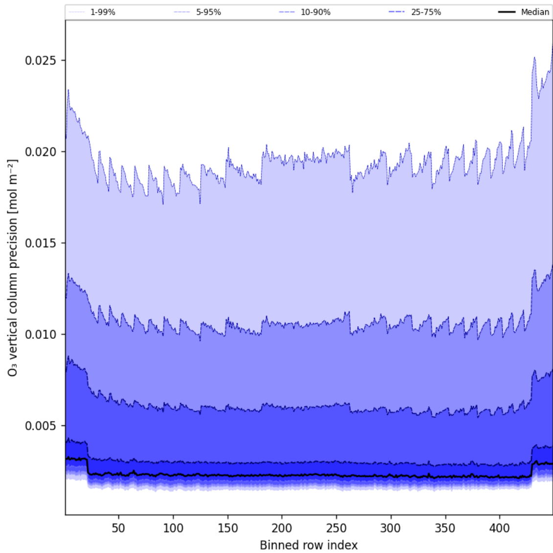
Figure 42: Along track statistics of “O 3 vertical column precision” for 2025-08-11 to 2025-08-12
