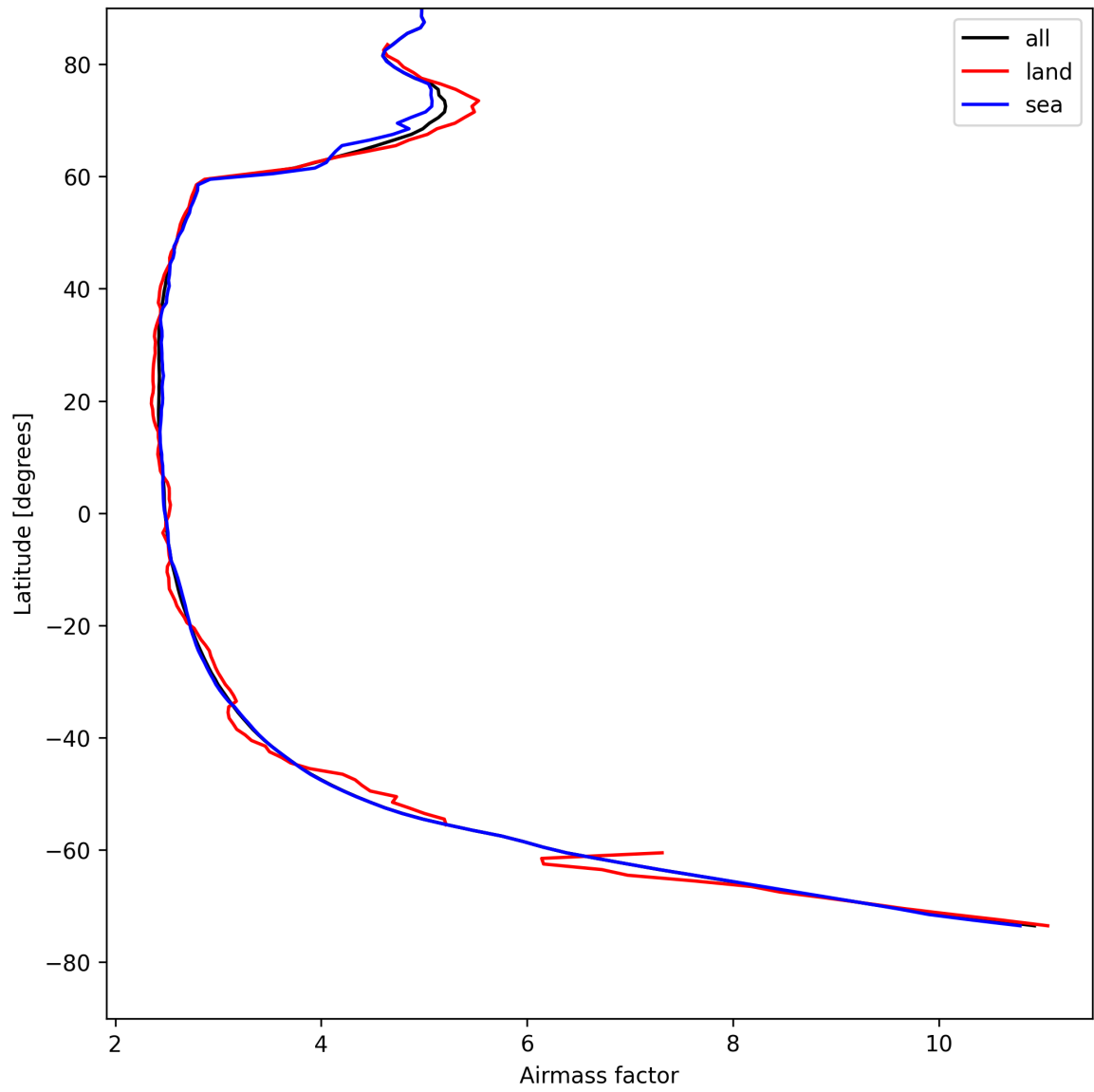
Figure 25: Zonal average of “Airmass factor” for 2025-08-11 to 2025-08-12.
