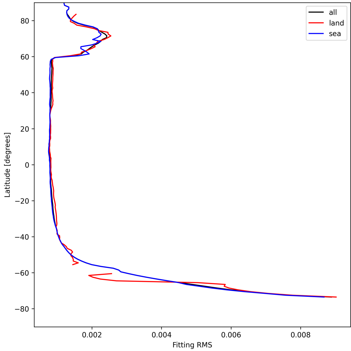
Figure 22: Zonal average of “Fitting RMS” for 2025-08-11 to 2025-08-12.
