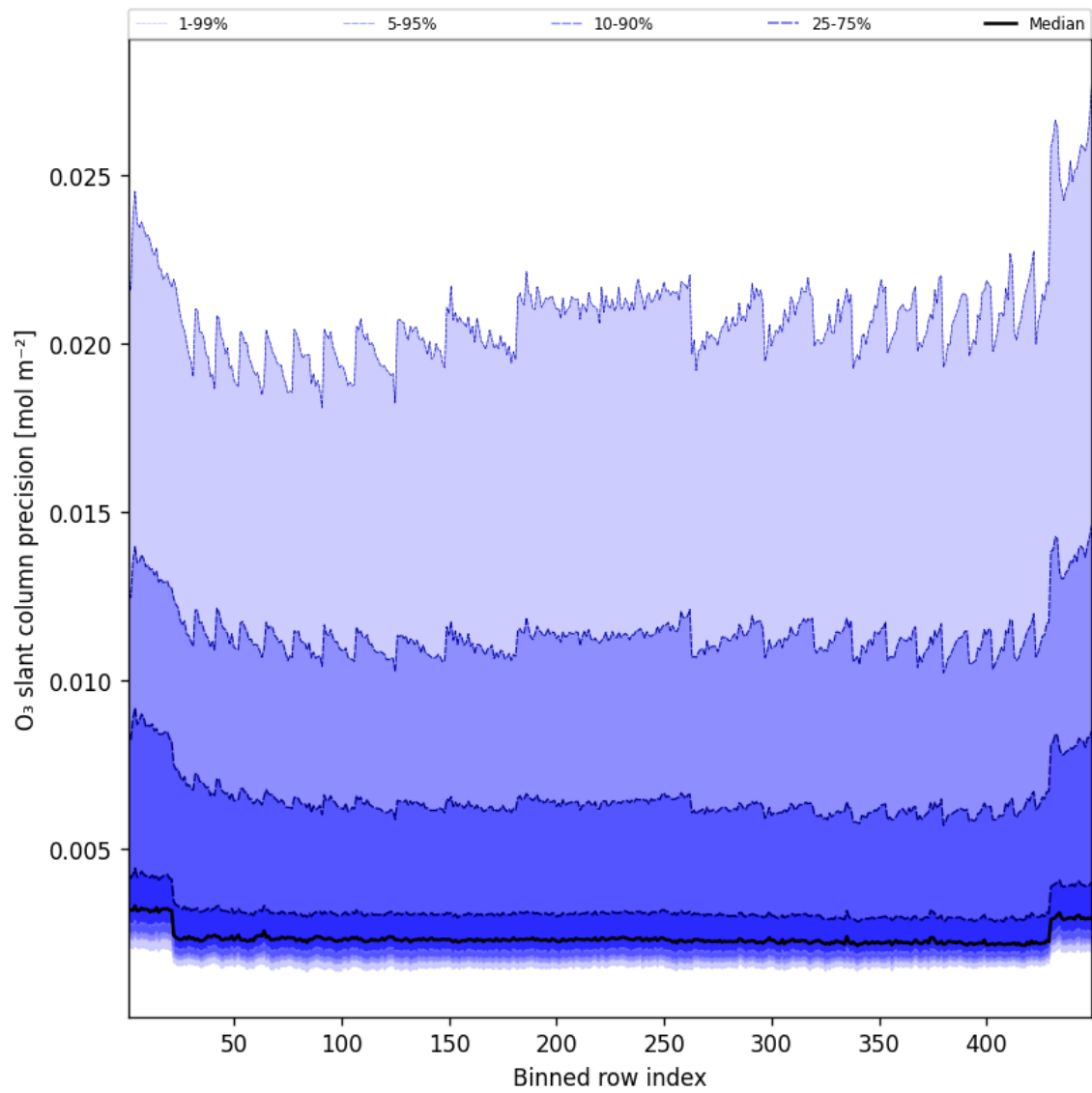
Figure 44: Along track statistics of “O 3 slant column precision” for 2025-08-11 to 2025-08-12
