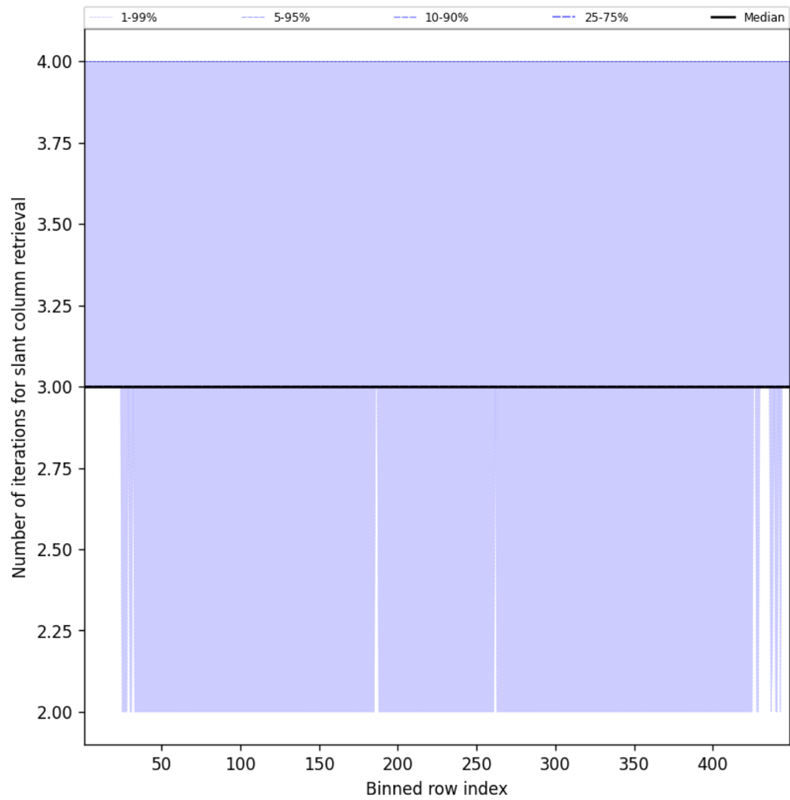
Figure 45: Along track statistics of “Number of iterations for slant column retrieval” for 2025-08-11 to 2025-08-12
