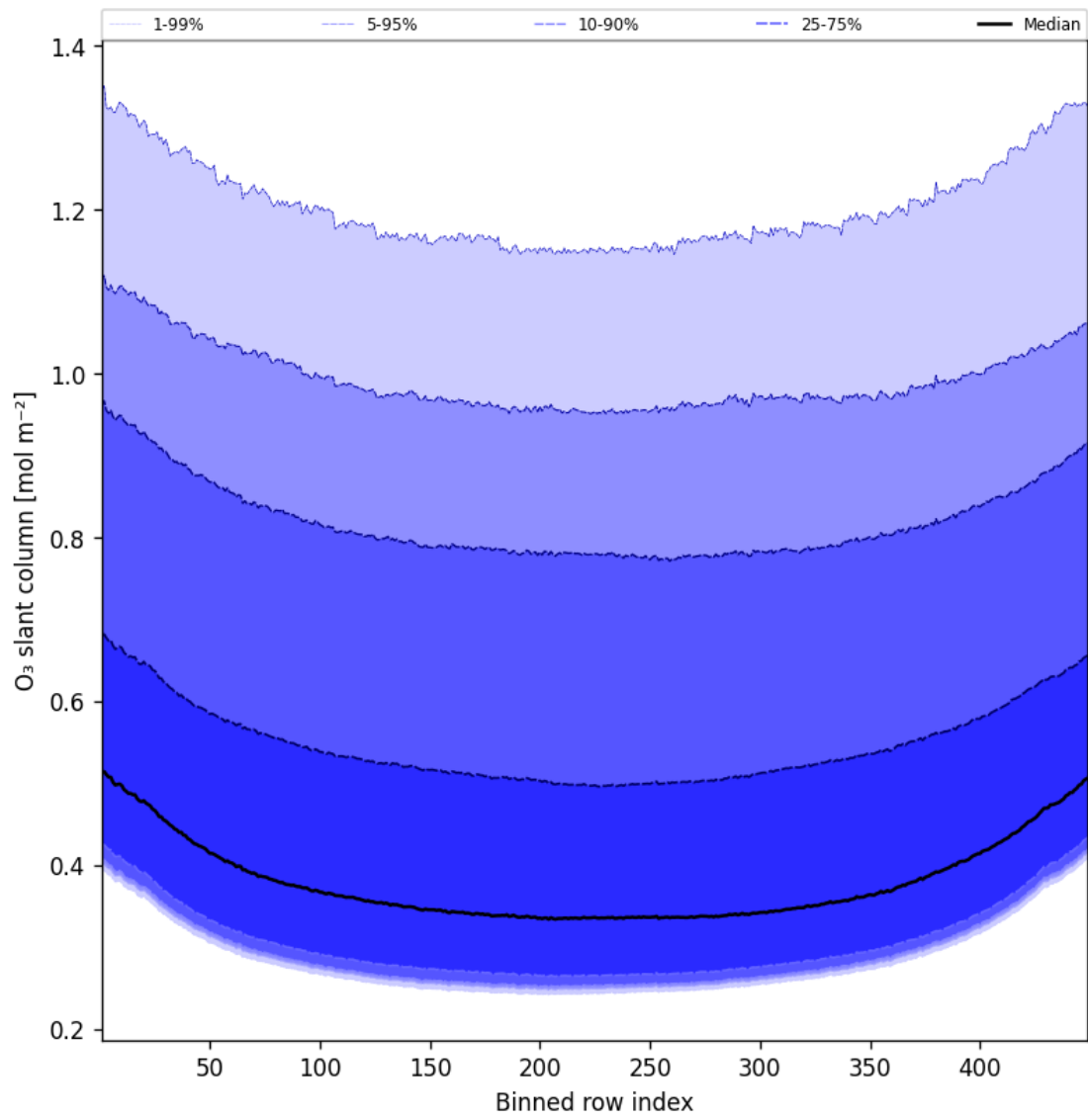
Figure 43: Along track statistics of “O 3 slant column” for 2025-08-11 to 2025-08-12
