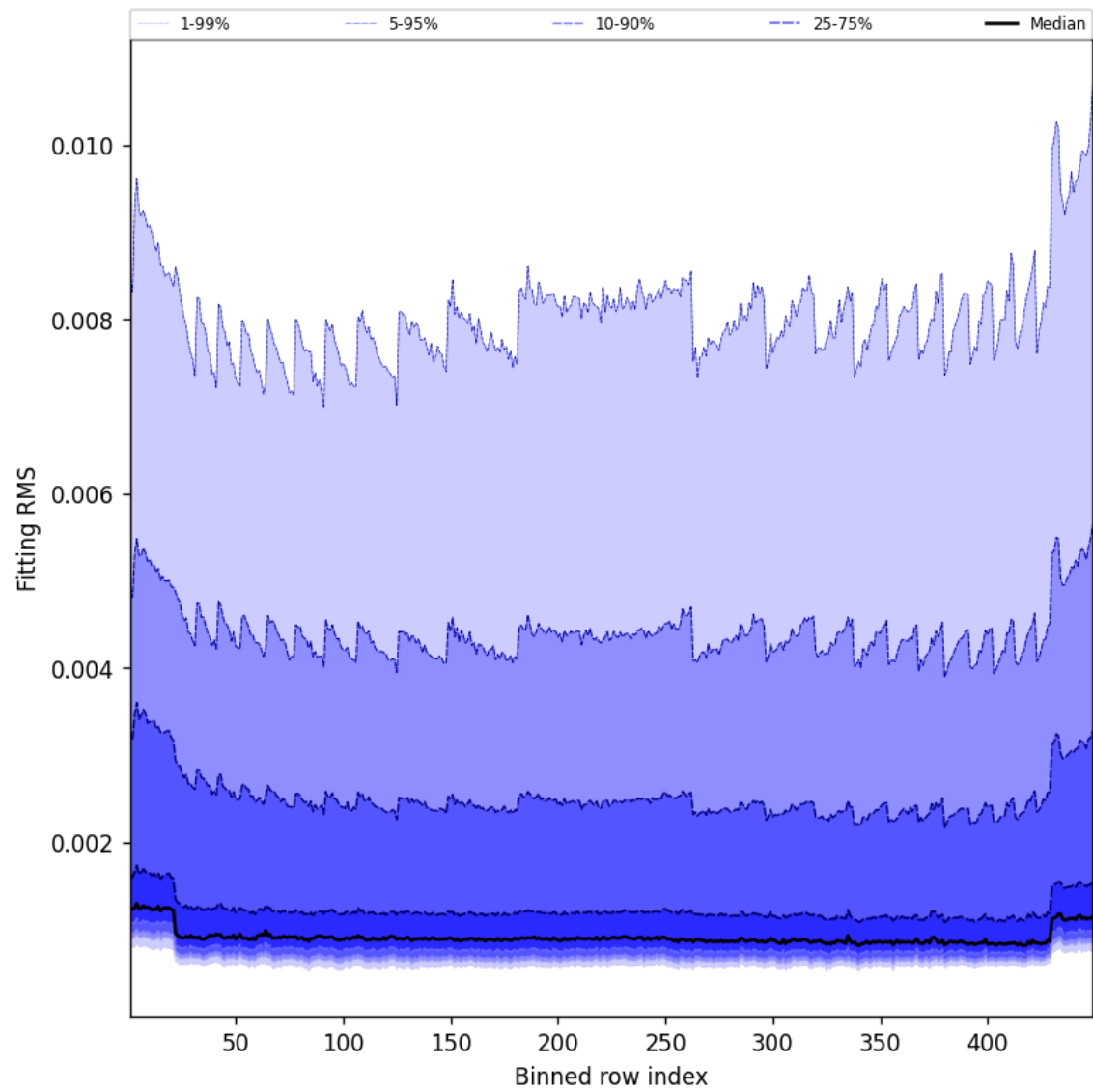
Figure 46: Along track statistics of “Fitting RMS” for 2025-08-11 to 2025-08-12
