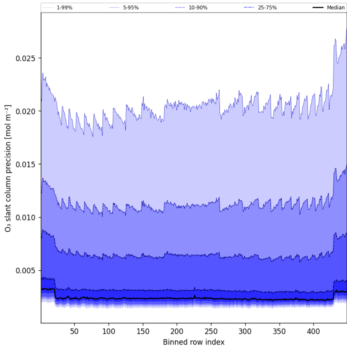
Figure 44: Along track statistics of “O 3 slant column precision” for 2025-08-12 to 2025-08-12
