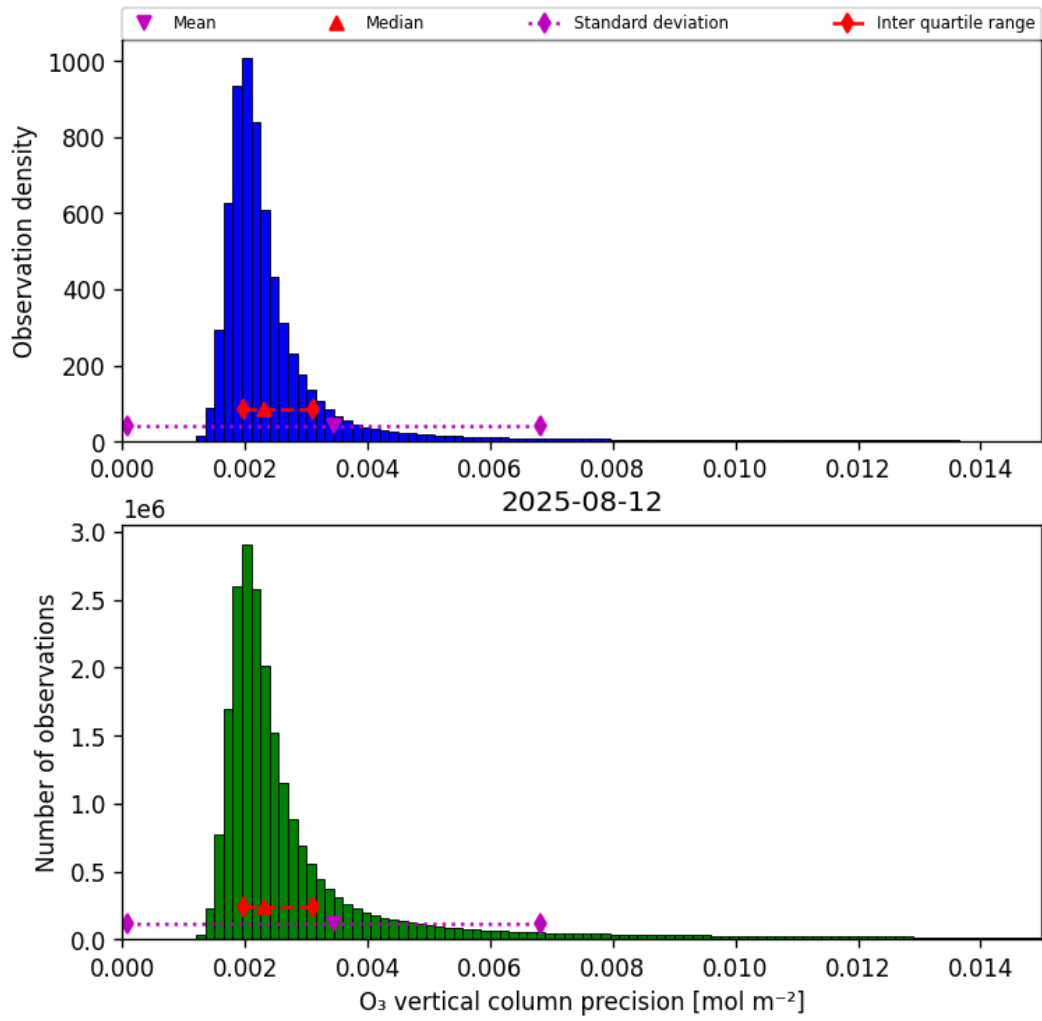
Figure 30: Histogram of “O 3 vertical column precision” for 2025-08-12 to 2025-08-12
