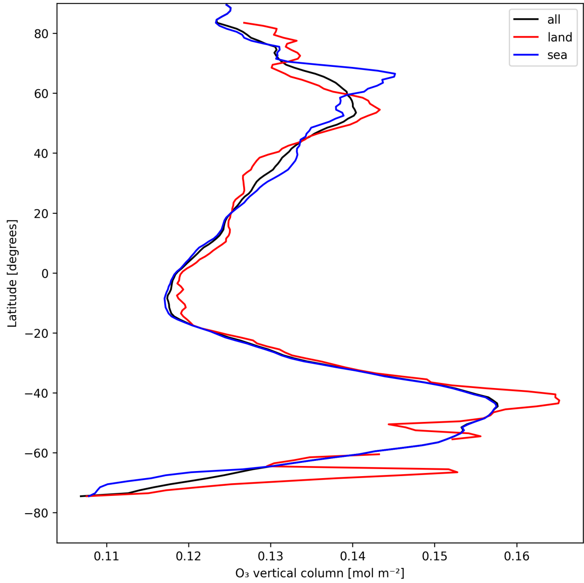
Figure 17: Zonal average of “O 3 vertical column” for 2025-08-12 to 2025-08-12.
