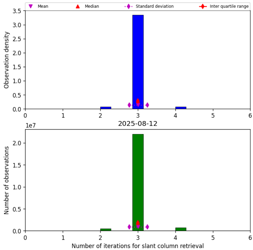
Figure 33: Histogram of “Number of iterations for slant column retrieval” for 2025-08-12 to 2025-08-12
