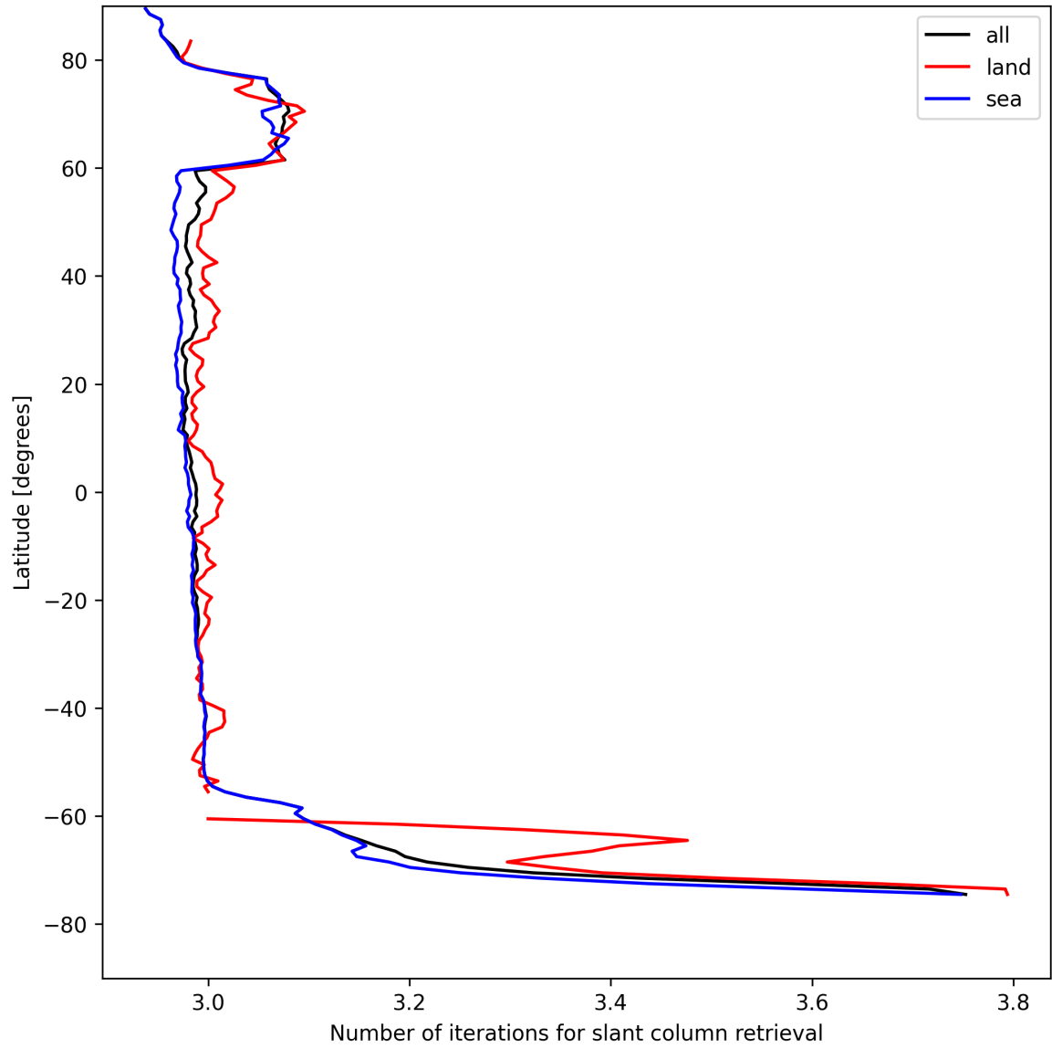
Figure 21: Zonal average of “Number of iterations for slant column retrieval” for 2025-08-12 to 2025-08-12.
