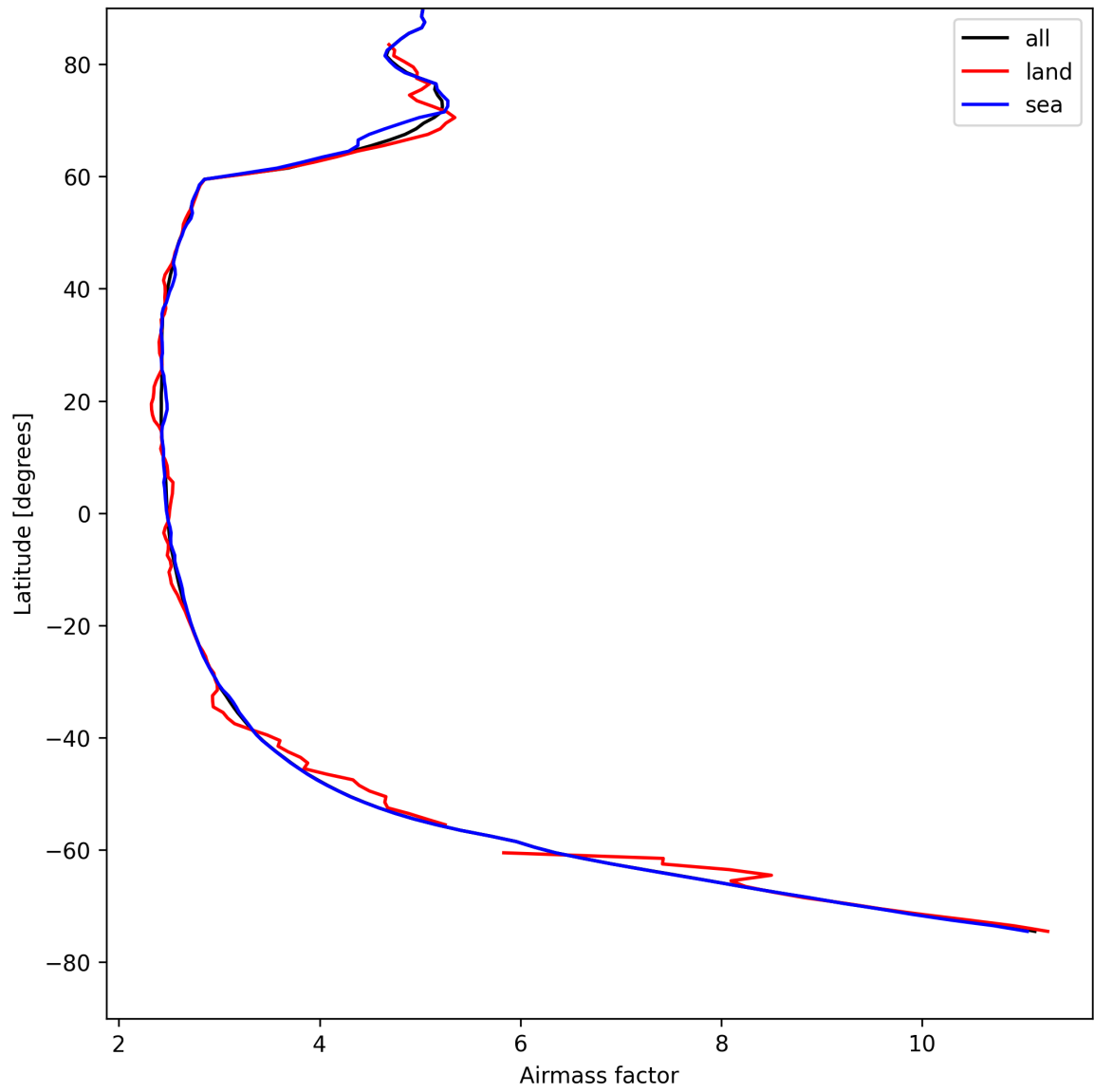
Figure 25: Zonal average of “Airmass factor” for 2025-08-12 to 2025-08-12.
