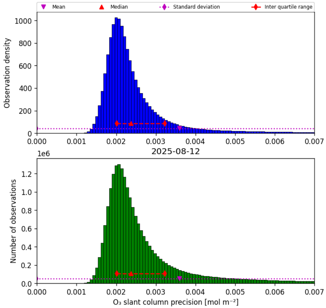
Figure 32: Histogram of “O 3 slant column precision” for 2025-08-12 to 2025-08-12
