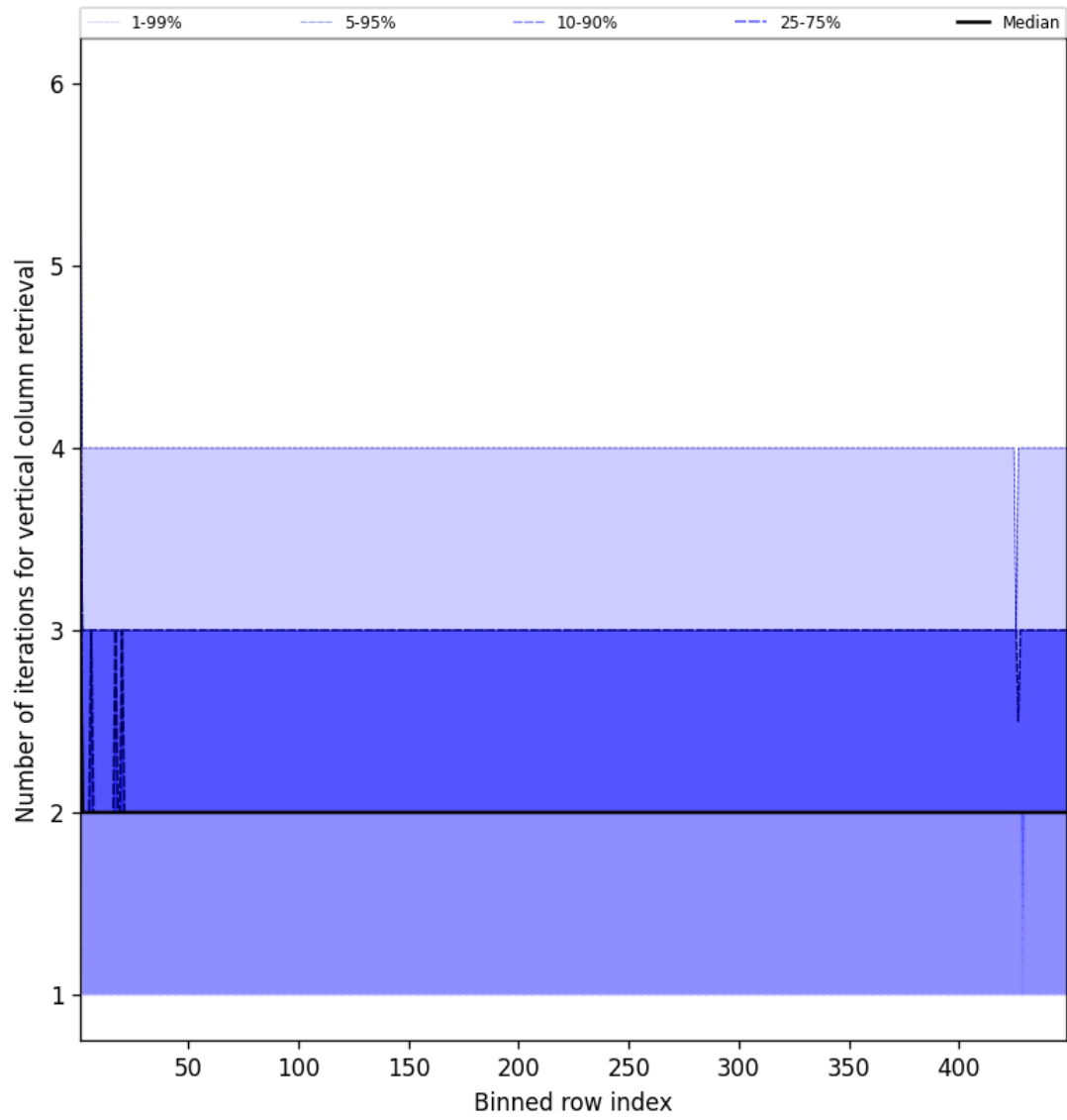
Figure 51: Along track statistics of “Number of iterations for vertical column retrieval” for 2025-08-12 to 2025-08-12
