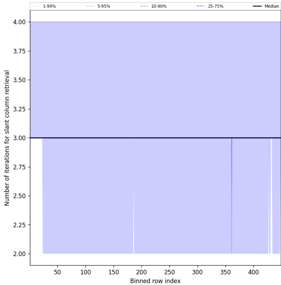
Figure 45: Along track statistics of “Number of iterations for slant column retrieval” for 2025-08-12 to 2025-08-12
