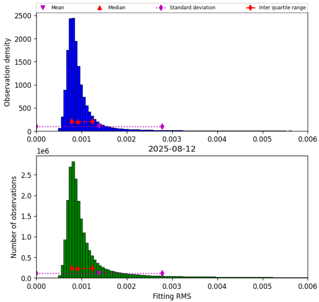
Figure 34: Histogram of “Fitting RMS” for 2025-08-12 to 2025-08-12
