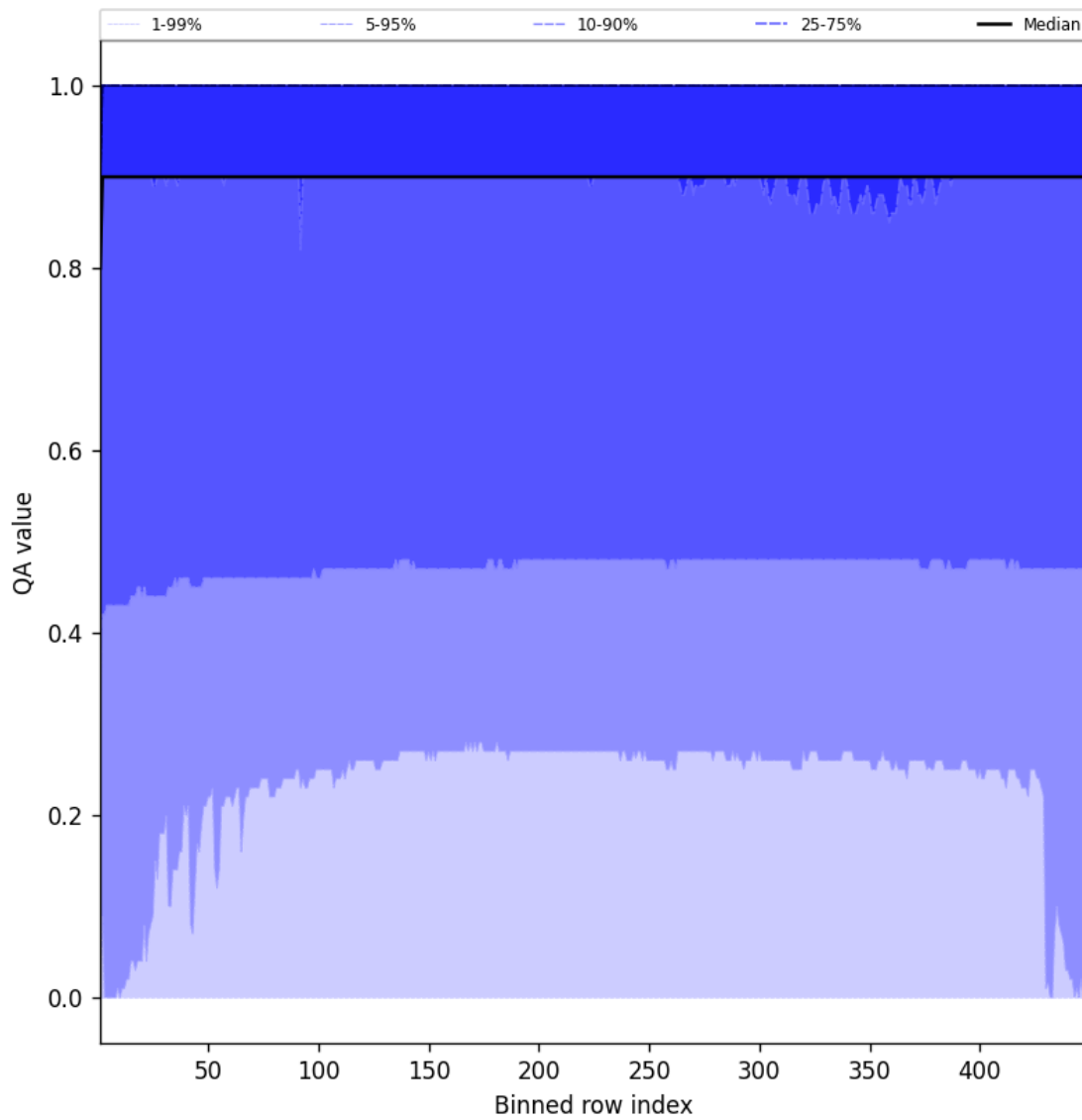
Figure 40: Along track statistics of “QA value” for 2025-08-12 to 2025-08-12
