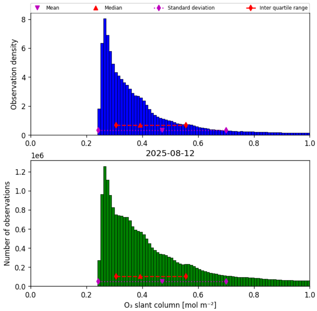
Figure 31: Histogram of “O 3 slant column” for 2025-08-12 to 2025-08-12
