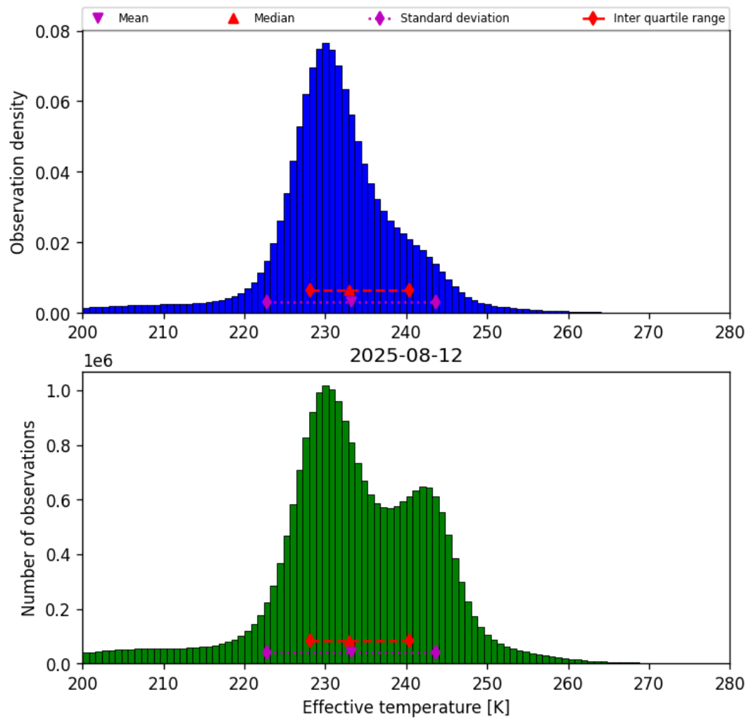
Figure 38: Histogram of “Effective temperature” for 2025-08-12 to 2025-08-12
