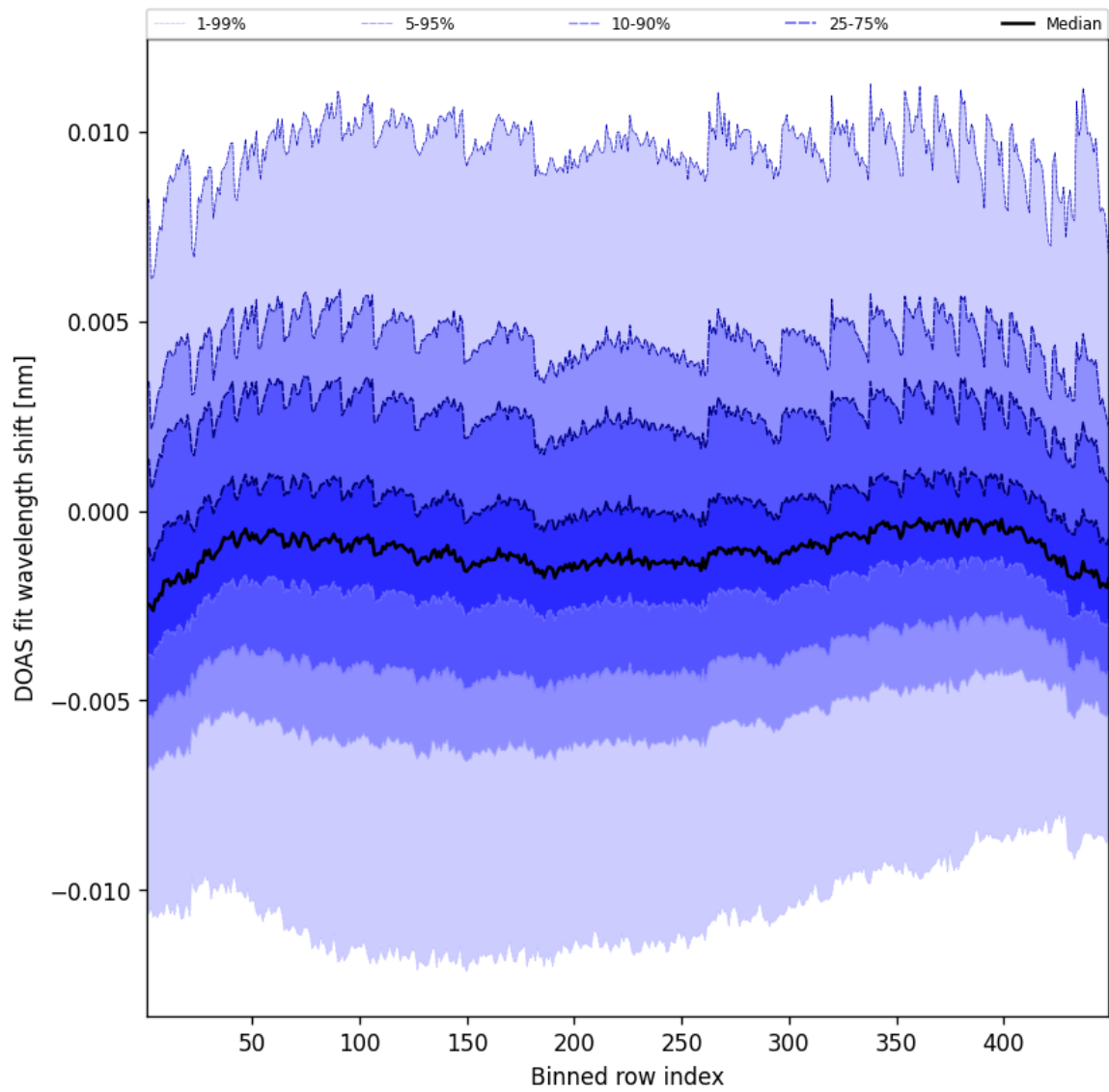
Figure 47: Along track statistics of “DOAS fit wavelength shift” for 2025-08-12 to 2025-08-12
