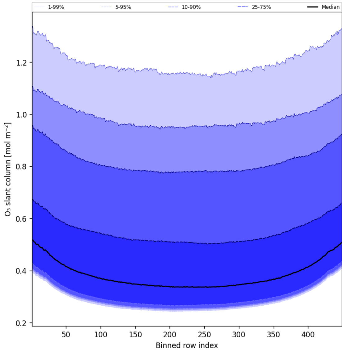
Figure 43: Along track statistics of “O 3 slant column” for 2025-08-12 to 2025-08-12
