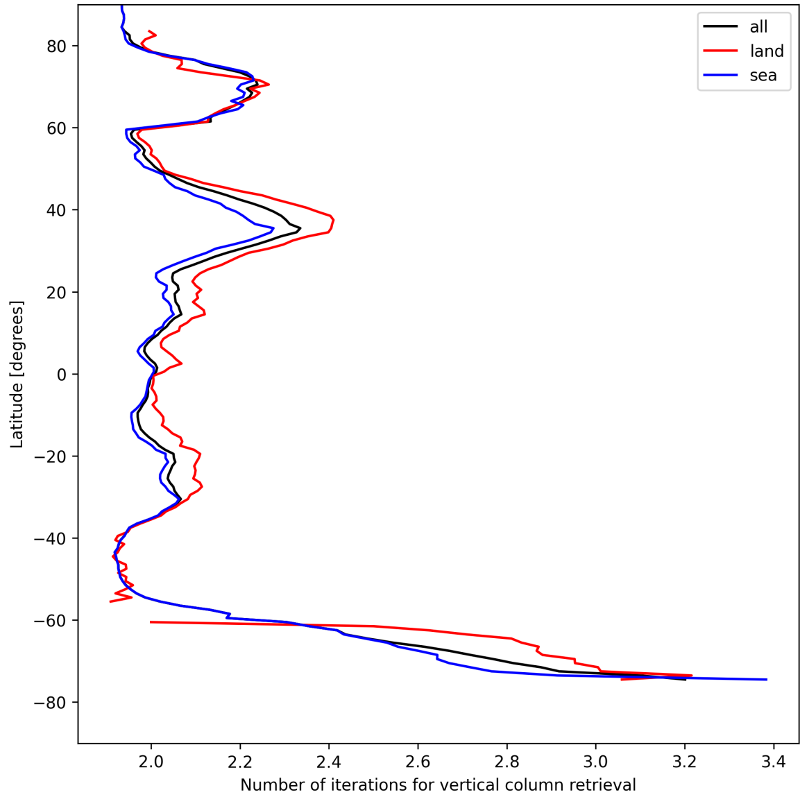
Figure 27: Zonal average of “Number of iterations for vertical column retrieval” for 2025-08-12 to 2025-08-12.
