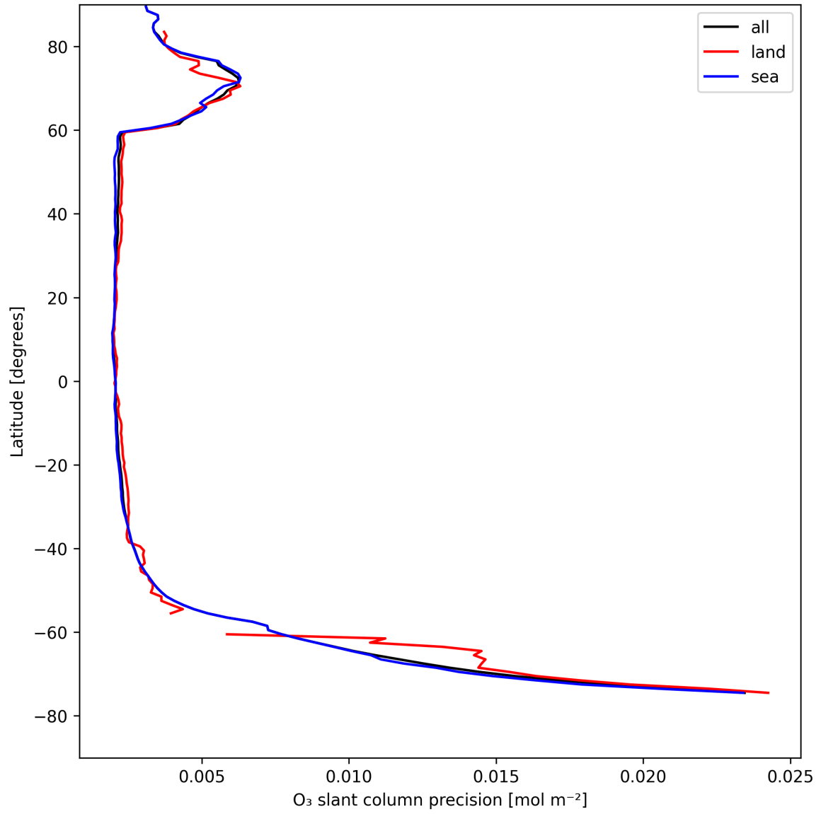
Figure 20: Zonal average of “O 3 slant column precision” for 2025-08-12 to 2025-08-12.
