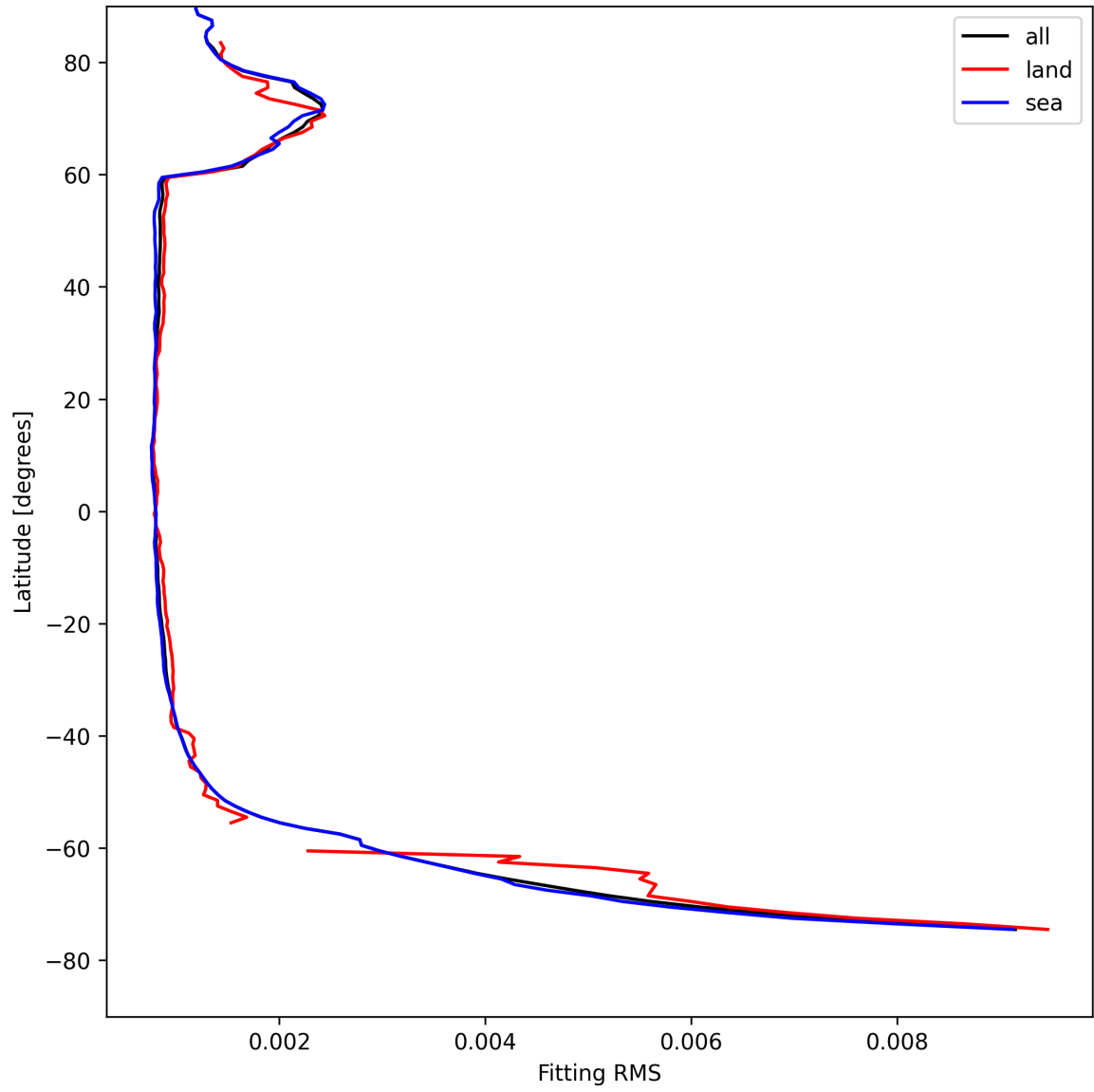
Figure 22: Zonal average of “Fitting RMS” for 2025-08-12 to 2025-08-12.
