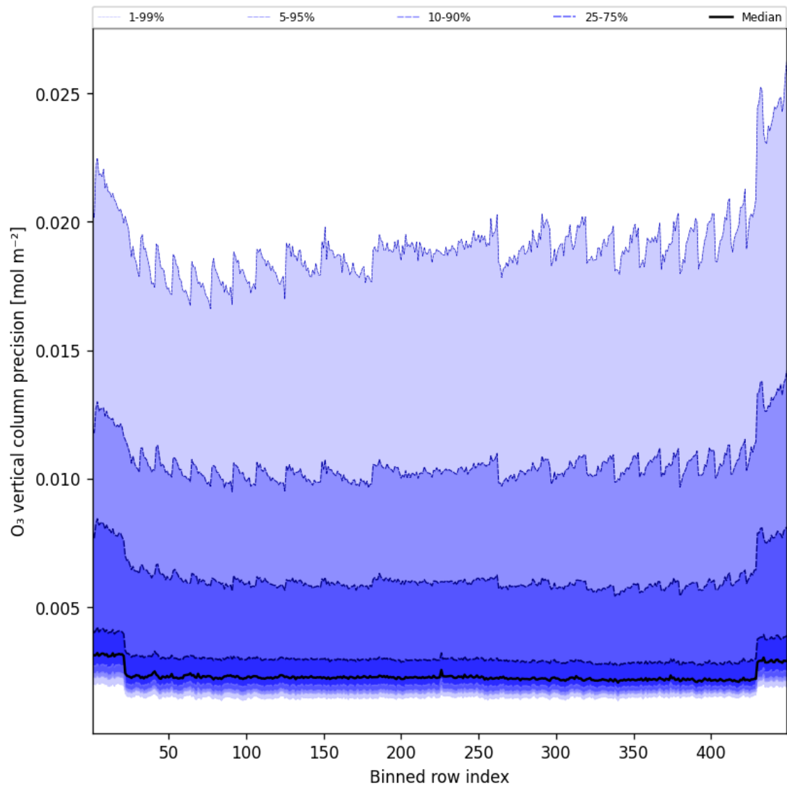
Figure 42: Along track statistics of “O 3 vertical column precision” for 2025-08-12 to 2025-08-12
