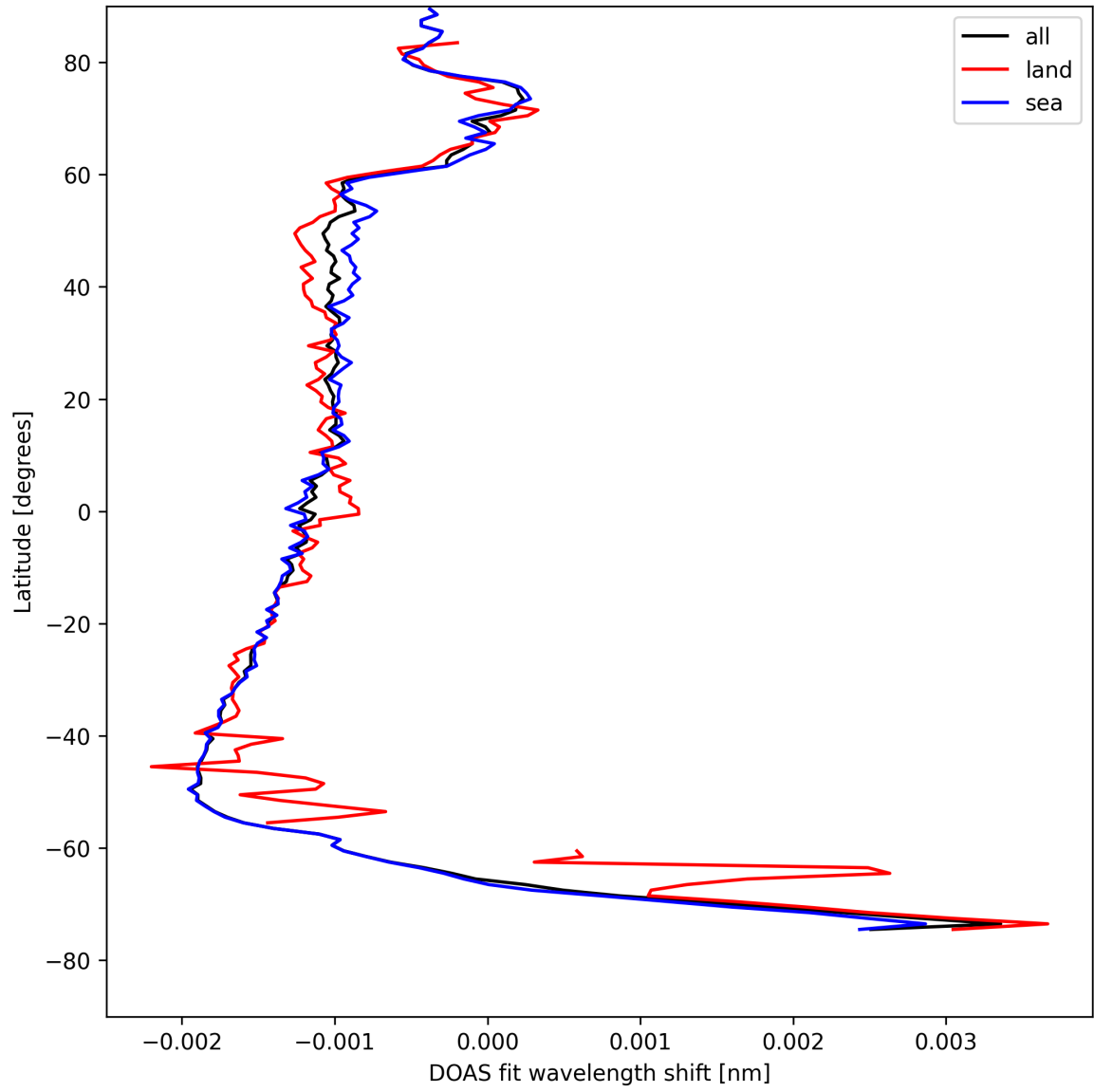
Figure 23: Zonal average of “DOAS fit wavelength shift” for 2025-08-12 to 2025-08-12.
