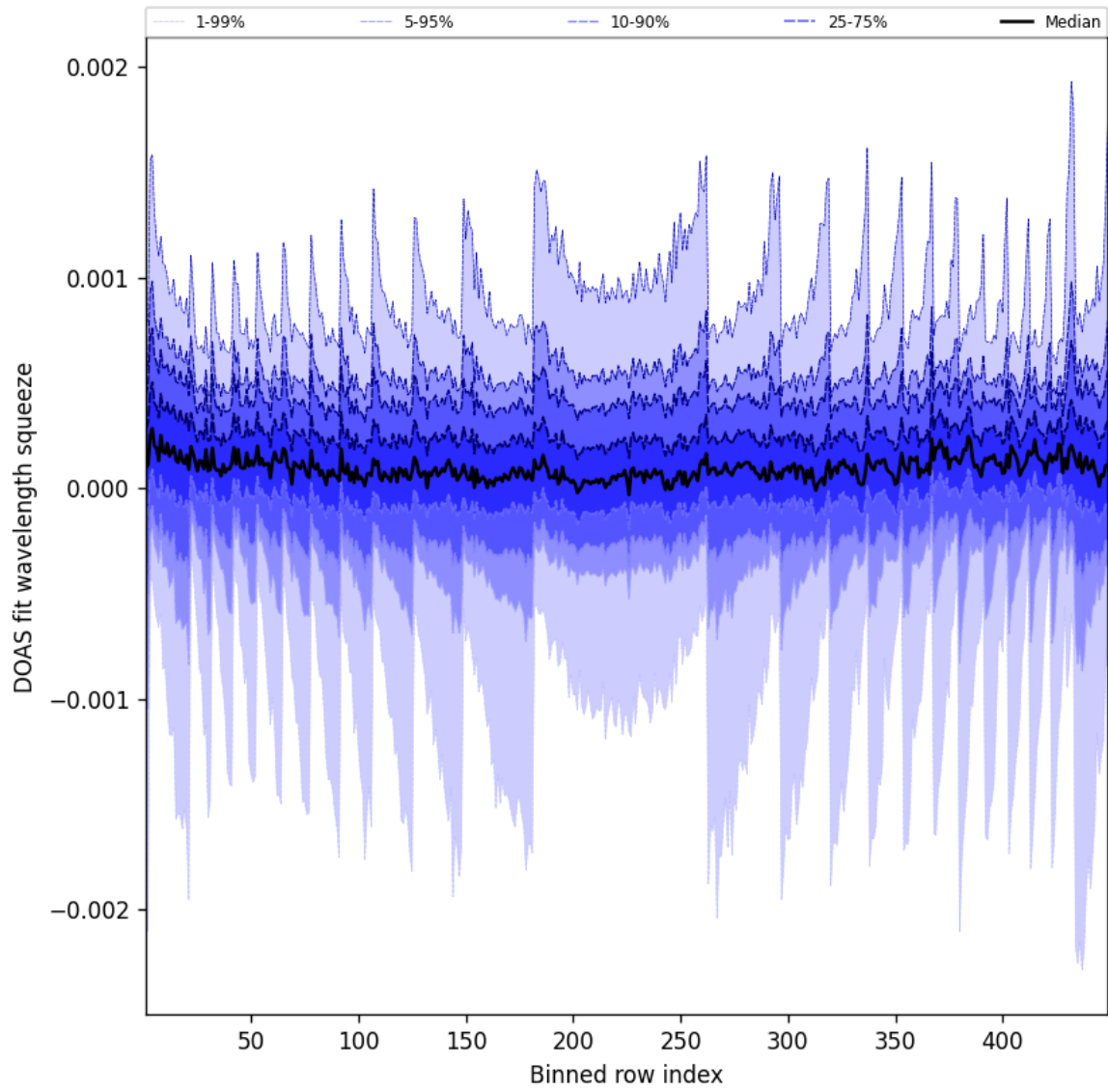
Figure 48: Along track statistics of “DOAS fit wavelength squeeze” for 2025-08-12 to 2025-08-12
