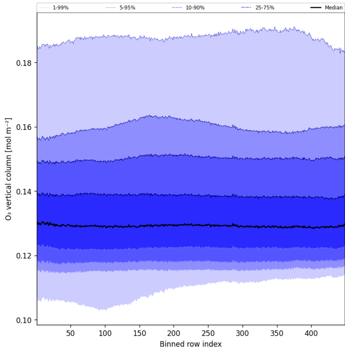
Figure 41: Along track statistics of “O 3 vertical column” for 2025-08-12 to 2025-08-12
