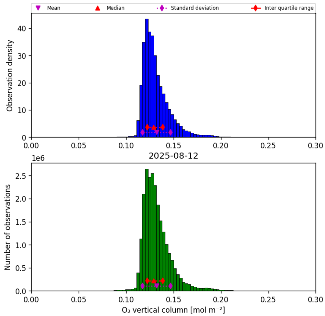
Figure 29: Histogram of “O 3 vertical column” for 2025-08-12 to 2025-08-12
