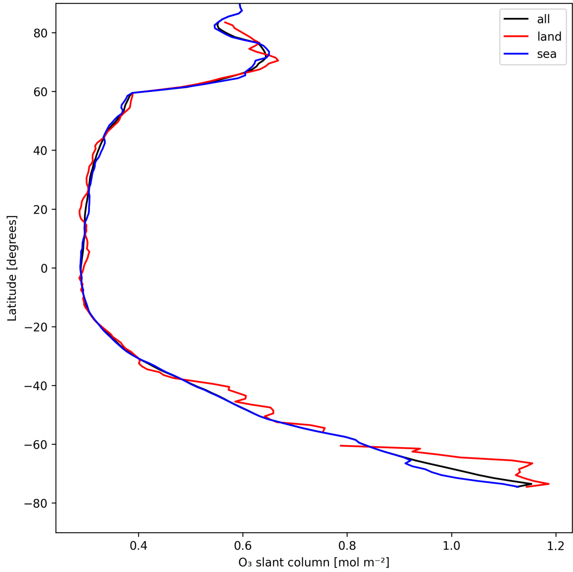
Figure 19: Zonal average of “O 3 slant column” for 2025-08-12 to 2025-08-12.
