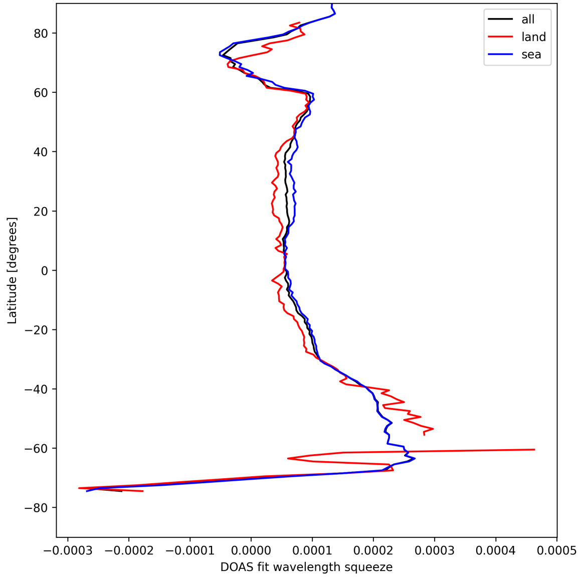
Figure 24: Zonal average of “DOAS fit wavelength squeeze” for 2025-08-12 to 2025-08-12.
