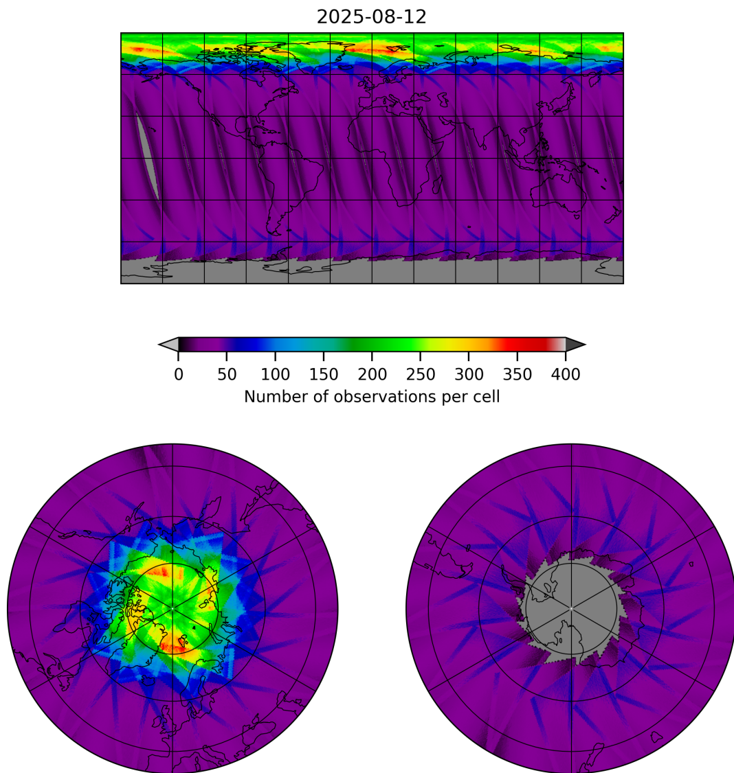
Figure 15: Map of the number of observations for 2025-08-12 to 2025-08-12
