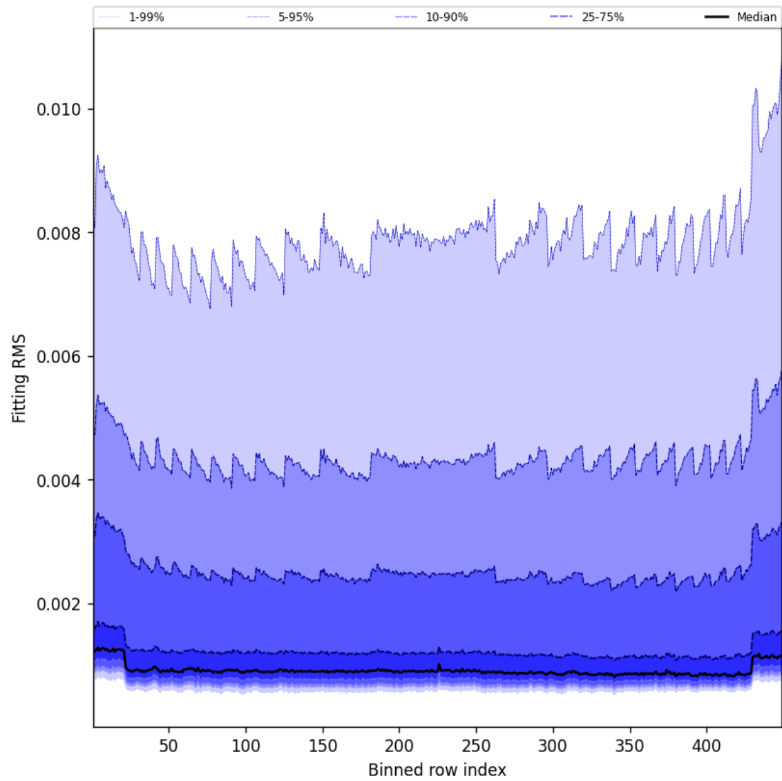
Figure 46: Along track statistics of “Fitting RMS” for 2025-08-12 to 2025-08-12
