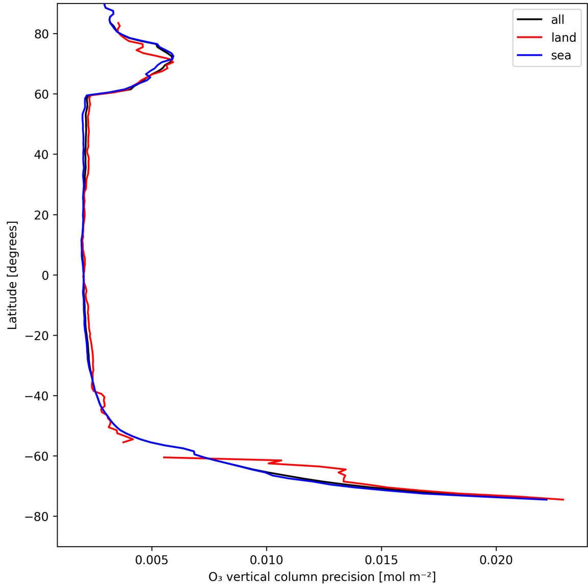
Figure 18: Zonal average of “O 3 vertical column precision” for 2025-08-12 to 2025-08-12.
