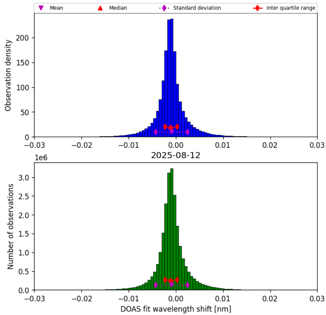
Figure 35: Histogram of “DOAS fit wavelength shift” for 2025-08-12 to 2025-08-12
