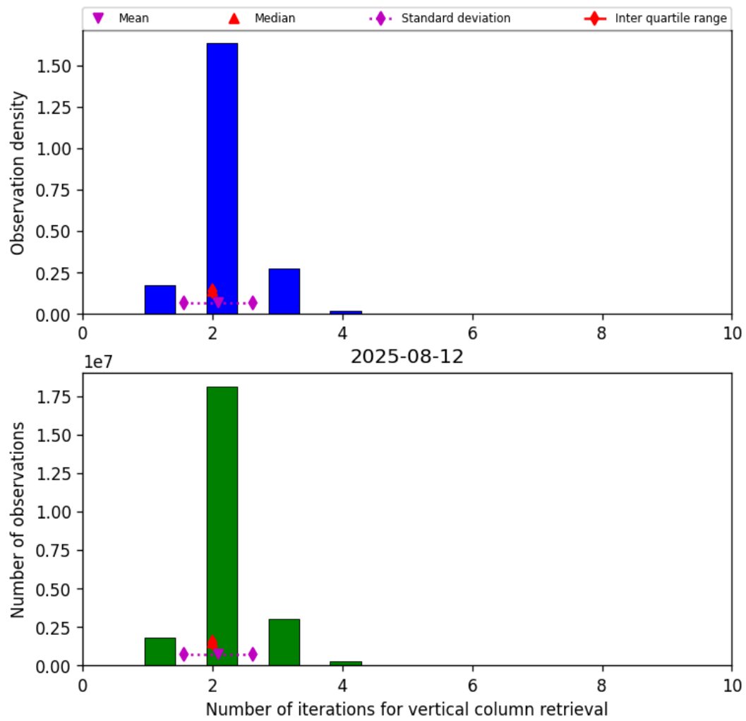
Figure 39: Histogram of “Number of iterations for vertical column retrieval” for 2025-08-12 to 2025-08-12
