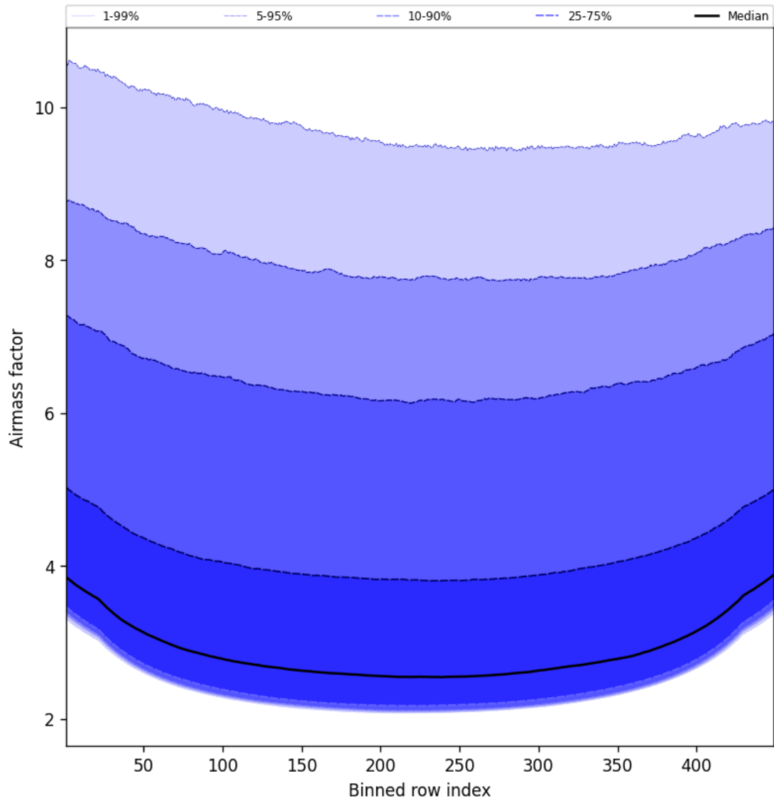
Figure 49: Along track statistics of “Airmass factor” for 2025-08-12 to 2025-08-12
