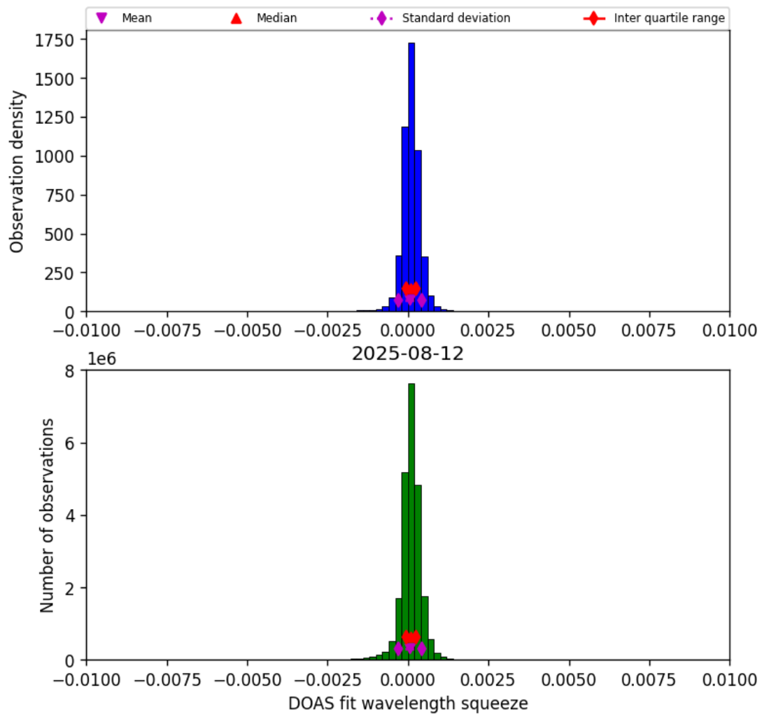
Figure 36: Histogram of “DOAS fit wavelength squeeze” for 2025-08-12 to 2025-08-12
