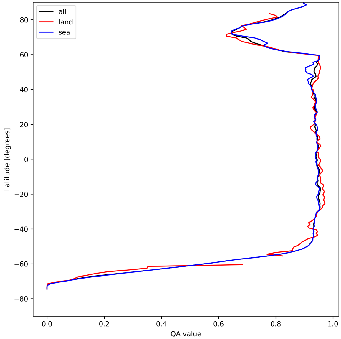
Figure 16: Zonal average of “QA value” for 2025-08-12 to 2025-08-12.
