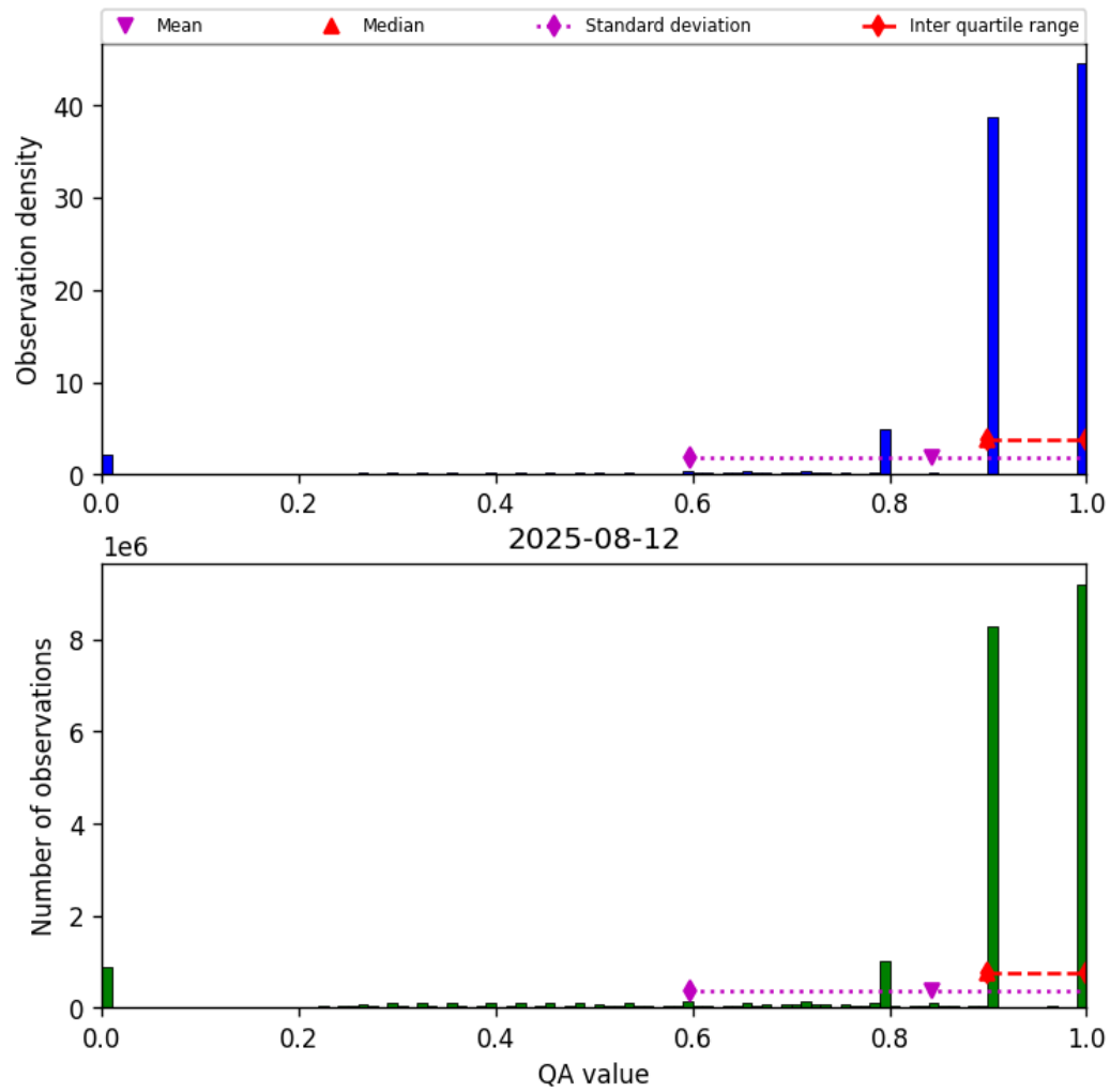
Figure 28: Histogram of “QA value” for 2025-08-12 to 2025-08-12
