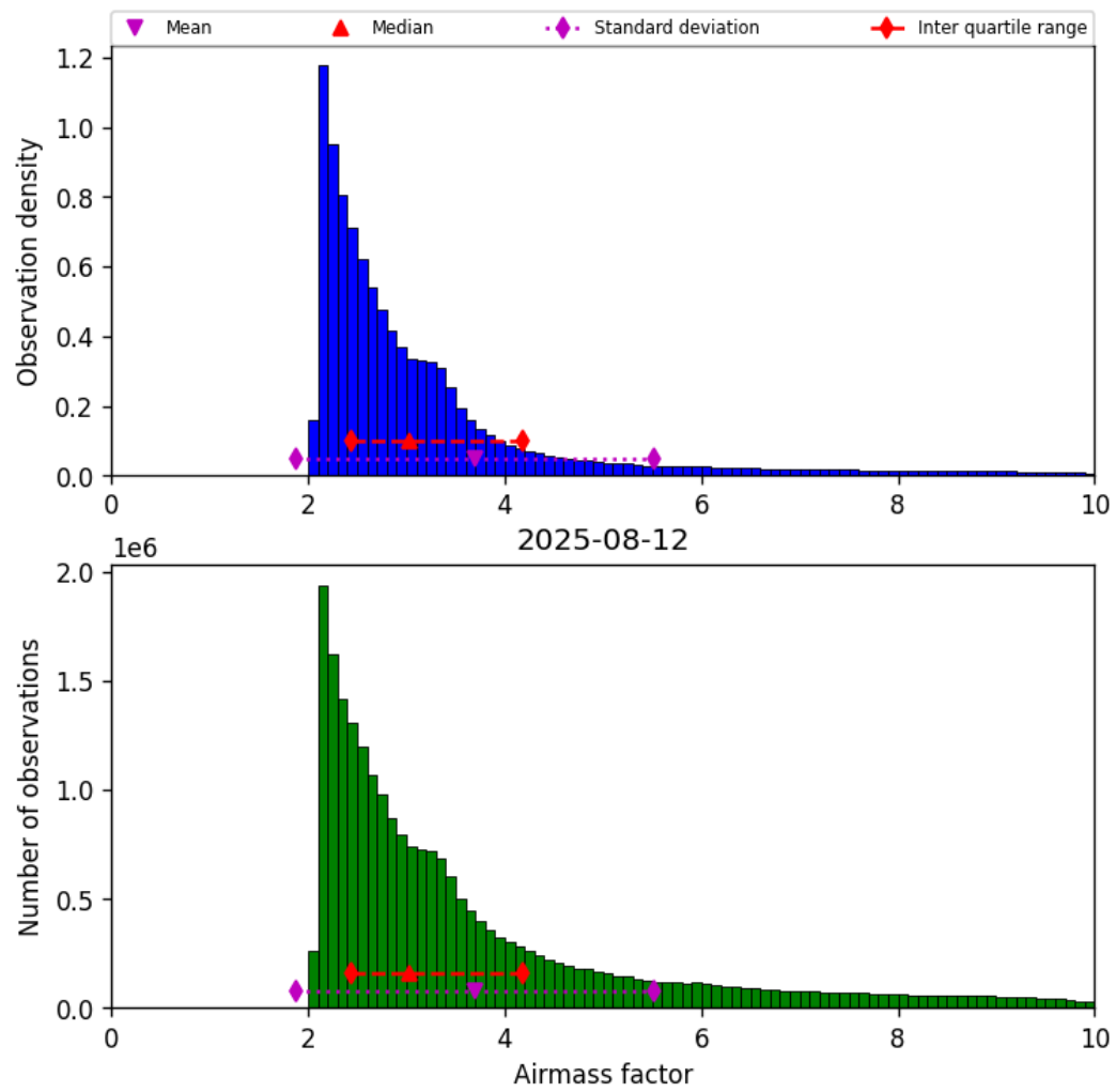
Figure 37: Histogram of “Airmass factor” for 2025-08-12 to 2025-08-12
