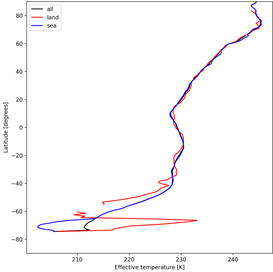
Figure 26: Zonal average of “Effective temperature” for 2025-08-12 to 2025-08-12.
