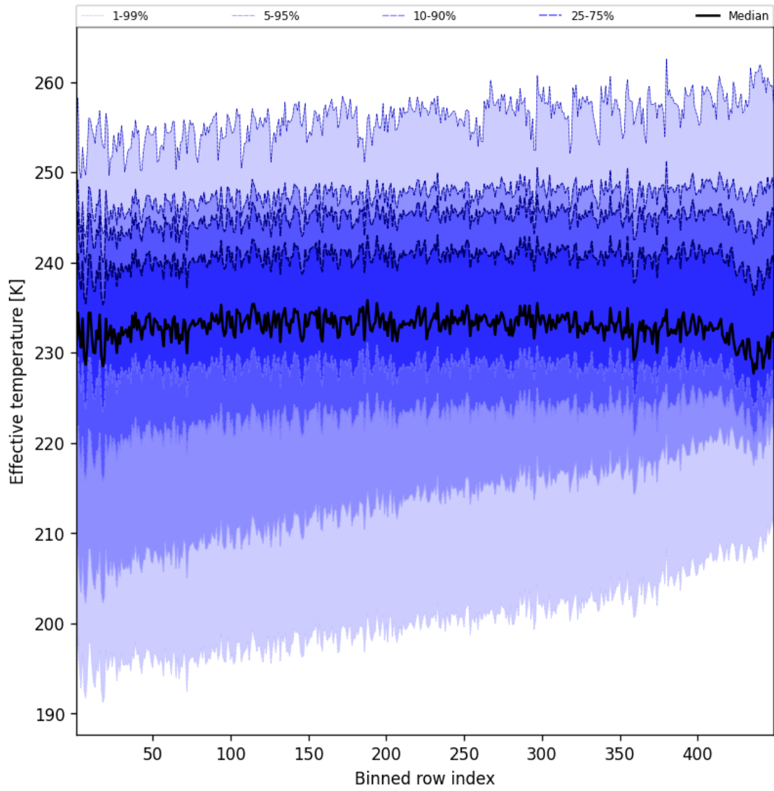
Figure 50: Along track statistics of “Effective temperature” for 2025-08-12 to 2025-08-12
