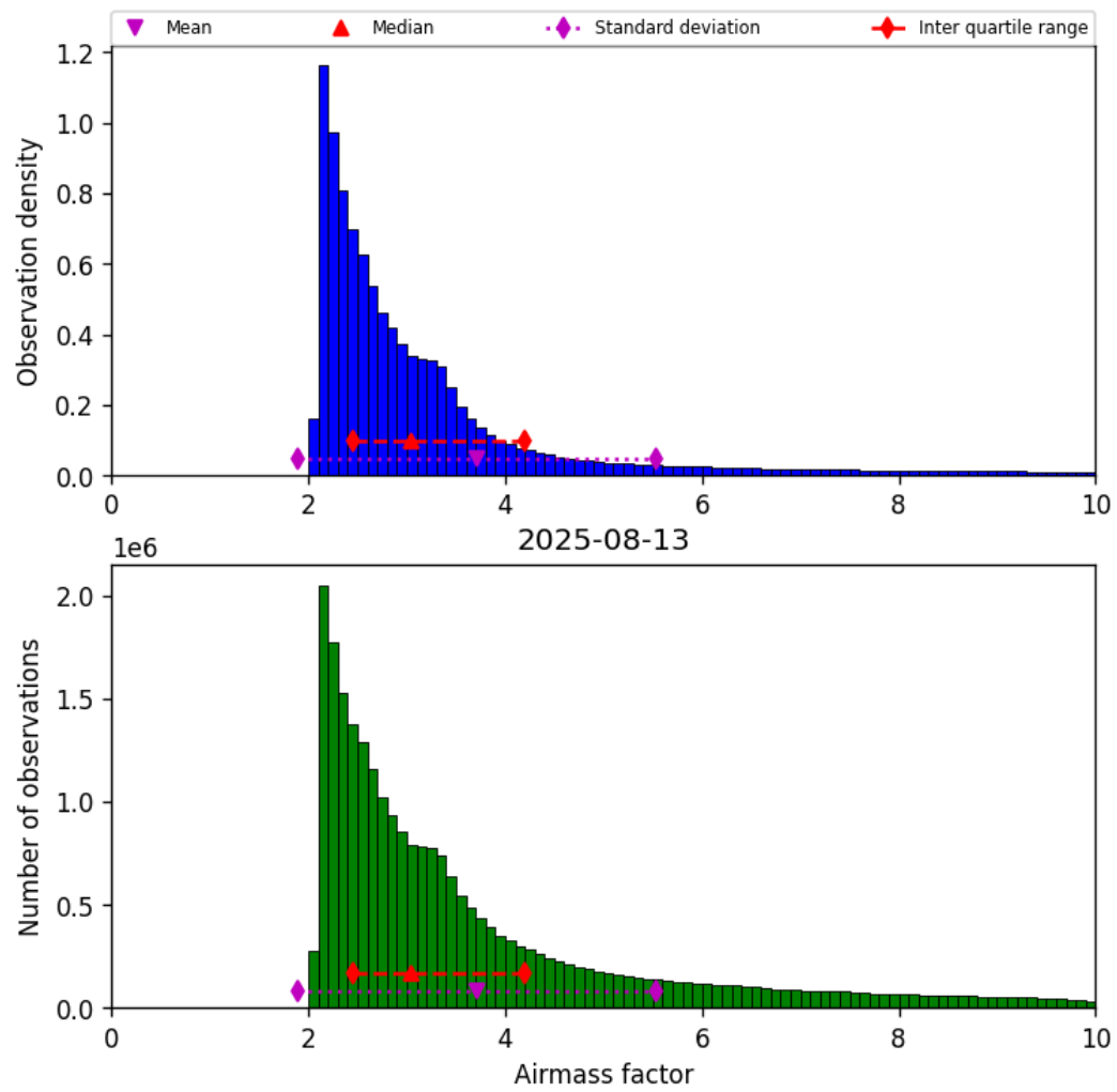
Figure 37: Histogram of “Airmass factor” for 2025-08-13 to 2025-08-14
