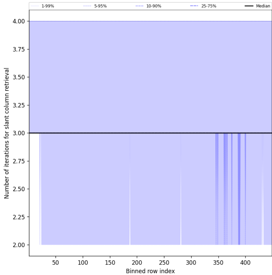
Figure 45: Along track statistics of “Number of iterations for slant column retrieval” for 2025-08-13 to 2025-08-14
