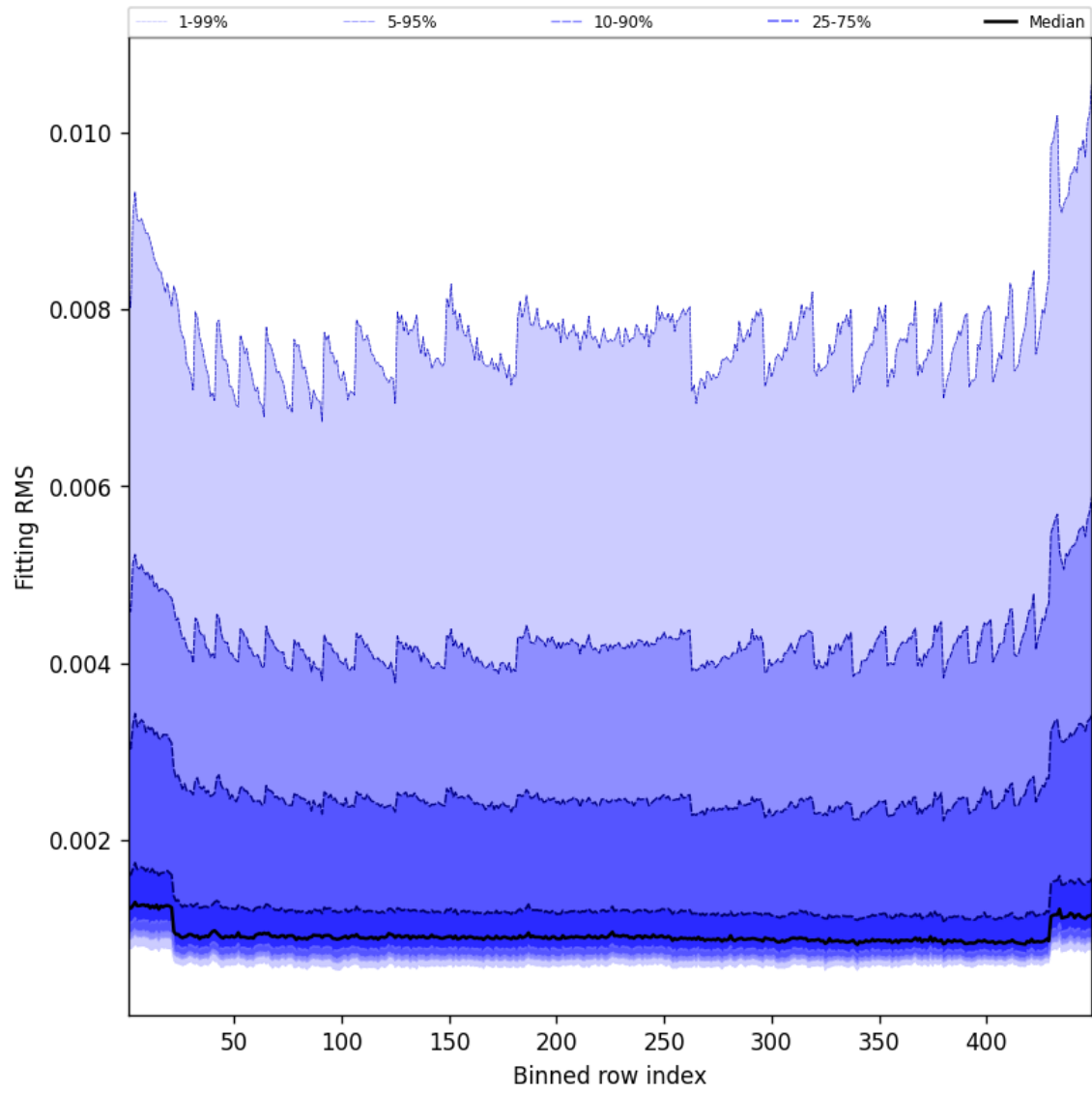
Figure 46: Along track statistics of “Fitting RMS” for 2025-08-13 to 2025-08-14
