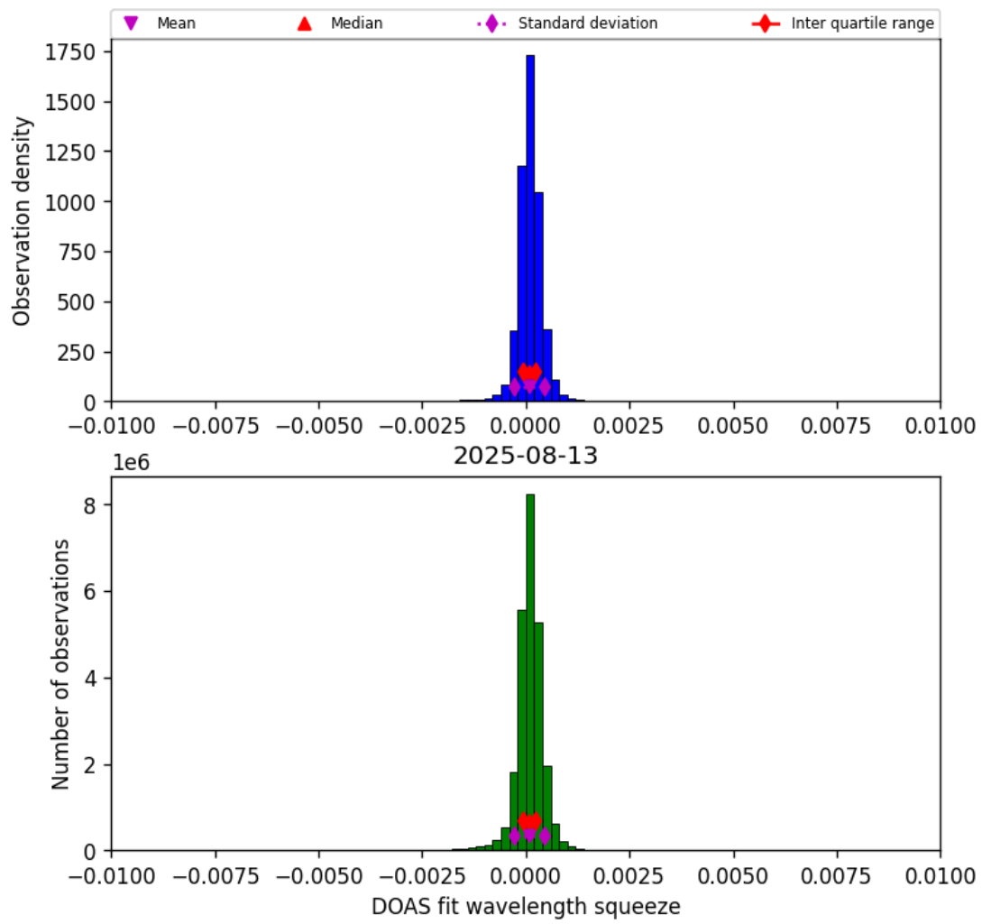
Figure 36: Histogram of “DOAS fit wavelength squeeze” for 2025-08-13 to 2025-08-14
