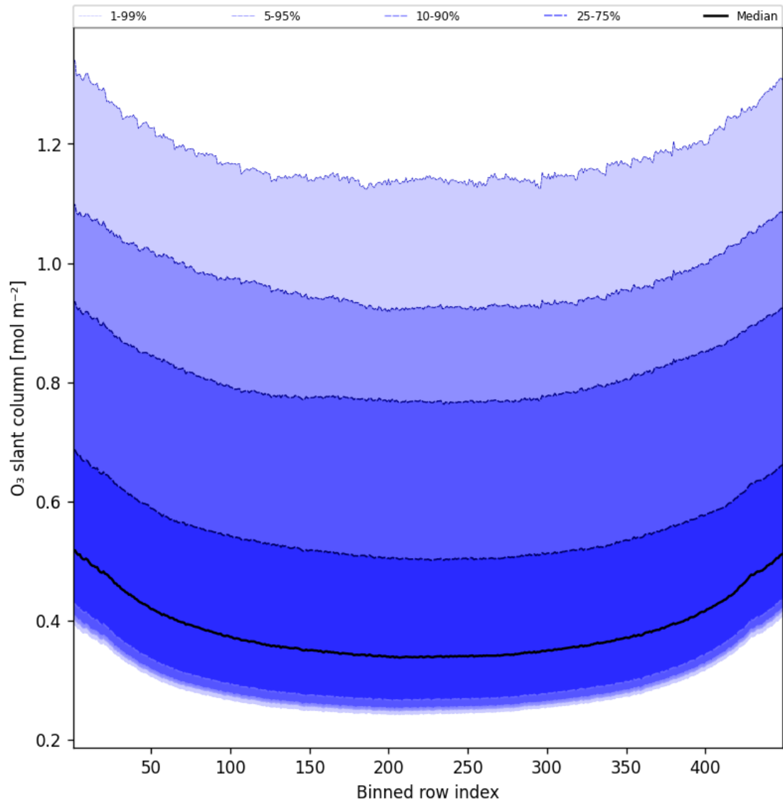
Figure 43: Along track statistics of “ O_3 slant column” for 2025-08-13 to 2025-08-14
