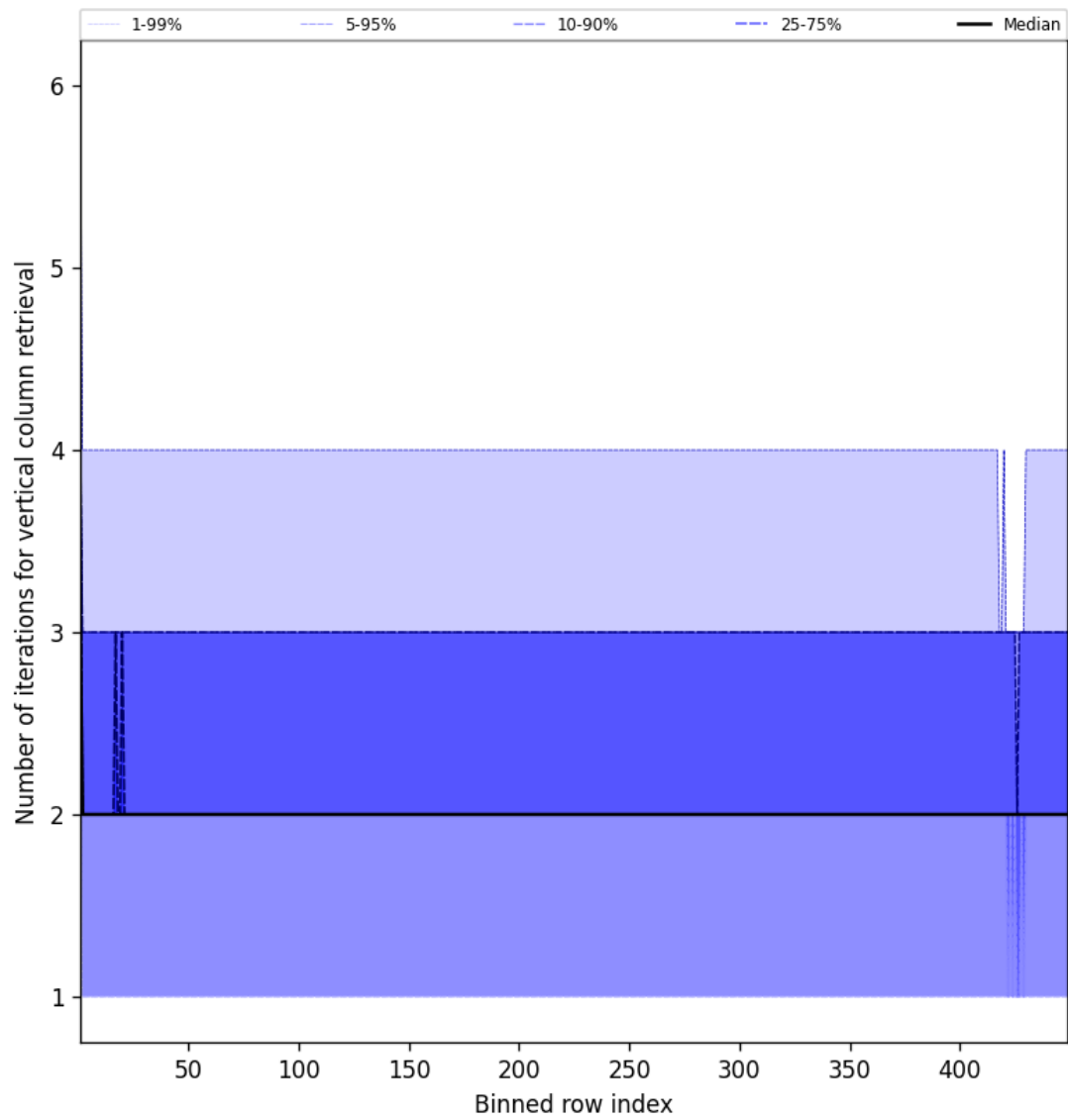
Figure 51: Along track statistics of “Number of iterations for vertical column retrieval” for 2025-08-13 to 2025-08-14
