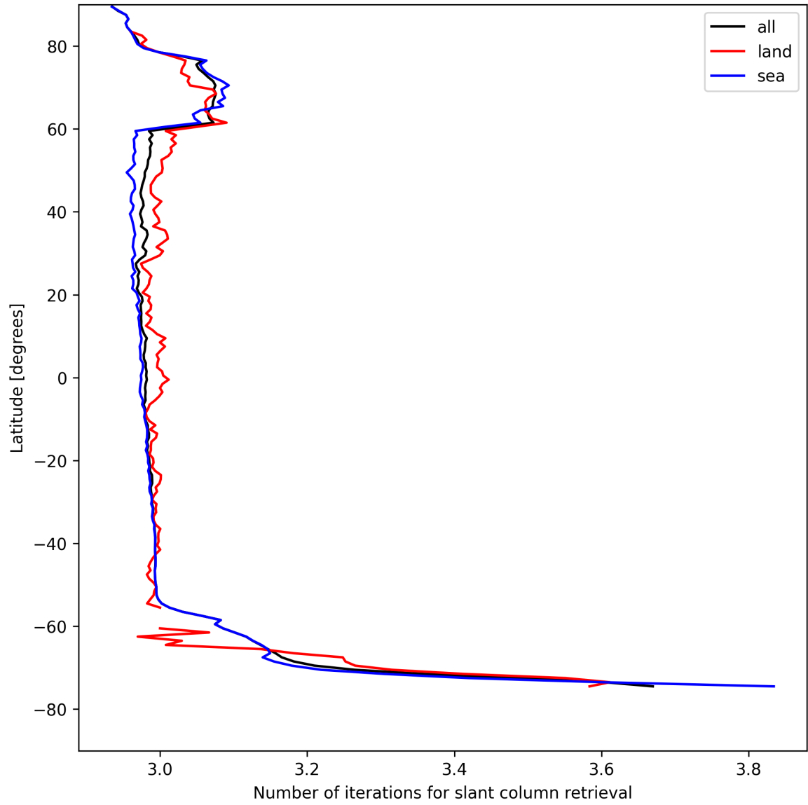
Figure 21: Zonal average of “Number of iterations for slant column retrieval” for 2025-08-13 to 2025-08-14.
