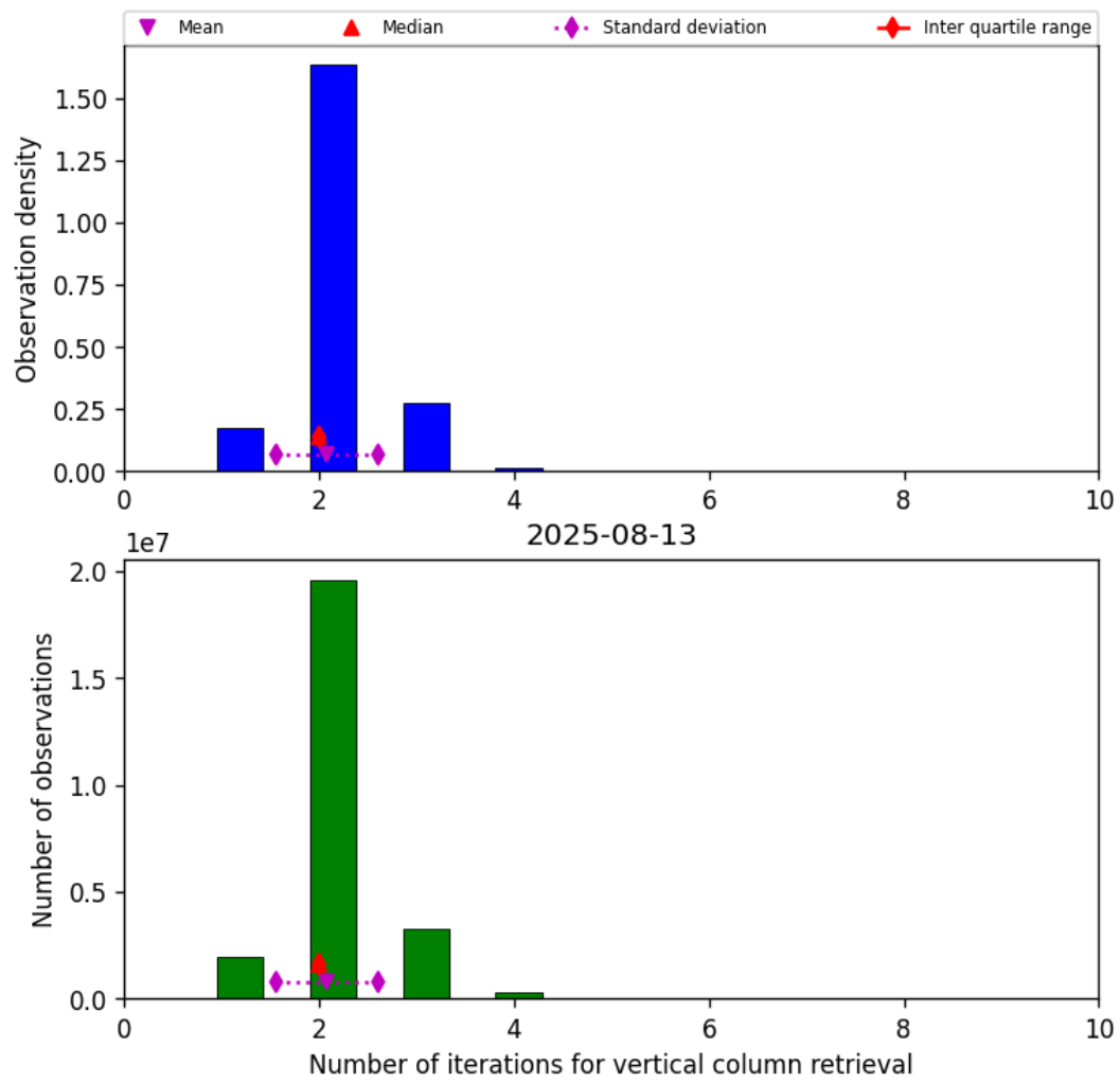
Figure 39: Histogram of “Number of iterations for vertical column retrieval” for 2025-08-13 to 2025-08-14
