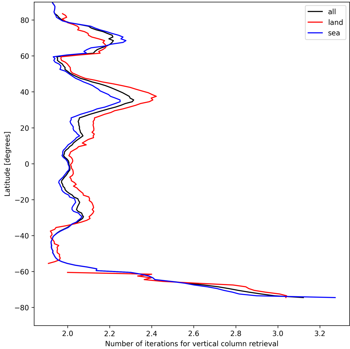
Figure 27: Zonal average of “Number of iterations for vertical column retrieval” for 2025-08-13 to 2025-08-14.
