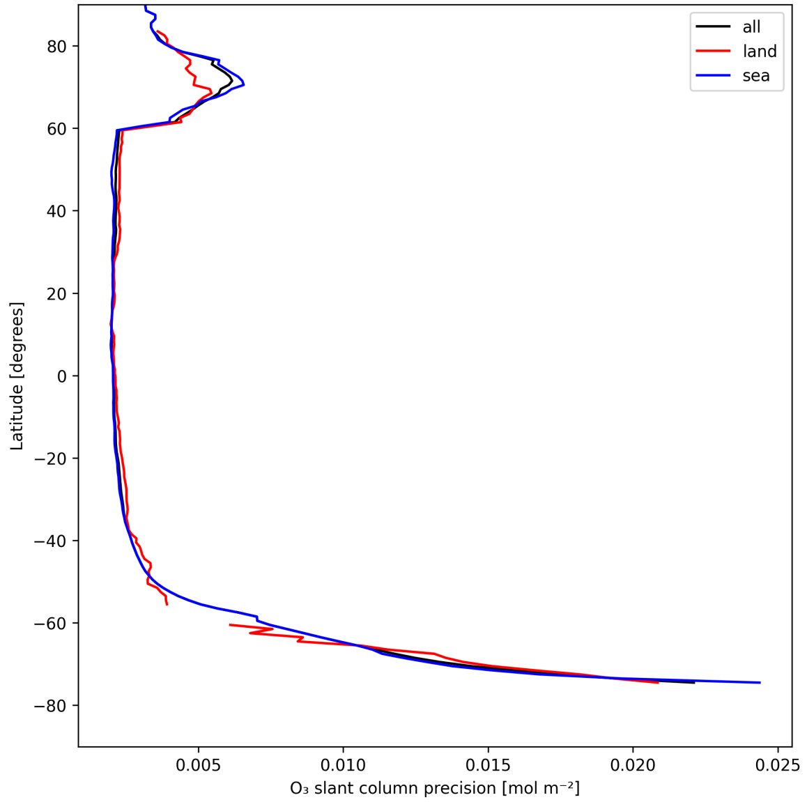
Figure 20: Zonal average of "O 3 slant column precision" for 2025-08-13 to 2025-08-14.
