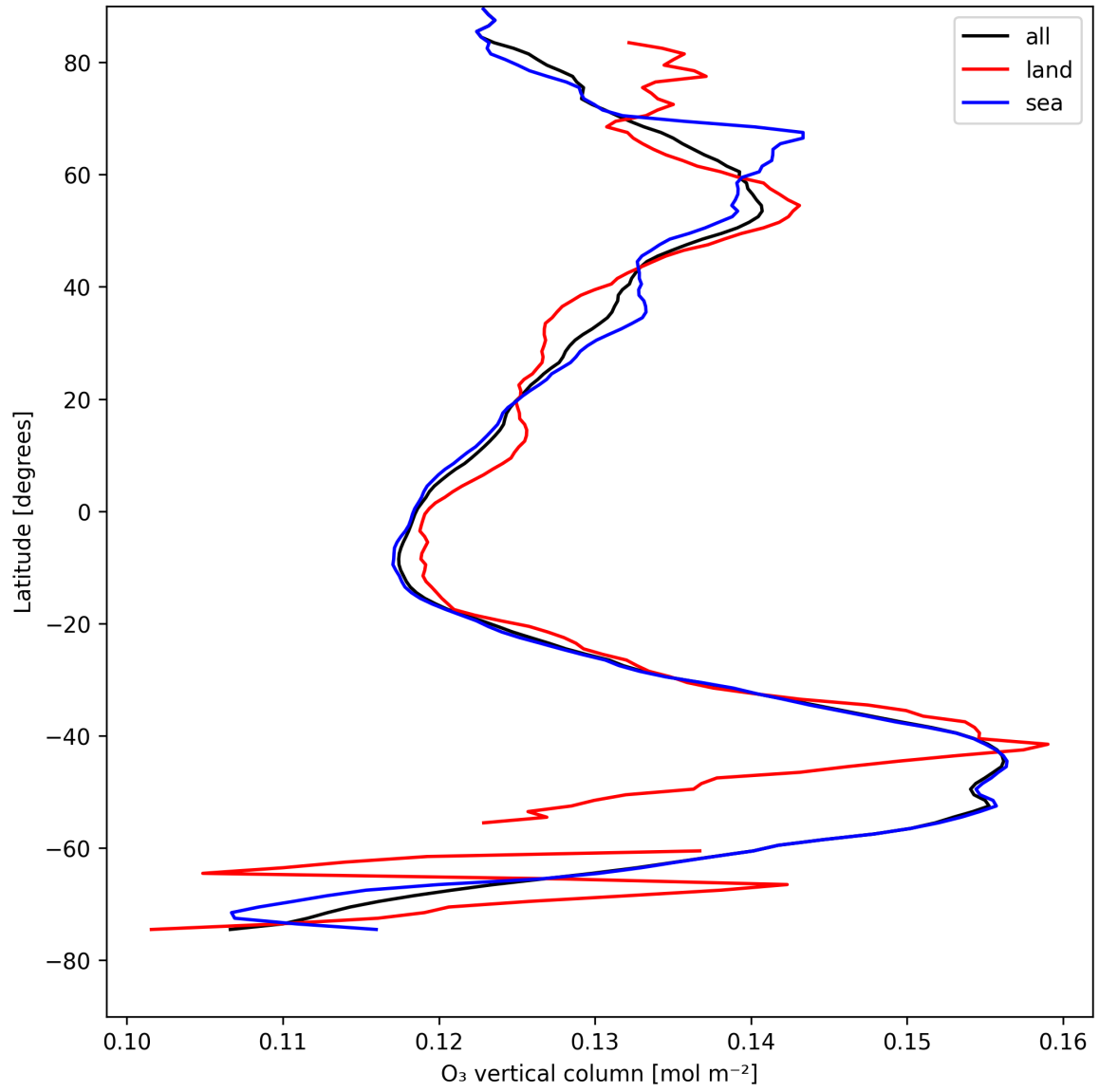
Figure 17: Zonal average of “O 3 vertical column” for 2025-08-13 to 2025-08-14.
