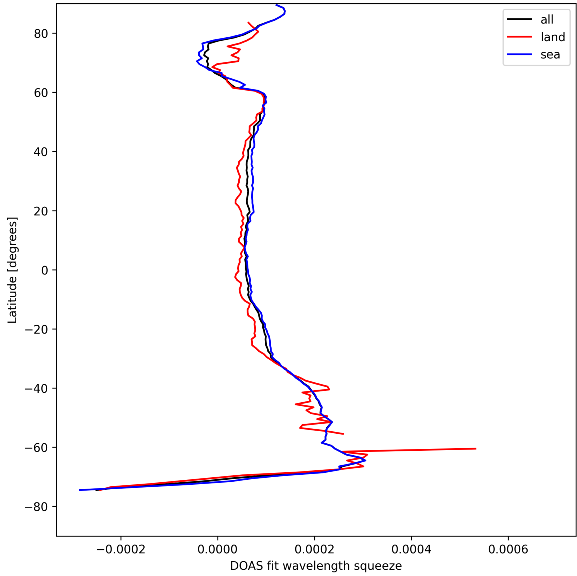
Figure 24: Zonal average of “DOAS fit wavelength squeeze” for 2025-08-13 to 2025-08-14.
