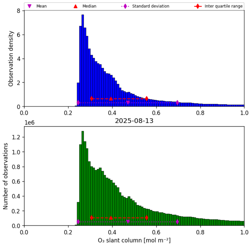
Figure 31: Histogram of “O 3 slant column” for 2025-08-13 to 2025-08-14
