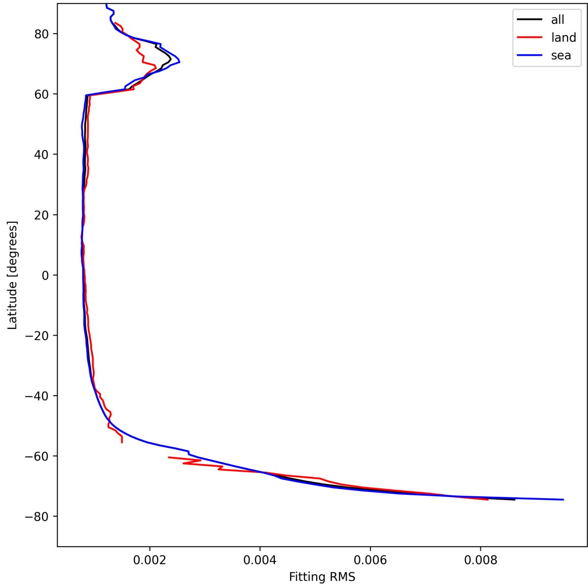
Figure 22: Zonal average of “Fitting RMS” for 2025-08-13 to 2025-08-14.
