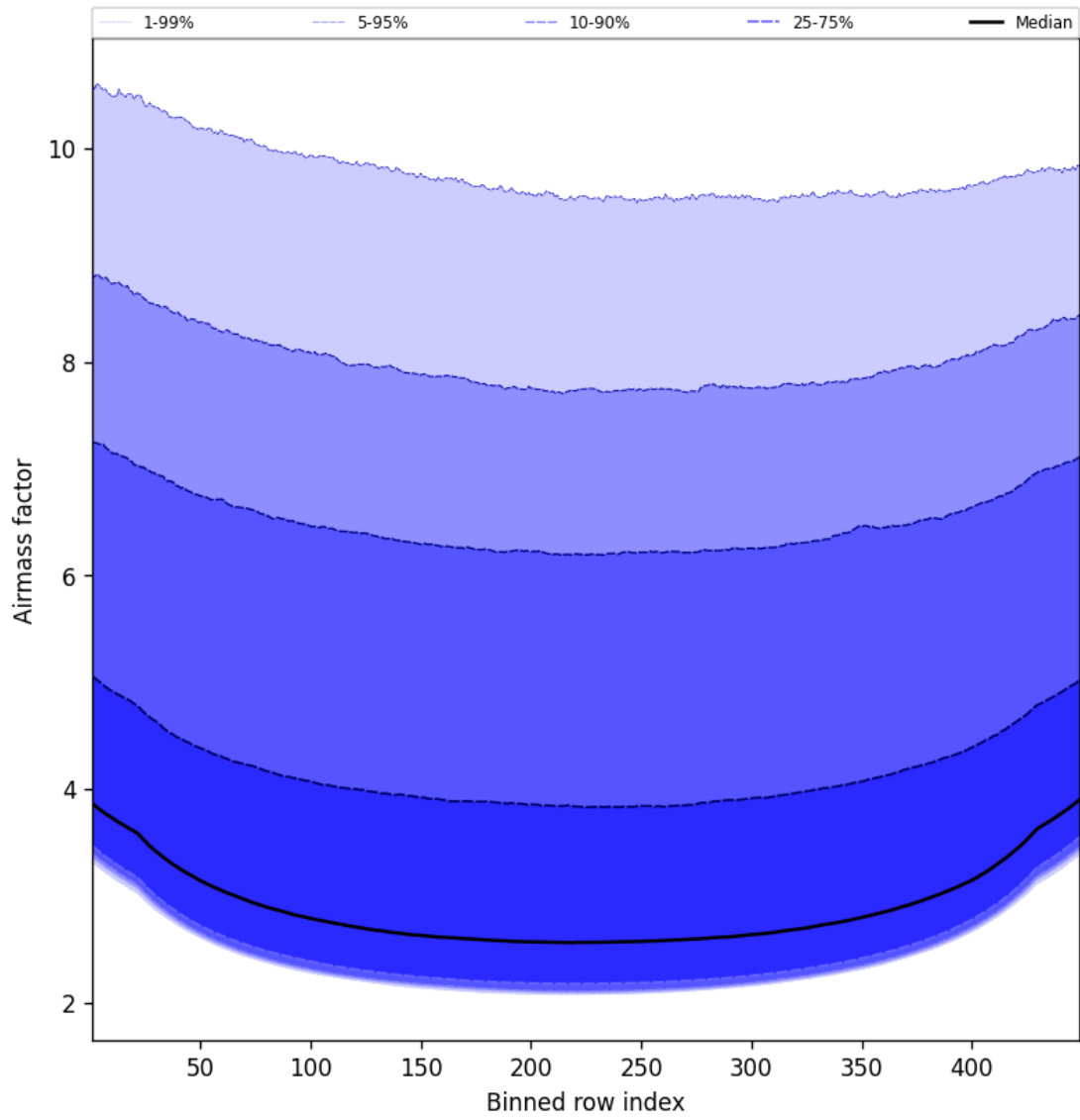
Figure 49: Along track statistics of “Airmass factor” for 2025-08-13 to 2025-08-14
