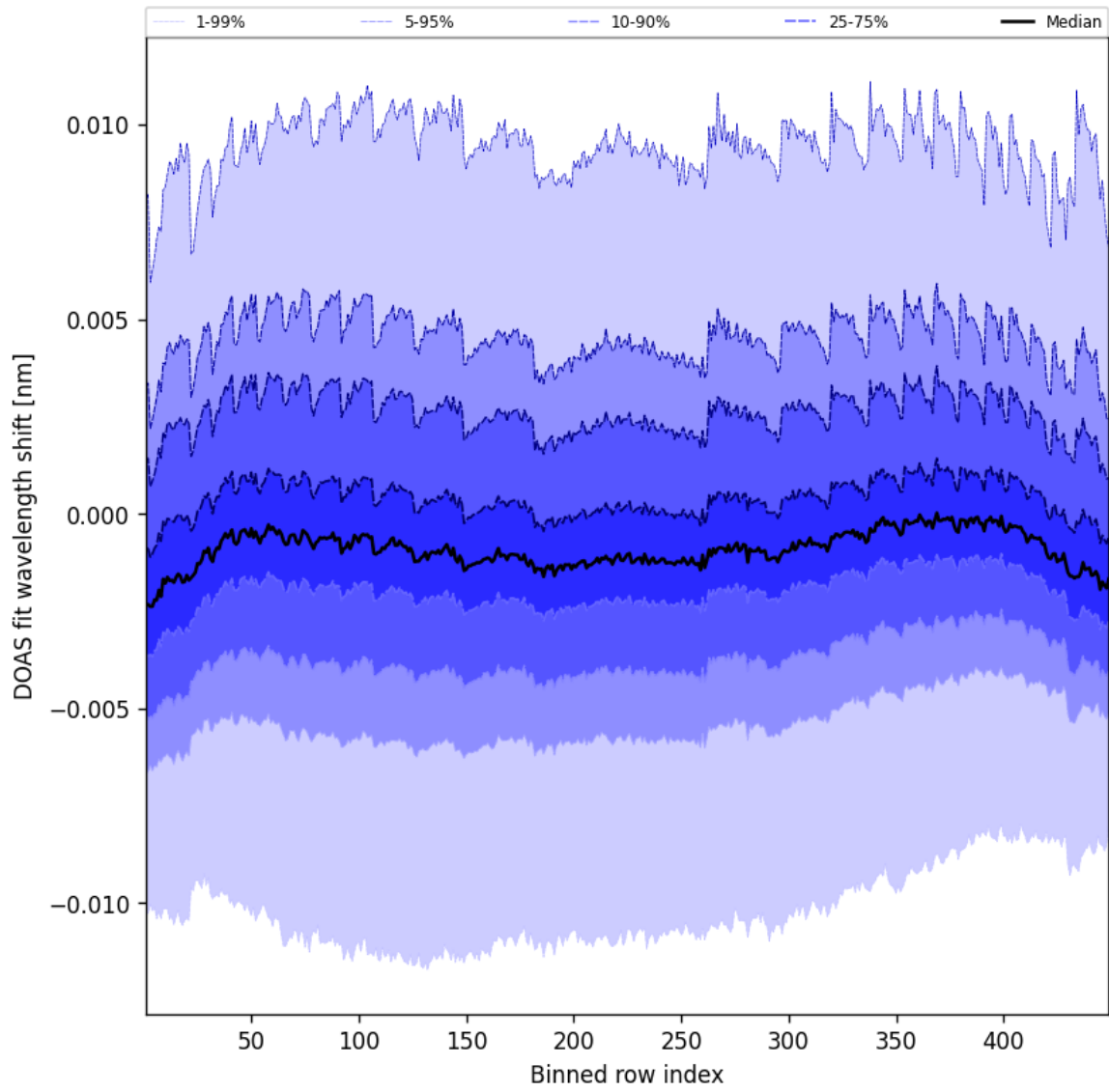
Figure 47: Along track statistics of “DOAS fit wavelength shift” for 2025-08-13 to 2025-08-14
