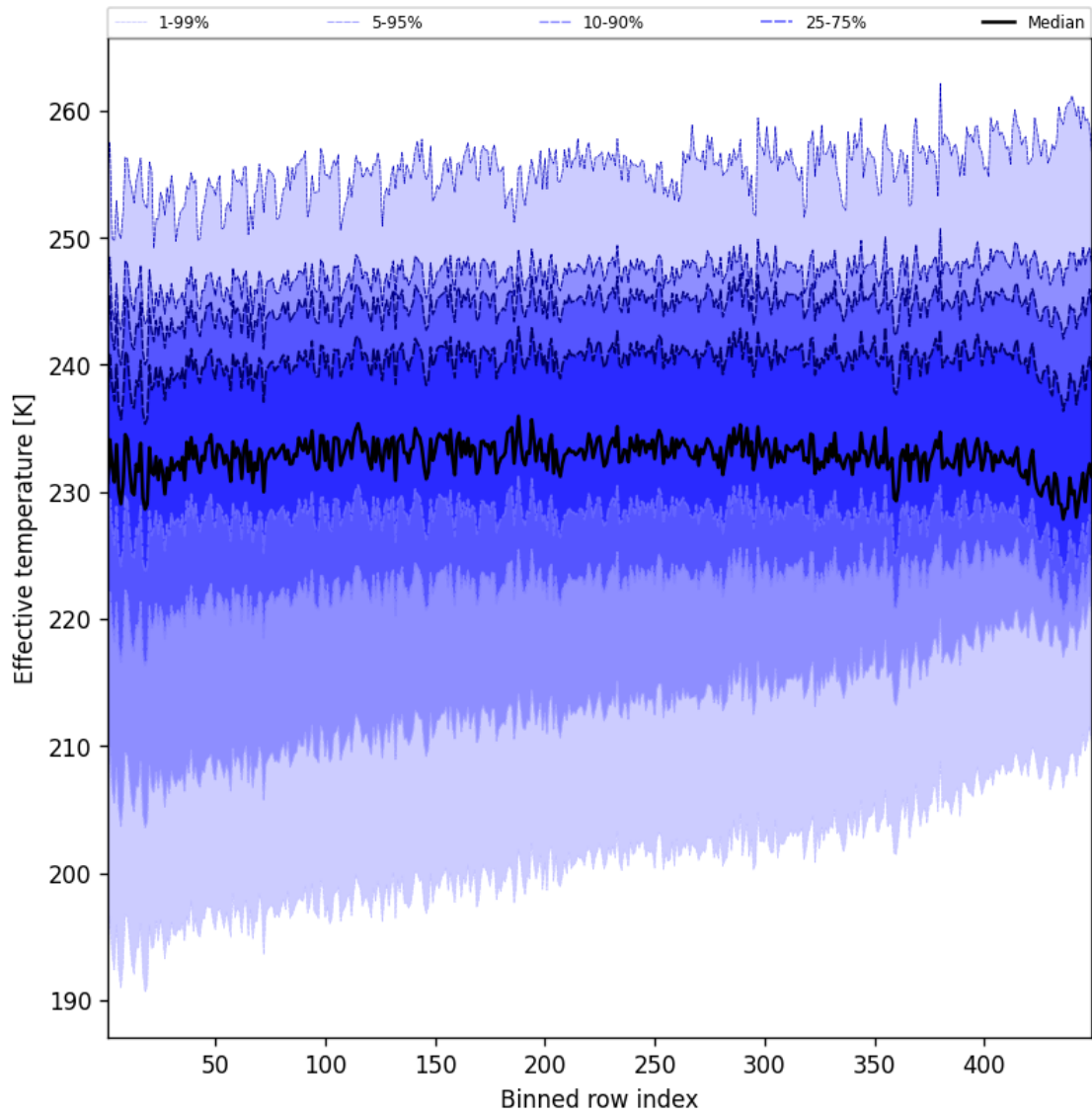
Figure 50: Along track statistics of “Effective temperature” for 2025-08-13 to 2025-08-14
