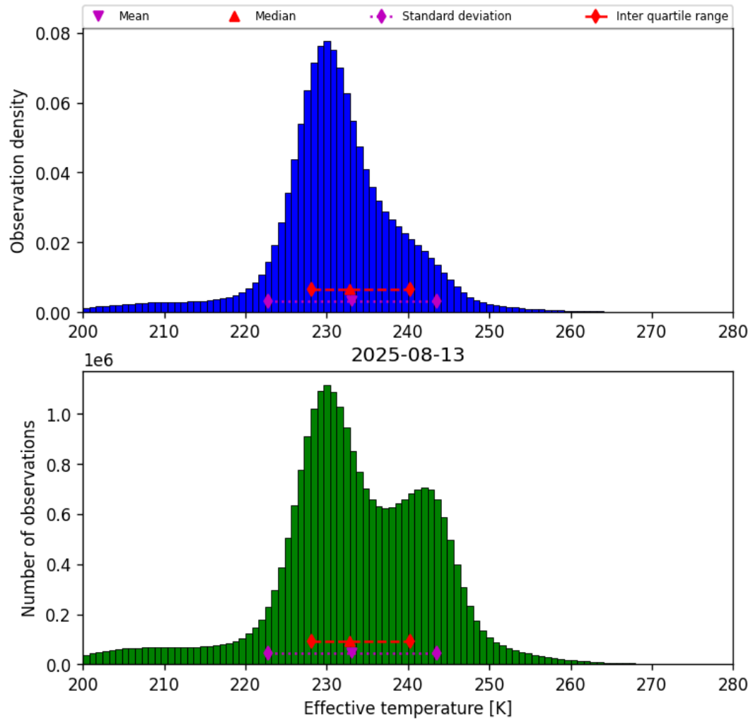
Figure 38: Histogram of “Effective temperature” for 2025-08-13 to 2025-08-14
