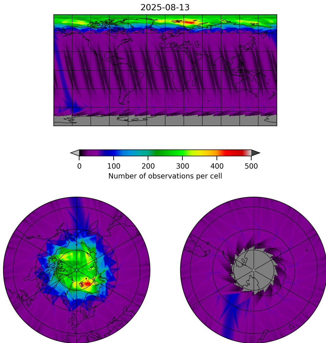
Figure 15: Map of the number of observations for 2025-08-13 to 2025-08-14
