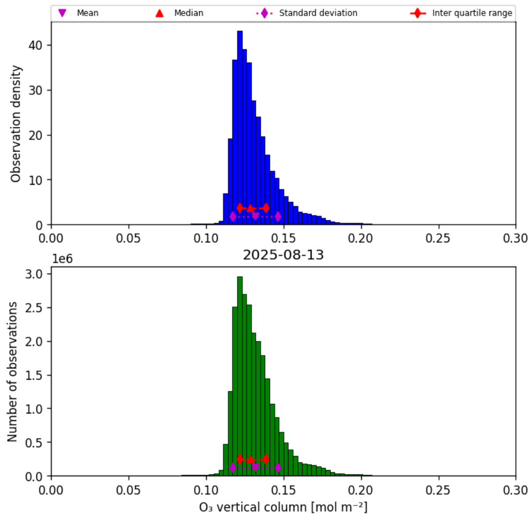
Figure 29: Histogram of “O 3 vertical column” for 2025-08-13 to 2025-08-14
