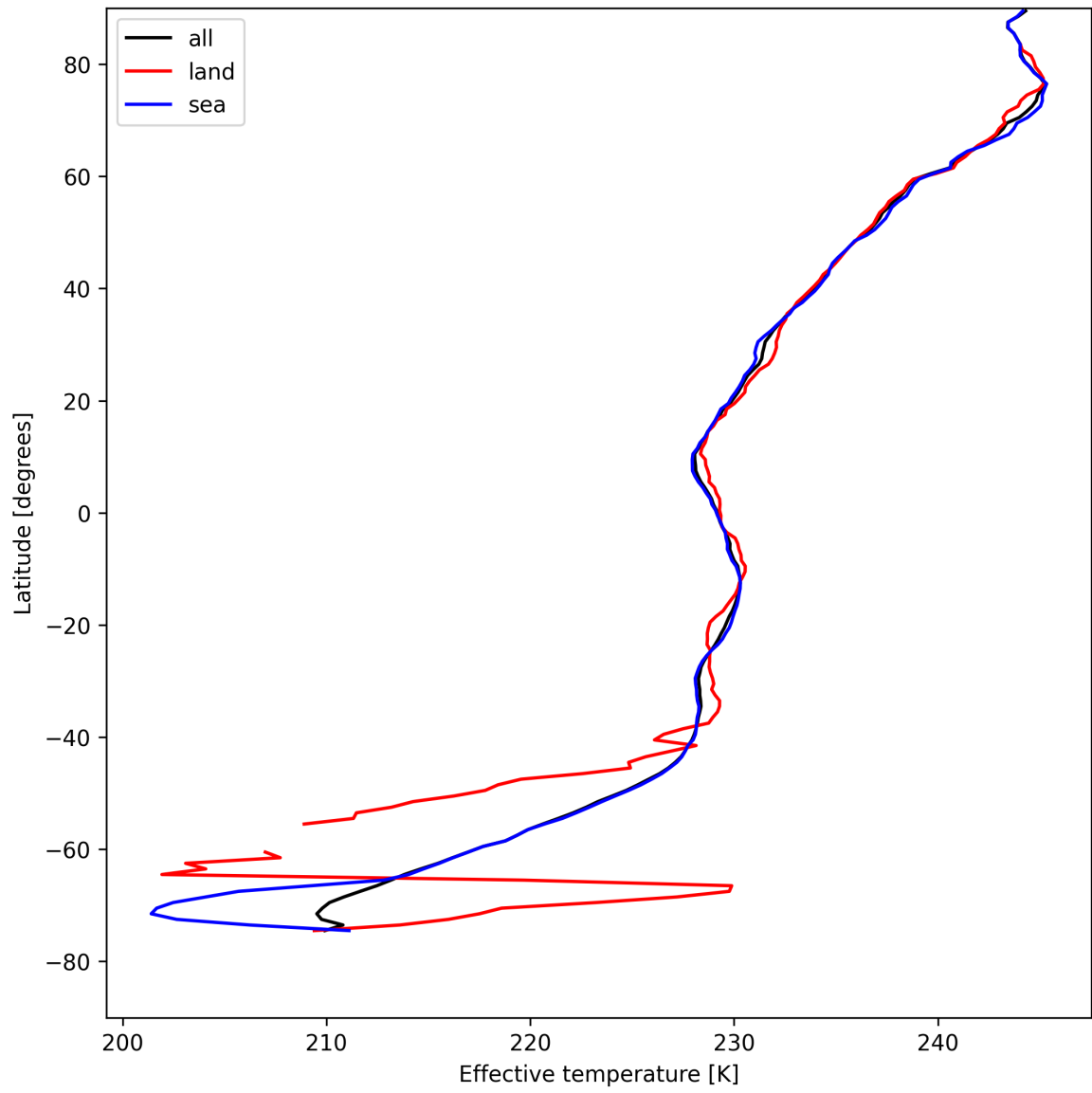
Figure 26: Zonal average of “Effective temperature” for 2025-08-13 to 2025-08-14.
