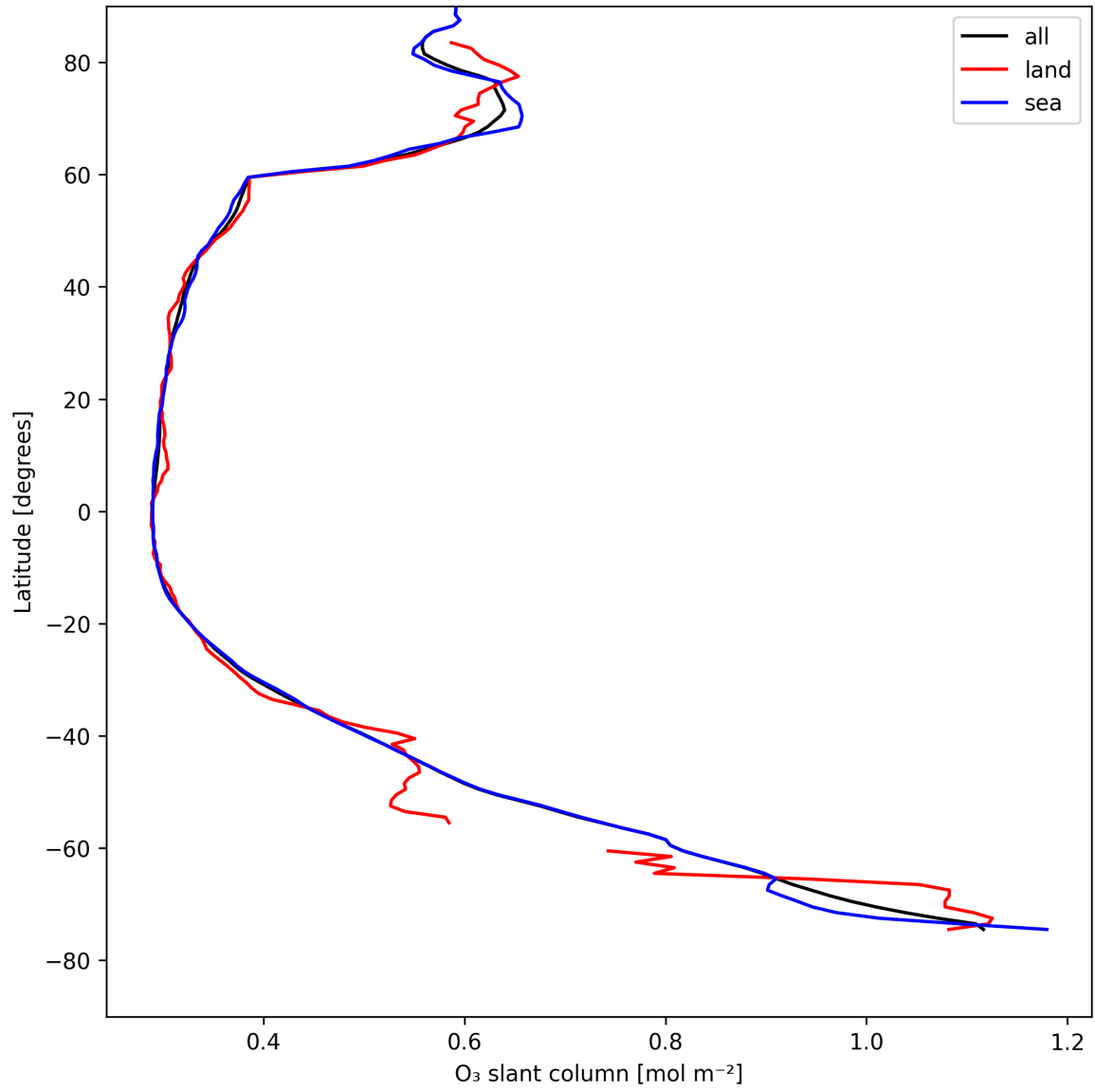
Figure 19: Zonal average of “O 3 slant column” for 2025-08-13 to 2025-08-14.
