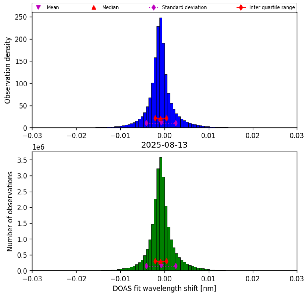
Figure 35: Histogram of “DOAS fit wavelength shift” for 2025-08-13 to 2025-08-14
