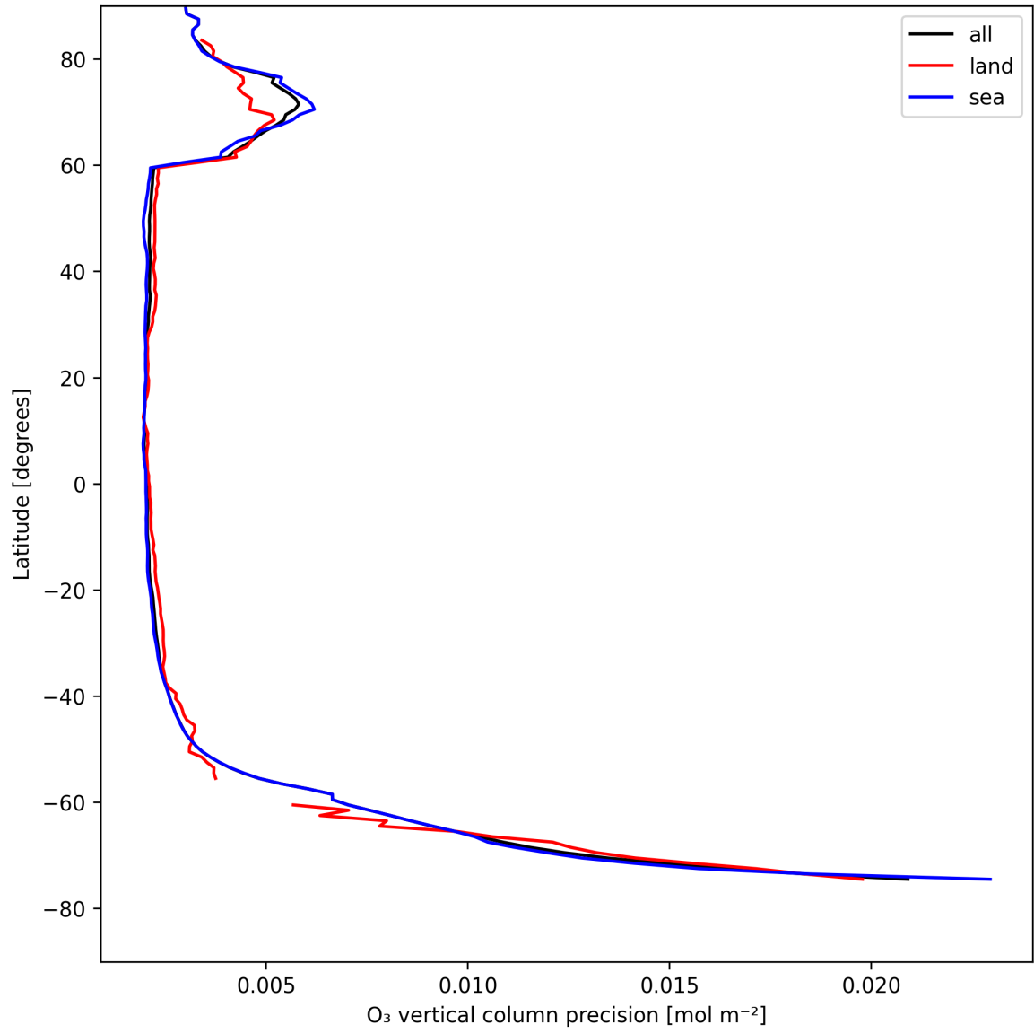
Figure 18: Zonal average of “O 3 vertical column precision” for 2025-08-13 to 2025-08-14.
