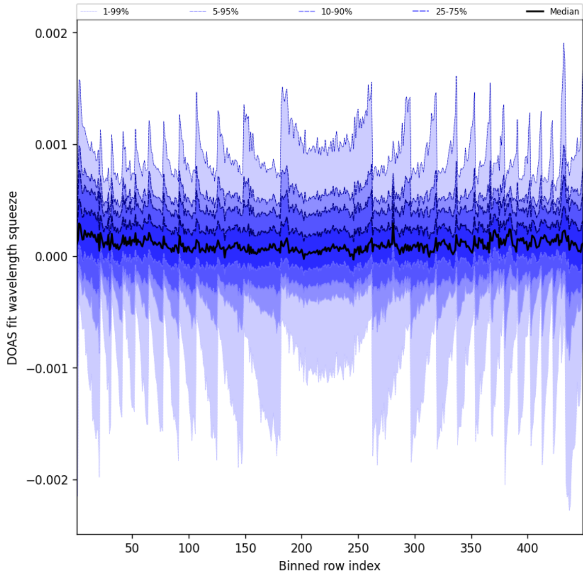
Figure 48: Along track statistics of “DOAS fit wavelength squeeze” for 2025-08-13 to 2025-08-14
