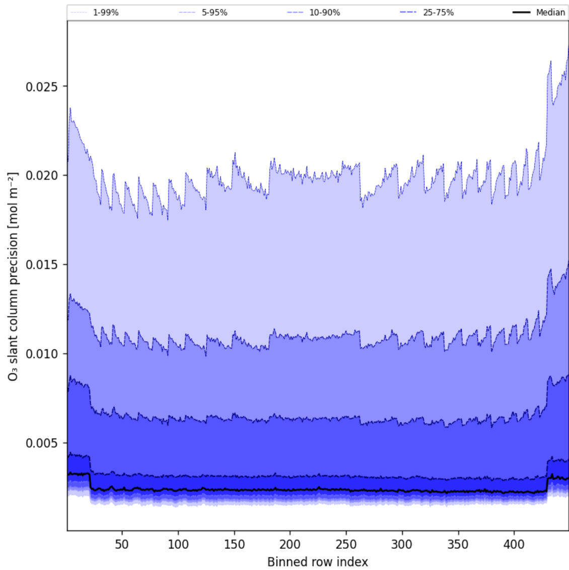
Figure 44: Along track statistics of “O 3 slant column precision” for 2025-08-13 to 2025-08-14
