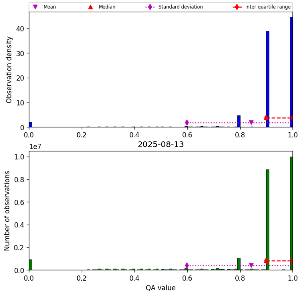
Figure 28: Histogram of “QA value” for 2025-08-13 to 2025-08-14
