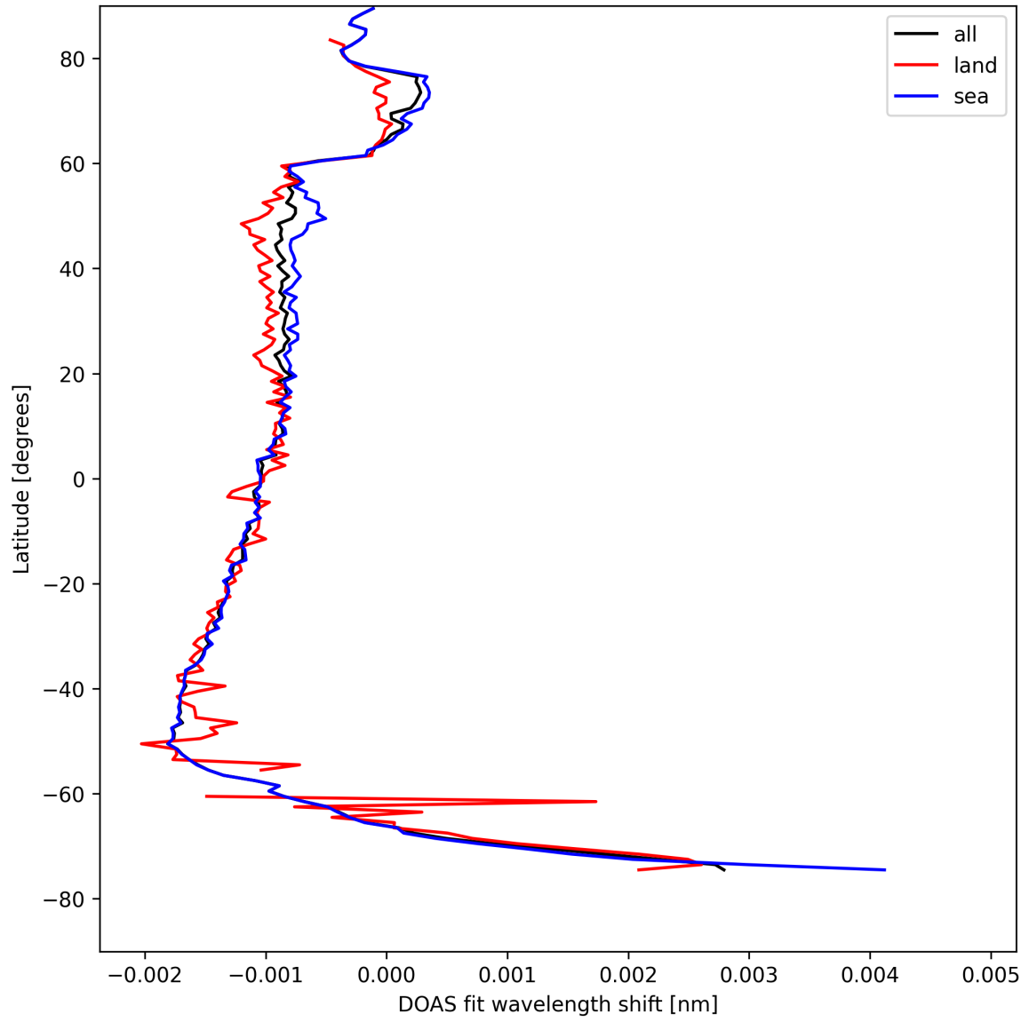
Figure 23: Zonal average of “DOAS fit wavelength shift” for 2025-08-13 to 2025-08-14.
