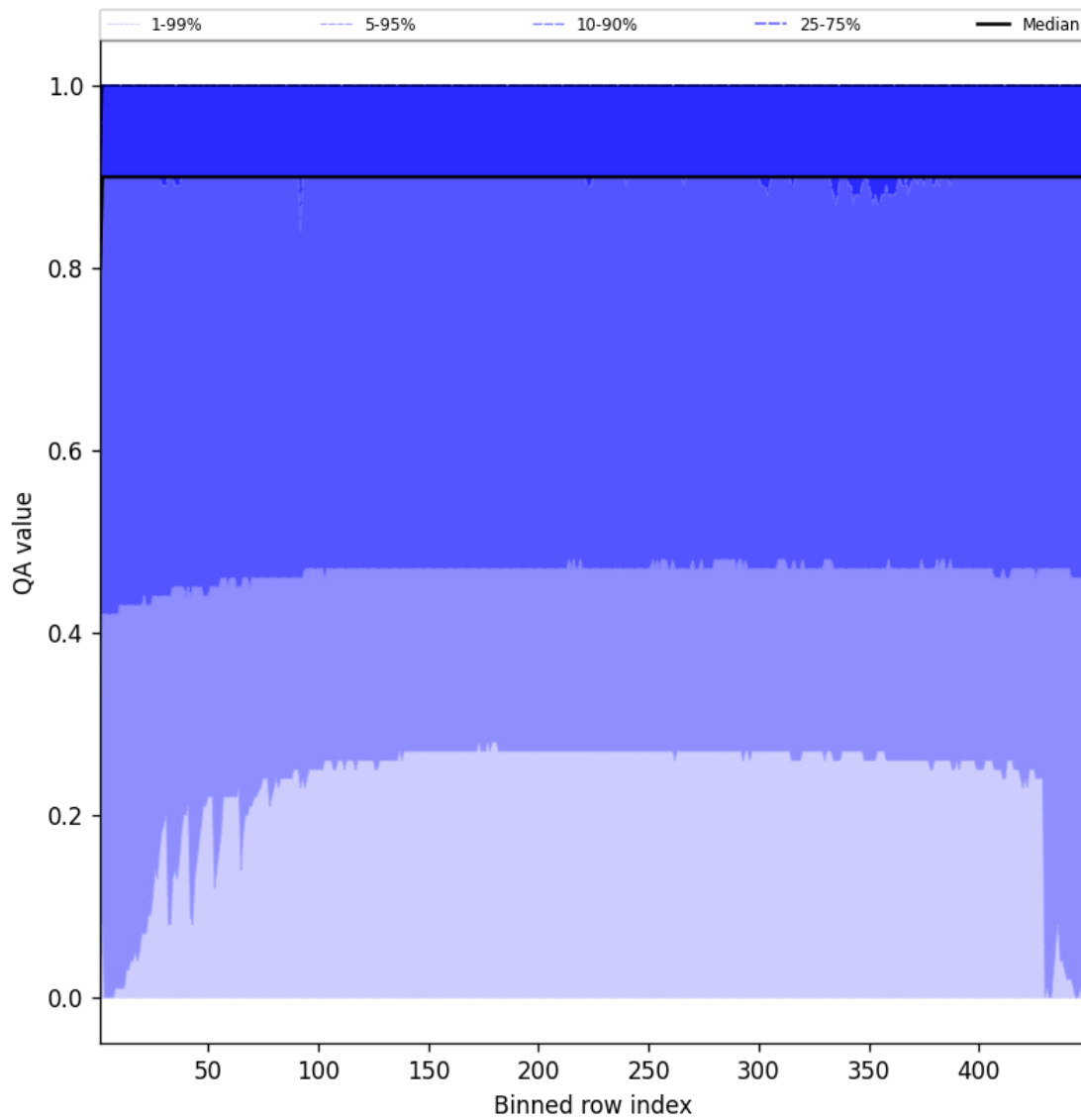
Figure 40: Along track statistics of “QA value” for 2025-08-13 to 2025-08-14
