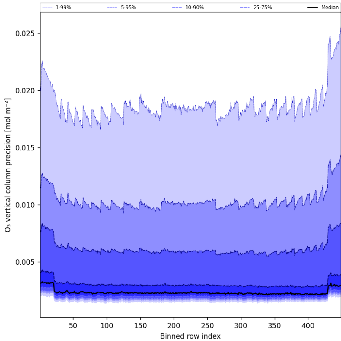
Figure 42: Along track statistics of “O 3 vertical column precision” for 2025-08-13 to 2025-08-14
