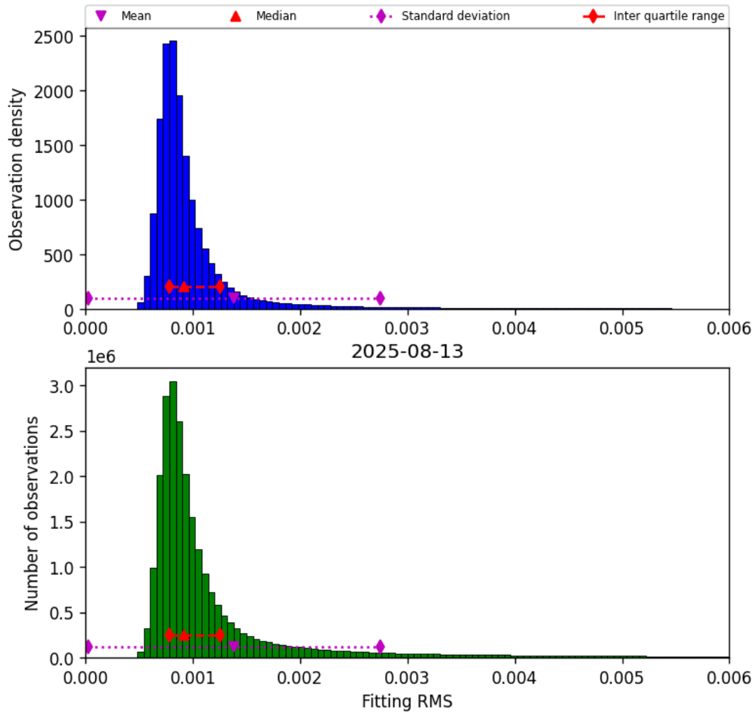
Figure 34: Histogram of “Fitting RMS” for 2025-08-13 to 2025-08-14
