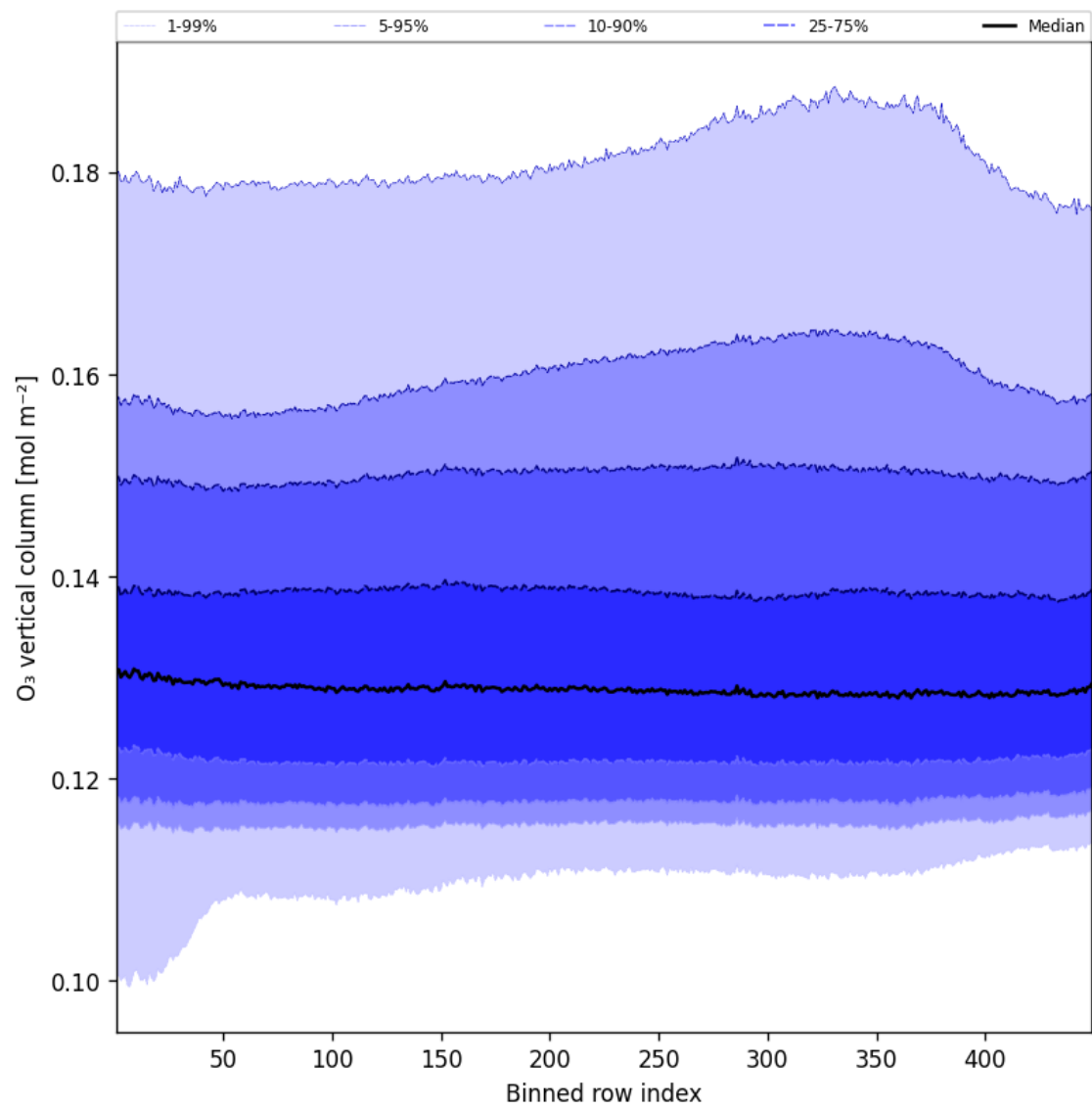
Figure 41: Along track statistics of “O 3 vertical column” for 2025-08-13 to 2025-08-14
