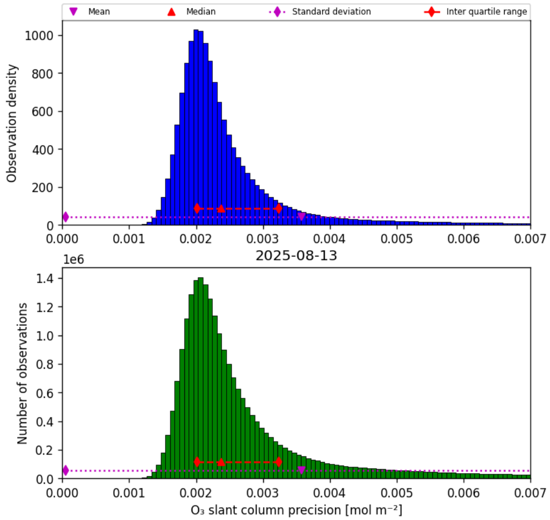
Figure 32: Histogram of “O 3 slant column precision” for 2025-08-13 to 2025-08-14
