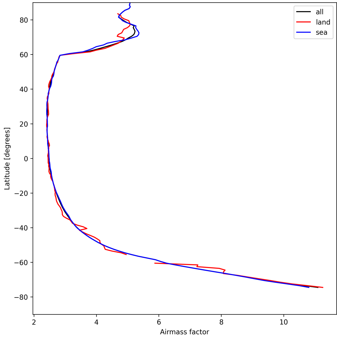
Figure 25: Zonal average of “Airmass factor” for 2025-08-13 to 2025-08-14.
