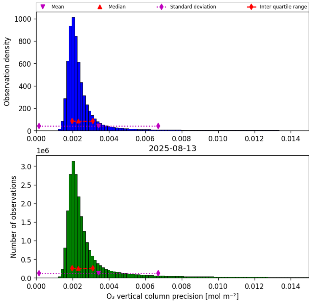
Figure 30: Histogram of “O 3 vertical column precision” for 2025-08-13 to 2025-08-14
