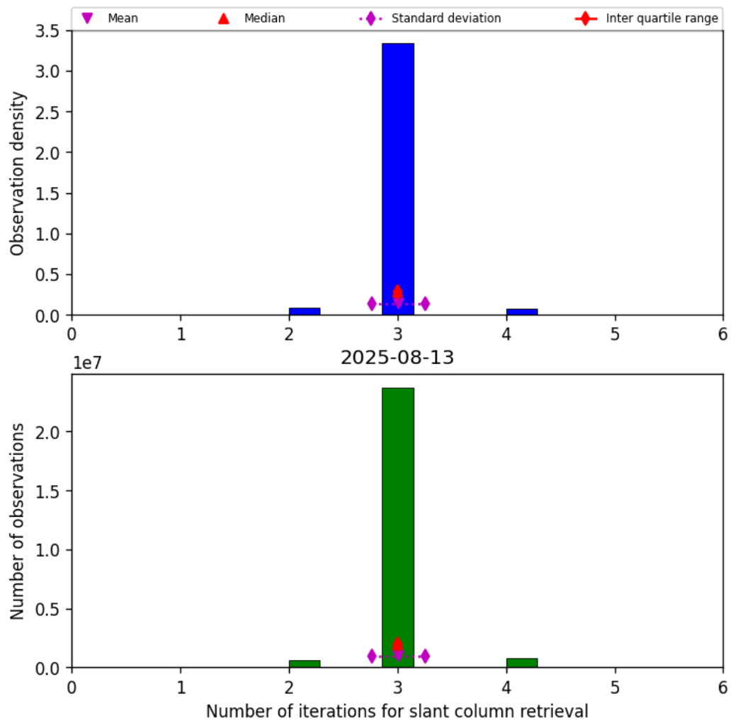
Figure 33: Histogram of “Number of iterations for slant column retrieval” for 2025-08-13 to 2025-08-14
