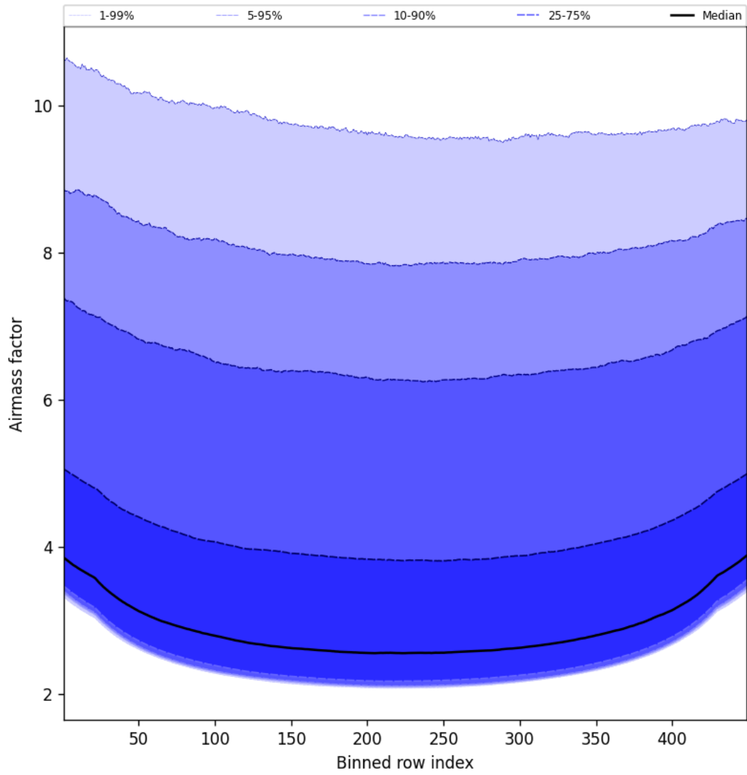
Figure 49: Along track statistics of “Airmass factor” for 2025-08-14 to 2025-08-15
