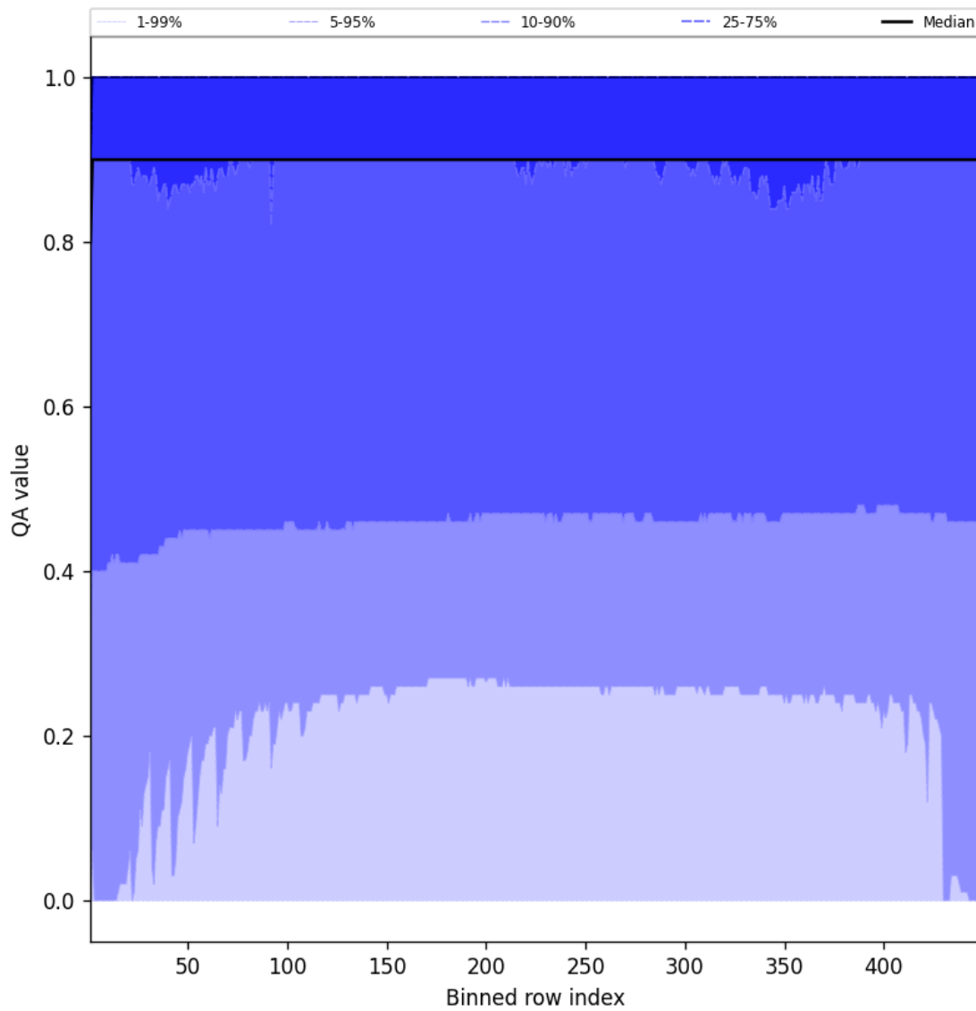
Figure 40: Along track statistics of “QA value” for 2025-08-14 to 2025-08-15
