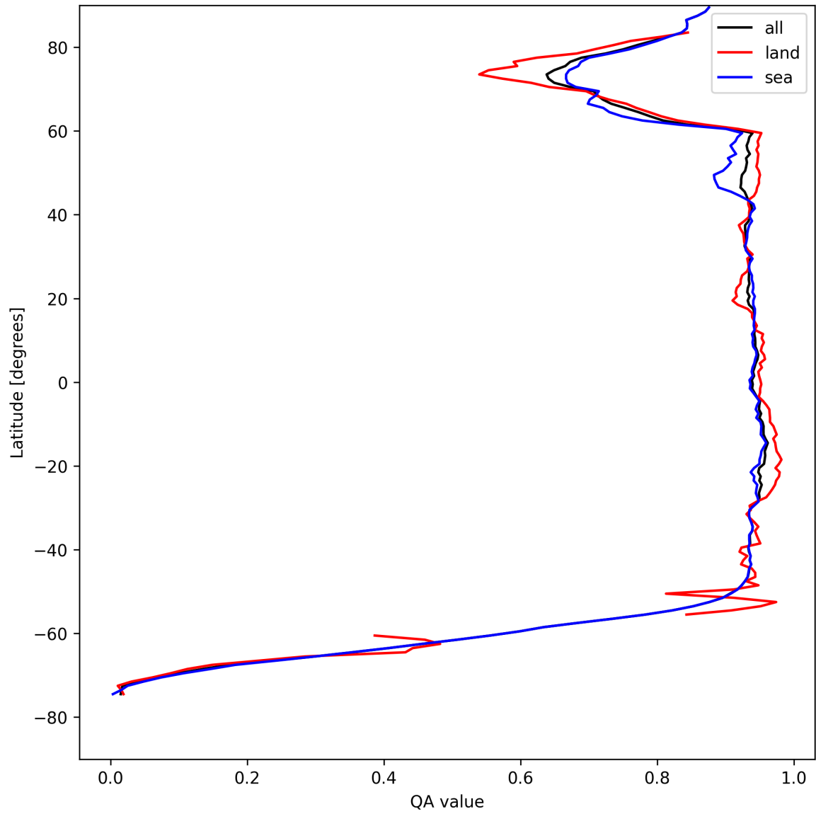
Figure 16: Zonal average of “QA value” for 2025-08-14 to 2025-08-15.
