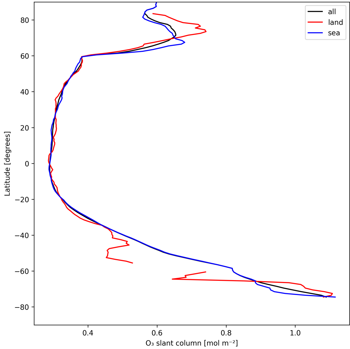
Figure 19: Zonal average of “O 3 slant column” for 2025-08-14 to 2025-08-15.
