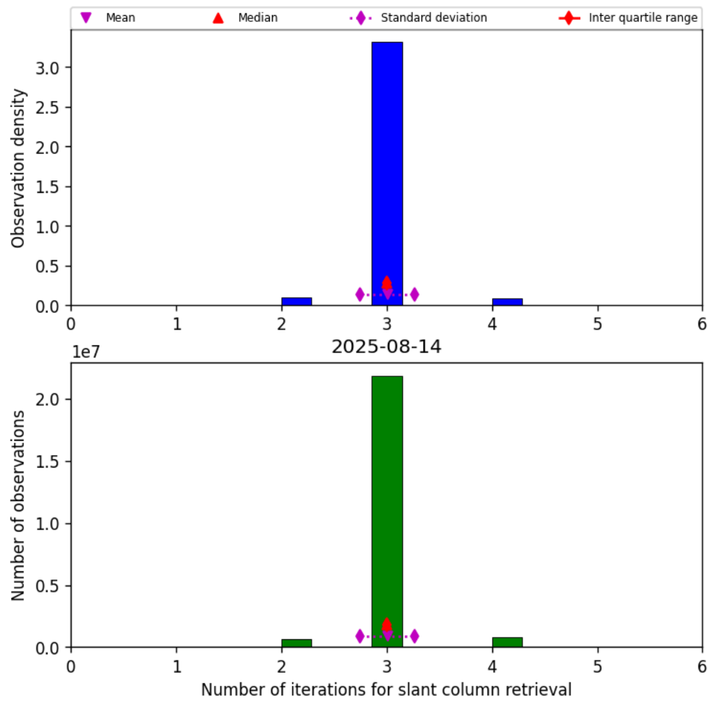
Figure 33: Histogram of “Number of iterations for slant column retrieval” for 2025-08-14 to 2025-08-15
