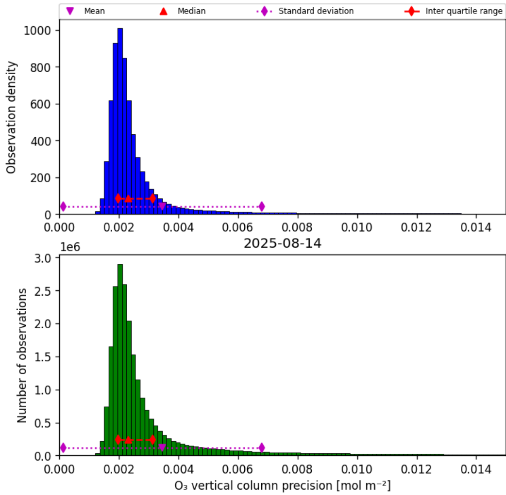
Figure 30: Histogram of “O 3 vertical column precision” for 2025-08-14 to 2025-08-15
