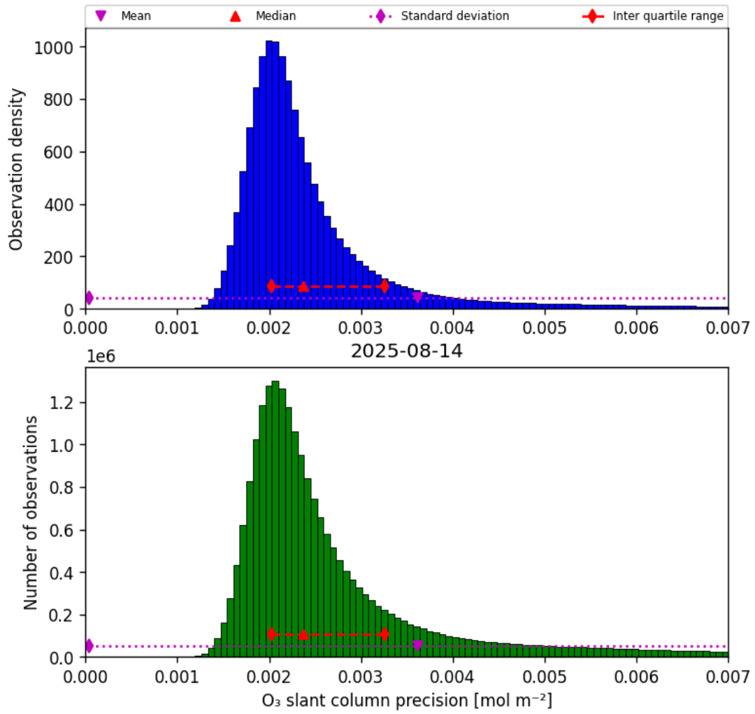
Figure 32: Histogram of “O 3 slant column precision” for 2025-08-14 to 2025-08-15
