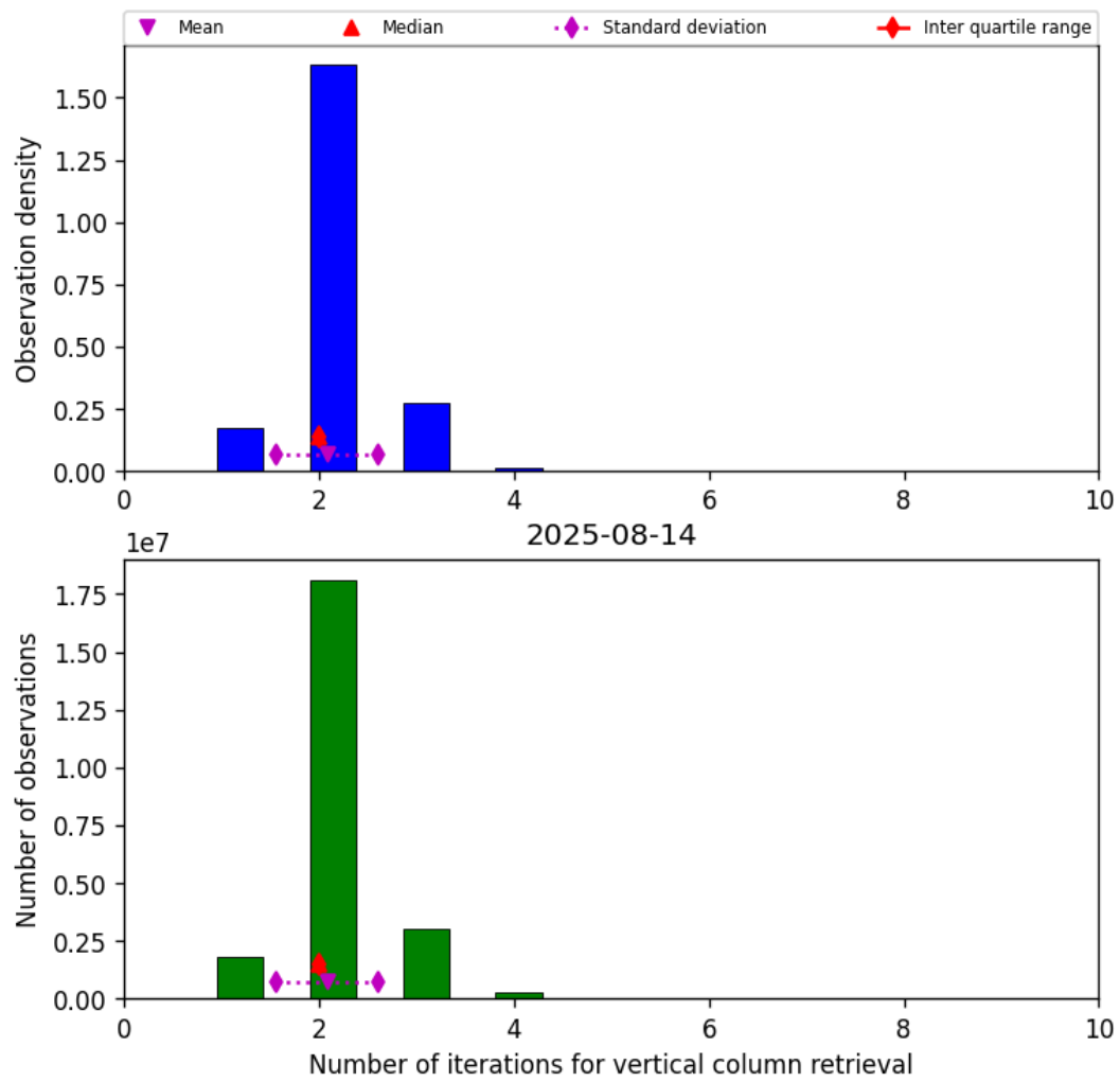
Figure 39: Histogram of “Number of iterations for vertical column retrieval” for 2025-08-14 to 2025-08-15
