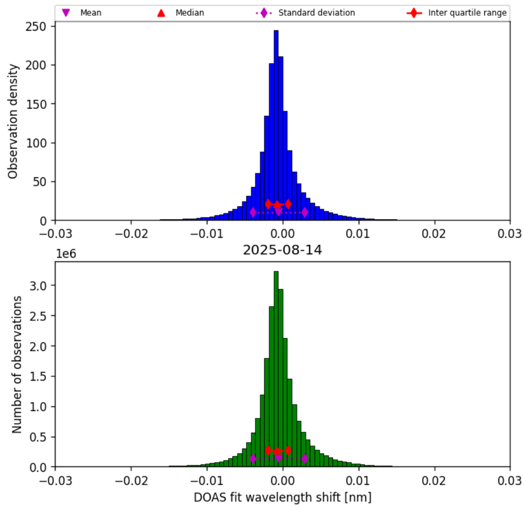
Figure 35: Histogram of “DOAS fit wavelength shift” for 2025-08-14 to 2025-08-15
