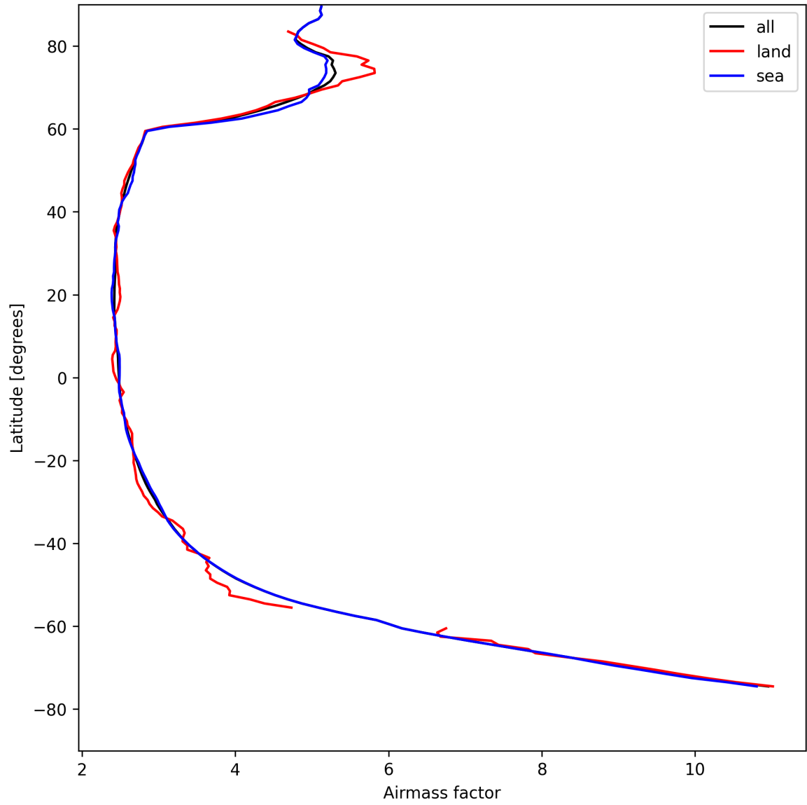
Figure 25: Zonal average of “Airmass factor” for 2025-08-14 to 2025-08-15.
