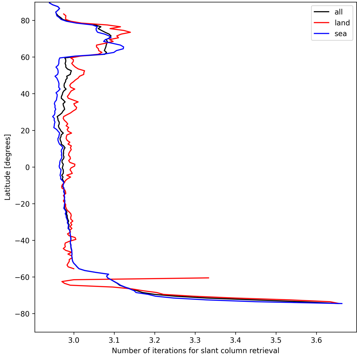
Figure 21: Zonal average of “Number of iterations for slant column retrieval” for 2025-08-14 to 2025-08-15.
