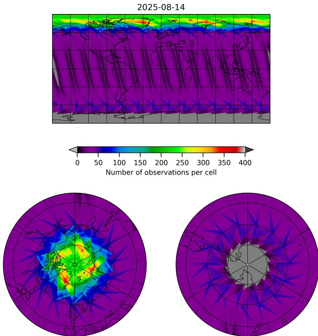
Figure 15: Map of the number of observations for 2025-08-14 to 2025-08-15
