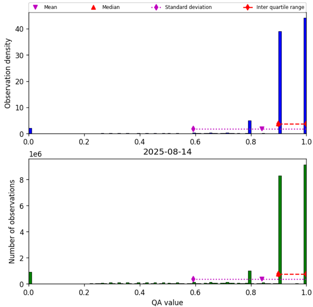
Figure 28: Histogram of “QA value” for 2025-08-14 to 2025-08-15
