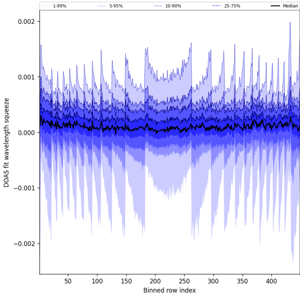
Figure 48: Along track statistics of “DOAS fit wavelength squeeze” for 2025-08-14 to 2025-08-15
