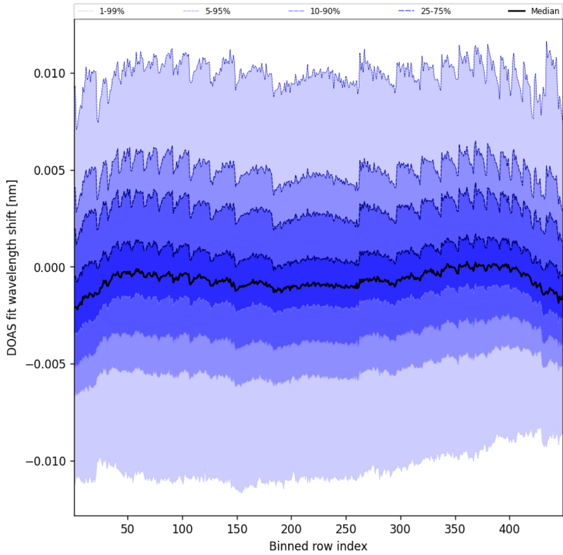
Figure 47: Along track statistics of "DOAS fit wavelength shift" for 2025-08-14 to 2025-08-15
