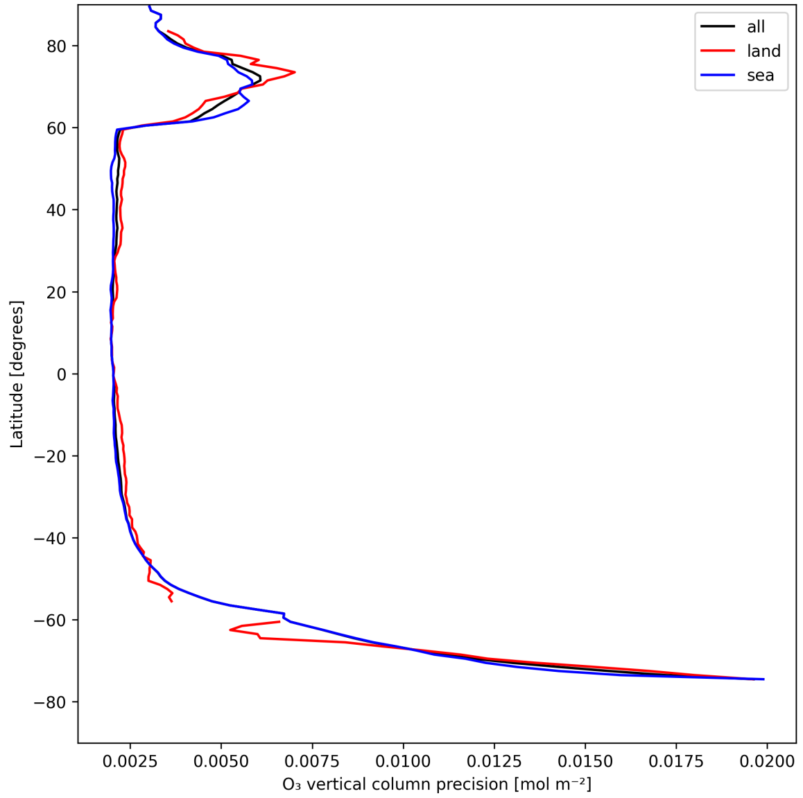
Figure 18: Zonal average of "O 3 vertical column precision" for 2025-08-14 to 2025-08-15.
