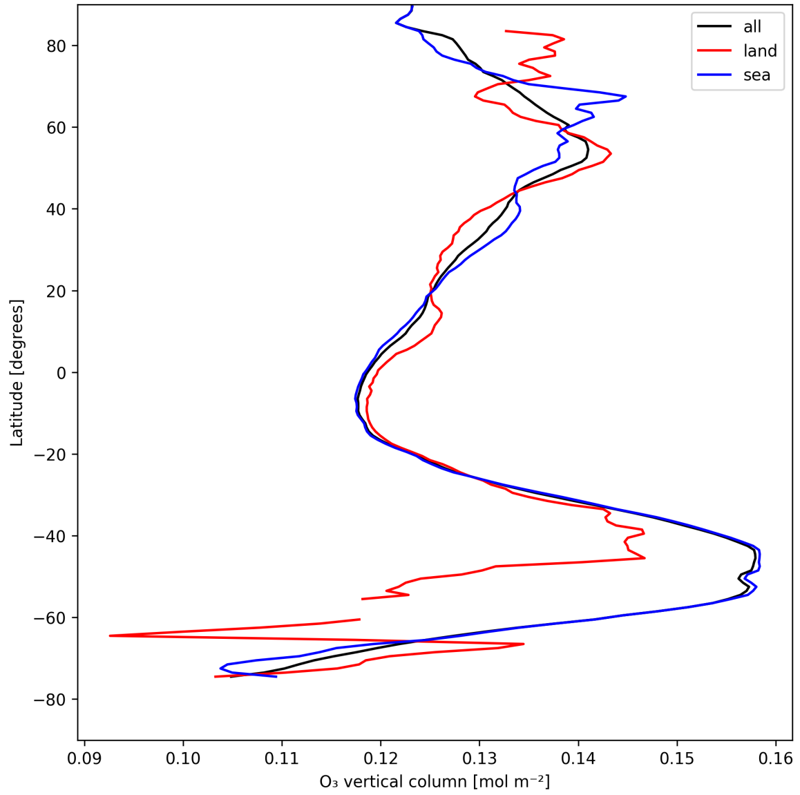
Figure 17: Zonal average of “O 3 vertical column” for 2025-08-14 to 2025-08-15.
