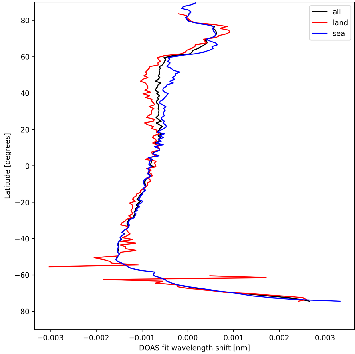
Figure 23: Zonal average of “DOAS fit wavelength shift” for 2025-08-14 to 2025-08-15.
