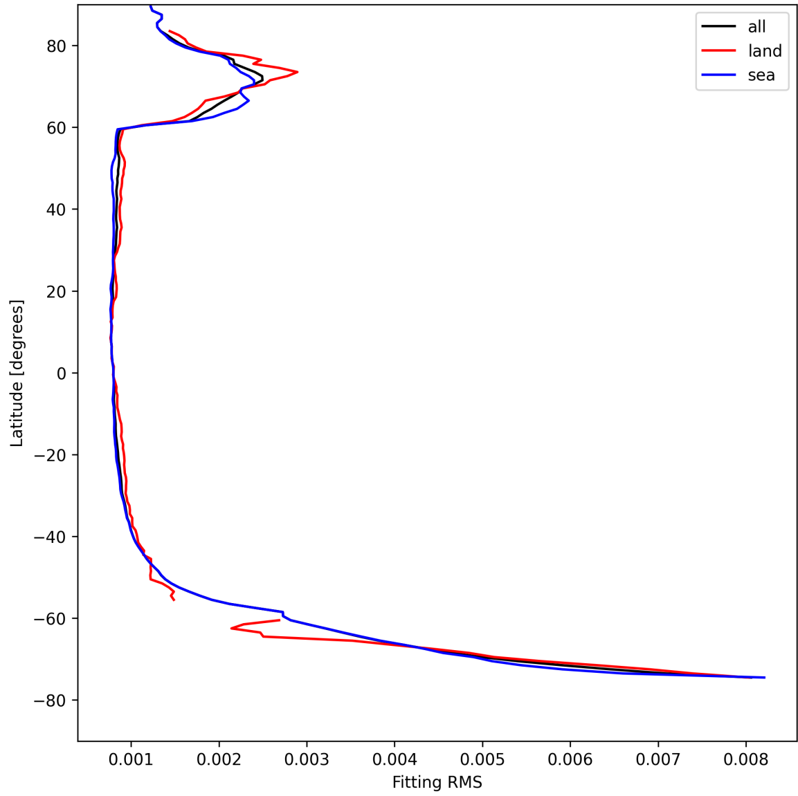
Figure 22: Zonal average of “Fitting RMS” for 2025-08-14 to 2025-08-15.
