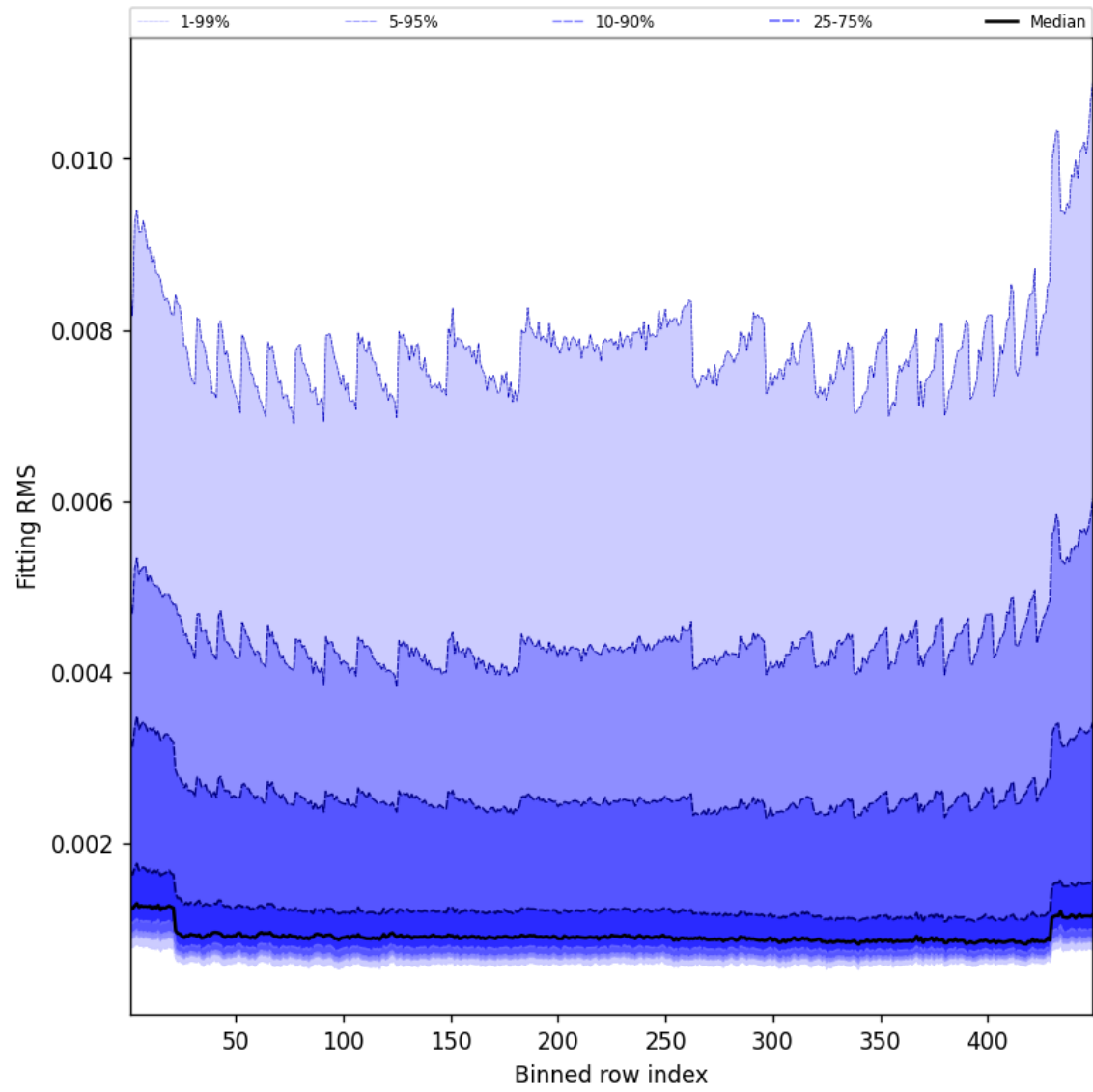
Figure 46: Along track statistics of “Fitting RMS” for 2025-08-14 to 2025-08-15
