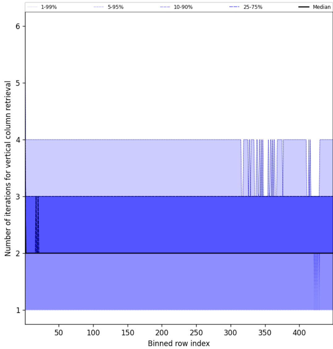
Figure 51: Along track statistics of “Number of iterations for vertical column retrieval” for 2025-08-14 to 2025-08-15
