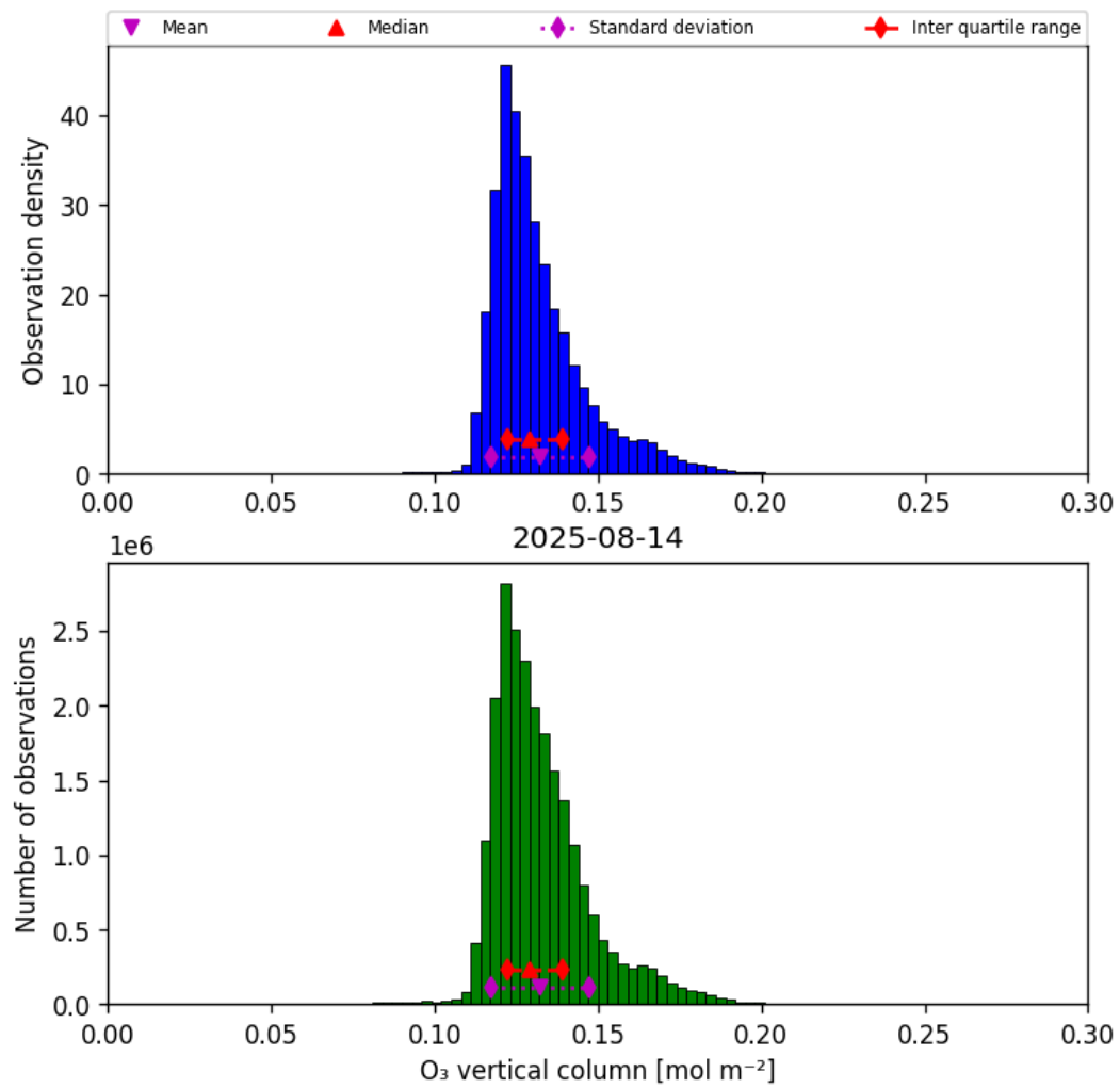
Figure 29: Histogram of “O 3 vertical column” for 2025-08-14 to 2025-08-15
