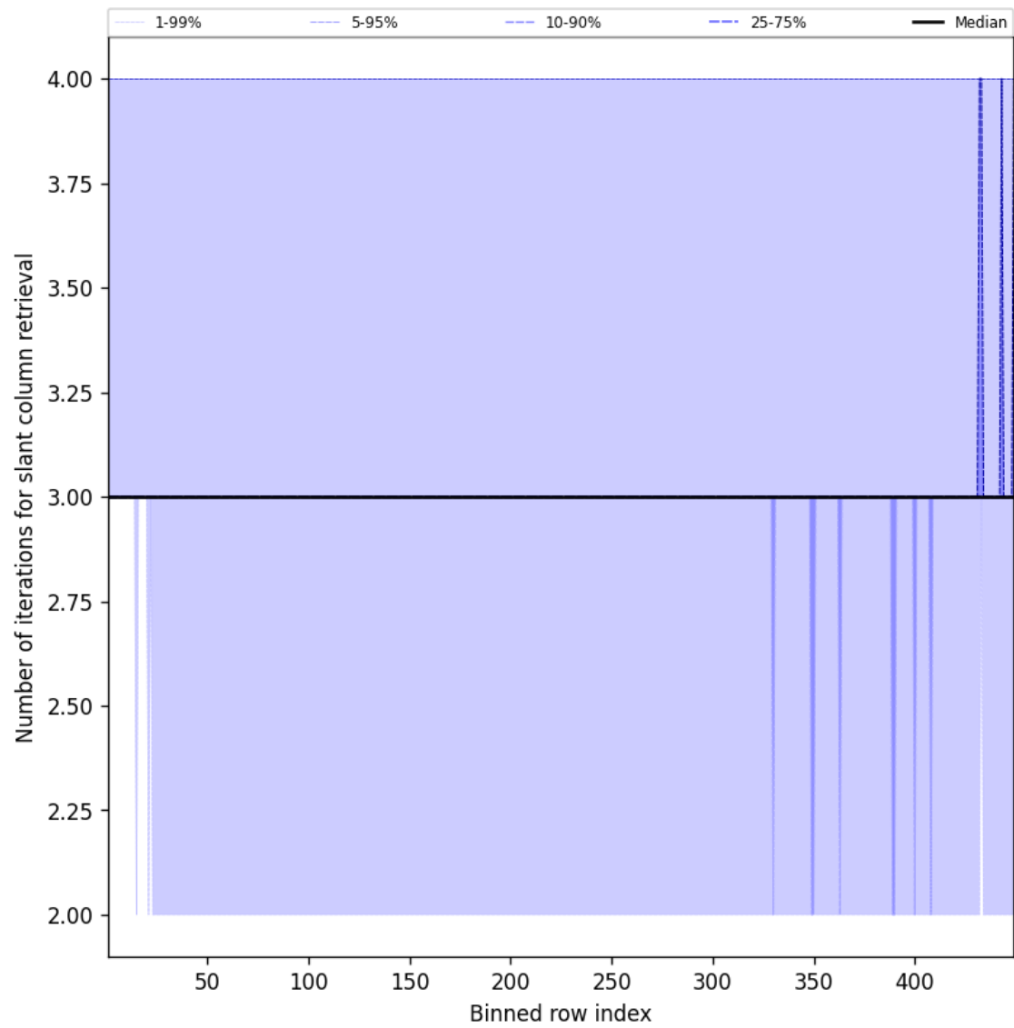
Figure 45: Along track statistics of “Number of iterations for slant column retrieval” for 2025-08-14 to 2025-08-15
