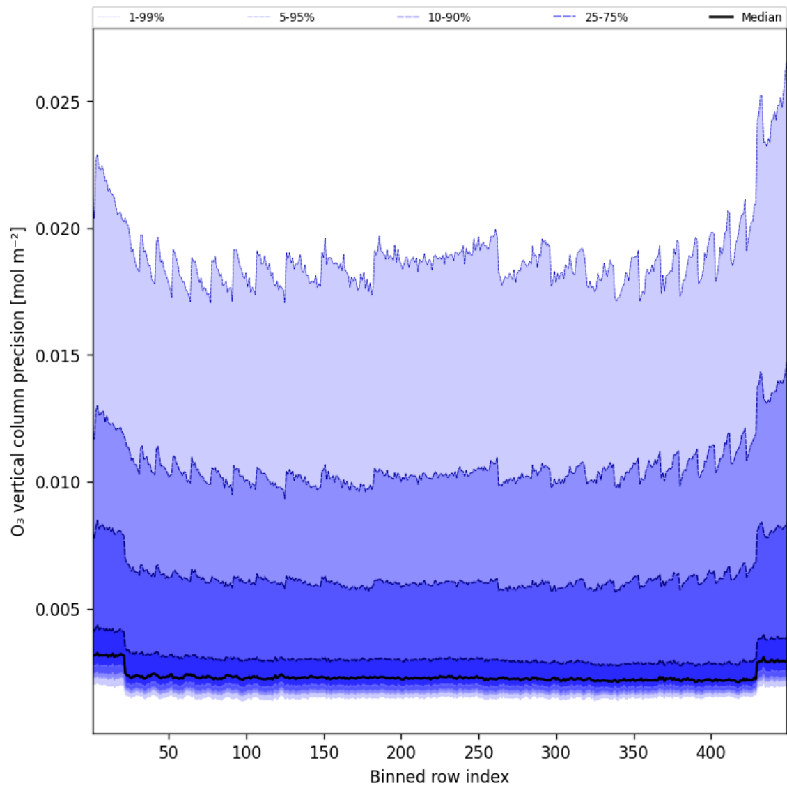
Figure 42: Along track statistics of “O 3 vertical column precision” for 2025-08-14 to 2025-08-15
