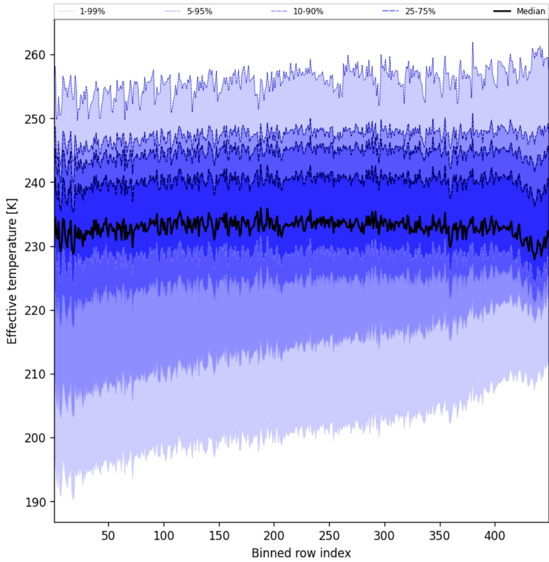
Figure 50: Along track statistics of “Effective temperature” for 2025-08-14 to 2025-08-15
