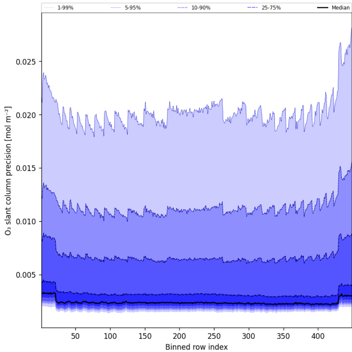
Figure 44: Along track statistics of “O 3 slant column precision” for 2025-08-14 to 2025-08-15
