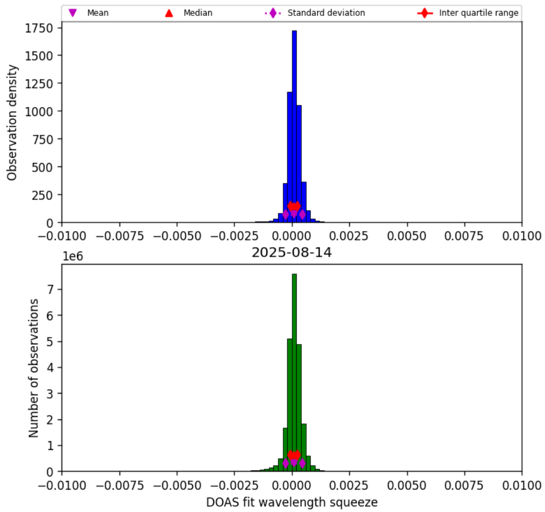
Figure 36: Histogram of “DOAS fit wavelength squeeze” for 2025-08-14 to 2025-08-15
