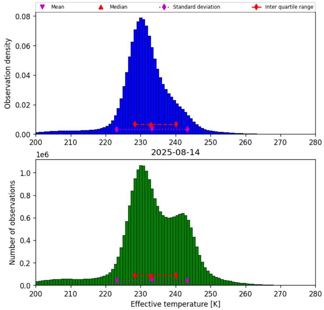
Figure 38: Histogram of “Effective temperature” for 2025-08-14 to 2025-08-15
