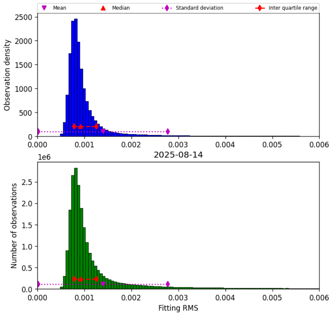
Figure 34: Histogram of “Fitting RMS” for 2025-08-14 to 2025-08-15
