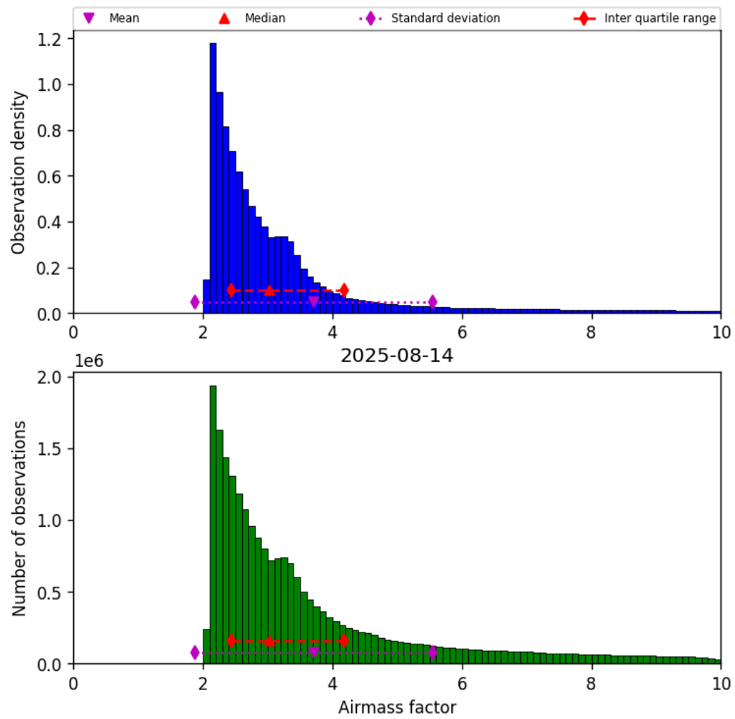
Figure 37: Histogram of “Airmass factor” for 2025-08-14 to 2025-08-15
