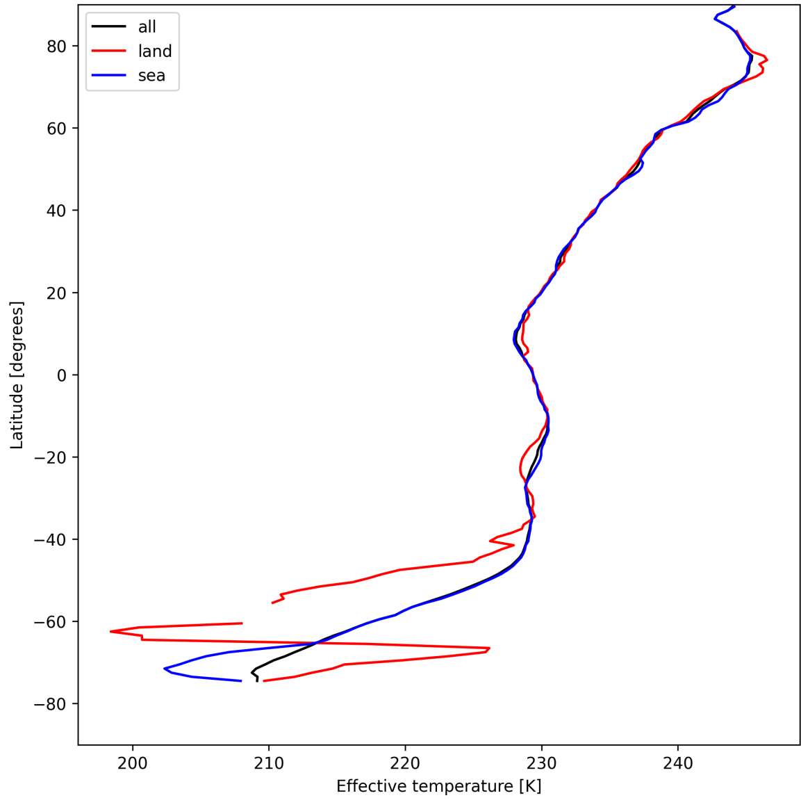
Figure 26: Zonal average of “Effective temperature” for 2025-08-14 to 2025-08-15.
