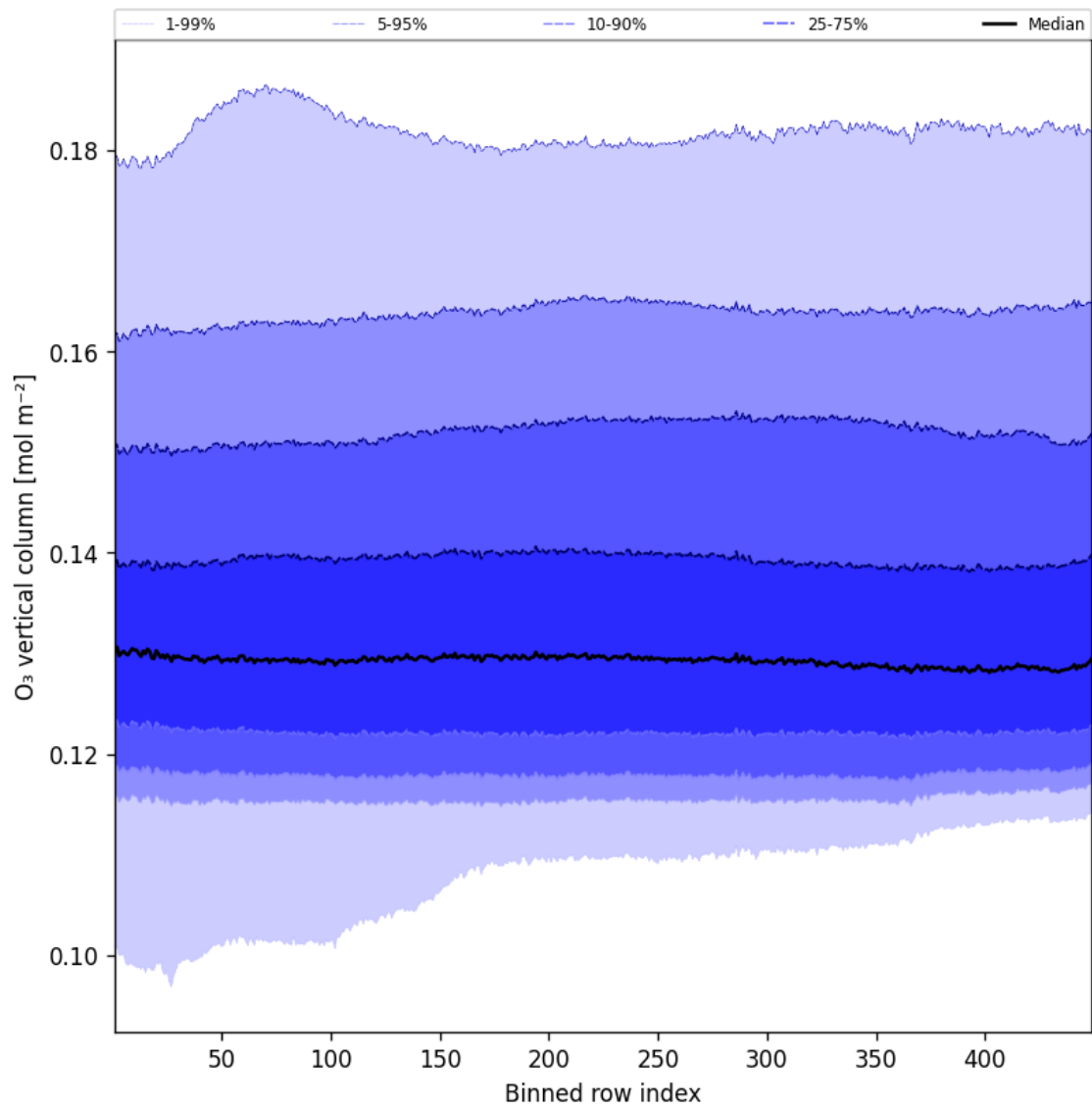
Figure 41: Along track statistics of “O 3 vertical column” for 2025-08-14 to 2025-08-15
