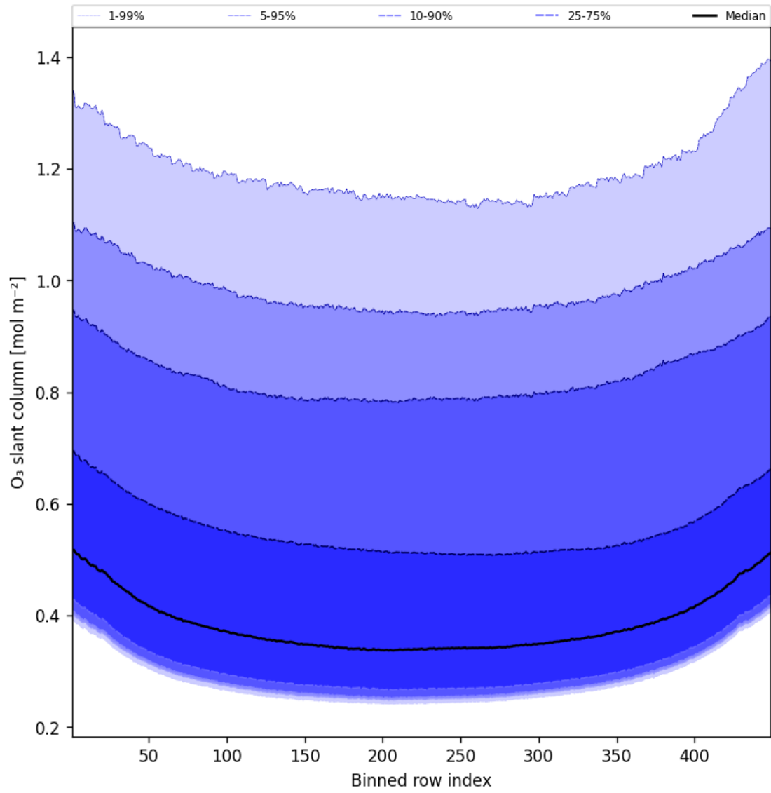
Figure 43: Along track statistics of “O 3 slant column” for 2025-08-14 to 2025-08-15
