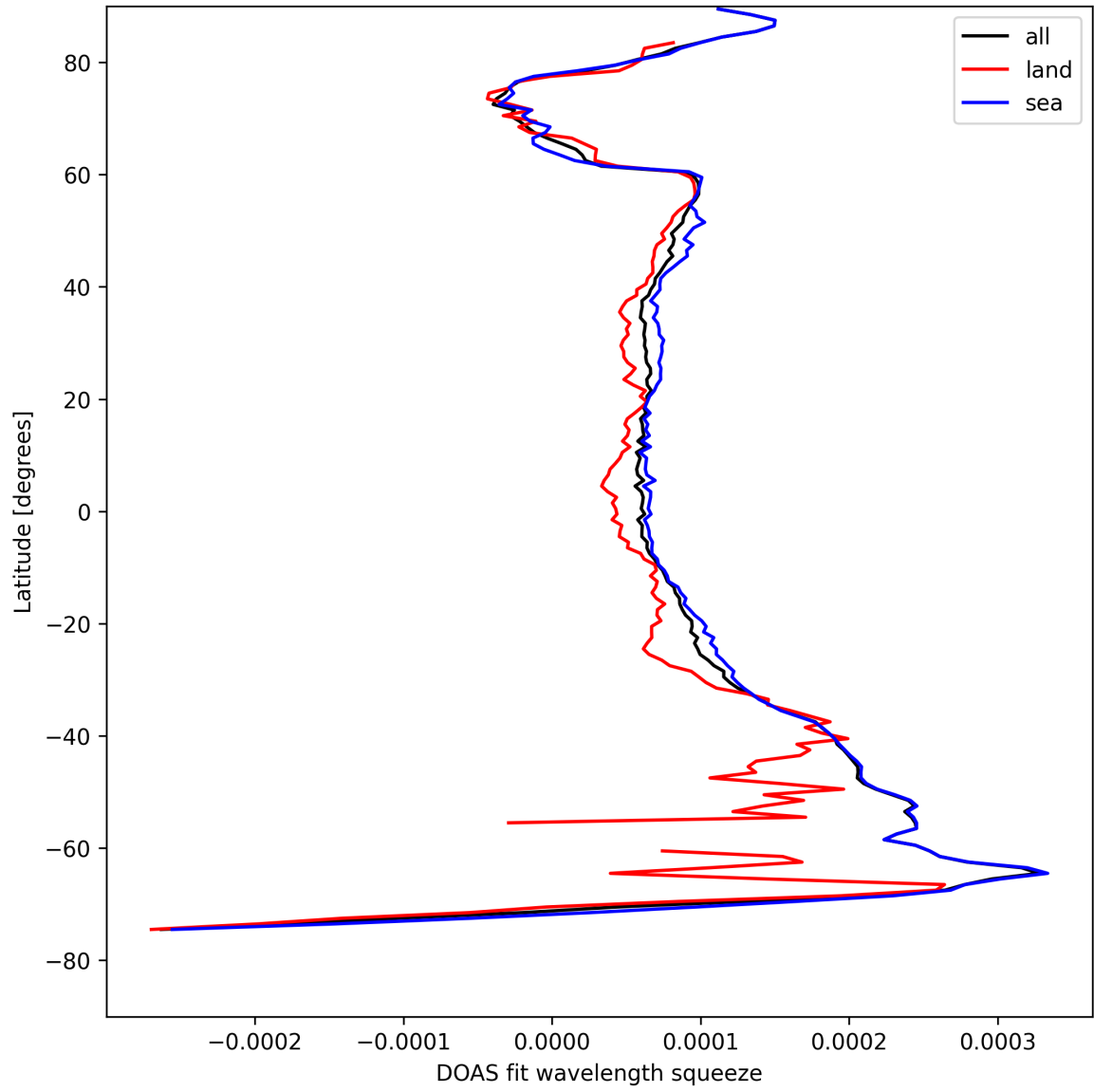
Figure 24: Zonal average of "DOAS fit wavelength squeeze" for 2025-08-14 to 2025-08-15.
