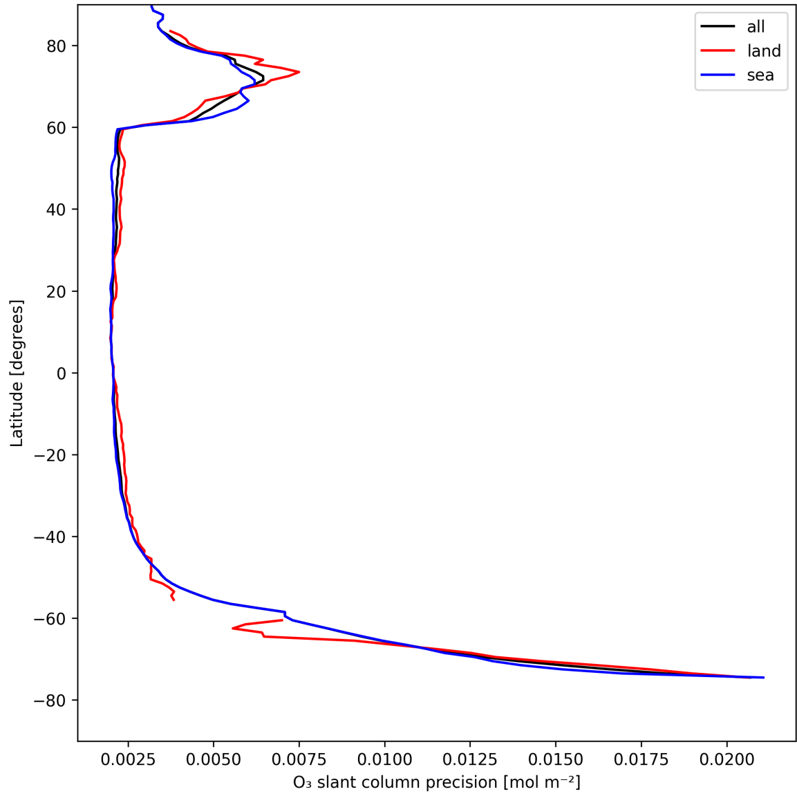
Figure 20: Zonal average of "O 3 slant column precision" for 2025-08-14 to 2025-08-15.
