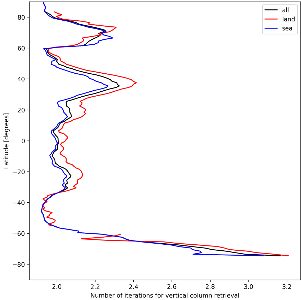
Figure 27: Zonal average of “Number of iterations for vertical column retrieval” for 2025-08-14 to 2025-08-15.
