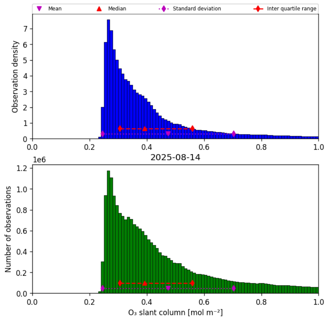
Figure 31: Histogram of “O 3 slant column” for 2025-08-14 to 2025-08-15
