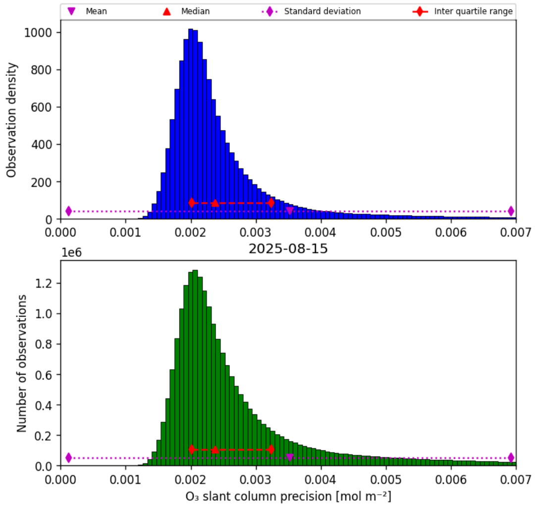
Figure 32: Histogram of “O 3 slant column precision” for 2025-08-15 to 2025-08-16
