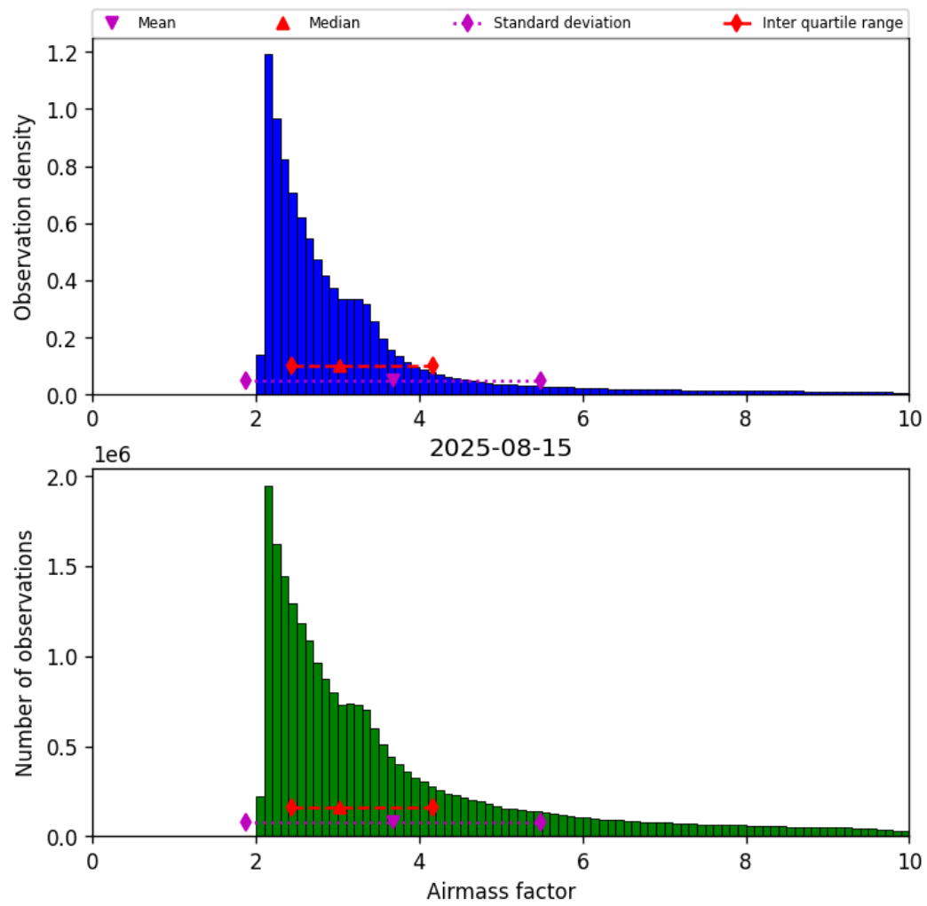
Figure 37: Histogram of “Airmass factor” for 2025-08-15 to 2025-08-16
