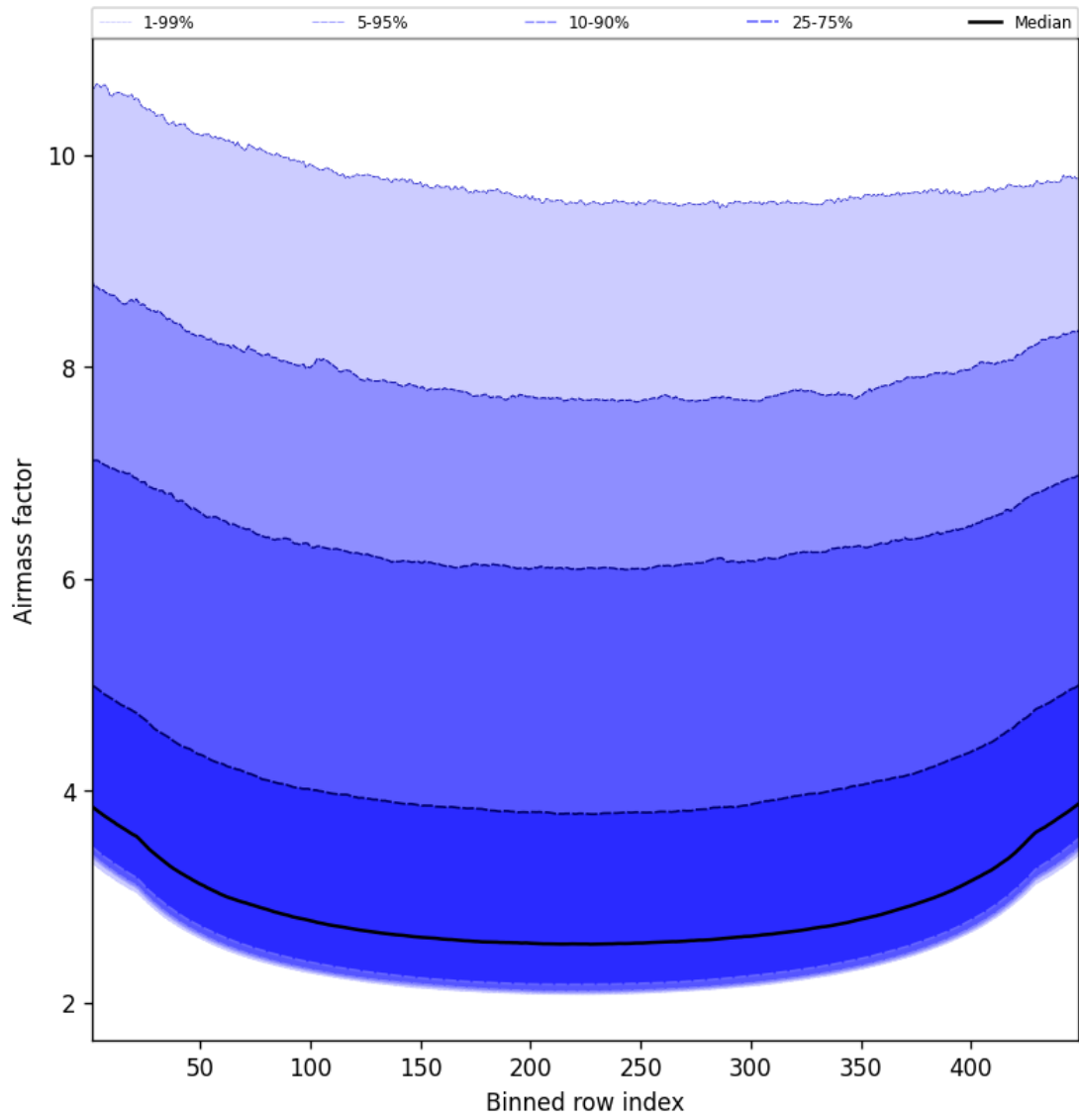
Figure 49: Along track statistics of “Airmass factor” for 2025-08-15 to 2025-08-16
