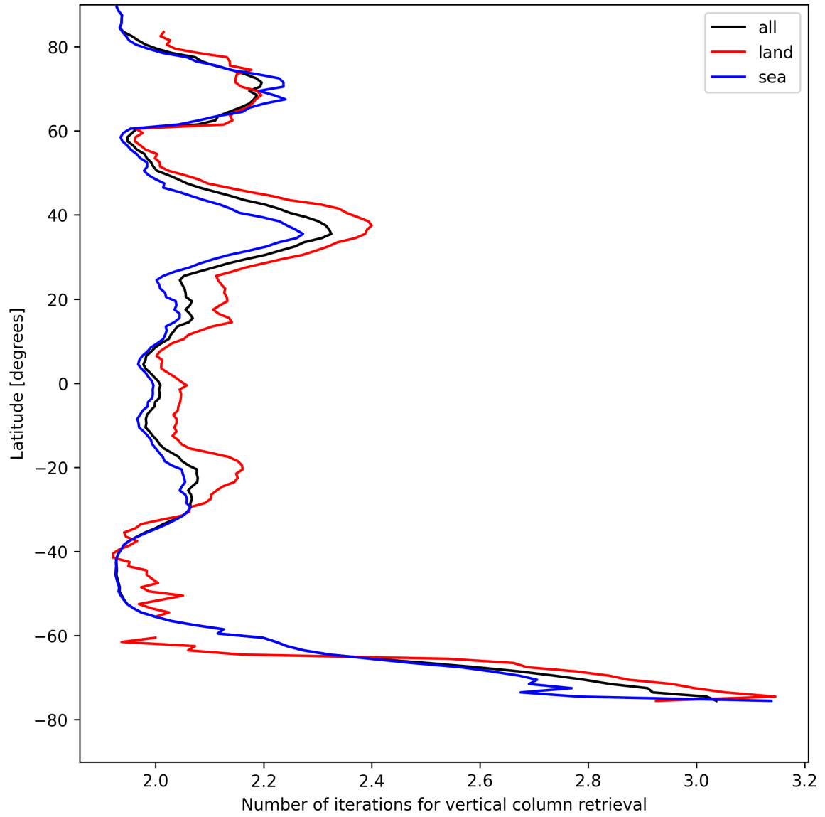
Figure 27: Zonal average of “Number of iterations for vertical column retrieval” for 2025-08-15 to 2025-08-16.
