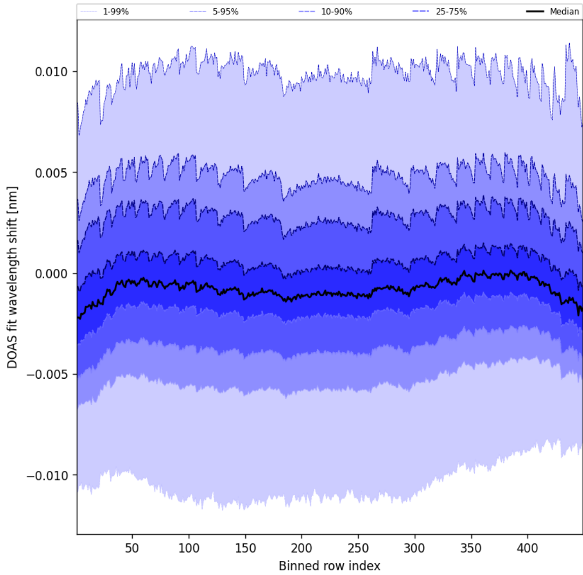
Figure 47: Along track statistics of “DOAS fit wavelength shift” for 2025-08-15 to 2025-08-16
