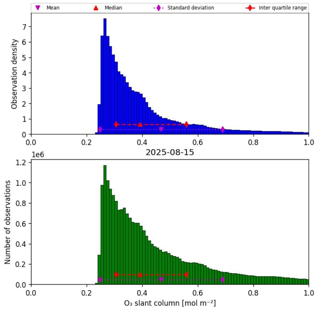
Figure 31: Histogram of “O 3 slant column” for 2025-08-15 to 2025-08-16
