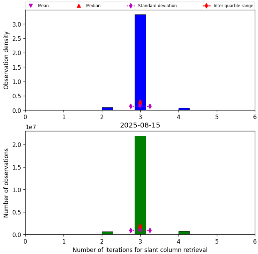
Figure 33: Histogram of “Number of iterations for slant column retrieval” for 2025-08-15 to 2025-08-16
