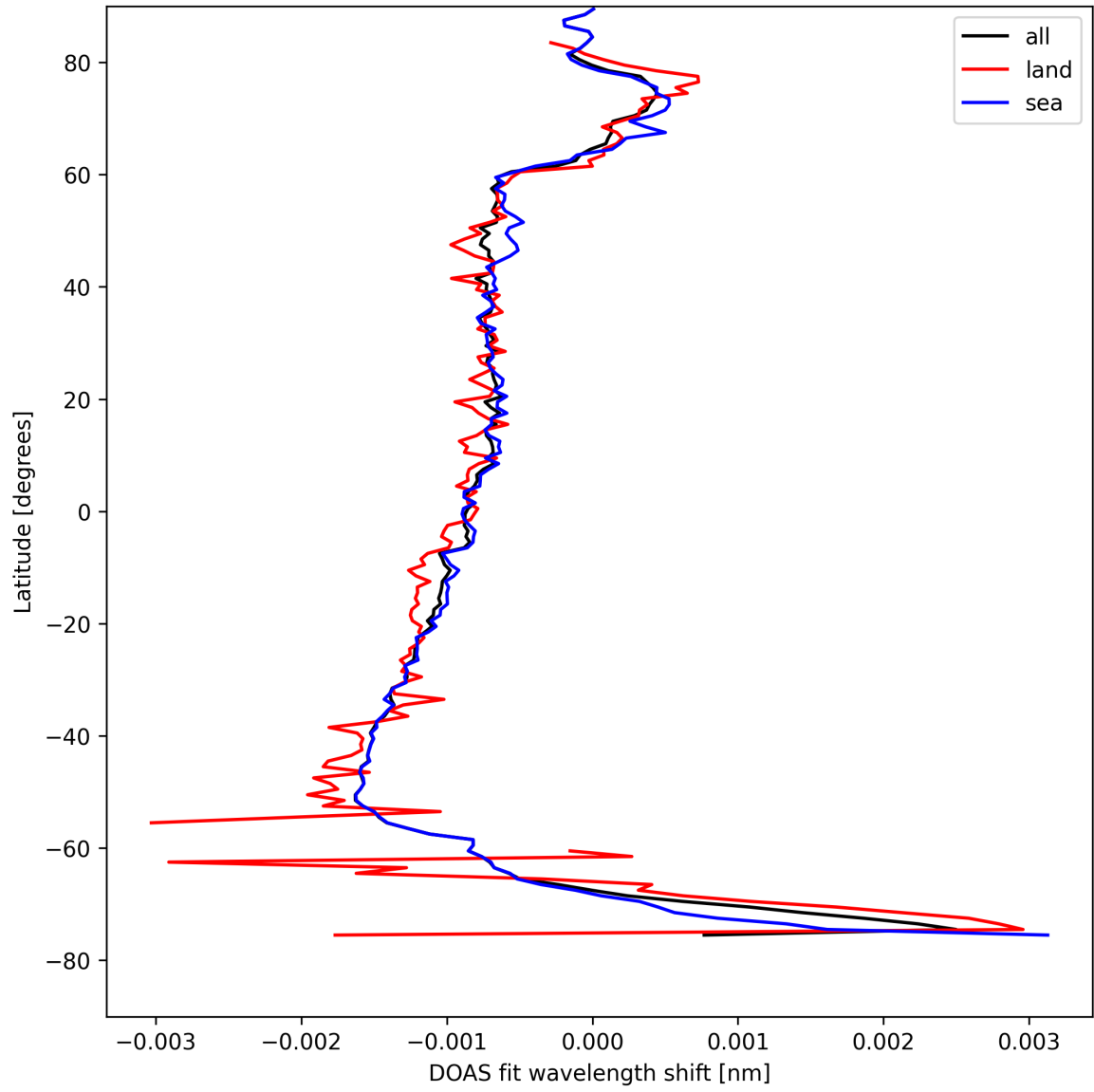
Figure 23: Zonal average of "DOAS fit wavelength shift" for 2025-08-15 to 2025-08-16.
