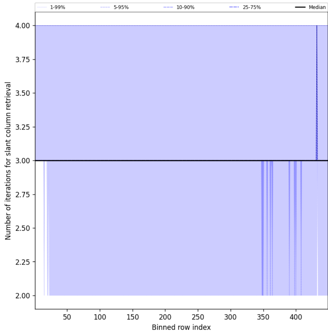
Figure 45: Along track statistics of “Number of iterations for slant column retrieval” for 2025-08-15 to 2025-08-16
