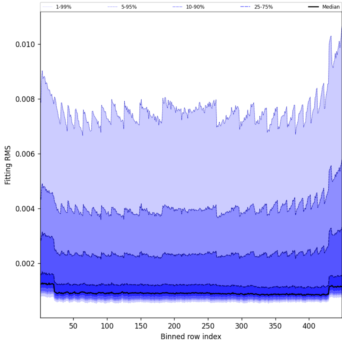
Figure 46: Along track statistics of “Fitting RMS” for 2025-08-15 to 2025-08-16
