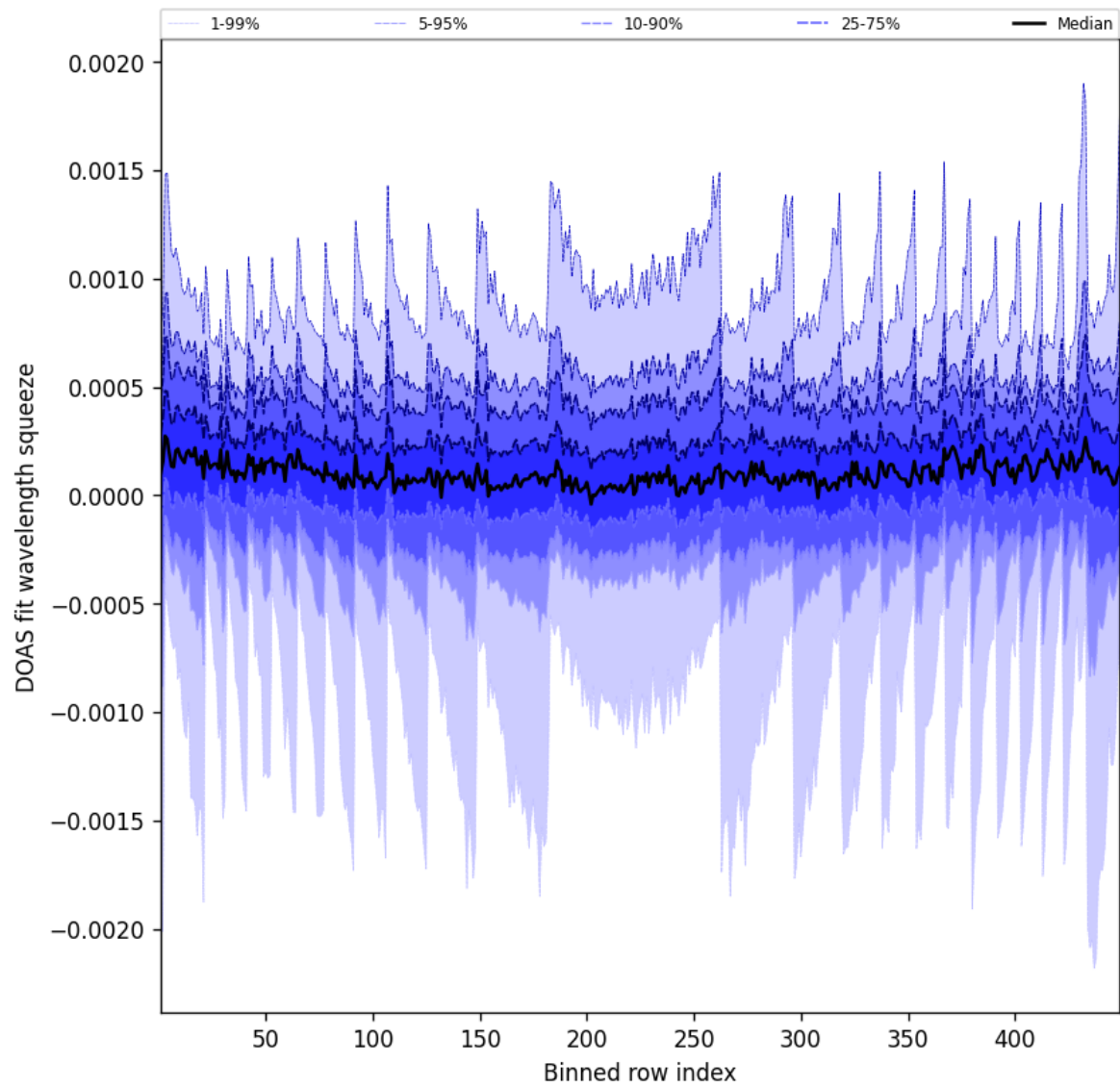
Figure 48: Along track statistics of “DOAS fit wavelength squeeze” for 2025-08-15 to 2025-08-16
