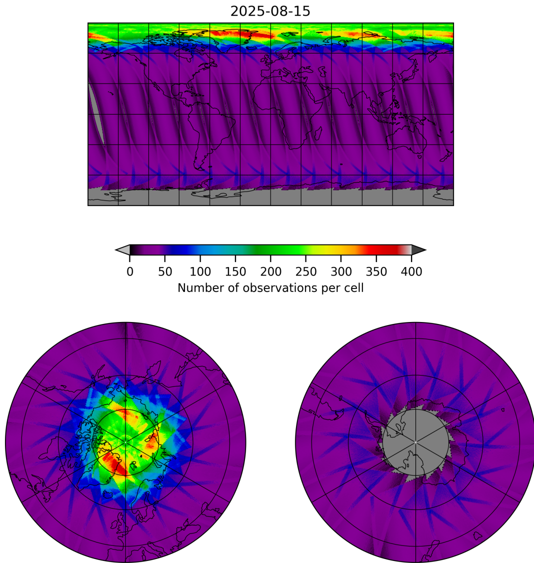
Figure 15: Map of the number of observations for 2025-08-15 to 2025-08-16
