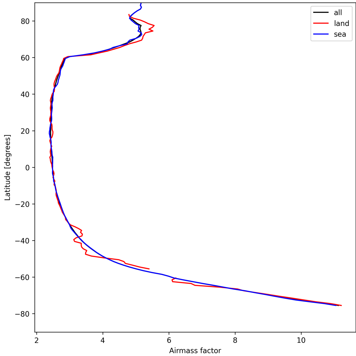
Figure 25: Zonal average of “Airmass factor” for 2025-08-15 to 2025-08-16.
