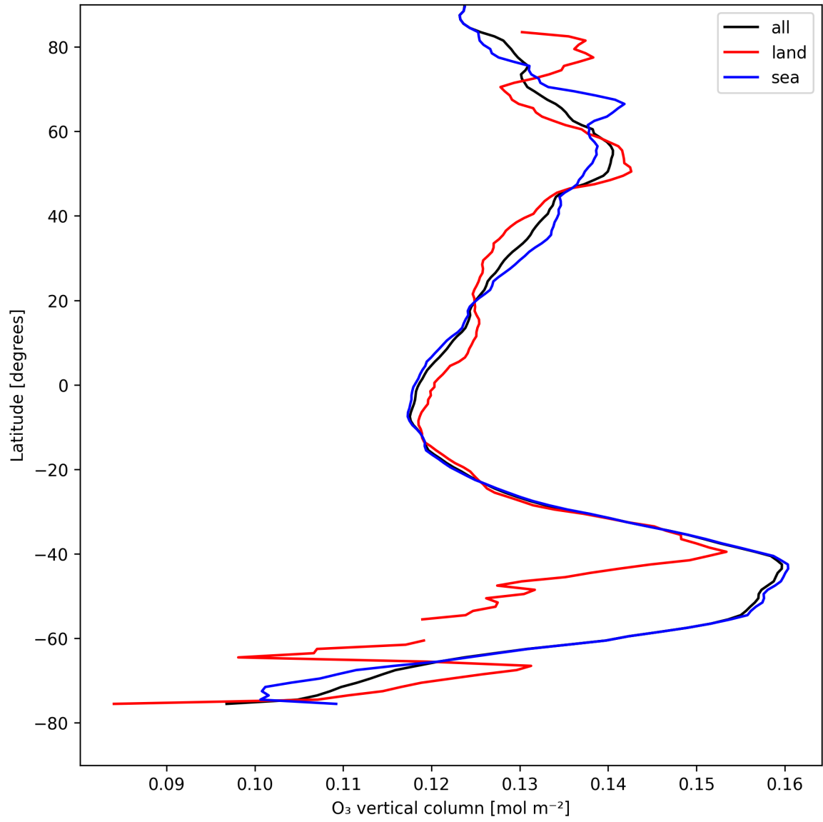
Figure 17: Zonal average of “O 3 vertical column” for 2025-08-15 to 2025-08-16.
