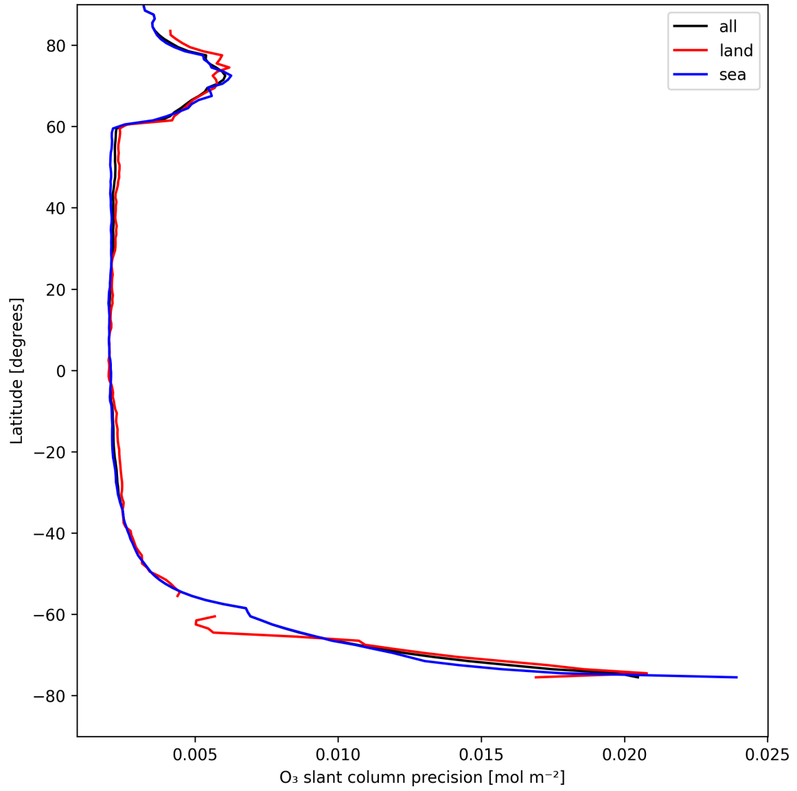
Figure 20: Zonal average of “O 3 slant column precision” for 2025-08-15 to 2025-08-16.
