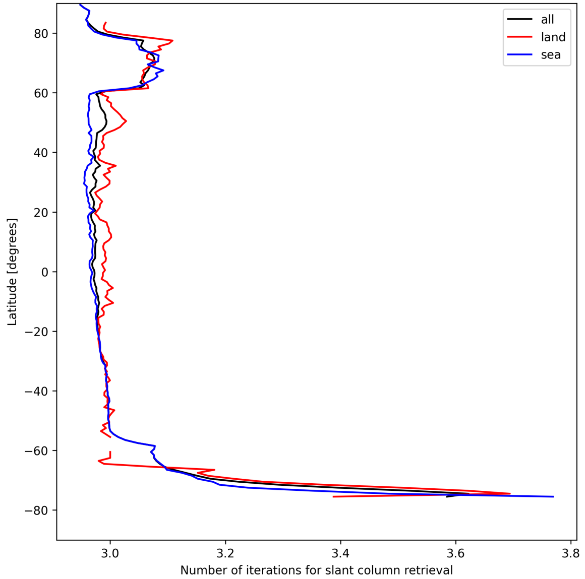
Figure 21: Zonal average of “Number of iterations for slant column retrieval” for 2025-08-15 to 2025-08-16.
