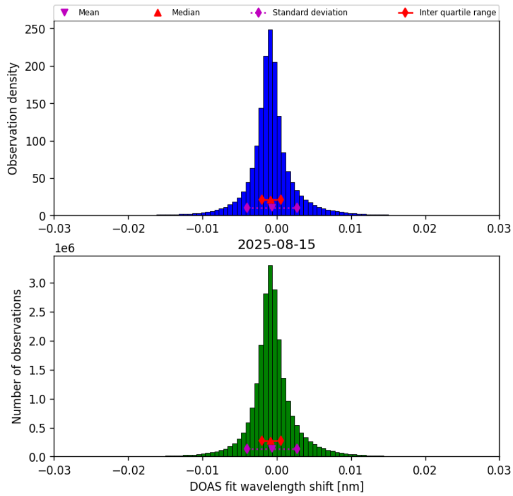
Figure 35: Histogram of “DOAS fit wavelength shift” for 2025-08-15 to 2025-08-16
