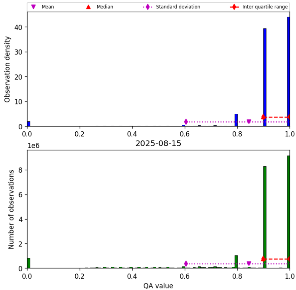
Figure 28: Histogram of “QA value” for 2025-08-15 to 2025-08-16
