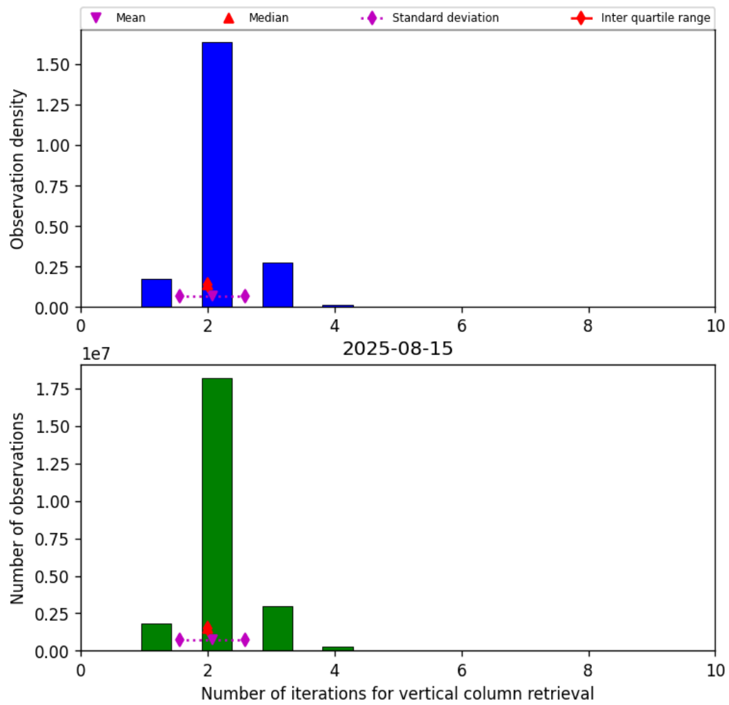
Figure 39: Histogram of “Number of iterations for vertical column retrieval” for 2025-08-15 to 2025-08-16
