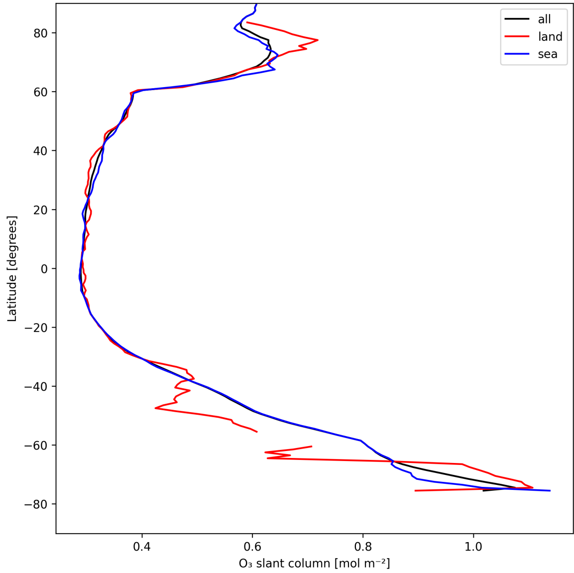
Figure 19: Zonal average of “O 3 slant column” for 2025-08-15 to 2025-08-16.
