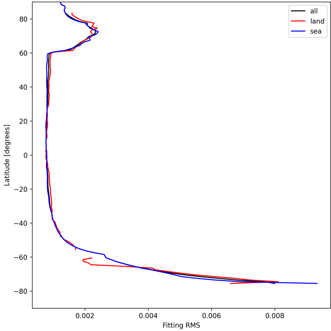
Figure 22: Zonal average of “Fitting RMS” for 2025-08-15 to 2025-08-16.
