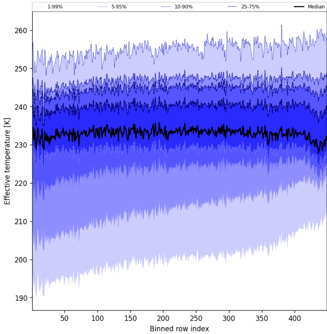
Figure 50: Along track statistics of “Effective temperature” for 2025-08-15 to 2025-08-16
