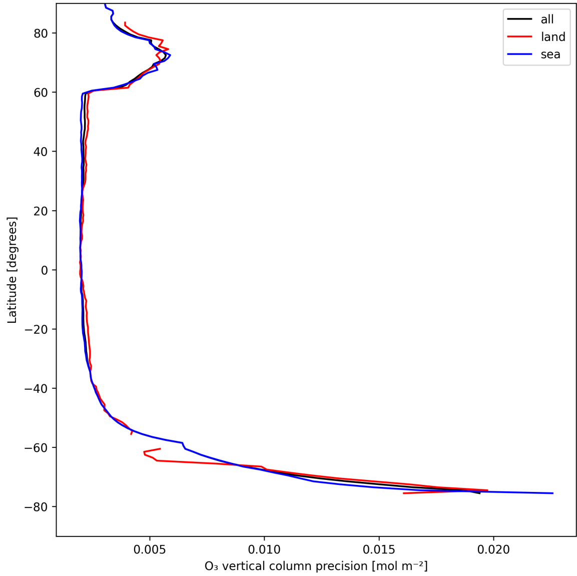
Figure 18: Zonal average of “O 3 vertical column precision” for 2025-08-15 to 2025-08-16.
