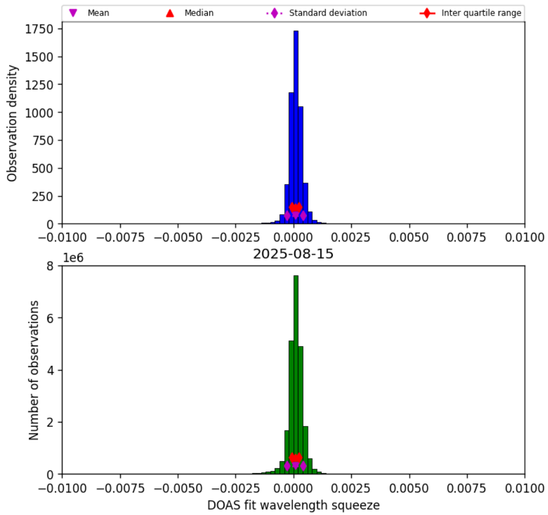
Figure 36: Histogram of “DOAS fit wavelength squeeze” for 2025-08-15 to 2025-08-16
