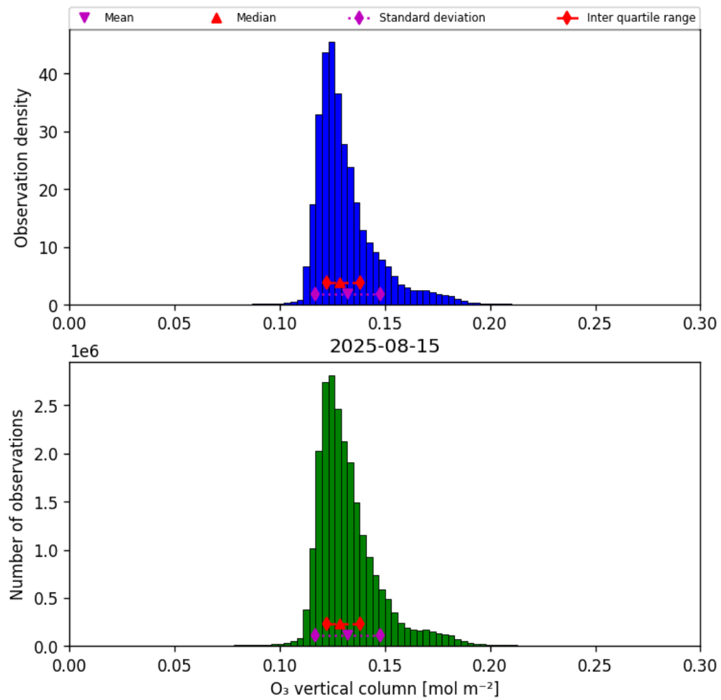
Figure 29: Histogram of “O 3 vertical column” for 2025-08-15 to 2025-08-16
