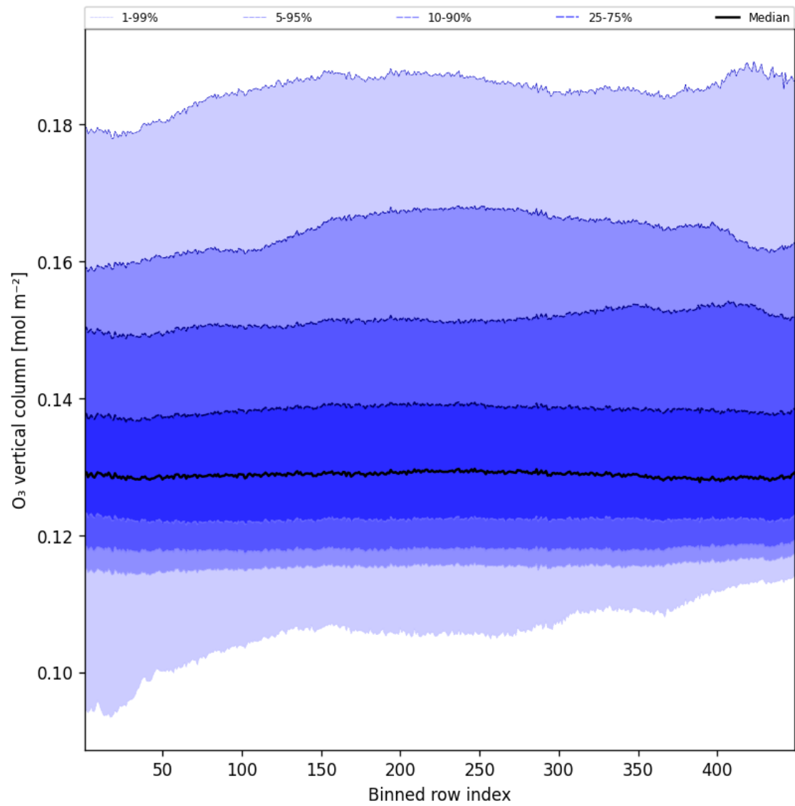
Figure 41: Along track statistics of “O 3 vertical column” for 2025-08-15 to 2025-08-16
