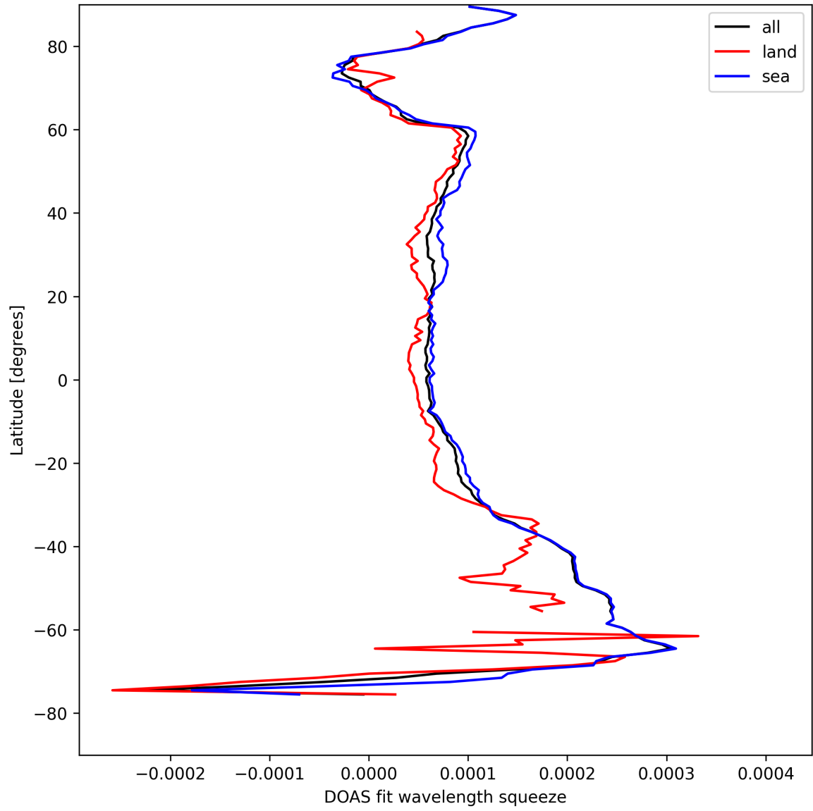
Figure 24: Zonal average of “DOAS fit wavelength squeeze” for 2025-08-15 to 2025-08-16.
