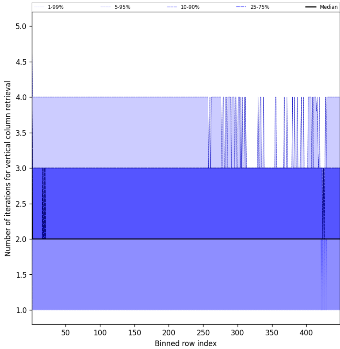
Figure 51: Along track statistics of “Number of iterations for vertical column retrieval” for 2025-08-15 to 2025-08-16
