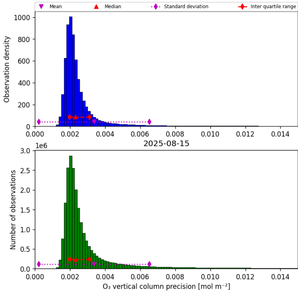
Figure 30: Histogram of “O 3 vertical column precision” for 2025-08-15 to 2025-08-16
