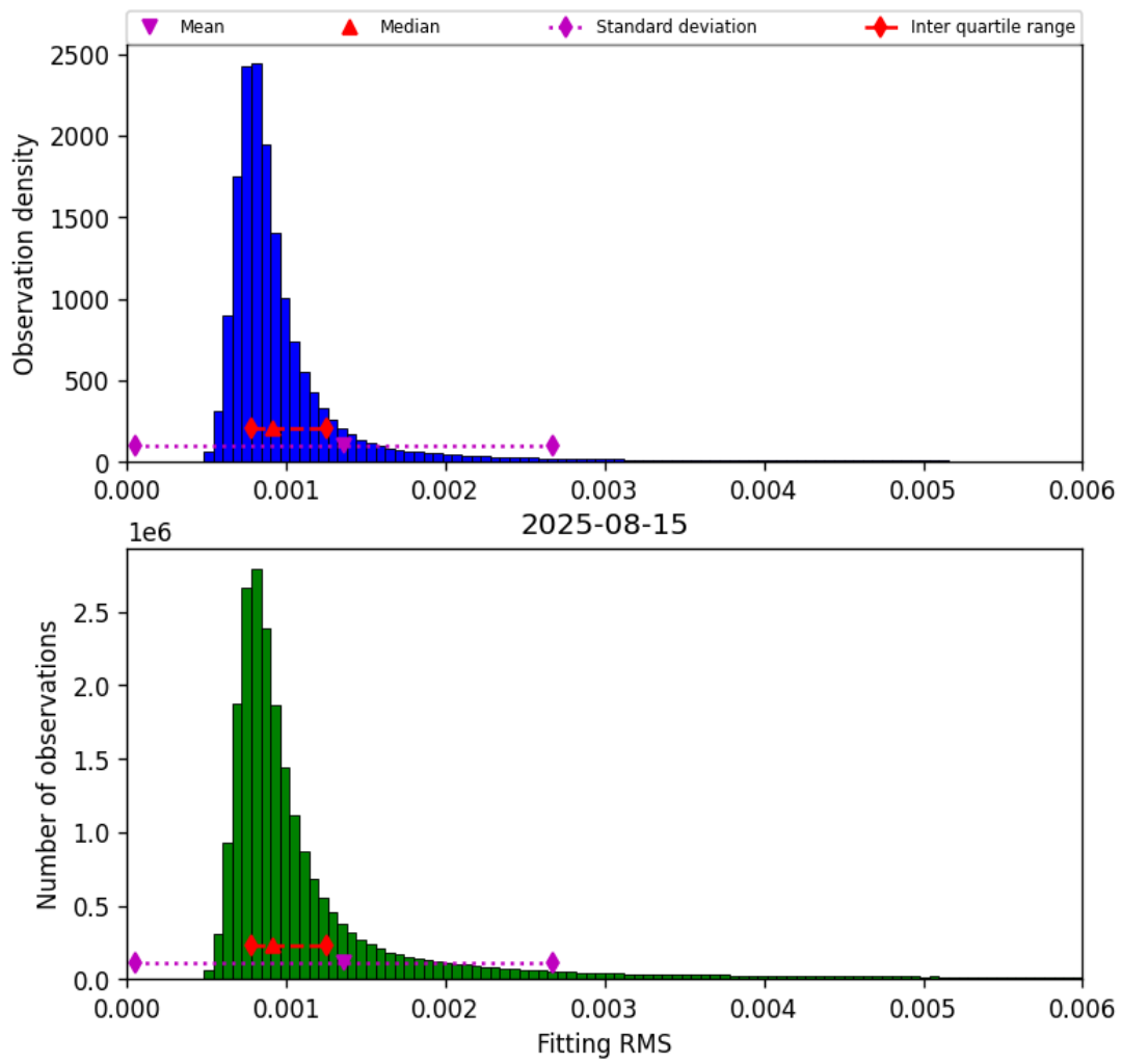
Figure 34: Histogram of “Fitting RMS” for 2025-08-15 to 2025-08-16
