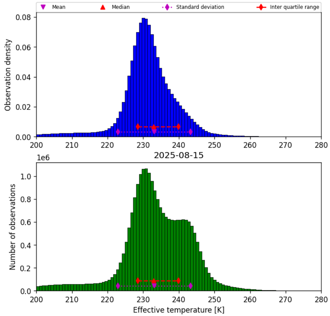
Figure 38: Histogram of “Effective temperature” for 2025-08-15 to 2025-08-16
