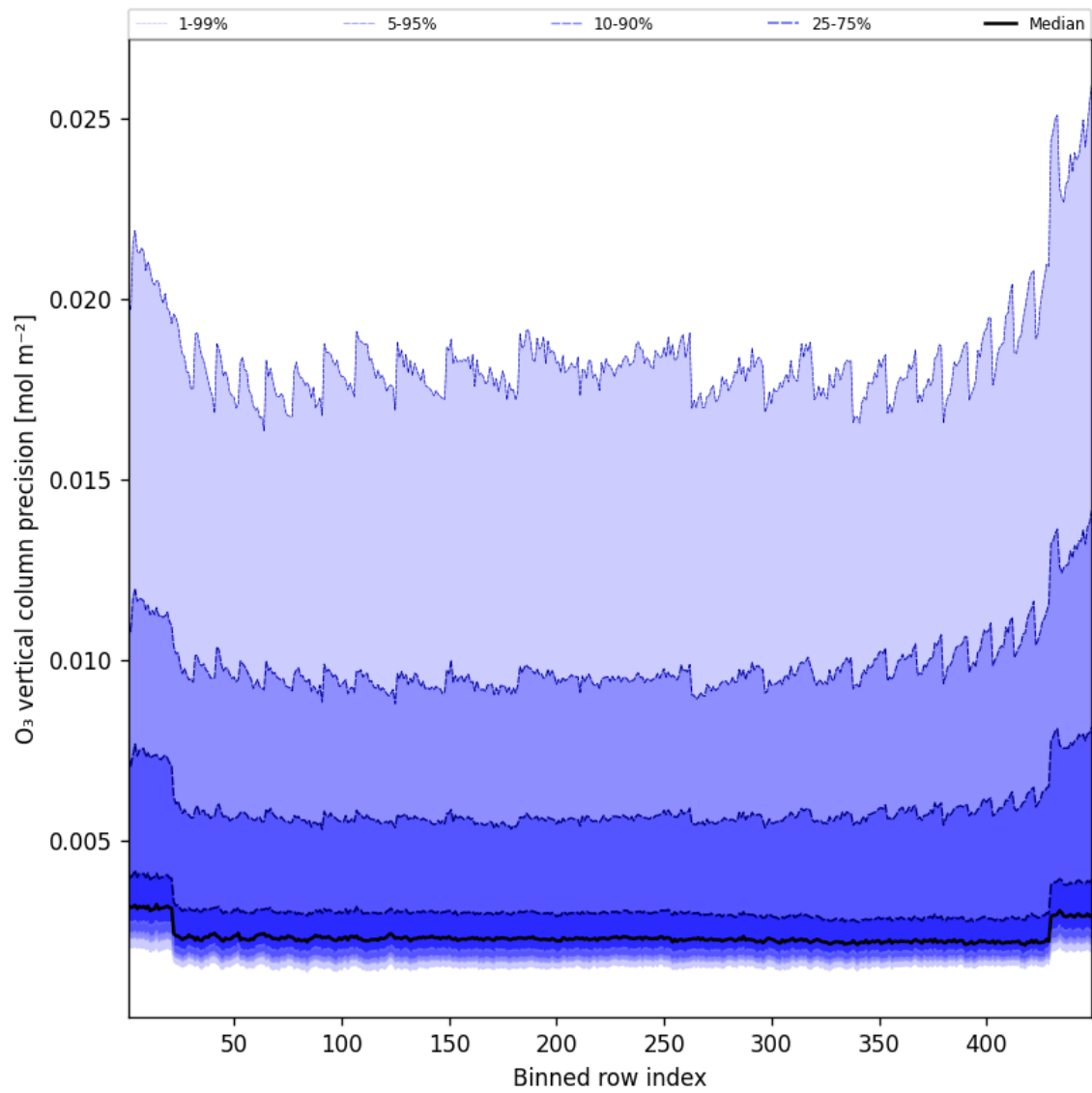
Figure 42: Along track statistics of “O 3 vertical column precision” for 2025-08-15 to 2025-08-16
