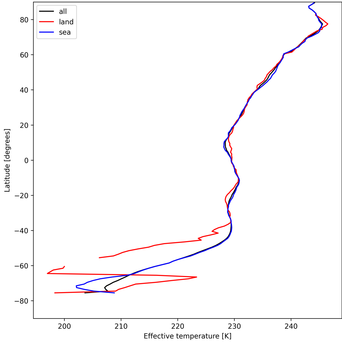
Figure 26: Zonal average of “Effective temperature” for 2025-08-15 to 2025-08-16.
