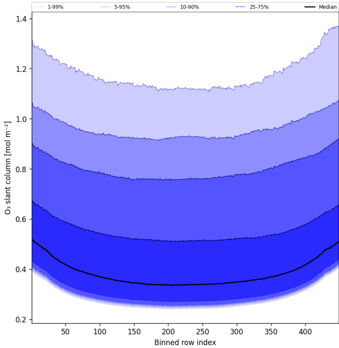
Figure 43: Along track statistics of “O 3 slant column” for 2025-08-15 to 2025-08-16
