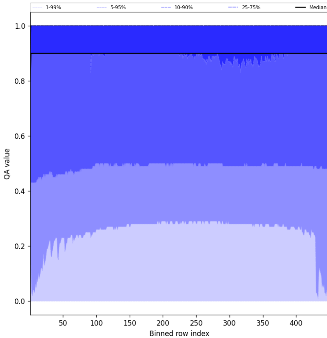
Figure 40: Along track statistics of “QA value” for 2025-08-15 to 2025-08-16
