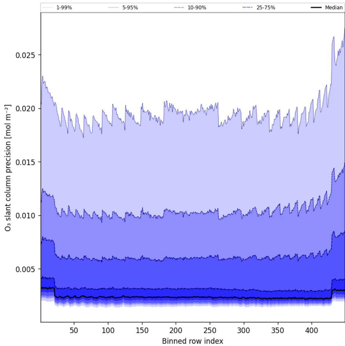
Figure 44: Along track statistics of “O 3 slant column precision” for 2025-08-15 to 2025-08-16
