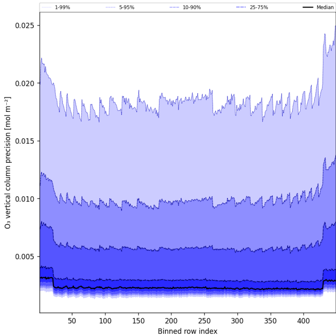
Figure 42: Along track statistics of “O 3 vertical column precision” for 2025-08-16 to 2025-08-17
