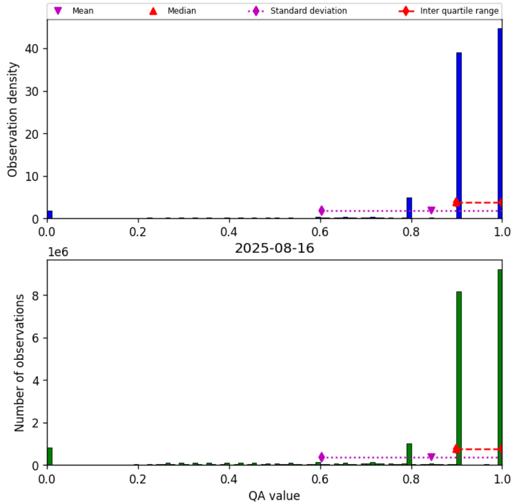
Figure 28: Histogram of “QA value” for 2025-08-16 to 2025-08-17
