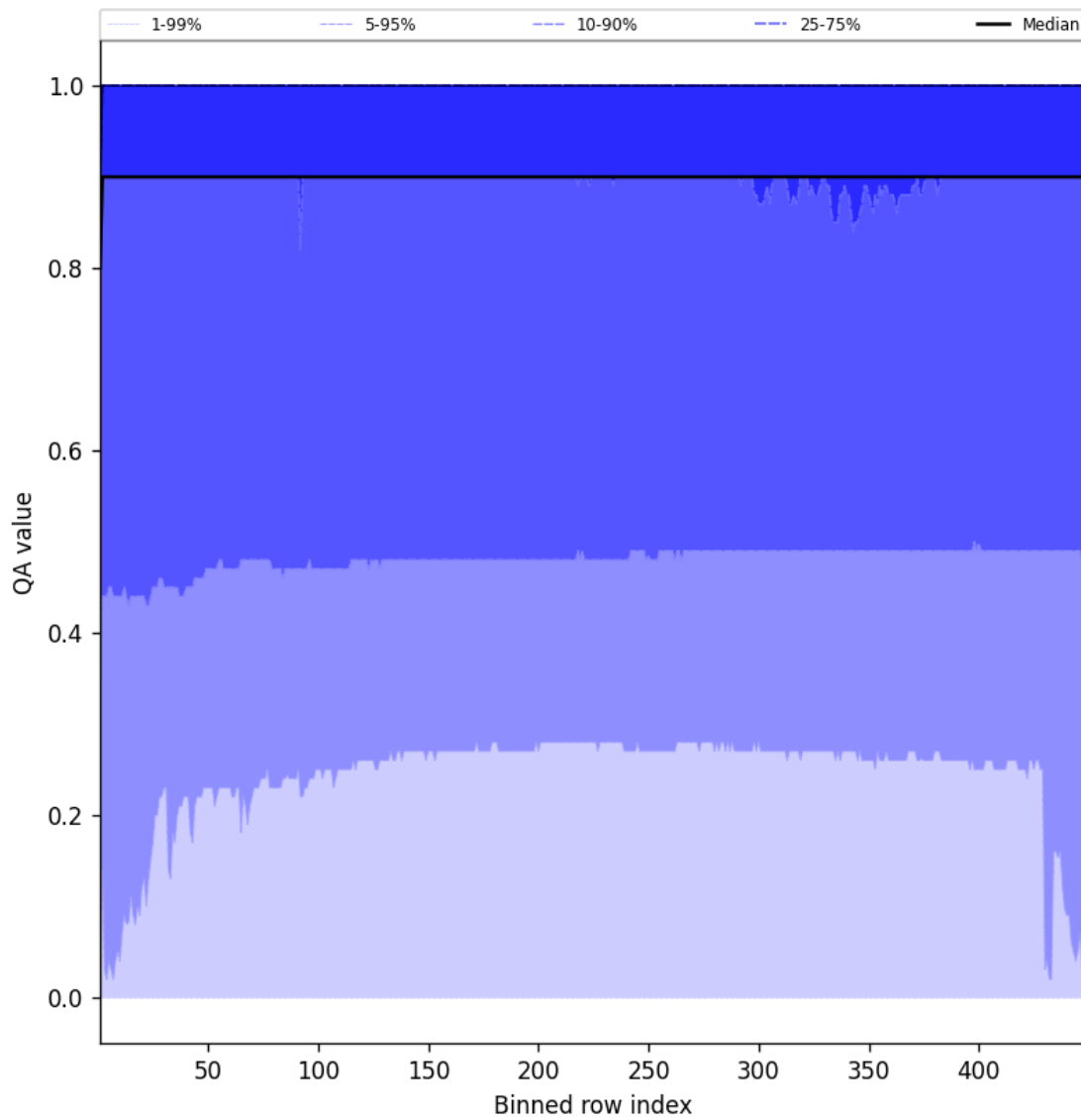
Figure 40: Along track statistics of “QA value” for 2025-08-16 to 2025-08-17
