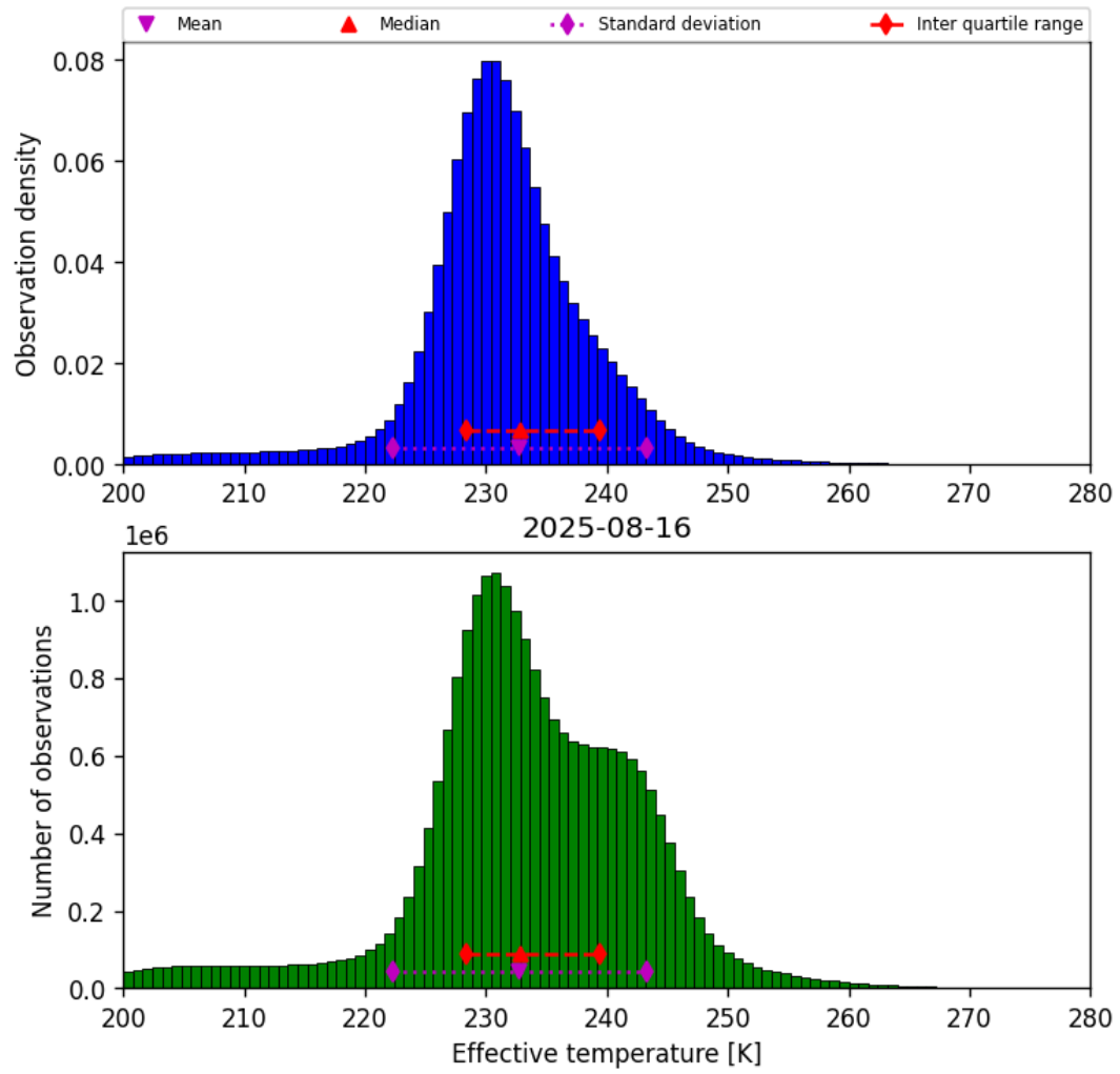
Figure 38: Histogram of “Effective temperature” for 2025-08-16 to 2025-08-17
