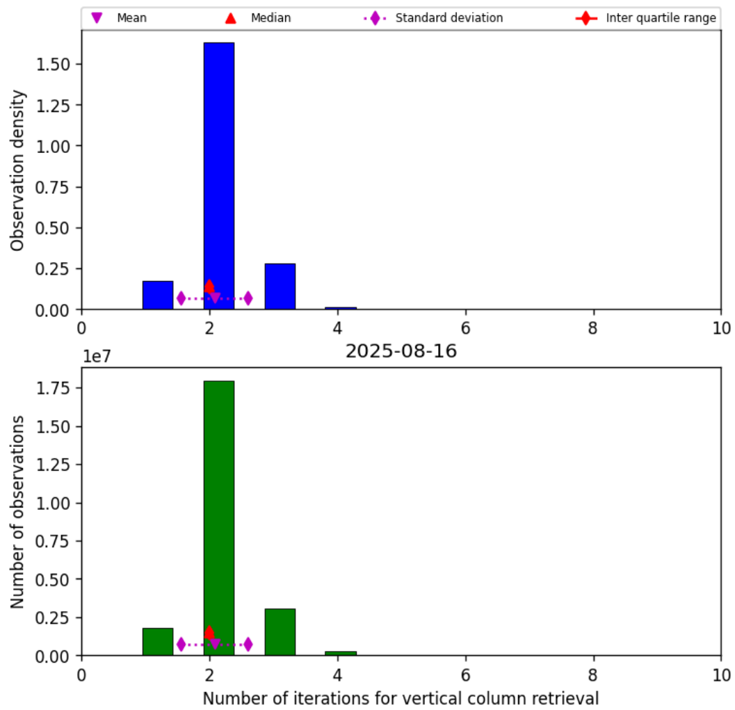
Figure 39: Histogram of “Number of iterations for vertical column retrieval” for 2025-08-16 to 2025-08-17
