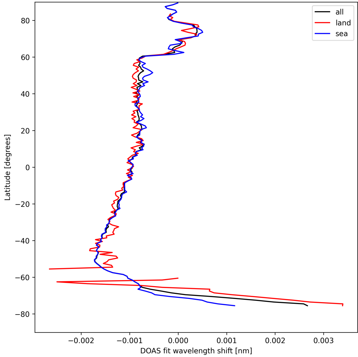
Figure 23: Zonal average of “DOAS fit wavelength shift” for 2025-08-16 to 2025-08-17.
