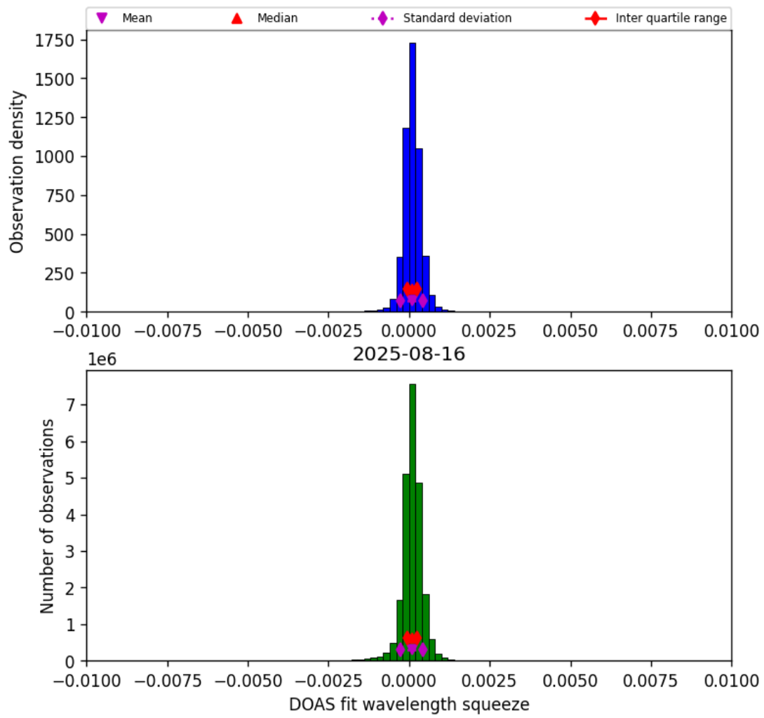
Figure 36: Histogram of “DOAS fit wavelength squeeze” for 2025-08-16 to 2025-08-17
