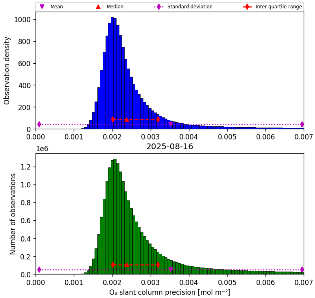
Figure 32: Histogram of “O 3 slant column precision” for 2025-08-16 to 2025-08-17
