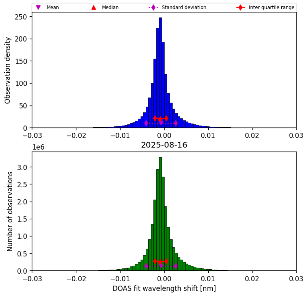
Figure 35: Histogram of “DOAS fit wavelength shift” for 2025-08-16 to 2025-08-17
