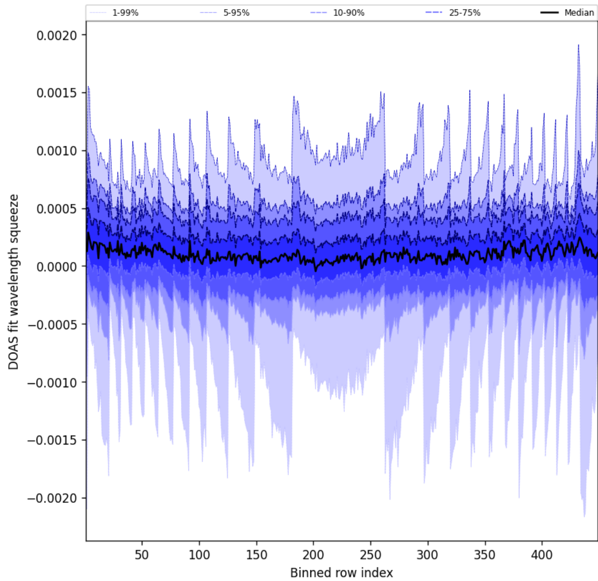
Figure 48: Along track statistics of “DOAS fit wavelength squeeze” for 2025-08-16 to 2025-08-17
