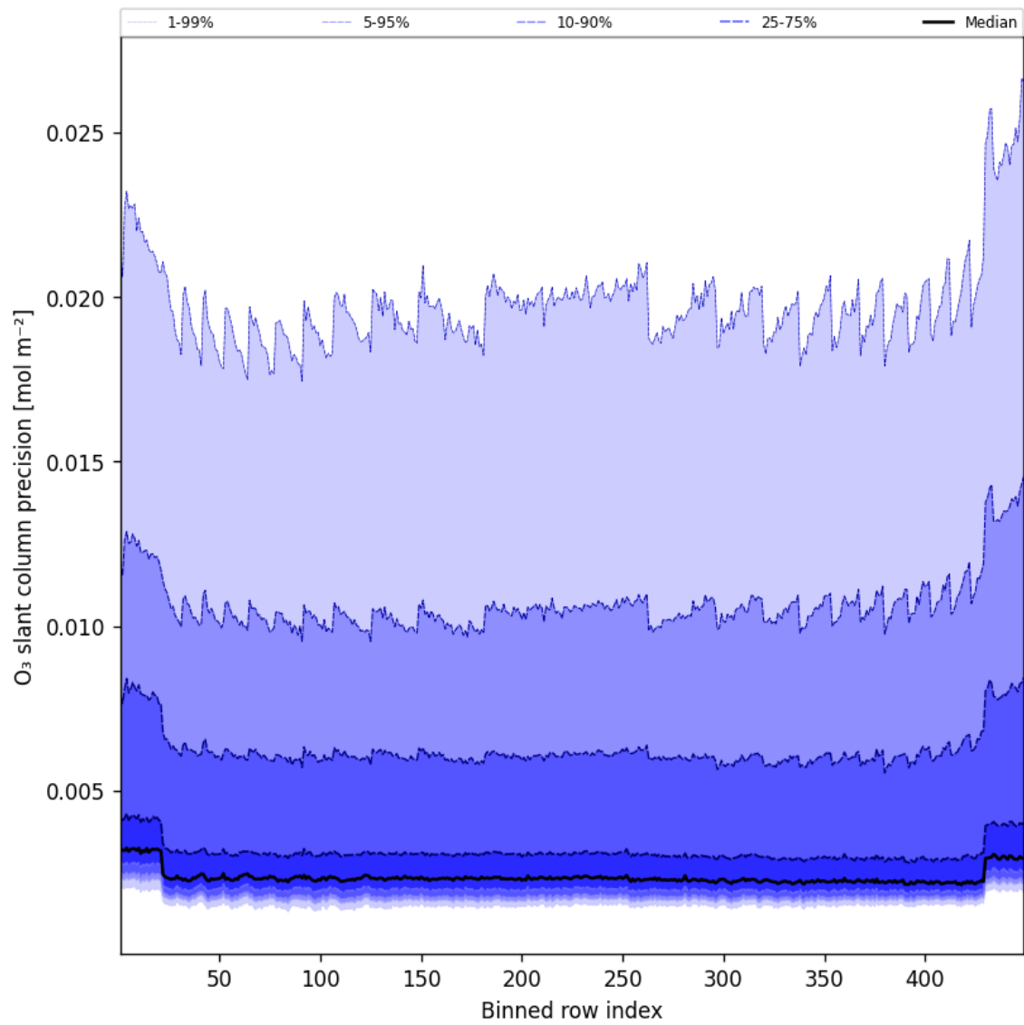
Figure 44: Along track statistics of “O 3 slant column precision” for 2025-08-16 to 2025-08-17
