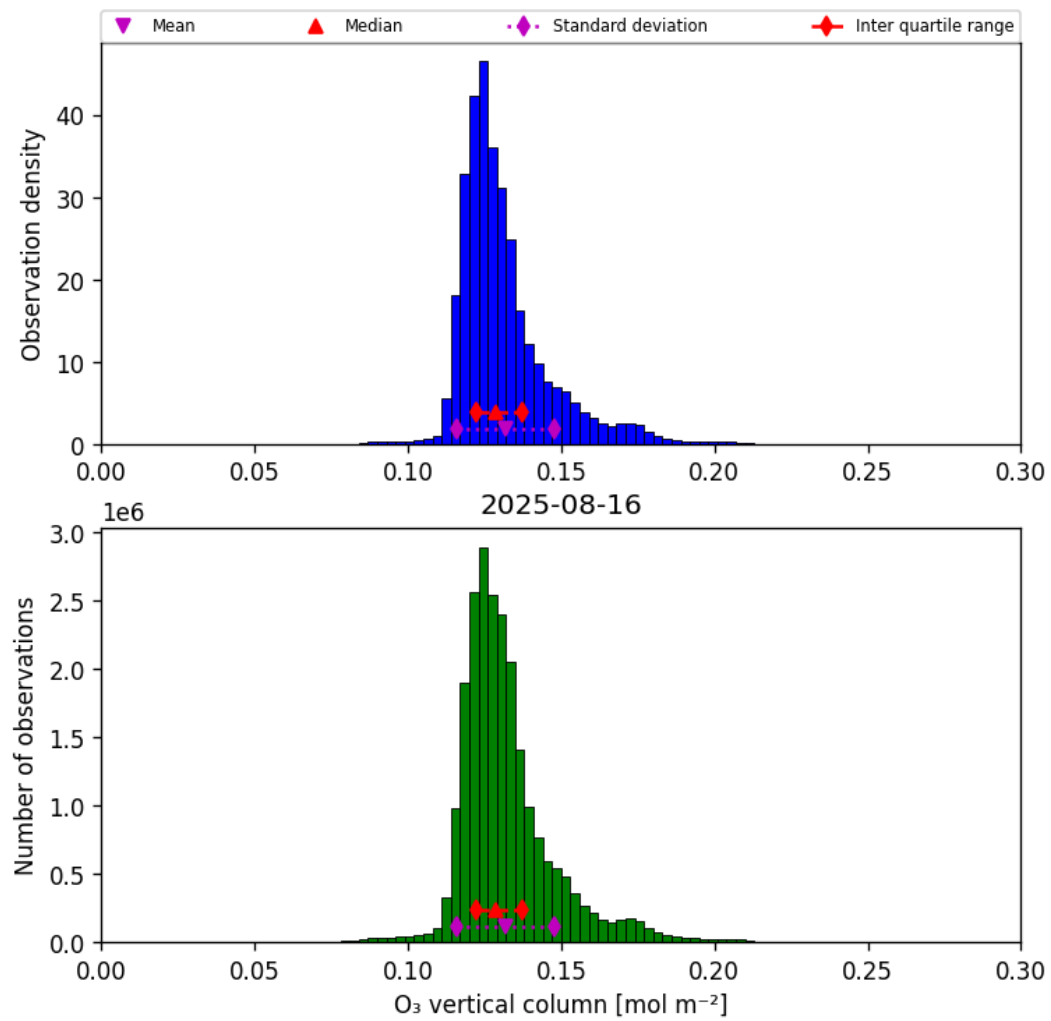
Figure 29: Histogram of “O 3 vertical column” for 2025-08-16 to 2025-08-17
