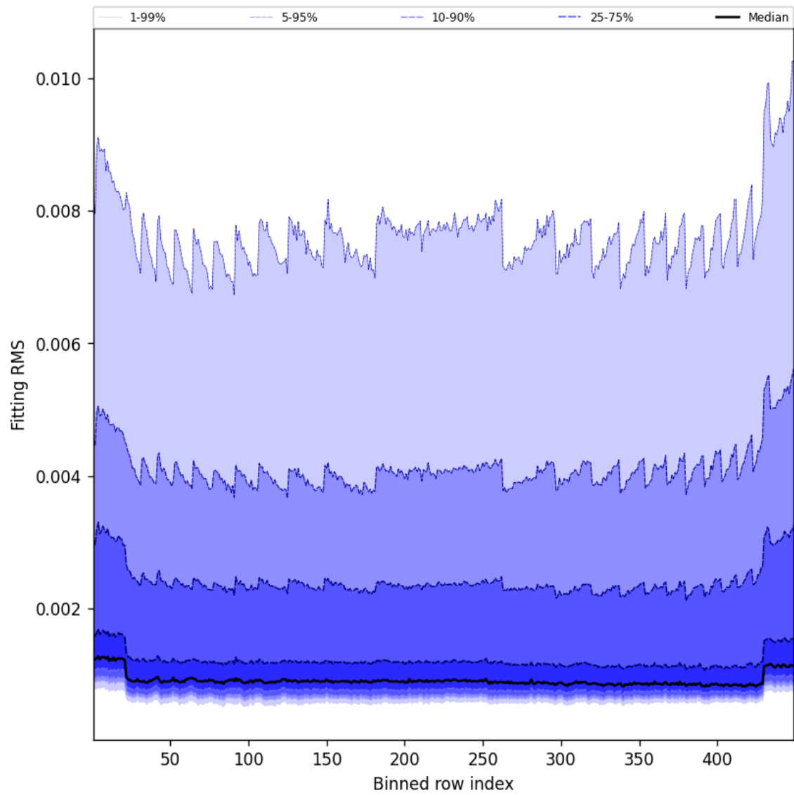
Figure 46: Along track statistics of “Fitting RMS” for 2025-08-16 to 2025-08-17
