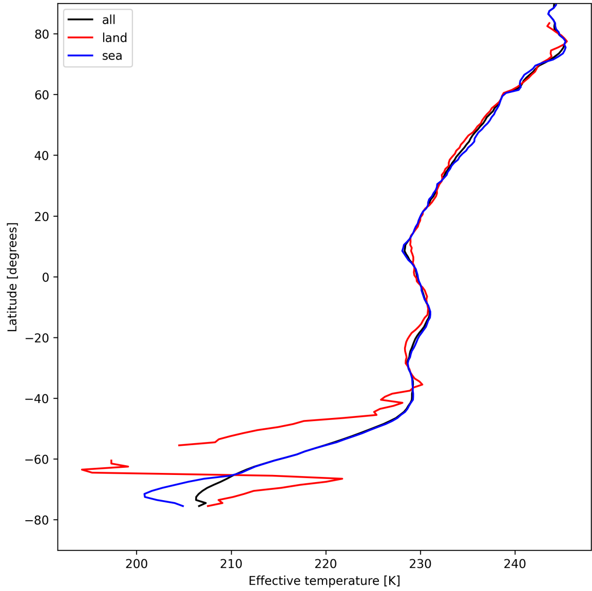
Figure 26: Zonal average of “Effective temperature” for 2025-08-16 to 2025-08-17.
