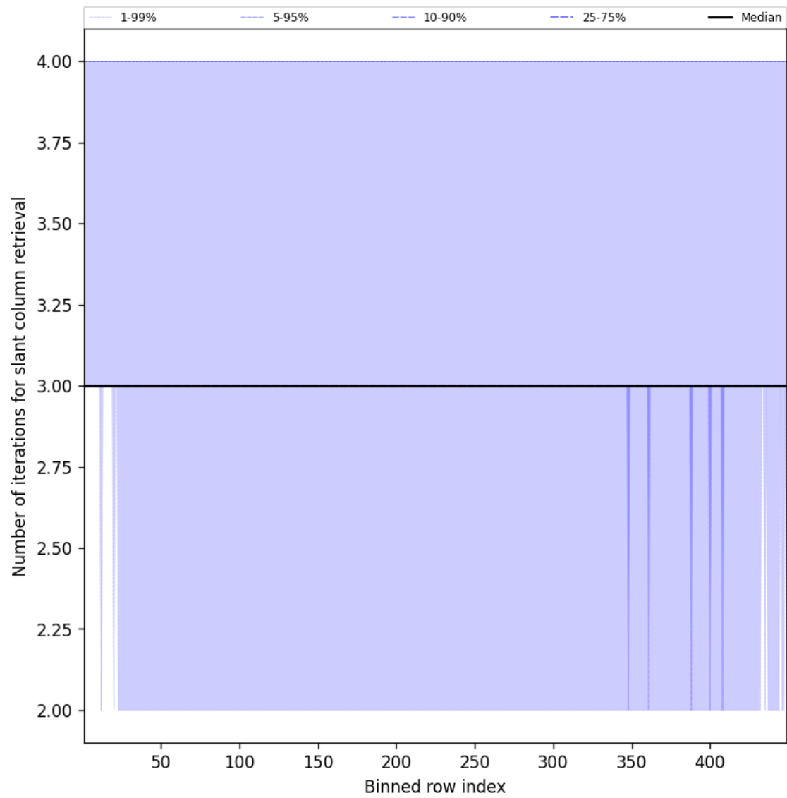
Figure 45: Along track statistics of “Number of iterations for slant column retrieval” for 2025-08-16 to 2025-08-17
