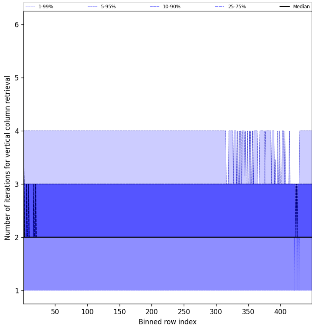
Figure 51: Along track statistics of “Number of iterations for vertical column retrieval” for 2025-08-16 to 2025-08-17
