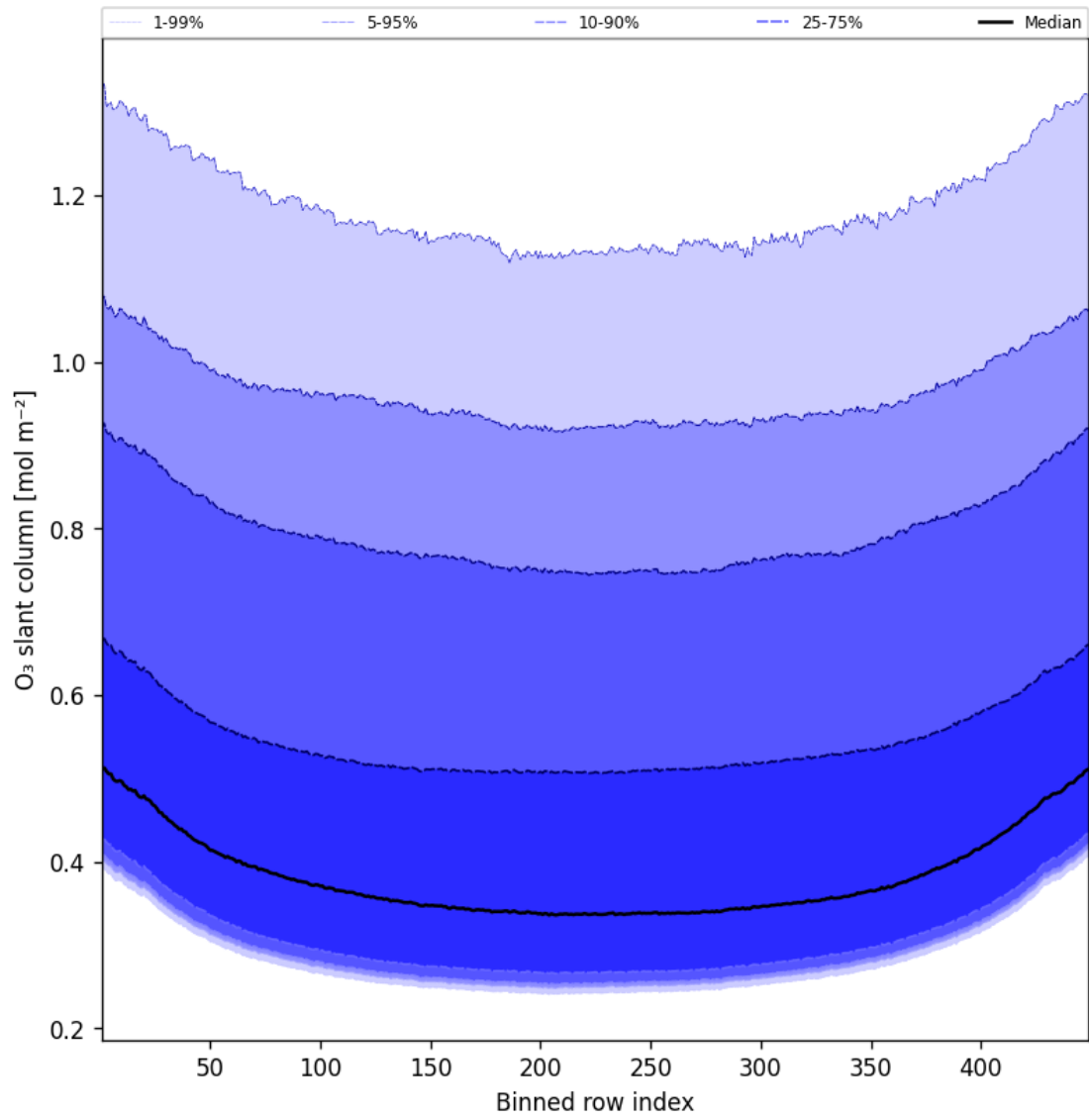
Figure 43: Along track statistics of “O 3 slant column” for 2025-08-16 to 2025-08-17
