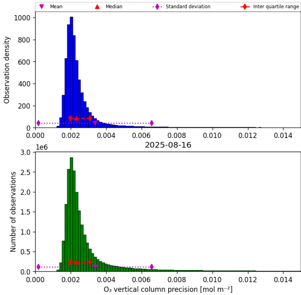
Figure 30: Histogram of “O 3 vertical column precision” for 2025-08-16 to 2025-08-17
