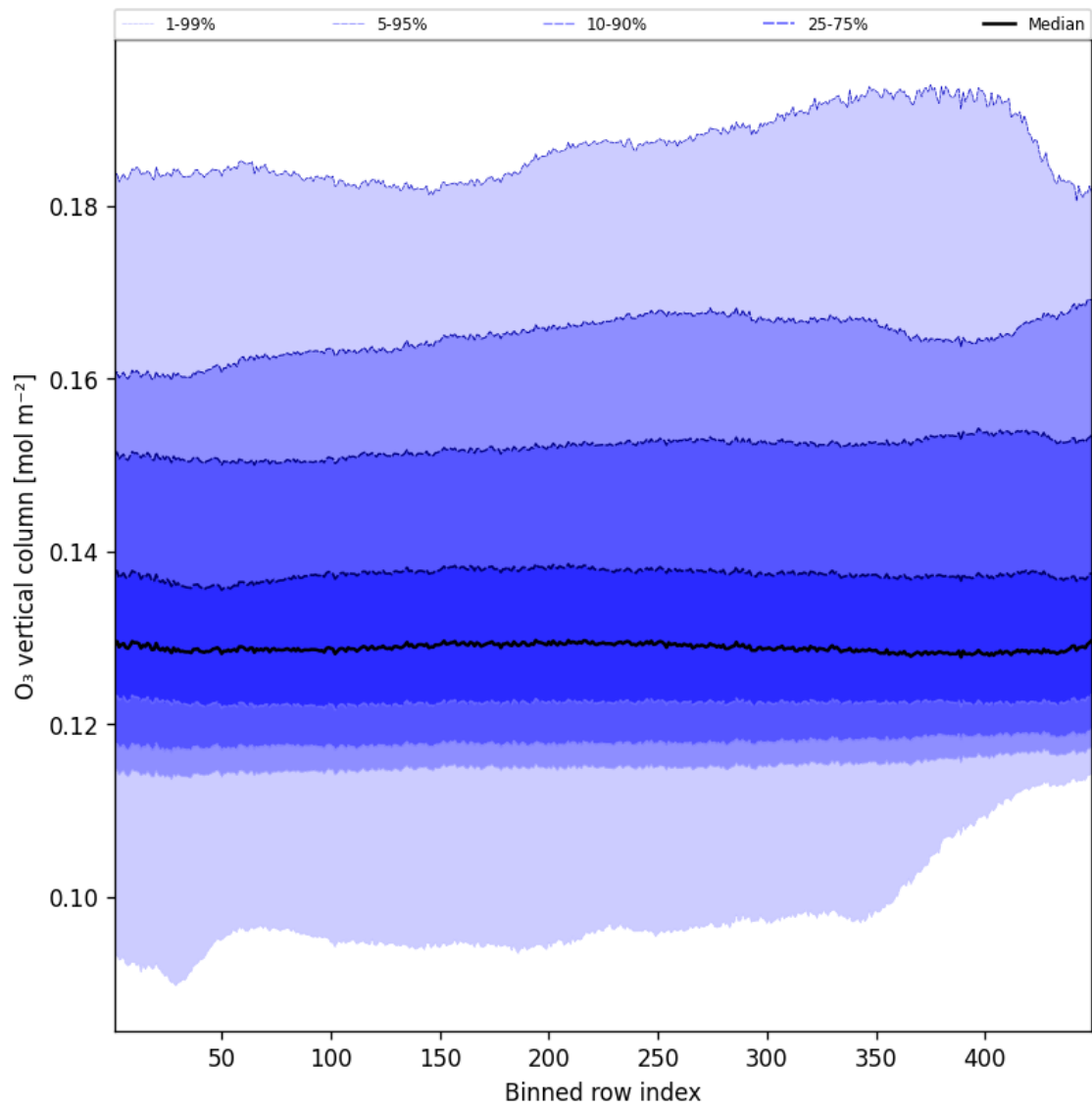
Figure 41: Along track statistics of “O 3 vertical column” for 2025-08-16 to 2025-08-17
