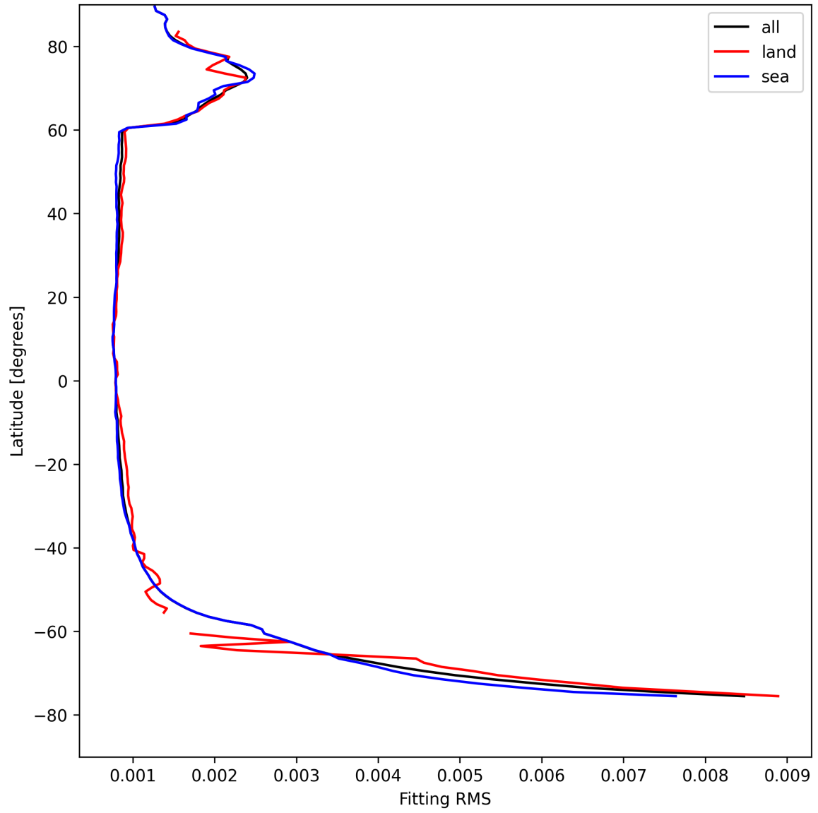
Figure 22: Zonal average of “Fitting RMS” for 2025-08-16 to 2025-08-17.
