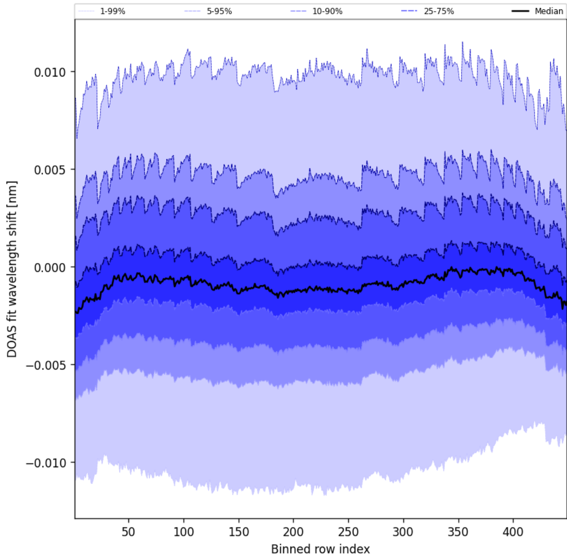
Figure 47: Along track statistics of “DOAS fit wavelength shift” for 2025-08-16 to 2025-08-17
