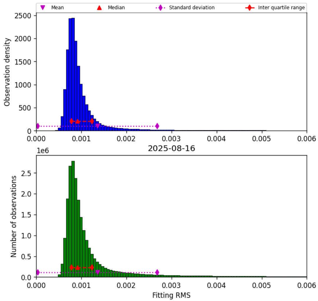
Figure 34: Histogram of “Fitting RMS” for 2025-08-16 to 2025-08-17
