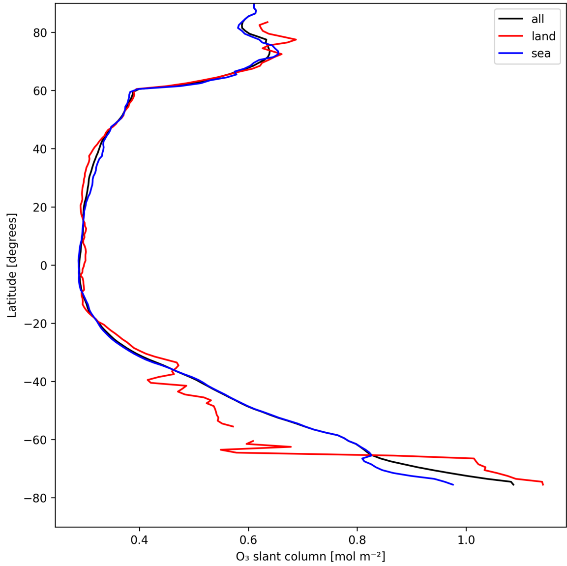
Figure 19: Zonal average of “O 3 slant column” for 2025-08-16 to 2025-08-17.
