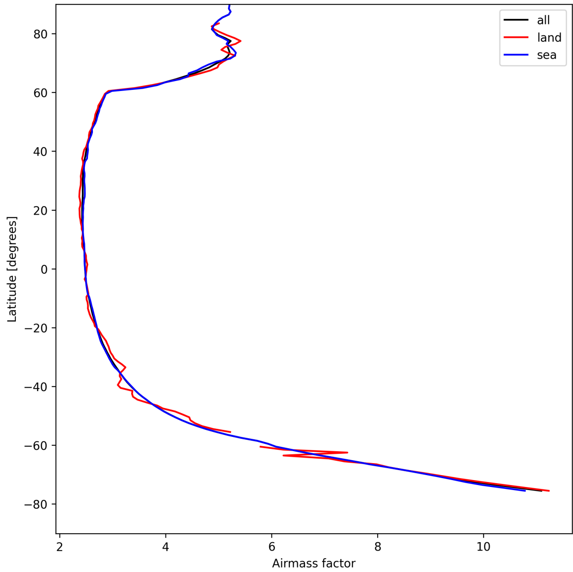
Figure 25: Zonal average of “Airmass factor” for 2025-08-16 to 2025-08-17.
