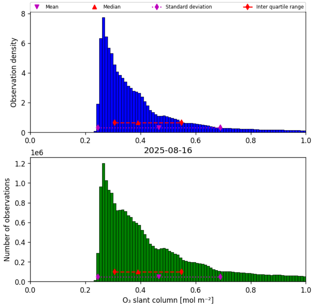
Figure 31: Histogram of “O 3 slant column” for 2025-08-16 to 2025-08-17
