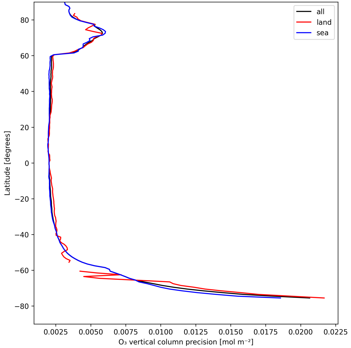
Figure 18: Zonal average of “O 3 vertical column precision” for 2025-08-16 to 2025-08-17.
