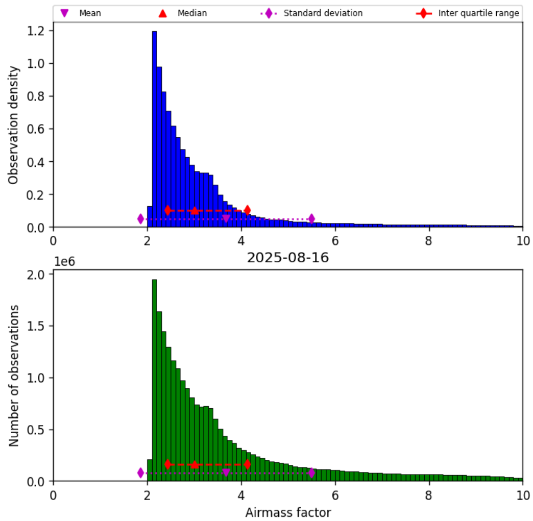
Figure 37: Histogram of “Airmass factor” for 2025-08-16 to 2025-08-17
