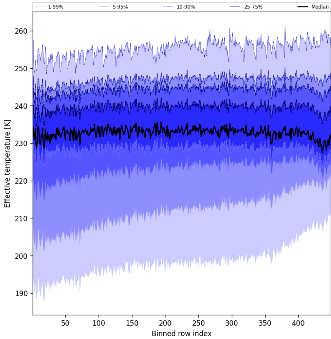
Figure 50: Along track statistics of “Effective temperature” for 2025-08-16 to 2025-08-17
