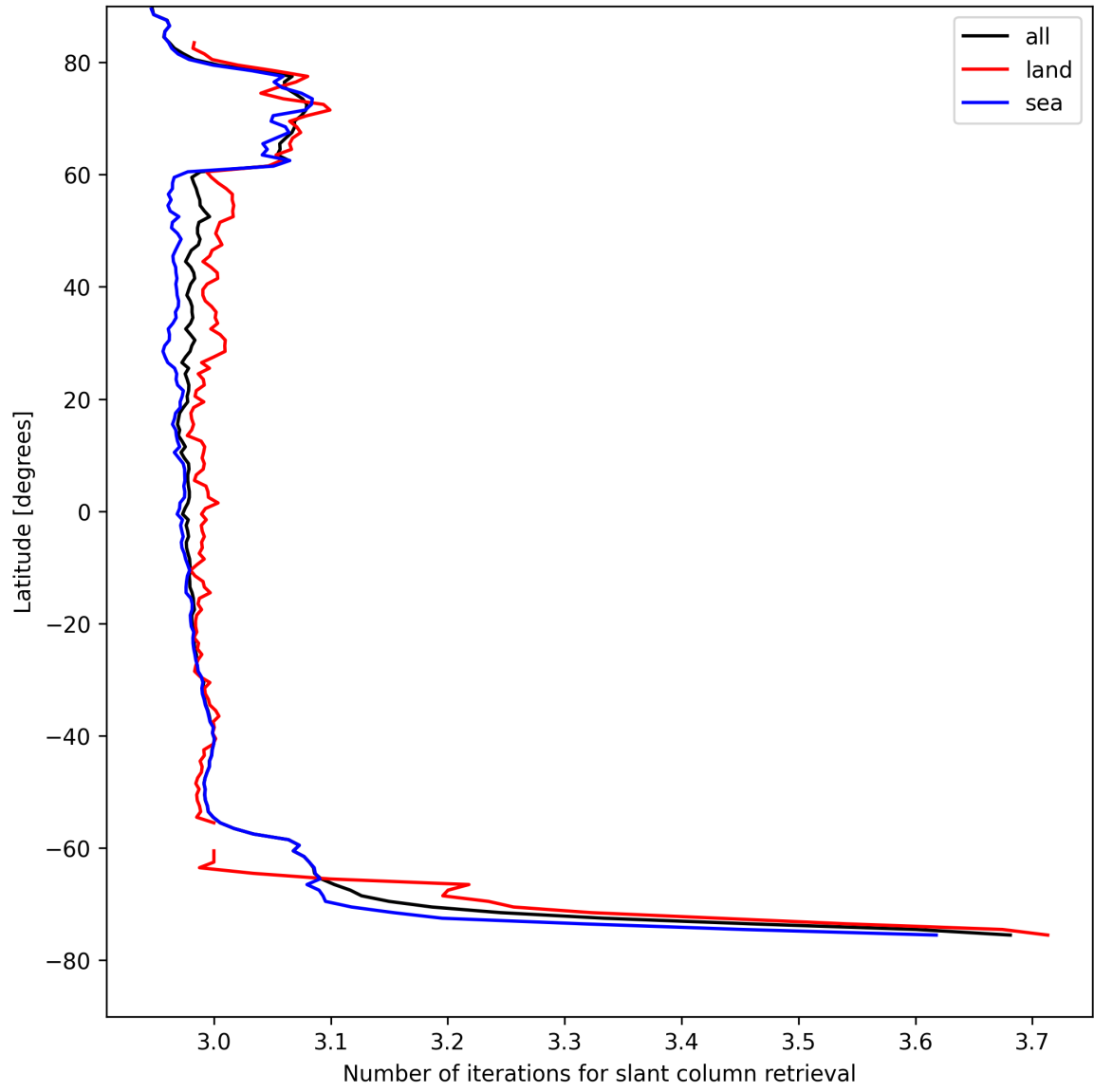
Figure 21: Zonal average of “Number of iterations for slant column retrieval” for 2025-08-16 to 2025-08-17.
