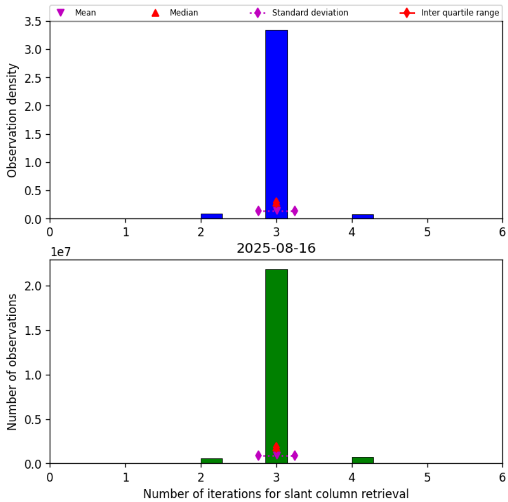
Figure 33: Histogram of “Number of iterations for slant column retrieval” for 2025-08-16 to 2025-08-17
