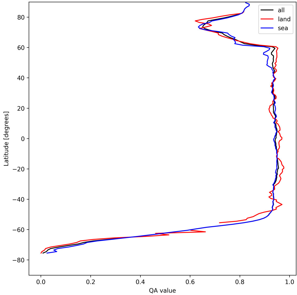
Figure 16: Zonal average of “QA value” for 2025-08-16 to 2025-08-17.
