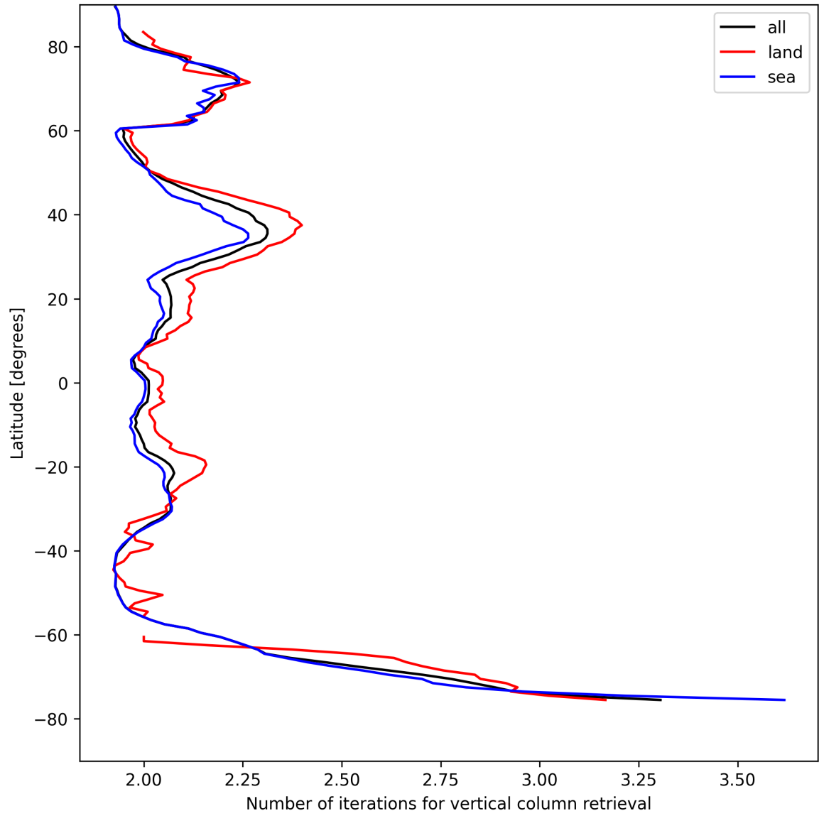
Figure 27: Zonal average of “Number of iterations for vertical column retrieval” for 2025-08-16 to 2025-08-17.
