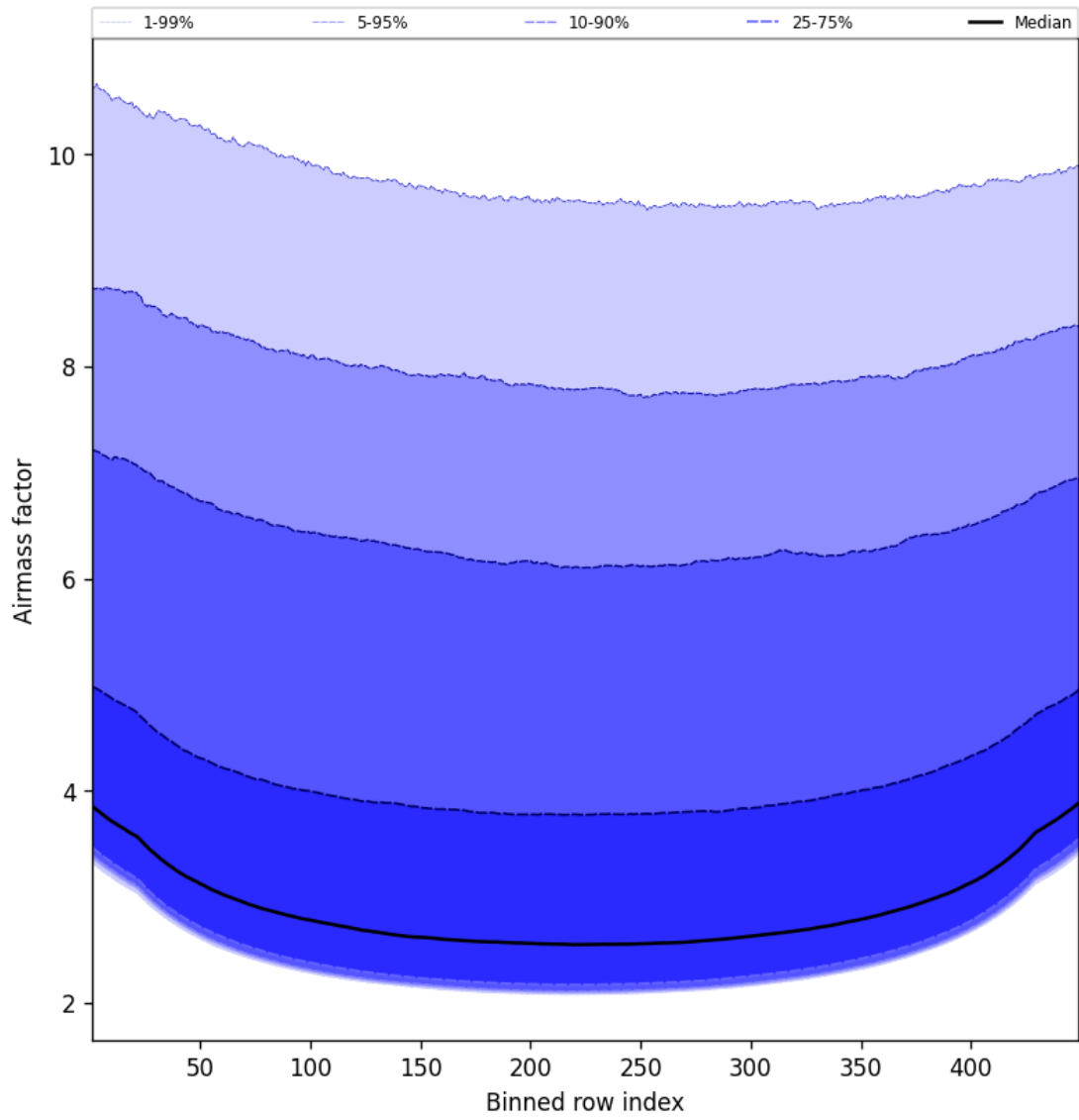
Figure 49: Along track statistics of “Airmass factor” for 2025-08-16 to 2025-08-17
