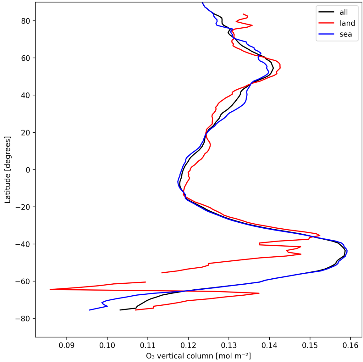
Figure 17: Zonal average of “O 3 vertical column” for 2025-08-16 to 2025-08-17.
