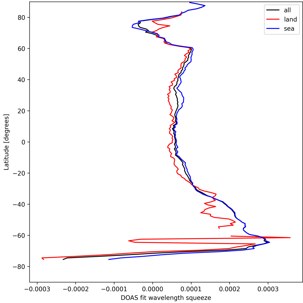
Figure 24: Zonal average of “DOAS fit wavelength squeeze” for 2025-08-16 to 2025-08-17.
