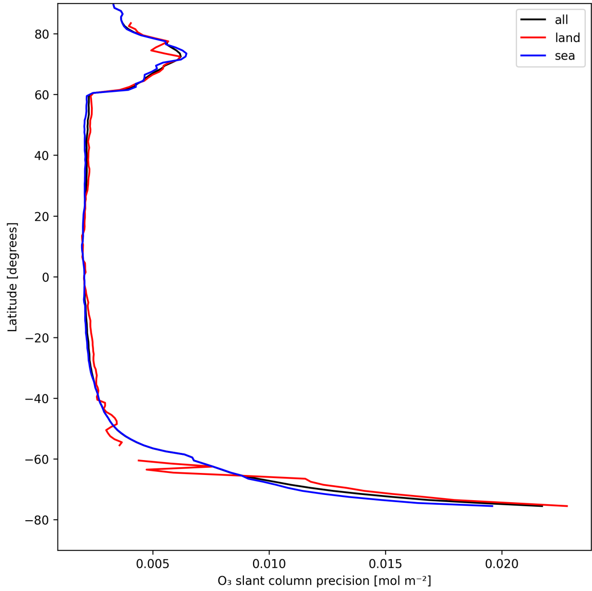
Figure 20: Zonal average of “O 3 slant column precision” for 2025-08-16 to 2025-08-17.
