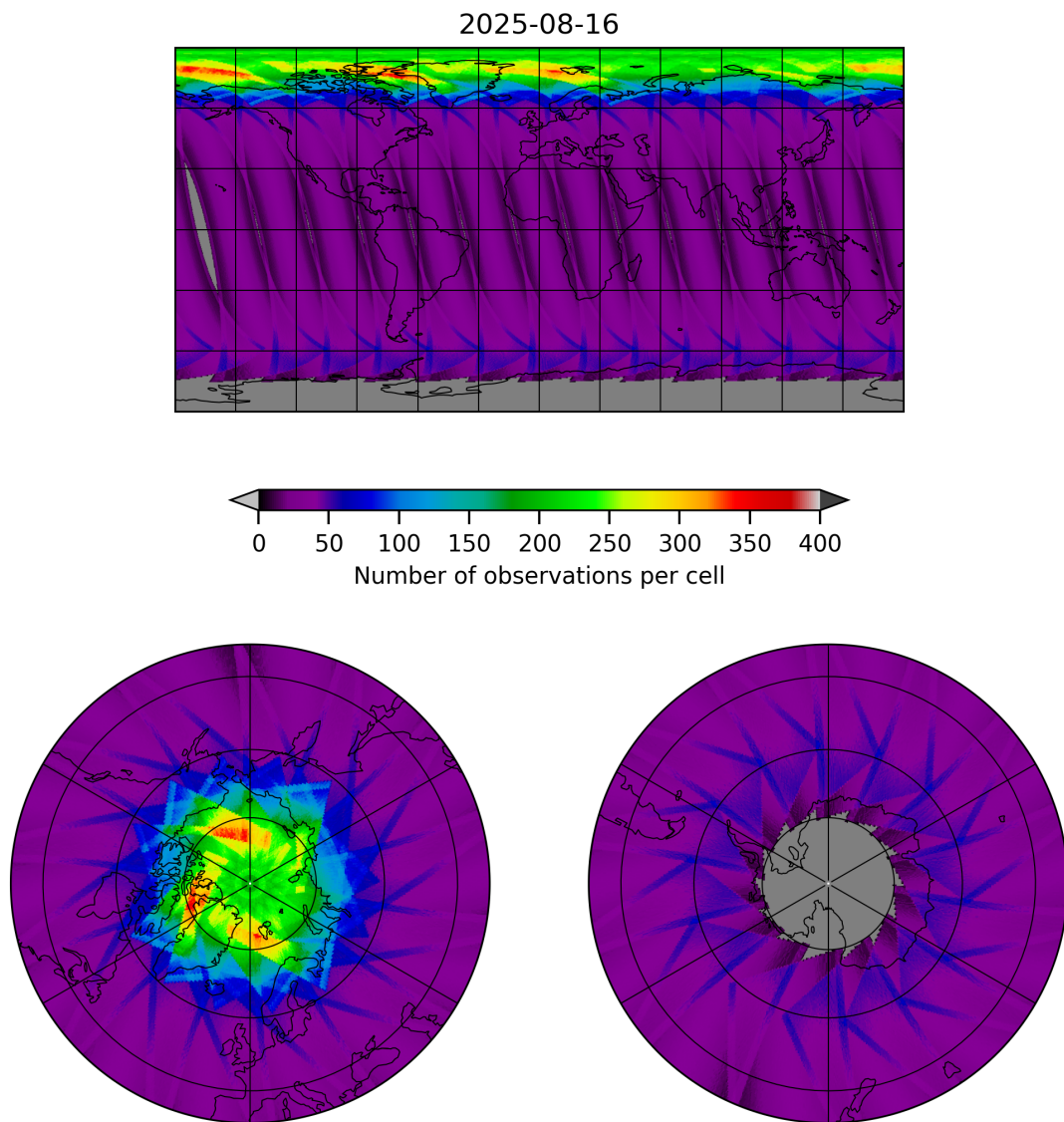
Figure 15: Map of the number of observations for 2025-08-16 to 2025-08-17
