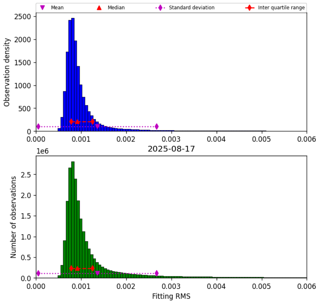
Figure 34: Histogram of “Fitting RMS” for 2025-08-17 to 2025-08-17
