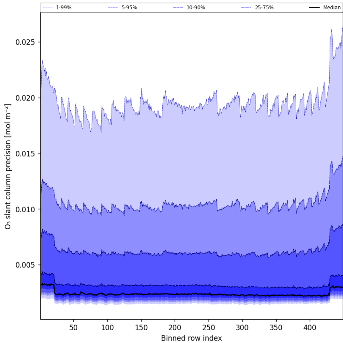
Figure 44: Along track statistics of “O 3 slant column precision” for 2025-08-17 to 2025-08-17
