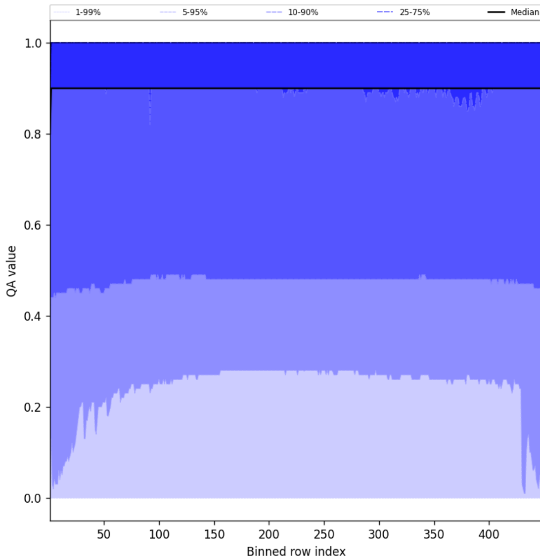
Figure 40: Along track statistics of “QA value” for 2025-08-17 to 2025-08-17
