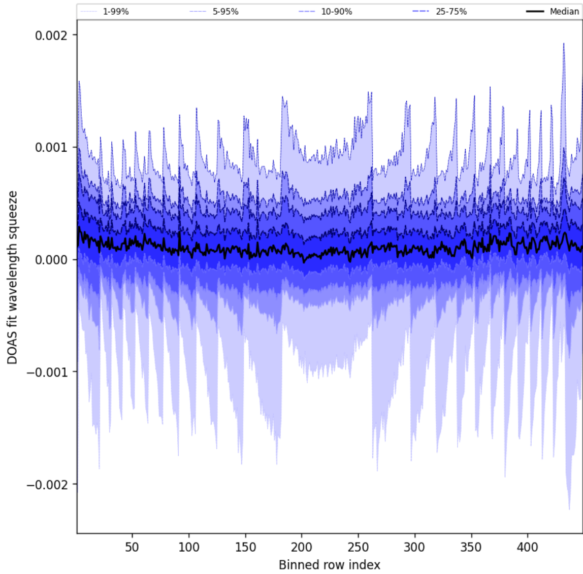
Figure 48: Along track statistics of “DOAS fit wavelength squeeze” for 2025-08-17 to 2025-08-17
