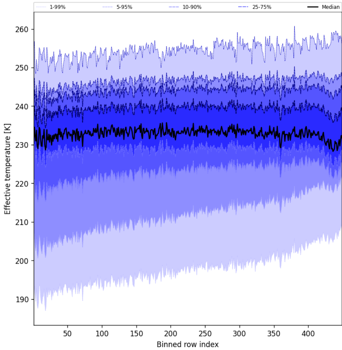
Figure 50: Along track statistics of “Effective temperature” for 2025-08-17 to 2025-08-17
