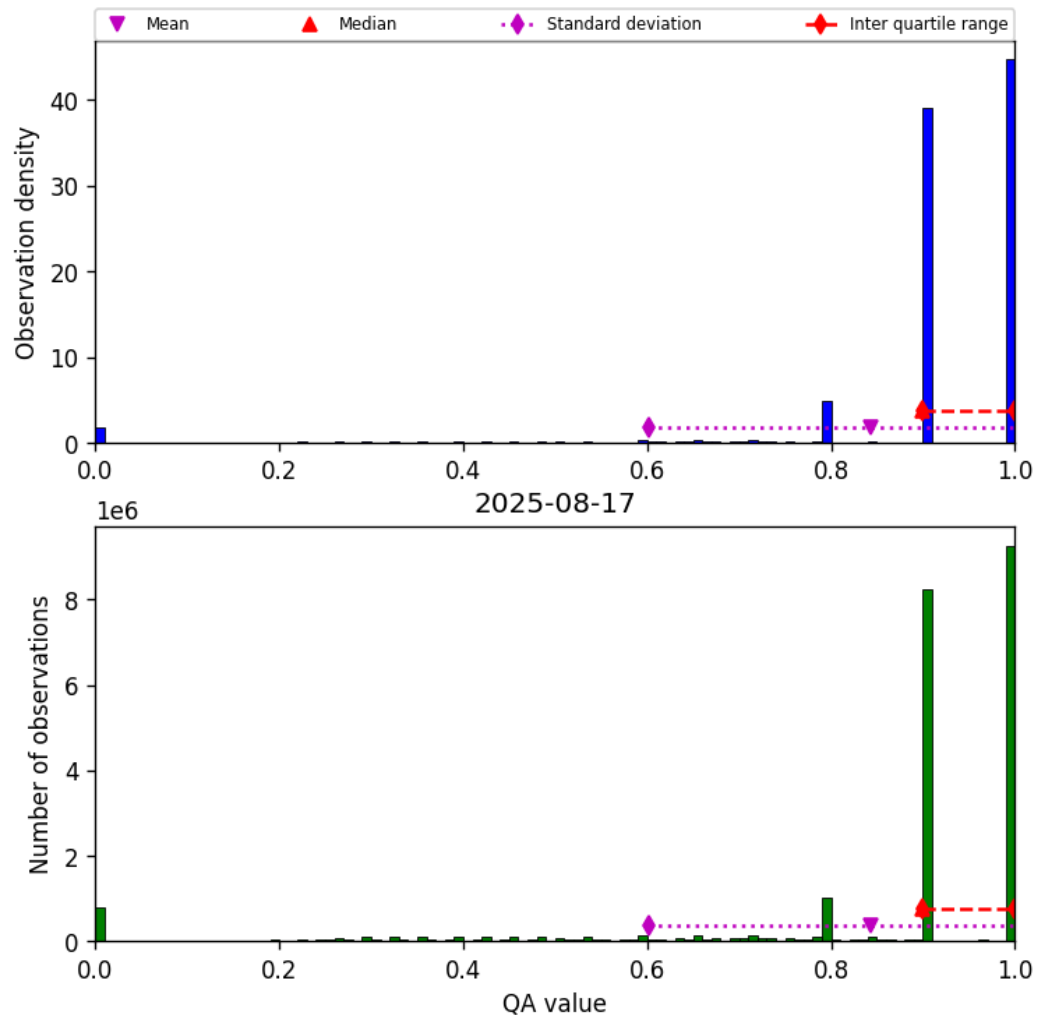
Figure 28: Histogram of “QA value” for 2025-08-17 to 2025-08-17
