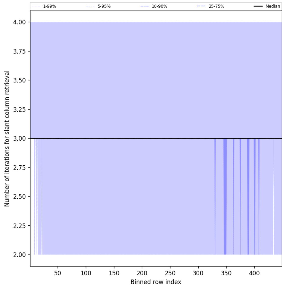
Figure 45: Along track statistics of “Number of iterations for slant column retrieval” for 2025-08-17 to 2025-08-17
