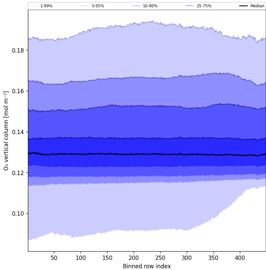
Figure 41: Along track statistics of “O 3 vertical column” for 2025-08-17 to 2025-08-17
