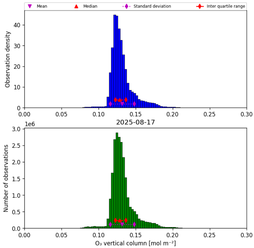
Figure 29: Histogram of “O 3 vertical column” for 2025-08-17 to 2025-08-17
