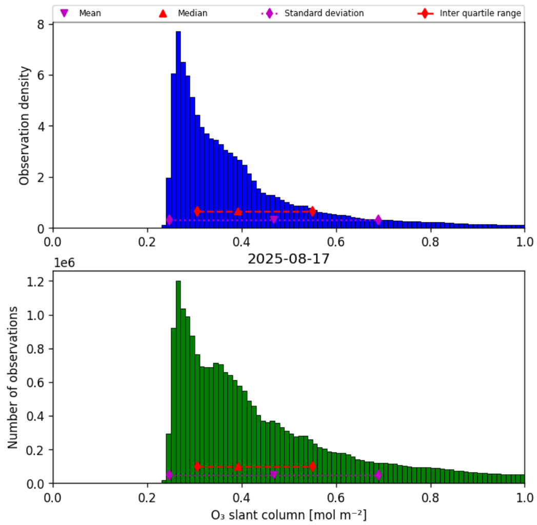
Figure 31: Histogram of “O 3 slant column” for 2025-08-17 to 2025-08-17
