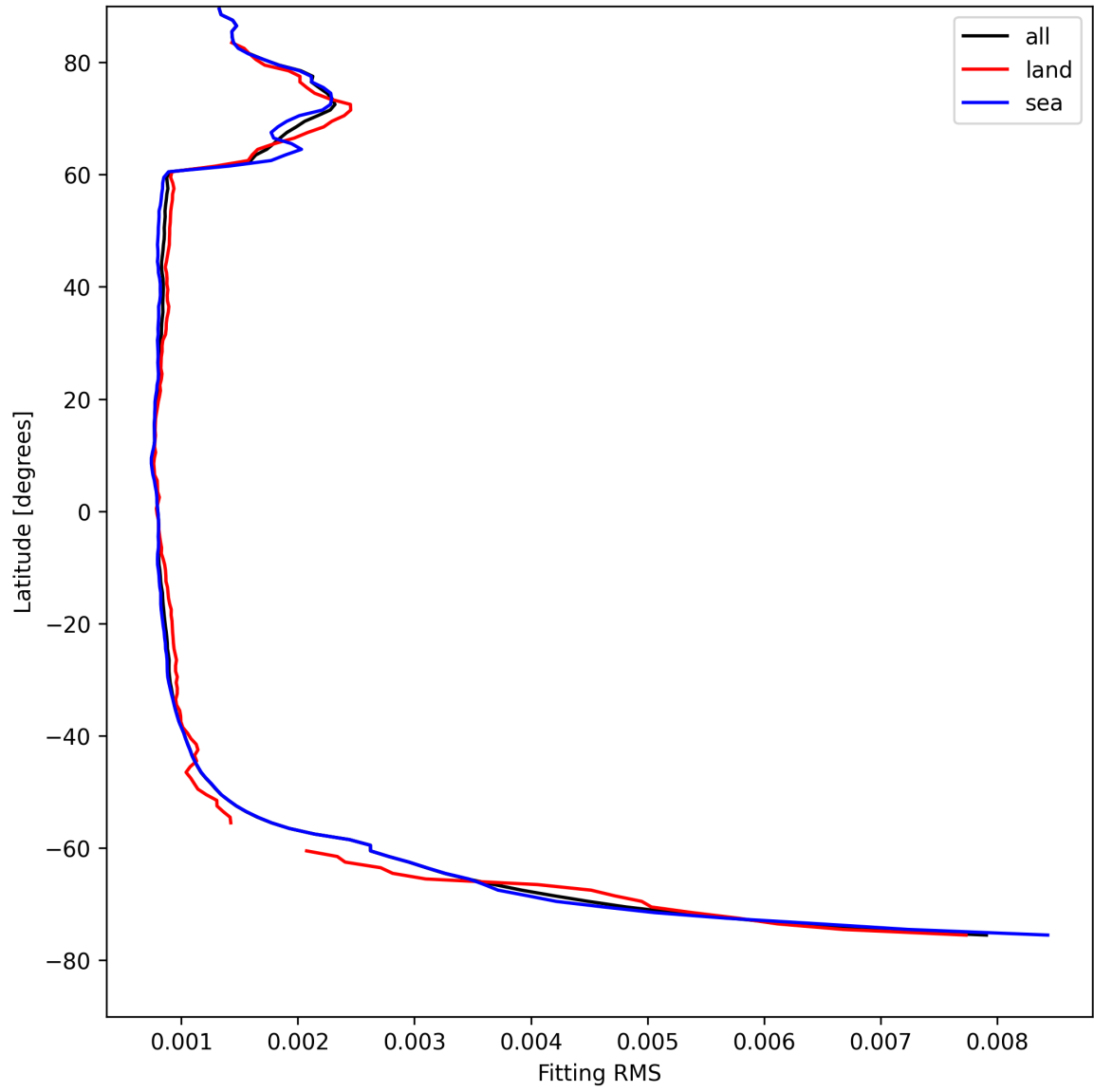
Figure 22: Zonal average of “Fitting RMS” for 2025-08-17 to 2025-08-17.
