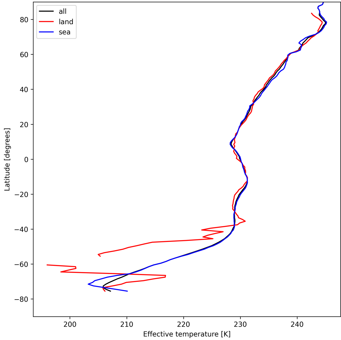
Figure 26: Zonal average of "Effective temperature" for 2025-08-17 to 2025-08-17.
