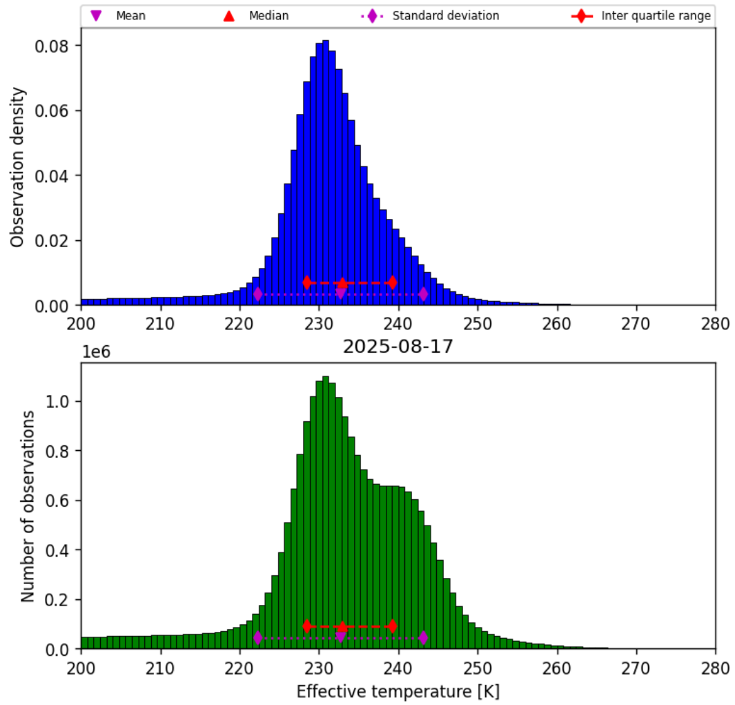
Figure 38: Histogram of “Effective temperature” for 2025-08-17 to 2025-08-17
