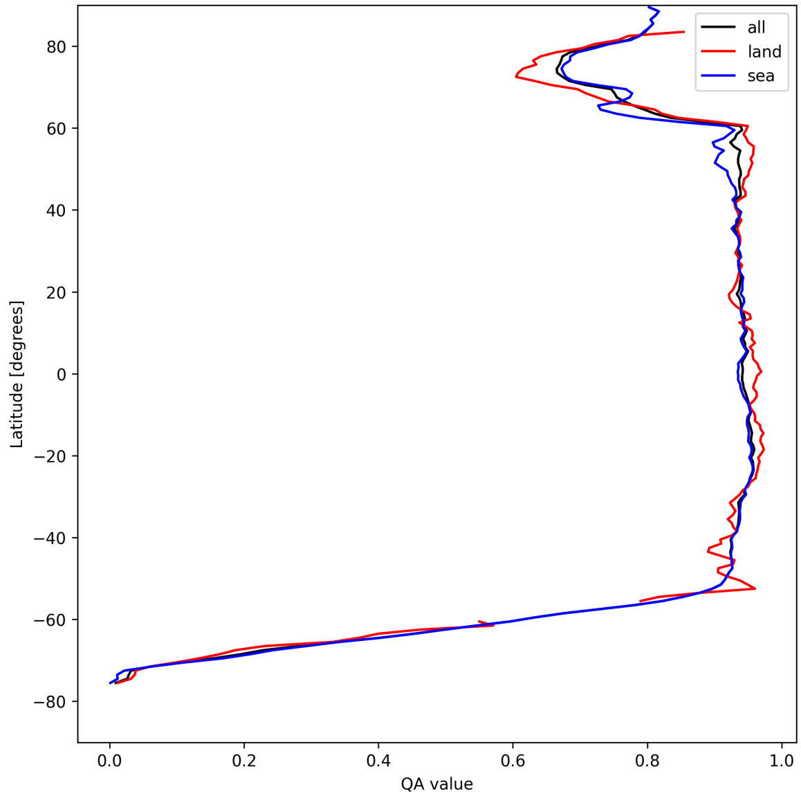
Figure 16: Zonal average of “QA value” for 2025-08-17 to 2025-08-17.
