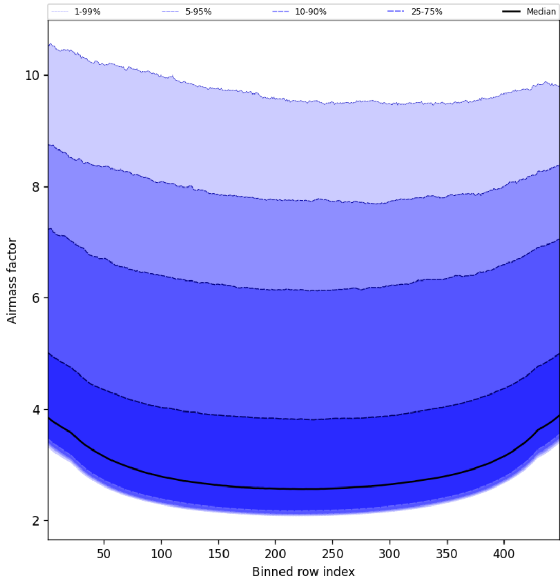
Figure 49: Along track statistics of “Airmass factor” for 2025-08-17 to 2025-08-17
