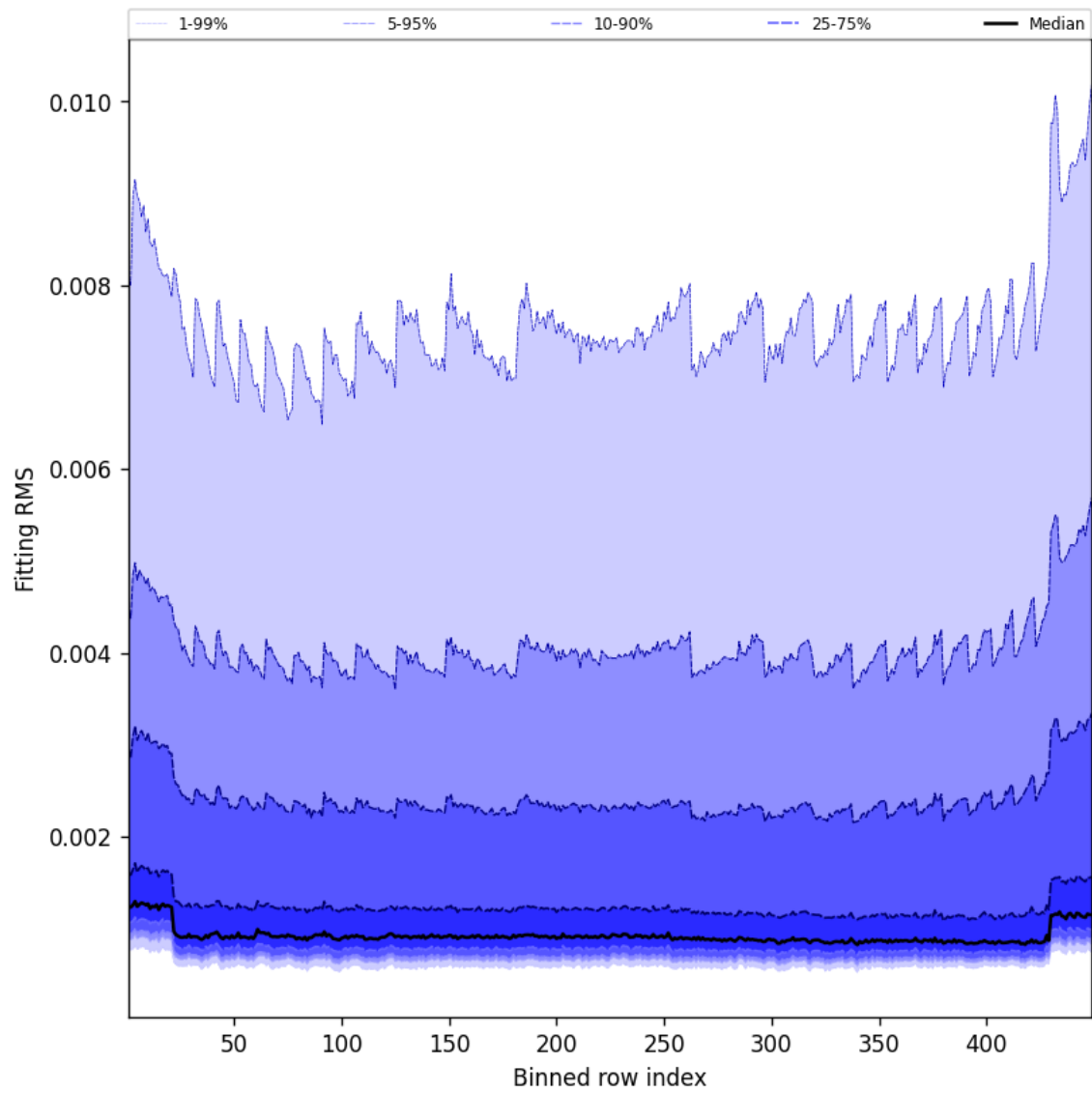
Figure 46: Along track statistics of “Fitting RMS” for 2025-08-17 to 2025-08-17
