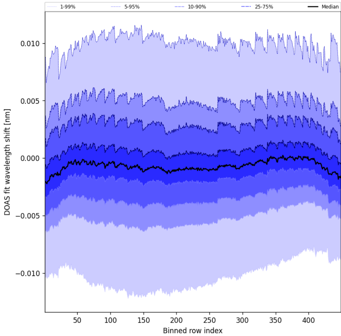
Figure 47: Along track statistics of “DOAS fit wavelength shift” for 2025-08-17 to 2025-08-17
