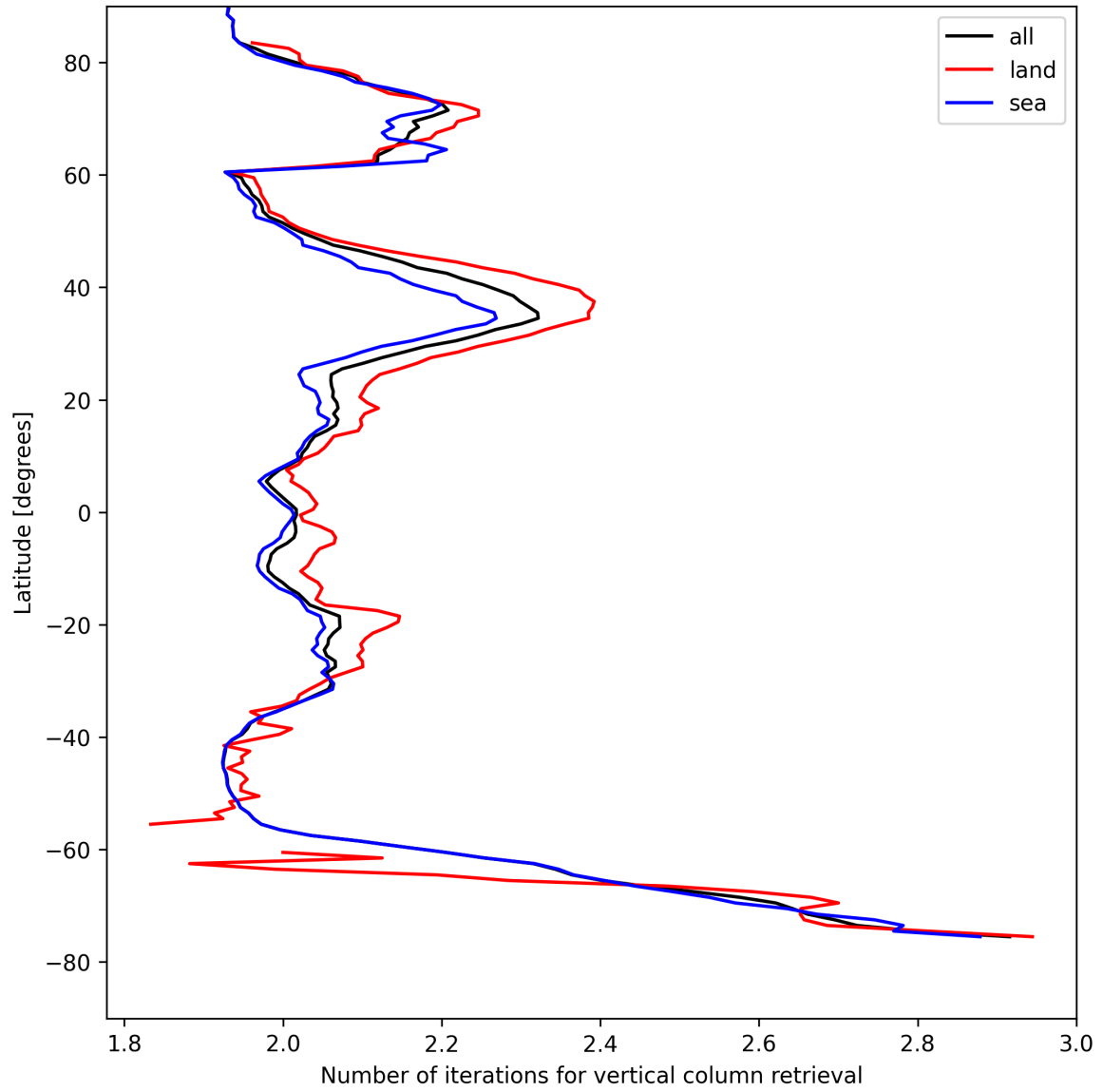
Figure 27: Zonal average of “Number of iterations for vertical column retrieval” for 2025-08-17 to 2025-08-17.
