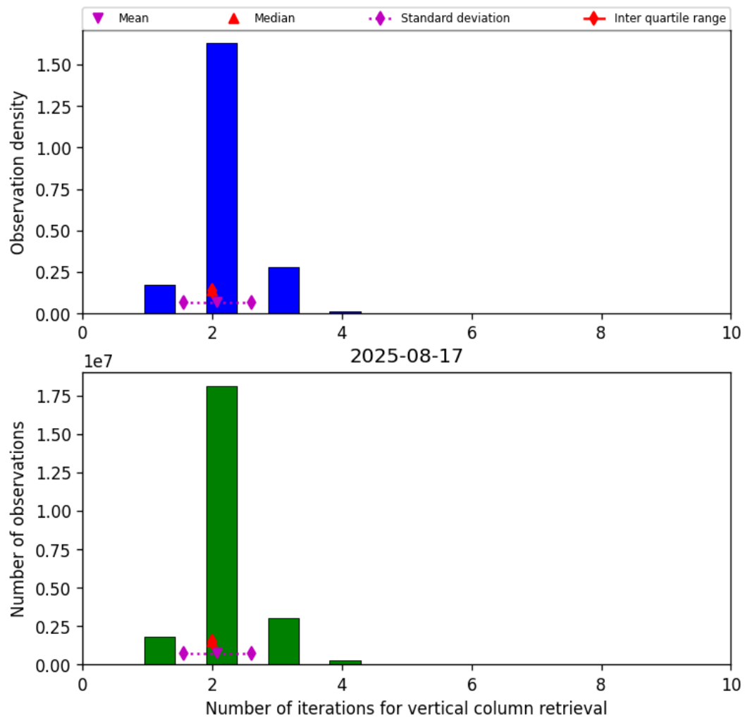
Figure 39: Histogram of “Number of iterations for vertical column retrieval” for 2025-08-17 to 2025-08-17
