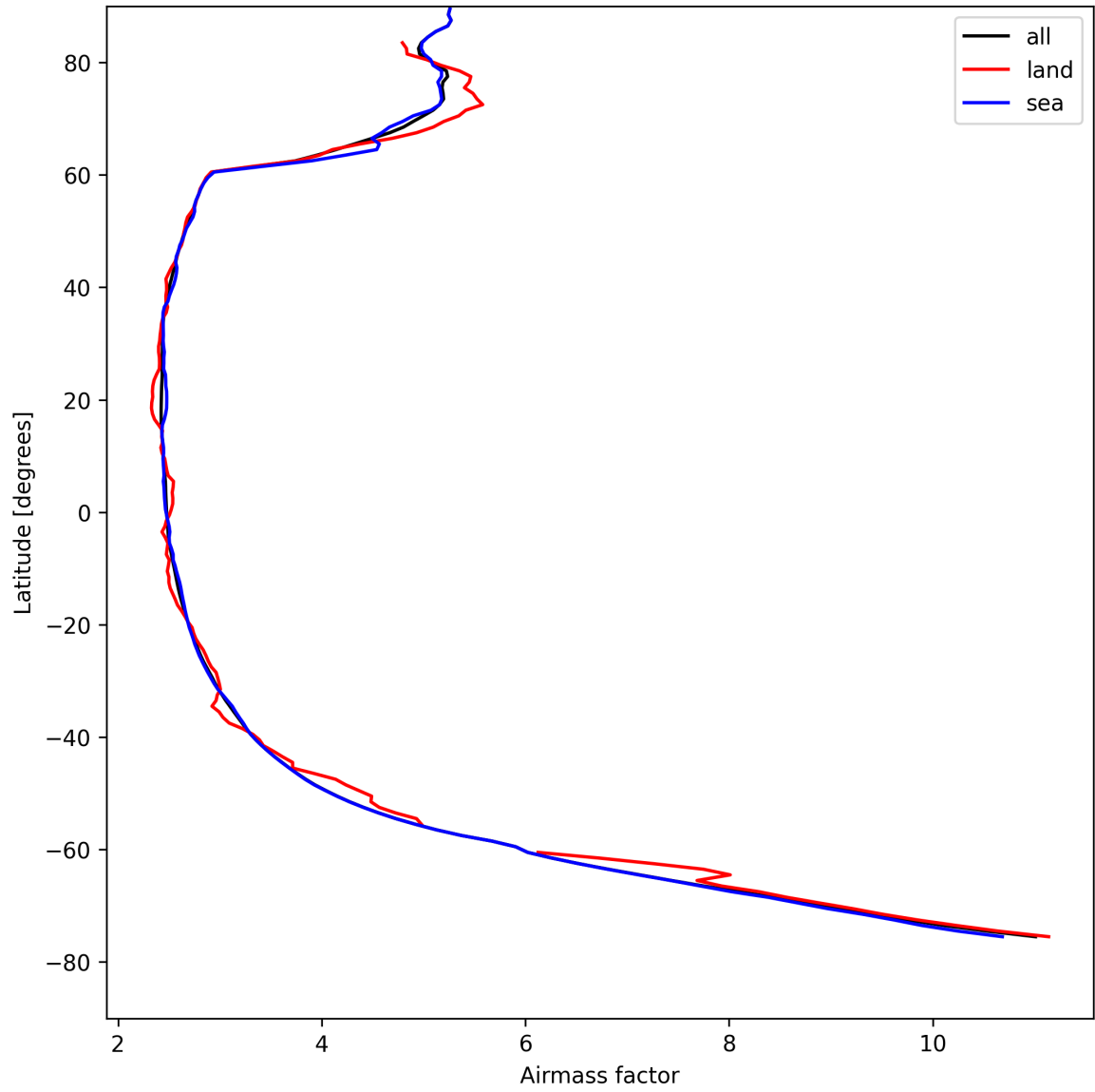
Figure 25: Zonal average of “Airmass factor” for 2025-08-17 to 2025-08-17.
