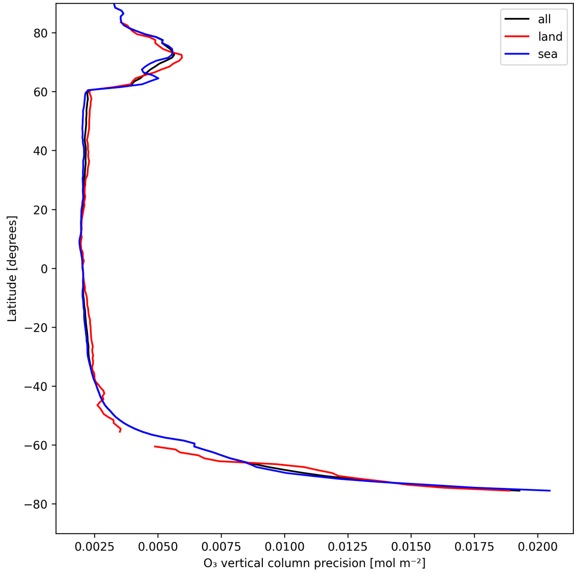
Figure 18: Zonal average of “O 3 vertical column precision” for 2025-08-17 to 2025-08-17.
