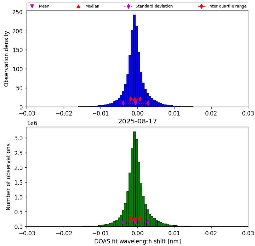
Figure 35: Histogram of “DOAS fit wavelength shift” for 2025-08-17 to 2025-08-17
