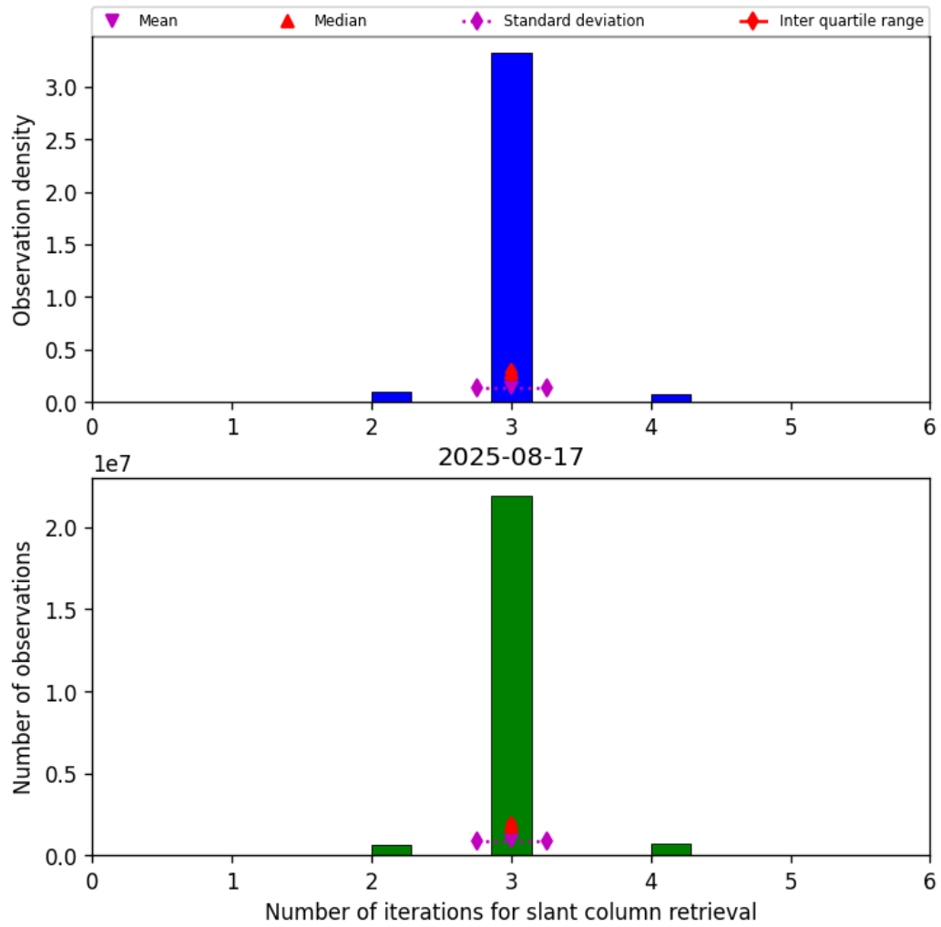
Figure 33: Histogram of “Number of iterations for slant column retrieval” for 2025-08-17 to 2025-08-17
