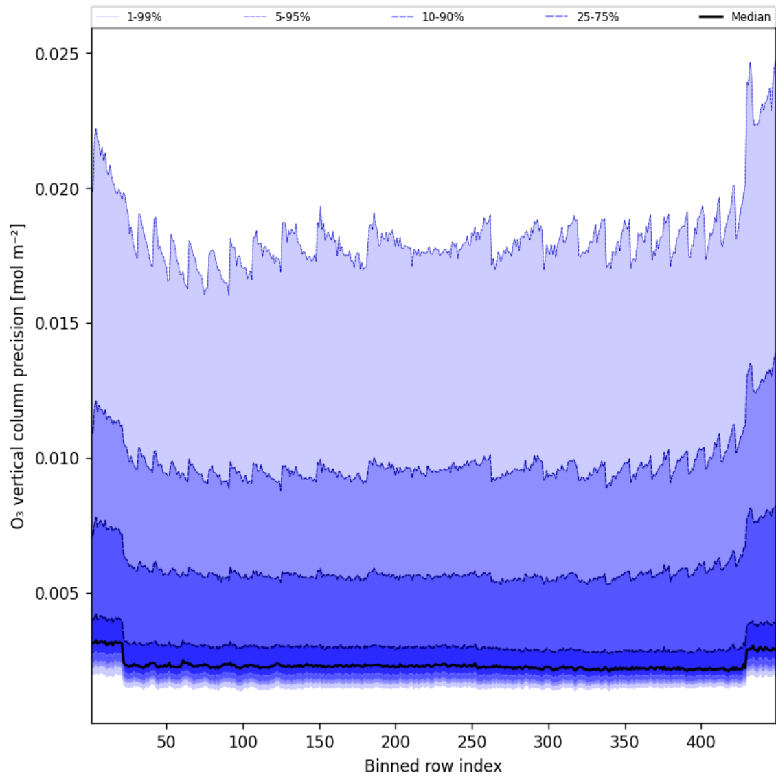
Figure 42: Along track statistics of “O 3 vertical column precision” for 2025-08-17 to 2025-08-17
