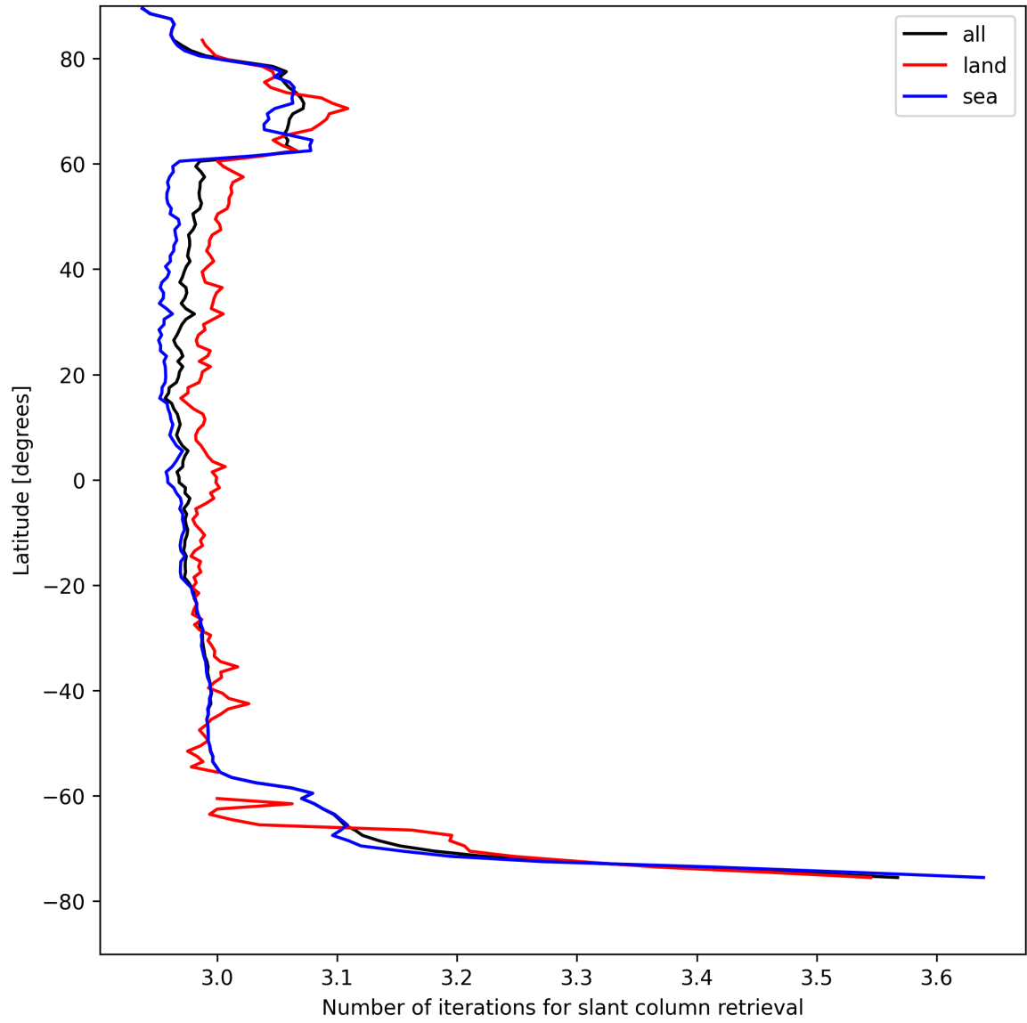
Figure 21: Zonal average of “Number of iterations for slant column retrieval” for 2025-08-17 to 2025-08-17.
