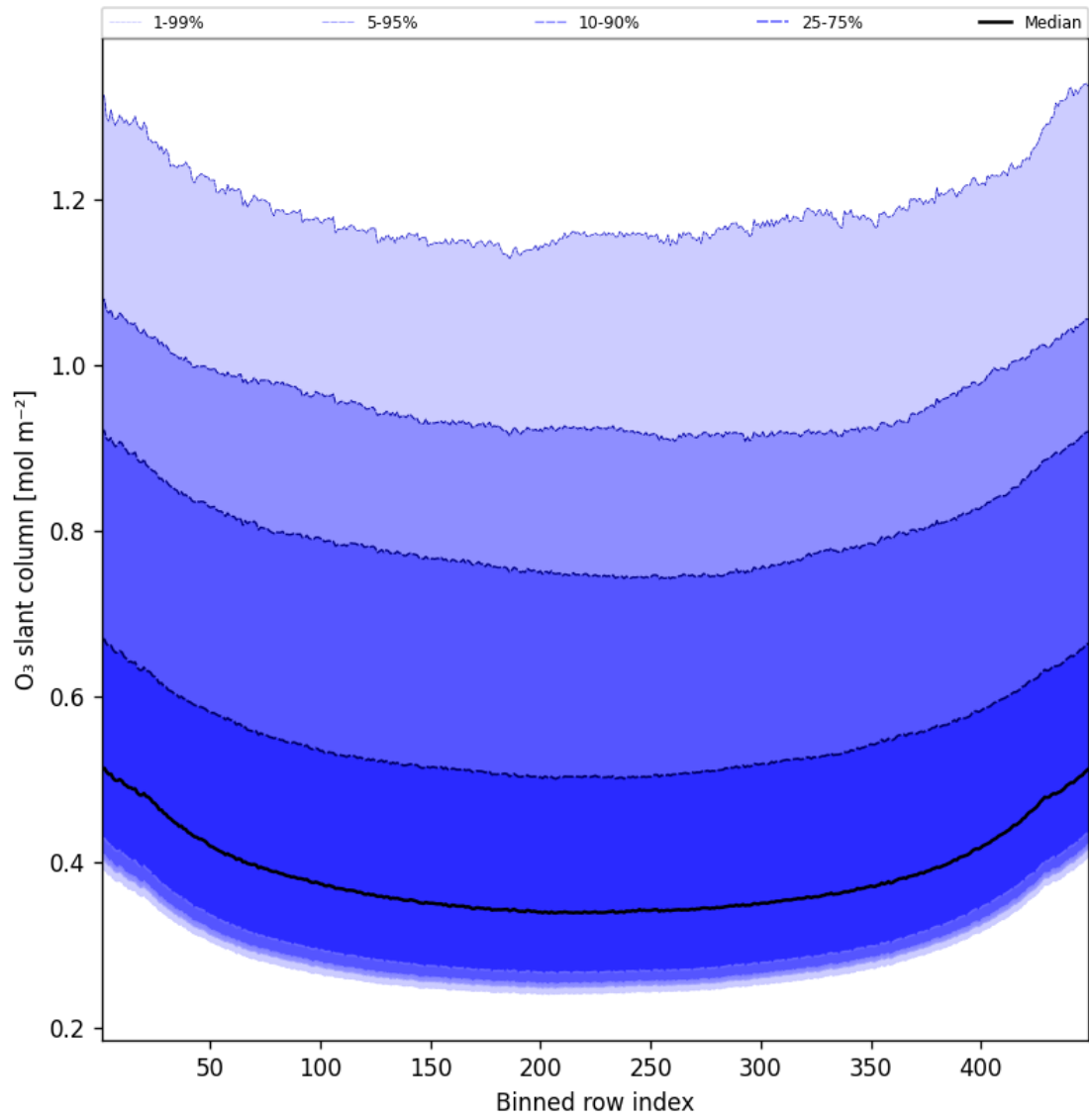
Figure 43: Along track statistics of “O 3 slant column” for 2025-08-17 to 2025-08-17
