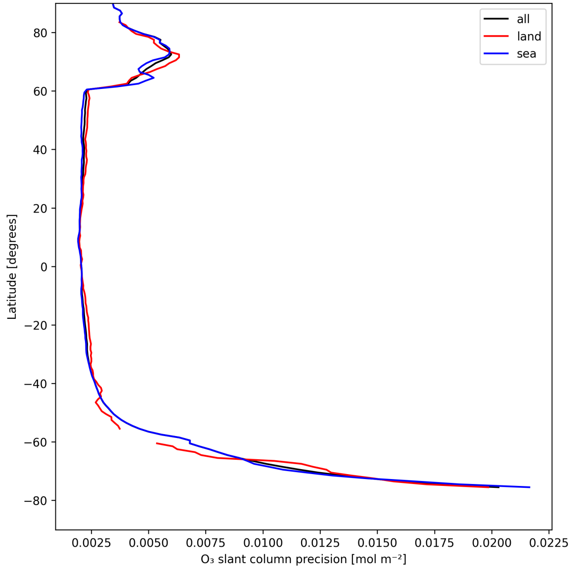
Figure 20: Zonal average of “O 3 slant column precision” for 2025-08-17 to 2025-08-17.
