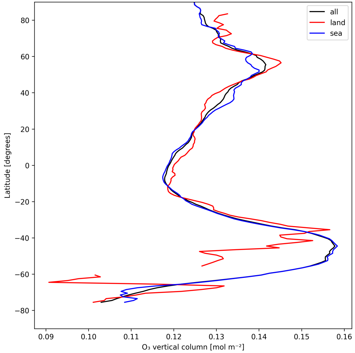
Figure 17: Zonal average of “O 3 vertical column” for 2025-08-17 to 2025-08-17.
