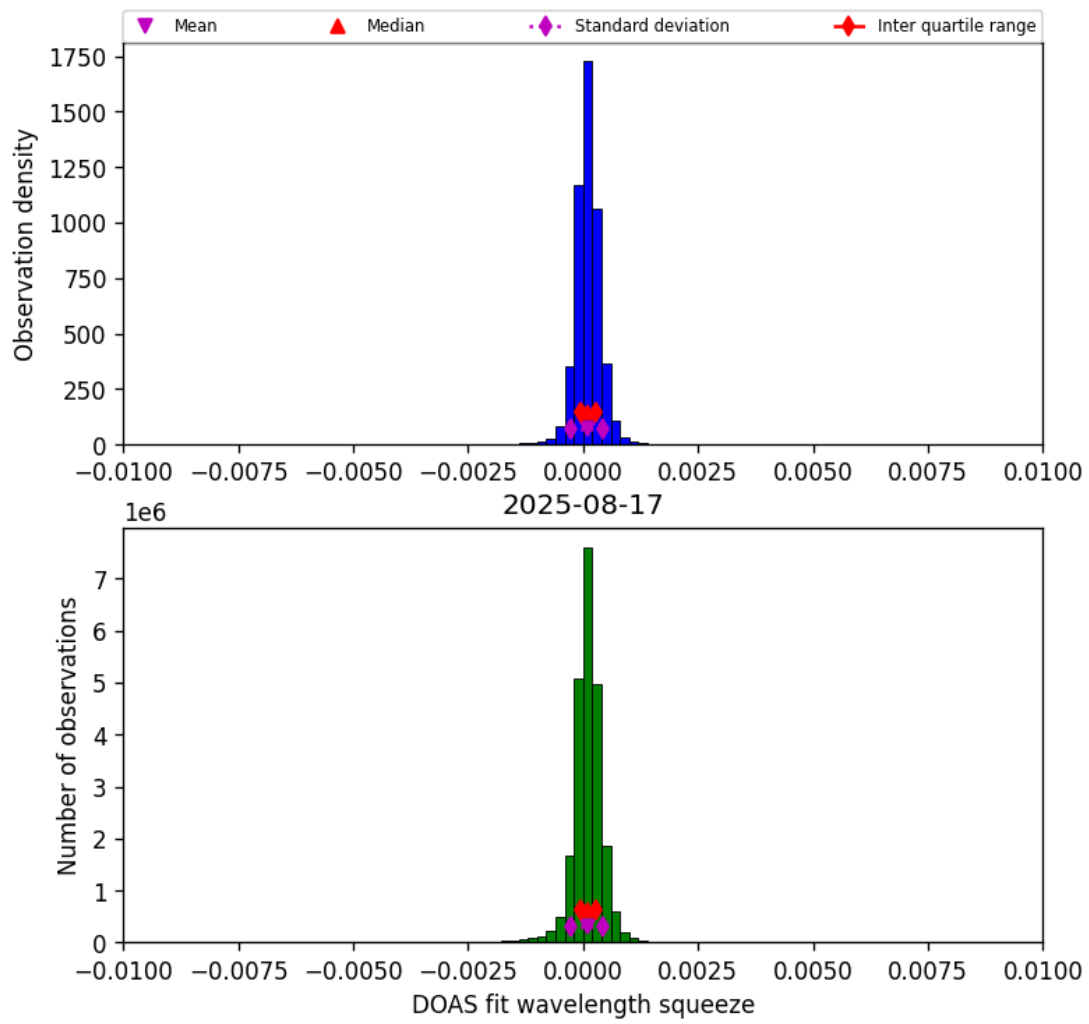
Figure 36: Histogram of “DOAS fit wavelength squeeze” for 2025-08-17 to 2025-08-17
