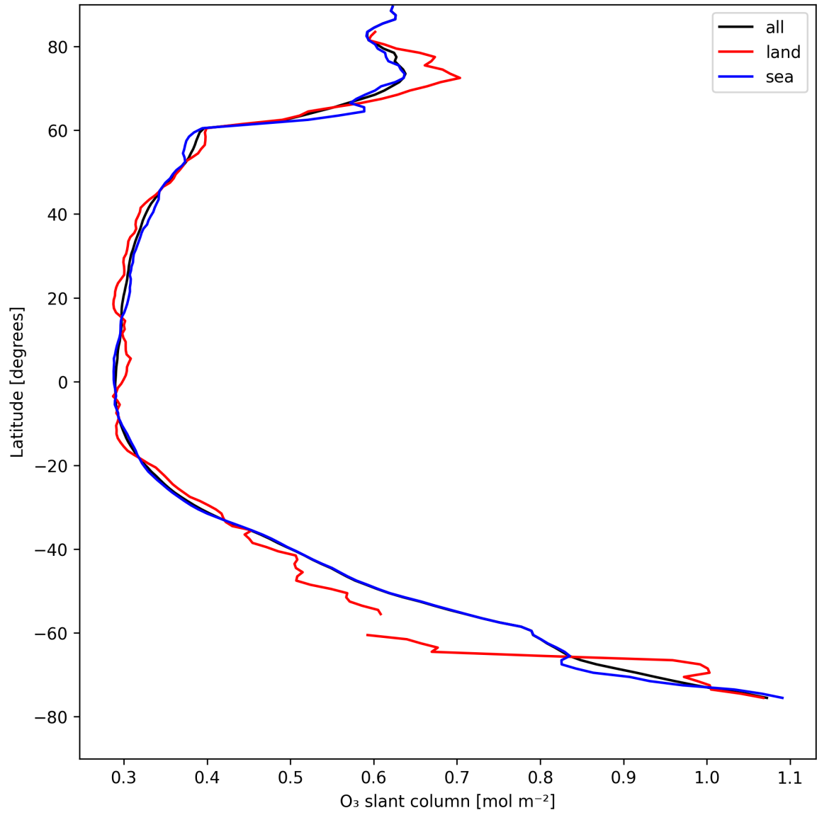
Figure 19: Zonal average of “O 3 slant column” for 2025-08-17 to 2025-08-17.
