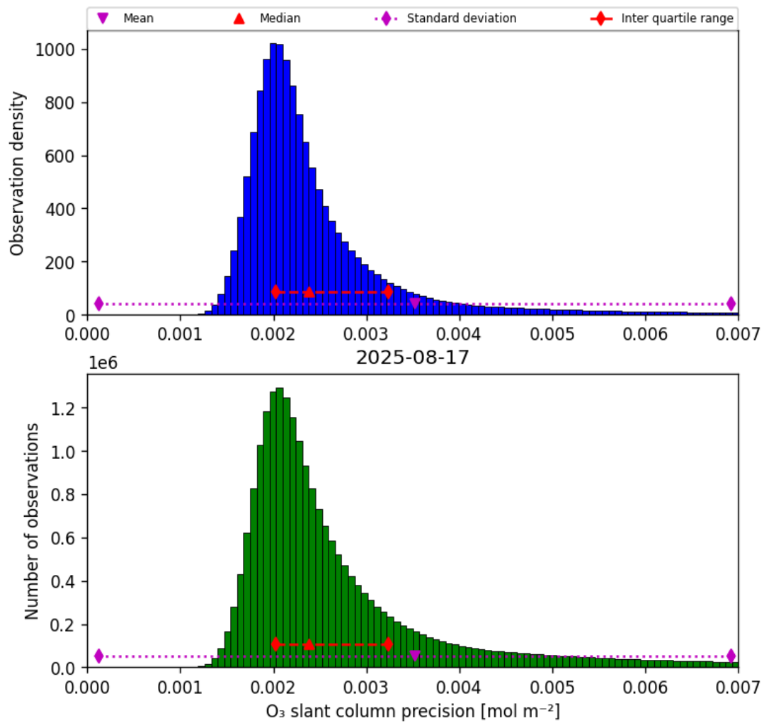
Figure 32: Histogram of “O 3 slant column precision” for 2025-08-17 to 2025-08-17
