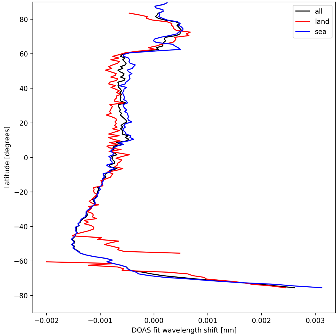
Figure 23: Zonal average of “DOAS fit wavelength shift” for 2025-08-17 to 2025-08-17.
