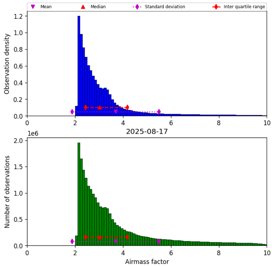
Figure 37: Histogram of “Airmass factor” for 2025-08-17 to 2025-08-17
