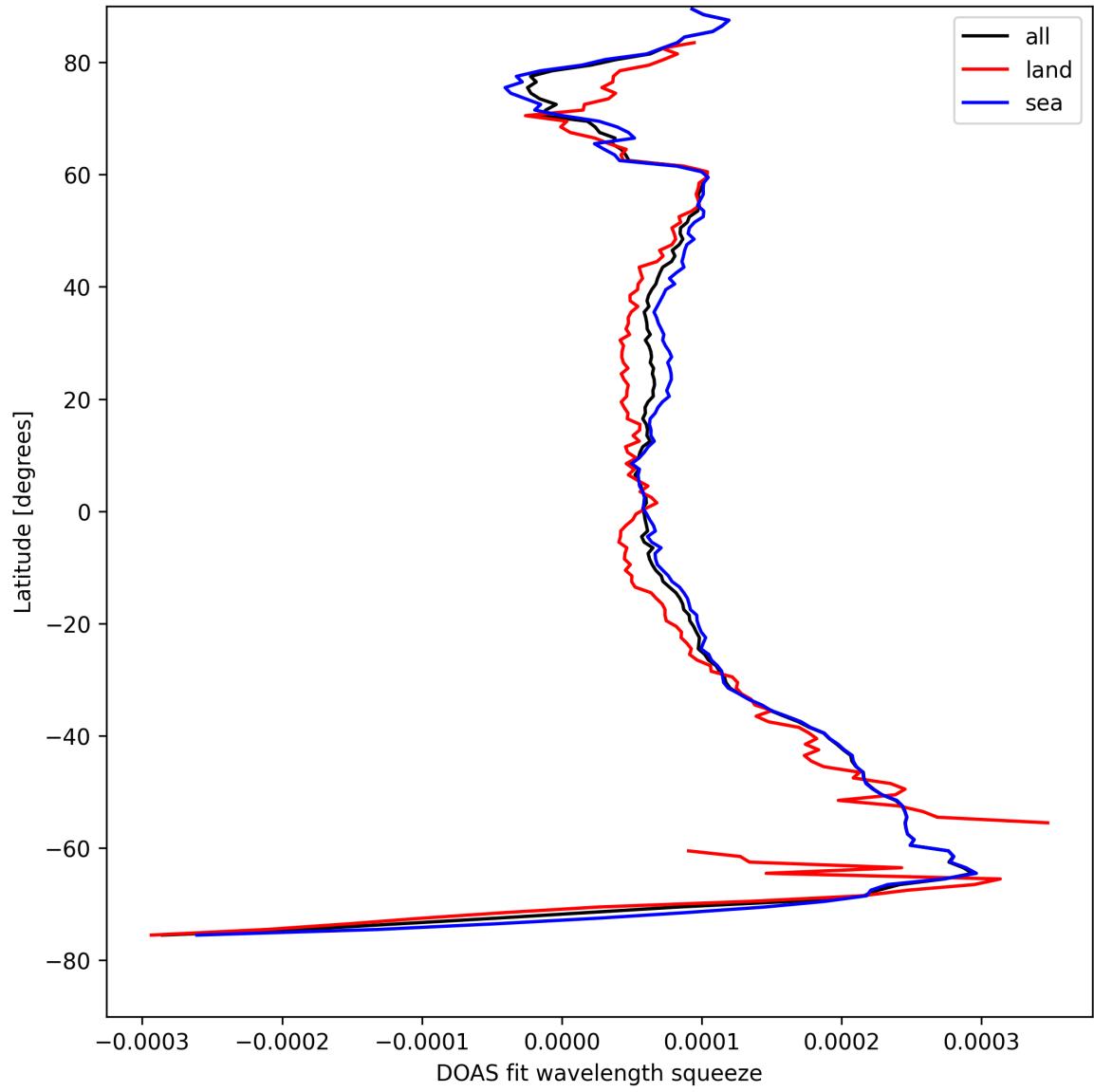
Figure 24: Zonal average of “DOAS fit wavelength squeeze” for 2025-08-17 to 2025-08-17.
