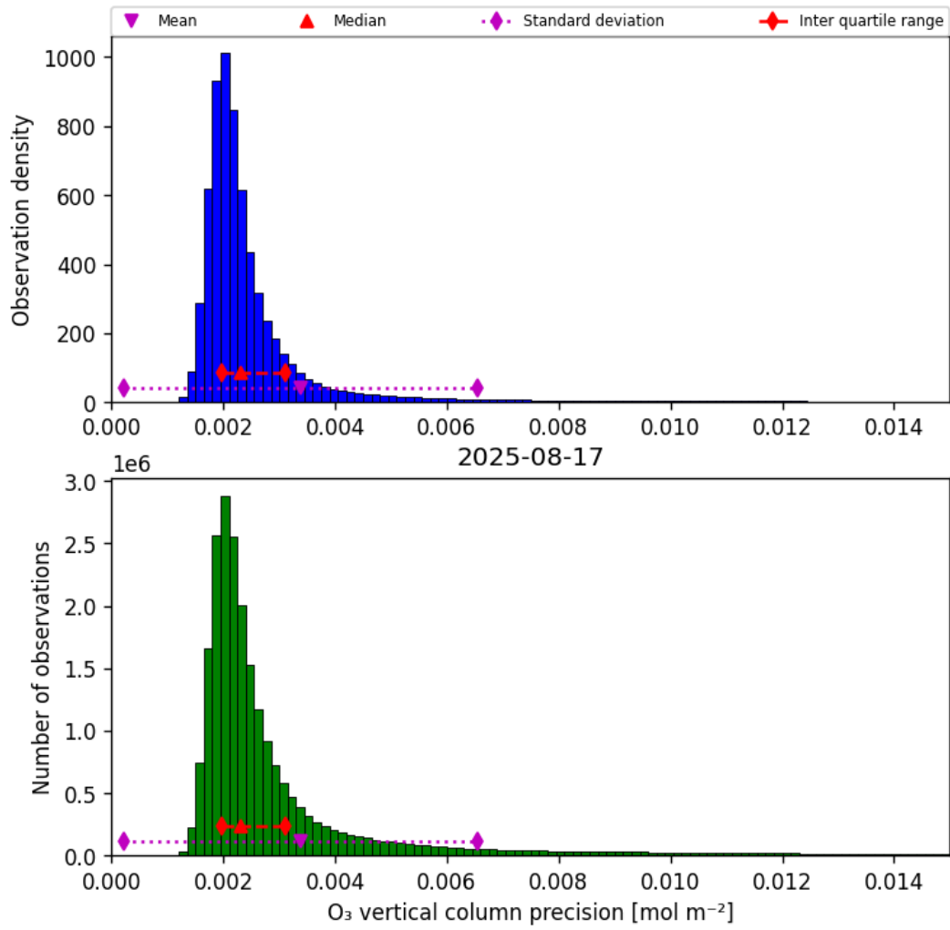
Figure 30: Histogram of “O 3 vertical column precision” for 2025-08-17 to 2025-08-17
