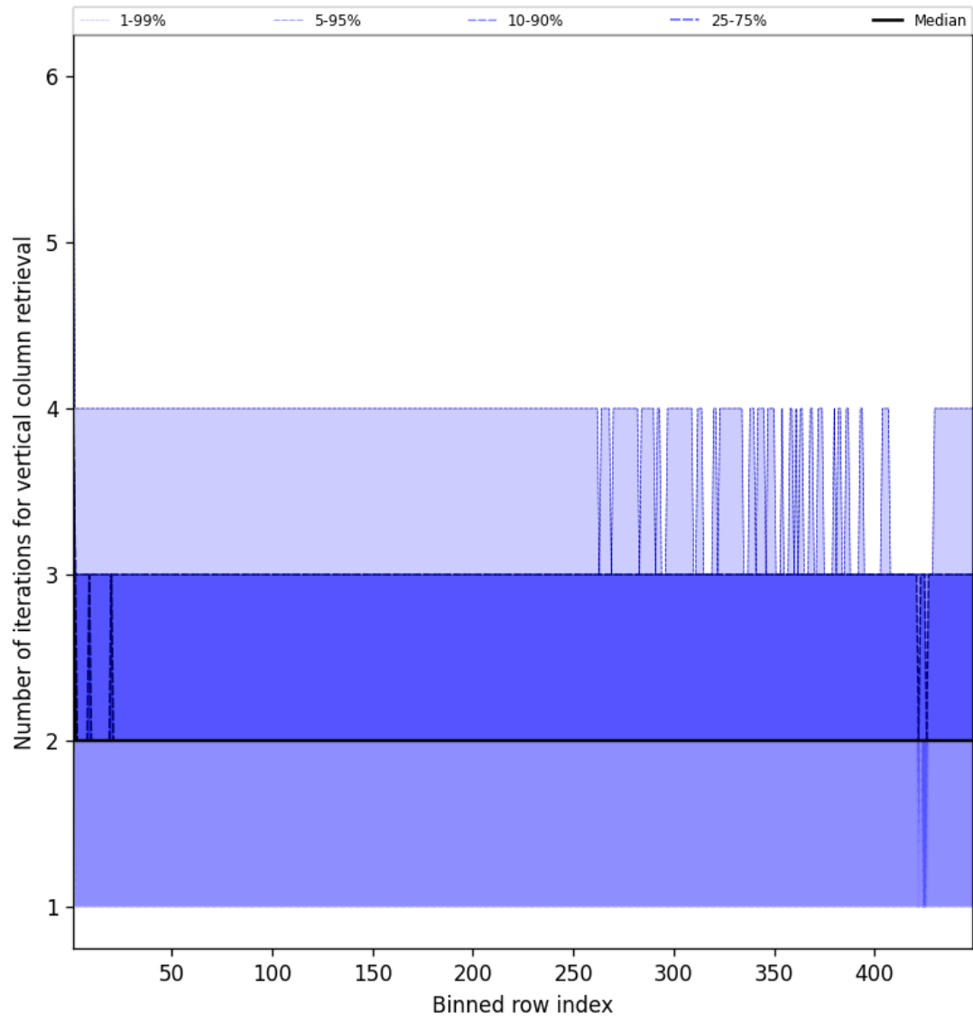
Figure 51: Along track statistics of “Number of iterations for vertical column retrieval” for 2025-08-17 to 2025-08-17
