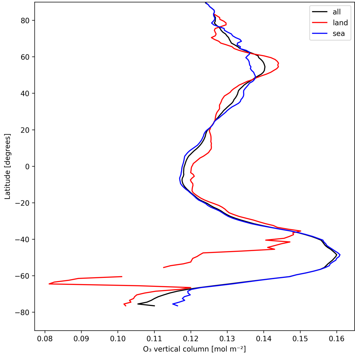
Figure 17: Zonal average of “O 3 vertical column” for 2025-08-18 to 2025-08-19.
