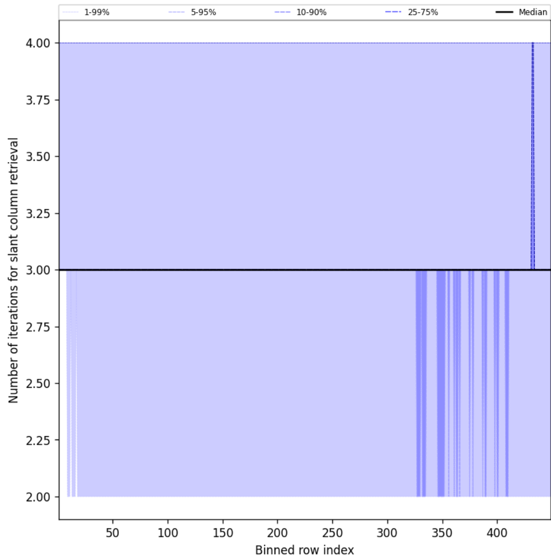
Figure 45: Along track statistics of “Number of iterations for slant column retrieval” for 2025-08-18 to 2025-08-19
