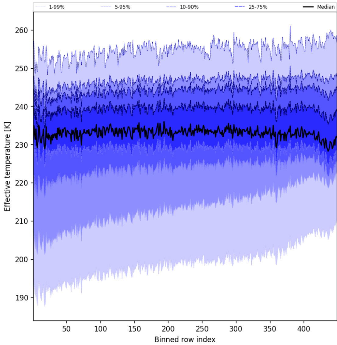
Figure 50: Along track statistics of “Effective temperature” for 2025-08-18 to 2025-08-19
