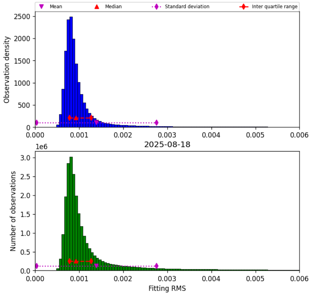
Figure 34: Histogram of “Fitting RMS” for 2025-08-18 to 2025-08-19
