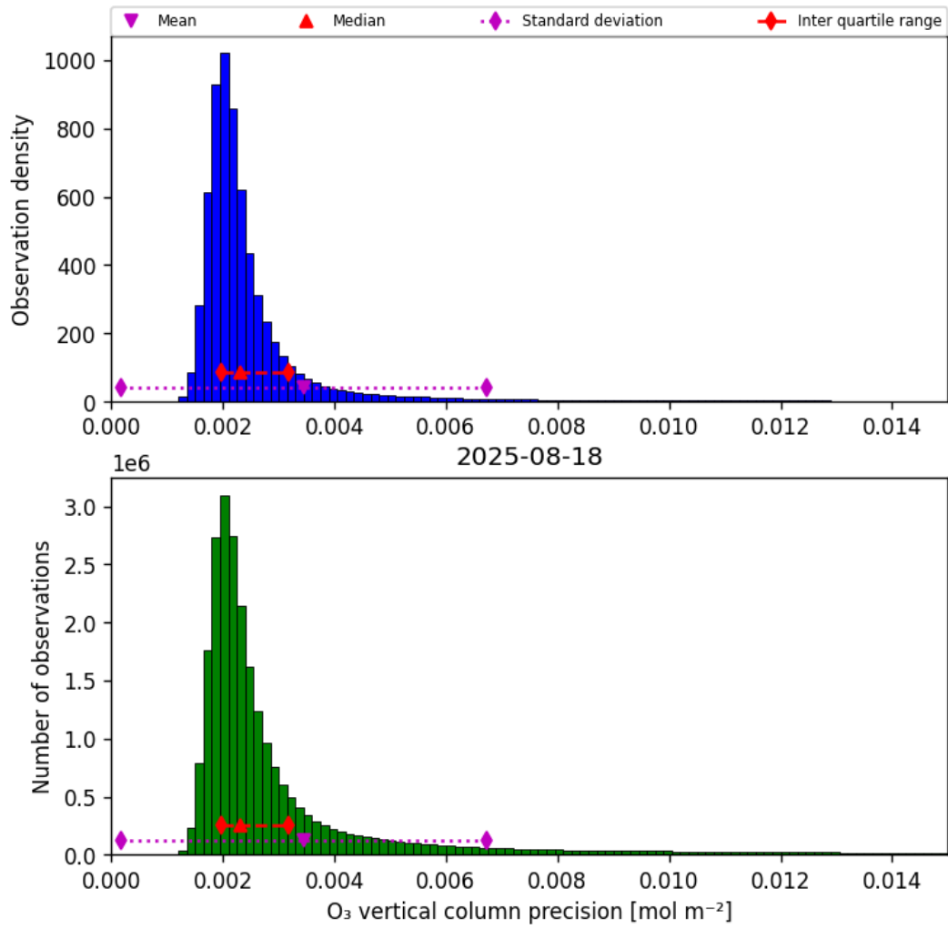
Figure 30: Histogram of “O 3 vertical column precision” for 2025-08-18 to 2025-08-19
