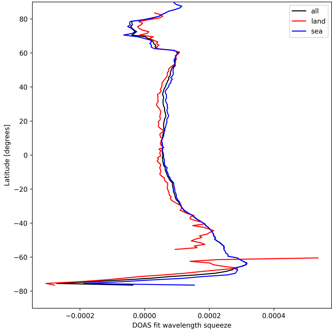
Figure 24: Zonal average of “DOAS fit wavelength squeeze” for 2025-08-18 to 2025-08-19.
