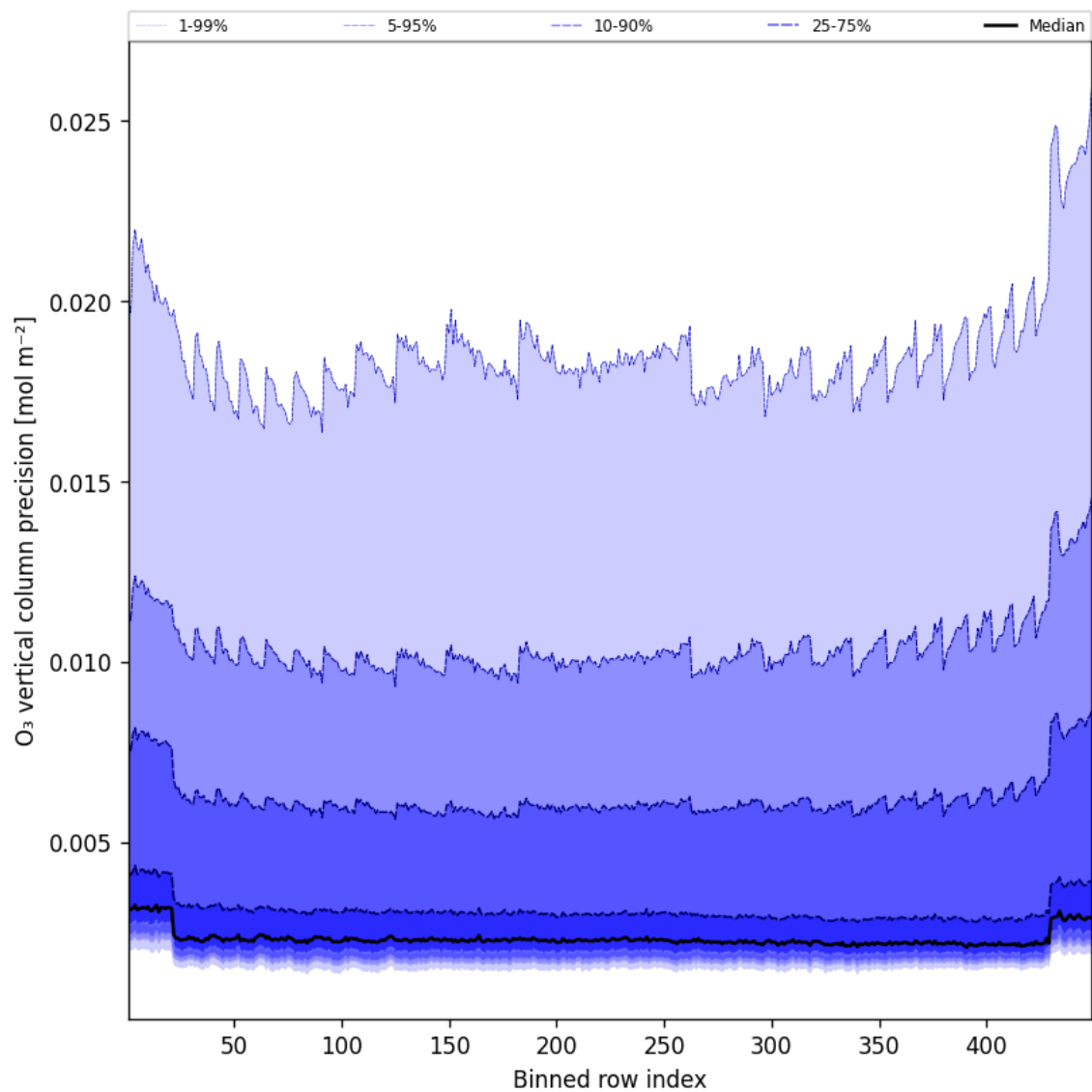
Figure 42: Along track statistics of “O 3 vertical column precision” for 2025-08-18 to 2025-08-19
