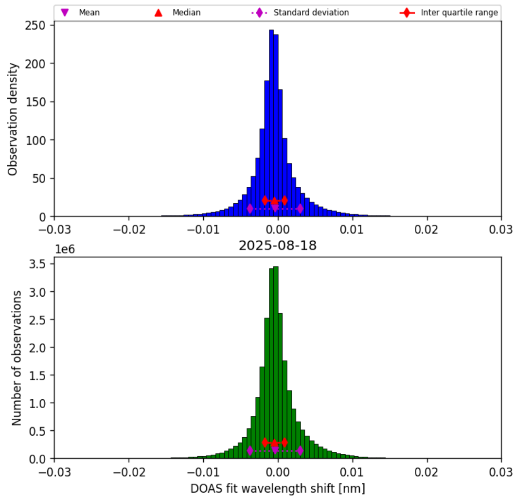
Figure 35: Histogram of “DOAS fit wavelength shift” for 2025-08-18 to 2025-08-19
