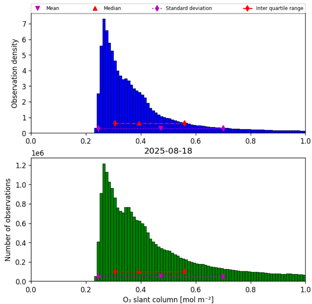
Figure 31: Histogram of “O 3 slant column” for 2025-08-18 to 2025-08-19
