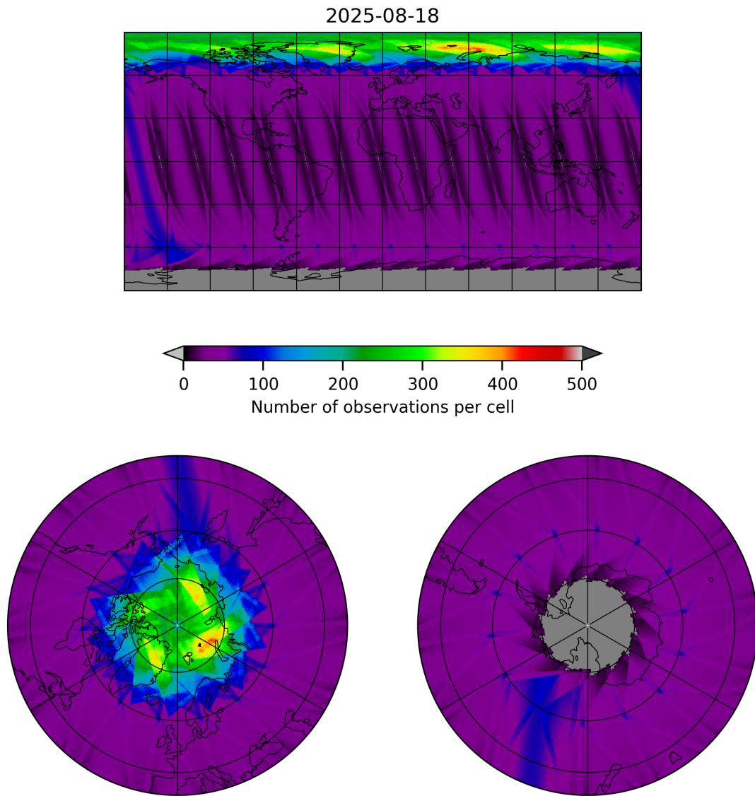
Figure 15: Map of the number of observations for 2025-08-18 to 2025-08-19
