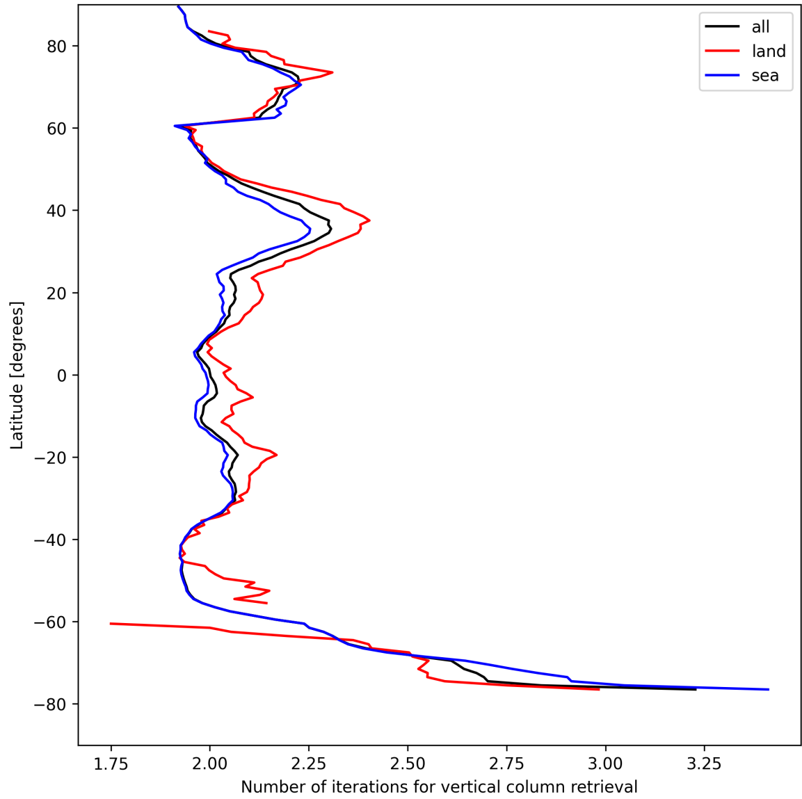
Figure 27: Zonal average of “Number of iterations for vertical column retrieval” for 2025-08-18 to 2025-08-19.
