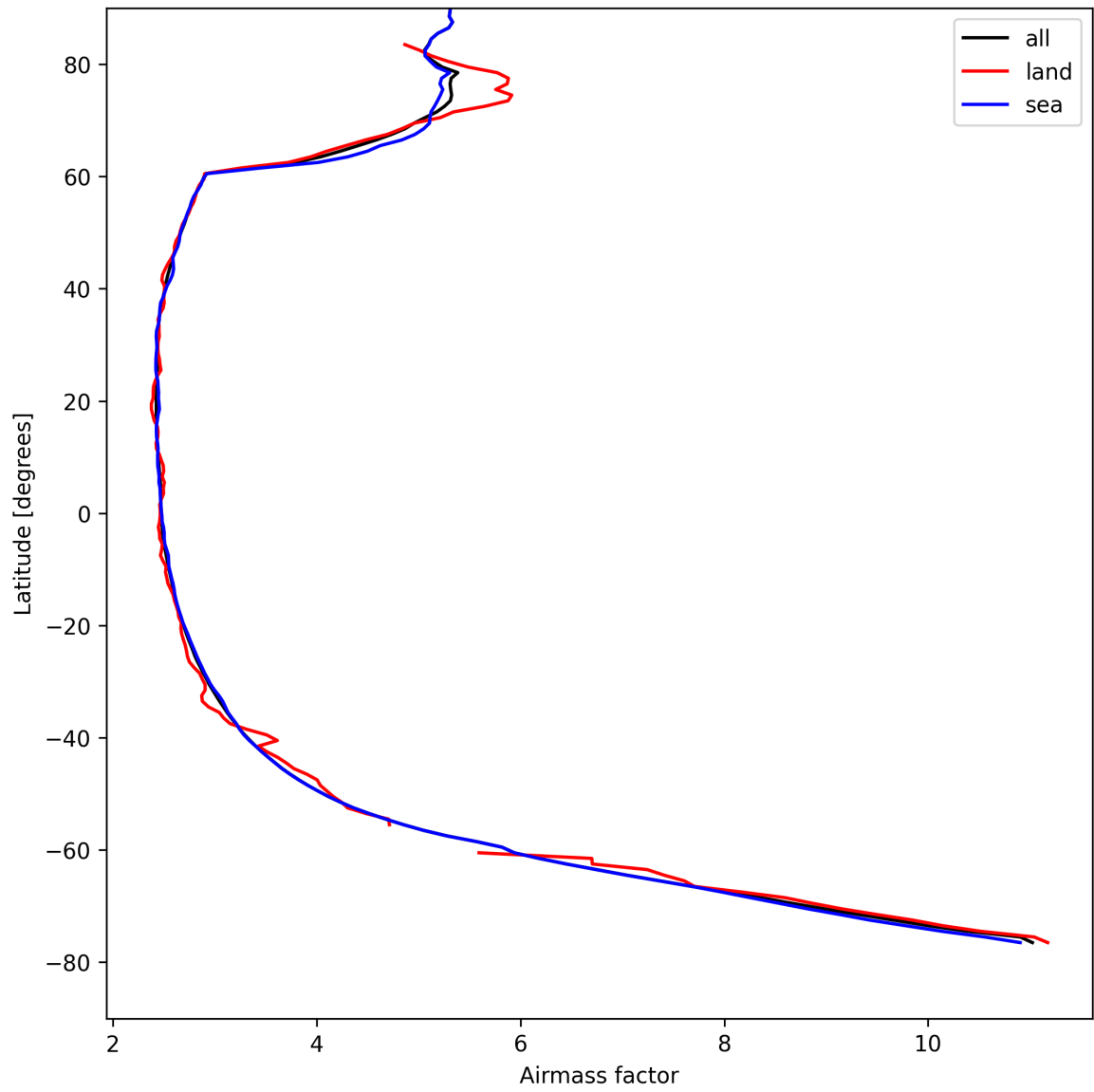
Figure 25: Zonal average of “Airmass factor” for 2025-08-18 to 2025-08-19.
