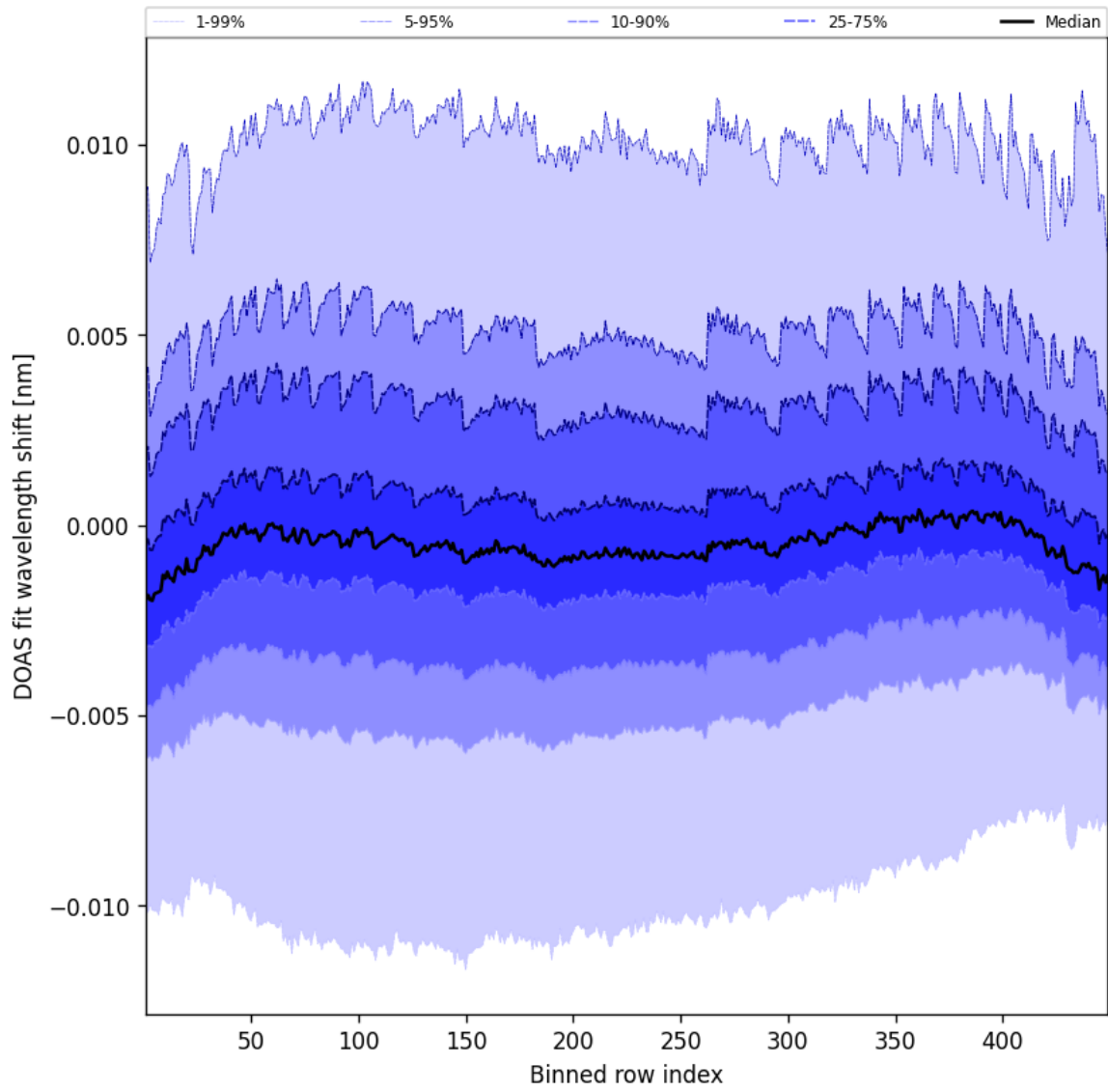
Figure 47: Along track statistics of “DOAS fit wavelength shift” for 2025-08-18 to 2025-08-19
