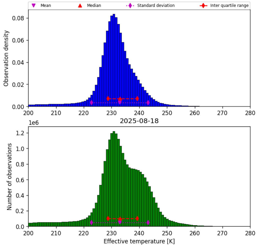
Figure 38: Histogram of “Effective temperature” for 2025-08-18 to 2025-08-19
