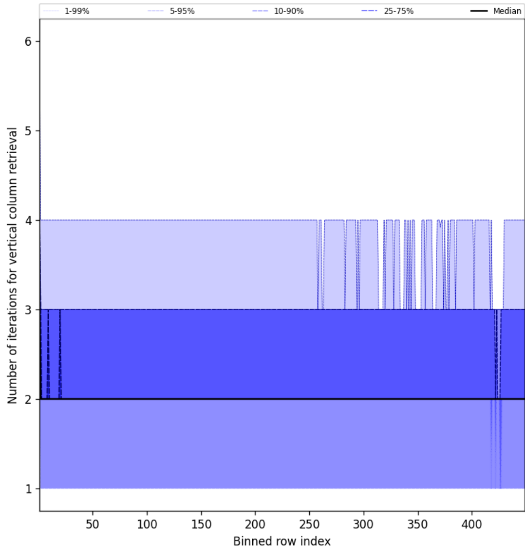
Figure 51: Along track statistics of “Number of iterations for vertical column retrieval” for 2025-08-18 to 2025-08-19
