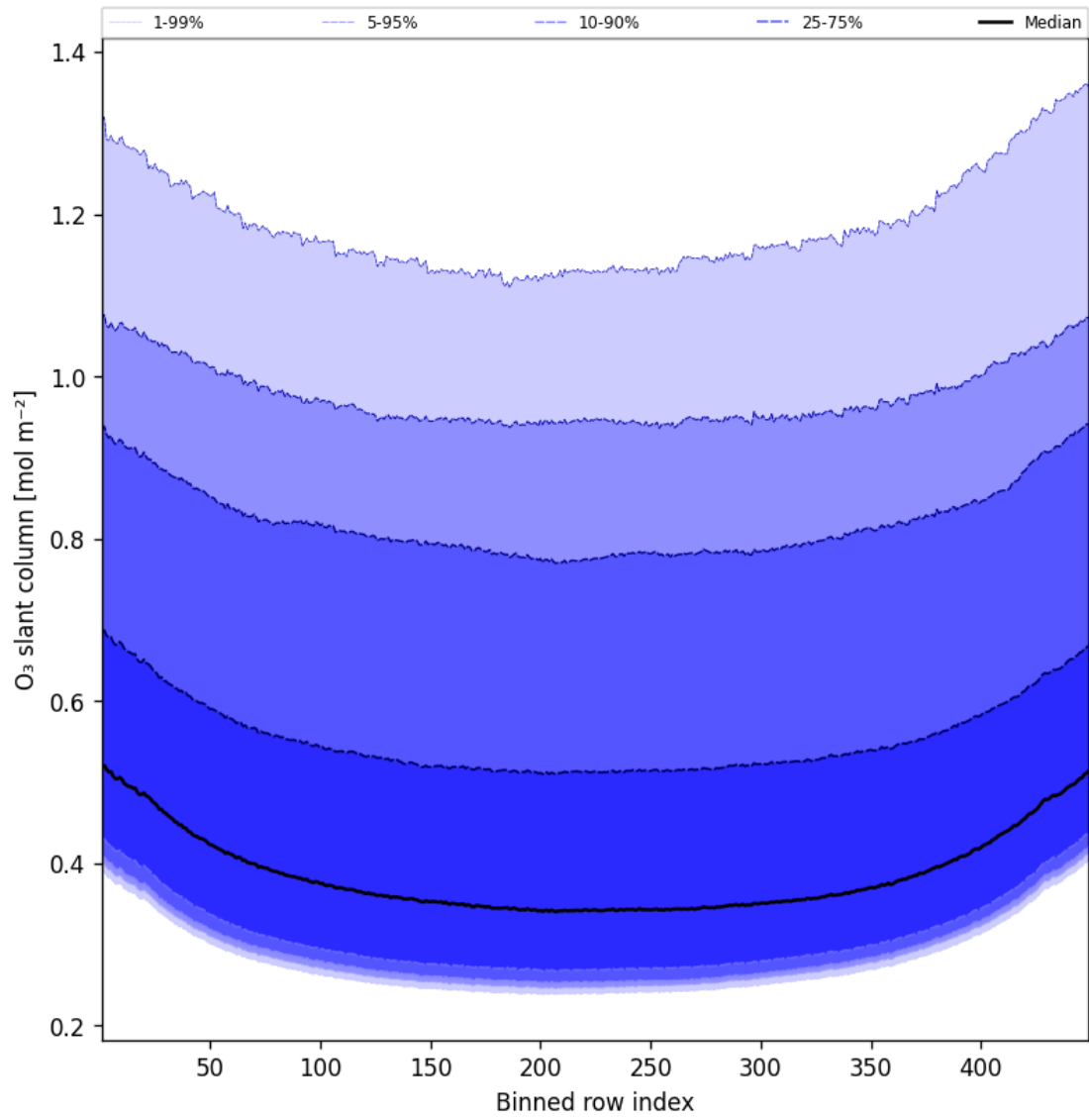
Figure 43: Along track statistics of “O 3 slant column” for 2025-08-18 to 2025-08-19
