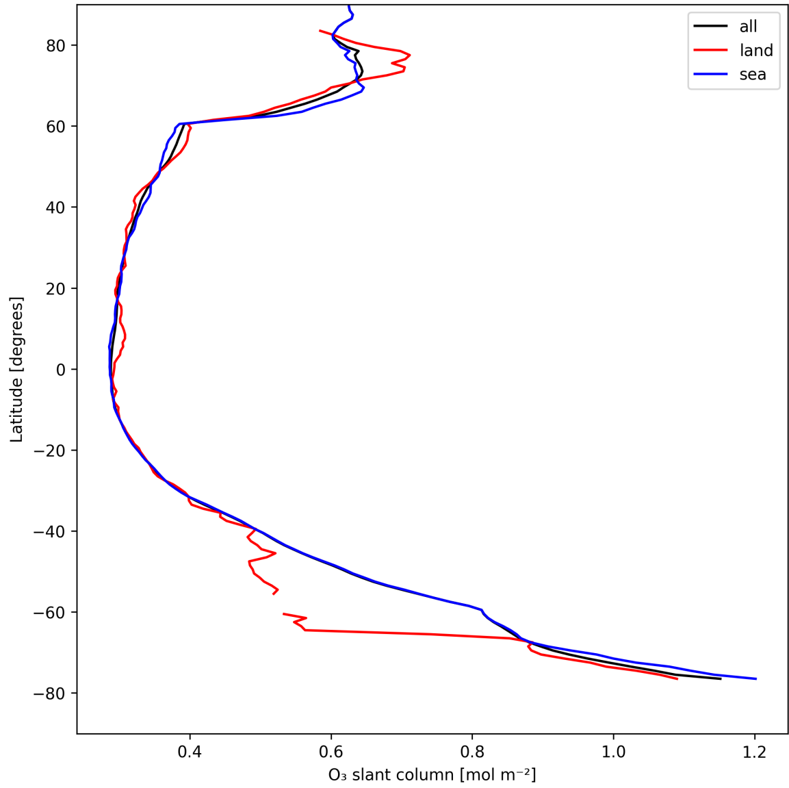
Figure 19: Zonal average of “O 3 slant column” for 2025-08-18 to 2025-08-19.
