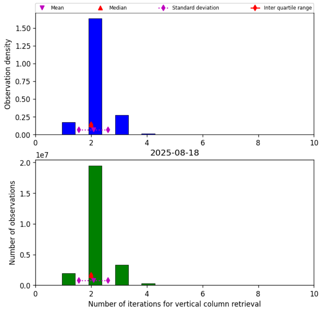
Figure 39: Histogram of “Number of iterations for vertical column retrieval” for 2025-08-18 to 2025-08-19
