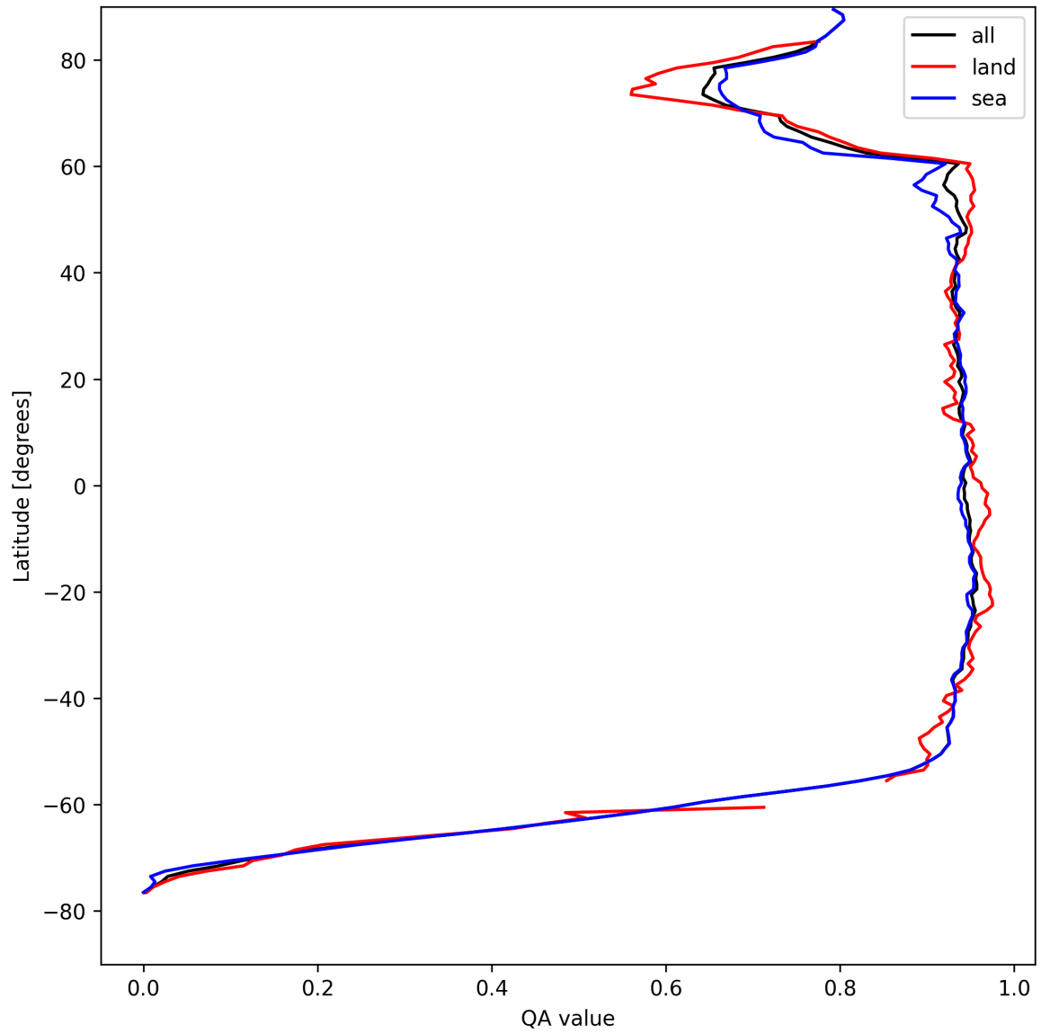
Figure 16: Zonal average of “QA value” for 2025-08-18 to 2025-08-19.
