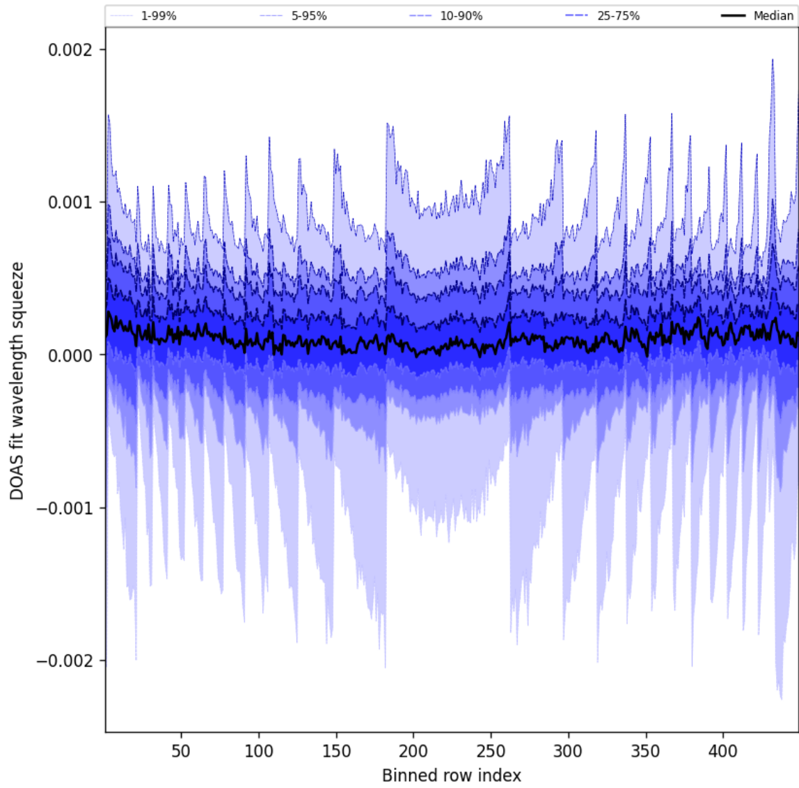
Figure 48: Along track statistics of “DOAS fit wavelength squeeze” for 2025-08-18 to 2025-08-19
