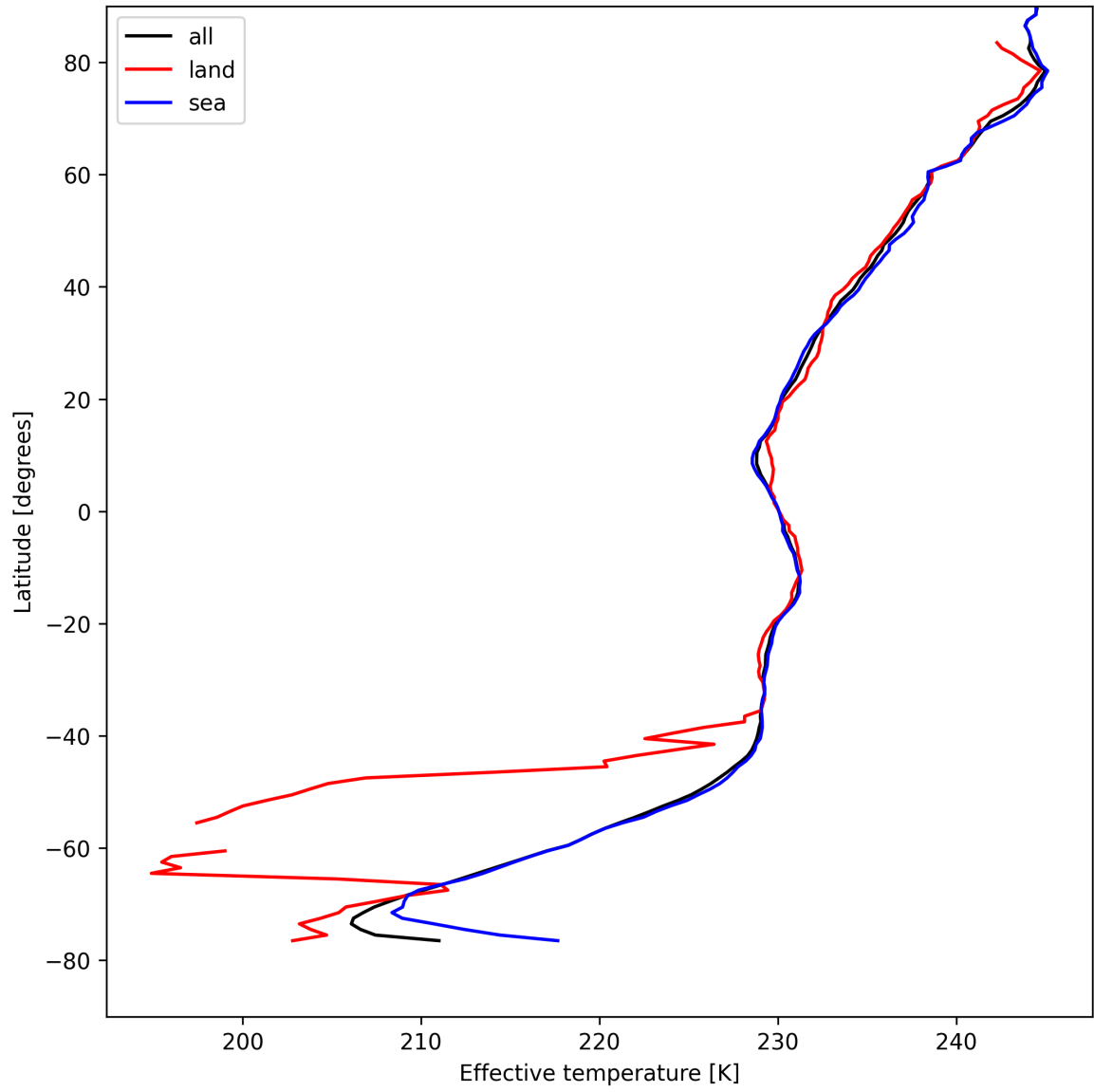
Figure 26: Zonal average of “Effective temperature” for 2025-08-18 to 2025-08-19.
