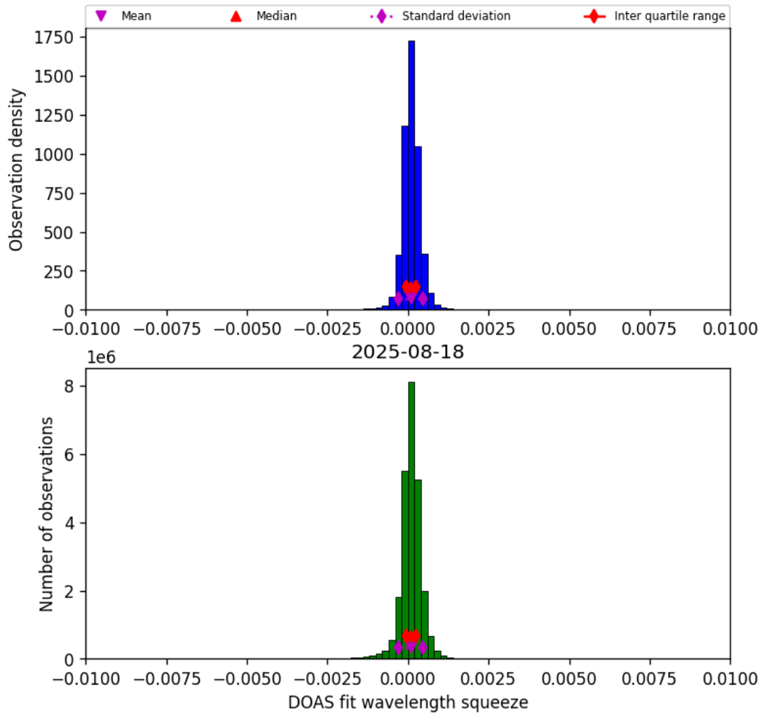
Figure 36: Histogram of “DOAS fit wavelength squeeze” for 2025-08-18 to 2025-08-19
