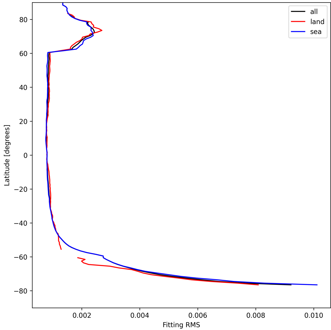
Figure 22: Zonal average of “Fitting RMS” for 2025-08-18 to 2025-08-19.
