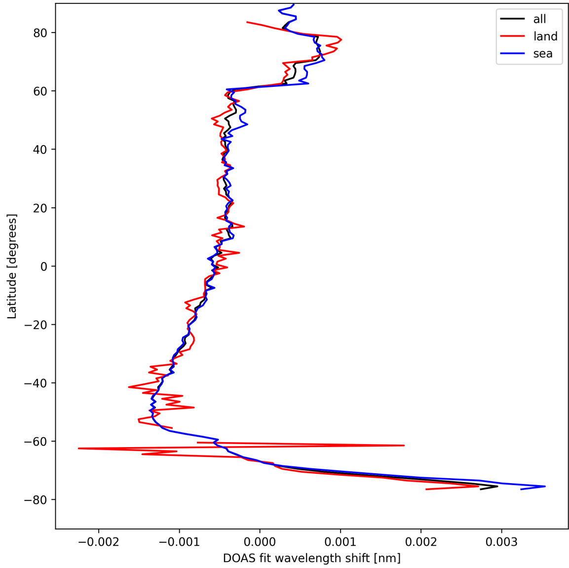
Figure 23: Zonal average of “DOAS fit wavelength shift” for 2025-08-18 to 2025-08-19.
