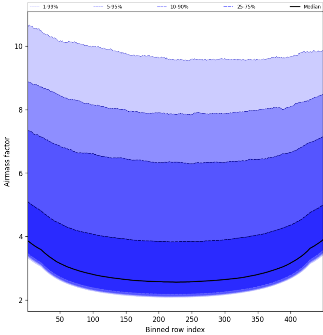
Figure 49: Along track statistics of “Airmass factor” for 2025-08-18 to 2025-08-19
