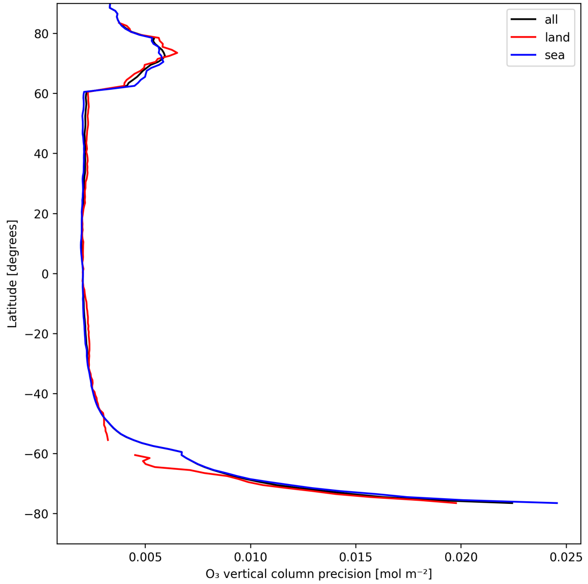
Figure 18: Zonal average of “O 3 vertical column precision” for 2025-08-18 to 2025-08-19.
