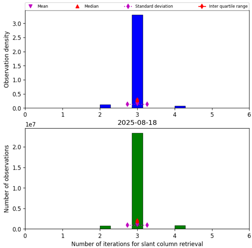
Figure 33: Histogram of “Number of iterations for slant column retrieval” for 2025-08-18 to 2025-08-19
