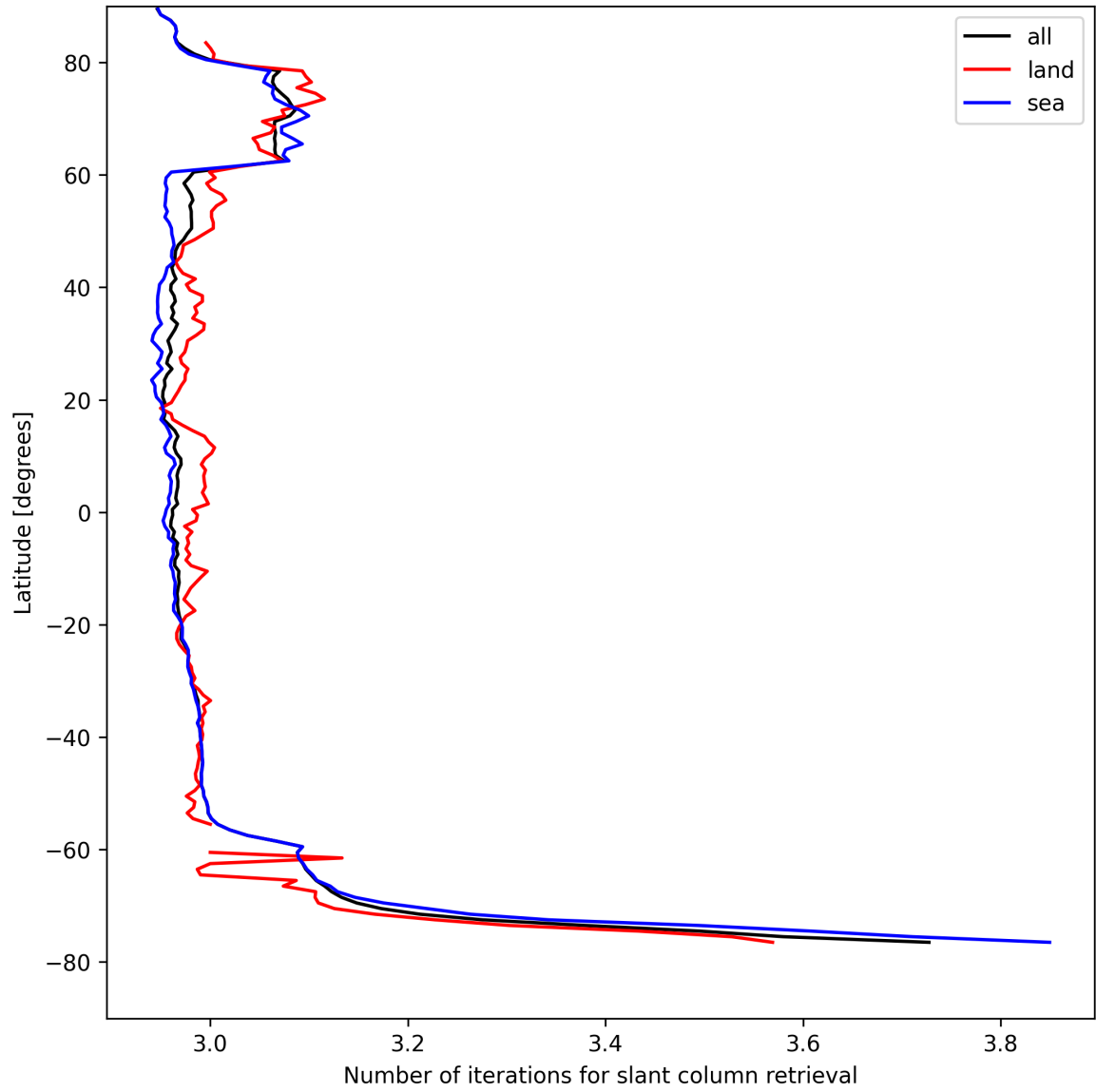
Figure 21: Zonal average of “Number of iterations for slant column retrieval” for 2025-08-18 to 2025-08-19.
