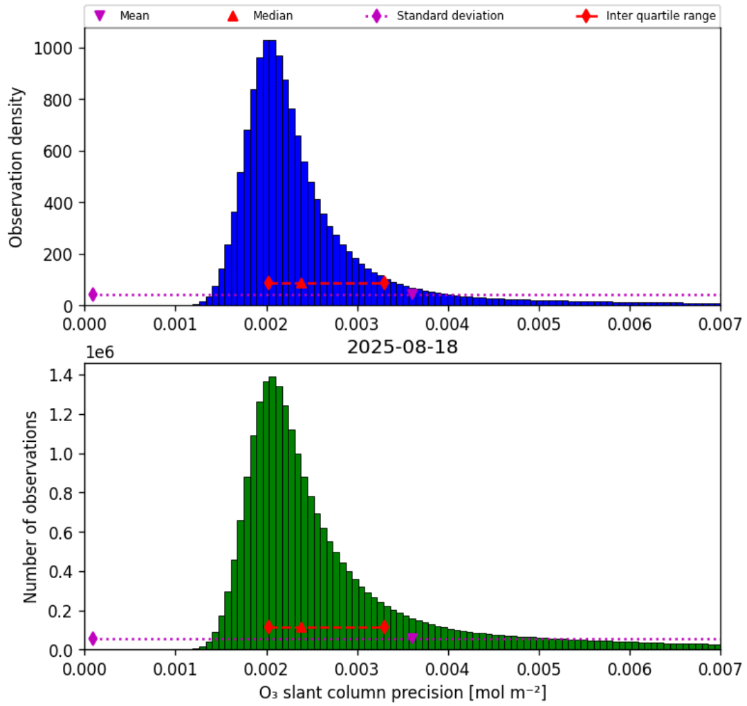
Figure 32: Histogram of “O 3 slant column precision” for 2025-08-18 to 2025-08-19
