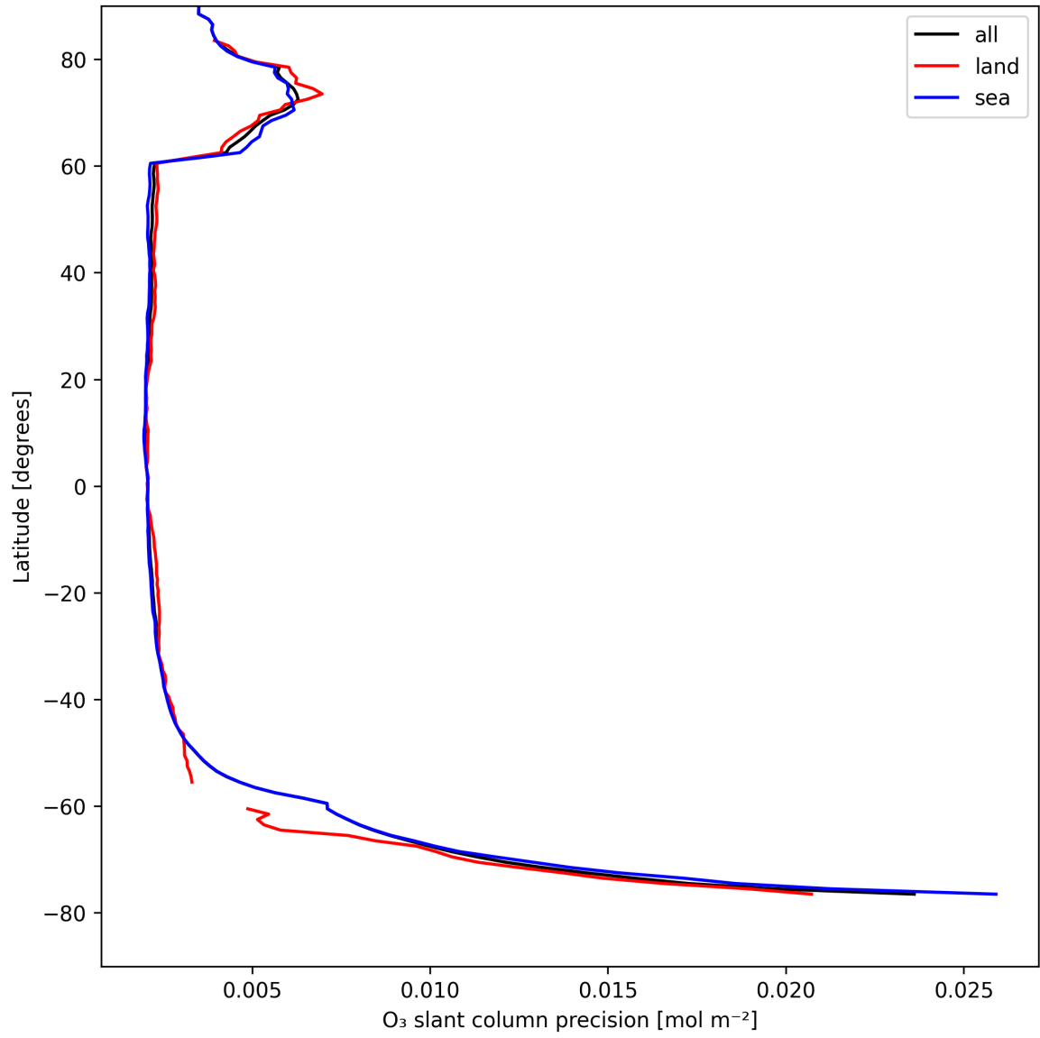
Figure 20: Zonal average of “O 3 slant column precision” for 2025-08-18 to 2025-08-19.
