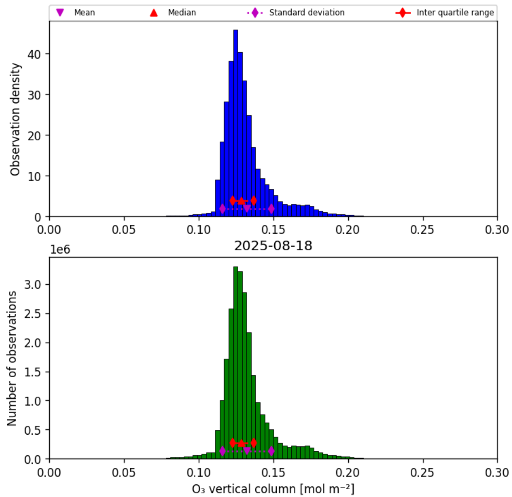
Figure 29: Histogram of “O 3 vertical column” for 2025-08-18 to 2025-08-19
