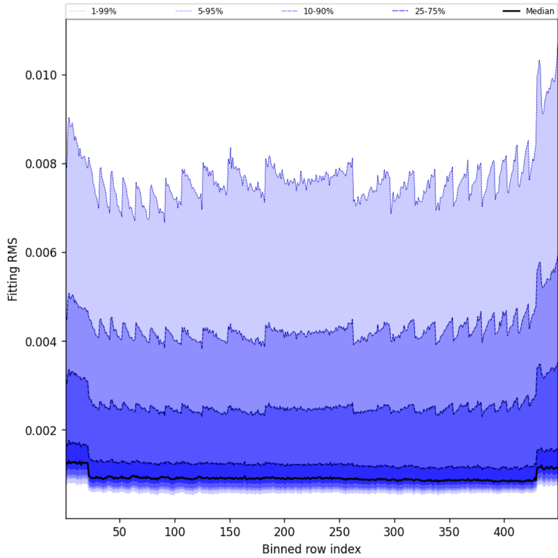
Figure 46: Along track statistics of “Fitting RMS” for 2025-08-18 to 2025-08-19
