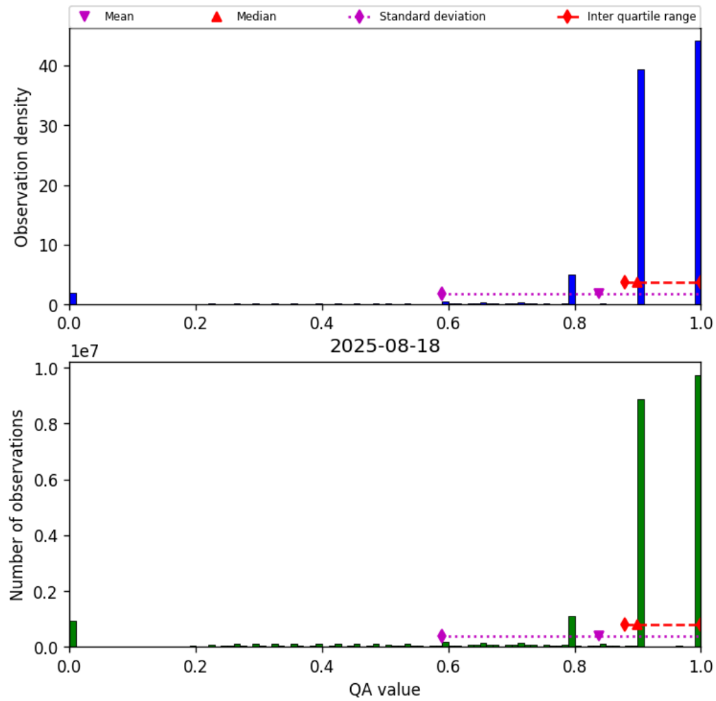
Figure 28: Histogram of “QA value” for 2025-08-18 to 2025-08-19
