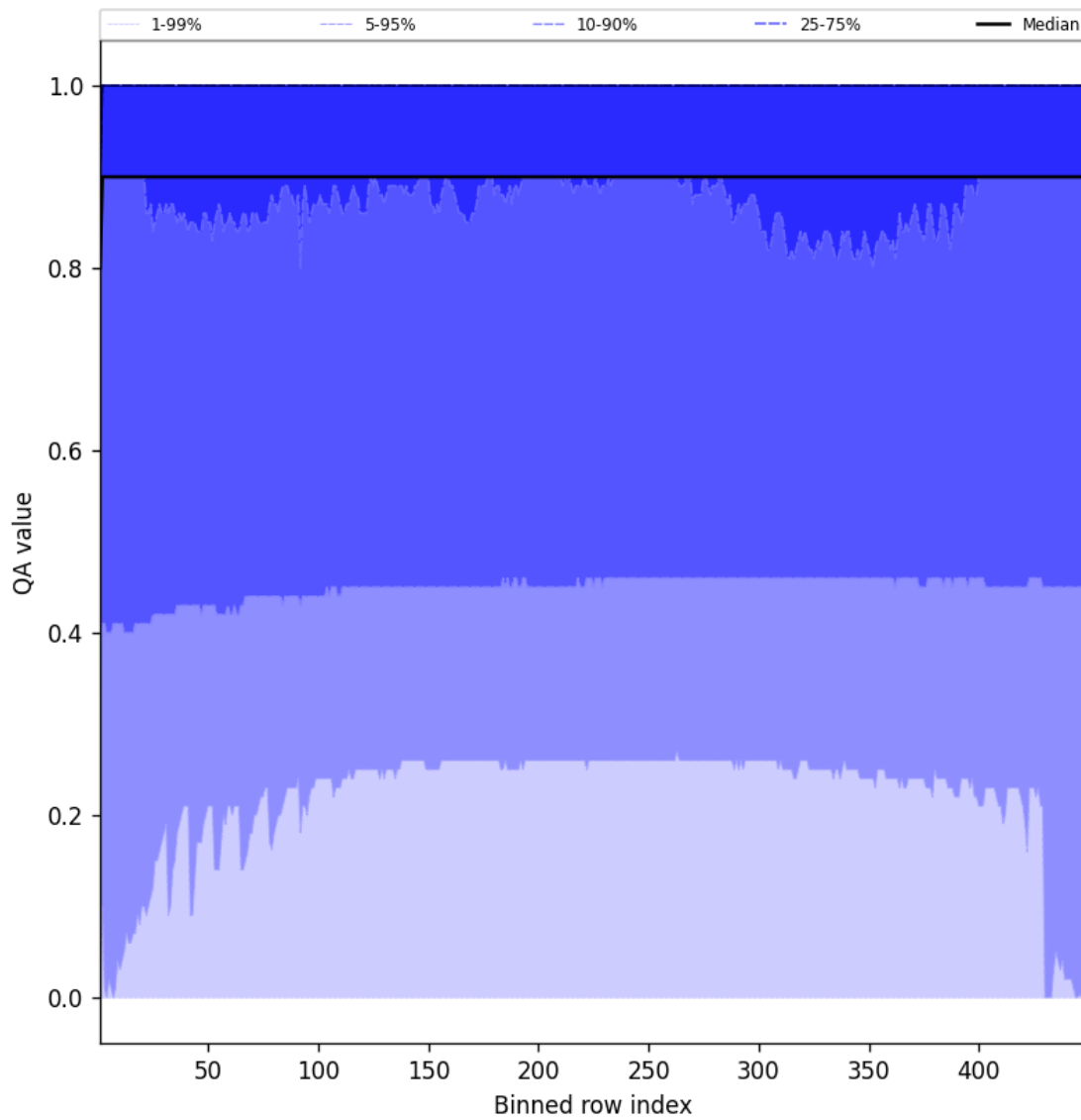
Figure 40: Along track statistics of “QA value” for 2025-08-18 to 2025-08-19
