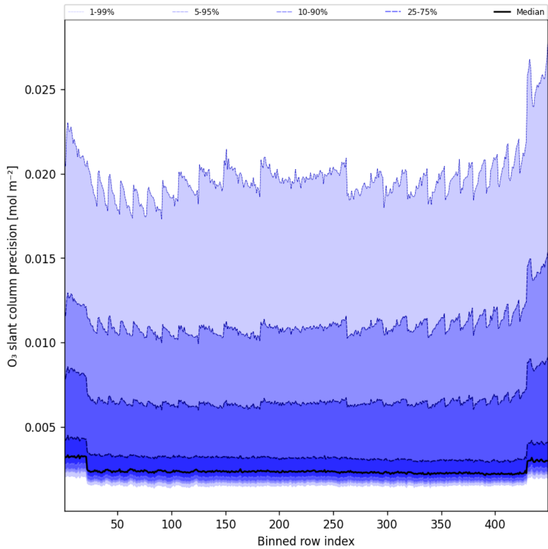
Figure 44: Along track statistics of “O 3 slant column precision” for 2025-08-18 to 2025-08-19
