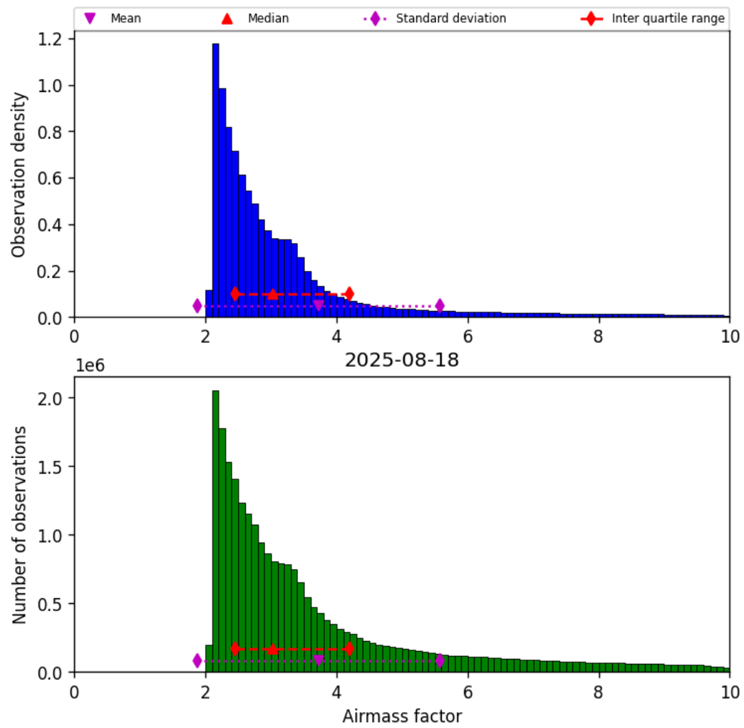
Figure 37: Histogram of “Airmass factor” for 2025-08-18 to 2025-08-19
