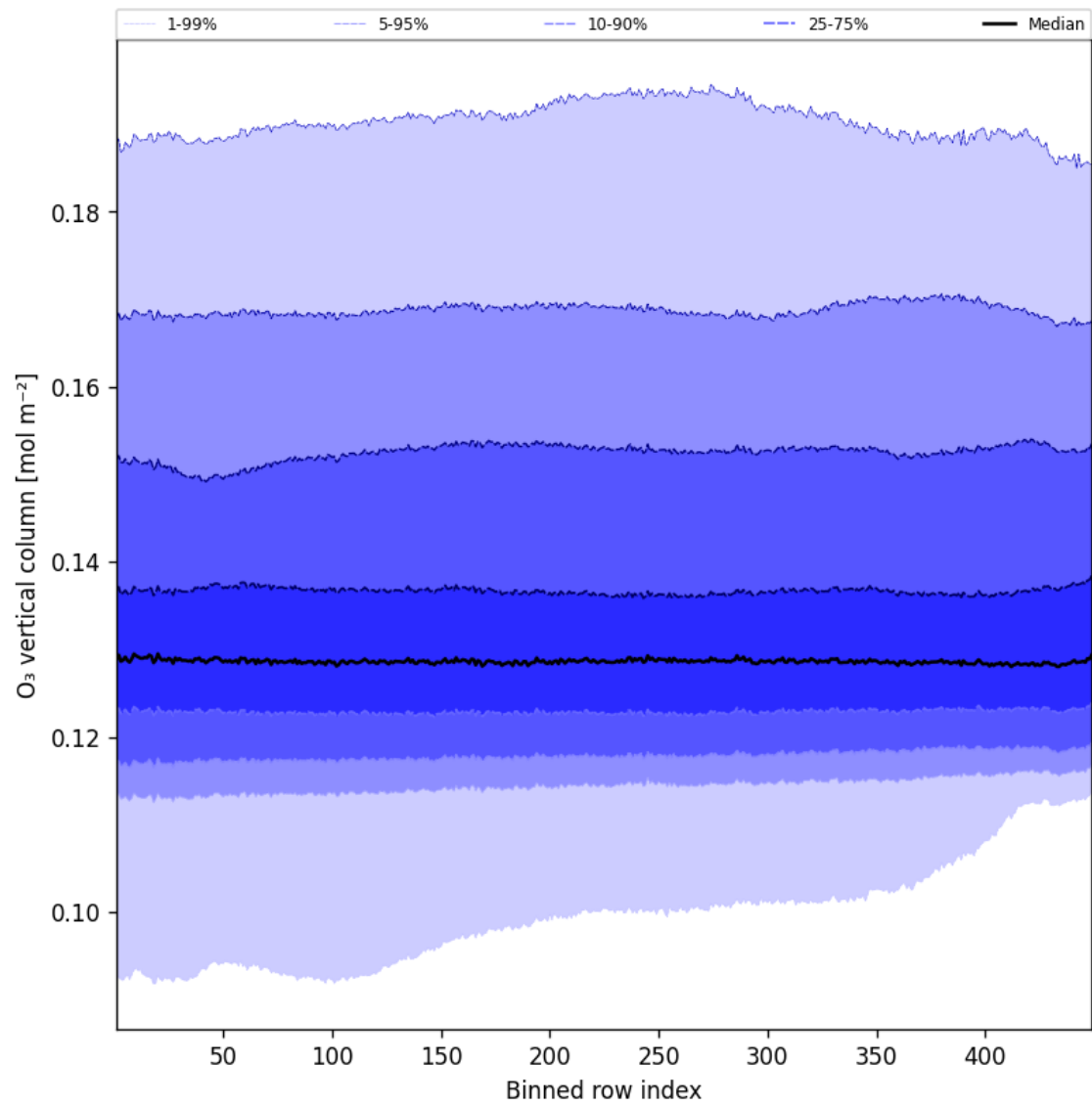
Figure 41: Along track statistics of “O 3 vertical column” for 2025-08-18 to 2025-08-19
