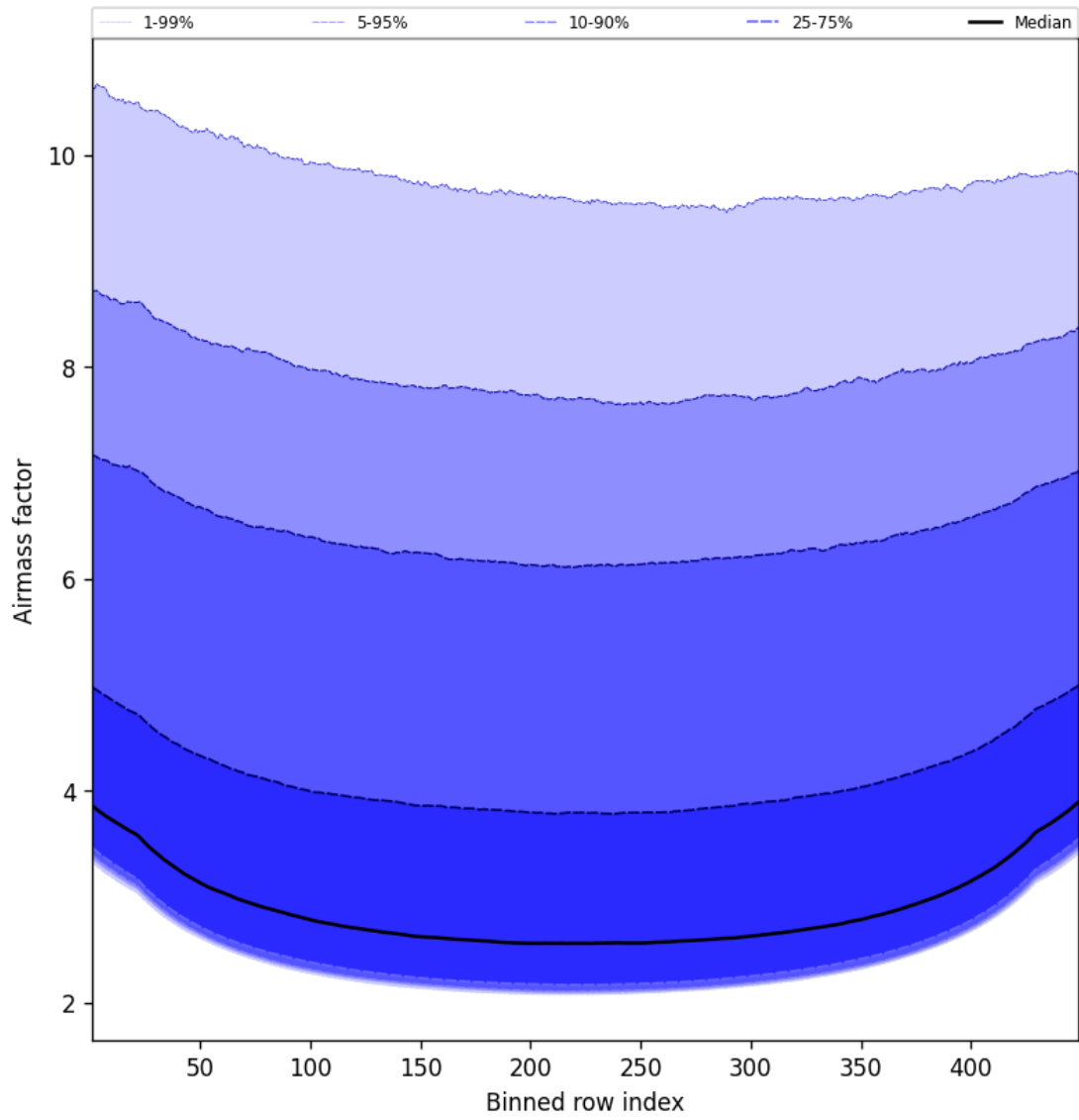
Figure 49: Along track statistics of “Airmass factor” for 2025-08-19 to 2025-08-20
