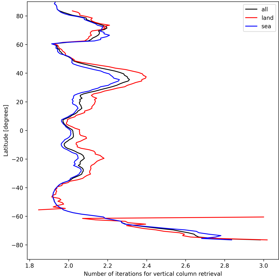
Figure 27: Zonal average of “Number of iterations for vertical column retrieval” for 2025-08-19 to 2025-08-20.
