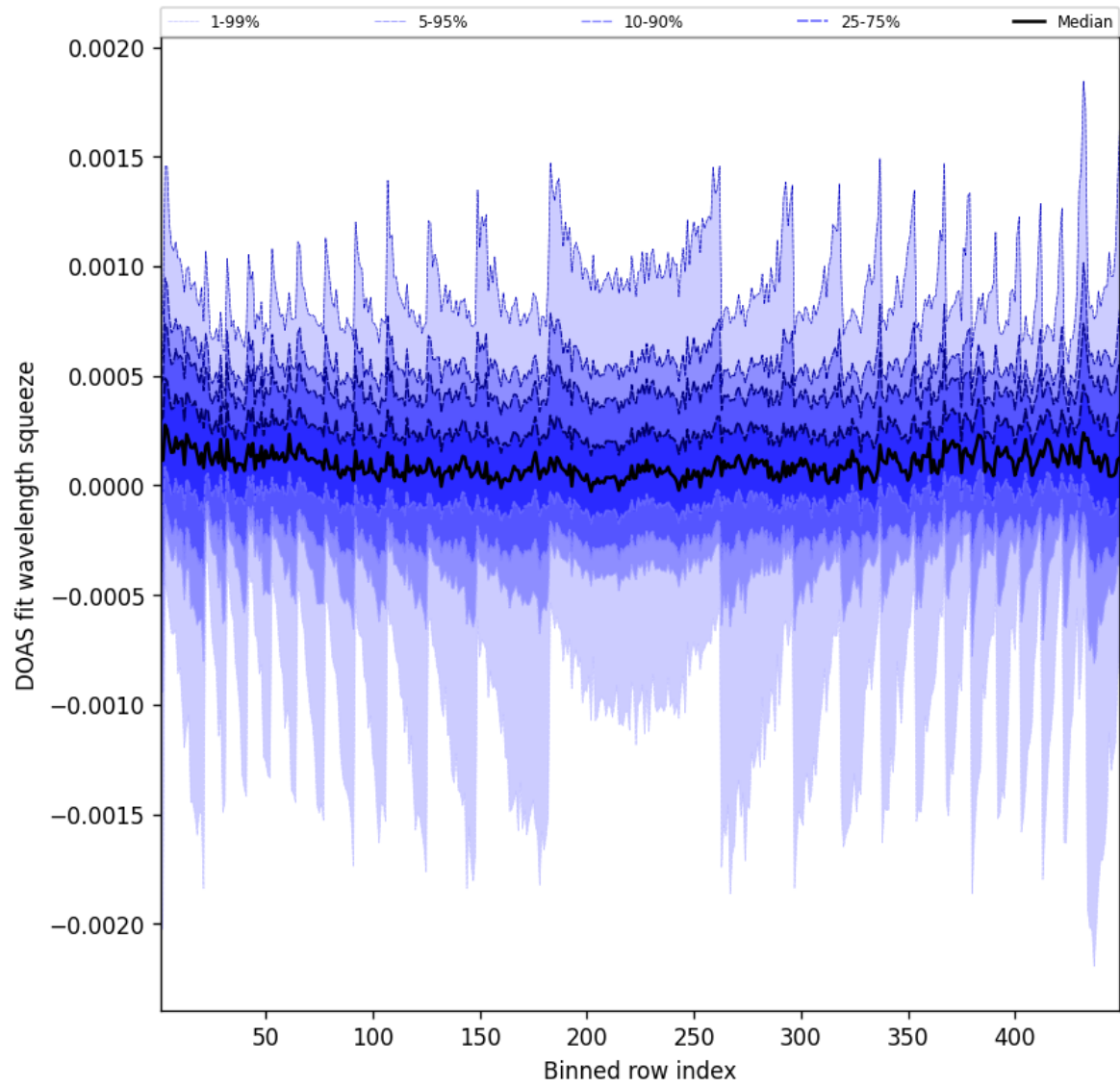
Figure 48: Along track statistics of “DOAS fit wavelength squeeze” for 2025-08-19 to 2025-08-20
