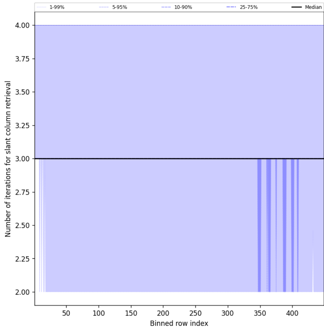
Figure 45: Along track statistics of “Number of iterations for slant column retrieval” for 2025-08-19 to 2025-08-20
