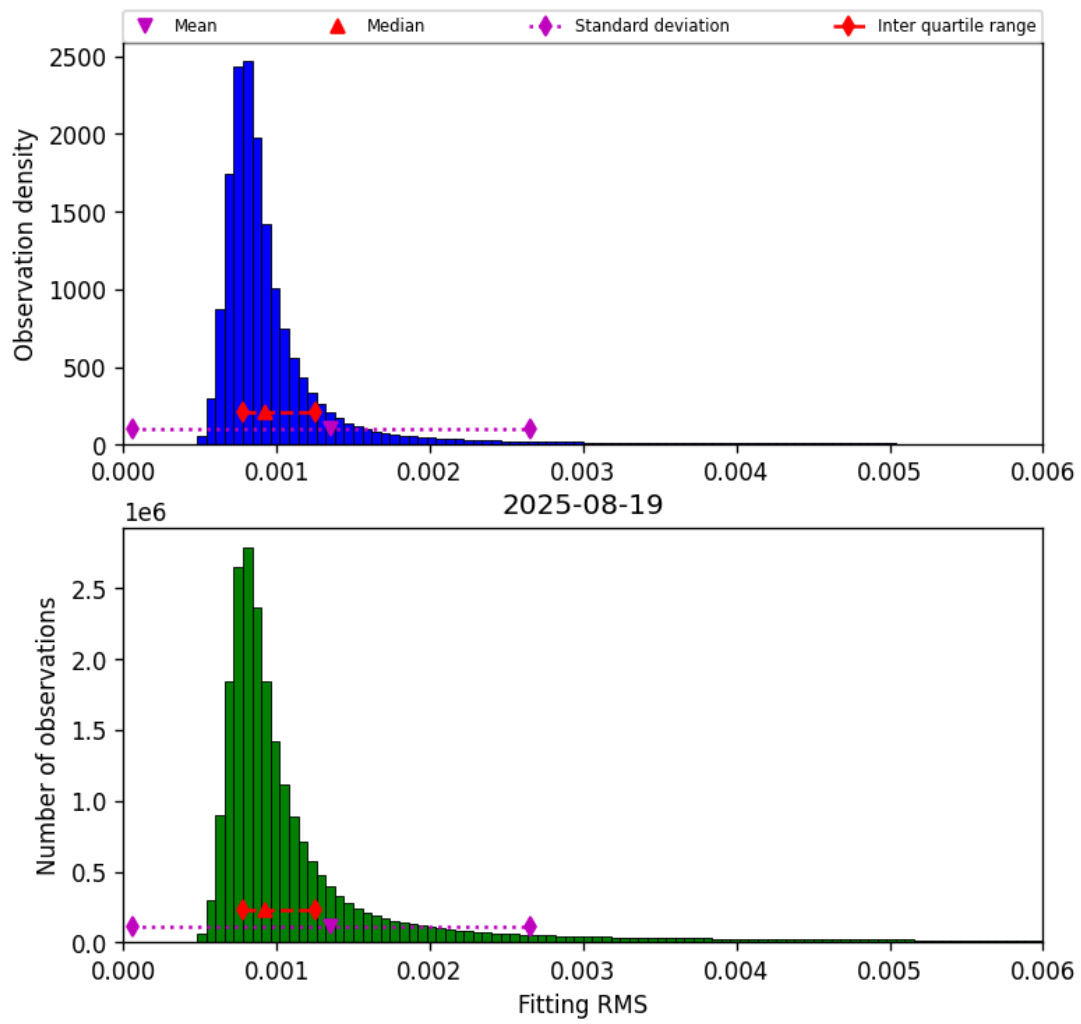
Figure 34: Histogram of “Fitting RMS” for 2025-08-19 to 2025-08-20
