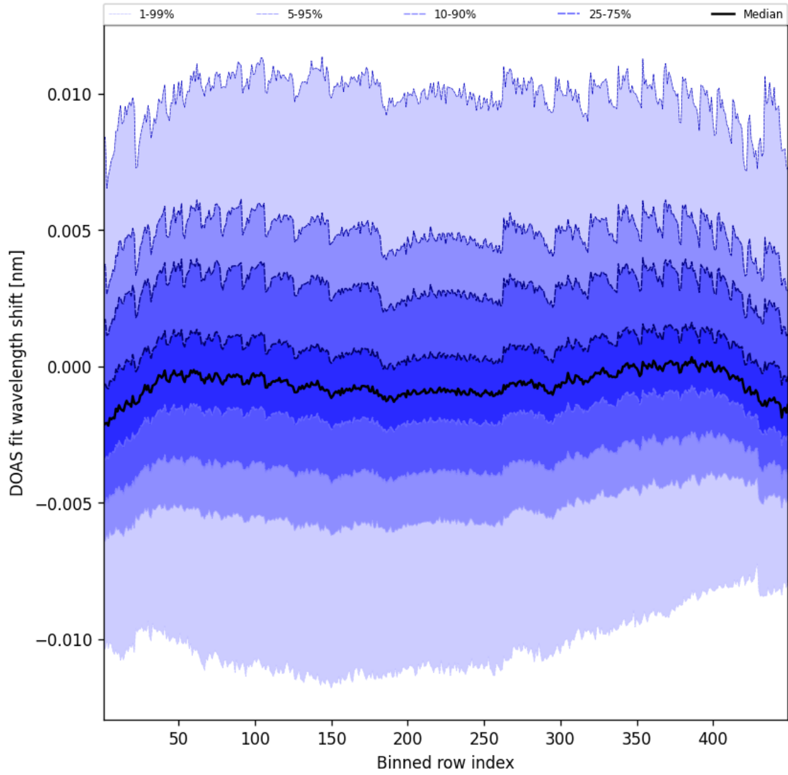
Figure 47: Along track statistics of “DOAS fit wavelength shift” for 2025-08-19 to 2025-08-20
