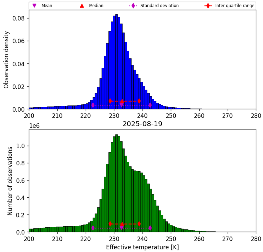
Figure 38: Histogram of “Effective temperature” for 2025-08-19 to 2025-08-20
