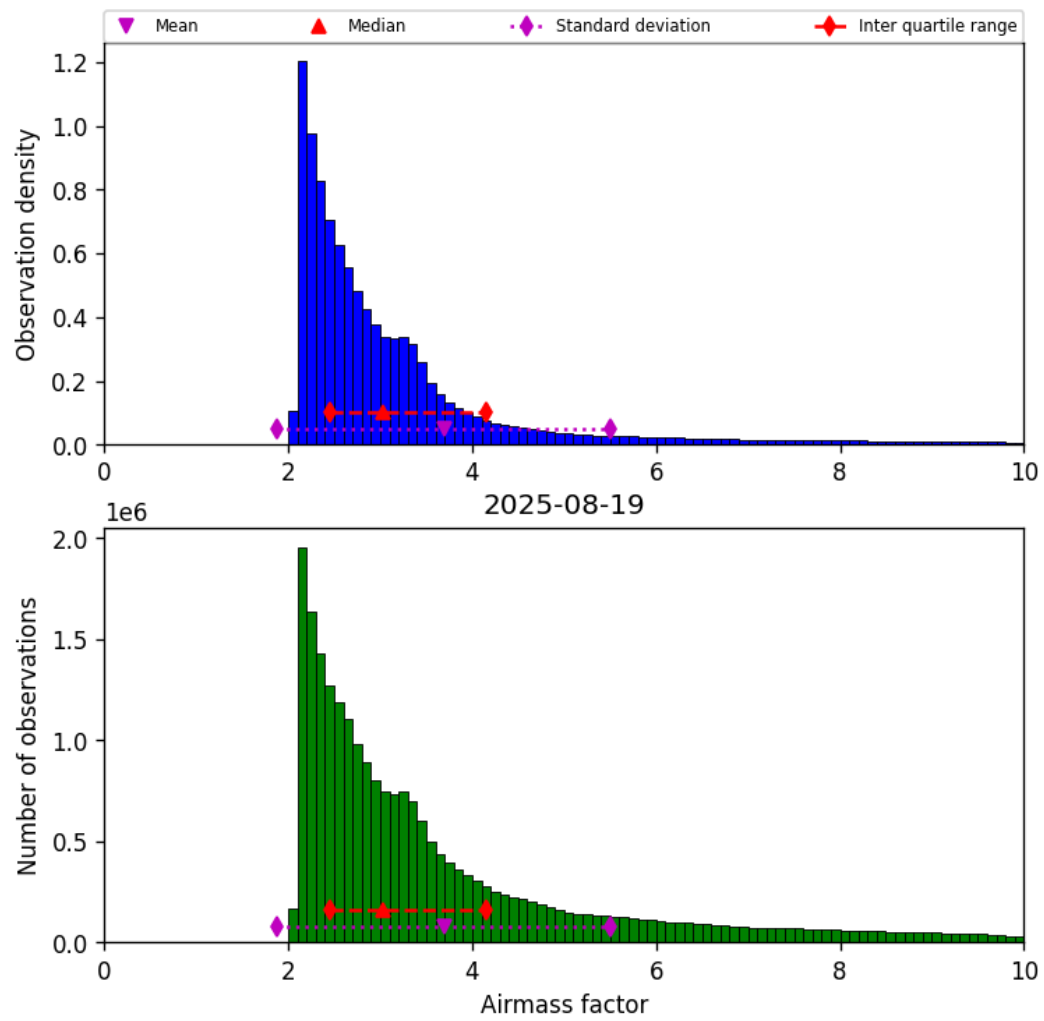
Figure 37: Histogram of “Airmass factor” for 2025-08-19 to 2025-08-20
