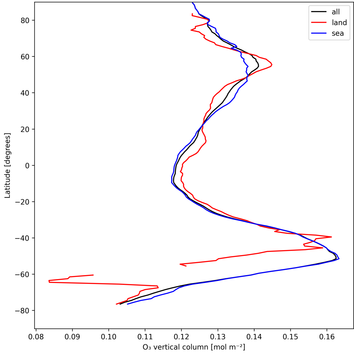
Figure 17: Zonal average of “O 3 vertical column” for 2025-08-19 to 2025-08-20.
