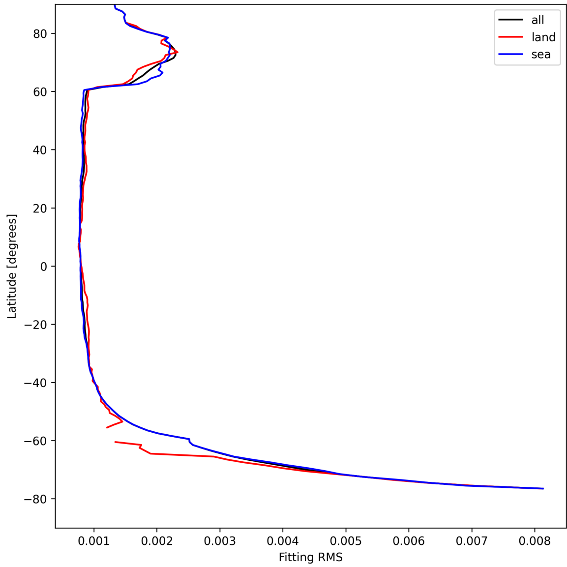
Figure 22: Zonal average of “Fitting RMS” for 2025-08-19 to 2025-08-20.
