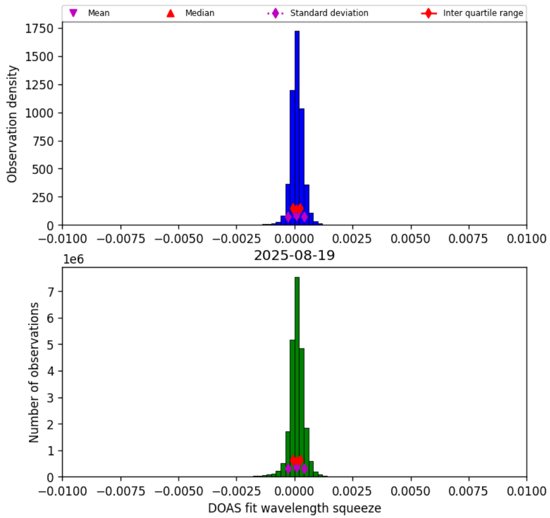
Figure 36: Histogram of “DOAS fit wavelength squeeze” for 2025-08-19 to 2025-08-20
