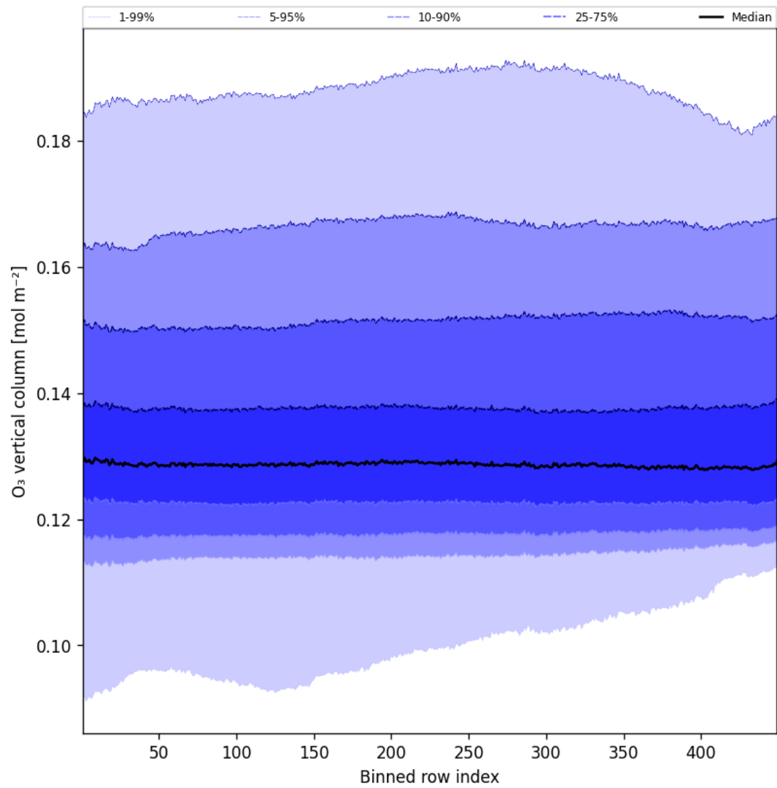
Figure 41: Along track statistics of “O 3 vertical column” for 2025-08-19 to 2025-08-20
