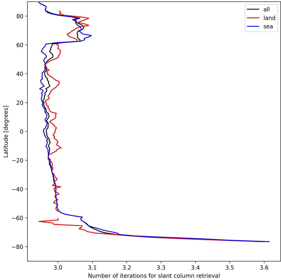
Figure 21: Zonal average of “Number of iterations for slant column retrieval” for 2025-08-19 to 2025-08-20.
