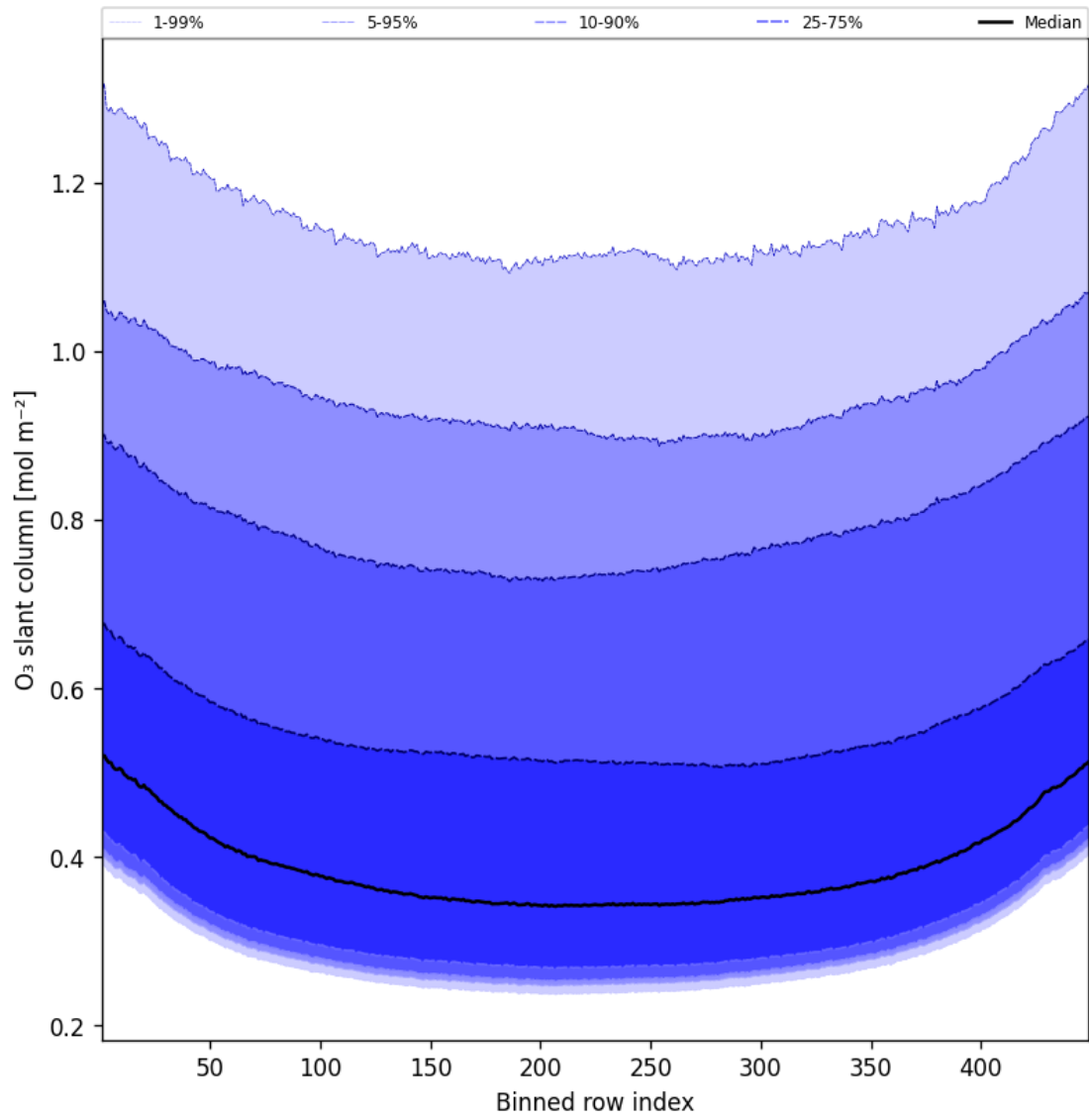
Figure 43: Along track statistics of “O 3 slant column” for 2025-08-19 to 2025-08-20
