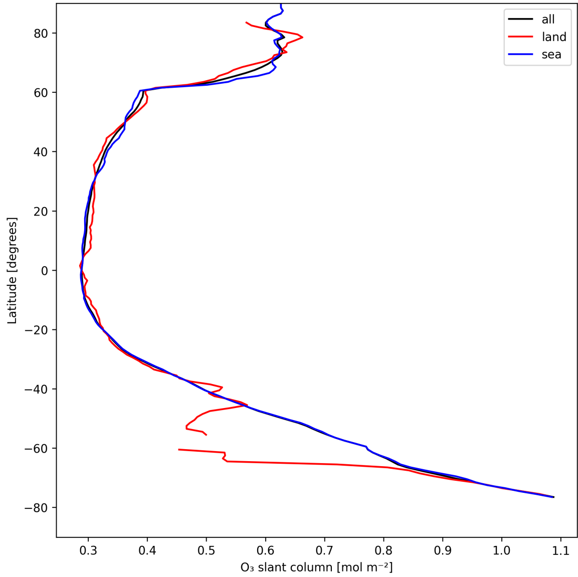
Figure 19: Zonal average of “O 3 slant column” for 2025-08-19 to 2025-08-20.
