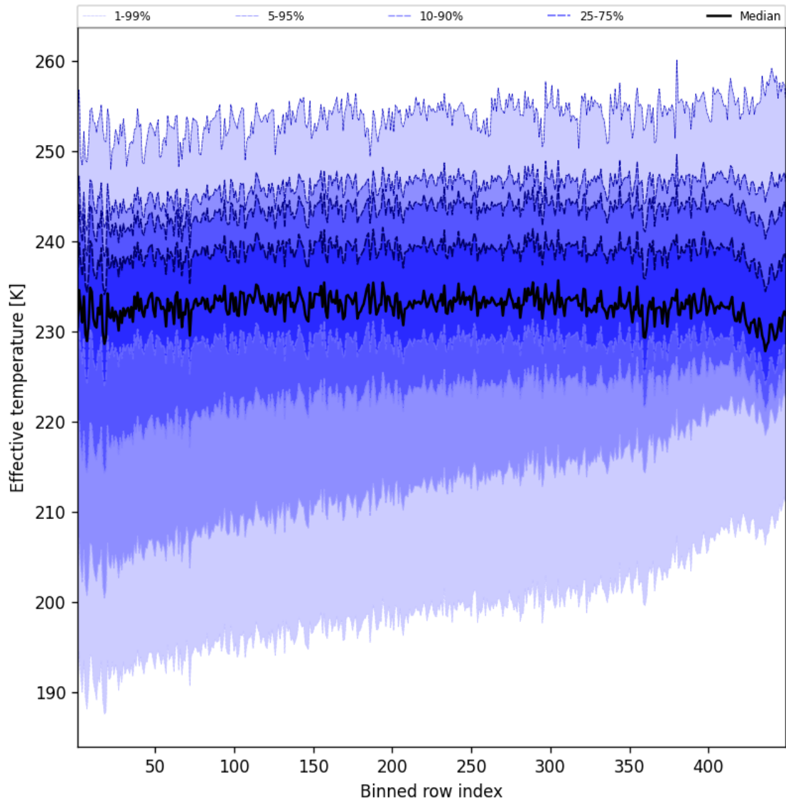
Figure 50: Along track statistics of “Effective temperature” for 2025-08-19 to 2025-08-20
