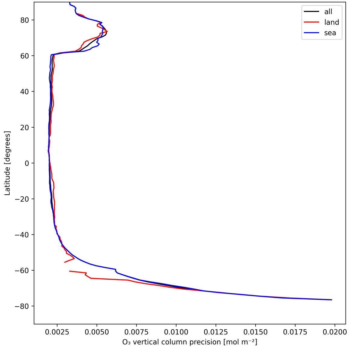
Figure 18: Zonal average of “O 3 vertical column precision” for 2025-08-19 to 2025-08-20.
