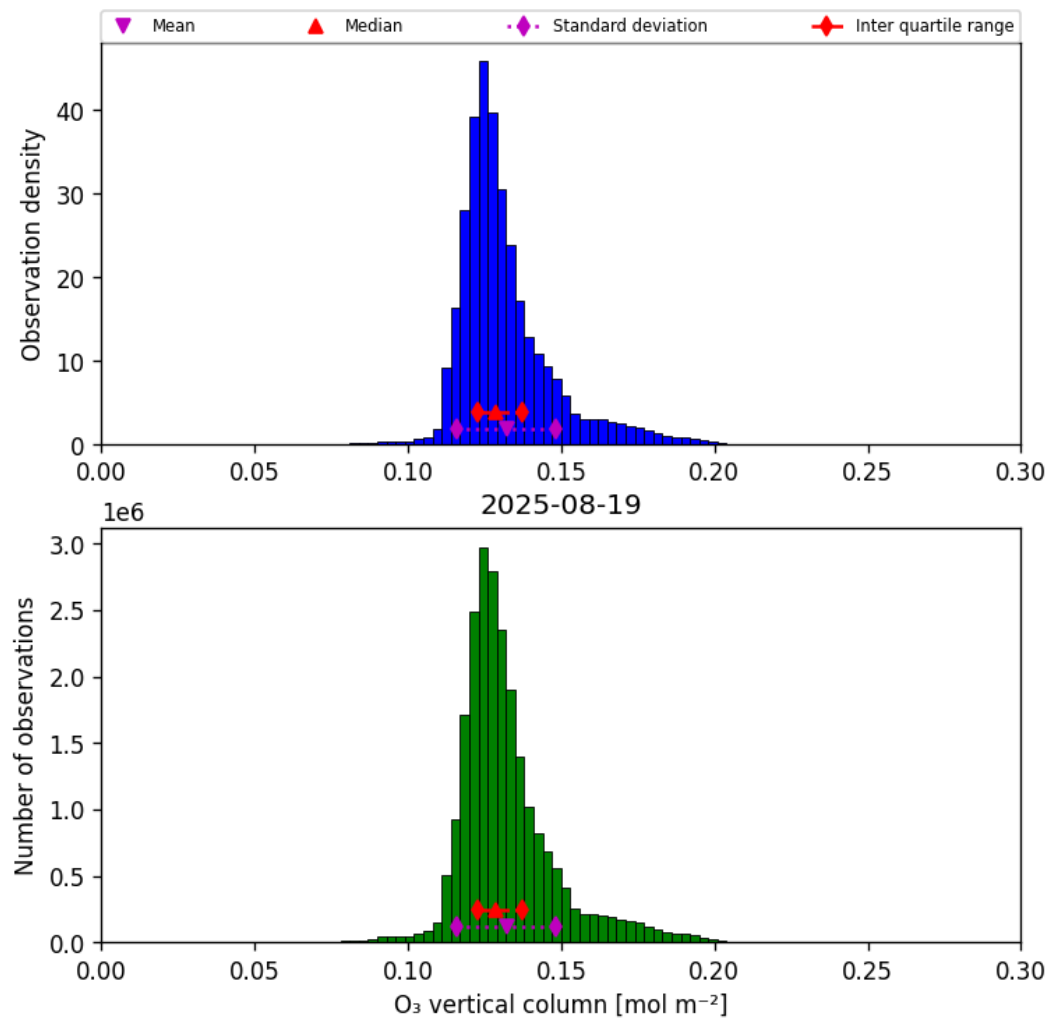
Figure 29: Histogram of “O 3 vertical column” for 2025-08-19 to 2025-08-20
