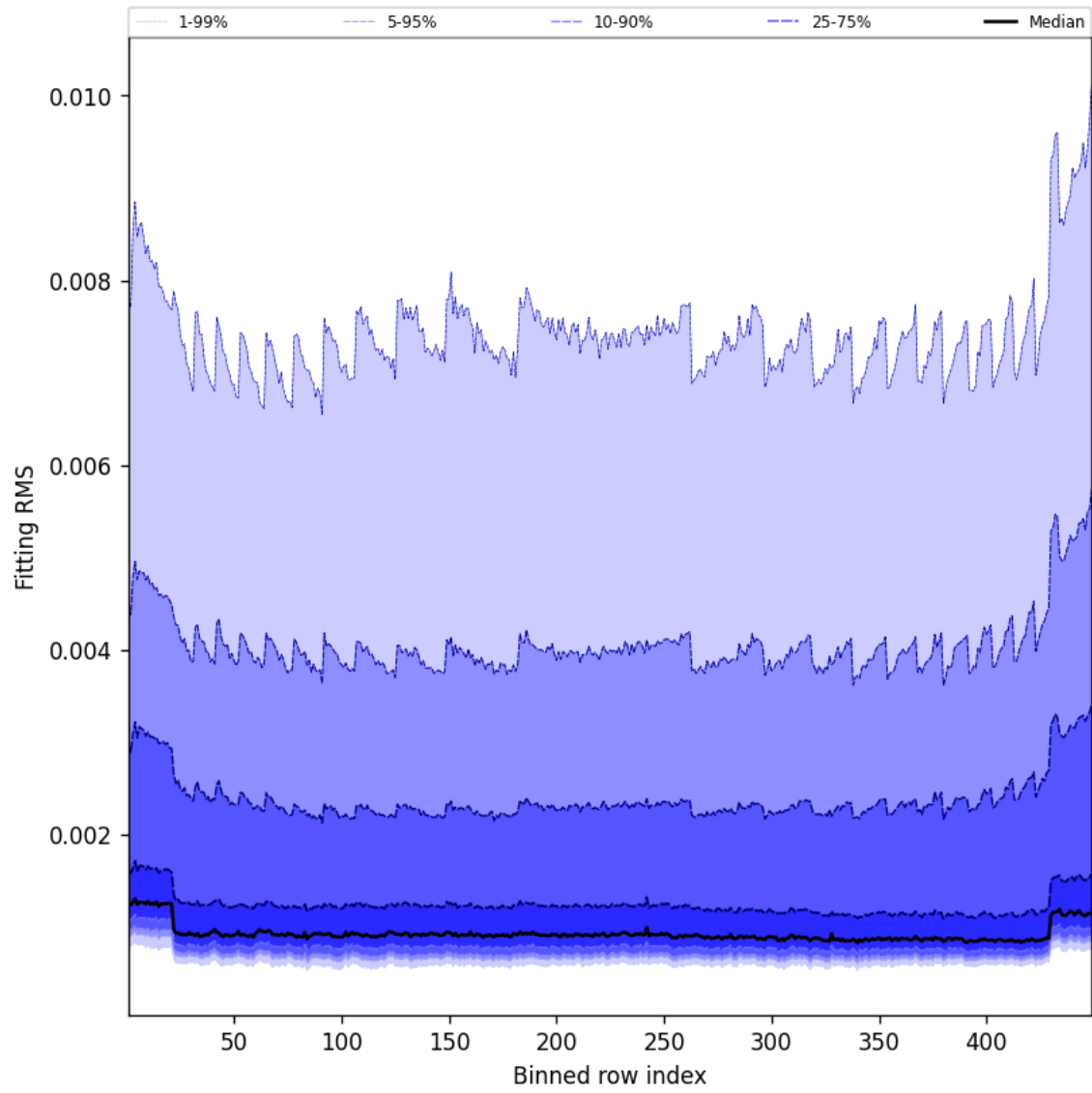
Figure 46: Along track statistics of “Fitting RMS” for 2025-08-19 to 2025-08-20
