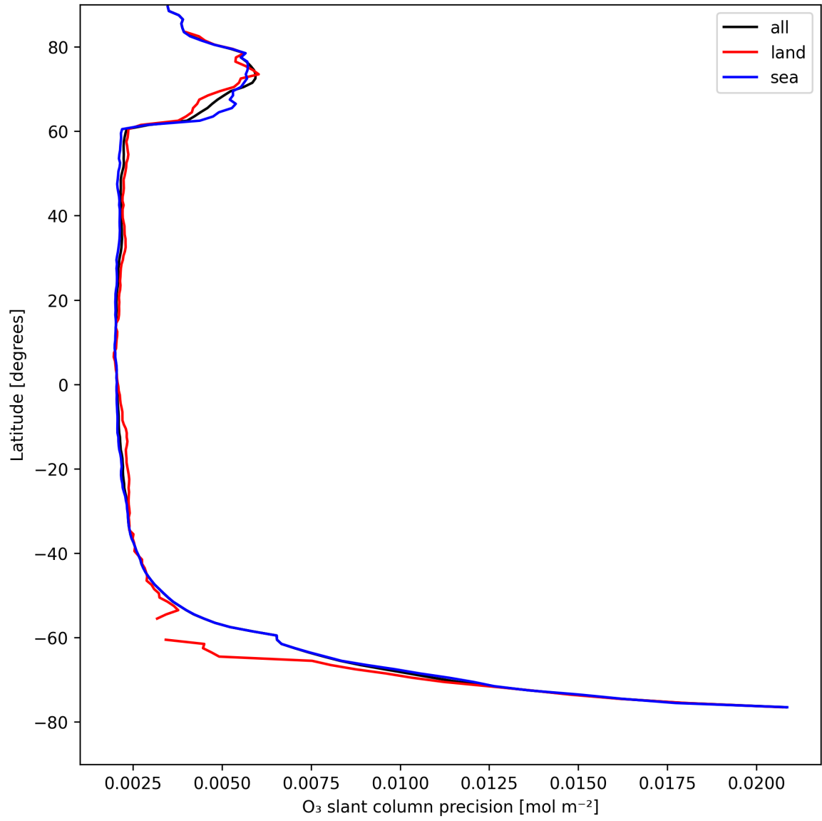
Figure 20: Zonal average of “O 3 slant column precision” for 2025-08-19 to 2025-08-20.
