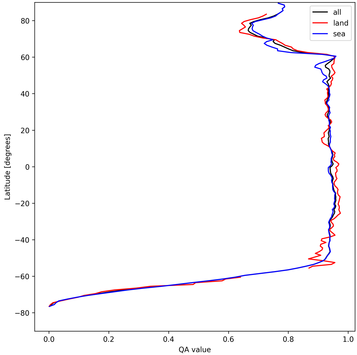
Figure 16: Zonal average of “QA value” for 2025-08-19 to 2025-08-20.
