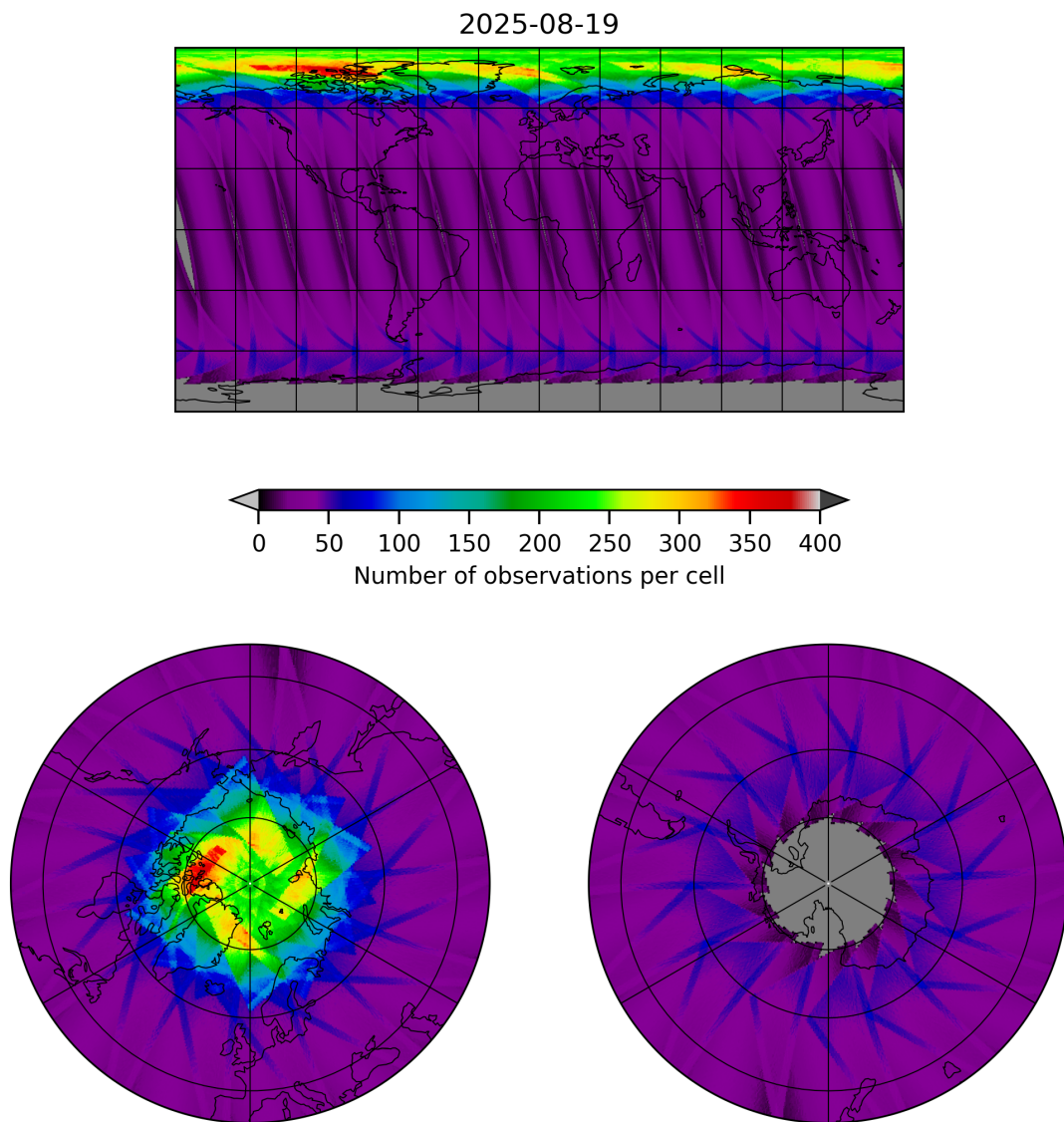
Figure 15: Map of the number of observations for 2025-08-19 to 2025-08-20
