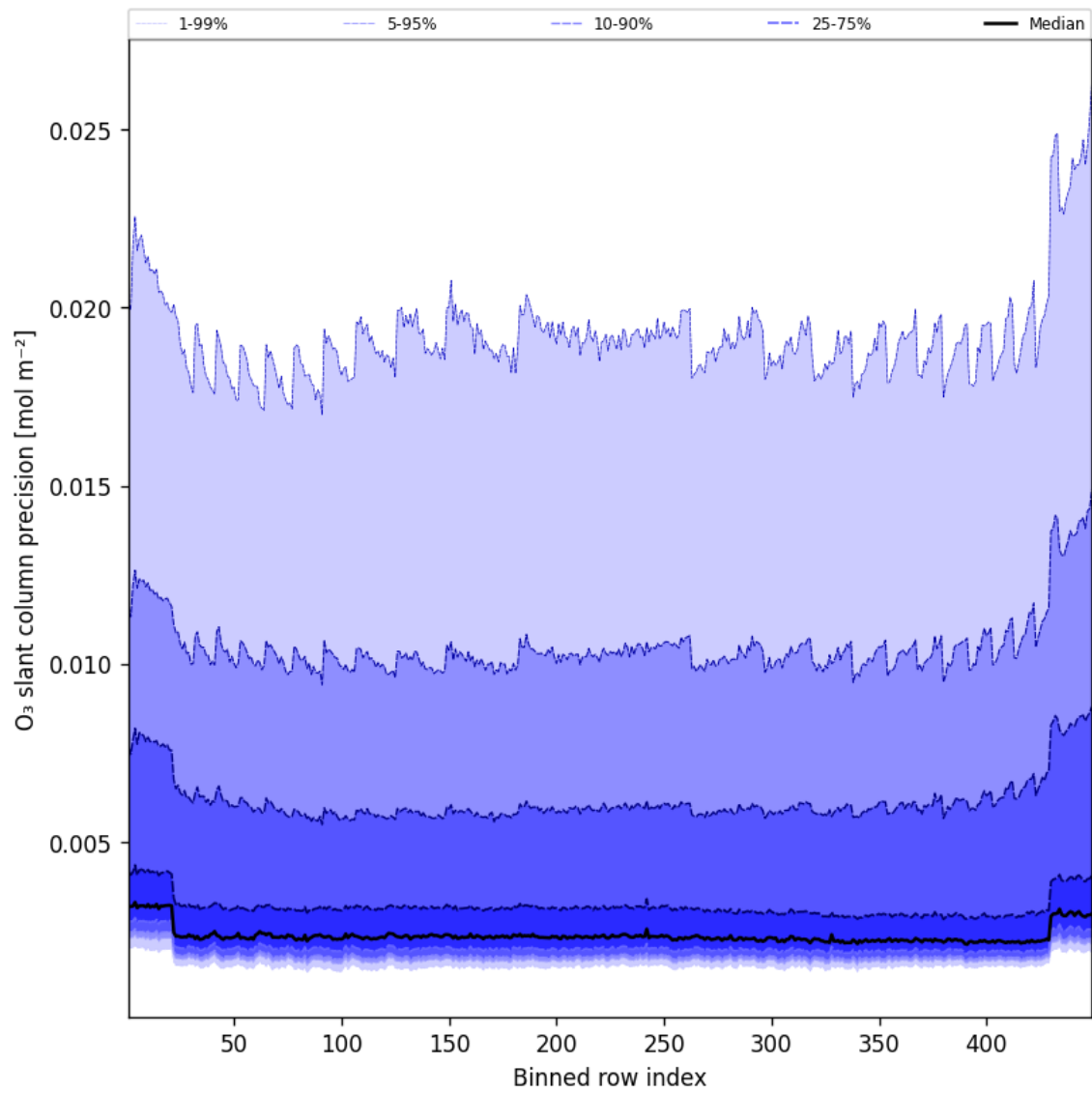
Figure 44: Along track statistics of “O 3 slant column precision” for 2025-08-19 to 2025-08-20
