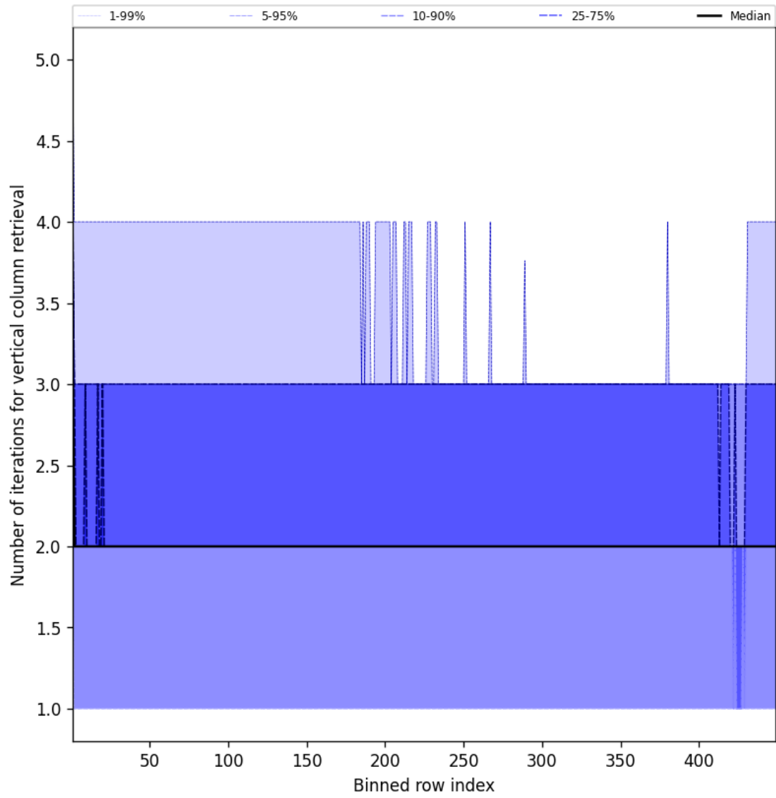
Figure 51: Along track statistics of “Number of iterations for vertical column retrieval” for 2025-08-19 to 2025-08-20
