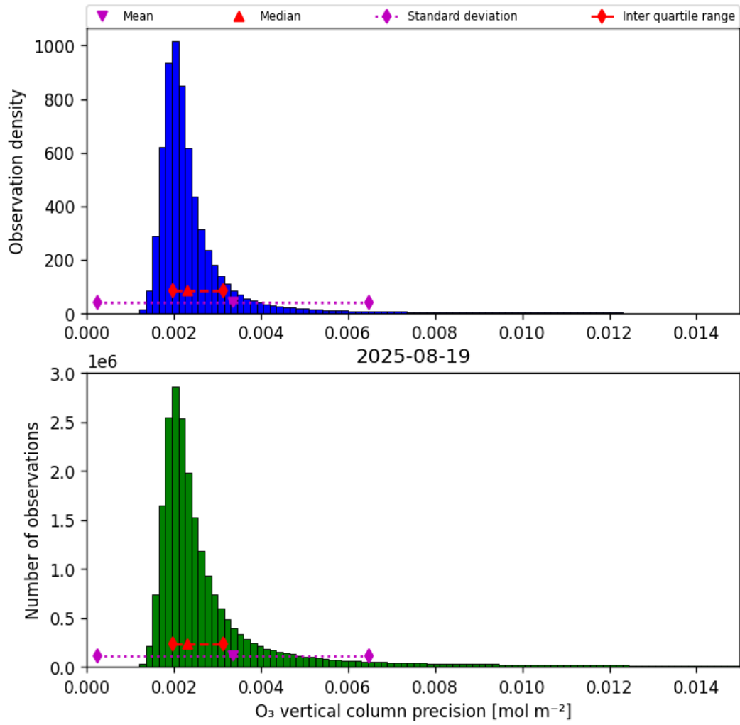
Figure 30: Histogram of “O 3 vertical column precision” for 2025-08-19 to 2025-08-20
