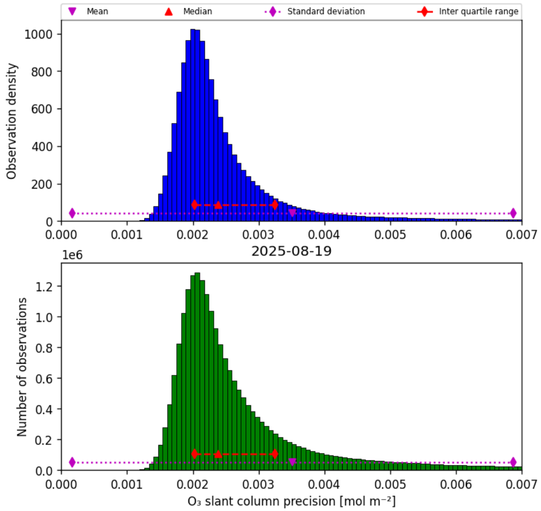
Figure 32: Histogram of “O 3 slant column precision” for 2025-08-19 to 2025-08-20
