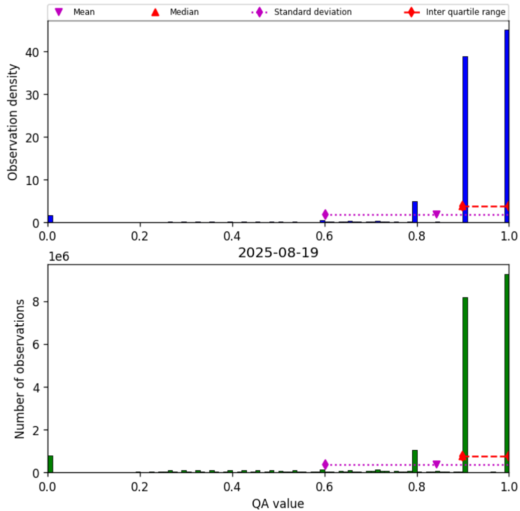
Figure 28: Histogram of “QA value” for 2025-08-19 to 2025-08-20
