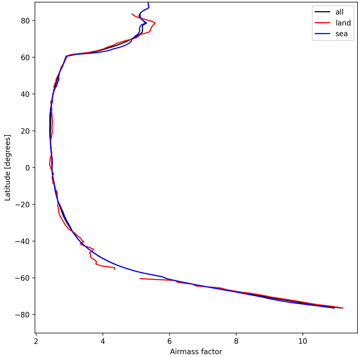
Figure 25: Zonal average of “Airmass factor” for 2025-08-19 to 2025-08-20.
