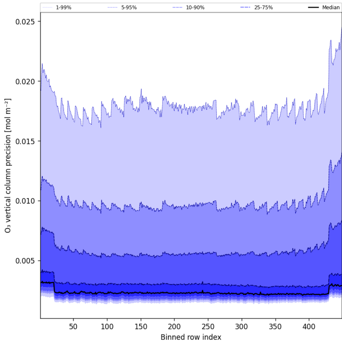
Figure 42: Along track statistics of “O 3 vertical column precision” for 2025-08-19 to 2025-08-20
