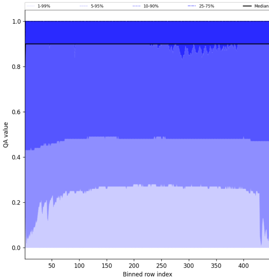
Figure 40: Along track statistics of “QA value” for 2025-08-19 to 2025-08-20
