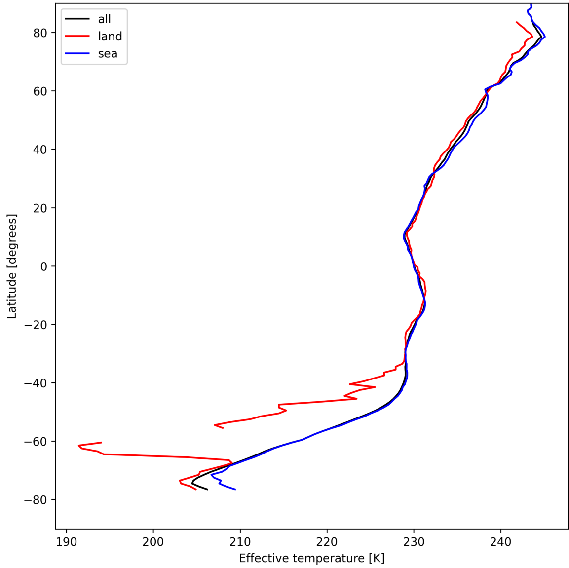
Figure 26: Zonal average of "Effective temperature" for 2025-08-19 to 2025-08-20.
