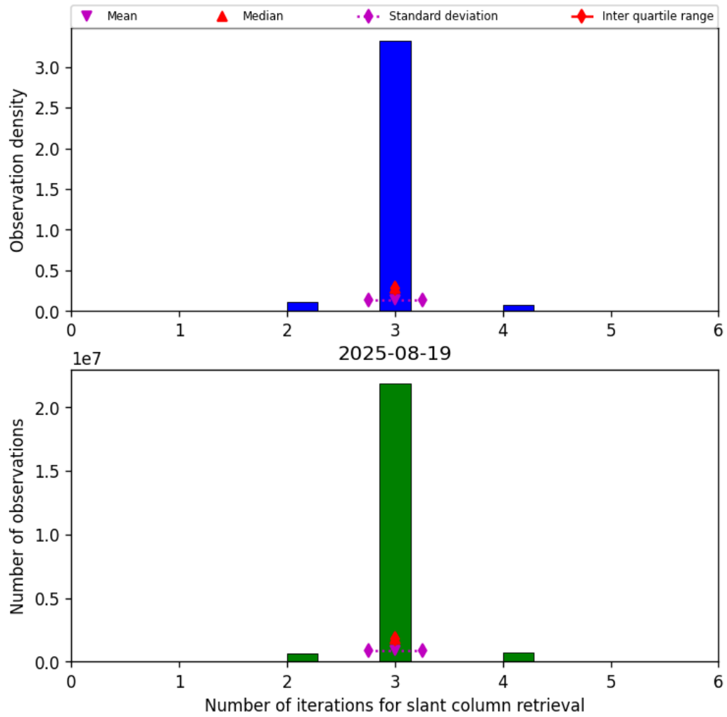
Figure 33: Histogram of “Number of iterations for slant column retrieval” for 2025-08-19 to 2025-08-20
