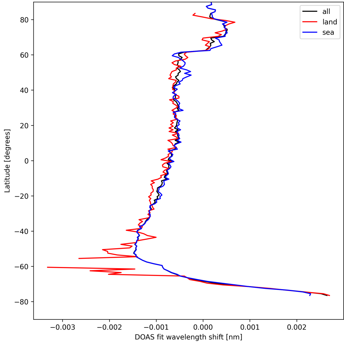
Figure 23: Zonal average of “DOAS fit wavelength shift” for 2025-08-19 to 2025-08-20.
