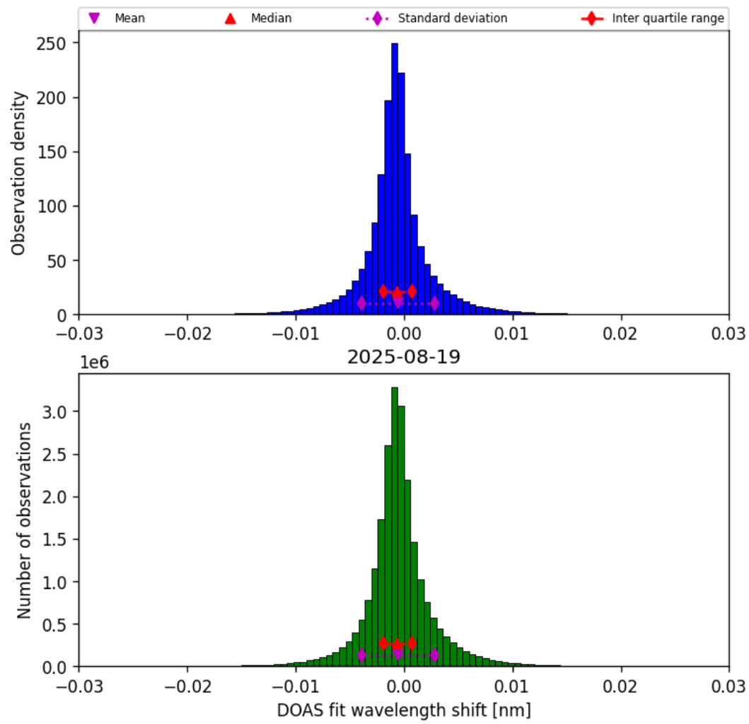
Figure 35: Histogram of “DOAS fit wavelength shift” for 2025-08-19 to 2025-08-20
