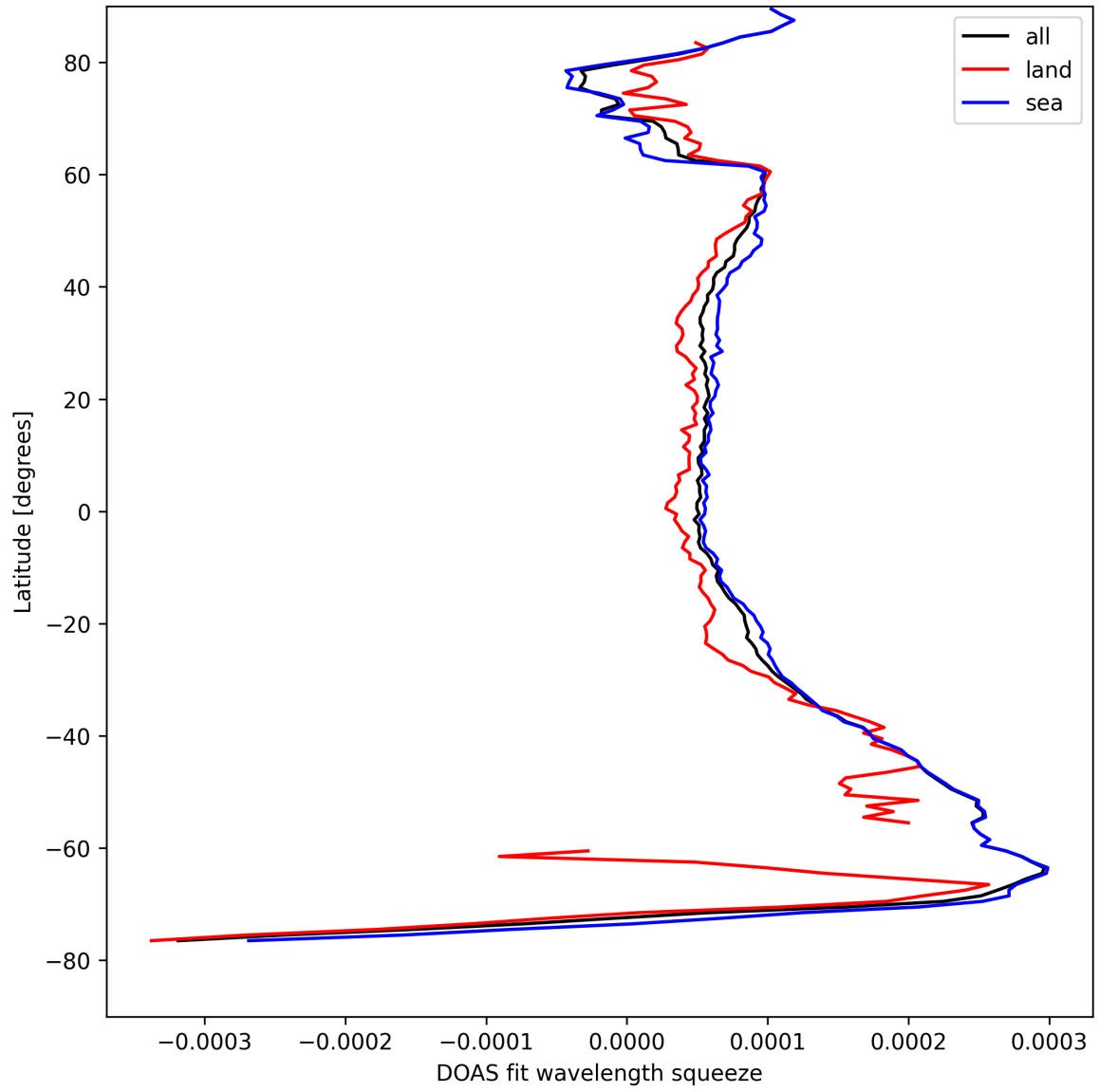
Figure 24: Zonal average of “DOAS fit wavelength squeeze” for 2025-08-19 to 2025-08-20.
