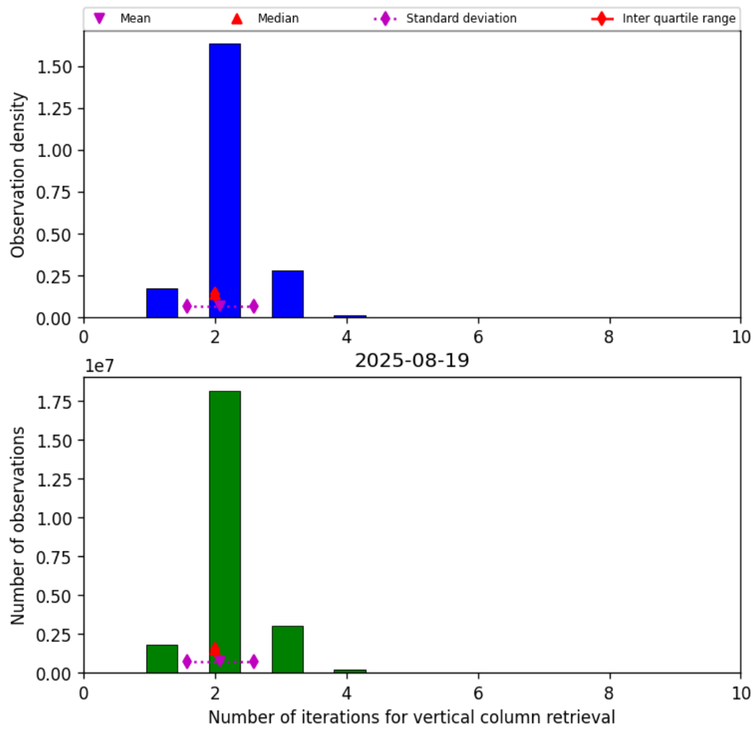
Figure 39: Histogram of “Number of iterations for vertical column retrieval” for 2025-08-19 to 2025-08-20
