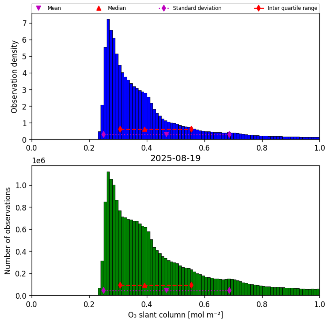
Figure 31: Histogram of “O 3 slant column” for 2025-08-19 to 2025-08-20
