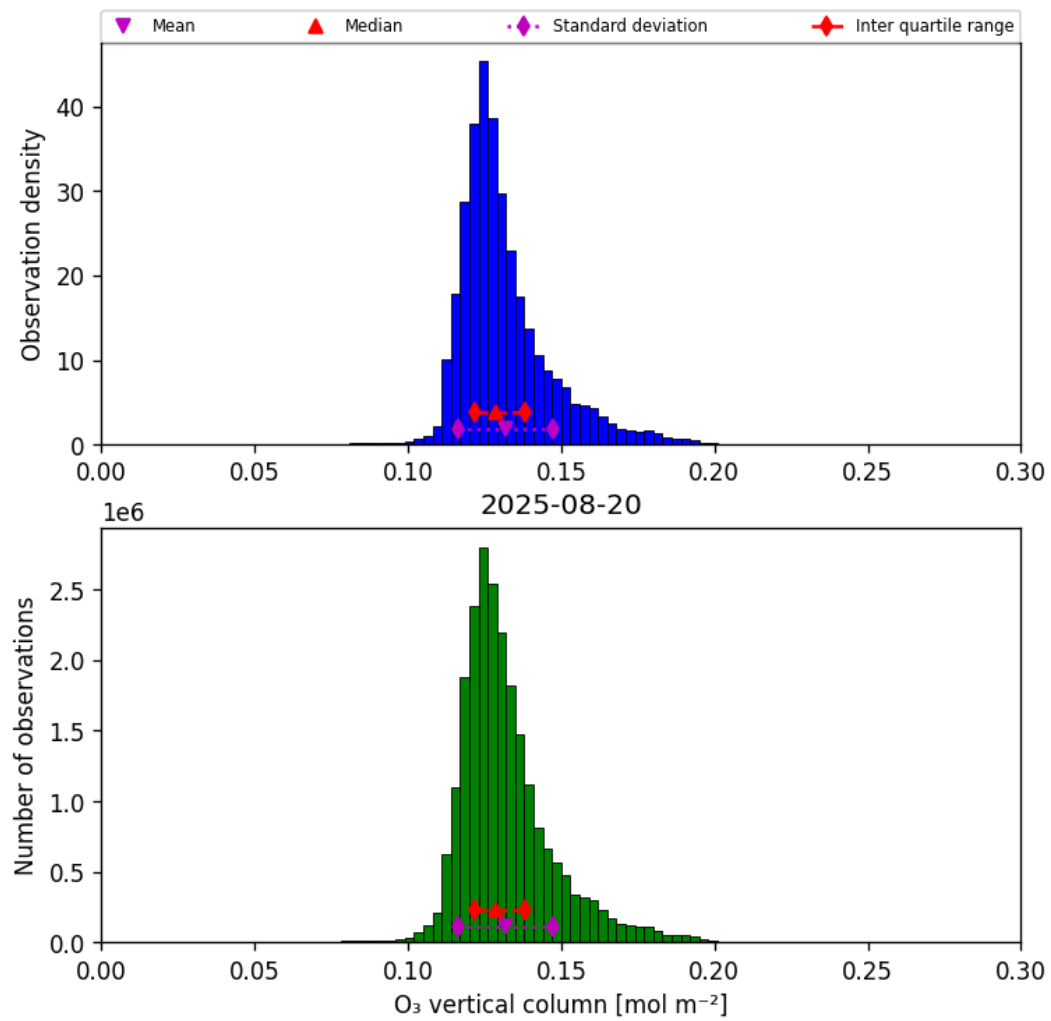
Figure 29: Histogram of “O 3 vertical column” for 2025-08-20 to 2025-08-21
