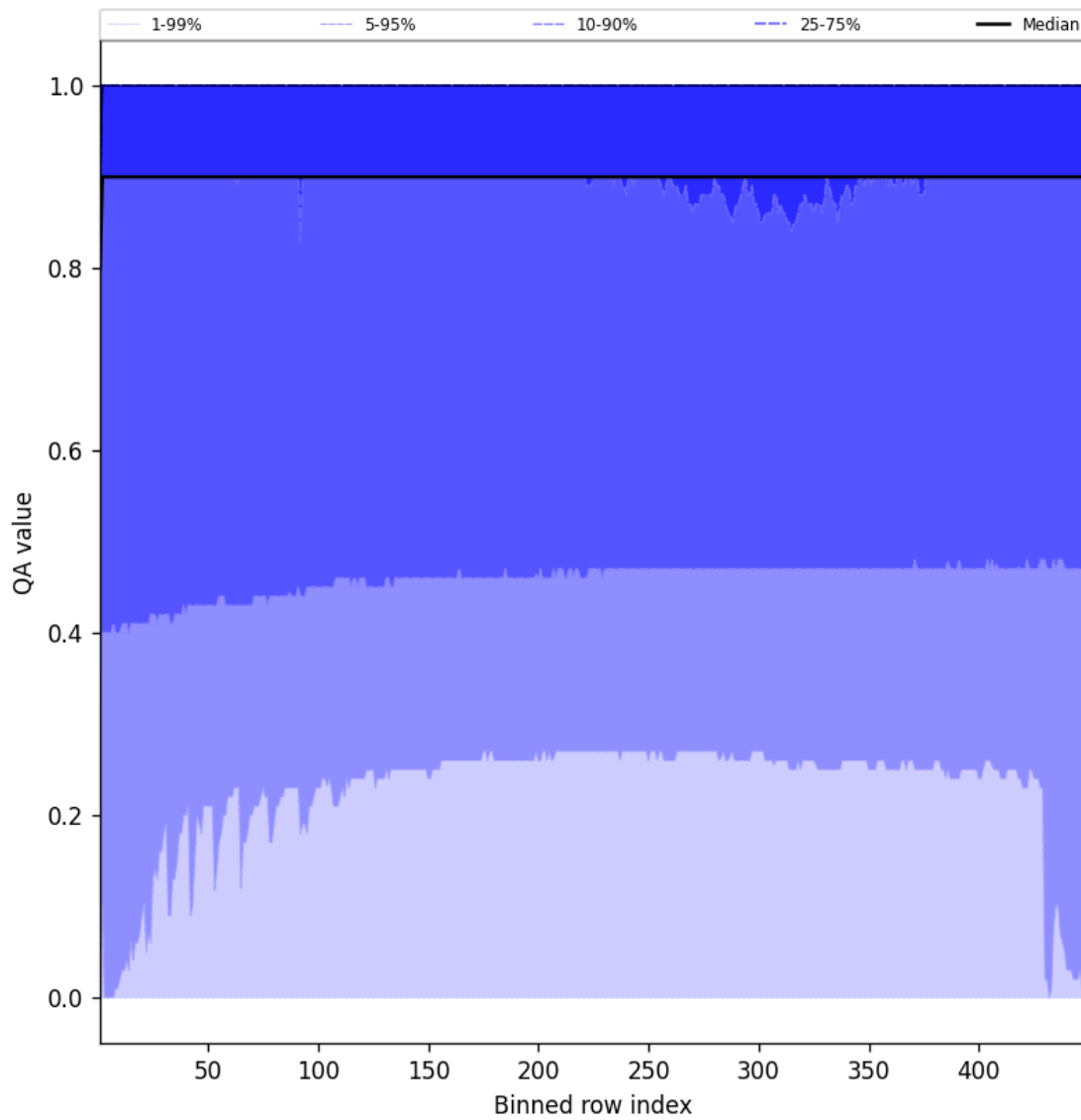
Figure 40: Along track statistics of “QA value” for 2025-08-20 to 2025-08-21
