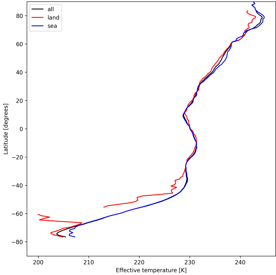
Figure 26: Zonal average of "Effective temperature" for 2025-08-20 to 2025-08-21.
