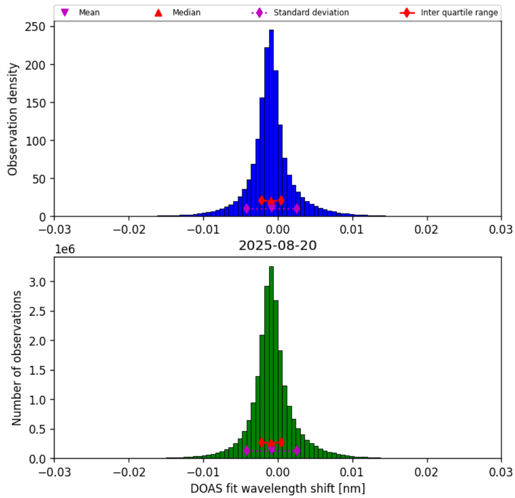
Figure 35: Histogram of “DOAS fit wavelength shift” for 2025-08-20 to 2025-08-21
