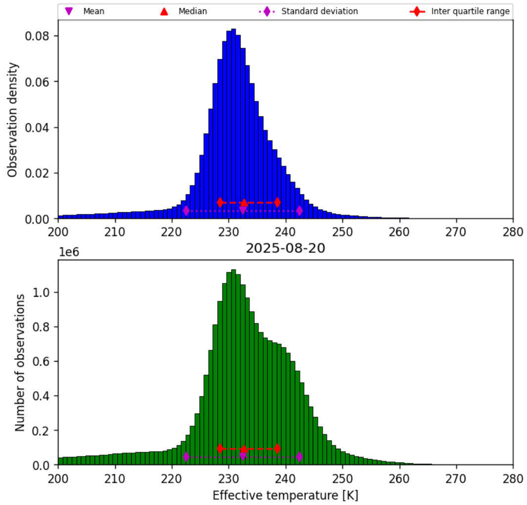
Figure 38: Histogram of “Effective temperature” for 2025-08-20 to 2025-08-21
