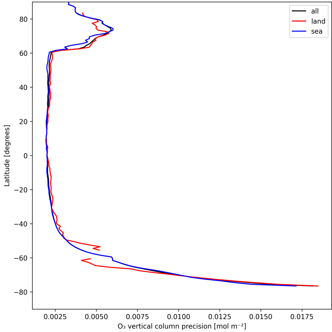
Figure 18: Zonal average of “O 3 vertical column precision” for 2025-08-20 to 2025-08-21.
