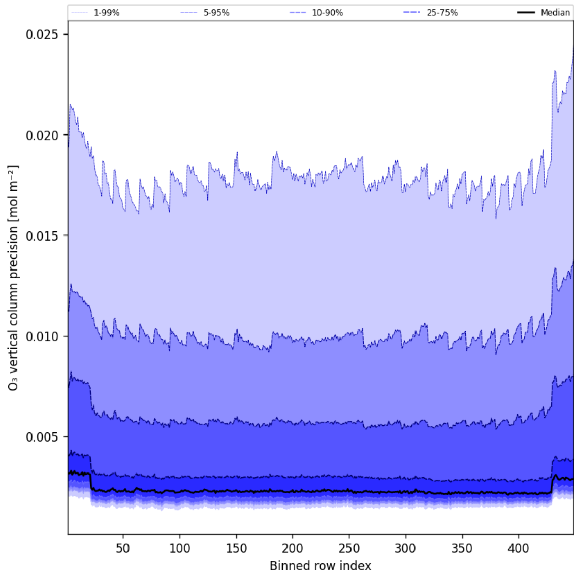
Figure 42: Along track statistics of “O 3 vertical column precision” for 2025-08-20 to 2025-08-21
