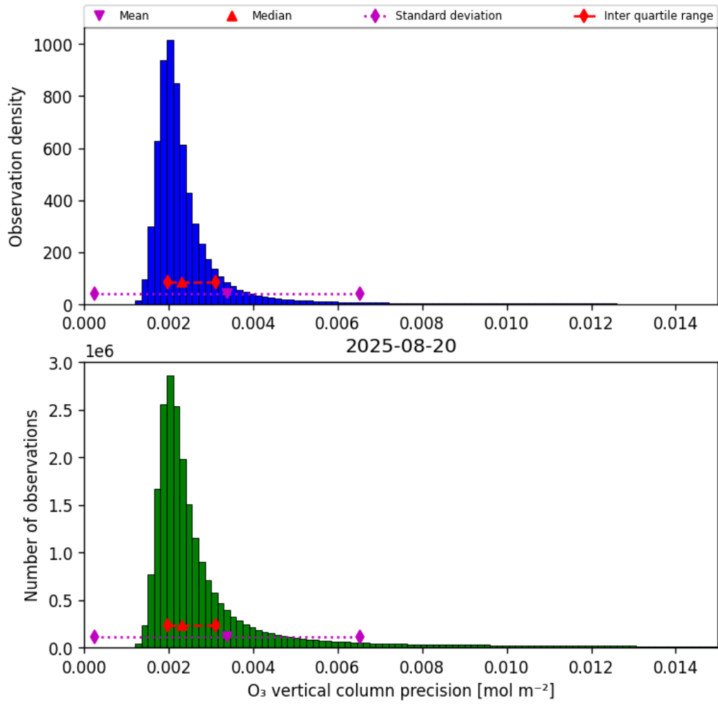
Figure 30: Histogram of “O 3 vertical column precision” for 2025-08-20 to 2025-08-21
