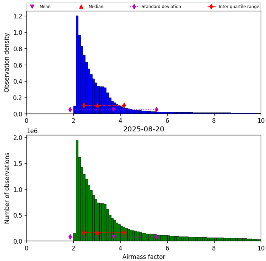
Figure 37: Histogram of “Airmass factor” for 2025-08-20 to 2025-08-21
