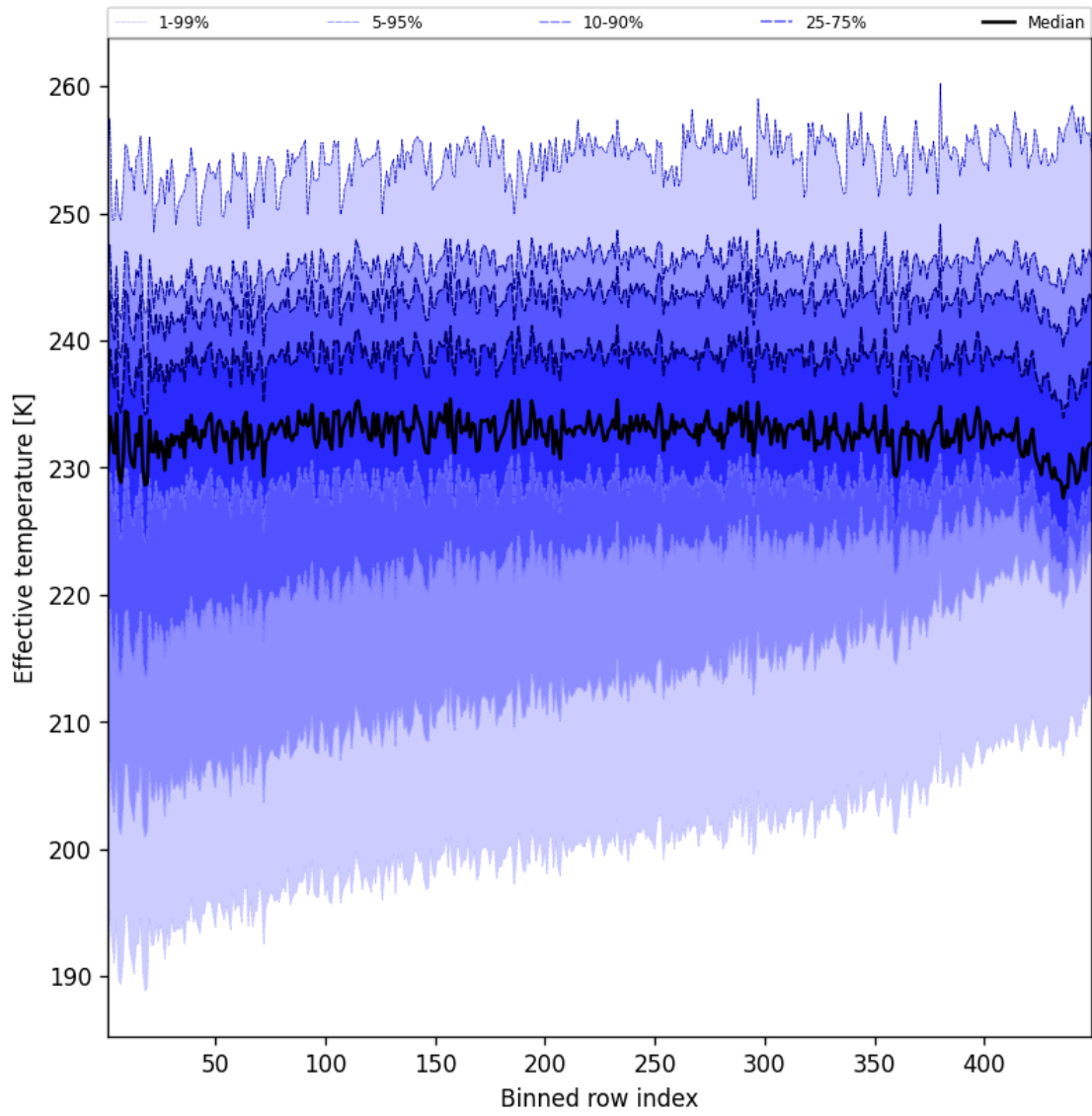
Figure 50: Along track statistics of “Effective temperature” for 2025-08-20 to 2025-08-21
