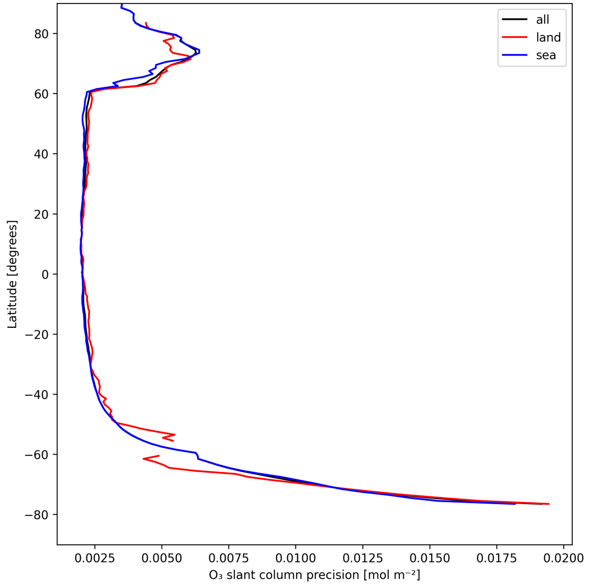
Figure 20: Zonal average of “O 3 slant column precision” for 2025-08-20 to 2025-08-21.
