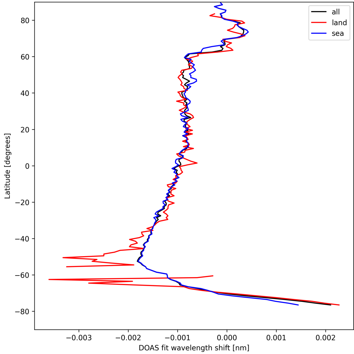
Figure 23: Zonal average of “DOAS fit wavelength shift” for 2025-08-20 to 2025-08-21.
