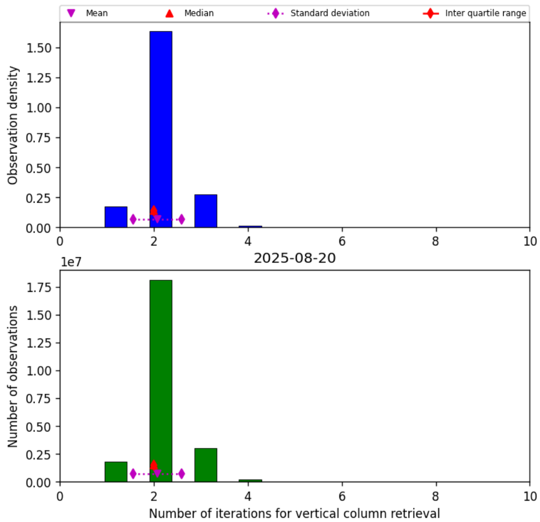
Figure 39: Histogram of “Number of iterations for vertical column retrieval” for 2025-08-20 to 2025-08-21
