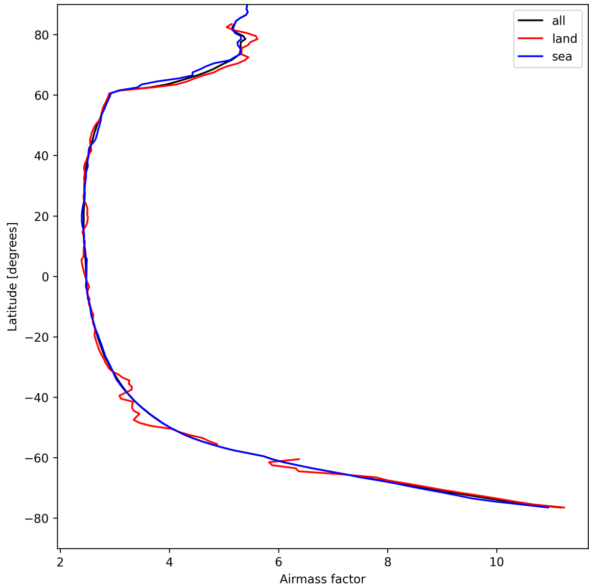
Figure 25: Zonal average of “Airmass factor” for 2025-08-20 to 2025-08-21.
