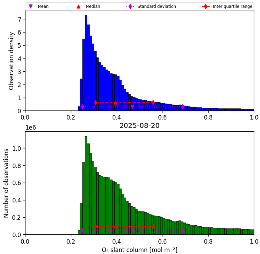
Figure 31: Histogram of “O 3 slant column” for 2025-08-20 to 2025-08-21
