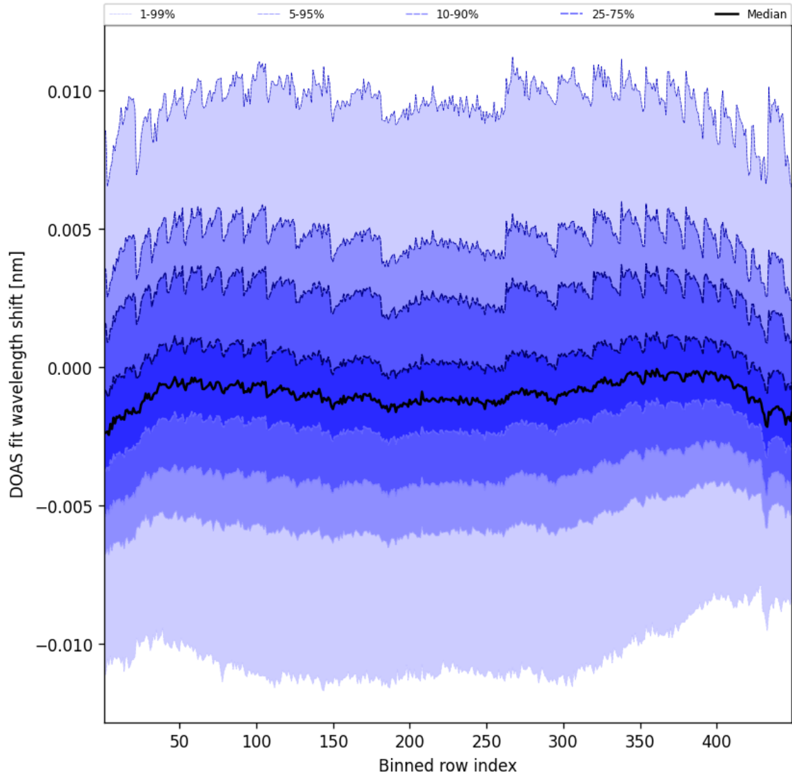
Figure 47: Along track statistics of “DOAS fit wavelength shift” for 2025-08-20 to 2025-08-21
