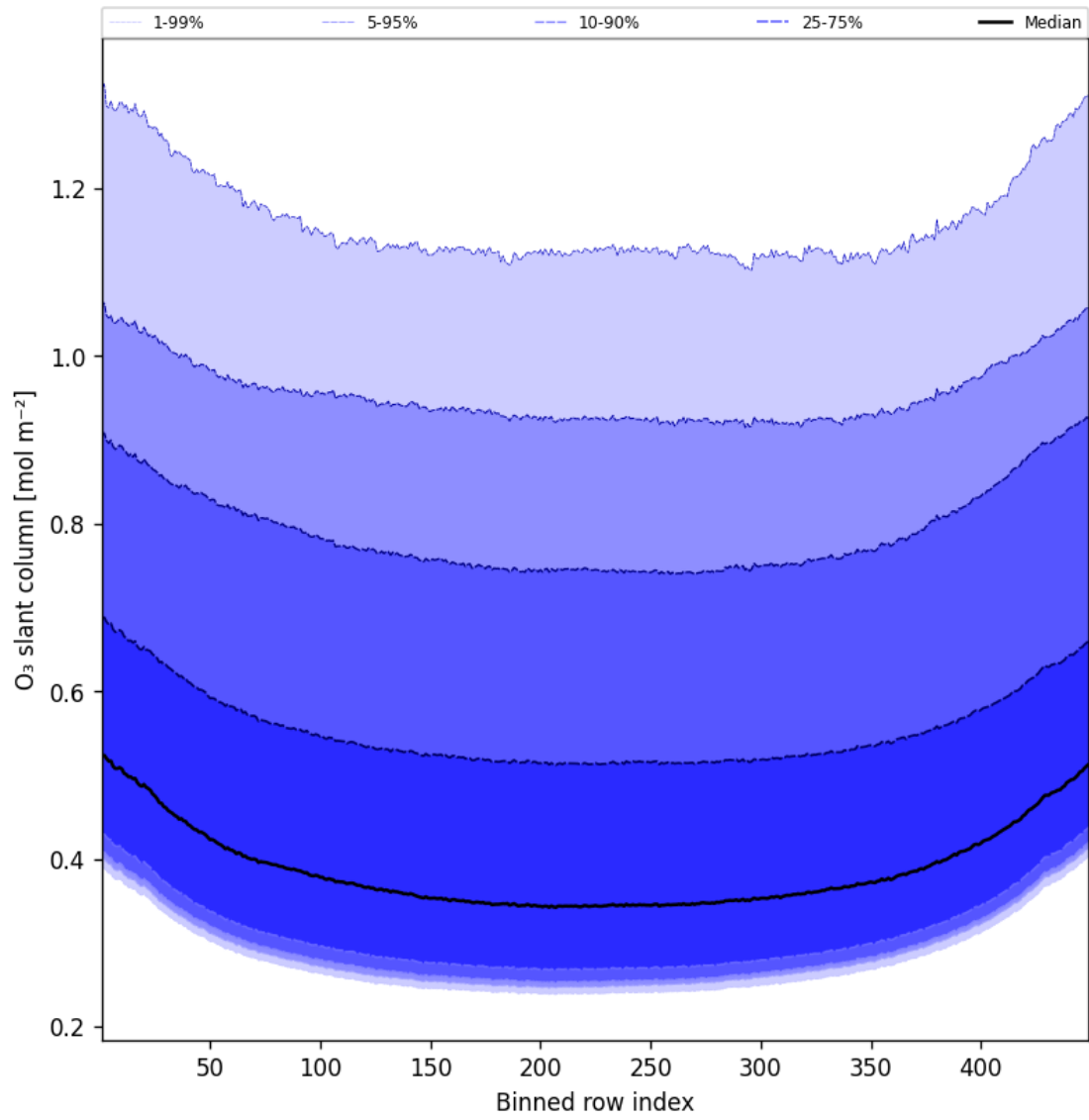
Figure 43: Along track statistics of "O 3 slant column" for 2025-08-20 to 2025-08-21
