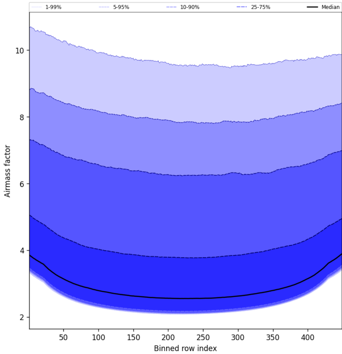
Figure 49: Along track statistics of “Airmass factor” for 2025-08-20 to 2025-08-21
