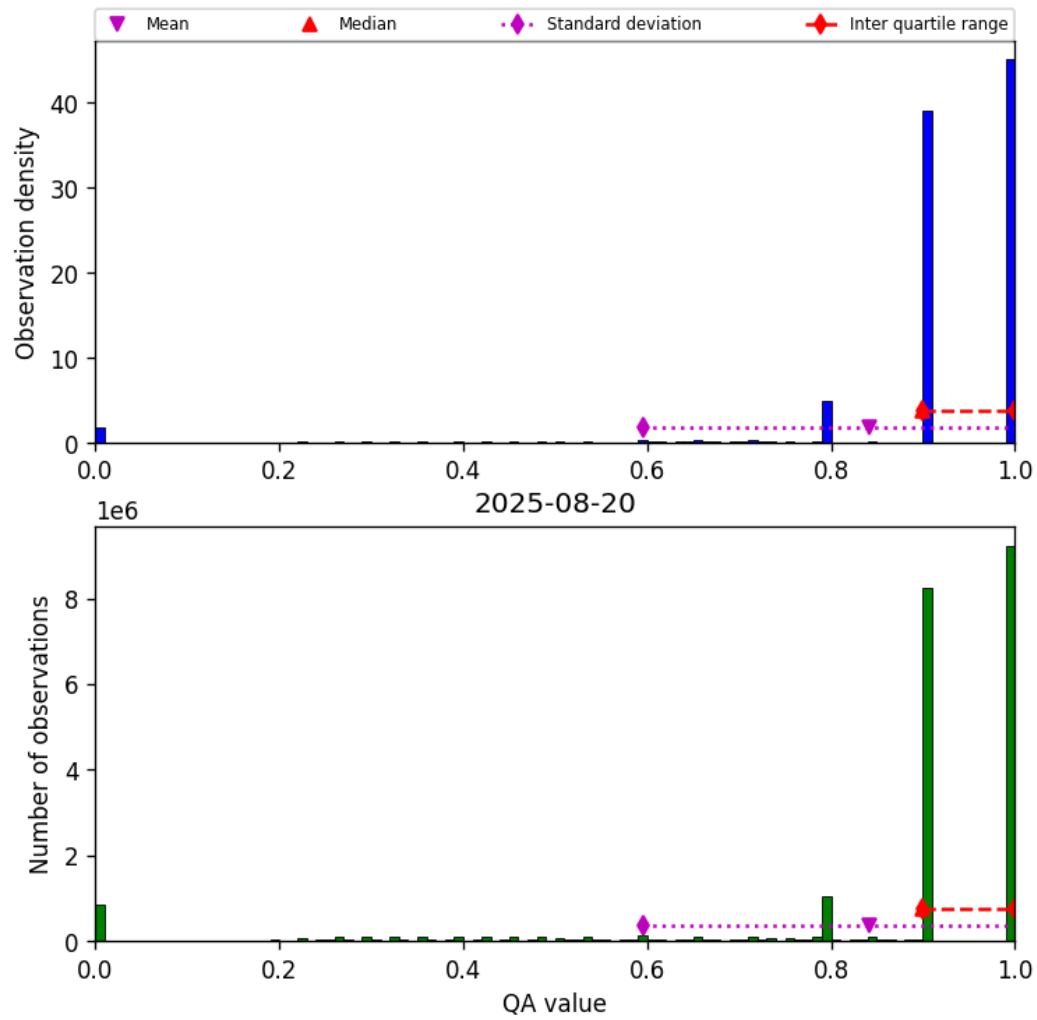
Figure 28: Histogram of “QA value” for 2025-08-20 to 2025-08-21
