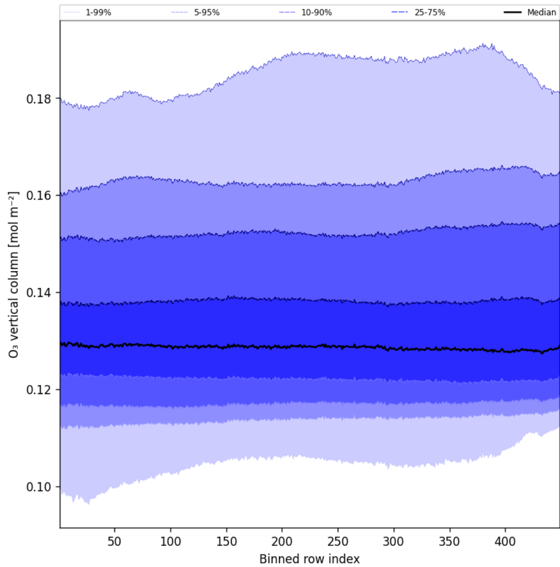
Figure 41: Along track statistics of “O 3 vertical column” for 2025-08-20 to 2025-08-21
