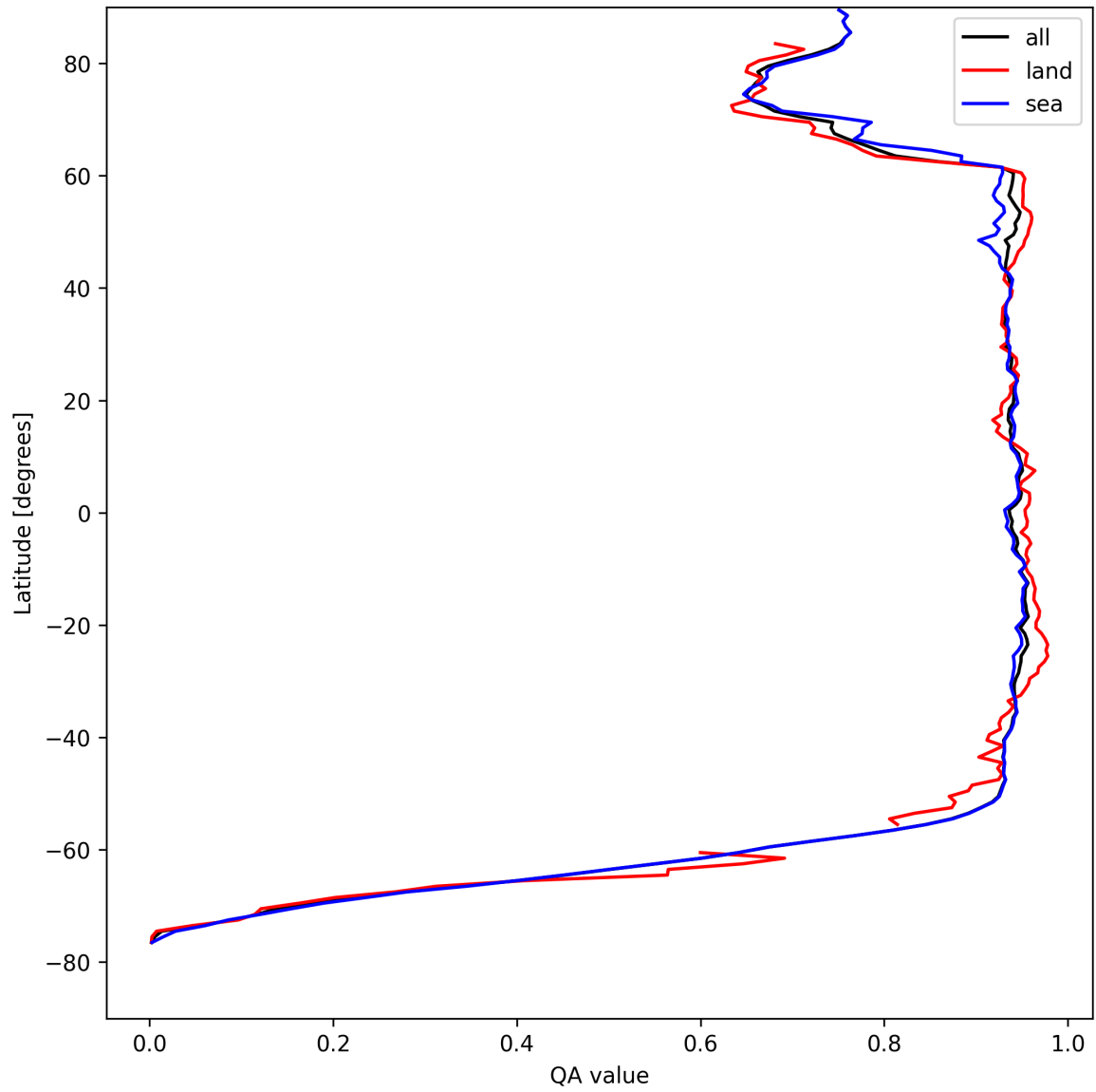
Figure 16: Zonal average of “QA value” for 2025-08-20 to 2025-08-21.
