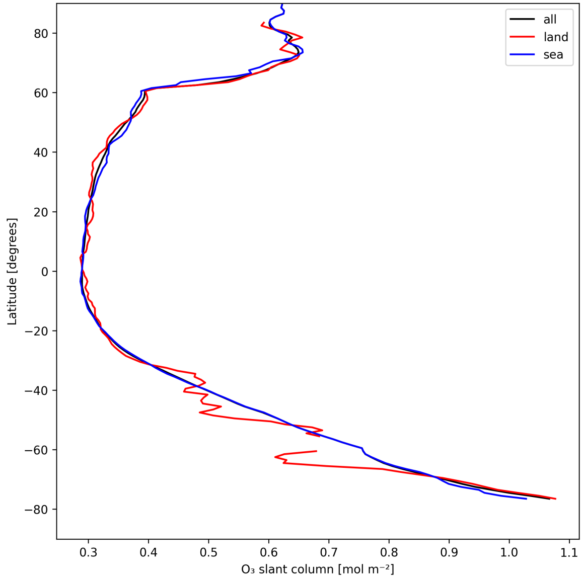
Figure 19: Zonal average of “O 3 slant column” for 2025-08-20 to 2025-08-21.
