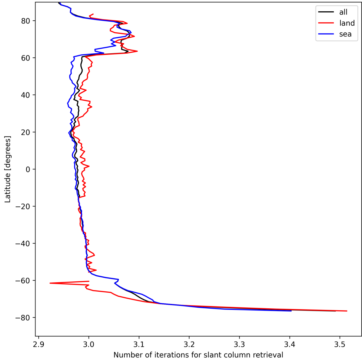
Figure 21: Zonal average of “Number of iterations for slant column retrieval” for 2025-08-20 to 2025-08-21.
