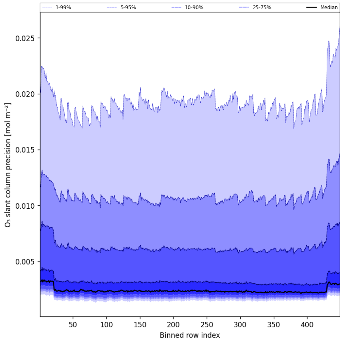
Figure 44: Along track statistics of “O 3 slant column precision” for 2025-08-20 to 2025-08-21
