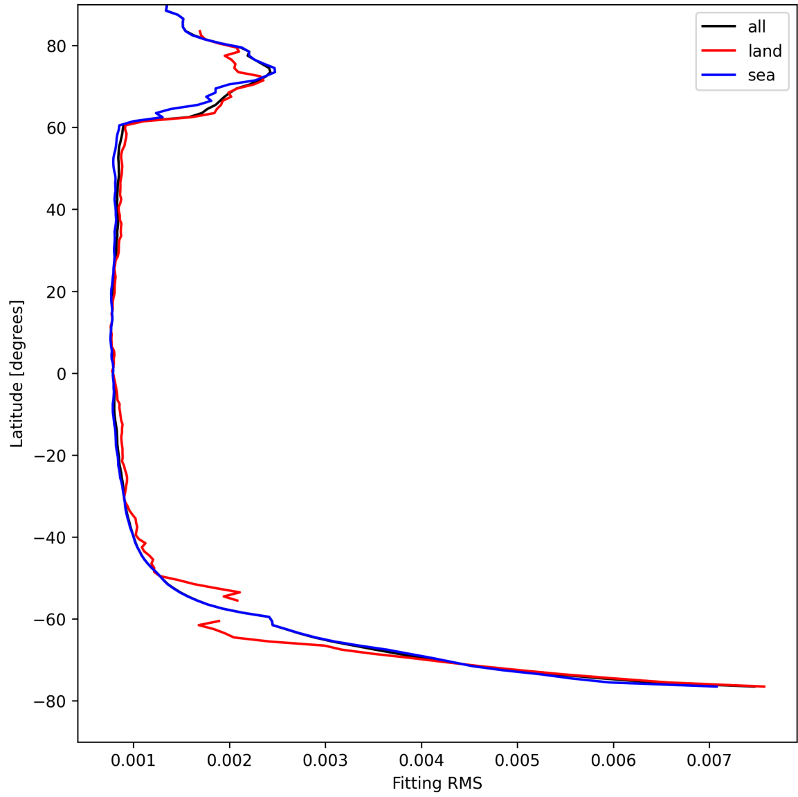
Figure 22: Zonal average of “Fitting RMS” for 2025-08-20 to 2025-08-21.
