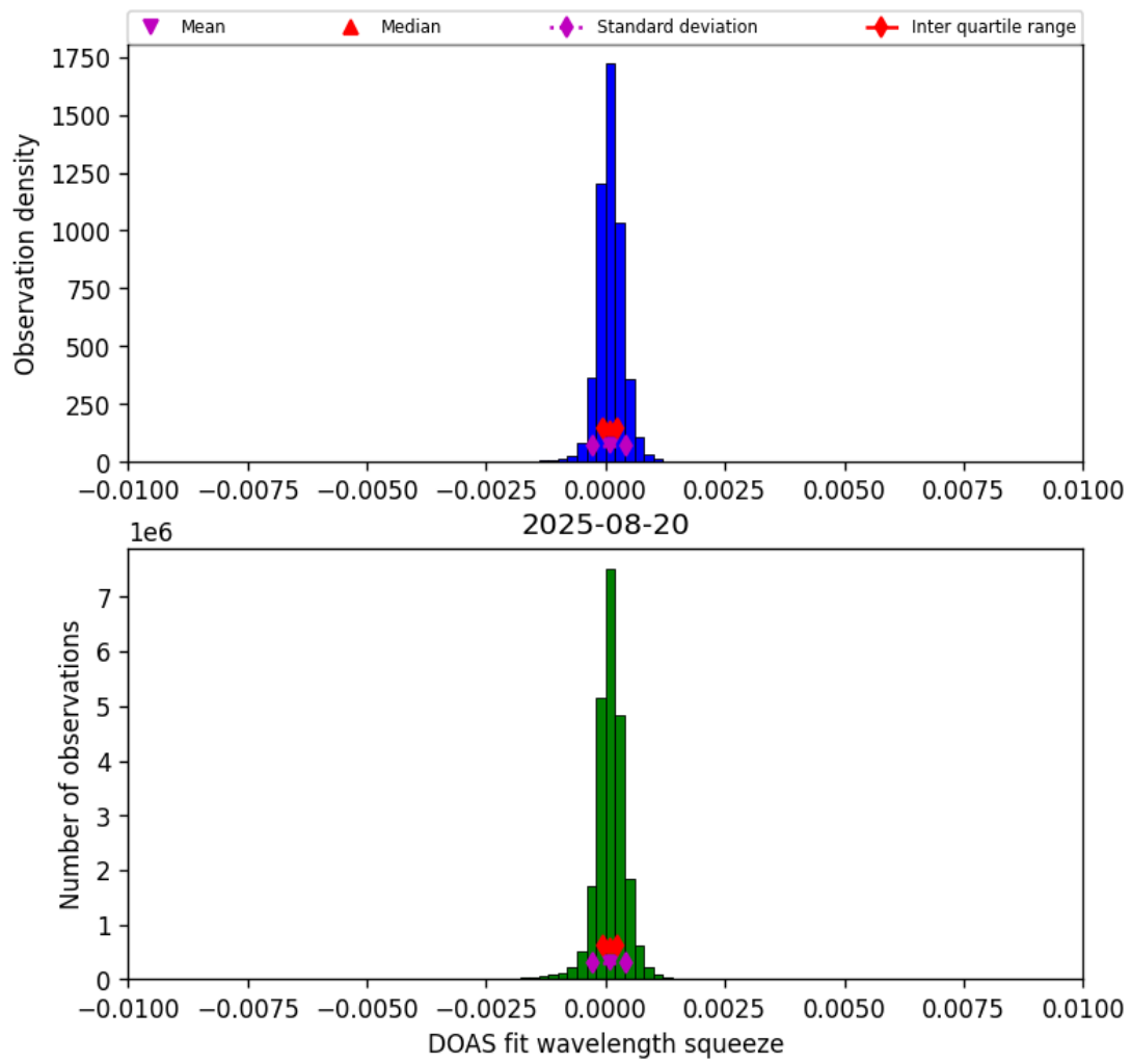
Figure 36: Histogram of “DOAS fit wavelength squeeze” for 2025-08-20 to 2025-08-21
