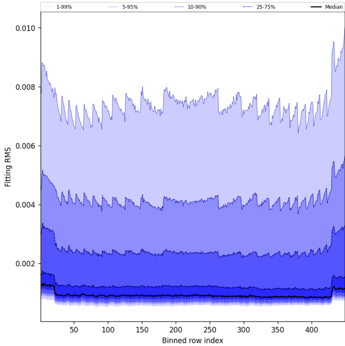
Figure 46: Along track statistics of “Fitting RMS” for 2025-08-20 to 2025-08-21
