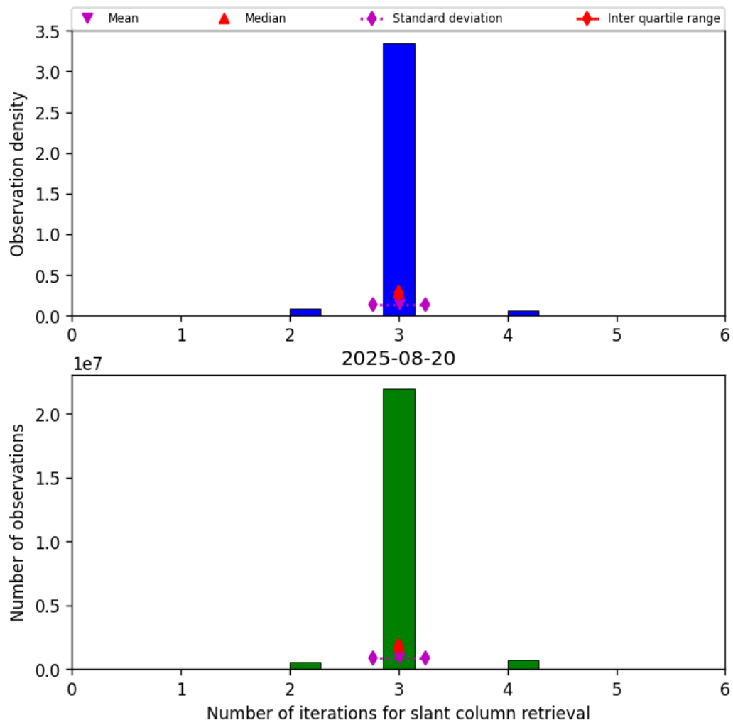
Figure 33: Histogram of “Number of iterations for slant column retrieval” for 2025-08-20 to 2025-08-21
