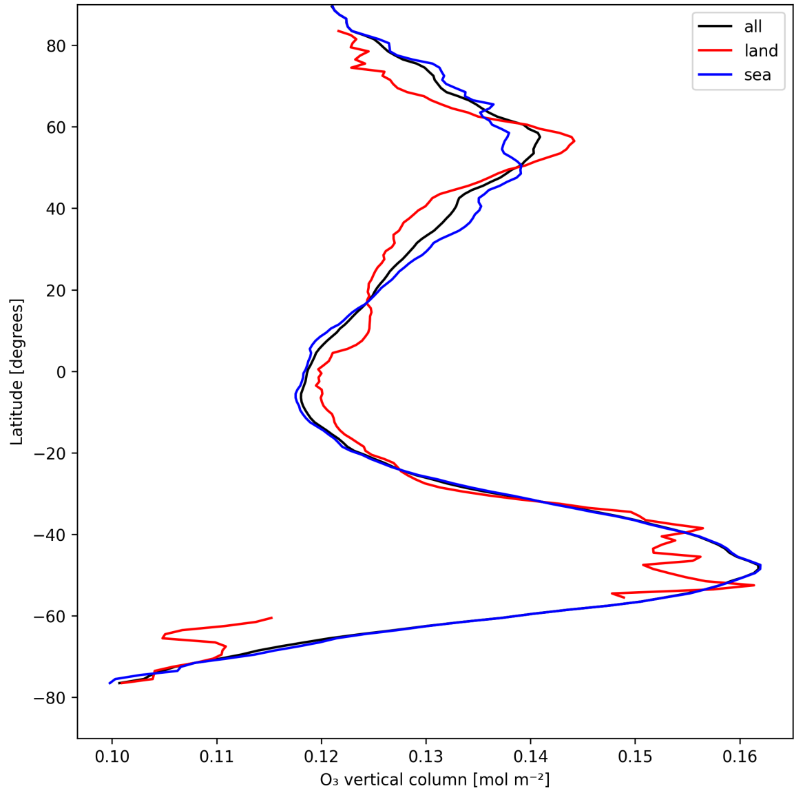
Figure 17: Zonal average of “O 3 vertical column” for 2025-08-20 to 2025-08-21.
