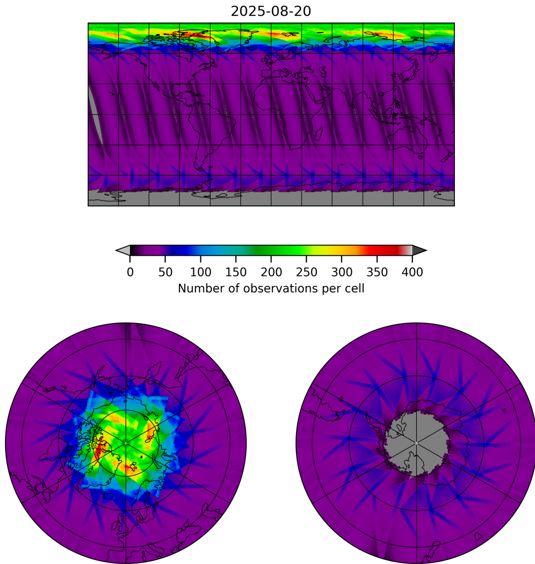
Figure 15: Map of the number of observations for 2025-08-20 to 2025-08-21
