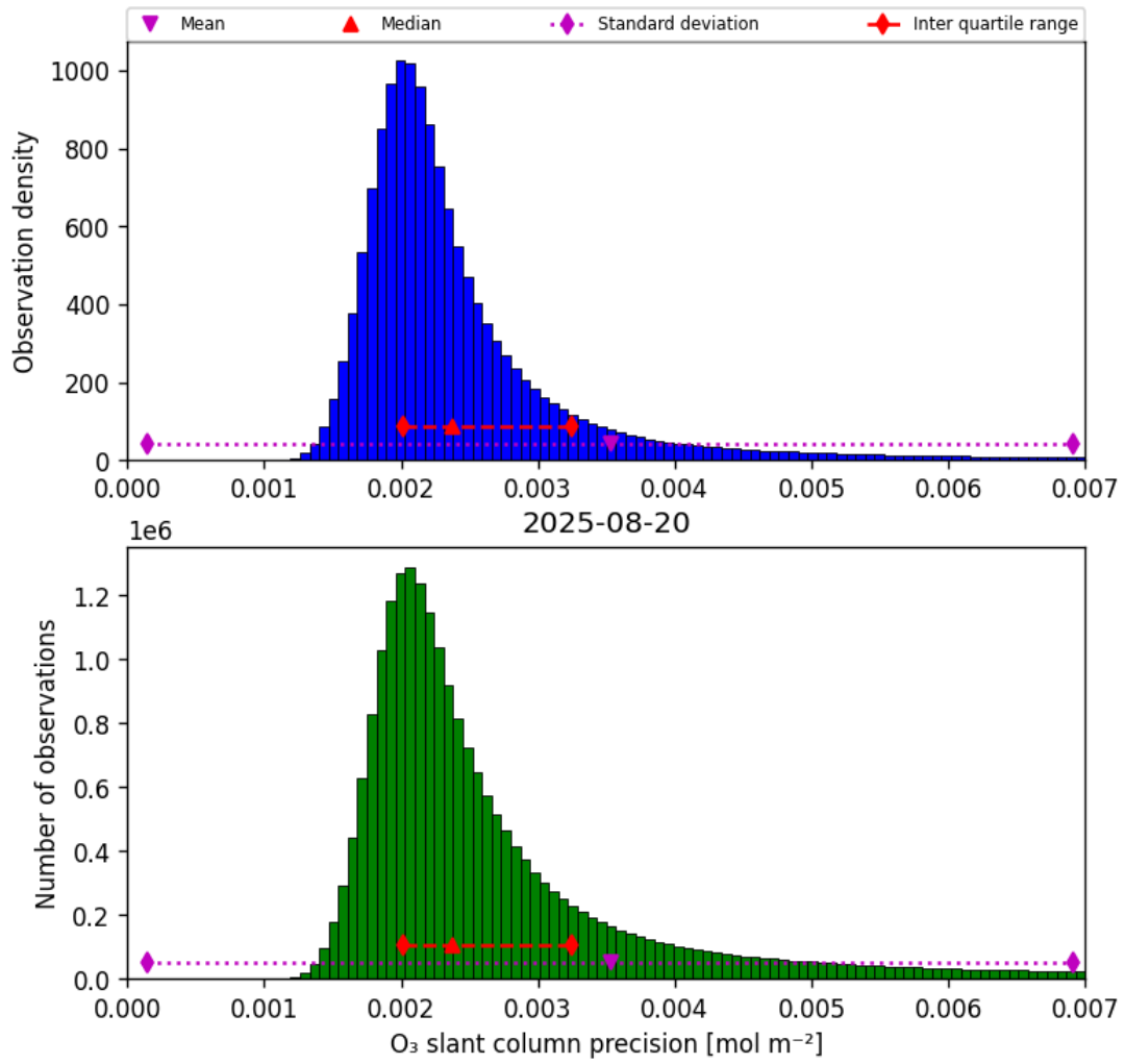
Figure 32: Histogram of “O 3 slant column precision” for 2025-08-20 to 2025-08-21
