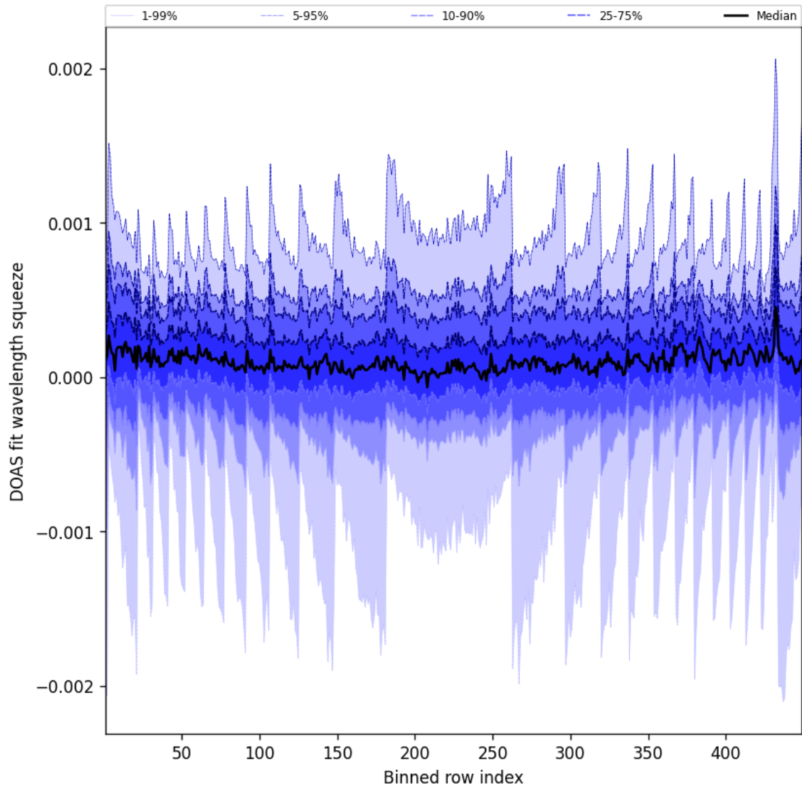
Figure 48: Along track statistics of “DOAS fit wavelength squeeze” for 2025-08-20 to 2025-08-21
