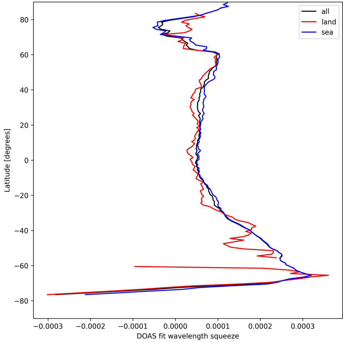
Figure 24: Zonal average of “DOAS fit wavelength squeeze” for 2025-08-20 to 2025-08-21.
