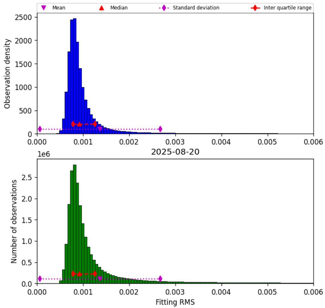
Figure 34: Histogram of “Fitting RMS” for 2025-08-20 to 2025-08-21
