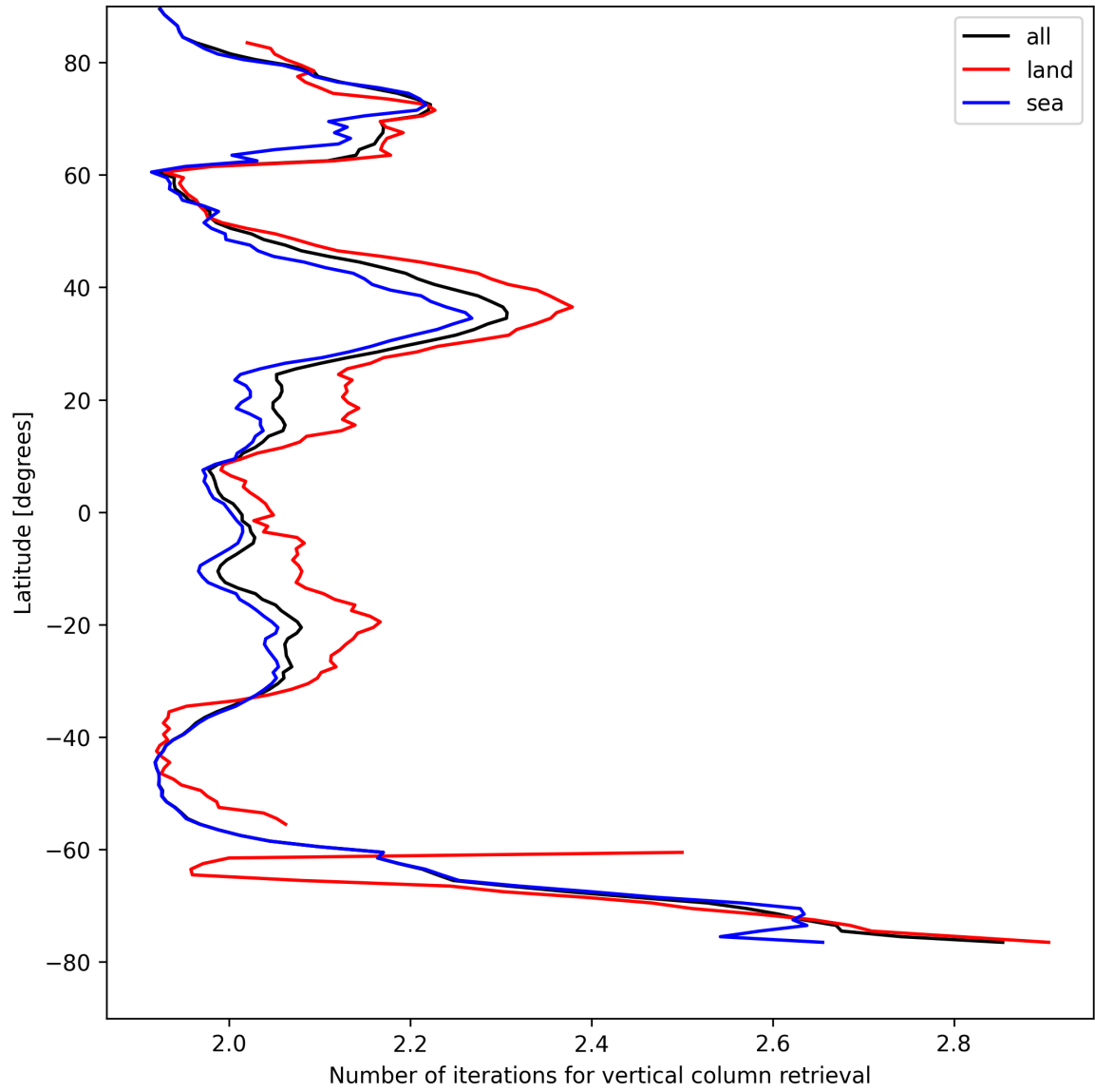
Figure 27: Zonal average of “Number of iterations for vertical column retrieval” for 2025-08-20 to 2025-08-21.
