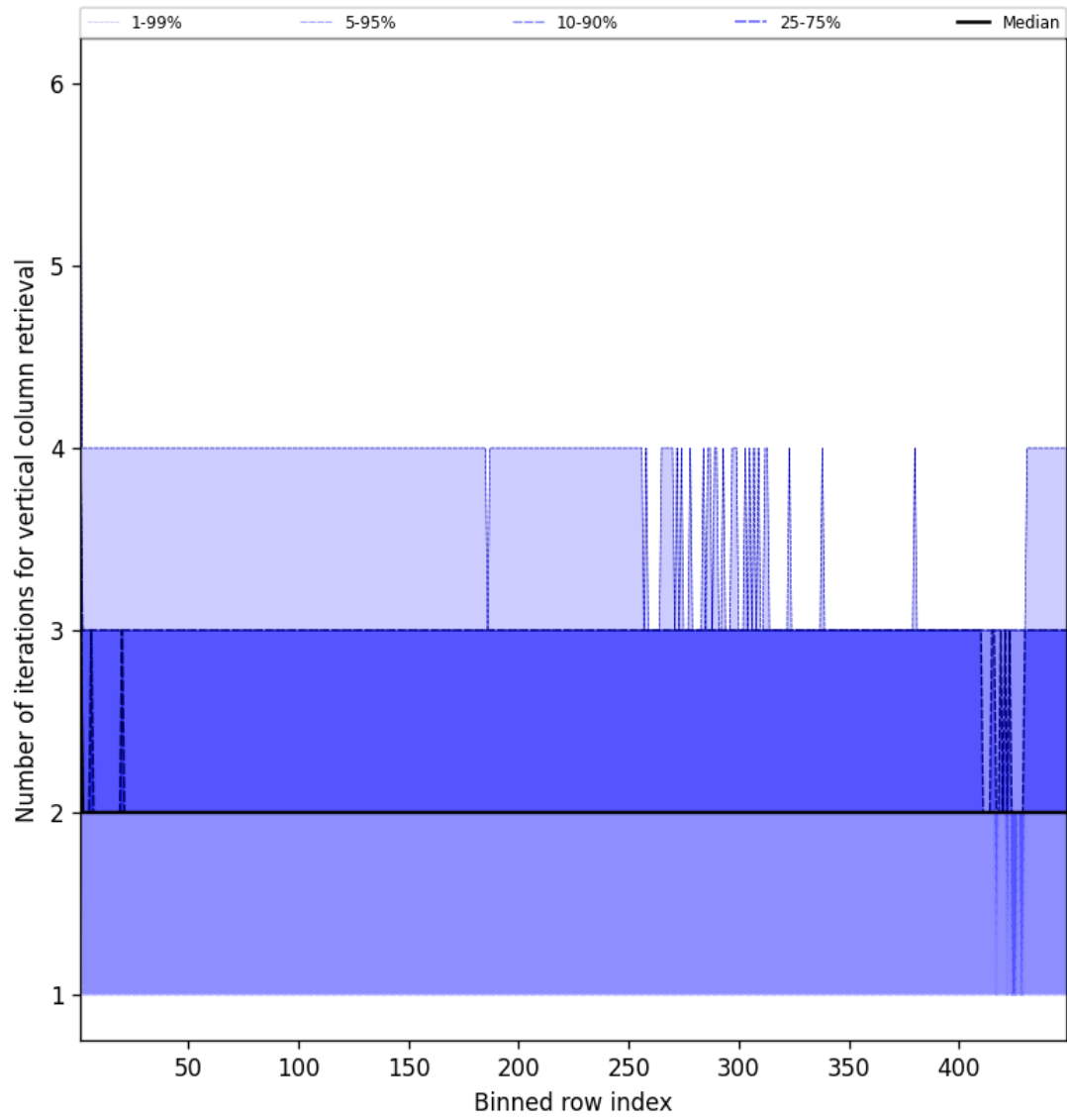
Figure 51: Along track statistics of “Number of iterations for vertical column retrieval” for 2025-08-20 to 2025-08-21
