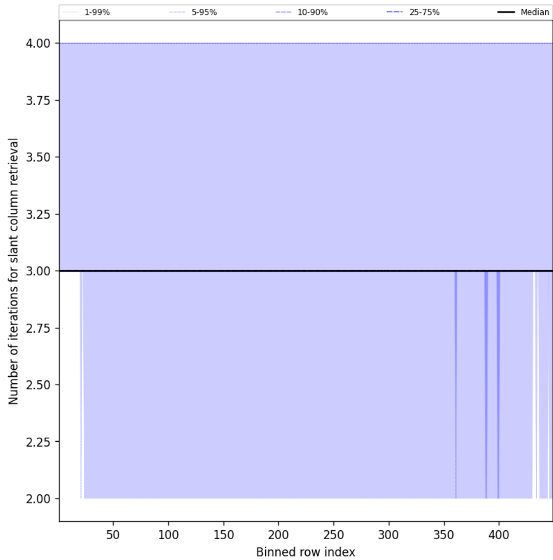
Figure 45: Along track statistics of “Number of iterations for slant column retrieval” for 2025-08-20 to 2025-08-21
