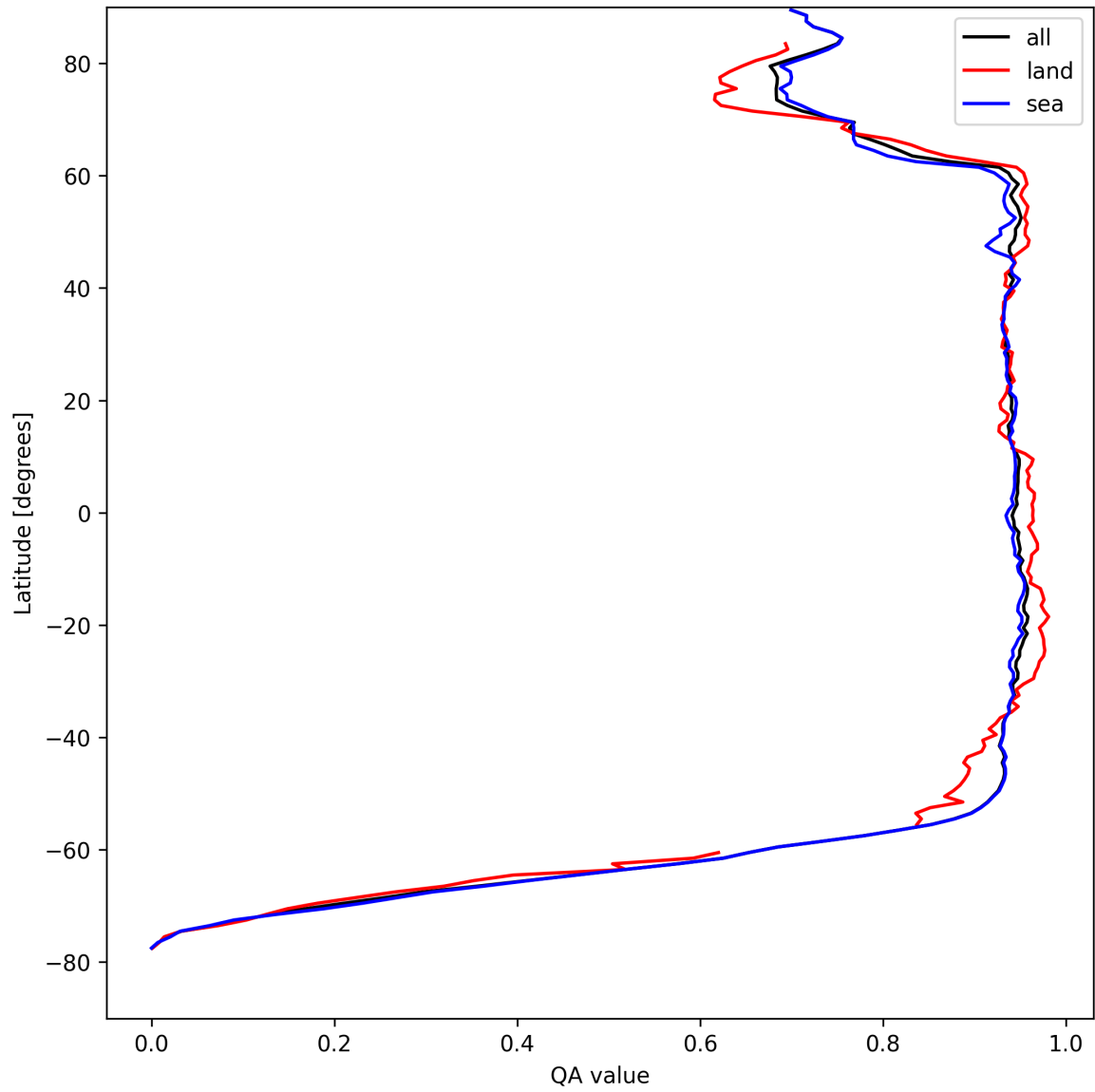
Figure 16: Zonal average of “QA value” for 2025-08-21 to 2025-08-22.
