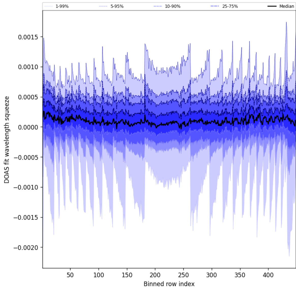
Figure 48: Along track statistics of “DOAS fit wavelength squeeze” for 2025-08-21 to 2025-08-22
