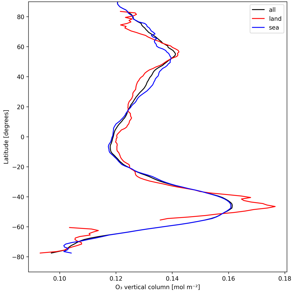
Figure 17: Zonal average of “O 3 vertical column” for 2025-08-21 to 2025-08-22.
