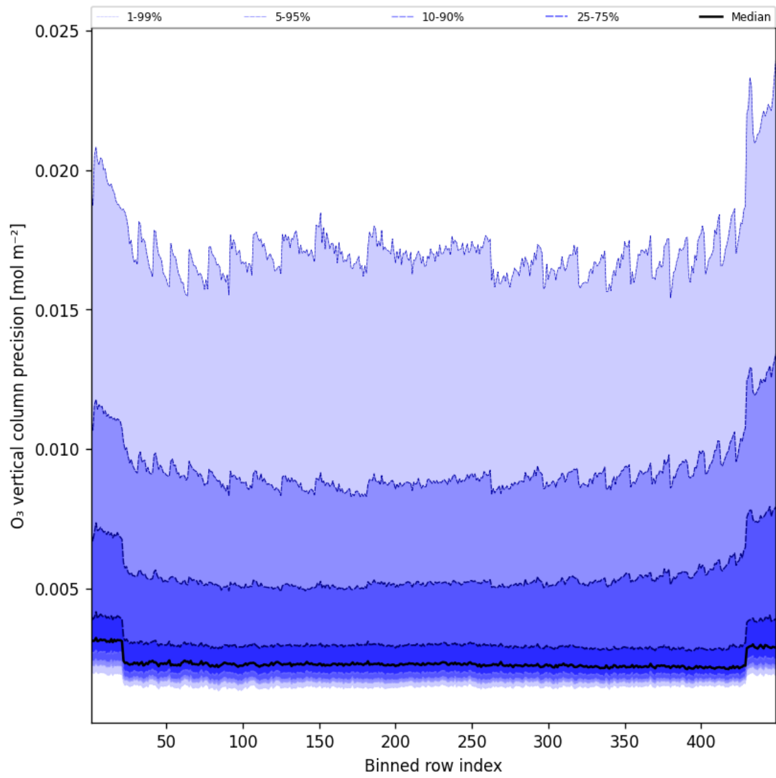
Figure 42: Along track statistics of “O 3 vertical column precision” for 2025-08-21 to 2025-08-22
