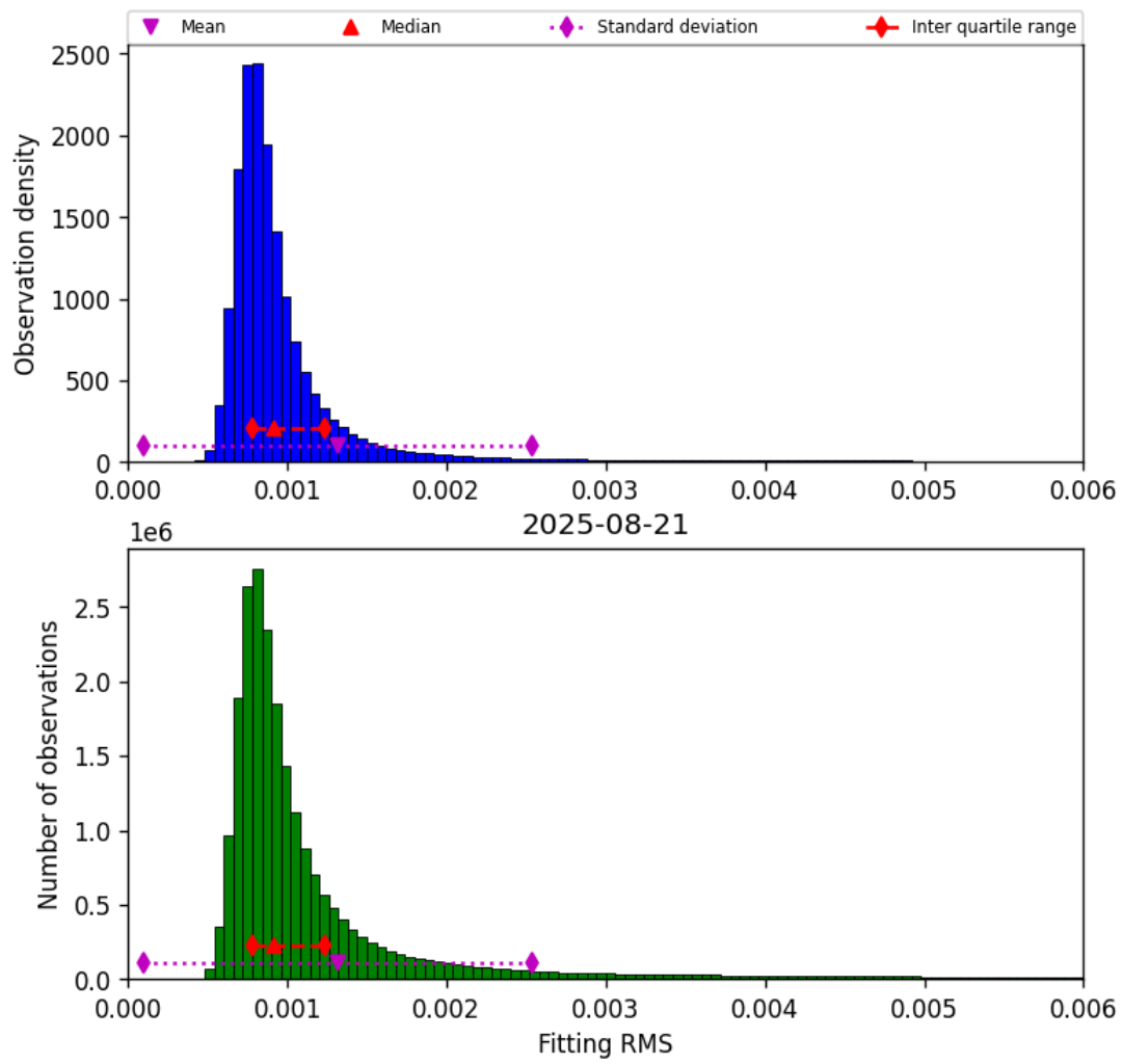
Figure 34: Histogram of “Fitting RMS” for 2025-08-21 to 2025-08-22
