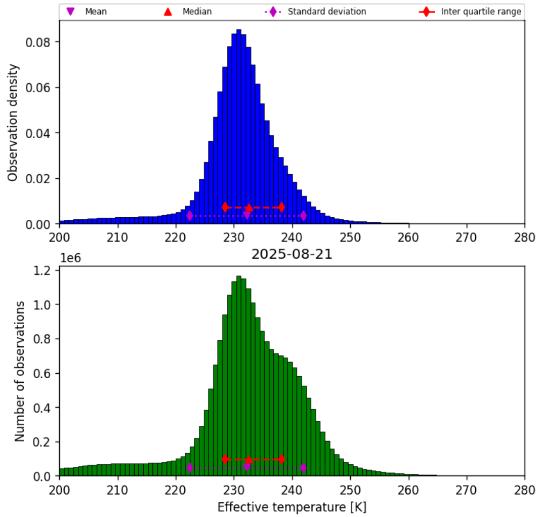
Figure 38: Histogram of “Effective temperature” for 2025-08-21 to 2025-08-22
