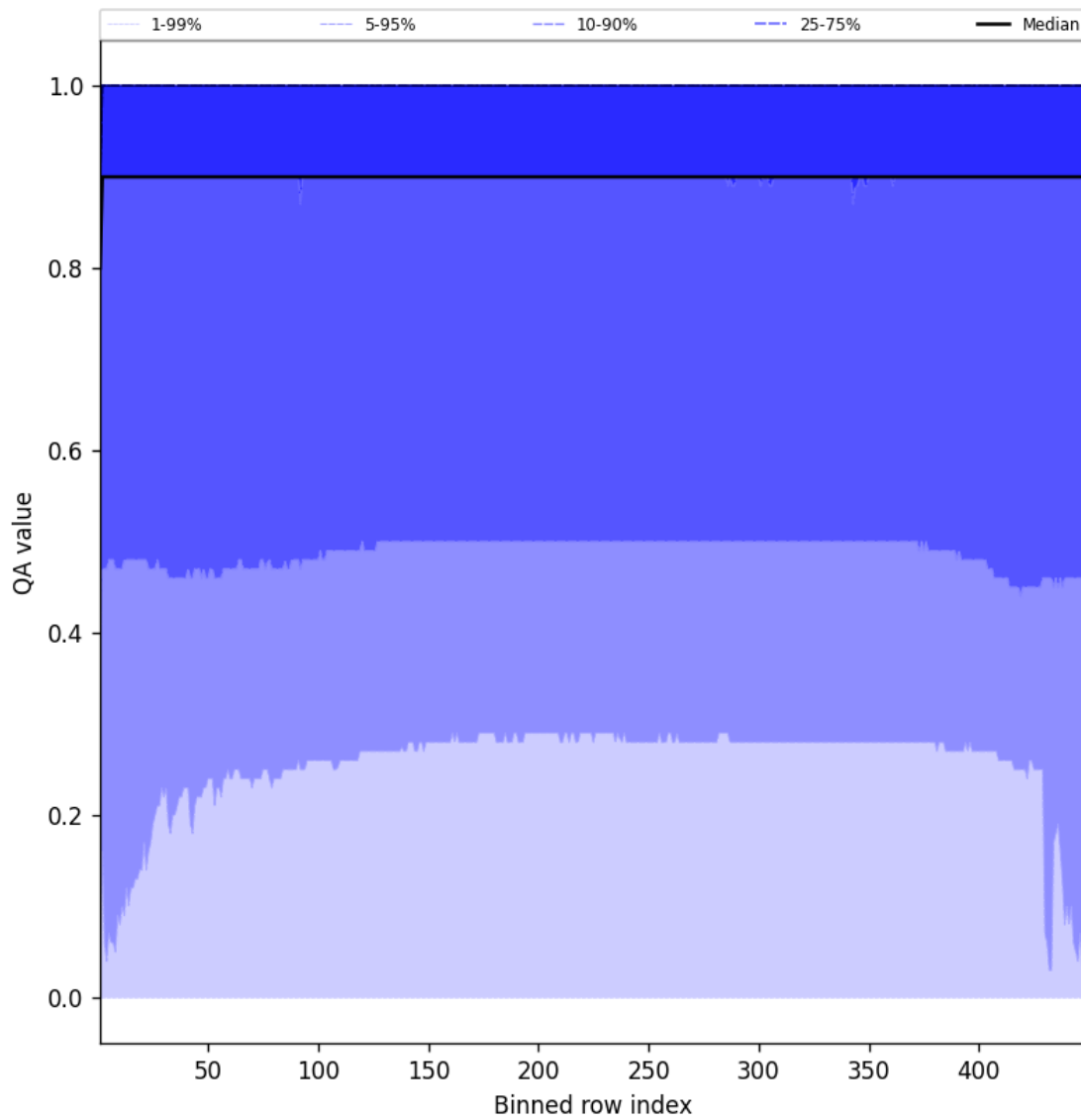
Figure 40: Along track statistics of “QA value” for 2025-08-21 to 2025-08-22
