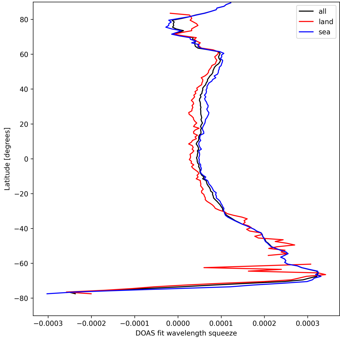
Figure 24: Zonal average of “DOAS fit wavelength squeeze” for 2025-08-21 to 2025-08-22.
