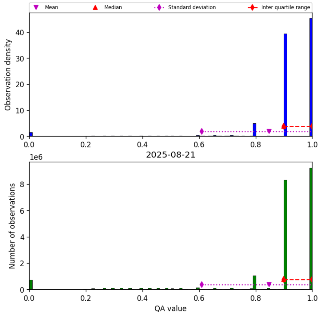
Figure 28: Histogram of “QA value” for 2025-08-21 to 2025-08-22
