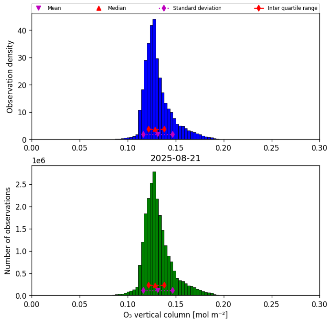
Figure 29: Histogram of “O 3 vertical column” for 2025-08-21 to 2025-08-22
