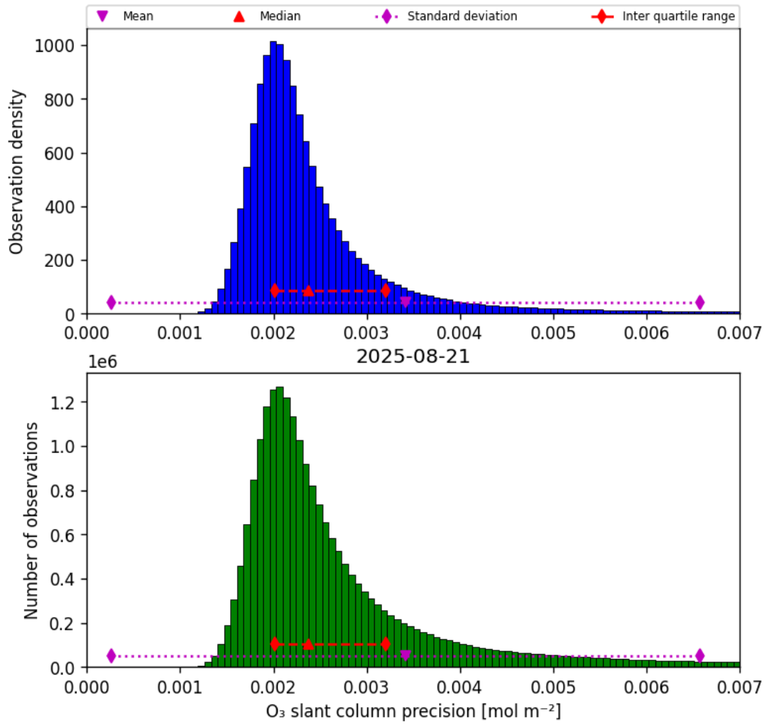
Figure 32: Histogram of “O 3 slant column precision” for 2025-08-21 to 2025-08-22
