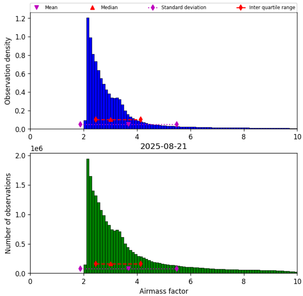
Figure 37: Histogram of “Airmass factor” for 2025-08-21 to 2025-08-22
