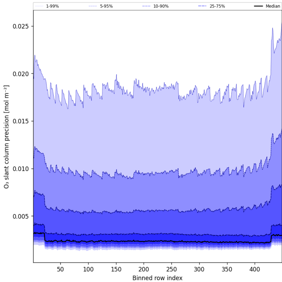
Figure 44: Along track statistics of “O 3 slant column precision” for 2025-08-21 to 2025-08-22
