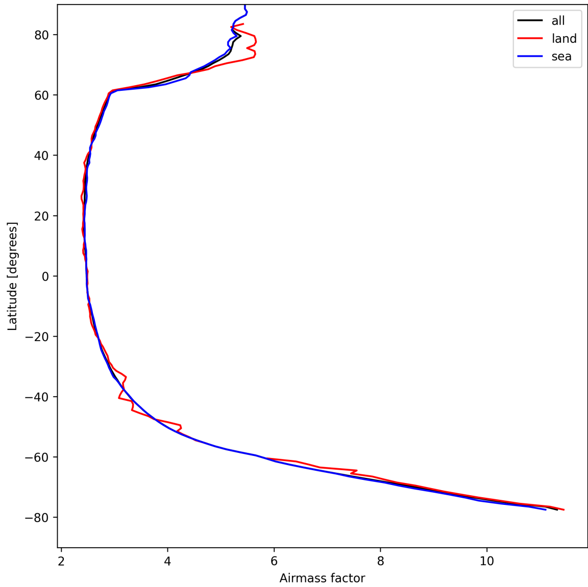
Figure 25: Zonal average of “Airmass factor” for 2025-08-21 to 2025-08-22.
