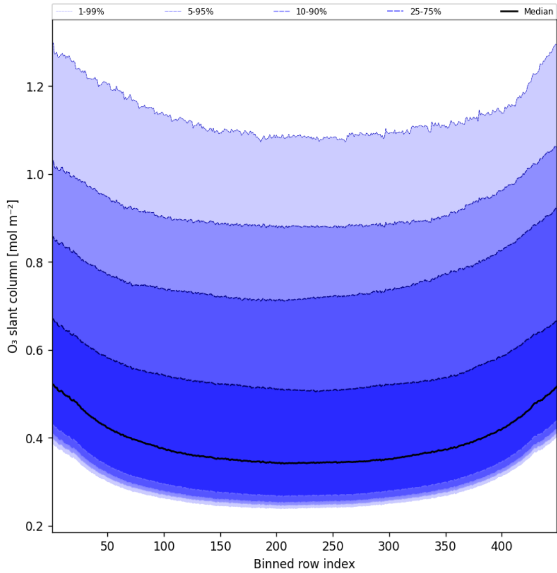
Figure 43: Along track statistics of “O 3 slant column” for 2025-08-21 to 2025-08-22
