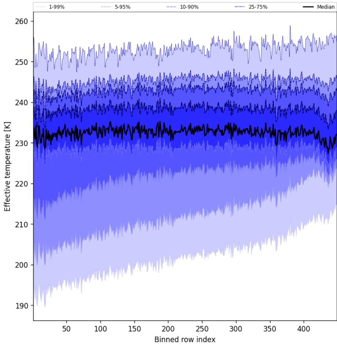
Figure 50: Along track statistics of “Effective temperature” for 2025-08-21 to 2025-08-22
