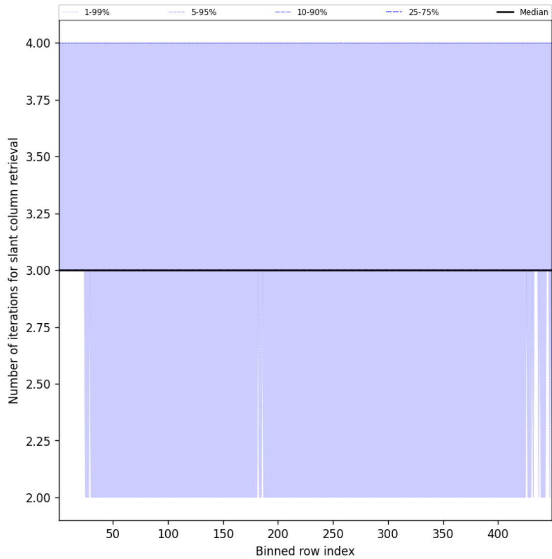
Figure 45: Along track statistics of “Number of iterations for slant column retrieval” for 2025-08-21 to 2025-08-22
