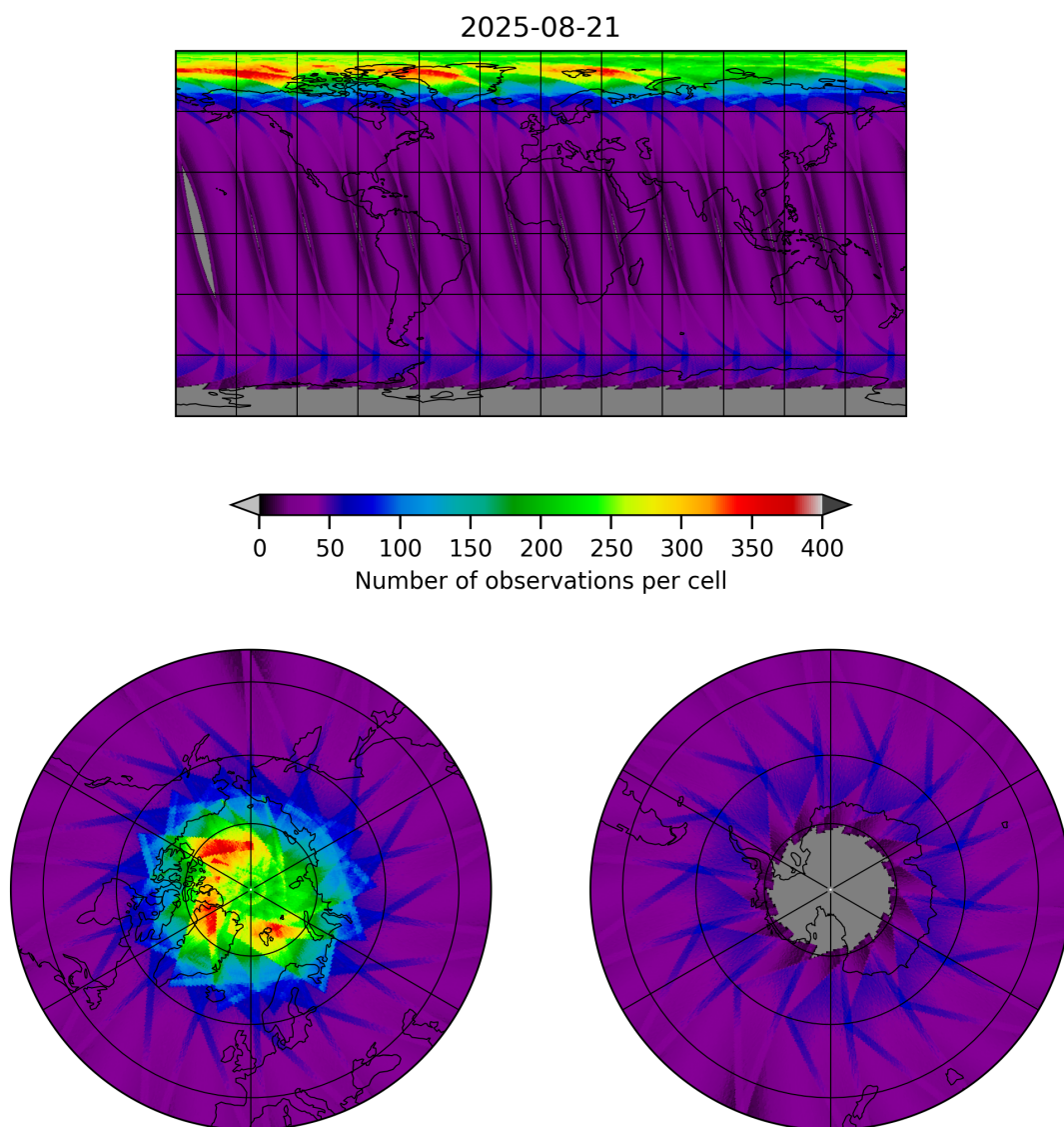
Figure 15: Map of the number of observations for 2025-08-21 to 2025-08-22
