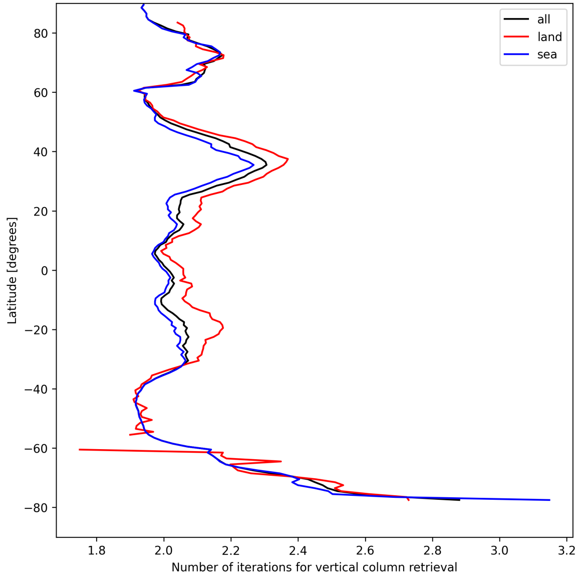
Figure 27: Zonal average of “Number of iterations for vertical column retrieval” for 2025-08-21 to 2025-08-22.
