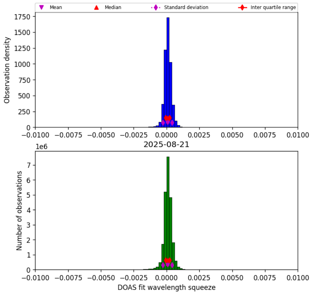
Figure 36: Histogram of “DOAS fit wavelength squeeze” for 2025-08-21 to 2025-08-22
