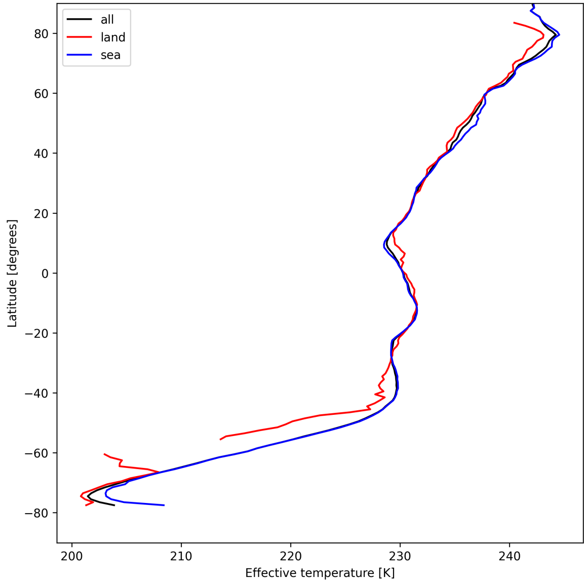
Figure 26: Zonal average of “Effective temperature” for 2025-08-21 to 2025-08-22.
