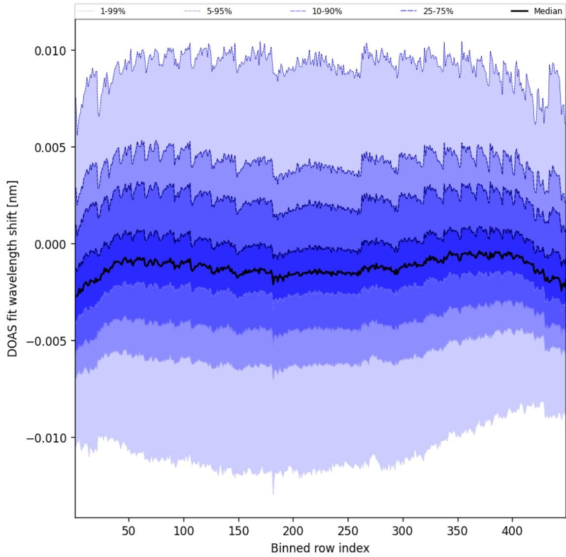
Figure 47: Along track statistics of “DOAS fit wavelength shift” for 2025-08-21 to 2025-08-22
