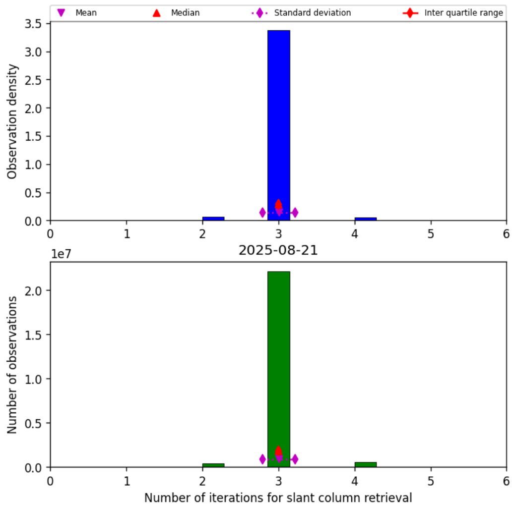
Figure 33: Histogram of “Number of iterations for slant column retrieval” for 2025-08-21 to 2025-08-22
