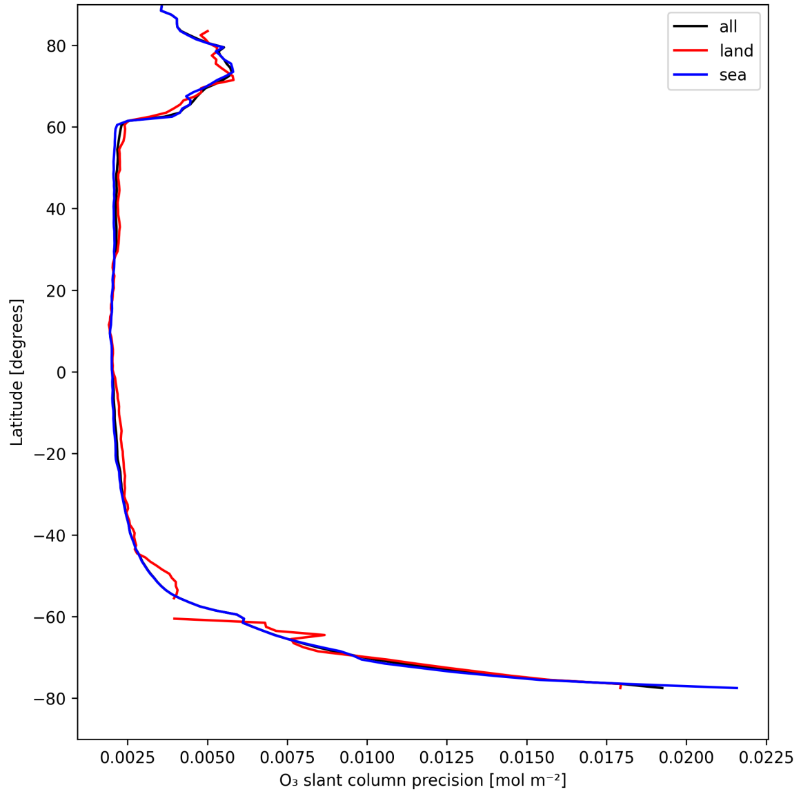
Figure 20: Zonal average of “O 3 slant column precision” for 2025-08-21 to 2025-08-22.
