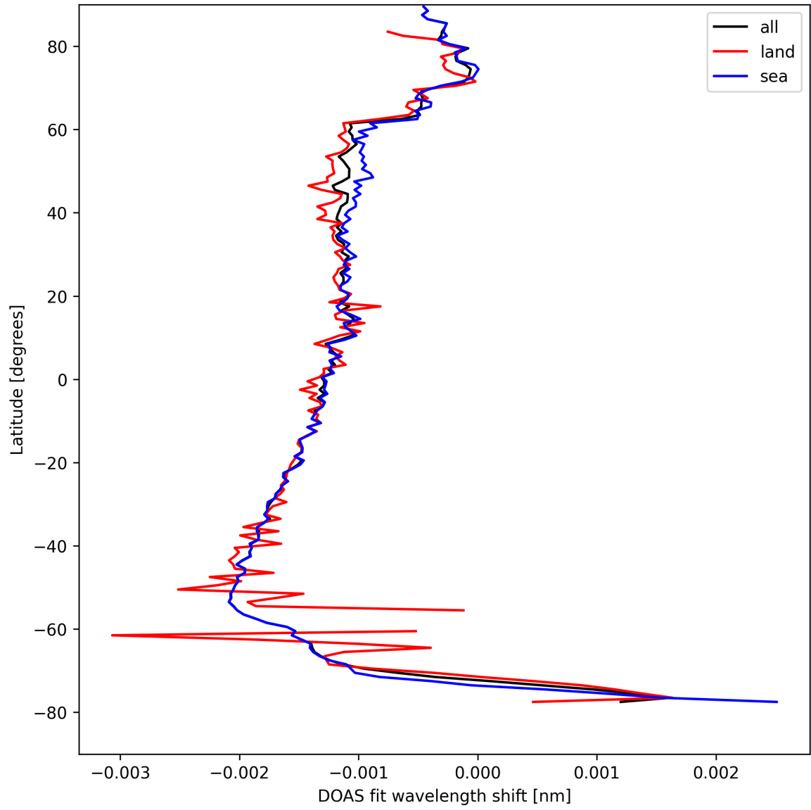
Figure 23: Zonal average of “DOAS fit wavelength shift” for 2025-08-21 to 2025-08-22.
