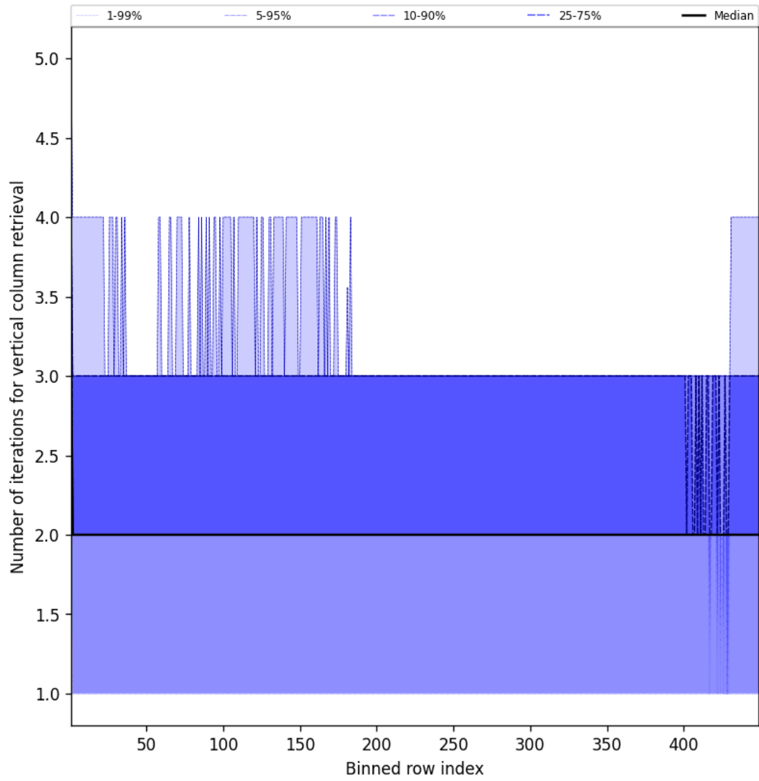
Figure 51: Along track statistics of “Number of iterations for vertical column retrieval” for 2025-08-21 to 2025-08-22
