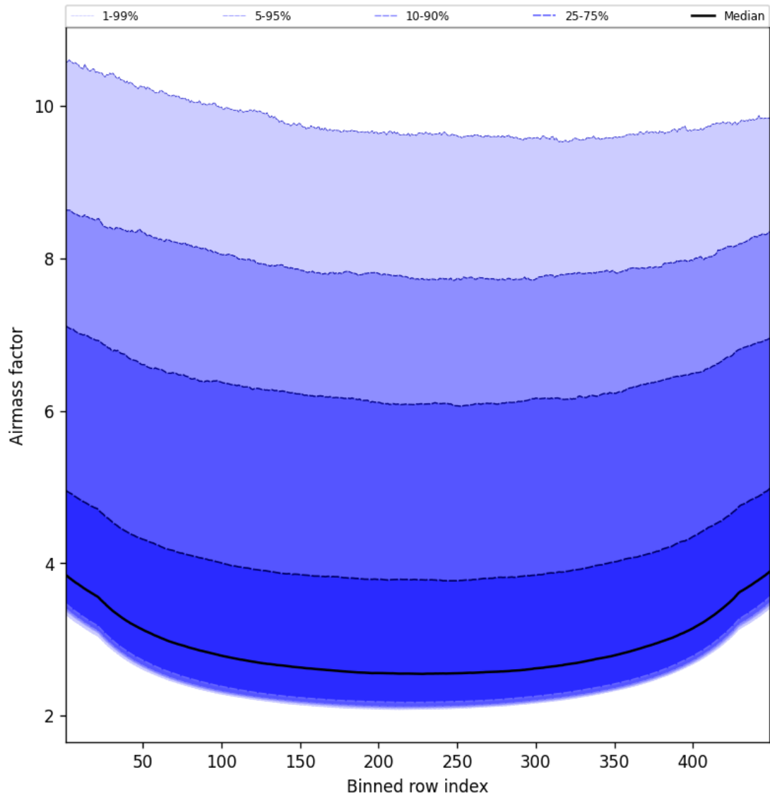
Figure 49: Along track statistics of “Airmass factor” for 2025-08-21 to 2025-08-22
