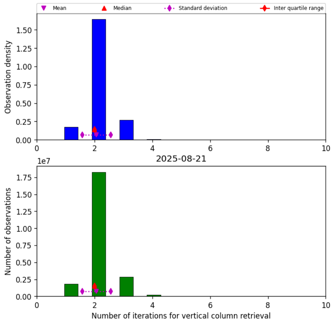
Figure 39: Histogram of “Number of iterations for vertical column retrieval” for 2025-08-21 to 2025-08-22
