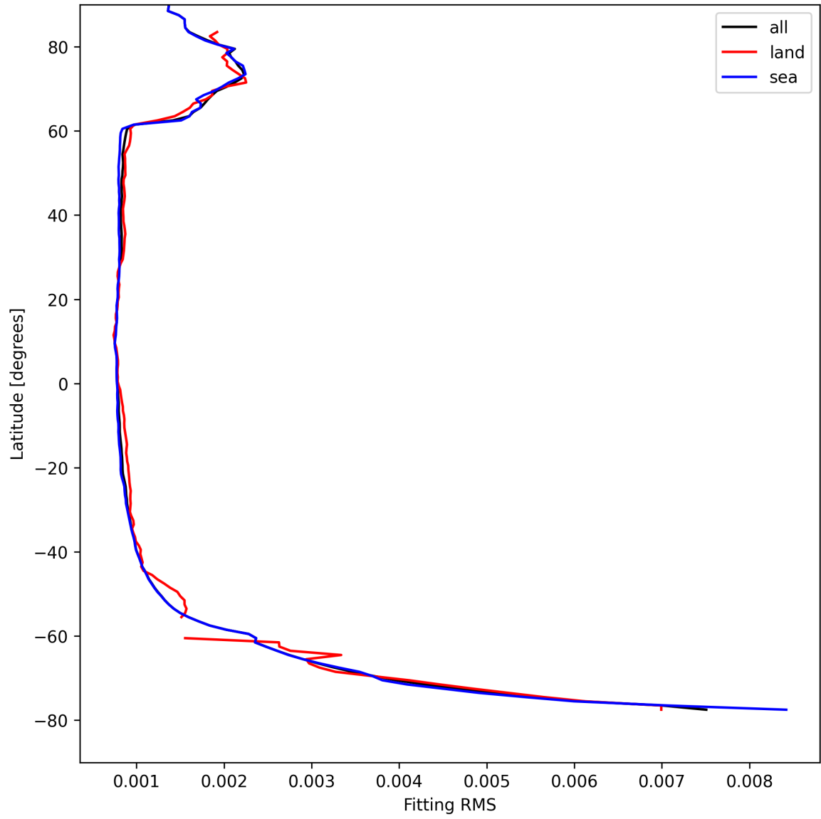
Figure 22: Zonal average of “Fitting RMS” for 2025-08-21 to 2025-08-22.
