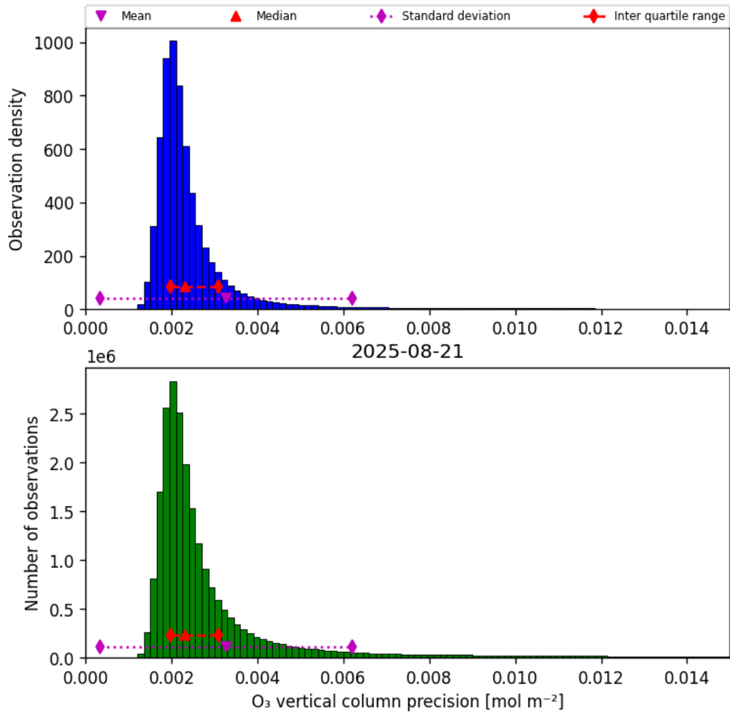
Figure 30: Histogram of “O 3 vertical column precision” for 2025-08-21 to 2025-08-22
