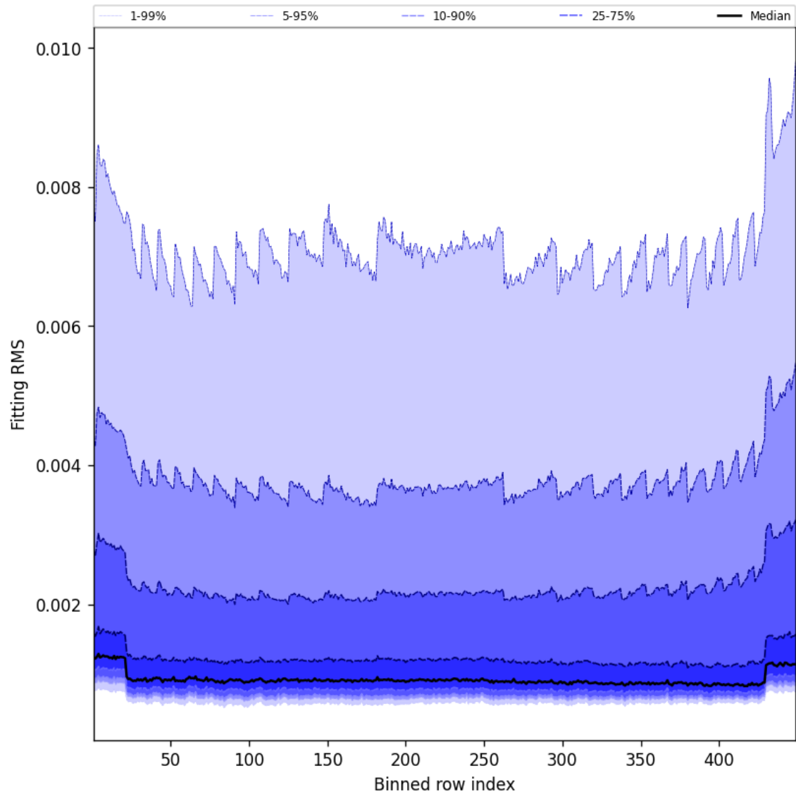
Figure 46: Along track statistics of “Fitting RMS” for 2025-08-21 to 2025-08-22
