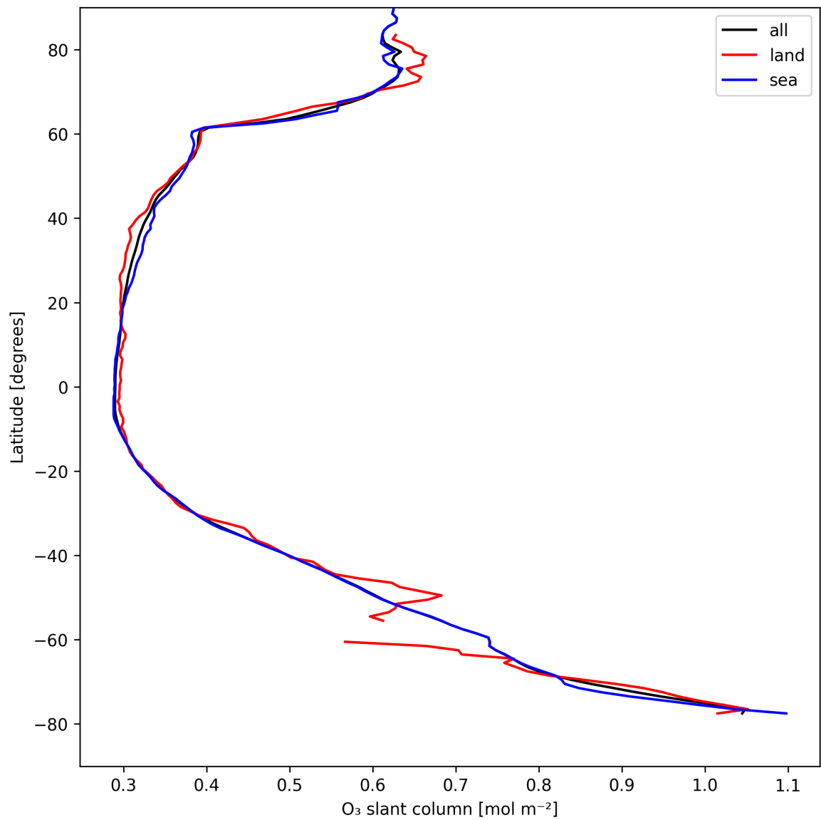
Figure 19: Zonal average of “O 3 slant column” for 2025-08-21 to 2025-08-22.
