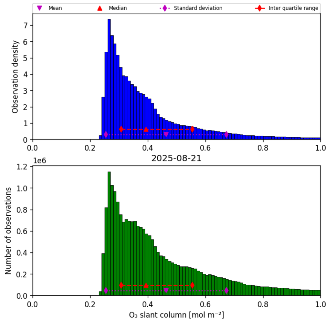
Figure 31: Histogram of “O 3 slant column” for 2025-08-21 to 2025-08-22
