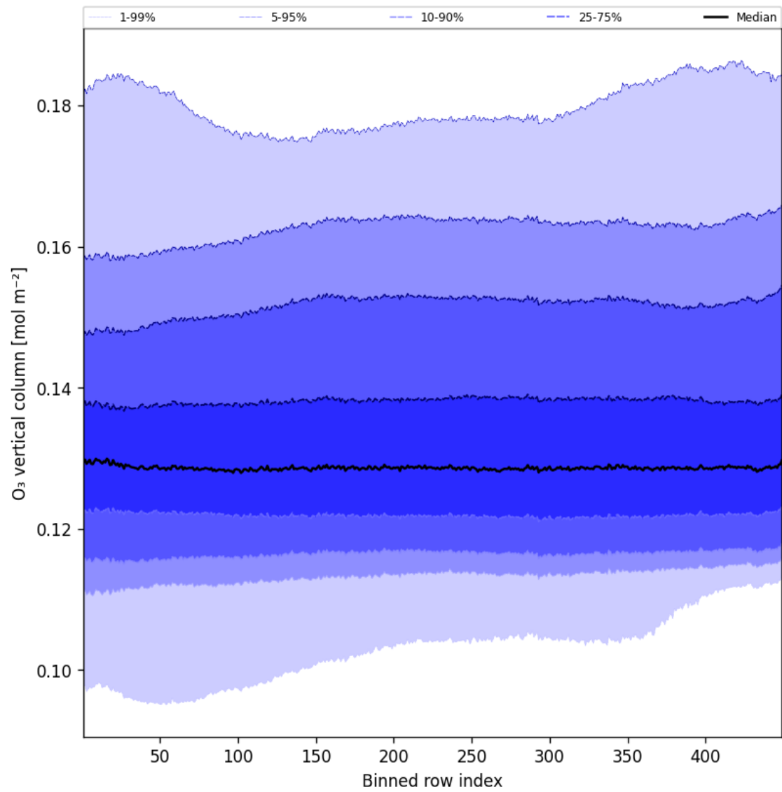
Figure 41: Along track statistics of “O 3 vertical column” for 2025-08-21 to 2025-08-22
