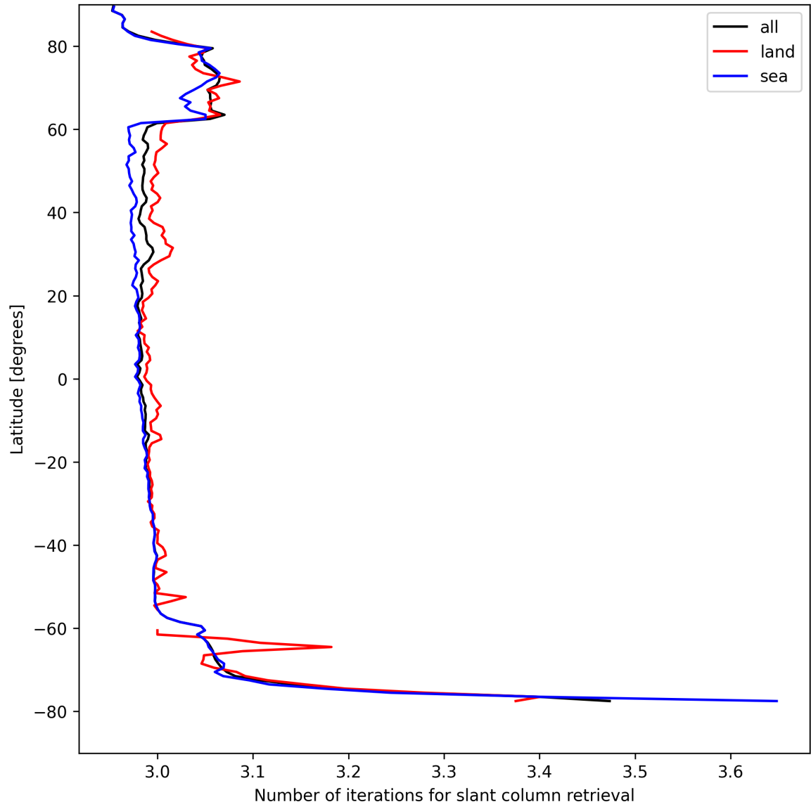
Figure 21: Zonal average of “Number of iterations for slant column retrieval” for 2025-08-21 to 2025-08-22.
