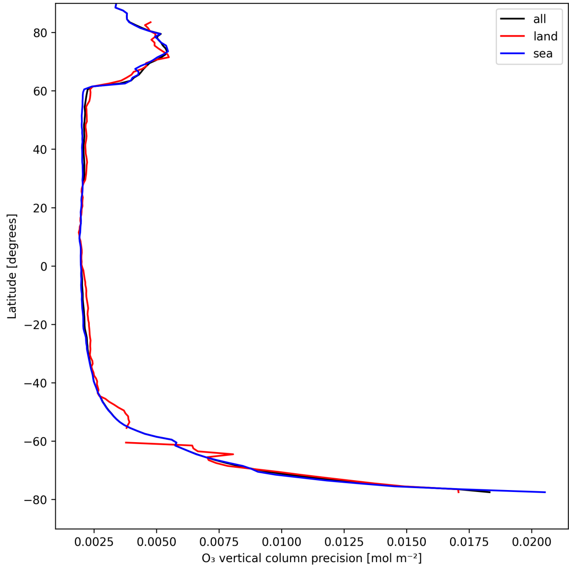
Figure 18: Zonal average of “O 3 vertical column precision” for 2025-08-21 to 2025-08-22.
