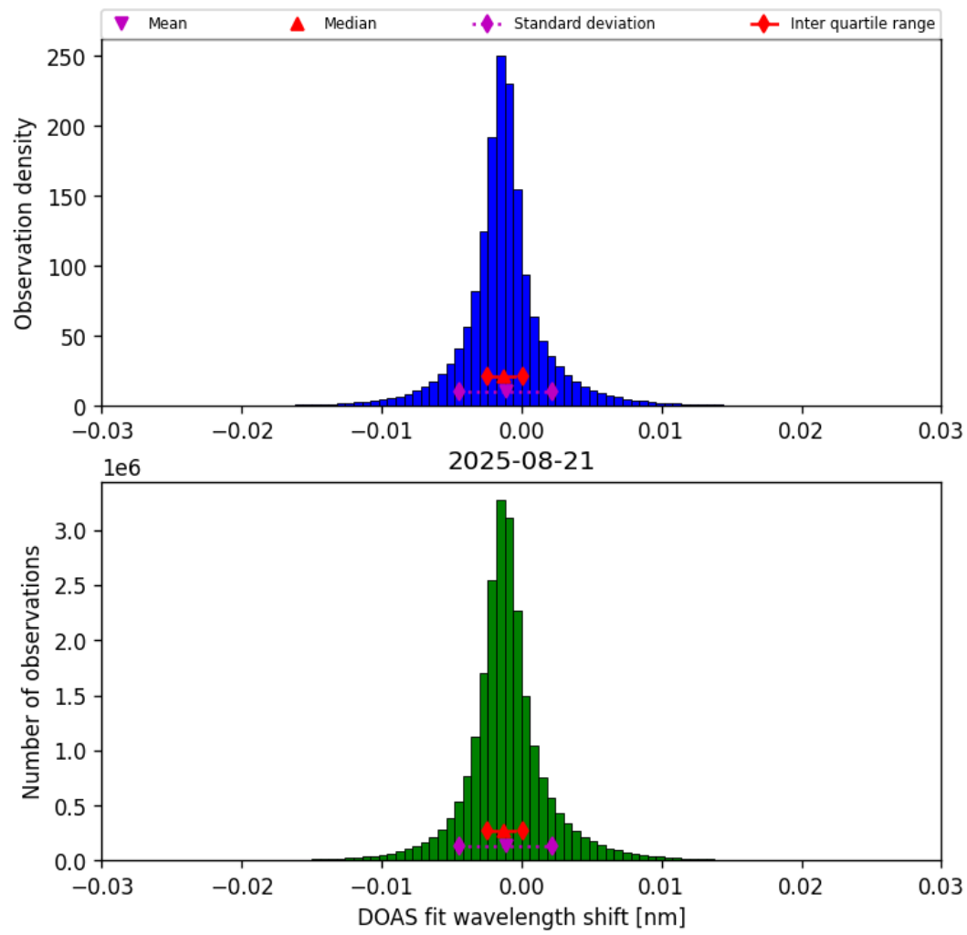
Figure 35: Histogram of “DOAS fit wavelength shift” for 2025-08-21 to 2025-08-22
