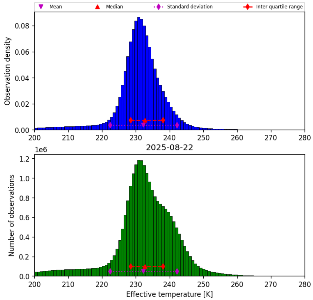
Figure 38: Histogram of “Effective temperature” for 2025-08-22 to 2025-08-23
