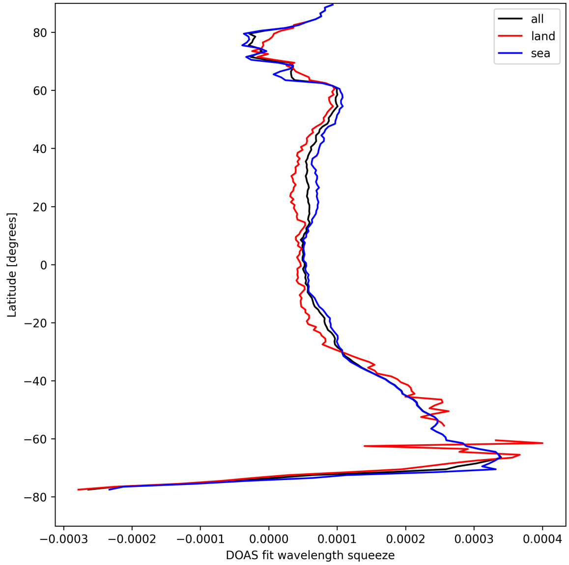
Figure 24: Zonal average of “DOAS fit wavelength squeeze” for 2025-08-22 to 2025-08-23.
