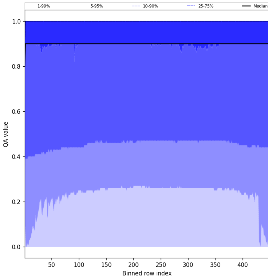
Figure 40: Along track statistics of “QA value” for 2025-08-22 to 2025-08-23
