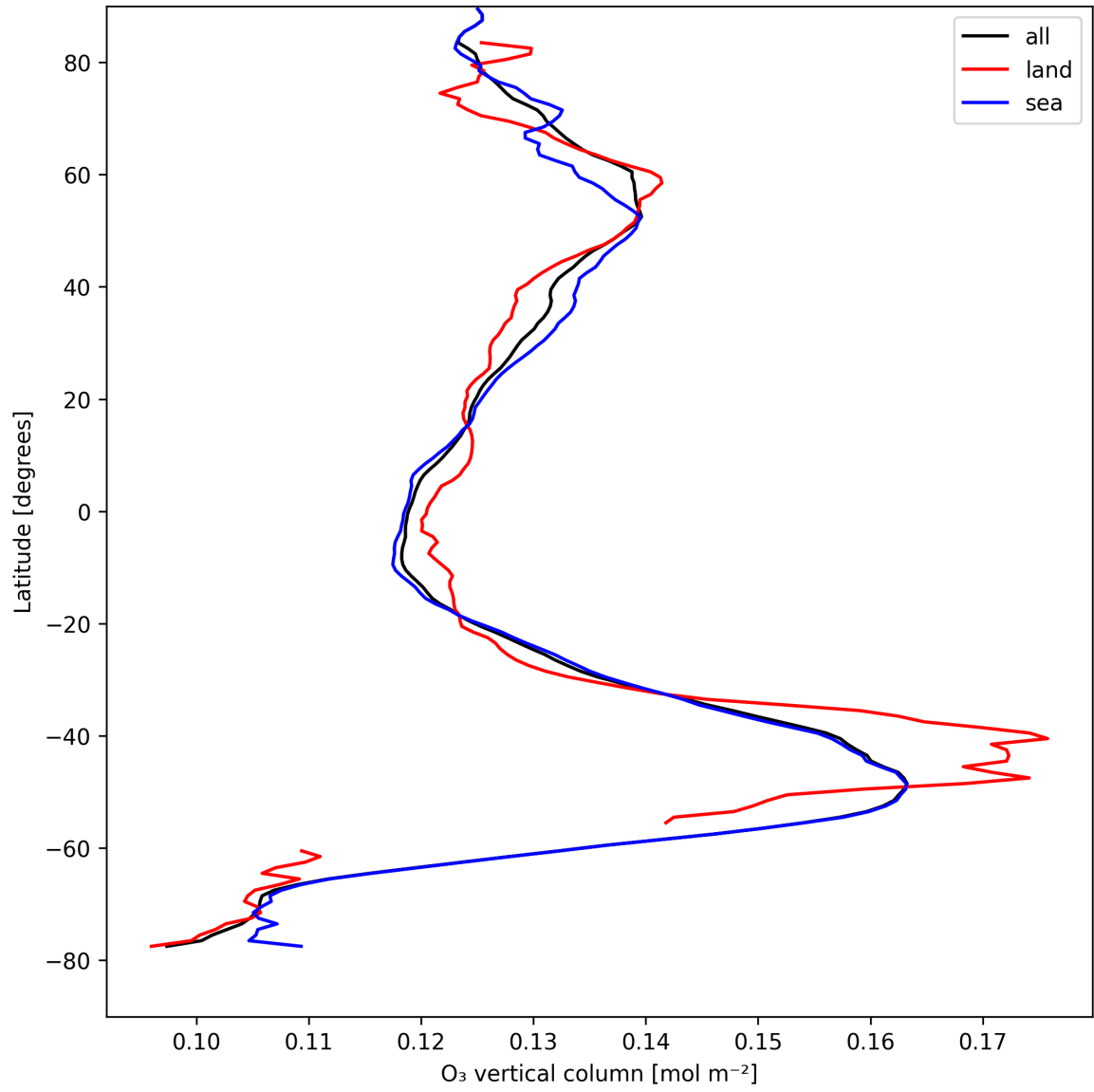
Figure 17: Zonal average of “O 3 vertical column” for 2025-08-22 to 2025-08-23.
