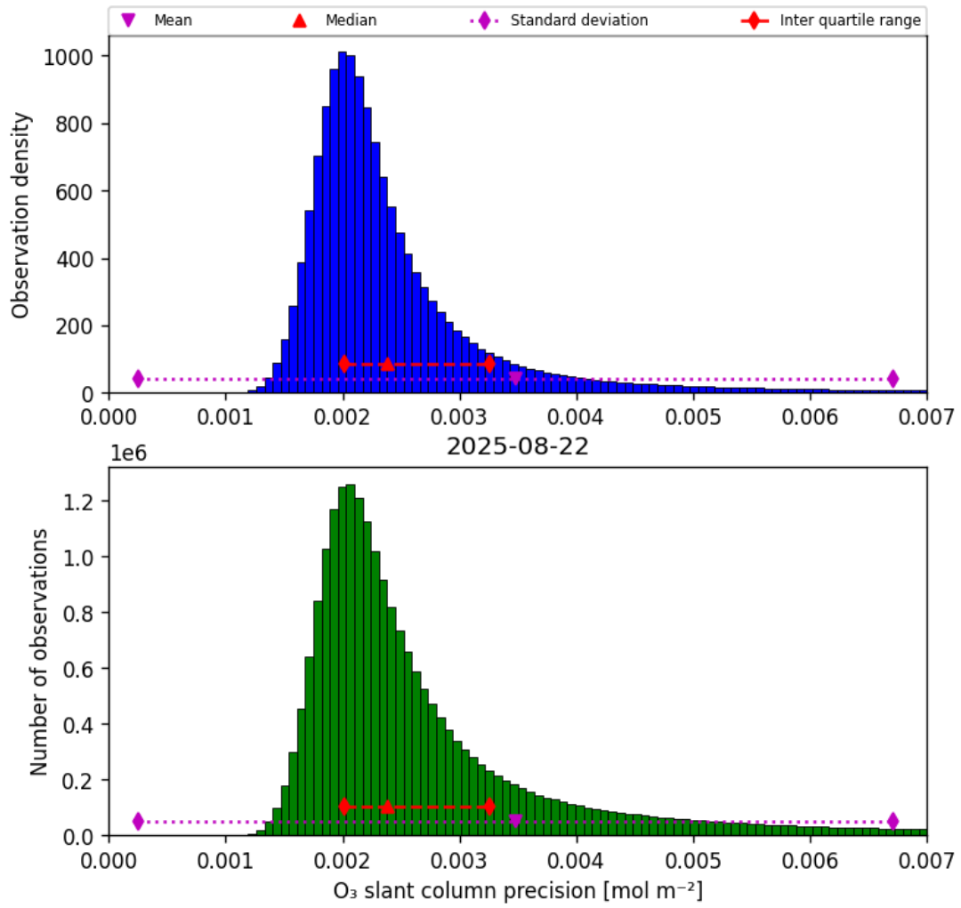
Figure 32: Histogram of “O 3 slant column precision” for 2025-08-22 to 2025-08-23
