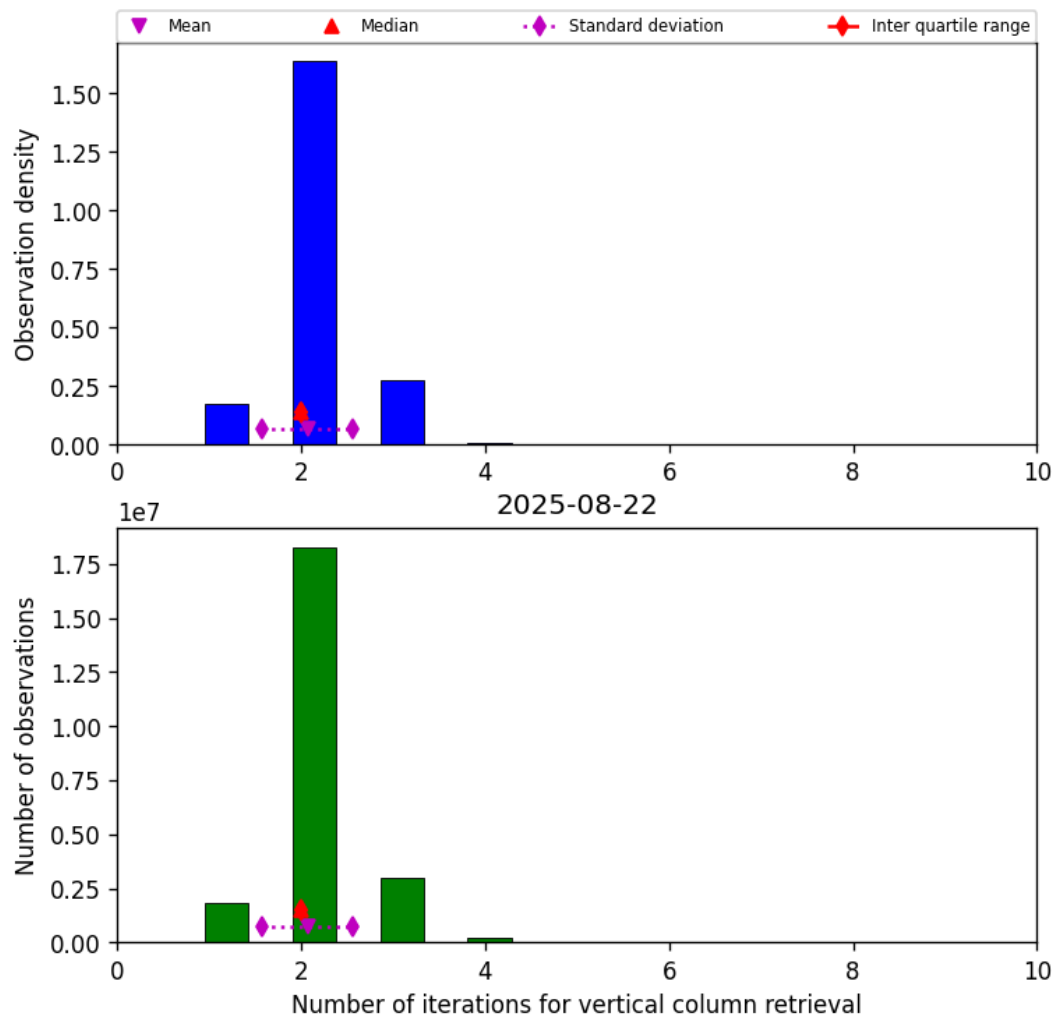
Figure 39: Histogram of “Number of iterations for vertical column retrieval” for 2025-08-22 to 2025-08-23
