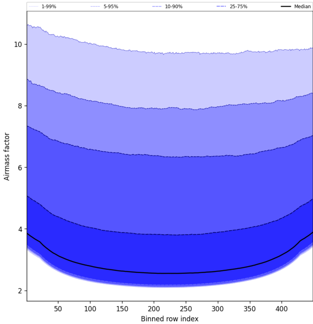
Figure 49: Along track statistics of “Airmass factor” for 2025-08-22 to 2025-08-23
