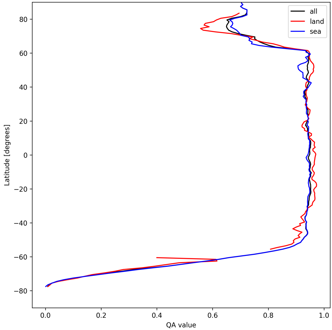
Figure 16: Zonal average of “QA value” for 2025-08-22 to 2025-08-23.
