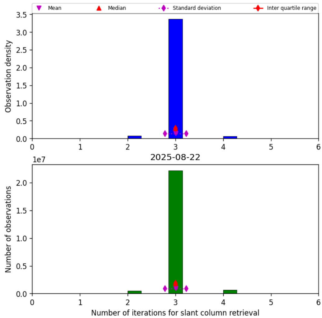
Figure 33: Histogram of “Number of iterations for slant column retrieval” for 2025-08-22 to 2025-08-23
