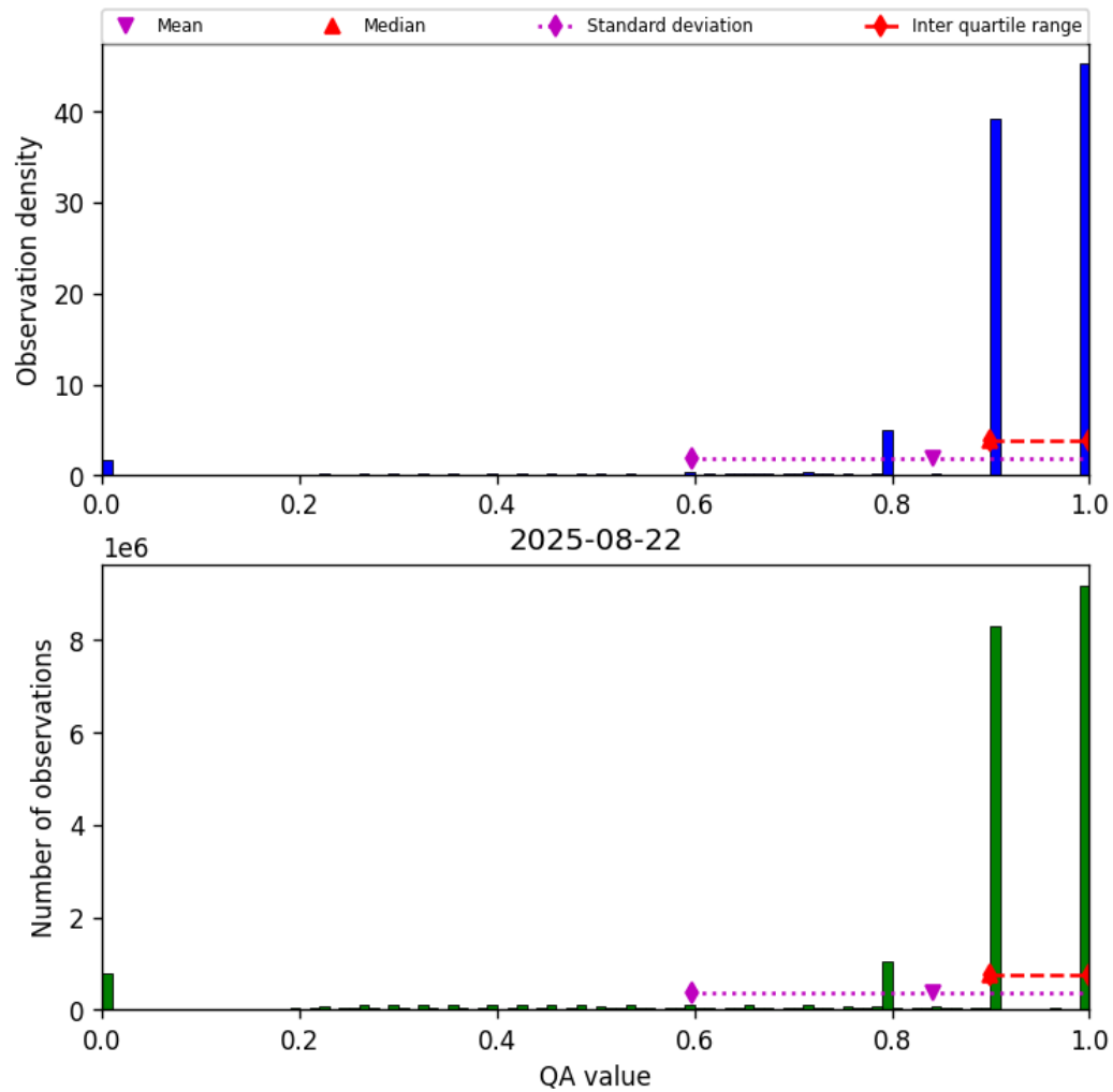
Figure 28: Histogram of “QA value” for 2025-08-22 to 2025-08-23
