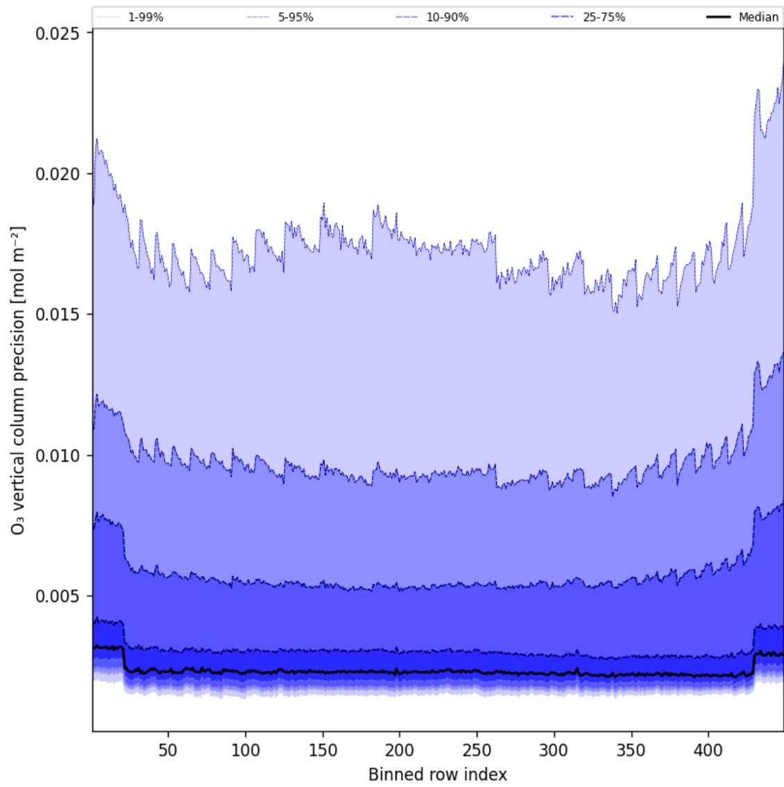
Figure 42: Along track statistics of “O 3 vertical column precision” for 2025-08-22 to 2025-08-23
