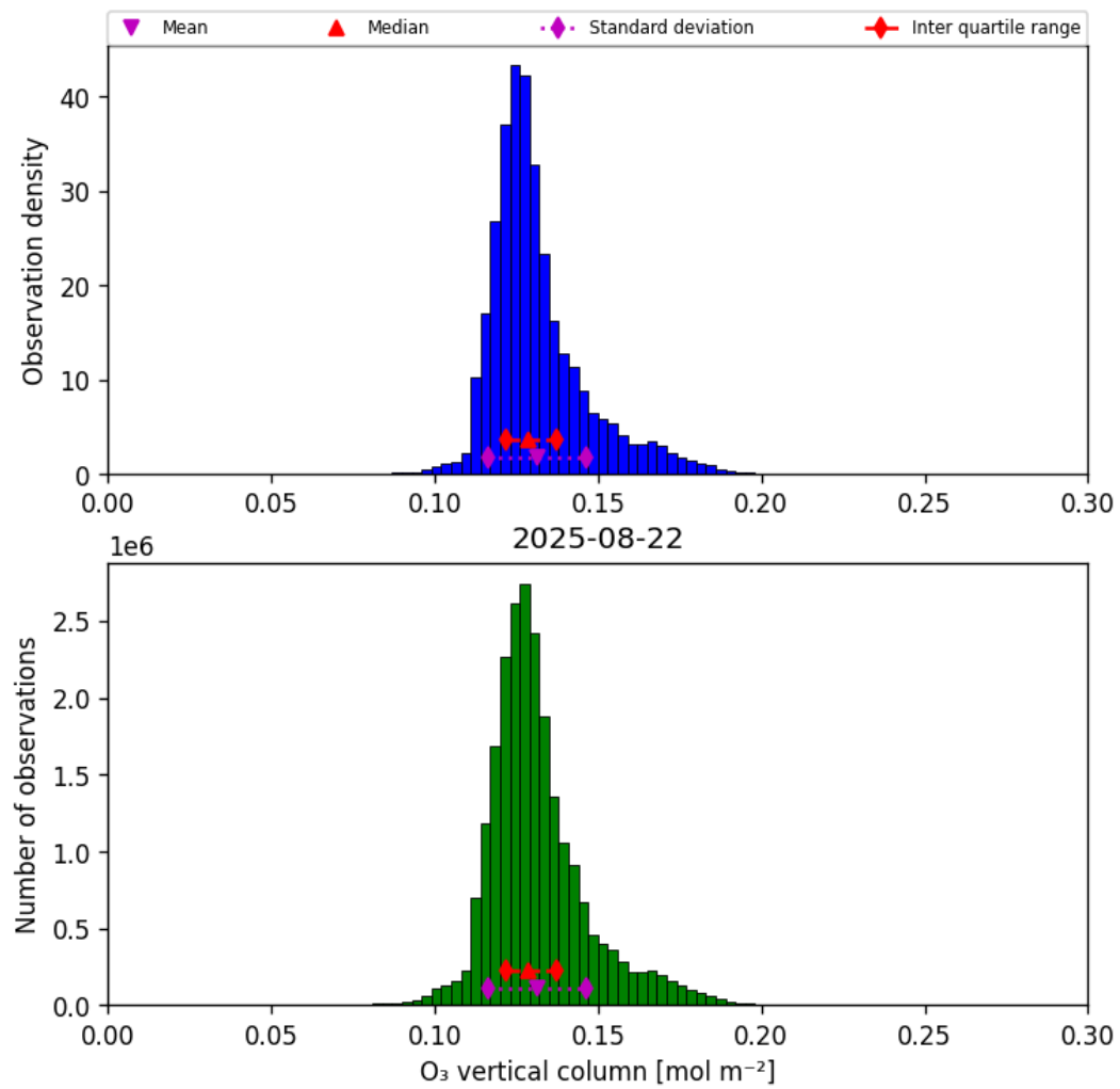
Figure 29: Histogram of “O 3 vertical column” for 2025-08-22 to 2025-08-23
