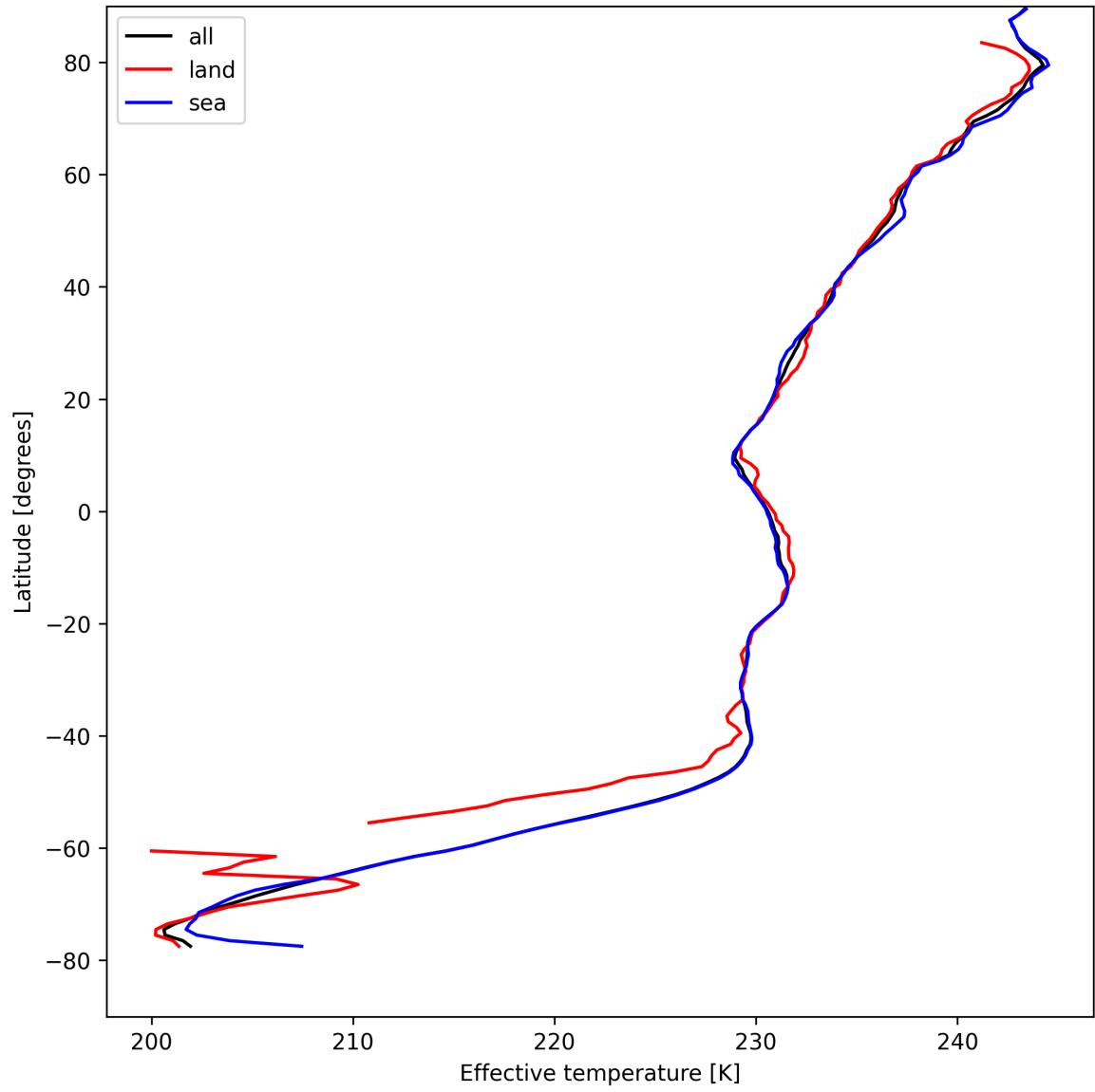
Figure 26: Zonal average of “Effective temperature” for 2025-08-22 to 2025-08-23.
