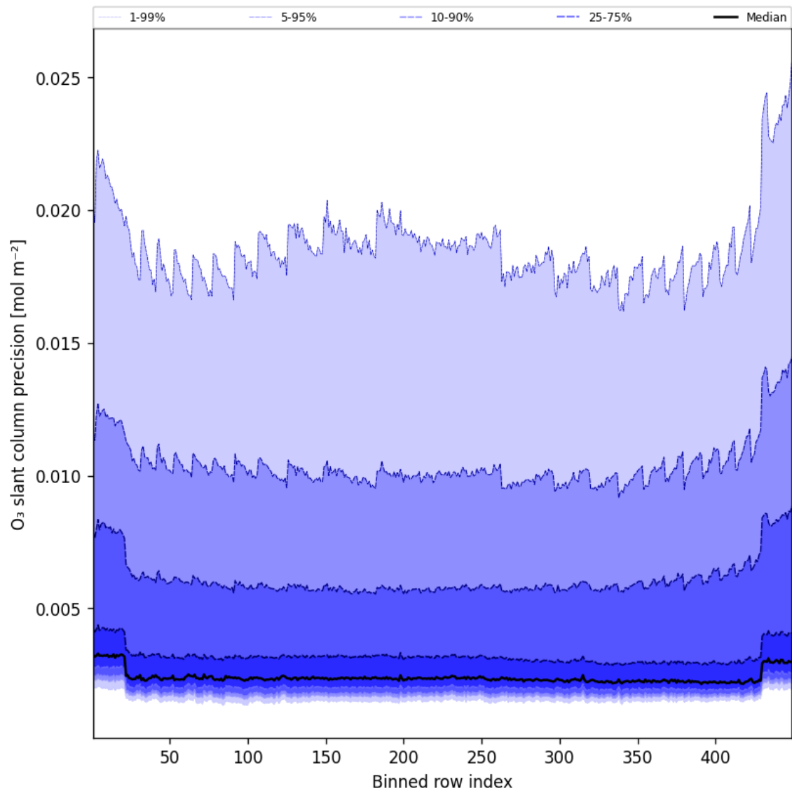
Figure 44: Along track statistics of “O 3 slant column precision” for 2025-08-22 to 2025-08-23
