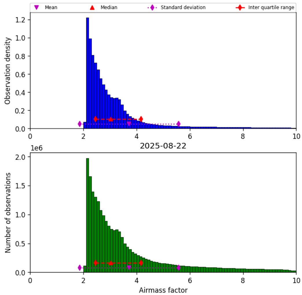
Figure 37: Histogram of “Airmass factor” for 2025-08-22 to 2025-08-23
