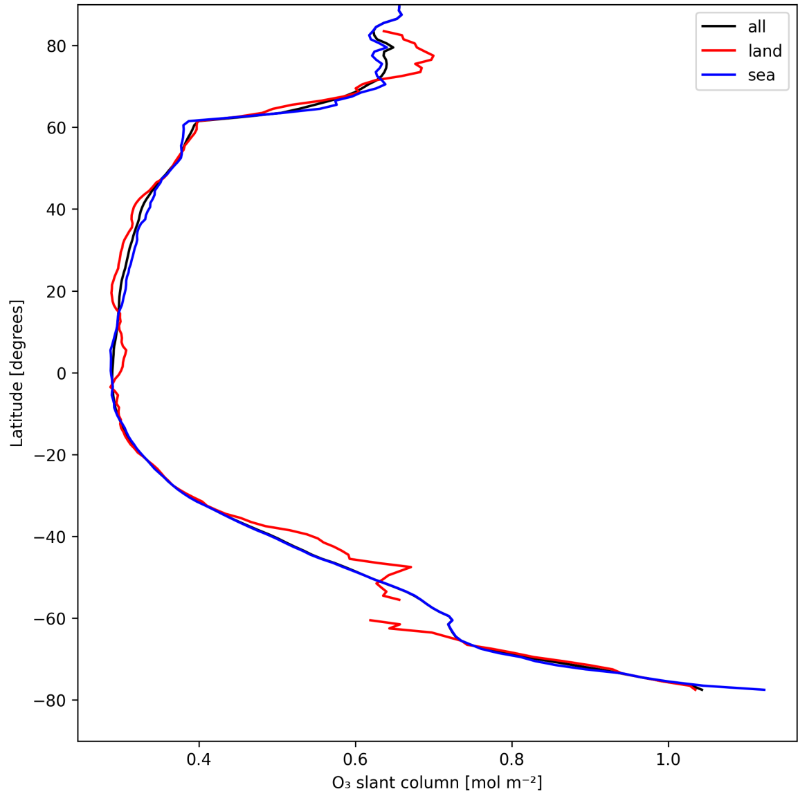
Figure 19: Zonal average of “O 3 slant column” for 2025-08-22 to 2025-08-23.
