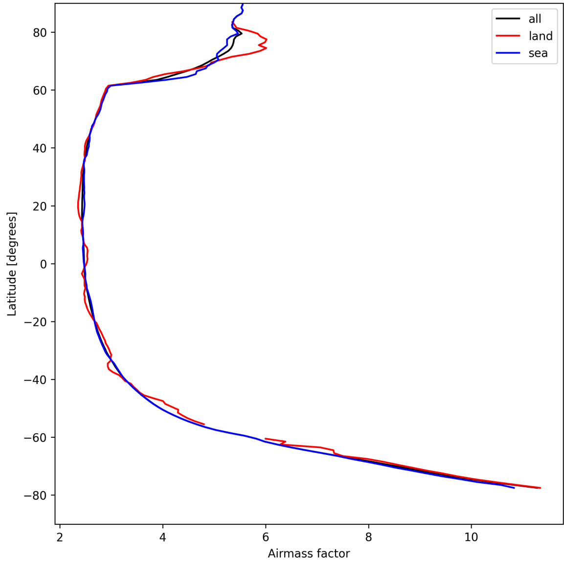
Figure 25: Zonal average of “Airmass factor” for 2025-08-22 to 2025-08-23.
