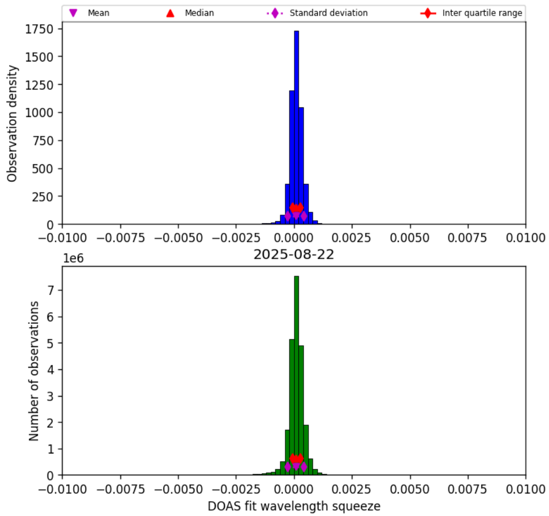
Figure 36: Histogram of “DOAS fit wavelength squeeze” for 2025-08-22 to 2025-08-23
