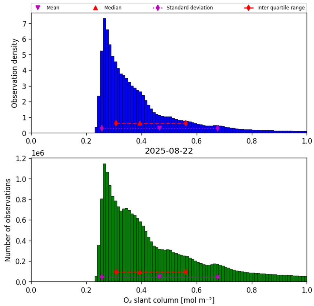
Figure 31: Histogram of “O 3 slant column” for 2025-08-22 to 2025-08-23
