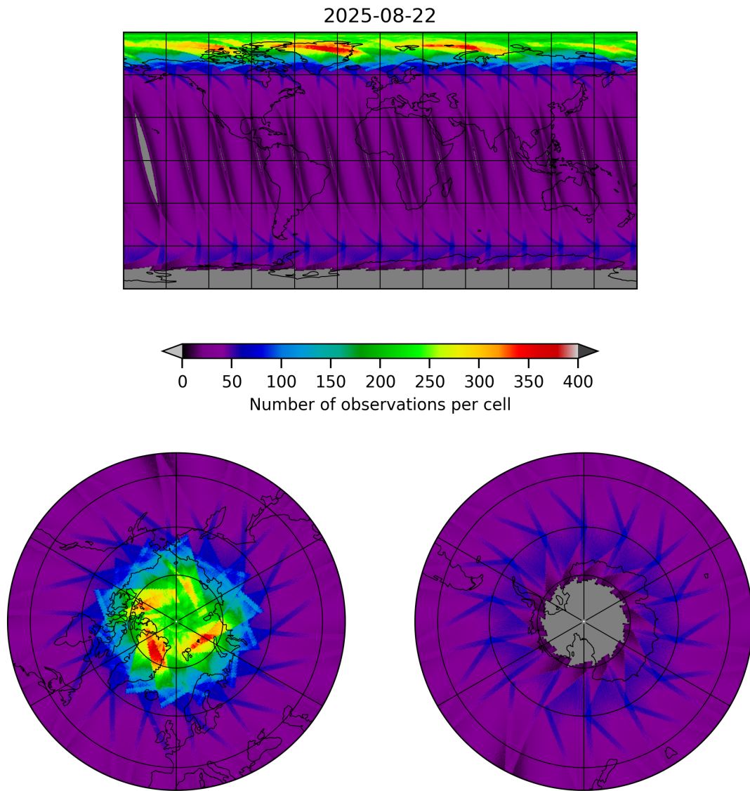
Figure 15: Map of the number of observations for 2025-08-22 to 2025-08-23
