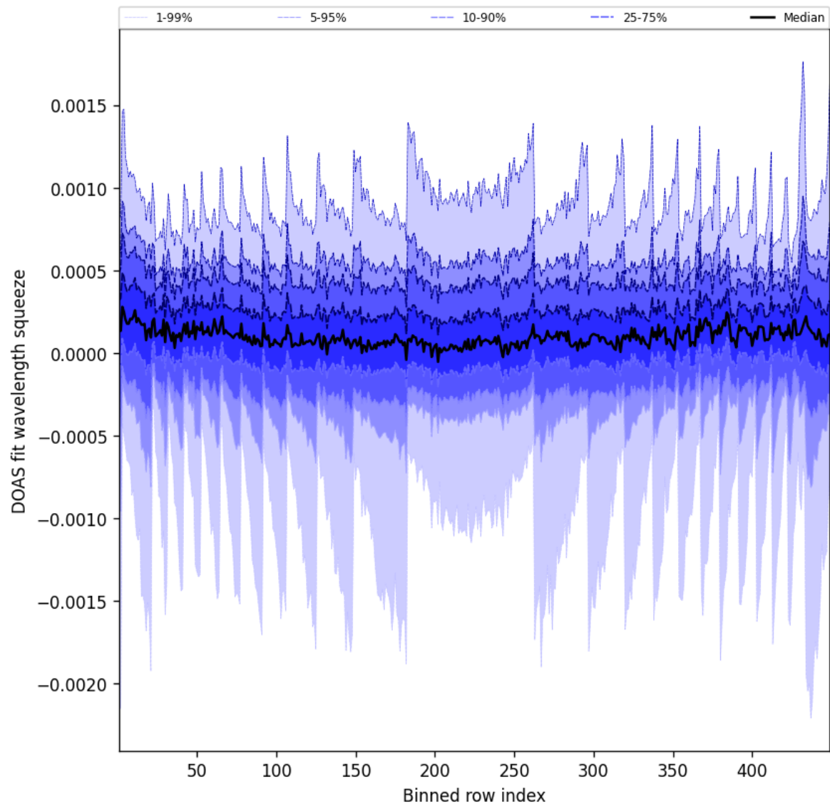
Figure 48: Along track statistics of “DOAS fit wavelength squeeze” for 2025-08-22 to 2025-08-23
