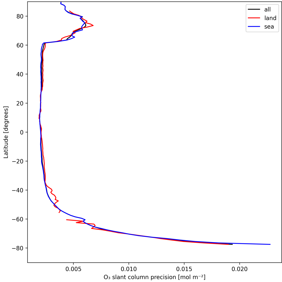
Figure 20: Zonal average of “O 3 slant column precision” for 2025-08-22 to 2025-08-23.
