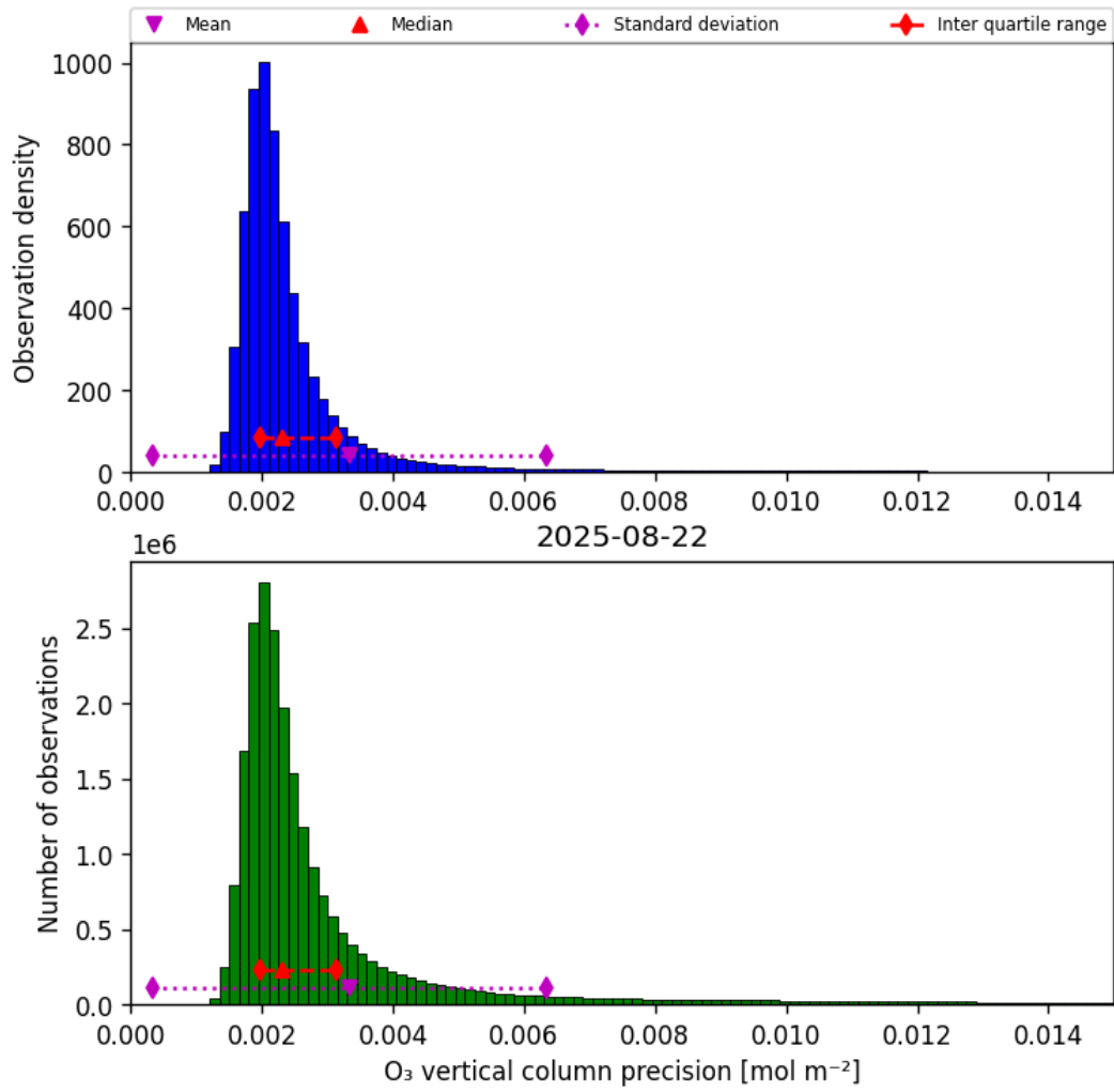
Figure 30: Histogram of “O 3 vertical column precision” for 2025-08-22 to 2025-08-23
