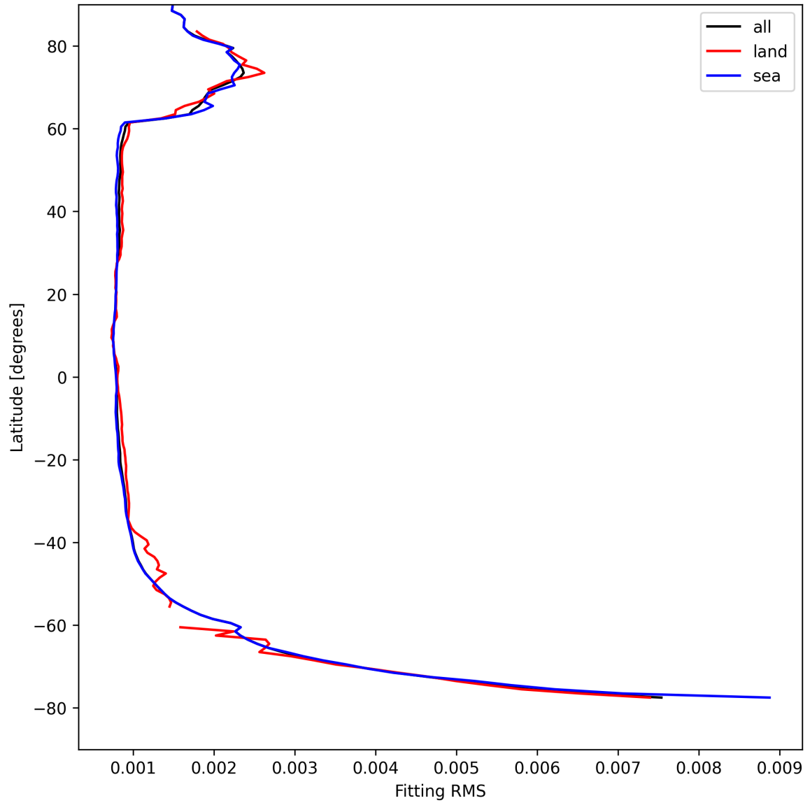
Figure 22: Zonal average of “Fitting RMS” for 2025-08-22 to 2025-08-23.
