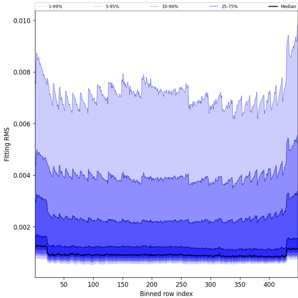
Figure 46: Along track statistics of “Fitting RMS” for 2025-08-22 to 2025-08-23
