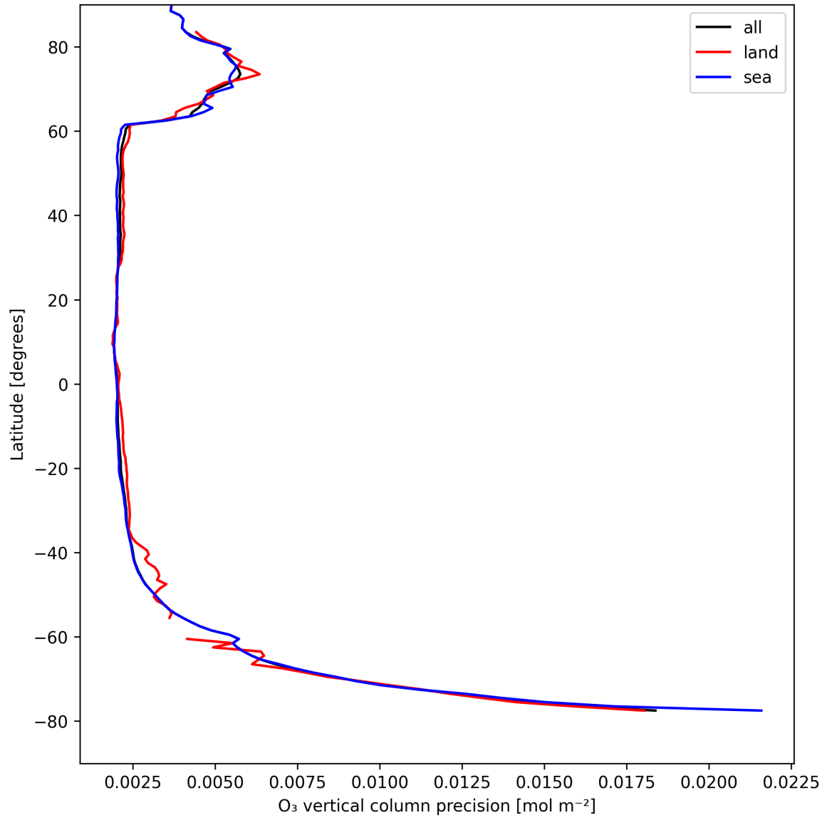
Figure 18: Zonal average of "O 3 vertical column precision" for 2025-08-22 to 2025-08-23.
