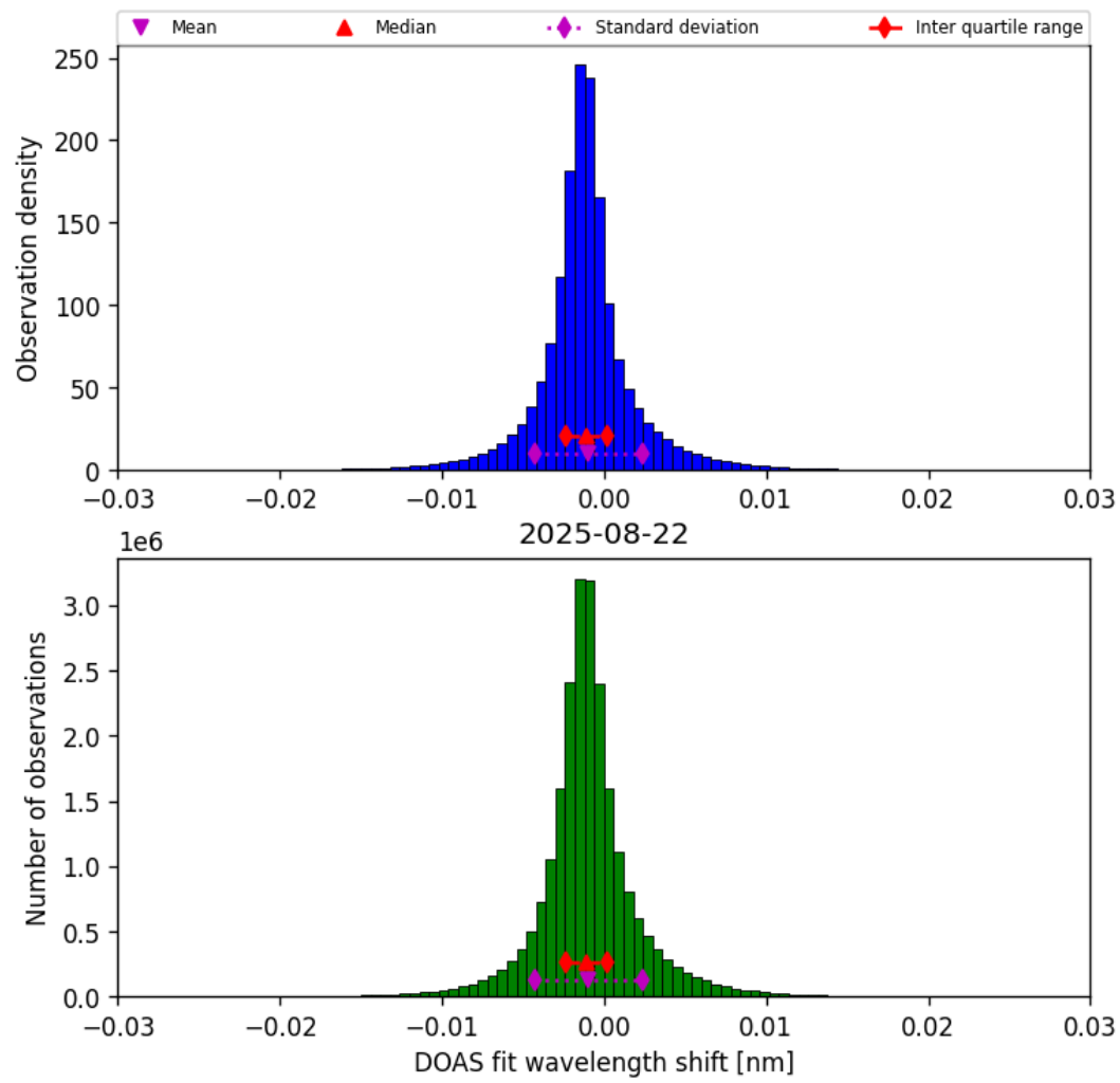
Figure 35: Histogram of “DOAS fit wavelength shift” for 2025-08-22 to 2025-08-23
