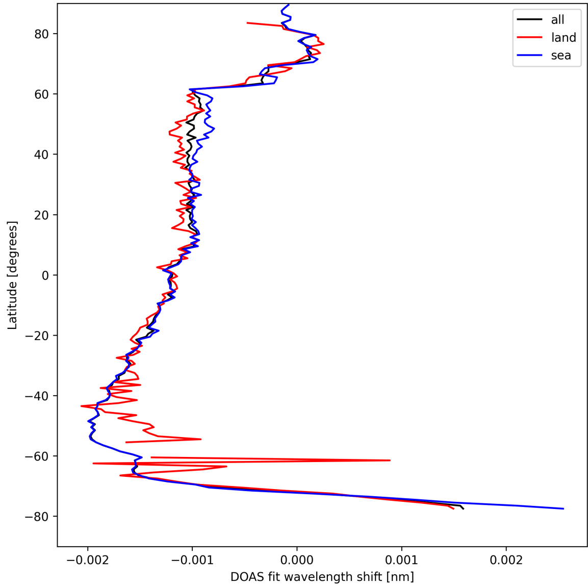
Figure 23: Zonal average of “DOAS fit wavelength shift” for 2025-08-22 to 2025-08-23.
