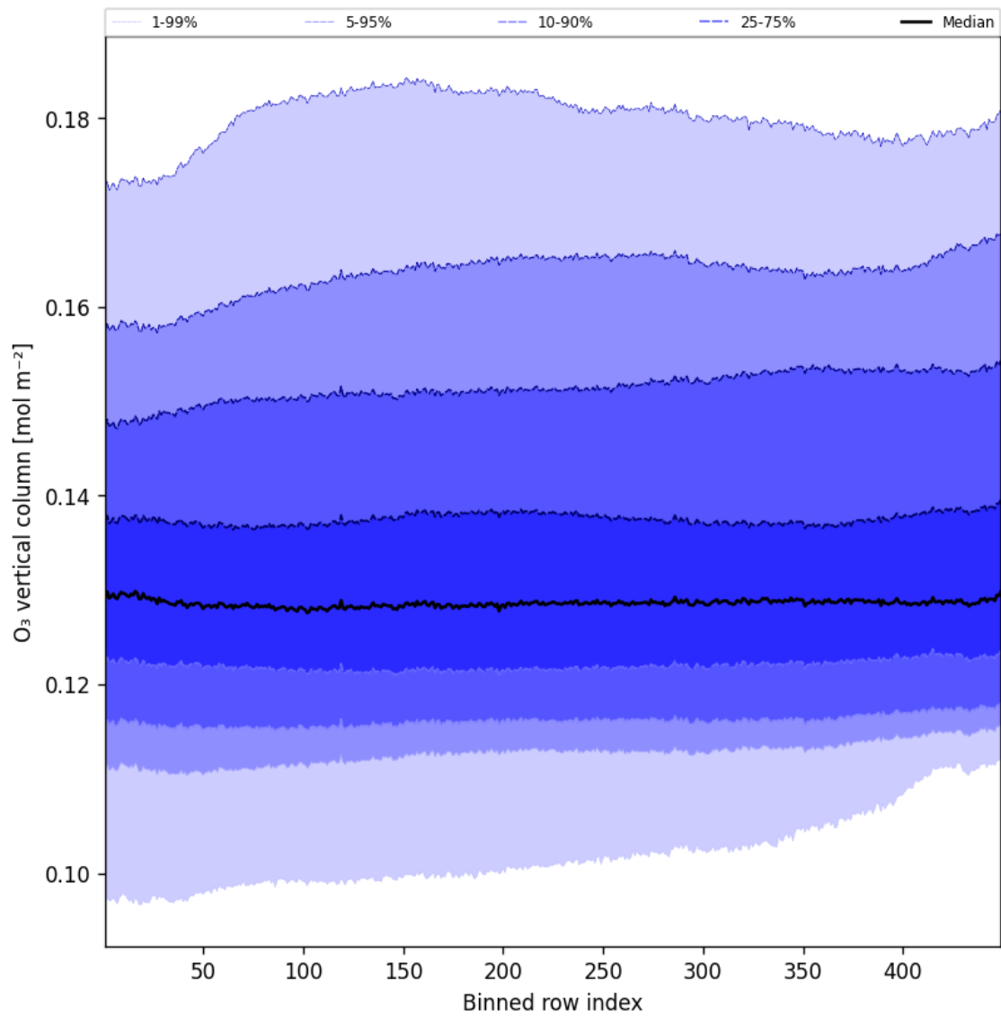
Figure 41: Along track statistics of “O 3 vertical column” for 2025-08-22 to 2025-08-23
