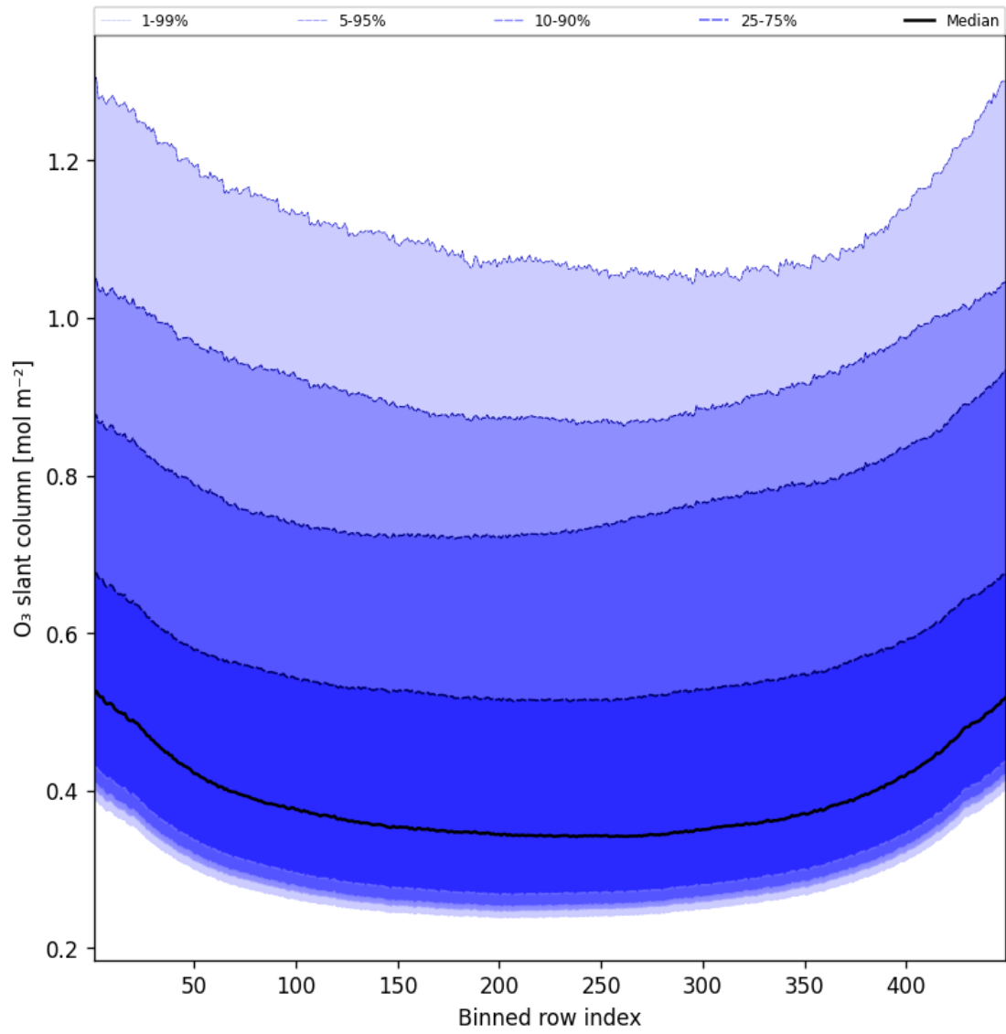
Figure 43: Along track statistics of “O 3 slant column” for 2025-08-22 to 2025-08-23
