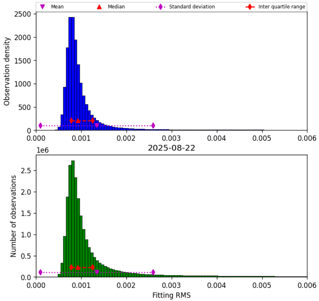
Figure 34: Histogram of “Fitting RMS” for 2025-08-22 to 2025-08-23
