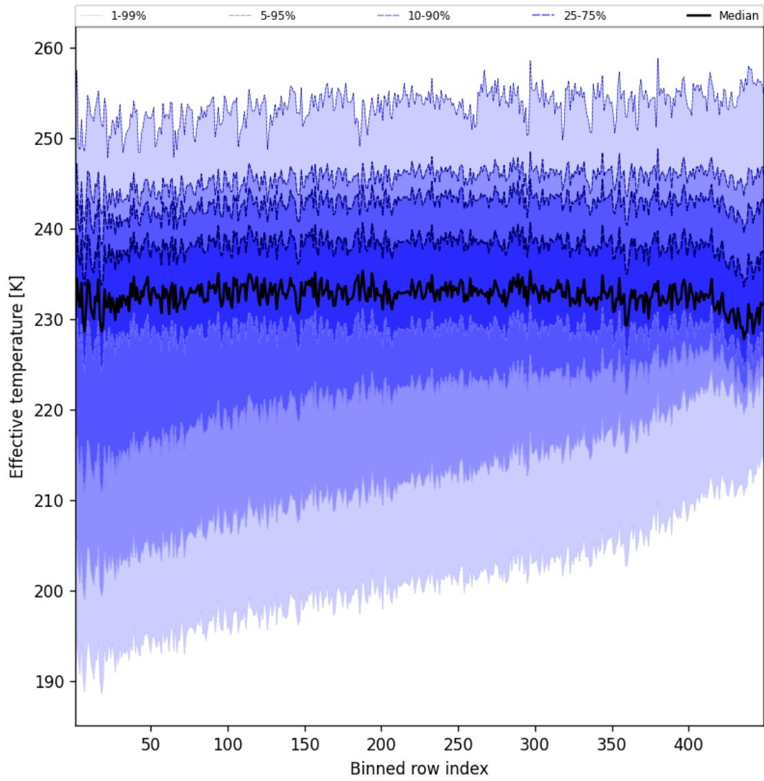
Figure 50: Along track statistics of “Effective temperature” for 2025-08-22 to 2025-08-23
