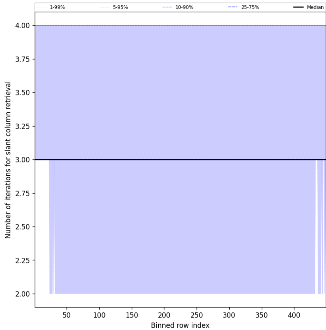
Figure 45: Along track statistics of “Number of iterations for slant column retrieval” for 2025-08-22 to 2025-08-23
