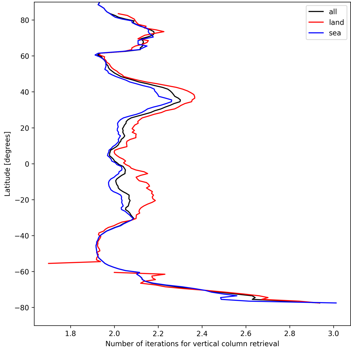
Figure 27: Zonal average of “Number of iterations for vertical column retrieval” for 2025-08-22 to 2025-08-23.
