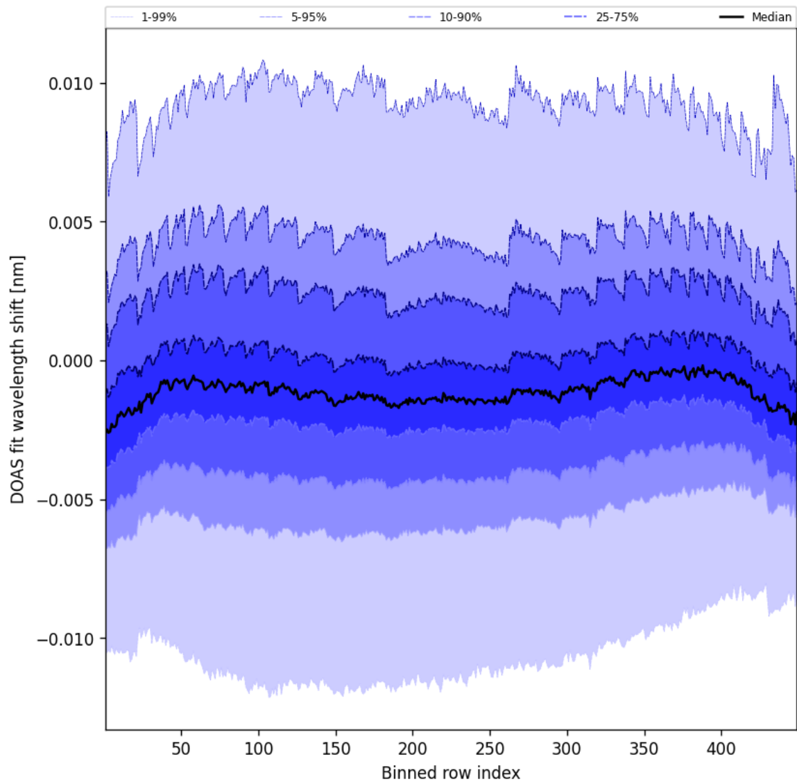
Figure 47: Along track statistics of “DOAS fit wavelength shift” for 2025-08-22 to 2025-08-23
