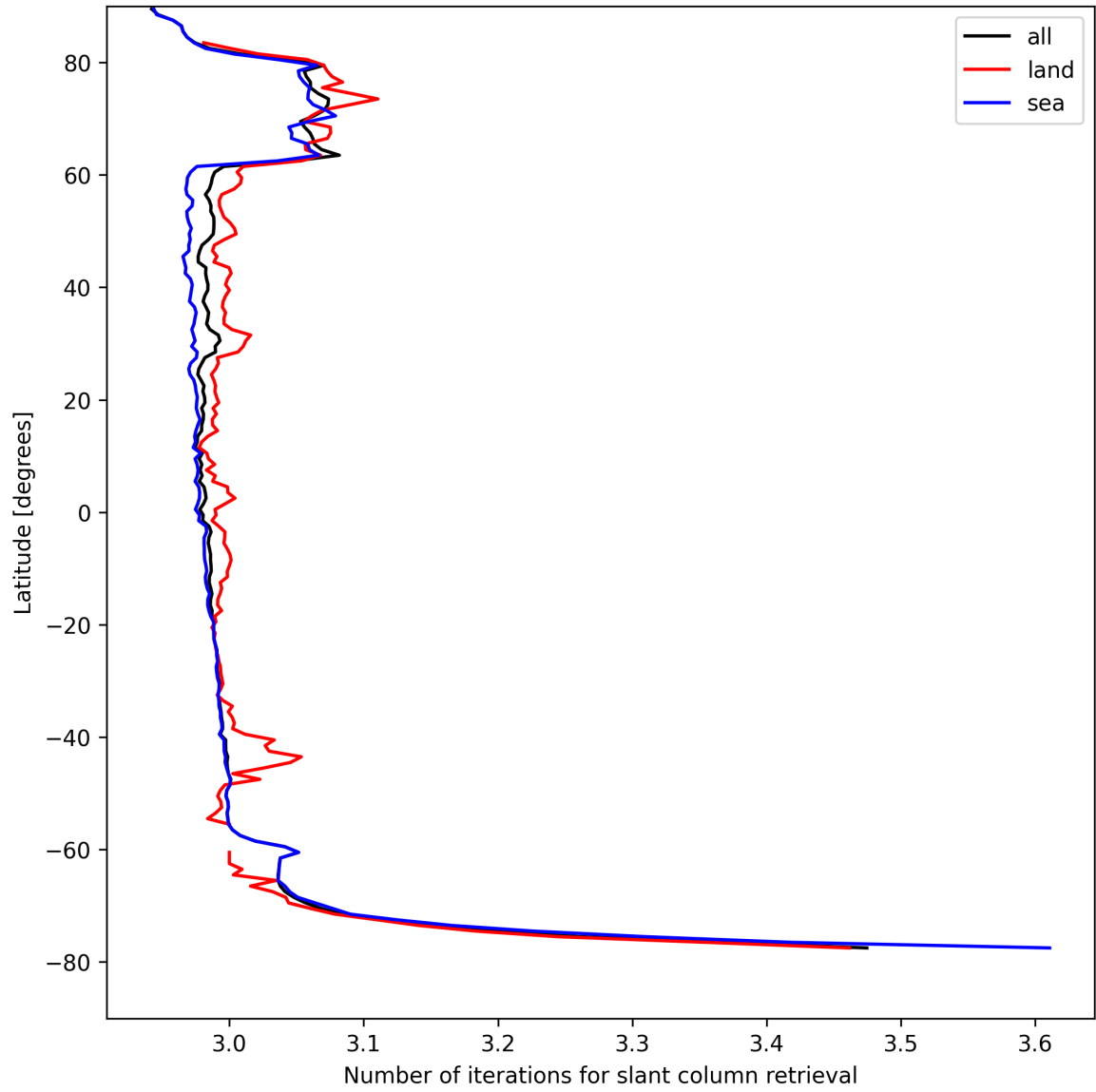
Figure 21: Zonal average of “Number of iterations for slant column retrieval” for 2025-08-22 to 2025-08-23.
