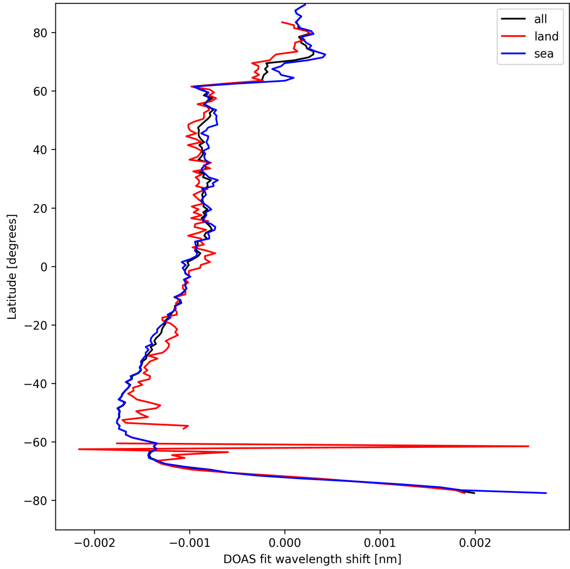
Figure 23: Zonal average of “DOAS fit wavelength shift” for 2025-08-23 to 2025-08-23.
