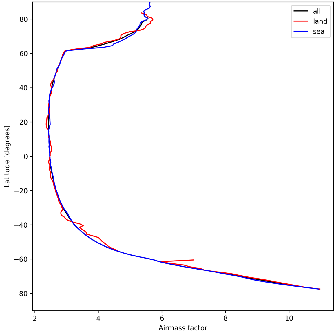
Figure 25: Zonal average of “Airmass factor” for 2025-08-23 to 2025-08-23.
