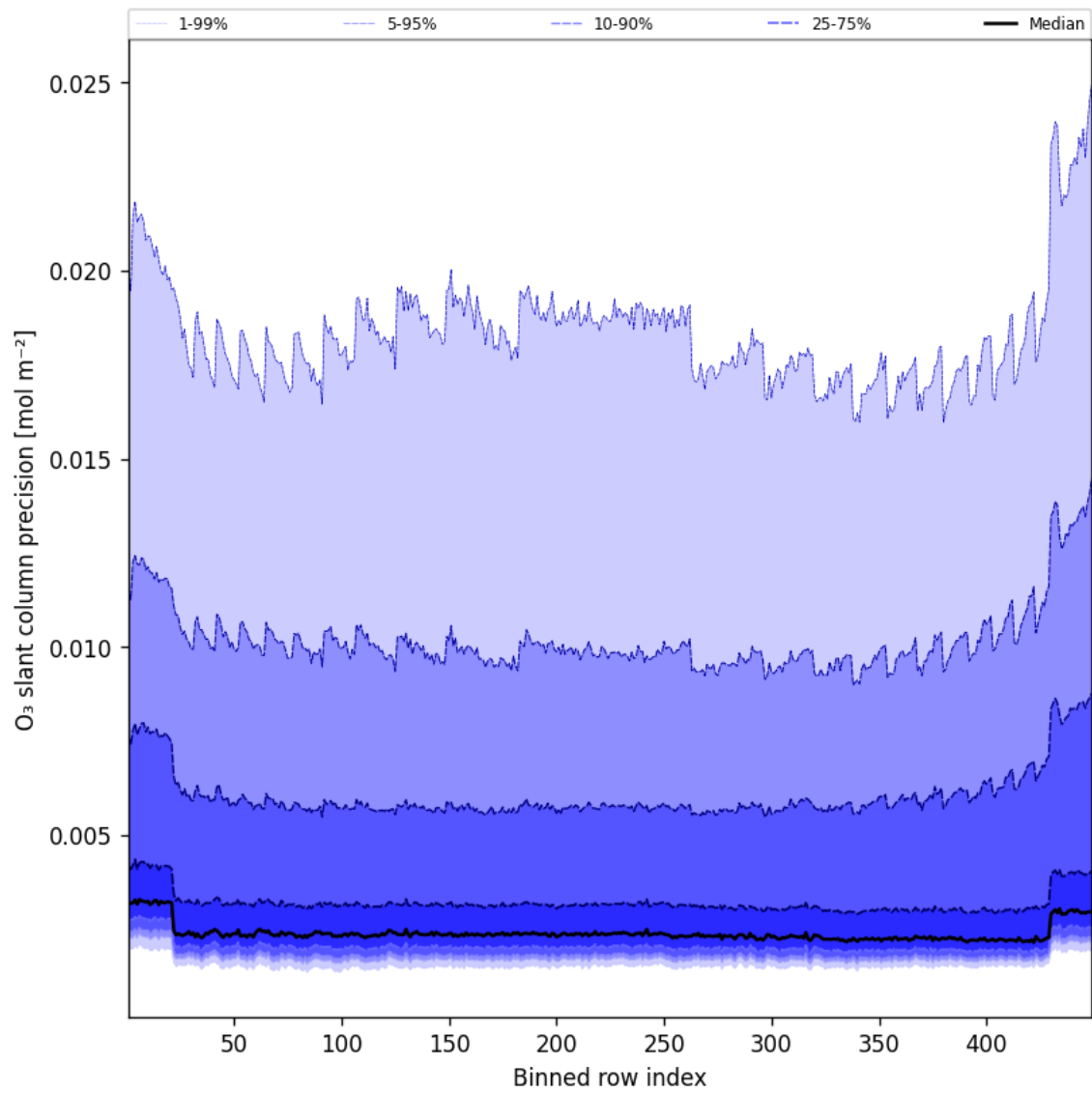
Figure 44: Along track statistics of “O 3 slant column precision” for 2025-08-23 to 2025-08-23
