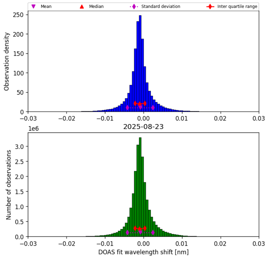
Figure 35: Histogram of “DOAS fit wavelength shift” for 2025-08-23 to 2025-08-23
