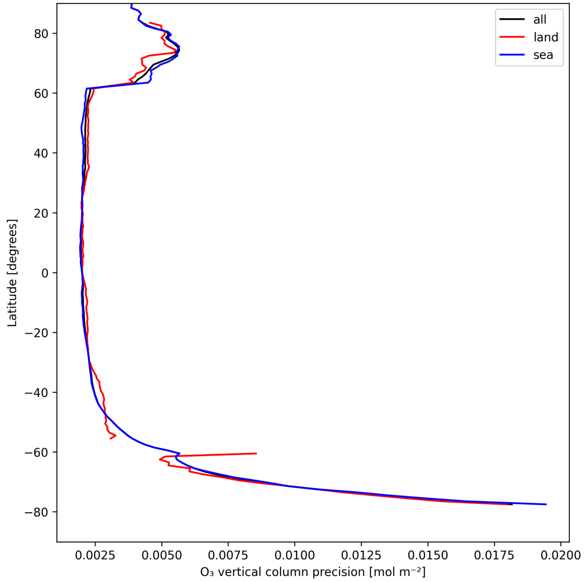
Figure 18: Zonal average of “O 3 vertical column precision” for 2025-08-23 to 2025-08-23.
