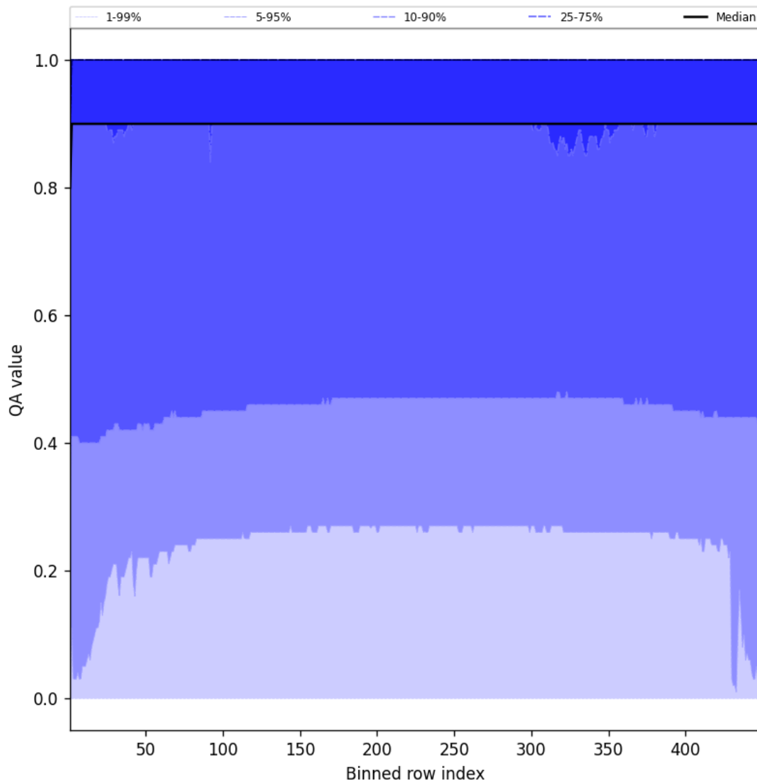
Figure 40: Along track statistics of “QA value” for 2025-08-23 to 2025-08-23
