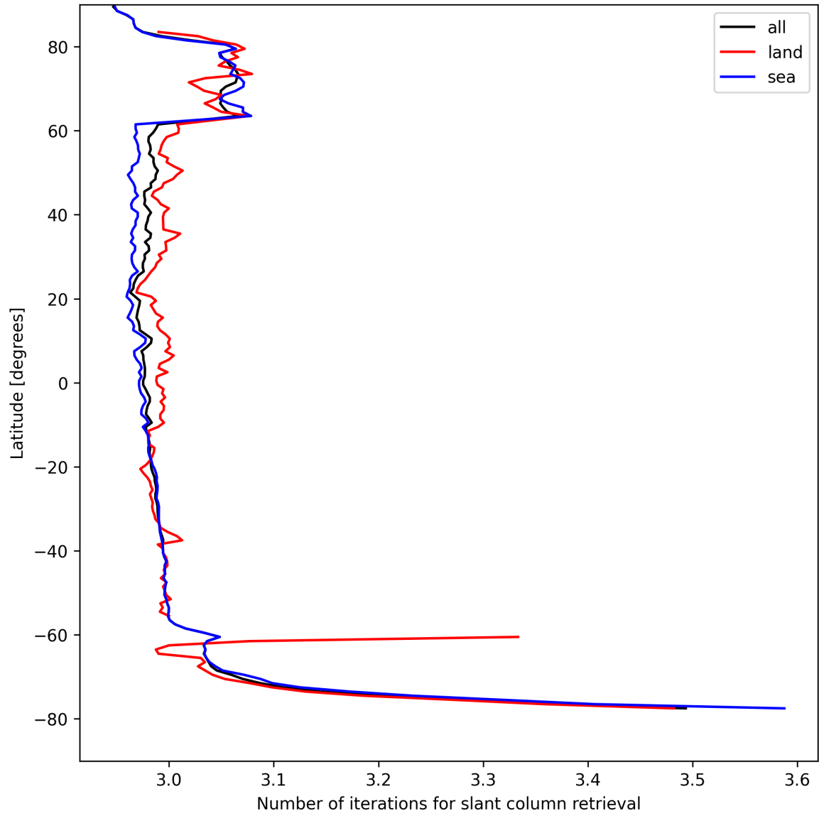
Figure 21: Zonal average of “Number of iterations for slant column retrieval” for 2025-08-23 to 2025-08-23.
