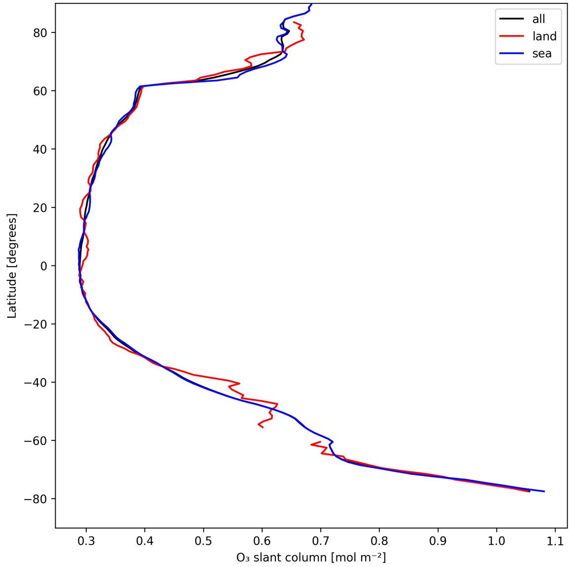
Figure 19: Zonal average of “O 3 slant column” for 2025-08-23 to 2025-08-23.
