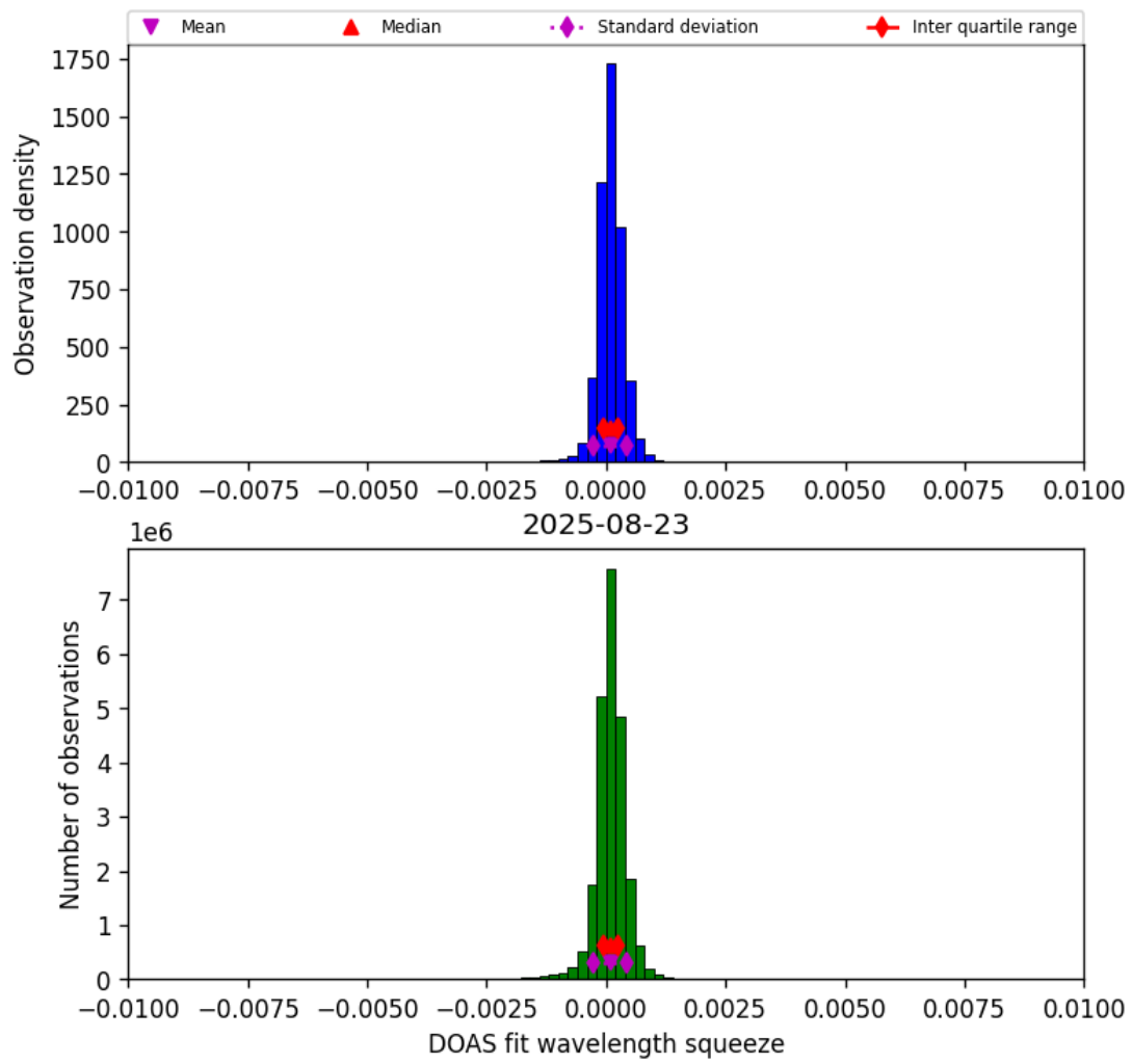
Figure 36: Histogram of “DOAS fit wavelength squeeze” for 2025-08-23 to 2025-08-23
