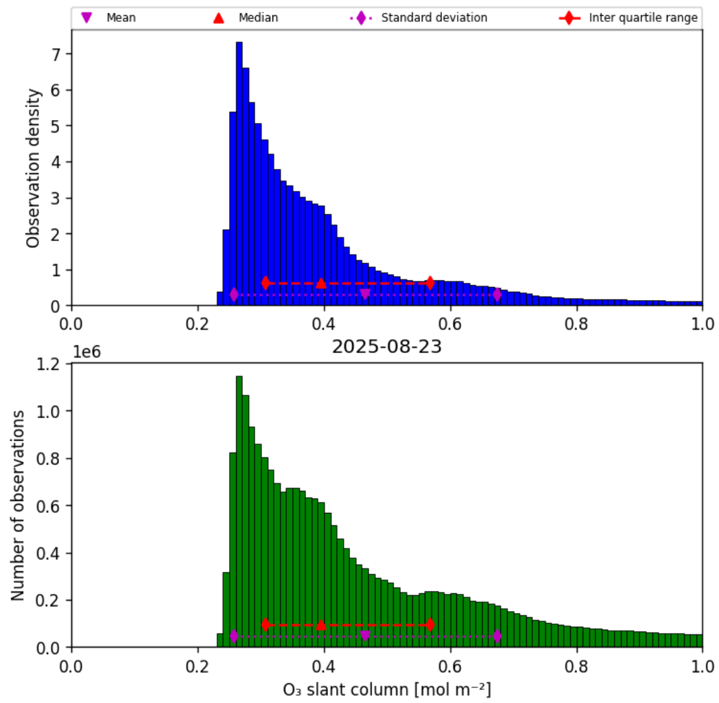
Figure 31: Histogram of “O 3 slant column” for 2025-08-23 to 2025-08-23
