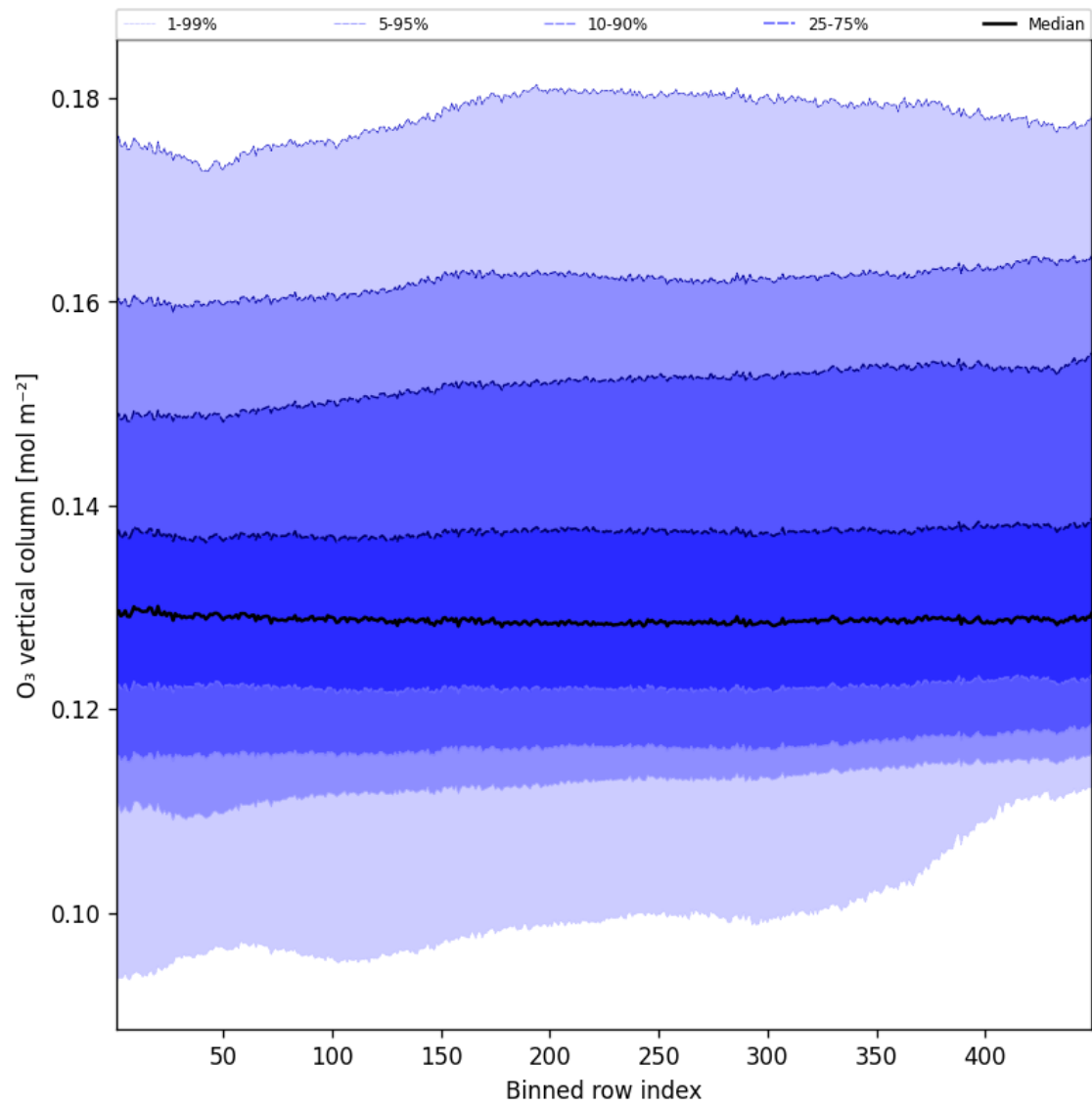
Figure 41: Along track statistics of “O 3 vertical column” for 2025-08-23 to 2025-08-23
