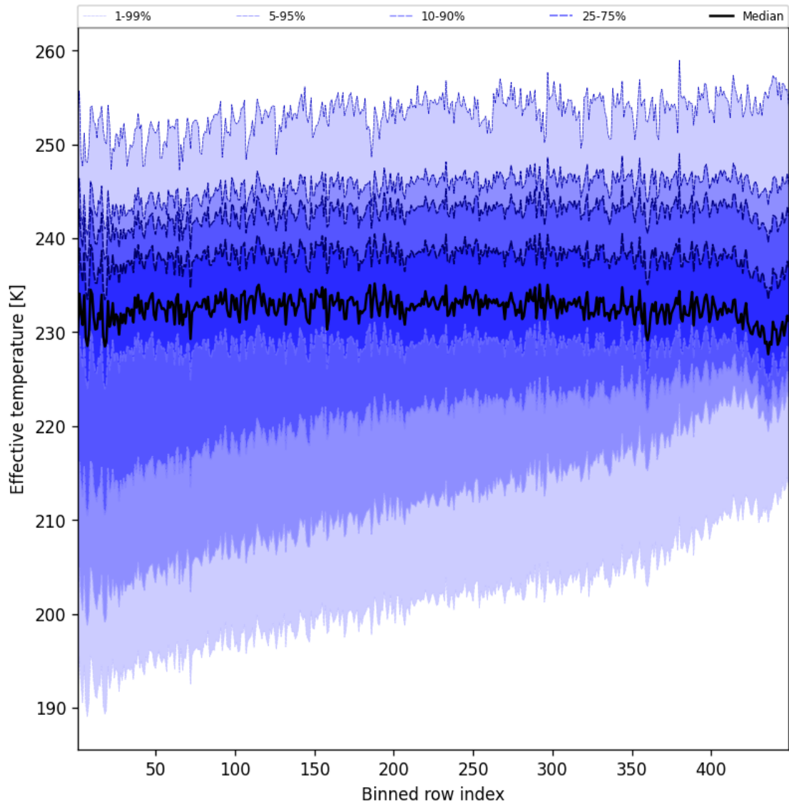
Figure 50: Along track statistics of “Effective temperature” for 2025-08-23 to 2025-08-23
