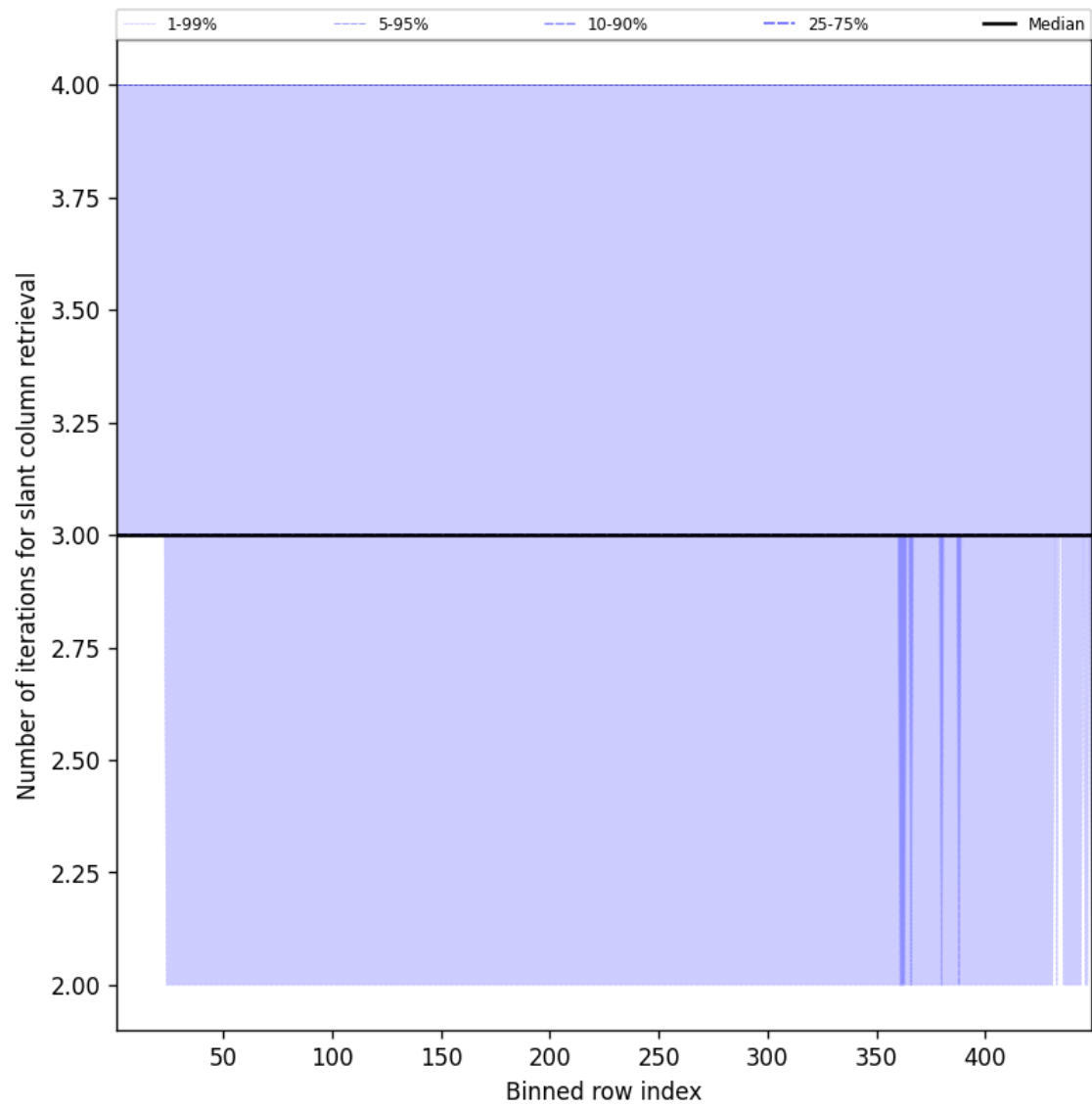
Figure 45: Along track statistics of “Number of iterations for slant column retrieval” for 2025-08-23 to 2025-08-23
