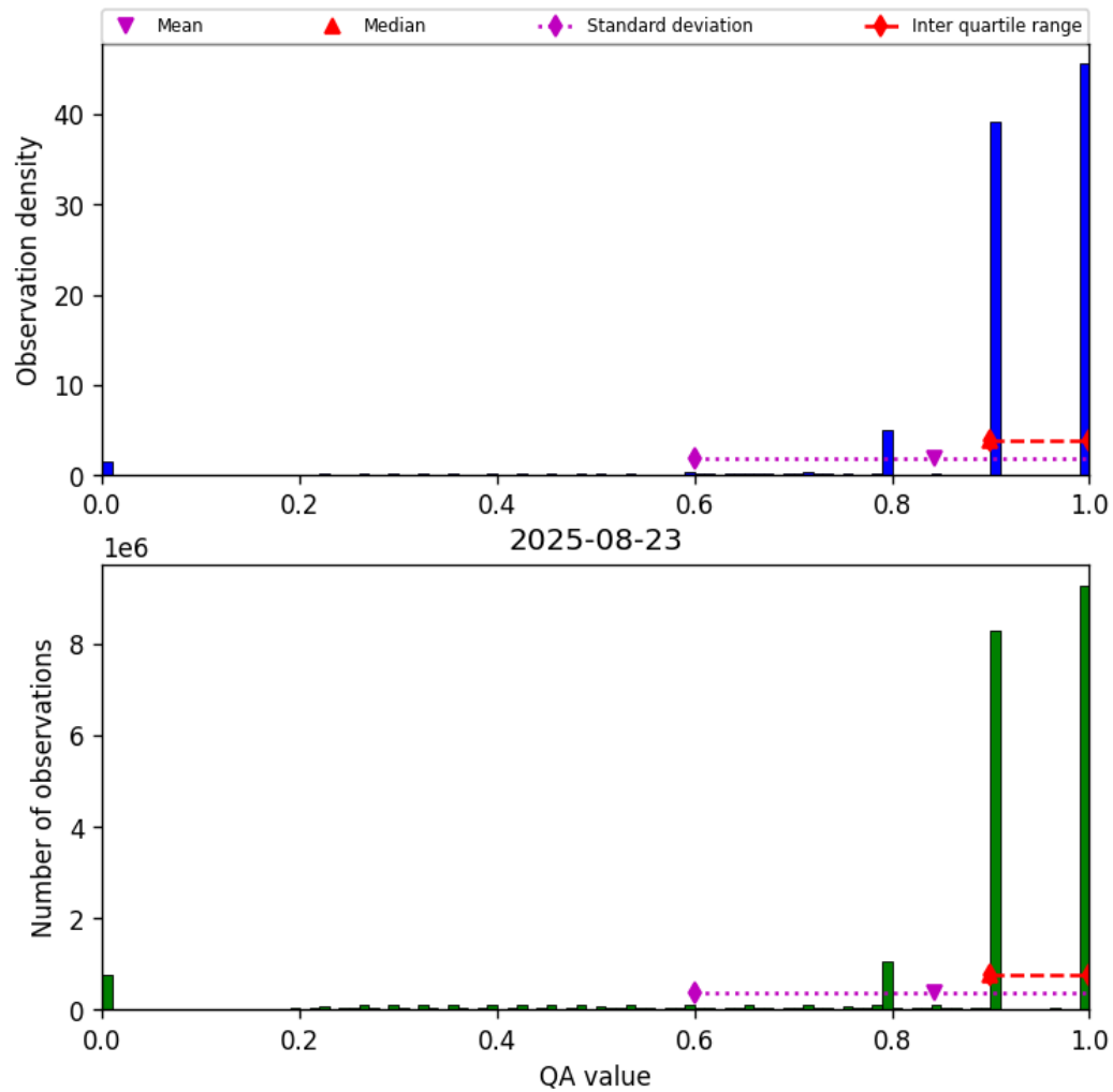
Figure 28: Histogram of “QA value” for 2025-08-23 to 2025-08-23
