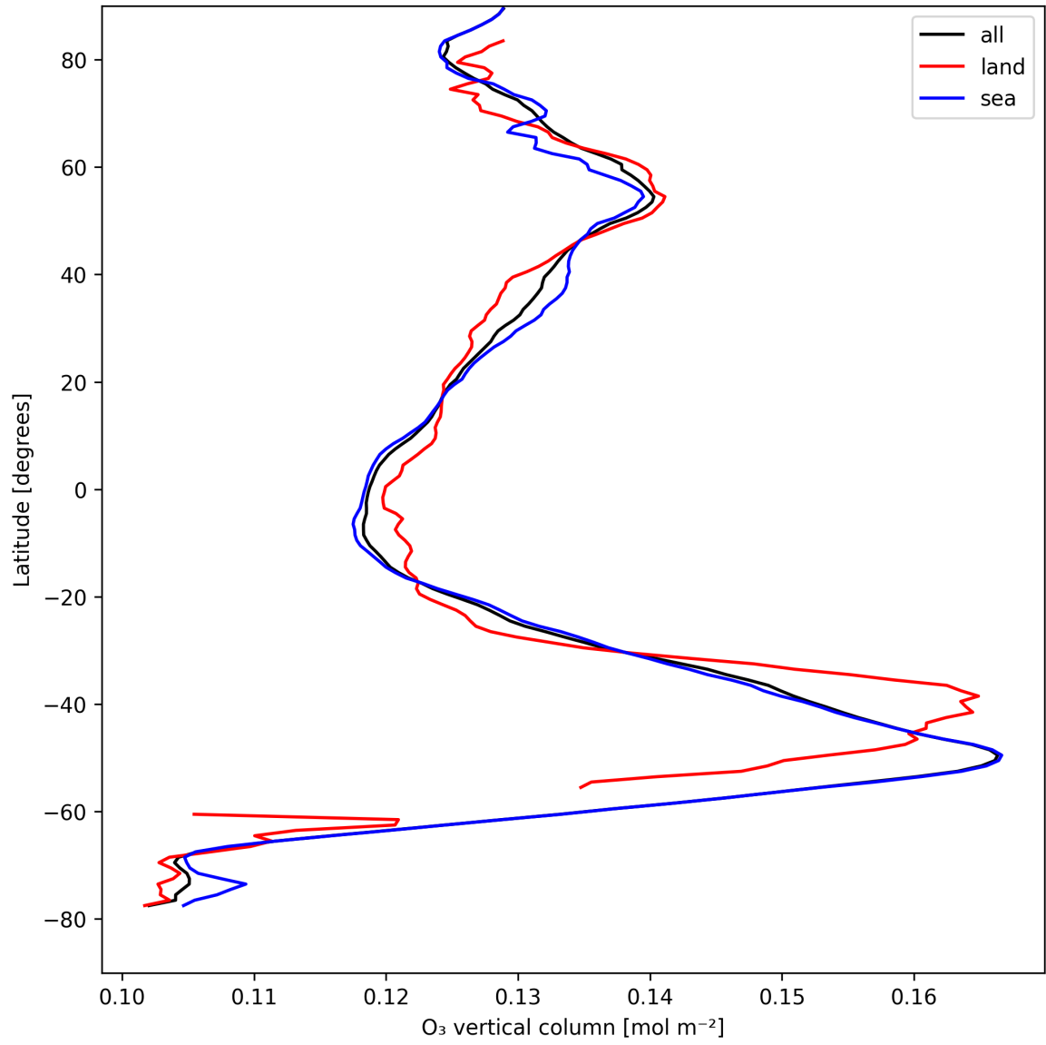
Figure 17: Zonal average of “O 3 vertical column” for 2025-08-23 to 2025-08-23.
