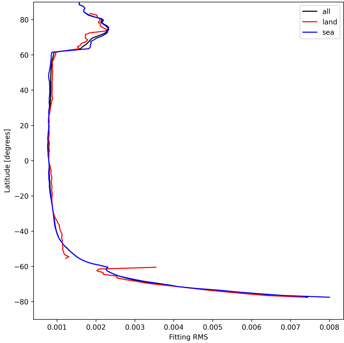
Figure 22: Zonal average of “Fitting RMS” for 2025-08-23 to 2025-08-23.
