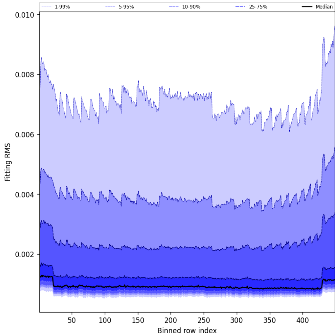
Figure 46: Along track statistics of “Fitting RMS” for 2025-08-23 to 2025-08-23
