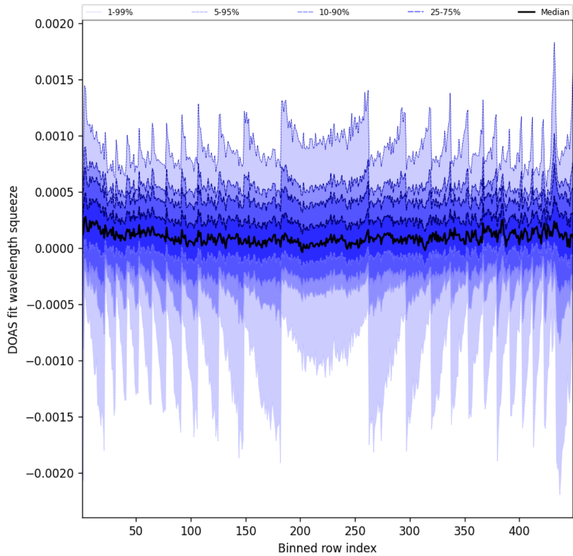
Figure 48: Along track statistics of “DOAS fit wavelength squeeze” for 2025-08-23 to 2025-08-23
