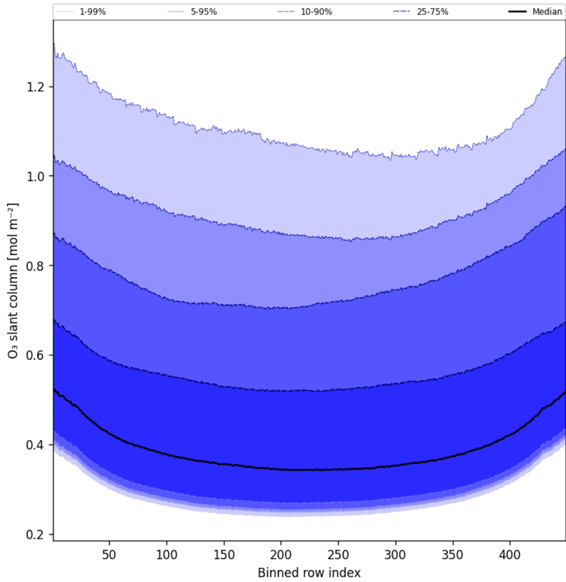
Figure 43: Along track statistics of “O 3 slant column” for 2025-08-23 to 2025-08-23
