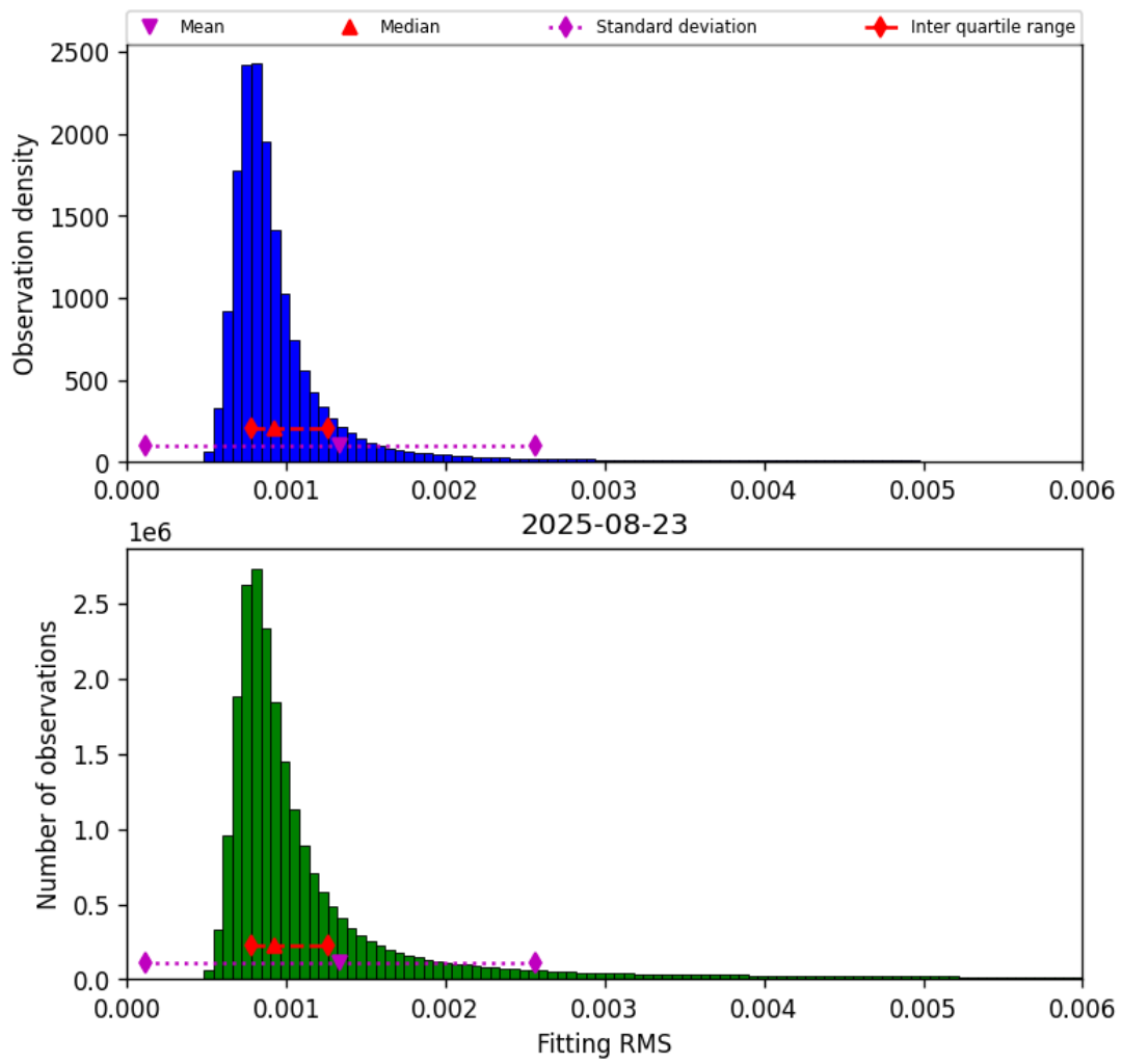
Figure 34: Histogram of “Fitting RMS” for 2025-08-23 to 2025-08-23
