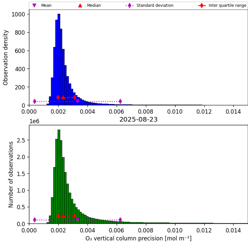
Figure 30: Histogram of “O 3 vertical column precision” for 2025-08-23 to 2025-08-23
