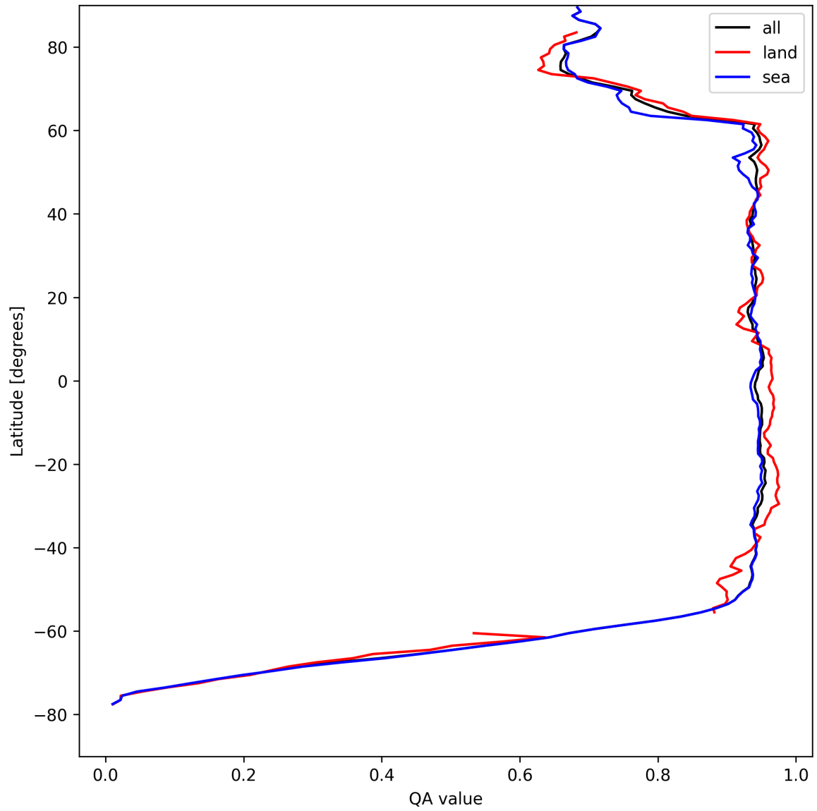
Figure 16: Zonal average of “QA value” for 2025-08-23 to 2025-08-23.
