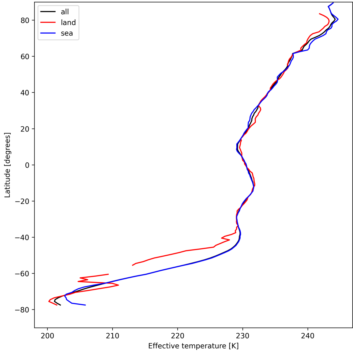
Figure 26: Zonal average of "Effective temperature" for 2025-08-23 to 2025-08-23.
