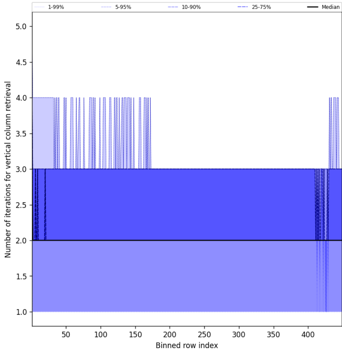
Figure 51: Along track statistics of “Number of iterations for vertical column retrieval” for 2025-08-23 to 2025-08-23
