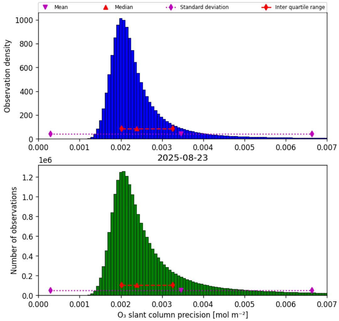
Figure 32: Histogram of “O 3 slant column precision” for 2025-08-23 to 2025-08-23
