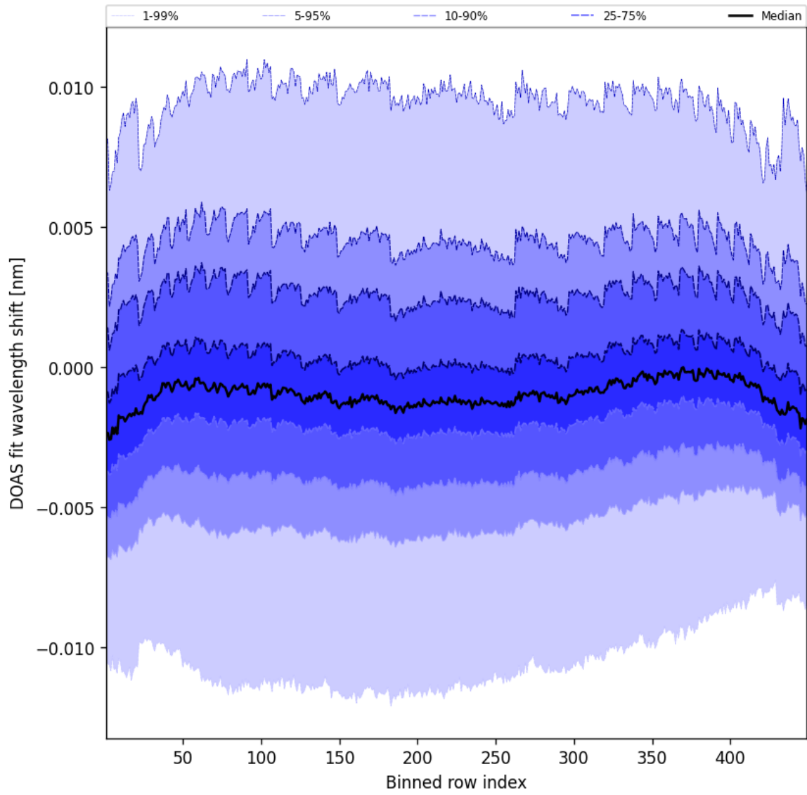
Figure 47: Along track statistics of “DOAS fit wavelength shift” for 2025-08-23 to 2025-08-23
