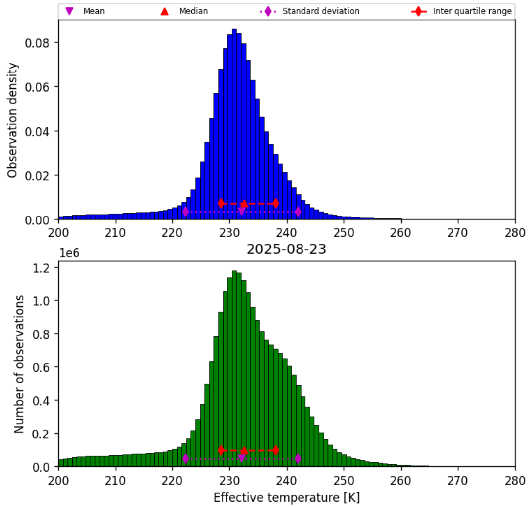
Figure 38: Histogram of “Effective temperature” for 2025-08-23 to 2025-08-23
