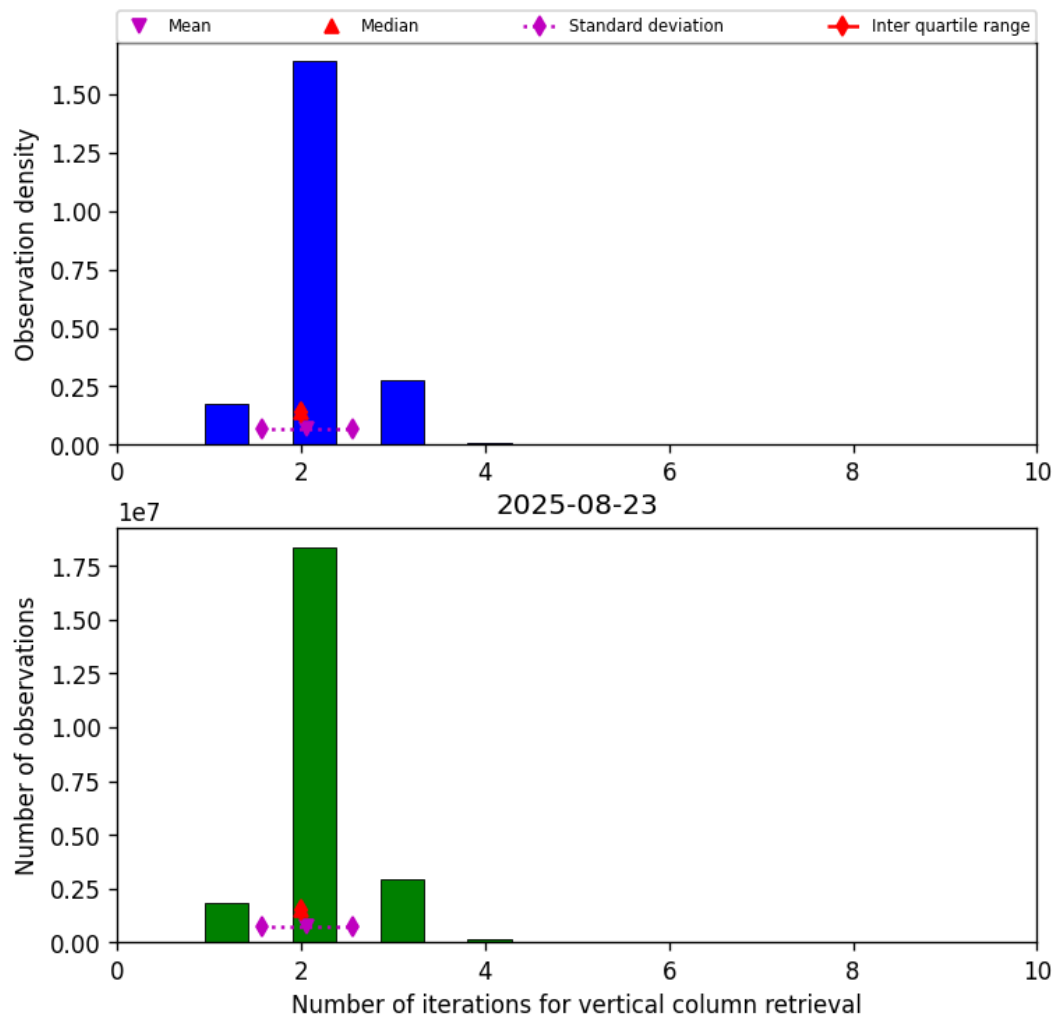
Figure 39: Histogram of “Number of iterations for vertical column retrieval” for 2025-08-23 to 2025-08-23
