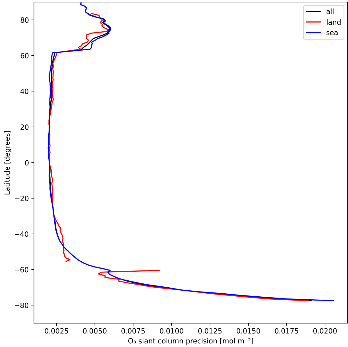
Figure 20: Zonal average of “O 3 slant column precision” for 2025-08-23 to 2025-08-23.
