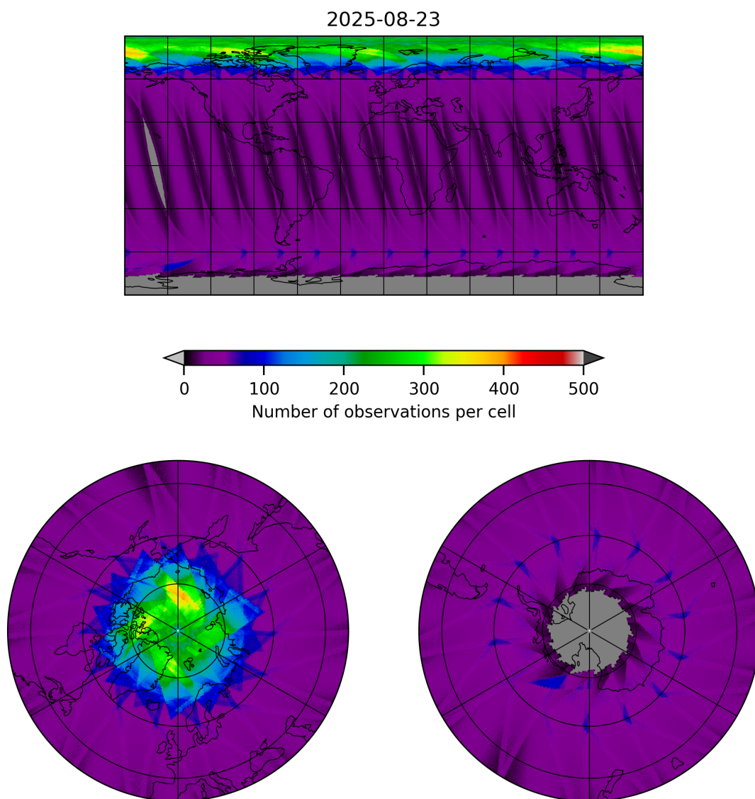
Figure 15: Map of the number of observations for 2025-08-23 to 2025-08-23
