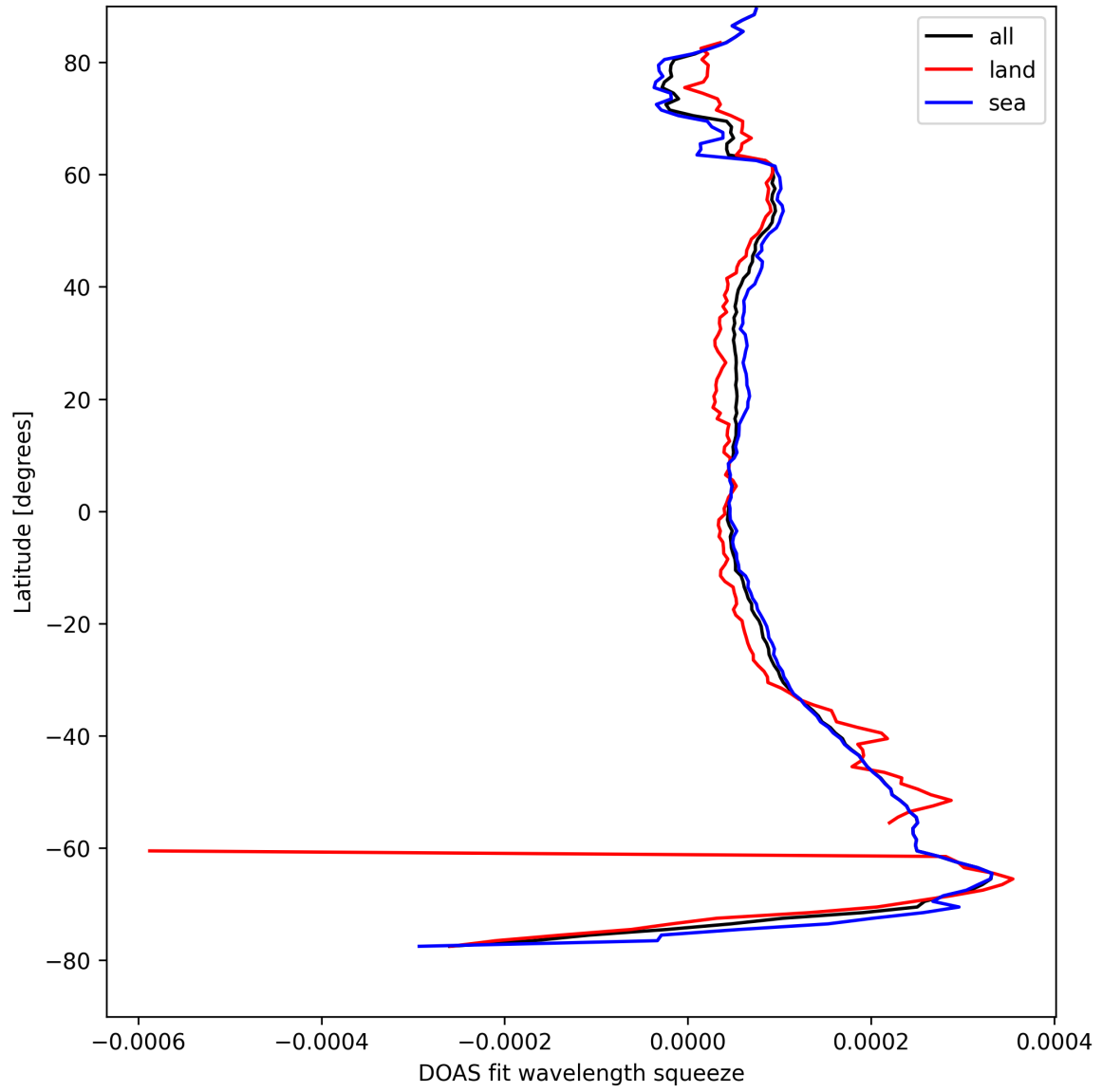
Figure 24: Zonal average of “DOAS fit wavelength squeeze” for 2025-08-23 to 2025-08-23.
