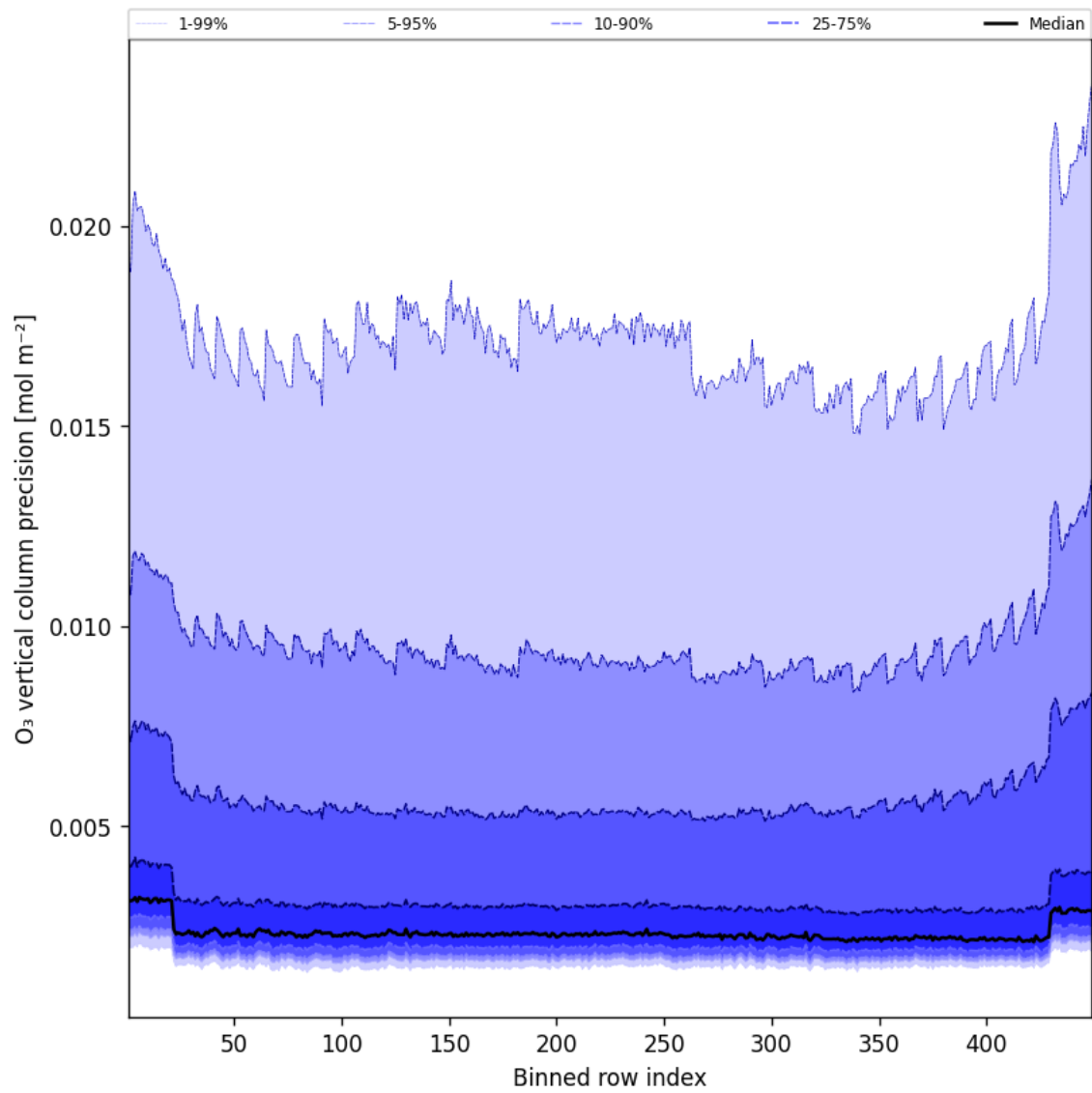
Figure 42: Along track statistics of “O 3 vertical column precision” for 2025-08-23 to 2025-08-23
