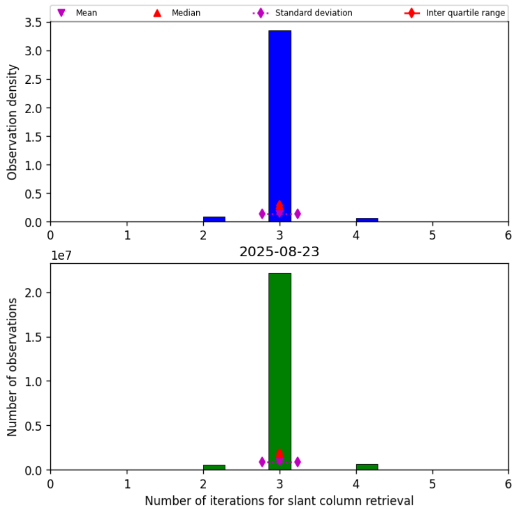
Figure 33: Histogram of “Number of iterations for slant column retrieval” for 2025-08-23 to 2025-08-23
