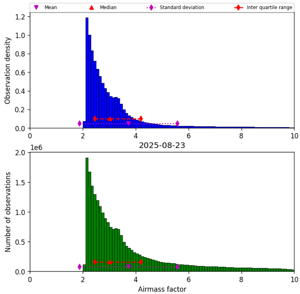
Figure 37: Histogram of “Airmass factor” for 2025-08-23 to 2025-08-23
