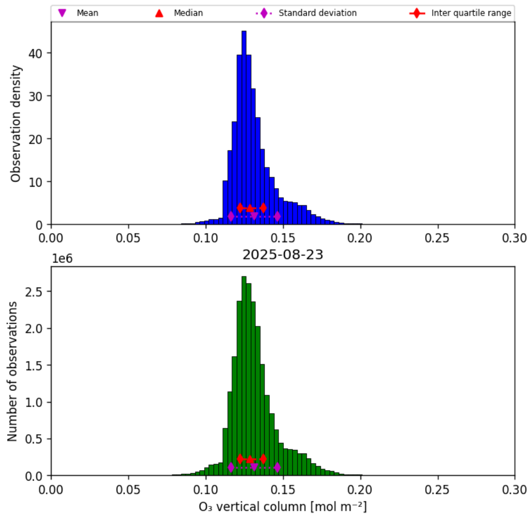
Figure 29: Histogram of “O 3 vertical column” for 2025-08-23 to 2025-08-23
