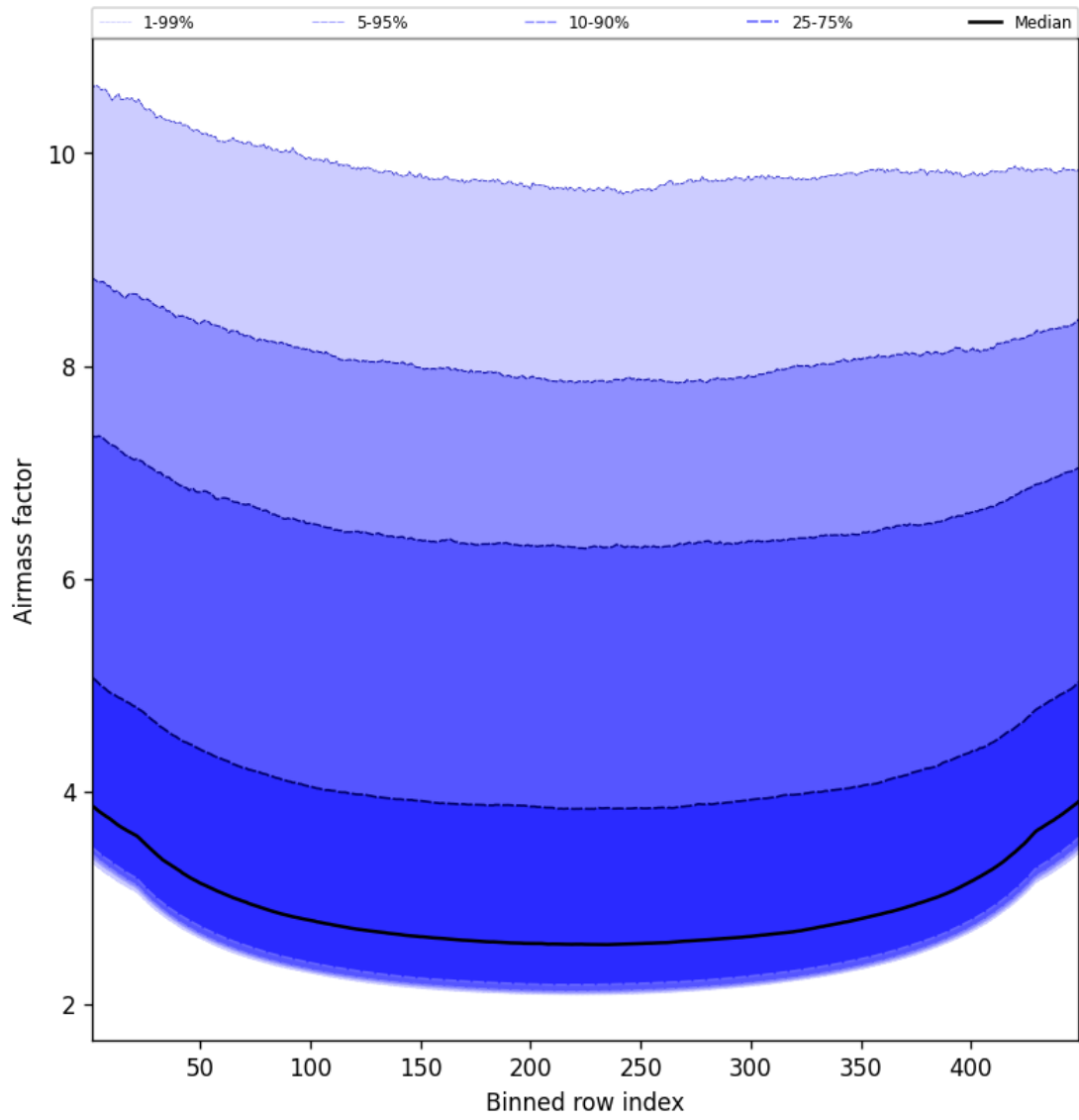
Figure 49: Along track statistics of “Airmass factor” for 2025-08-23 to 2025-08-23
