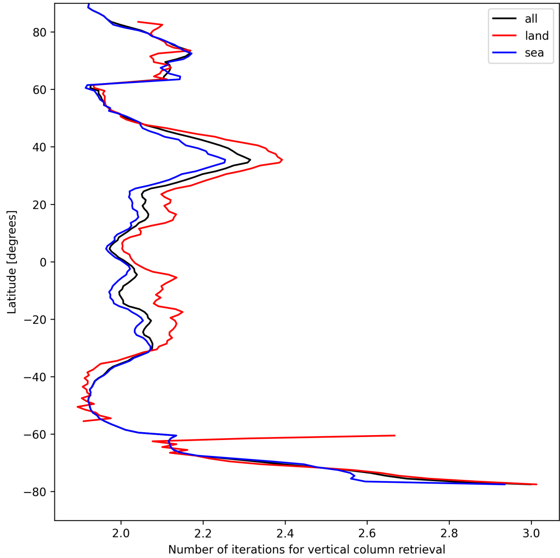
Figure 27: Zonal average of “Number of iterations for vertical column retrieval” for 2025-08-23 to 2025-08-23.
