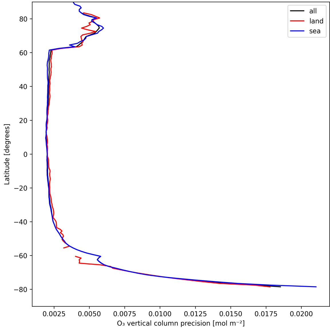
Figure 18: Zonal average of “O 3 vertical column precision” for 2025-08-24 to 2025-08-25.
