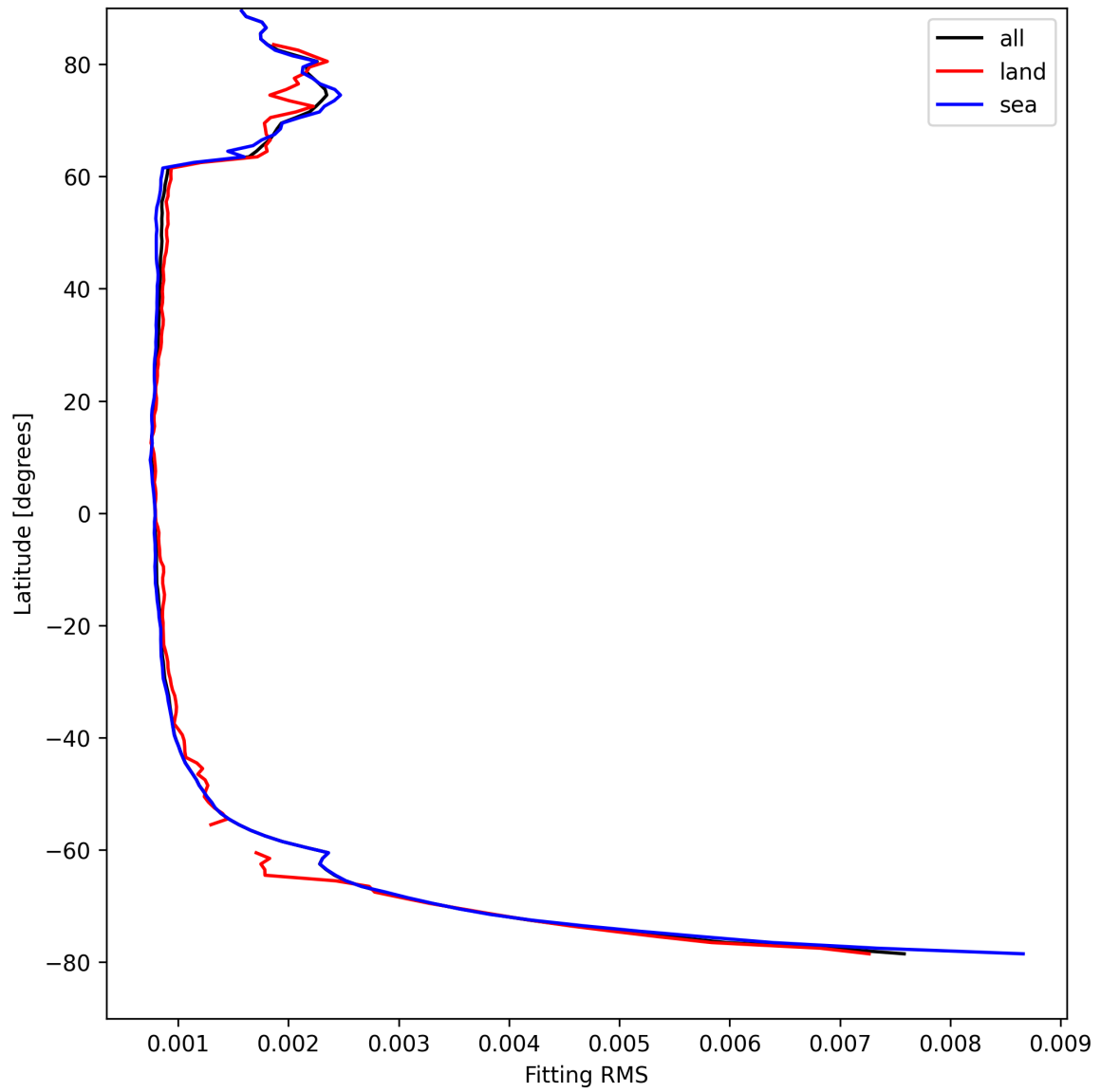
Figure 22: Zonal average of “Fitting RMS” for 2025-08-24 to 2025-08-25.
