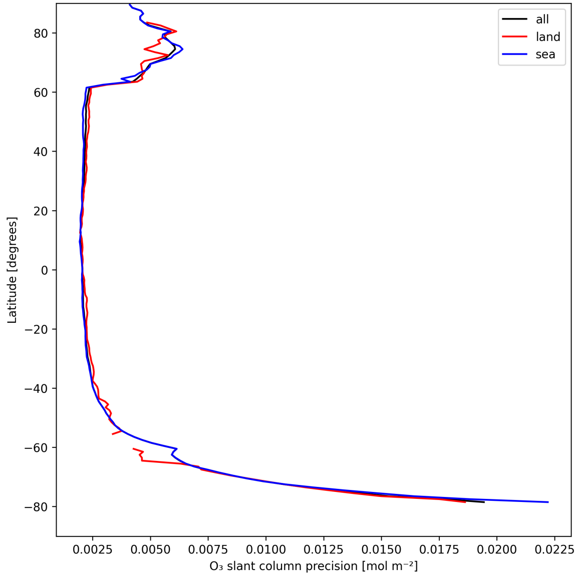
Figure 20: Zonal average of "O 3 slant column precision" for 2025-08-24 to 2025-08-25.
