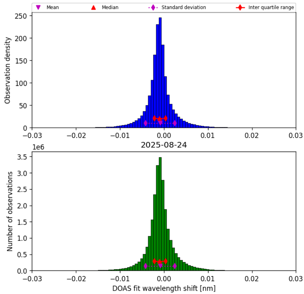
Figure 35: Histogram of “DOAS fit wavelength shift” for 2025-08-24 to 2025-08-25
