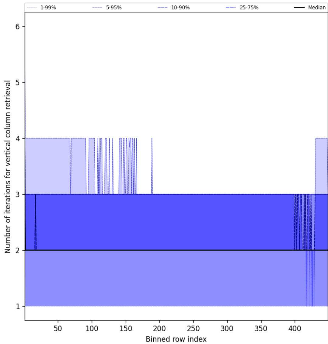
Figure 51: Along track statistics of “Number of iterations for vertical column retrieval” for 2025-08-24 to 2025-08-25
