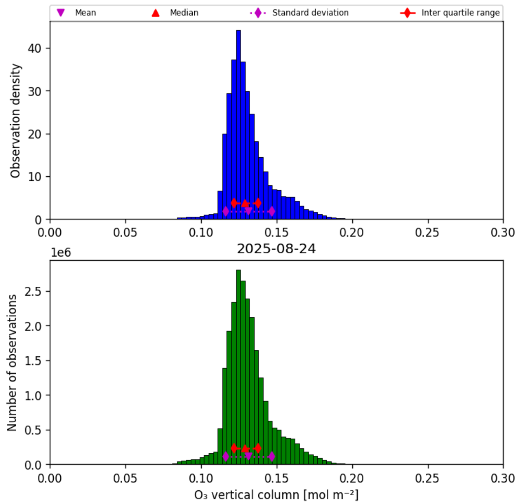
Figure 29: Histogram of “O 3 vertical column” for 2025-08-24 to 2025-08-25
