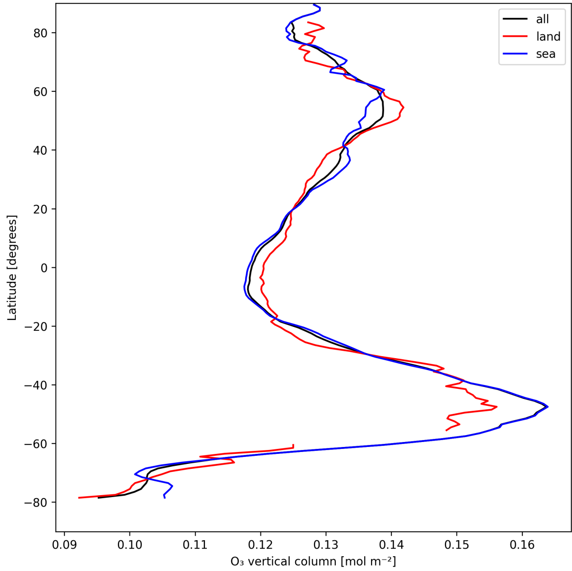
Figure 17: Zonal average of “O 3 vertical column” for 2025-08-24 to 2025-08-25.
