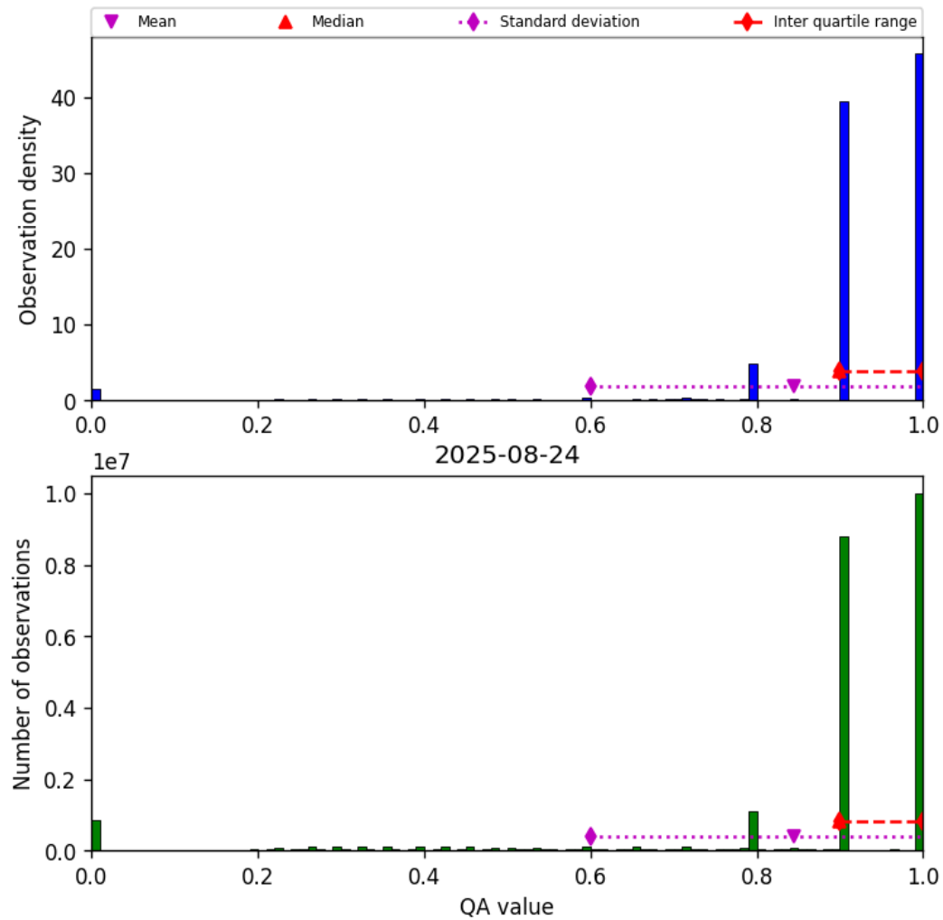
Figure 28: Histogram of “QA value” for 2025-08-24 to 2025-08-25
