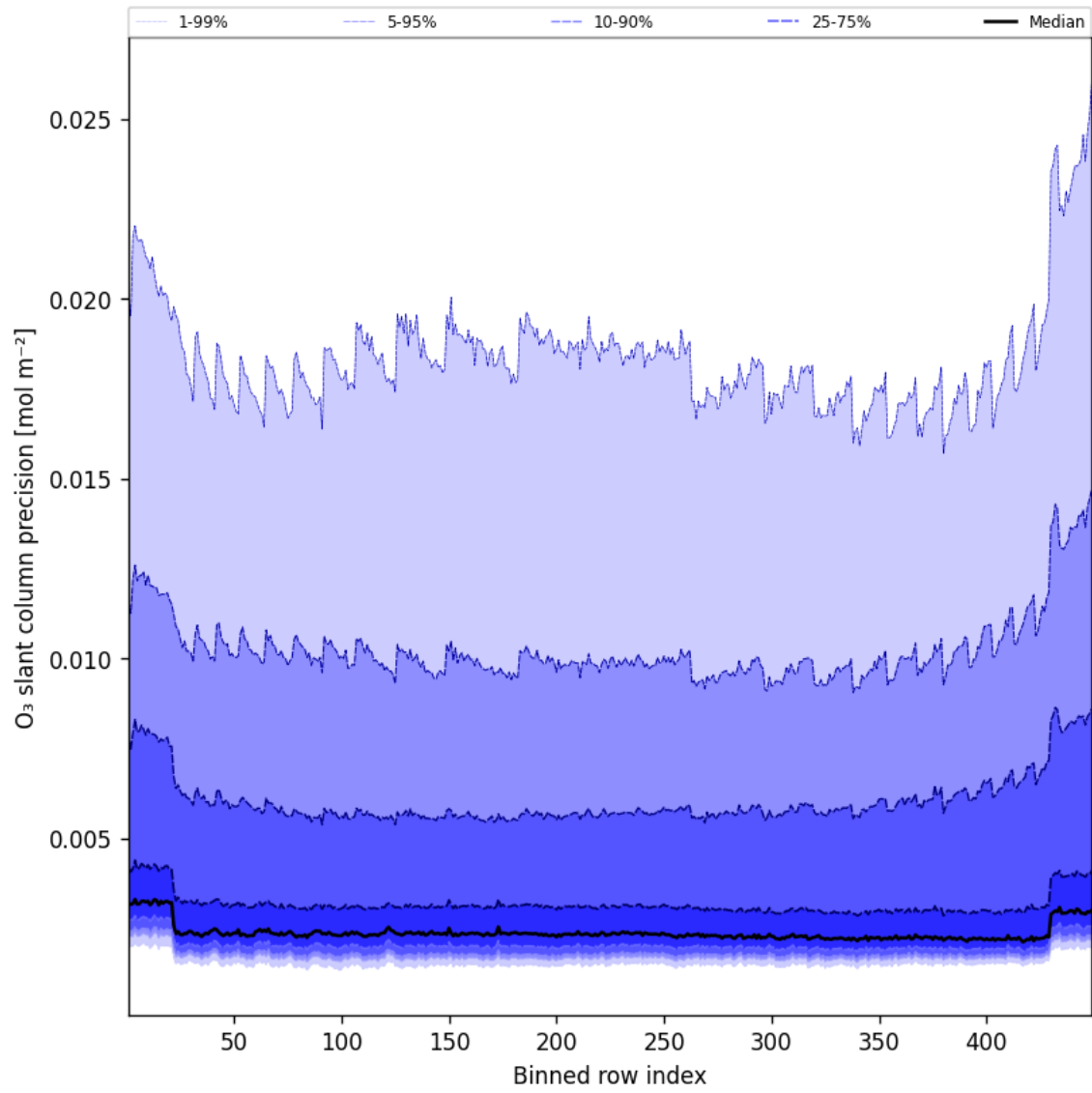
Figure 44: Along track statistics of “O 3 slant column precision” for 2025-08-24 to 2025-08-25
