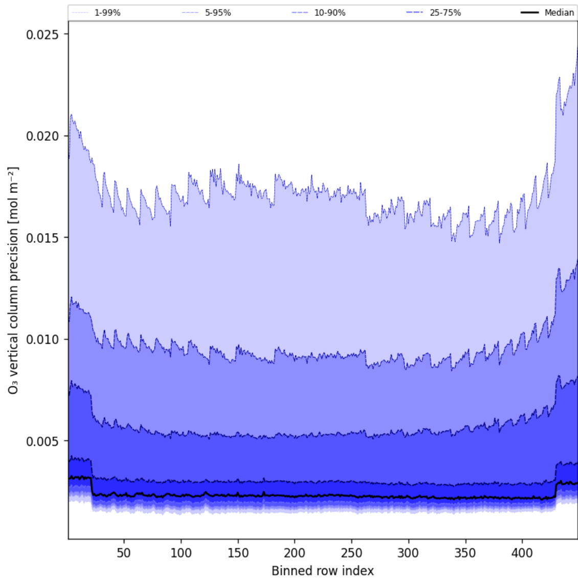
Figure 42: Along track statistics of “O 3 vertical column precision” for 2025-08-24 to 2025-08-25
