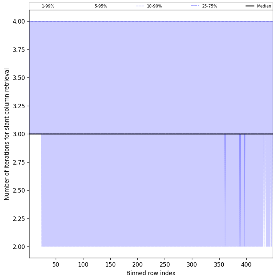
Figure 45: Along track statistics of “Number of iterations for slant column retrieval” for 2025-08-24 to 2025-08-25
