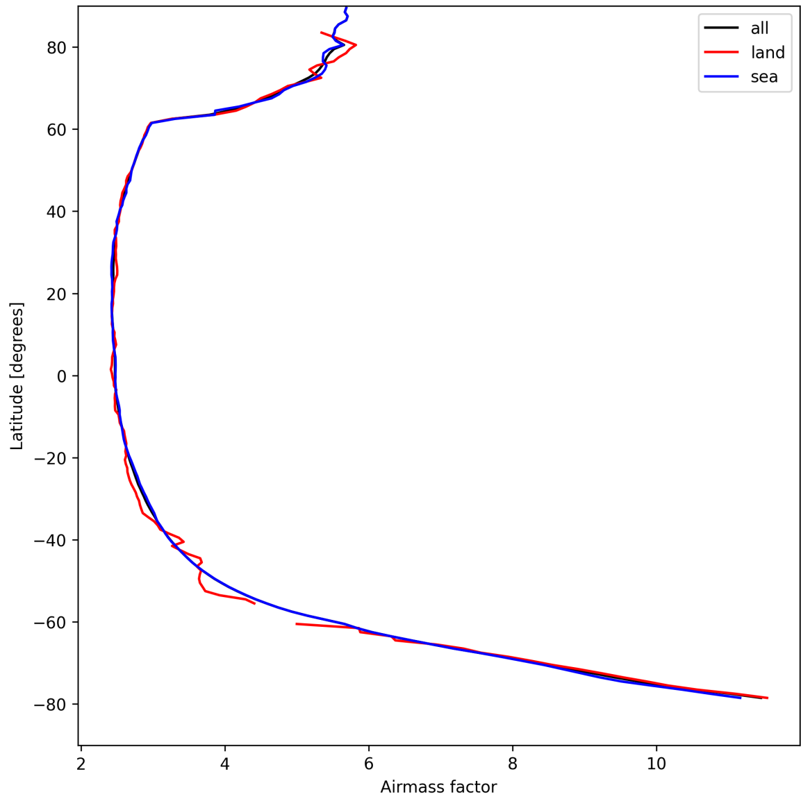
Figure 25: Zonal average of “Airmass factor” for 2025-08-24 to 2025-08-25.
