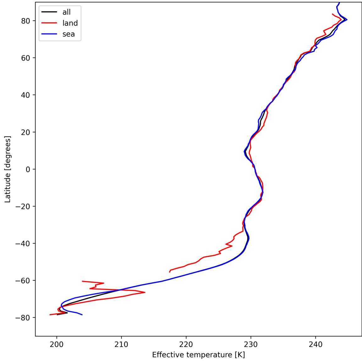
Figure 26: Zonal average of "Effective temperature" for 2025-08-24 to 2025-08-25.
