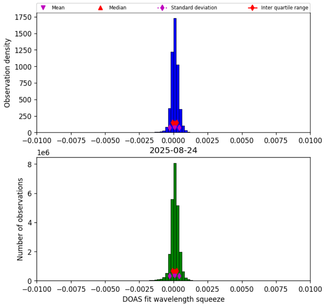
Figure 36: Histogram of “DOAS fit wavelength squeeze” for 2025-08-24 to 2025-08-25
