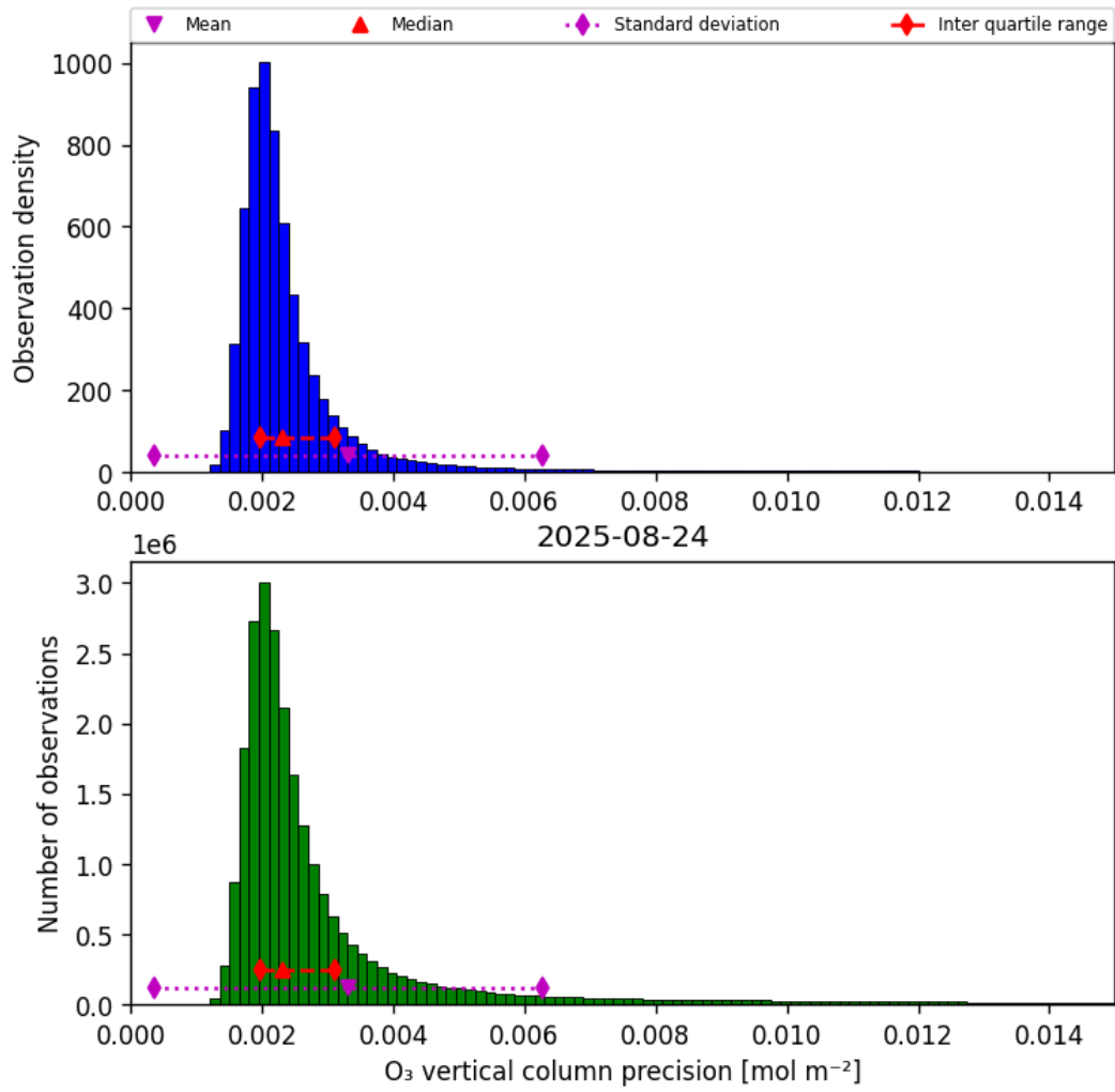
Figure 30: Histogram of “O 3 vertical column precision” for 2025-08-24 to 2025-08-25
