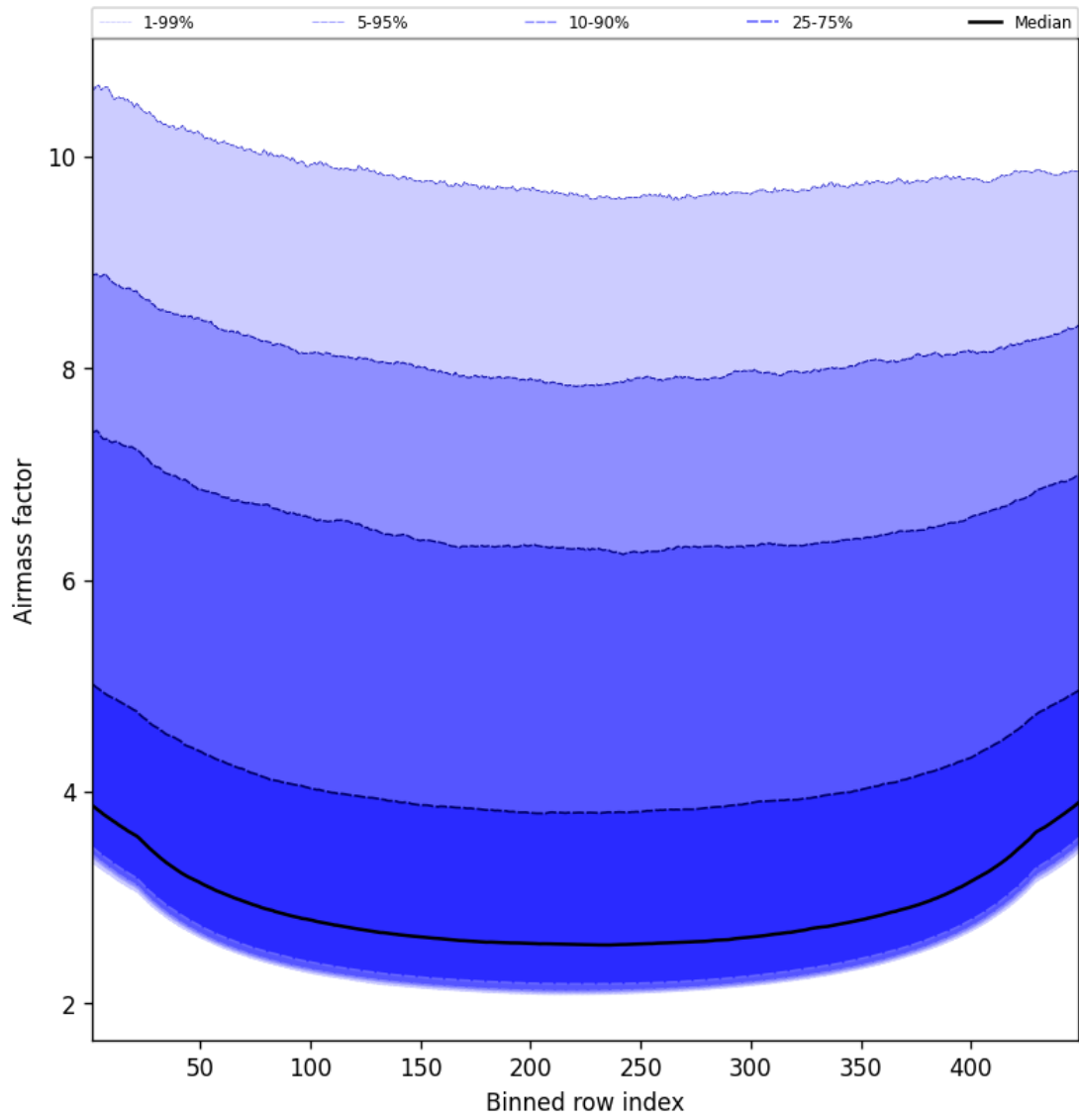
Figure 49: Along track statistics of “Airmass factor” for 2025-08-24 to 2025-08-25
