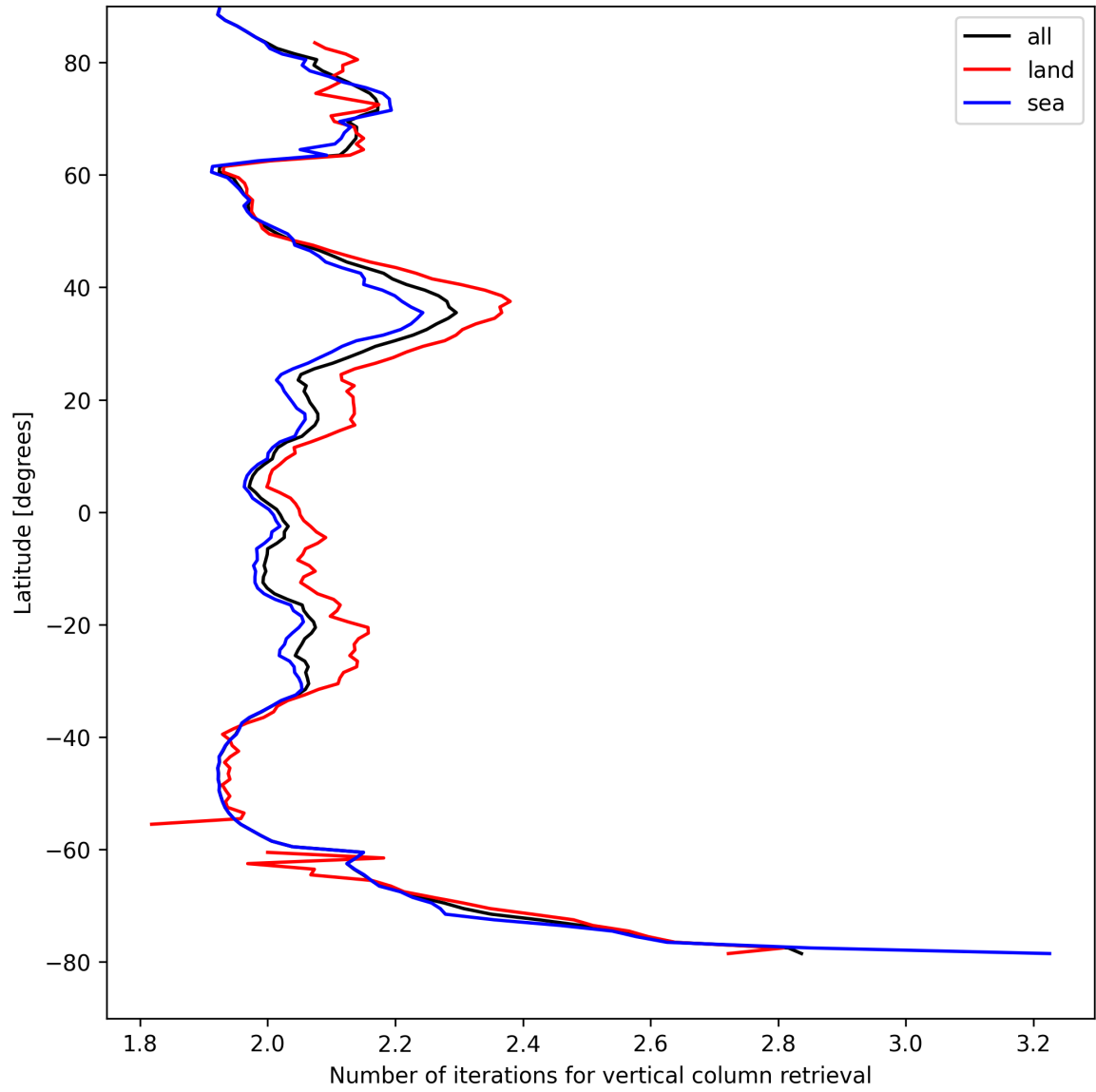
Figure 27: Zonal average of “Number of iterations for vertical column retrieval” for 2025-08-24 to 2025-08-25.
