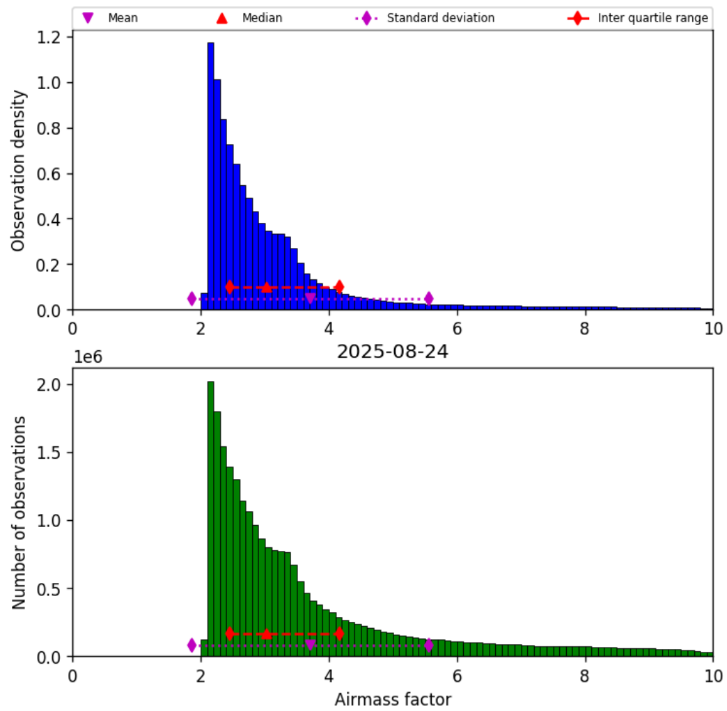
Figure 37: Histogram of “Airmass factor” for 2025-08-24 to 2025-08-25
