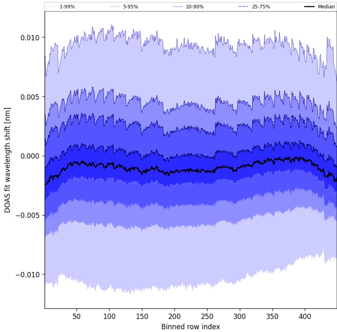
Figure 47: Along track statistics of “DOAS fit wavelength shift” for 2025-08-24 to 2025-08-25
