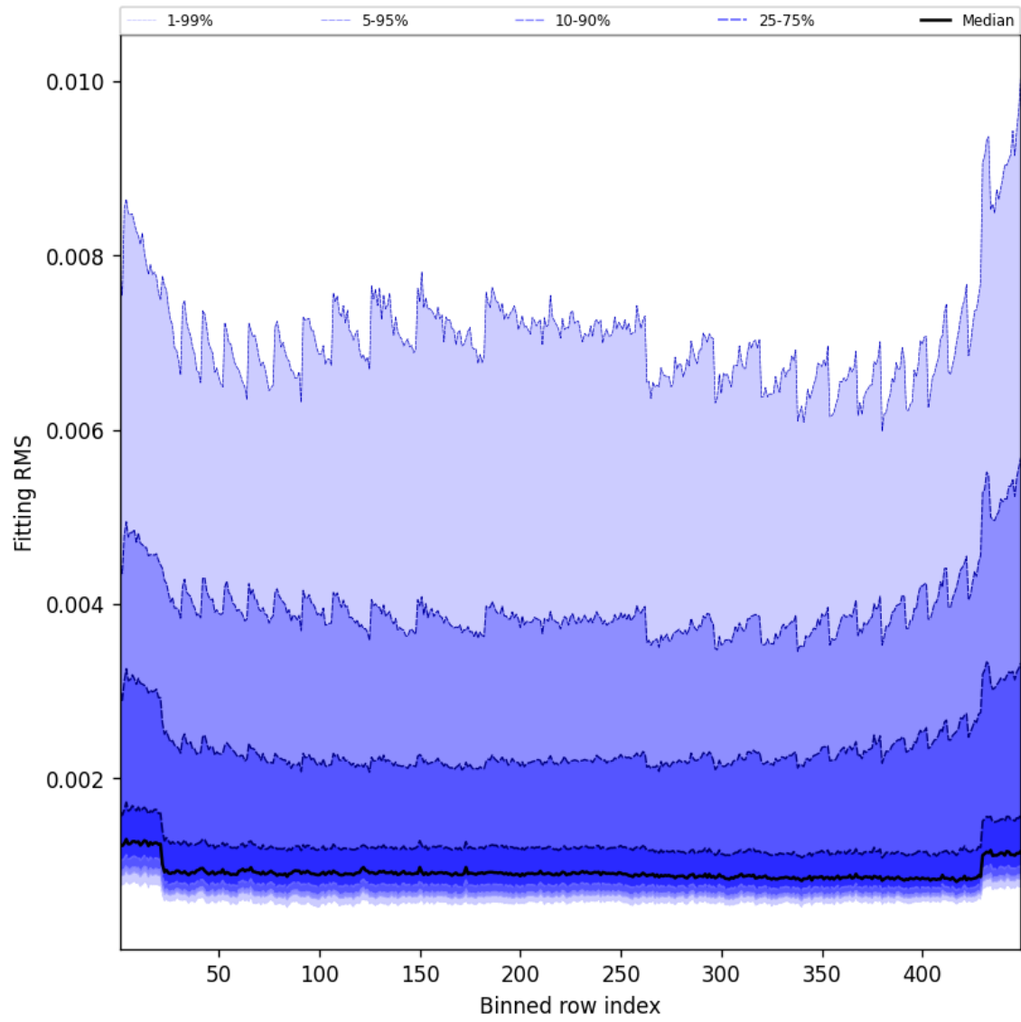
Figure 46: Along track statistics of “Fitting RMS” for 2025-08-24 to 2025-08-25
