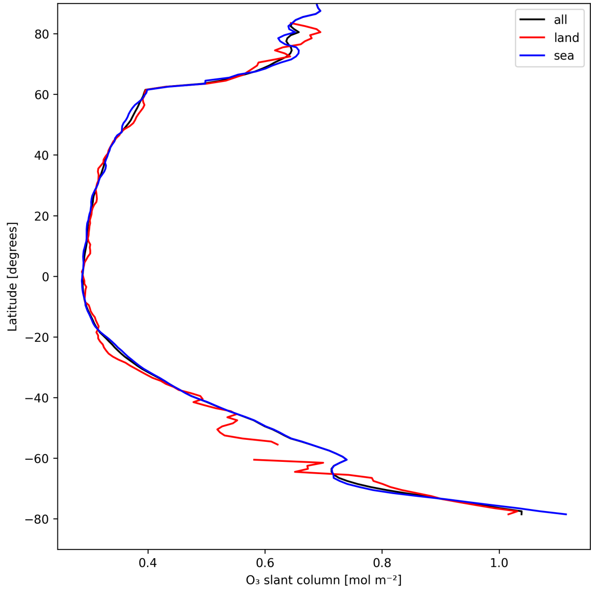
Figure 19: Zonal average of “O 3 slant column” for 2025-08-24 to 2025-08-25.
