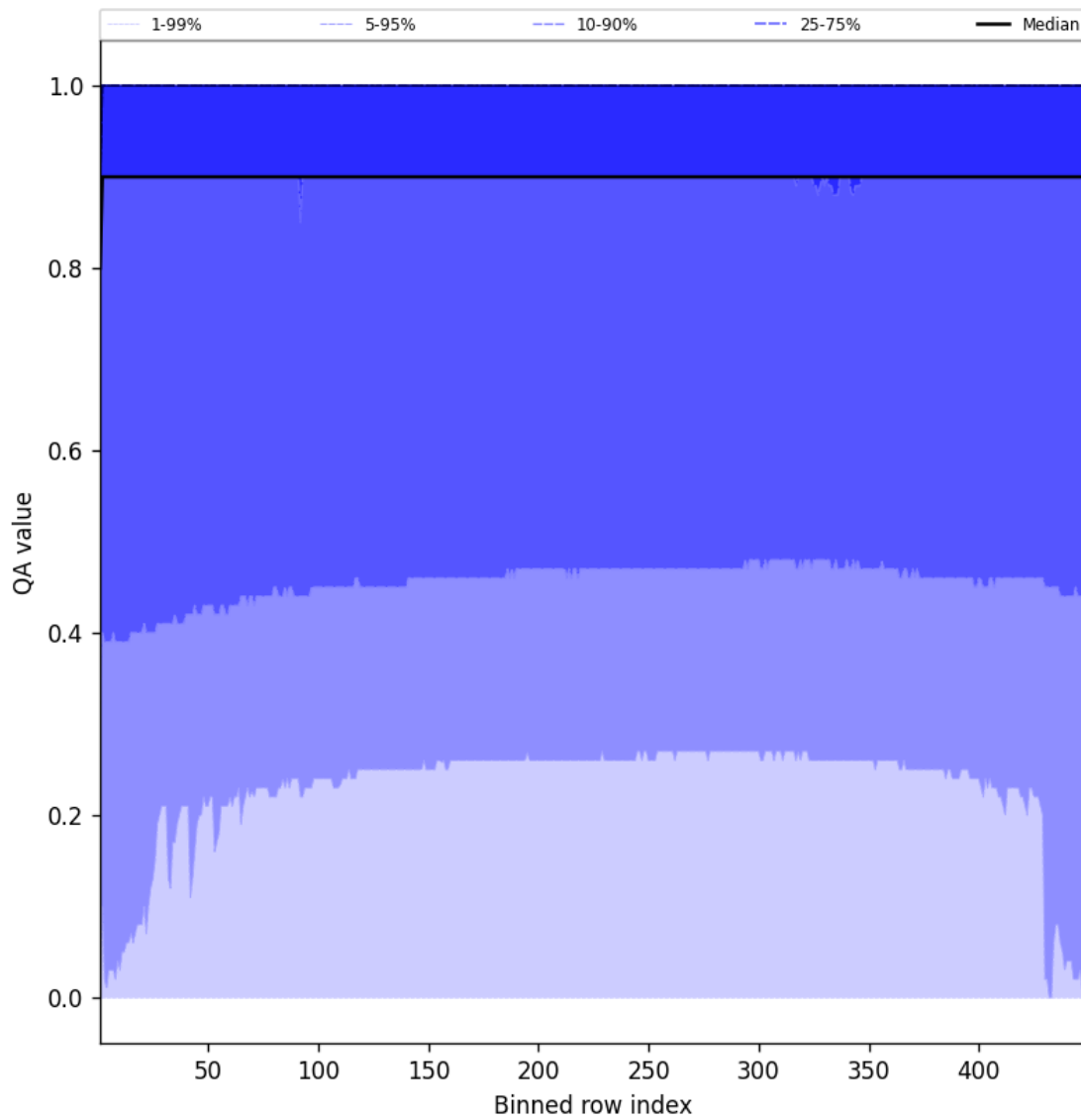
Figure 40: Along track statistics of “QA value” for 2025-08-24 to 2025-08-25
