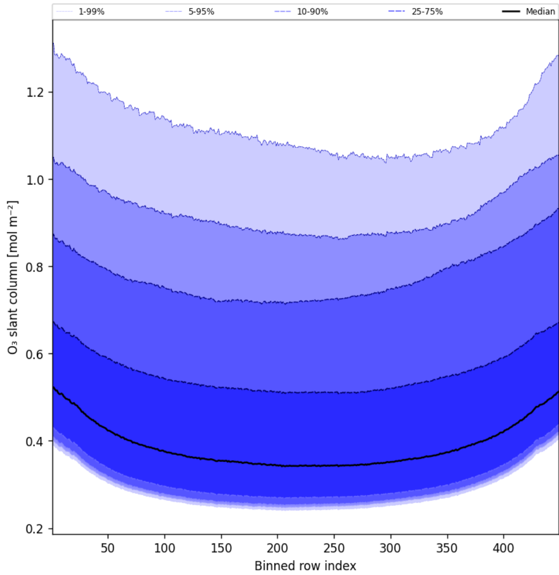
Figure 43: Along track statistics of “O 3 slant column” for 2025-08-24 to 2025-08-25
