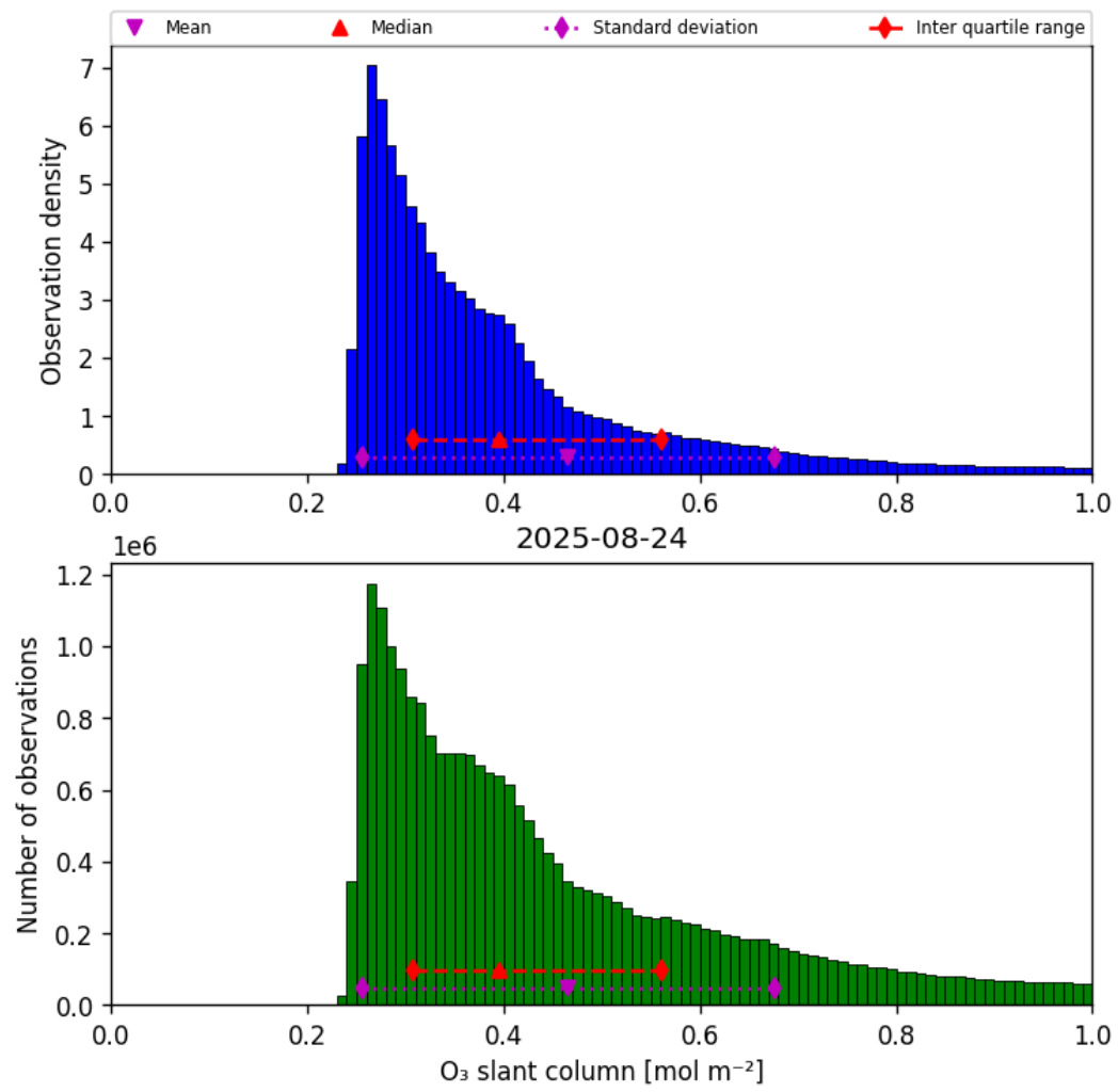
Figure 31: Histogram of “O 3 slant column” for 2025-08-24 to 2025-08-25
