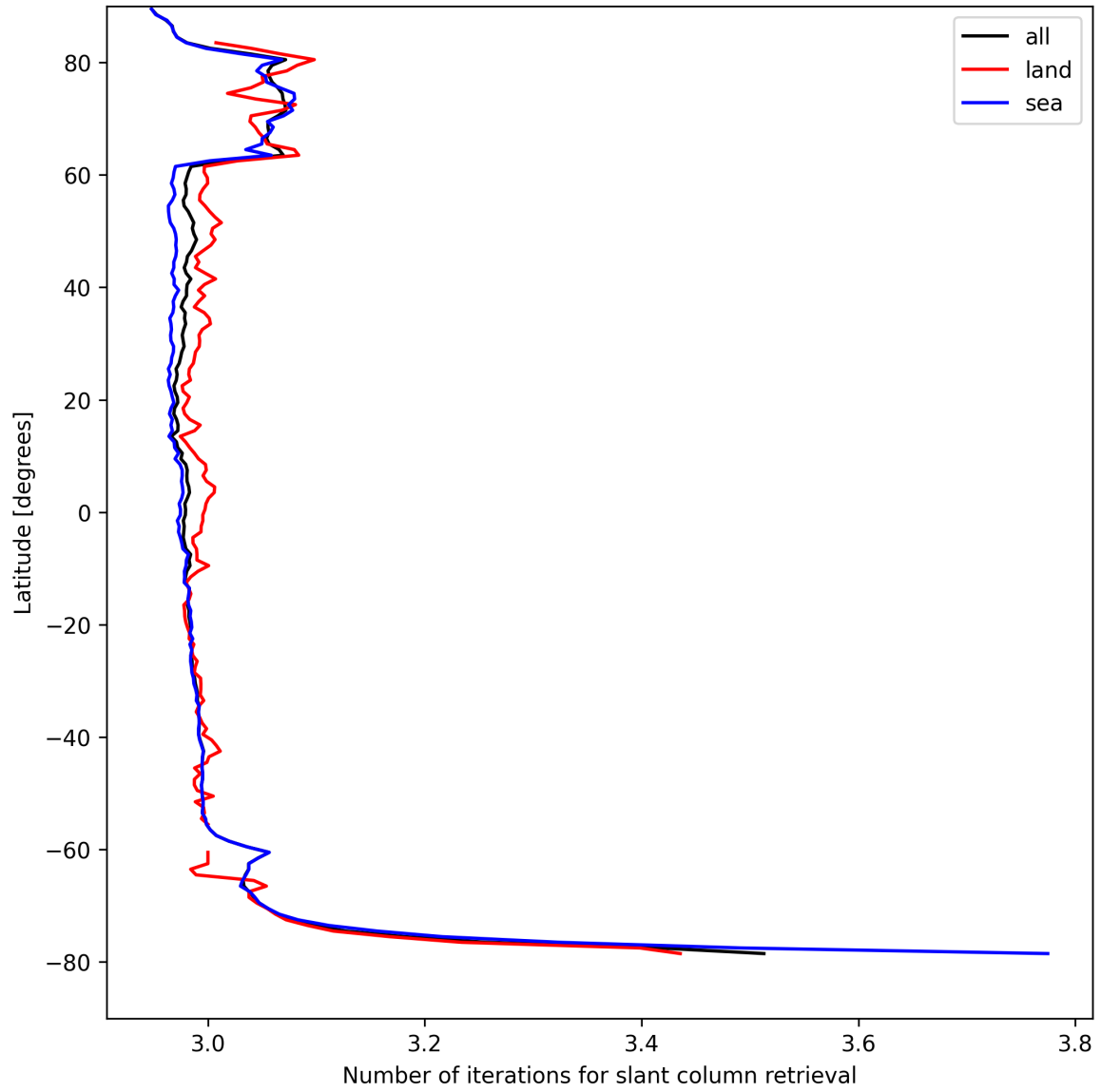
Figure 21: Zonal average of “Number of iterations for slant column retrieval” for 2025-08-24 to 2025-08-25.
