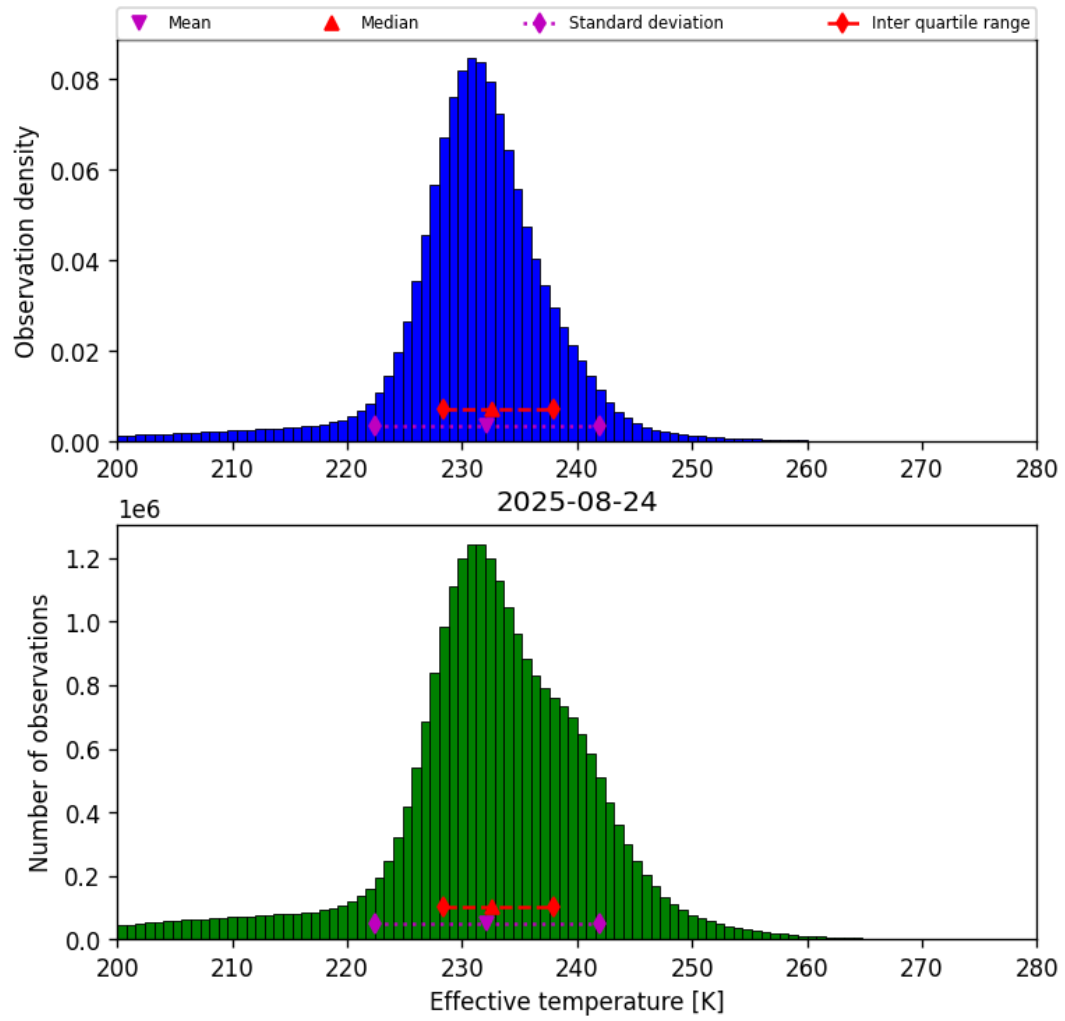
Figure 38: Histogram of “Effective temperature” for 2025-08-24 to 2025-08-25
