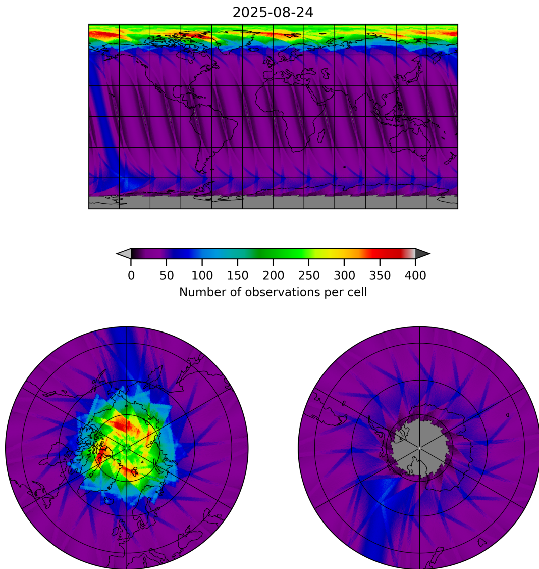
Figure 15: Map of the number of observations for 2025-08-24 to 2025-08-25
