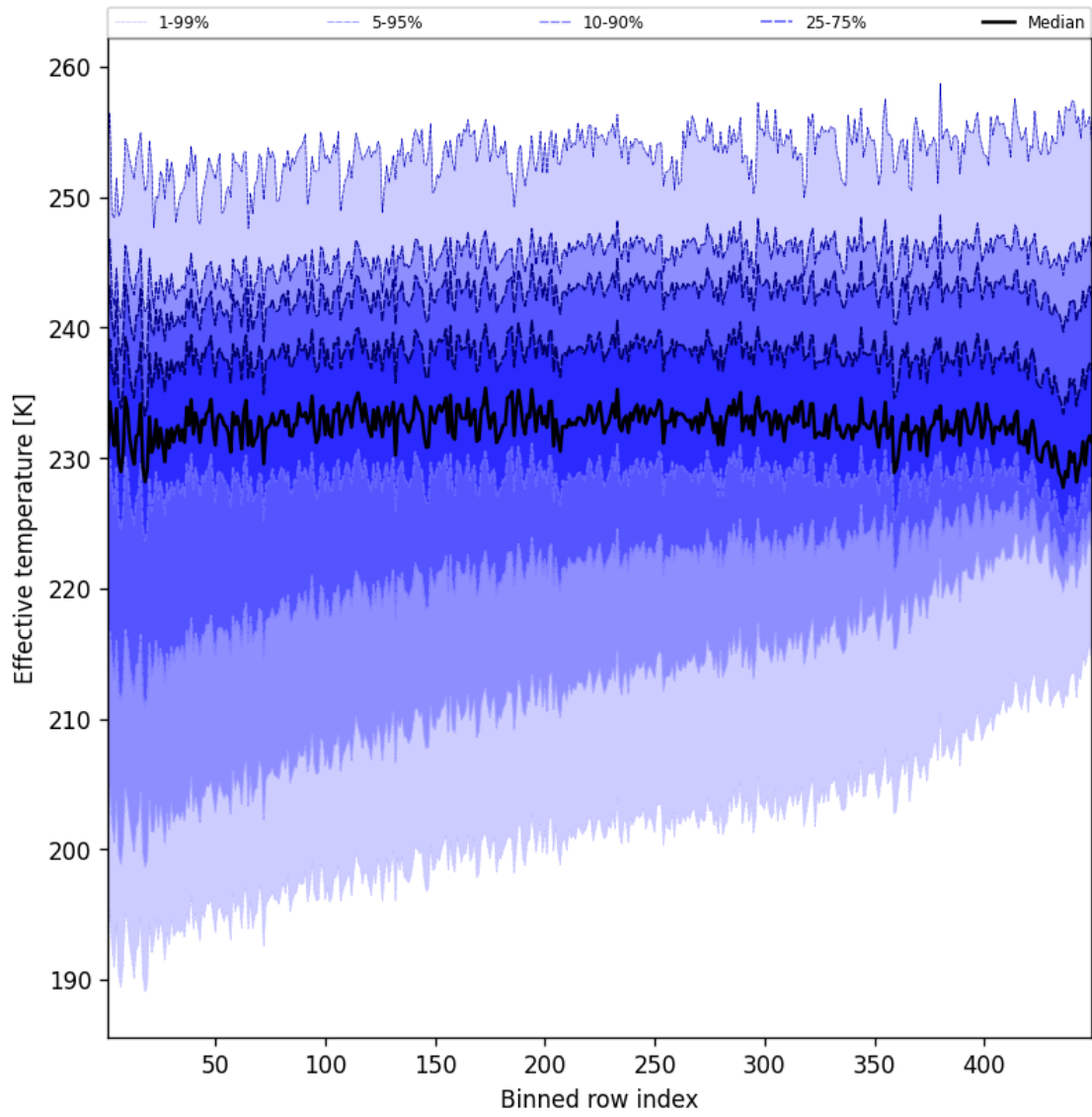
Figure 50: Along track statistics of “Effective temperature” for 2025-08-24 to 2025-08-25
