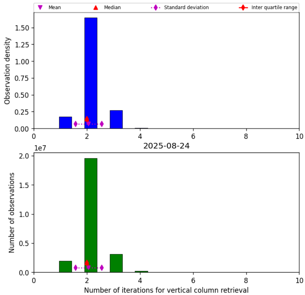
Figure 39: Histogram of “Number of iterations for vertical column retrieval” for 2025-08-24 to 2025-08-25
