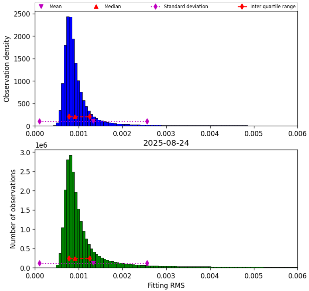
Figure 34: Histogram of “Fitting RMS” for 2025-08-24 to 2025-08-25
