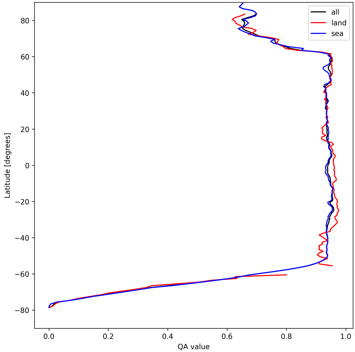
Figure 16: Zonal average of “QA value” for 2025-08-24 to 2025-08-25.
