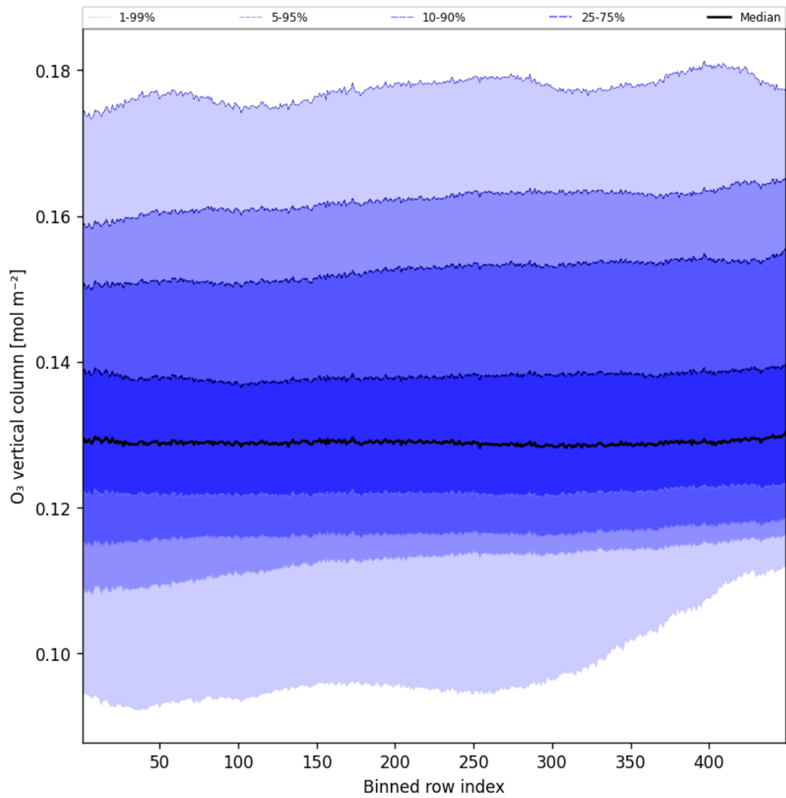
Figure 41: Along track statistics of “O 3 vertical column” for 2025-08-24 to 2025-08-25
