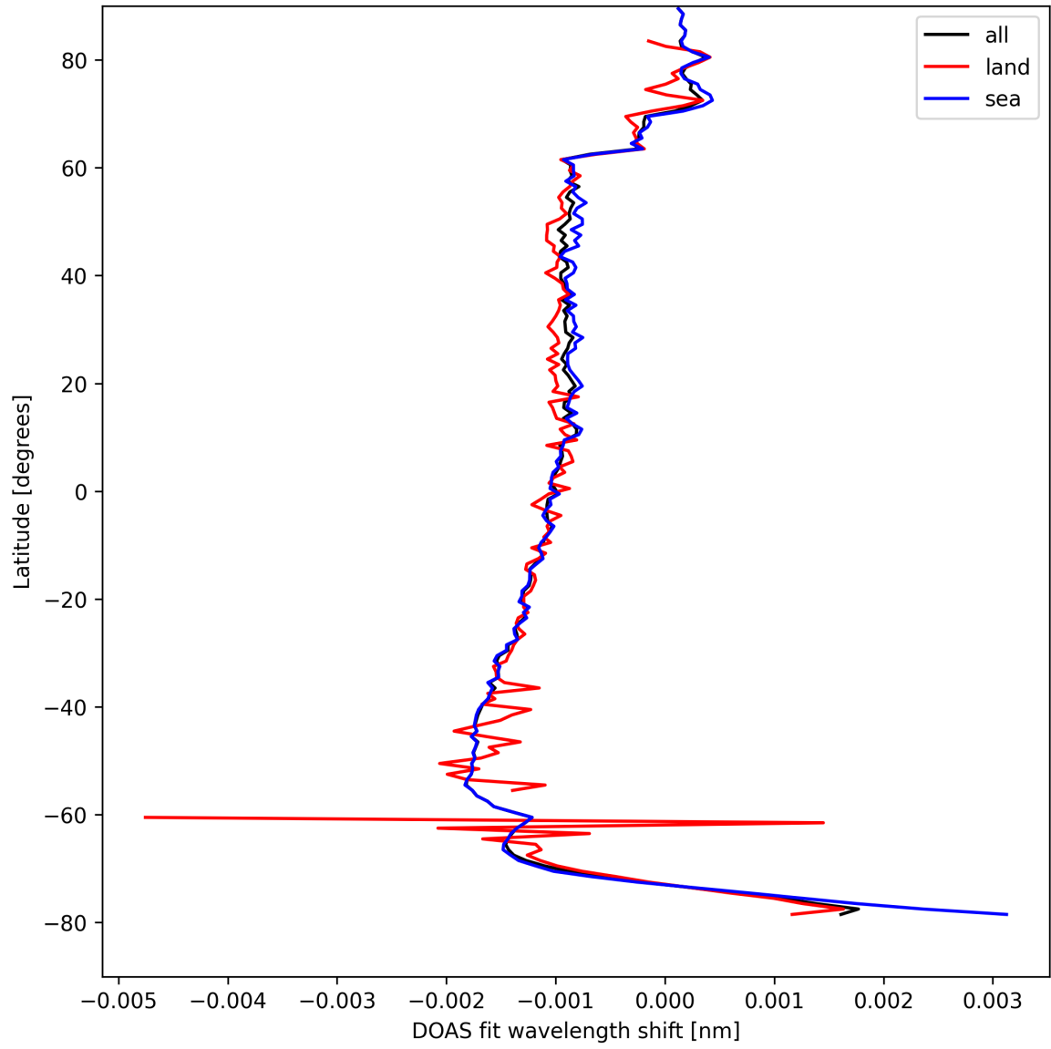
Figure 23: Zonal average of "DOAS fit wavelength shift" for 2025-08-24 to 2025-08-25.
