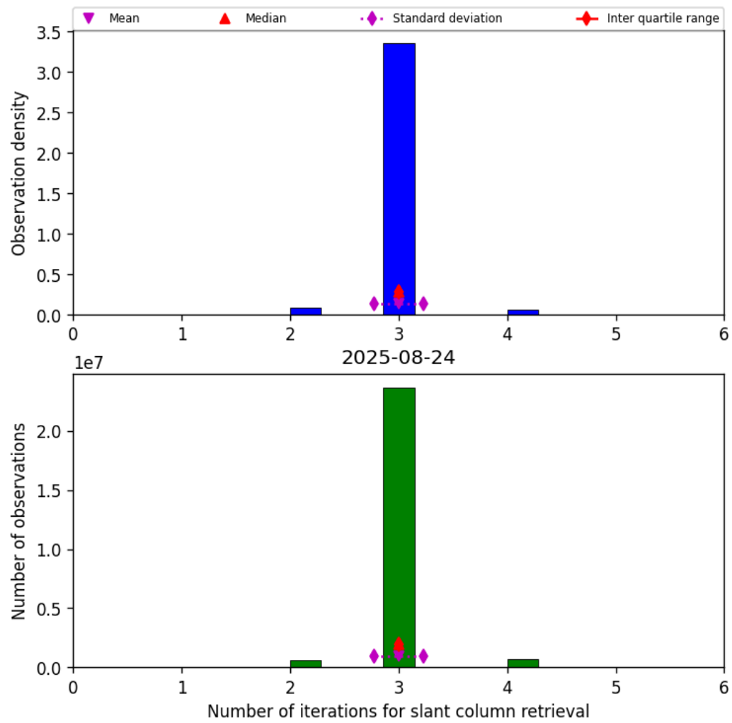
Figure 33: Histogram of “Number of iterations for slant column retrieval” for 2025-08-24 to 2025-08-25
