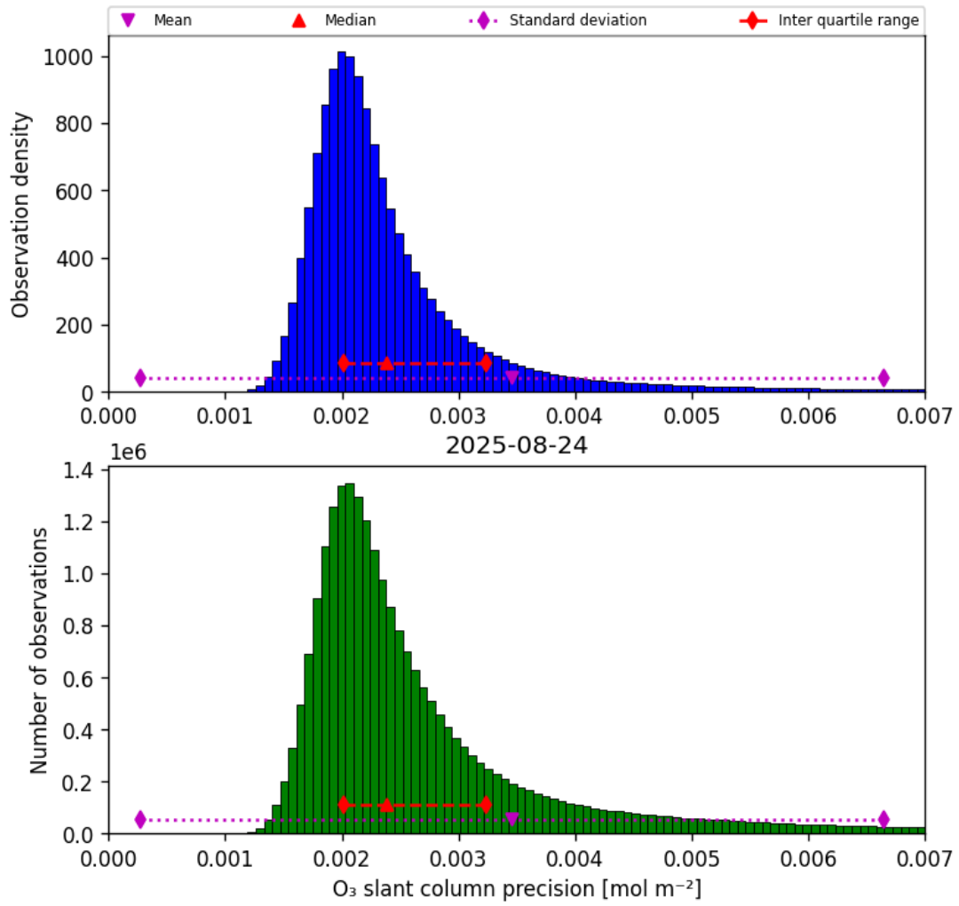
Figure 32: Histogram of “O 3 slant column precision” for 2025-08-24 to 2025-08-25
