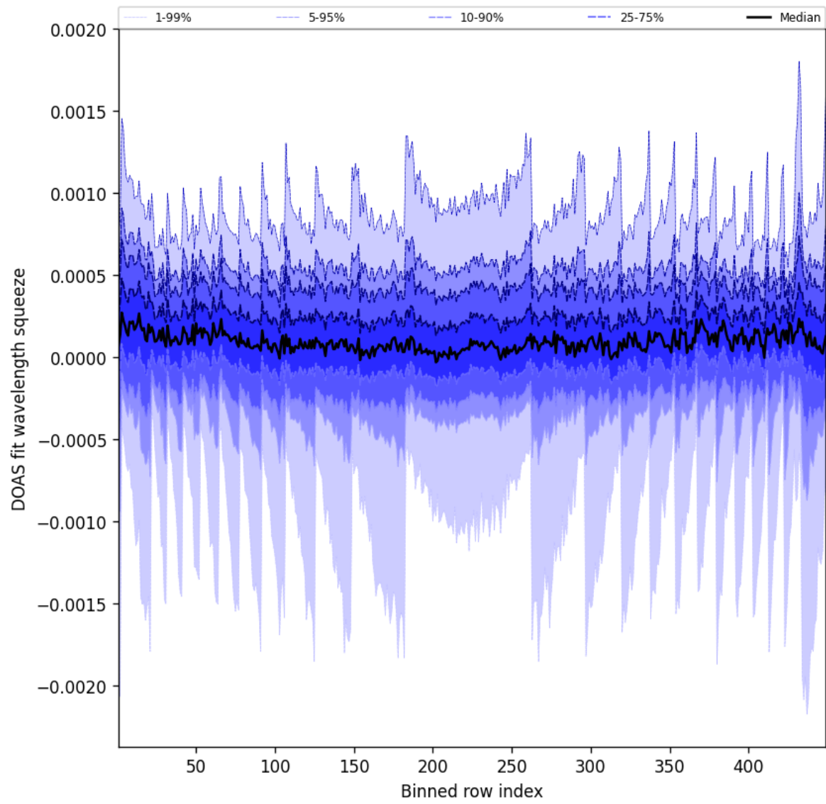
Figure 48: Along track statistics of “DOAS fit wavelength squeeze” for 2025-08-24 to 2025-08-25
