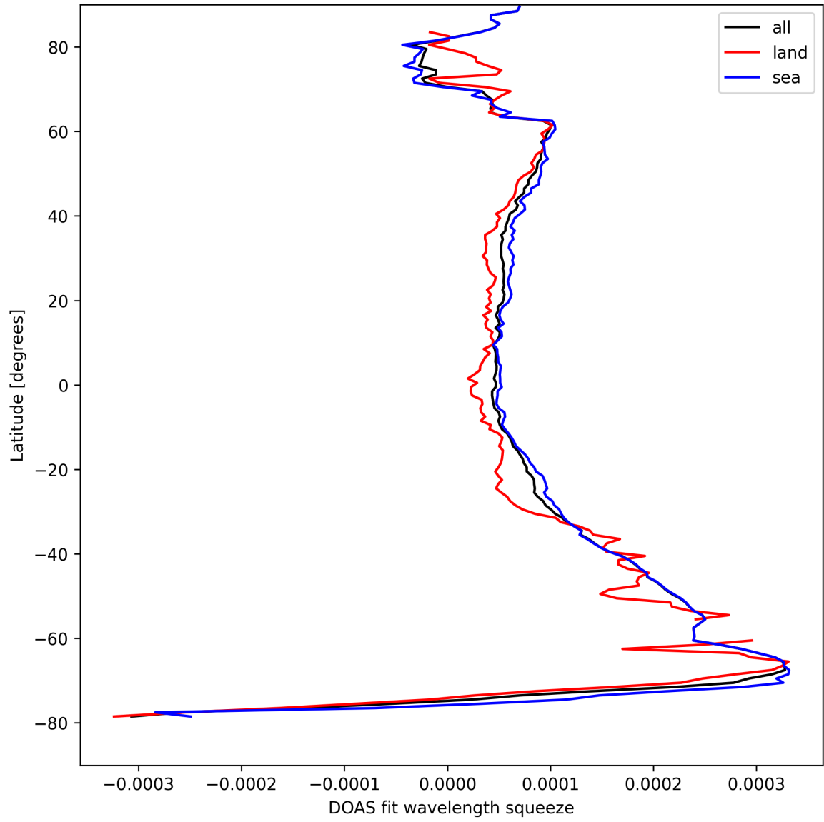
Figure 24: Zonal average of “DOAS fit wavelength squeeze” for 2025-08-24 to 2025-08-25.
