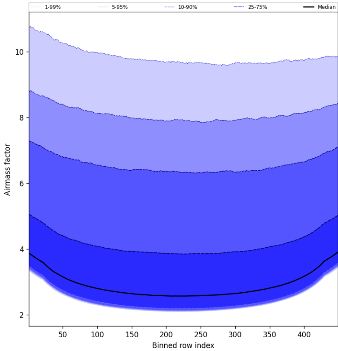
Figure 49: Along track statistics of “Airmass factor” for 2025-08-25 to 2025-08-26
