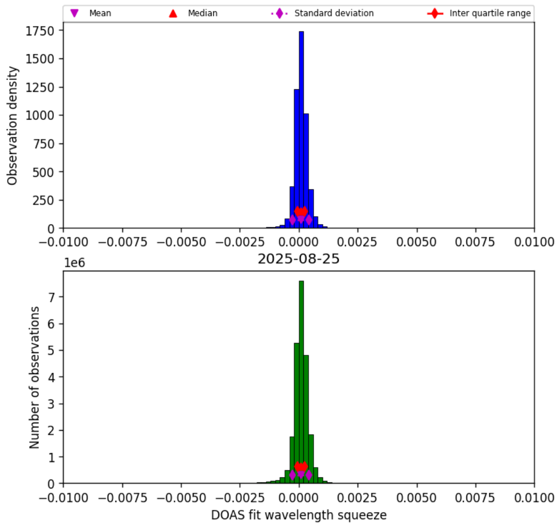
Figure 36: Histogram of “DOAS fit wavelength squeeze” for 2025-08-25 to 2025-08-26
