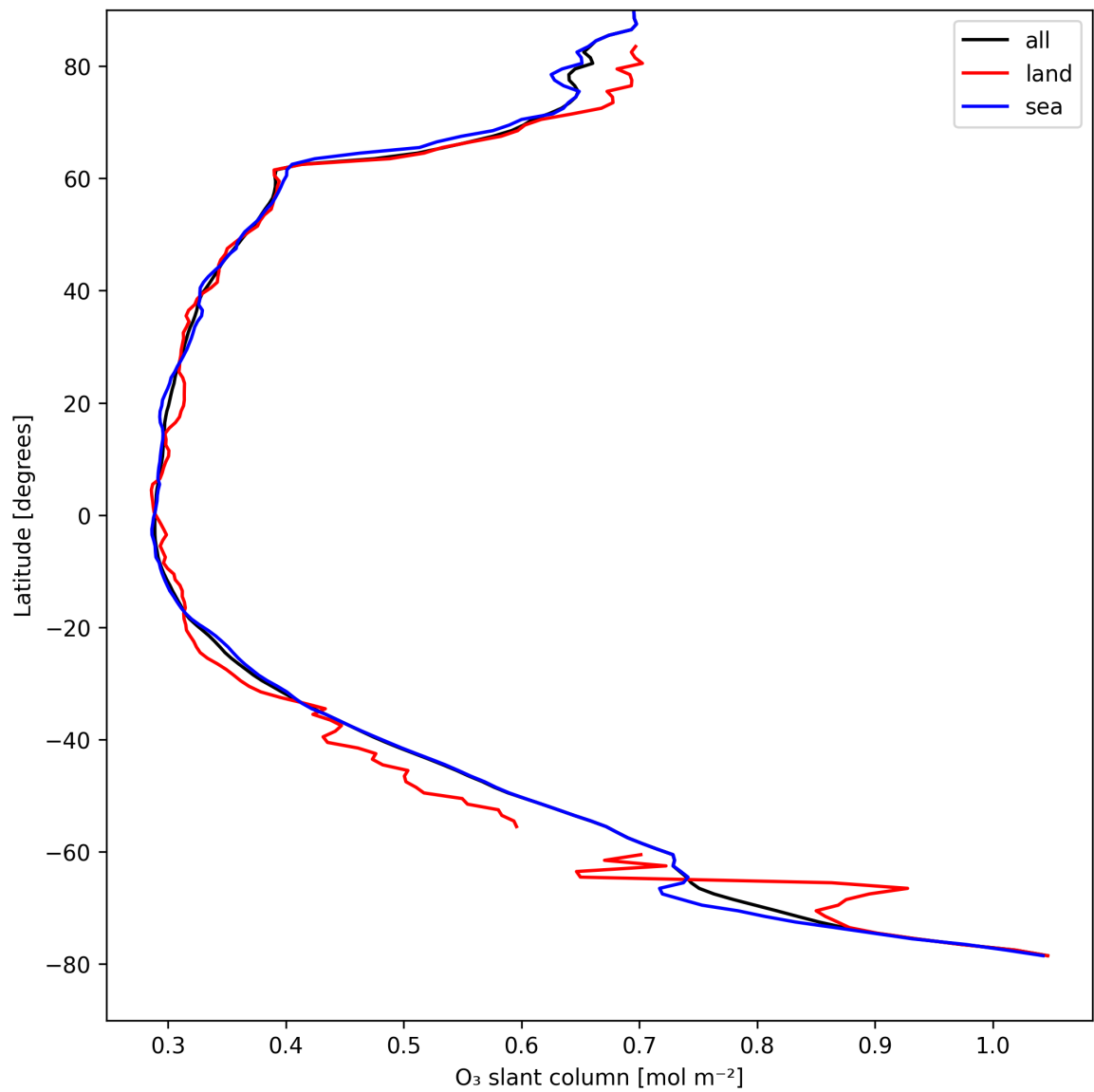
Figure 19: Zonal average of “O 3 slant column” for 2025-08-25 to 2025-08-26.
