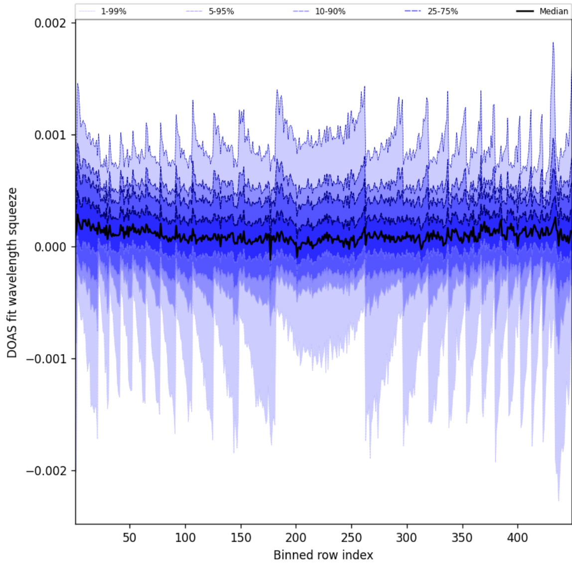
Figure 48: Along track statistics of “DOAS fit wavelength squeeze” for 2025-08-25 to 2025-08-26
