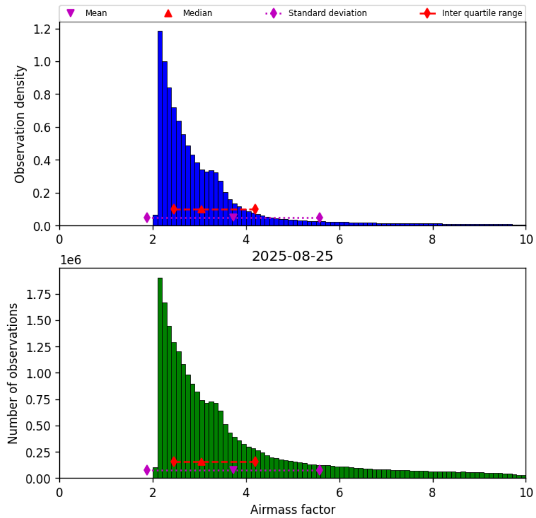
Figure 37: Histogram of “Airmass factor” for 2025-08-25 to 2025-08-26
