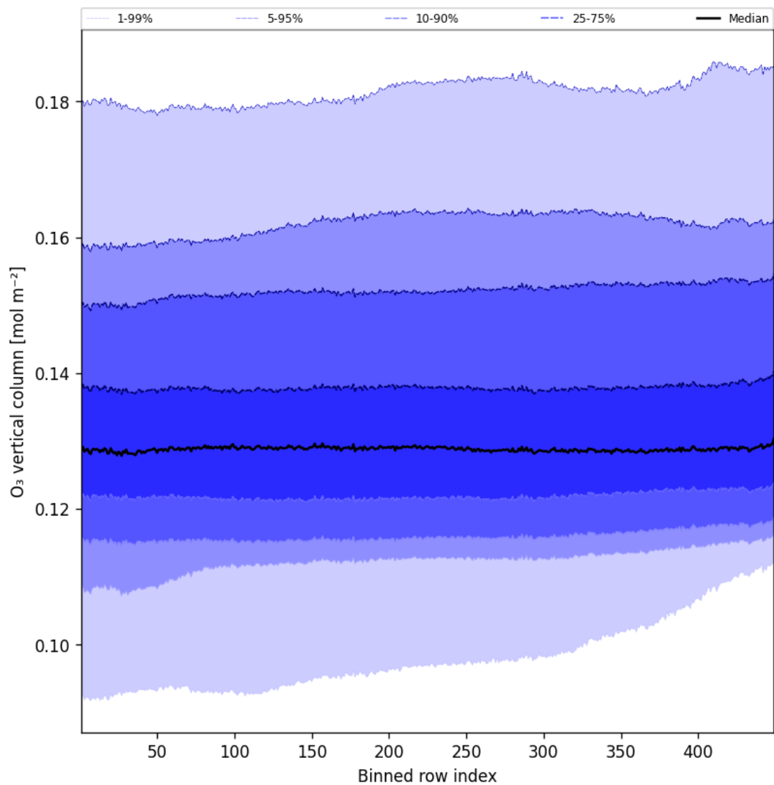
Figure 41: Along track statistics of “O 3 vertical column” for 2025-08-25 to 2025-08-26
