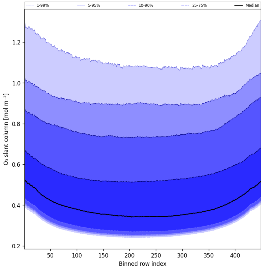
Figure 43: Along track statistics of “O 3 slant column” for 2025-08-25 to 2025-08-26
