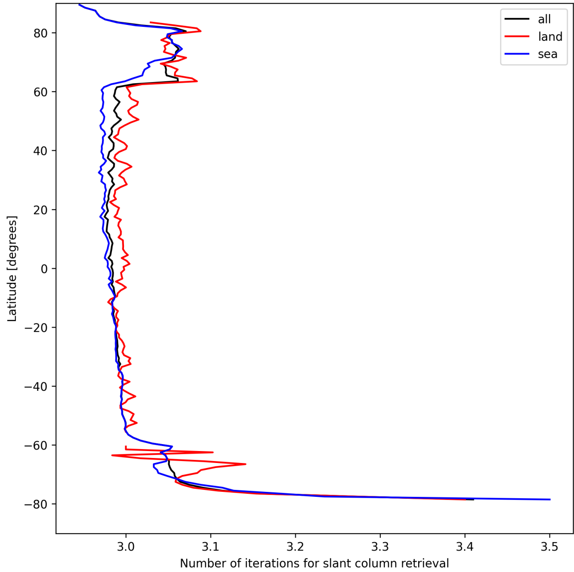
Figure 21: Zonal average of “Number of iterations for slant column retrieval” for 2025-08-25 to 2025-08-26.
