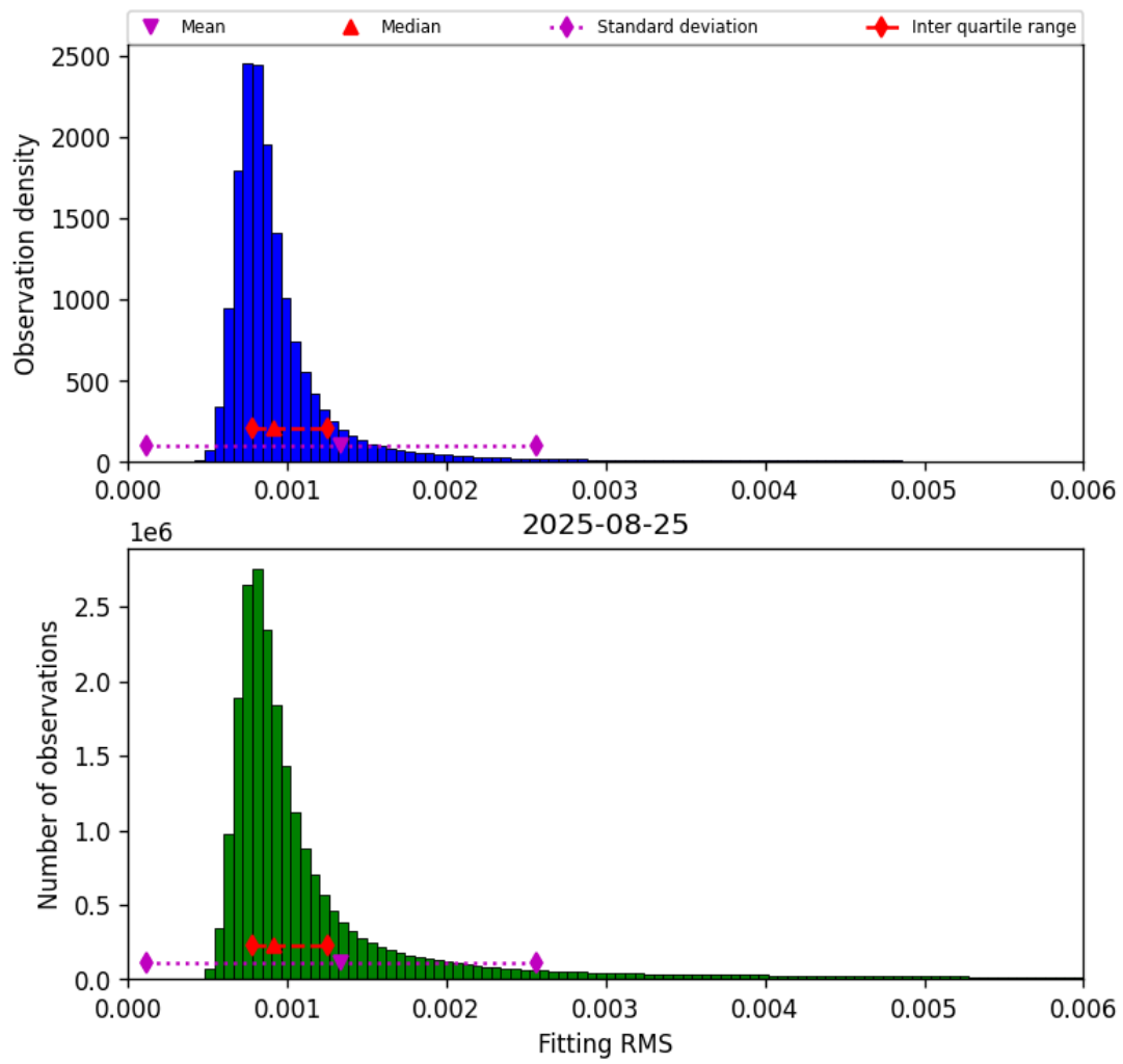
Figure 34: Histogram of “Fitting RMS” for 2025-08-25 to 2025-08-26
