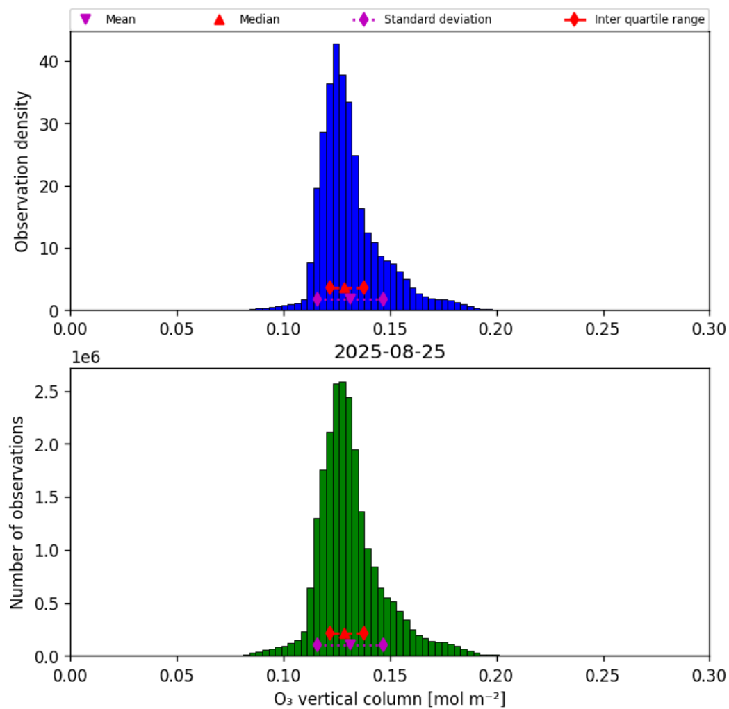
Figure 29: Histogram of “O 3 vertical column” for 2025-08-25 to 2025-08-26
