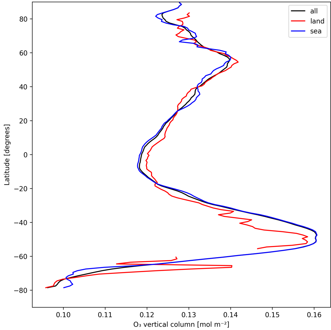
Figure 17: Zonal average of “O 3 vertical column” for 2025-08-25 to 2025-08-26.
