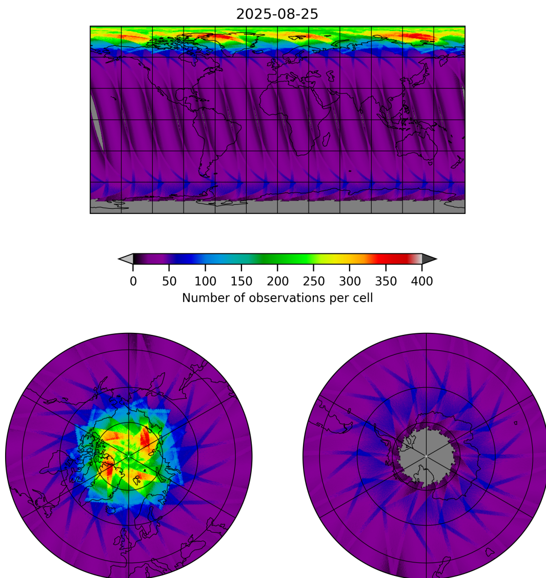
Figure 15: Map of the number of observations for 2025-08-25 to 2025-08-26
