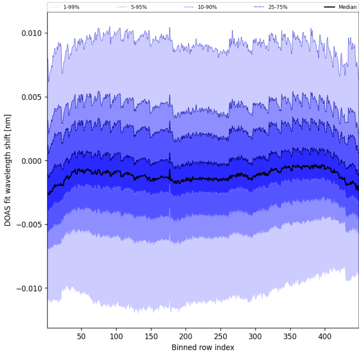
Figure 47: Along track statistics of “DOAS fit wavelength shift” for 2025-08-25 to 2025-08-26
