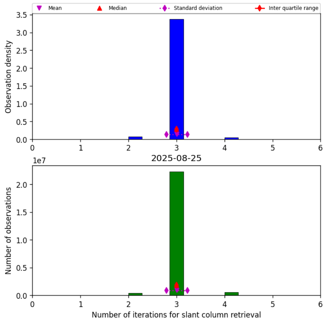
Figure 33: Histogram of “Number of iterations for slant column retrieval” for 2025-08-25 to 2025-08-26
