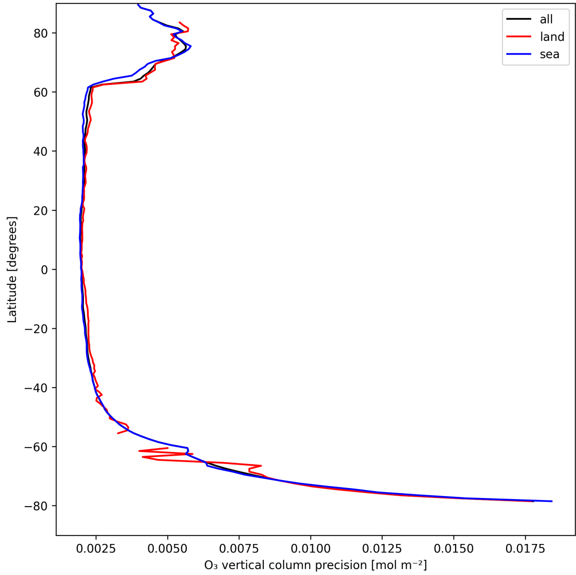
Figure 18: Zonal average of “O 3 vertical column precision” for 2025-08-25 to 2025-08-26.
