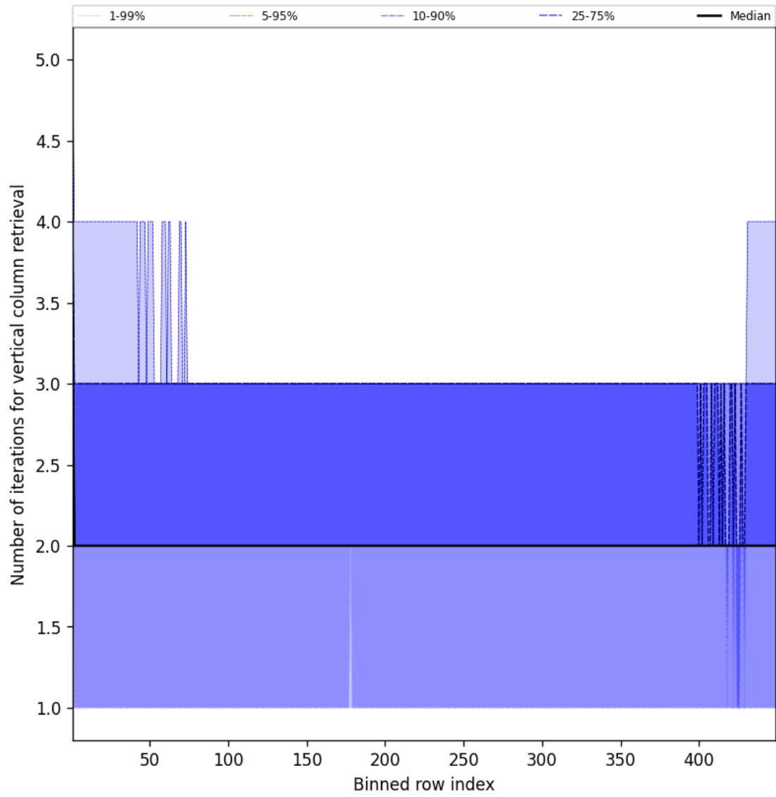
Figure 51: Along track statistics of “Number of iterations for vertical column retrieval” for 2025-08-25 to 2025-08-26
