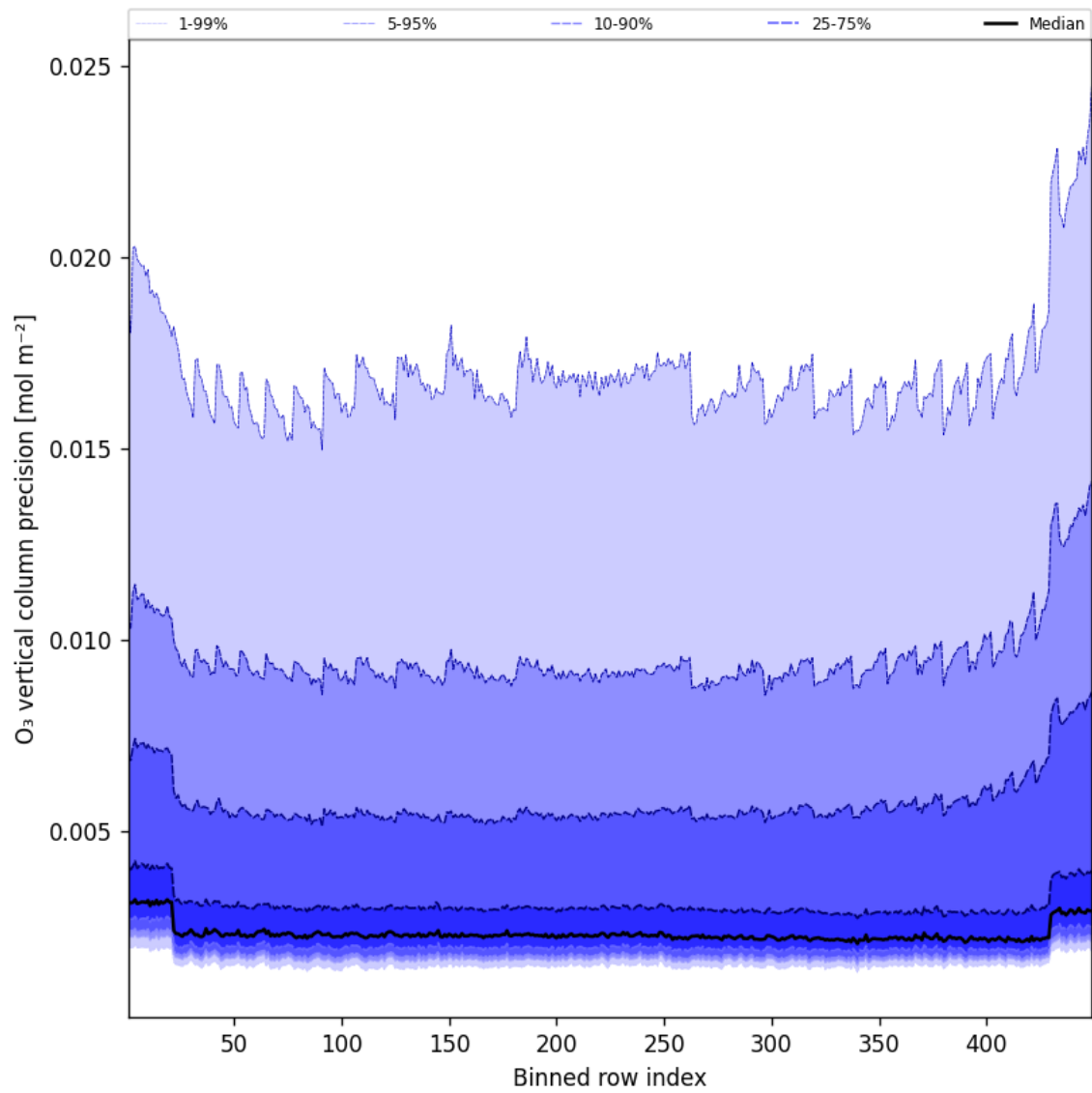
Figure 42: Along track statistics of “O 3 vertical column precision” for 2025-08-25 to 2025-08-26
