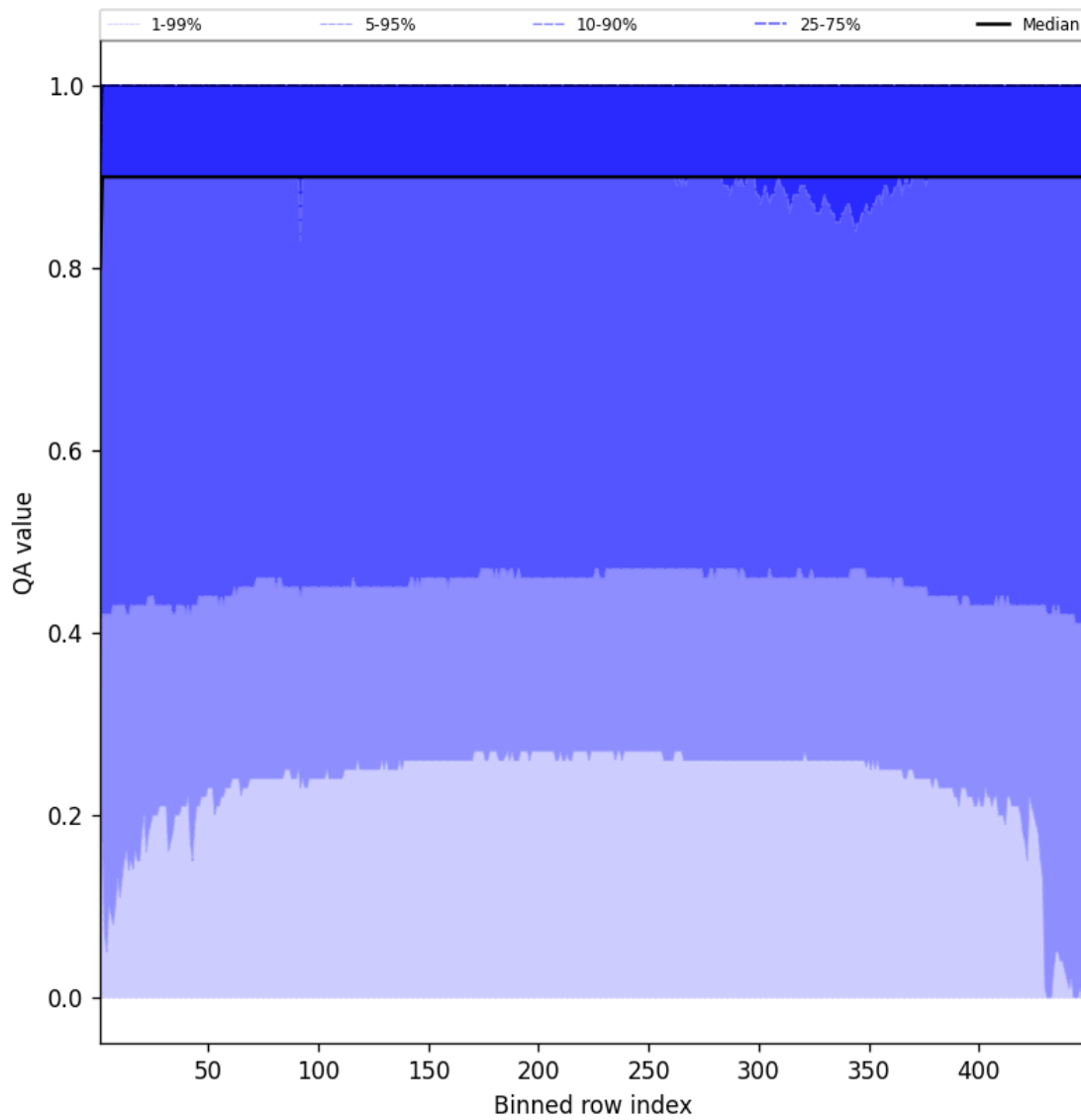
Figure 40: Along track statistics of “QA value” for 2025-08-25 to 2025-08-26
