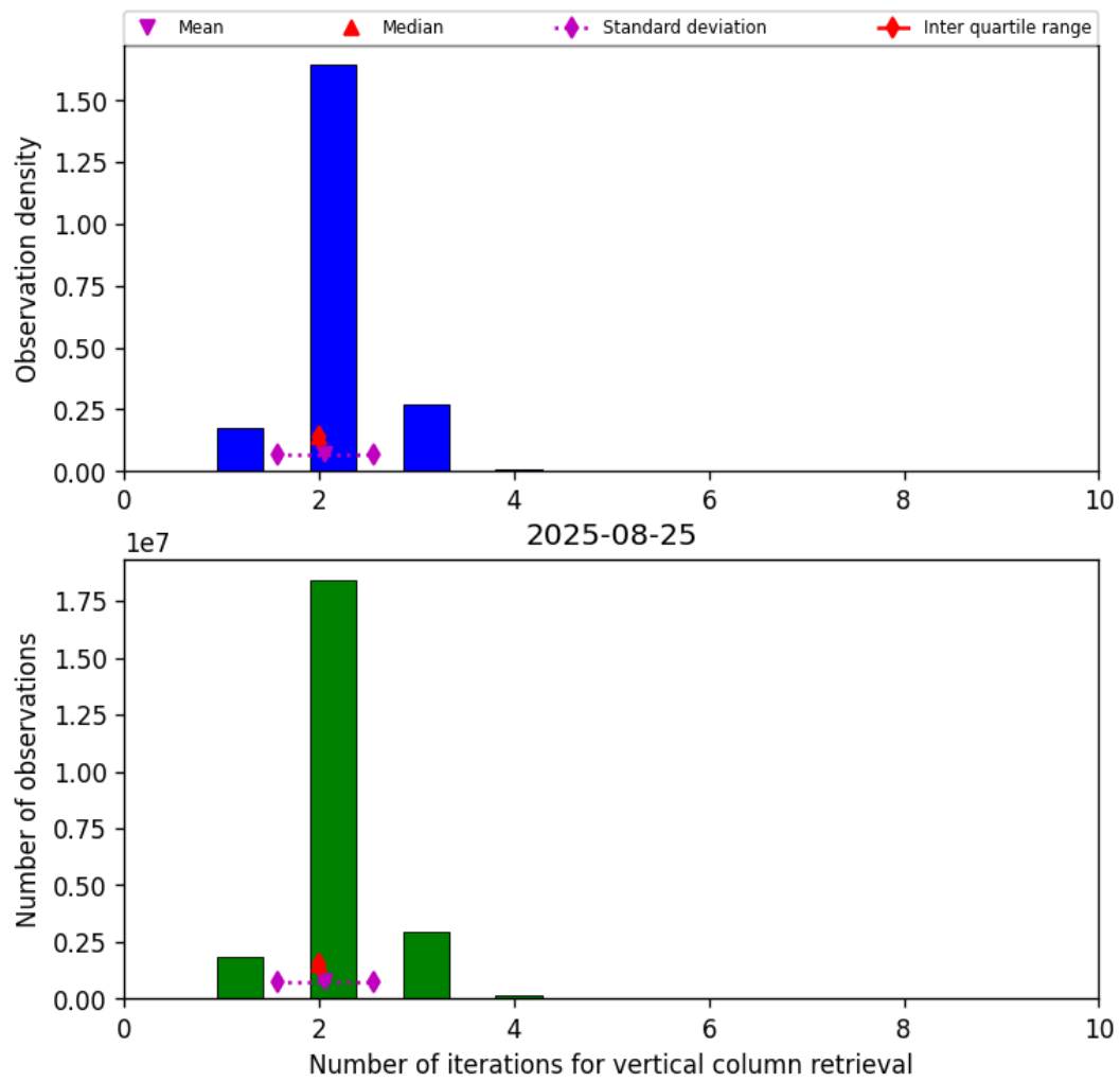
Figure 39: Histogram of “Number of iterations for vertical column retrieval” for 2025-08-25 to 2025-08-26
