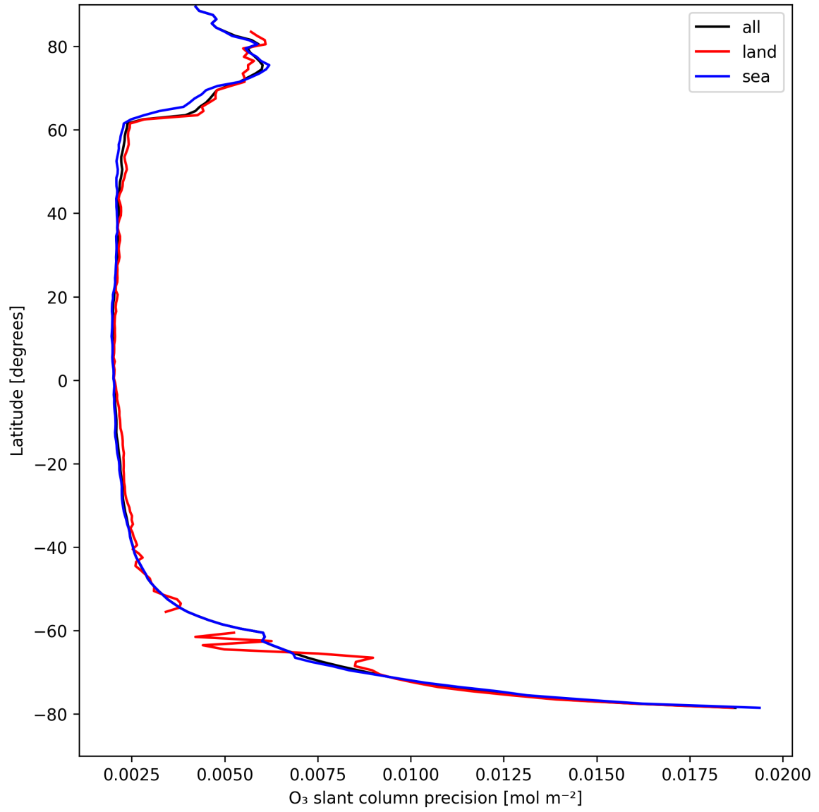
Figure 20: Zonal average of “O 3 slant column precision” for 2025-08-25 to 2025-08-26.
