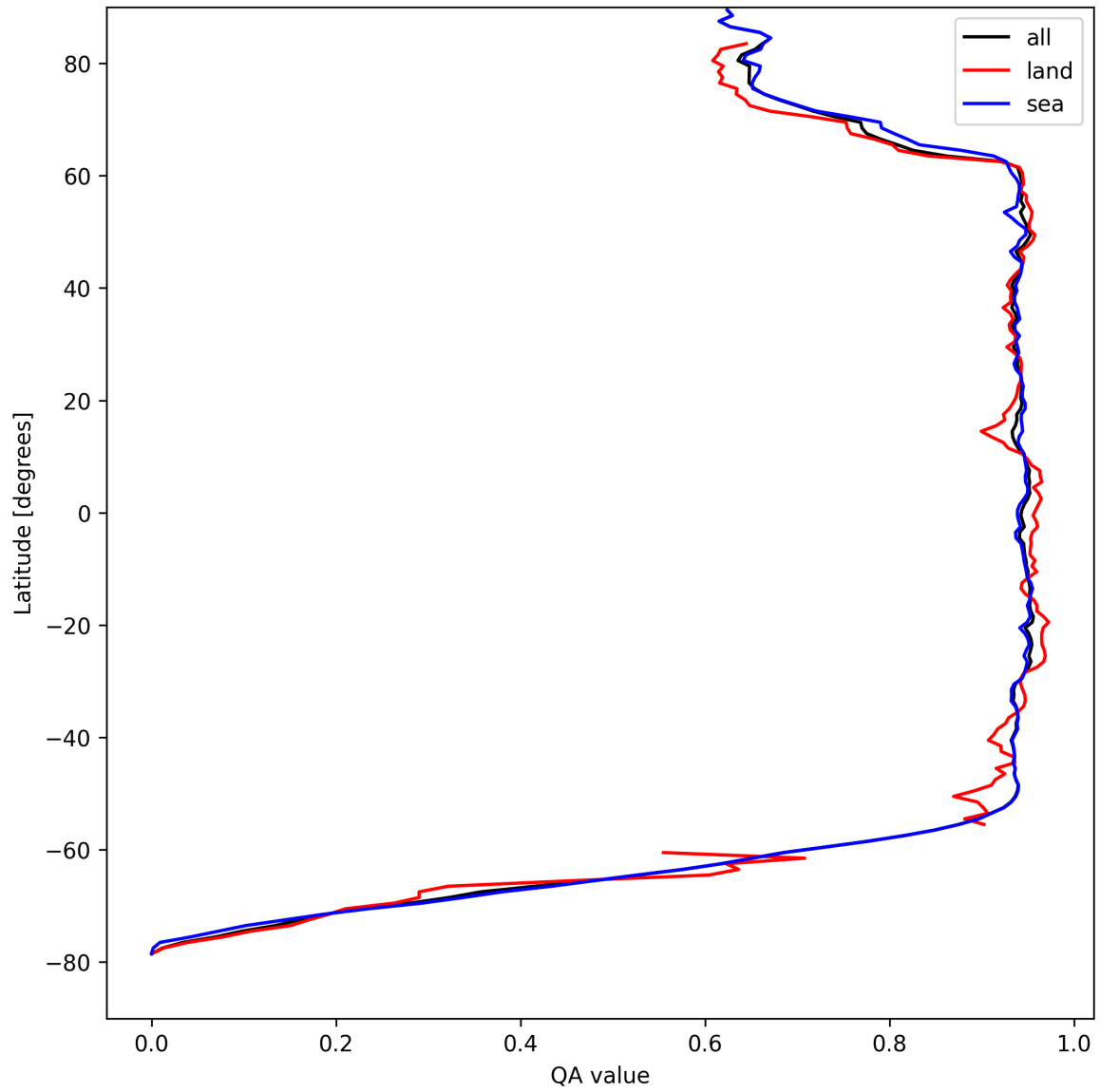
Figure 16: Zonal average of “QA value” for 2025-08-25 to 2025-08-26.
