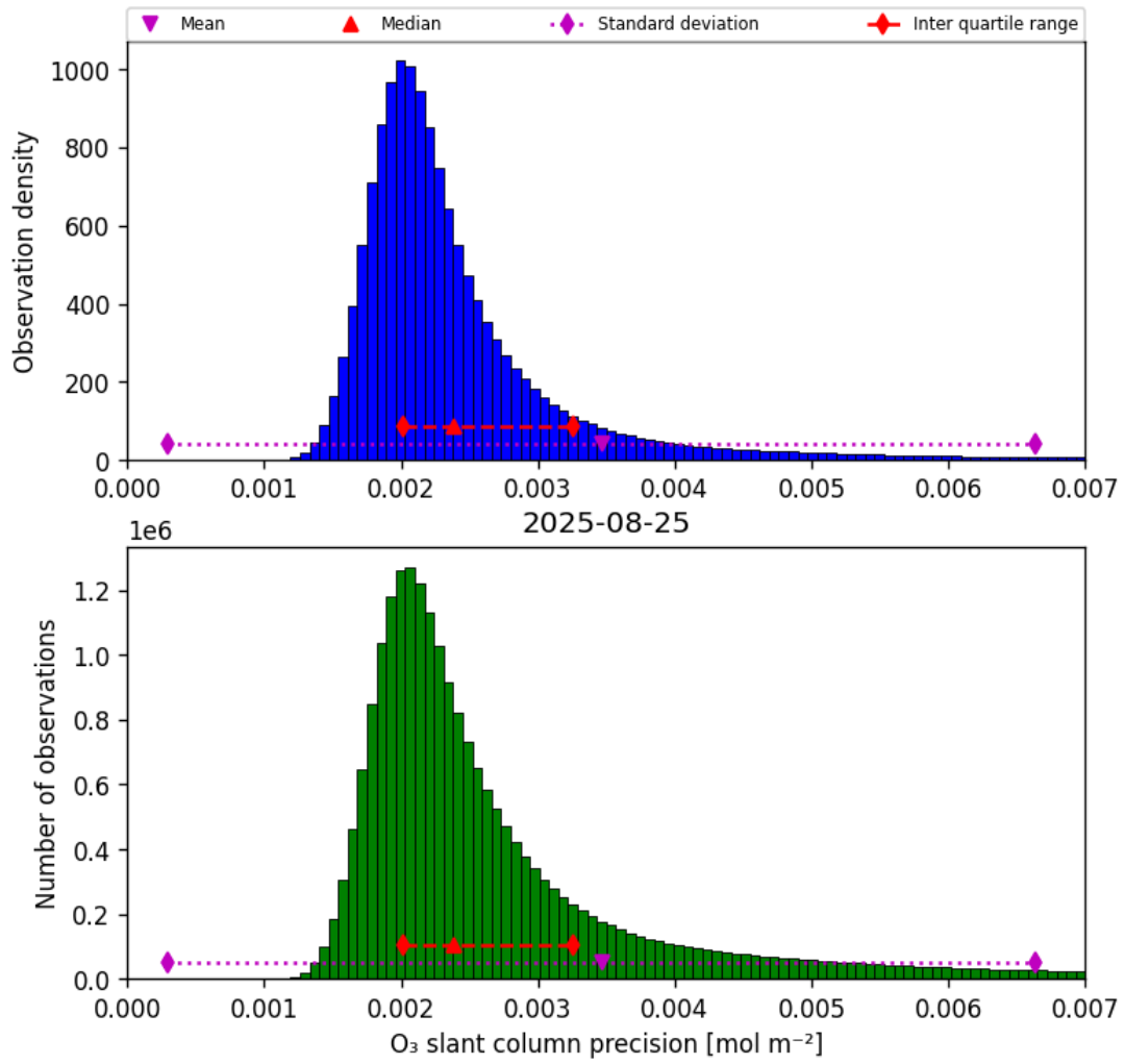
Figure 32: Histogram of “O 3 slant column precision” for 2025-08-25 to 2025-08-26
