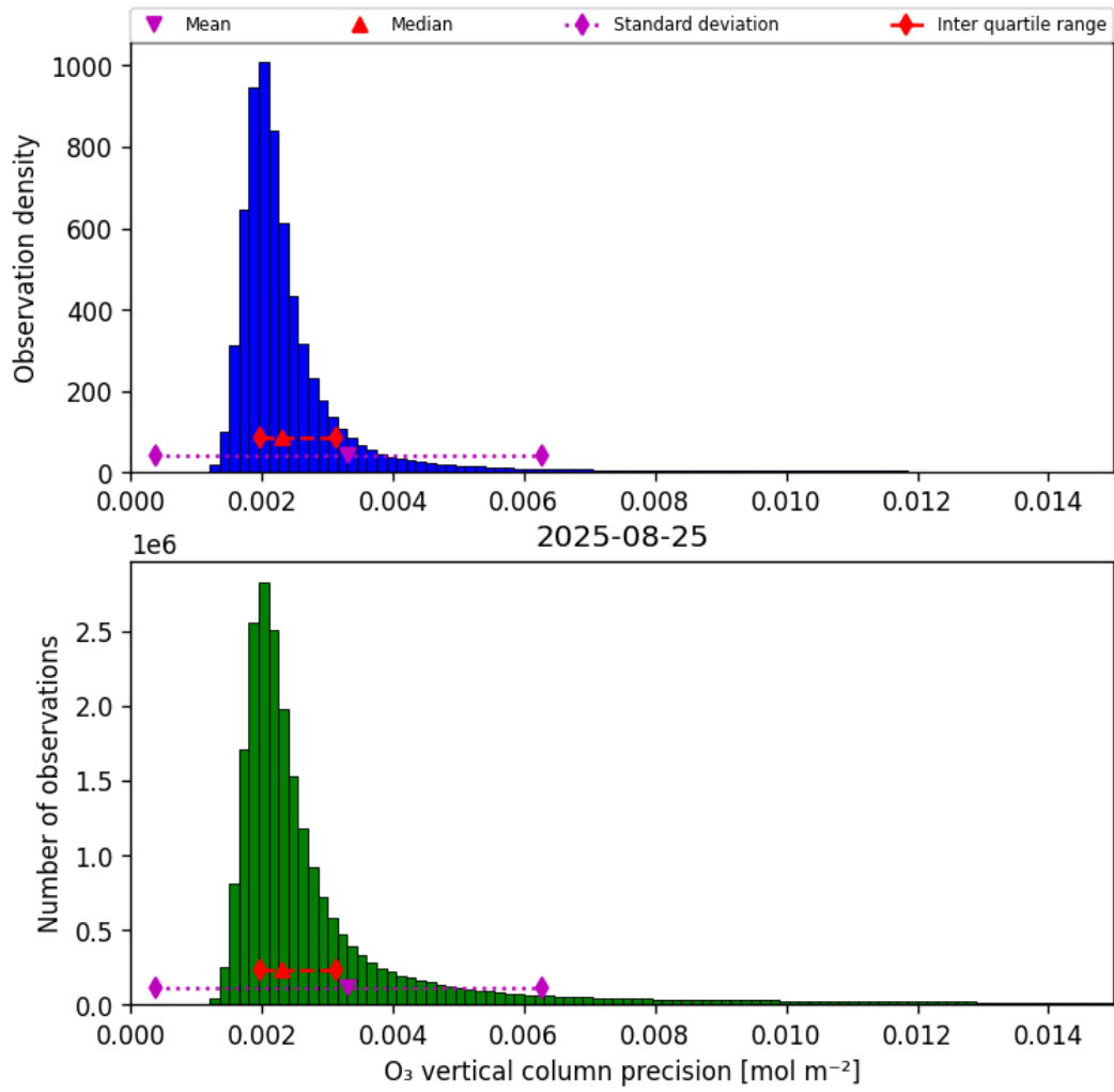
Figure 30: Histogram of “O 3 vertical column precision” for 2025-08-25 to 2025-08-26
