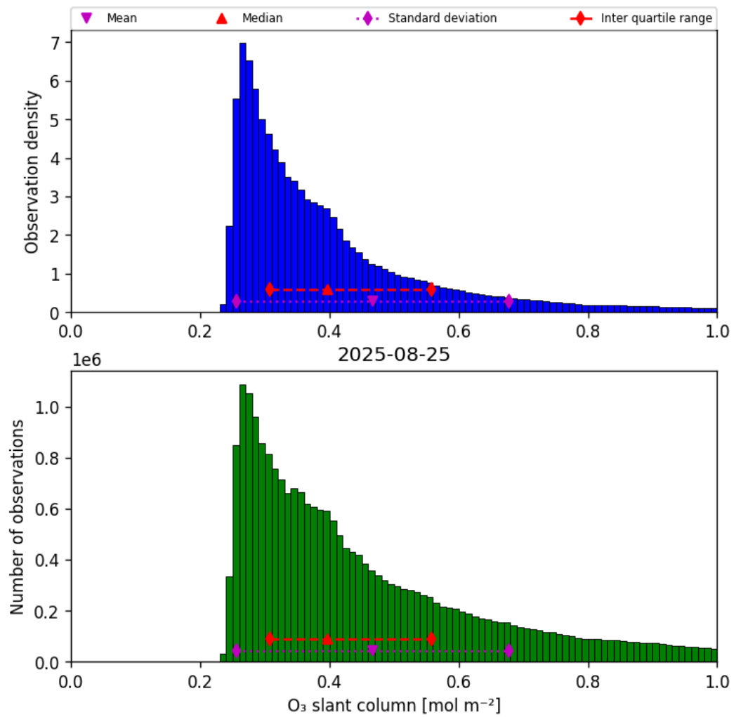
Figure 31: Histogram of “O 3 slant column” for 2025-08-25 to 2025-08-26
