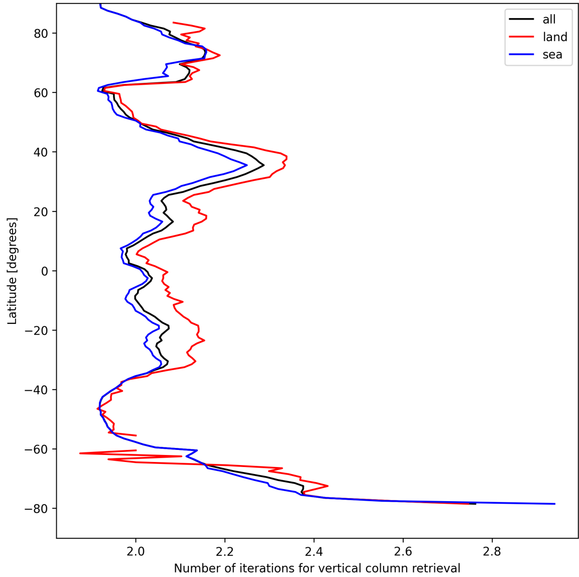
Figure 27: Zonal average of “Number of iterations for vertical column retrieval” for 2025-08-25 to 2025-08-26.
