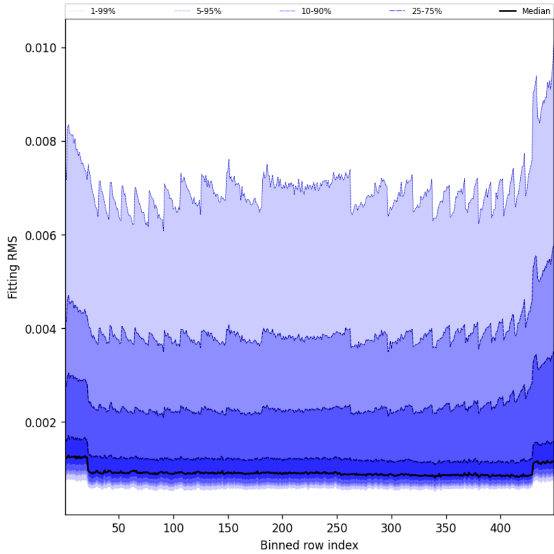
Figure 46: Along track statistics of “Fitting RMS” for 2025-08-25 to 2025-08-26
