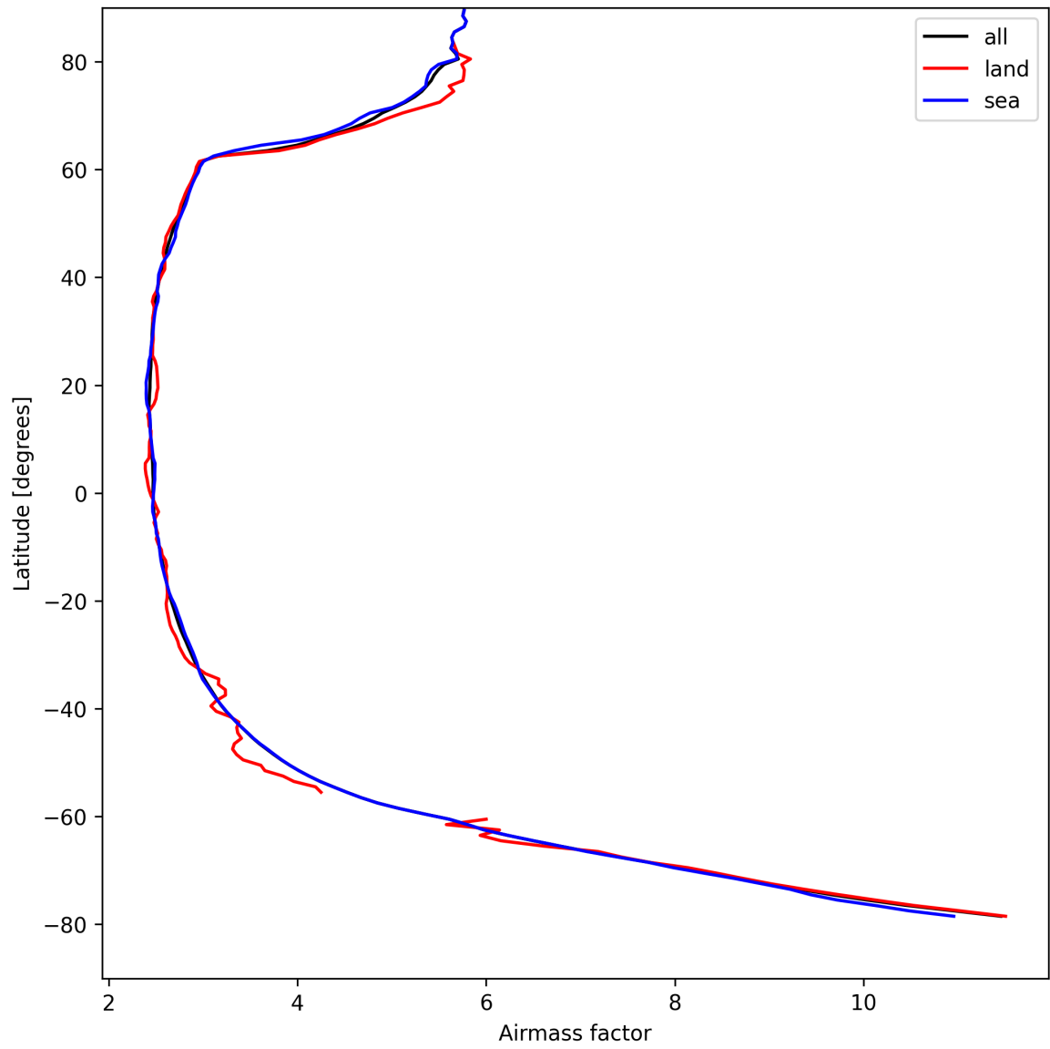
Figure 25: Zonal average of “Airmass factor” for 2025-08-25 to 2025-08-26.
