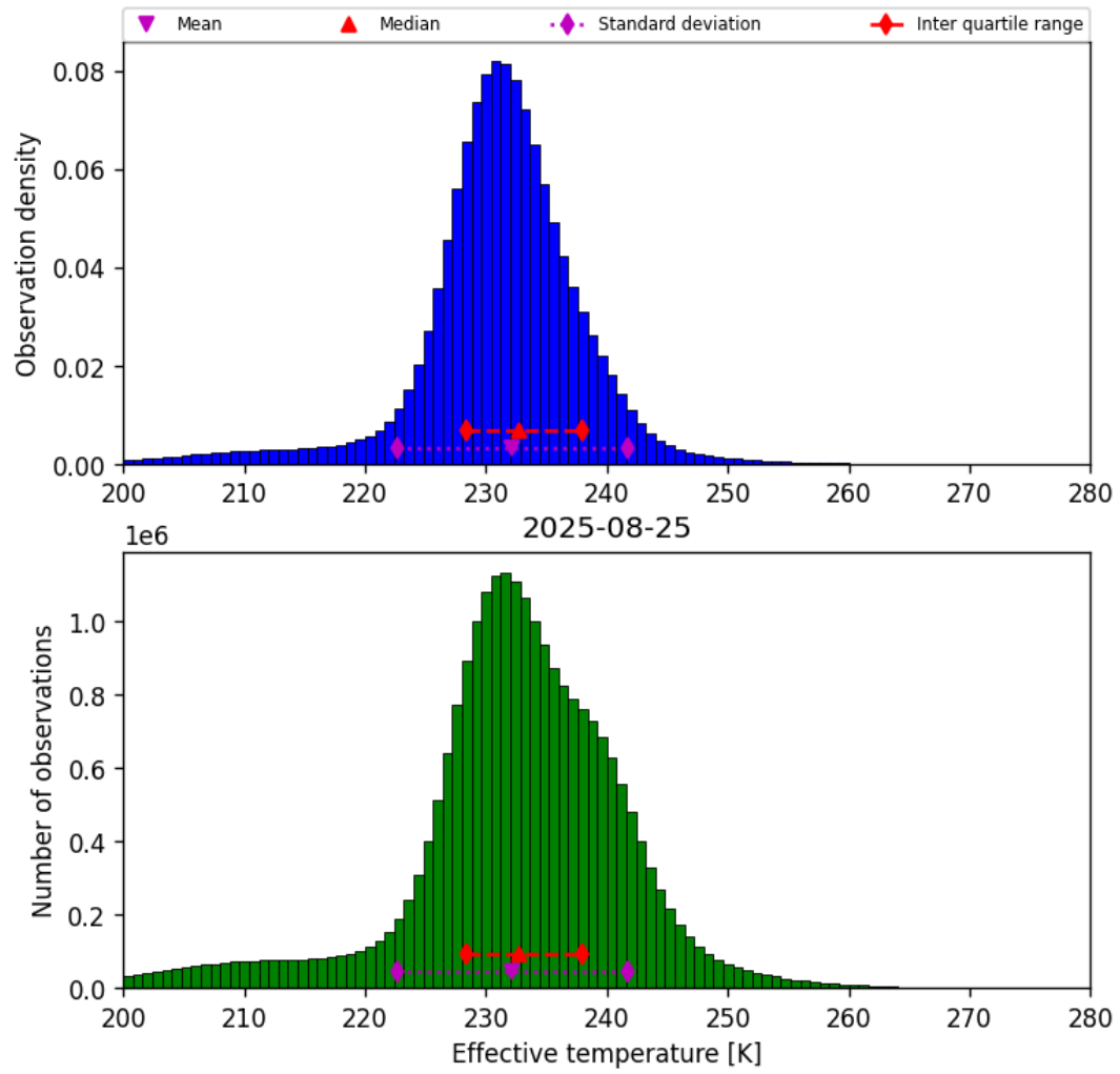
Figure 38: Histogram of “Effective temperature” for 2025-08-25 to 2025-08-26
