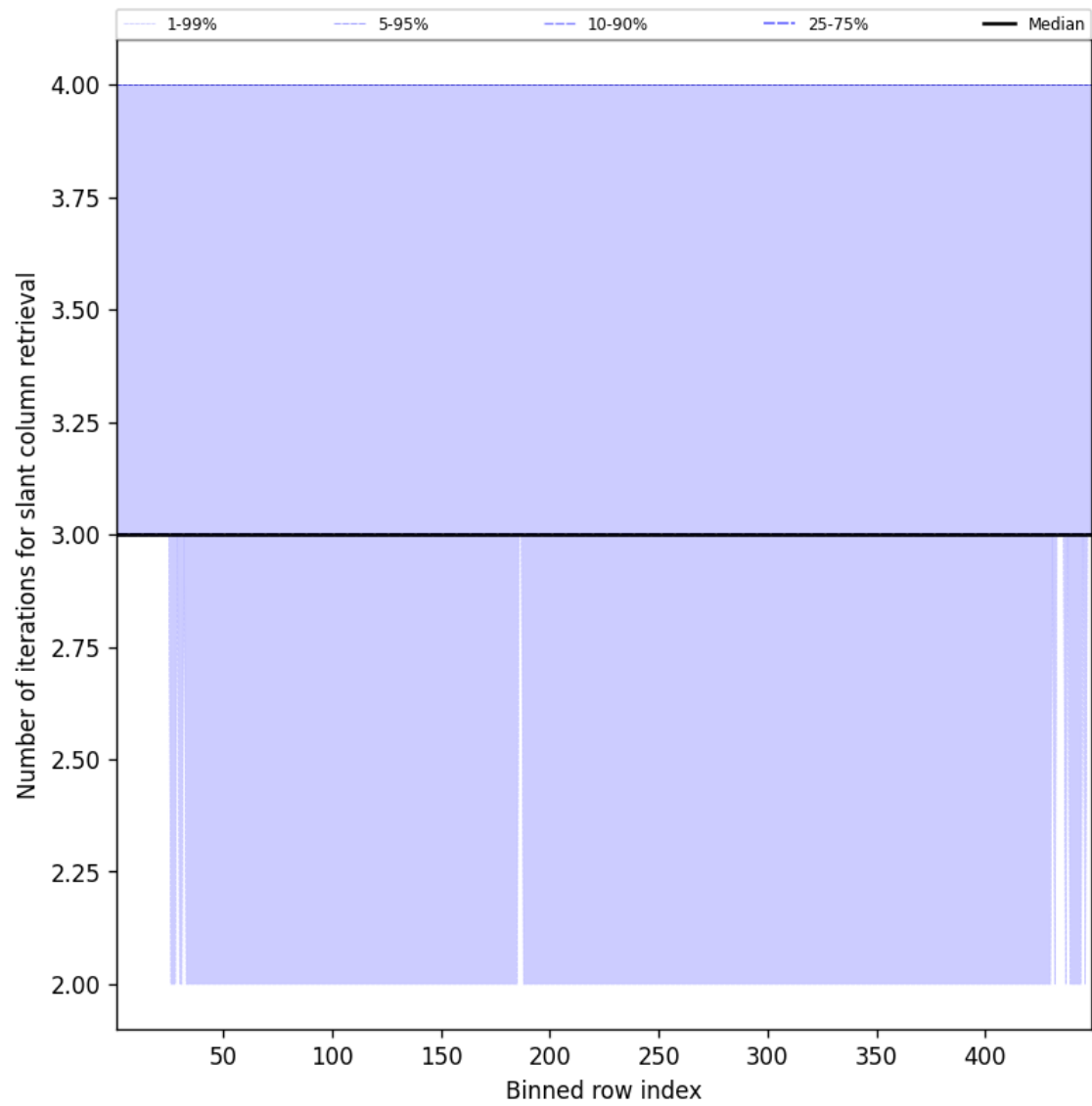
Figure 45: Along track statistics of “Number of iterations for slant column retrieval” for 2025-08-25 to 2025-08-26
