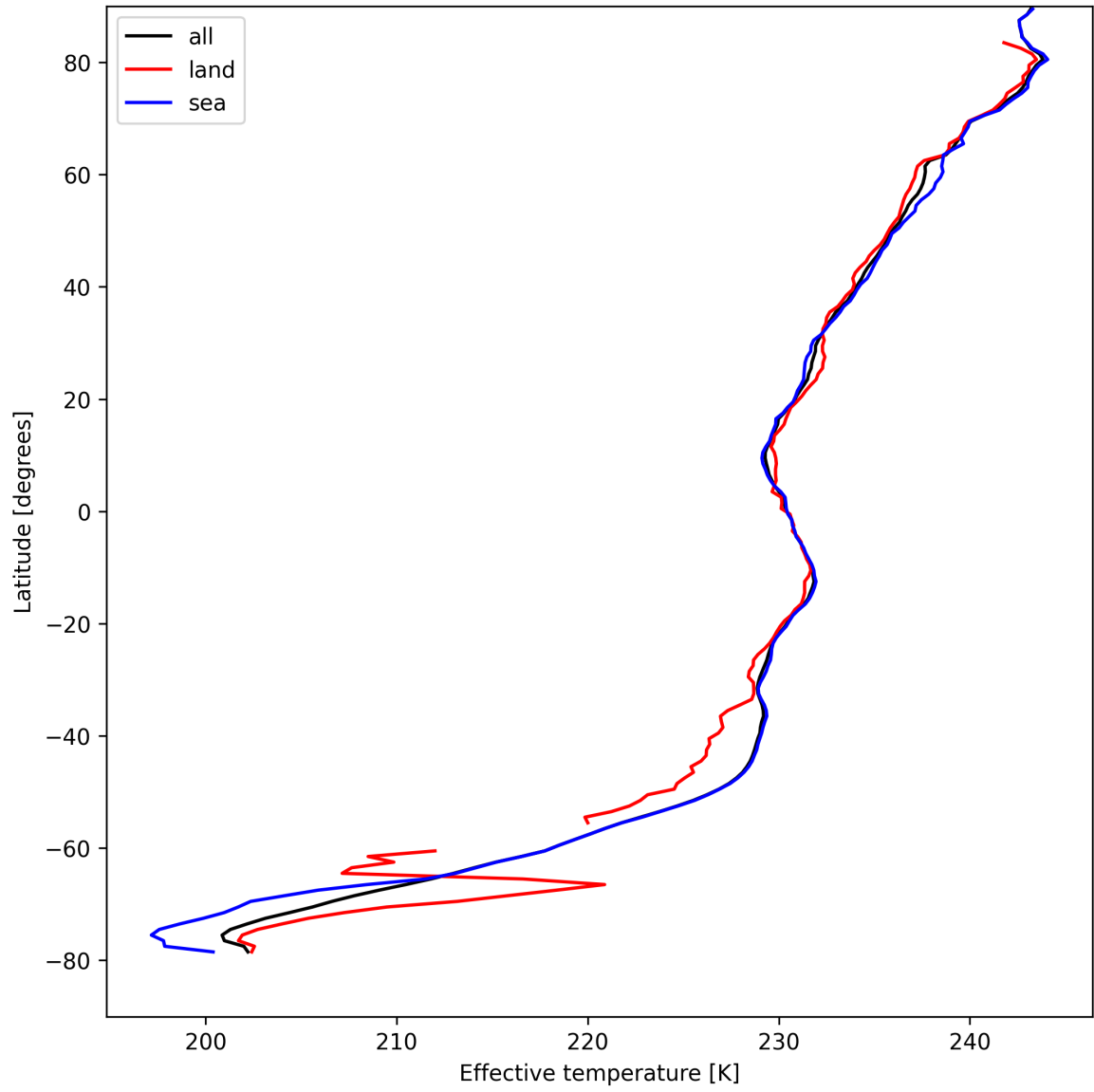
Figure 26: Zonal average of “Effective temperature” for 2025-08-25 to 2025-08-26.
