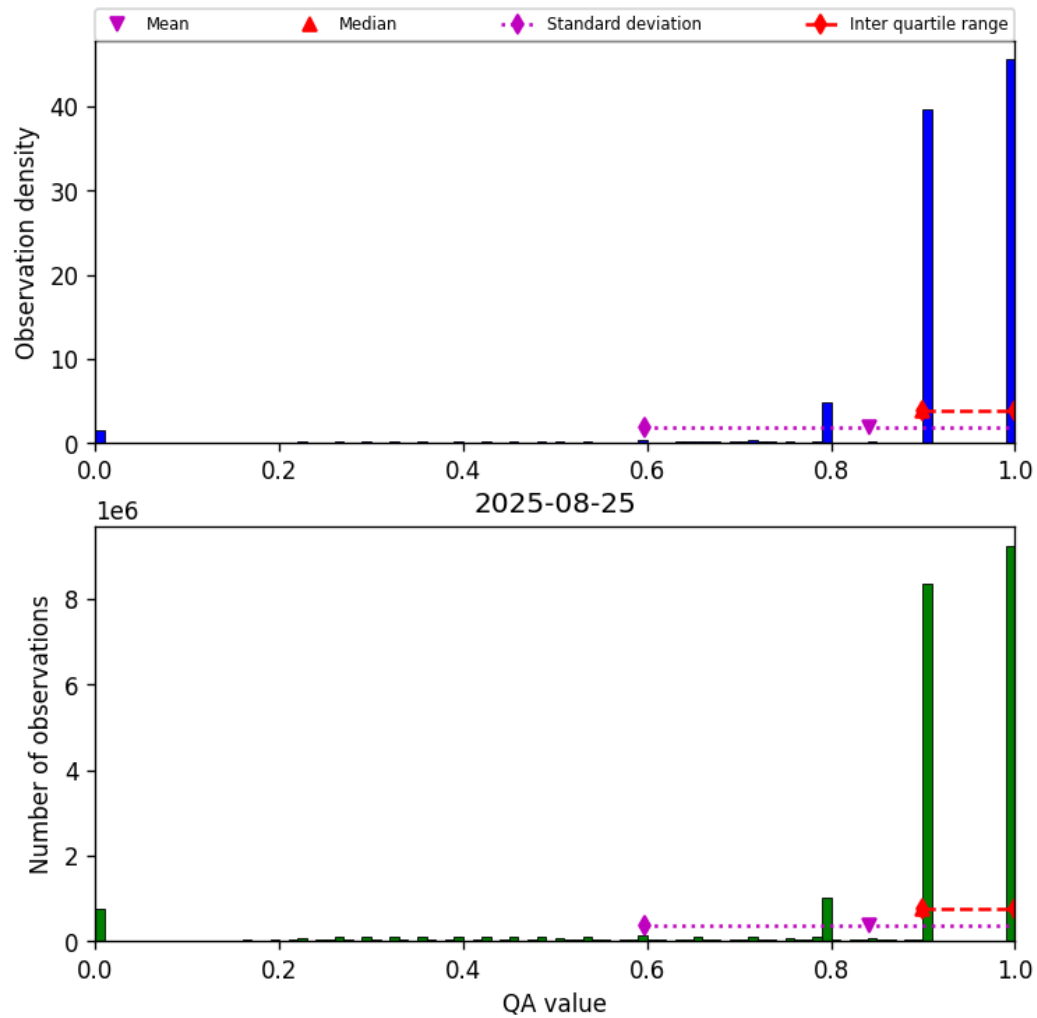
Figure 28: Histogram of “QA value” for 2025-08-25 to 2025-08-26
