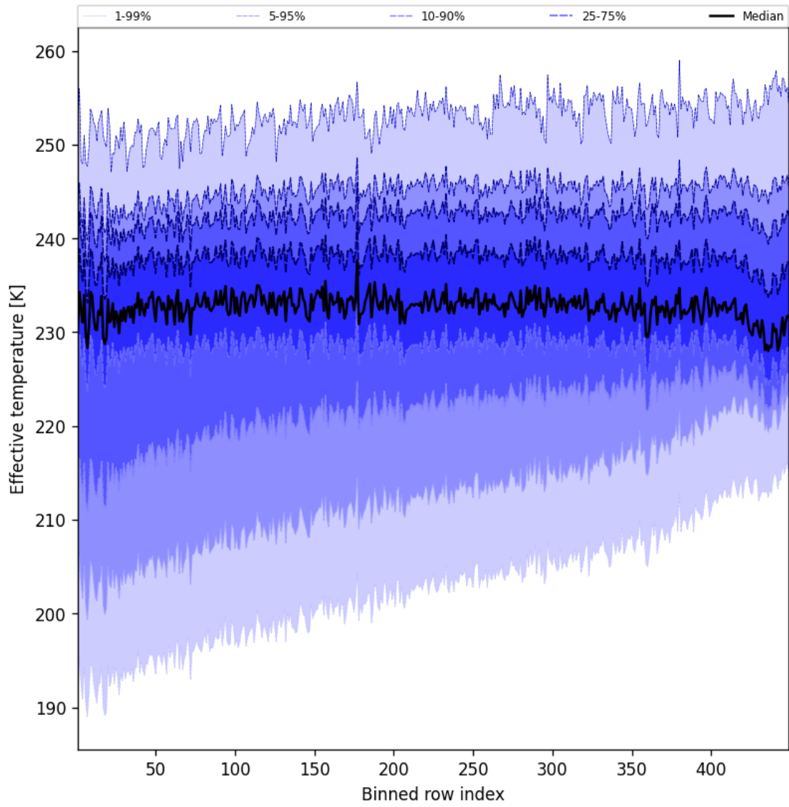
Figure 50: Along track statistics of “Effective temperature” for 2025-08-25 to 2025-08-26
