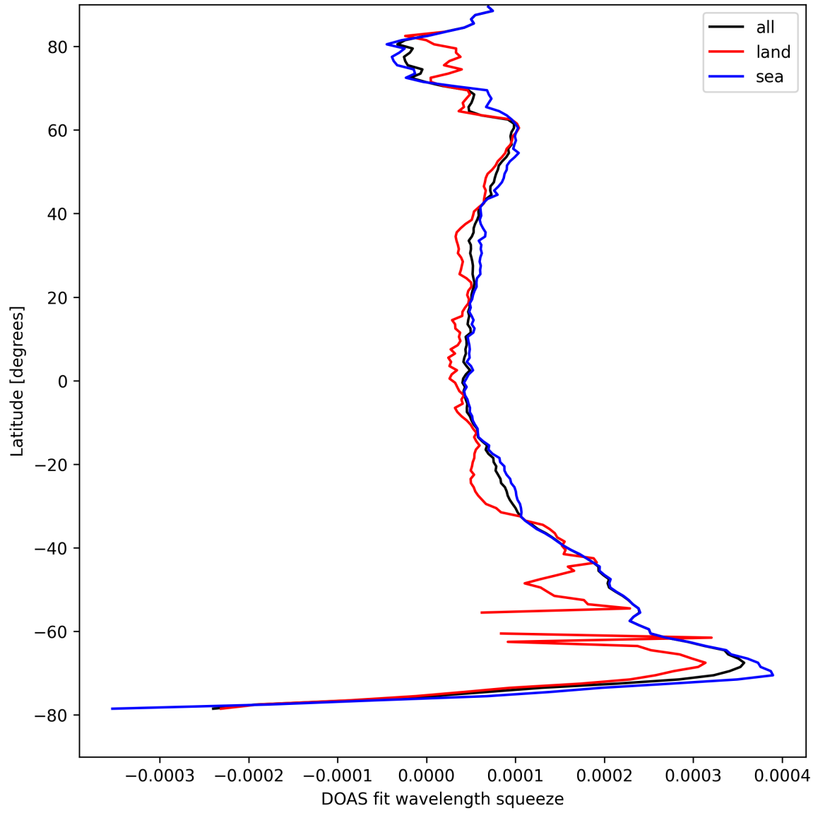
Figure 24: Zonal average of “DOAS fit wavelength squeeze” for 2025-08-25 to 2025-08-26.
