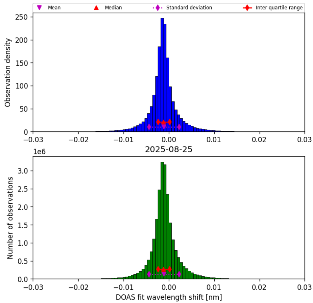
Figure 35: Histogram of “DOAS fit wavelength shift” for 2025-08-25 to 2025-08-26
