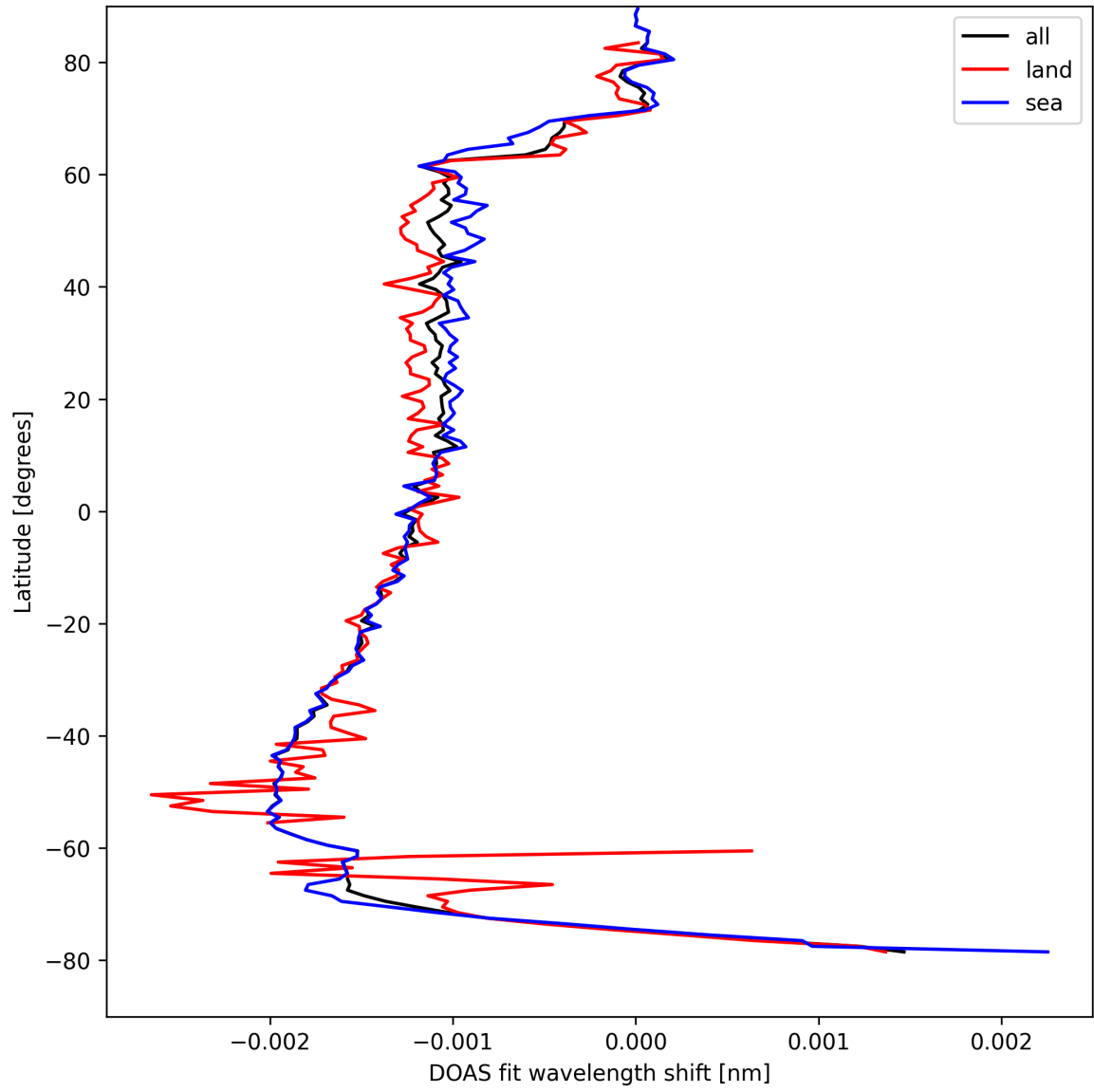
Figure 23: Zonal average of “DOAS fit wavelength shift” for 2025-08-25 to 2025-08-26.
