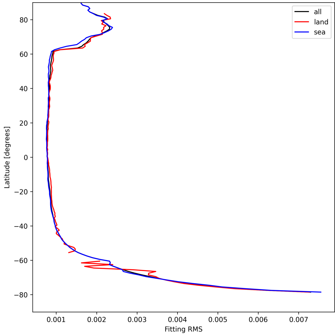
Figure 22: Zonal average of “Fitting RMS” for 2025-08-25 to 2025-08-26.
