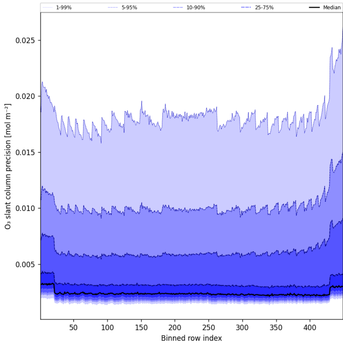
Figure 44: Along track statistics of “O 3 slant column precision” for 2025-08-25 to 2025-08-26
