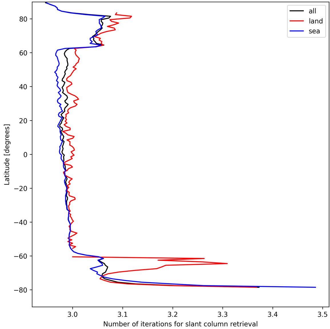
Figure 21: Zonal average of “Number of iterations for slant column retrieval” for 2025-08-26 to 2025-08-27.
