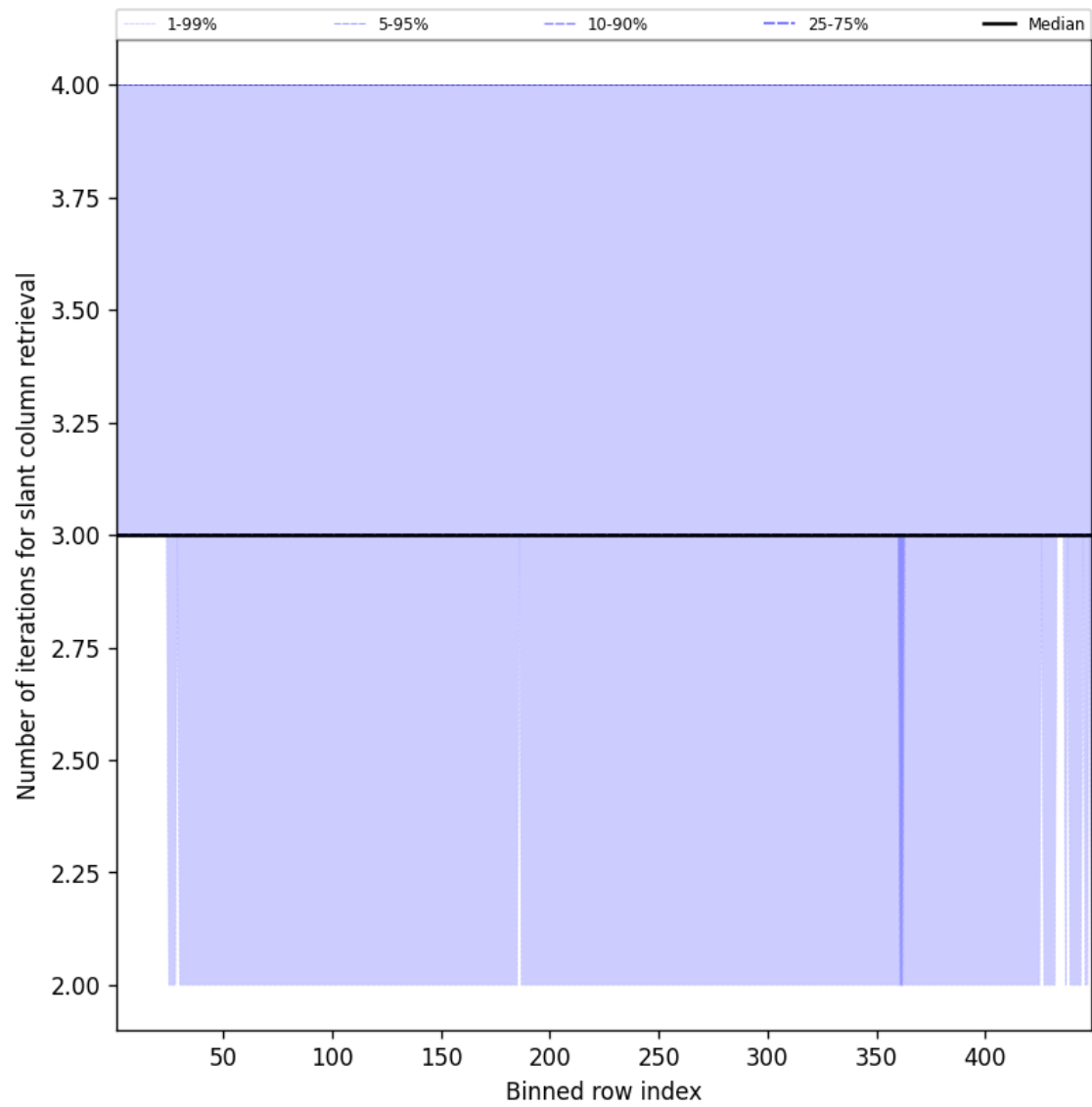
Figure 45: Along track statistics of “Number of iterations for slant column retrieval” for 2025-08-26 to 2025-08-27
