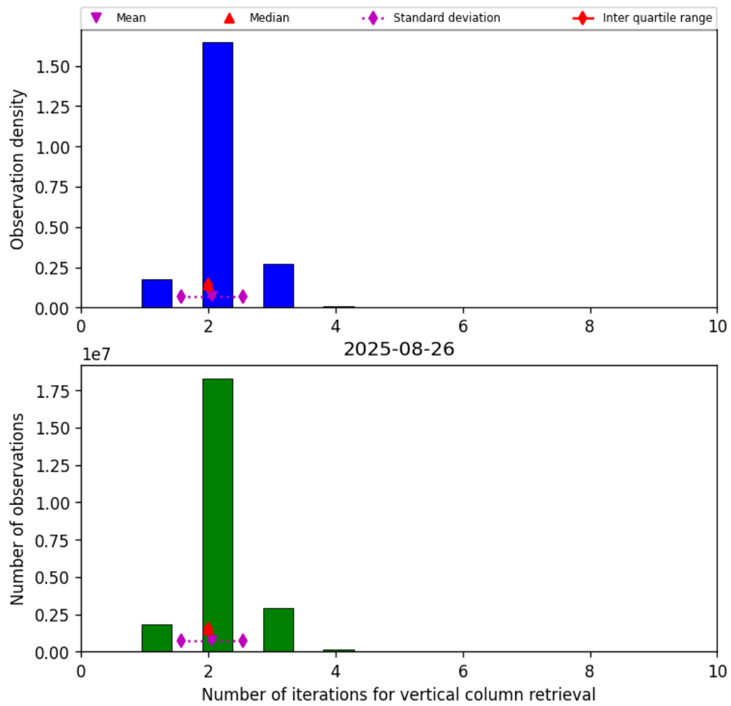
Figure 39: Histogram of “Number of iterations for vertical column retrieval” for 2025-08-26 to 2025-08-27
