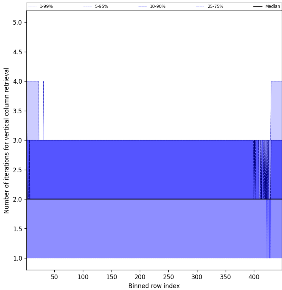
Figure 51: Along track statistics of “Number of iterations for vertical column retrieval” for 2025-08-26 to 2025-08-27
