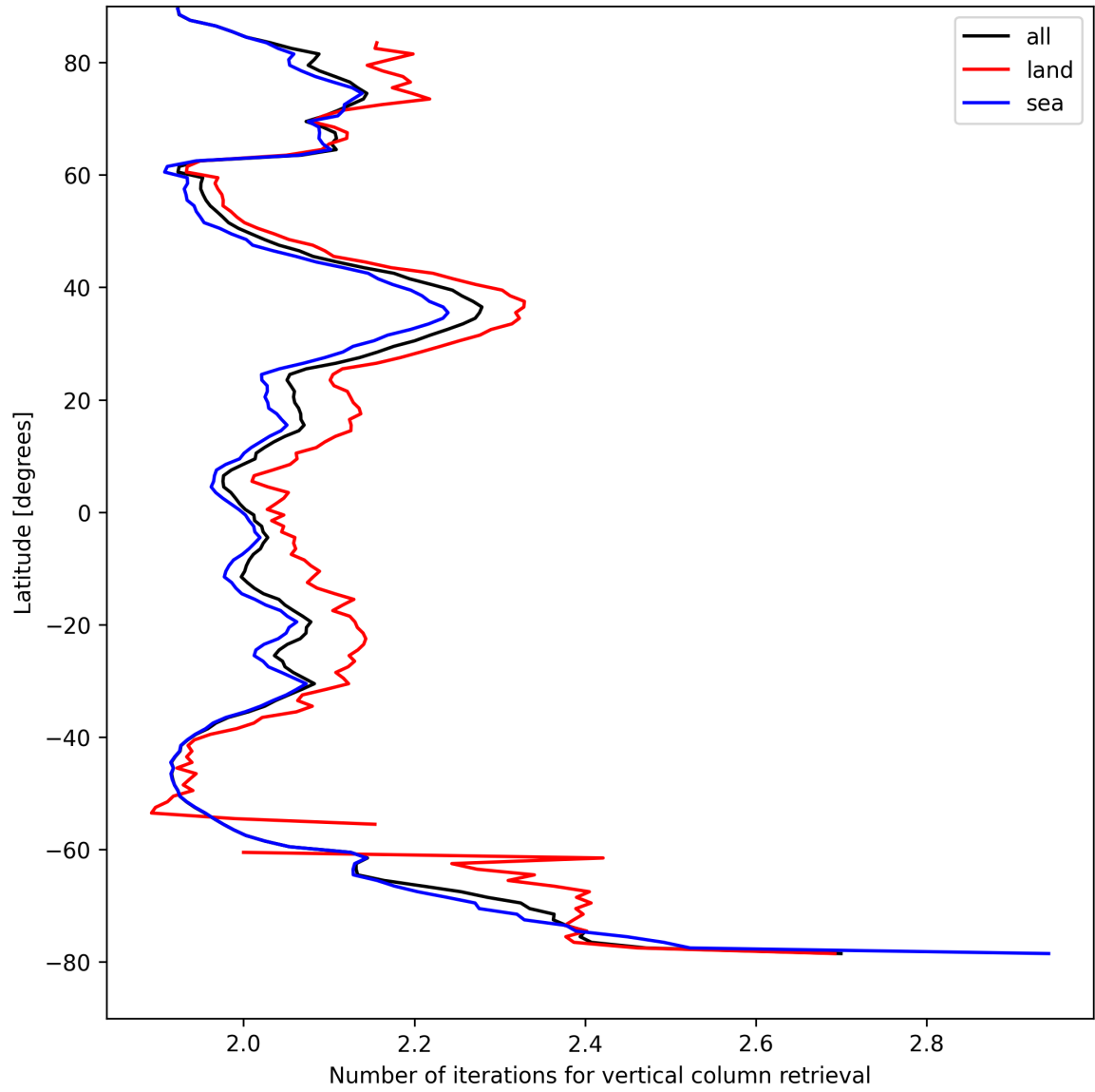
Figure 27: Zonal average of “Number of iterations for vertical column retrieval” for 2025-08-26 to 2025-08-27.
