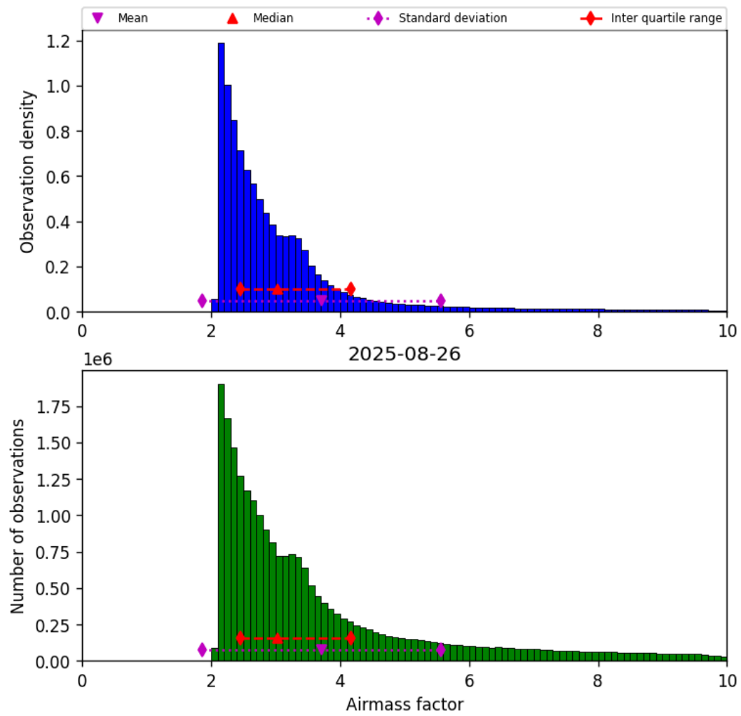
Figure 37: Histogram of “Airmass factor” for 2025-08-26 to 2025-08-27
