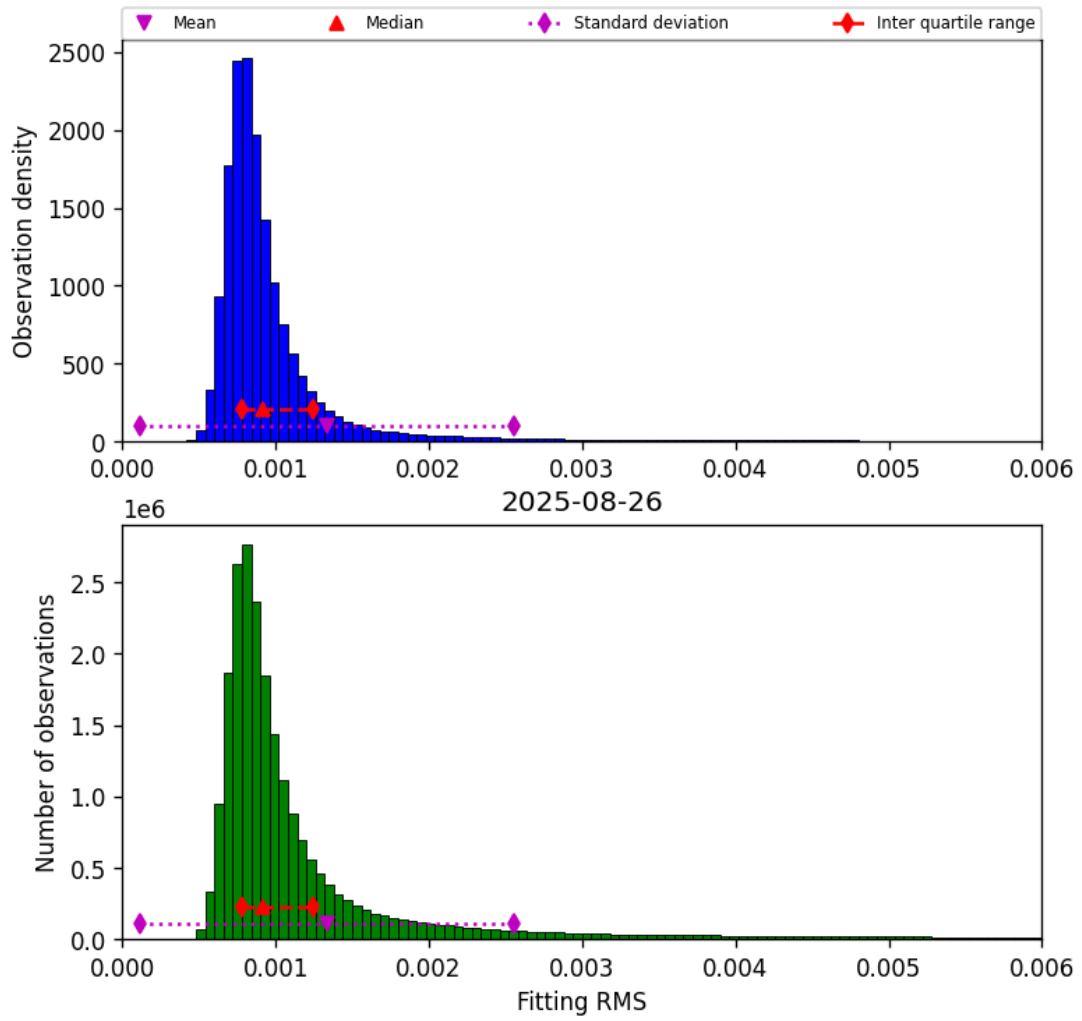
Figure 34: Histogram of "Fitting RMS" for 2025-08-26 to 2025-08-27
