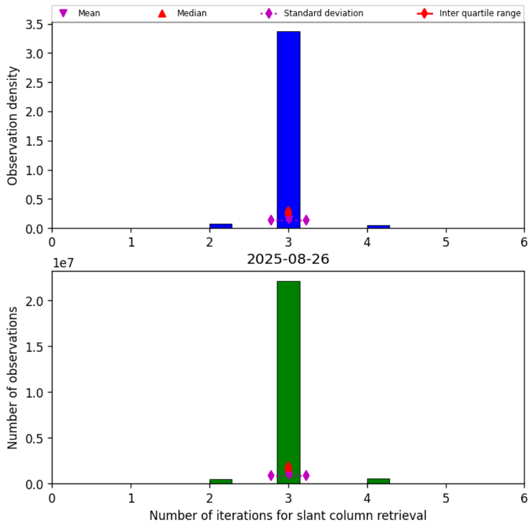
Figure 33: Histogram of "Number of iterations for slant column retrieval" for 2025-08-26 to 2025-08-27
