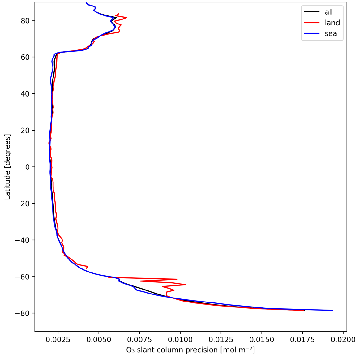
Figure 20: Zonal average of “O 3 slant column precision” for 2025-08-26 to 2025-08-27.
