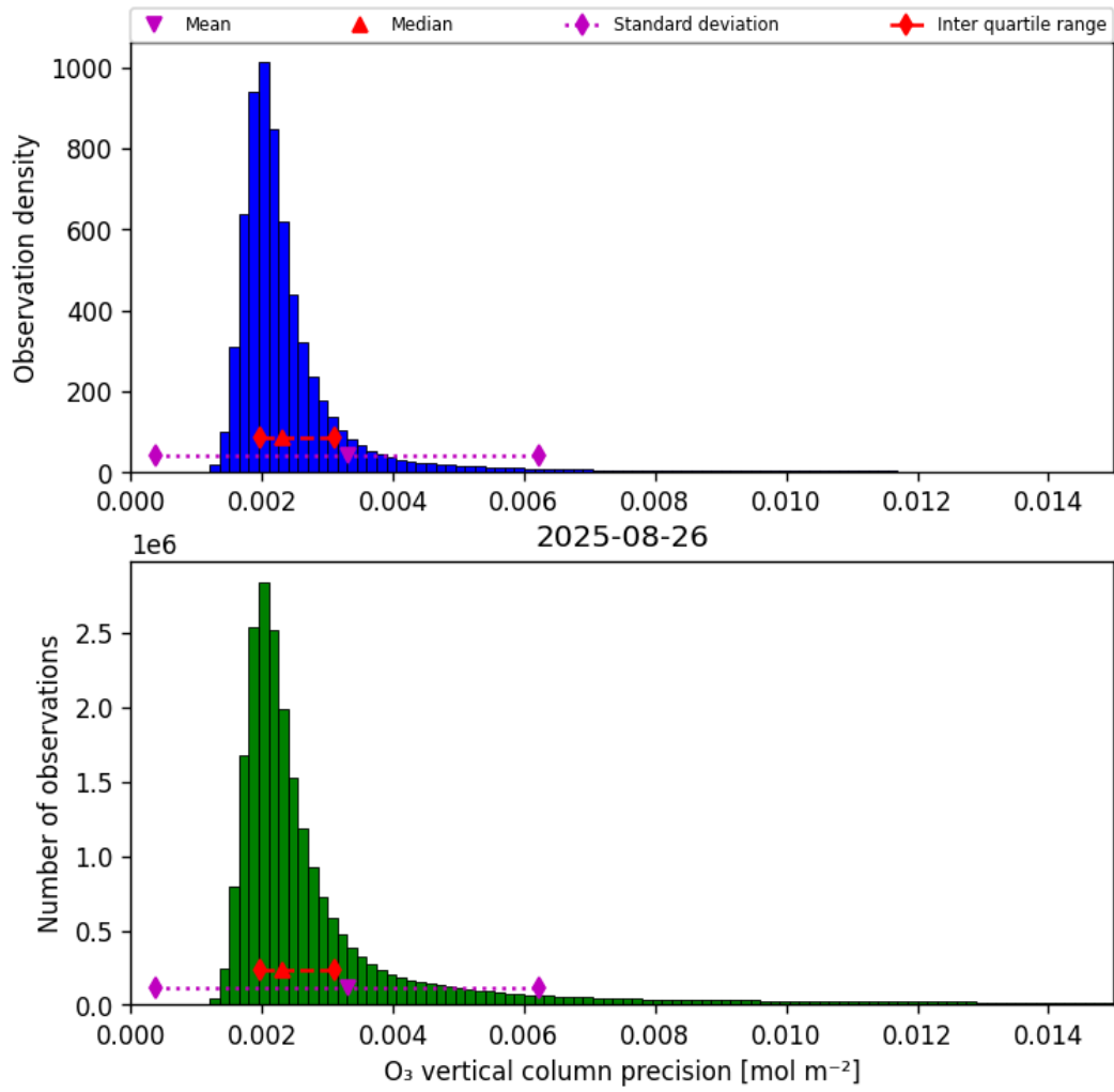
Figure 30: Histogram of “O 3 vertical column precision” for 2025-08-26 to 2025-08-27
