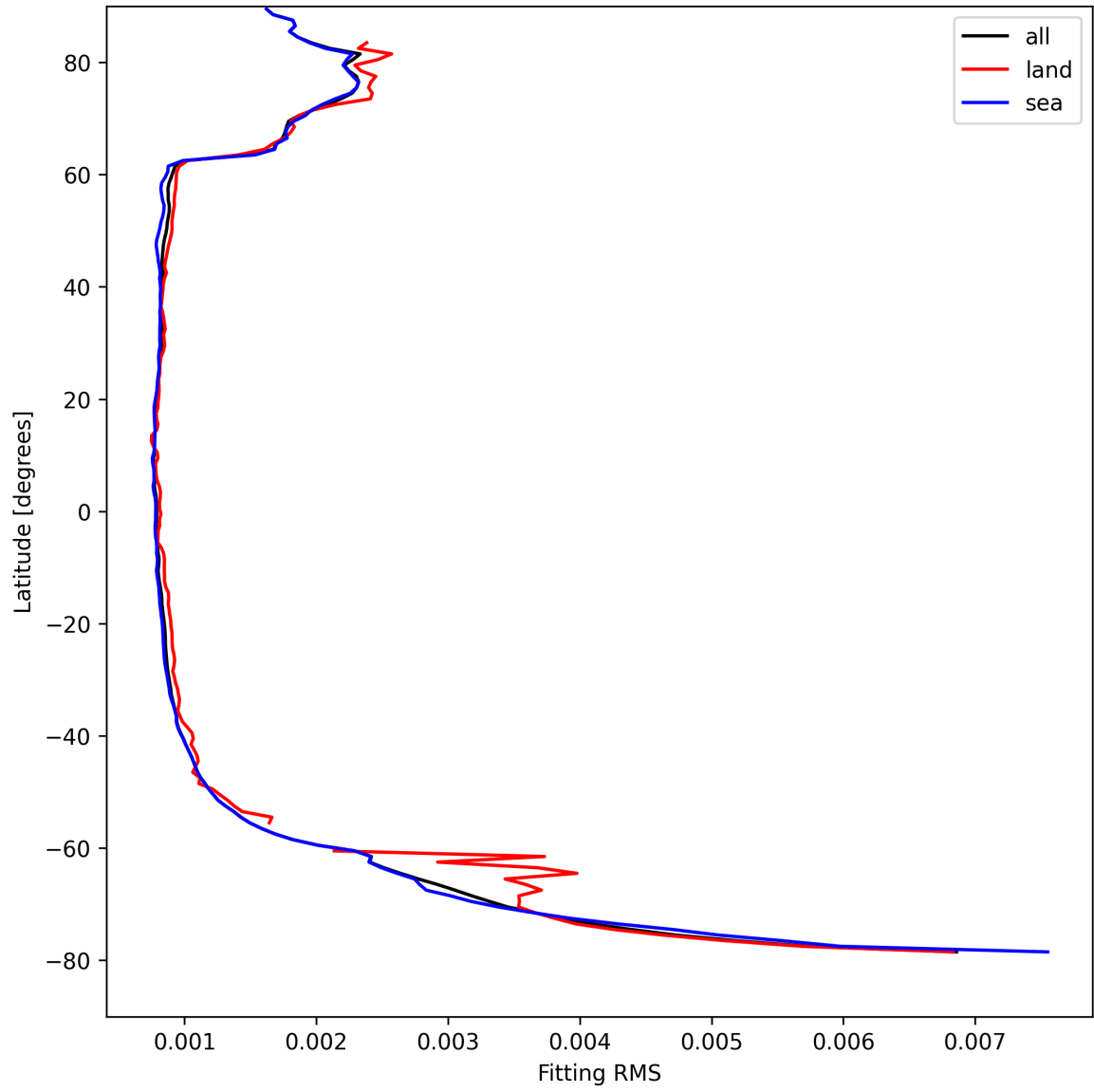
Figure 22: Zonal average of “Fitting RMS” for 2025-08-26 to 2025-08-27.
