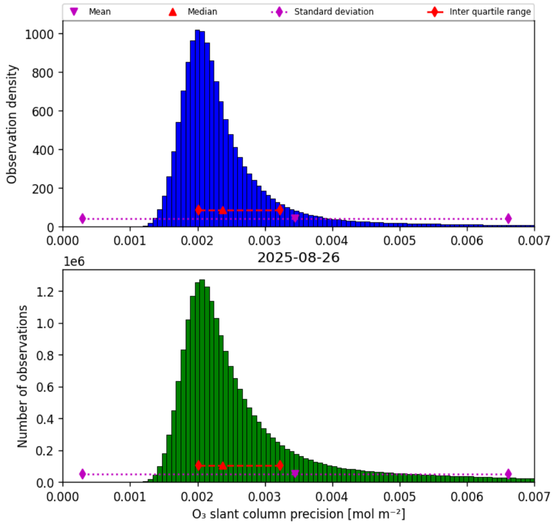
Figure 32: Histogram of “O 3 slant column precision” for 2025-08-26 to 2025-08-27
