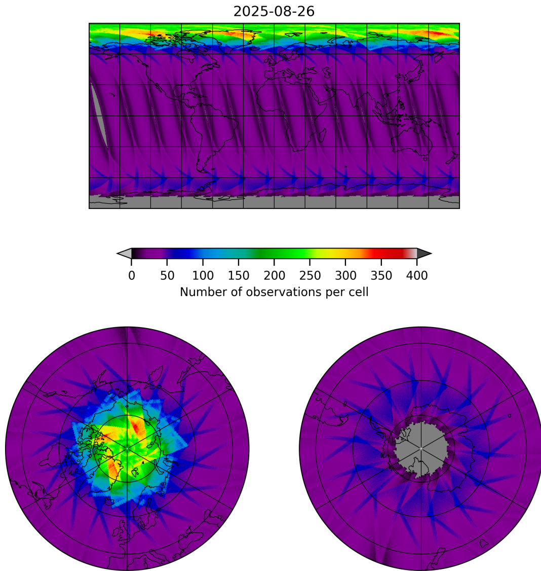
Figure 15: Map of the number of observations for 2025-08-26 to 2025-08-27
