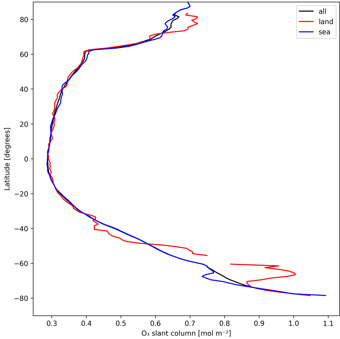
Figure 19: Zonal average of “O 3 slant column” for 2025-08-26 to 2025-08-27.
