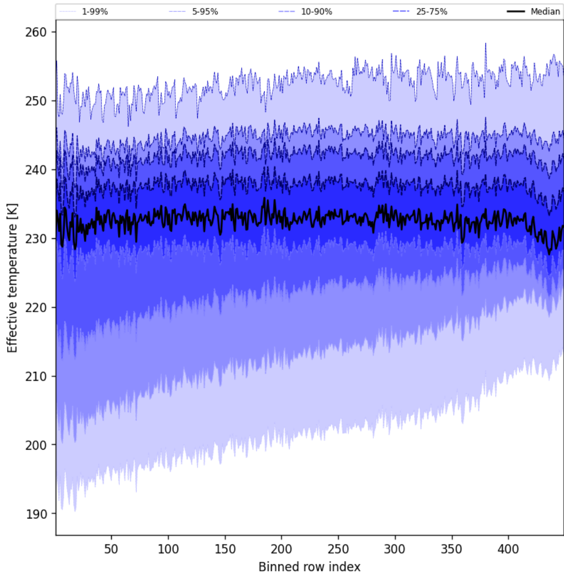
Figure 50: Along track statistics of “Effective temperature” for 2025-08-26 to 2025-08-27
