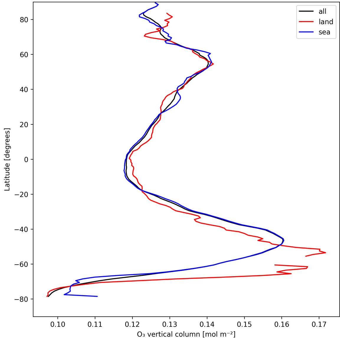
Figure 17: Zonal average of “O 3 vertical column” for 2025-08-26 to 2025-08-27.
