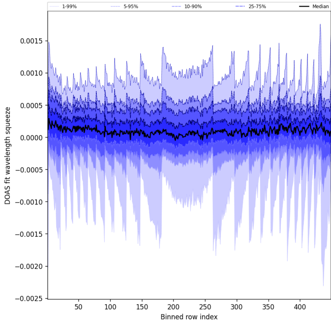
Figure 48: Along track statistics of “DOAS fit wavelength squeeze” for 2025-08-26 to 2025-08-27
