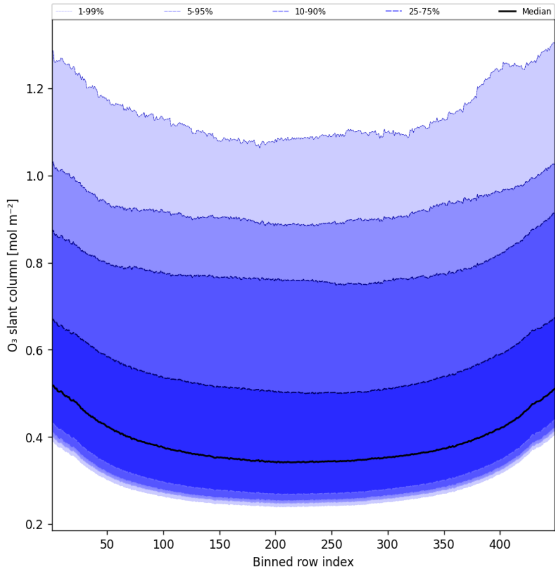
Figure 43: Along track statistics of “O 3 slant column” for 2025-08-26 to 2025-08-27
