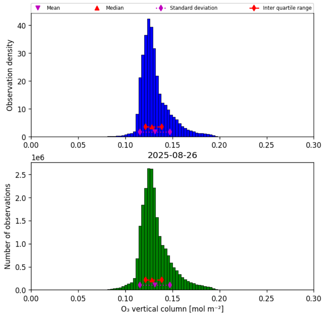
Figure 29: Histogram of “O 3 vertical column” for 2025-08-26 to 2025-08-27
