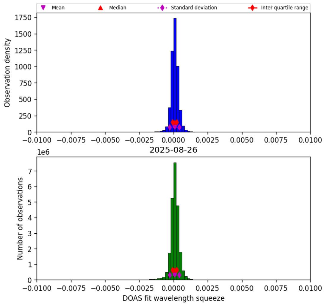
Figure 36: Histogram of “DOAS fit wavelength squeeze” for 2025-08-26 to 2025-08-27
