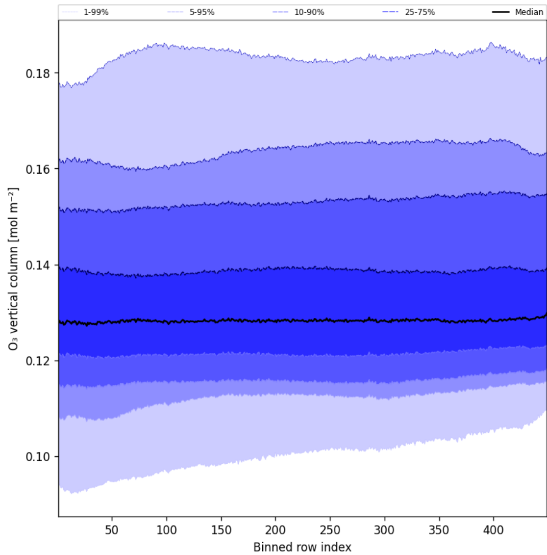
Figure 41: Along track statistics of “O 3 vertical column” for 2025-08-26 to 2025-08-27
