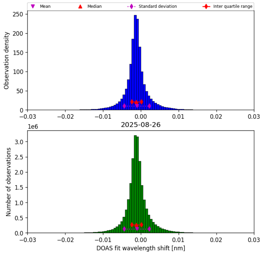
Figure 35: Histogram of “DOAS fit wavelength shift” for 2025-08-26 to 2025-08-27
