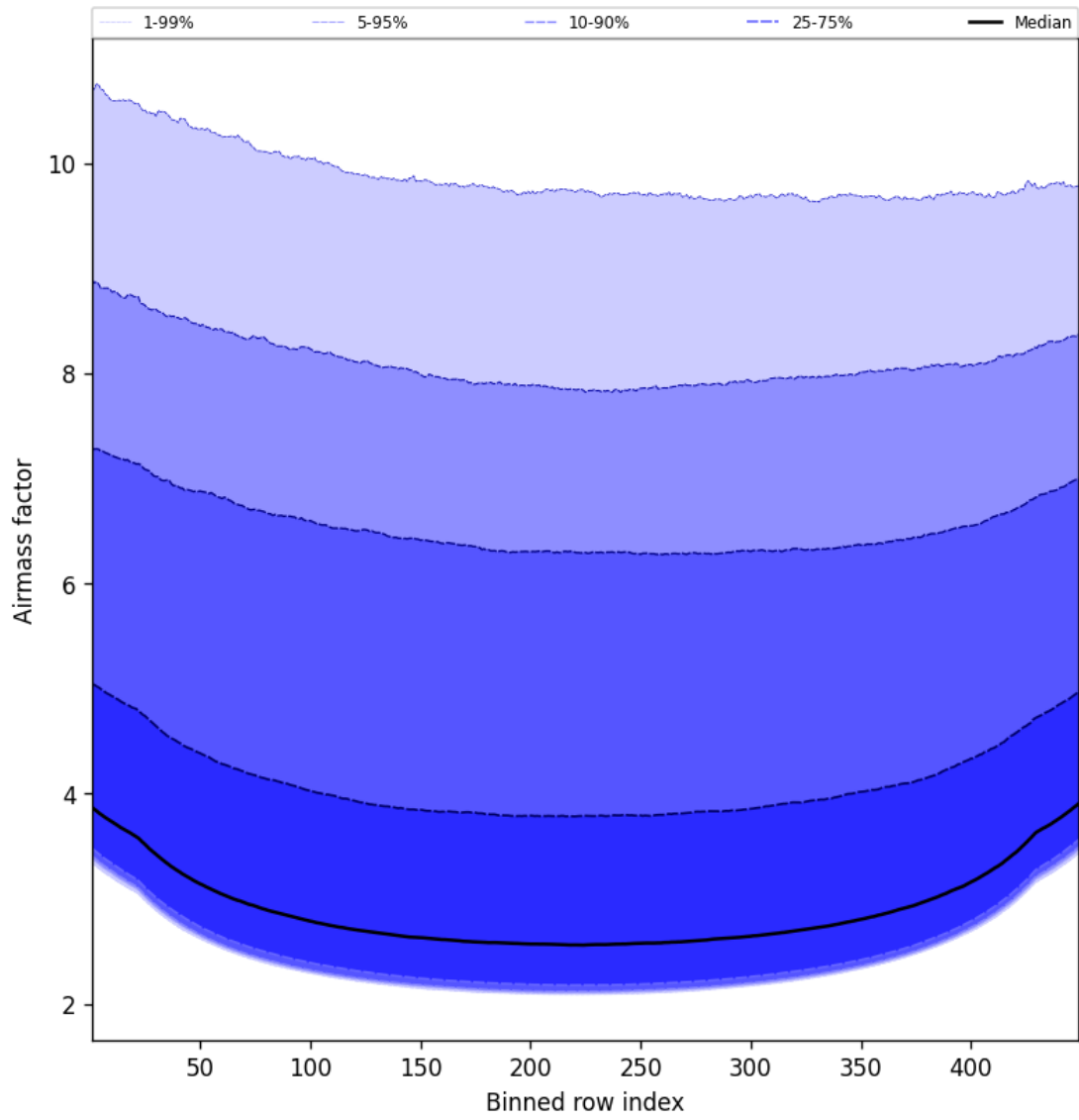
Figure 49: Along track statistics of “Airmass factor” for 2025-08-26 to 2025-08-27
