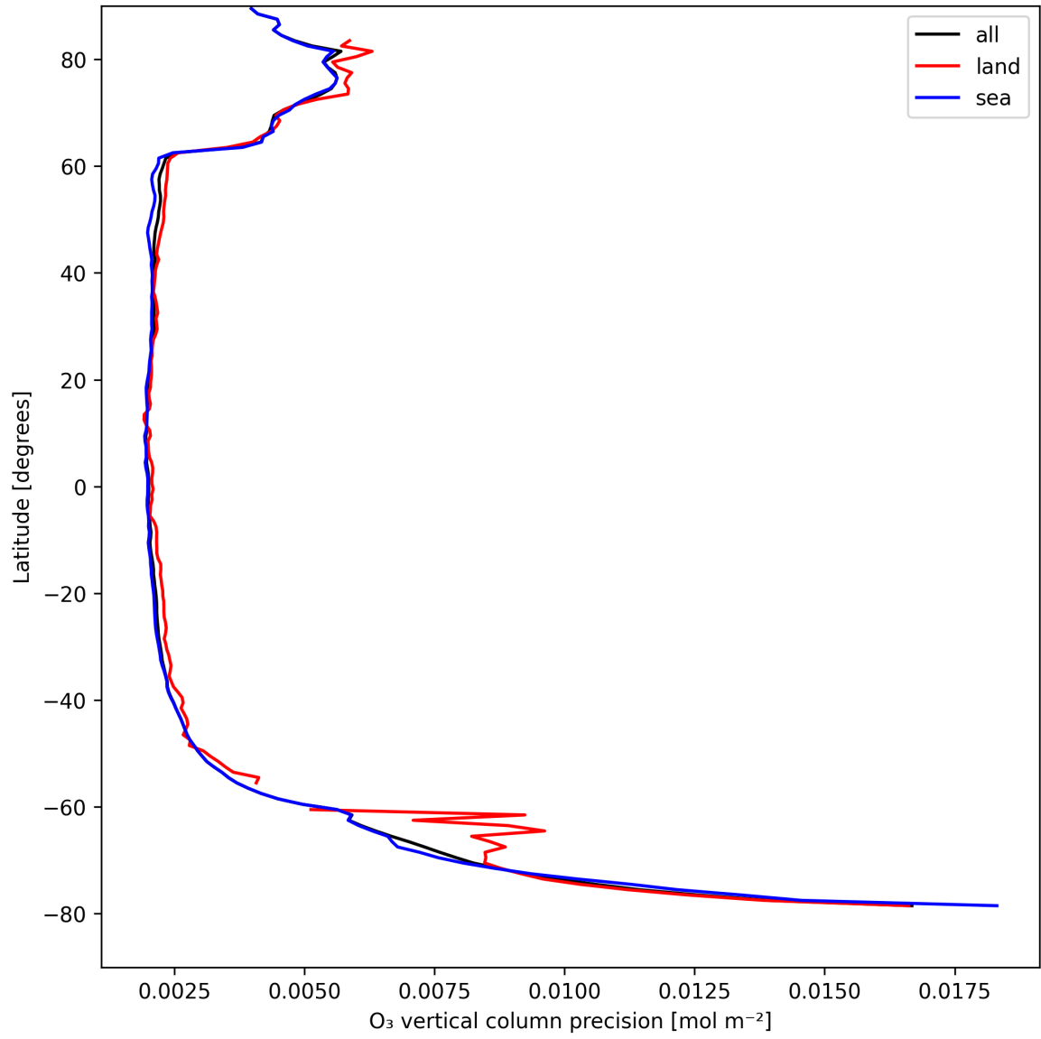
Figure 18: Zonal average of “O 3 vertical column precision” for 2025-08-26 to 2025-08-27.
