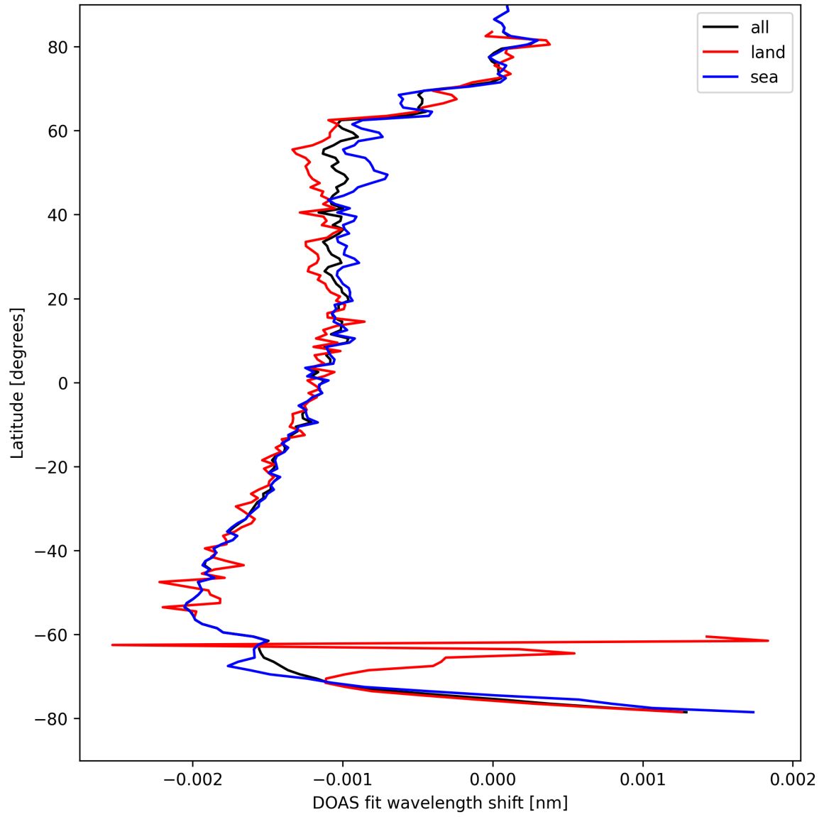
Figure 23: Zonal average of “DOAS fit wavelength shift” for 2025-08-26 to 2025-08-27.
