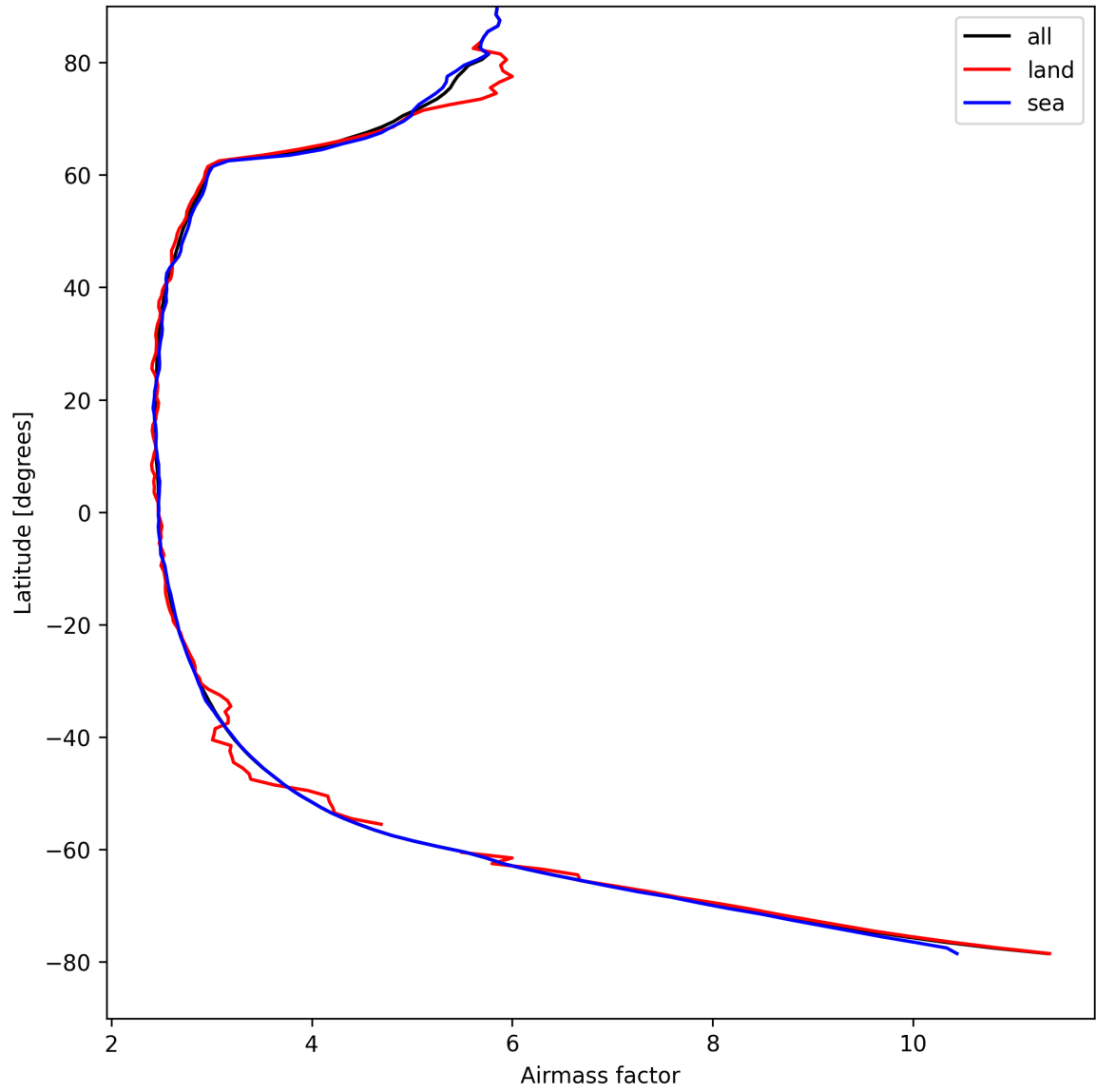
Figure 25: Zonal average of “Airmass factor” for 2025-08-26 to 2025-08-27.
