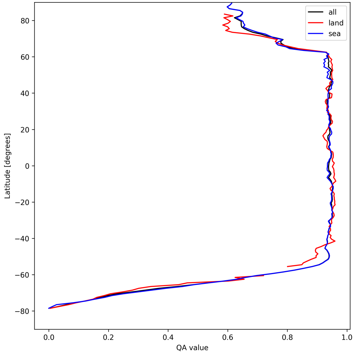
Figure 16: Zonal average of “QA value” for 2025-08-26 to 2025-08-27.
