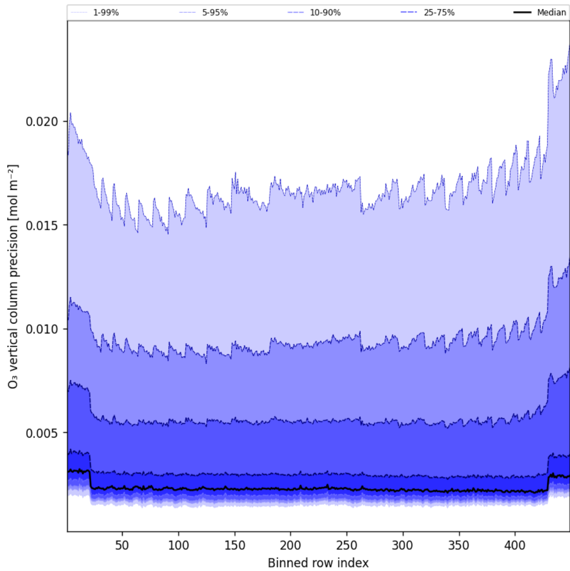
Figure 42: Along track statistics of “O 3 vertical column precision” for 2025-08-26 to 2025-08-27
