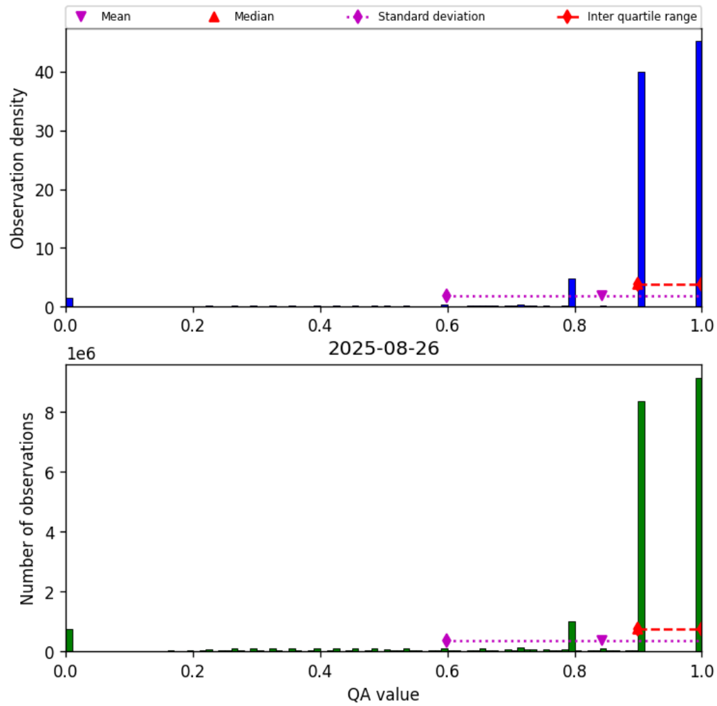
Figure 28: Histogram of “QA value” for 2025-08-26 to 2025-08-27
