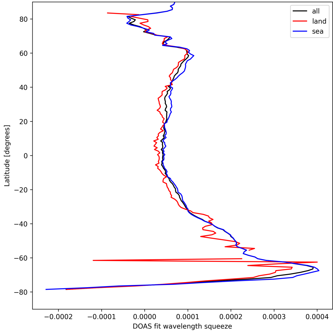
Figure 24: Zonal average of “DOAS fit wavelength squeeze” for 2025-08-26 to 2025-08-27.
