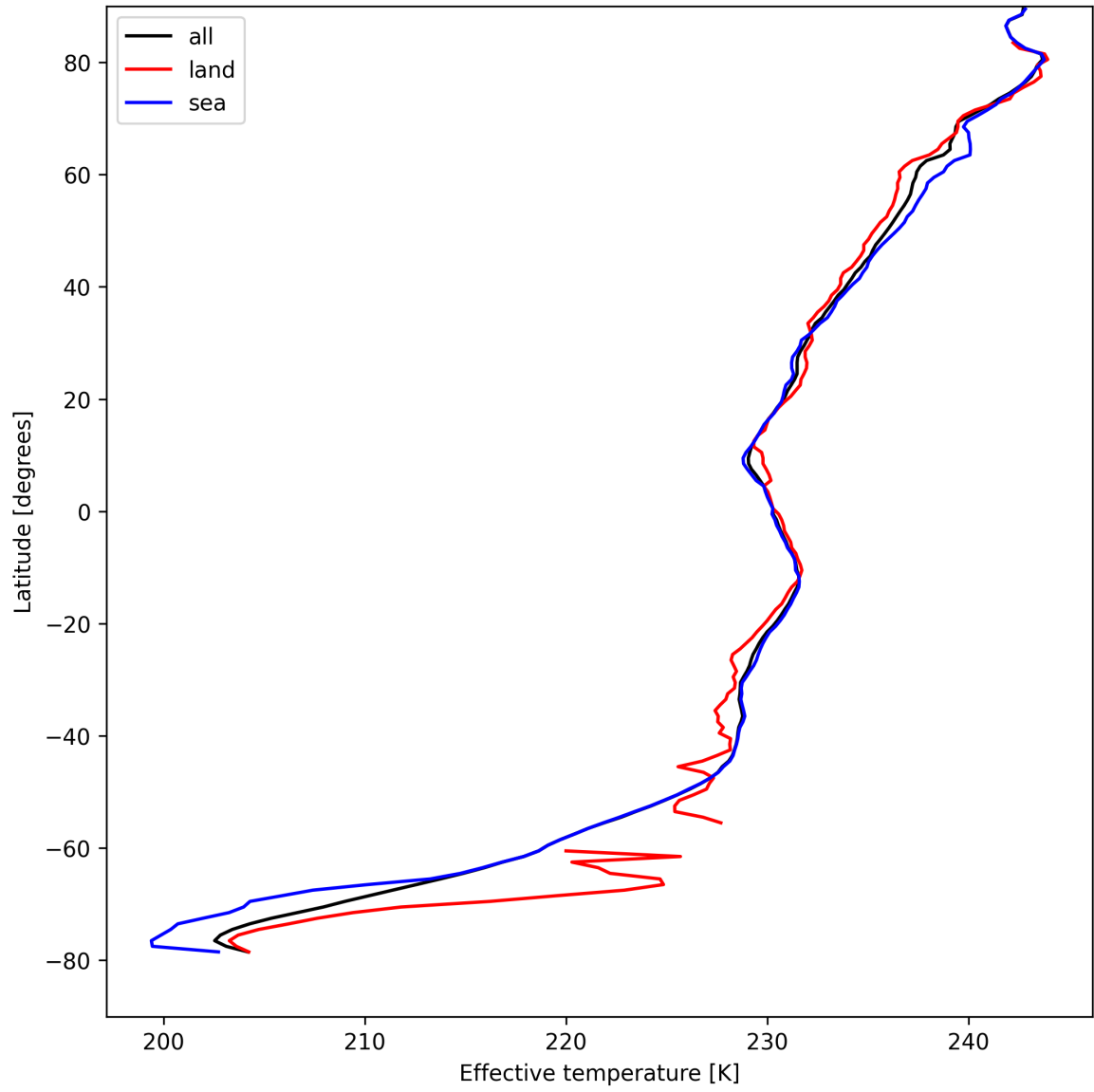
Figure 26: Zonal average of "Effective temperature" for 2025-08-26 to 2025-08-27.
