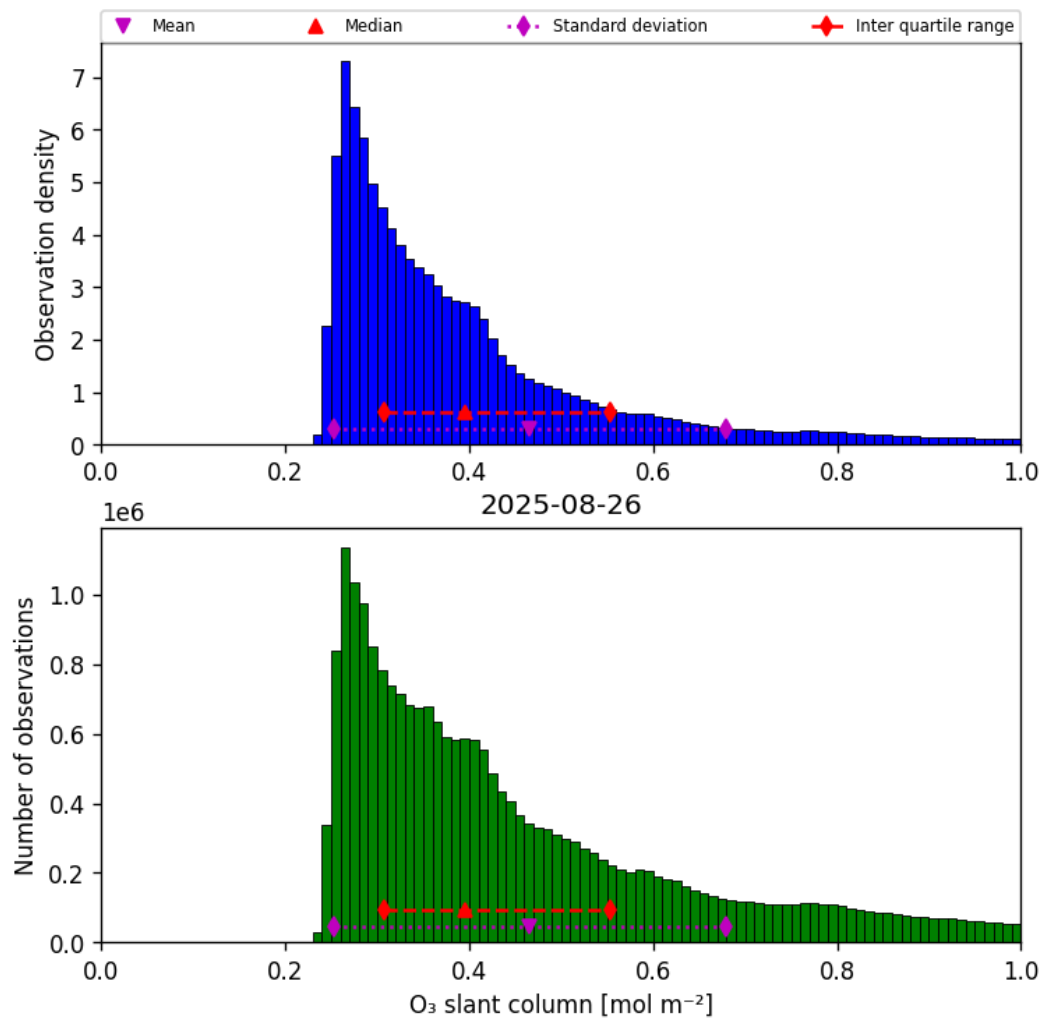
Figure 31: Histogram of “O 3 slant column” for 2025-08-26 to 2025-08-27
