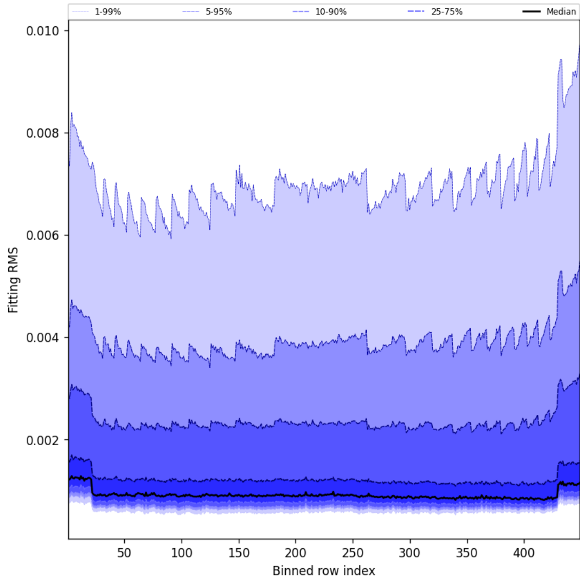
Figure 46: Along track statistics of “Fitting RMS” for 2025-08-26 to 2025-08-27
