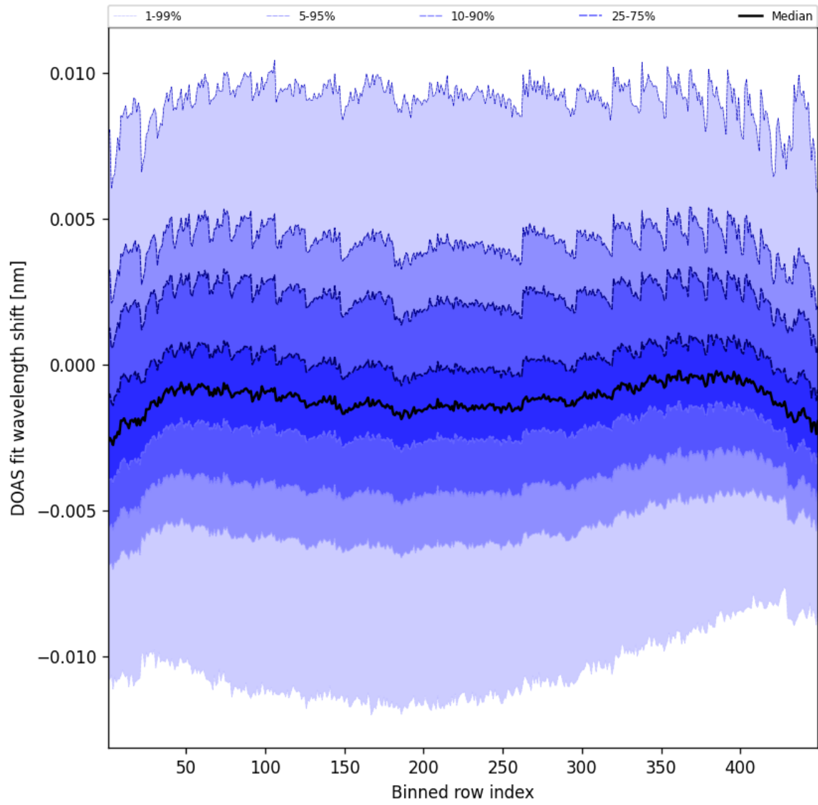
Figure 47: Along track statistics of “DOAS fit wavelength shift” for 2025-08-26 to 2025-08-27
