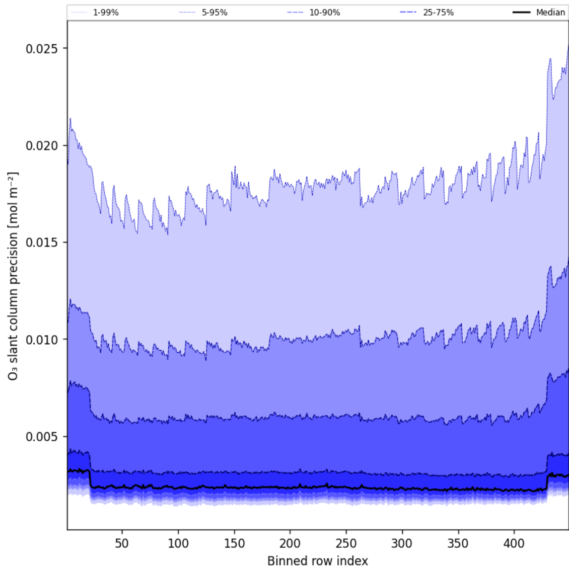
Figure 44: Along track statistics of “O 3 slant column precision” for 2025-08-26 to 2025-08-27
