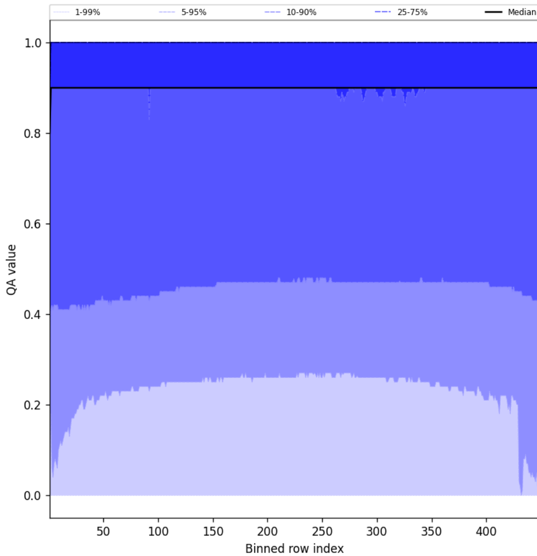
Figure 40: Along track statistics of “QA value” for 2025-08-26 to 2025-08-27
