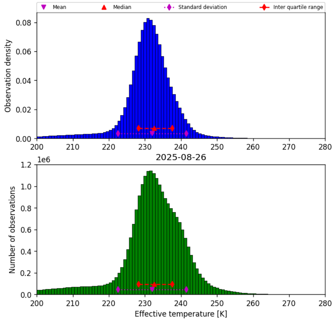
Figure 38: Histogram of “Effective temperature” for 2025-08-26 to 2025-08-27
