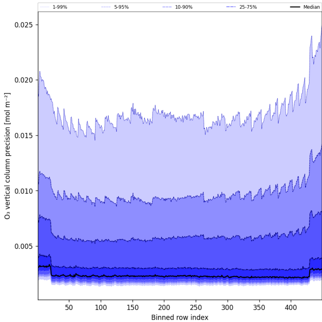
Figure 42: Along track statistics of “O 3 vertical column precision” for 2025-08-27 to 2025-08-28
