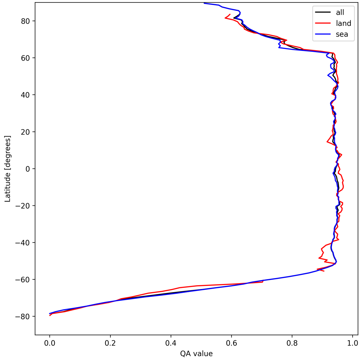
Figure 16: Zonal average of “QA value” for 2025-08-27 to 2025-08-28.
