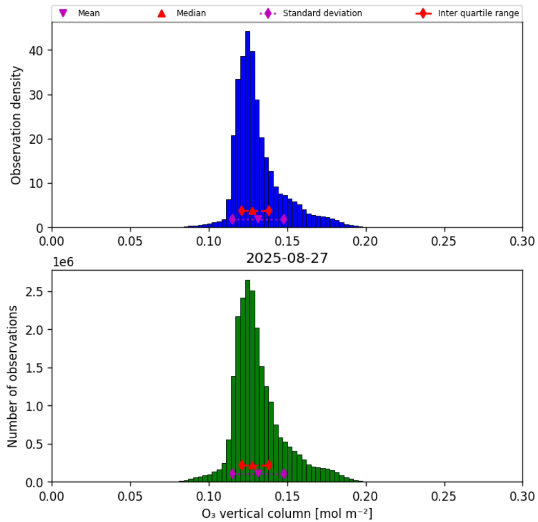
Figure 29: Histogram of “O 3 vertical column” for 2025-08-27 to 2025-08-28
