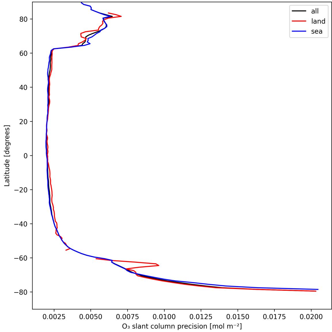
Figure 20: Zonal average of "O 3 slant column precision" for 2025-08-27 to 2025-08-28.
