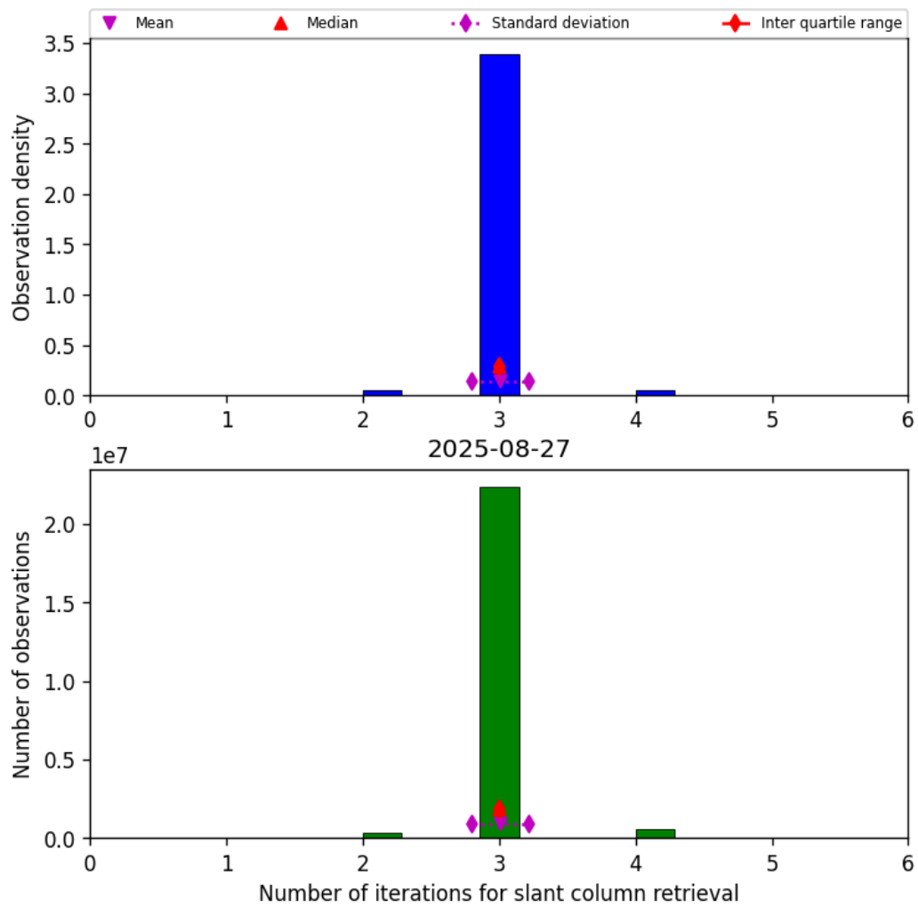
Figure 33: Histogram of “Number of iterations for slant column retrieval” for 2025-08-27 to 2025-08-28
