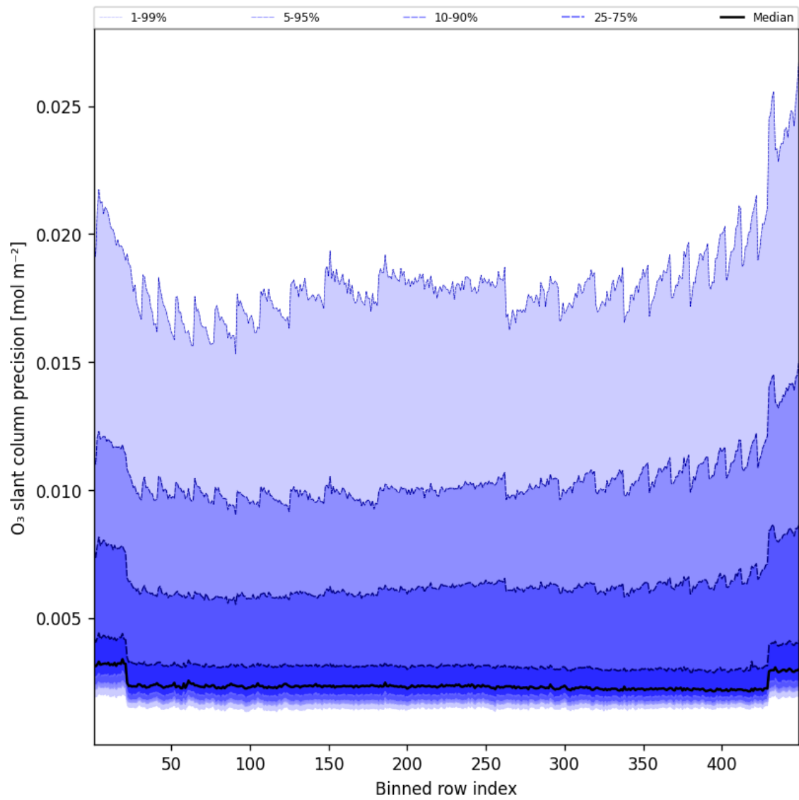
Figure 44: Along track statistics of “O 3 slant column precision” for 2025-08-27 to 2025-08-28
