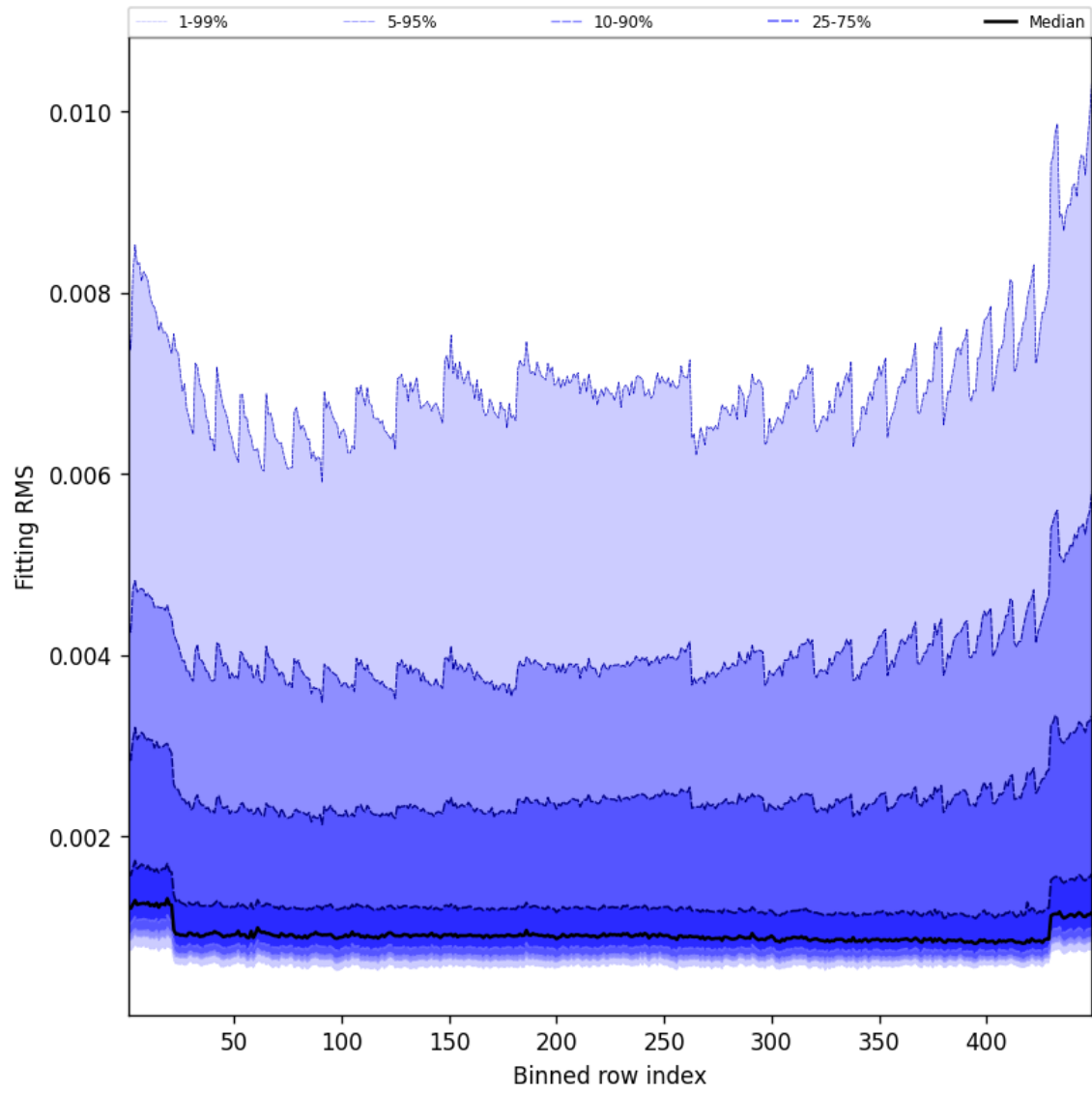
Figure 46: Along track statistics of “Fitting RMS” for 2025-08-27 to 2025-08-28
