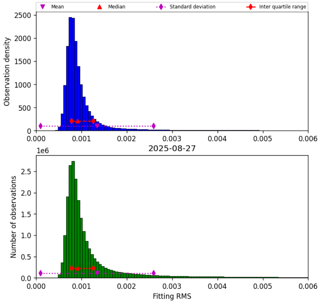
Figure 34: Histogram of "Fitting RMS" for 2025-08-27 to 2025-08-28
