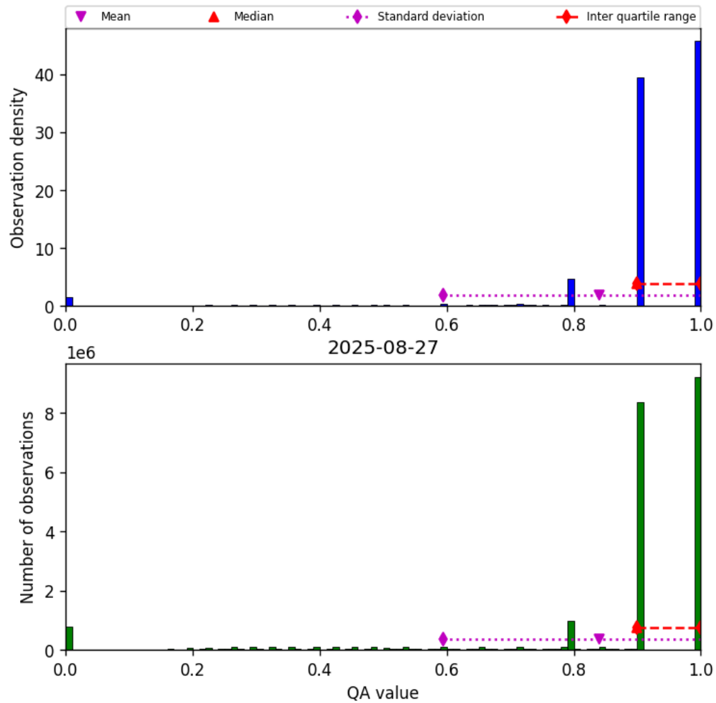
Figure 28: Histogram of “QA value” for 2025-08-27 to 2025-08-28
