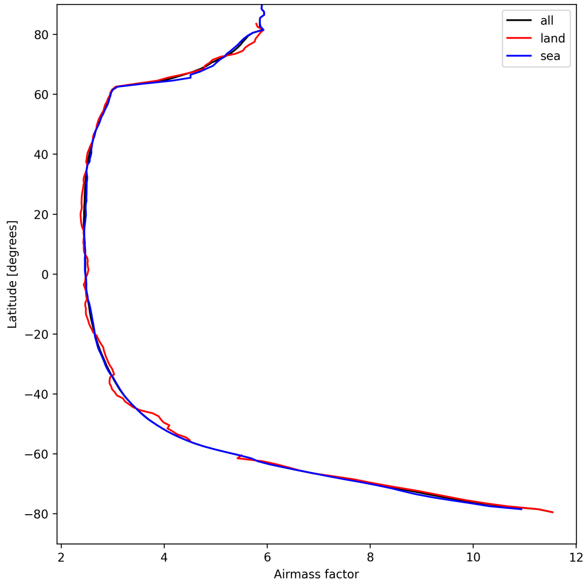
Figure 25: Zonal average of “Airmass factor” for 2025-08-27 to 2025-08-28.
