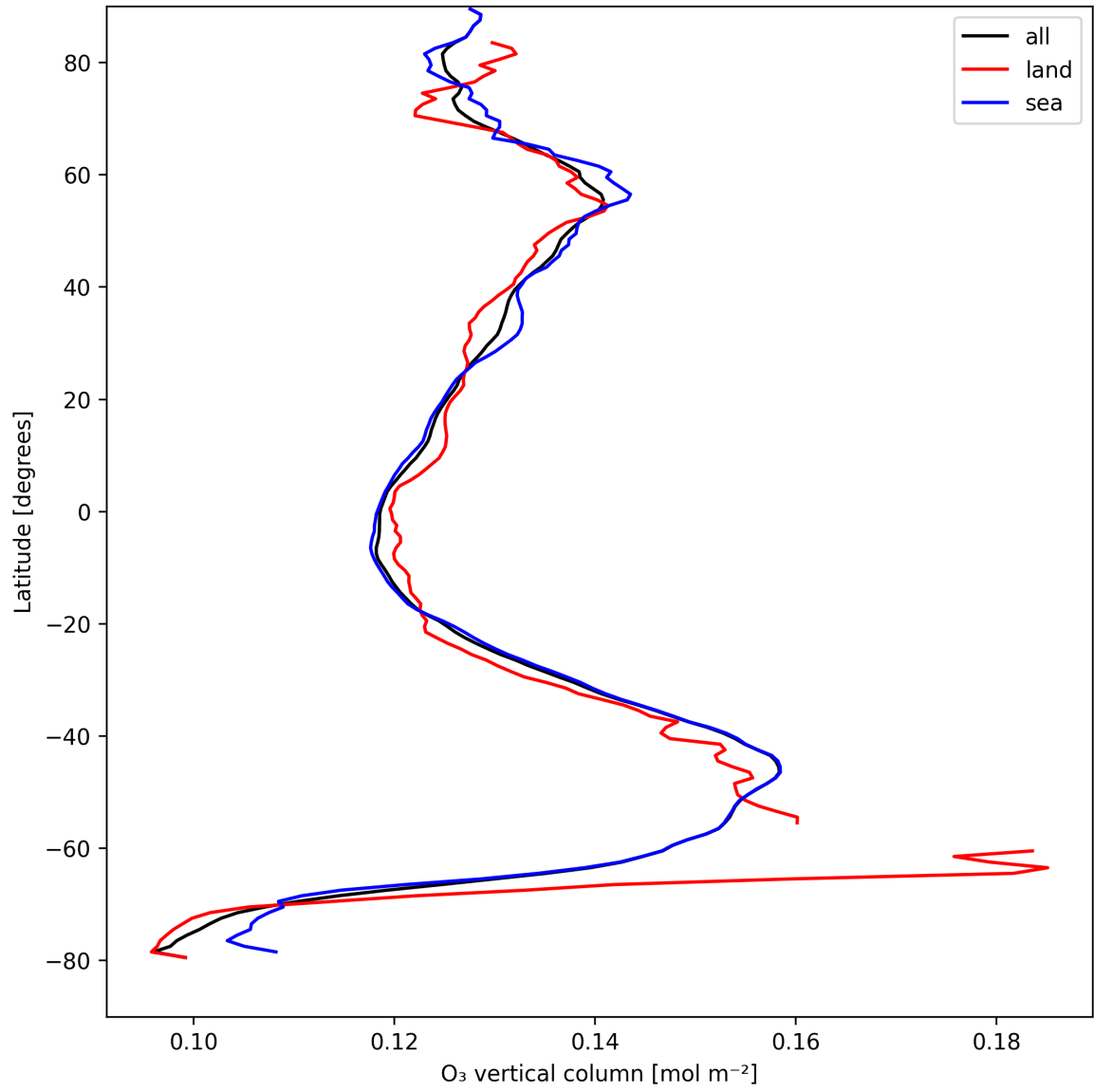
Figure 17: Zonal average of “O 3 vertical column” for 2025-08-27 to 2025-08-28.
