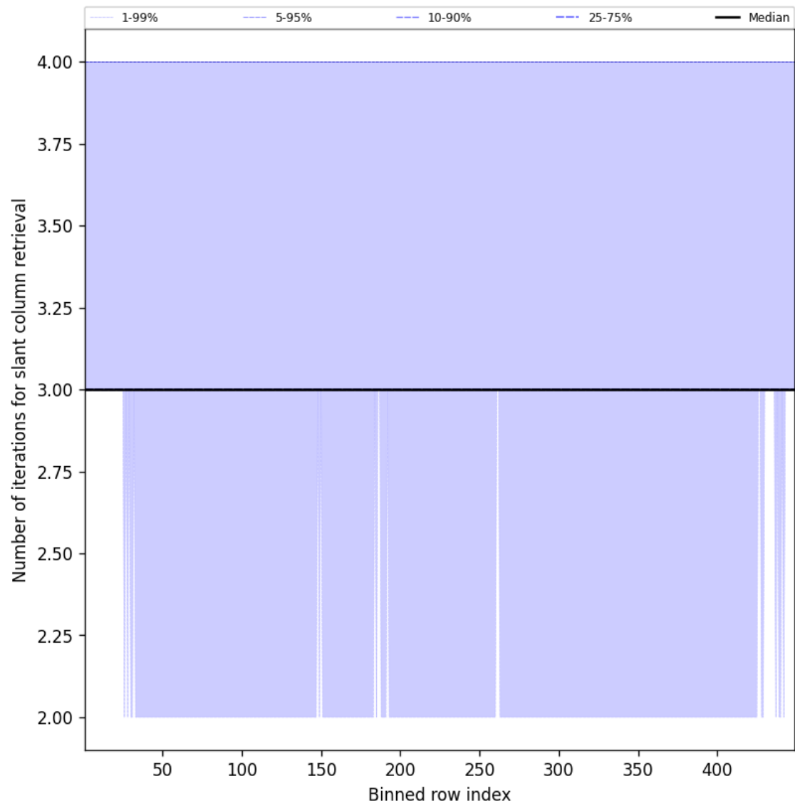
Figure 45: Along track statistics of “Number of iterations for slant column retrieval” for 2025-08-27 to 2025-08-28
