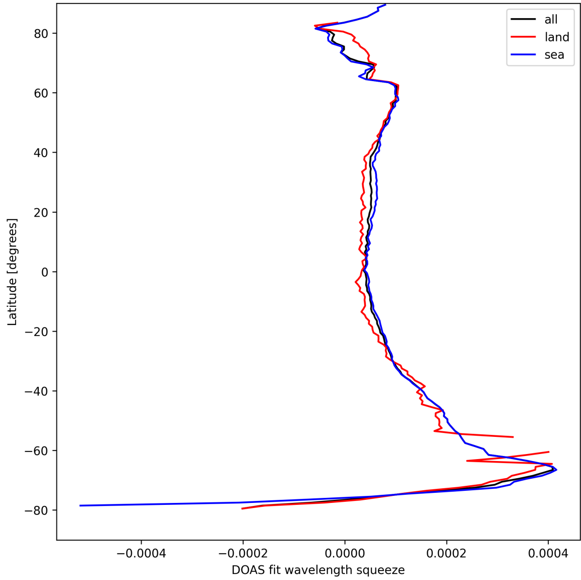
Figure 24: Zonal average of "DOAS fit wavelength squeeze" for 2025-08-27 to 2025-08-28.
