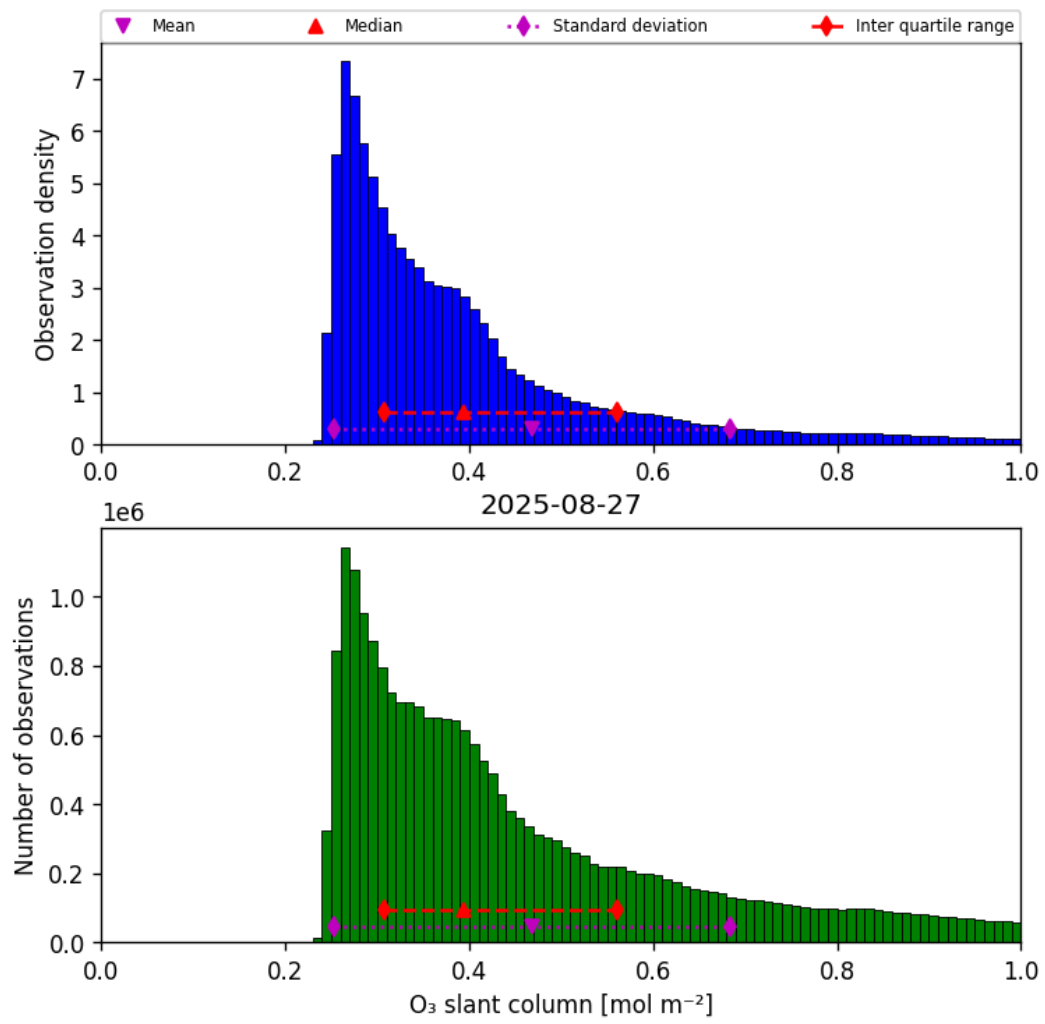
Figure 31: Histogram of “O 3 slant column” for 2025-08-27 to 2025-08-28
