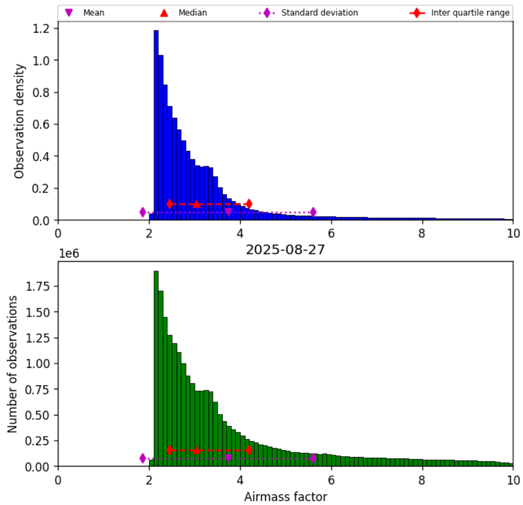
Figure 37: Histogram of “Airmass factor” for 2025-08-27 to 2025-08-28
