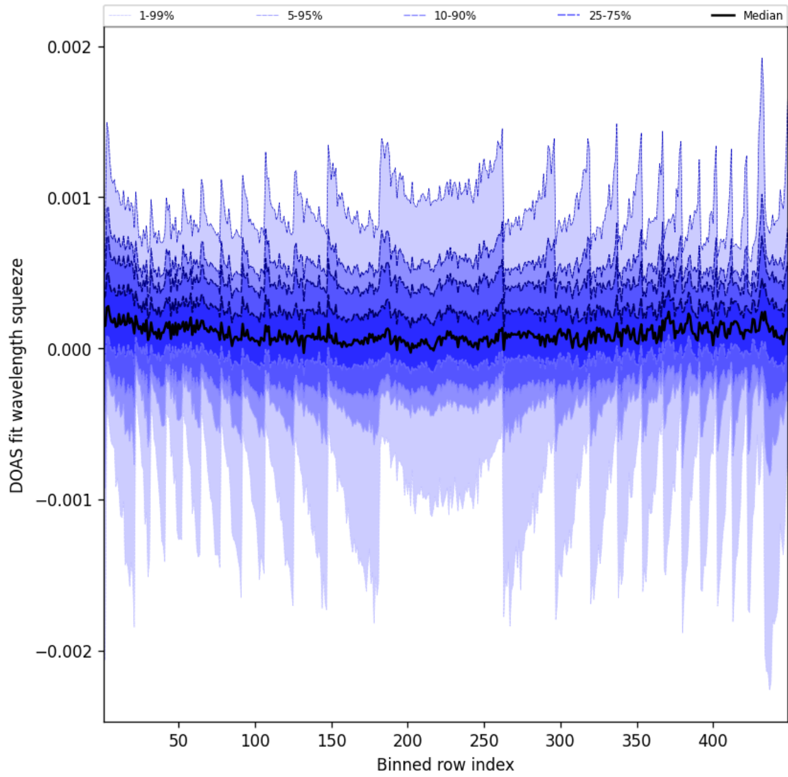
Figure 48: Along track statistics of “DOAS fit wavelength squeeze” for 2025-08-27 to 2025-08-28
