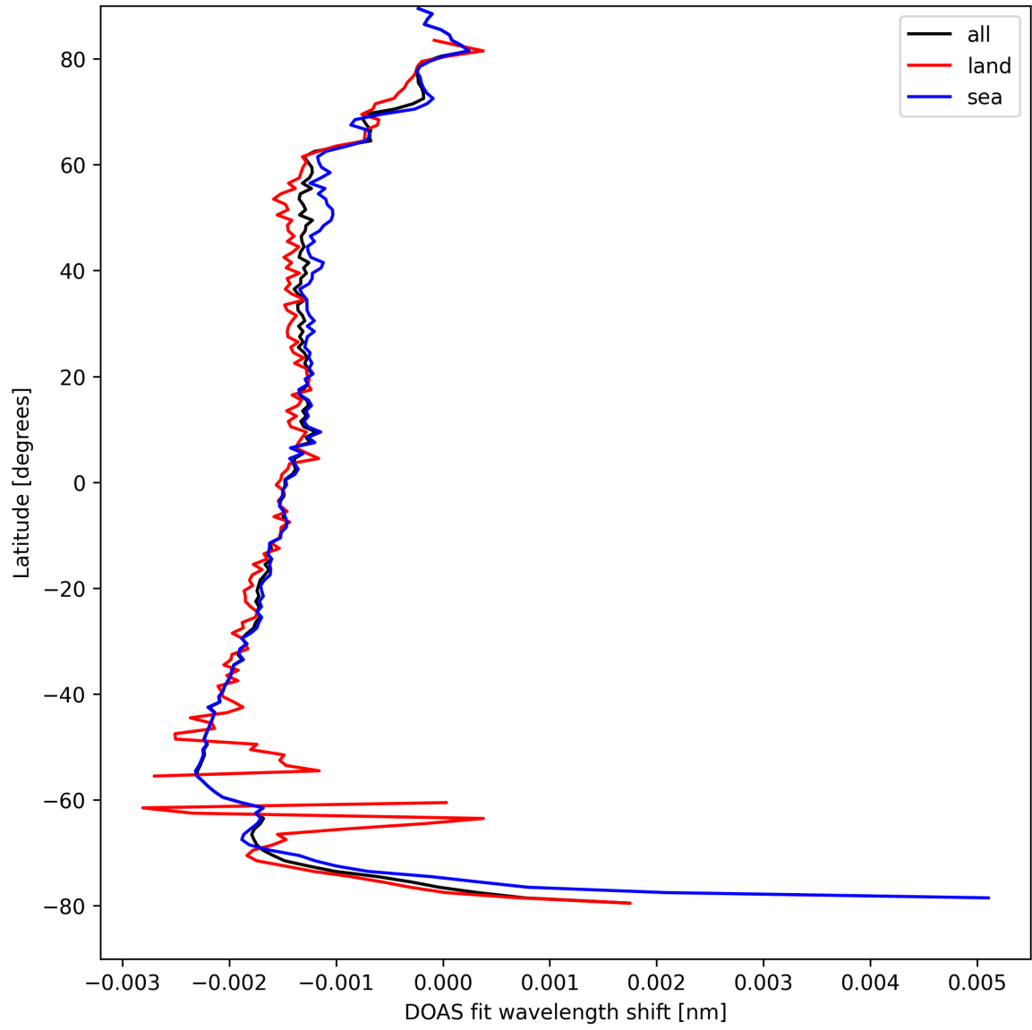
Figure 23: Zonal average of “DOAS fit wavelength shift” for 2025-08-27 to 2025-08-28.
