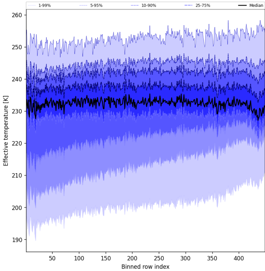
Figure 50: Along track statistics of “Effective temperature” for 2025-08-27 to 2025-08-28
