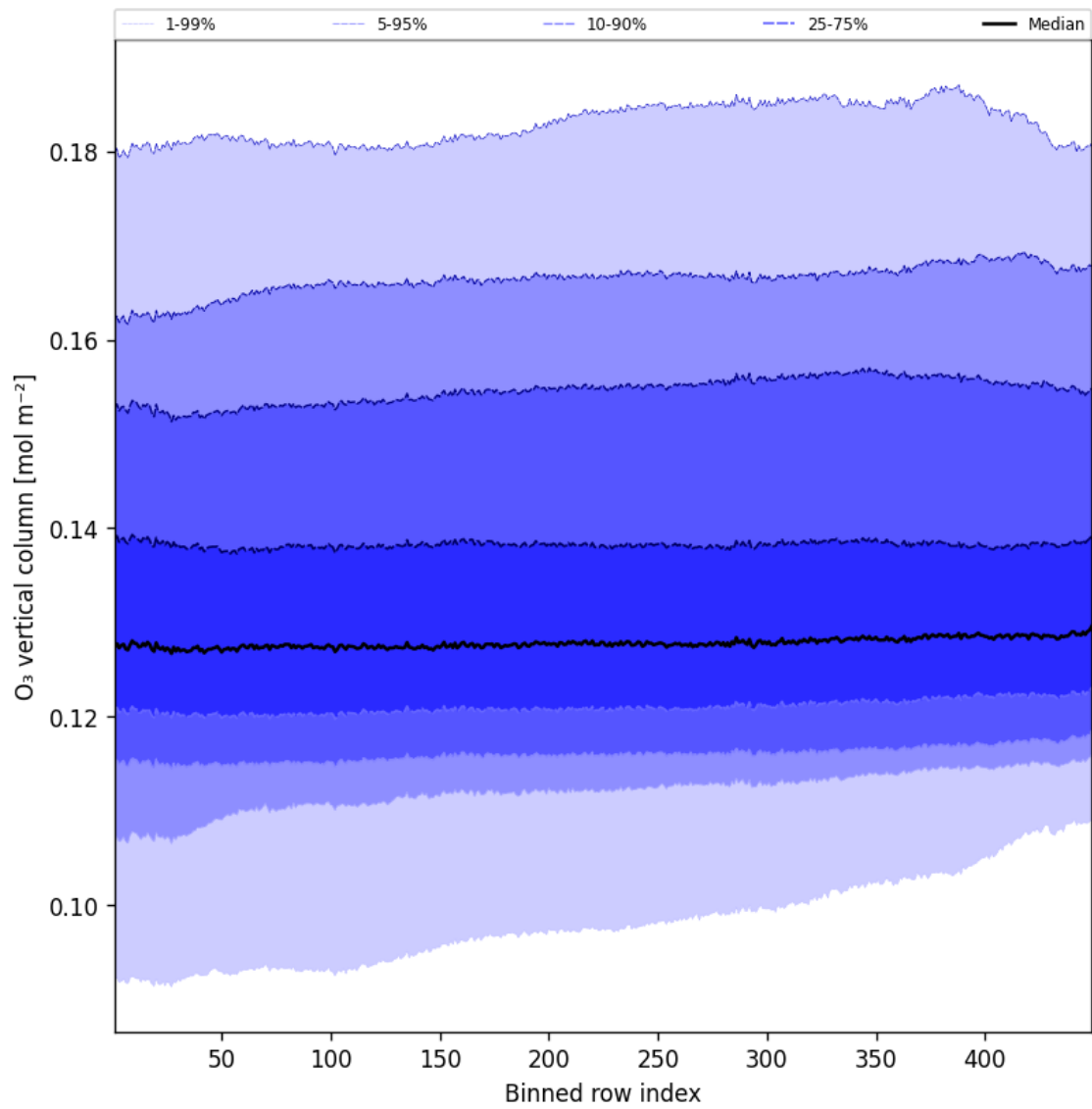
Figure 41: Along track statistics of “O 3 vertical column” for 2025-08-27 to 2025-08-28
