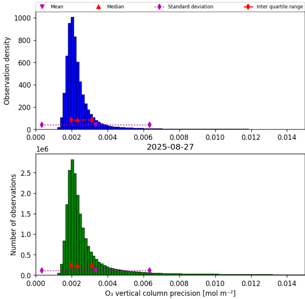
Figure 30: Histogram of “O 3 vertical column precision” for 2025-08-27 to 2025-08-28
