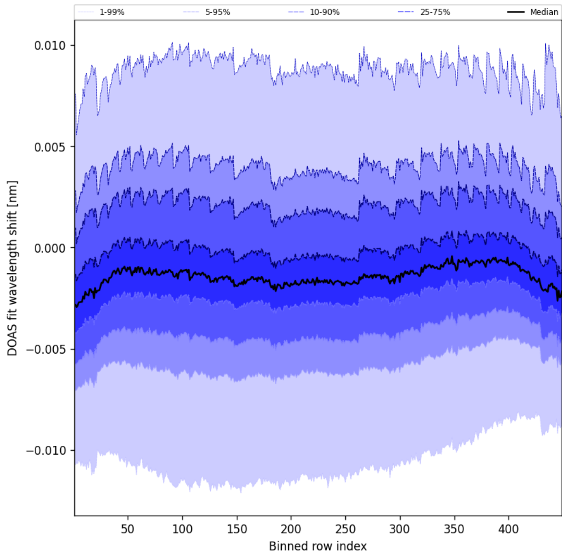
Figure 47: Along track statistics of “DOAS fit wavelength shift” for 2025-08-27 to 2025-08-28
