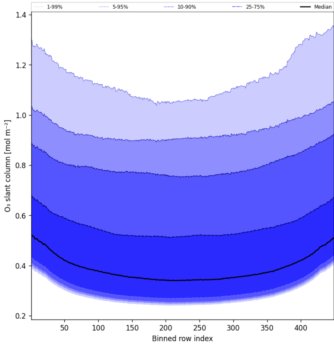
Figure 43: Along track statistics of “O 3 slant column” for 2025-08-27 to 2025-08-28
