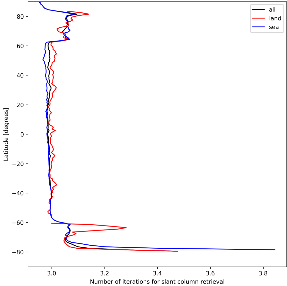
Figure 21: Zonal average of “Number of iterations for slant column retrieval” for 2025-08-27 to 2025-08-28.
