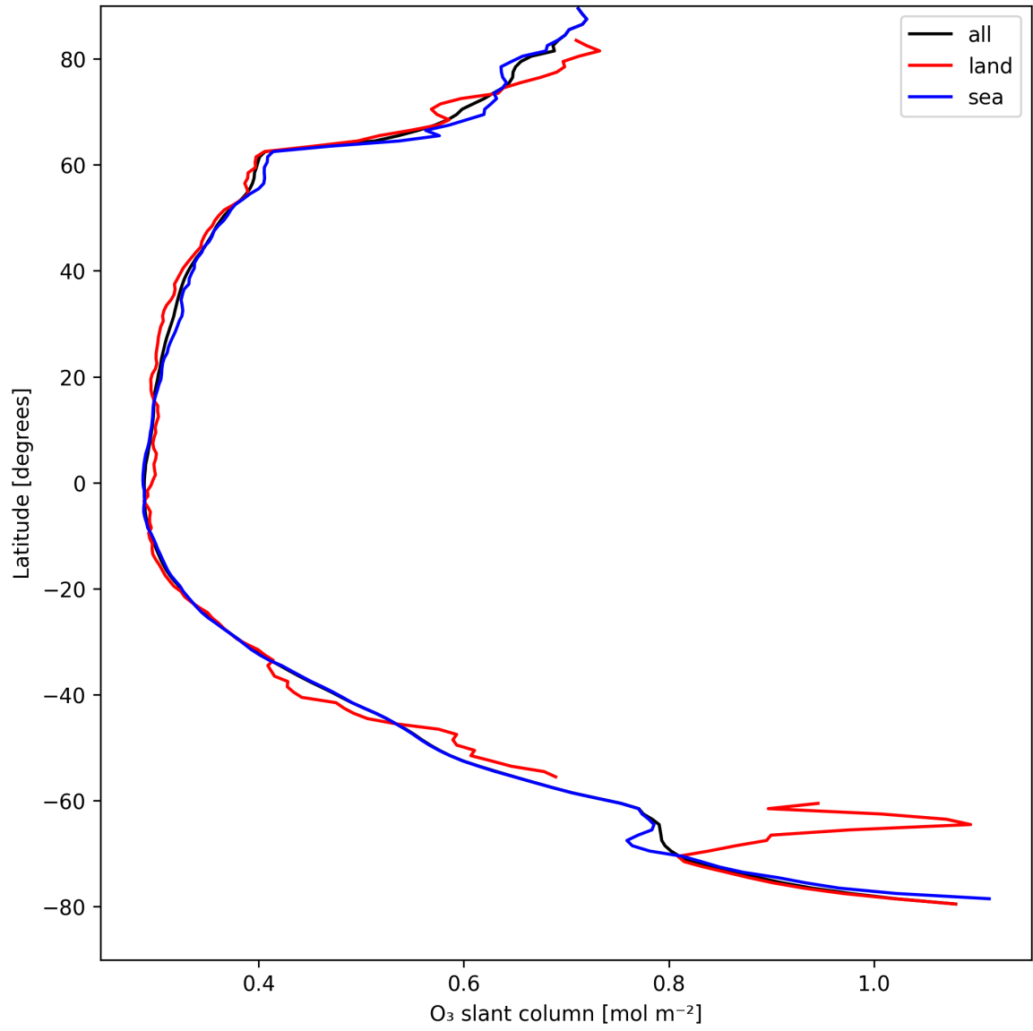
Figure 19: Zonal average of “O 3 slant column” for 2025-08-27 to 2025-08-28.
