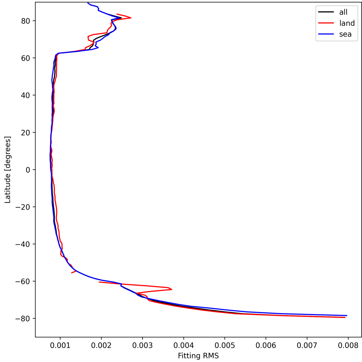
Figure 22: Zonal average of “Fitting RMS” for 2025-08-27 to 2025-08-28.
