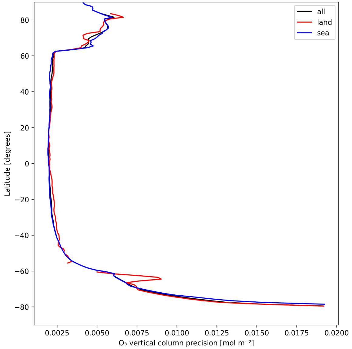
Figure 18: Zonal average of "O 3 vertical column precision" for 2025-08-27 to 2025-08-28.
