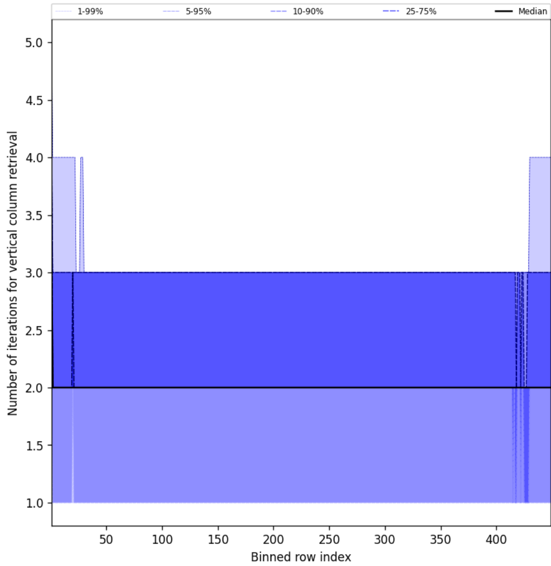
Figure 51: Along track statistics of “Number of iterations for vertical column retrieval” for 2025-08-27 to 2025-08-28
