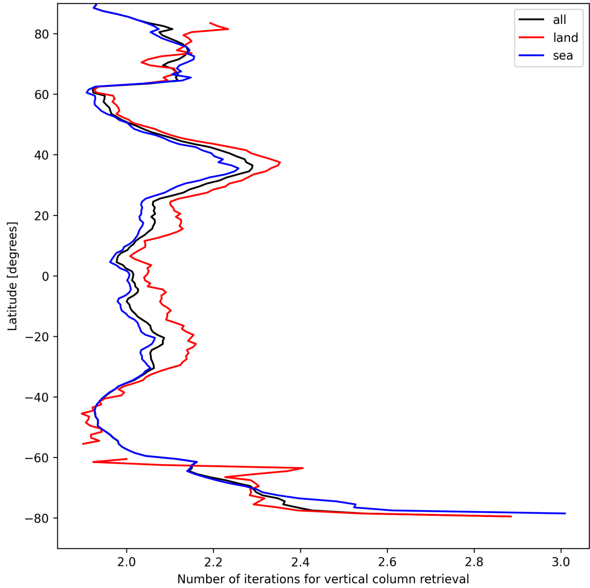
Figure 27: Zonal average of “Number of iterations for vertical column retrieval” for 2025-08-27 to 2025-08-28.
