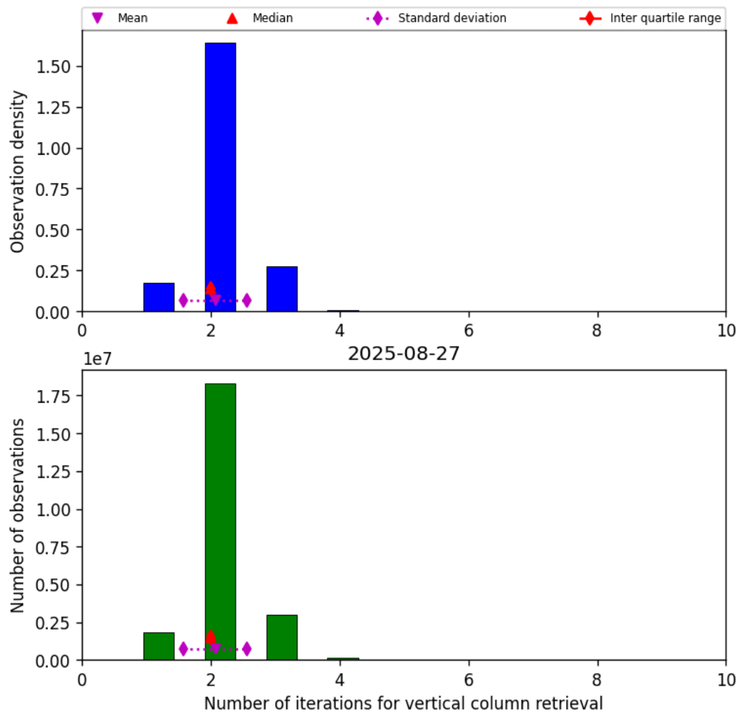
Figure 39: Histogram of “Number of iterations for vertical column retrieval” for 2025-08-27 to 2025-08-28
