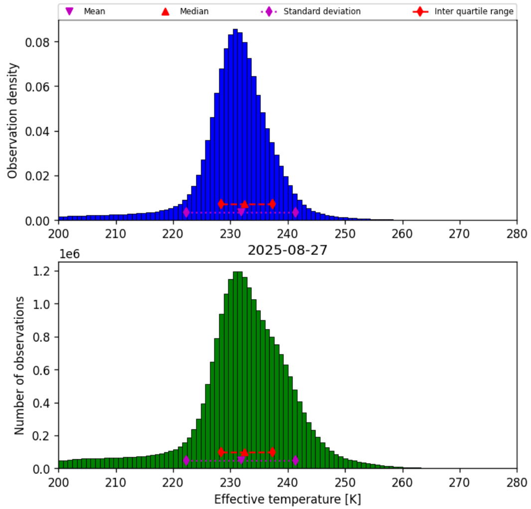
Figure 38: Histogram of “Effective temperature” for 2025-08-27 to 2025-08-28
