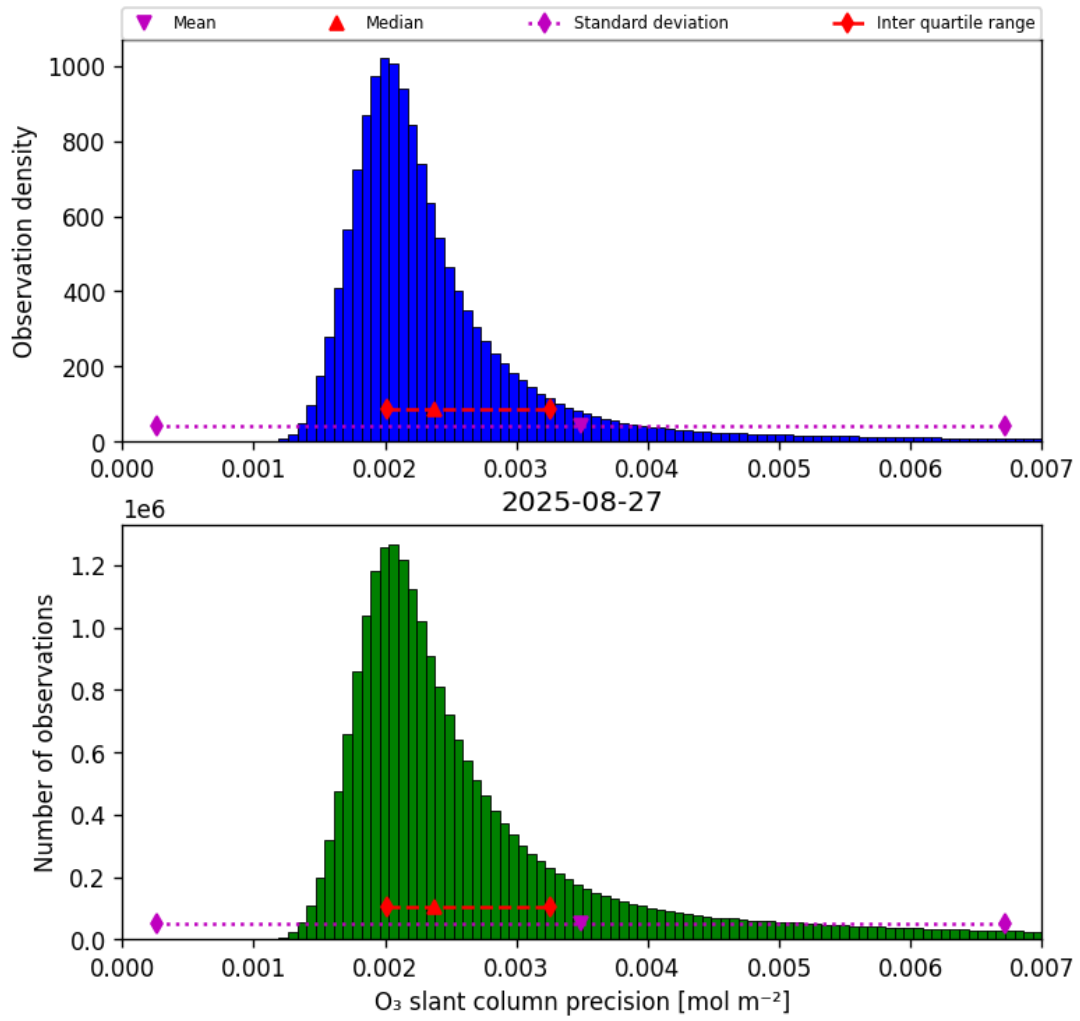
Figure 32: Histogram of “O 3 slant column precision” for 2025-08-27 to 2025-08-28
