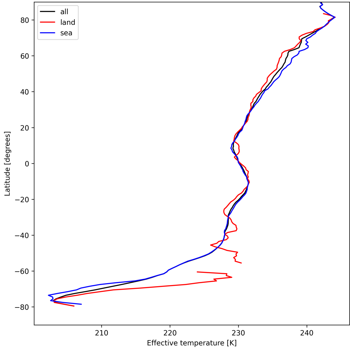
Figure 26: Zonal average of "Effective temperature" for 2025-08-27 to 2025-08-28.
