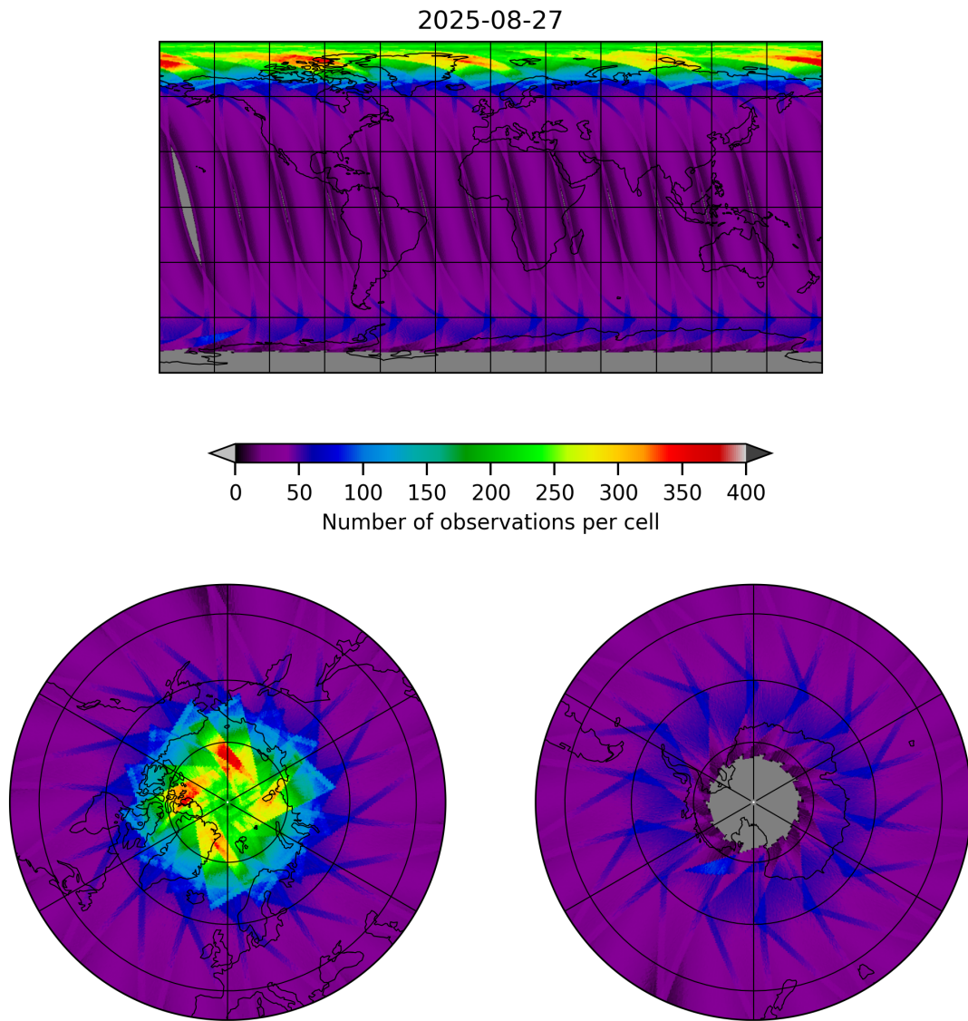
Figure 15: Map of the number of observations for 2025-08-27 to 2025-08-28
