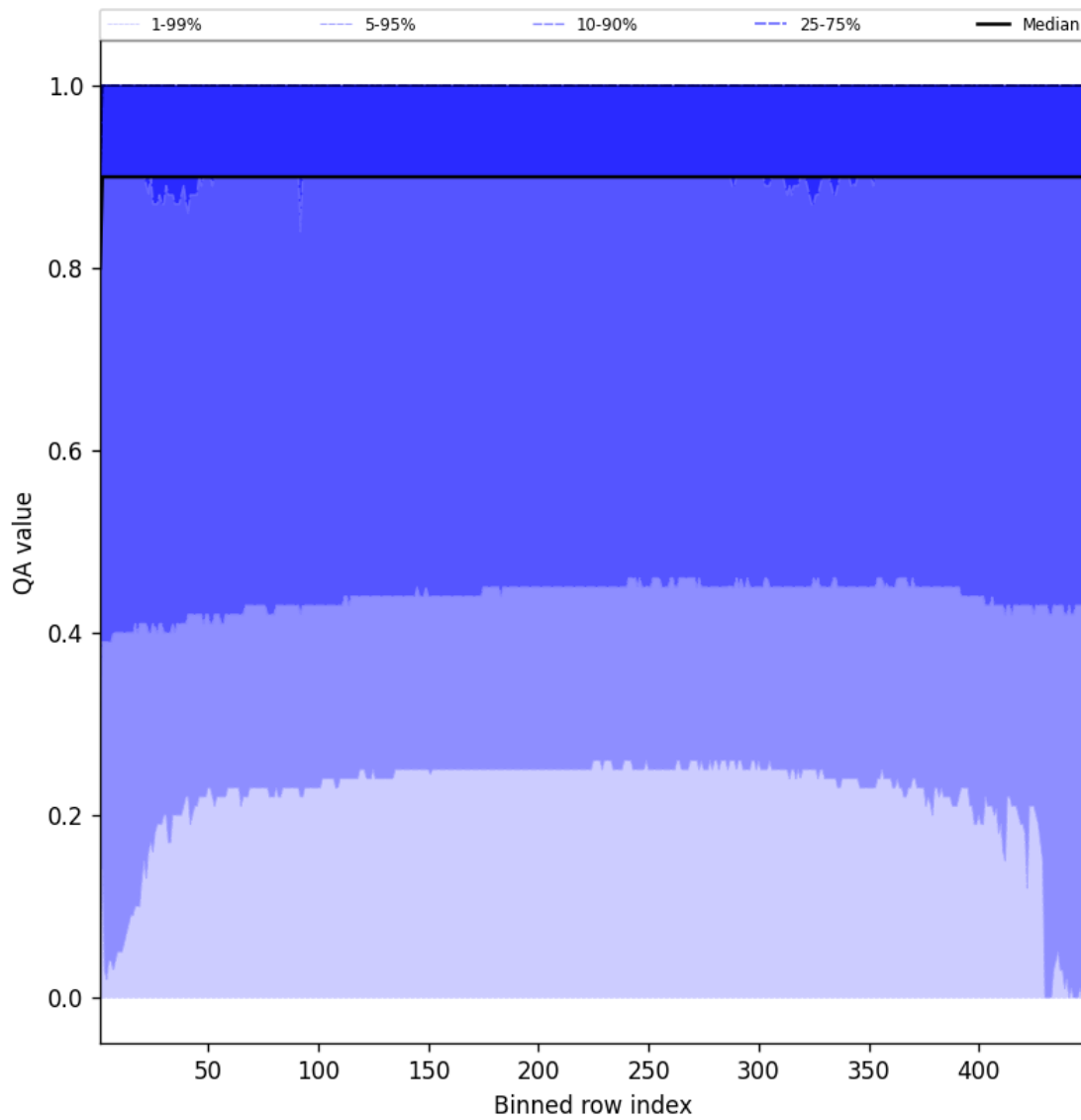
Figure 40: Along track statistics of “QA value” for 2025-08-27 to 2025-08-28
