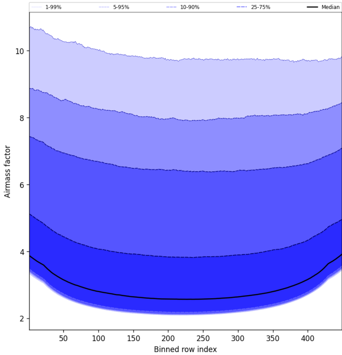
Figure 49: Along track statistics of “Airmass factor” for 2025-08-27 to 2025-08-28
