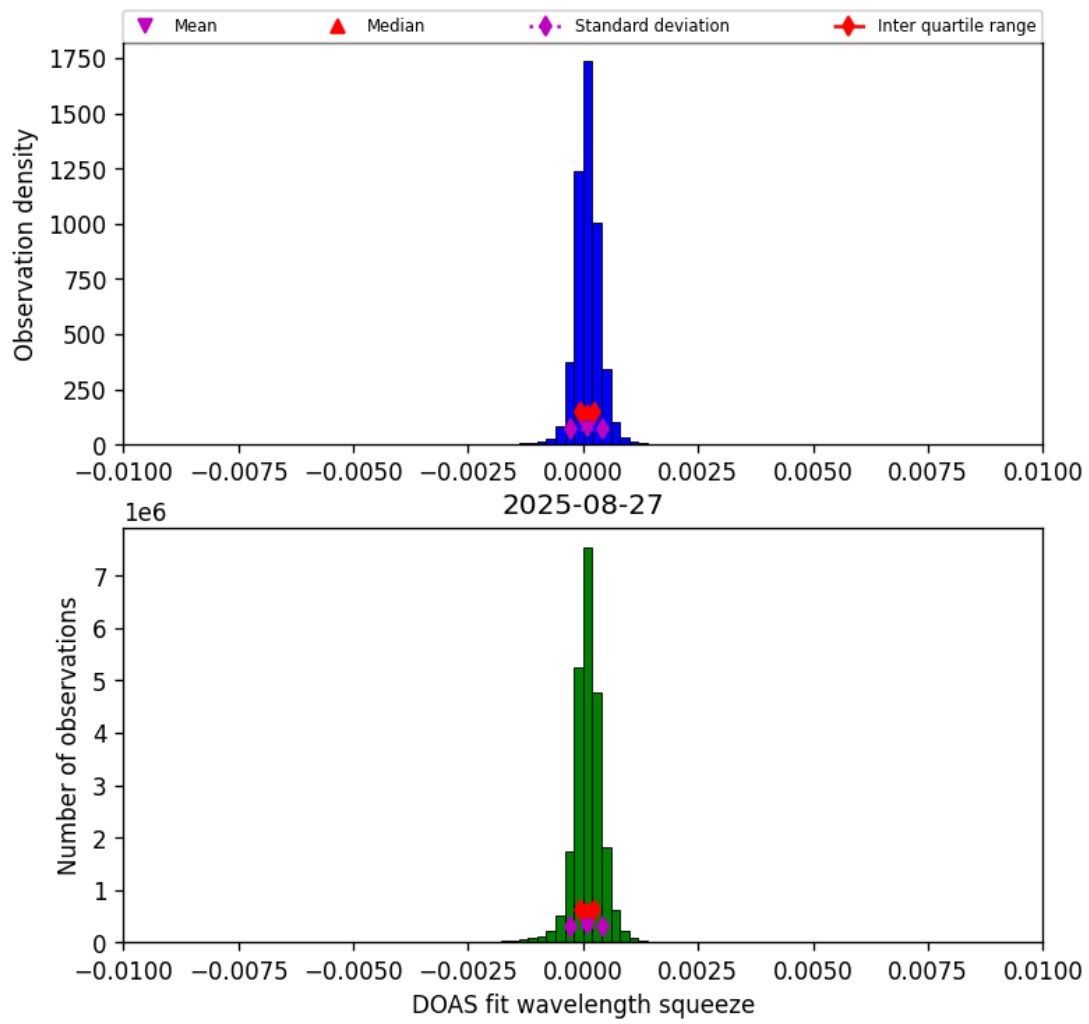
Figure 36: Histogram of “DOAS fit wavelength squeeze” for 2025-08-27 to 2025-08-28
