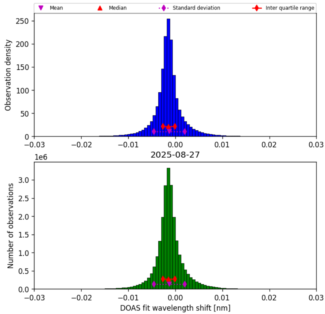
Figure 35: Histogram of “DOAS fit wavelength shift” for 2025-08-27 to 2025-08-28
