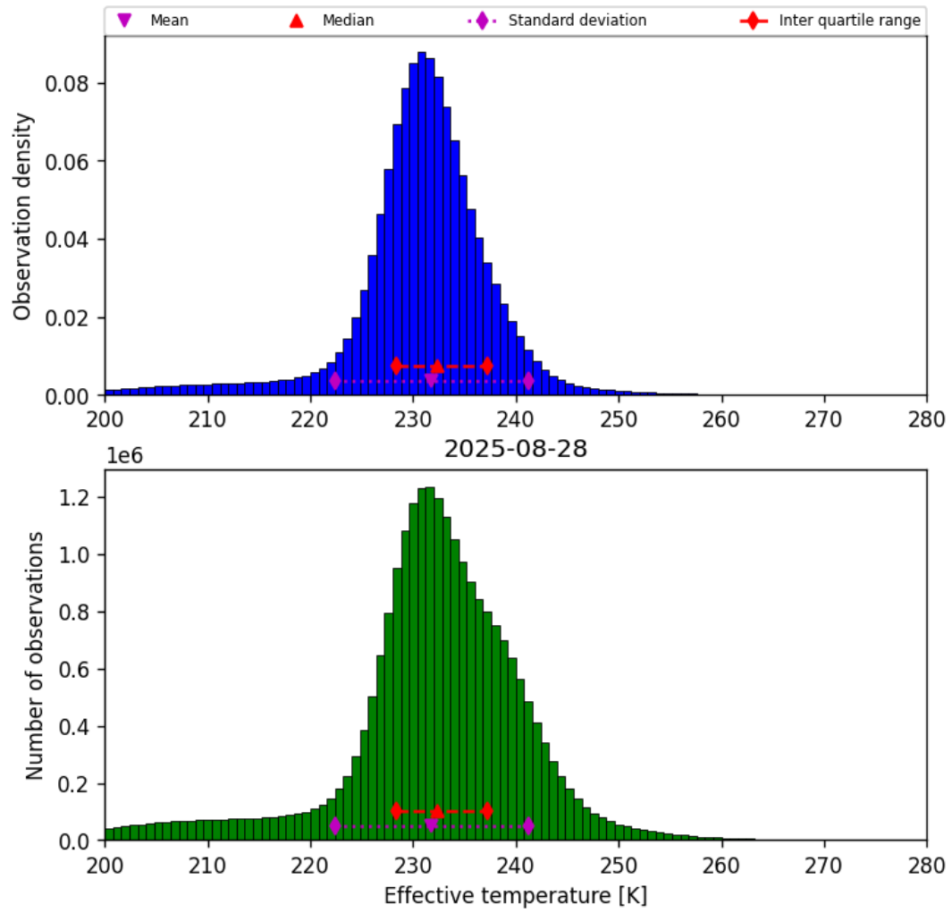
Figure 38: Histogram of “Effective temperature” for 2025-08-28 to 2025-08-28
