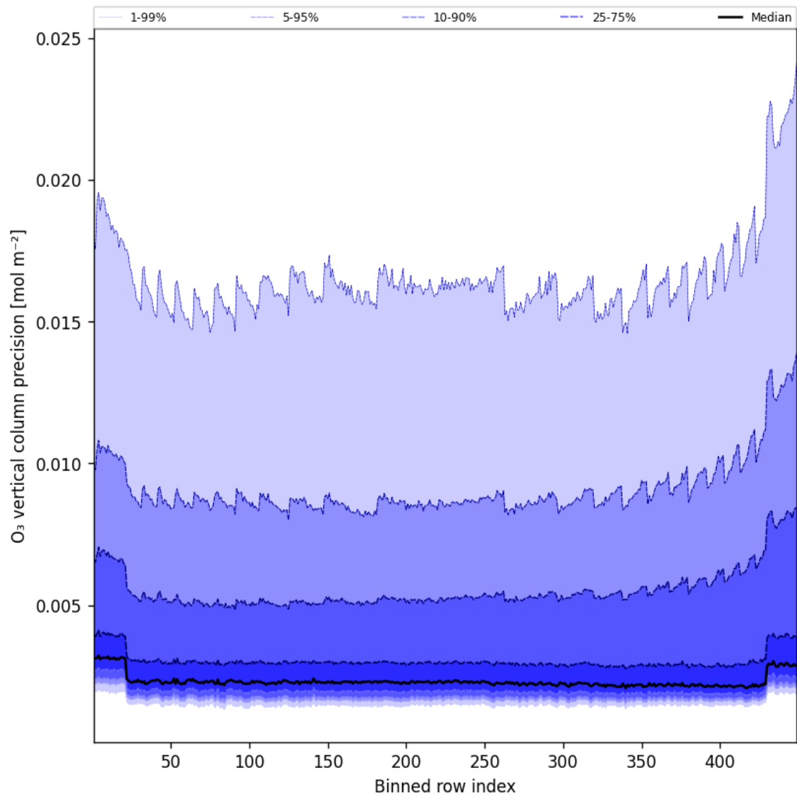
Figure 42: Along track statistics of “O 3 vertical column precision” for 2025-08-28 to 2025-08-28
