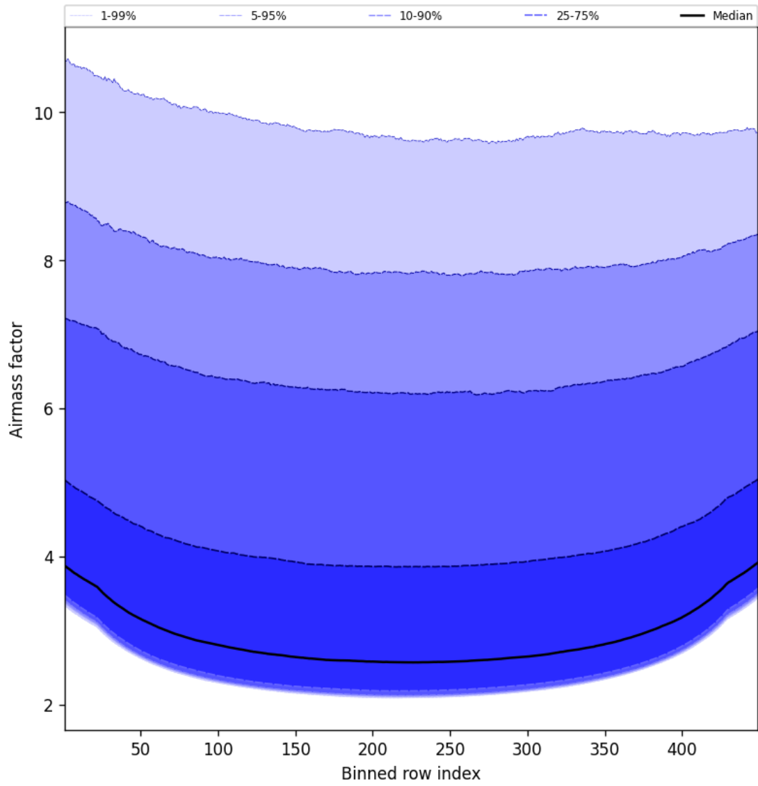
Figure 49: Along track statistics of “Airmass factor” for 2025-08-28 to 2025-08-28
