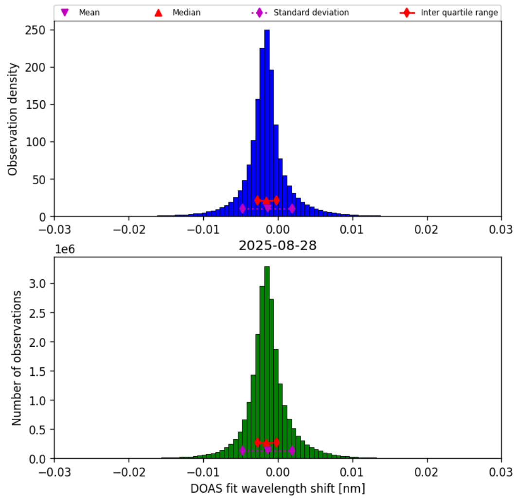
Figure 35: Histogram of “DOAS fit wavelength shift” for 2025-08-28 to 2025-08-28
