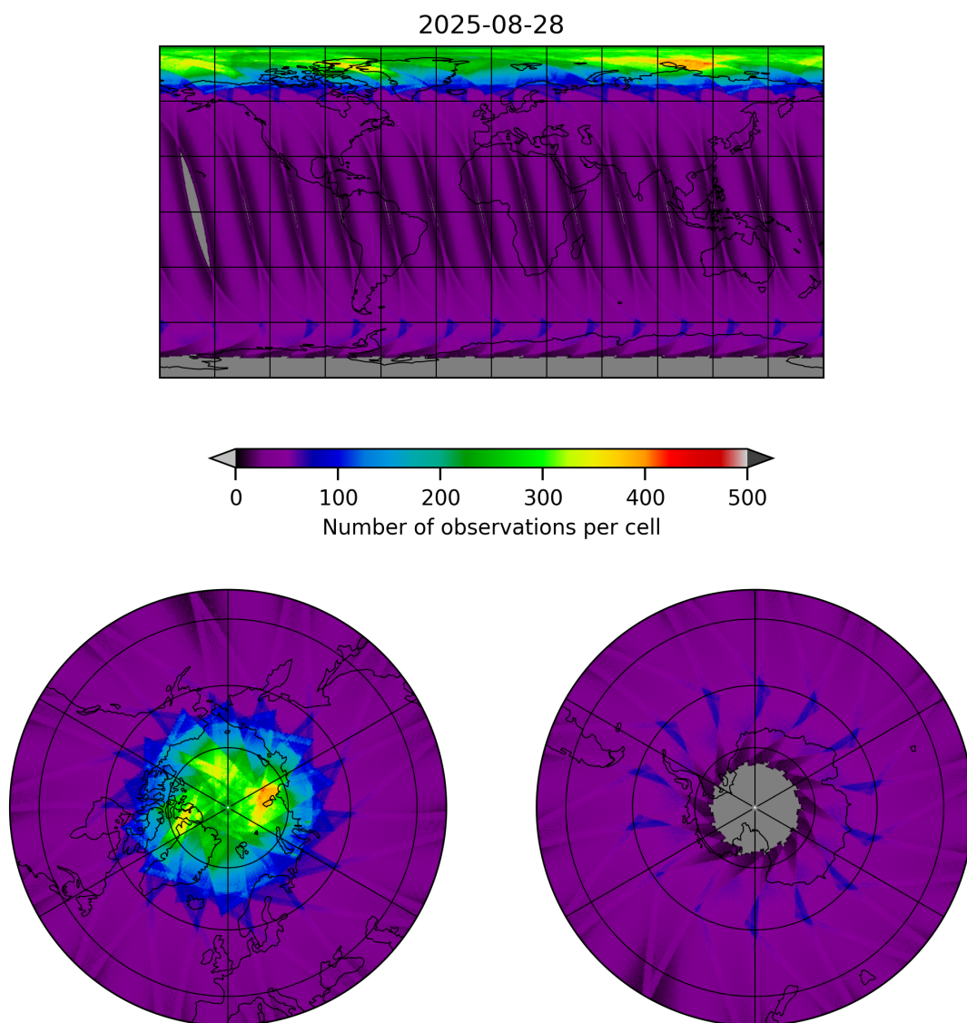
Figure 15: Map of the number of observations for 2025-08-28 to 2025-08-28
