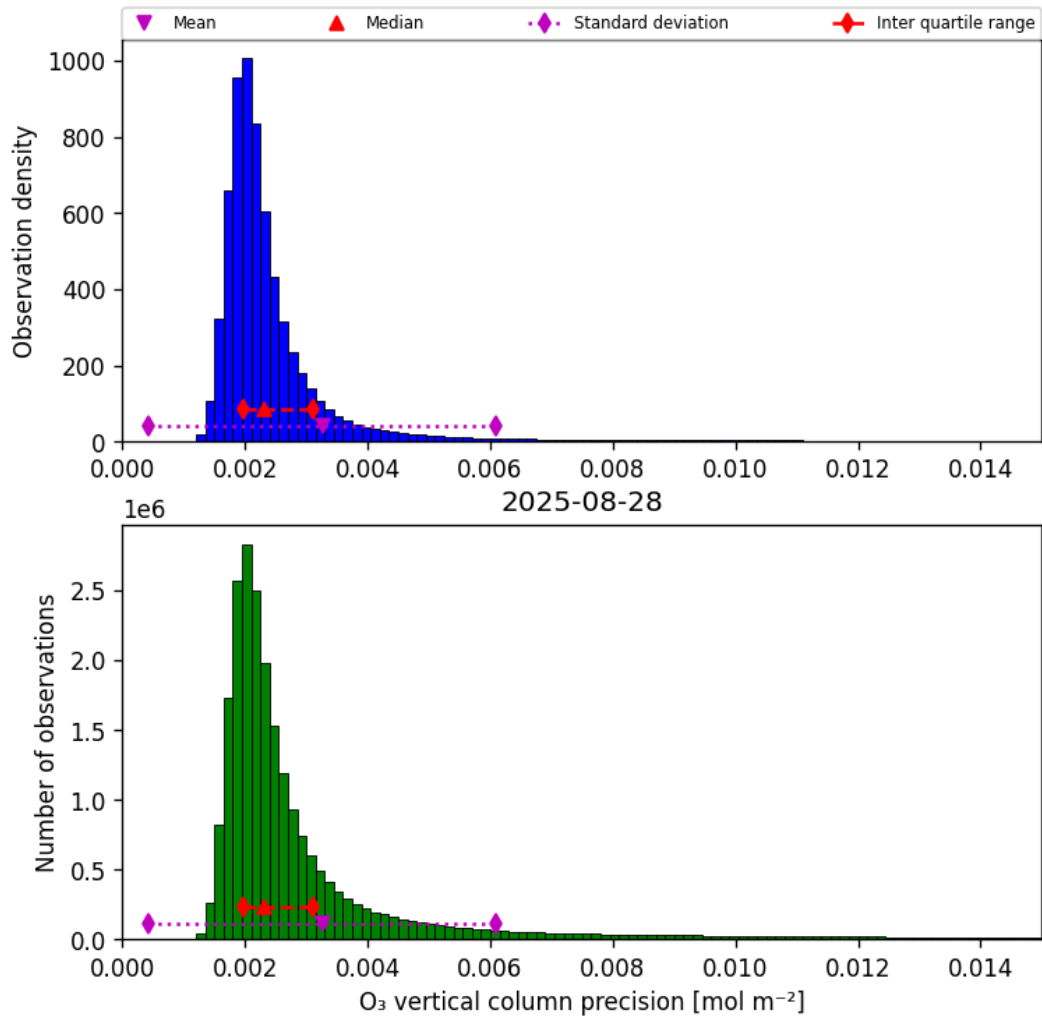
Figure 30: Histogram of "O 3 vertical column precision" for 2025-08-28 to 2025-08-28
