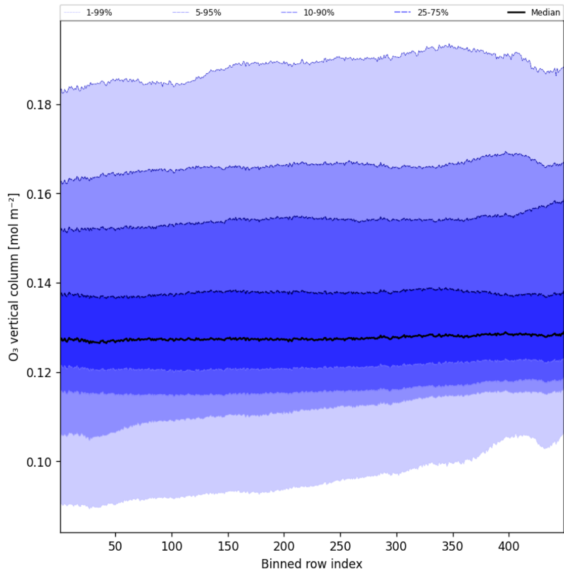
Figure 41: Along track statistics of “O 3 vertical column” for 2025-08-28 to 2025-08-28
