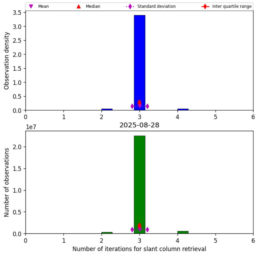
Figure 33: Histogram of “Number of iterations for slant column retrieval” for 2025-08-28 to 2025-08-28
