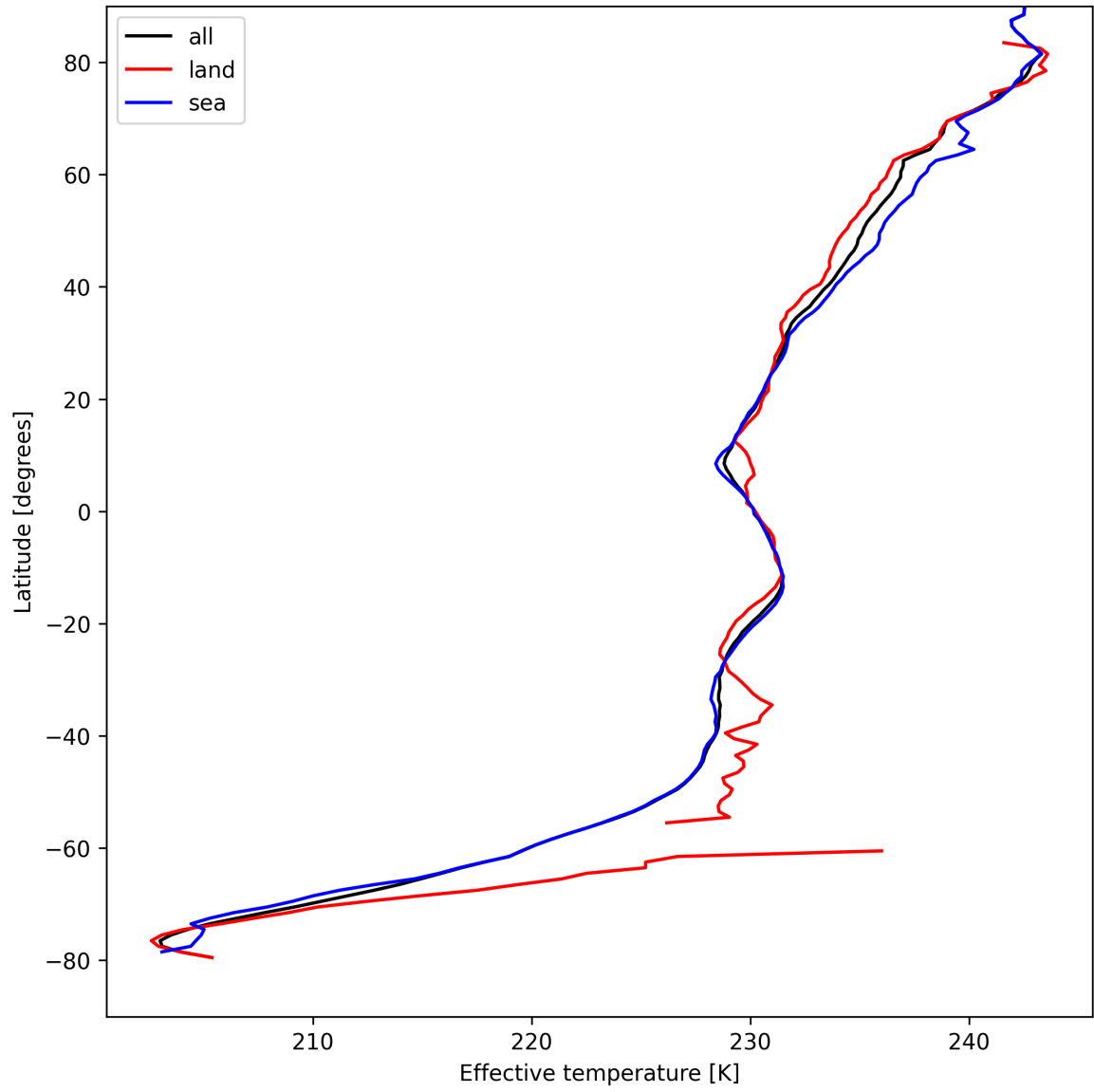
Figure 26: Zonal average of “Effective temperature” for 2025-08-28 to 2025-08-28.
