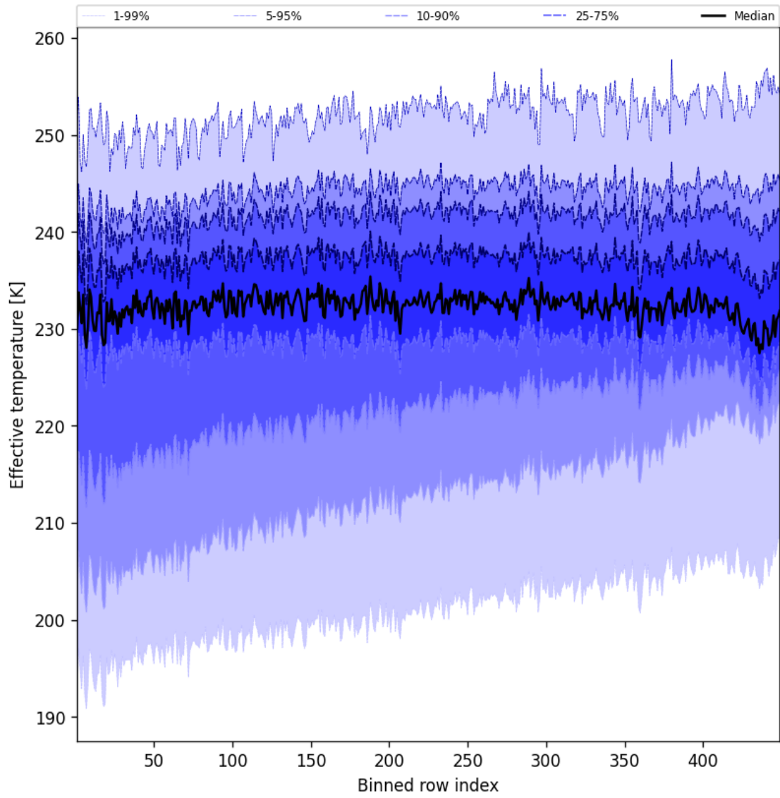
Figure 50: Along track statistics of “Effective temperature” for 2025-08-28 to 2025-08-28
