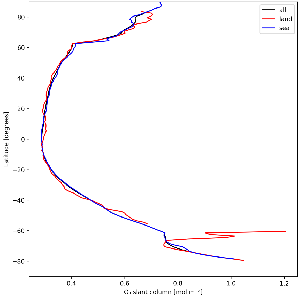
Figure 19: Zonal average of “O 3 slant column” for 2025-08-28 to 2025-08-28.
