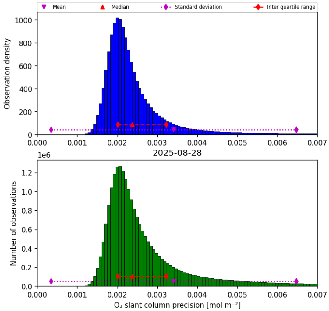
Figure 32: Histogram of “O 3 slant column precision” for 2025-08-28 to 2025-08-28
