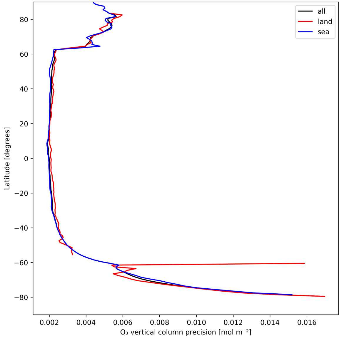
Figure 18: Zonal average of “O 3 vertical column precision” for 2025-08-28 to 2025-08-28.
