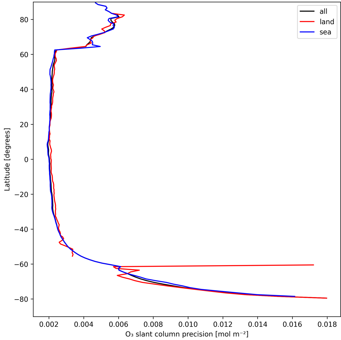
Figure 20: Zonal average of “O 3 slant column precision” for 2025-08-28 to 2025-08-28.
