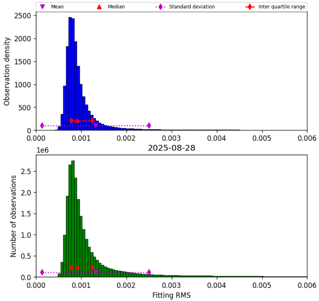
Figure 34: Histogram of “Fitting RMS” for 2025-08-28 to 2025-08-28
