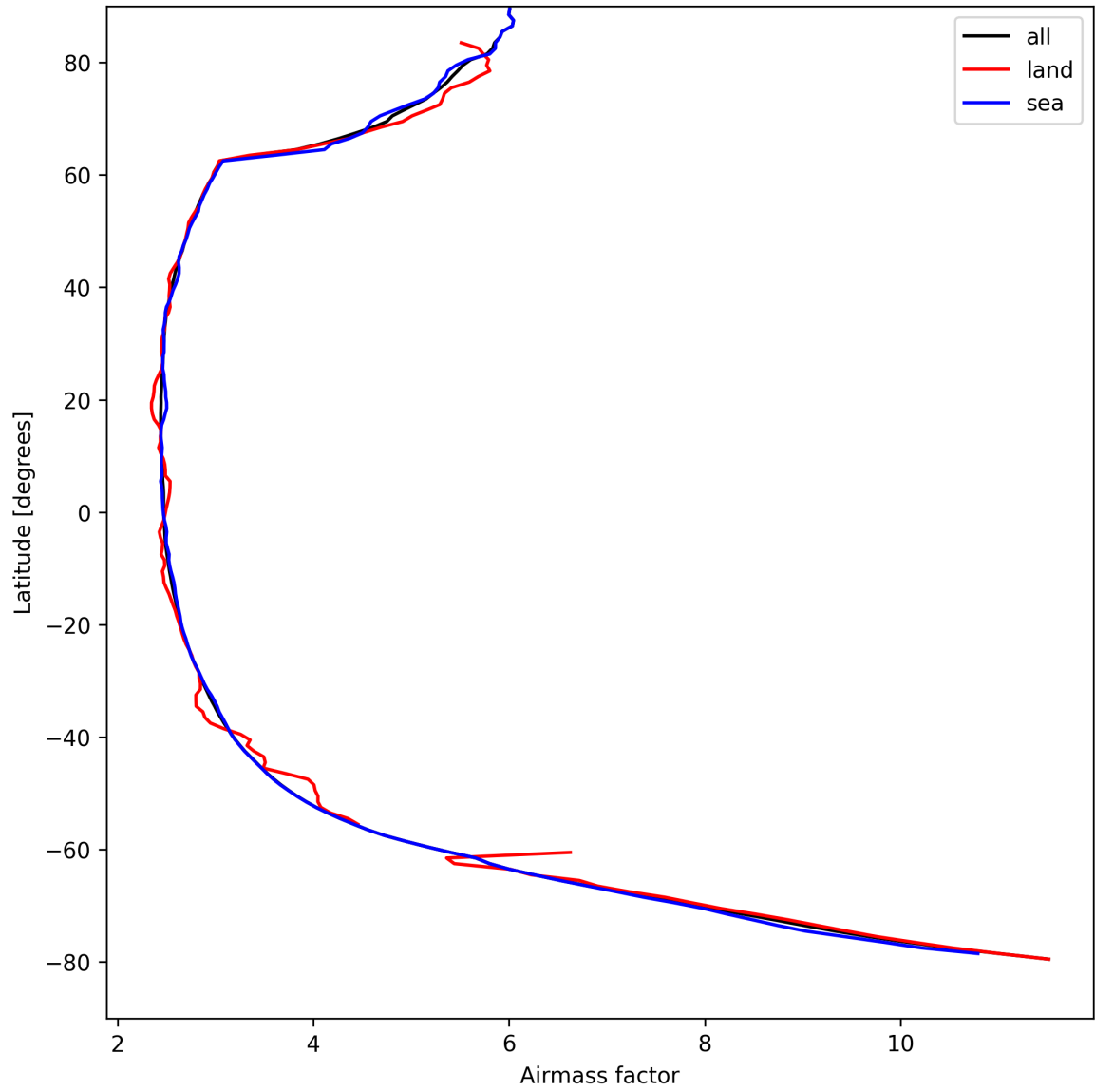
Figure 25: Zonal average of “Airmass factor” for 2025-08-28 to 2025-08-28.
