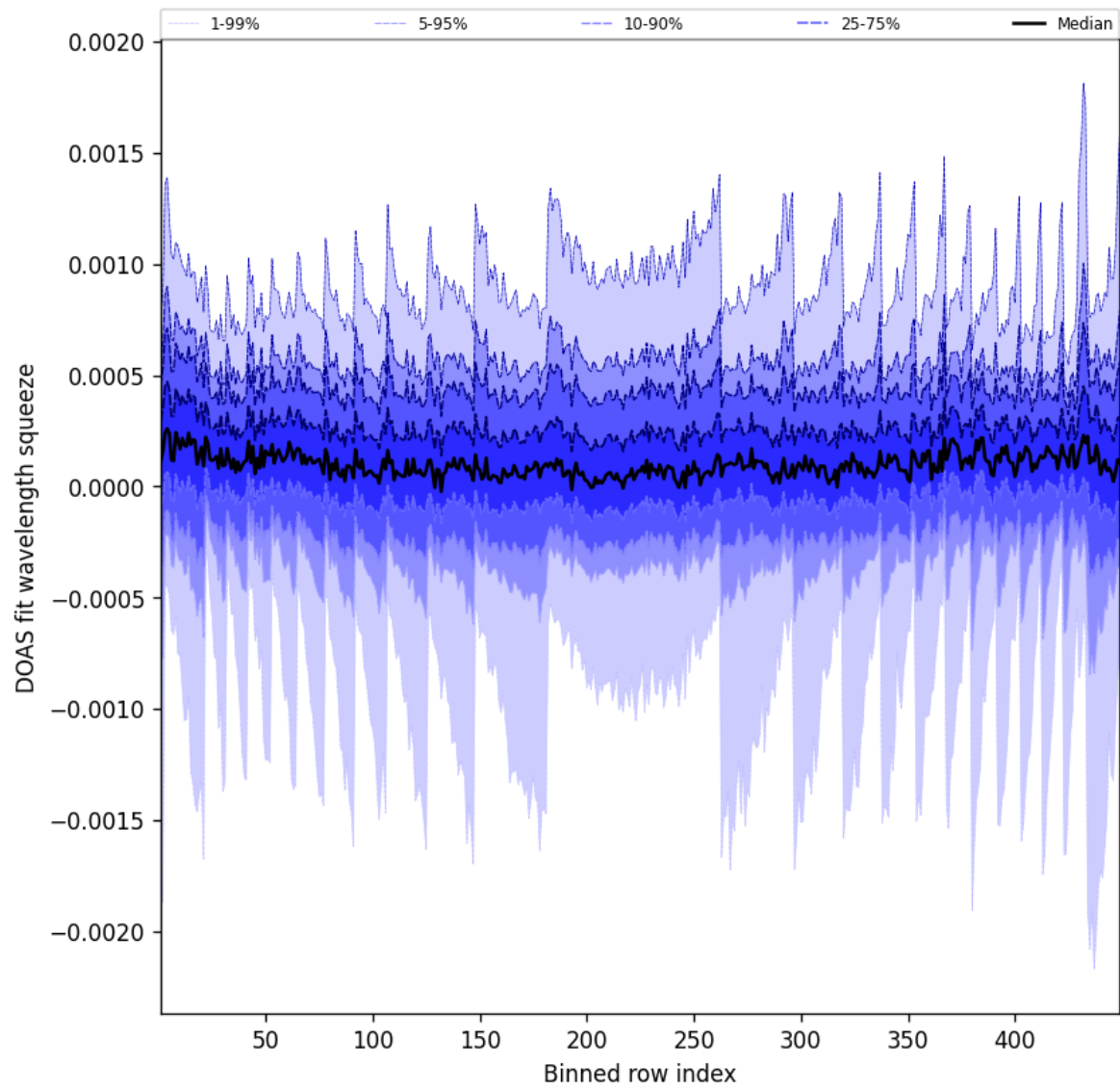
Figure 48: Along track statistics of “DOAS fit wavelength squeeze” for 2025-08-28 to 2025-08-28
