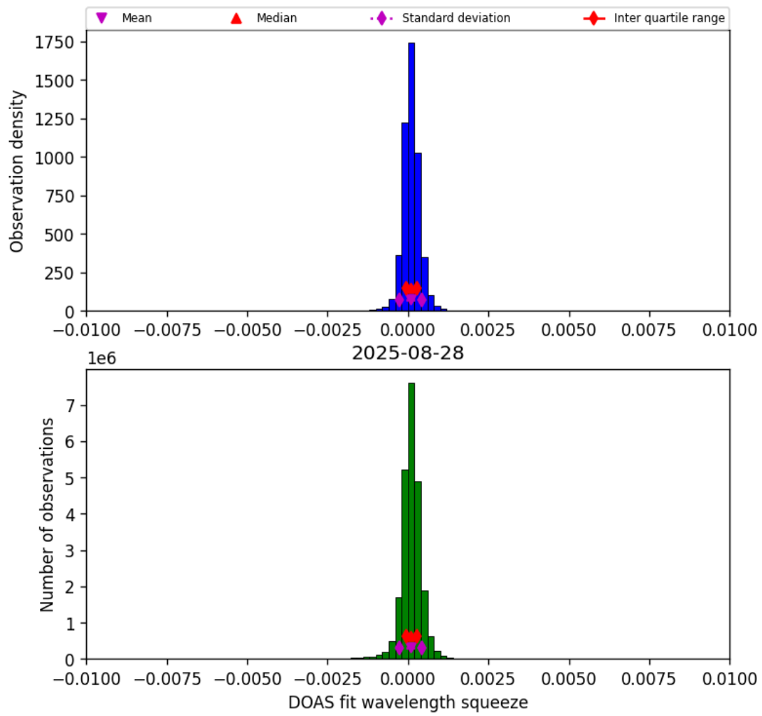
Figure 36: Histogram of “DOAS fit wavelength squeeze” for 2025-08-28 to 2025-08-28
