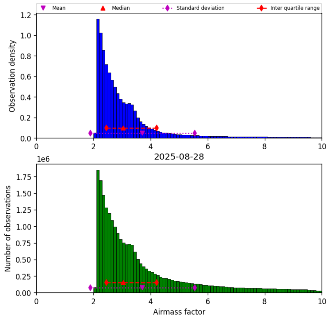
Figure 37: Histogram of “Airmass factor” for 2025-08-28 to 2025-08-28
