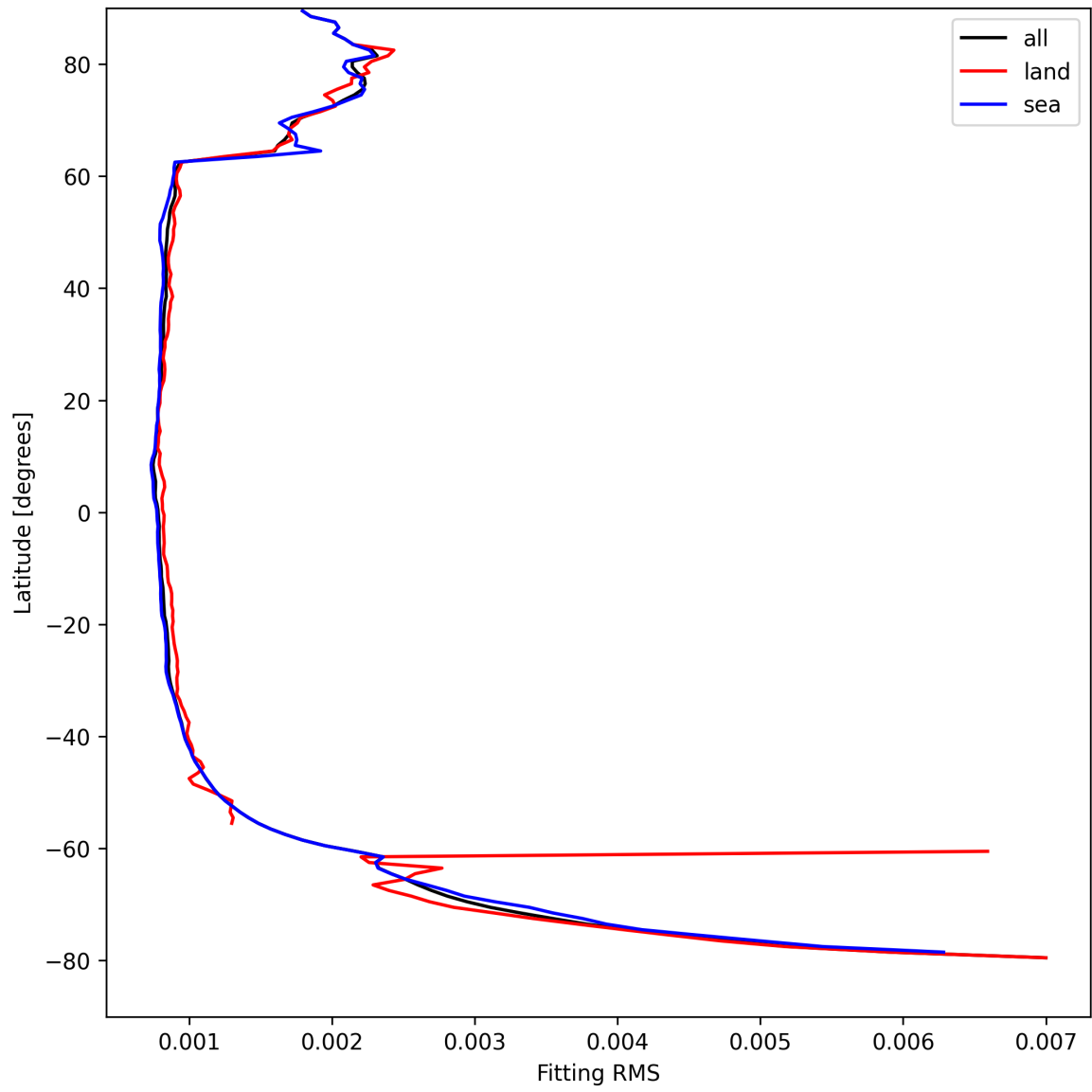
Figure 22: Zonal average of “Fitting RMS” for 2025-08-28 to 2025-08-28.
