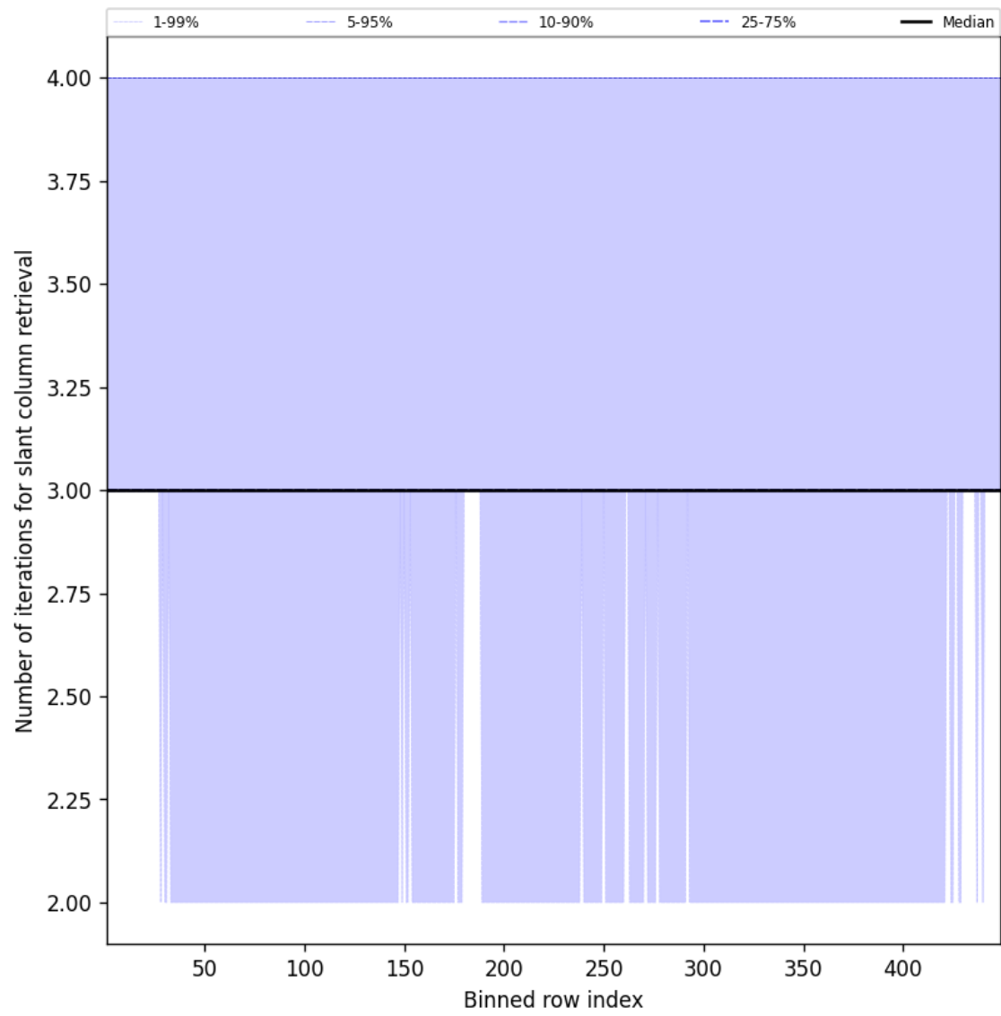
Figure 45: Along track statistics of “Number of iterations for slant column retrieval” for 2025-08-28 to 2025-08-28
