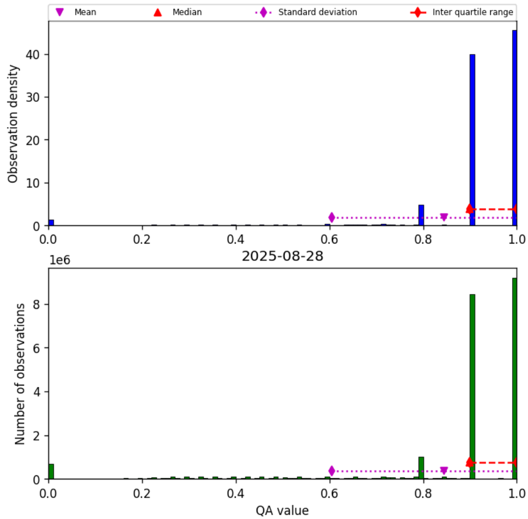
Figure 28: Histogram of “QA value” for 2025-08-28 to 2025-08-28
