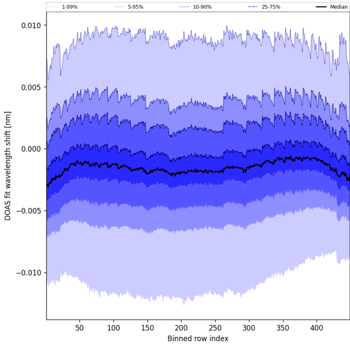
Figure 47: Along track statistics of “DOAS fit wavelength shift” for 2025-08-28 to 2025-08-28
