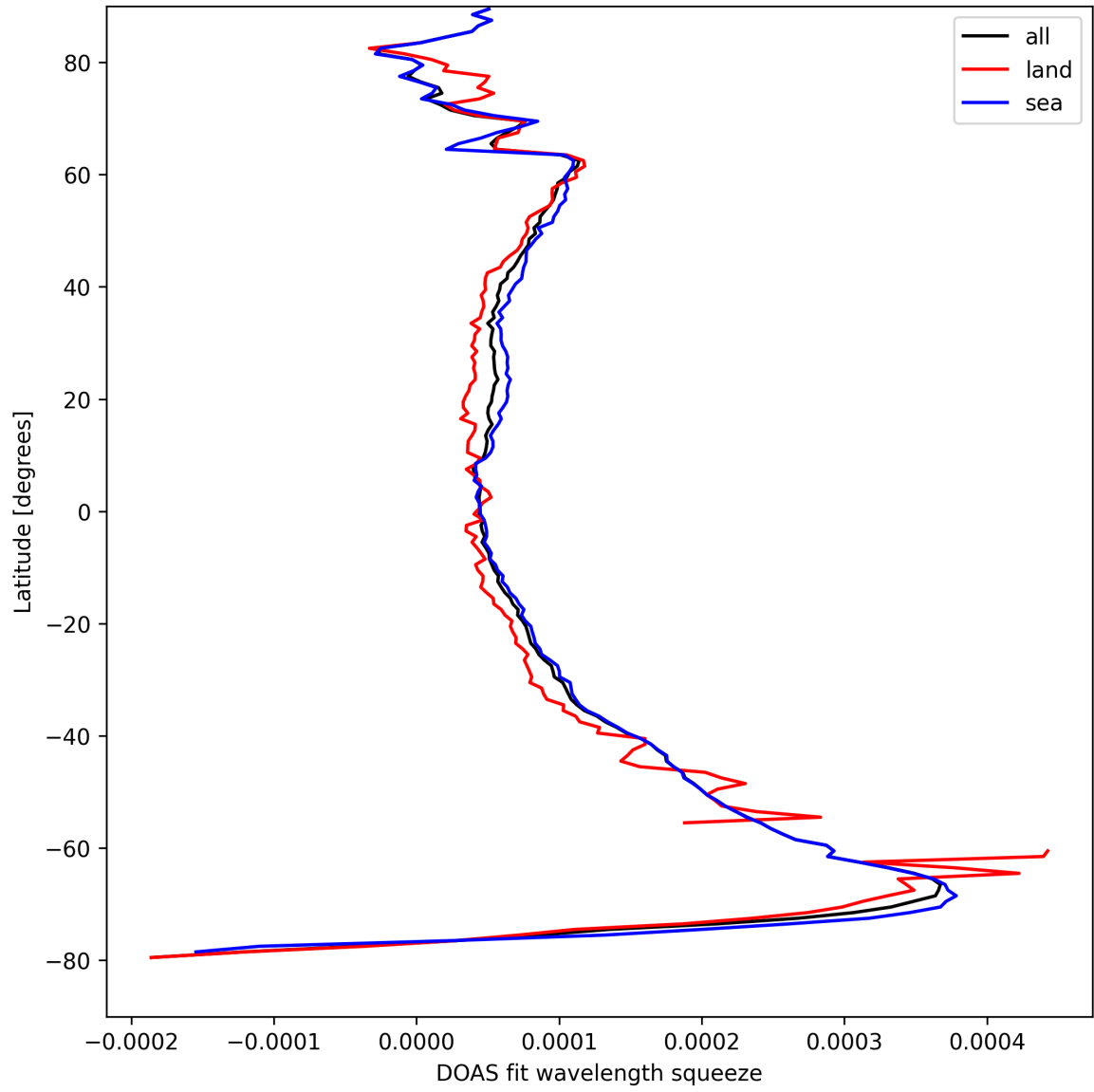
Figure 24: Zonal average of “DOAS fit wavelength squeeze” for 2025-08-28 to 2025-08-28.
