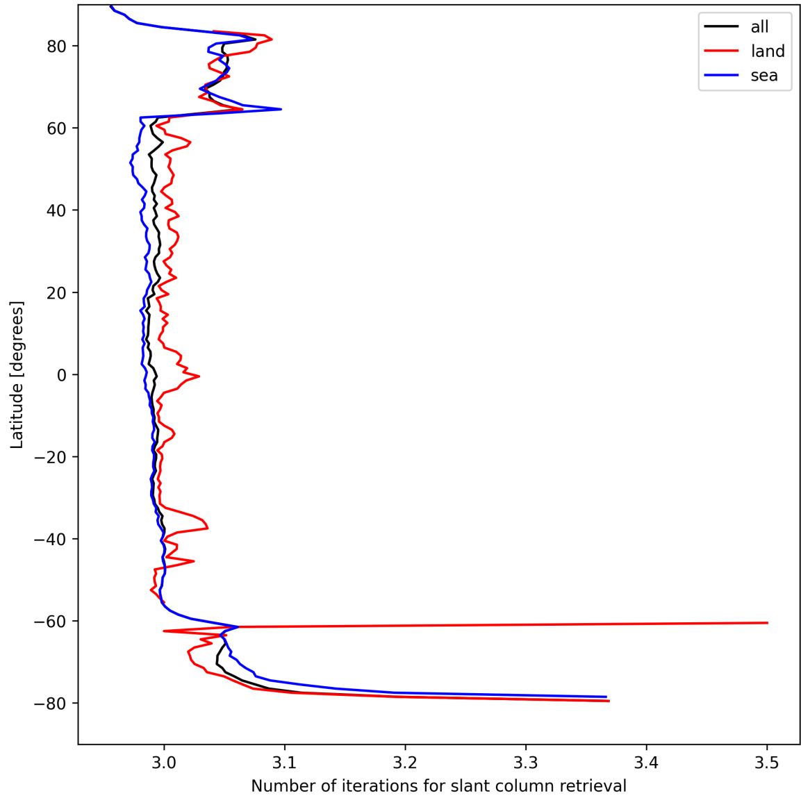
Figure 21: Zonal average of “Number of iterations for slant column retrieval” for 2025-08-28 to 2025-08-28.
