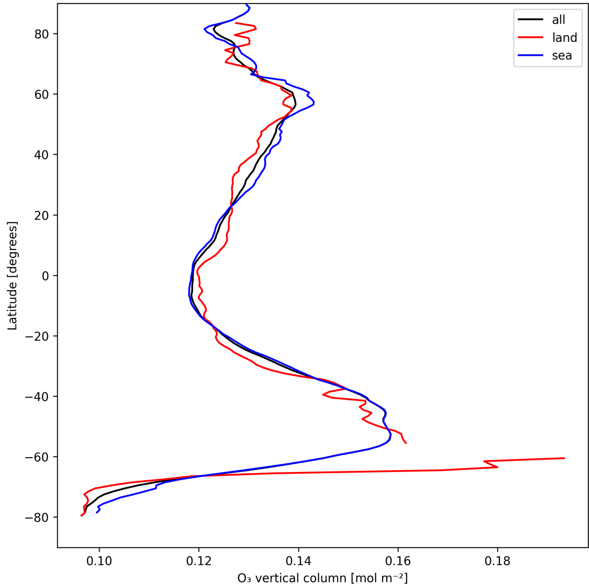
Figure 17: Zonal average of “O 3 vertical column” for 2025-08-28 to 2025-08-28.
