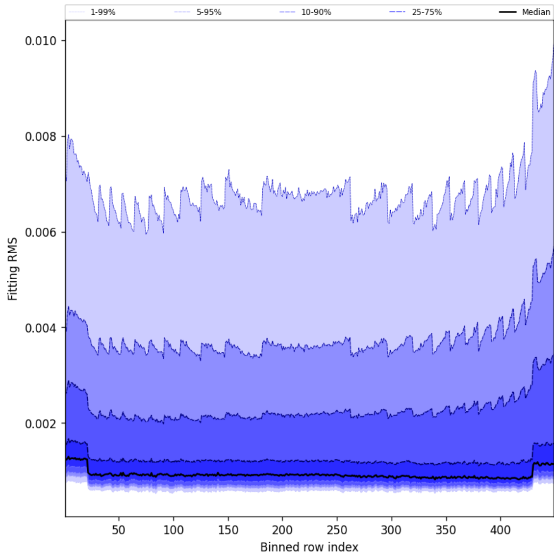
Figure 46: Along track statistics of “Fitting RMS” for 2025-08-28 to 2025-08-28
