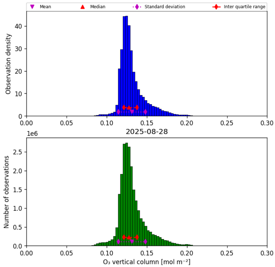
Figure 29: Histogram of “O 3 vertical column” for 2025-08-28 to 2025-08-28
