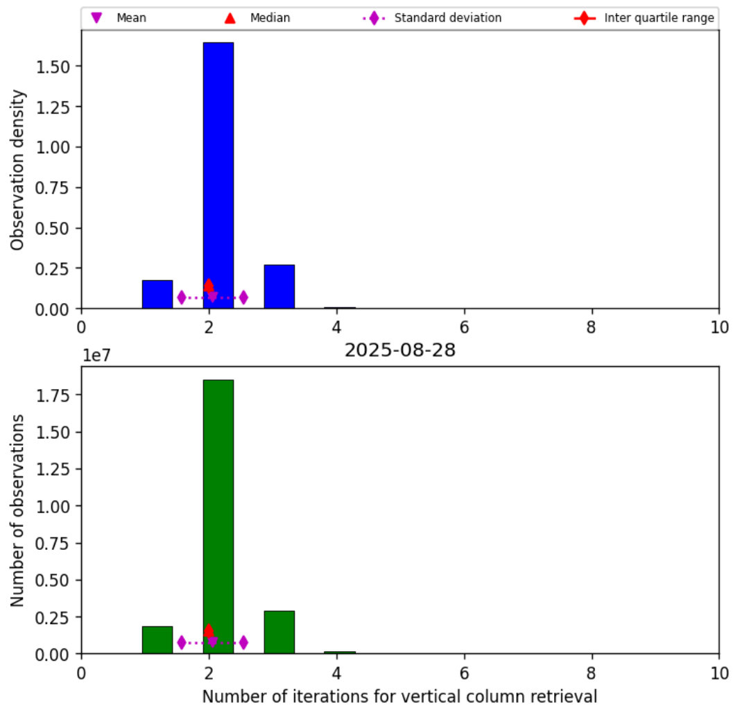
Figure 39: Histogram of “Number of iterations for vertical column retrieval” for 2025-08-28 to 2025-08-28
