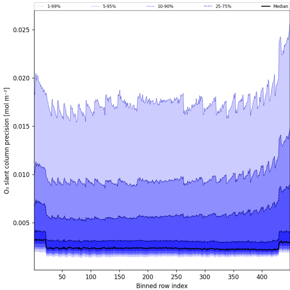
Figure 44: Along track statistics of “O 3 slant column precision” for 2025-08-28 to 2025-08-28
