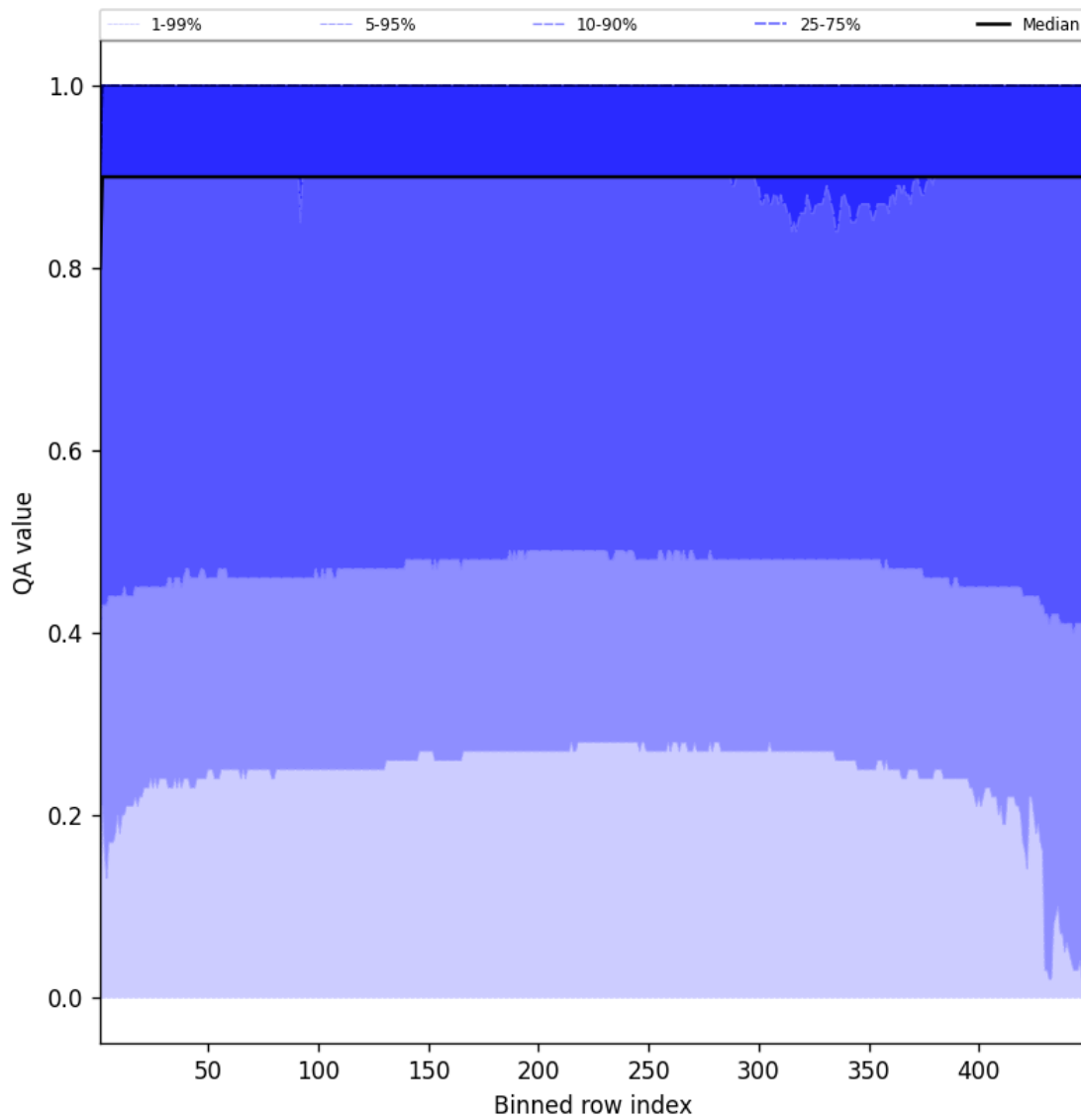
Figure 40: Along track statistics of “QA value” for 2025-08-28 to 2025-08-28
