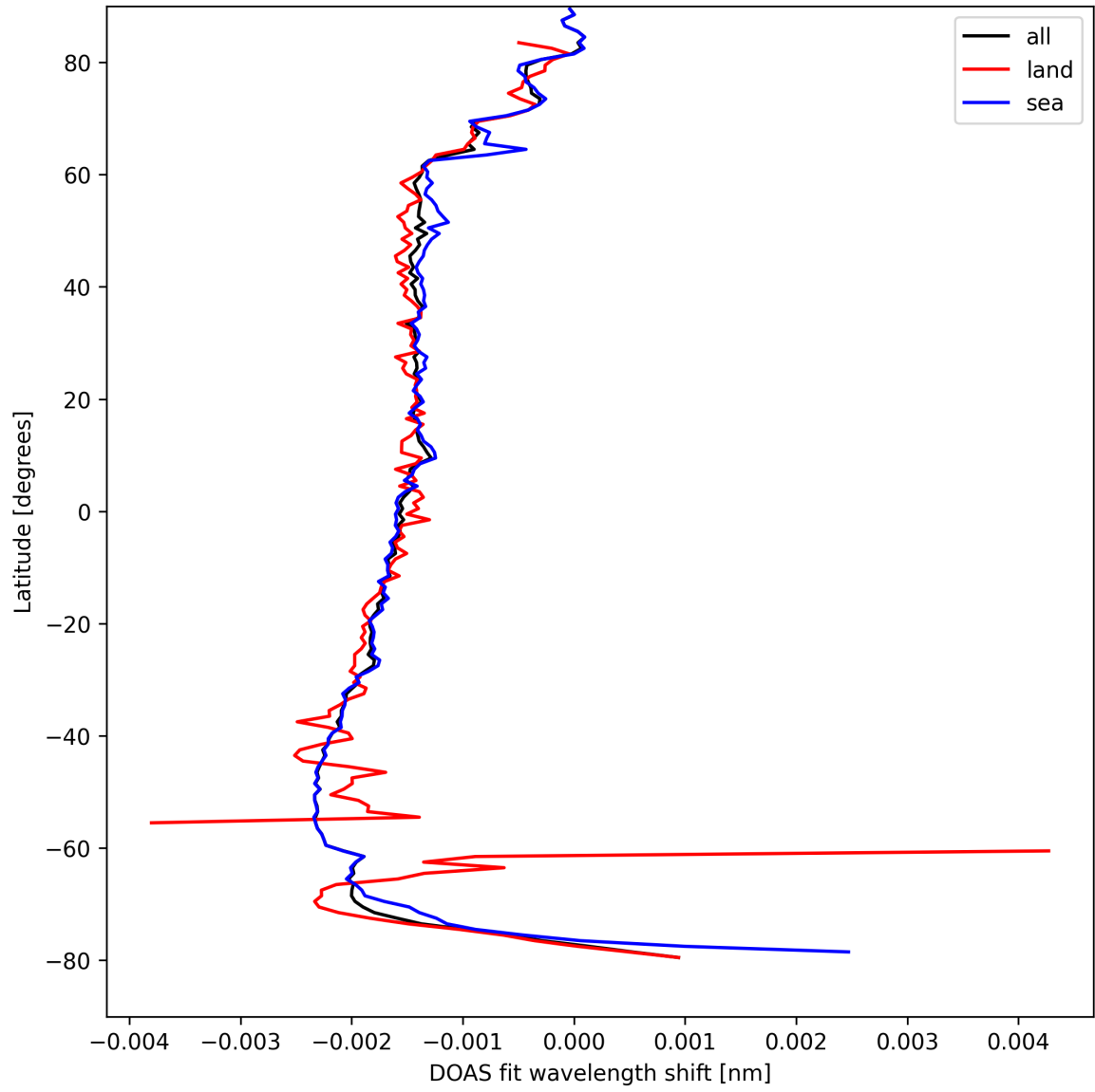
Figure 23: Zonal average of "DOAS fit wavelength shift" for 2025-08-28 to 2025-08-28.
