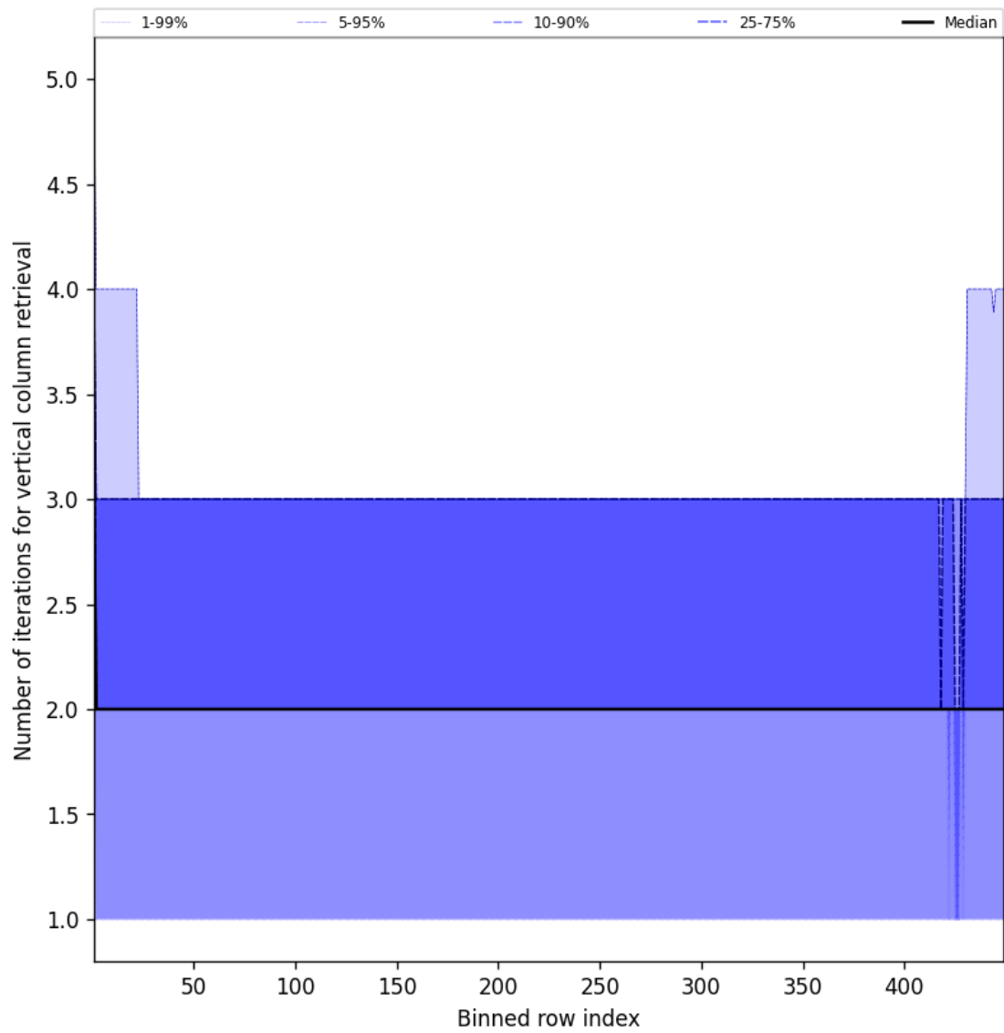
Figure 51: Along track statistics of “Number of iterations for vertical column retrieval” for 2025-08-28 to 2025-08-28
