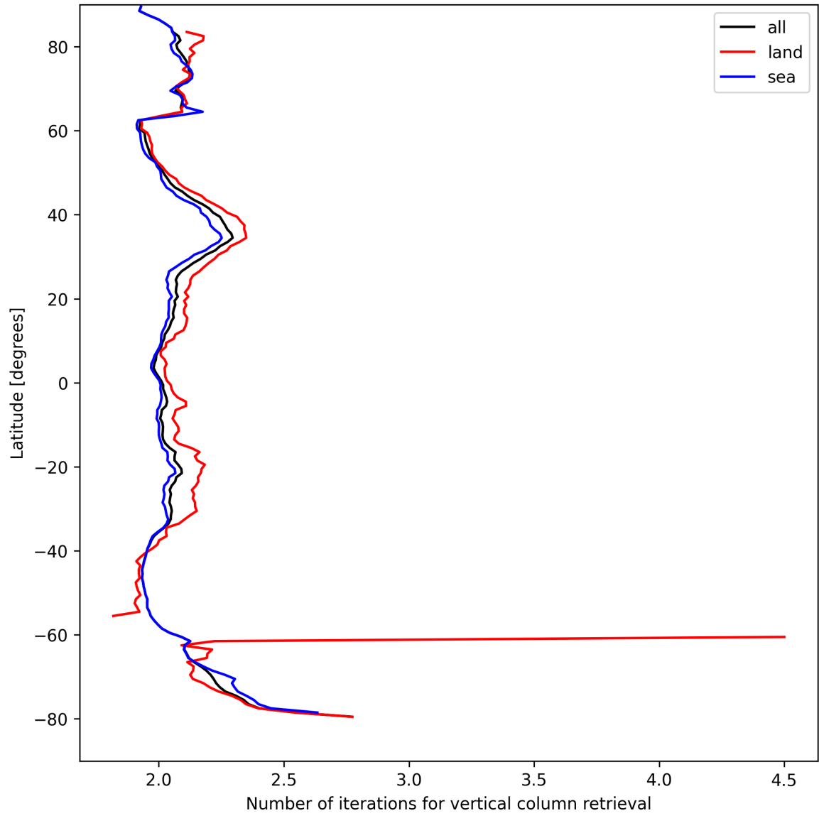
Figure 27: Zonal average of “Number of iterations for vertical column retrieval” for 2025-08-28 to 2025-08-28.
