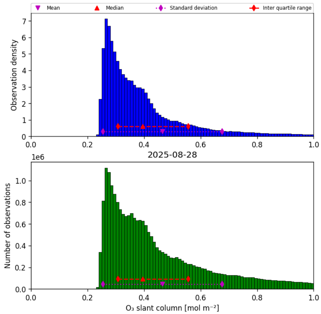
Figure 31: Histogram of “O 3 slant column” for 2025-08-28 to 2025-08-28
