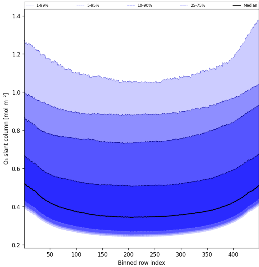
Figure 43: Along track statistics of “O 3 slant column” for 2025-08-28 to 2025-08-28
