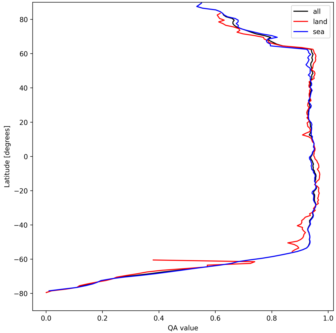
Figure 16: Zonal average of “QA value” for 2025-08-28 to 2025-08-28.
