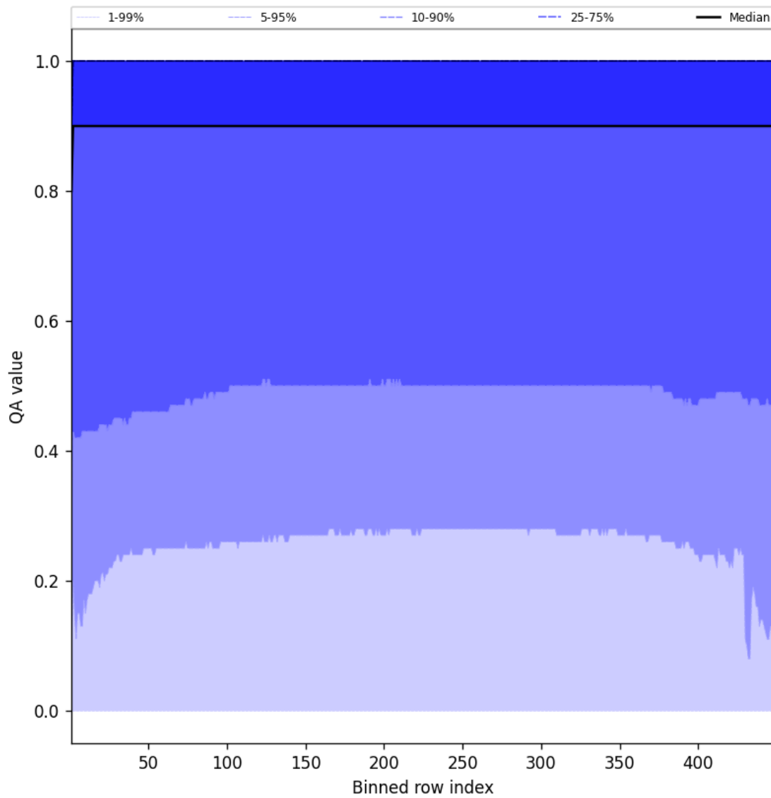
Figure 40: Along track statistics of “QA value” for 2025-08-29 to 2025-08-30
