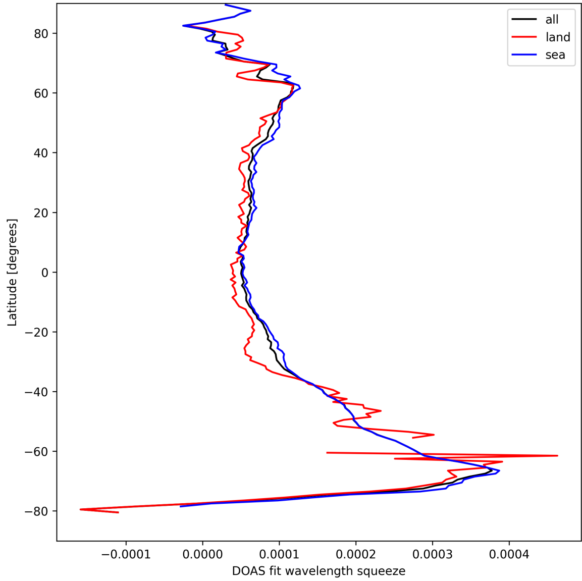
Figure 24: Zonal average of “DOAS fit wavelength squeeze” for 2025-08-29 to 2025-08-30.
