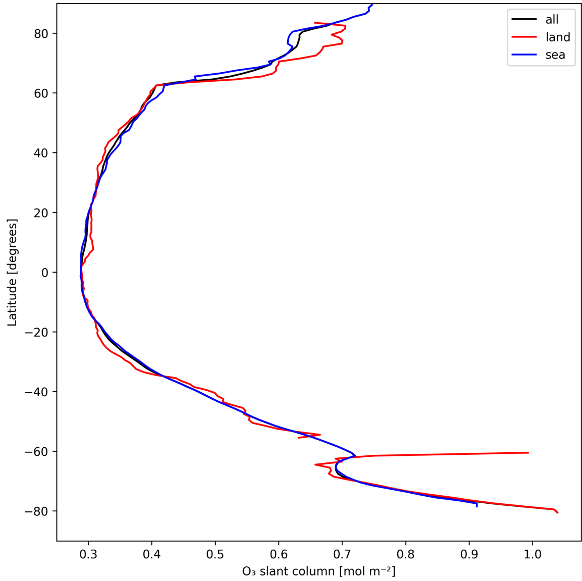
Figure 19: Zonal average of “O 3 slant column” for 2025-08-29 to 2025-08-30.
