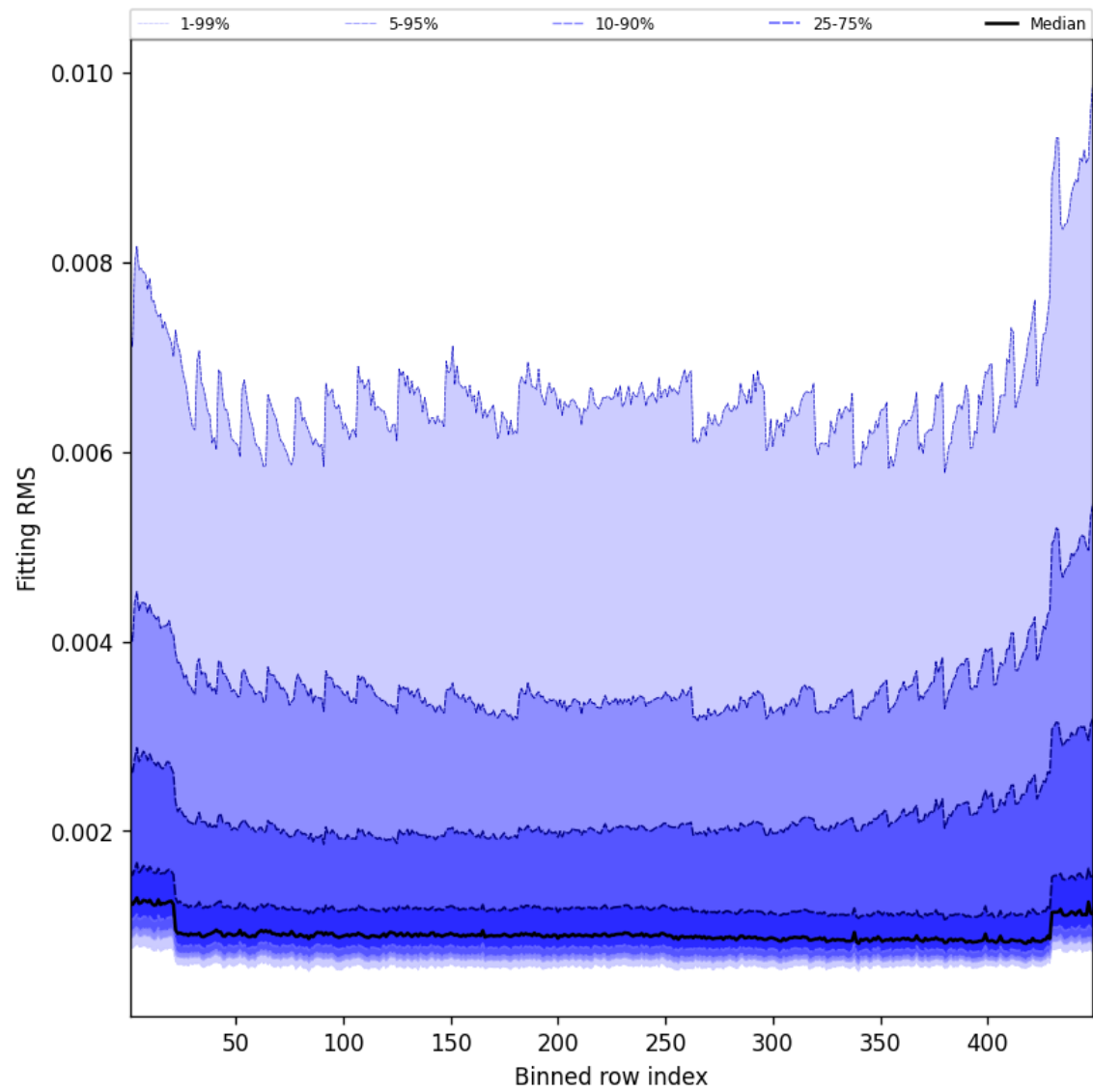
Figure 46: Along track statistics of “Fitting RMS” for 2025-08-29 to 2025-08-30
