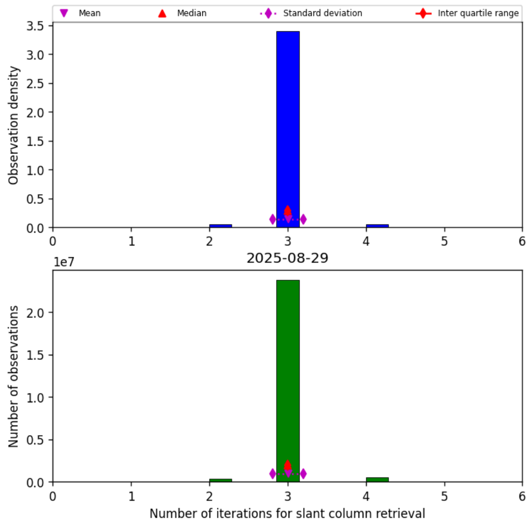
Figure 33: Histogram of “Number of iterations for slant column retrieval” for 2025-08-29 to 2025-08-30
