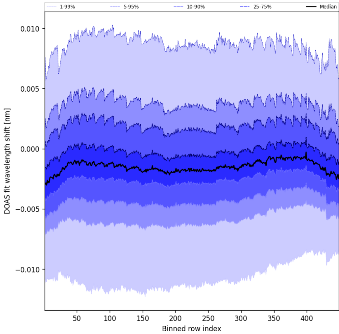
Figure 47: Along track statistics of “DOAS fit wavelength shift” for 2025-08-29 to 2025-08-30
