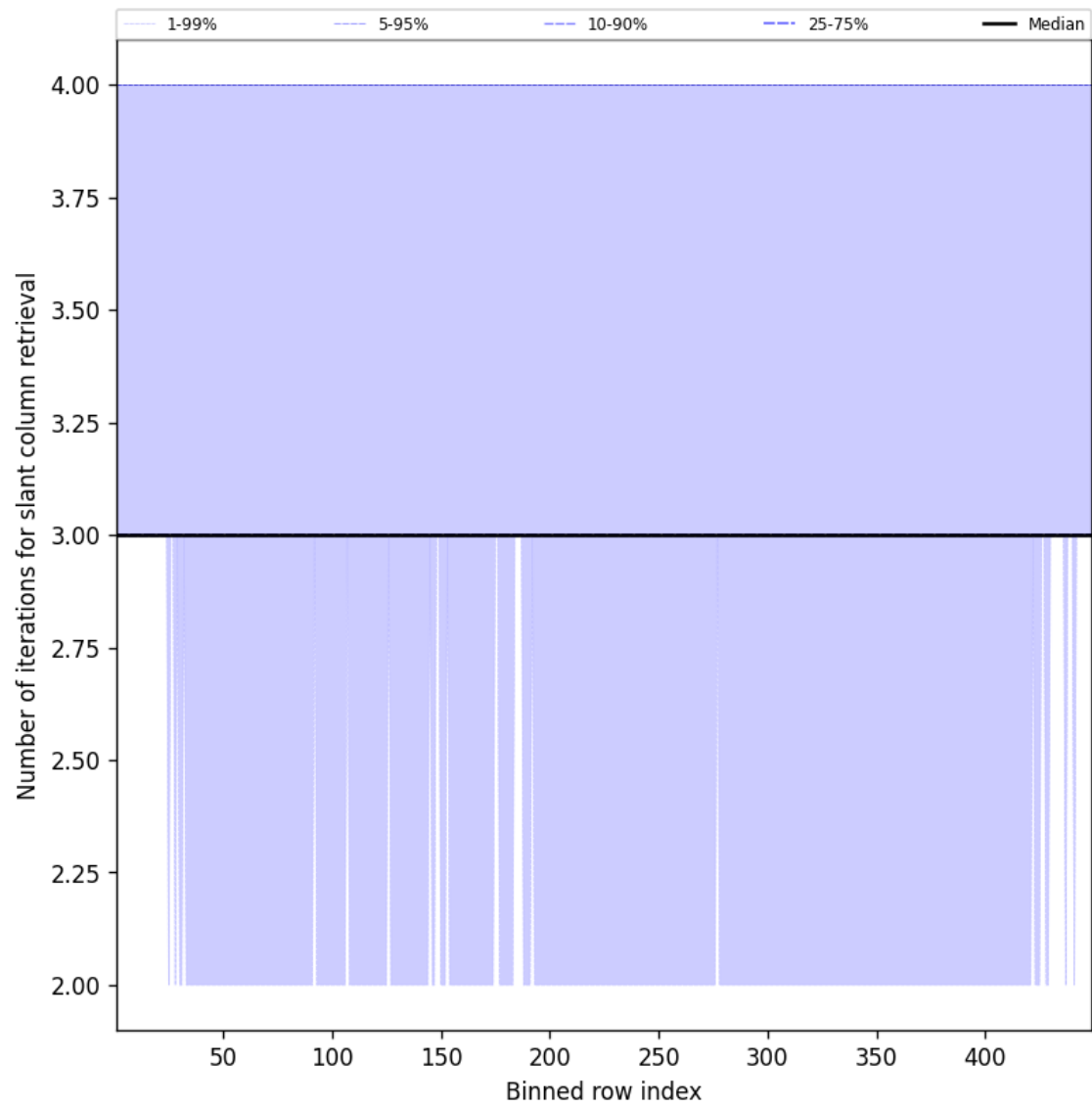
Figure 45: Along track statistics of “Number of iterations for slant column retrieval” for 2025-08-29 to 2025-08-30
