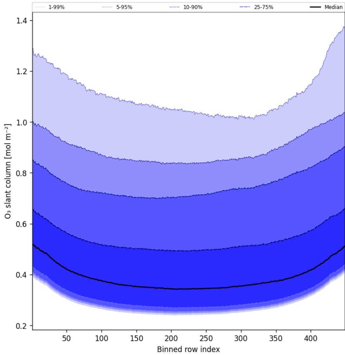
Figure 43: Along track statistics of “O 3 slant column” for 2025-08-29 to 2025-08-30
