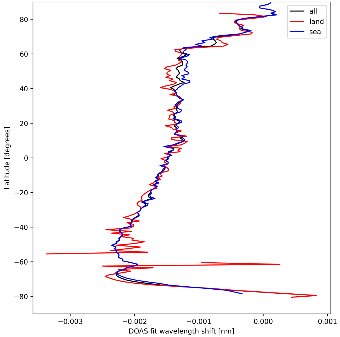
Figure 23: Zonal average of “DOAS fit wavelength shift” for 2025-08-29 to 2025-08-30.
