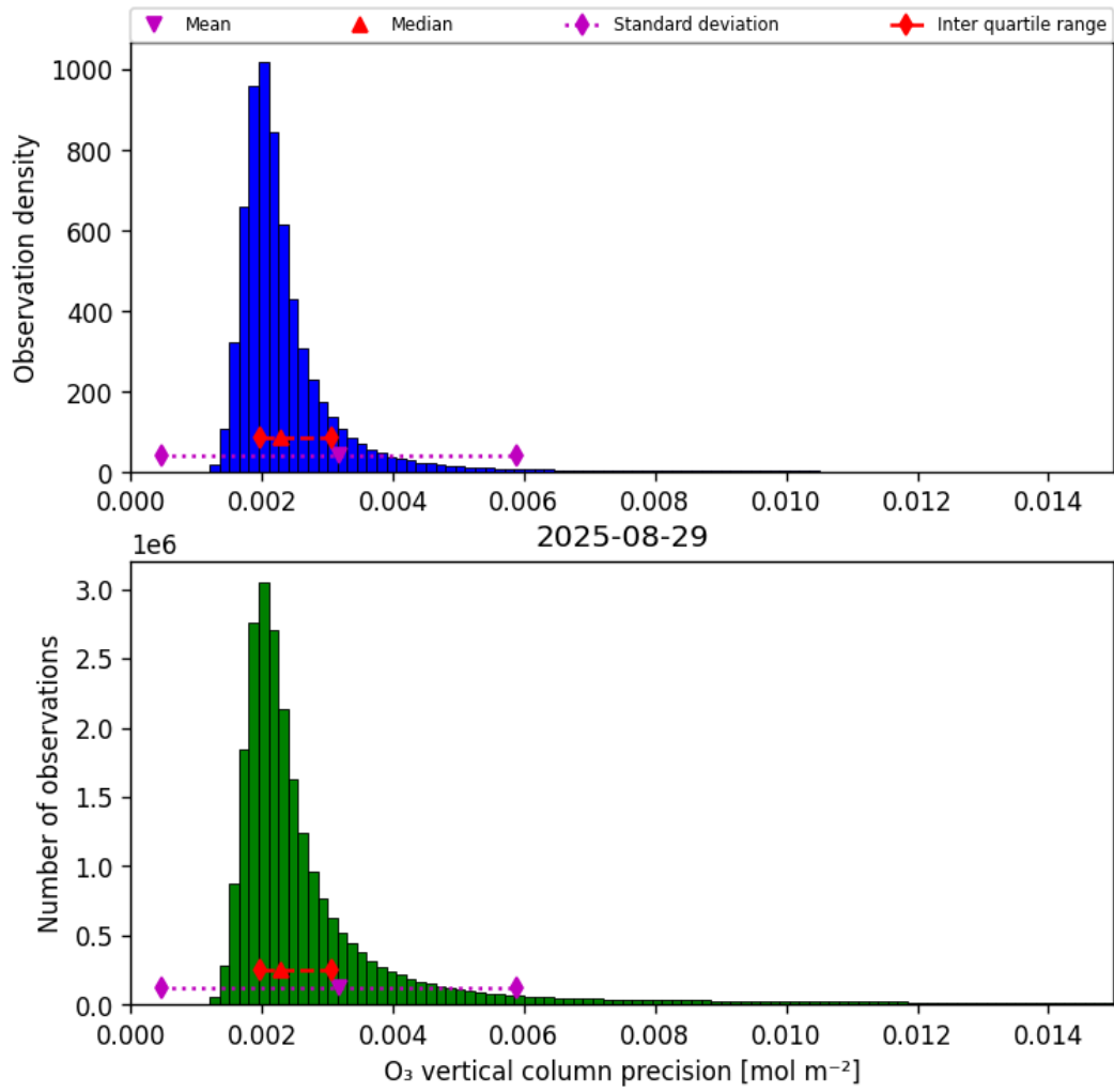
Figure 30: Histogram of “O 3 vertical column precision” for 2025-08-29 to 2025-08-30
