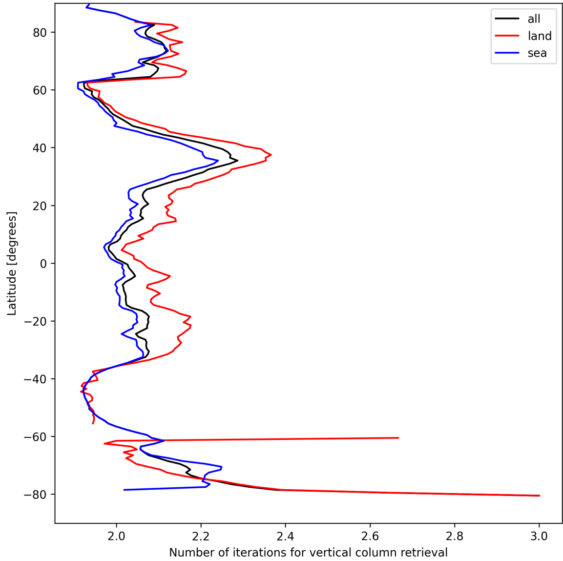
Figure 27: Zonal average of “Number of iterations for vertical column retrieval” for 2025-08-29 to 2025-08-30.
