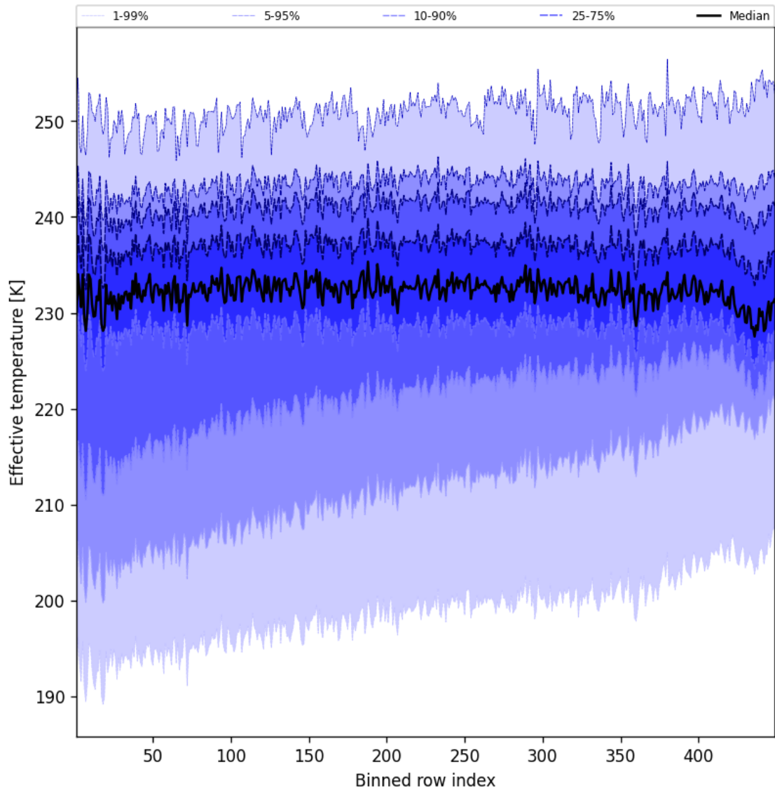
Figure 50: Along track statistics of “Effective temperature” for 2025-08-29 to 2025-08-30
