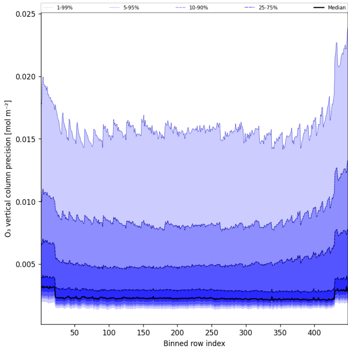
Figure 42: Along track statistics of “O 3 vertical column precision” for 2025-08-29 to 2025-08-30
