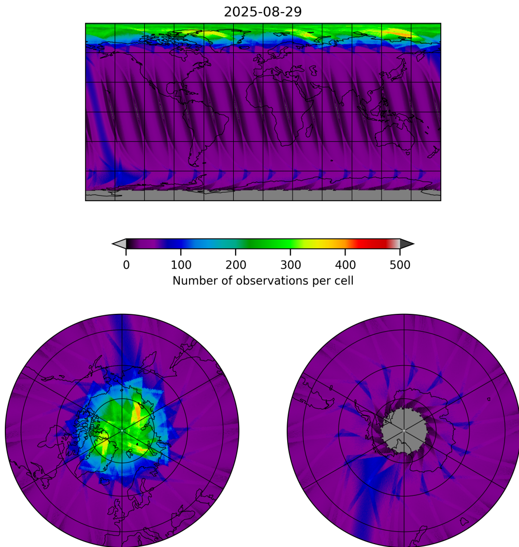
Figure 15: Map of the number of observations for 2025-08-29 to 2025-08-30
