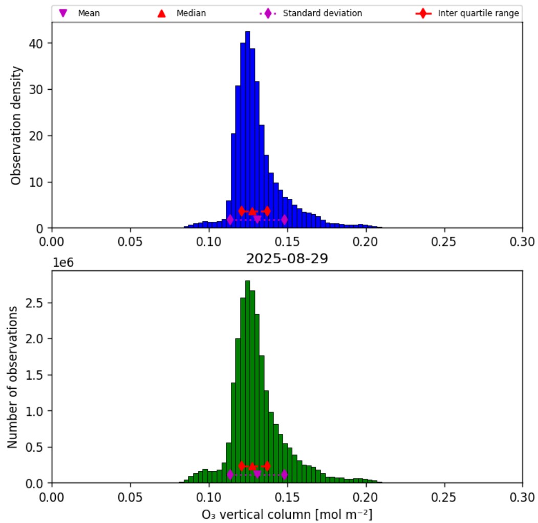
Figure 29: Histogram of “O 3 vertical column” for 2025-08-29 to 2025-08-30
