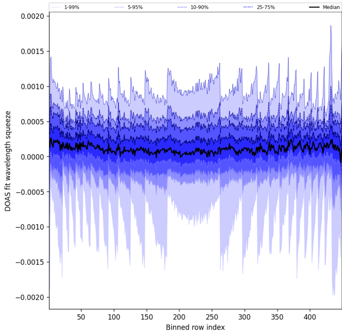
Figure 48: Along track statistics of “DOAS fit wavelength squeeze” for 2025-08-29 to 2025-08-30
