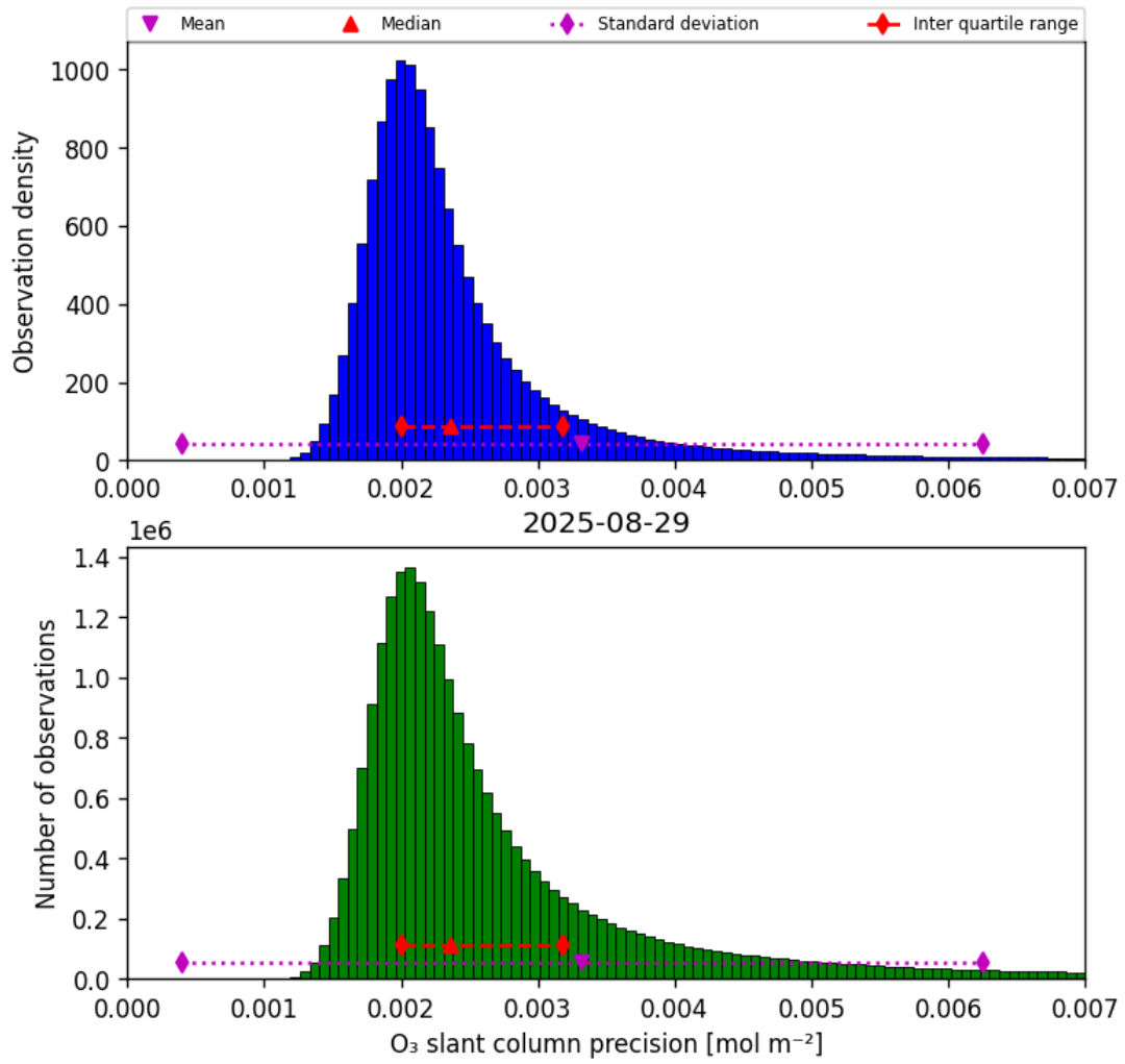
Figure 32: Histogram of “O 3 slant column precision” for 2025-08-29 to 2025-08-30
