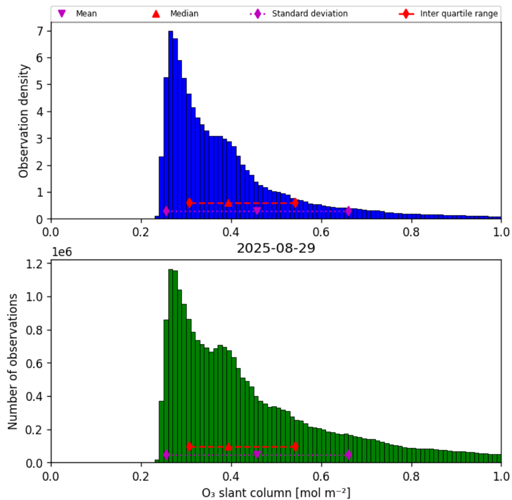
Figure 31: Histogram of “O 3 slant column” for 2025-08-29 to 2025-08-30
