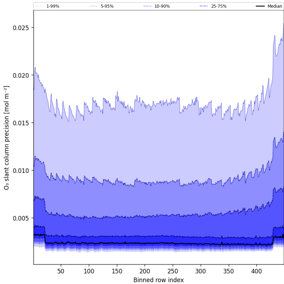
Figure 44: Along track statistics of “O 3 slant column precision” for 2025-08-29 to 2025-08-30
