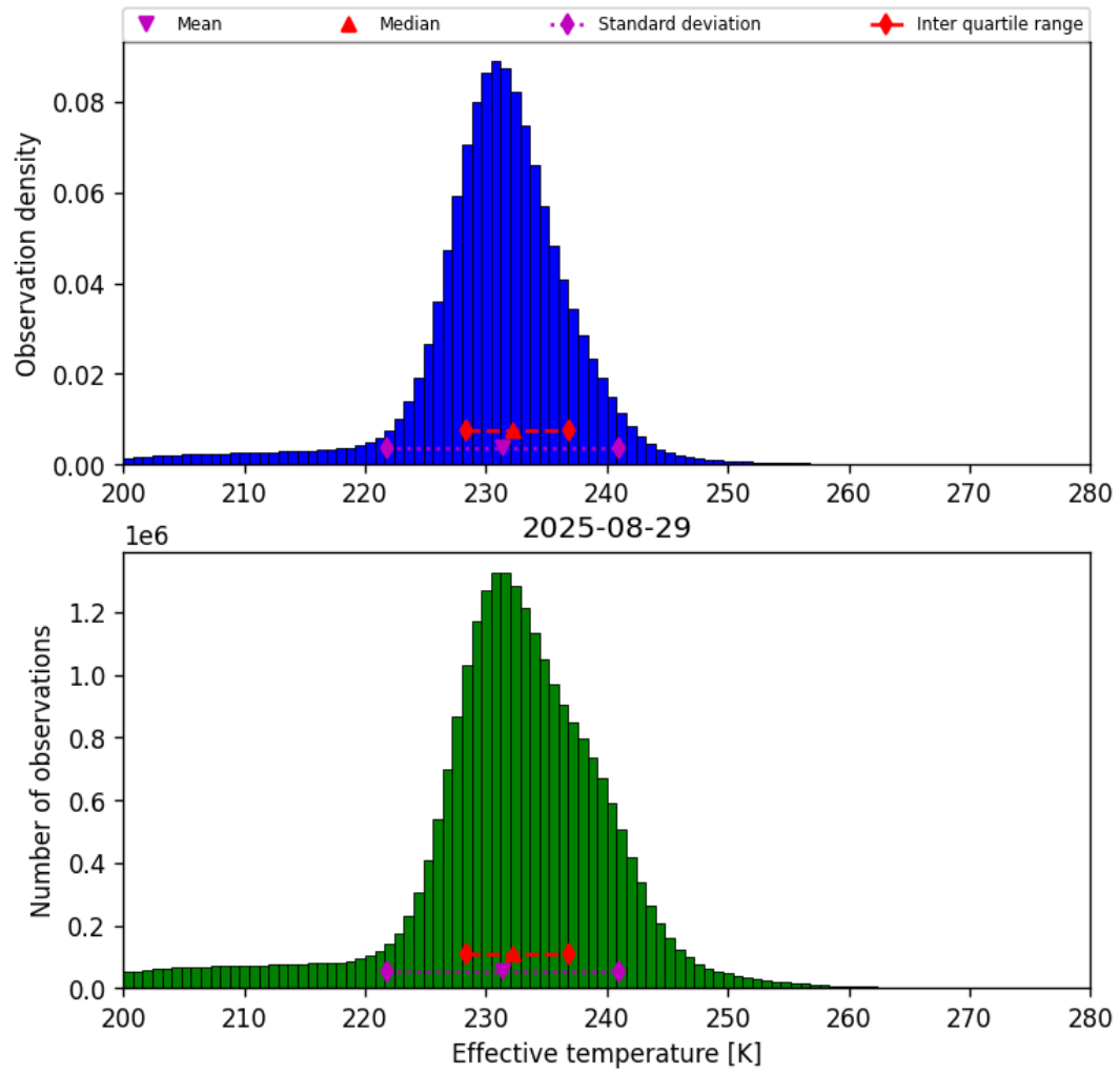
Figure 38: Histogram of “Effective temperature” for 2025-08-29 to 2025-08-30
