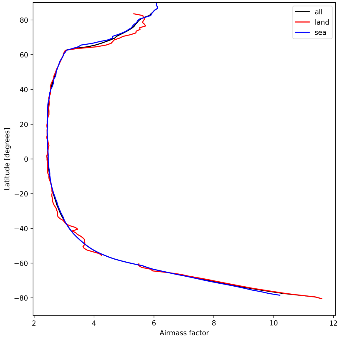
Figure 25: Zonal average of “Airmass factor” for 2025-08-29 to 2025-08-30.
