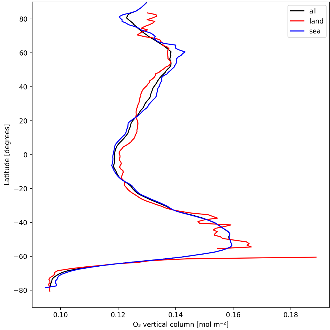
Figure 17: Zonal average of “O 3 vertical column” for 2025-08-29 to 2025-08-30.
