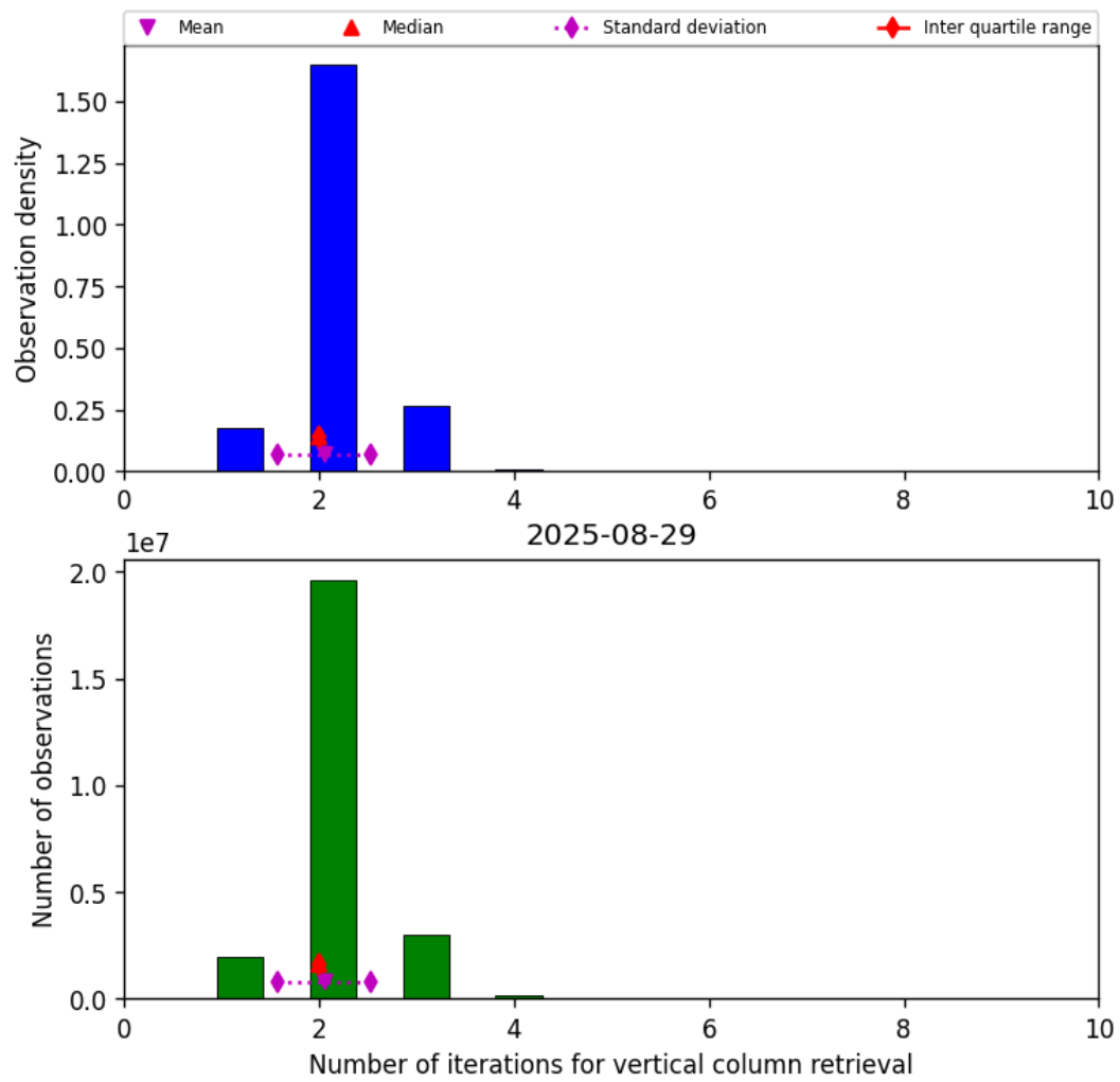
Figure 39: Histogram of “Number of iterations for vertical column retrieval” for 2025-08-29 to 2025-08-30
