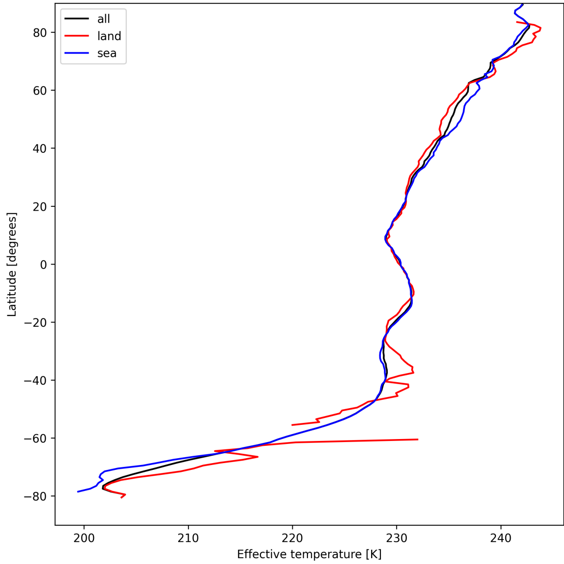
Figure 26: Zonal average of "Effective temperature" for 2025-08-29 to 2025-08-30.
