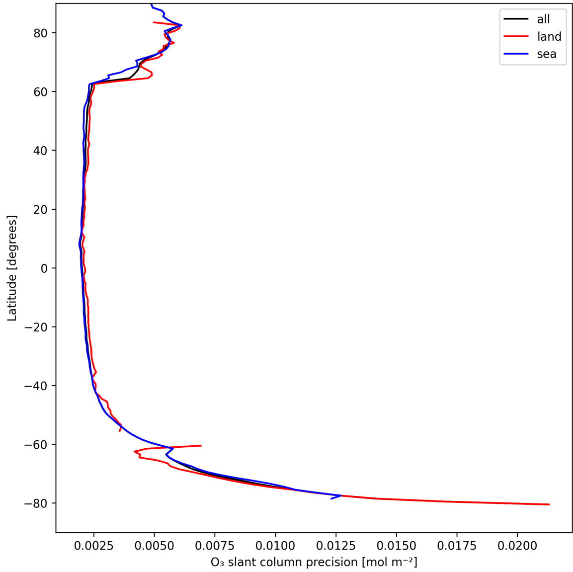
Figure 20: Zonal average of "O 3 slant column precision" for 2025-08-29 to 2025-08-30.
