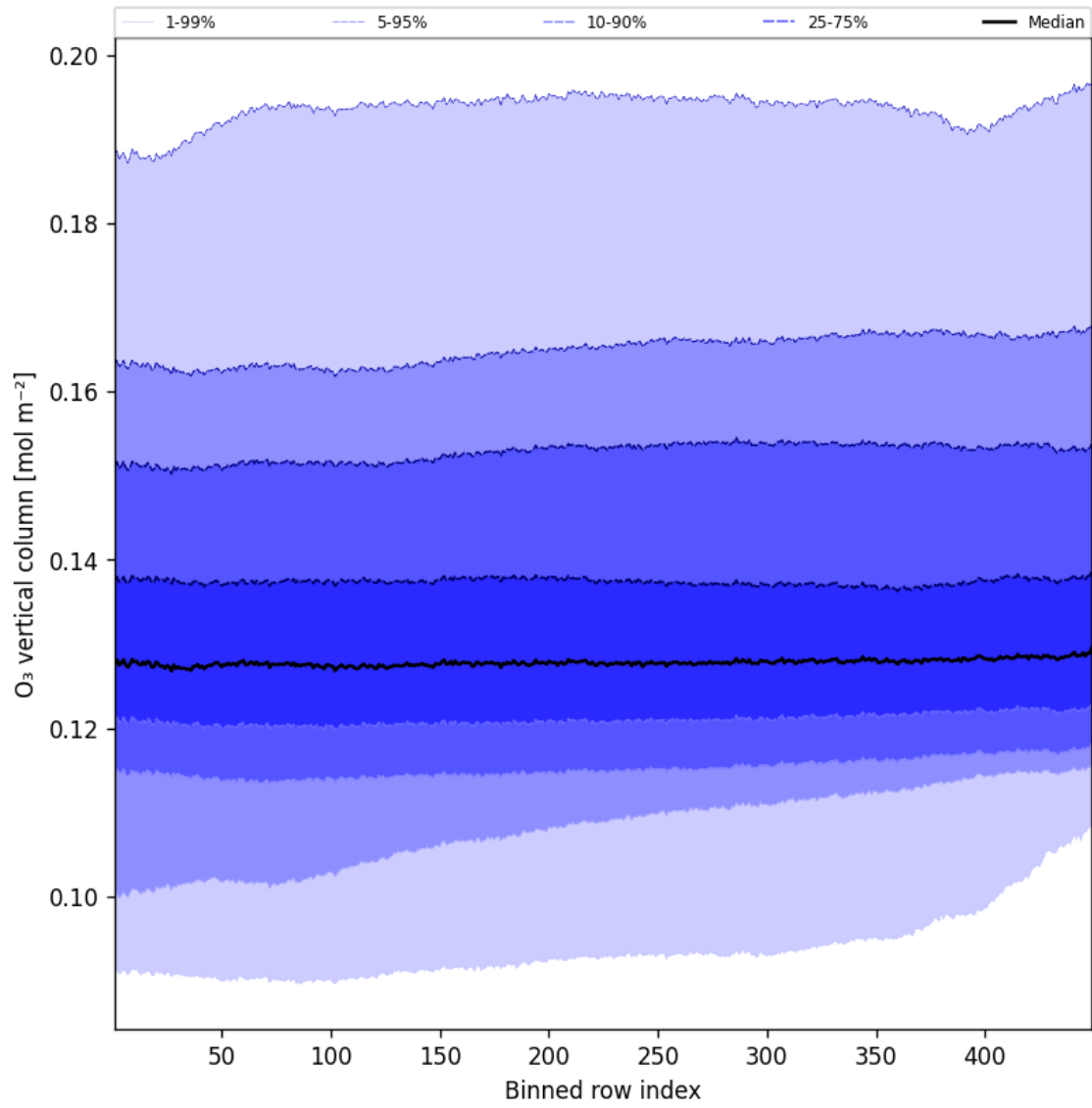
Figure 41: Along track statistics of “O 3 vertical column” for 2025-08-29 to 2025-08-30
