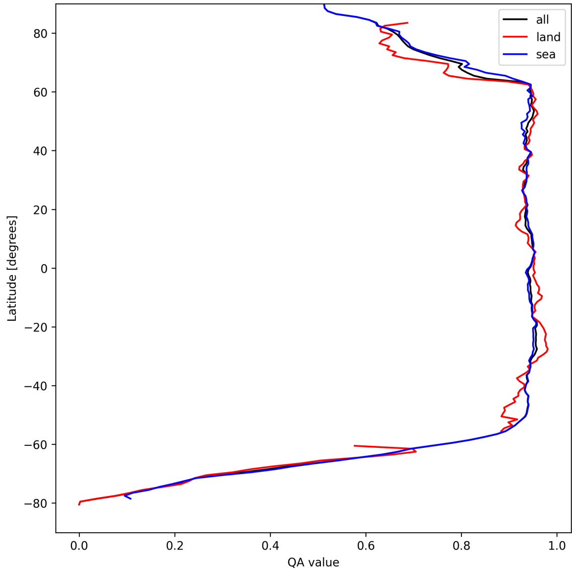
Figure 16: Zonal average of “QA value” for 2025-08-29 to 2025-08-30.
