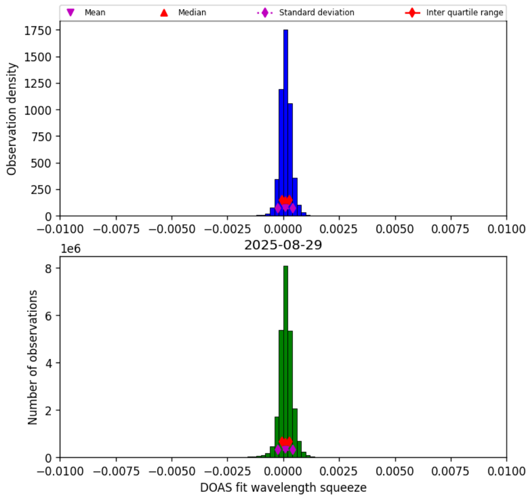
Figure 36: Histogram of “DOAS fit wavelength squeeze” for 2025-08-29 to 2025-08-30
