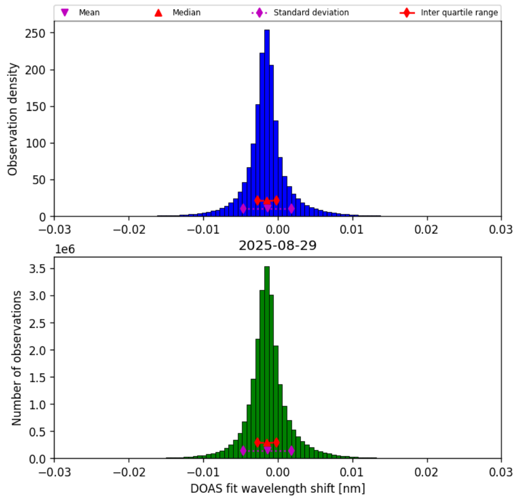
Figure 35: Histogram of “DOAS fit wavelength shift” for 2025-08-29 to 2025-08-30
