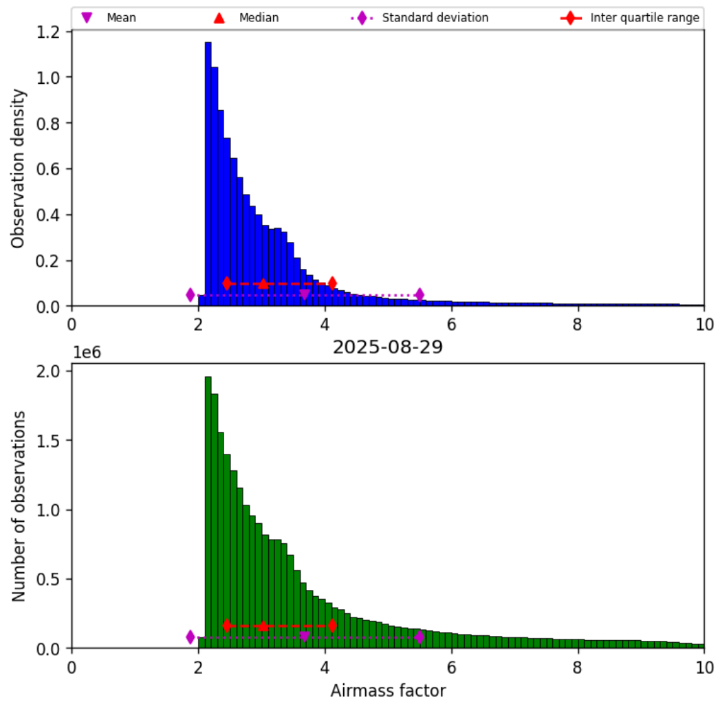
Figure 37: Histogram of “Airmass factor” for 2025-08-29 to 2025-08-30
