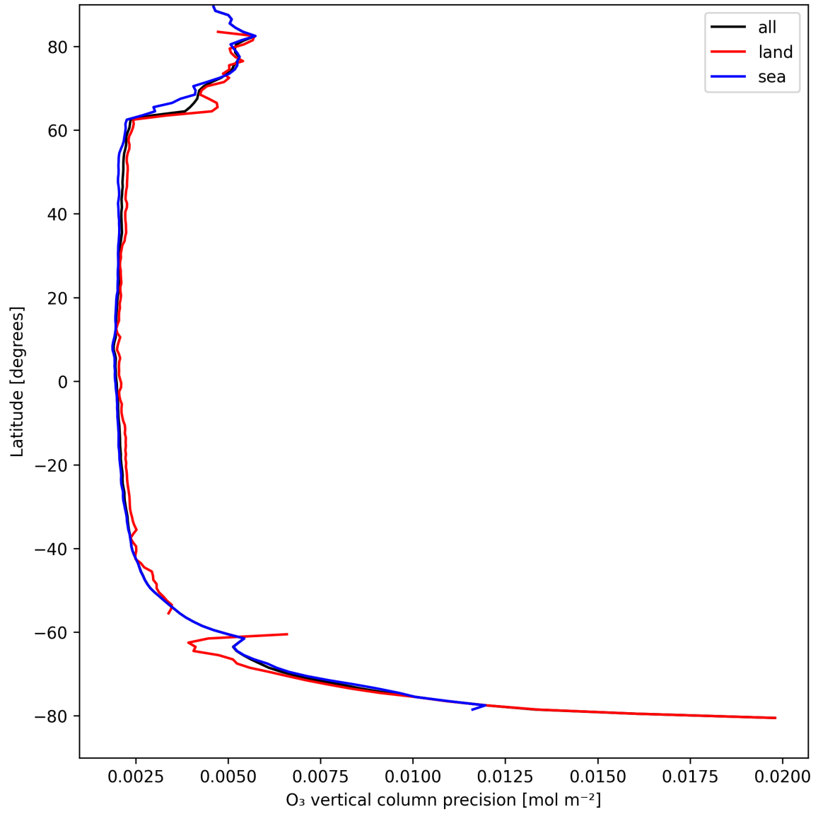
Figure 18: Zonal average of “O 3 vertical column precision” for 2025-08-29 to 2025-08-30.
