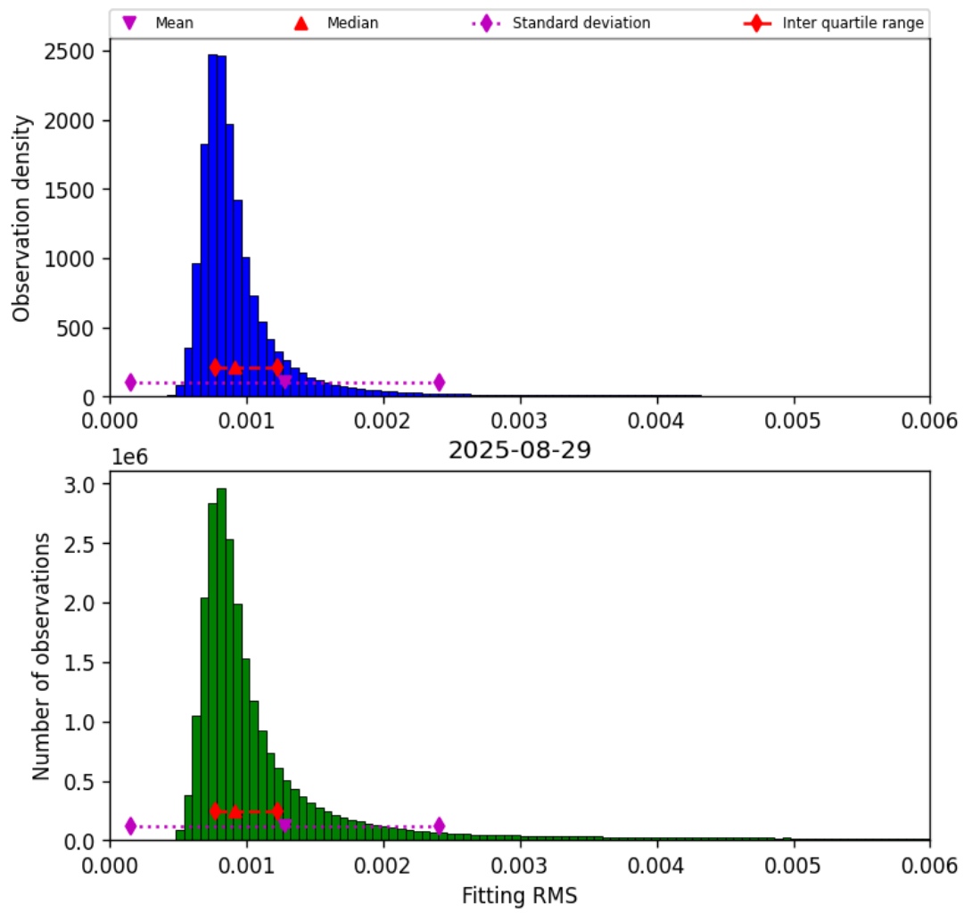
Figure 34: Histogram of “Fitting RMS” for 2025-08-29 to 2025-08-30
