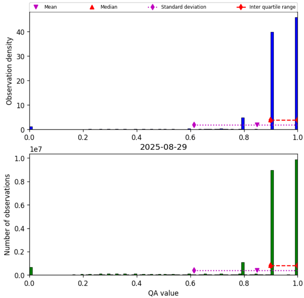
Figure 28: Histogram of “QA value” for 2025-08-29 to 2025-08-30
