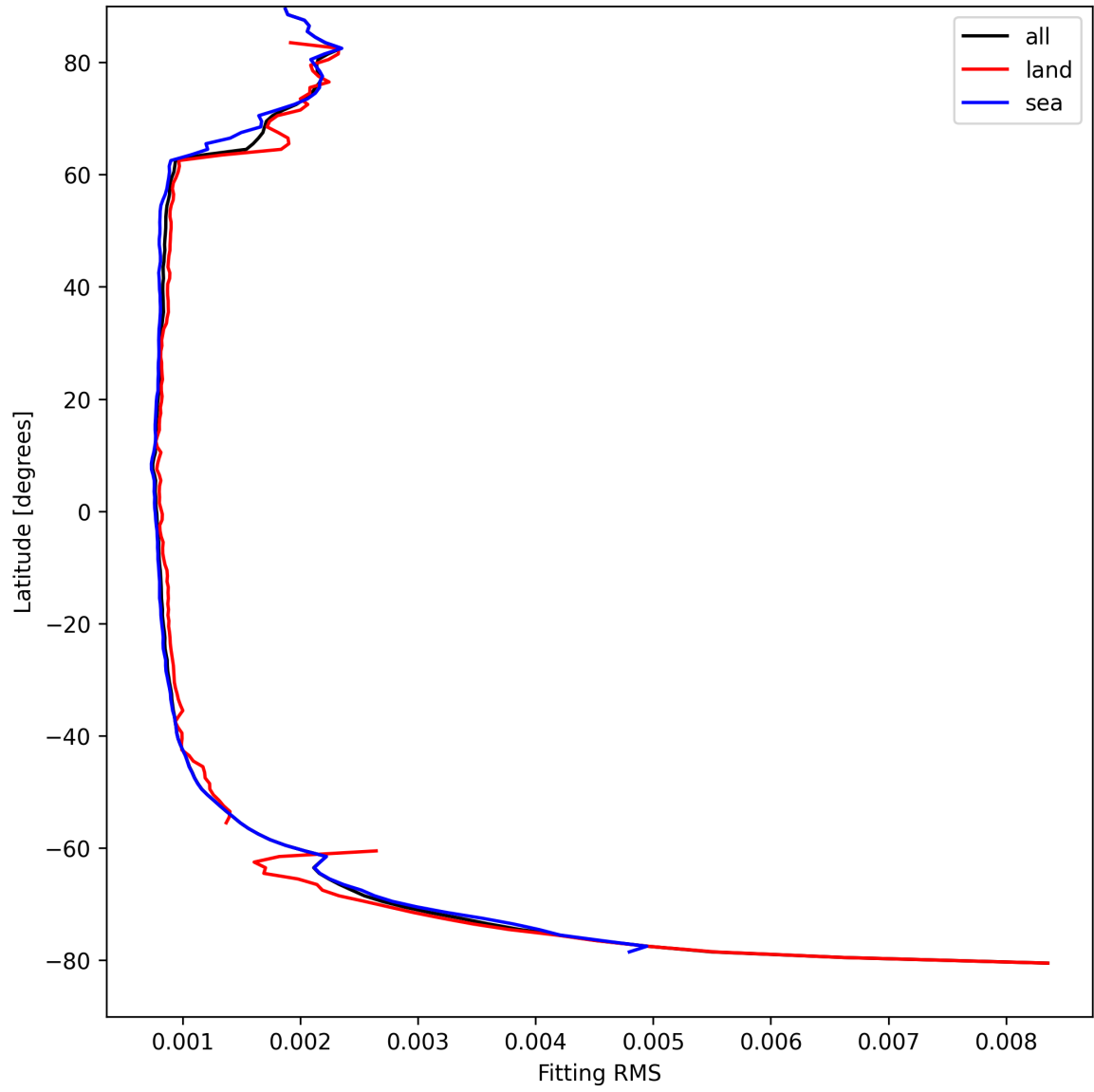
Figure 22: Zonal average of “Fitting RMS” for 2025-08-29 to 2025-08-30.
