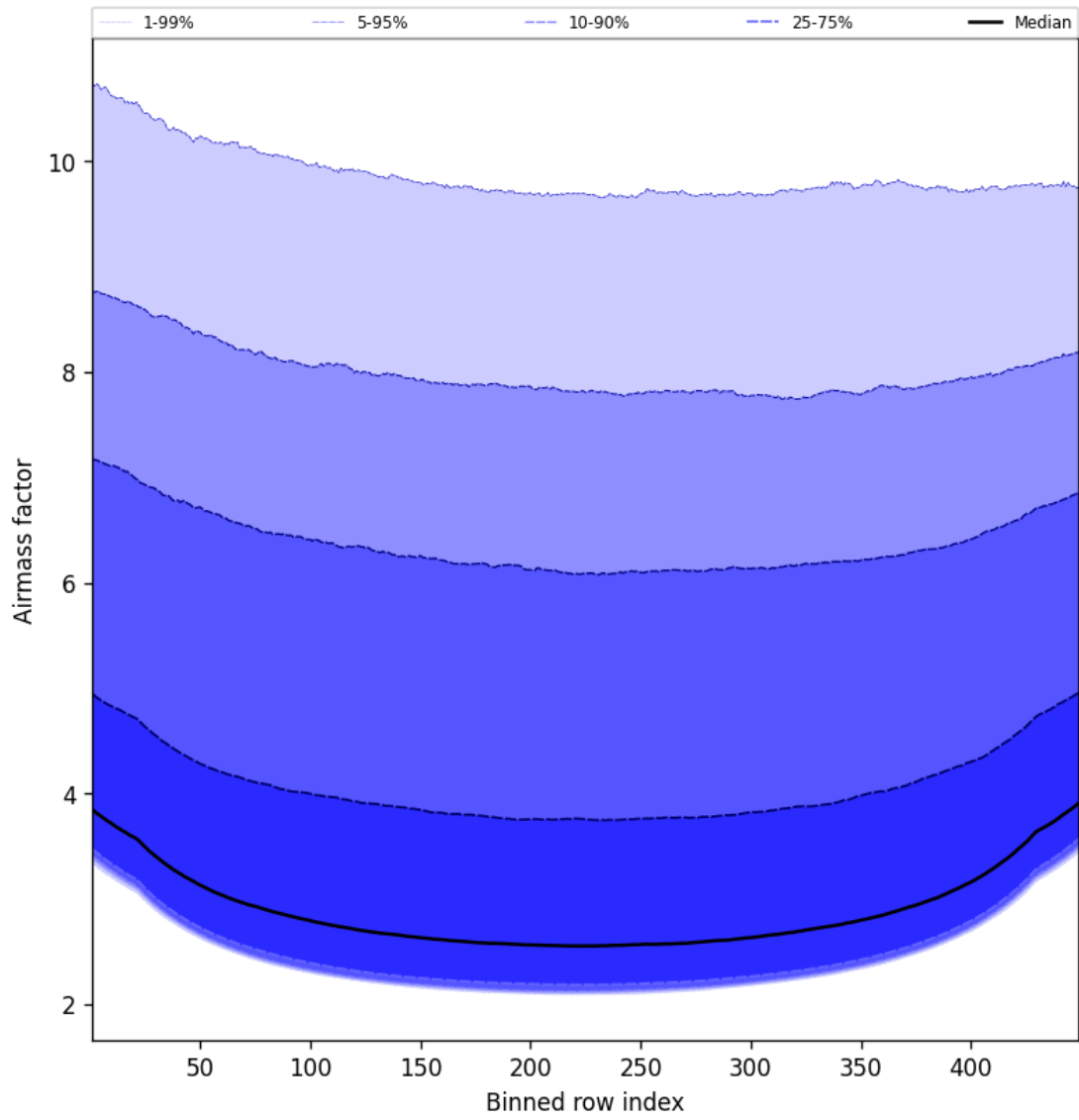
Figure 49: Along track statistics of “Airmass factor” for 2025-08-29 to 2025-08-30
