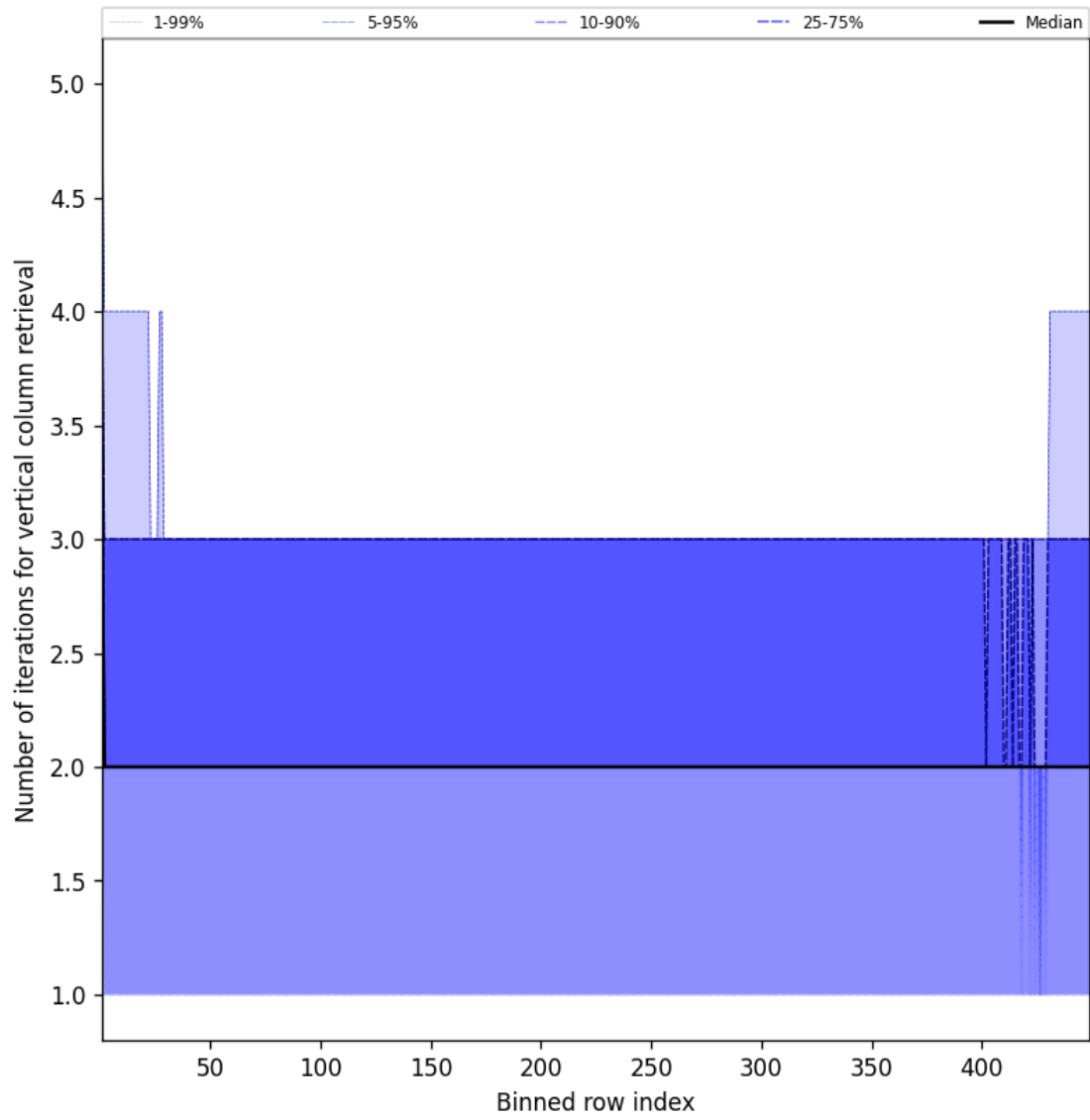
Figure 51: Along track statistics of “Number of iterations for vertical column retrieval” for 2025-08-29 to 2025-08-30
