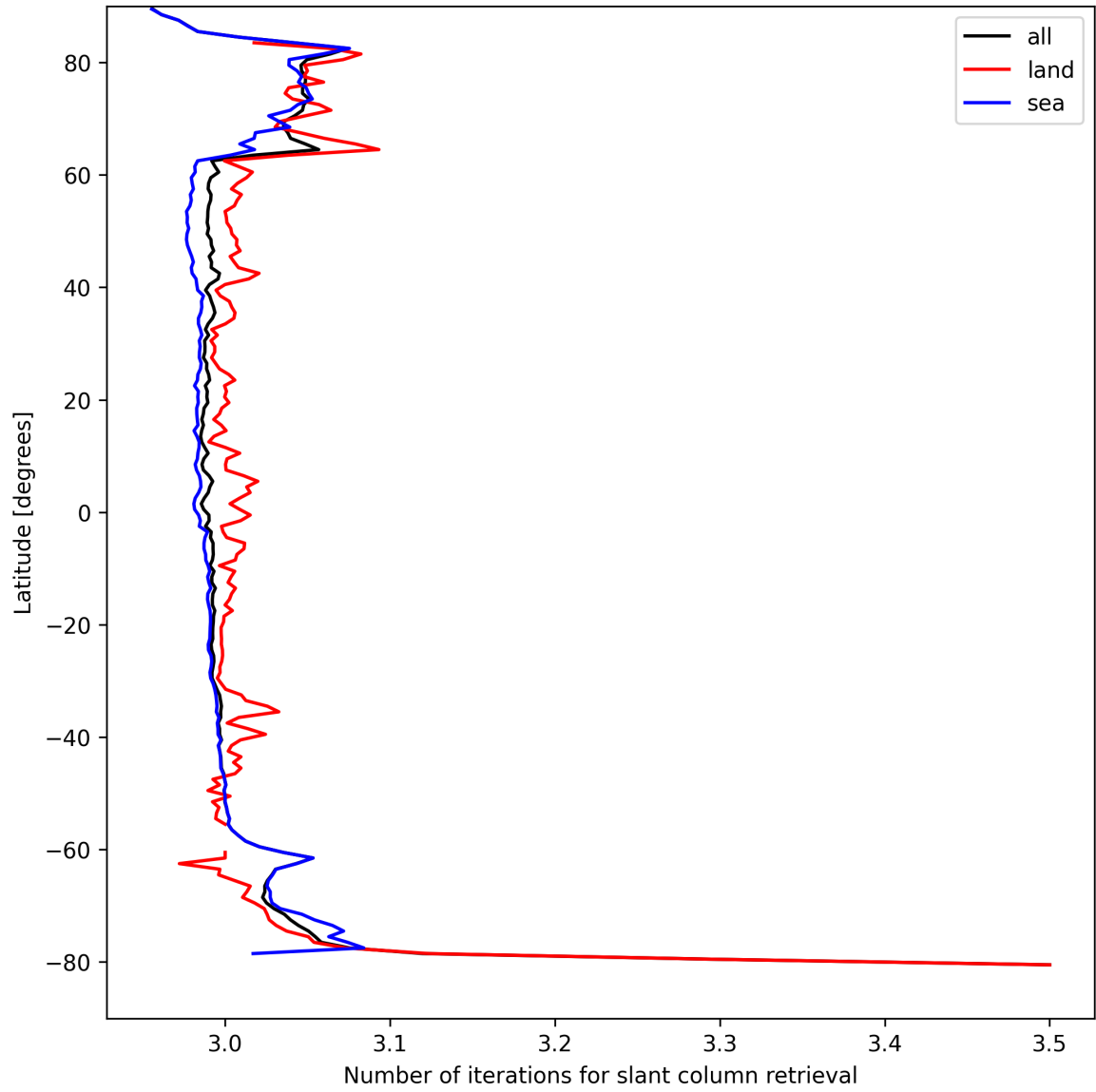
Figure 21: Zonal average of “Number of iterations for slant column retrieval” for 2025-08-29 to 2025-08-30.
