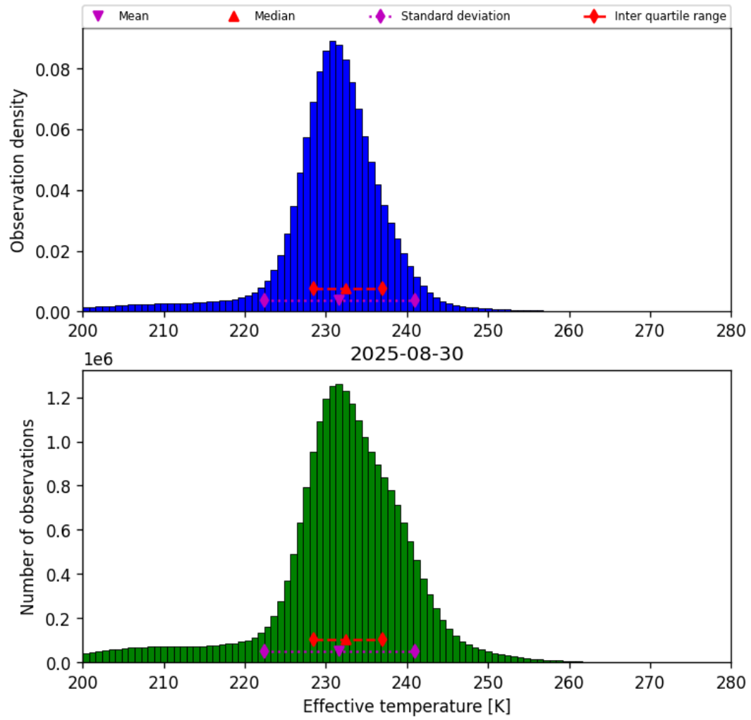
Figure 38: Histogram of “Effective temperature” for 2025-08-30 to 2025-08-31
