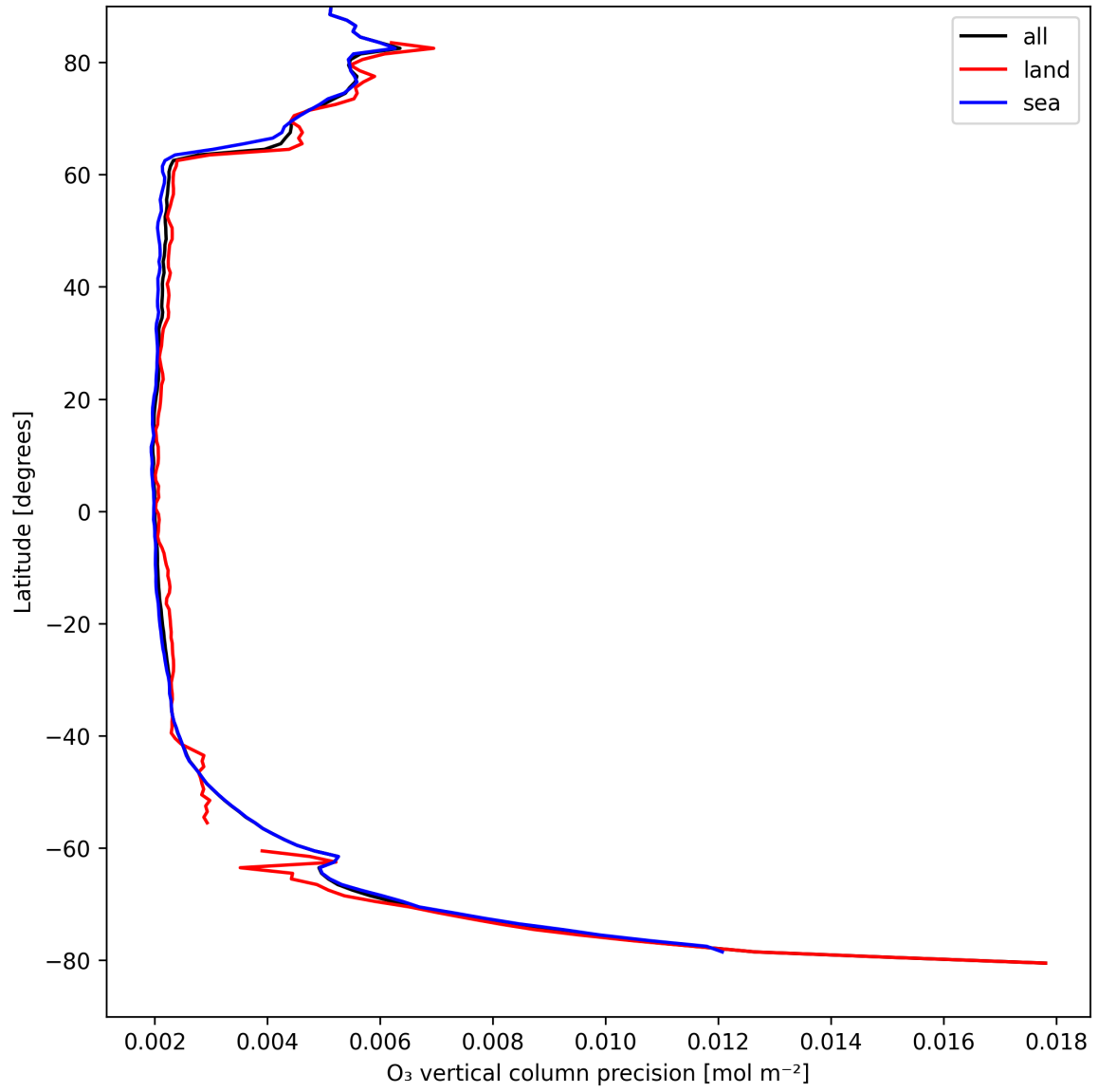
Figure 18: Zonal average of “O 3 vertical column precision” for 2025-08-30 to 2025-08-31.
