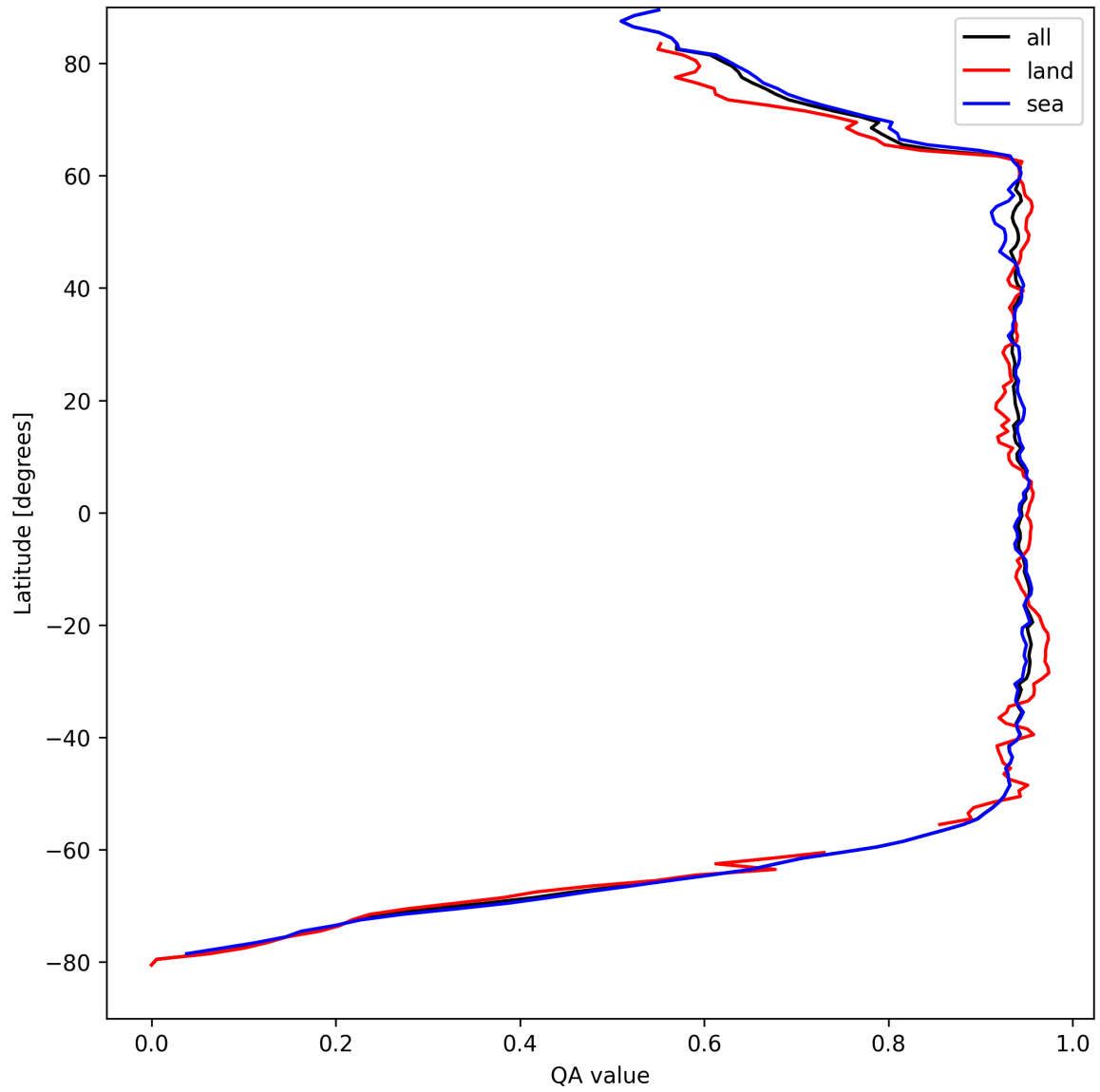
Figure 16: Zonal average of “QA value” for 2025-08-30 to 2025-08-31.
