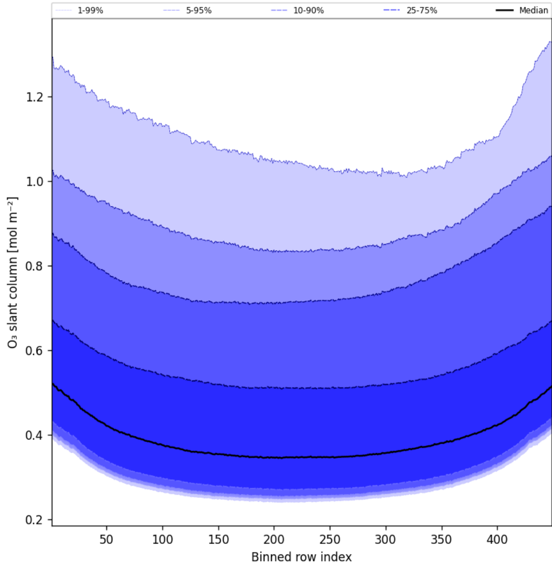
Figure 43: Along track statistics of “O 3 slant column” for 2025-08-30 to 2025-08-31
