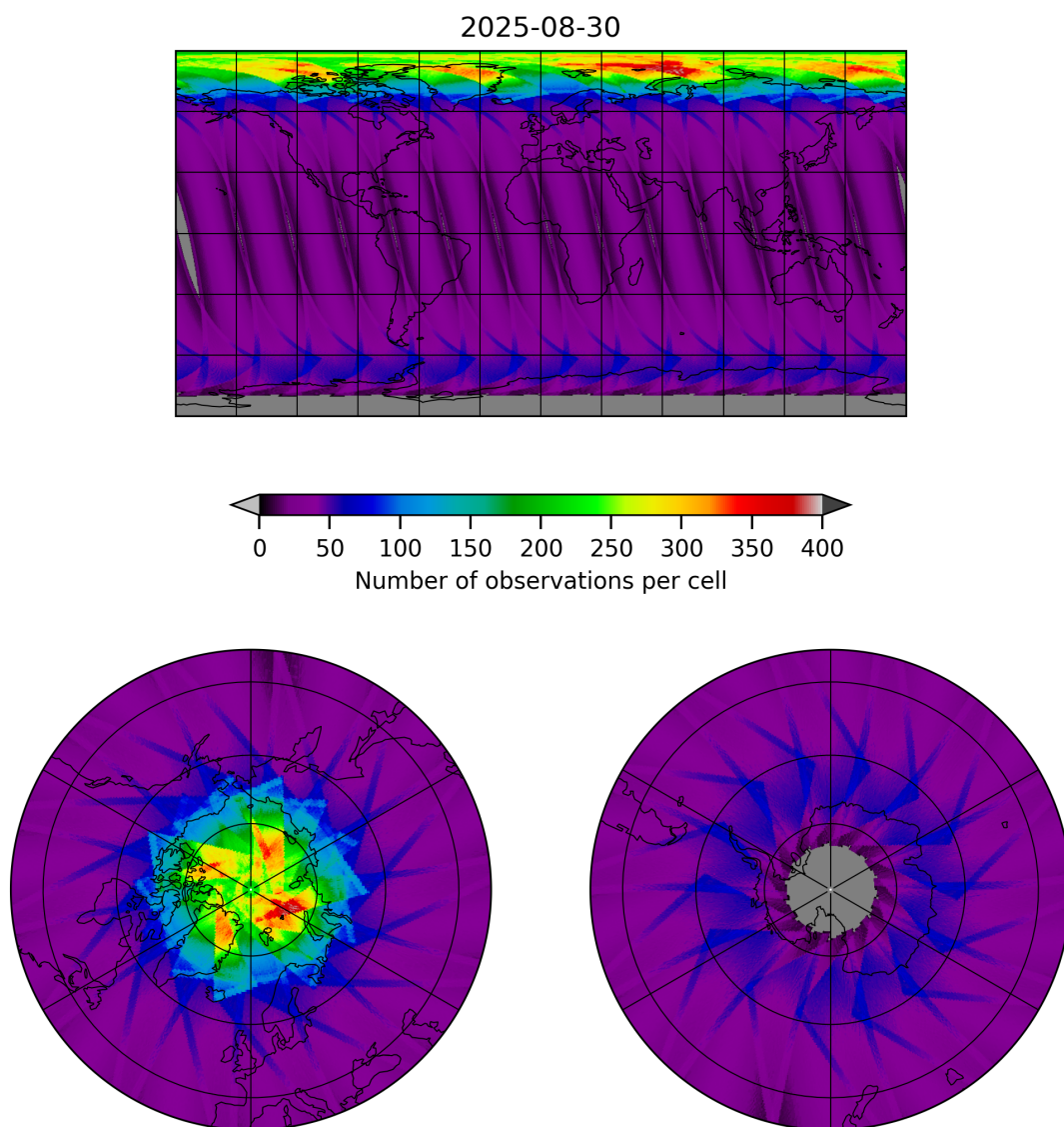
Figure 15: Map of the number of observations for 2025-08-30 to 2025-08-31
