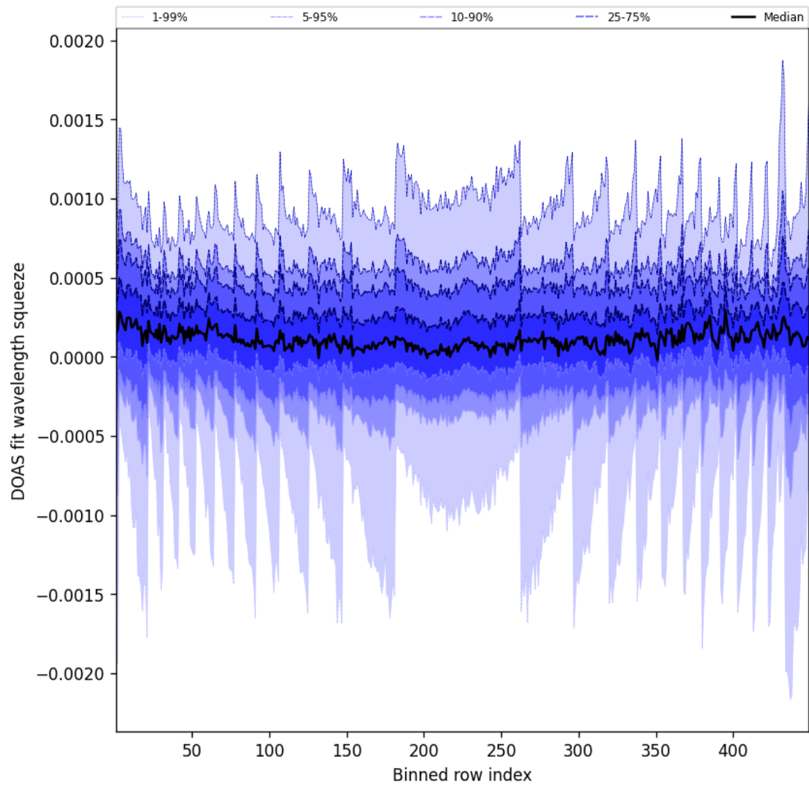
Figure 48: Along track statistics of “DOAS fit wavelength squeeze” for 2025-08-30 to 2025-08-31
