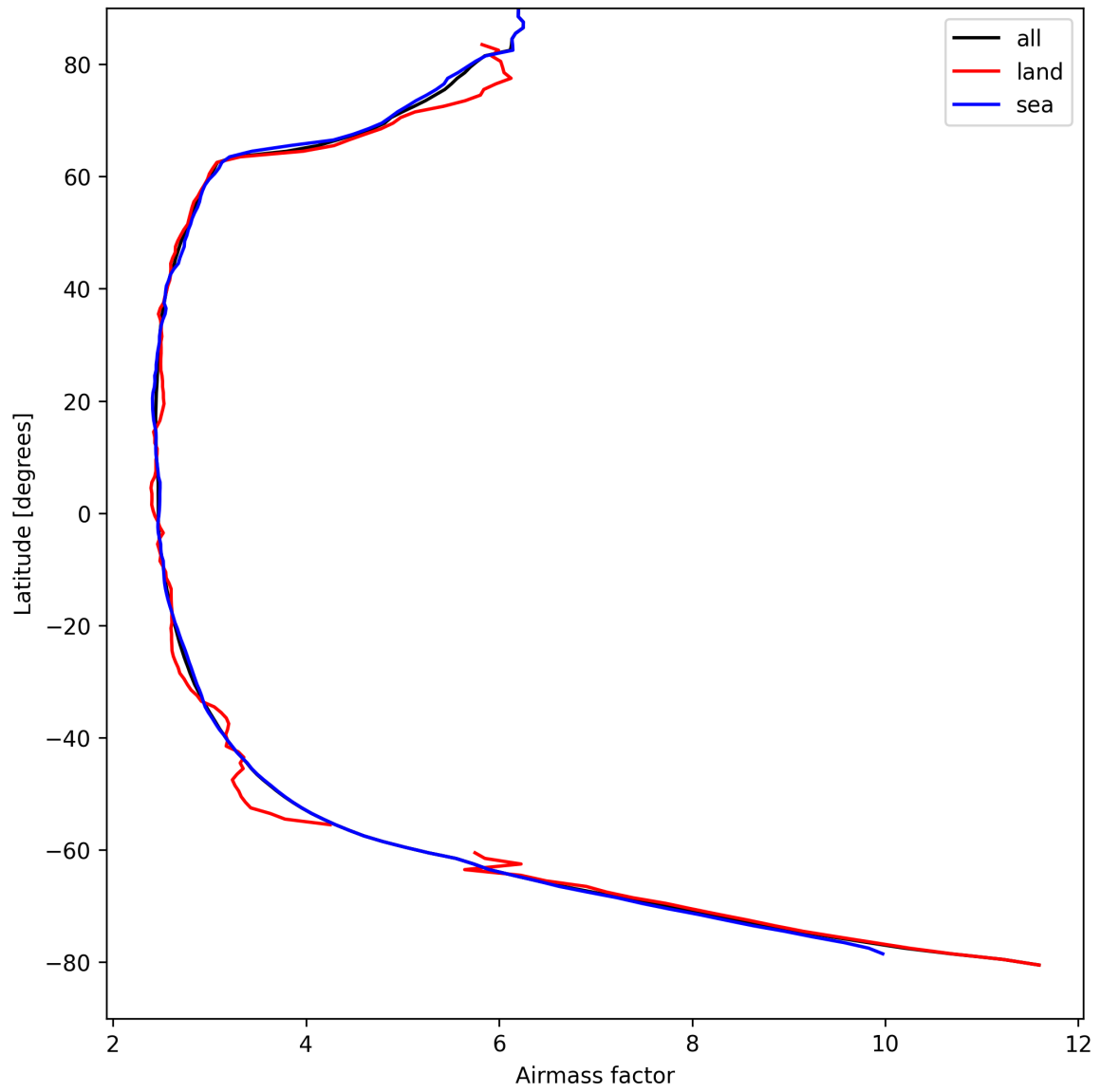
Figure 25: Zonal average of “Airmass factor” for 2025-08-30 to 2025-08-31.
