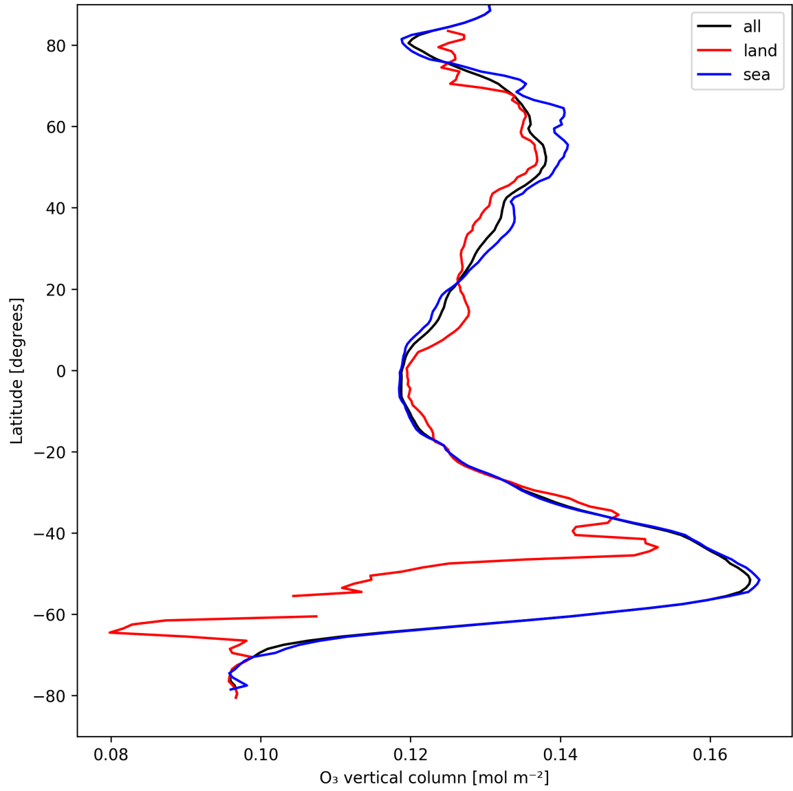
Figure 17: Zonal average of “O 3 vertical column” for 2025-08-30 to 2025-08-31.
