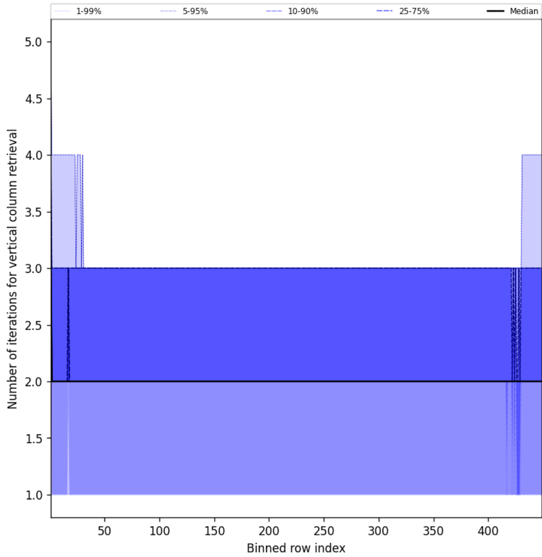
Figure 51: Along track statistics of “Number of iterations for vertical column retrieval” for 2025-08-30 to 2025-08-31
