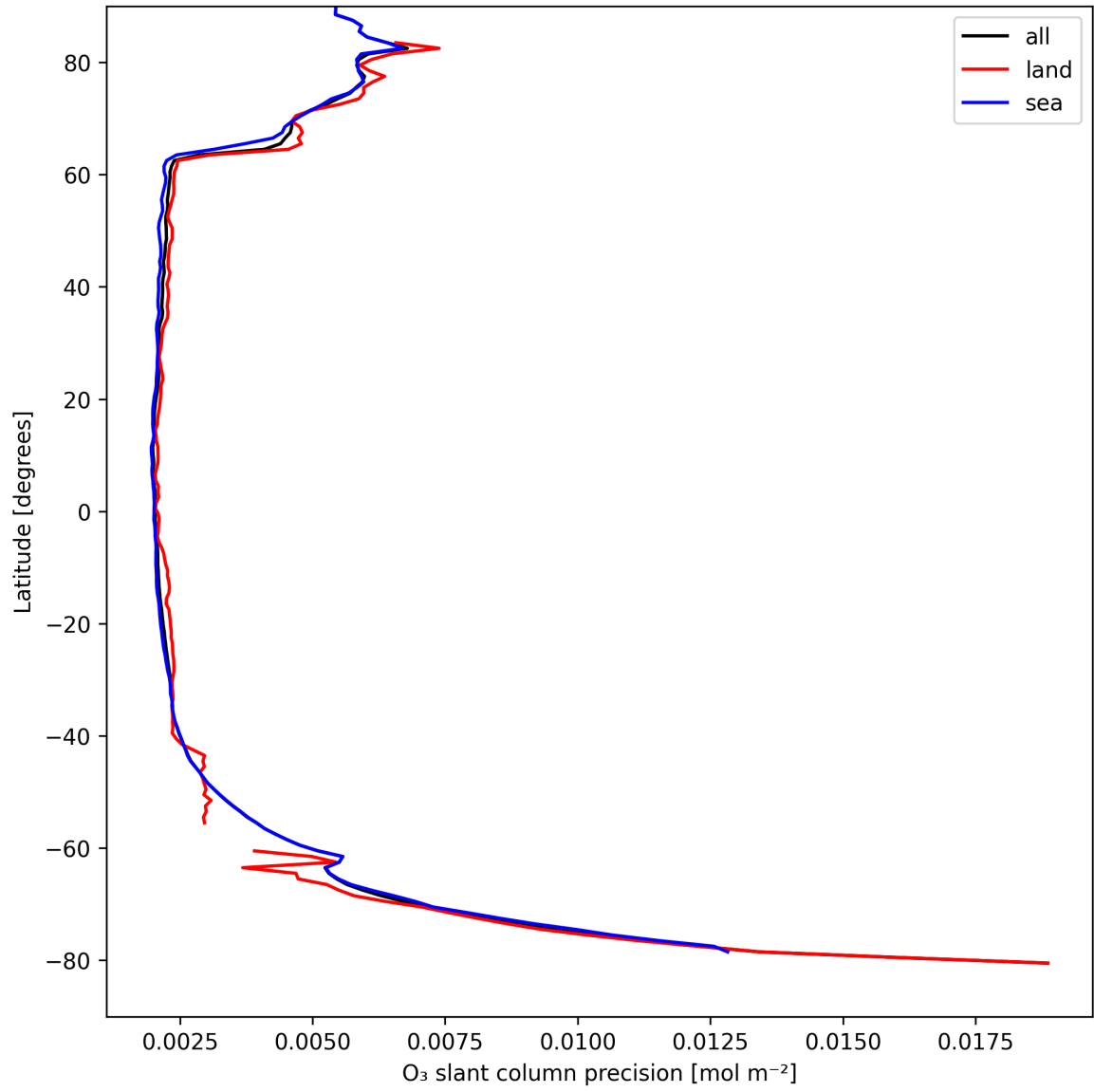
Figure 20: Zonal average of “O 3 slant column precision” for 2025-08-30 to 2025-08-31.
