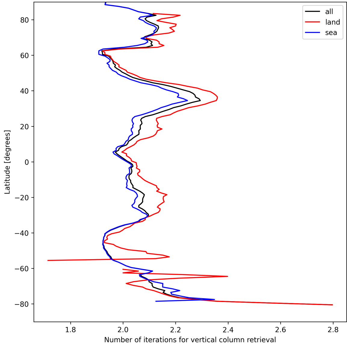
Figure 27: Zonal average of “Number of iterations for vertical column retrieval” for 2025-08-30 to 2025-08-31.
