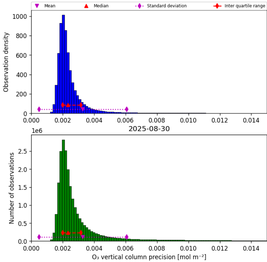
Figure 30: Histogram of “O 3 vertical column precision” for 2025-08-30 to 2025-08-31
