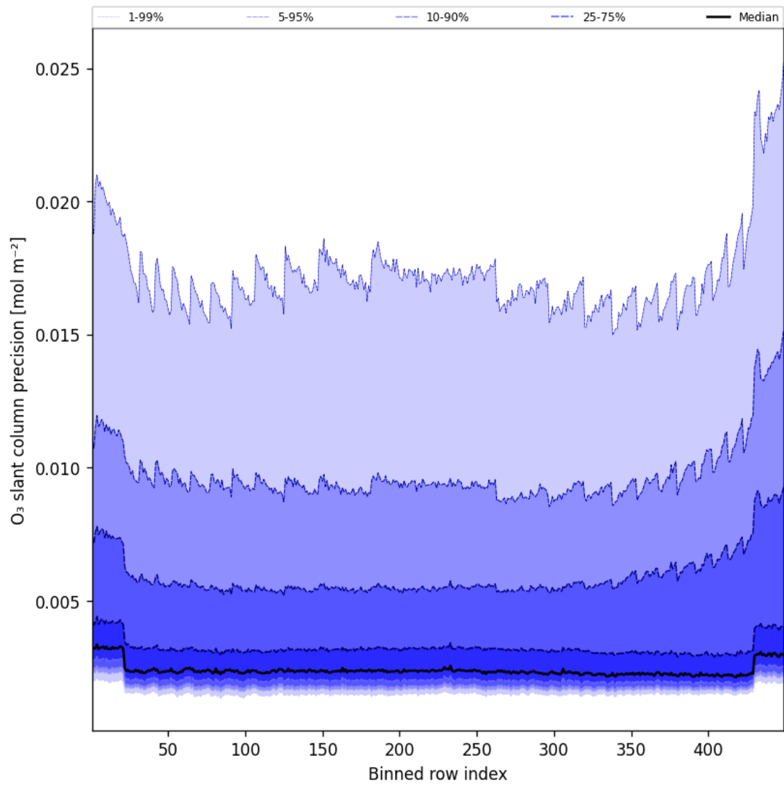
Figure 44: Along track statistics of “O 3 slant column precision” for 2025-08-30 to 2025-08-31
