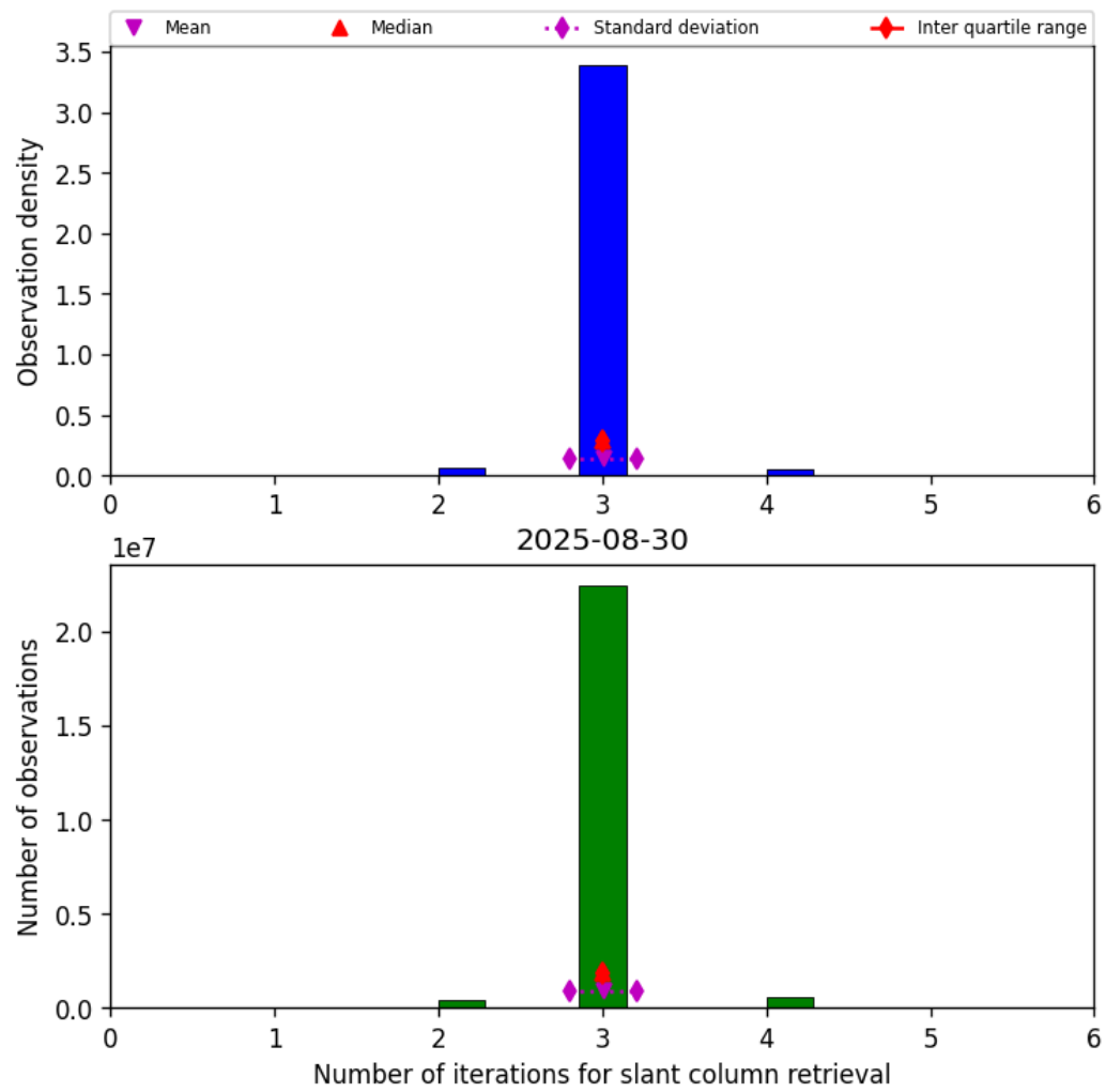
Figure 33: Histogram of “Number of iterations for slant column retrieval” for 2025-08-30 to 2025-08-31
