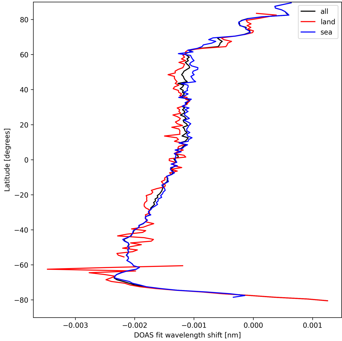
Figure 23: Zonal average of “DOAS fit wavelength shift” for 2025-08-30 to 2025-08-31.
