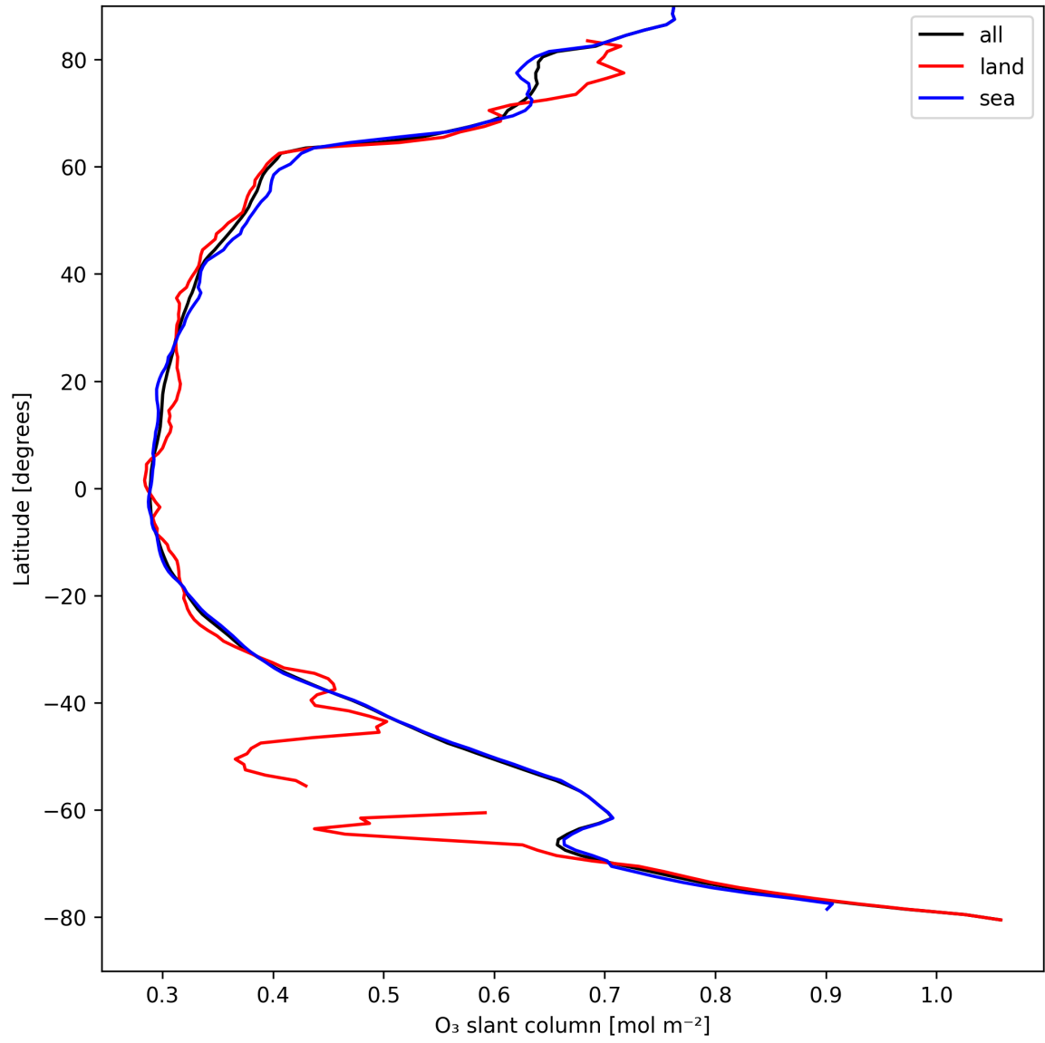
Figure 19: Zonal average of “O 3 slant column” for 2025-08-30 to 2025-08-31.
