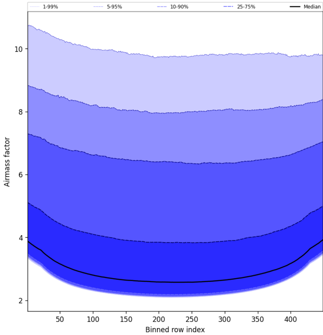
Figure 49: Along track statistics of “Airmass factor” for 2025-08-30 to 2025-08-31
