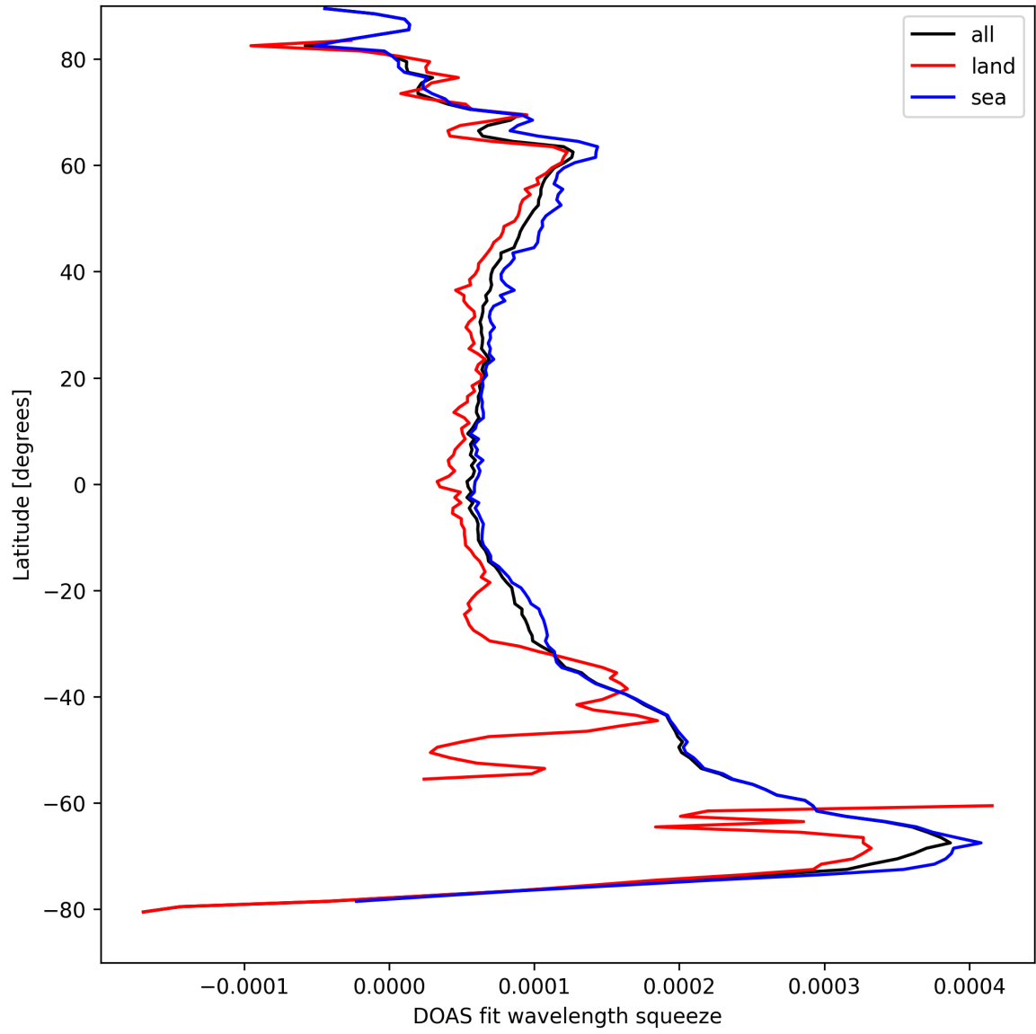
Figure 24: Zonal average of “DOAS fit wavelength squeeze” for 2025-08-30 to 2025-08-31.
