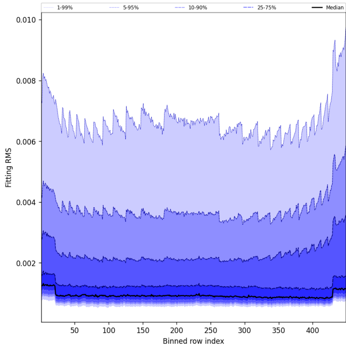
Figure 46: Along track statistics of “Fitting RMS” for 2025-08-30 to 2025-08-31
