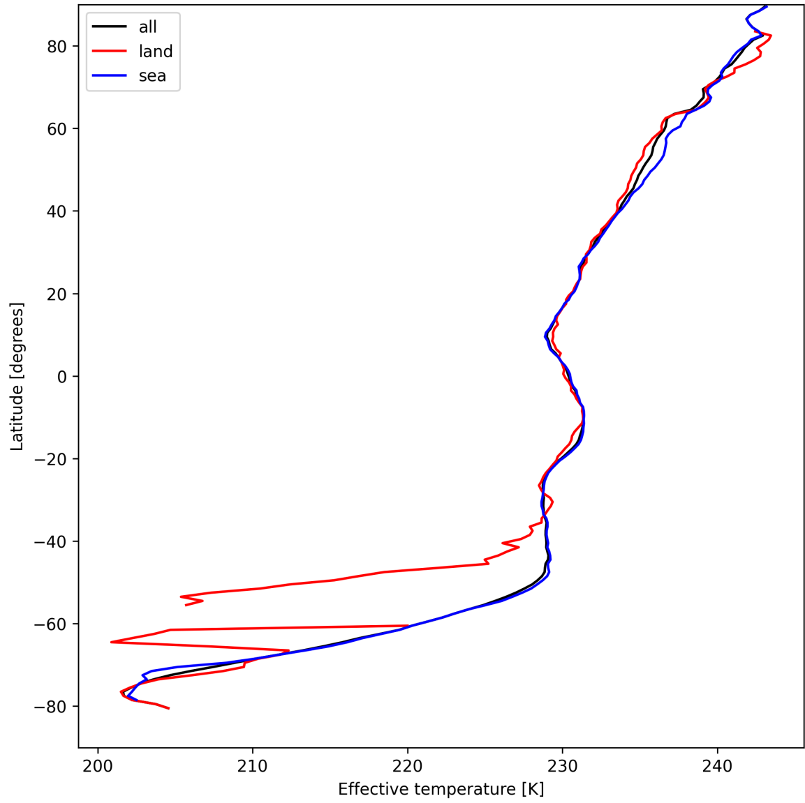
Figure 26: Zonal average of “Effective temperature” for 2025-08-30 to 2025-08-31.
