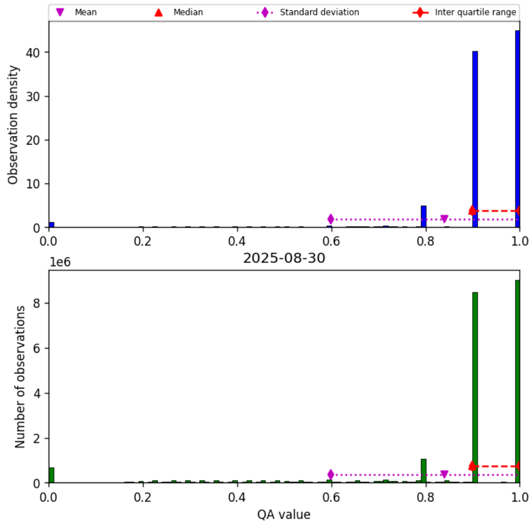
Figure 28: Histogram of “QA value” for 2025-08-30 to 2025-08-31
