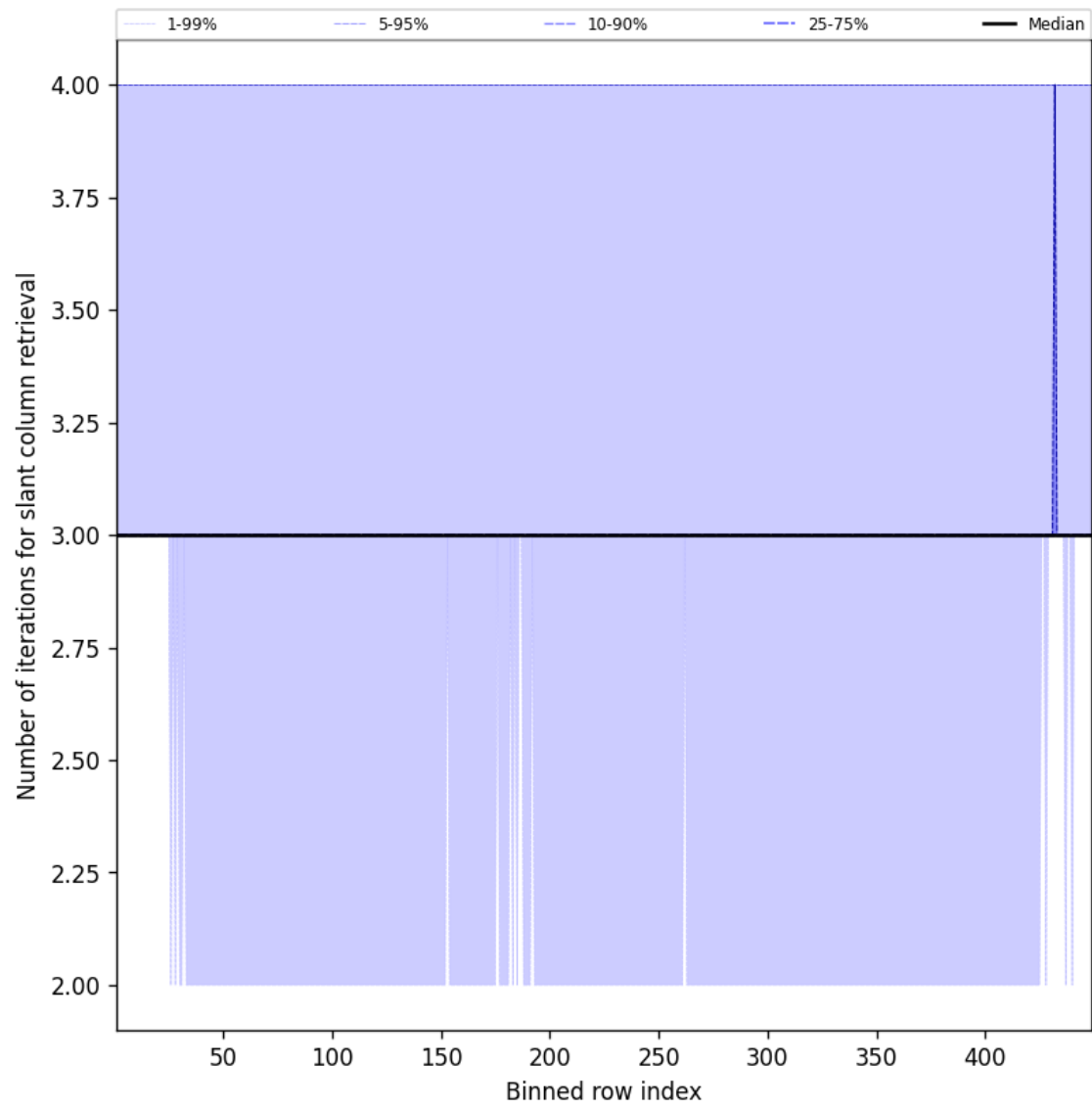
Figure 45: Along track statistics of “Number of iterations for slant column retrieval” for 2025-08-30 to 2025-08-31
