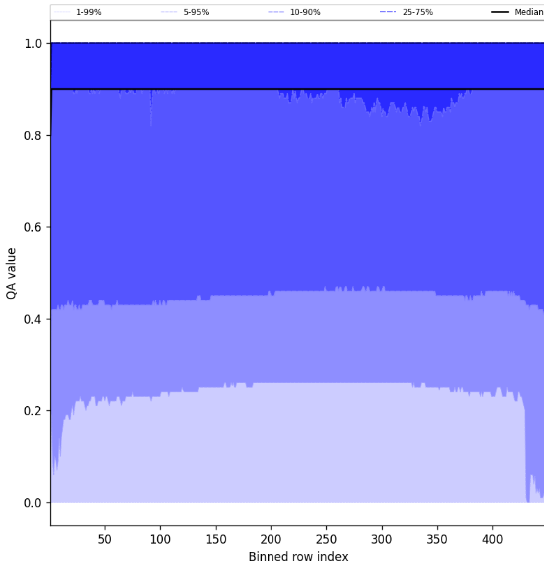
Figure 40: Along track statistics of “QA value” for 2025-08-30 to 2025-08-31
