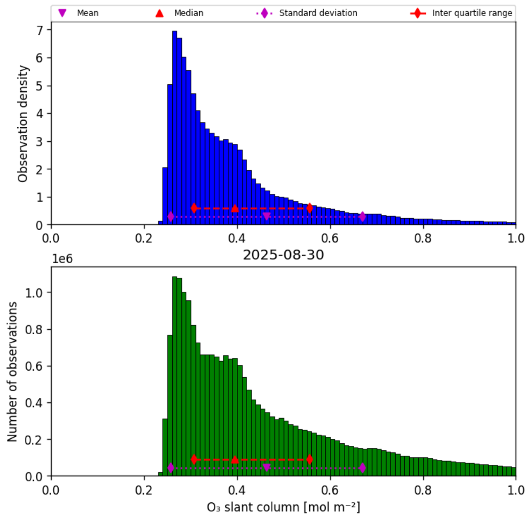
Figure 31: Histogram of “O 3 slant column” for 2025-08-30 to 2025-08-31
