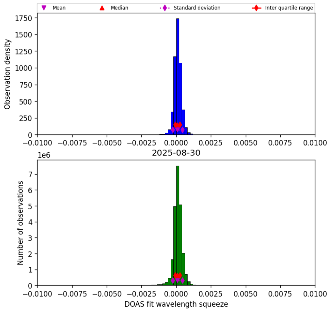
Figure 36: Histogram of “DOAS fit wavelength squeeze” for 2025-08-30 to 2025-08-31
