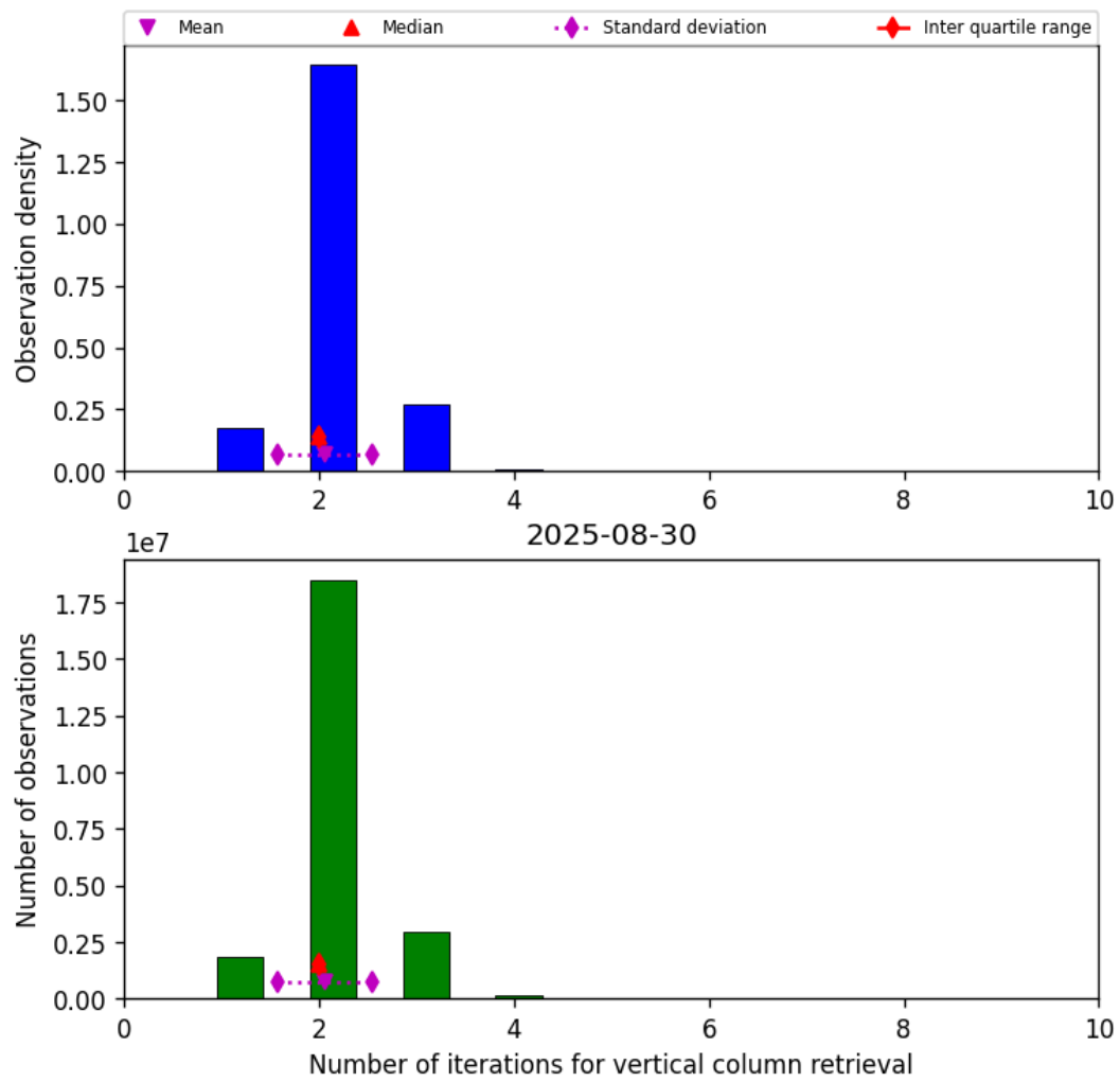
Figure 39: Histogram of “Number of iterations for vertical column retrieval” for 2025-08-30 to 2025-08-31
