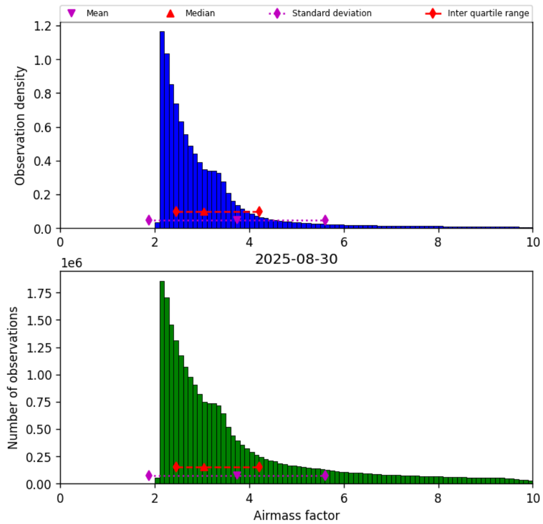
Figure 37: Histogram of “Airmass factor” for 2025-08-30 to 2025-08-31
