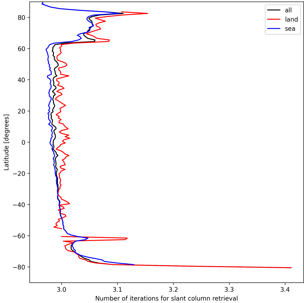
Figure 21: Zonal average of “Number of iterations for slant column retrieval” for 2025-08-30 to 2025-08-31.
