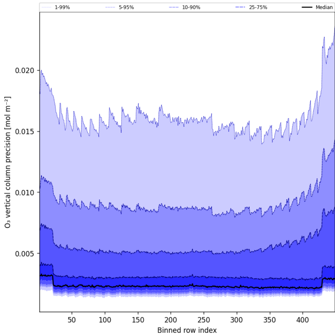
Figure 42: Along track statistics of “O 3 vertical column precision” for 2025-08-30 to 2025-08-31
