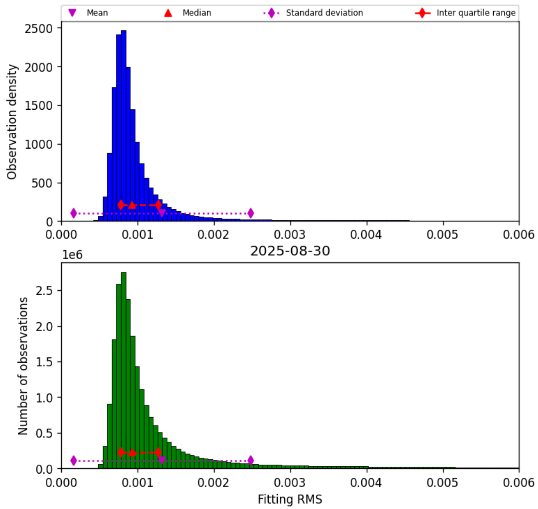
Figure 34: Histogram of “Fitting RMS” for 2025-08-30 to 2025-08-31
