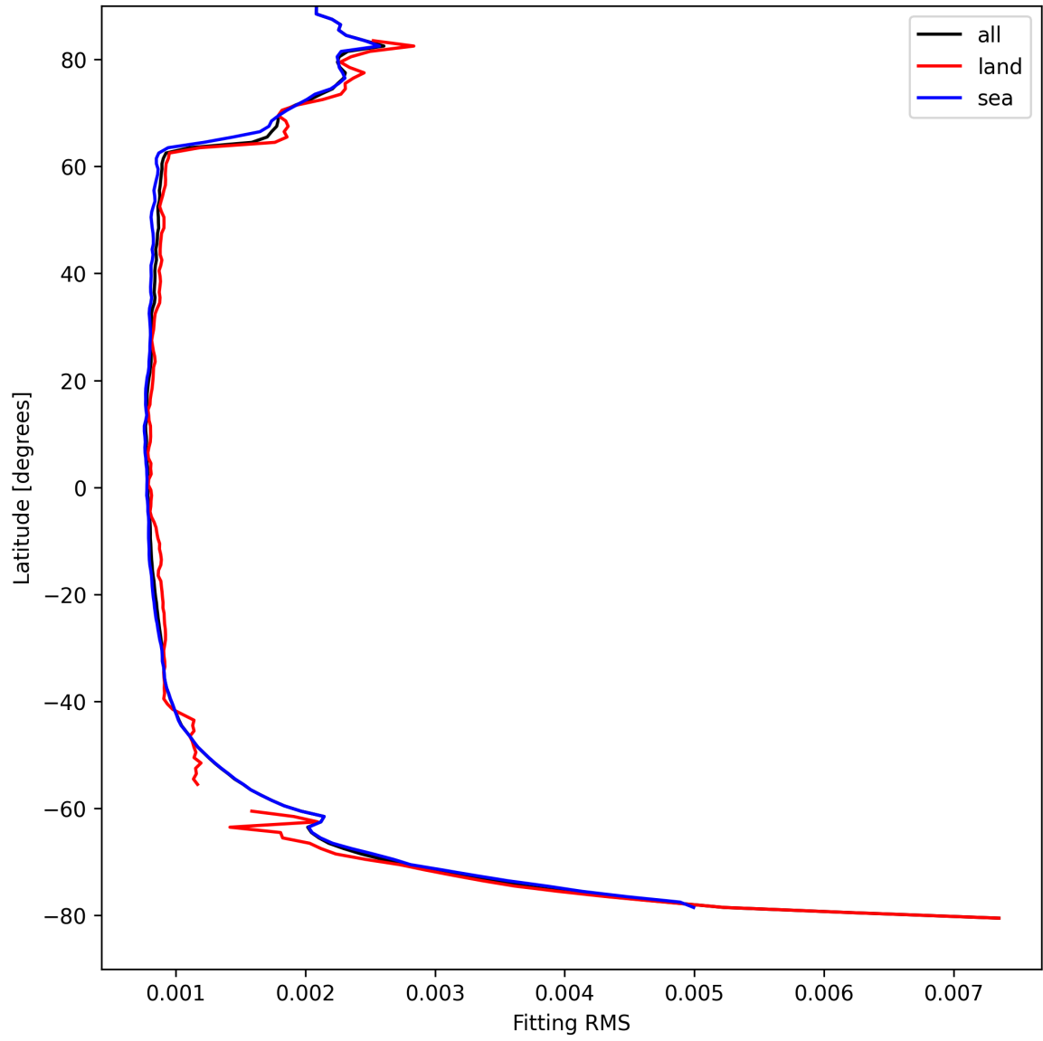
Figure 22: Zonal average of “Fitting RMS” for 2025-08-30 to 2025-08-31.
