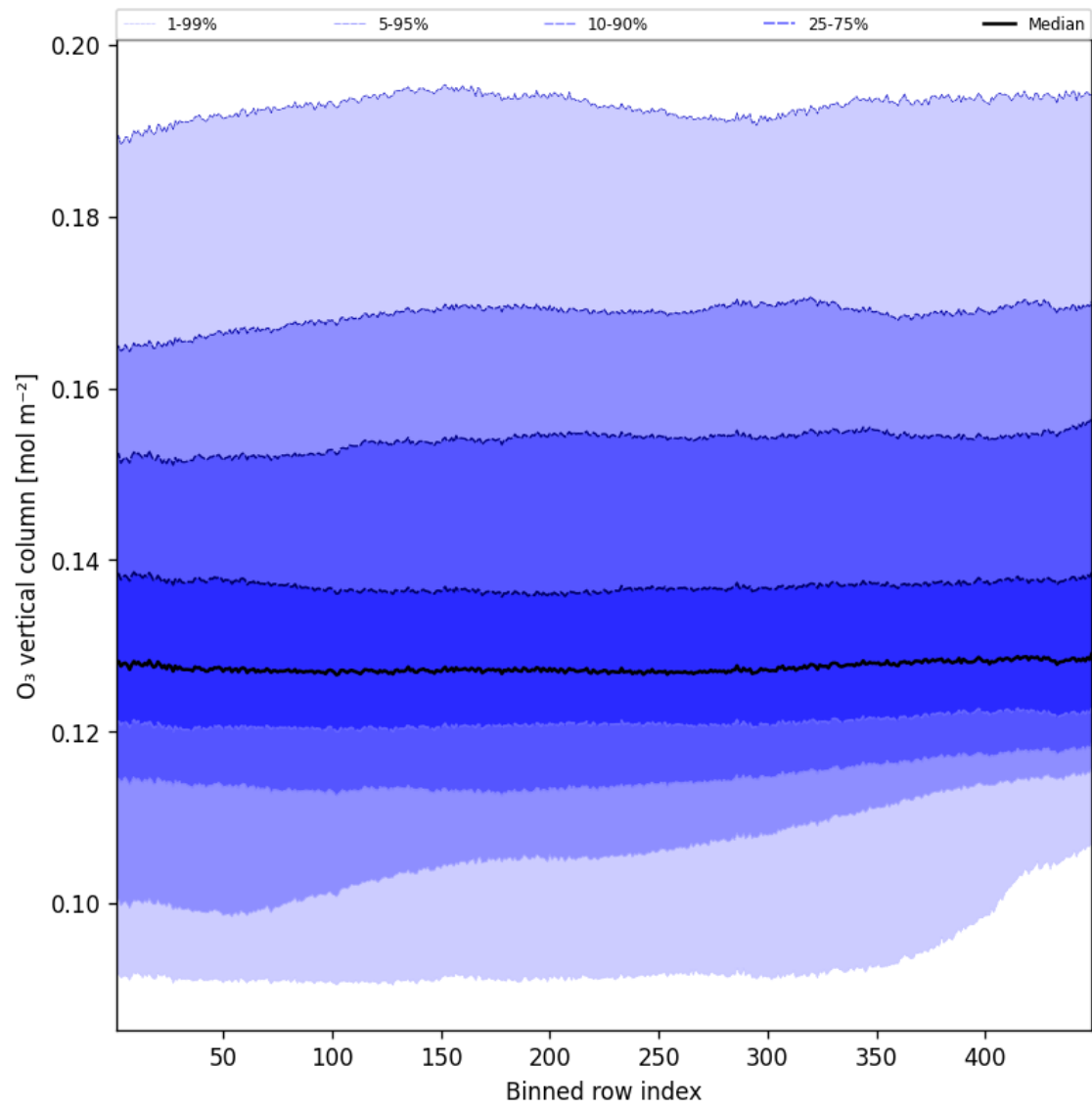
Figure 41: Along track statistics of “O 3 vertical column” for 2025-08-30 to 2025-08-31
