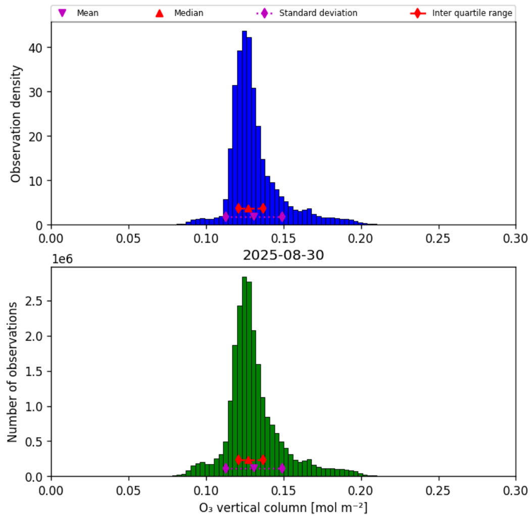
Figure 29: Histogram of “O 3 vertical column” for 2025-08-30 to 2025-08-31
