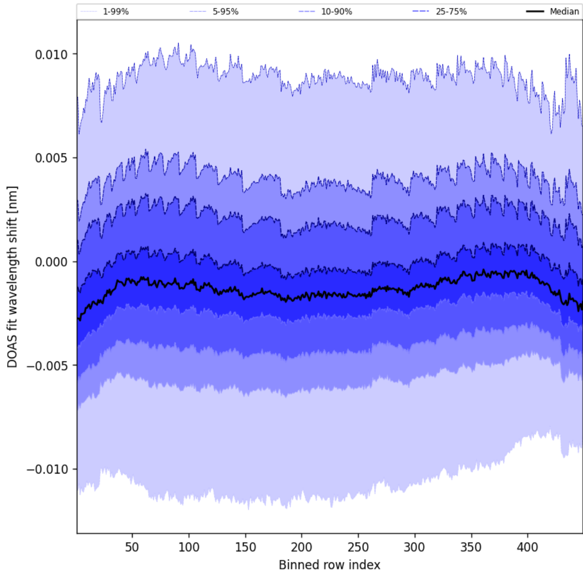
Figure 47: Along track statistics of “DOAS fit wavelength shift” for 2025-08-30 to 2025-08-31
