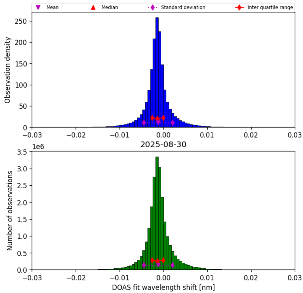
Figure 35: Histogram of “DOAS fit wavelength shift” for 2025-08-30 to 2025-08-31
