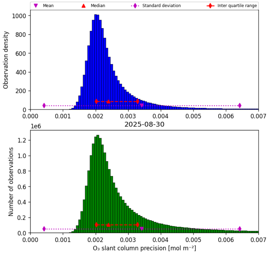
Figure 32: Histogram of “O 3 slant column precision” for 2025-08-30 to 2025-08-31
