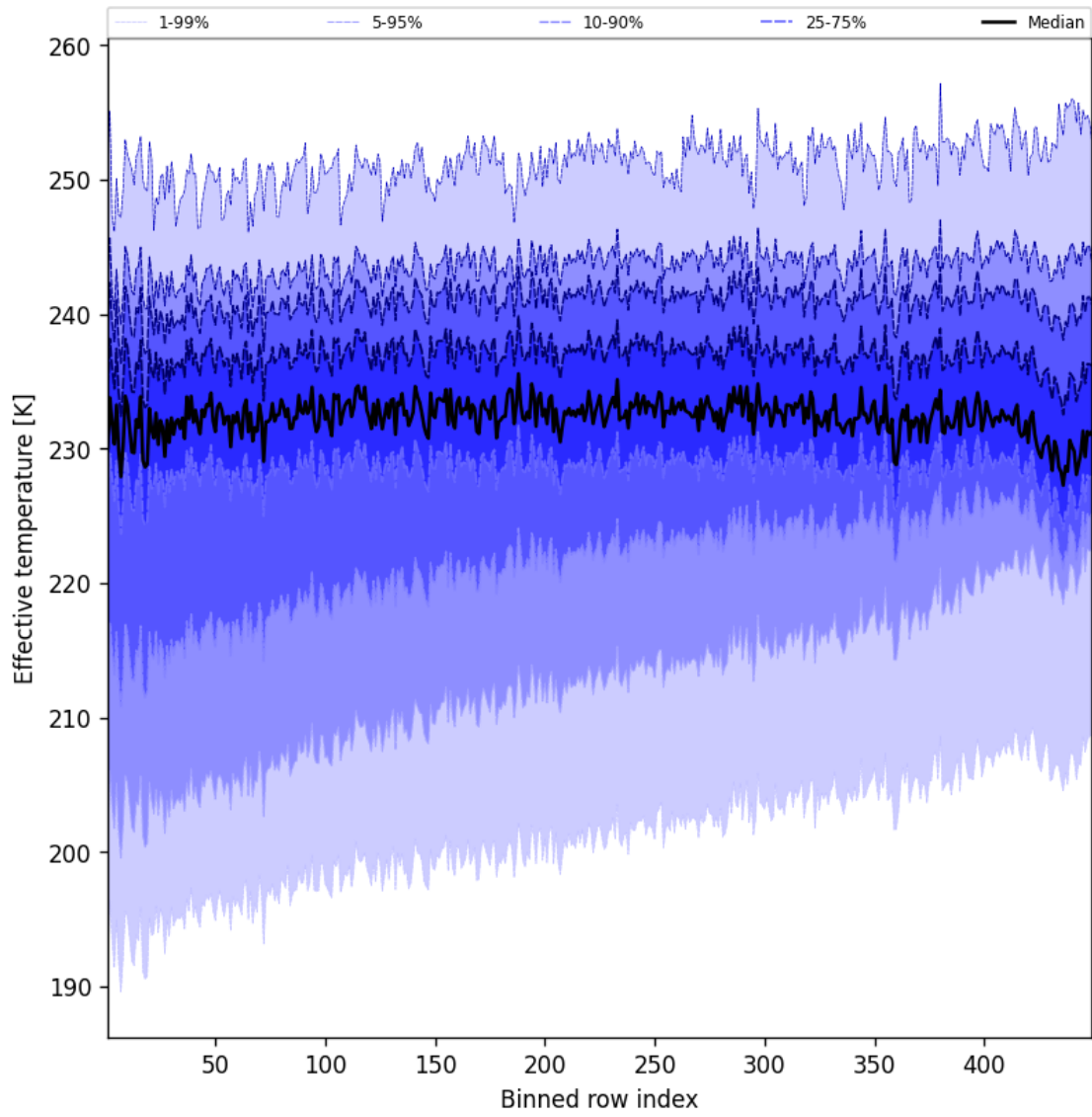
Figure 50: Along track statistics of “Effective temperature” for 2025-08-30 to 2025-08-31
