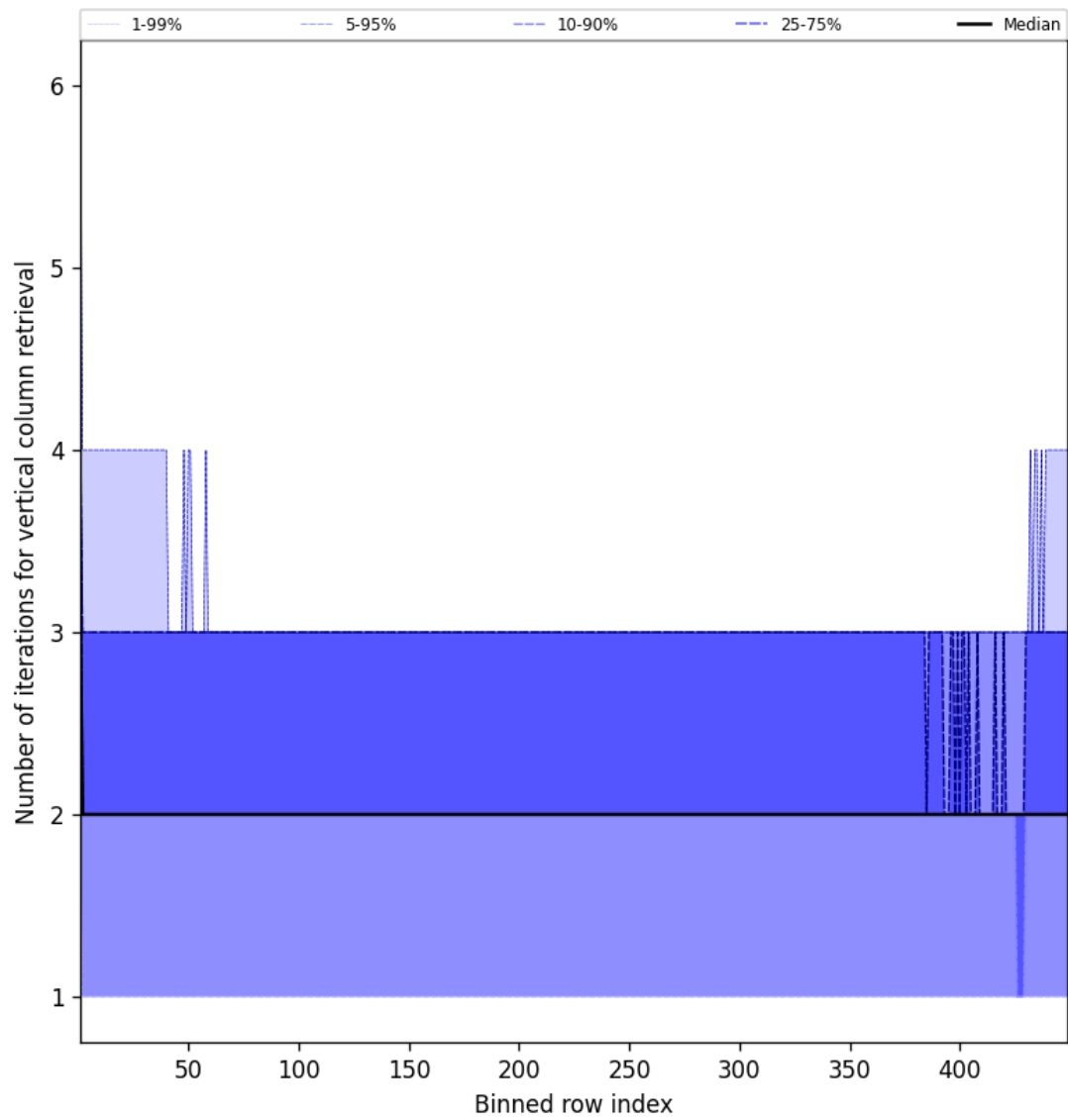
Figure 51: Along track statistics of “Number of iterations for vertical column retrieval” for 2025-08-31 to 2025-09-01
