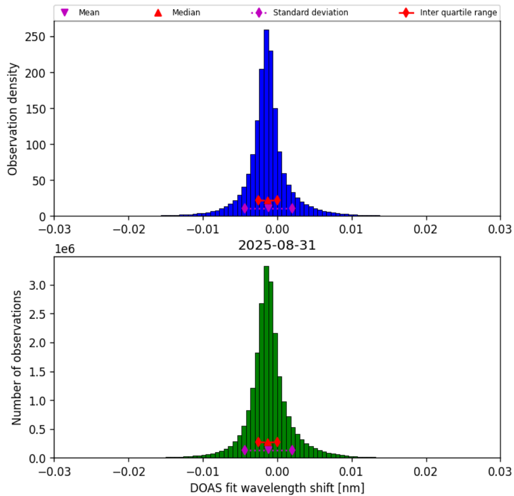
Figure 35: Histogram of “DOAS fit wavelength shift” for 2025-08-31 to 2025-09-01
