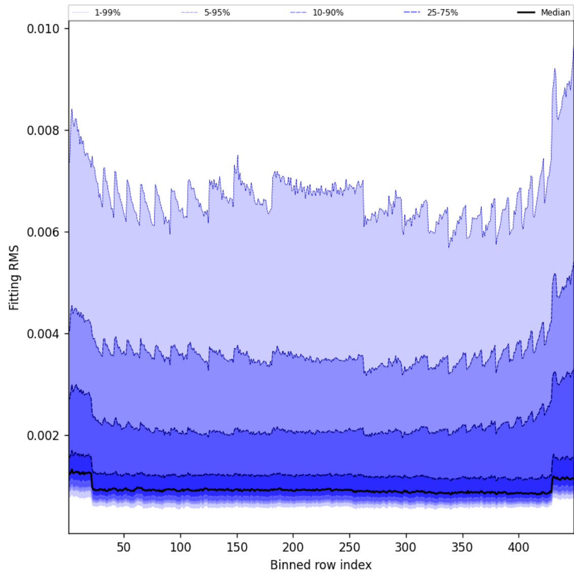
Figure 46: Along track statistics of “Fitting RMS” for 2025-08-31 to 2025-09-01
