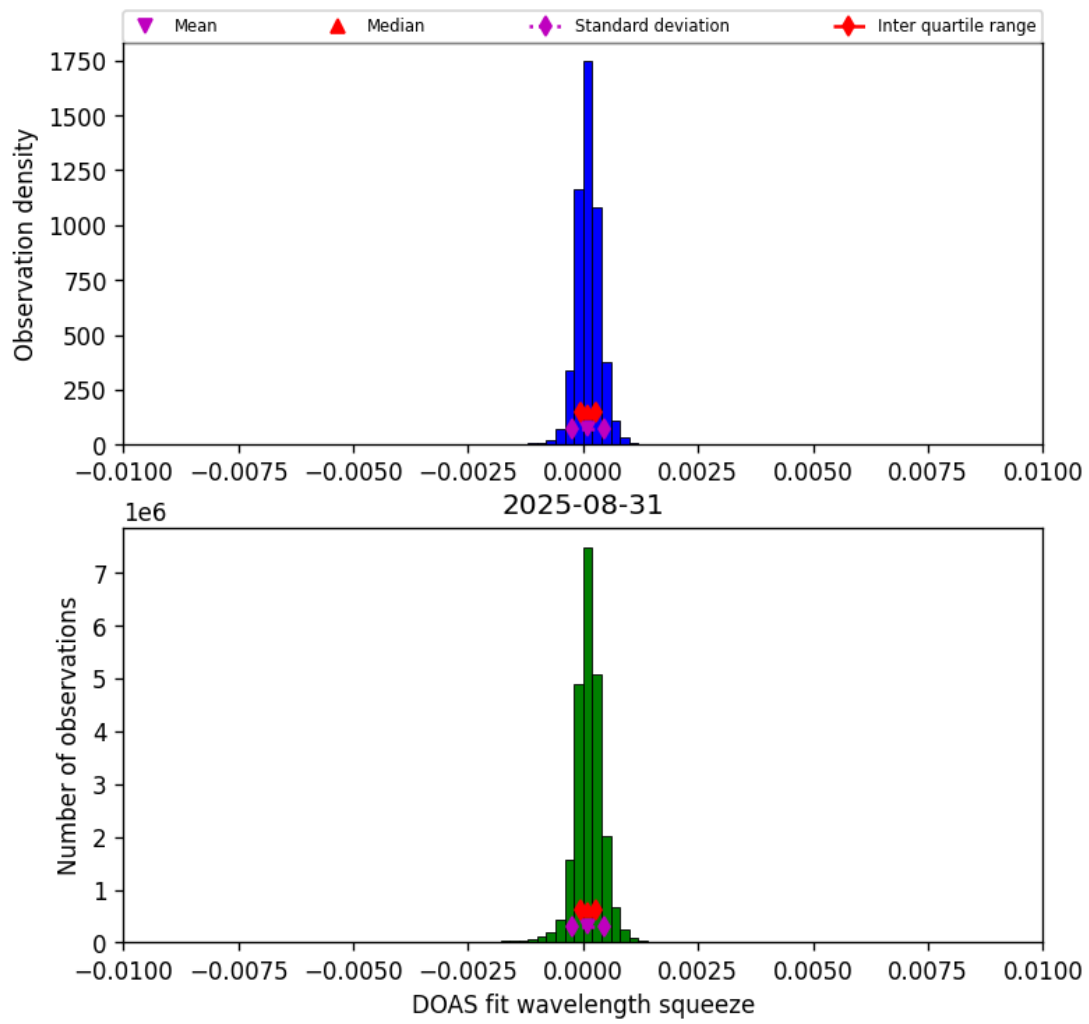
Figure 36: Histogram of “DOAS fit wavelength squeeze” for 2025-08-31 to 2025-09-01
