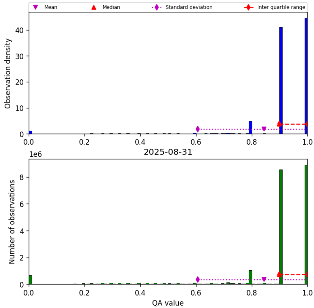
Figure 28: Histogram of “QA value” for 2025-08-31 to 2025-09-01
