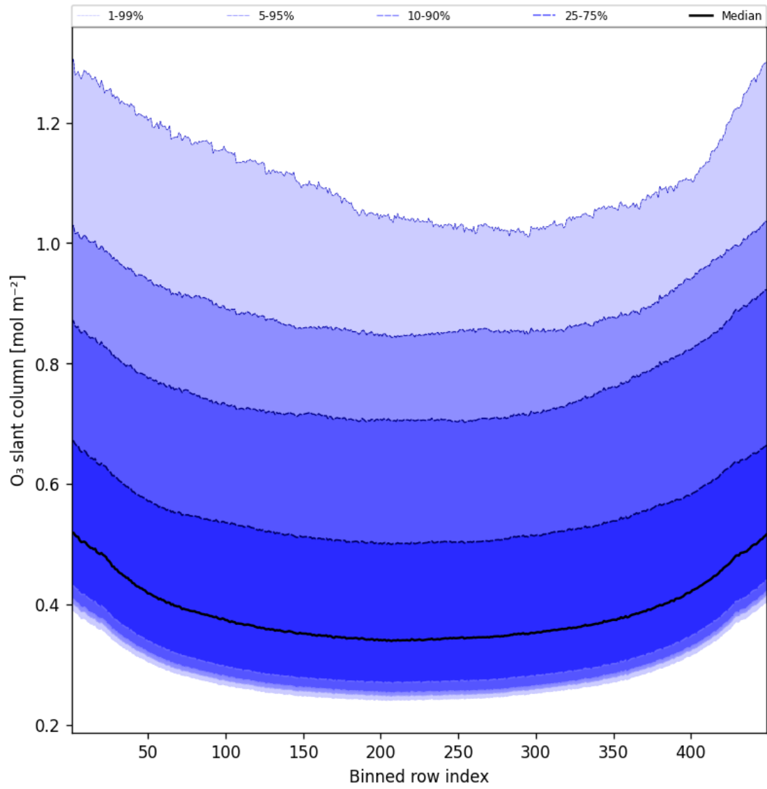
Figure 43: Along track statistics of “O 3 slant column” for 2025-08-31 to 2025-09-01
