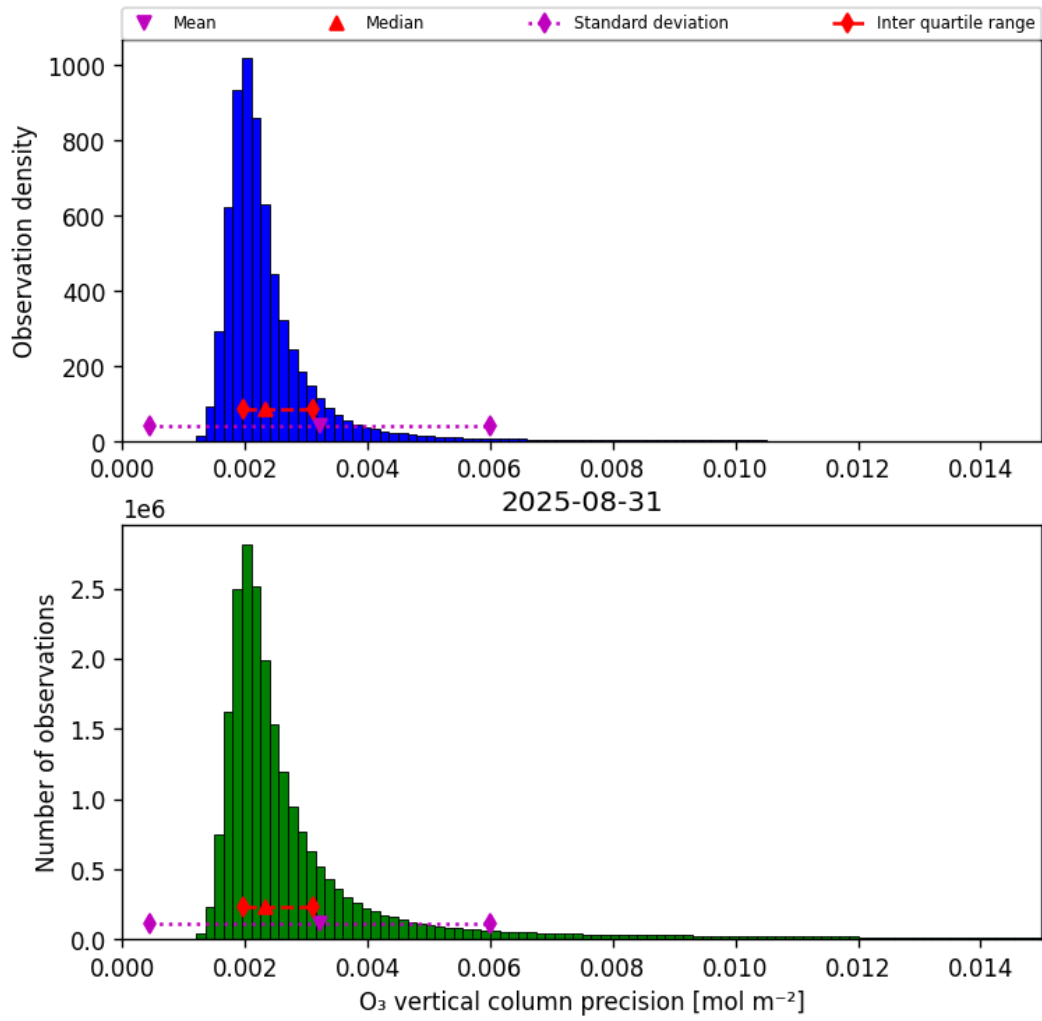
Figure 30: Histogram of “O 3 vertical column precision” for 2025-08-31 to 2025-09-01
