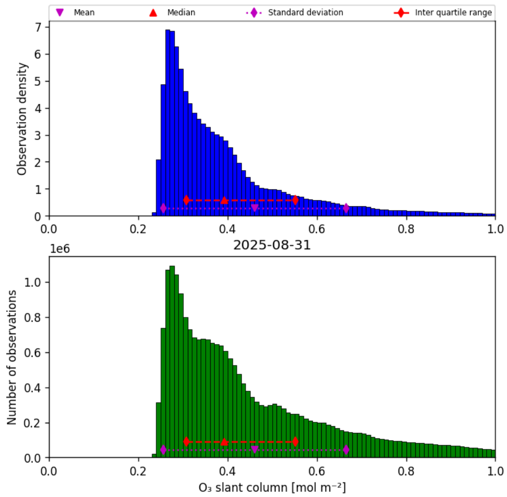
Figure 31: Histogram of “O 3 slant column” for 2025-08-31 to 2025-09-01
