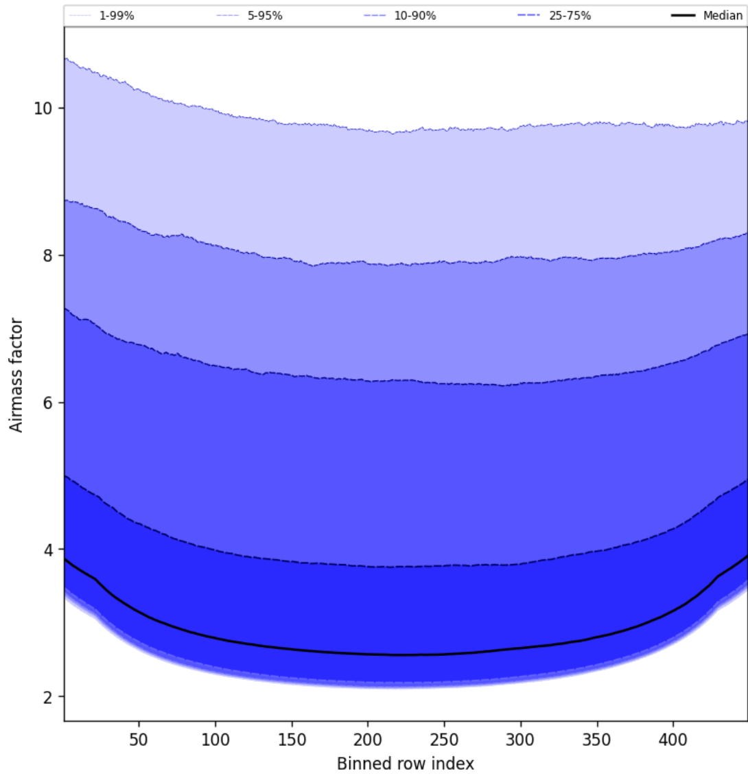
Figure 49: Along track statistics of “Airmass factor” for 2025-08-31 to 2025-09-01
