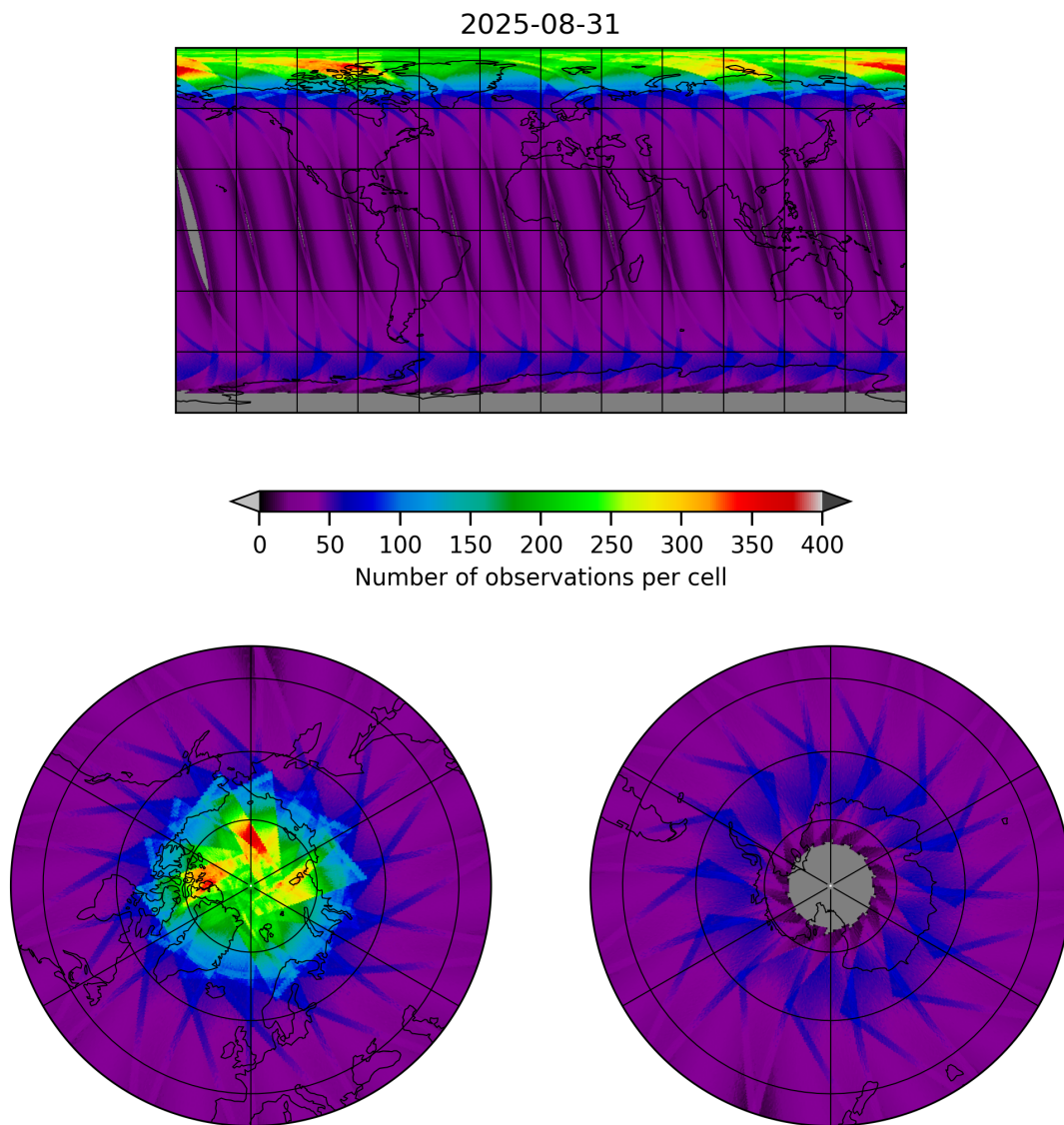
Figure 15: Map of the number of observations for 2025-08-31 to 2025-09-01
