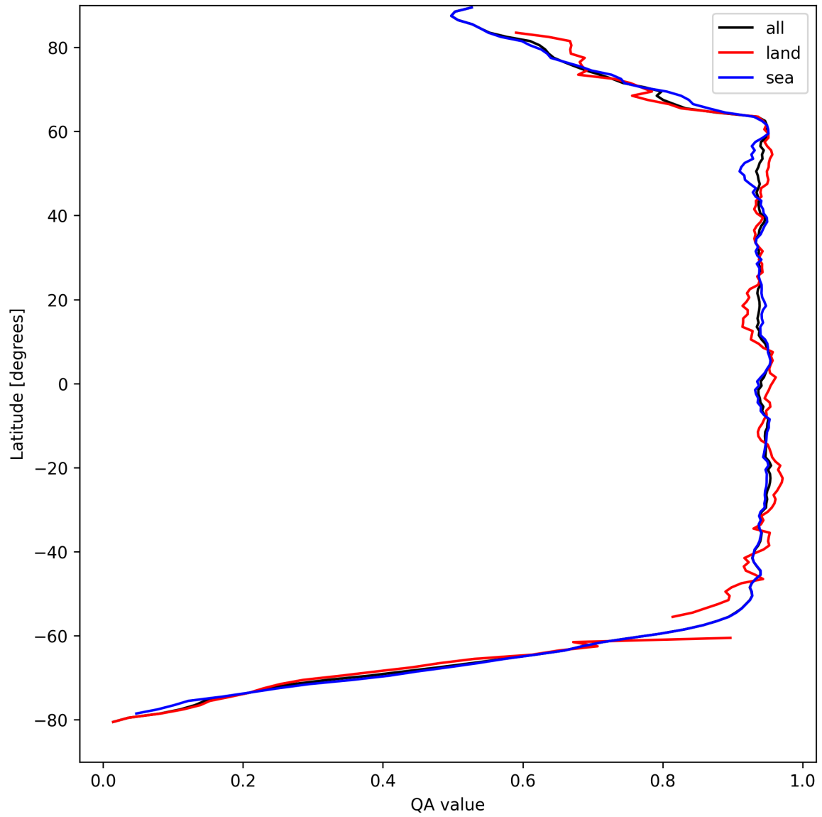
Figure 16: Zonal average of “QA value” for 2025-08-31 to 2025-09-01.
