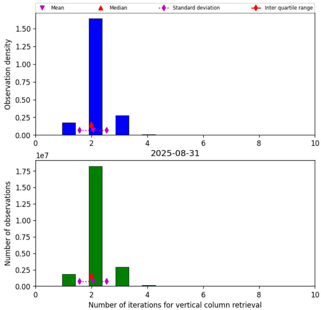
Figure 39: Histogram of “Number of iterations for vertical column retrieval” for 2025-08-31 to 2025-09-01
