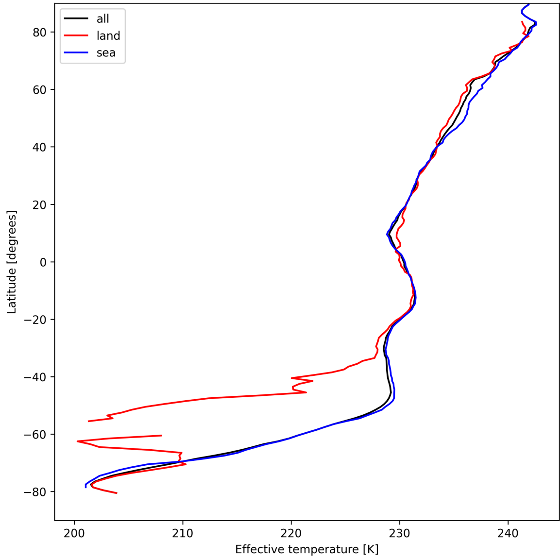
Figure 26: Zonal average of "Effective temperature" for 2025-08-31 to 2025-09-01.
