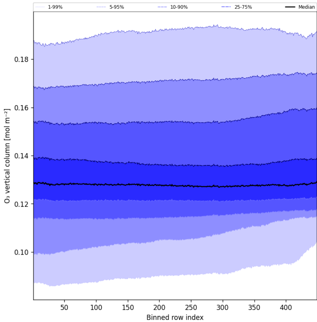
Figure 41: Along track statistics of “O 3 vertical column” for 2025-08-31 to 2025-09-01
