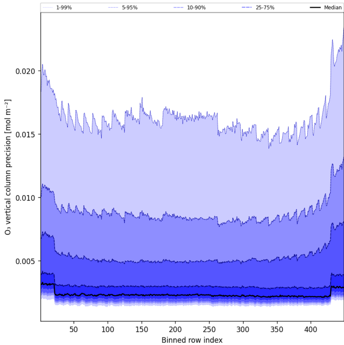
Figure 42: Along track statistics of “O 3 vertical column precision” for 2025-08-31 to 2025-09-01
