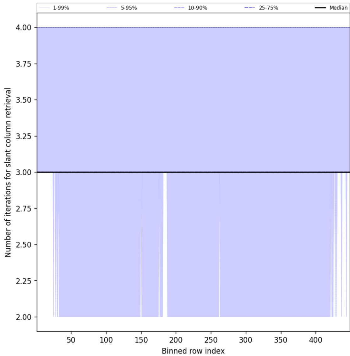
Figure 45: Along track statistics of “Number of iterations for slant column retrieval” for 2025-08-31 to 2025-09-01
