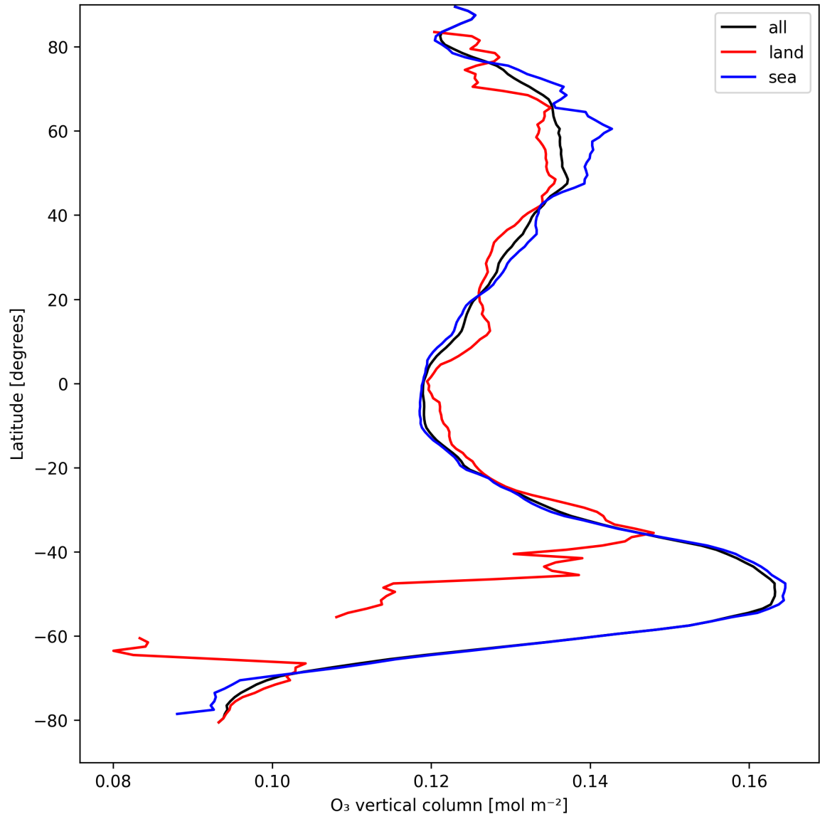
Figure 17: Zonal average of “O 3 vertical column” for 2025-08-31 to 2025-09-01.
