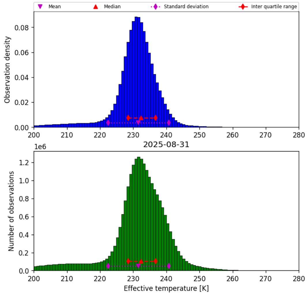
Figure 38: Histogram of “Effective temperature” for 2025-08-31 to 2025-09-01
