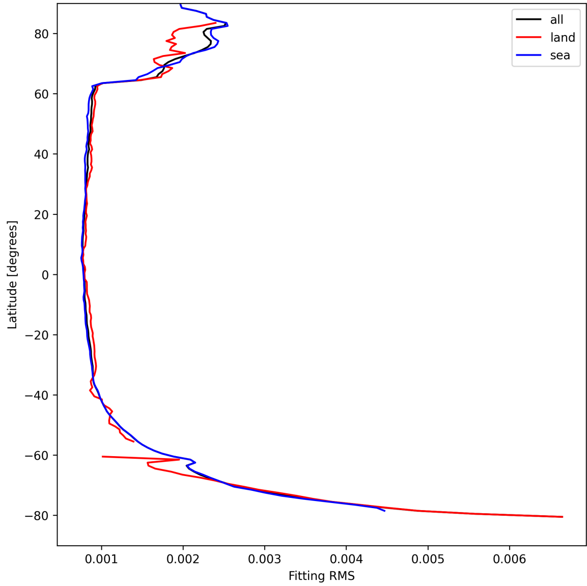
Figure 22: Zonal average of "Fitting RMS" for 2025-08-31 to 2025-09-01.
