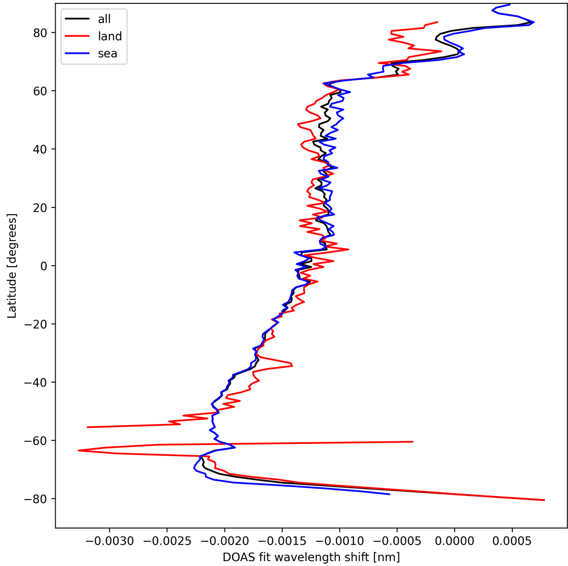
Figure 23: Zonal average of "DOAS fit wavelength shift" for 2025-08-31 to 2025-09-01.
