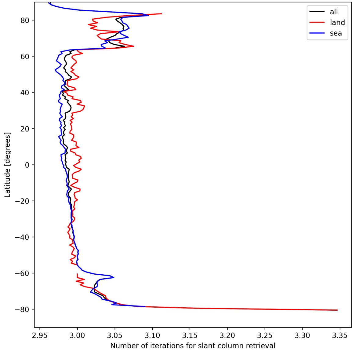
Figure 21: Zonal average of “Number of iterations for slant column retrieval” for 2025-08-31 to 2025-09-01.
