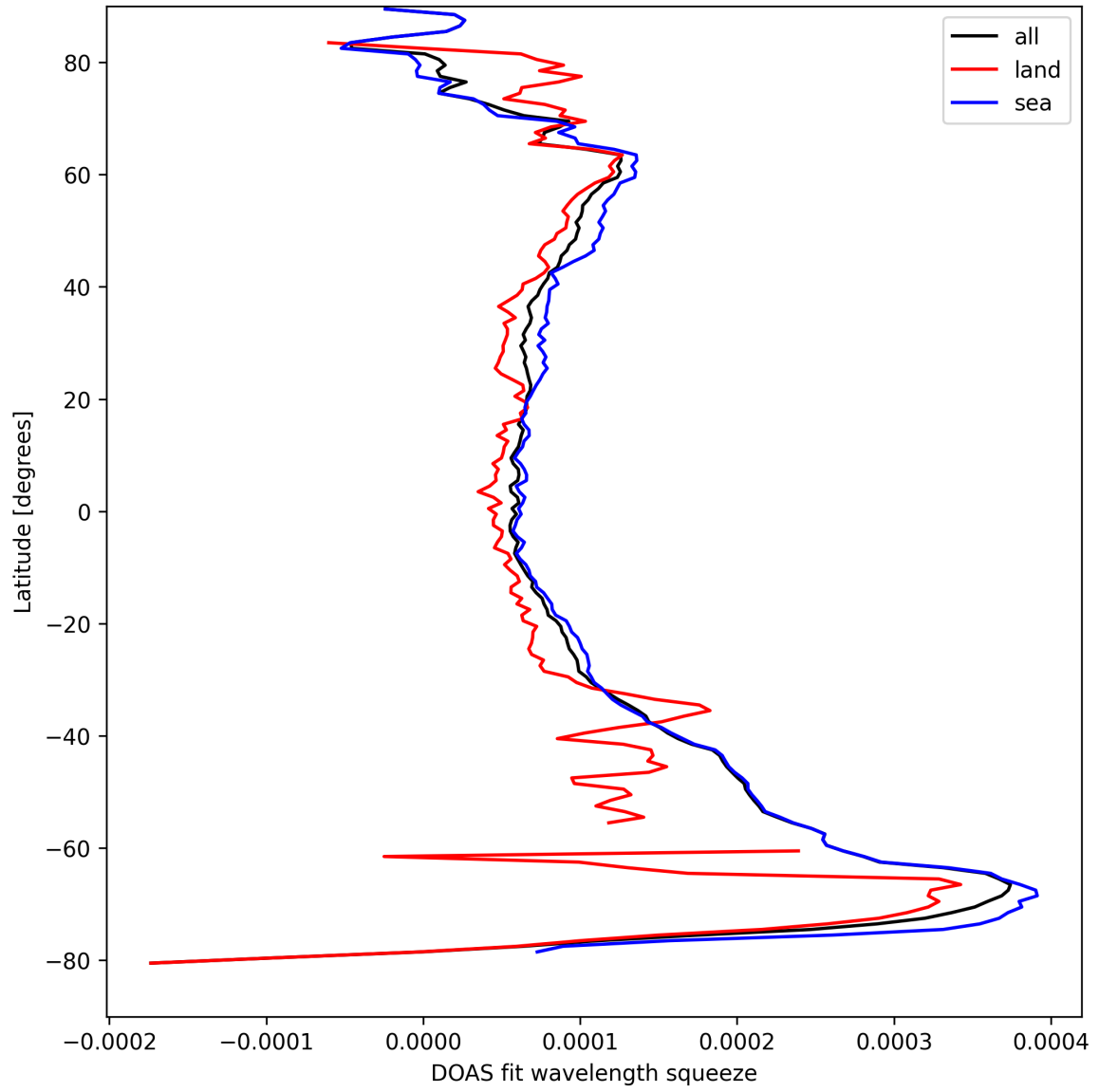
Figure 24: Zonal average of “DOAS fit wavelength squeeze” for 2025-08-31 to 2025-09-01.
