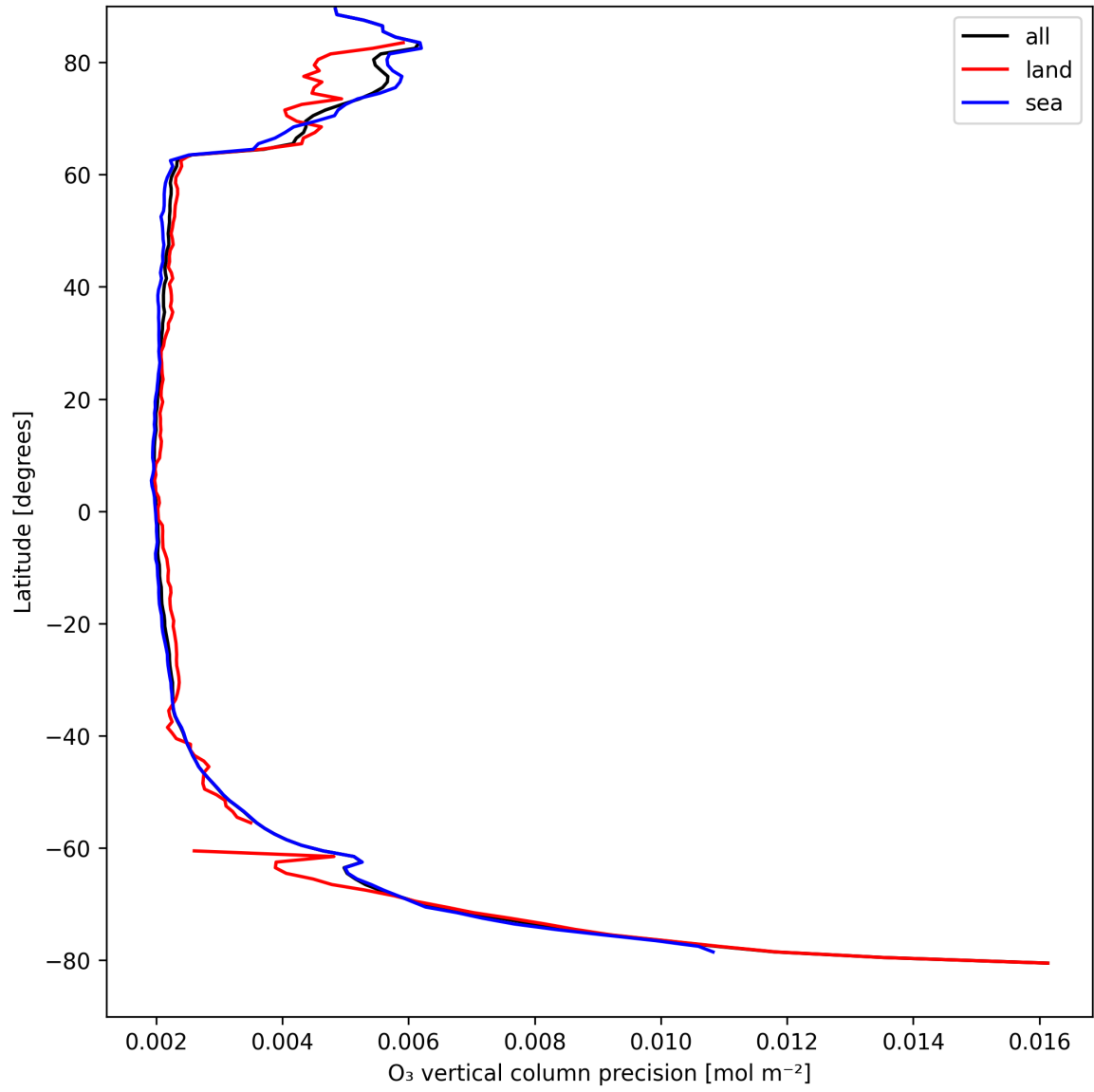
Figure 18: Zonal average of “O 3 vertical column precision” for 2025-08-31 to 2025-09-01.
