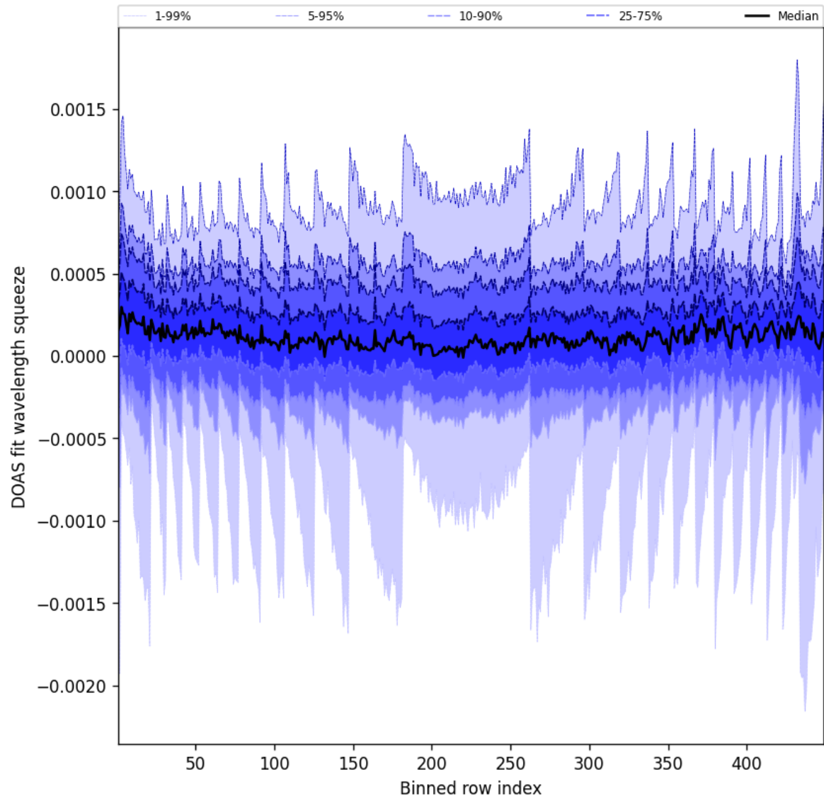
Figure 48: Along track statistics of “DOAS fit wavelength squeeze” for 2025-08-31 to 2025-09-01
