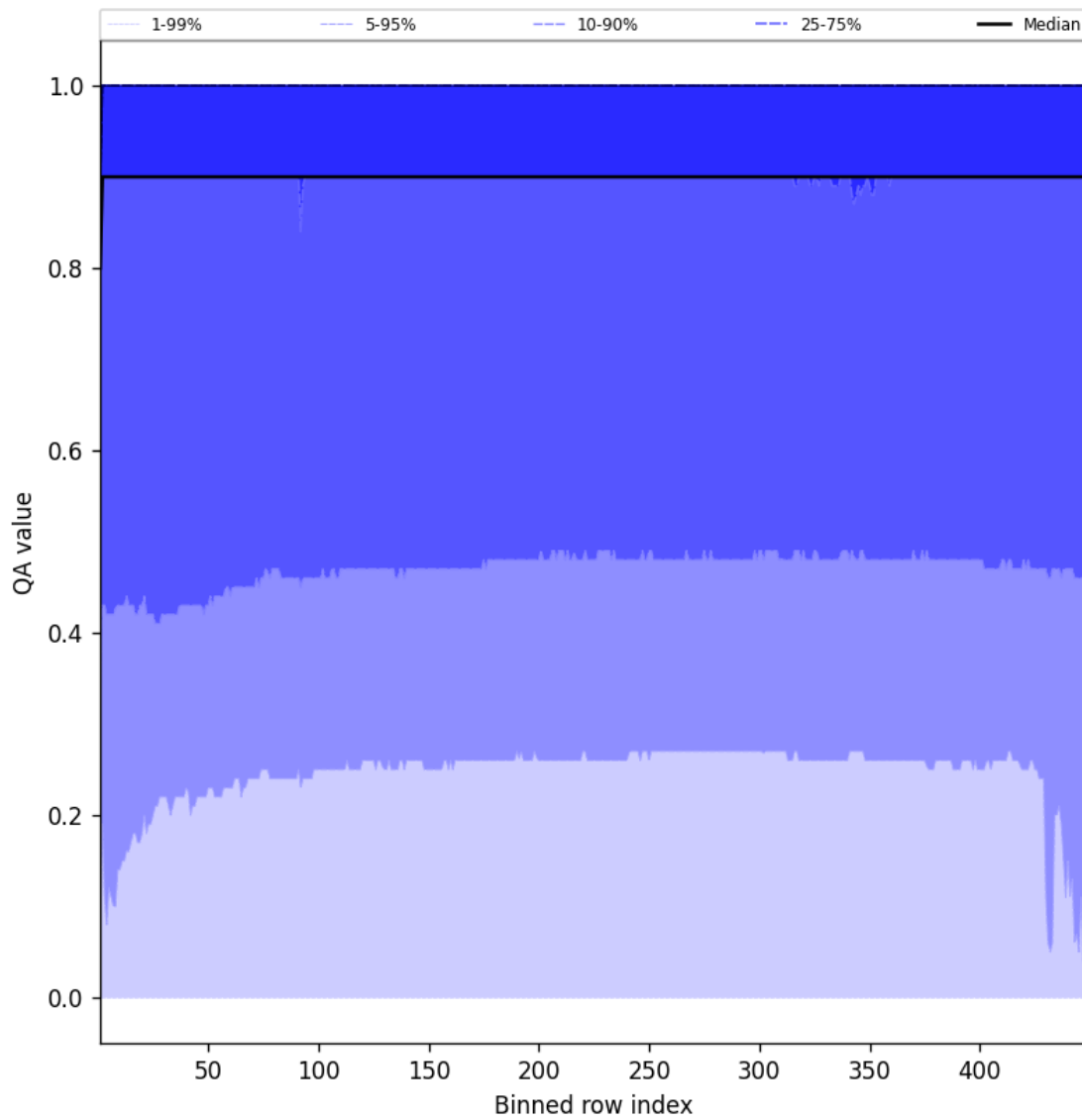
Figure 40: Along track statistics of “QA value” for 2025-08-31 to 2025-09-01
