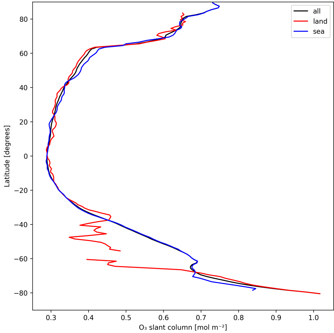
Figure 19: Zonal average of “O 3 slant column” for 2025-08-31 to 2025-09-01.
