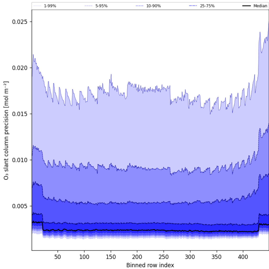
Figure 44: Along track statistics of “O 3 slant column precision” for 2025-08-31 to 2025-09-01
