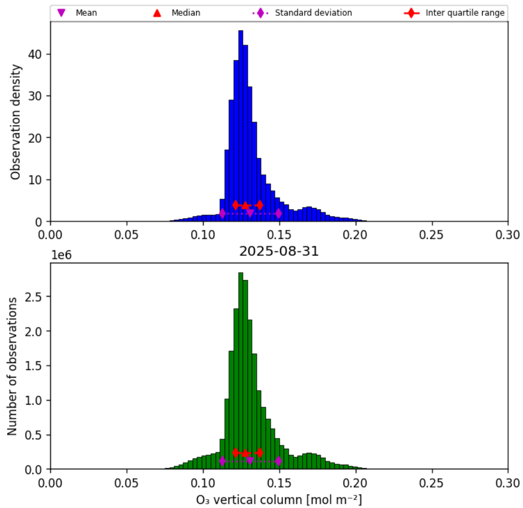
Figure 29: Histogram of “O 3 vertical column” for 2025-08-31 to 2025-09-01
