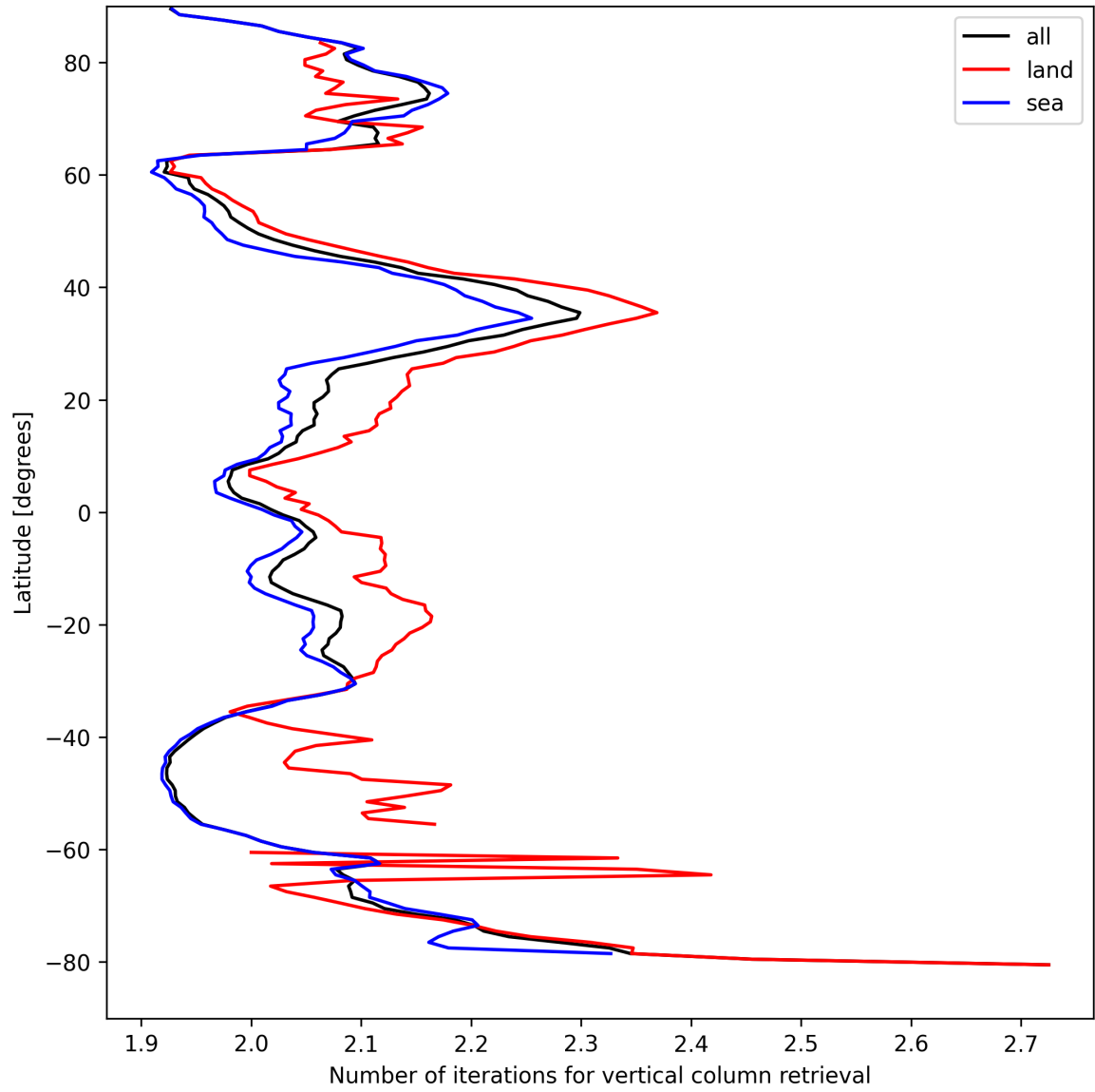
Figure 27: Zonal average of “Number of iterations for vertical column retrieval” for 2025-08-31 to 2025-09-01.
