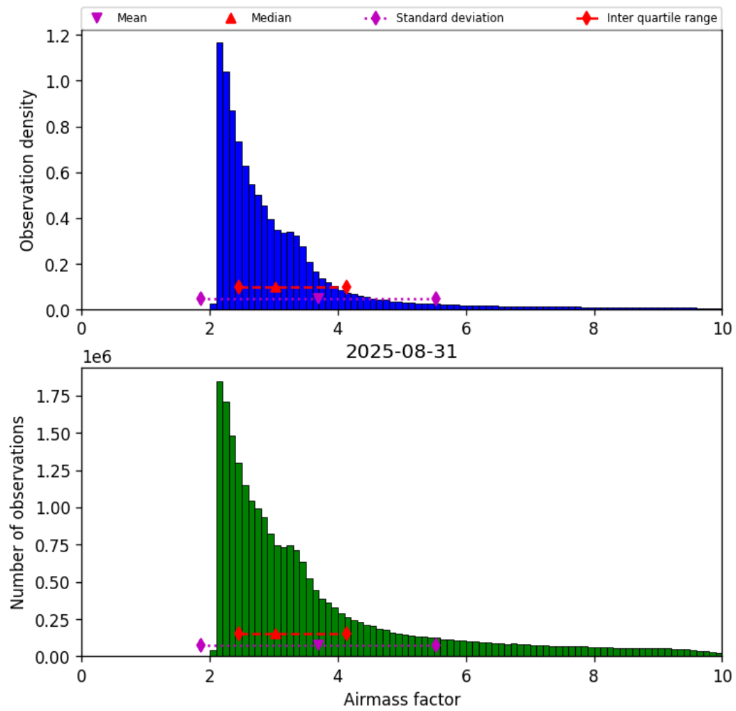
Figure 37: Histogram of “Airmass factor” for 2025-08-31 to 2025-09-01
