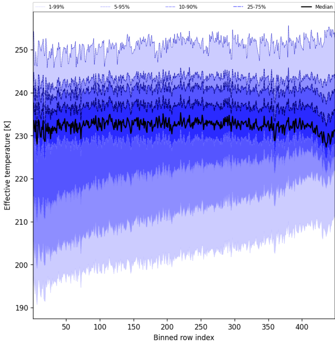
Figure 50: Along track statistics of “Effective temperature” for 2025-08-31 to 2025-09-01
