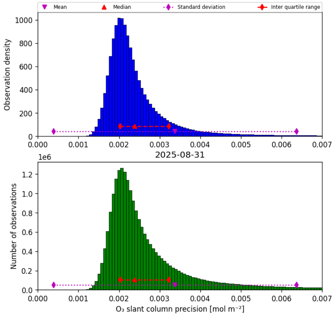
Figure 32: Histogram of “O 3 slant column precision” for 2025-08-31 to 2025-09-01
