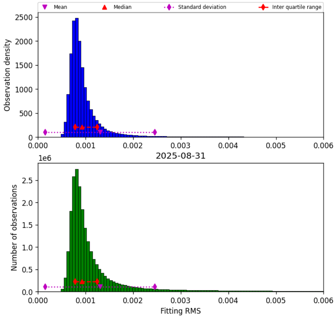
Figure 34: Histogram of “Fitting RMS” for 2025-08-31 to 2025-09-01
