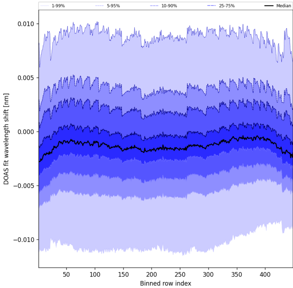
Figure 47: Along track statistics of "DOAS fit wavelength shift" for 2025-08-31 to 2025-09-01
