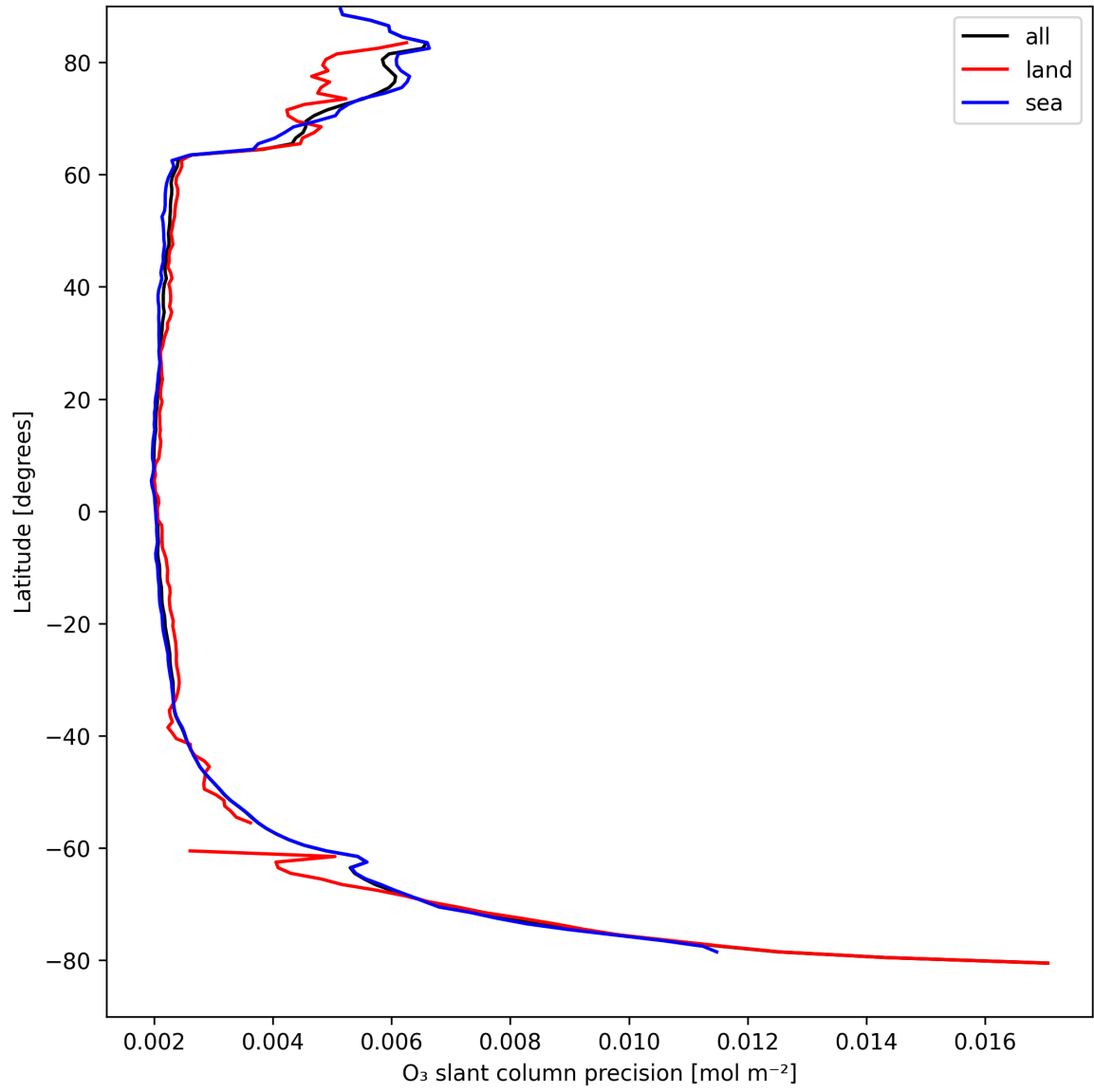
Figure 20: Zonal average of “O 3 slant column precision” for 2025-08-31 to 2025-09-01.
