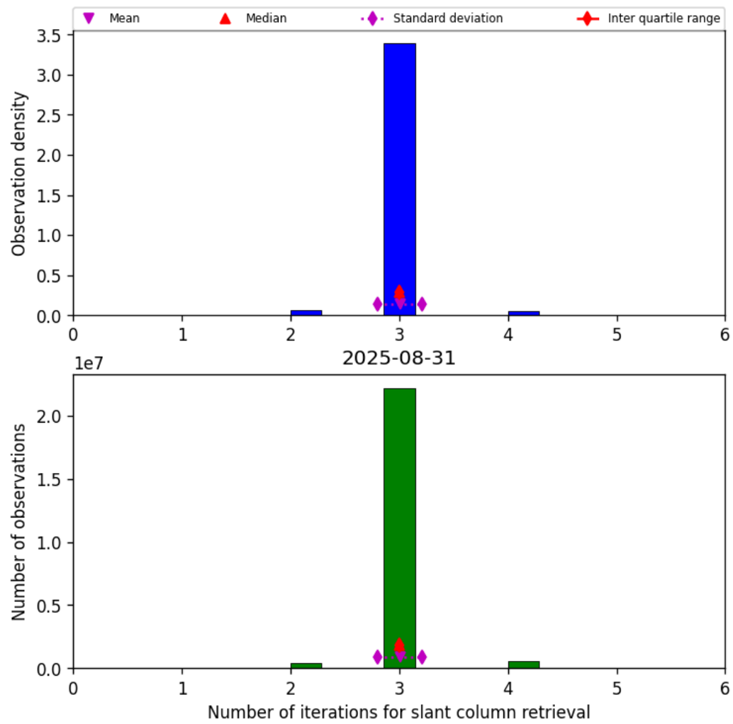
Figure 33: Histogram of “Number of iterations for slant column retrieval” for 2025-08-31 to 2025-09-01
