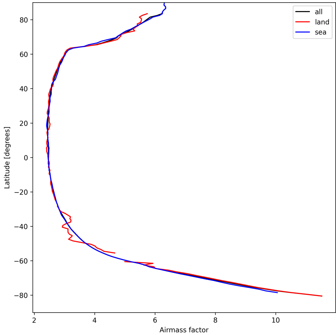
Figure 25: Zonal average of “Airmass factor” for 2025-08-31 to 2025-09-01.
