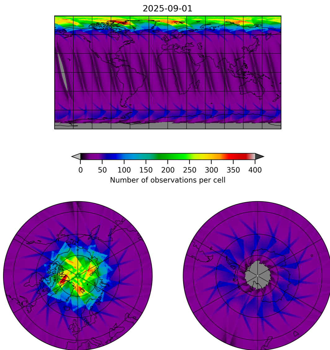
Figure 15: Map of the number of observations for 2025-09-01 to 2025-09-02
