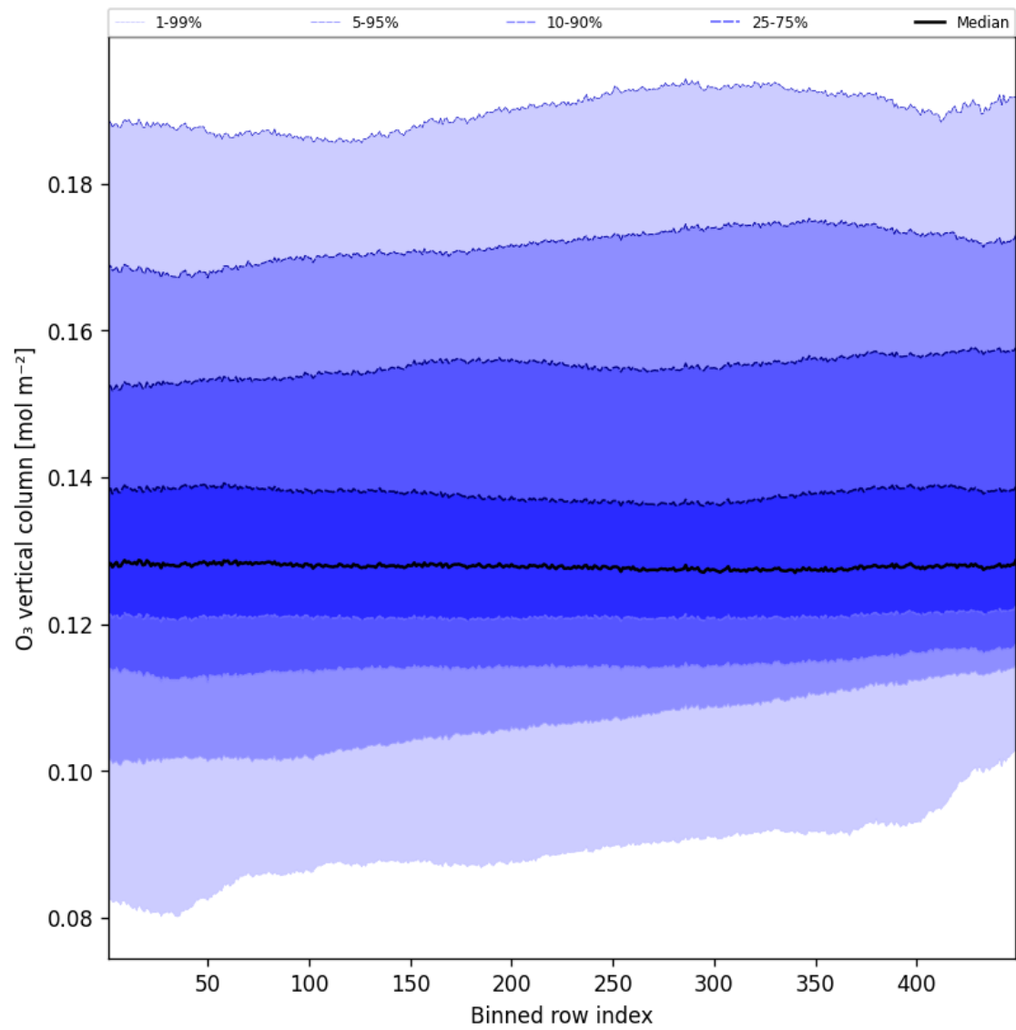
Figure 41: Along track statistics of “O 3 vertical column” for 2025-09-01 to 2025-09-02
