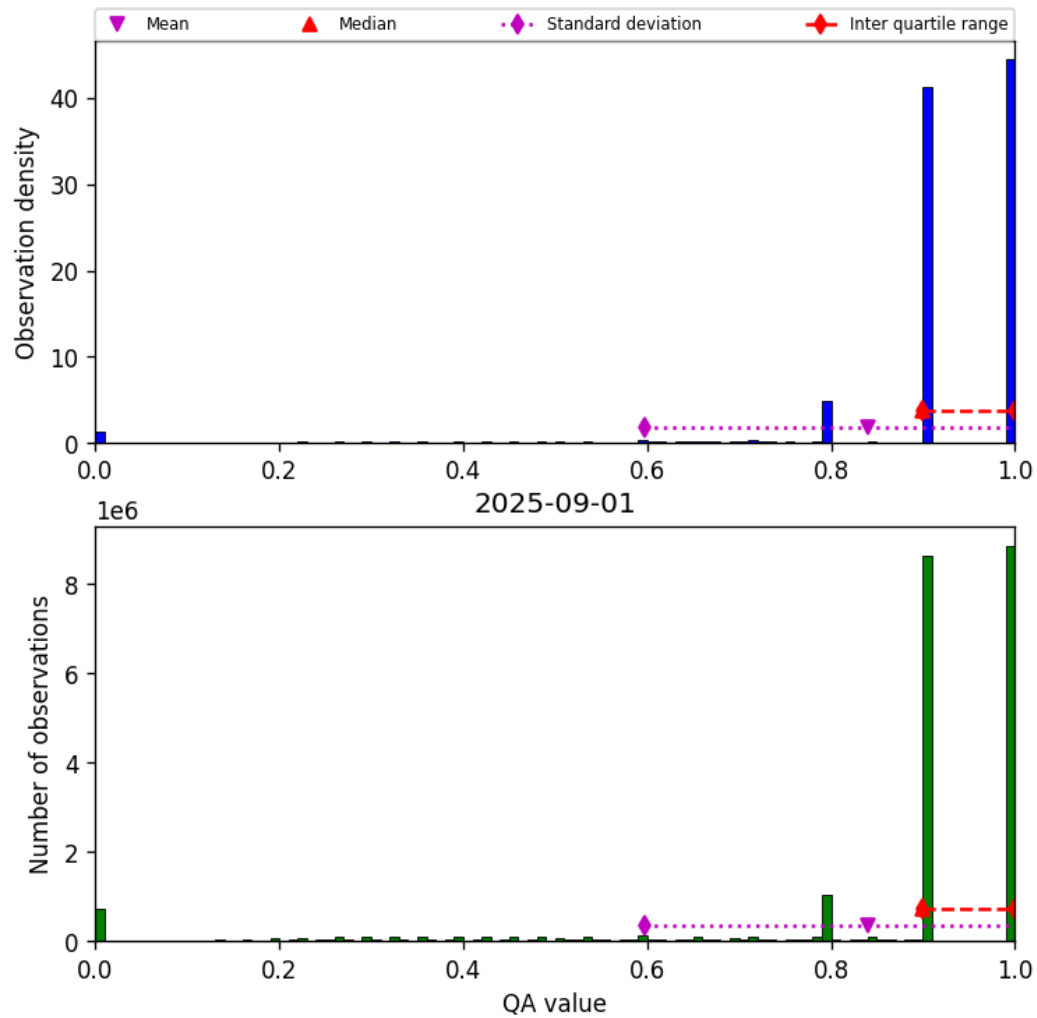
Figure 28: Histogram of “QA value” for 2025-09-01 to 2025-09-02
