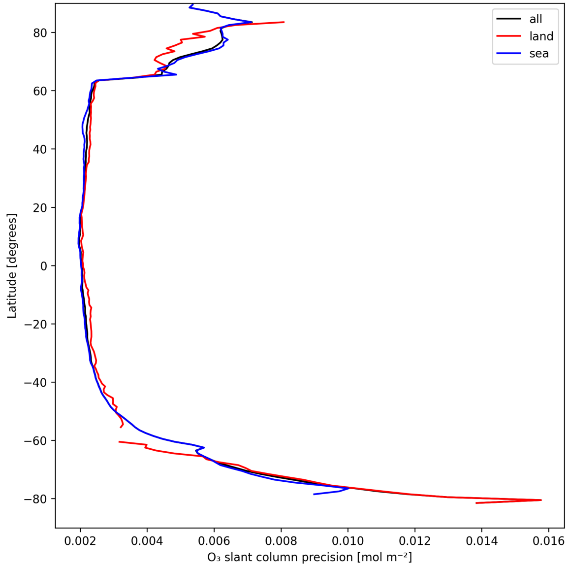
Figure 20: Zonal average of “O 3 slant column precision” for 2025-09-01 to 2025-09-02.
