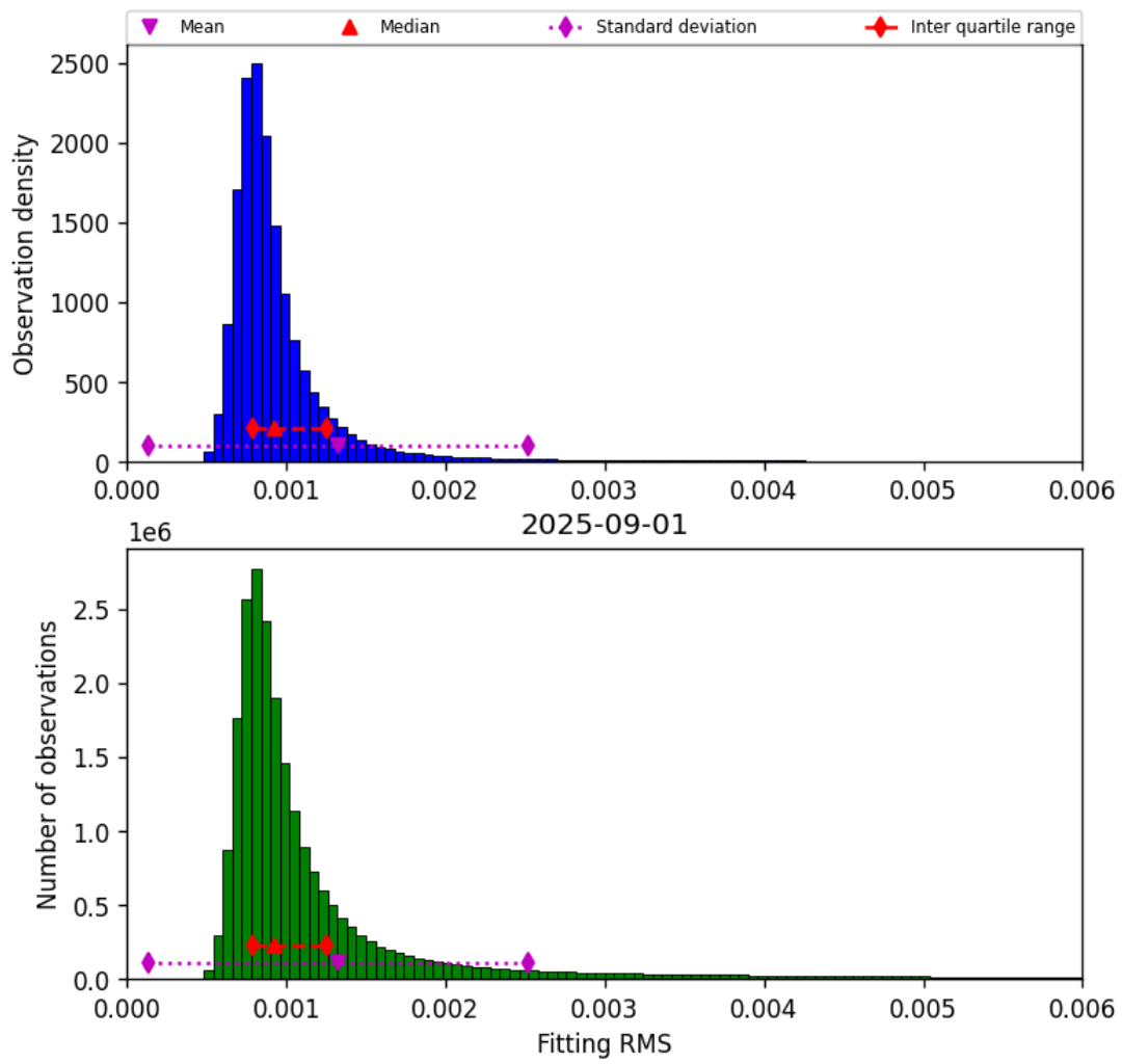
Figure 34: Histogram of “Fitting RMS” for 2025-09-01 to 2025-09-02
