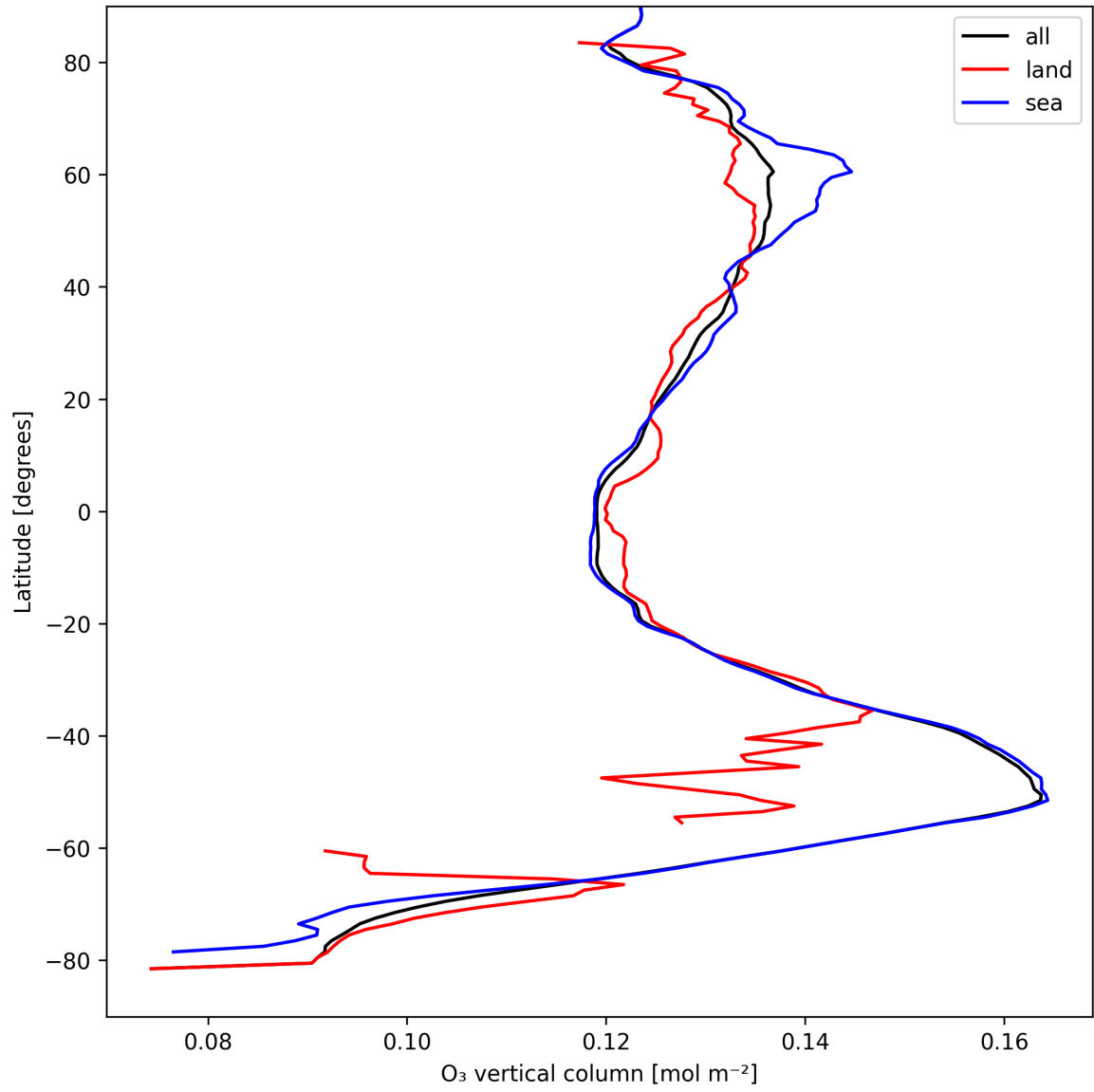
Figure 17: Zonal average of “O 3 vertical column” for 2025-09-01 to 2025-09-02.
