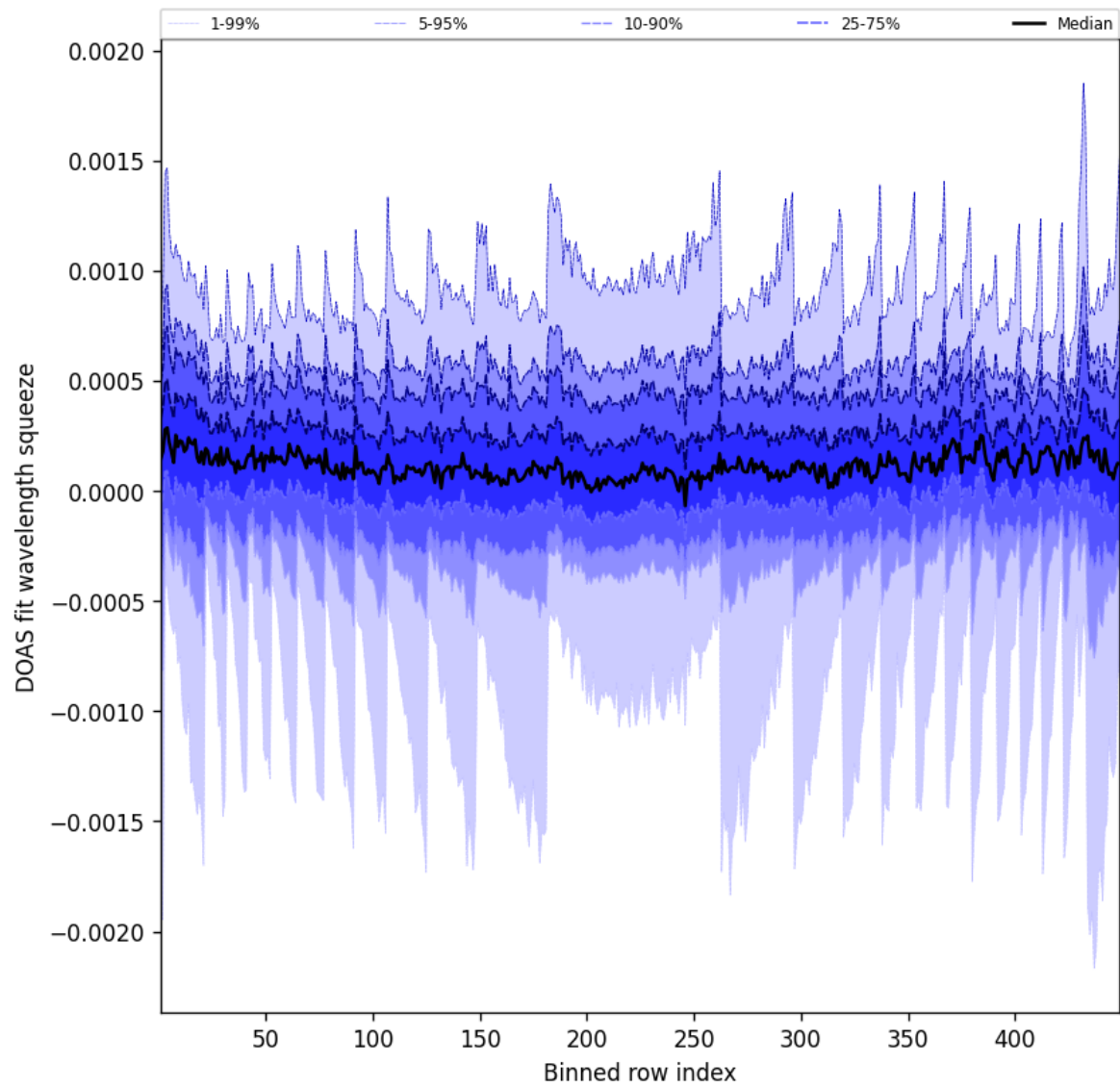
Figure 48: Along track statistics of “DOAS fit wavelength squeeze” for 2025-09-01 to 2025-09-02
