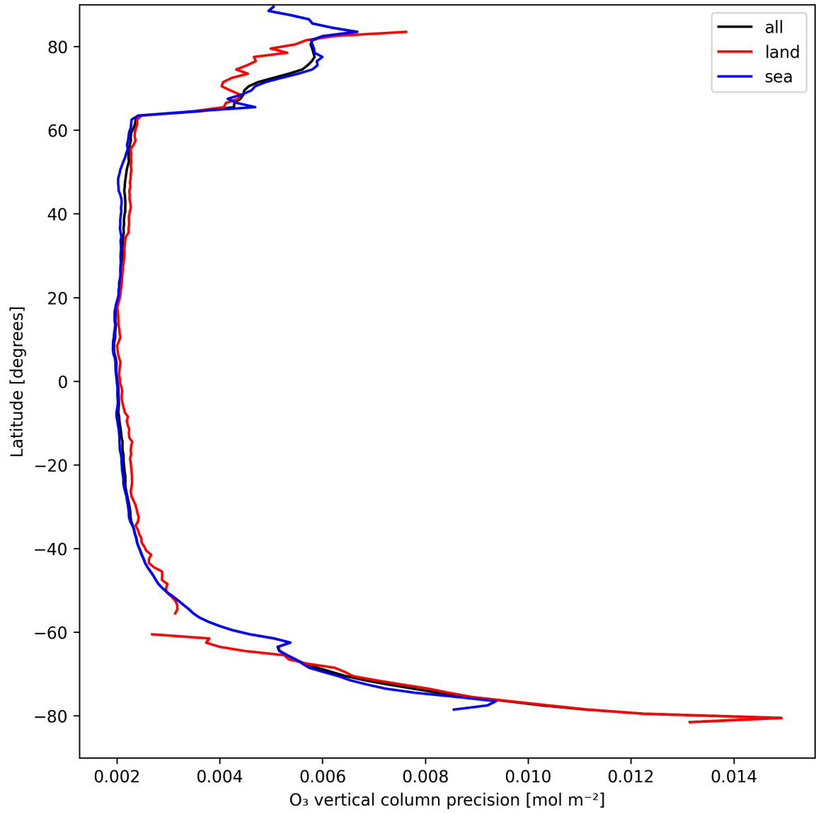
Figure 18: Zonal average of “O 3 vertical column precision” for 2025-09-01 to 2025-09-02.
