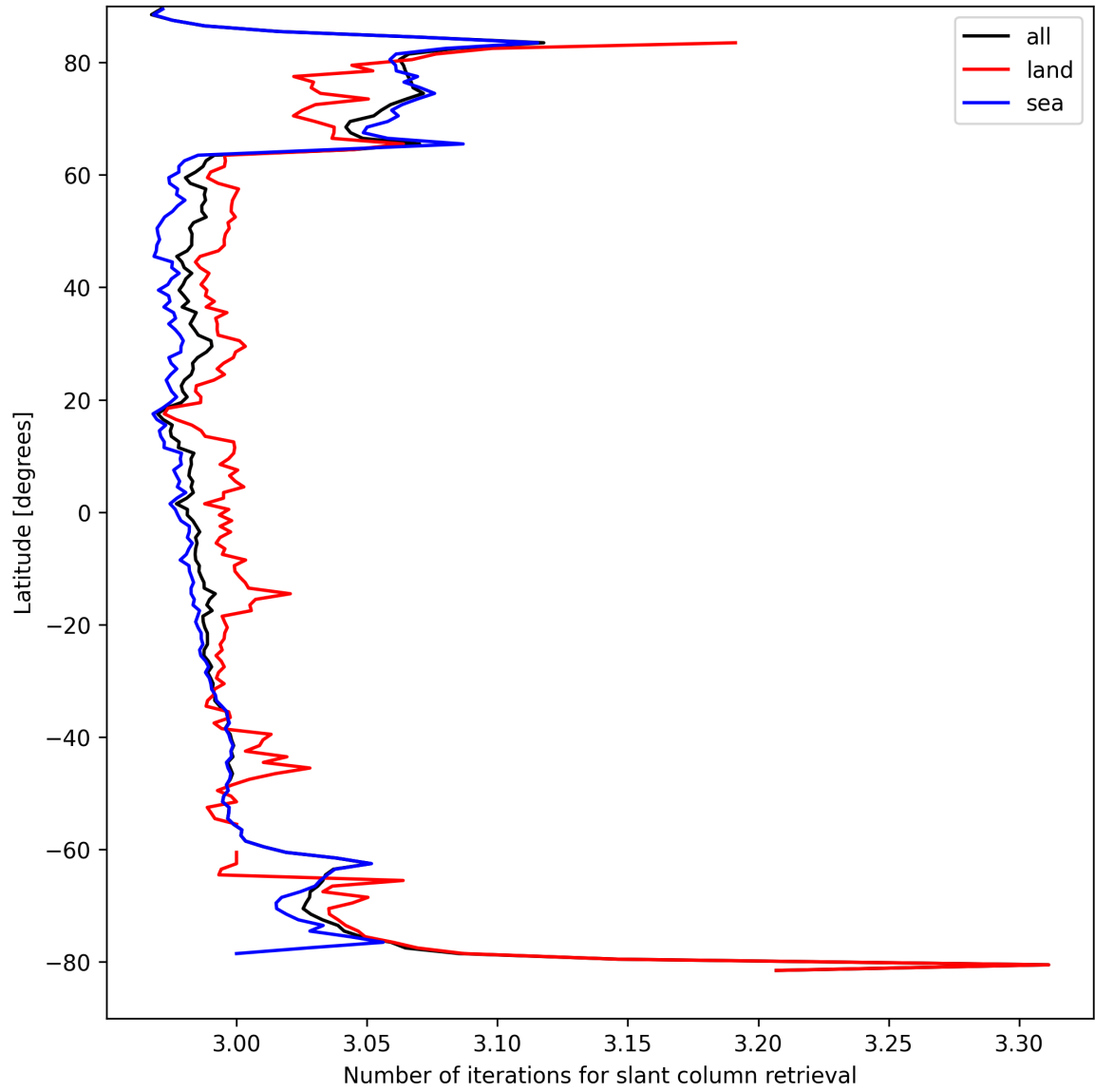
Figure 21: Zonal average of “Number of iterations for slant column retrieval” for 2025-09-01 to 2025-09-02.
