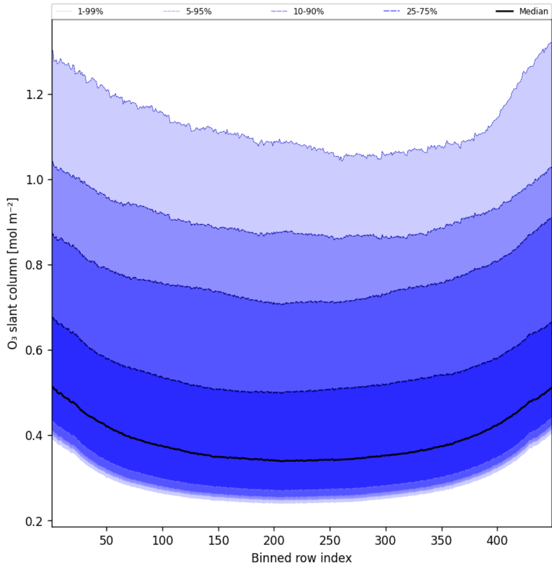
Figure 43: Along track statistics of “O 3 slant column” for 2025-09-01 to 2025-09-02
