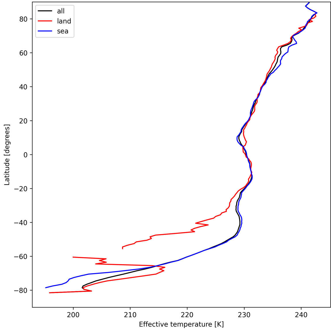
Figure 26: Zonal average of "Effective temperature" for 2025-09-01 to 2025-09-02.
