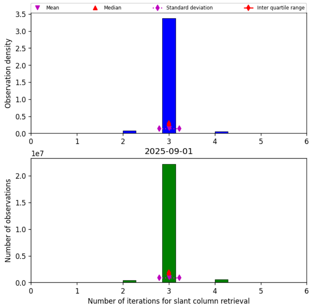
Figure 33: Histogram of “Number of iterations for slant column retrieval” for 2025-09-01 to 2025-09-02
