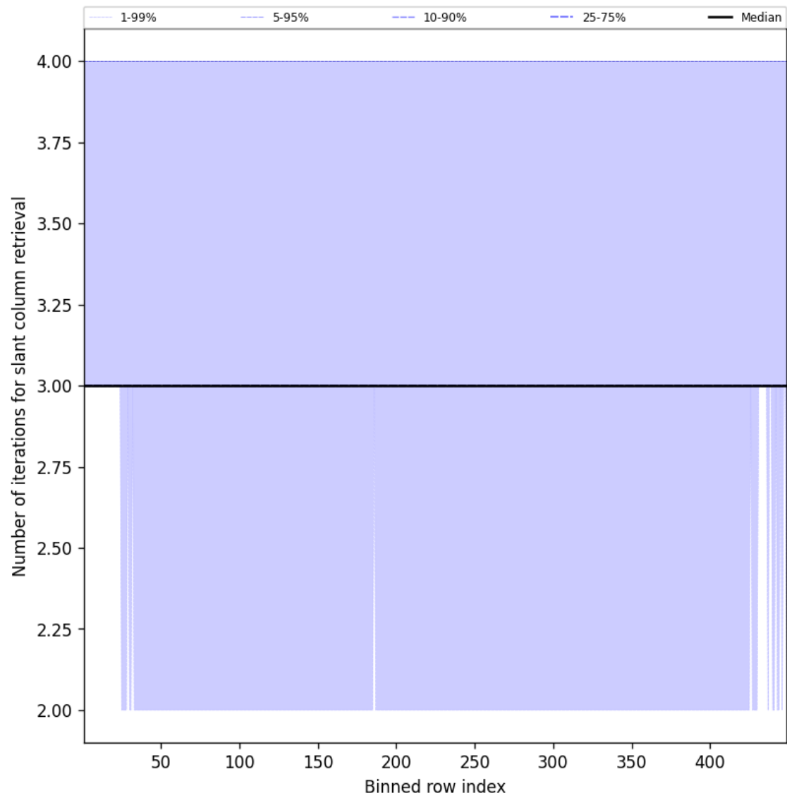
Figure 45: Along track statistics of “Number of iterations for slant column retrieval” for 2025-09-01 to 2025-09-02
