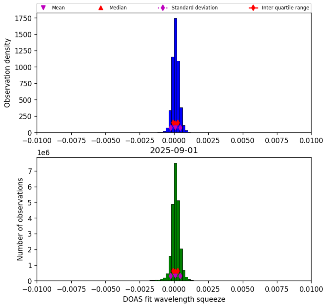
Figure 36: Histogram of “DOAS fit wavelength squeeze” for 2025-09-01 to 2025-09-02
