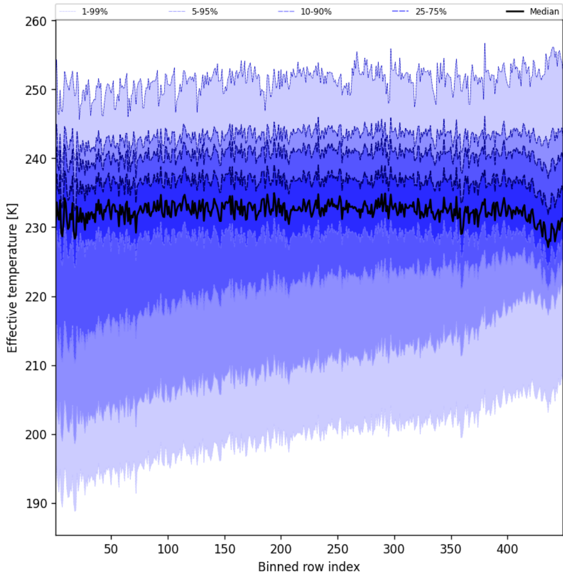
Figure 50: Along track statistics of “Effective temperature” for 2025-09-01 to 2025-09-02
