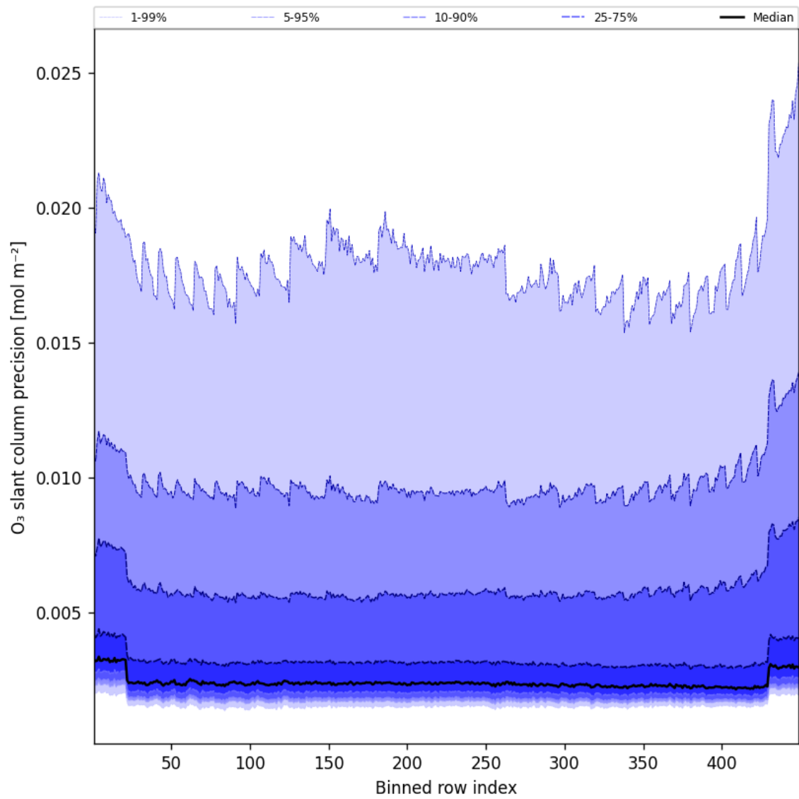
Figure 44: Along track statistics of “O 3 slant column precision” for 2025-09-01 to 2025-09-02
