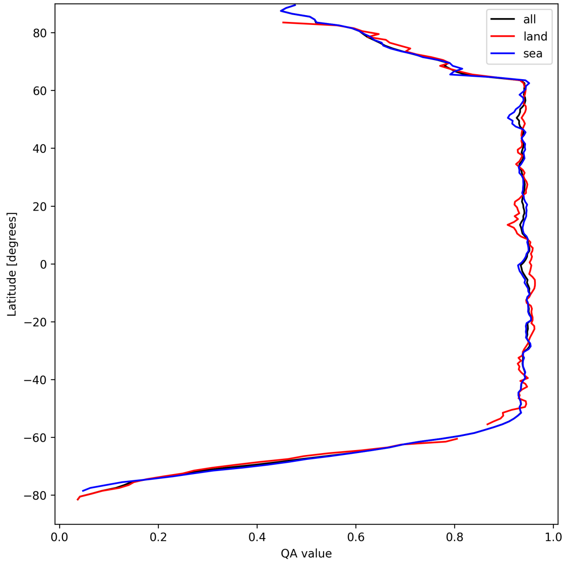
Figure 16: Zonal average of “QA value” for 2025-09-01 to 2025-09-02.
