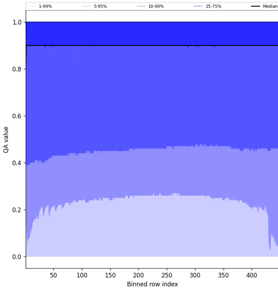
Figure 40: Along track statistics of “QA value” for 2025-09-01 to 2025-09-02
