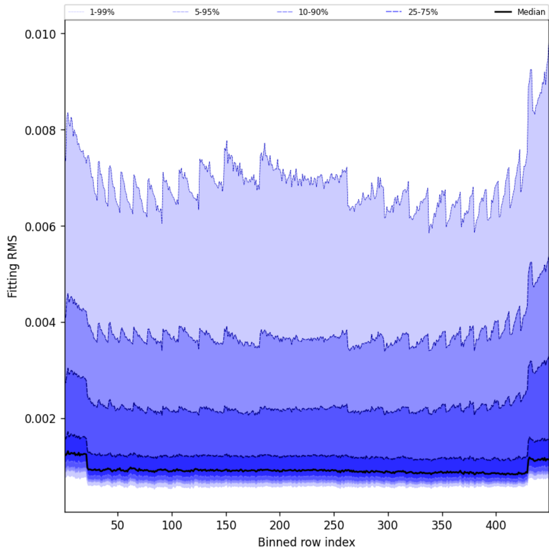
Figure 46: Along track statistics of “Fitting RMS” for 2025-09-01 to 2025-09-02
