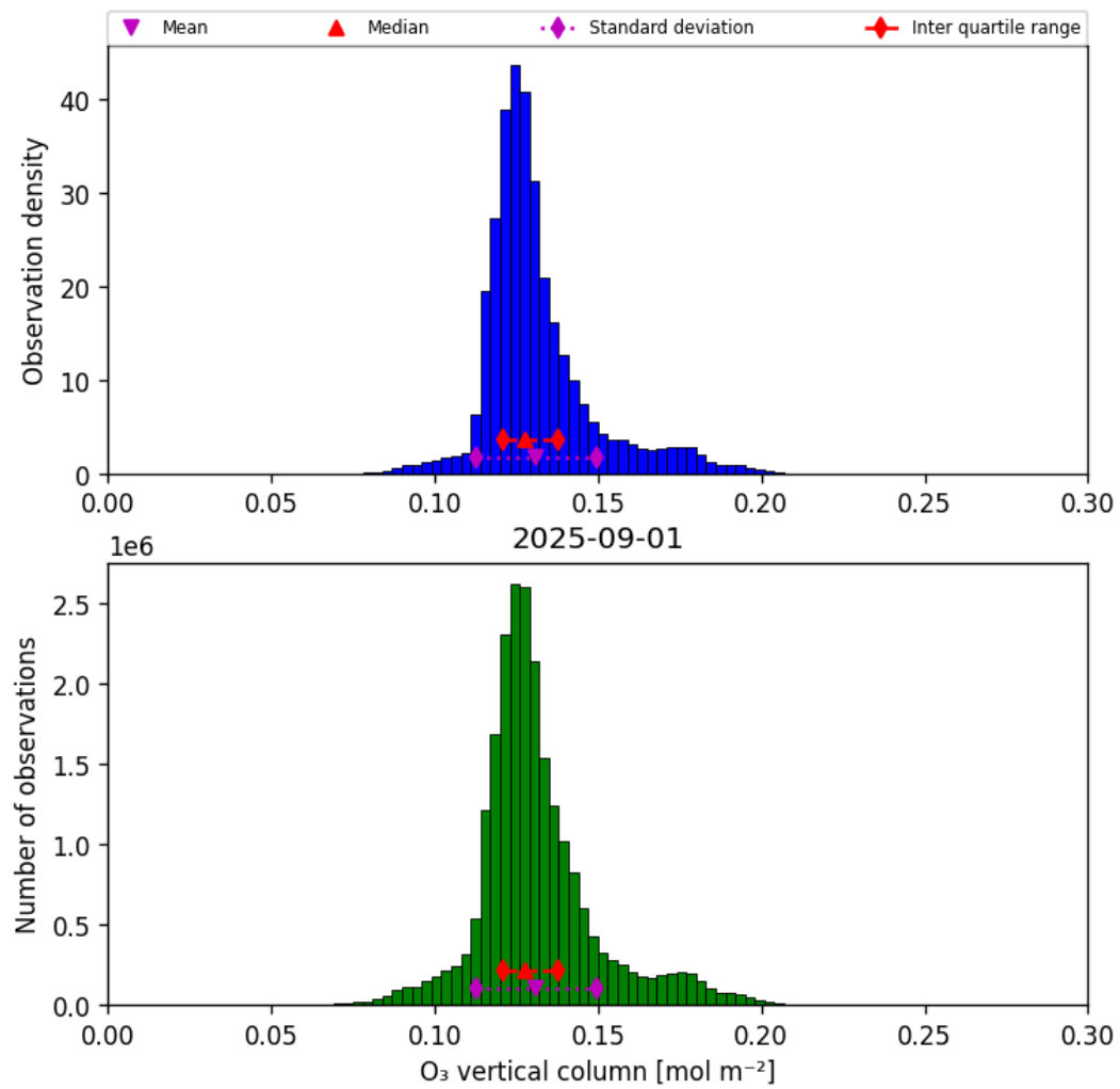
Figure 29: Histogram of “O 3 vertical column” for 2025-09-01 to 2025-09-02
