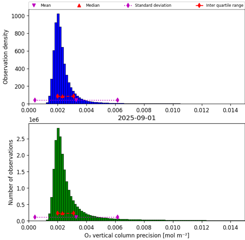
Figure 30: Histogram of “O 3 vertical column precision” for 2025-09-01 to 2025-09-02
