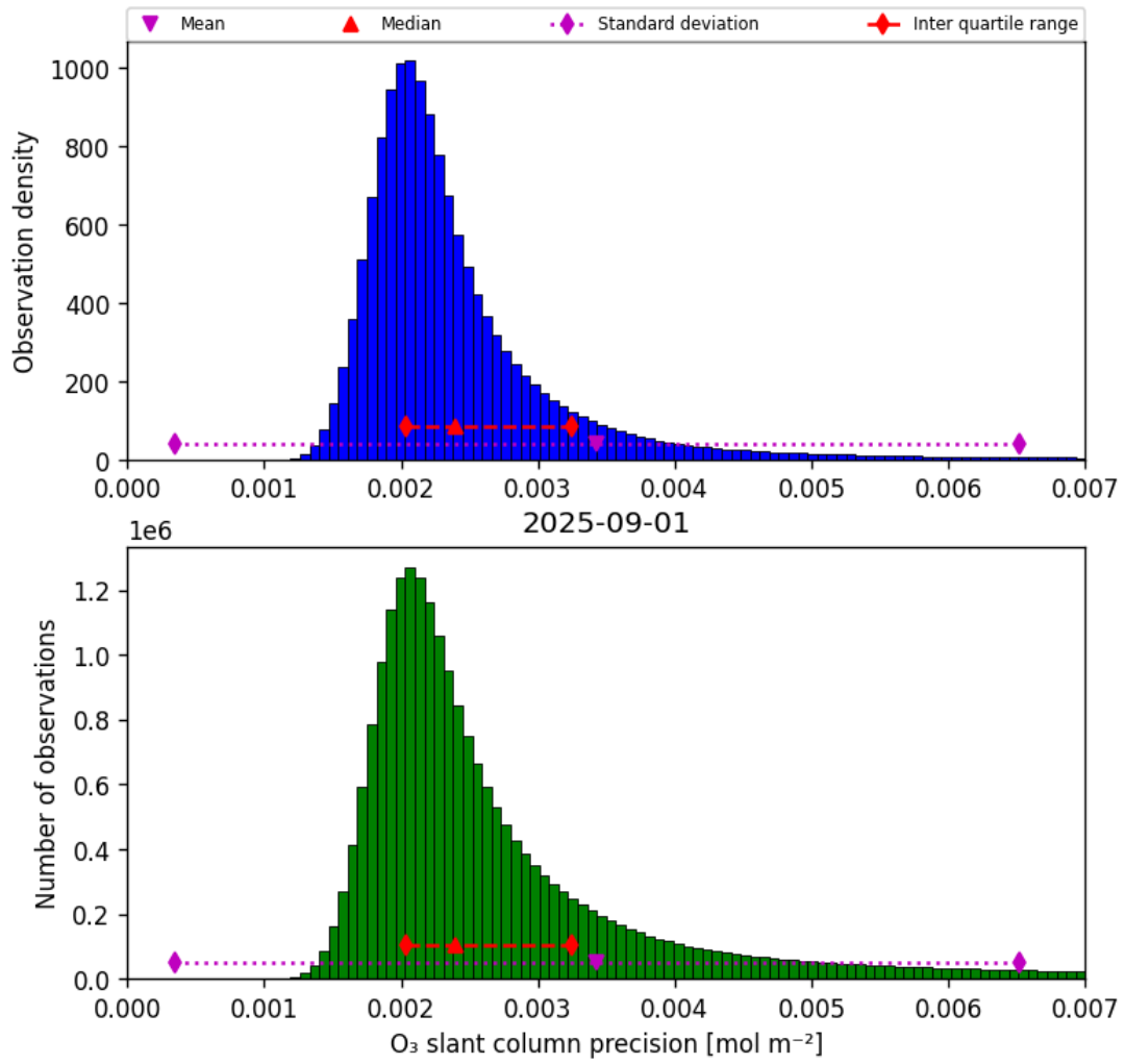
Figure 32: Histogram of “O 3 slant column precision” for 2025-09-01 to 2025-09-02
