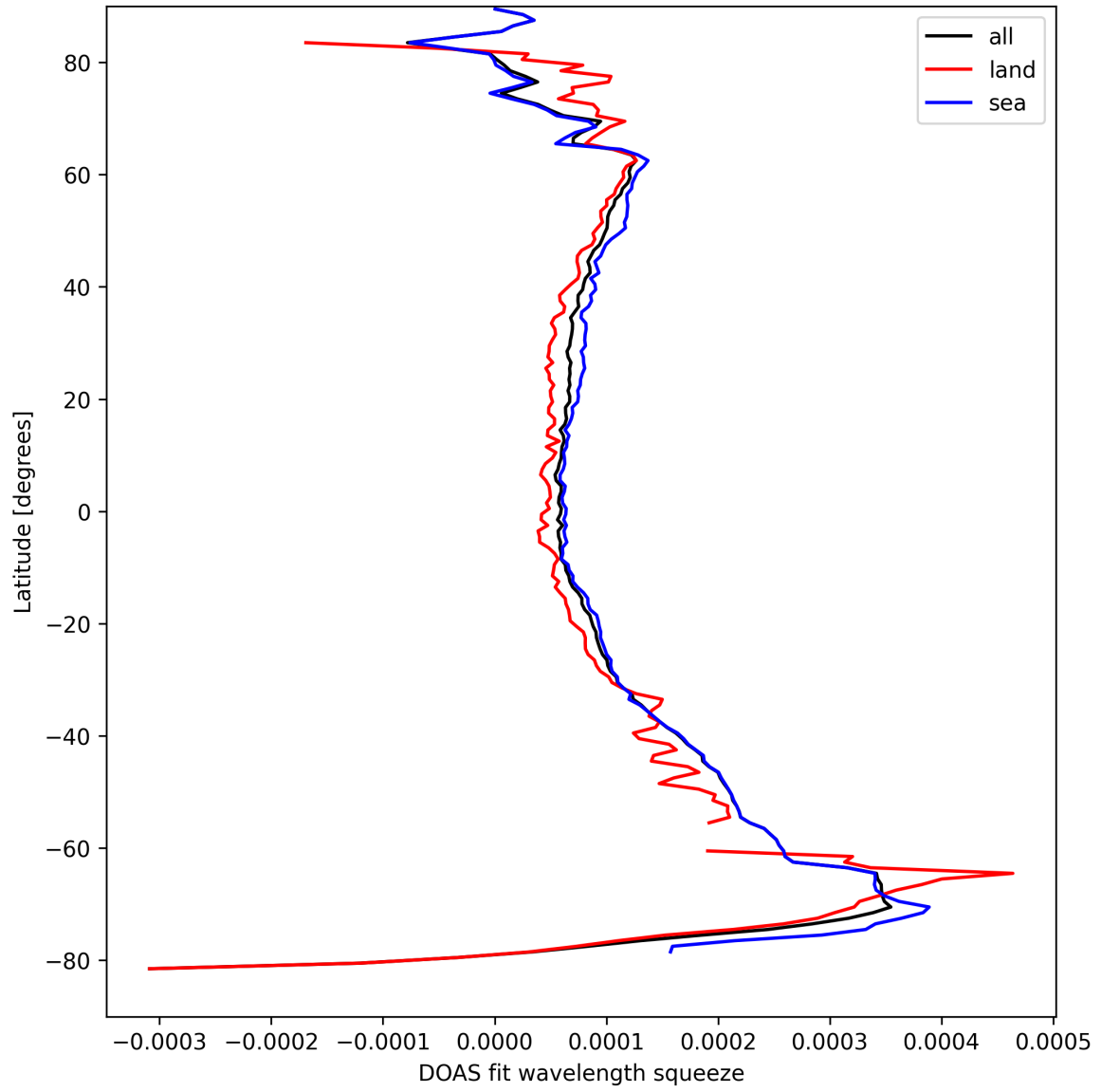
Figure 24: Zonal average of “DOAS fit wavelength squeeze” for 2025-09-01 to 2025-09-02.
