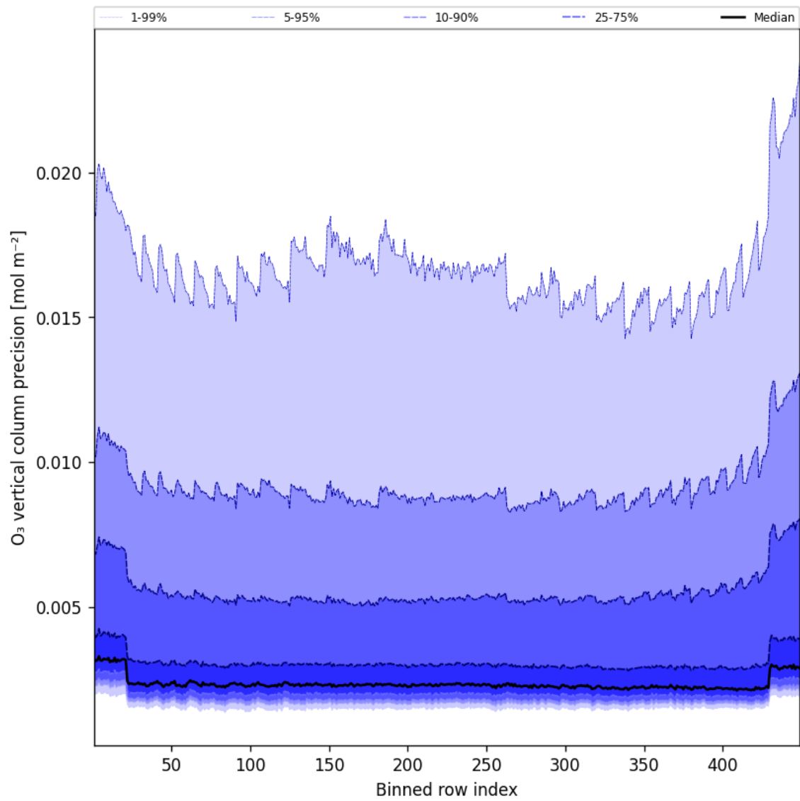
Figure 42: Along track statistics of “O 3 vertical column precision” for 2025-09-01 to 2025-09-02
