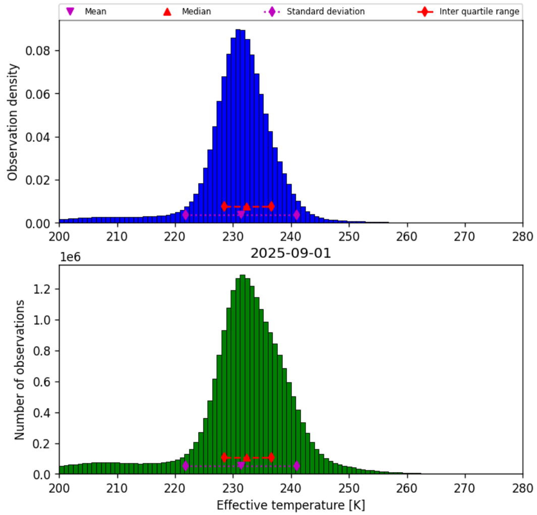
Figure 38: Histogram of “Effective temperature” for 2025-09-01 to 2025-09-02
