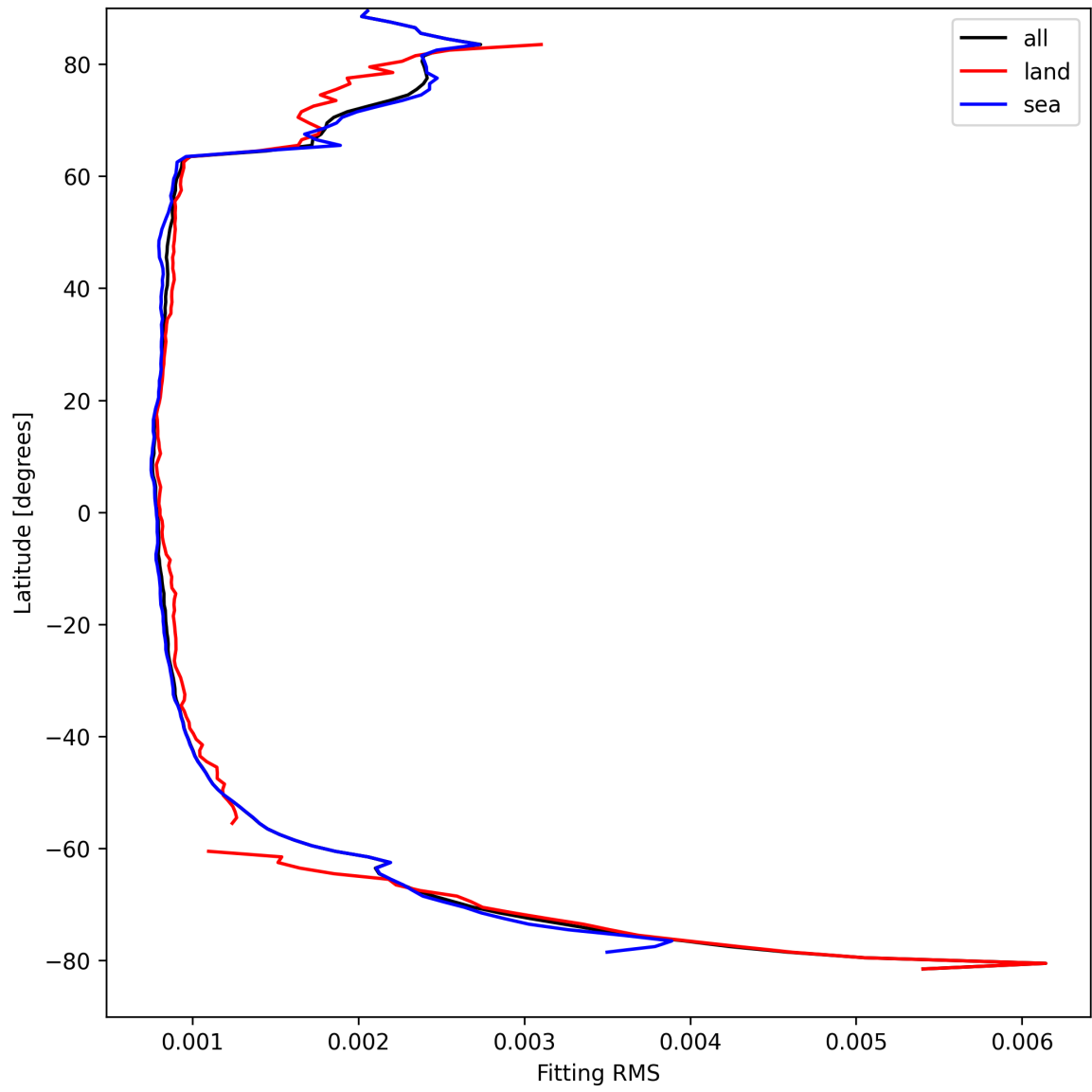
Figure 22: Zonal average of “Fitting RMS” for 2025-09-01 to 2025-09-02.
