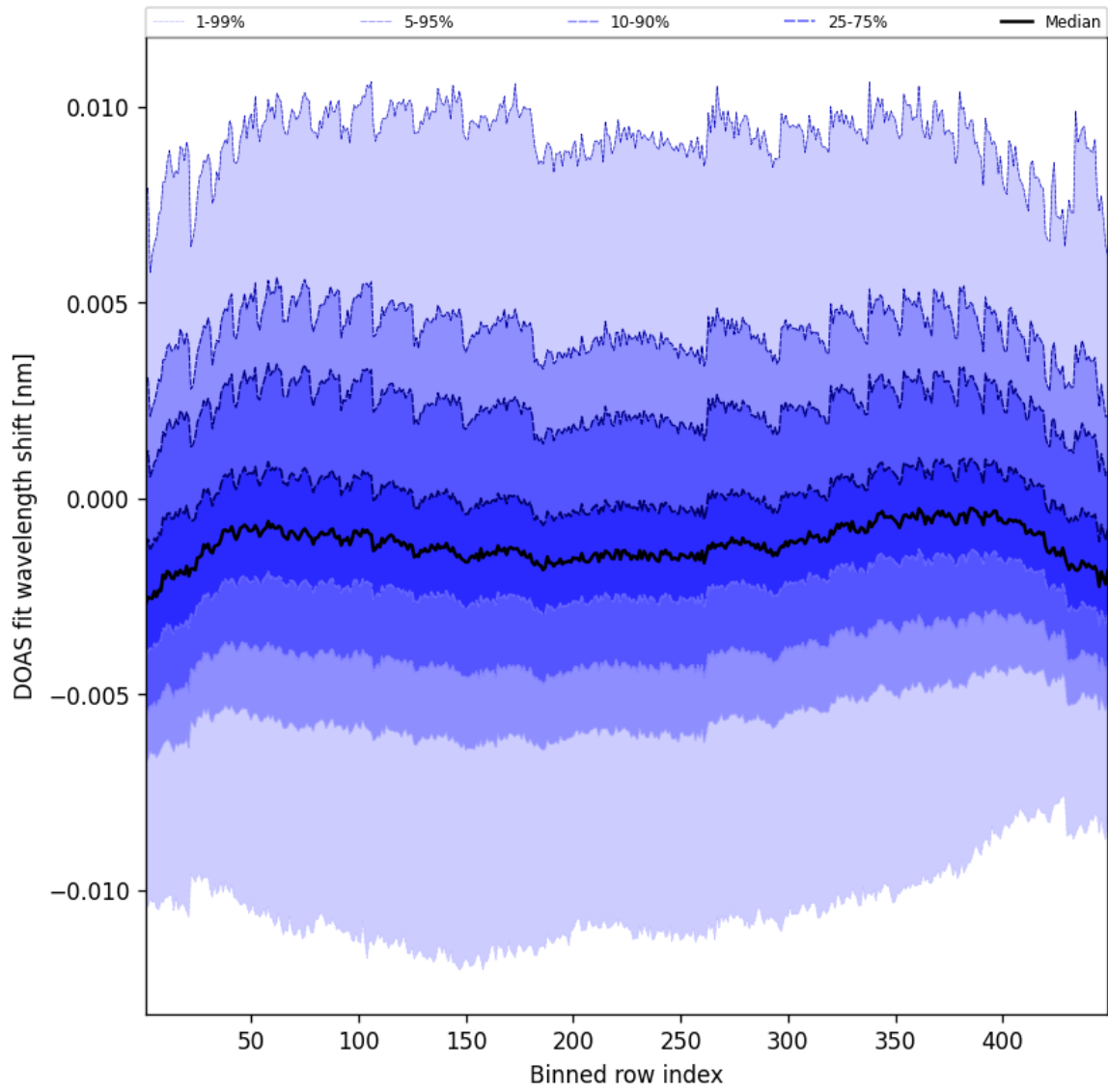
Figure 47: Along track statistics of “DOAS fit wavelength shift” for 2025-09-01 to 2025-09-02
