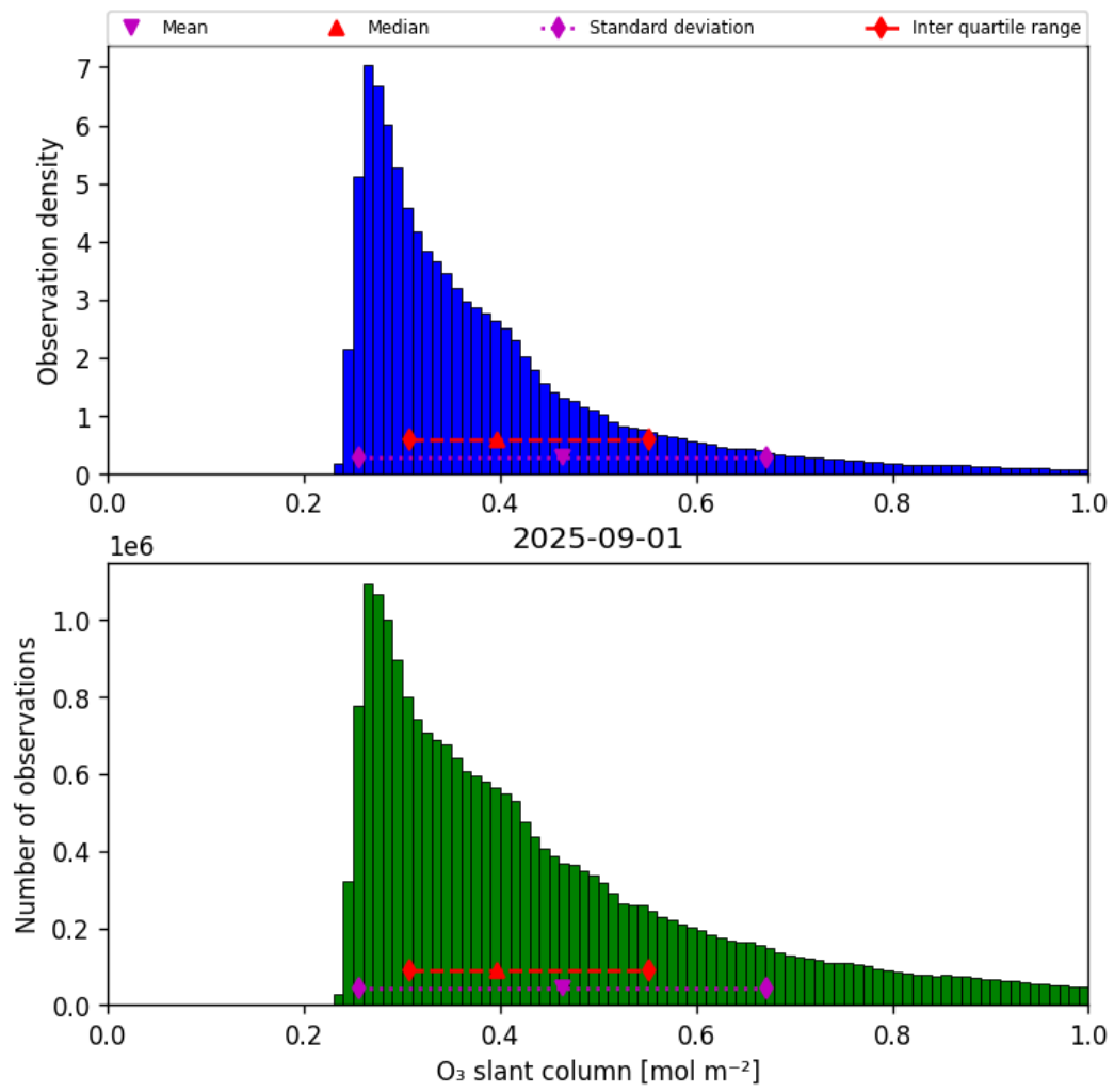
Figure 31: Histogram of “O 3 slant column” for 2025-09-01 to 2025-09-02
