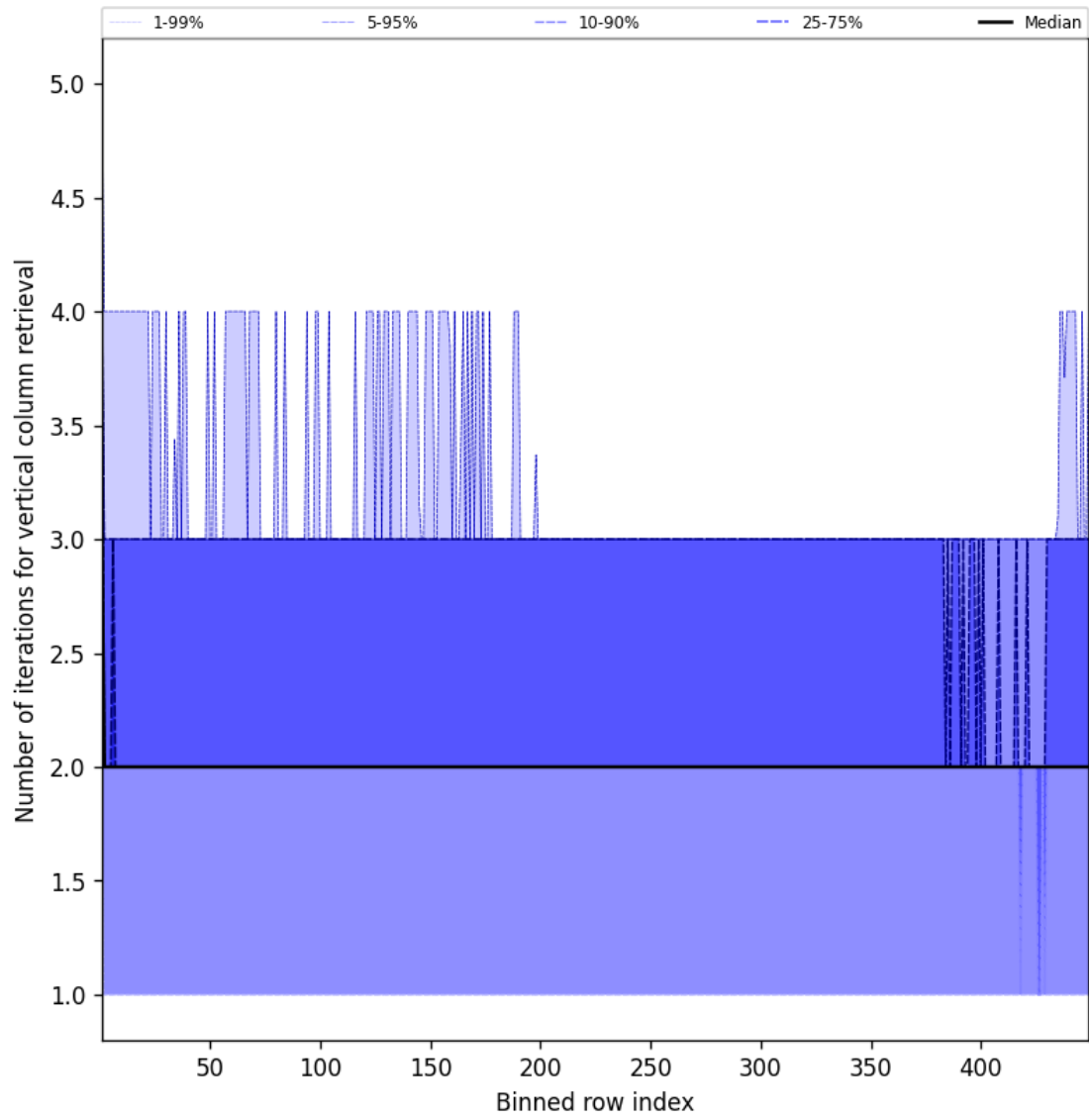
Figure 51: Along track statistics of “Number of iterations for vertical column retrieval” for 2025-09-01 to 2025-09-02
