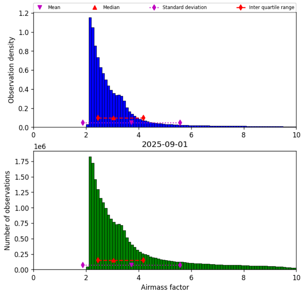
Figure 37: Histogram of “Airmass factor” for 2025-09-01 to 2025-09-02
