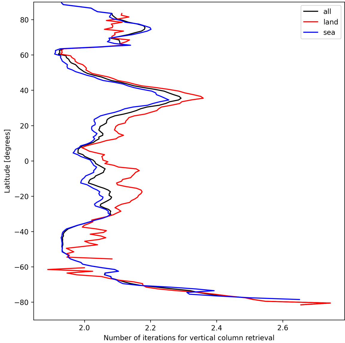
Figure 27: Zonal average of “Number of iterations for vertical column retrieval” for 2025-09-01 to 2025-09-02.
