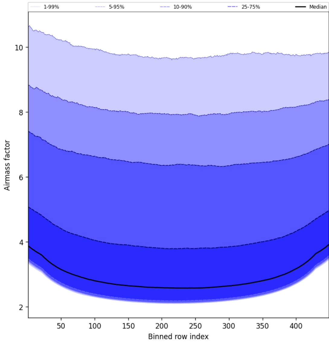
Figure 49: Along track statistics of “Airmass factor” for 2025-09-01 to 2025-09-02
