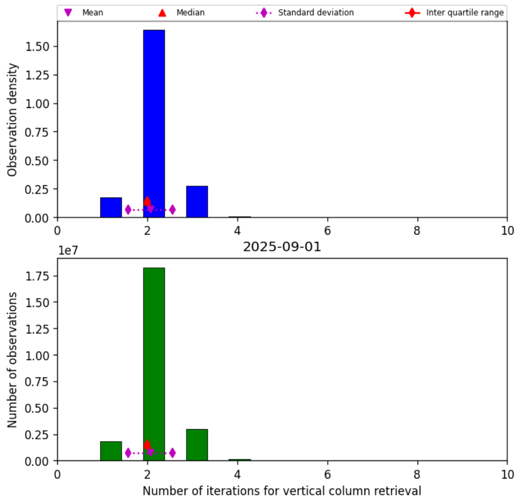
Figure 39: Histogram of “Number of iterations for vertical column retrieval” for 2025-09-01 to 2025-09-02
