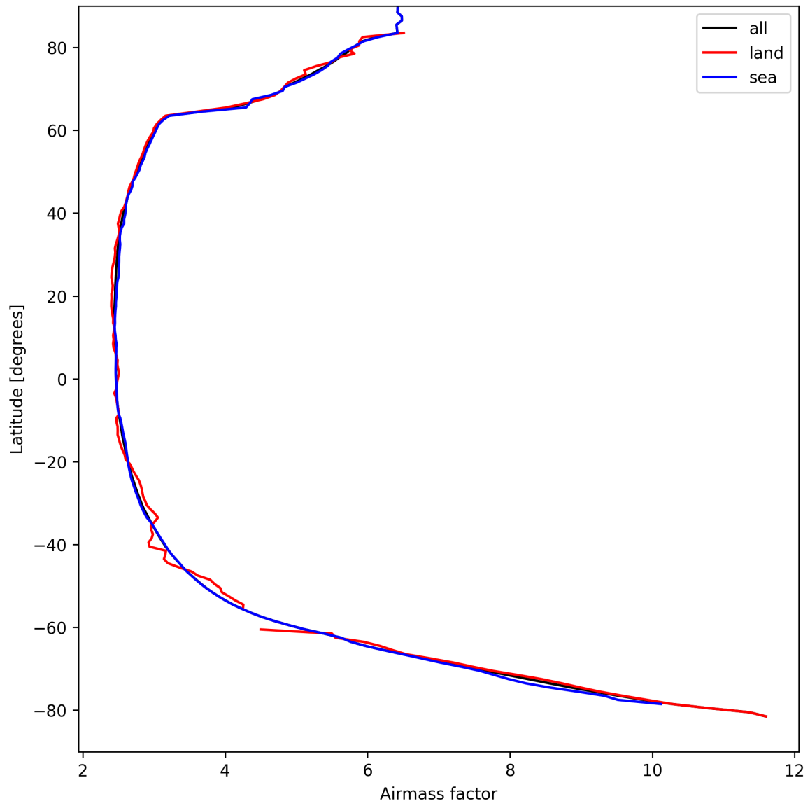
Figure 25: Zonal average of “Airmass factor” for 2025-09-01 to 2025-09-02.
