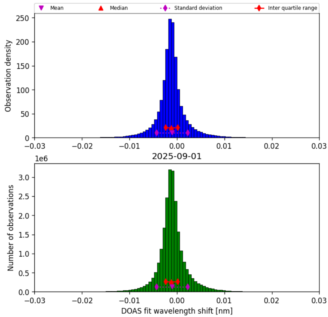
Figure 35: Histogram of “DOAS fit wavelength shift” for 2025-09-01 to 2025-09-02
