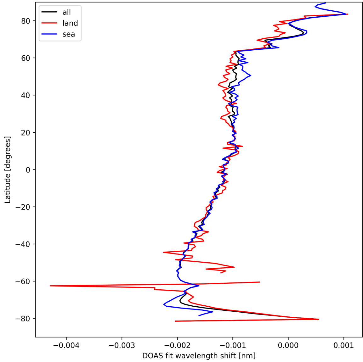
Figure 23: Zonal average of "DOAS fit wavelength shift" for 2025-09-01 to 2025-09-02.
