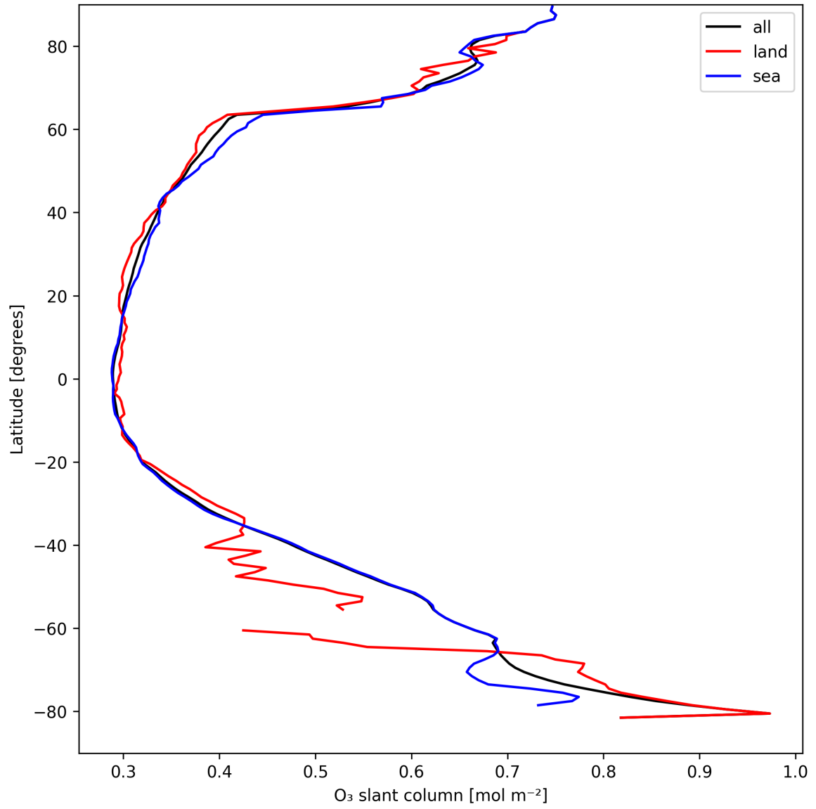
Figure 19: Zonal average of “O 3 slant column” for 2025-09-01 to 2025-09-02.
