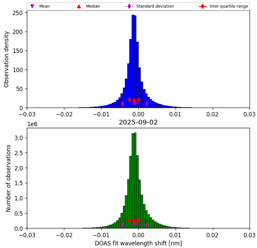
Figure 35: Histogram of “DOAS fit wavelength shift” for 2025-09-02 to 2025-09-02
