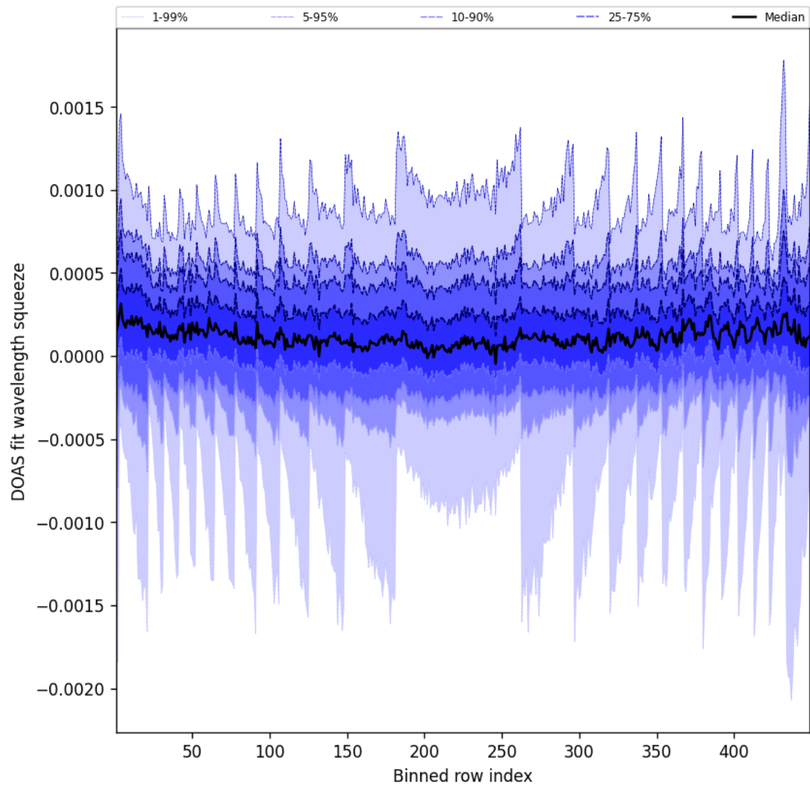
Figure 48: Along track statistics of “DOAS fit wavelength squeeze” for 2025-09-02 to 2025-09-02
