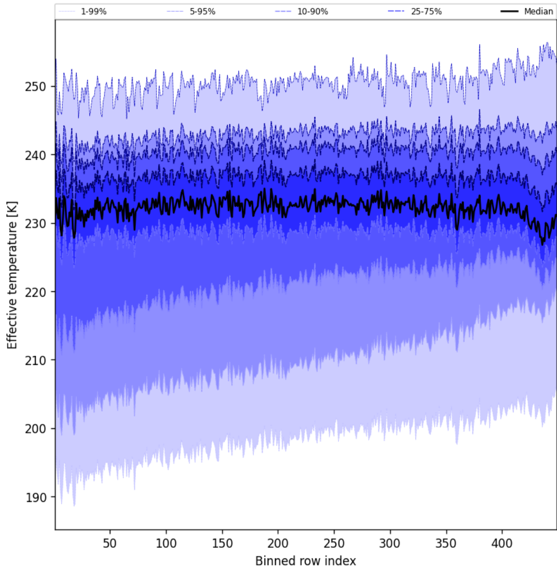
Figure 50: Along track statistics of “Effective temperature” for 2025-09-02 to 2025-09-02
