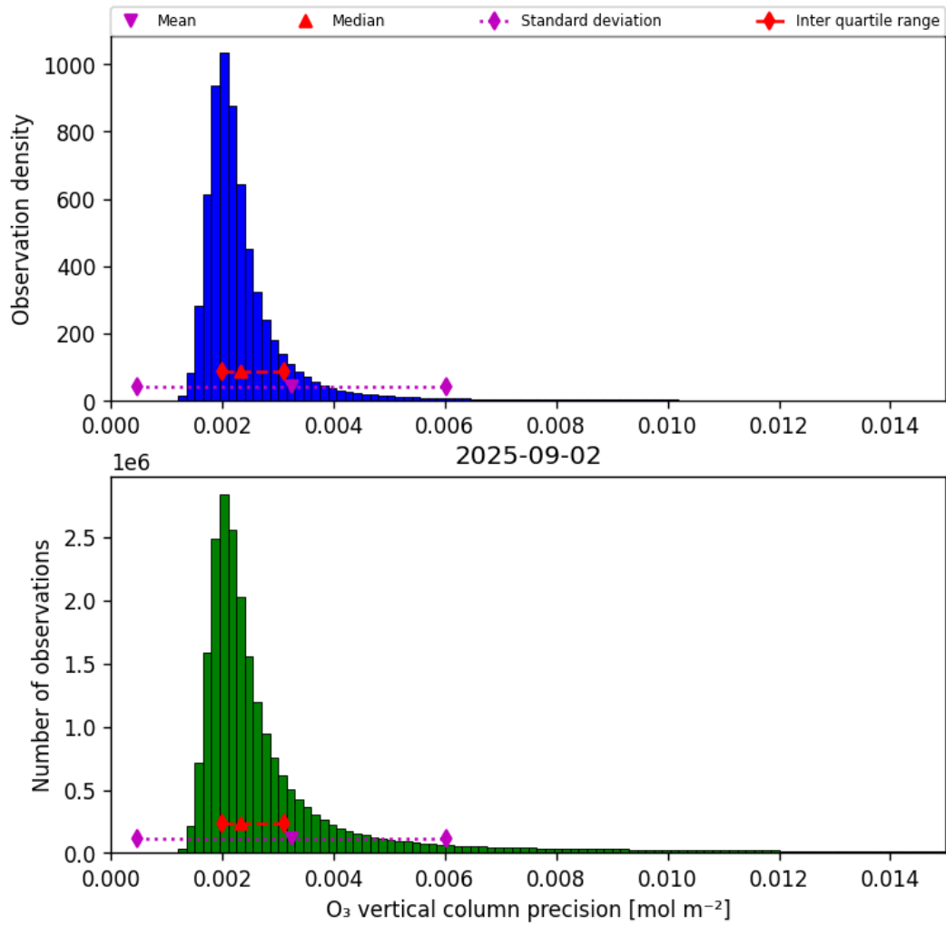
Figure 30: Histogram of “O 3 vertical column precision” for 2025-09-02 to 2025-09-02
