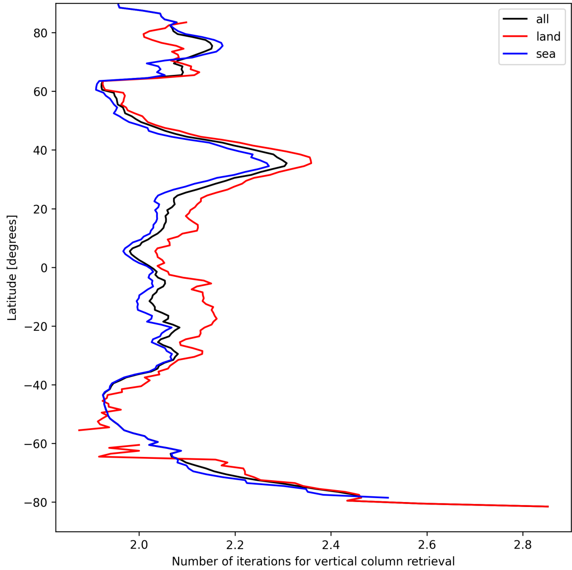
Figure 27: Zonal average of “Number of iterations for vertical column retrieval” for 2025-09-02 to 2025-09-02.
