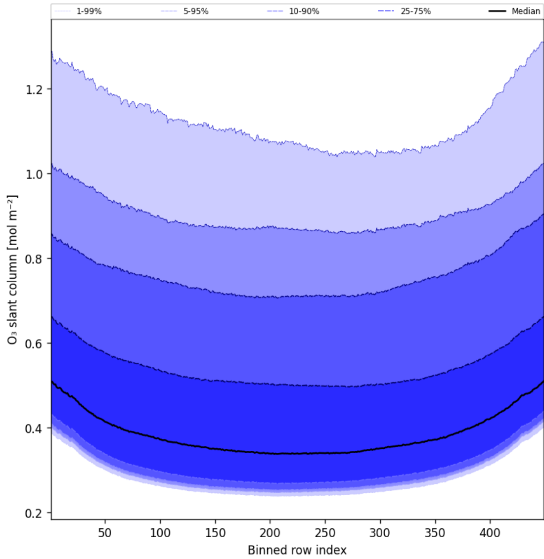
Figure 43: Along track statistics of “O 3 slant column” for 2025-09-02 to 2025-09-02
