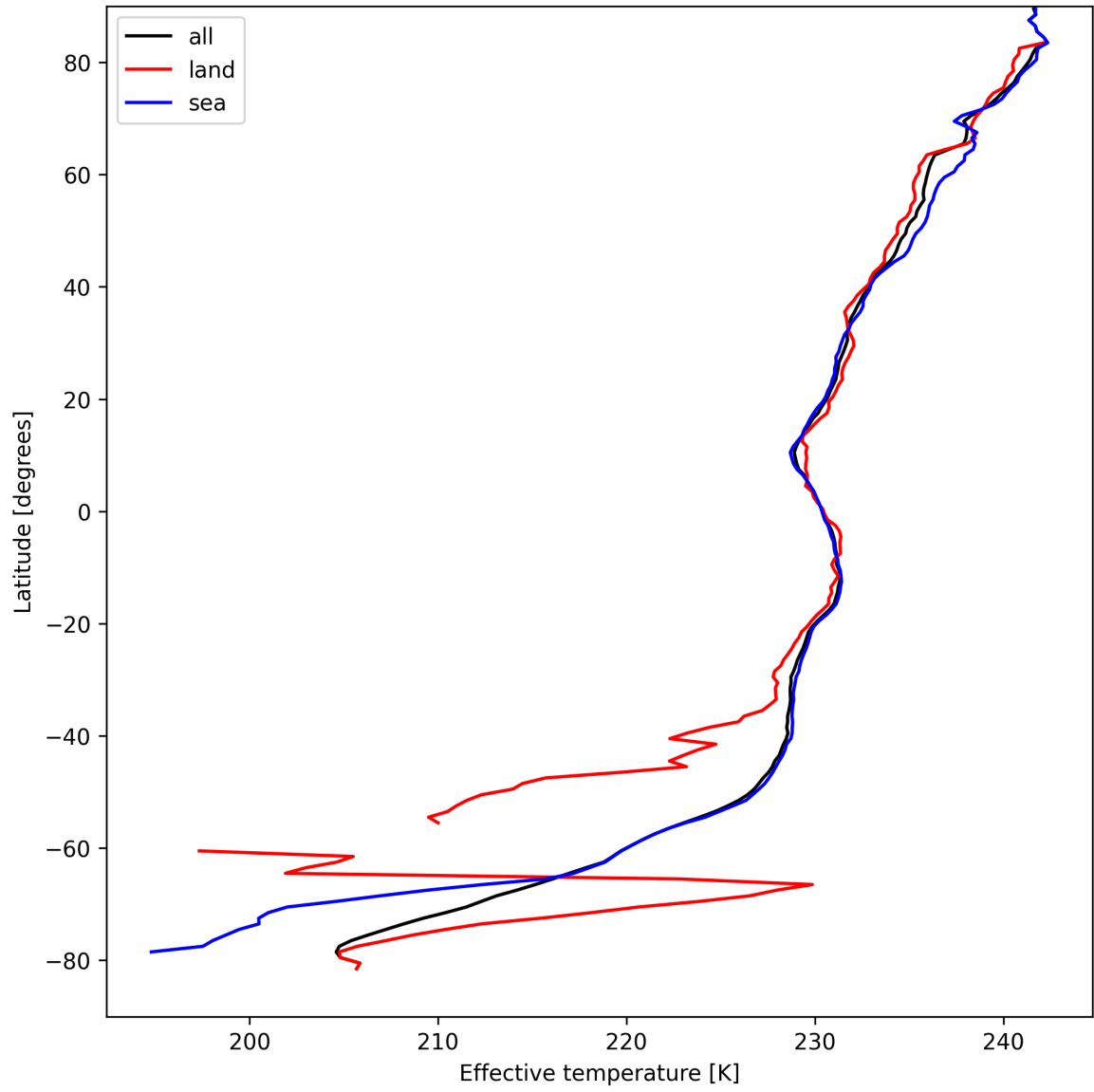
Figure 26: Zonal average of "Effective temperature" for 2025-09-02 to 2025-09-02.
