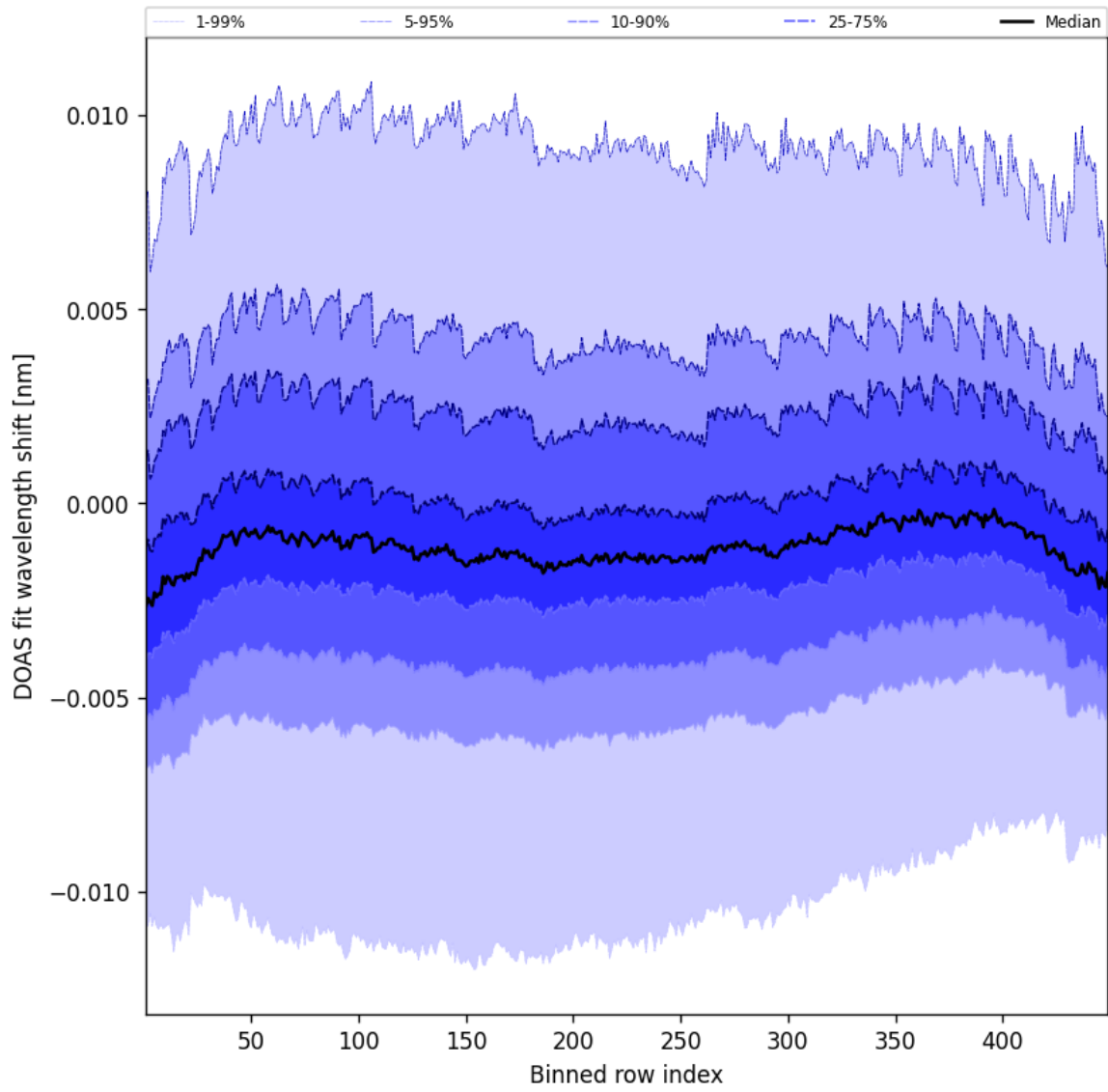
Figure 47: Along track statistics of “DOAS fit wavelength shift” for 2025-09-02 to 2025-09-02
