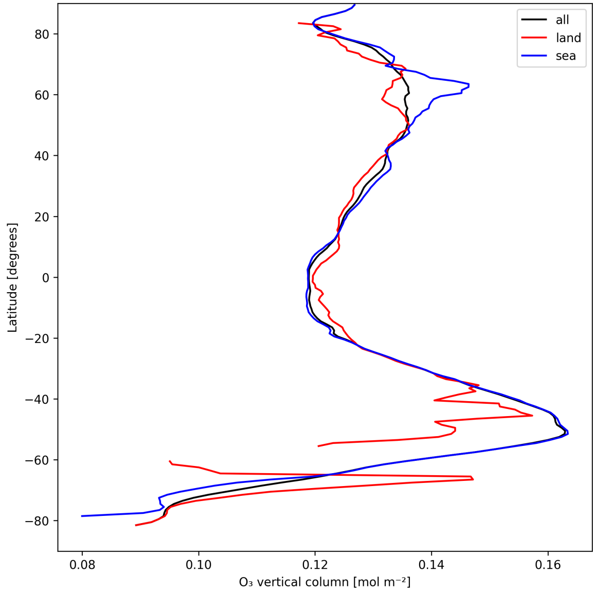
Figure 17: Zonal average of “O 3 vertical column” for 2025-09-02 to 2025-09-02.
