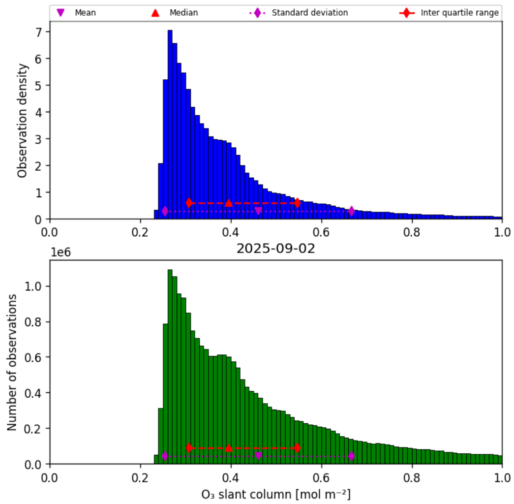
Figure 31: Histogram of “O 3 slant column” for 2025-09-02 to 2025-09-02
