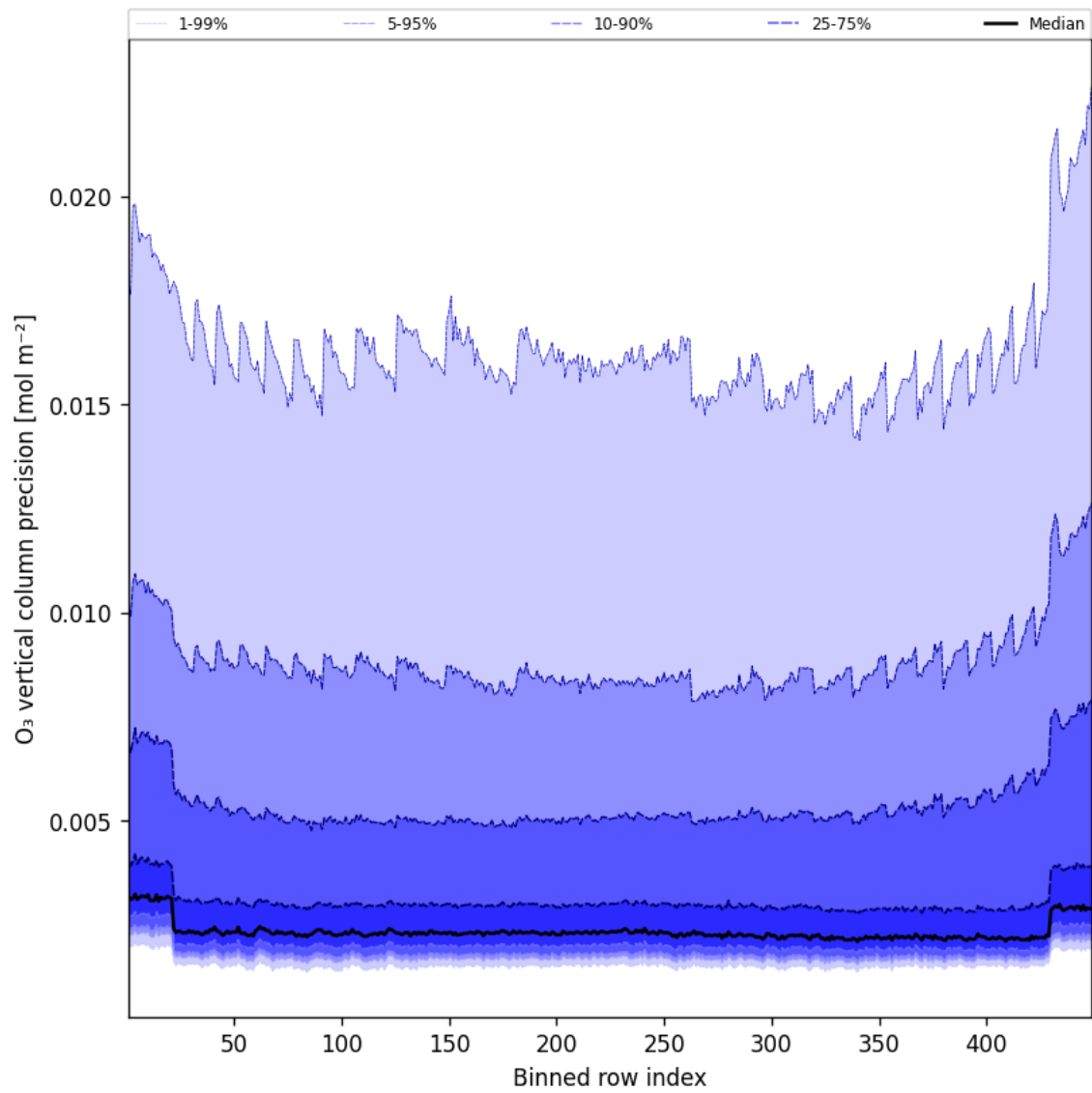
Figure 42: Along track statistics of “O 3 vertical column precision” for 2025-09-02 to 2025-09-02
