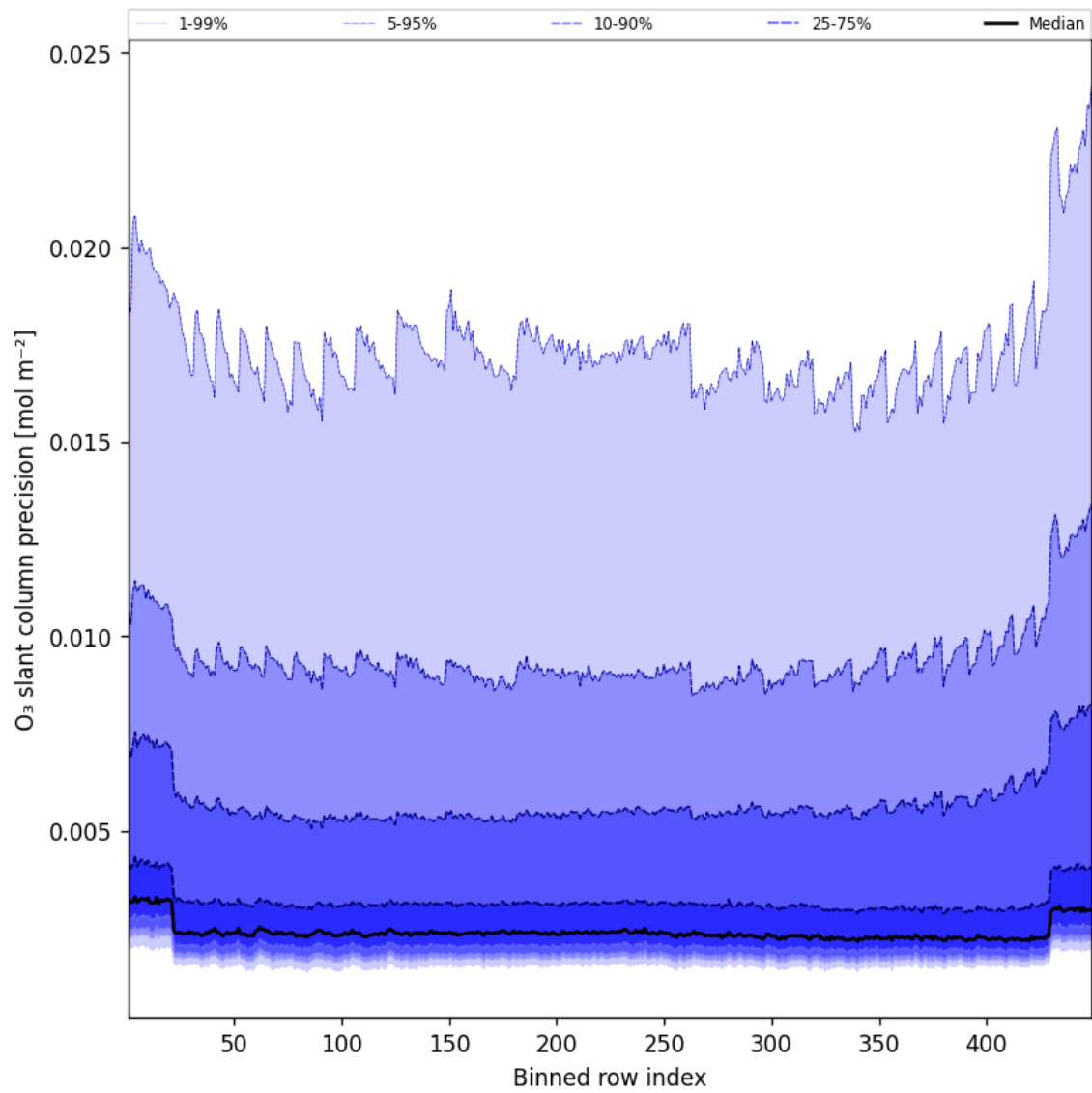
Figure 44: Along track statistics of “O 3 slant column precision” for 2025-09-02 to 2025-09-02
