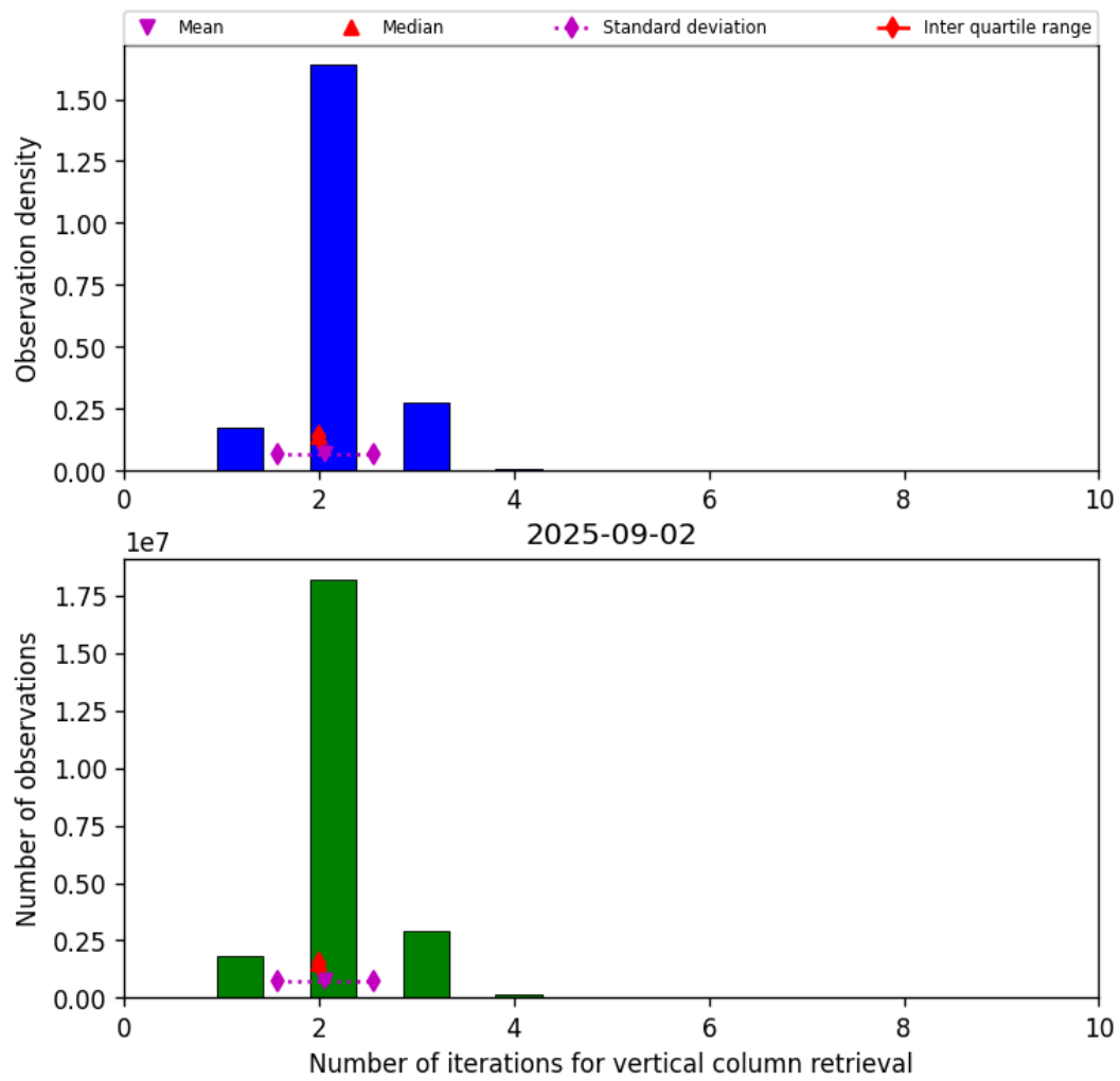
Figure 39: Histogram of “Number of iterations for vertical column retrieval” for 2025-09-02 to 2025-09-02
