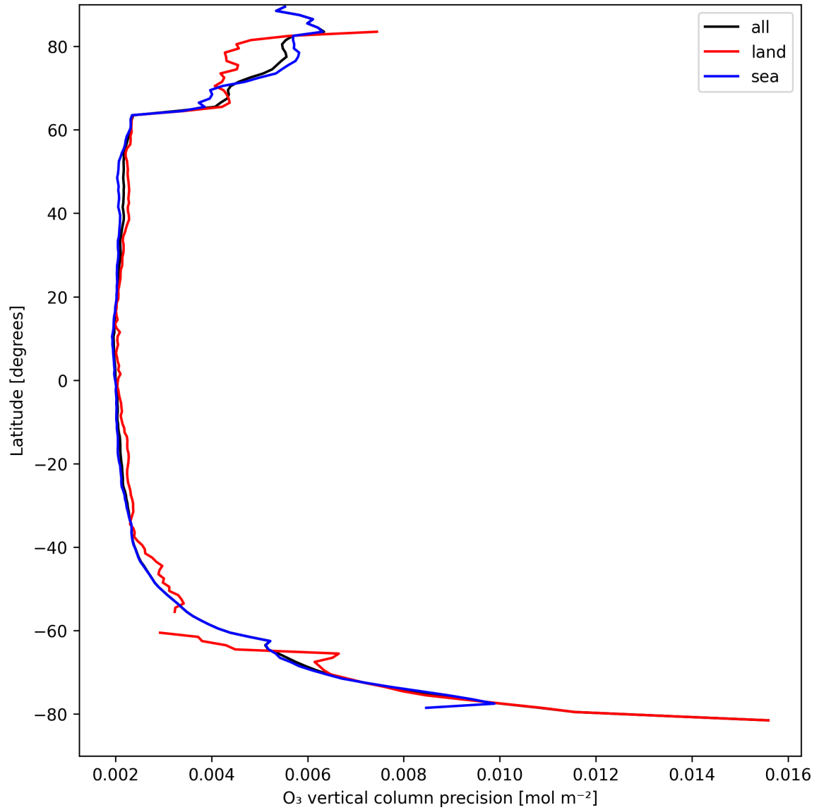
Figure 18: Zonal average of “O 3 vertical column precision” for 2025-09-02 to 2025-09-02.
