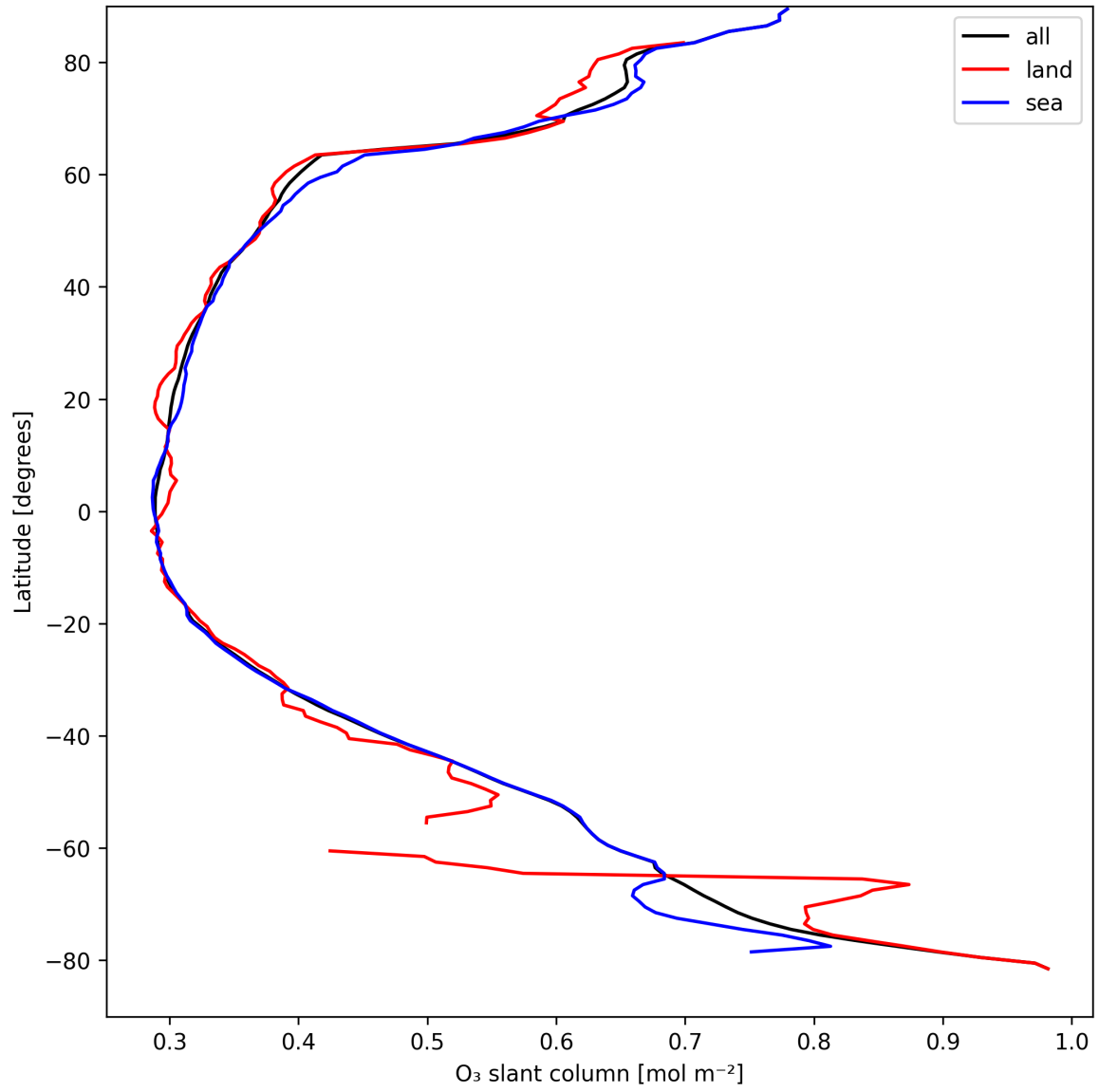
Figure 19: Zonal average of “O 3 slant column” for 2025-09-02 to 2025-09-02.
