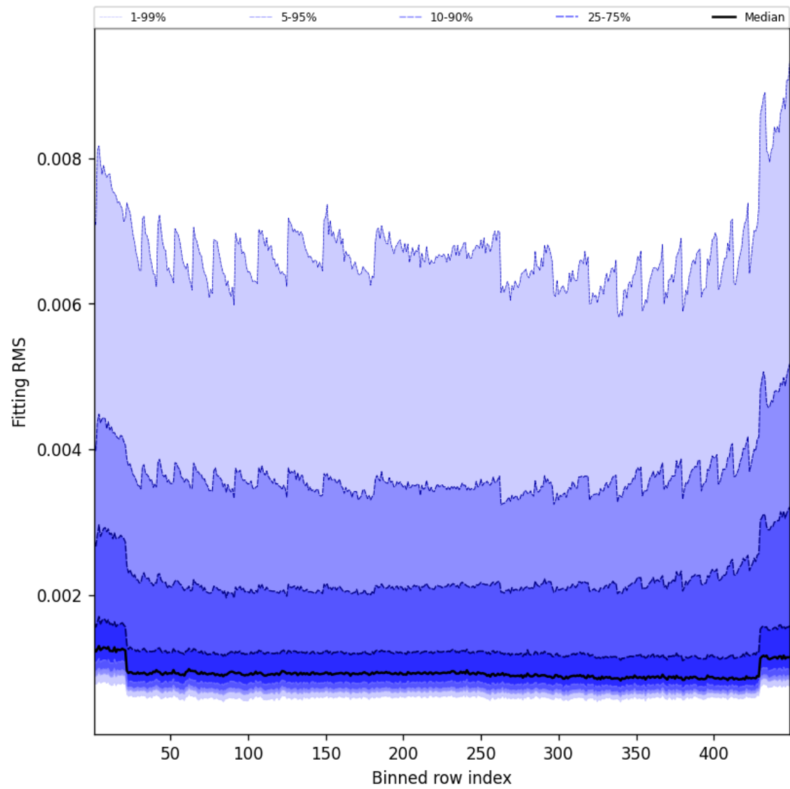
Figure 46: Along track statistics of “Fitting RMS” for 2025-09-02 to 2025-09-02
