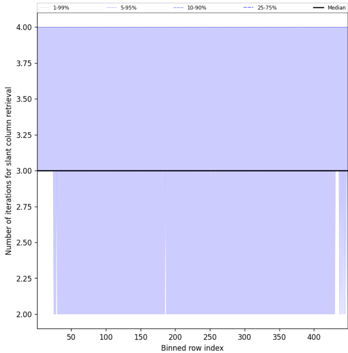
Figure 45: Along track statistics of “Number of iterations for slant column retrieval” for 2025-09-02 to 2025-09-02
