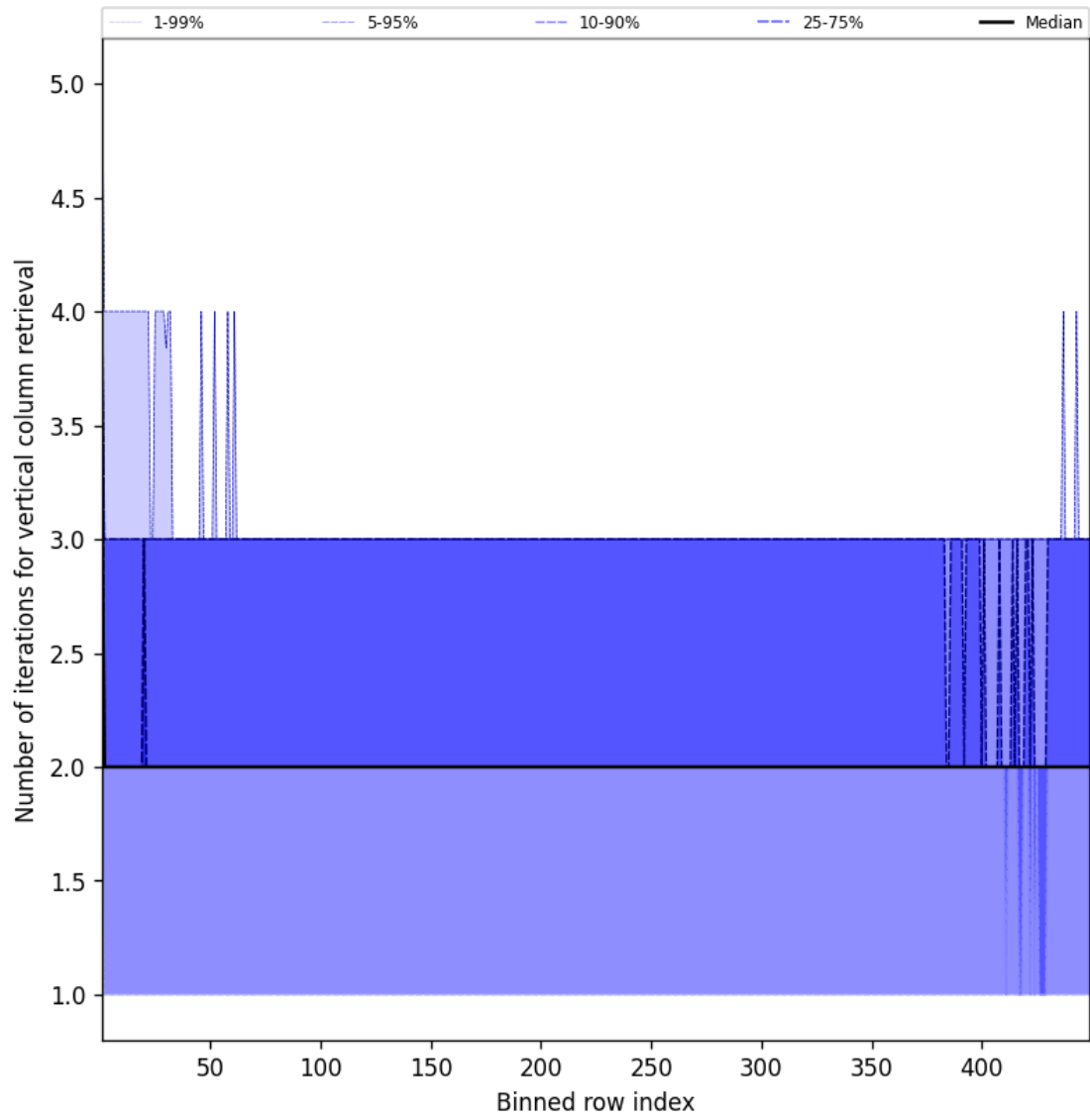
Figure 51: Along track statistics of “Number of iterations for vertical column retrieval” for 2025-09-02 to 2025-09-02
