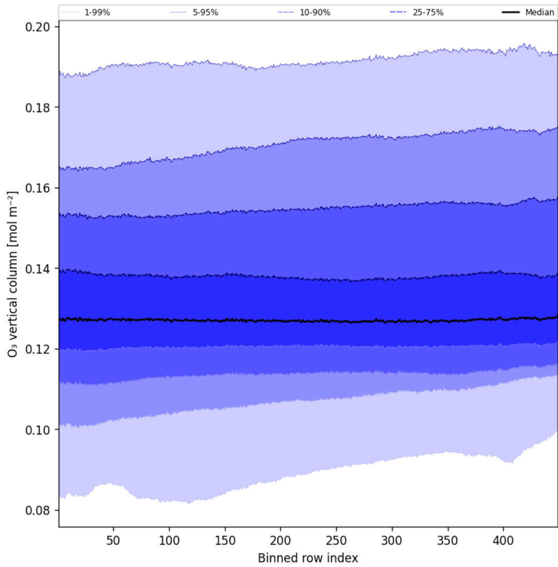
Figure 41: Along track statistics of “O 3 vertical column” for 2025-09-02 to 2025-09-02
