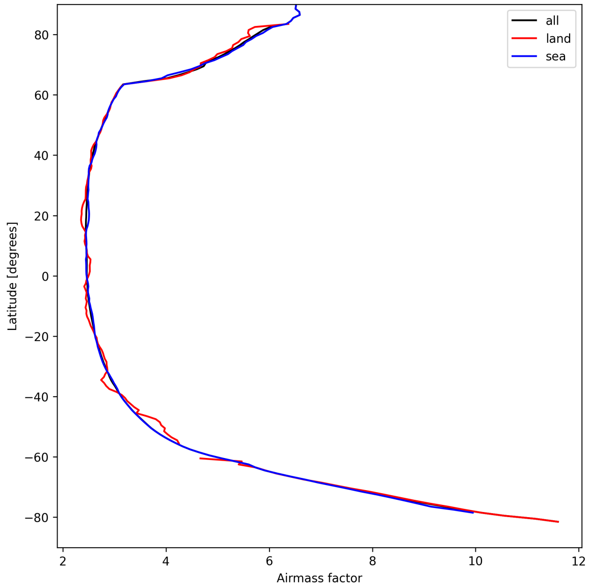
Figure 25: Zonal average of “Airmass factor” for 2025-09-02 to 2025-09-02.
