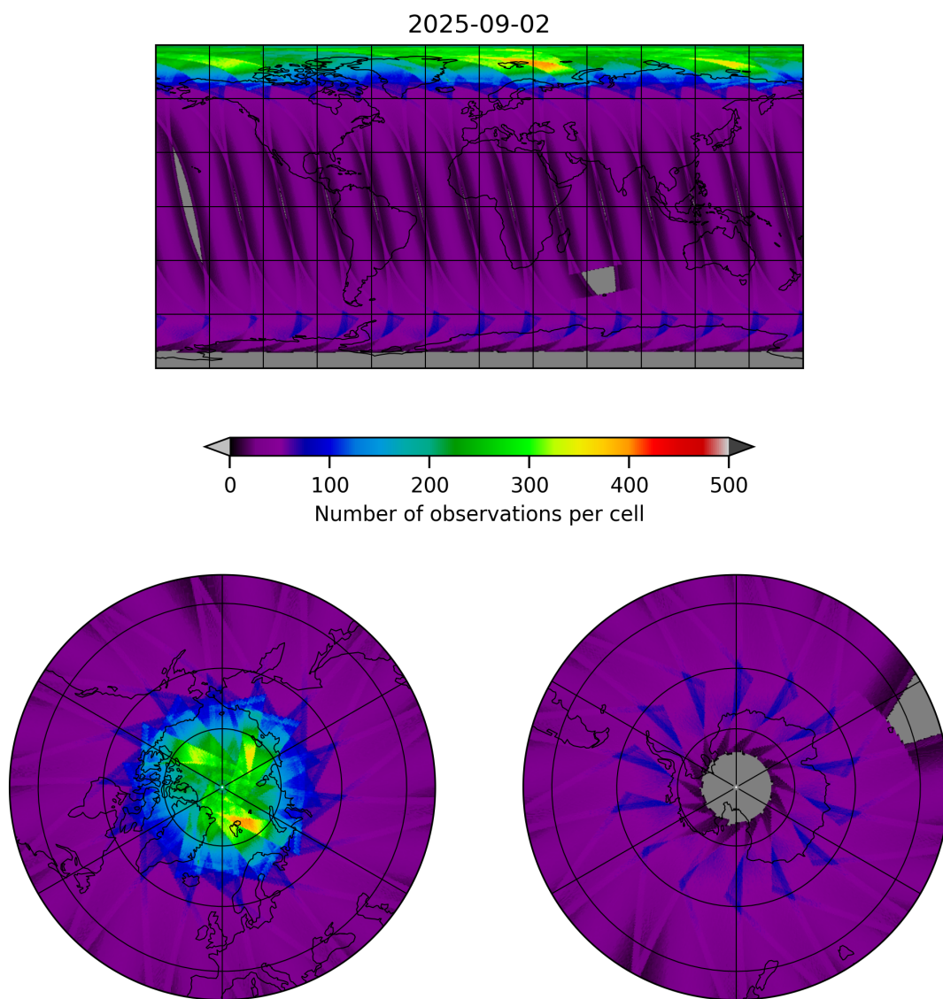
Figure 15: Map of the number of observations for 2025-09-02 to 2025-09-02
