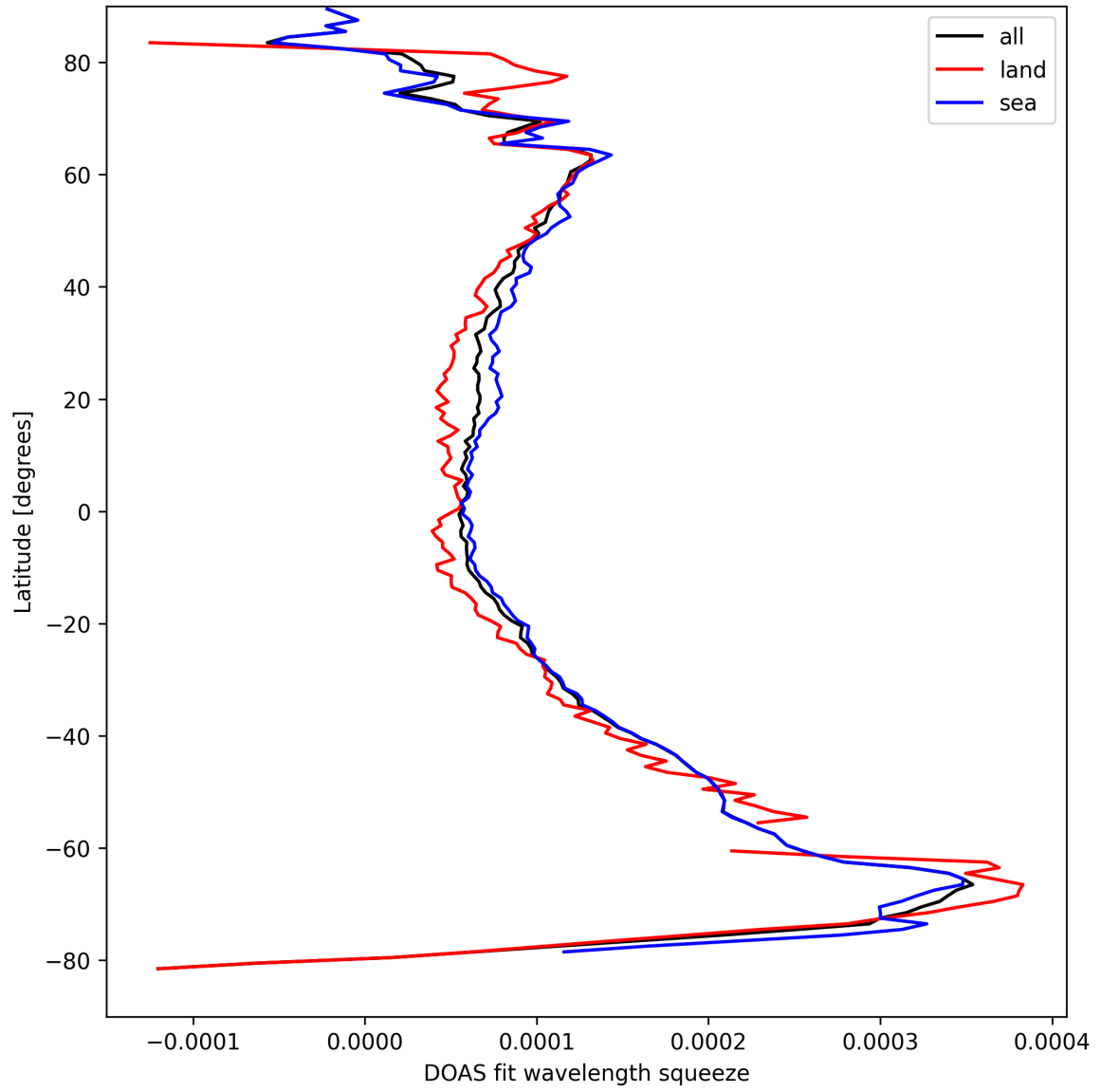
Figure 24: Zonal average of “DOAS fit wavelength squeeze” for 2025-09-02 to 2025-09-02.
