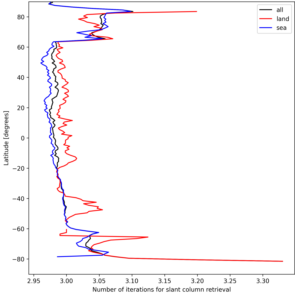
Figure 21: Zonal average of “Number of iterations for slant column retrieval” for 2025-09-02 to 2025-09-02.
