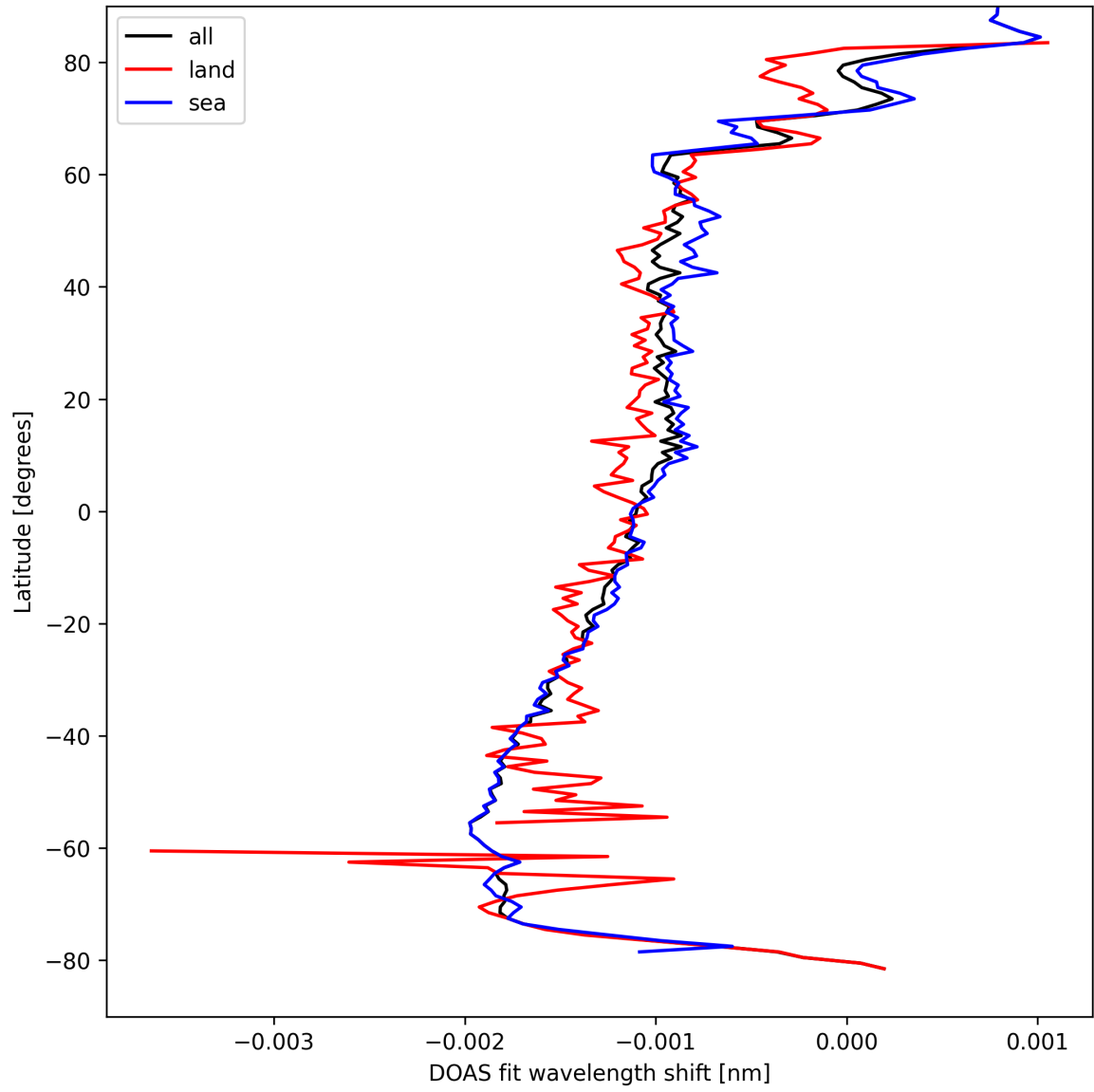
Figure 23: Zonal average of “DOAS fit wavelength shift” for 2025-09-02 to 2025-09-02.
