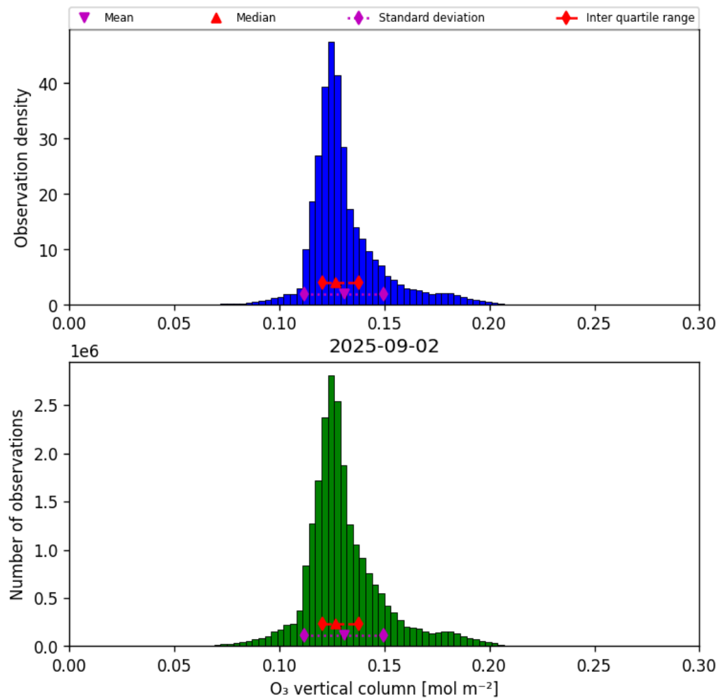
Figure 29: Histogram of “O 3 vertical column” for 2025-09-02 to 2025-09-02
