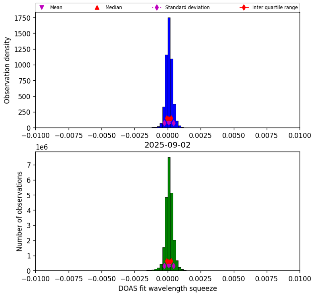
Figure 36: Histogram of “DOAS fit wavelength squeeze” for 2025-09-02 to 2025-09-02
