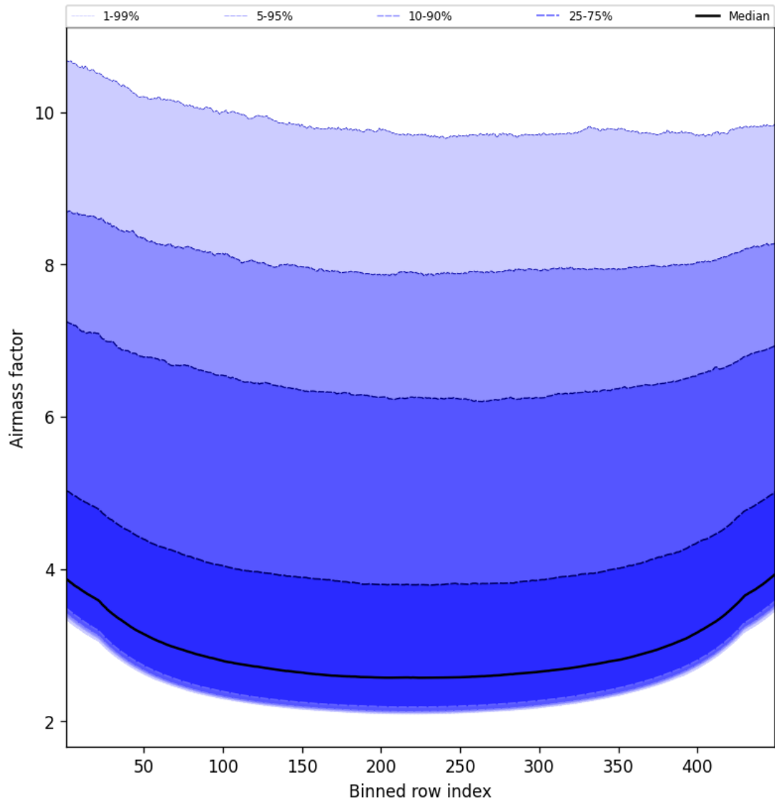
Figure 49: Along track statistics of “Airmass factor” for 2025-09-02 to 2025-09-02
