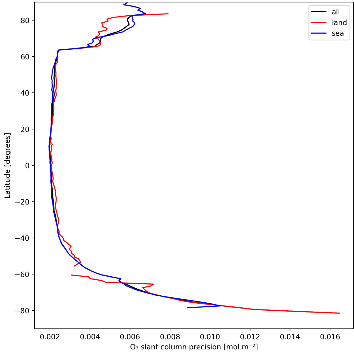
Figure 20: Zonal average of “O 3 slant column precision” for 2025-09-02 to 2025-09-02.
