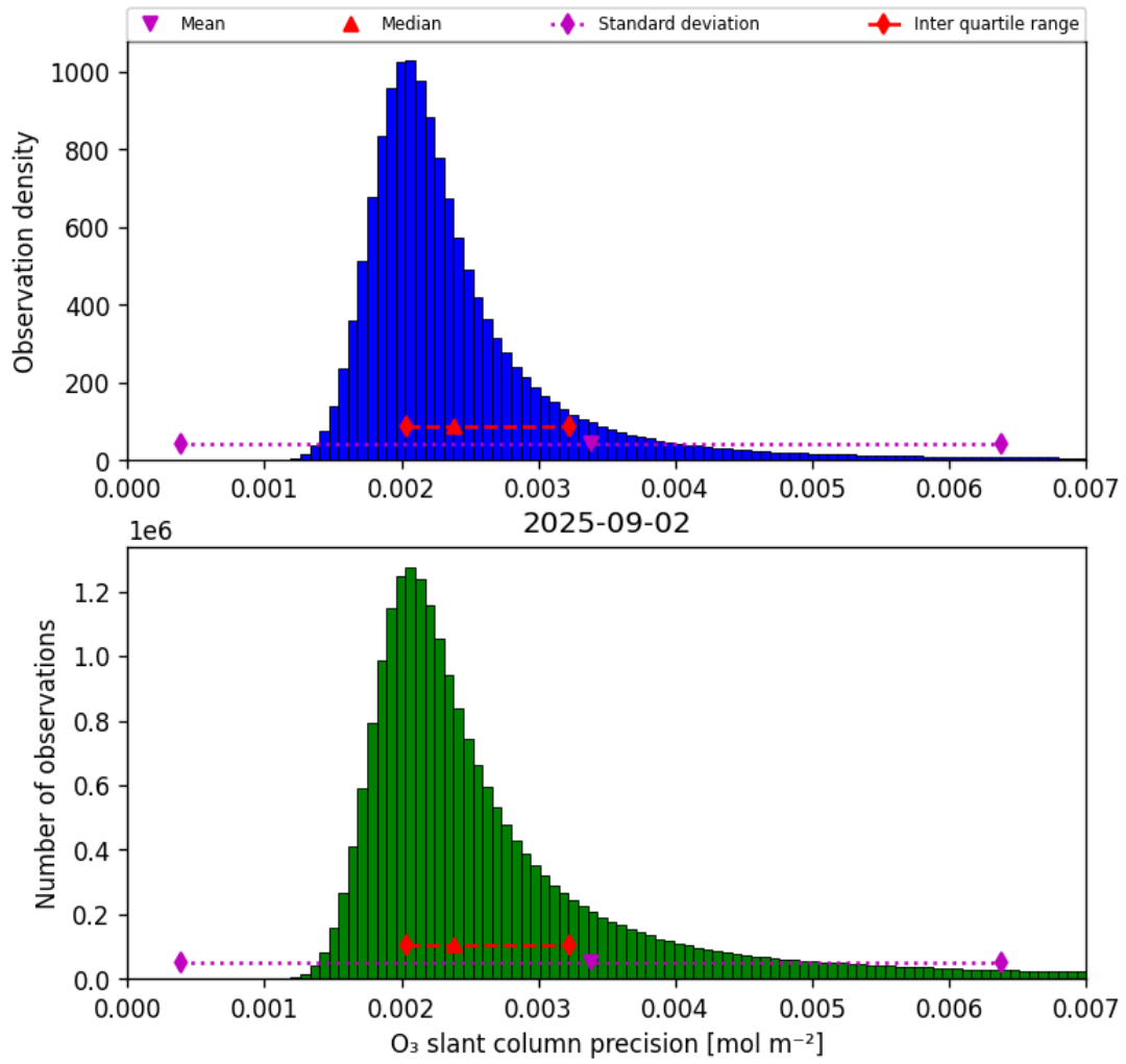
Figure 32: Histogram of “O 3 slant column precision” for 2025-09-02 to 2025-09-02
