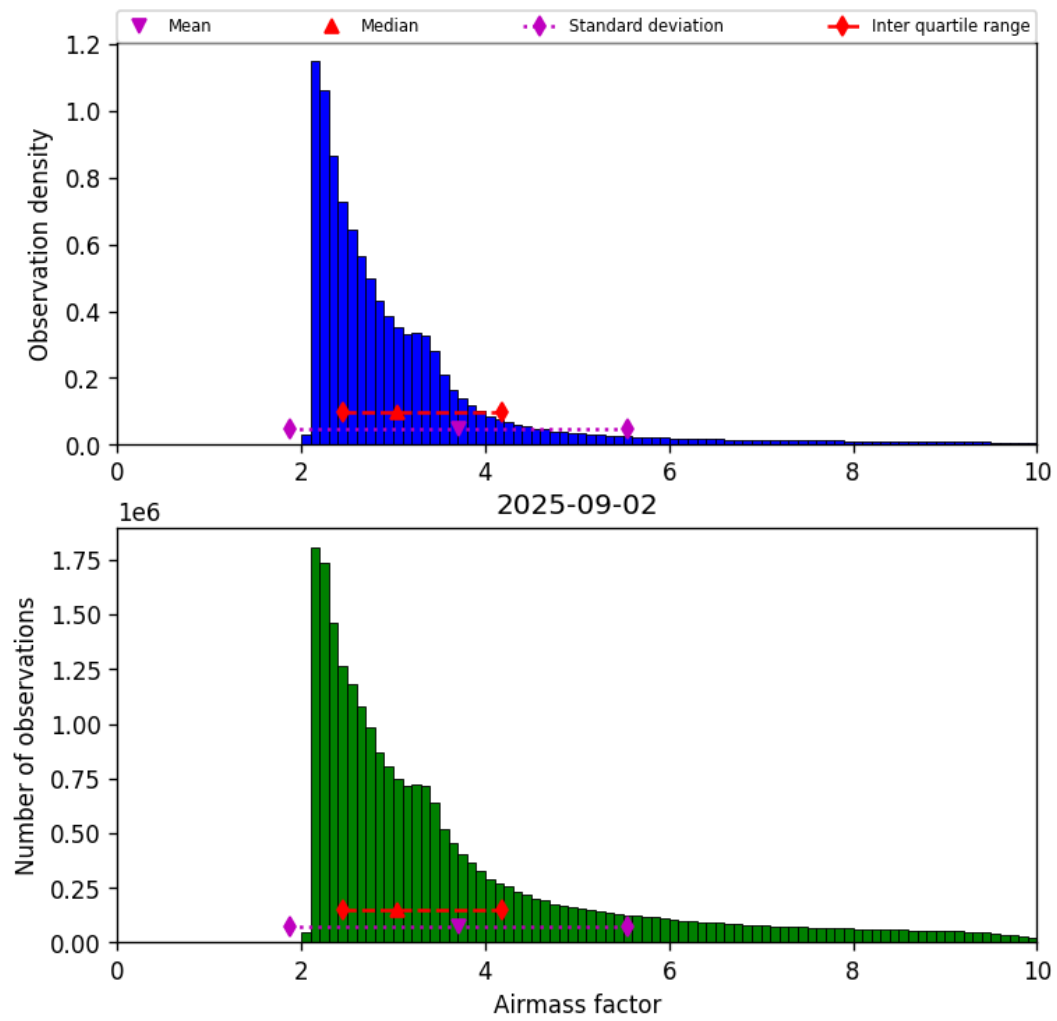
Figure 37: Histogram of “Airmass factor” for 2025-09-02 to 2025-09-02
