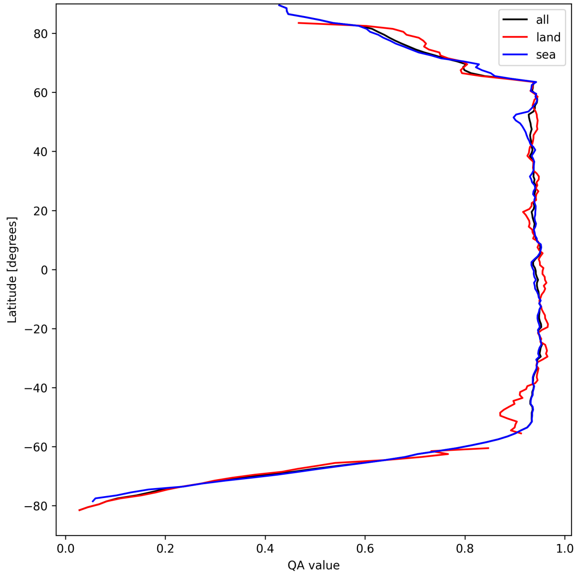
Figure 16: Zonal average of “QA value” for 2025-09-02 to 2025-09-02.
