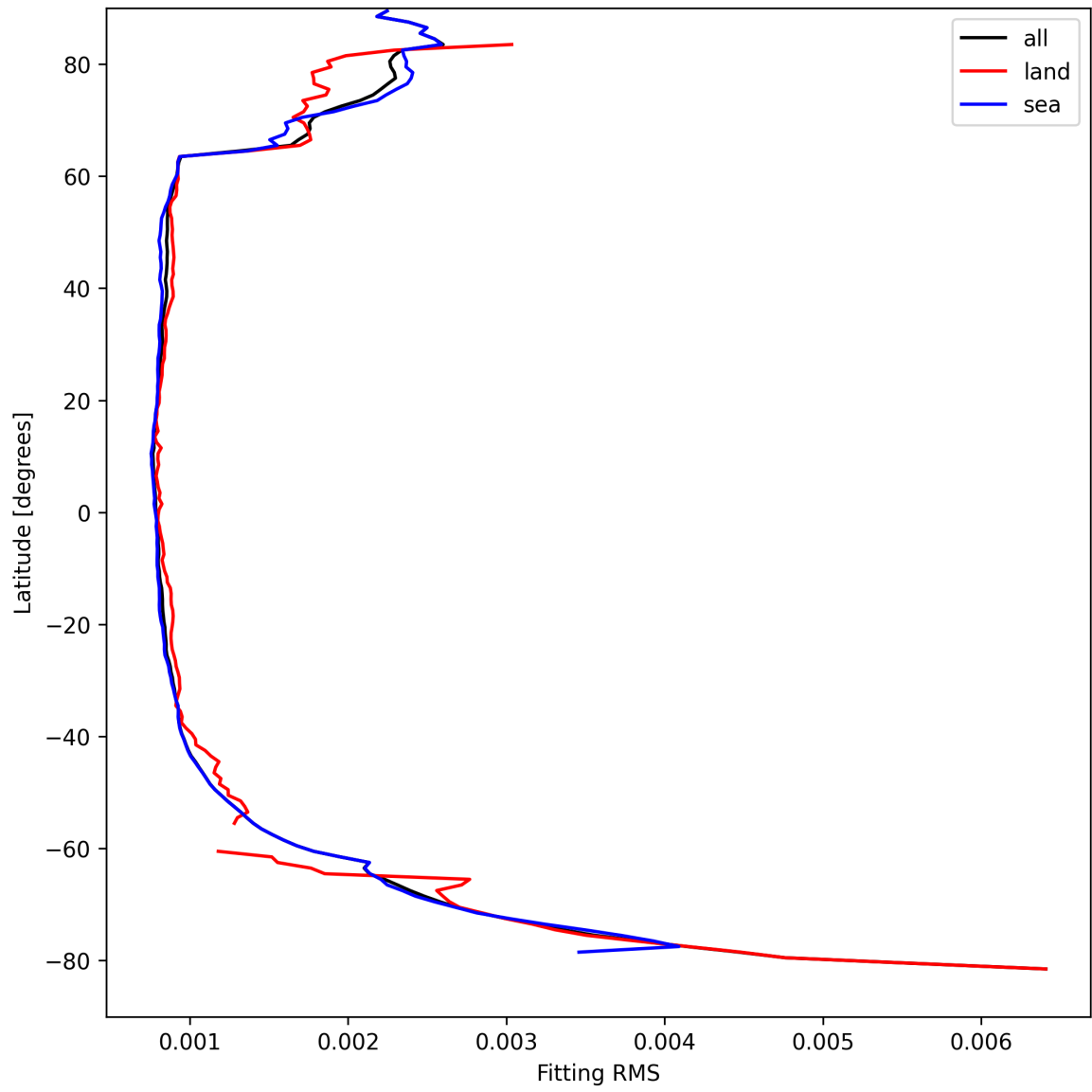
Figure 22: Zonal average of “Fitting RMS” for 2025-09-02 to 2025-09-02.
