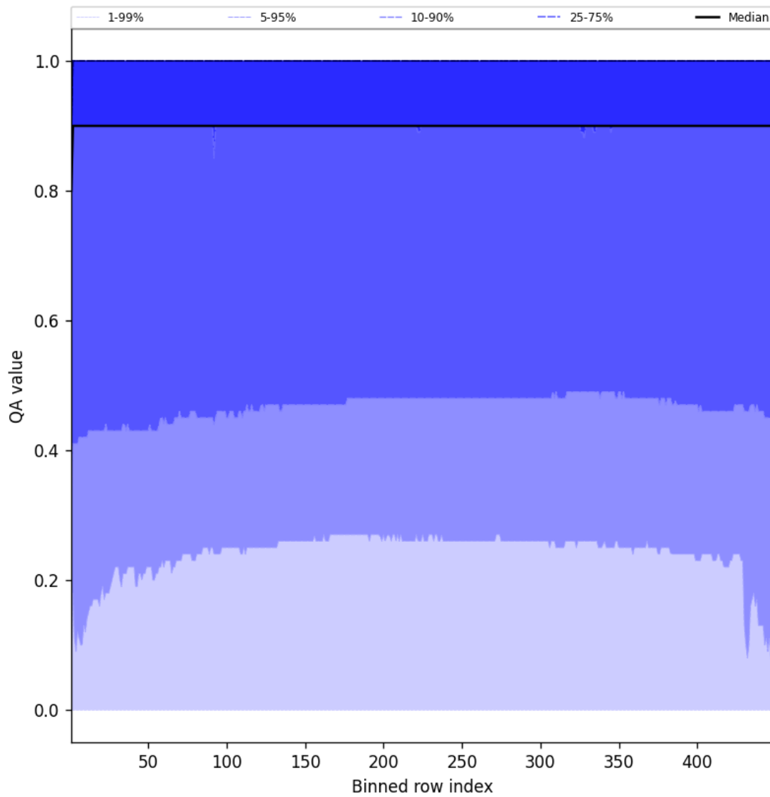
Figure 40: Along track statistics of “QA value” for 2025-09-02 to 2025-09-02
