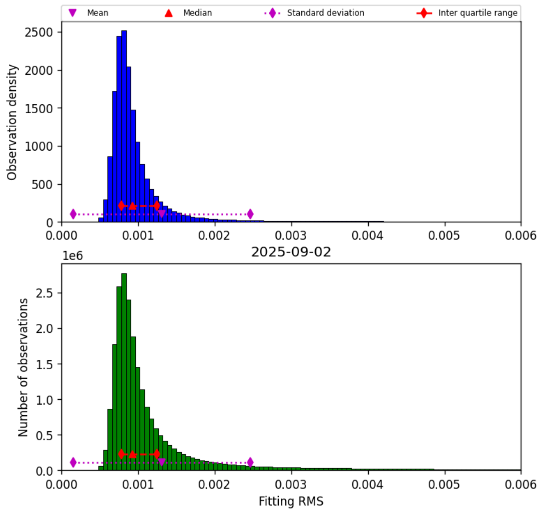
Figure 34: Histogram of “Fitting RMS” for 2025-09-02 to 2025-09-02
