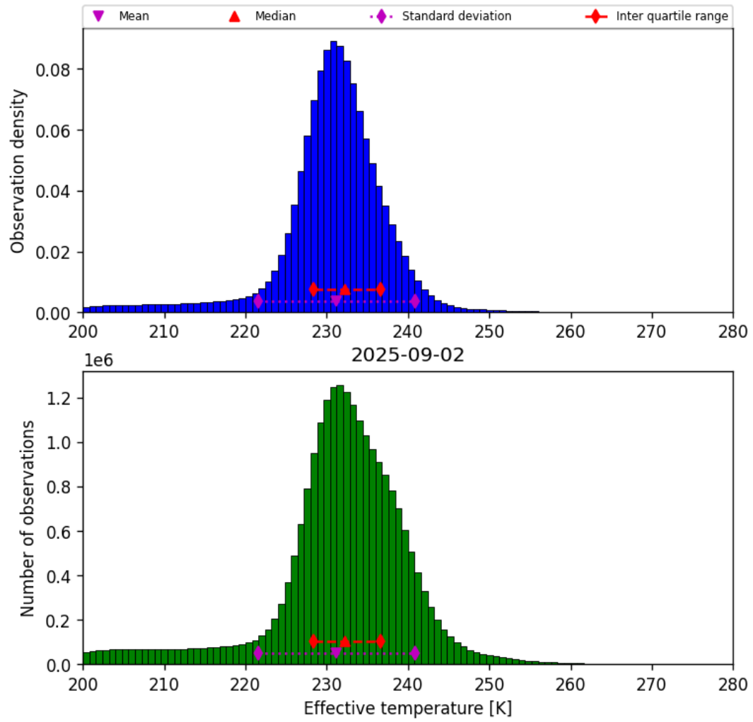
Figure 38: Histogram of “Effective temperature” for 2025-09-02 to 2025-09-02
