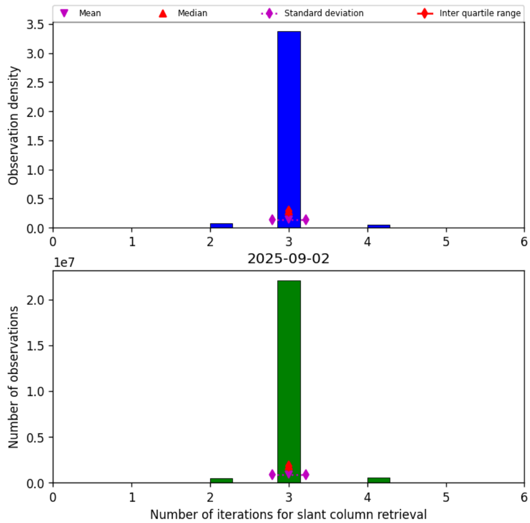
Figure 33: Histogram of “Number of iterations for slant column retrieval” for 2025-09-02 to 2025-09-02
