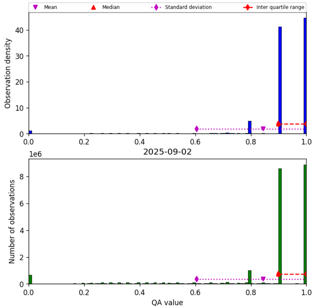
Figure 28: Histogram of “QA value” for 2025-09-02 to 2025-09-02
