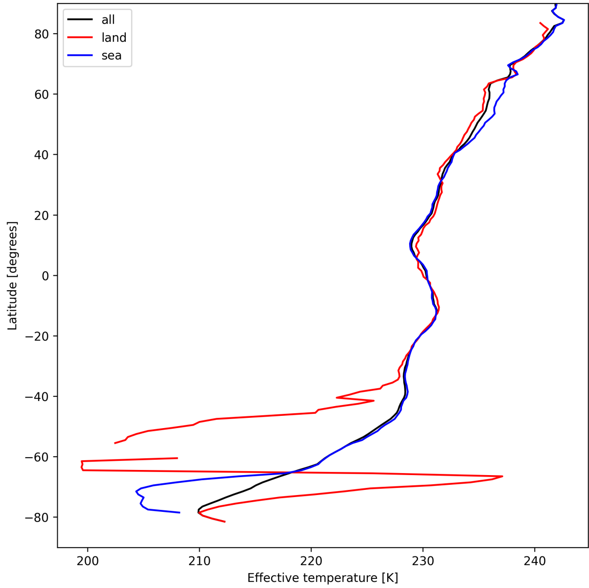
Figure 26: Zonal average of “Effective temperature” for 2025-09-03 to 2025-09-04.
