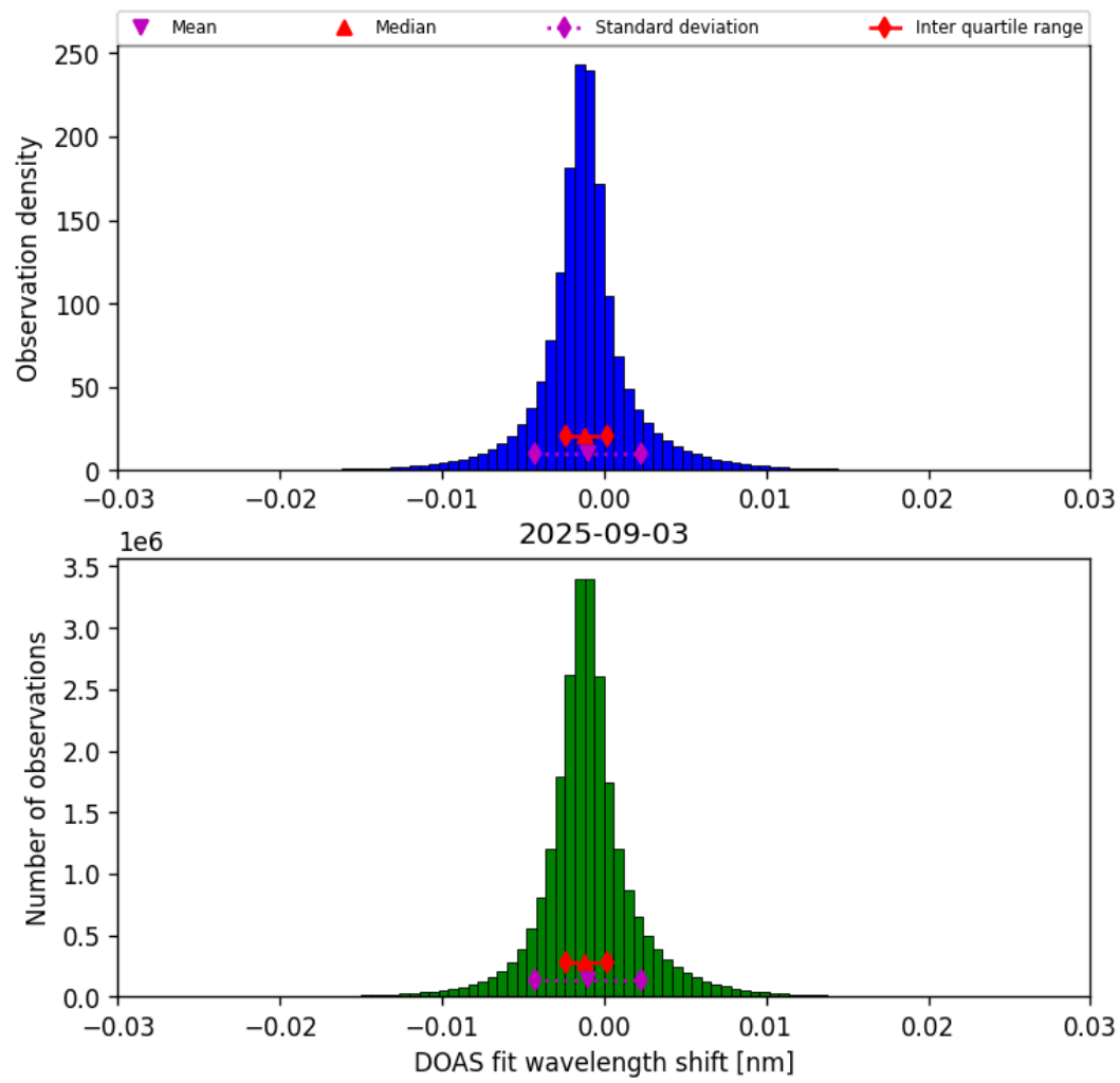
Figure 35: Histogram of “DOAS fit wavelength shift” for 2025-09-03 to 2025-09-04
