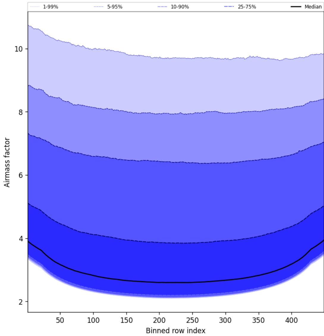
Figure 49: Along track statistics of “Airmass factor” for 2025-09-03 to 2025-09-04
