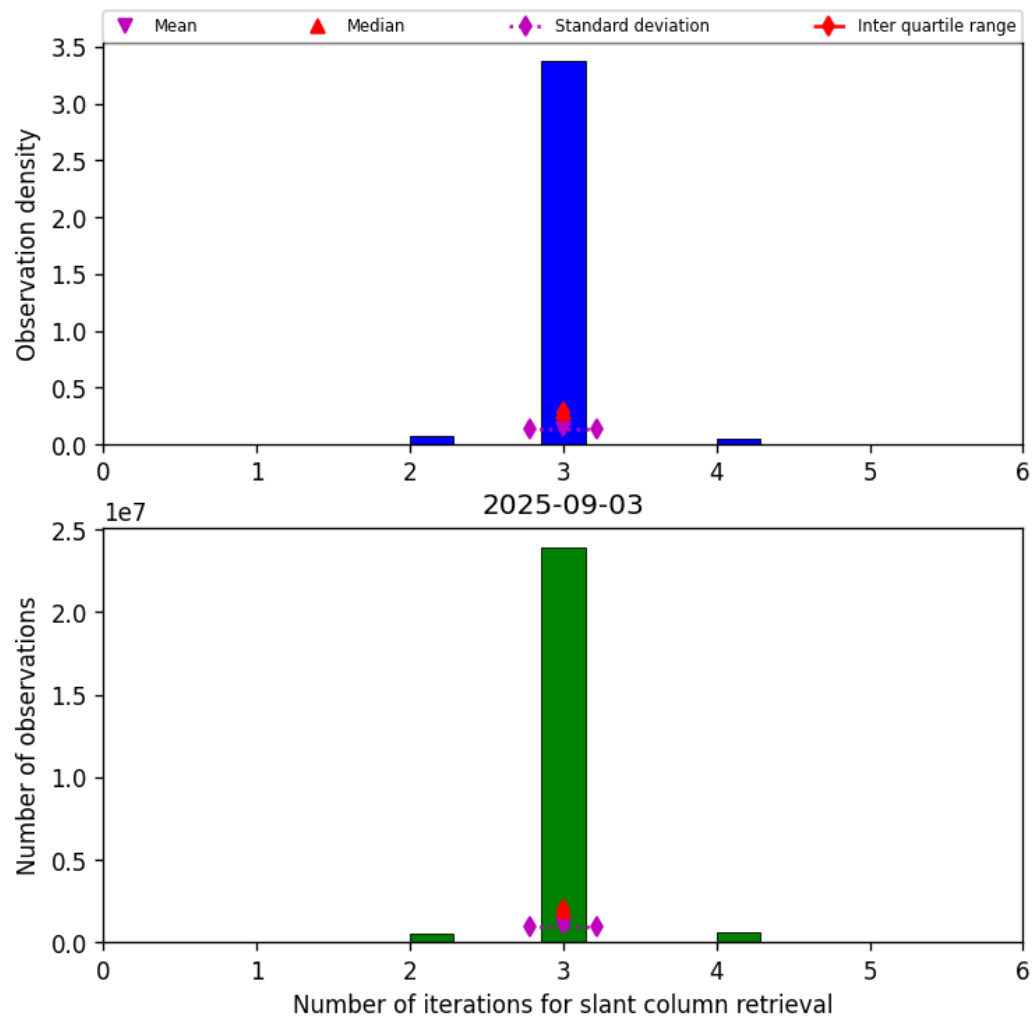
Figure 33: Histogram of “Number of iterations for slant column retrieval” for 2025-09-03 to 2025-09-04
