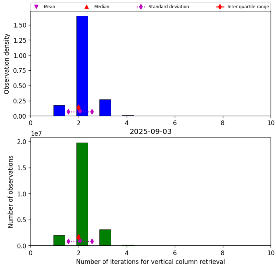
Figure 39: Histogram of “Number of iterations for vertical column retrieval” for 2025-09-03 to 2025-09-04
