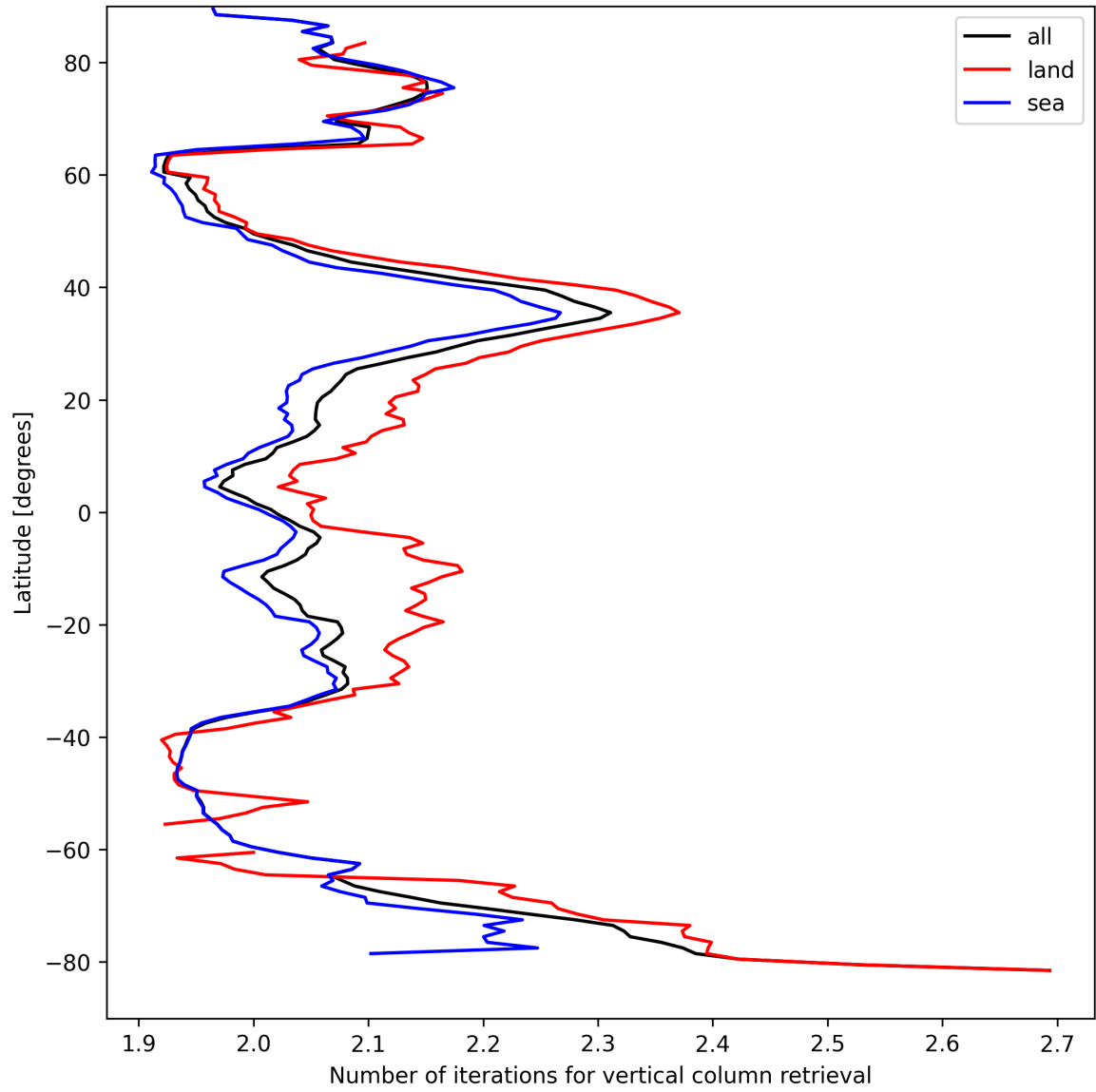
Figure 27: Zonal average of “Number of iterations for vertical column retrieval” for 2025-09-03 to 2025-09-04.
