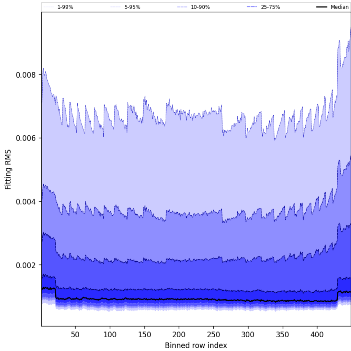
Figure 46: Along track statistics of “Fitting RMS” for 2025-09-03 to 2025-09-04
