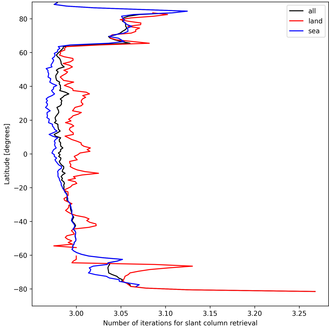
Figure 21: Zonal average of “Number of iterations for slant column retrieval” for 2025-09-03 to 2025-09-04.
