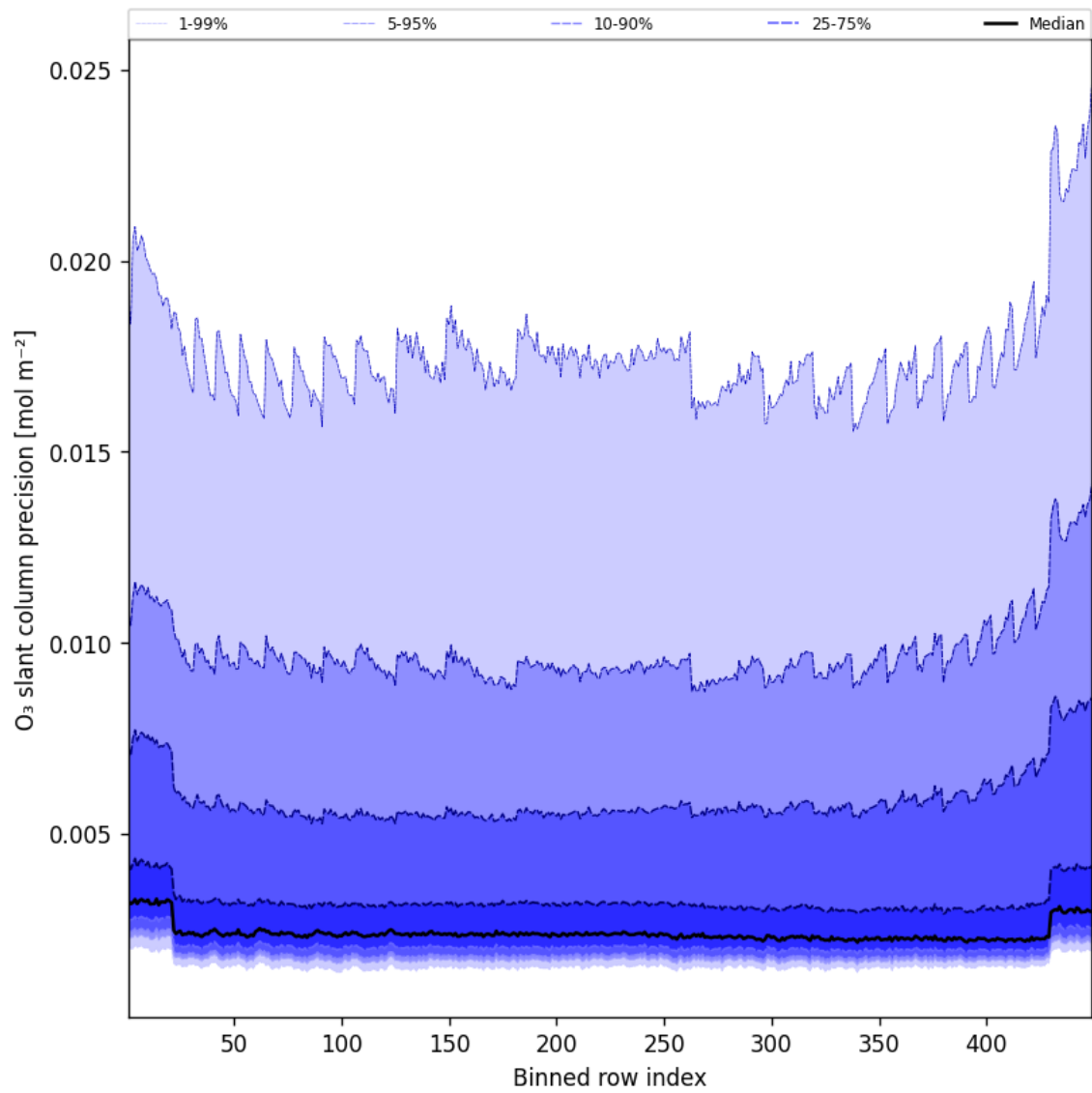
Figure 44: Along track statistics of “O 3 slant column precision” for 2025-09-03 to 2025-09-04
