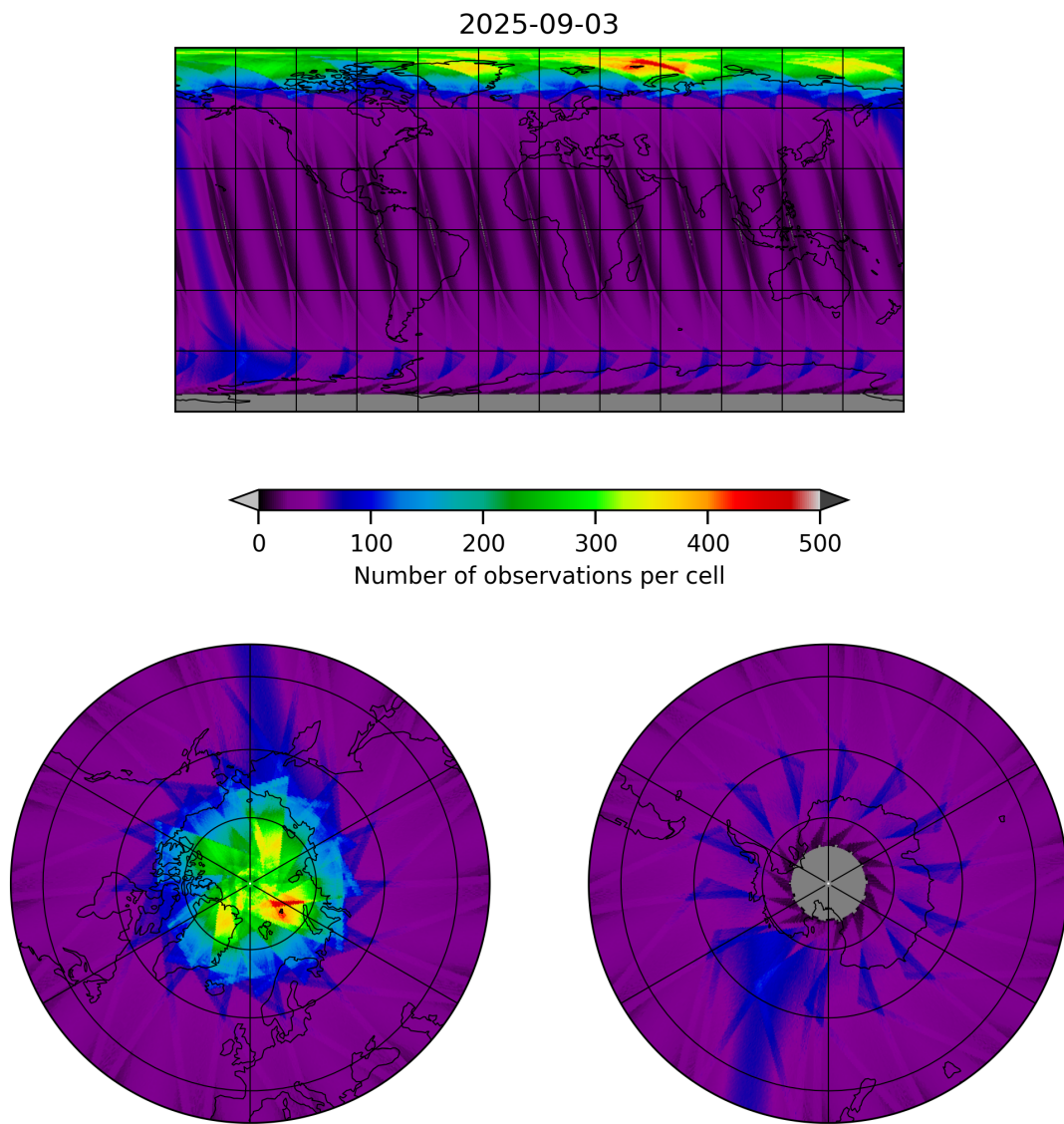
Figure 15: Map of the number of observations for 2025-09-03 to 2025-09-04
