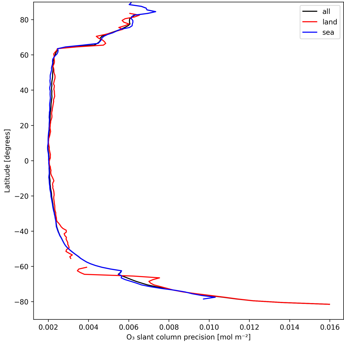
Figure 20: Zonal average of “O 3 slant column precision” for 2025-09-03 to 2025-09-04.
