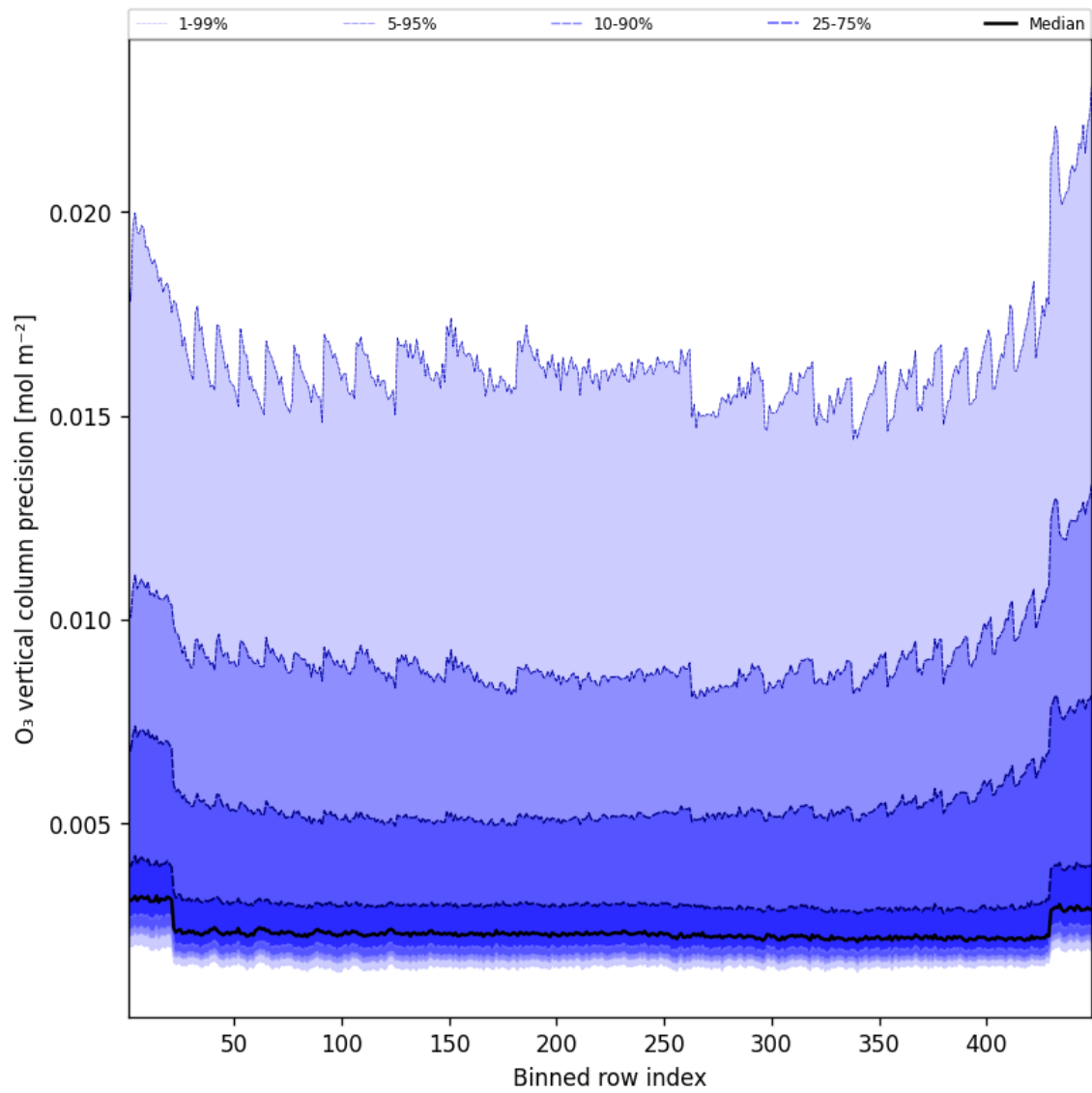
Figure 42: Along track statistics of “O 3 vertical column precision” for 2025-09-03 to 2025-09-04
