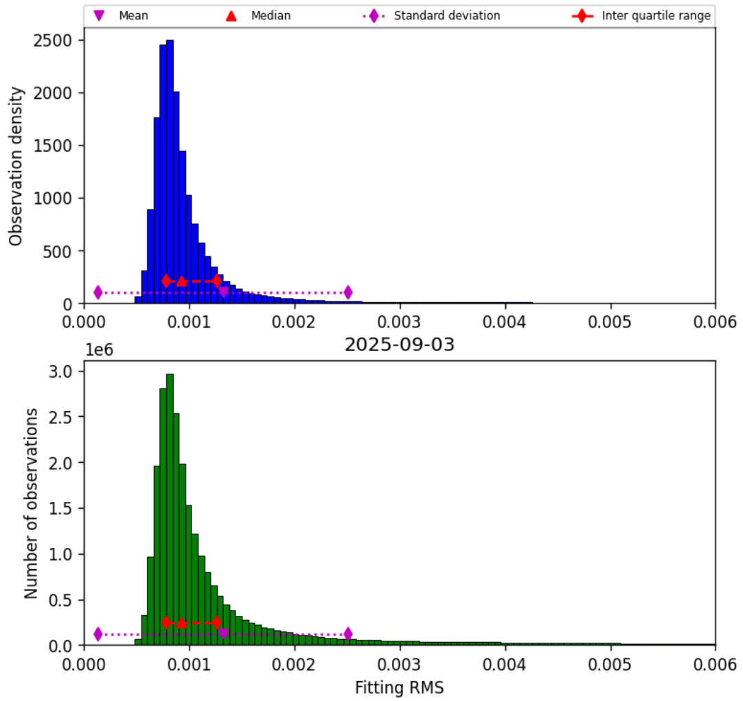
Figure 34: Histogram of “Fitting RMS” for 2025-09-03 to 2025-09-04
