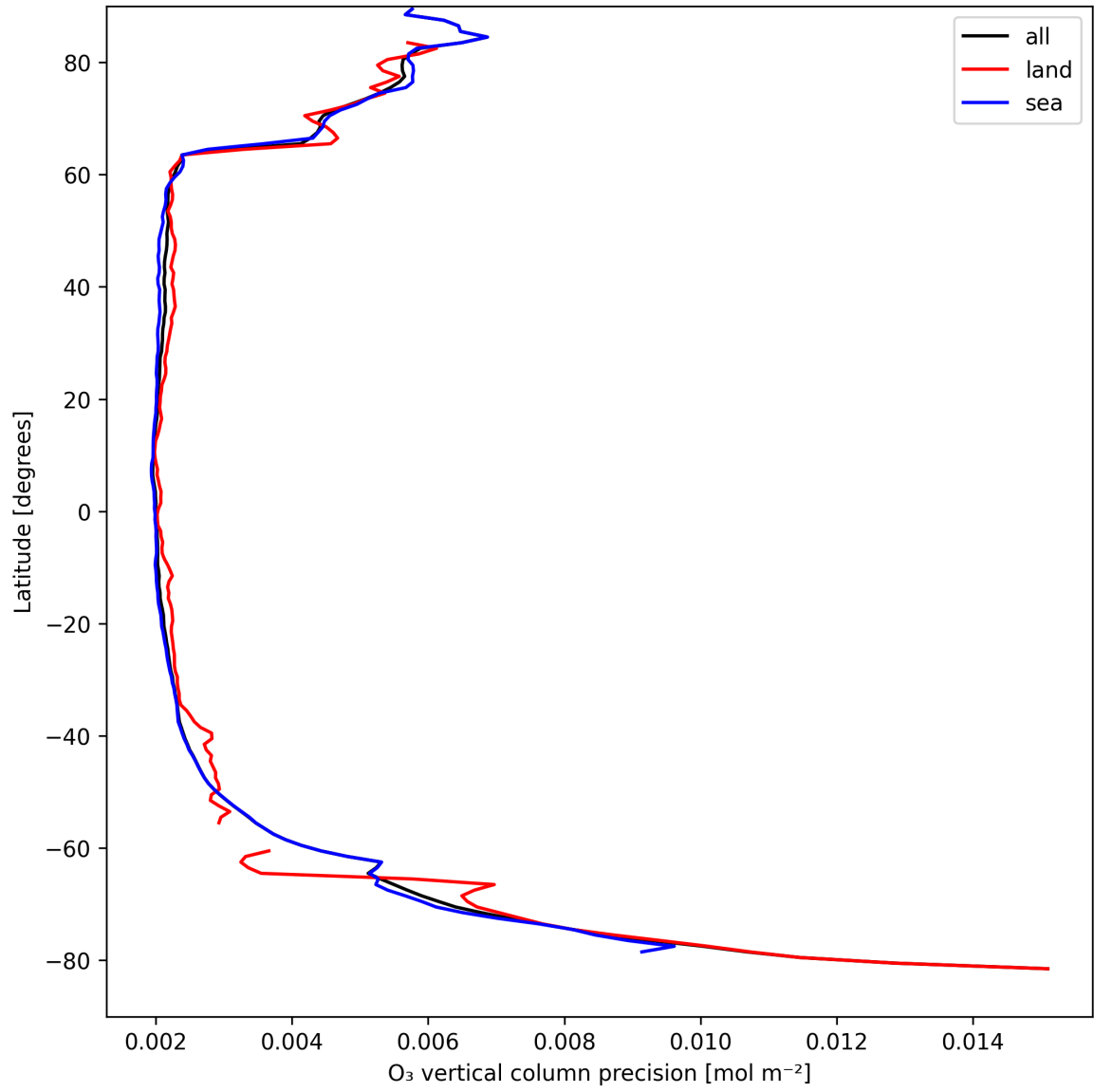
Figure 18: Zonal average of “O 3 vertical column precision” for 2025-09-03 to 2025-09-04.
