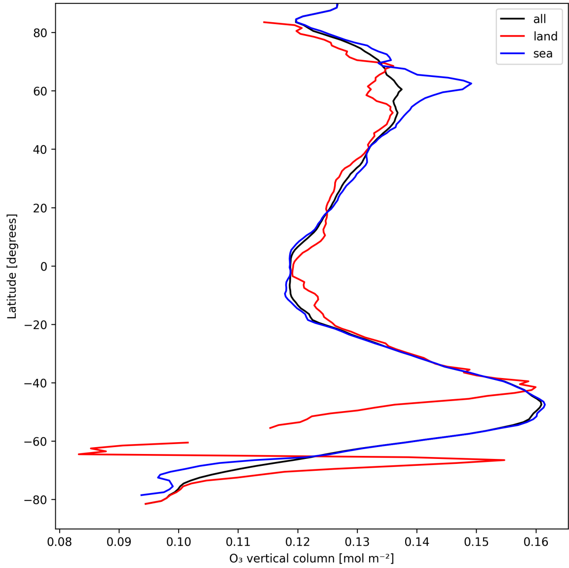
Figure 17: Zonal average of “O 3 vertical column” for 2025-09-03 to 2025-09-04.
