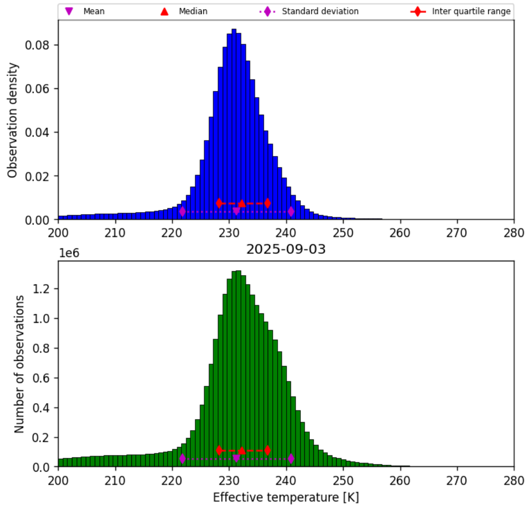
Figure 38: Histogram of “Effective temperature” for 2025-09-03 to 2025-09-04
