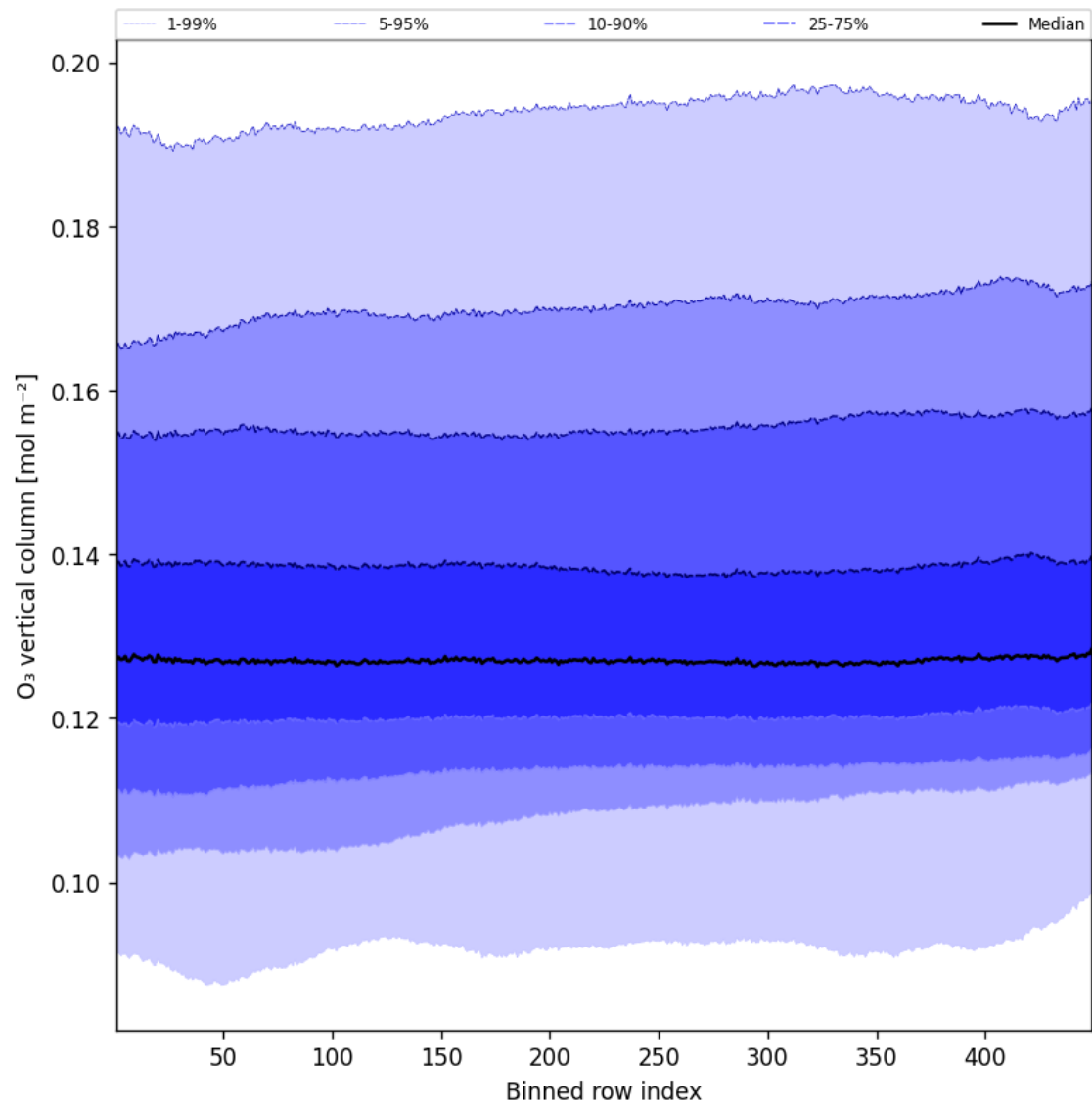
Figure 41: Along track statistics of “O 3 vertical column” for 2025-09-03 to 2025-09-04
