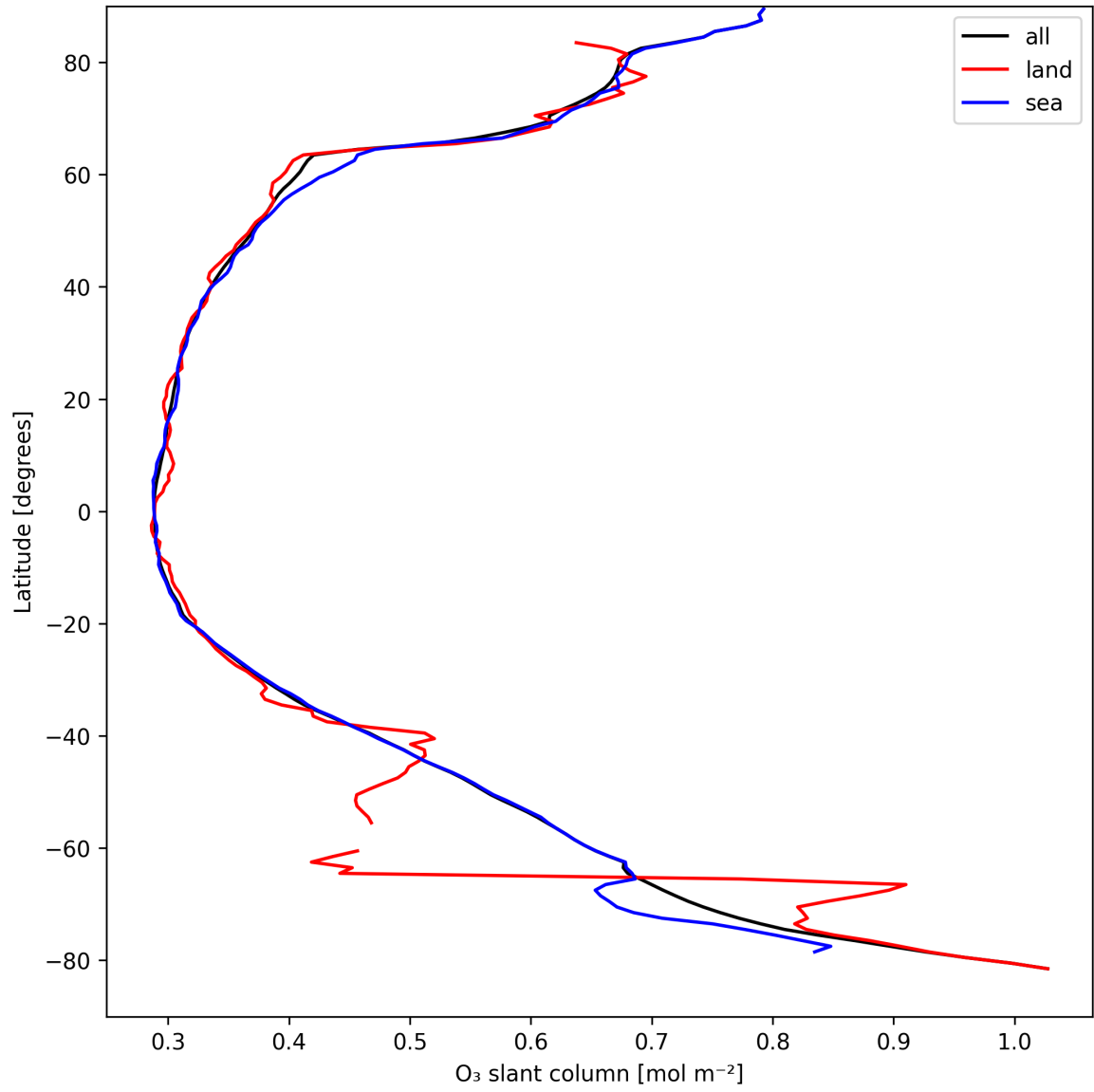
Figure 19: Zonal average of “O 3 slant column” for 2025-09-03 to 2025-09-04.
