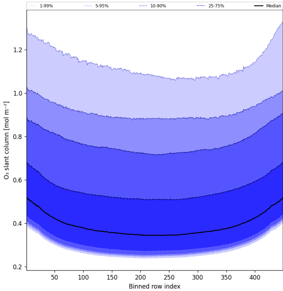
Figure 43: Along track statistics of “O 3 slant column” for 2025-09-03 to 2025-09-04
