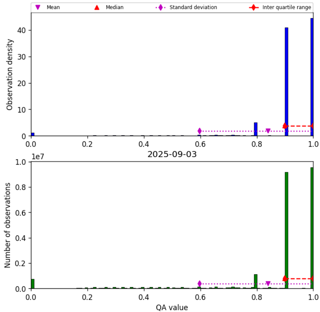
Figure 28: Histogram of “QA value” for 2025-09-03 to 2025-09-04
