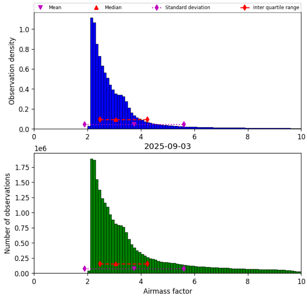
Figure 37: Histogram of “Airmass factor” for 2025-09-03 to 2025-09-04
