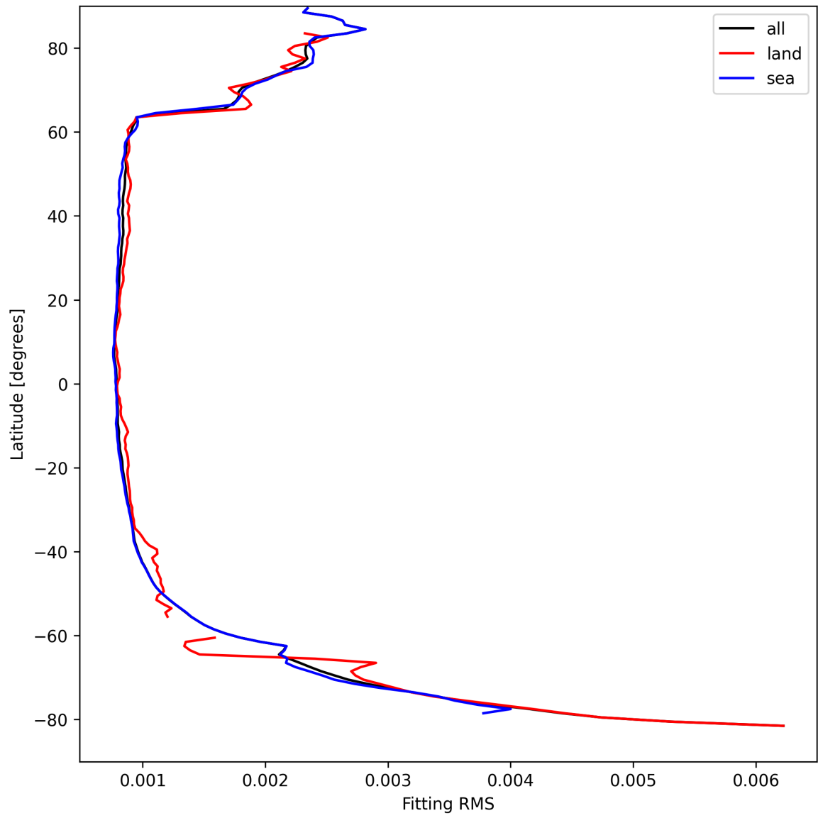
Figure 22: Zonal average of “Fitting RMS” for 2025-09-03 to 2025-09-04.
