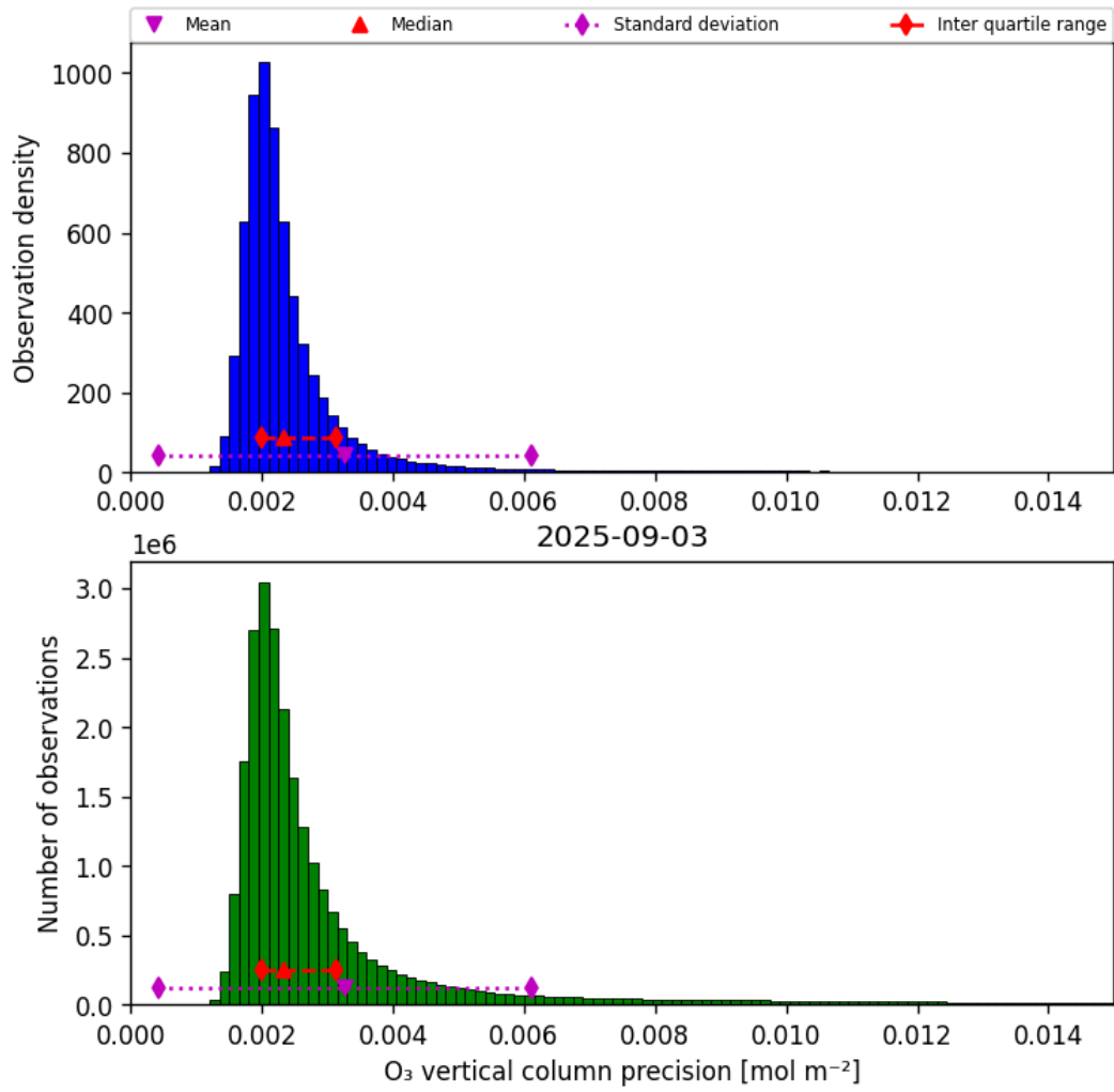
Figure 30: Histogram of “O 3 vertical column precision” for 2025-09-03 to 2025-09-04
