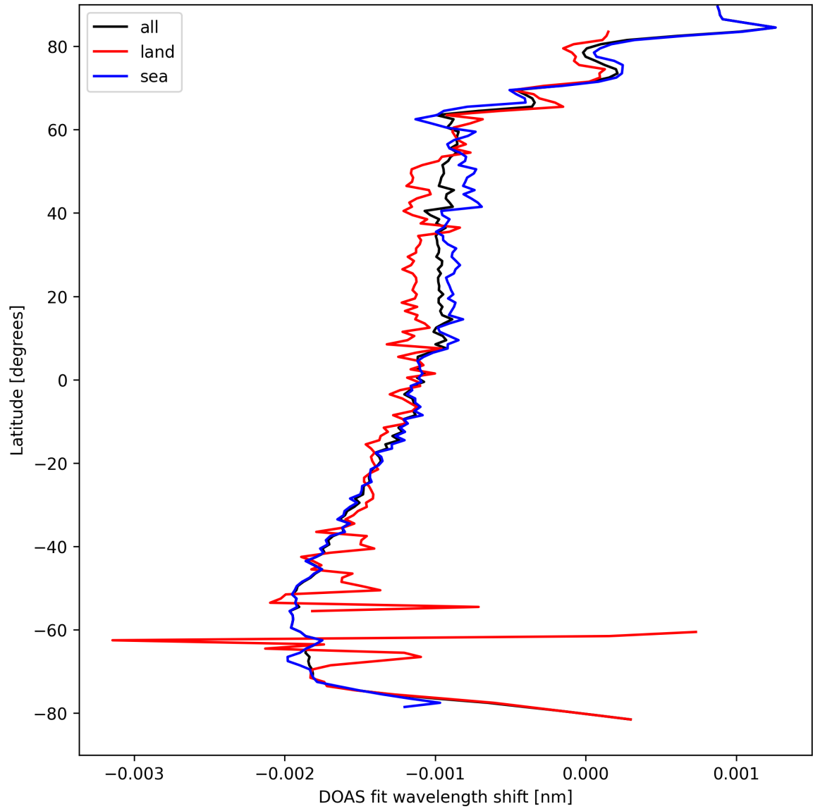
Figure 23: Zonal average of "DOAS fit wavelength shift" for 2025-09-03 to 2025-09-04.
