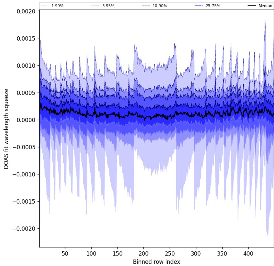
Figure 48: Along track statistics of “DOAS fit wavelength squeeze” for 2025-09-03 to 2025-09-04
