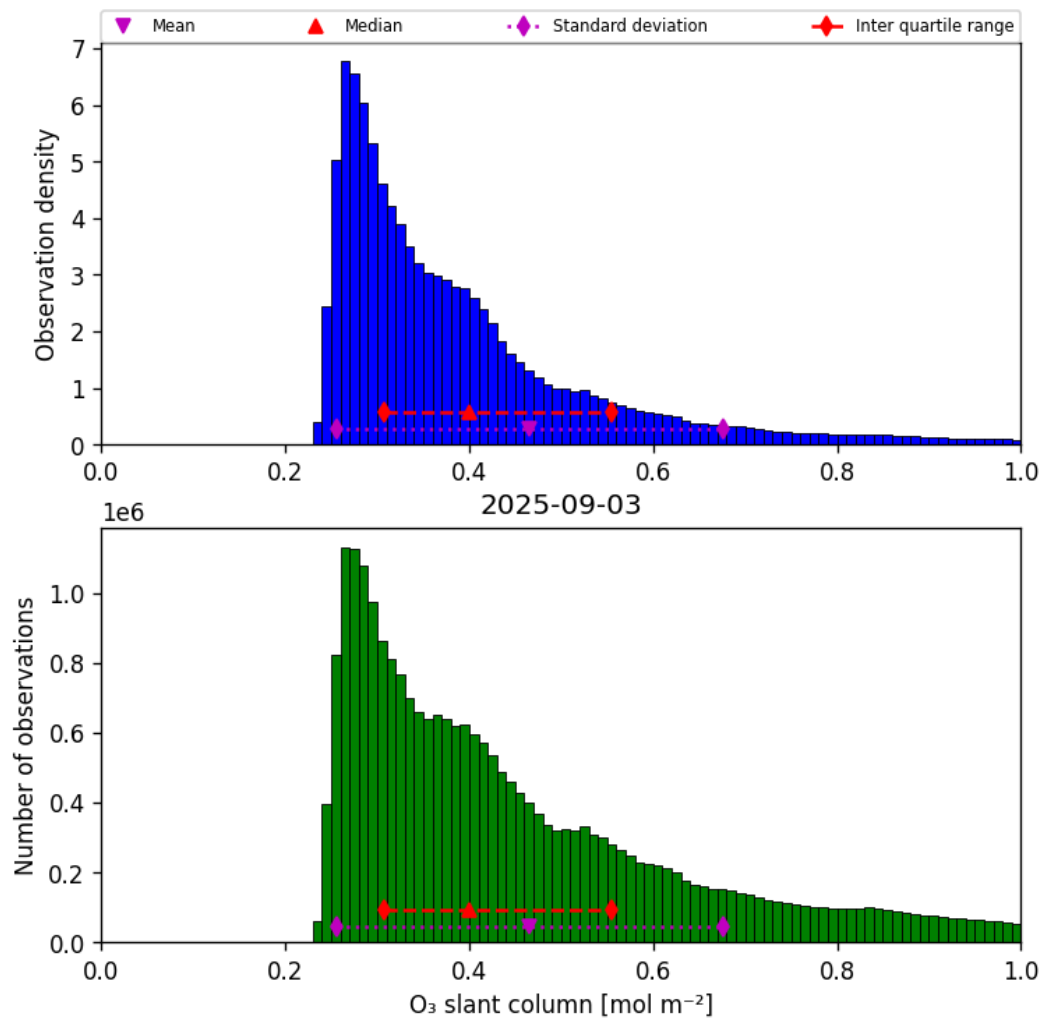
Figure 31: Histogram of “O 3 slant column” for 2025-09-03 to 2025-09-04
