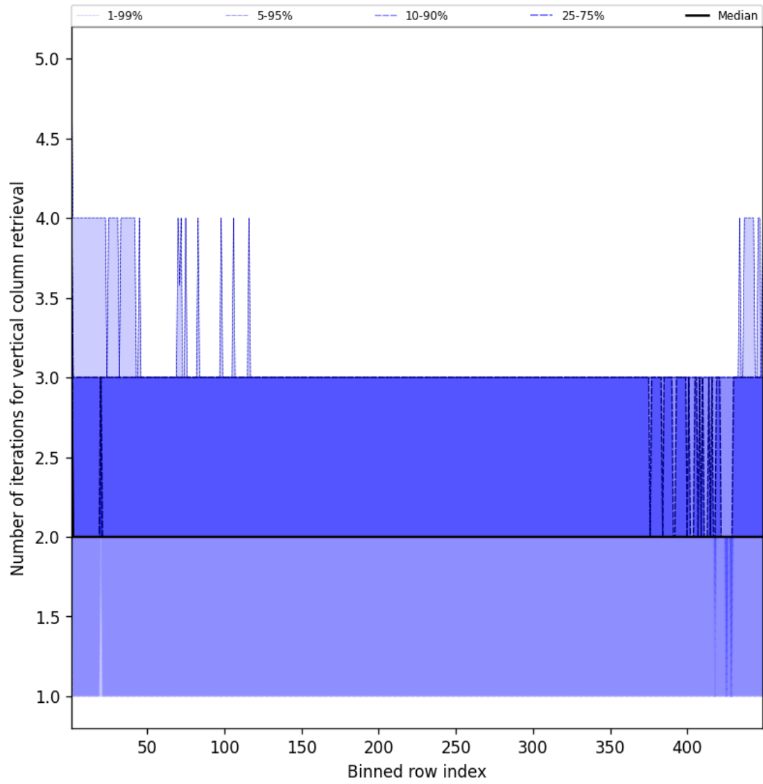
Figure 51: Along track statistics of “Number of iterations for vertical column retrieval” for 2025-09-03 to 2025-09-04
