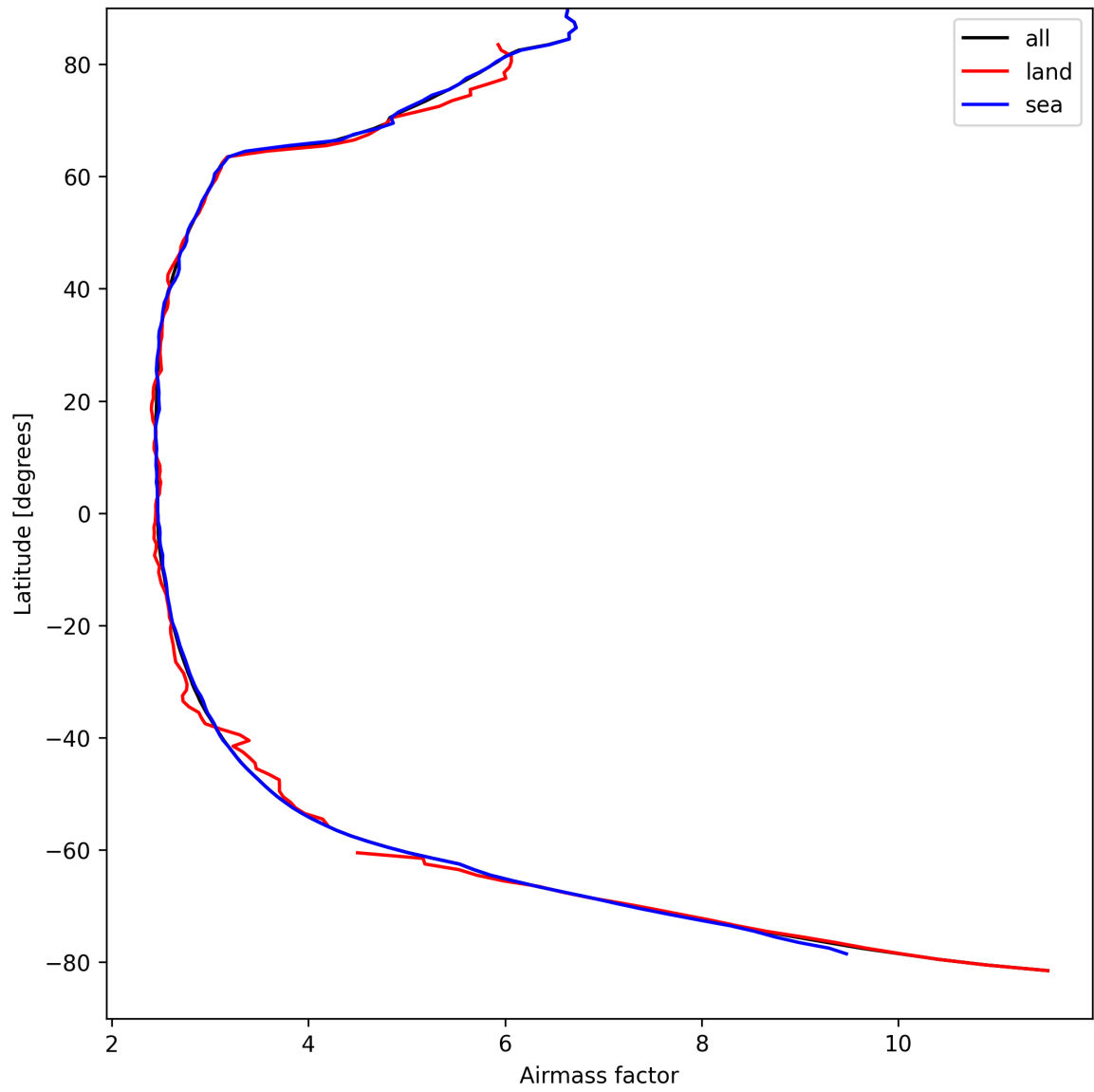
Figure 25: Zonal average of “Airmass factor” for 2025-09-03 to 2025-09-04.
