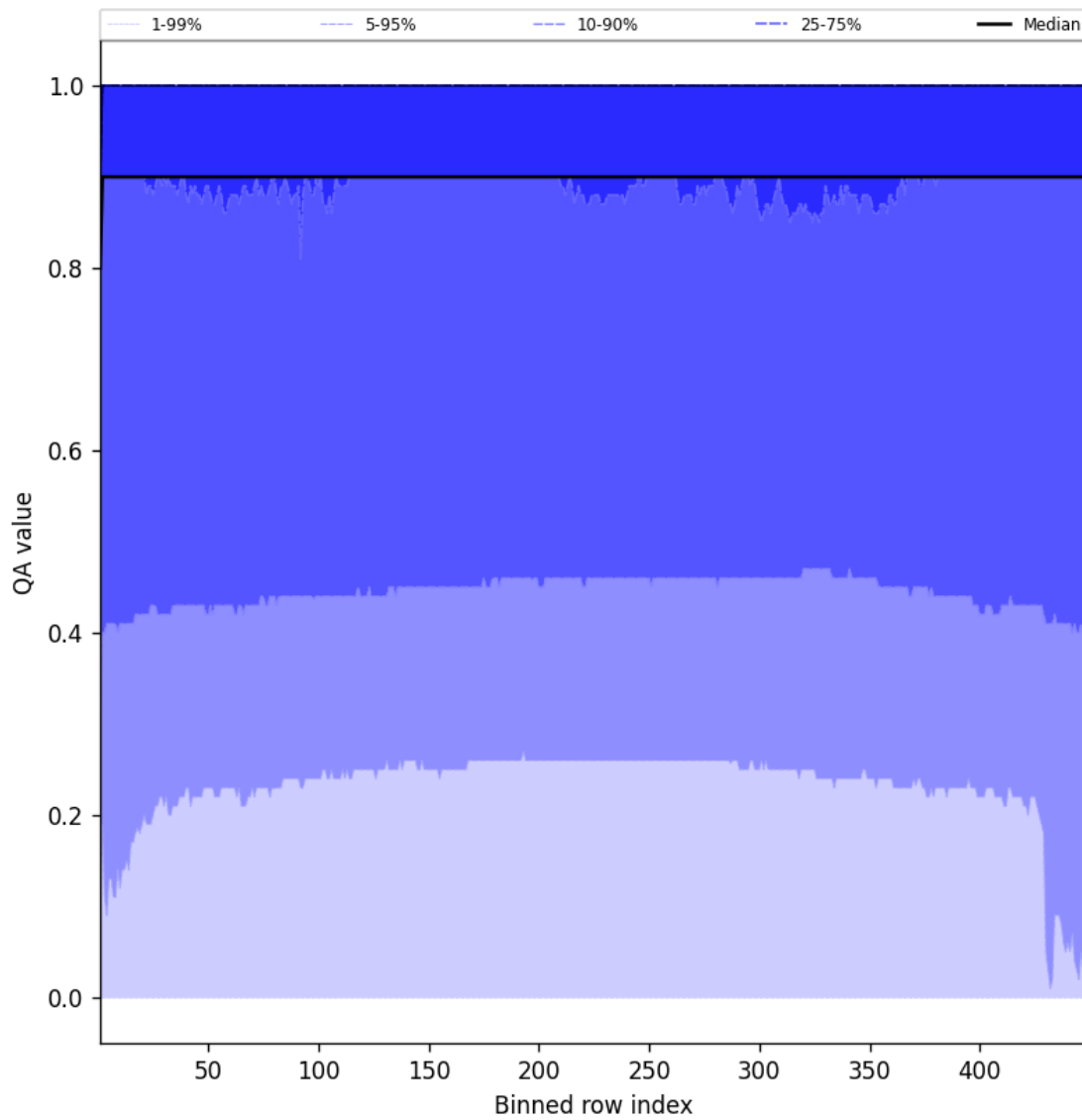
Figure 40: Along track statistics of “QA value” for 2025-09-03 to 2025-09-04
