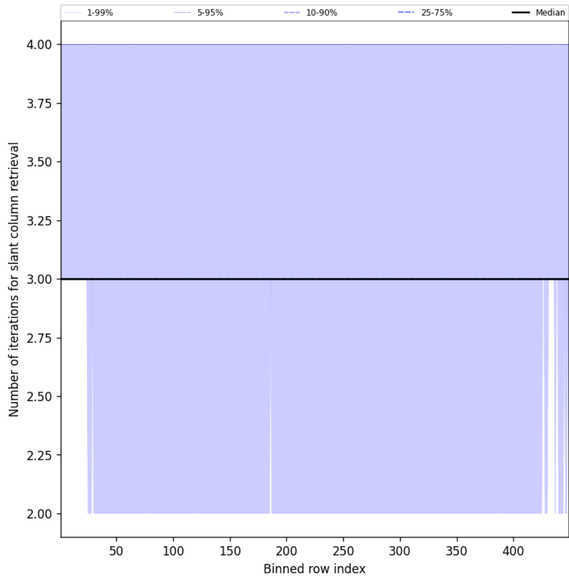
Figure 45: Along track statistics of “Number of iterations for slant column retrieval” for 2025-09-03 to 2025-09-04
