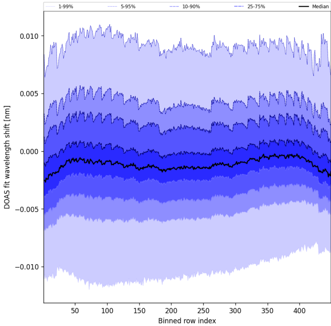
Figure 47: Along track statistics of “DOAS fit wavelength shift” for 2025-09-03 to 2025-09-04
