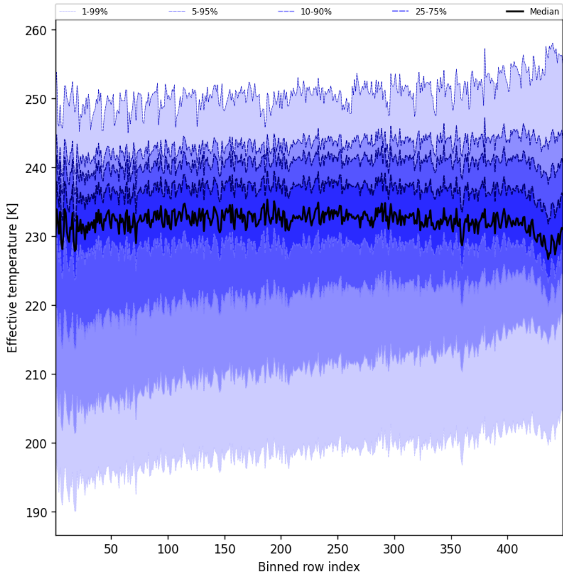
Figure 50: Along track statistics of “Effective temperature” for 2025-09-03 to 2025-09-04
