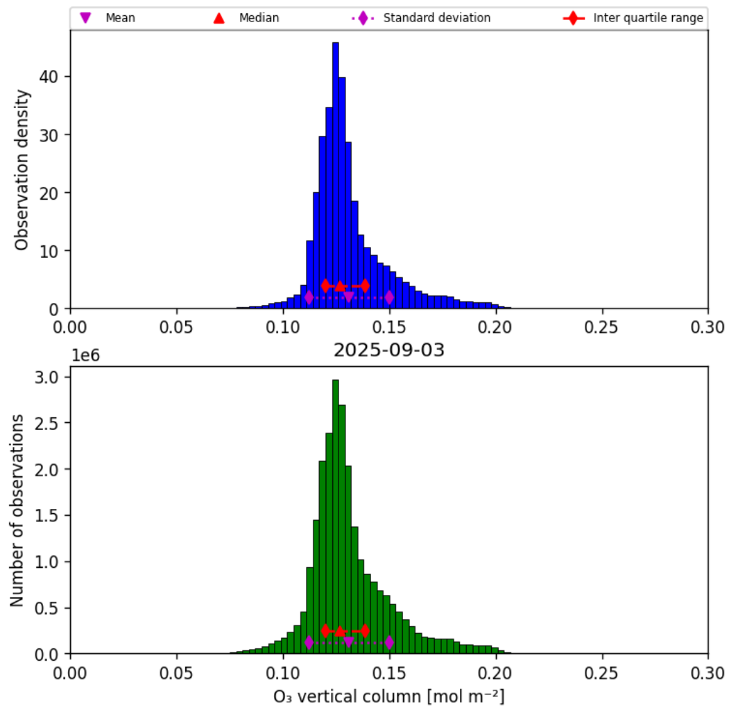
Figure 29: Histogram of “O 3 vertical column” for 2025-09-03 to 2025-09-04
