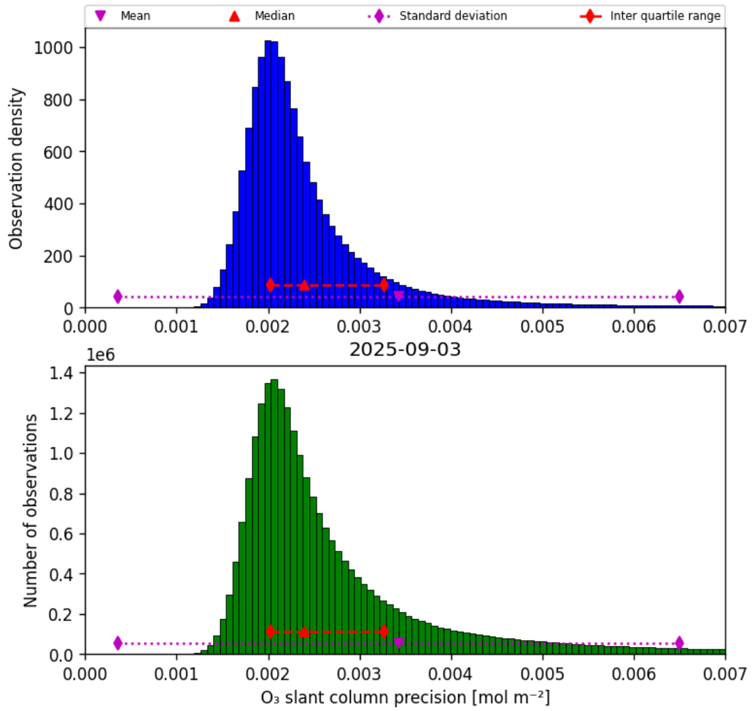
Figure 32: Histogram of “O 3 slant column precision” for 2025-09-03 to 2025-09-04
