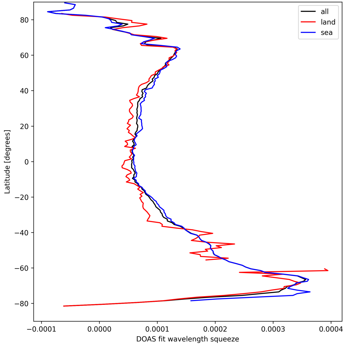
Figure 24: Zonal average of “DOAS fit wavelength squeeze” for 2025-09-03 to 2025-09-04.
