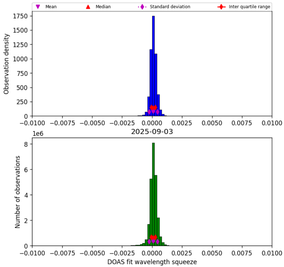
Figure 36: Histogram of “DOAS fit wavelength squeeze” for 2025-09-03 to 2025-09-04
