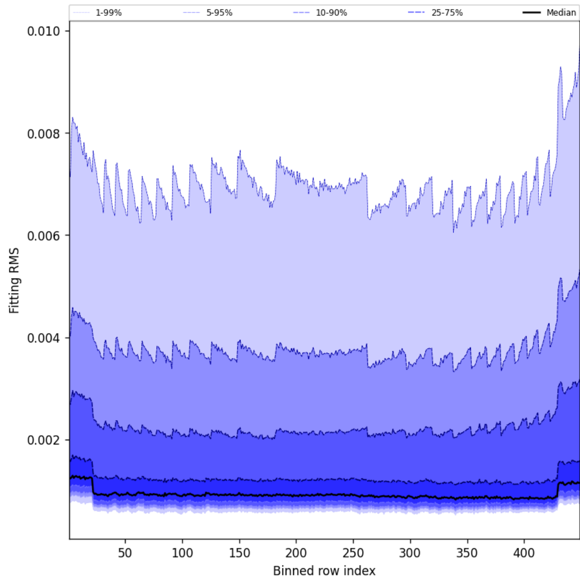
Figure 46: Along track statistics of “Fitting RMS” for 2025-09-04 to 2025-09-05
