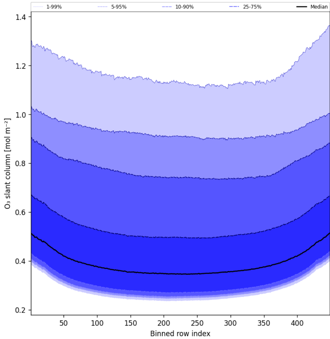
Figure 43: Along track statistics of “O 3 slant column” for 2025-09-04 to 2025-09-05
