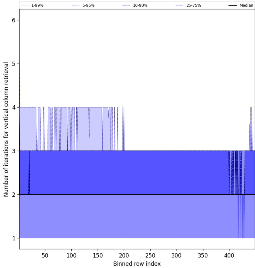
Figure 51: Along track statistics of “Number of iterations for vertical column retrieval” for 2025-09-04 to 2025-09-05
