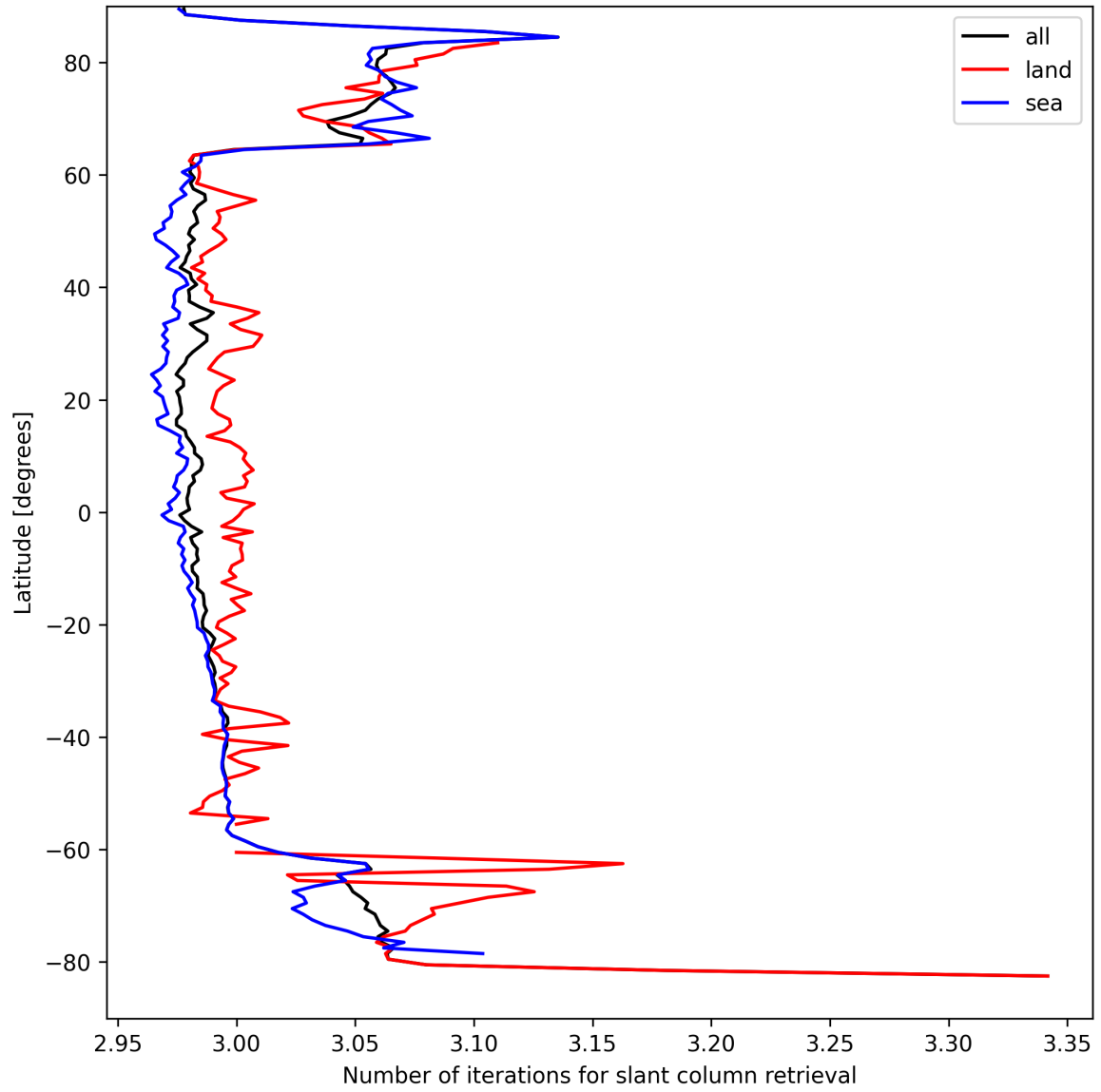
Figure 21: Zonal average of “Number of iterations for slant column retrieval” for 2025-09-04 to 2025-09-05.
