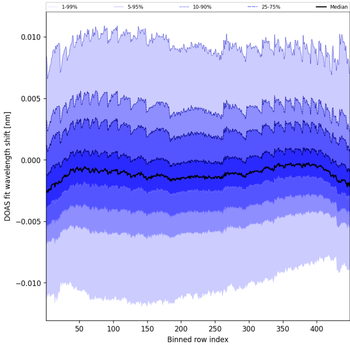
Figure 47: Along track statistics of “DOAS fit wavelength shift” for 2025-09-04 to 2025-09-05
