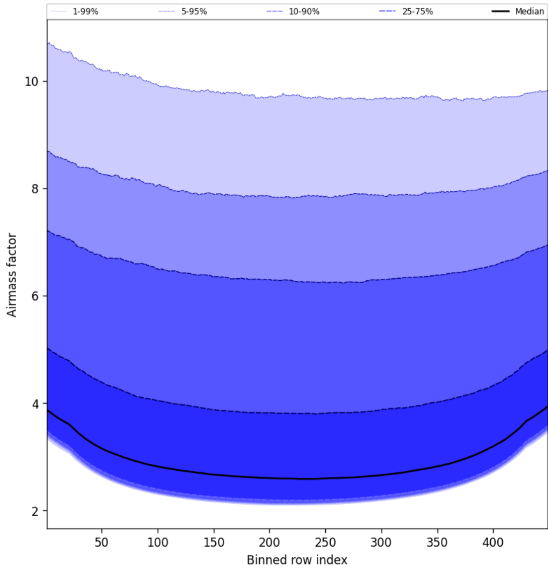
Figure 49: Along track statistics of “Airmass factor” for 2025-09-04 to 2025-09-05
