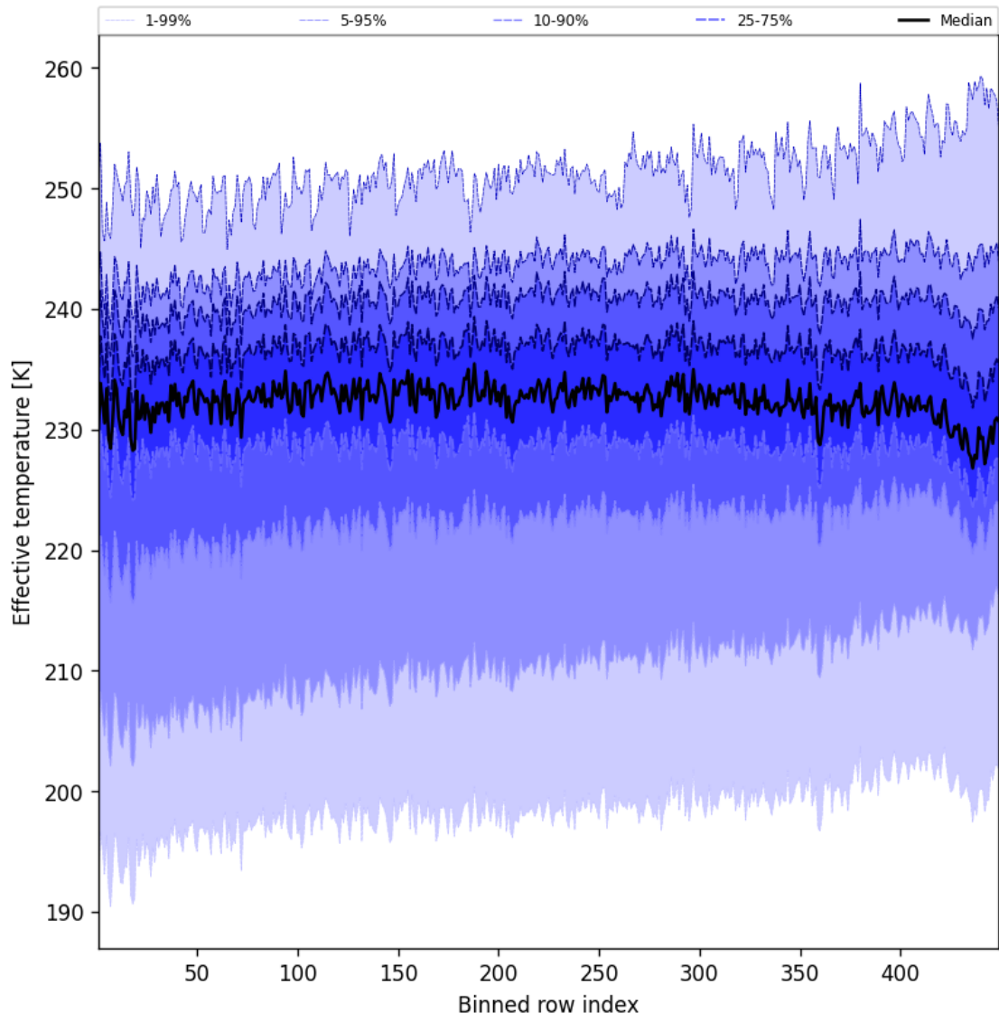
Figure 50: Along track statistics of “Effective temperature” for 2025-09-04 to 2025-09-05
