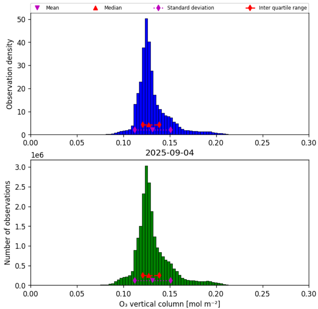
Figure 29: Histogram of “O 3 vertical column” for 2025-09-04 to 2025-09-05
