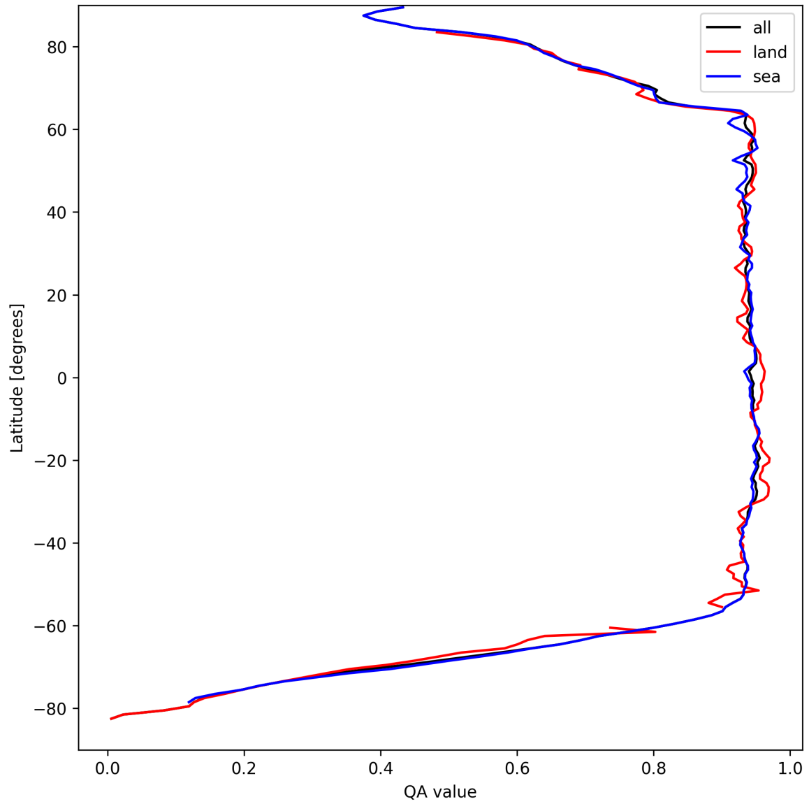
Figure 16: Zonal average of “QA value” for 2025-09-04 to 2025-09-05.
