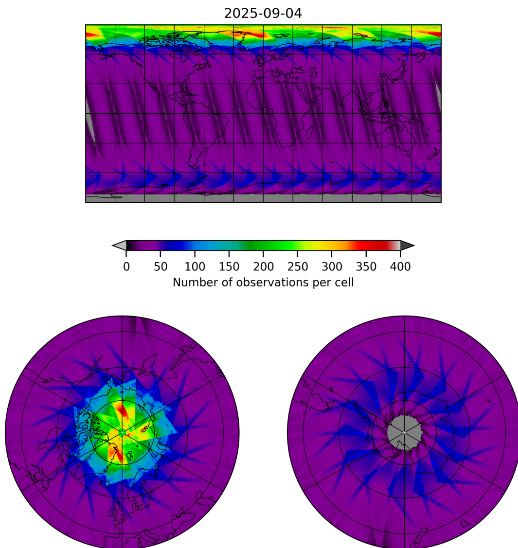
Figure 15: Map of the number of observations for 2025-09-04 to 2025-09-05
