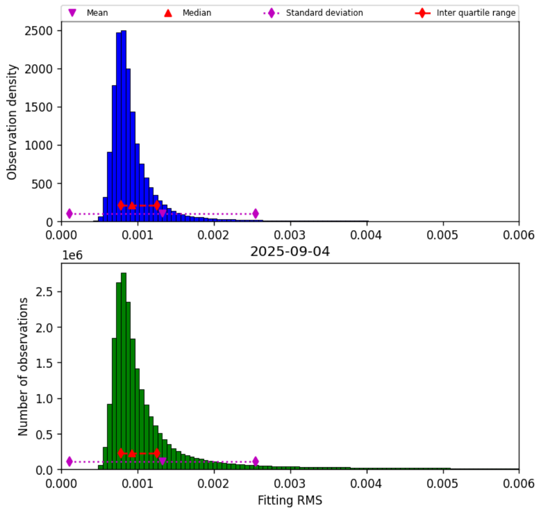
Figure 34: Histogram of “Fitting RMS” for 2025-09-04 to 2025-09-05
