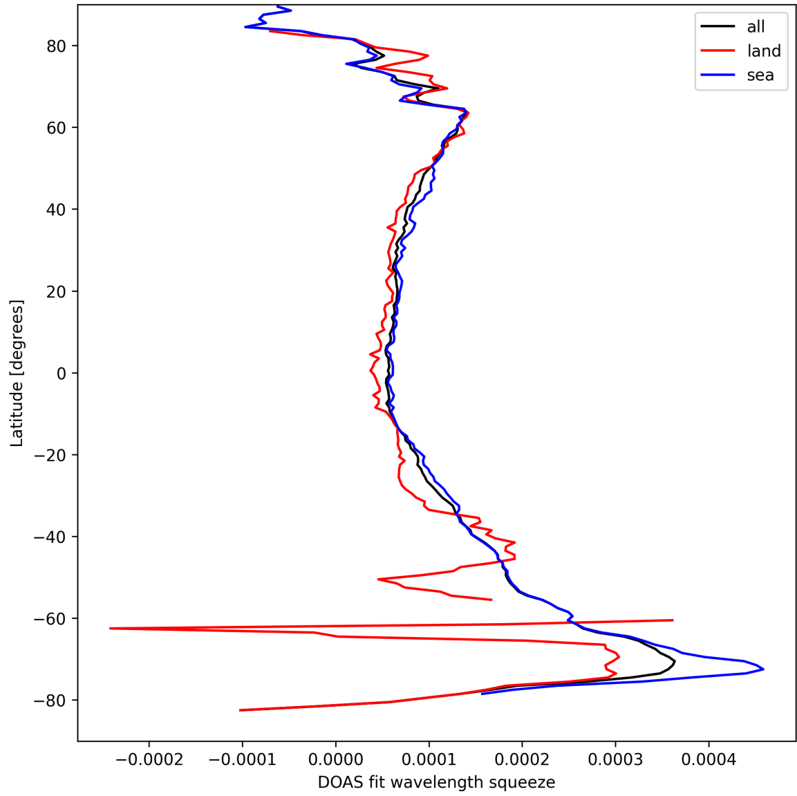
Figure 24: Zonal average of "DOAS fit wavelength squeeze" for 2025-09-04 to 2025-09-05.
