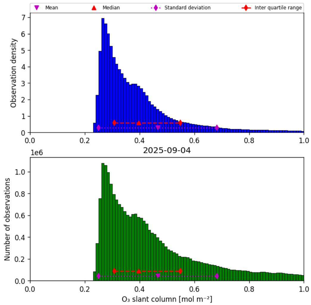
Figure 31: Histogram of “O 3 slant column” for 2025-09-04 to 2025-09-05
