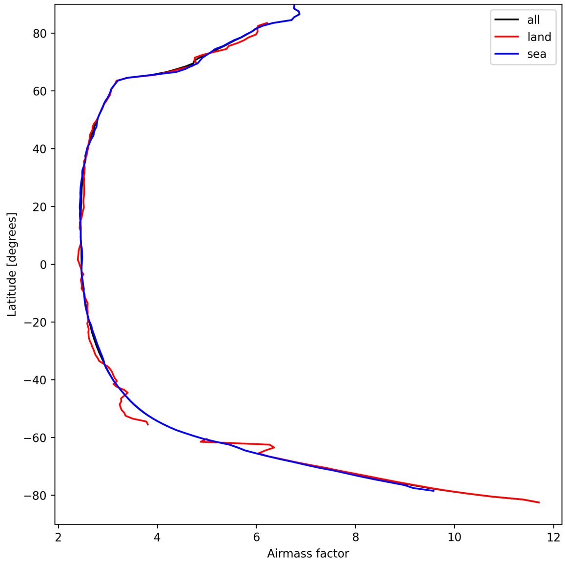
Figure 25: Zonal average of “Airmass factor” for 2025-09-04 to 2025-09-05.
