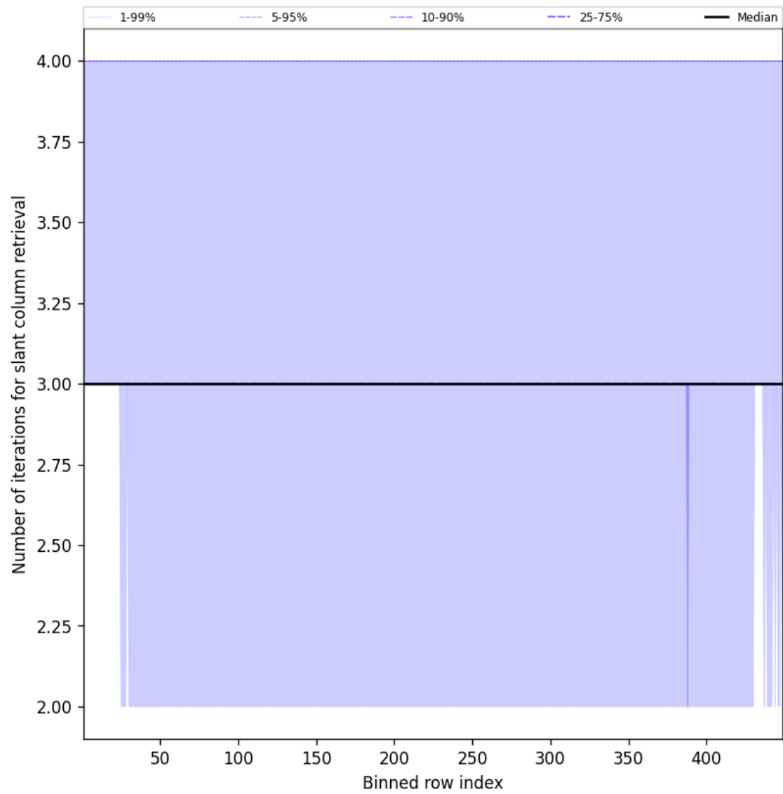
Figure 45: Along track statistics of “Number of iterations for slant column retrieval” for 2025-09-04 to 2025-09-05
