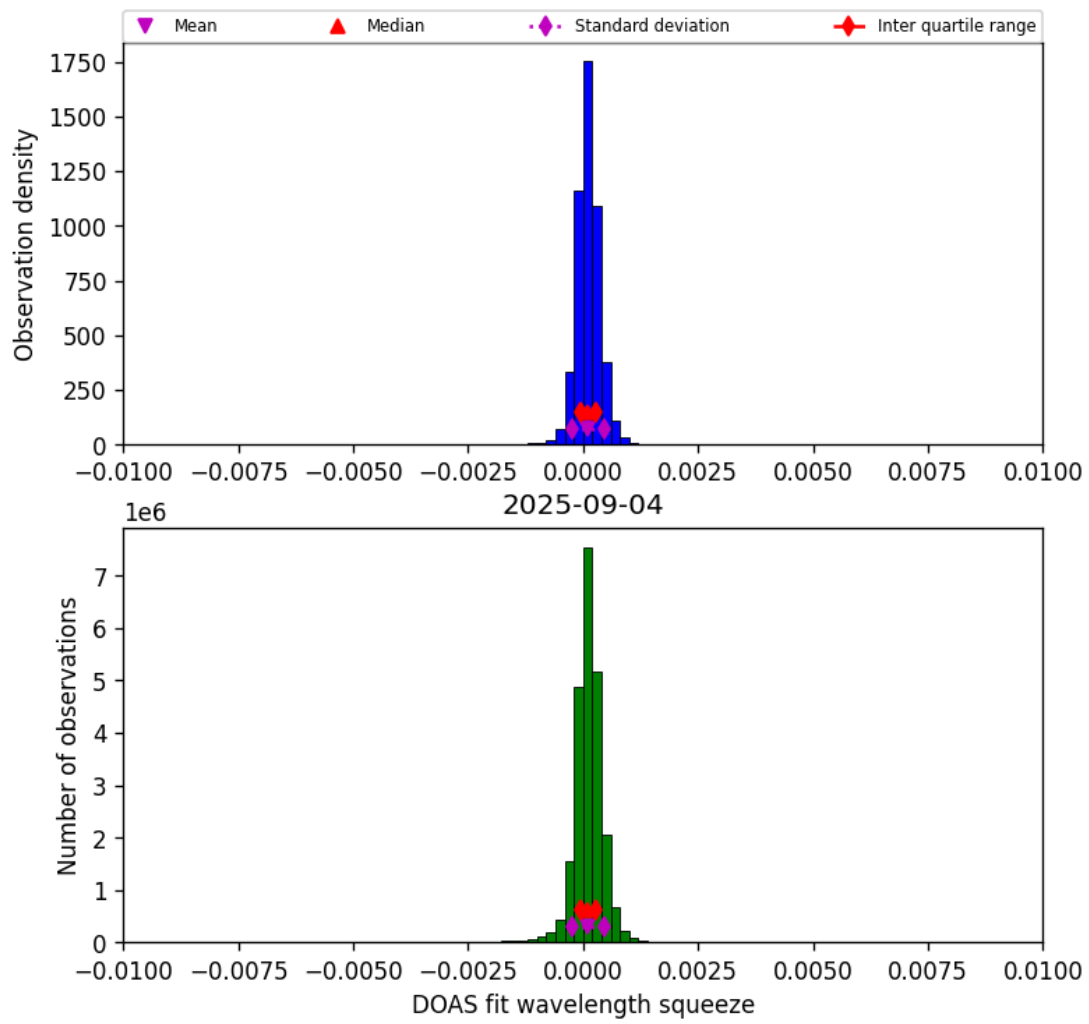
Figure 36: Histogram of “DOAS fit wavelength squeeze” for 2025-09-04 to 2025-09-05
