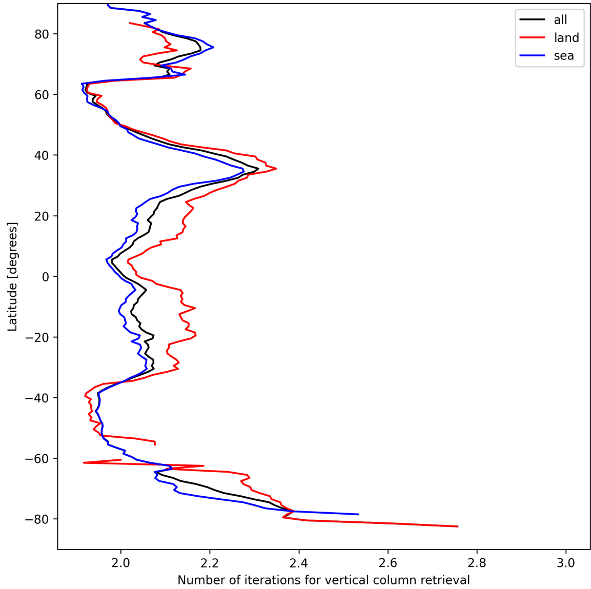
Figure 27: Zonal average of “Number of iterations for vertical column retrieval” for 2025-09-04 to 2025-09-05.
