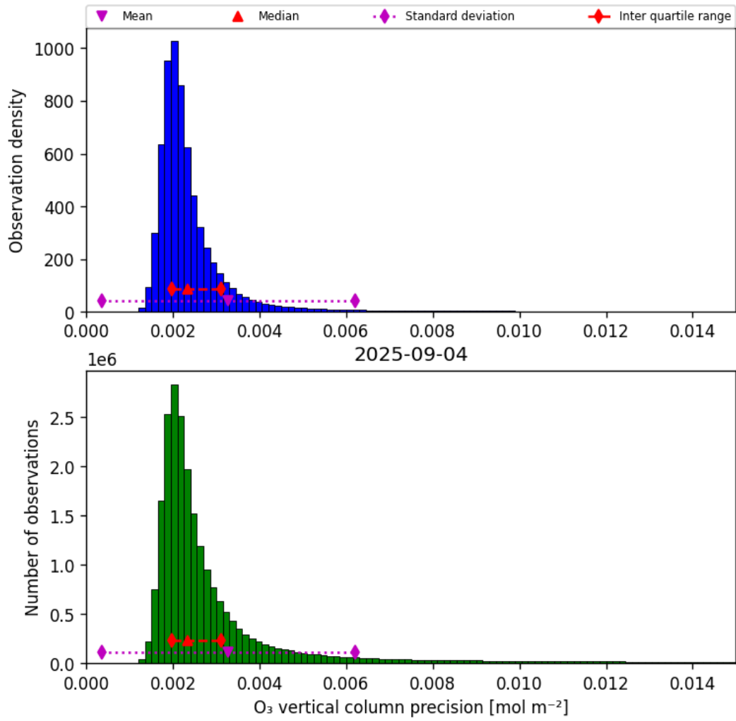
Figure 30: Histogram of “O 3 vertical column precision” for 2025-09-04 to 2025-09-05
