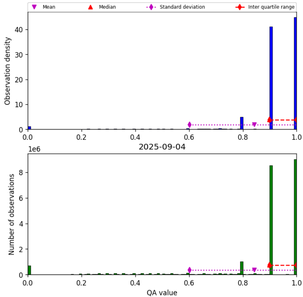
Figure 28: Histogram of “QA value” for 2025-09-04 to 2025-09-05
