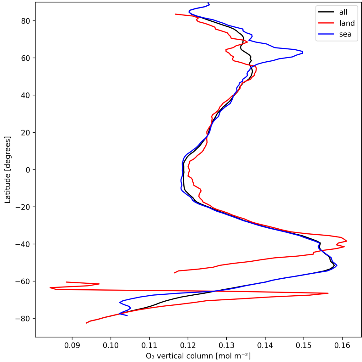
Figure 17: Zonal average of “O 3 vertical column” for 2025-09-04 to 2025-09-05.
