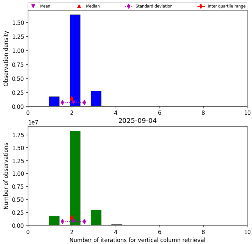
Figure 39: Histogram of “Number of iterations for vertical column retrieval” for 2025-09-04 to 2025-09-05
