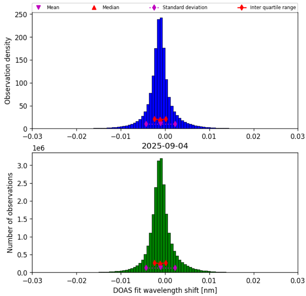
Figure 35: Histogram of “DOAS fit wavelength shift” for 2025-09-04 to 2025-09-05
