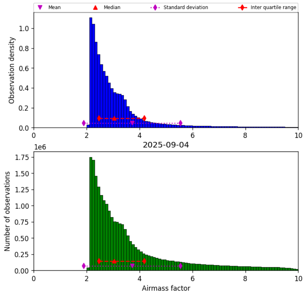
Figure 37: Histogram of “Airmass factor” for 2025-09-04 to 2025-09-05
