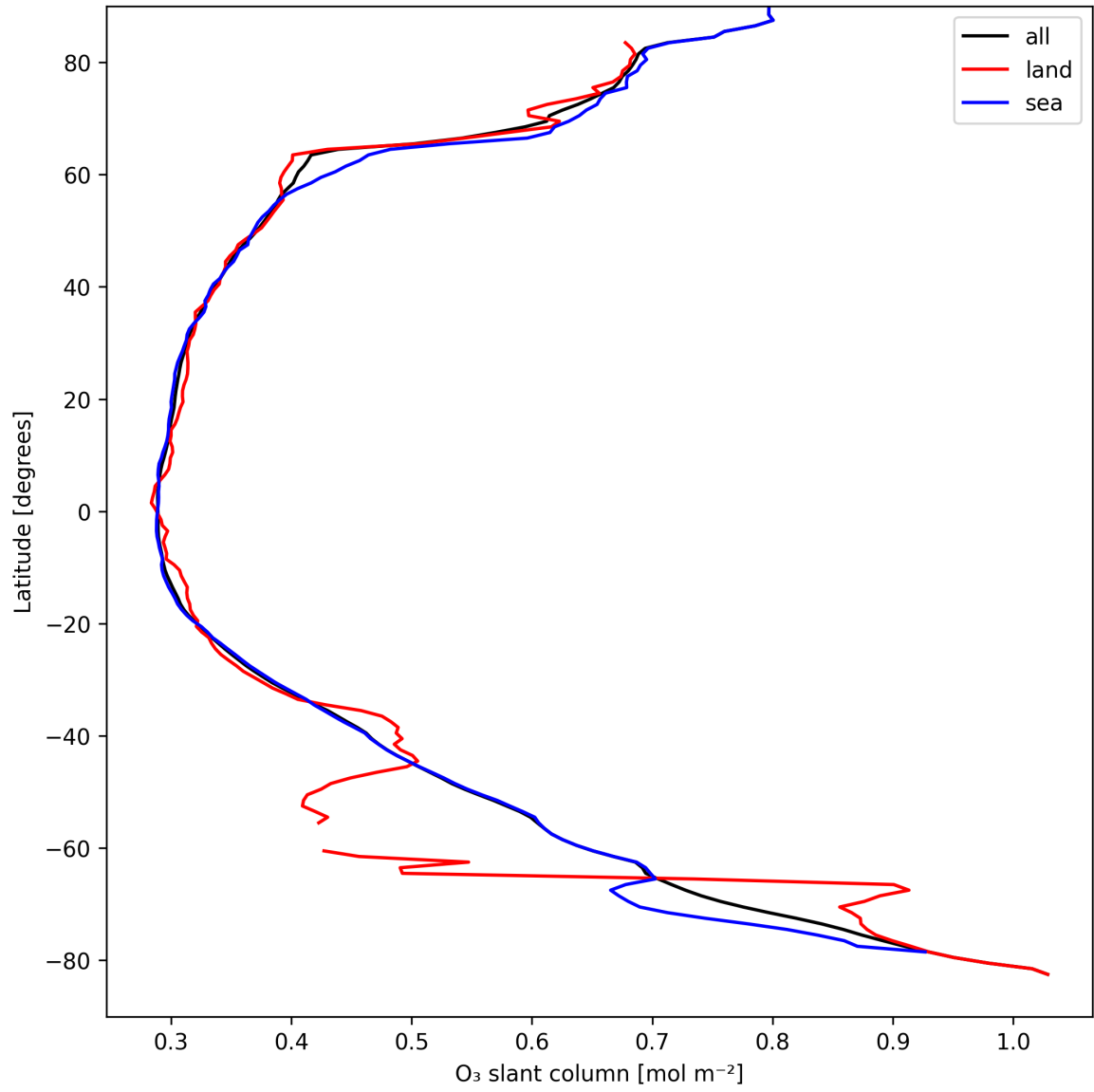
Figure 19: Zonal average of “O 3 slant column” for 2025-09-04 to 2025-09-05.
