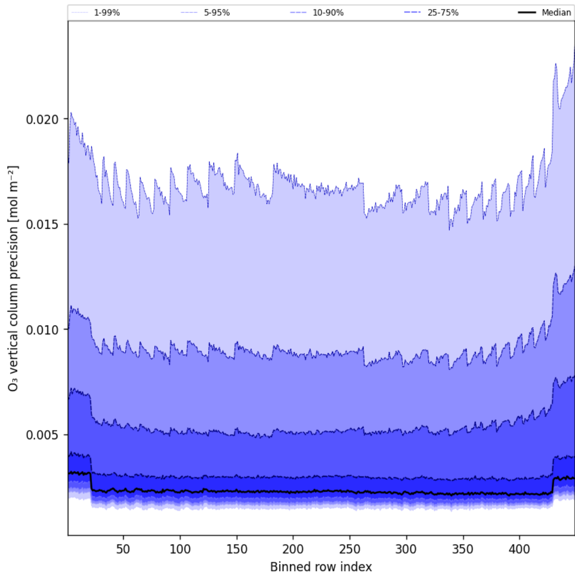
Figure 42: Along track statistics of “O 3 vertical column precision” for 2025-09-04 to 2025-09-05
