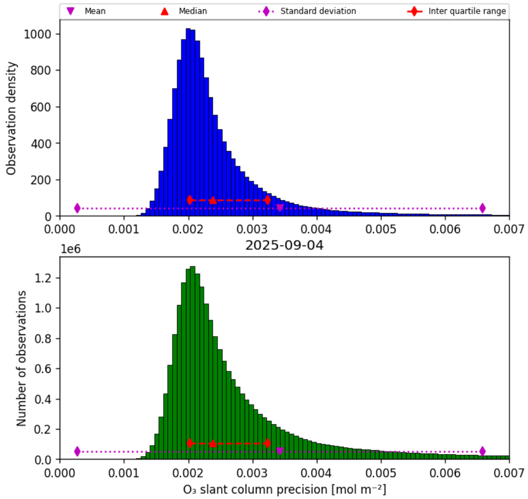
Figure 32: Histogram of “O 3 slant column precision” for 2025-09-04 to 2025-09-05
