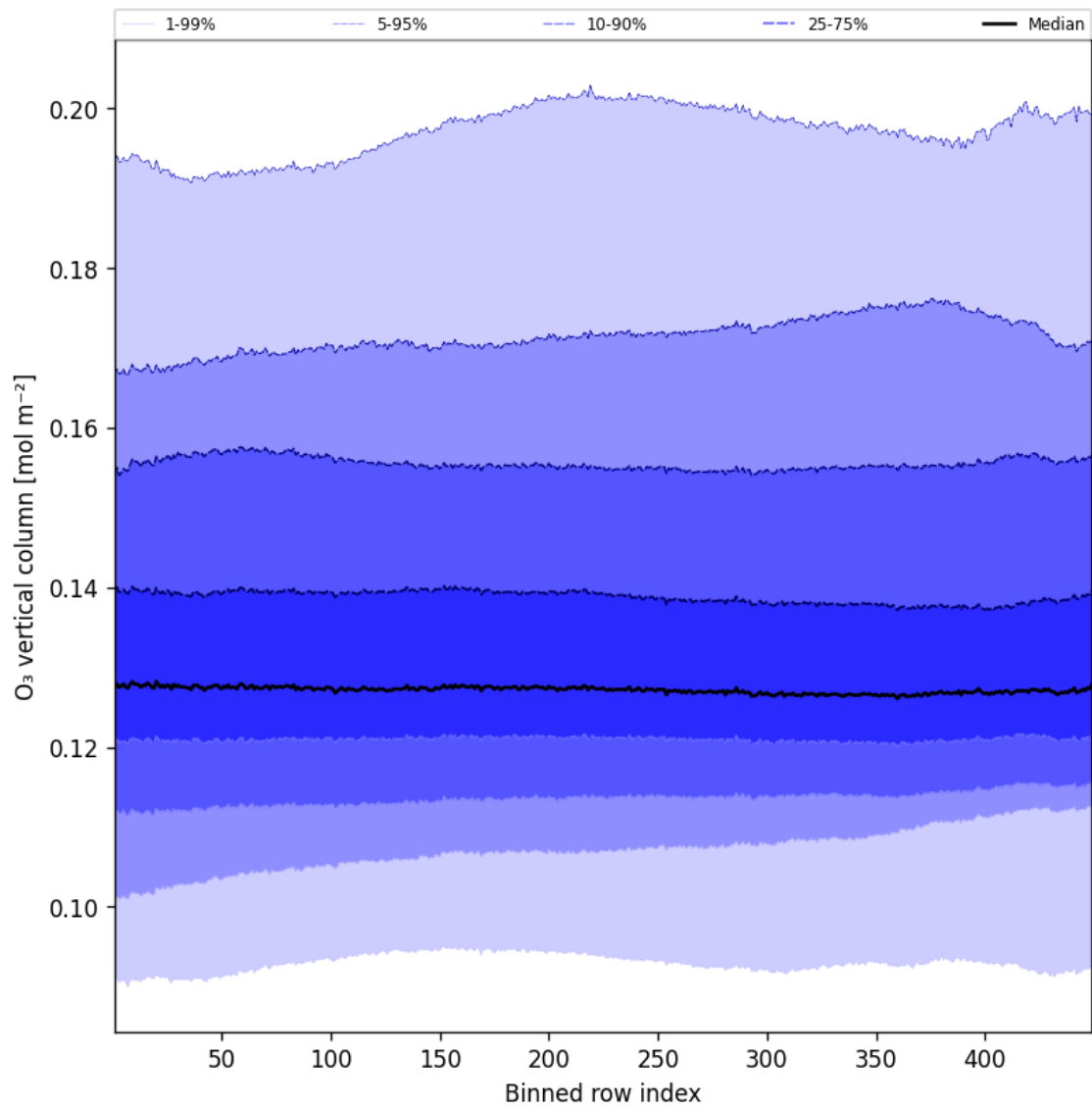
Figure 41: Along track statistics of “O 3 vertical column” for 2025-09-04 to 2025-09-05
