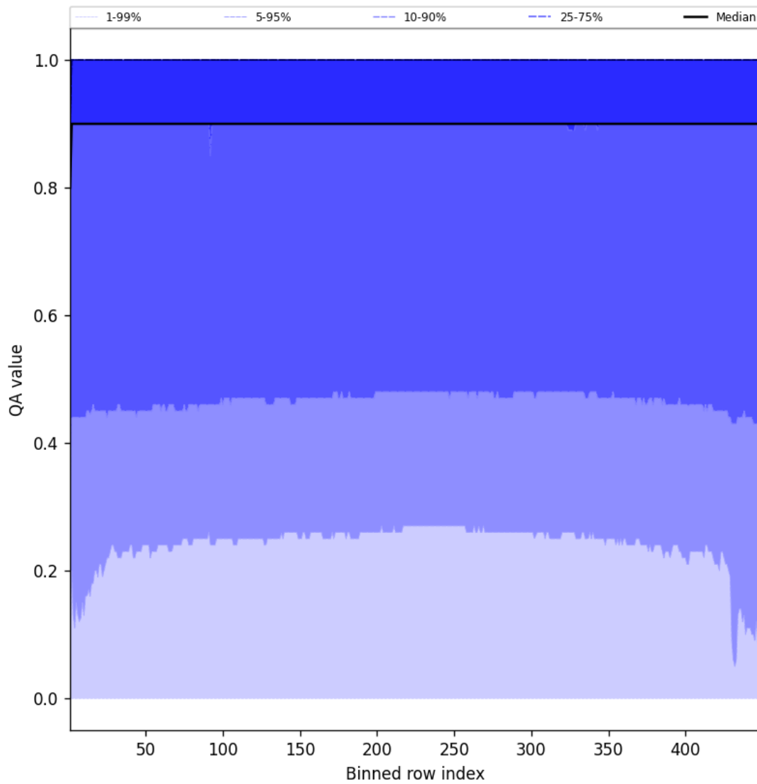
Figure 40: Along track statistics of “QA value” for 2025-09-04 to 2025-09-05
