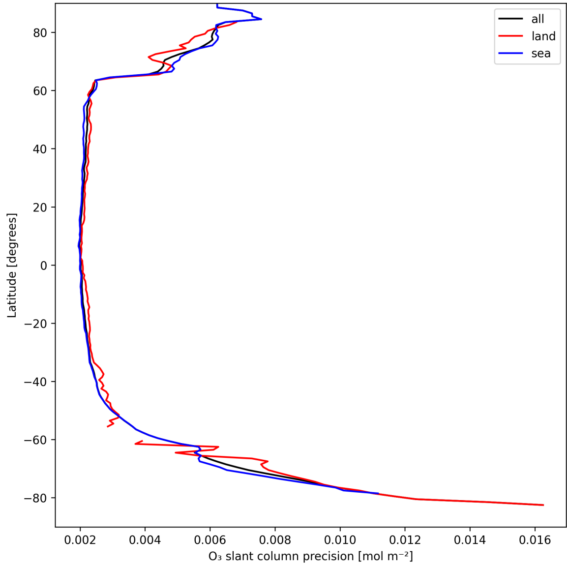
Figure 20: Zonal average of “O 3 slant column precision” for 2025-09-04 to 2025-09-05.
