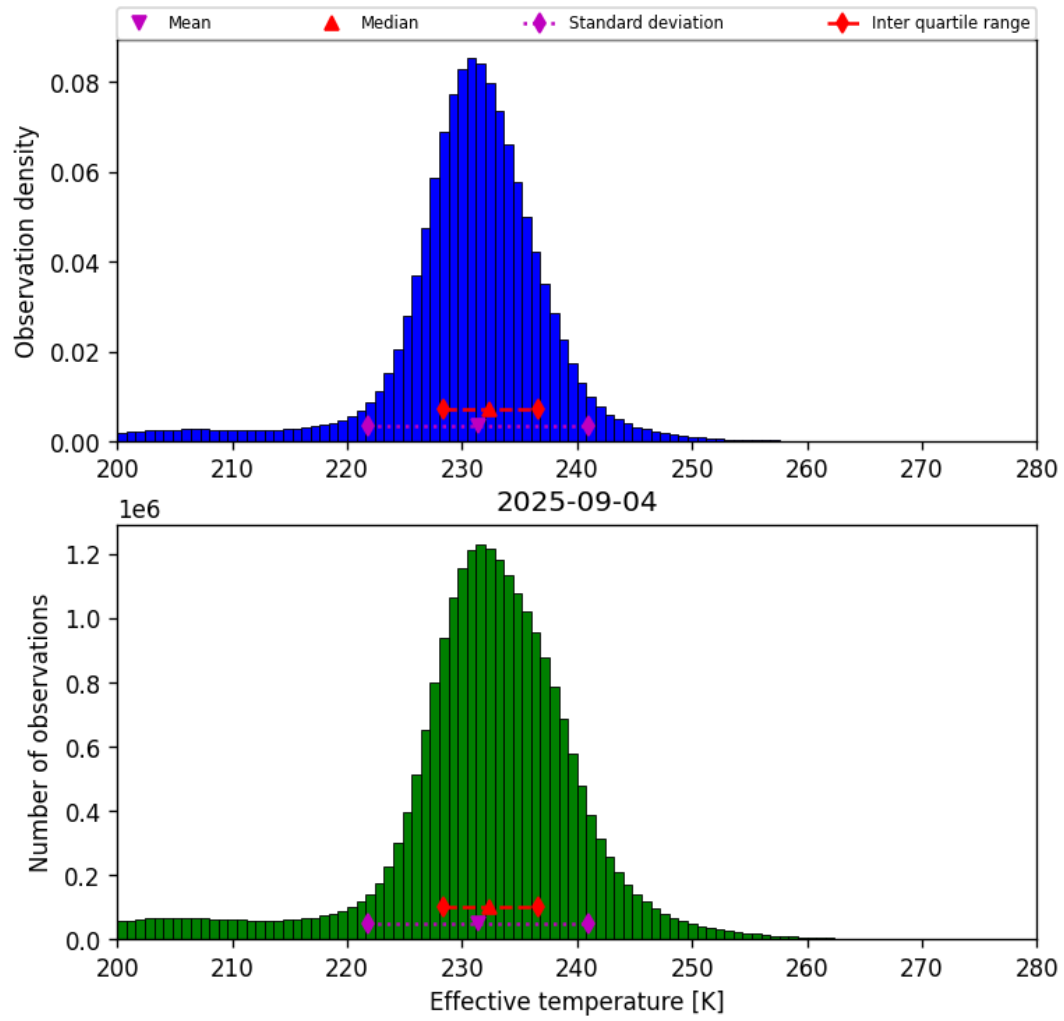
Figure 38: Histogram of “Effective temperature” for 2025-09-04 to 2025-09-05
