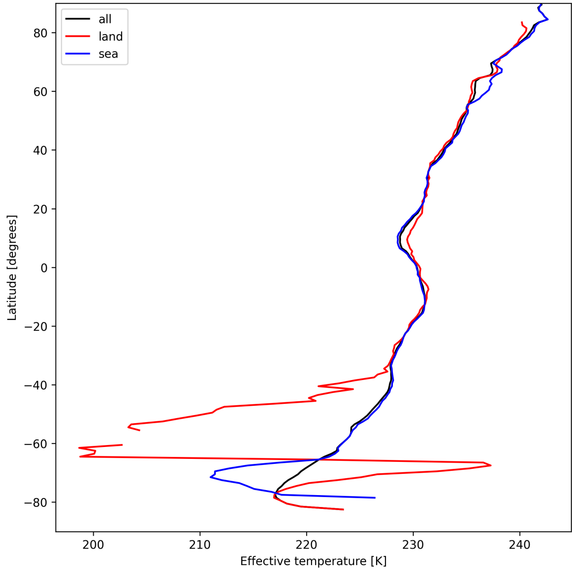
Figure 26: Zonal average of “Effective temperature” for 2025-09-04 to 2025-09-05.
