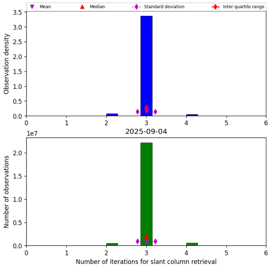
Figure 33: Histogram of “Number of iterations for slant column retrieval” for 2025-09-04 to 2025-09-05
