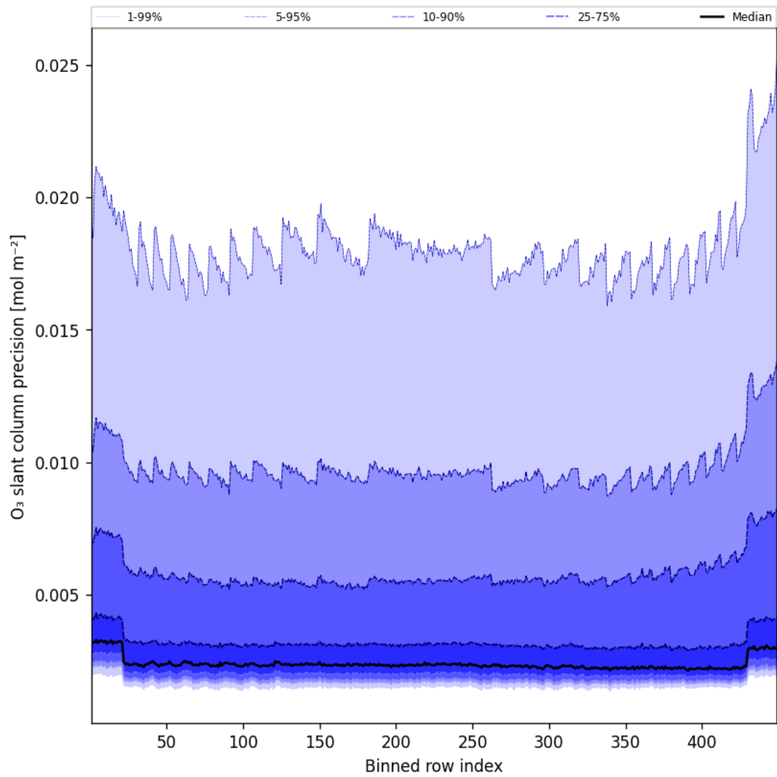
Figure 44: Along track statistics of “O 3 slant column precision” for 2025-09-04 to 2025-09-05
