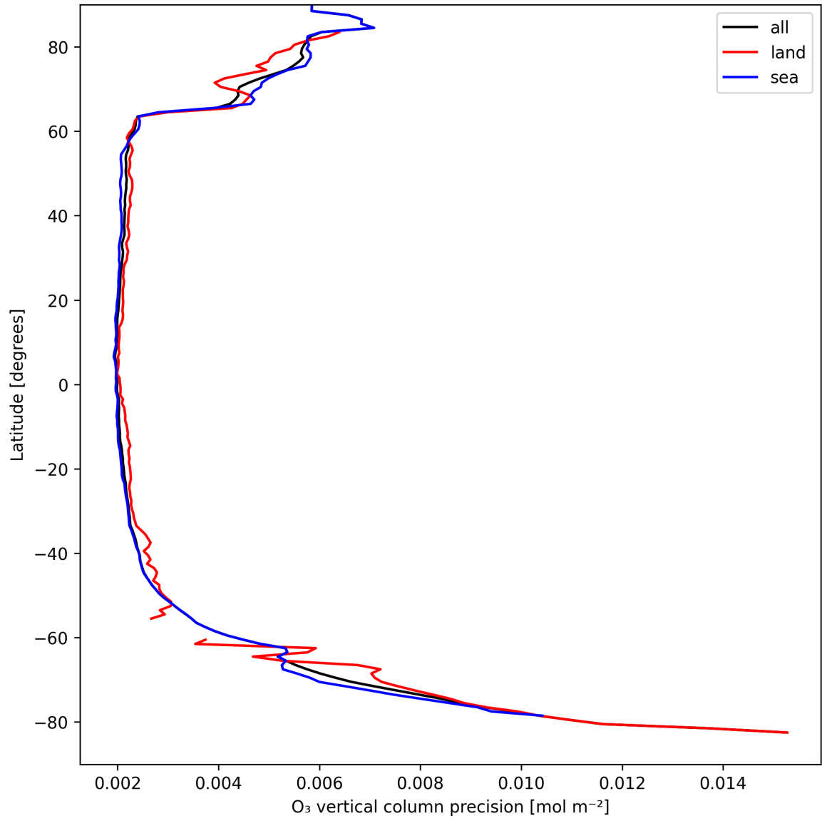
Figure 18: Zonal average of "O 3 vertical column precision" for 2025-09-04 to 2025-09-05.
