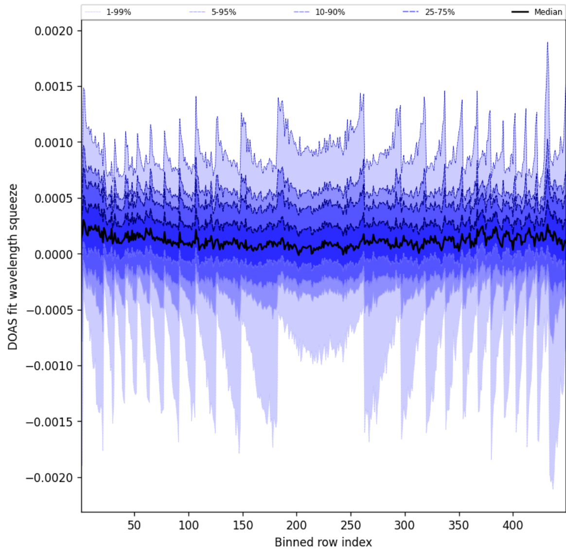
Figure 48: Along track statistics of “DOAS fit wavelength squeeze” for 2025-09-04 to 2025-09-05
