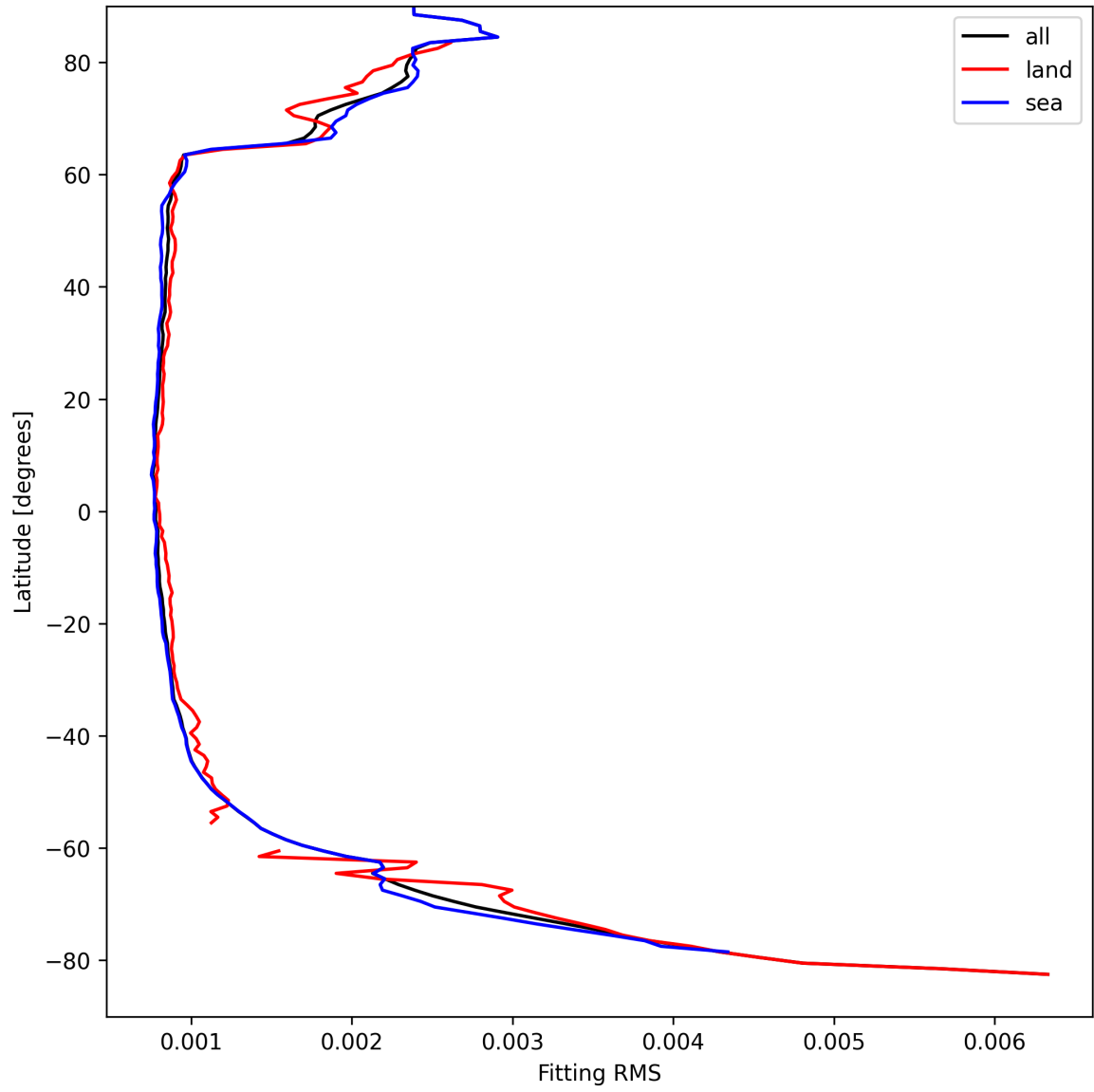
Figure 22: Zonal average of “Fitting RMS” for 2025-09-04 to 2025-09-05.
