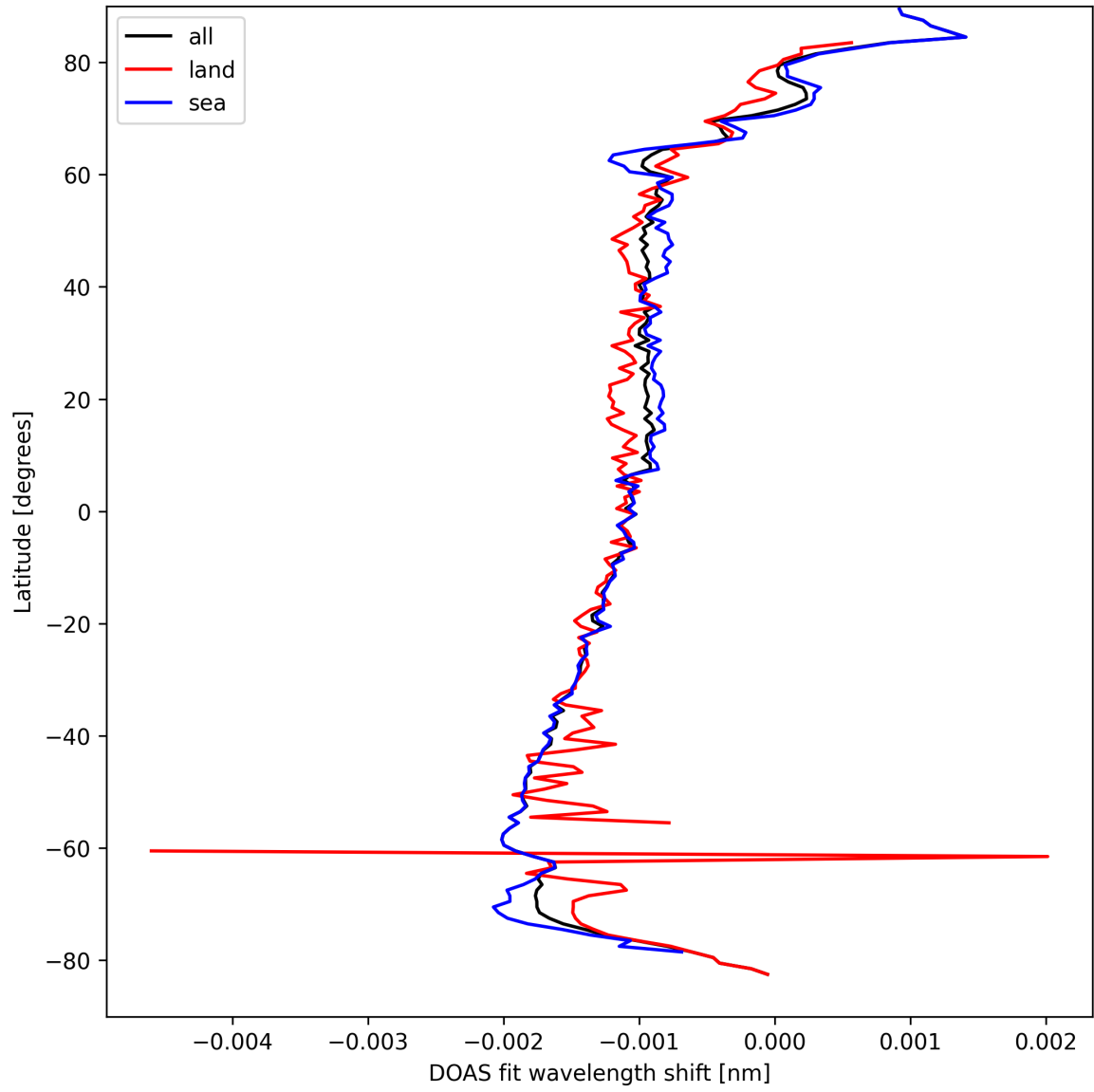
Figure 23: Zonal average of “DOAS fit wavelength shift” for 2025-09-04 to 2025-09-05.
