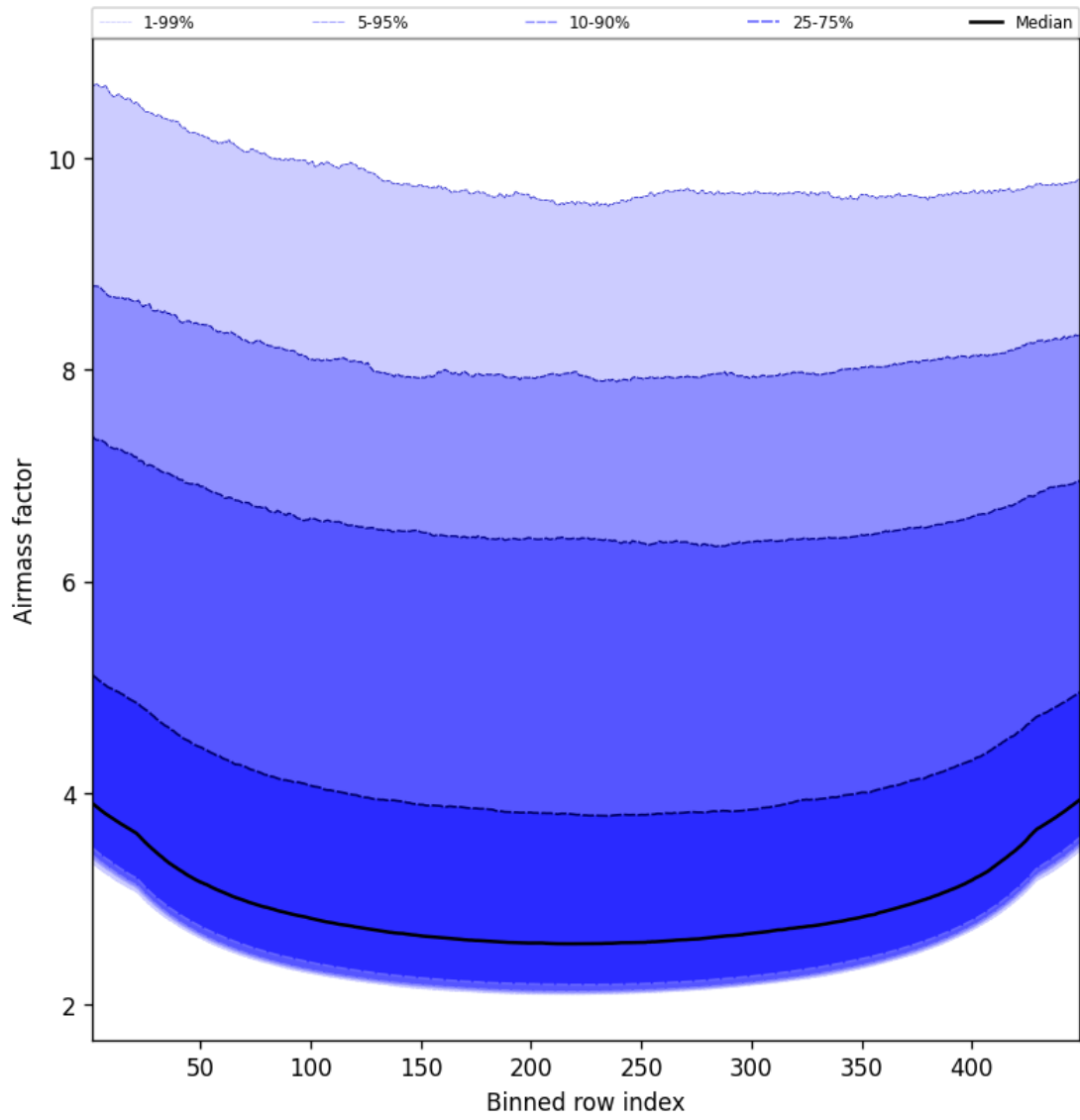
Figure 49: Along track statistics of “Airmass factor” for 2025-09-05 to 2025-09-06
