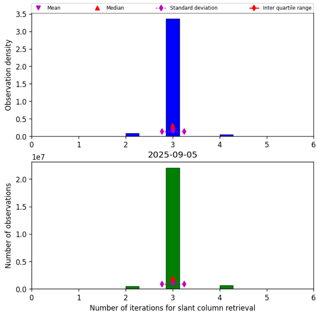
Figure 33: Histogram of “Number of iterations for slant column retrieval” for 2025-09-05 to 2025-09-06
