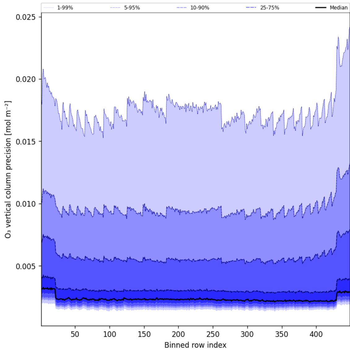
Figure 42: Along track statistics of “O 3 vertical column precision” for 2025-09-05 to 2025-09-06
