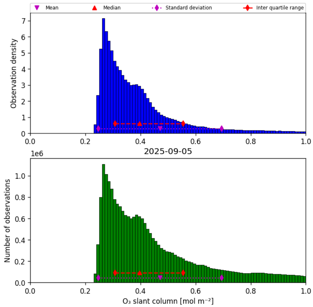
Figure 31: Histogram of “O 3 slant column” for 2025-09-05 to 2025-09-06
