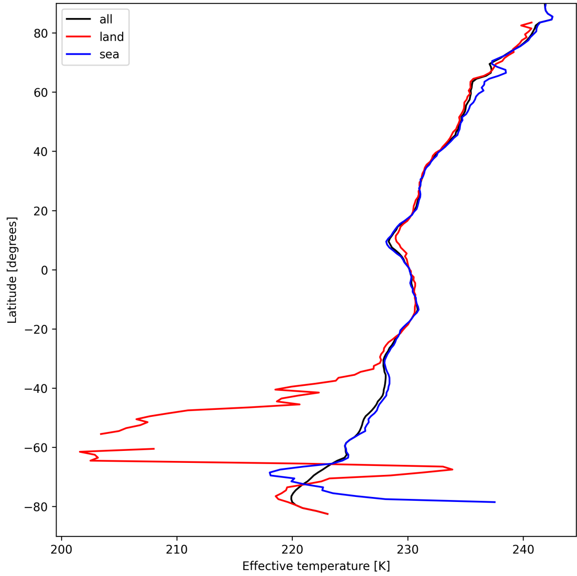
Figure 26: Zonal average of "Effective temperature" for 2025-09-05 to 2025-09-06.
