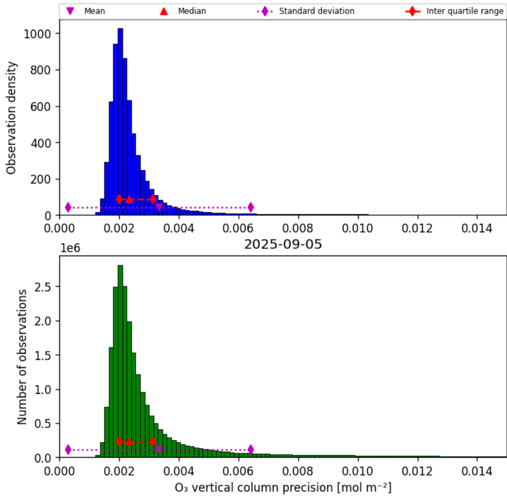
Figure 30: Histogram of “O 3 vertical column precision” for 2025-09-05 to 2025-09-06
