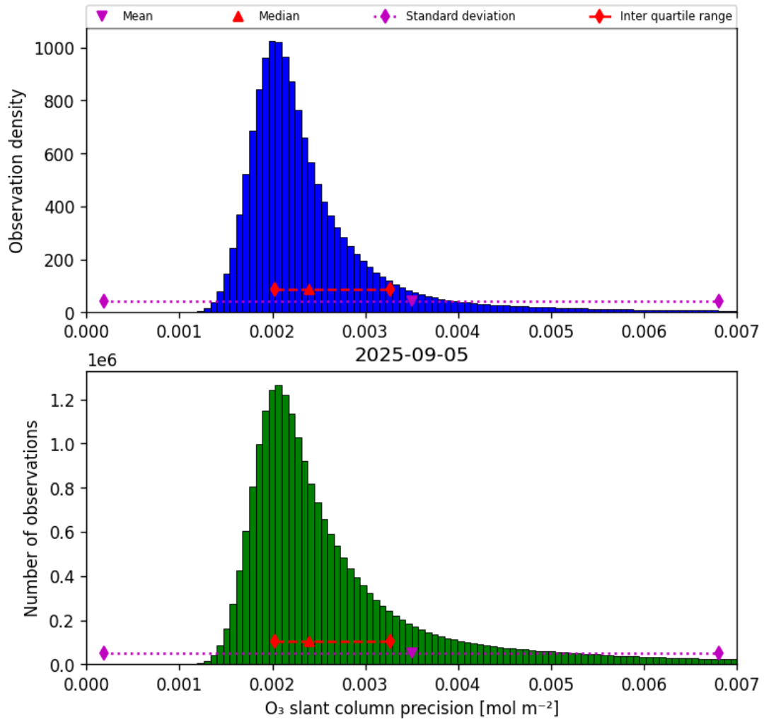
Figure 32: Histogram of “O 3 slant column precision” for 2025-09-05 to 2025-09-06
