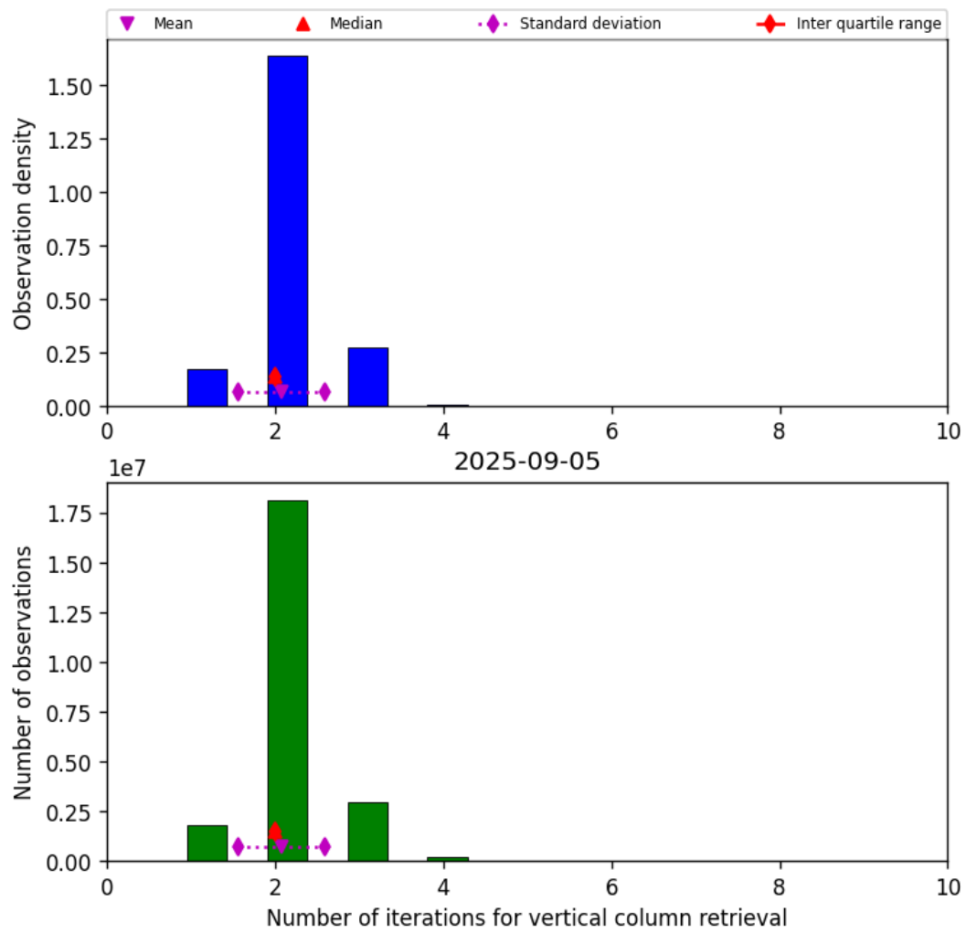
Figure 39: Histogram of “Number of iterations for vertical column retrieval” for 2025-09-05 to 2025-09-06
