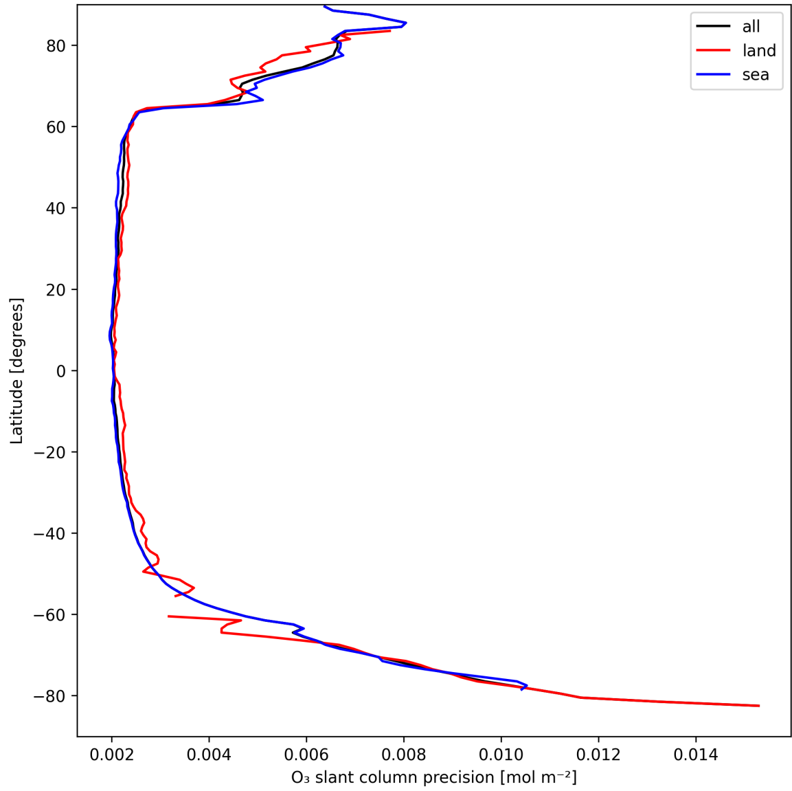
Figure 20: Zonal average of “O 3 slant column precision” for 2025-09-05 to 2025-09-06.
