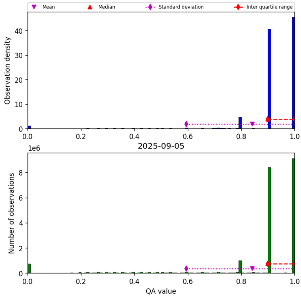
Figure 28: Histogram of “QA value” for 2025-09-05 to 2025-09-06
