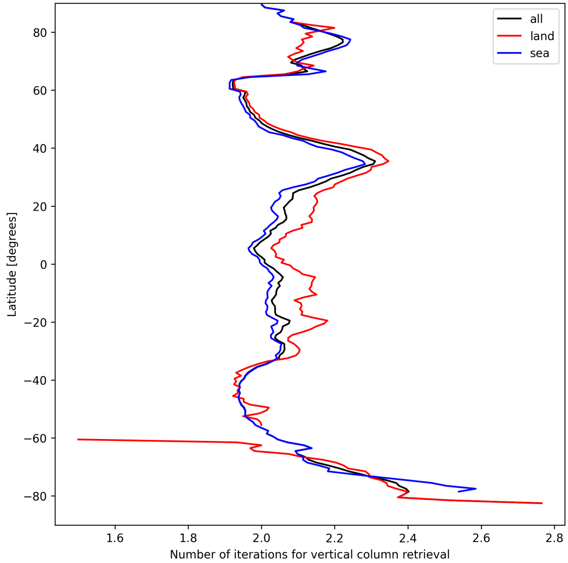
Figure 27: Zonal average of “Number of iterations for vertical column retrieval” for 2025-09-05 to 2025-09-06.
