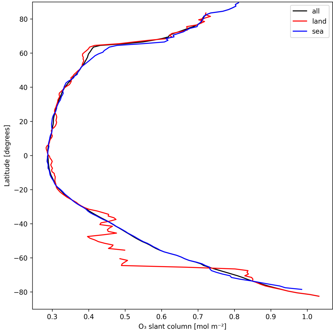
Figure 19: Zonal average of “O 3 slant column” for 2025-09-05 to 2025-09-06.
