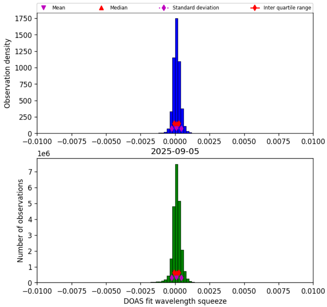
Figure 36: Histogram of “DOAS fit wavelength squeeze” for 2025-09-05 to 2025-09-06
