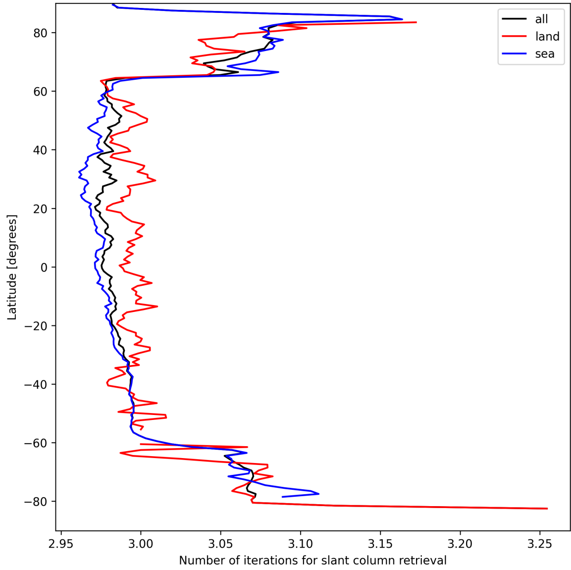
Figure 21: Zonal average of “Number of iterations for slant column retrieval” for 2025-09-05 to 2025-09-06.
