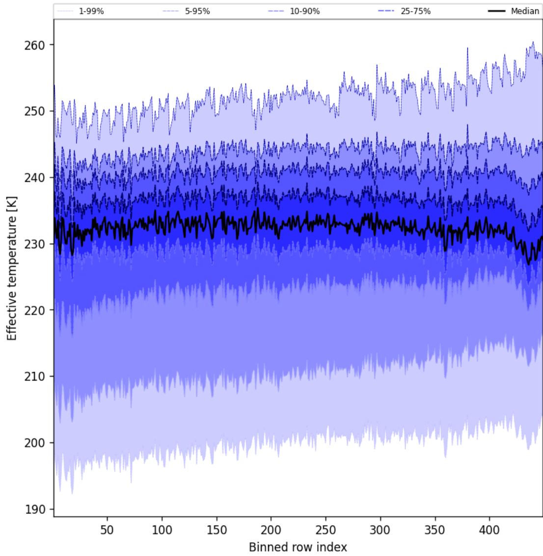
Figure 50: Along track statistics of “Effective temperature” for 2025-09-05 to 2025-09-06
