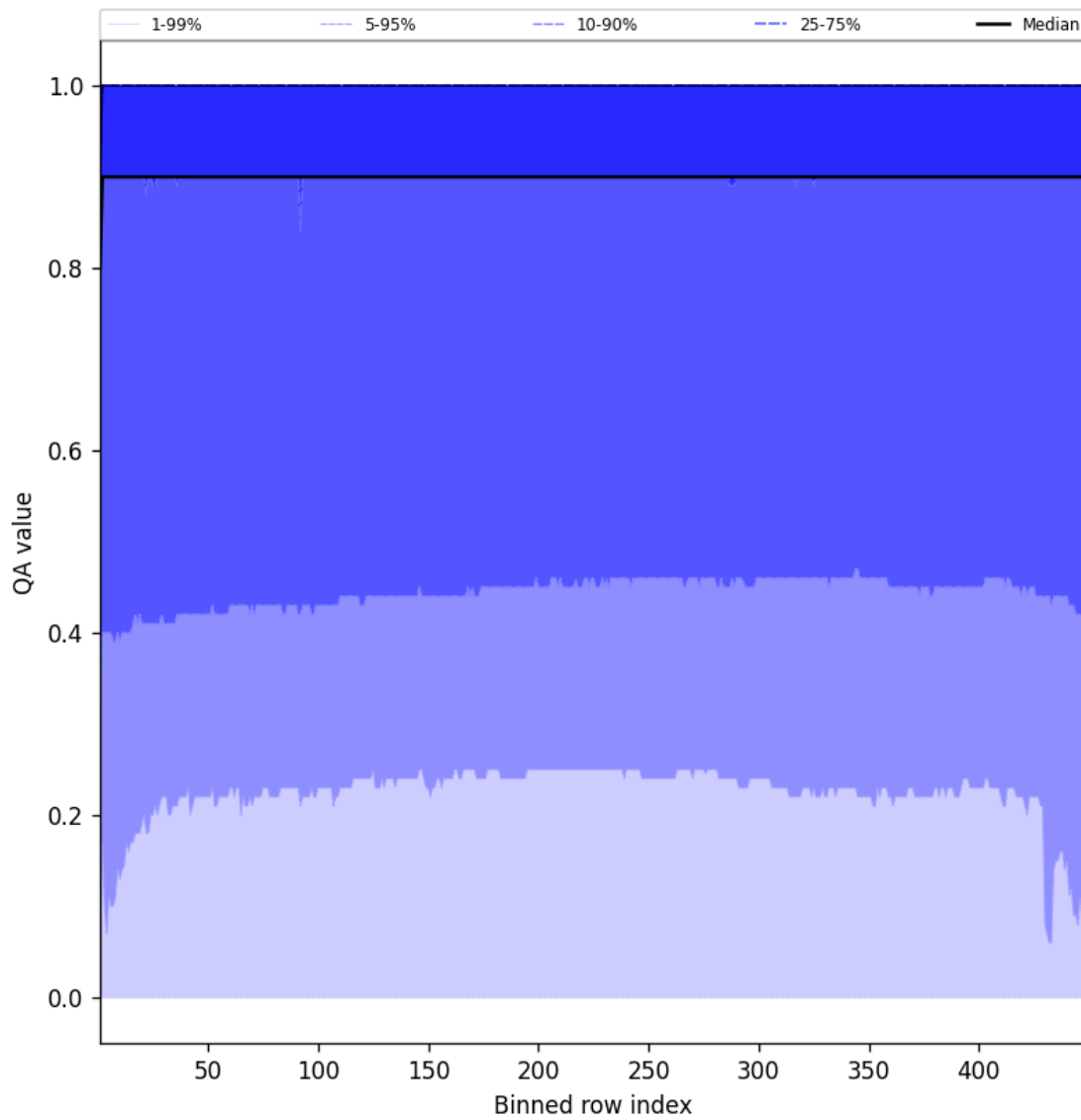
Figure 40: Along track statistics of “QA value” for 2025-09-05 to 2025-09-06
