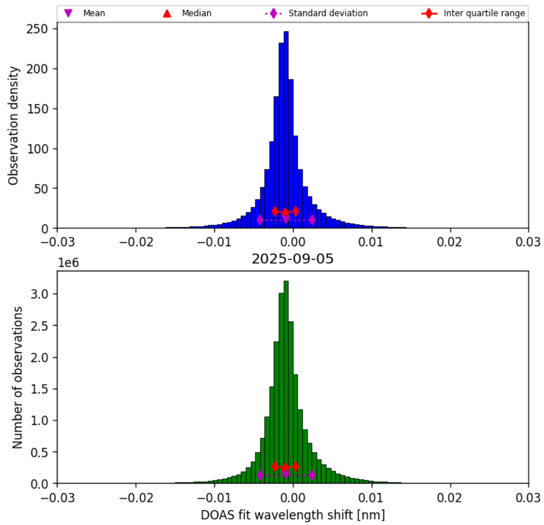
Figure 35: Histogram of “DOAS fit wavelength shift” for 2025-09-05 to 2025-09-06
