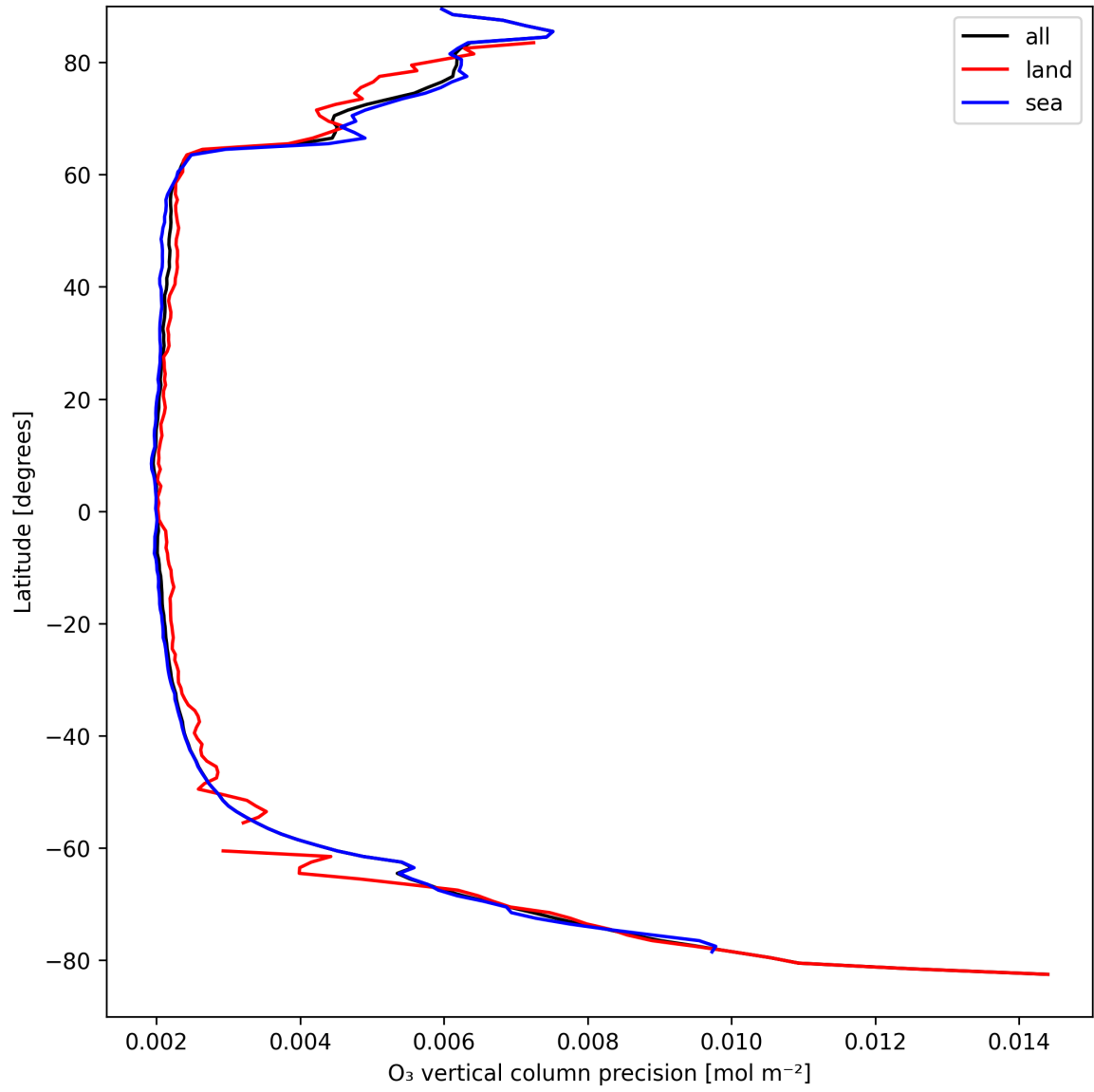
Figure 18: Zonal average of “O 3 vertical column precision” for 2025-09-05 to 2025-09-06.
