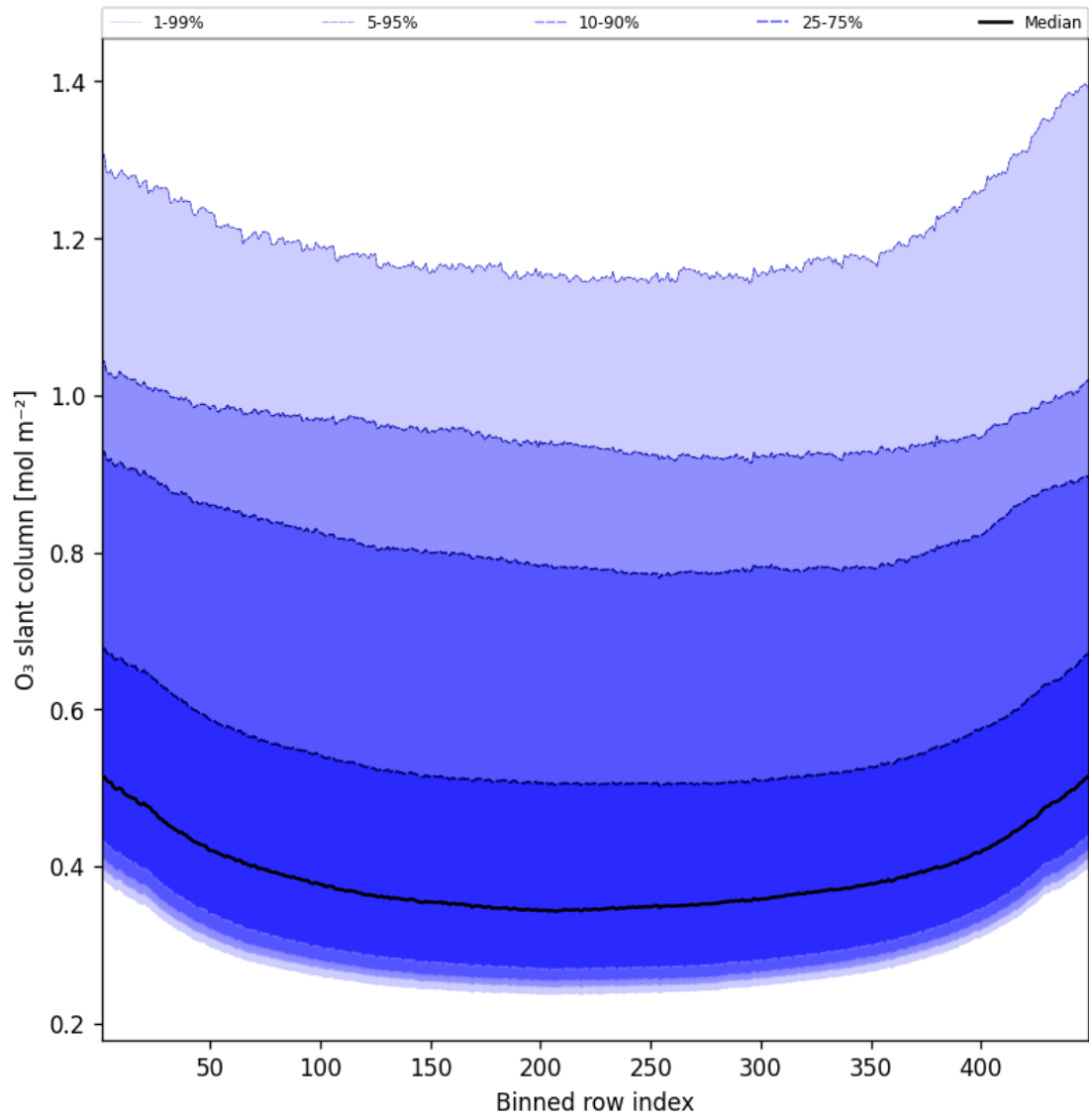
Figure 43: Along track statistics of “O 3 slant column” for 2025-09-05 to 2025-09-06
