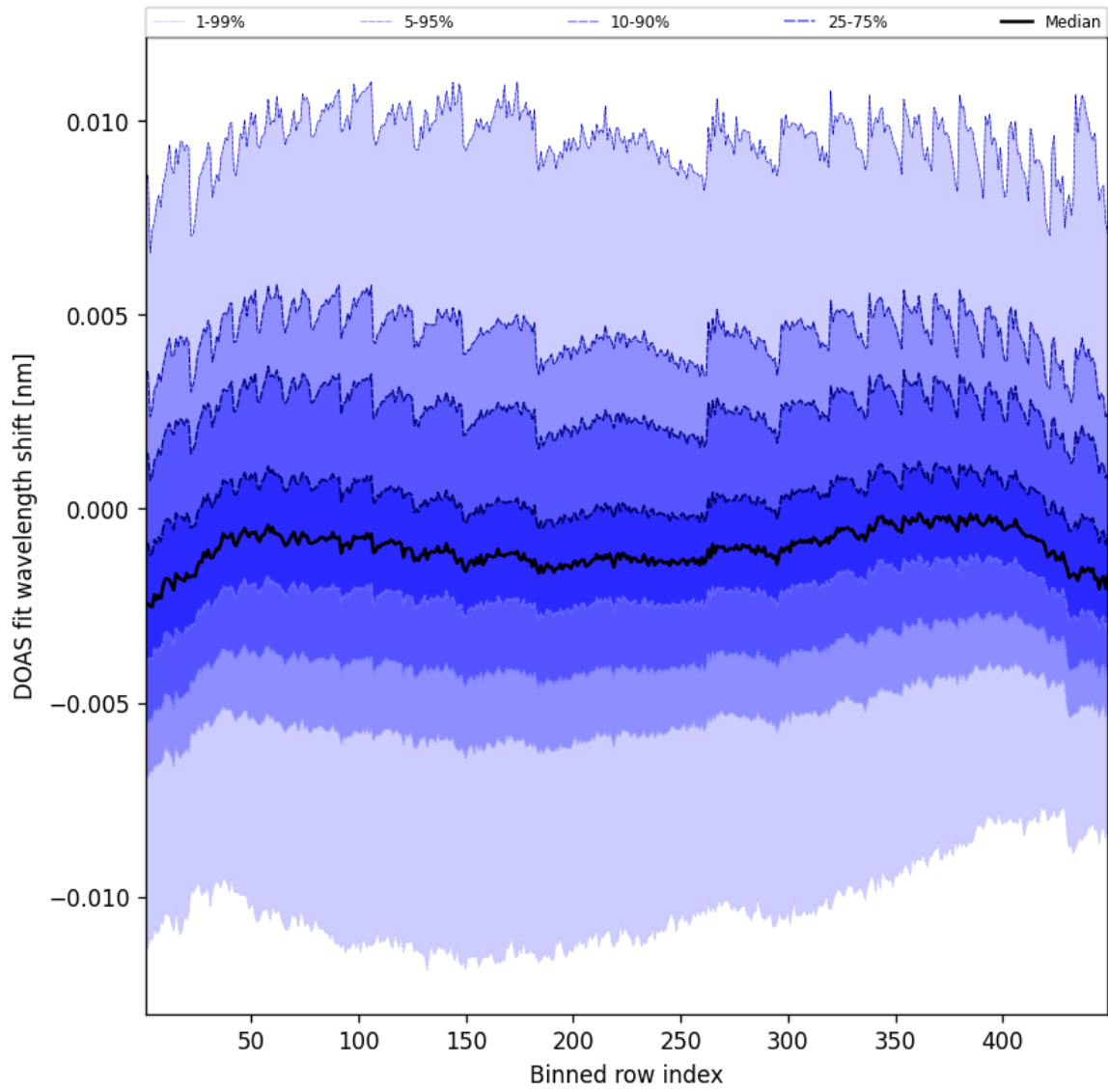
Figure 47: Along track statistics of "DOAS fit wavelength shift" for 2025-09-05 to 2025-09-06
