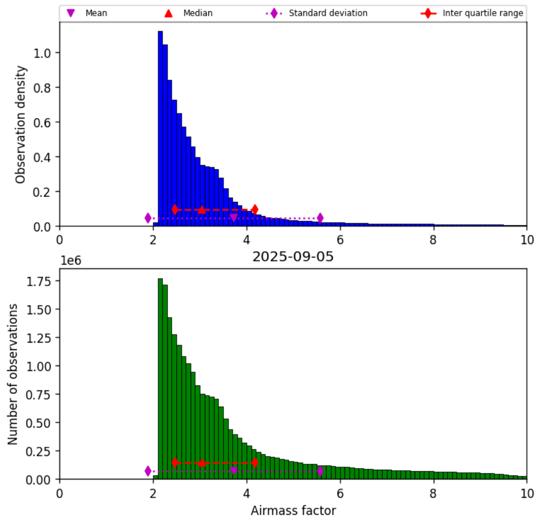
Figure 37: Histogram of “Airmass factor” for 2025-09-05 to 2025-09-06
