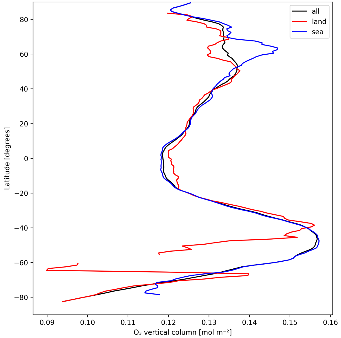
Figure 17: Zonal average of “O 3 vertical column” for 2025-09-05 to 2025-09-06.
