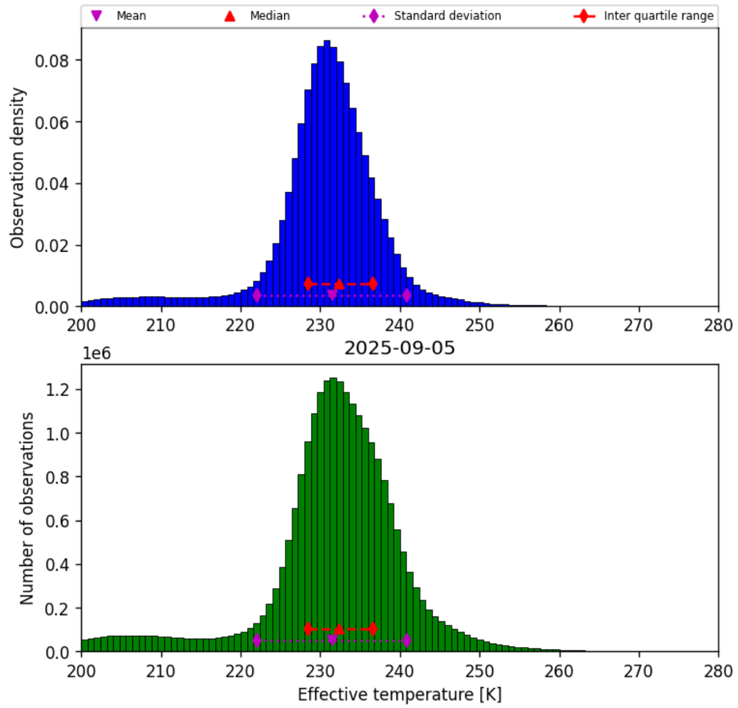
Figure 38: Histogram of “Effective temperature” for 2025-09-05 to 2025-09-06
