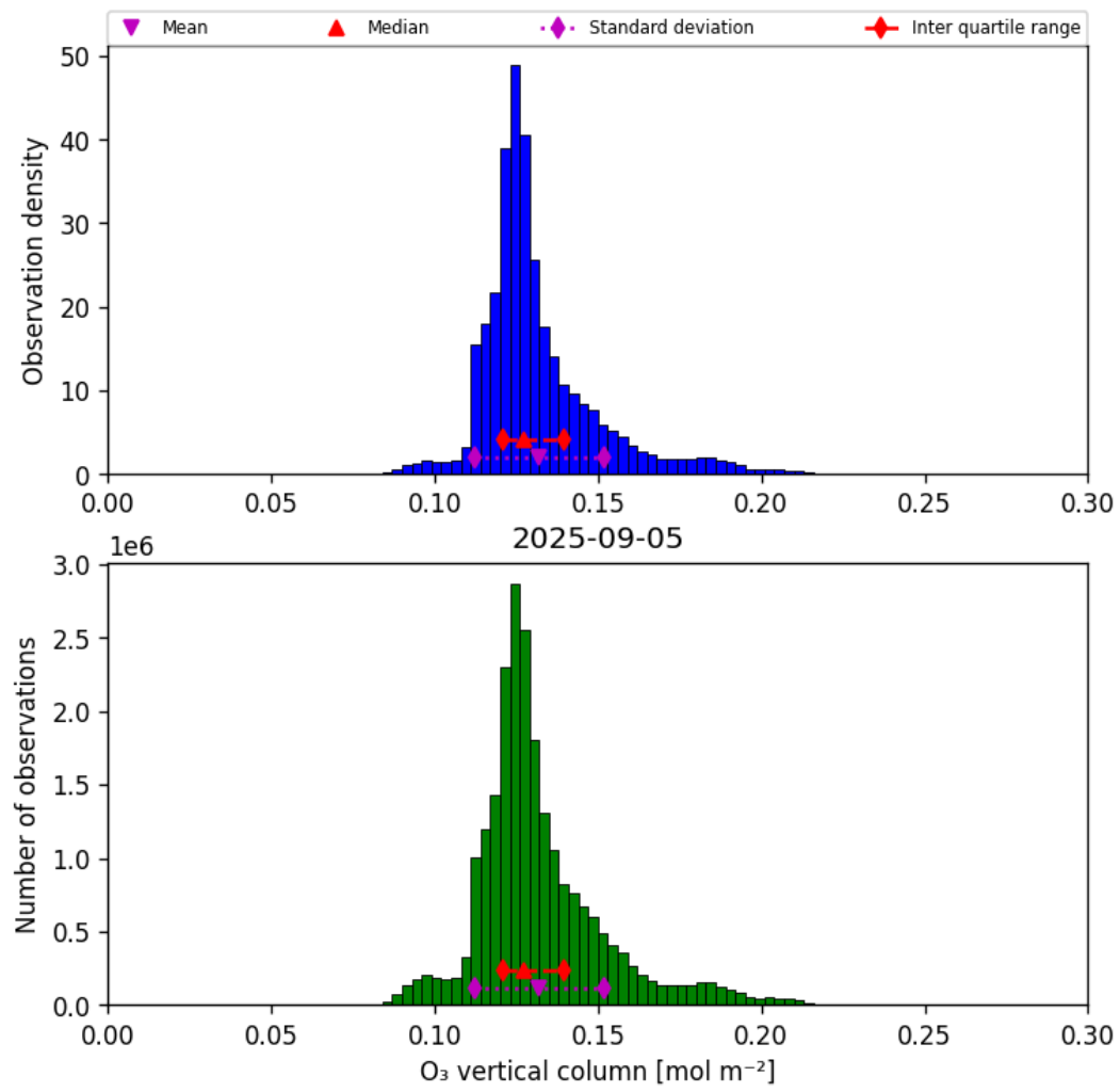
Figure 29: Histogram of “O 3 vertical column” for 2025-09-05 to 2025-09-06
