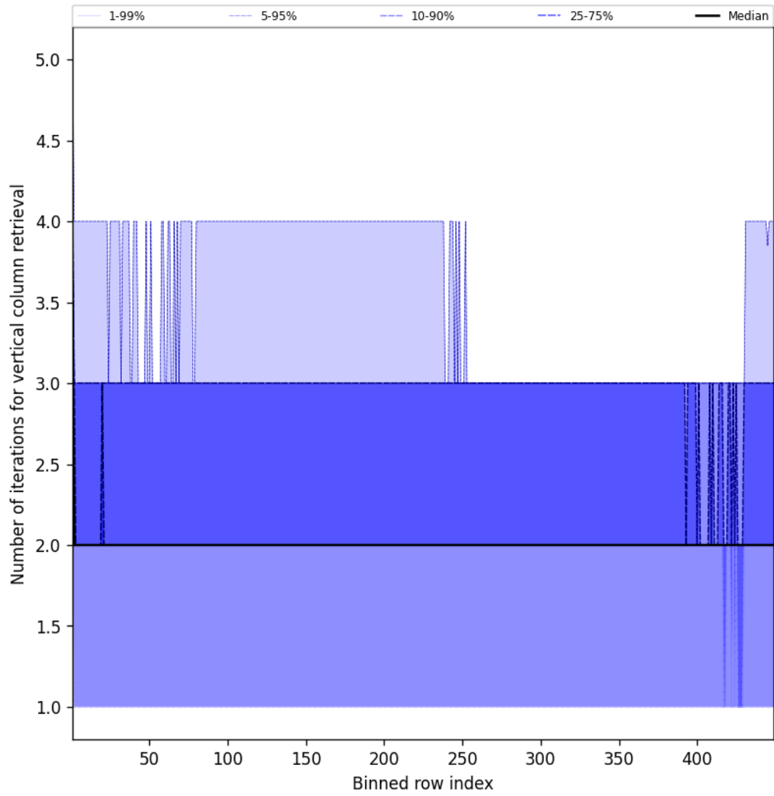
Figure 51: Along track statistics of “Number of iterations for vertical column retrieval” for 2025-09-05 to 2025-09-06
