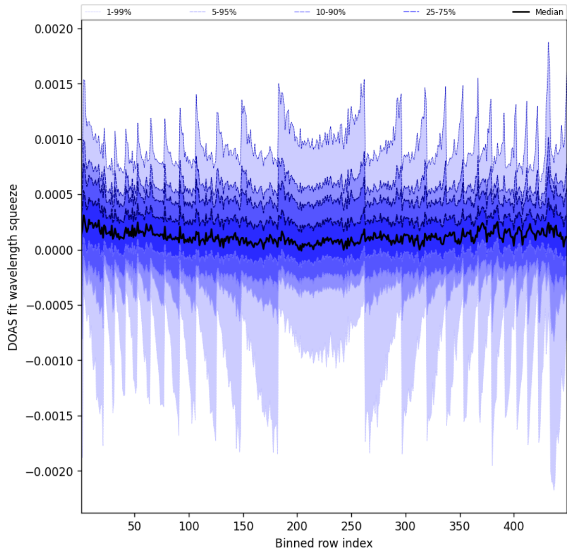
Figure 48: Along track statistics of “DOAS fit wavelength squeeze” for 2025-09-05 to 2025-09-06
