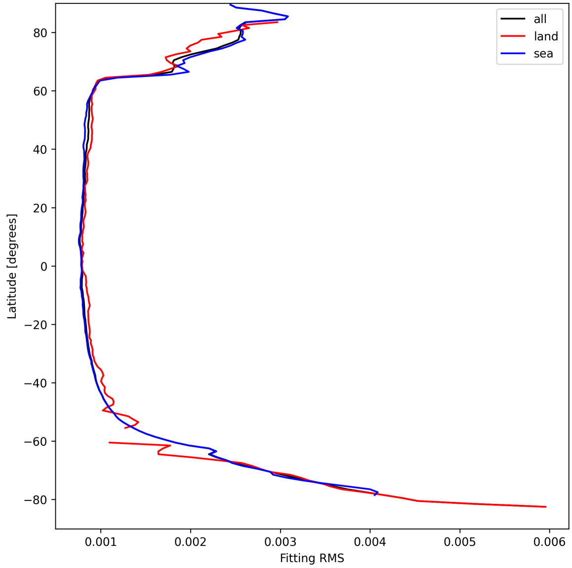
Figure 22: Zonal average of “Fitting RMS” for 2025-09-05 to 2025-09-06.
