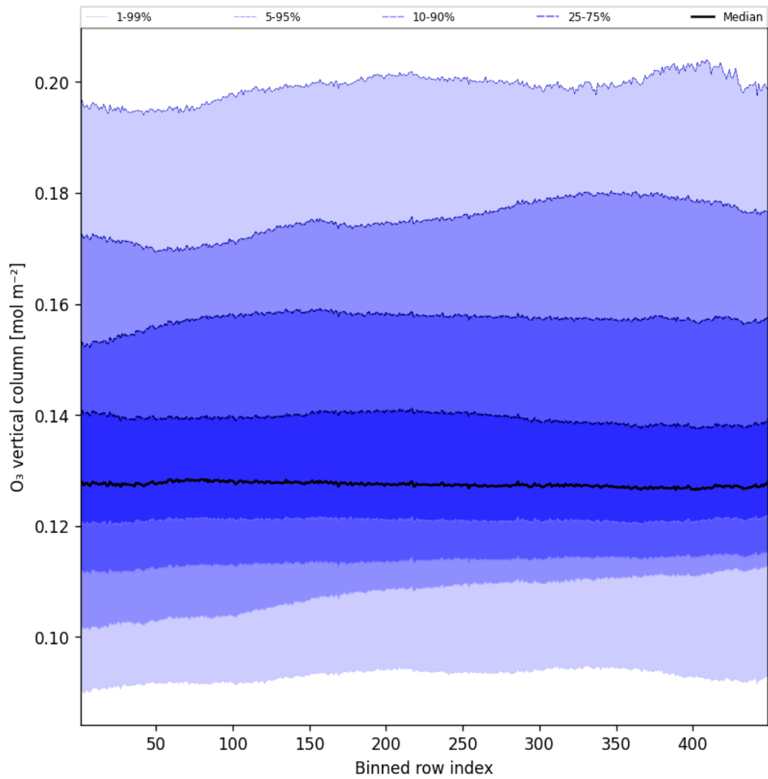
Figure 41: Along track statistics of “ \text{O}_3 vertical column” for 2025-09-05 to 2025-09-06
