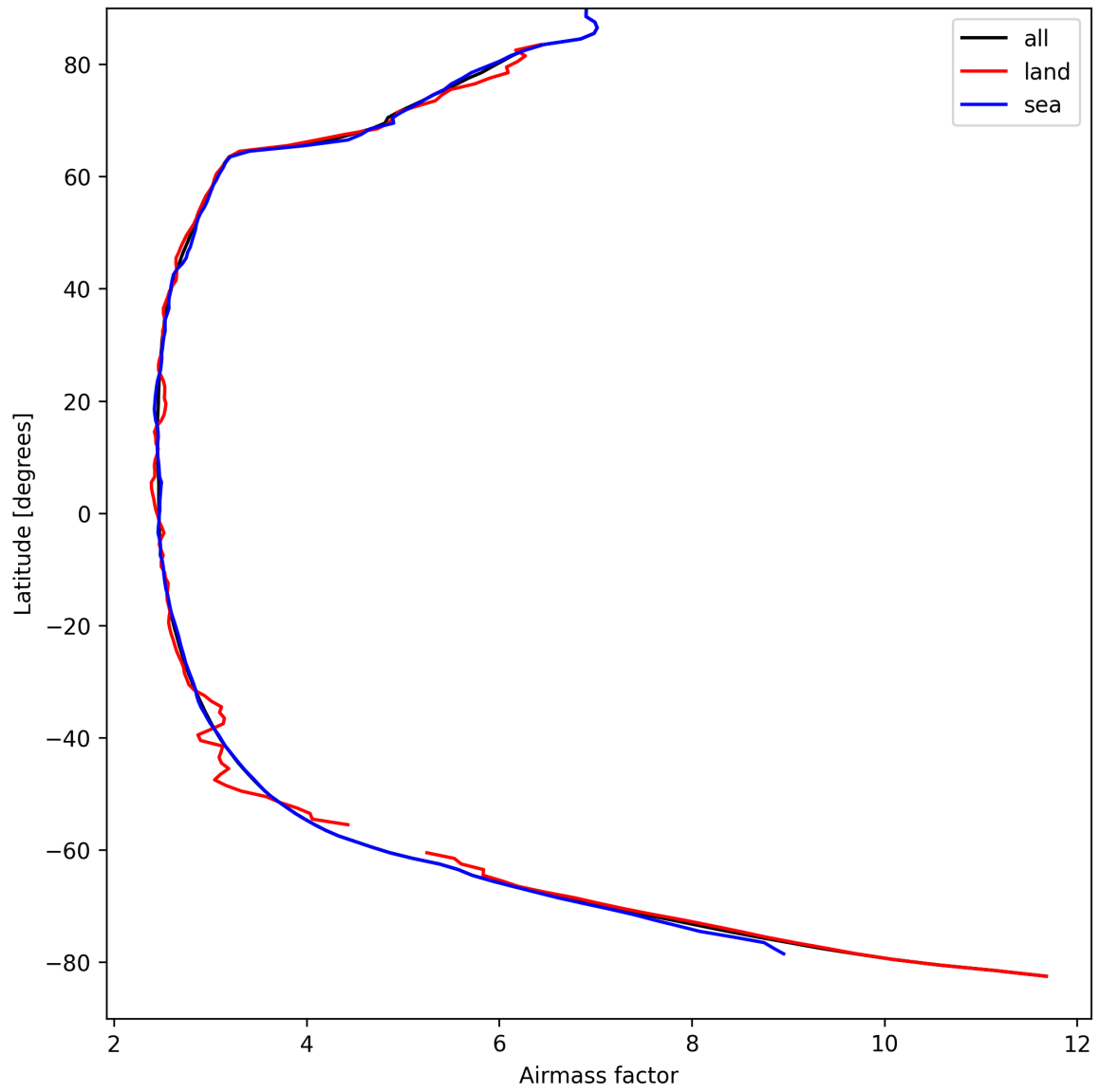
Figure 25: Zonal average of “Airmass factor” for 2025-09-05 to 2025-09-06.
