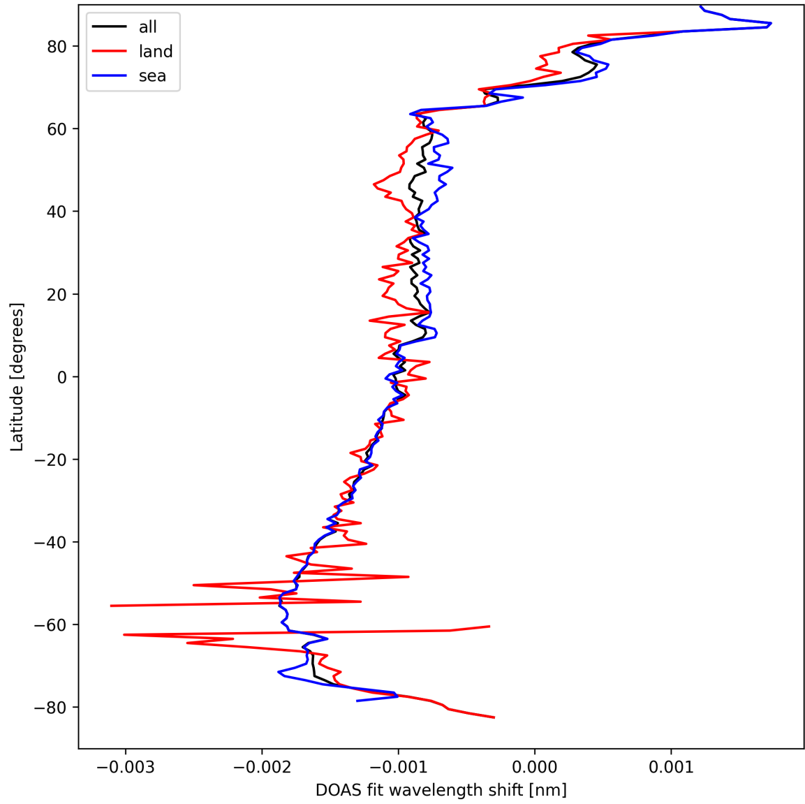
Figure 23: Zonal average of “DOAS fit wavelength shift” for 2025-09-05 to 2025-09-06.
