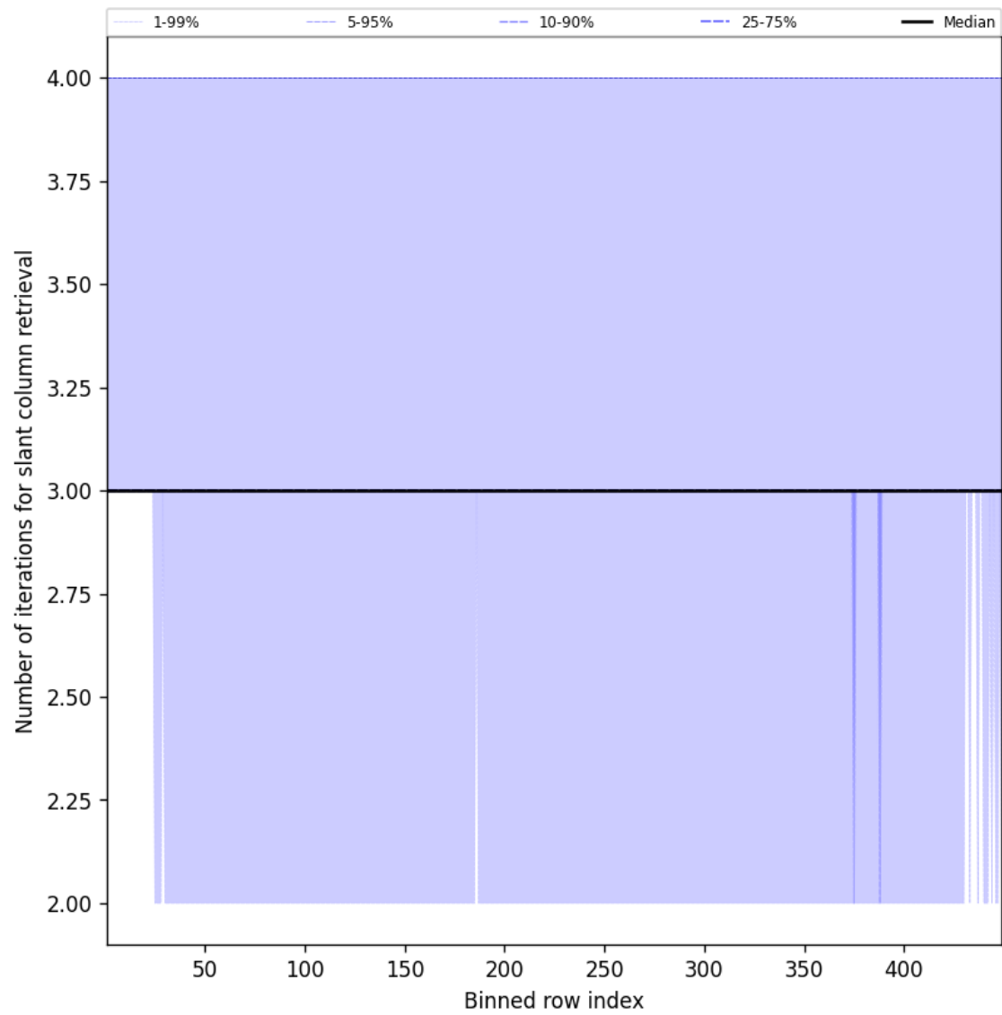
Figure 45: Along track statistics of “Number of iterations for slant column retrieval” for 2025-09-05 to 2025-09-06
