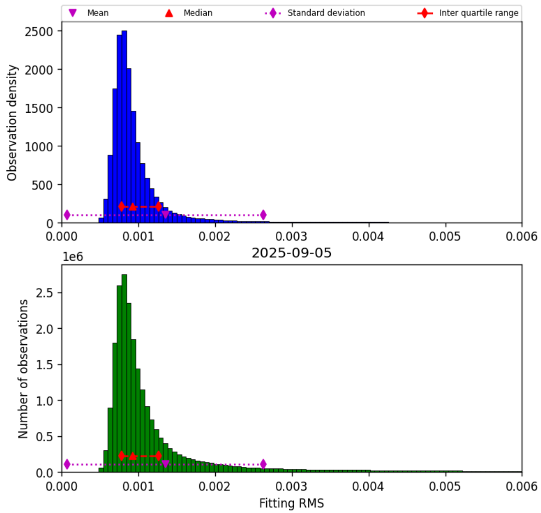
Figure 34: Histogram of “Fitting RMS” for 2025-09-05 to 2025-09-06
