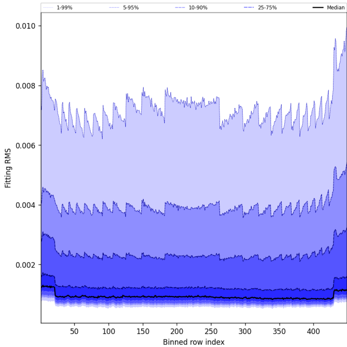
Figure 46: Along track statistics of “Fitting RMS” for 2025-09-05 to 2025-09-06
