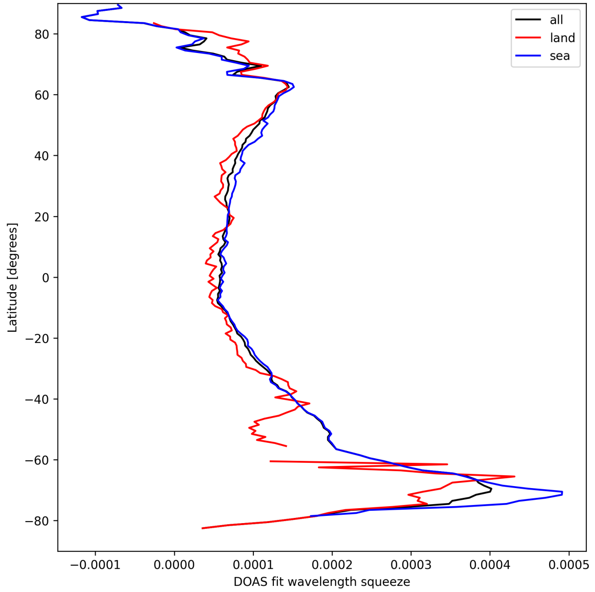
Figure 24: Zonal average of “DOAS fit wavelength squeeze” for 2025-09-05 to 2025-09-06.
