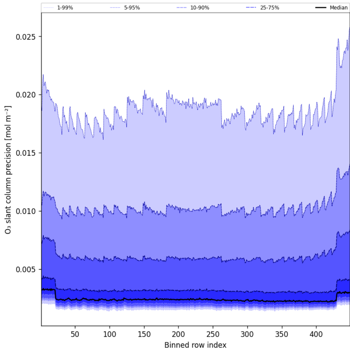
Figure 44: Along track statistics of “O 3 slant column precision” for 2025-09-05 to 2025-09-06
