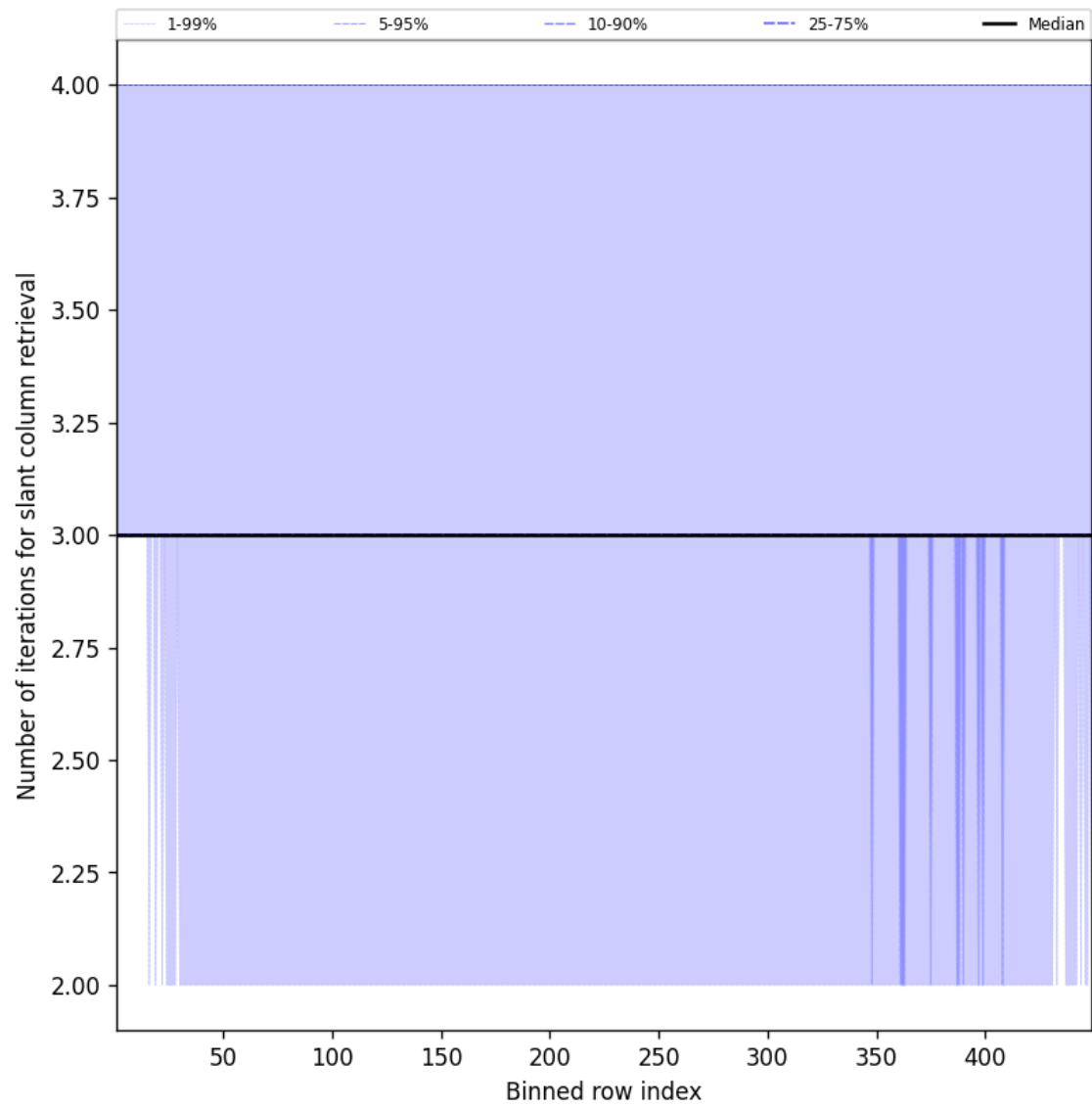
Figure 45: Along track statistics of “Number of iterations for slant column retrieval” for 2025-09-06 to 2025-09-07
