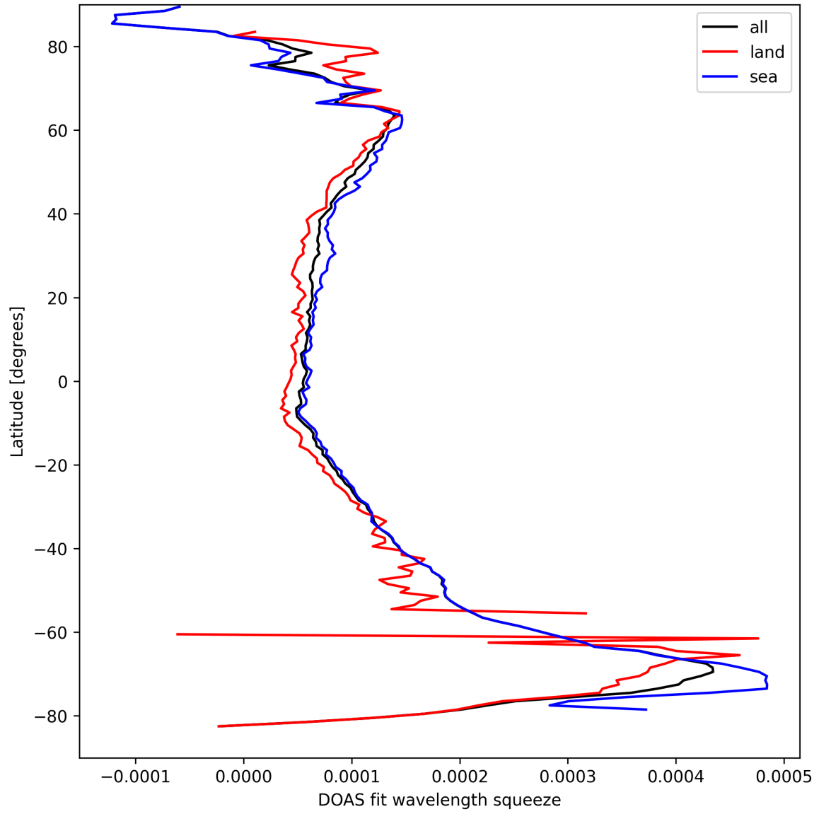
Figure 24: Zonal average of “DOAS fit wavelength squeeze” for 2025-09-06 to 2025-09-07.
