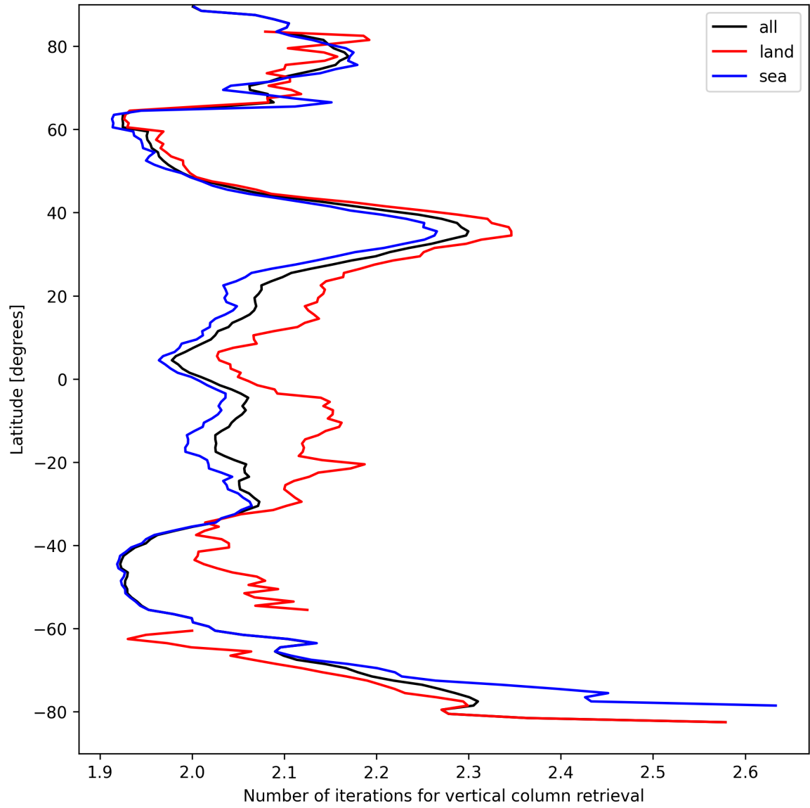
Figure 27: Zonal average of “Number of iterations for vertical column retrieval” for 2025-09-06 to 2025-09-07.
