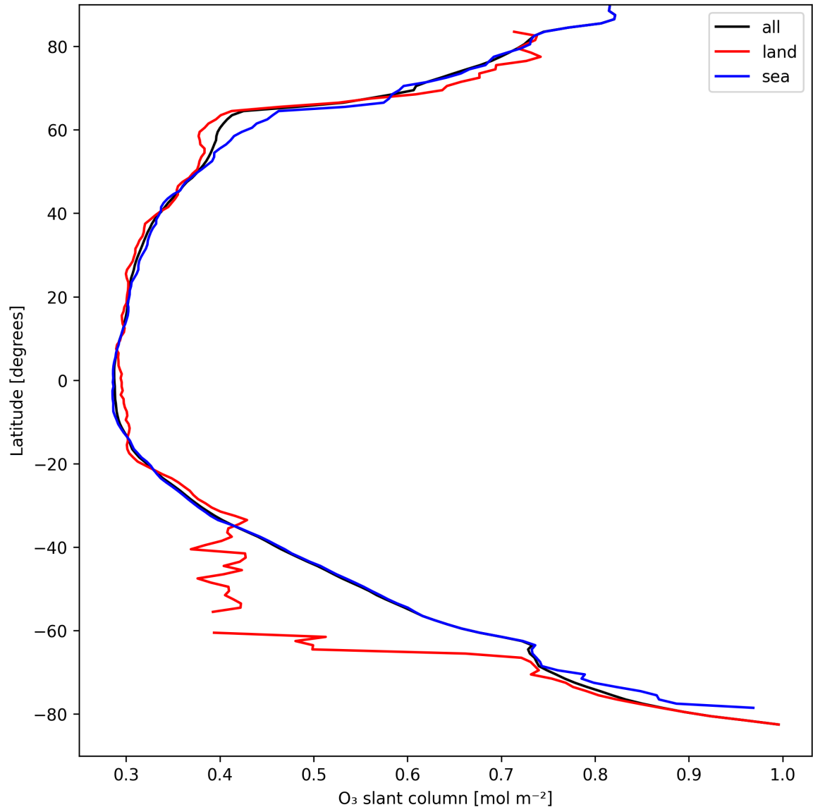
Figure 19: Zonal average of “O 3 slant column” for 2025-09-06 to 2025-09-07.
