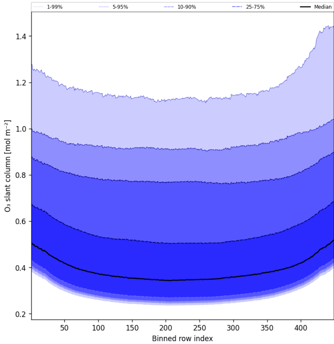
Figure 43: Along track statistics of “O 3 slant column” for 2025-09-06 to 2025-09-07
