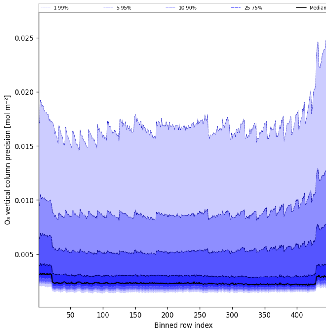
Figure 42: Along track statistics of “O 3 vertical column precision” for 2025-09-06 to 2025-09-07
