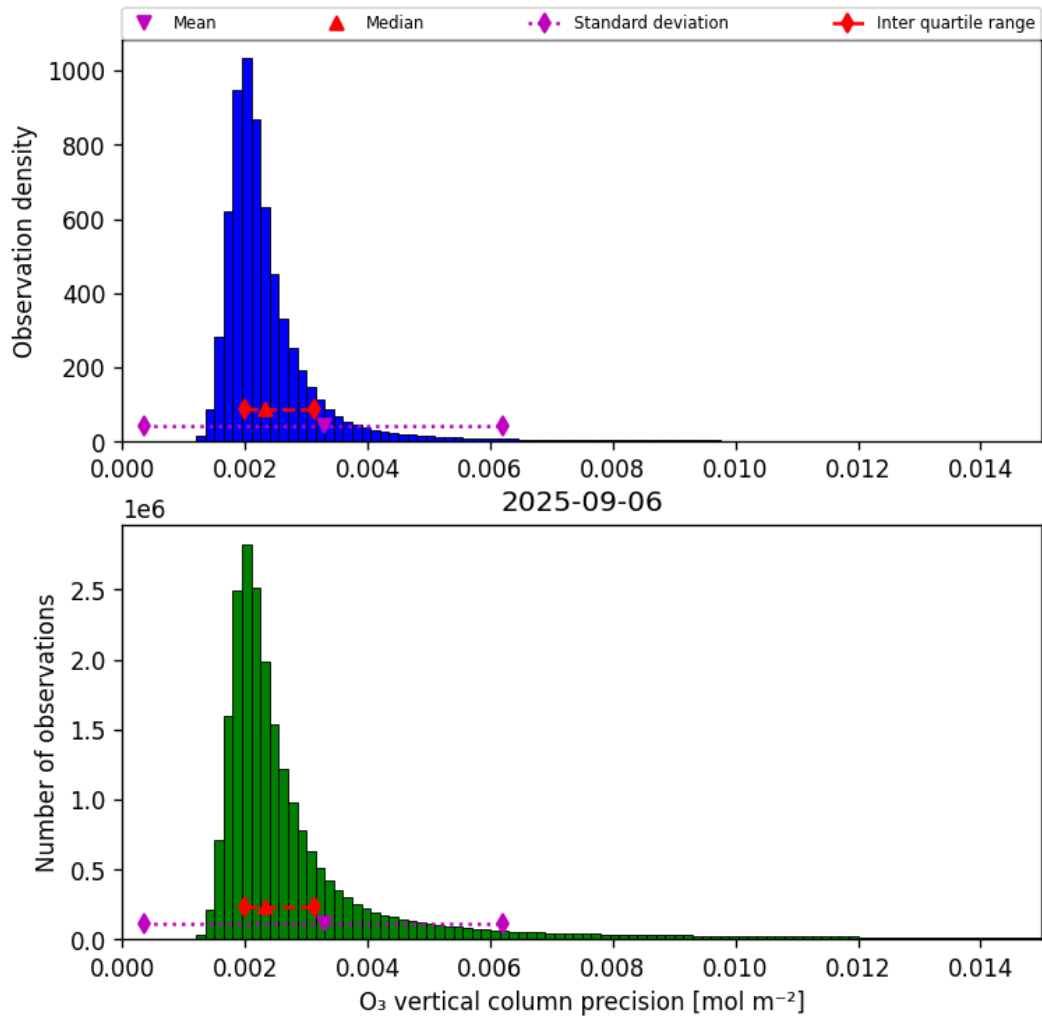
Figure 30: Histogram of “O 3 vertical column precision” for 2025-09-06 to 2025-09-07
