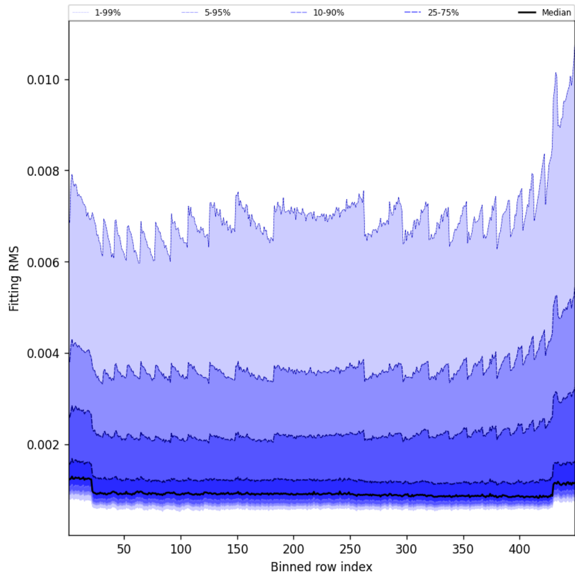
Figure 46: Along track statistics of “Fitting RMS” for 2025-09-06 to 2025-09-07
