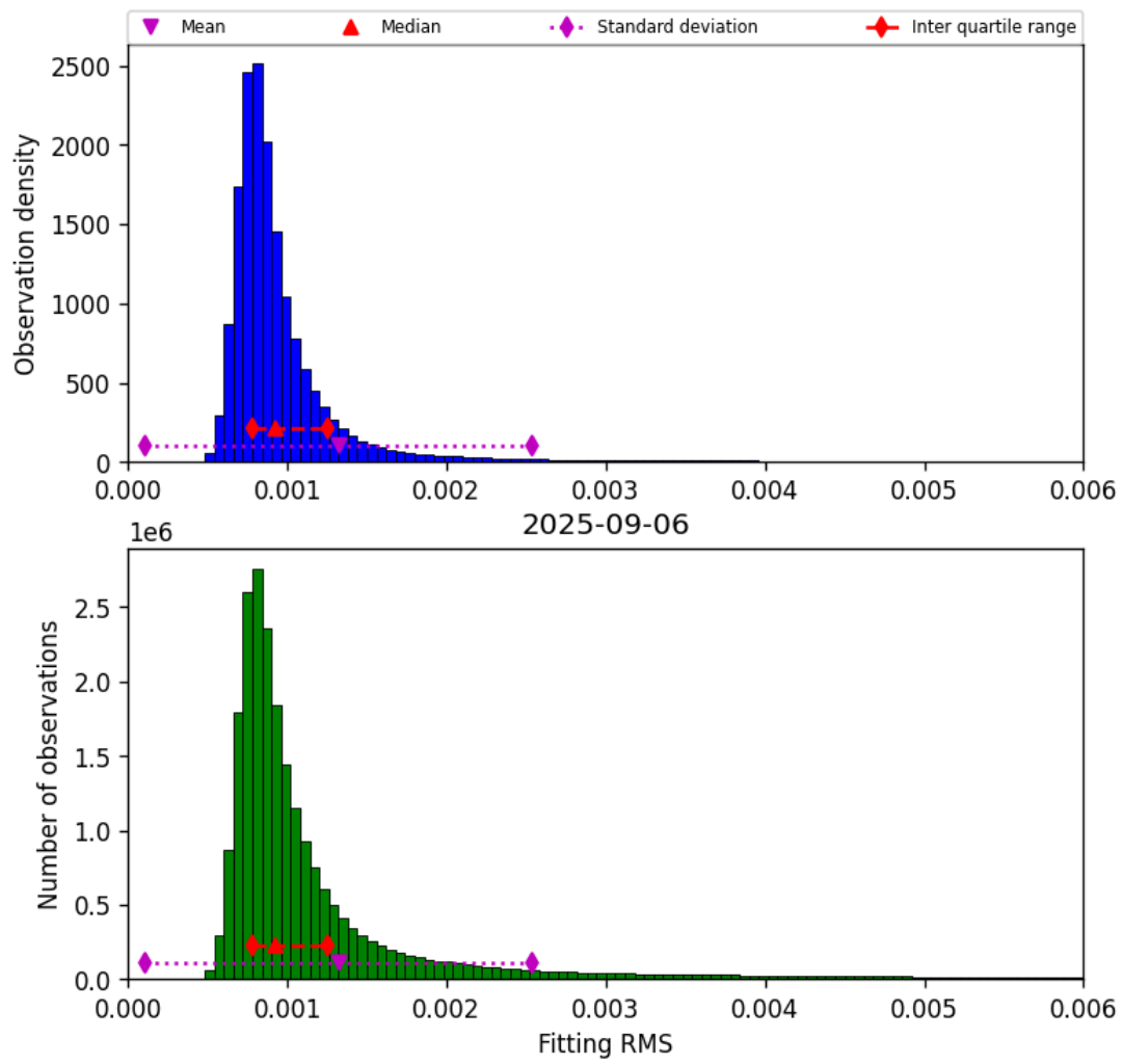
Figure 34: Histogram of “Fitting RMS” for 2025-09-06 to 2025-09-07
