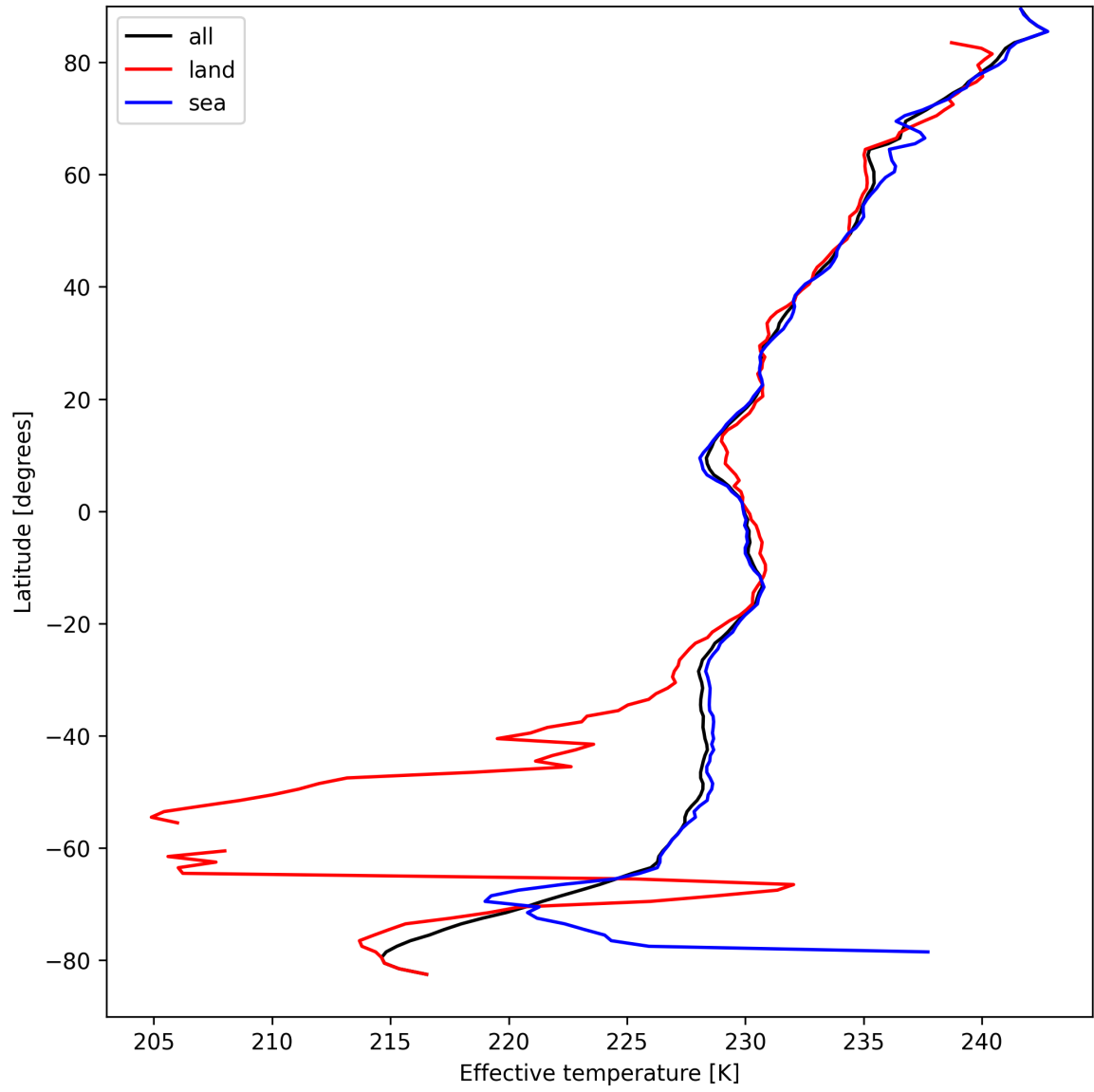
Figure 26: Zonal average of “Effective temperature” for 2025-09-06 to 2025-09-07.
