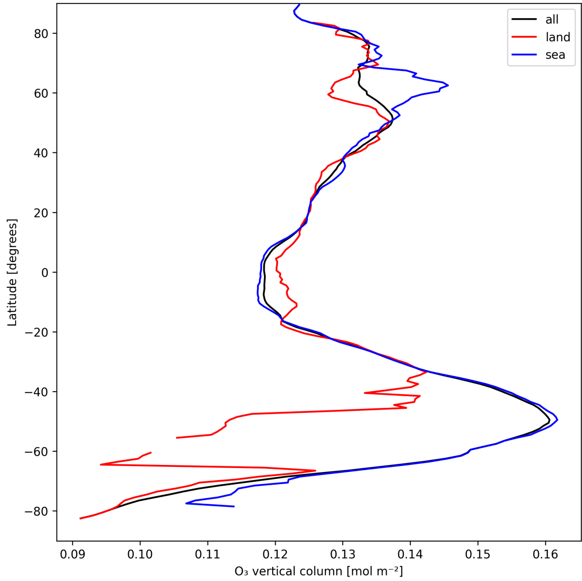
Figure 17: Zonal average of “O 3 vertical column” for 2025-09-06 to 2025-09-07.
