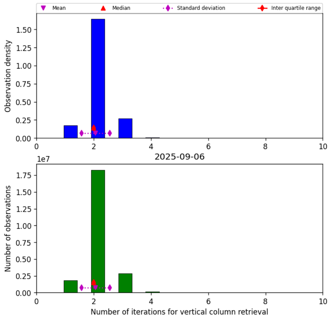
Figure 39: Histogram of “Number of iterations for vertical column retrieval” for 2025-09-06 to 2025-09-07
