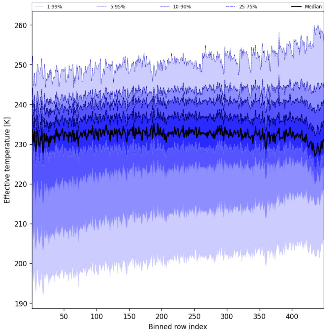
Figure 50: Along track statistics of “Effective temperature” for 2025-09-06 to 2025-09-07
