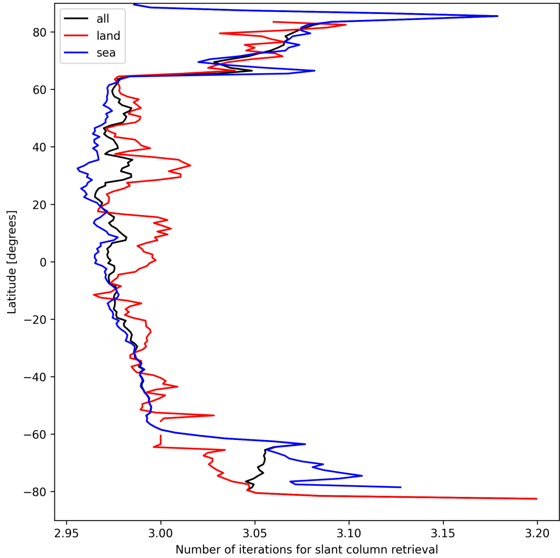
Figure 21: Zonal average of “Number of iterations for slant column retrieval” for 2025-09-06 to 2025-09-07.
