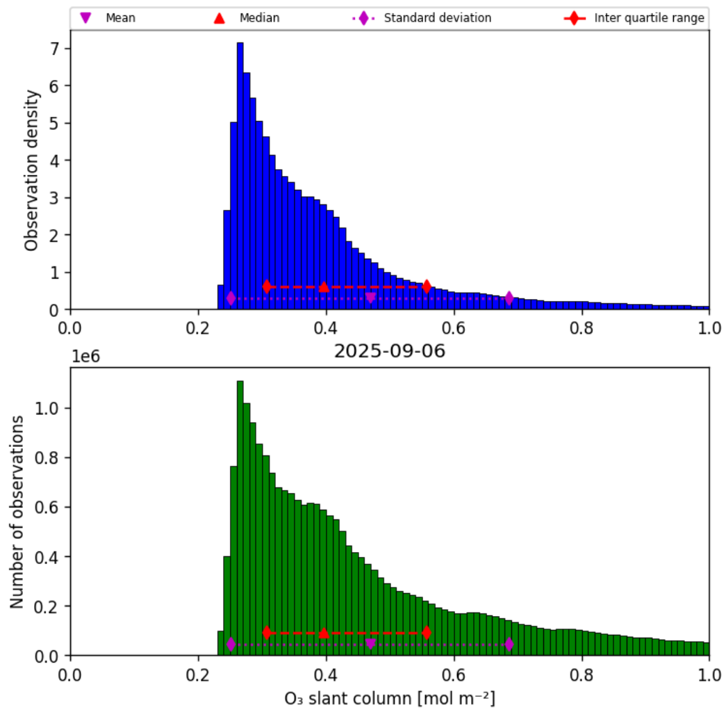
Figure 31: Histogram of “O 3 slant column” for 2025-09-06 to 2025-09-07
