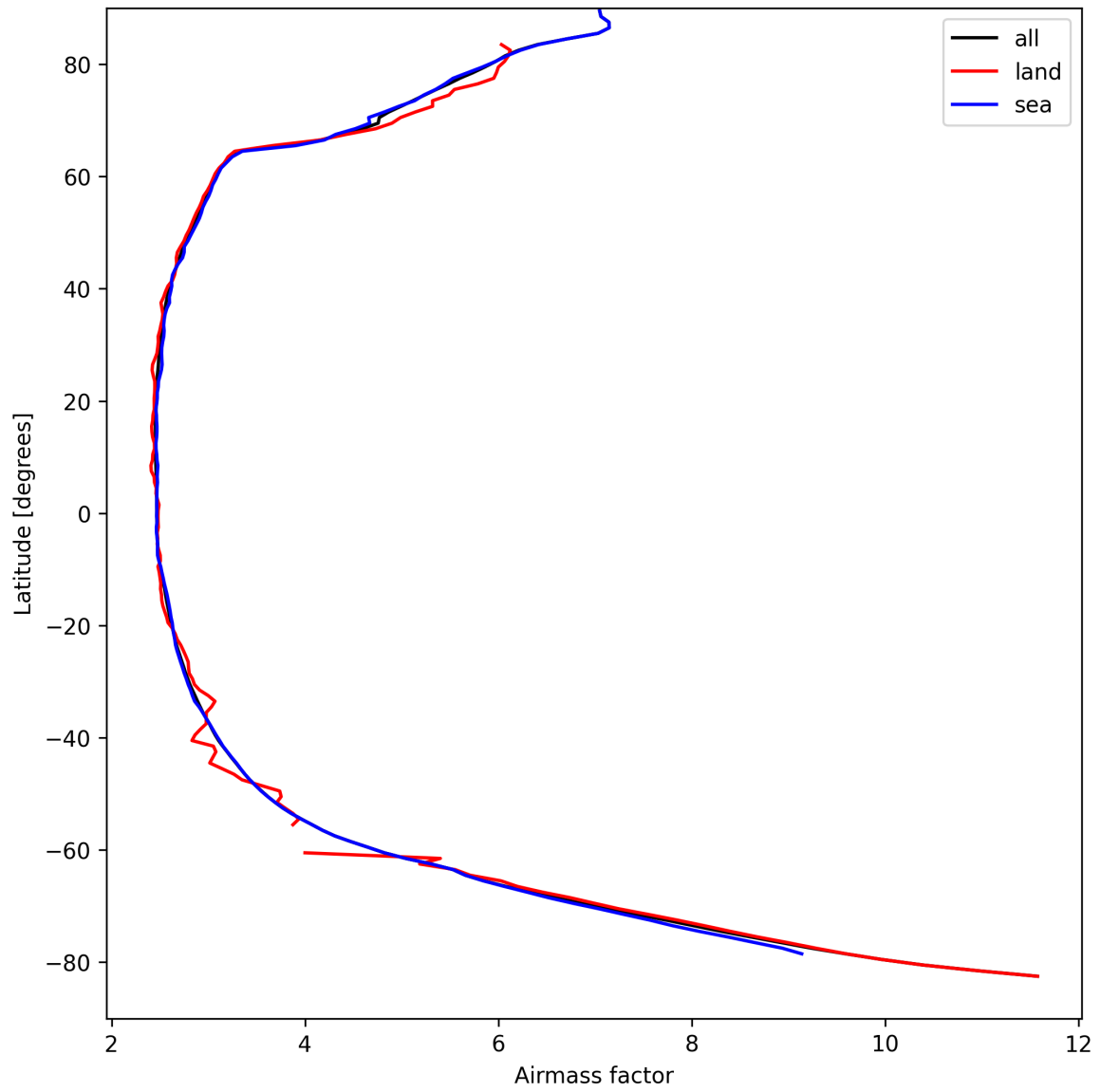
Figure 25: Zonal average of “Airmass factor” for 2025-09-06 to 2025-09-07.
