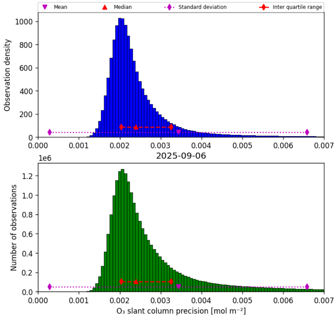
Figure 32: Histogram of “O 3 slant column precision” for 2025-09-06 to 2025-09-07
