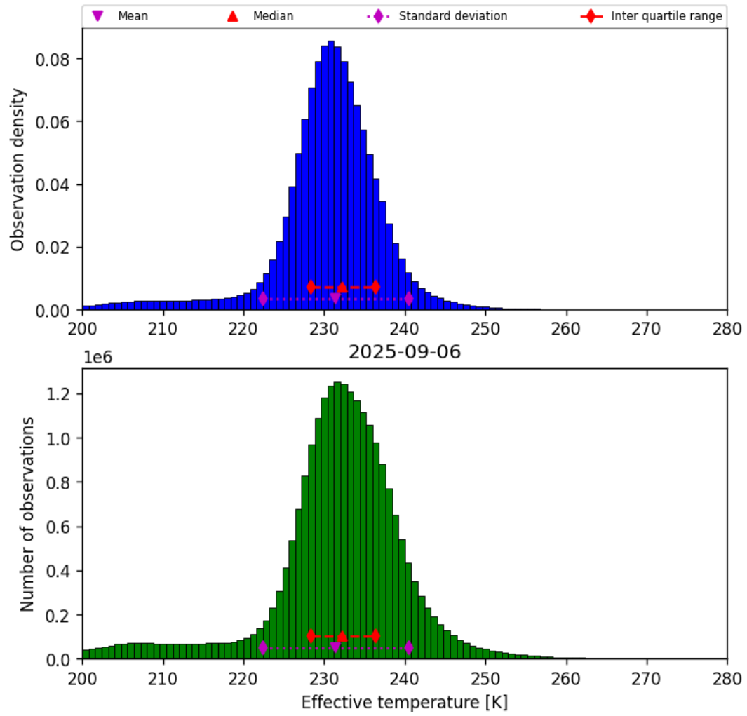
Figure 38: Histogram of “Effective temperature” for 2025-09-06 to 2025-09-07
