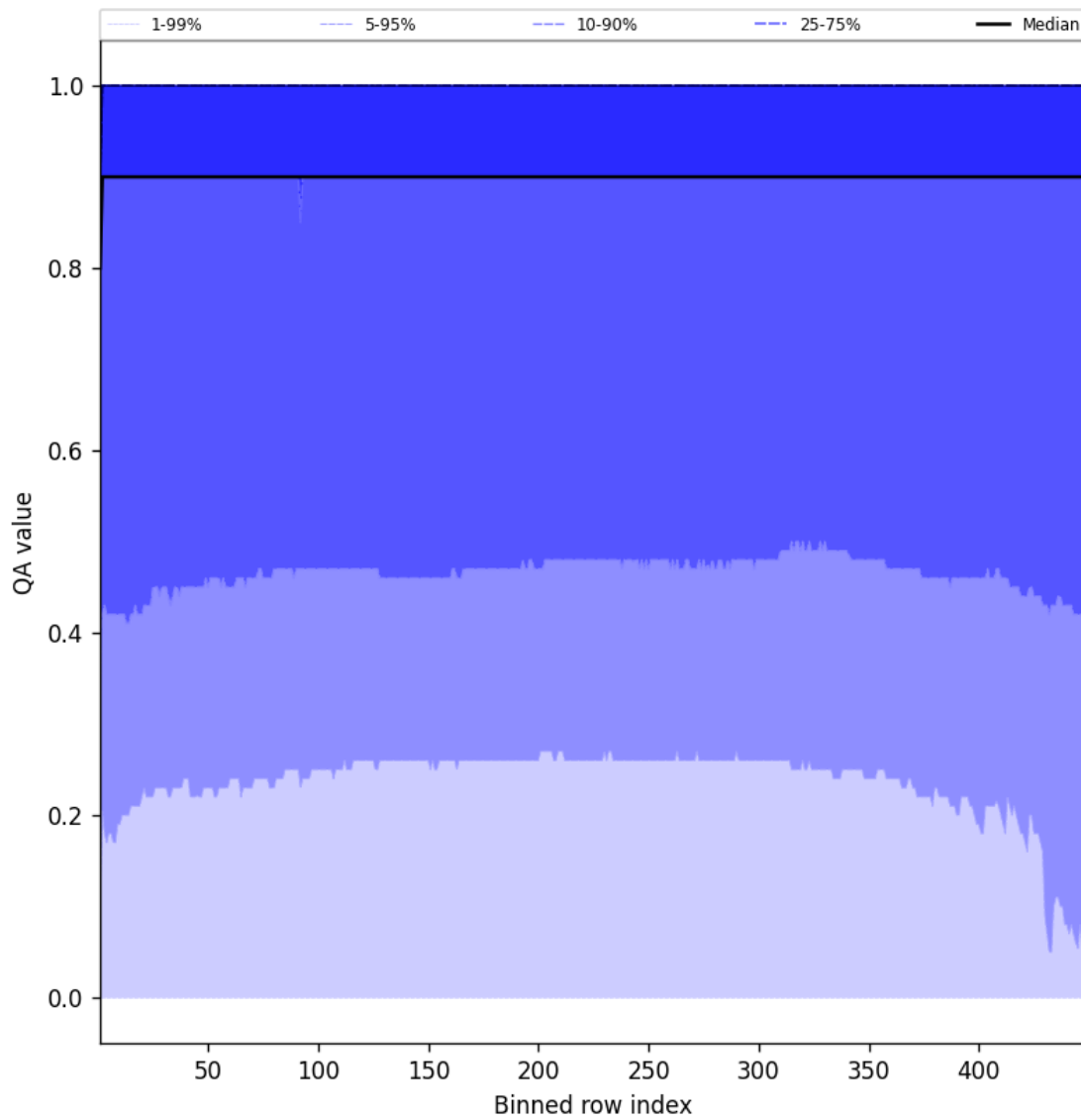
Figure 40: Along track statistics of “QA value” for 2025-09-06 to 2025-09-07
