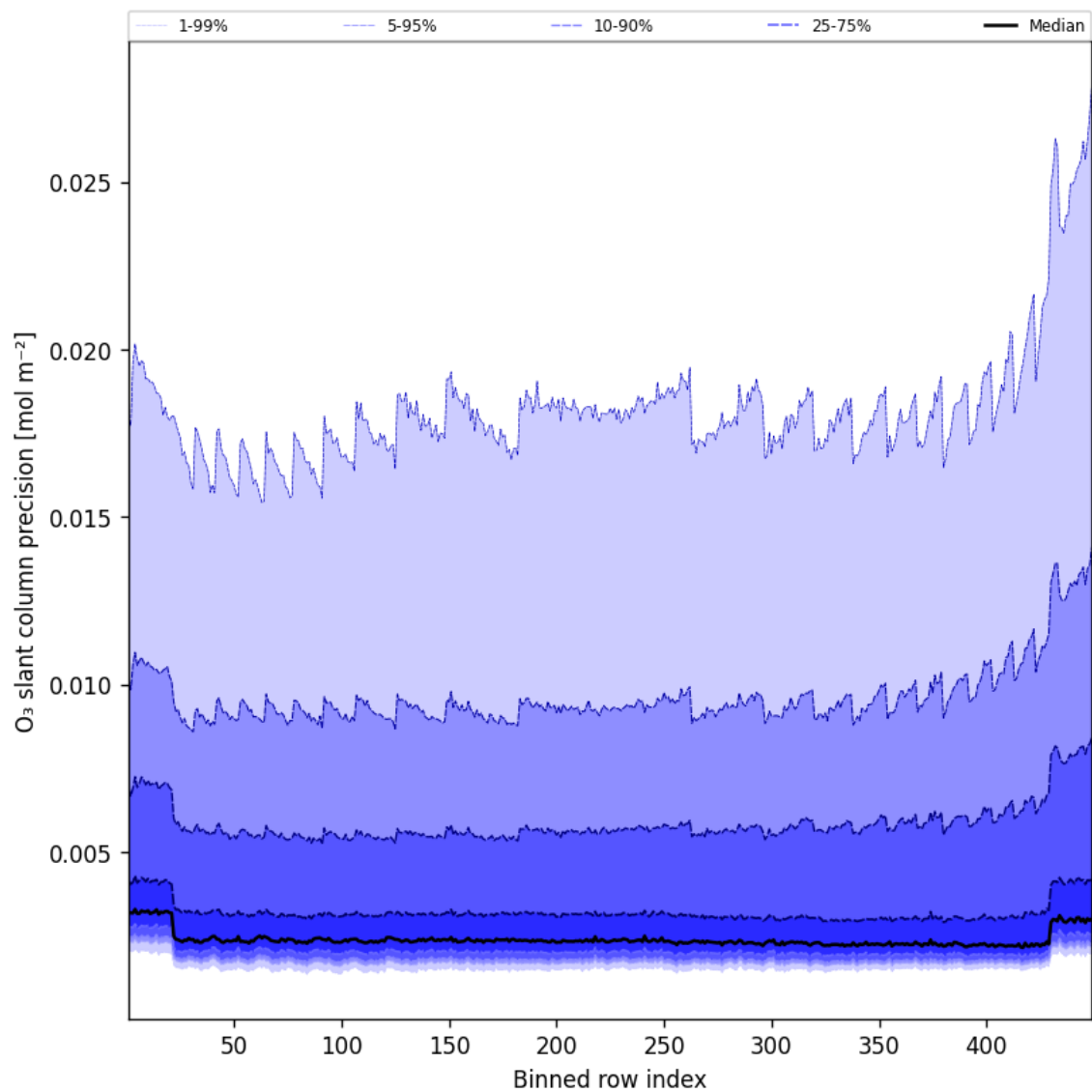
Figure 44: Along track statistics of “O 3 slant column precision” for 2025-09-06 to 2025-09-07
