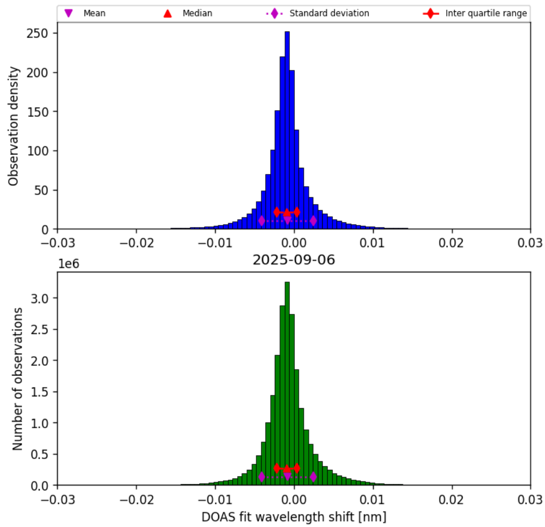
Figure 35: Histogram of “DOAS fit wavelength shift” for 2025-09-06 to 2025-09-07
