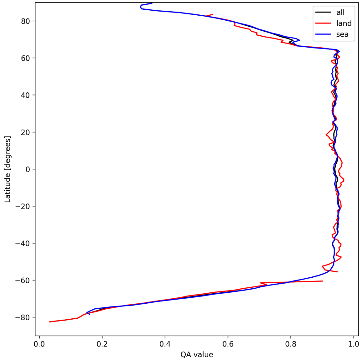
Figure 16: Zonal average of “QA value” for 2025-09-06 to 2025-09-07.
