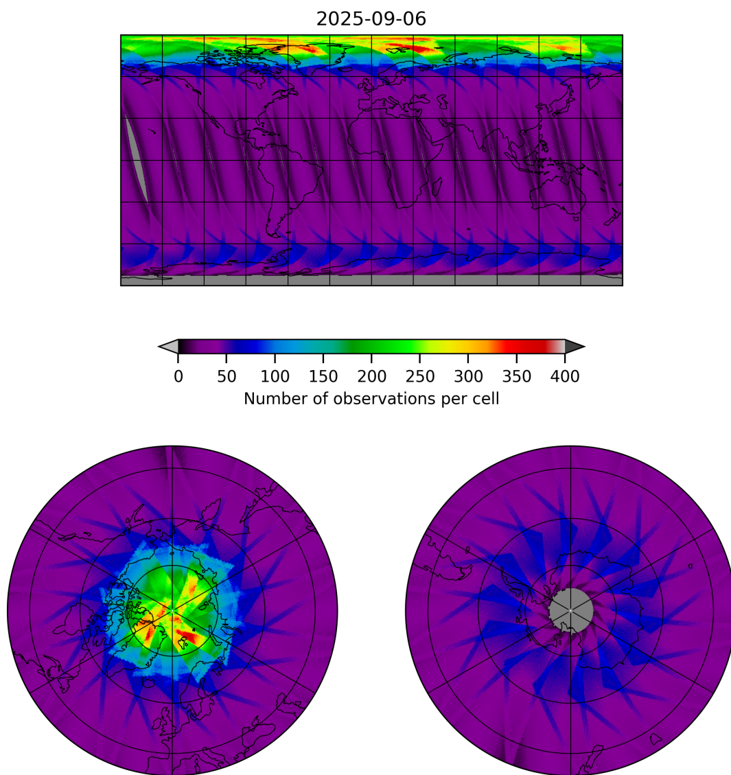
Figure 15: Map of the number of observations for 2025-09-06 to 2025-09-07
