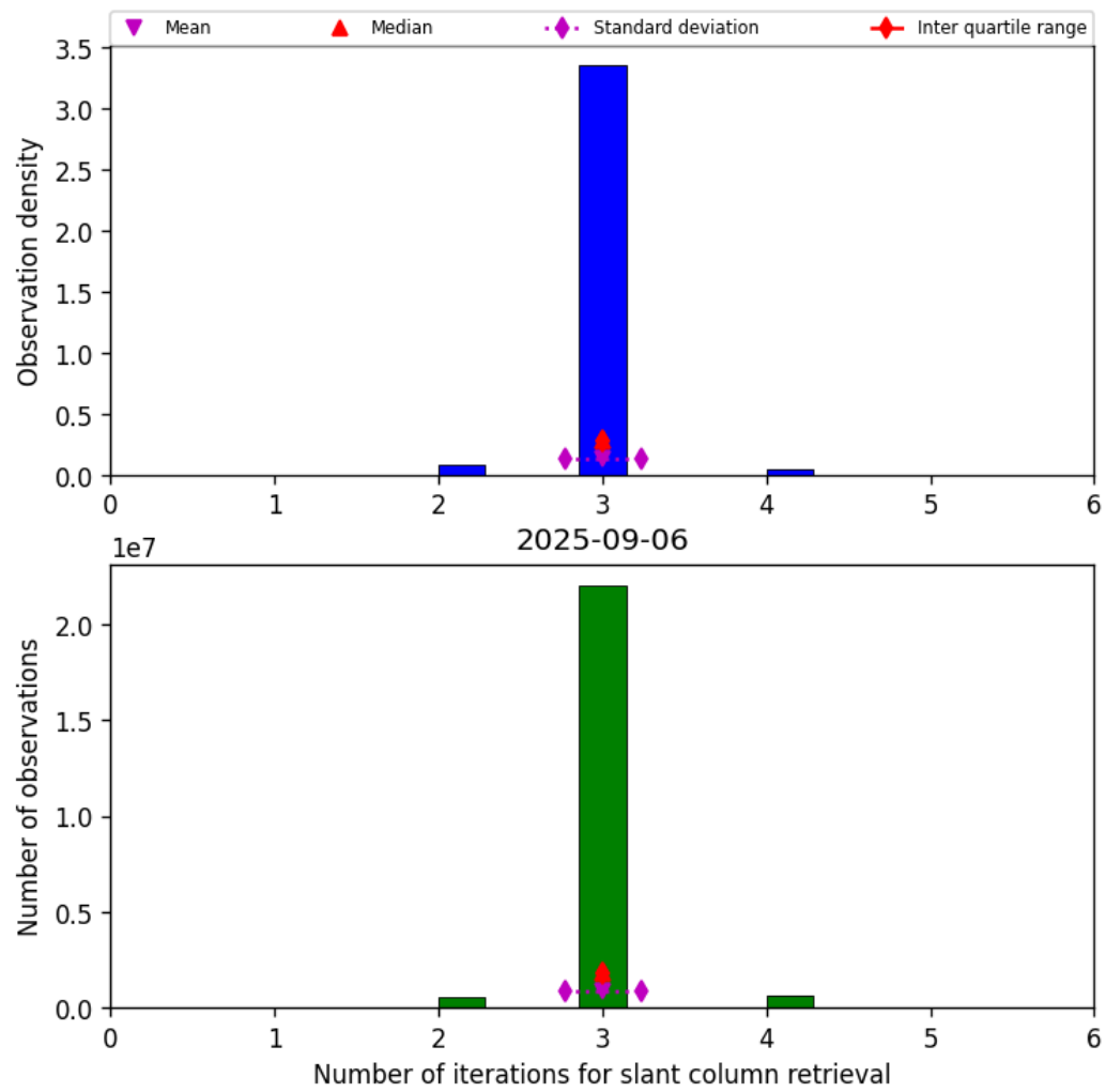
Figure 33: Histogram of “Number of iterations for slant column retrieval” for 2025-09-06 to 2025-09-07
