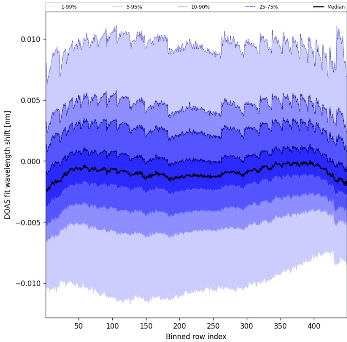
Figure 47: Along track statistics of “DOAS fit wavelength shift” for 2025-09-06 to 2025-09-07
