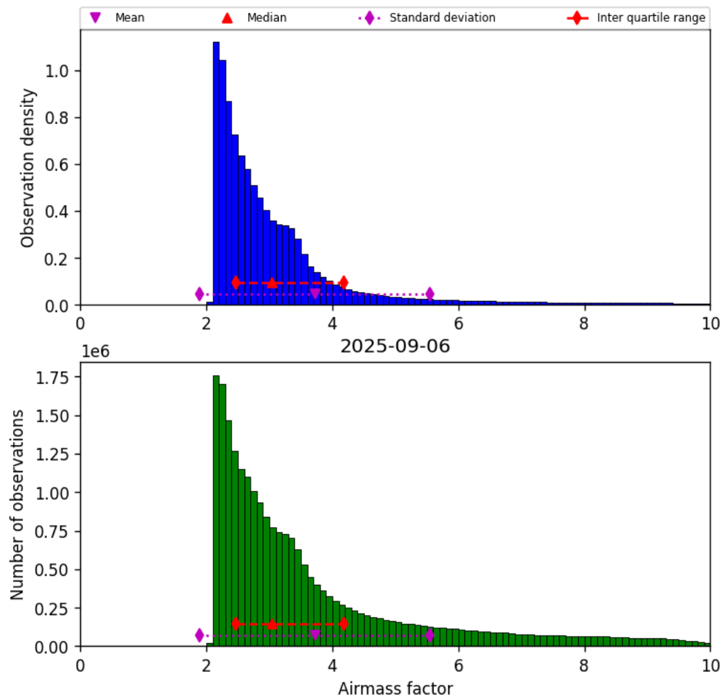
Figure 37: Histogram of “Airmass factor” for 2025-09-06 to 2025-09-07
