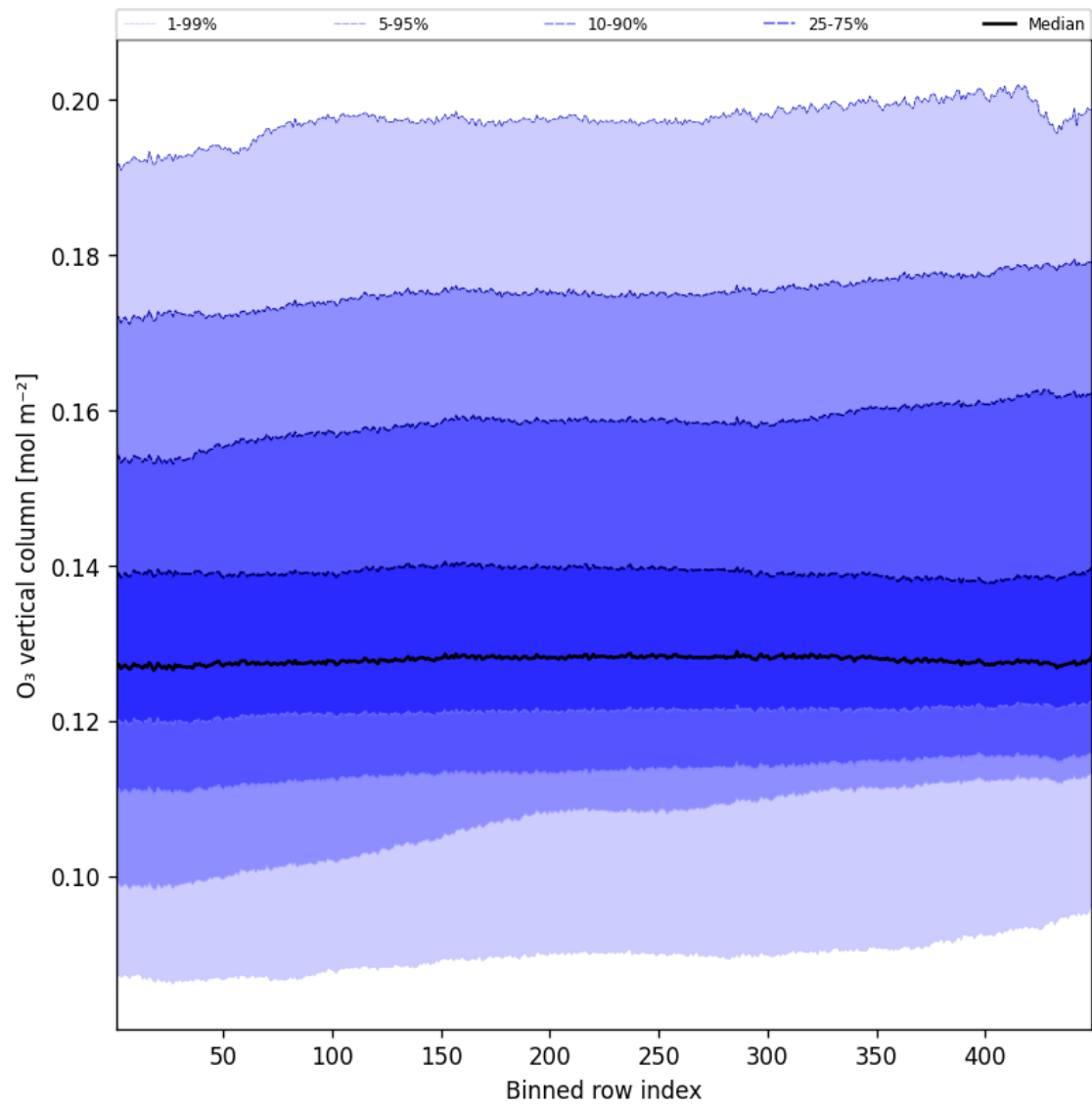
Figure 41: Along track statistics of “O 3 vertical column” for 2025-09-06 to 2025-09-07
