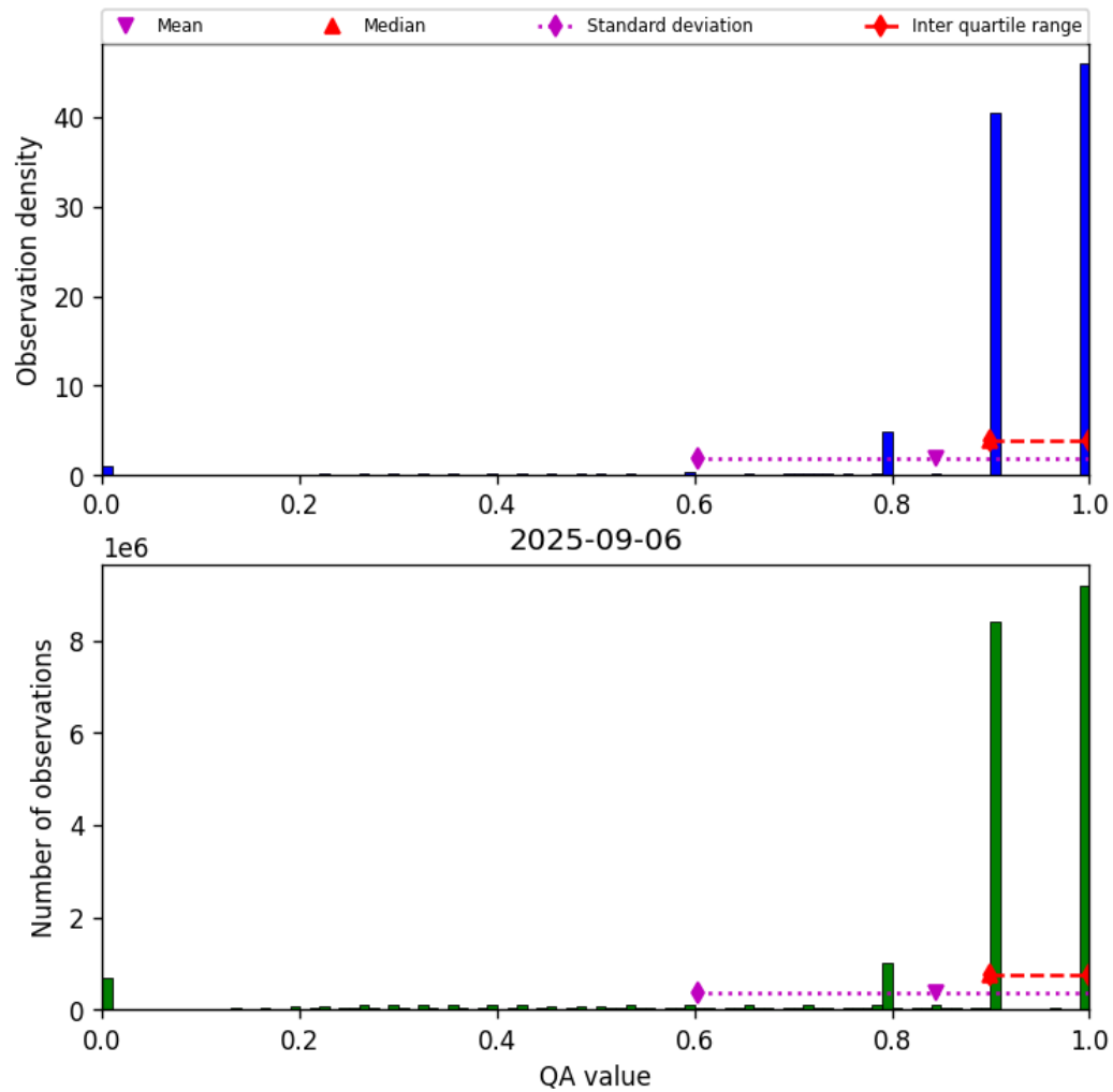
Figure 28: Histogram of “QA value” for 2025-09-06 to 2025-09-07
