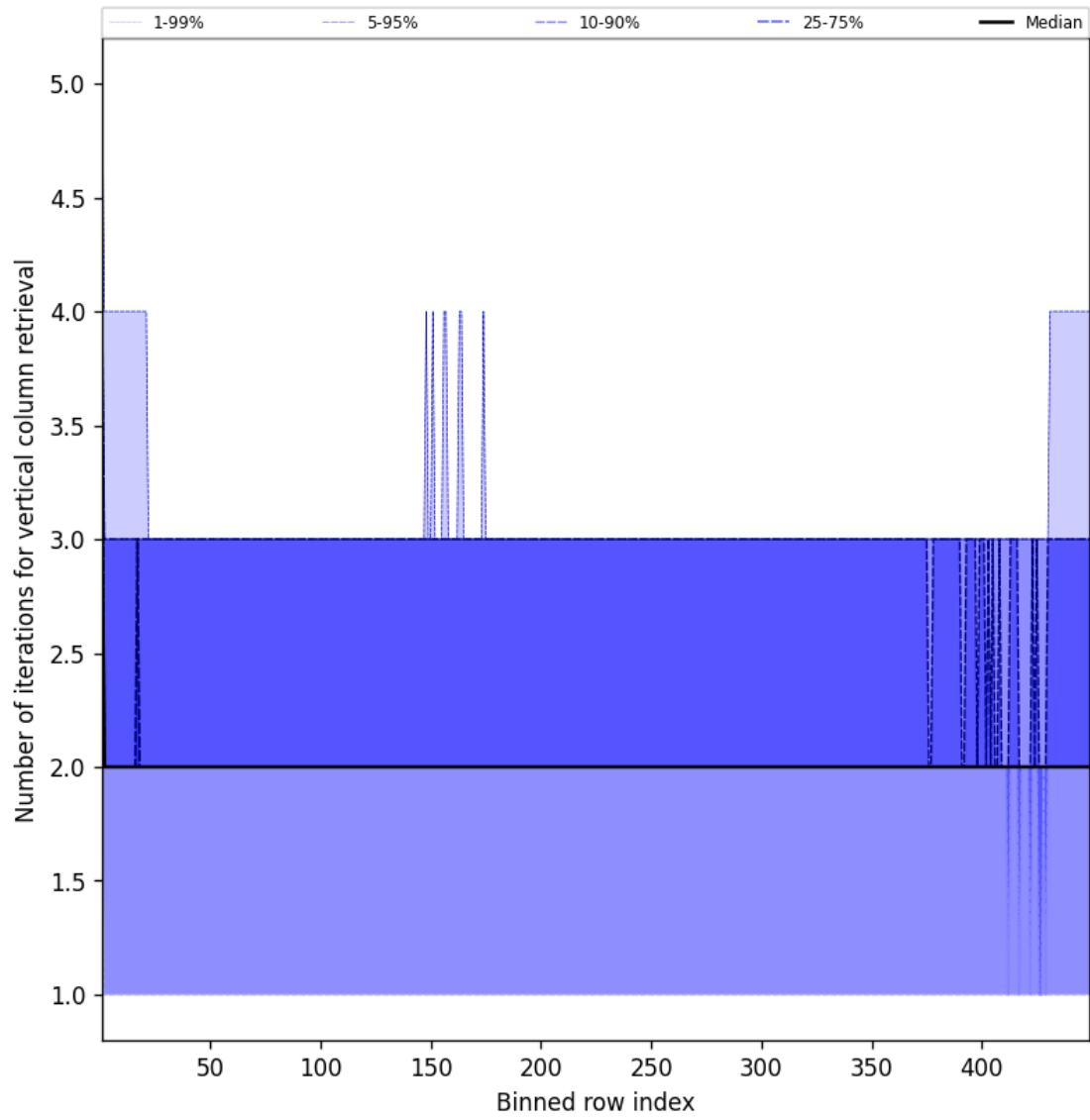
Figure 51: Along track statistics of “Number of iterations for vertical column retrieval” for 2025-09-06 to 2025-09-07
