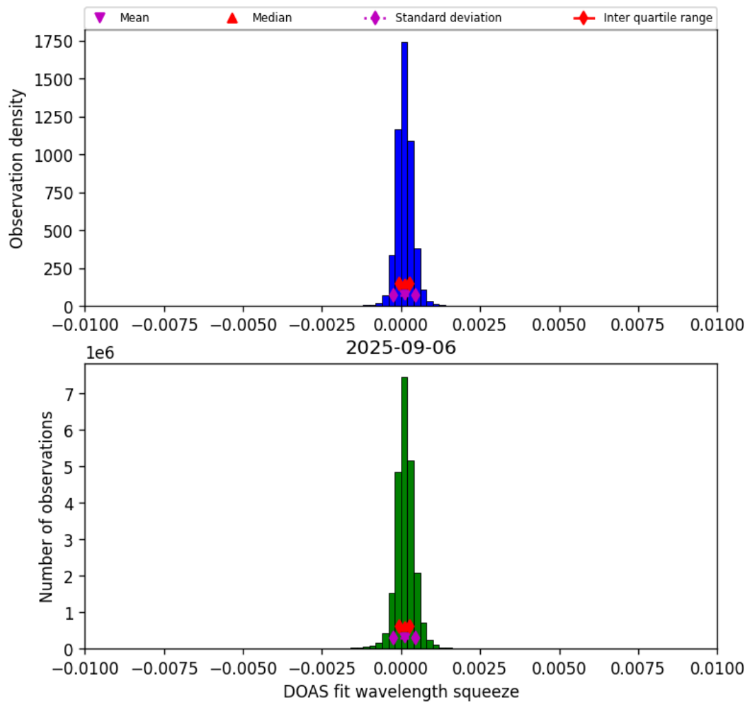
Figure 36: Histogram of “DOAS fit wavelength squeeze” for 2025-09-06 to 2025-09-07
