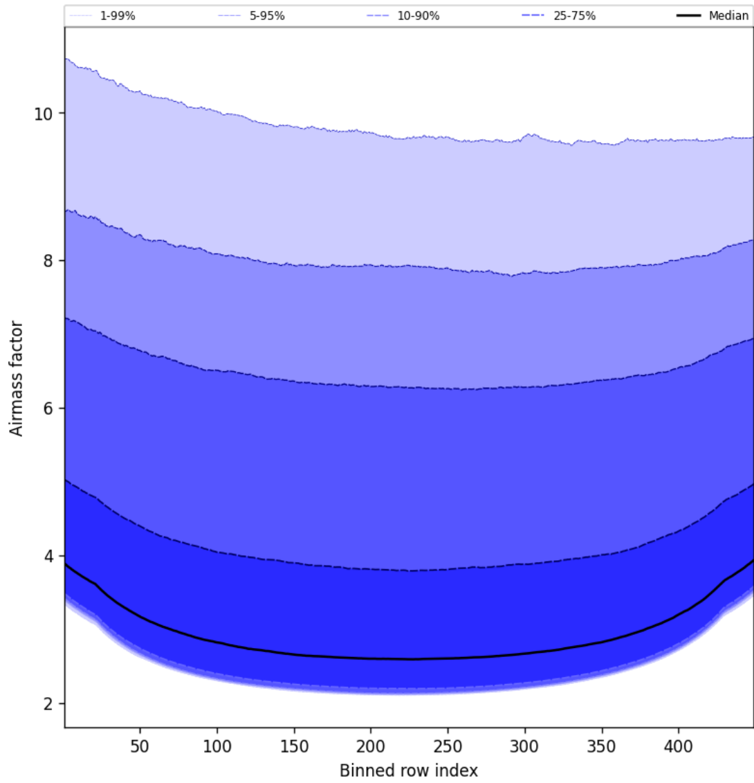
Figure 49: Along track statistics of “Airmass factor” for 2025-09-06 to 2025-09-07
