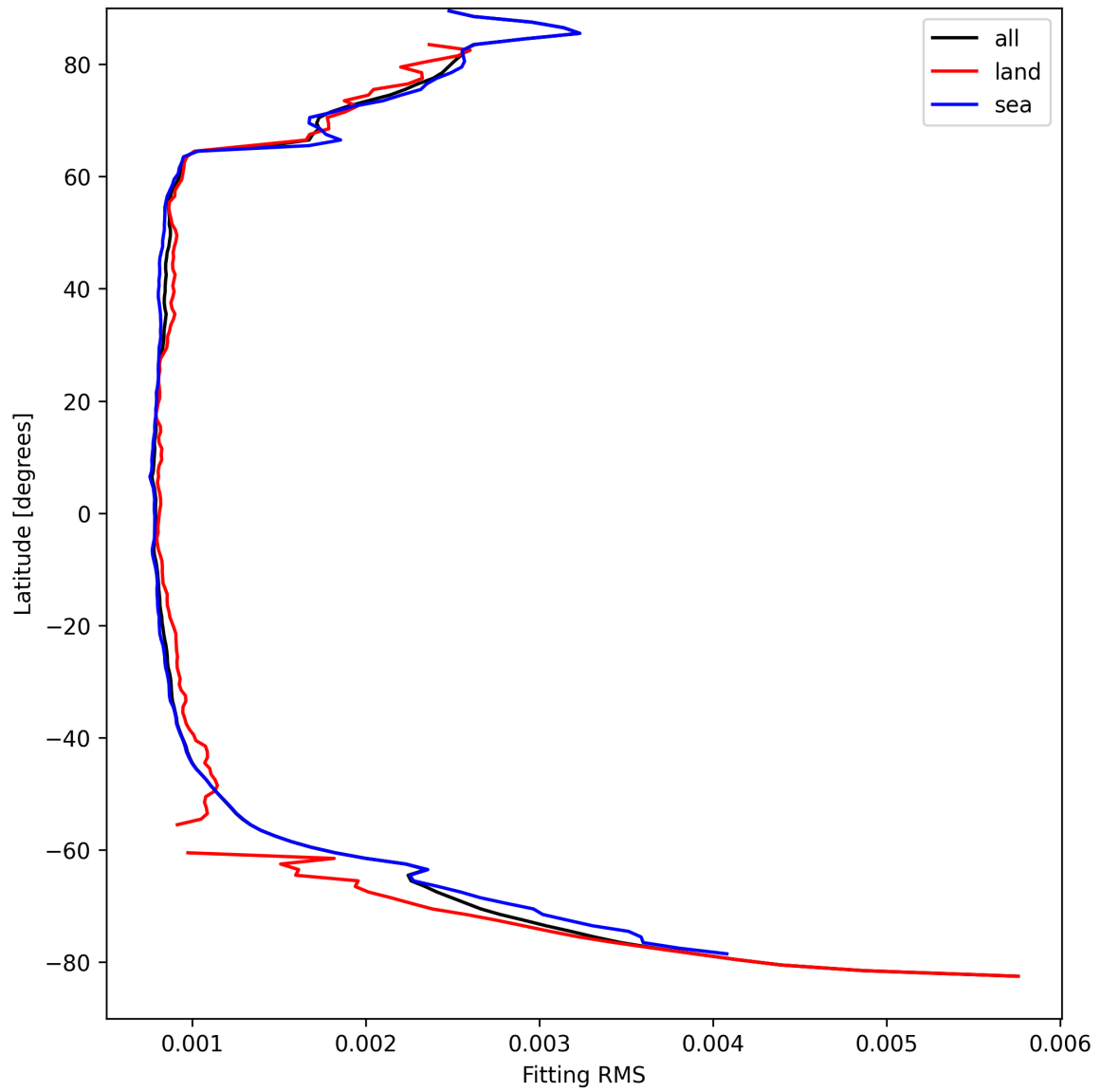
Figure 22: Zonal average of “Fitting RMS” for 2025-09-06 to 2025-09-07.
