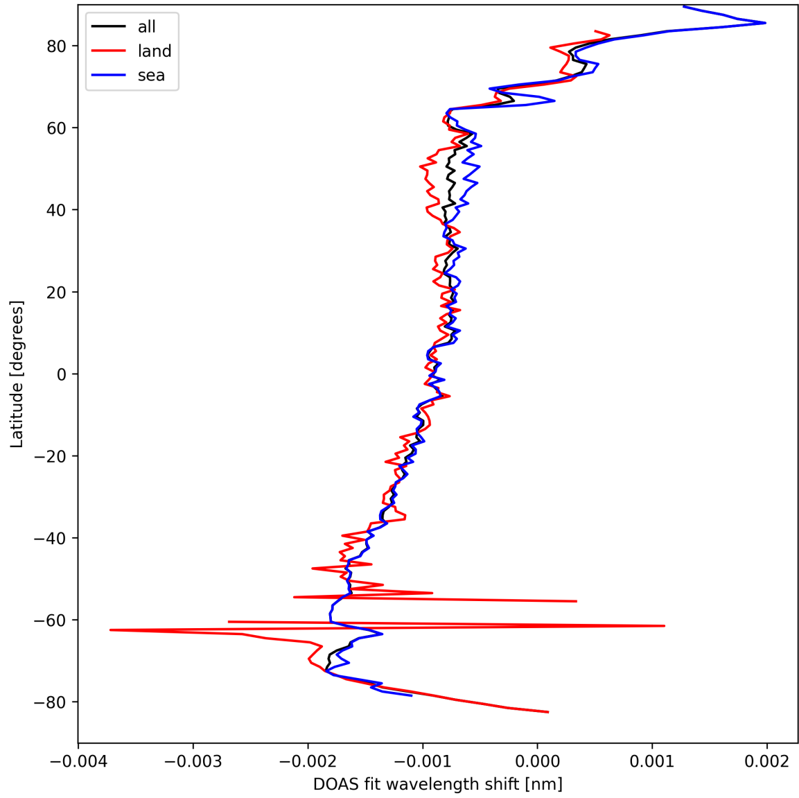
Figure 23: Zonal average of “DOAS fit wavelength shift” for 2025-09-06 to 2025-09-07.
