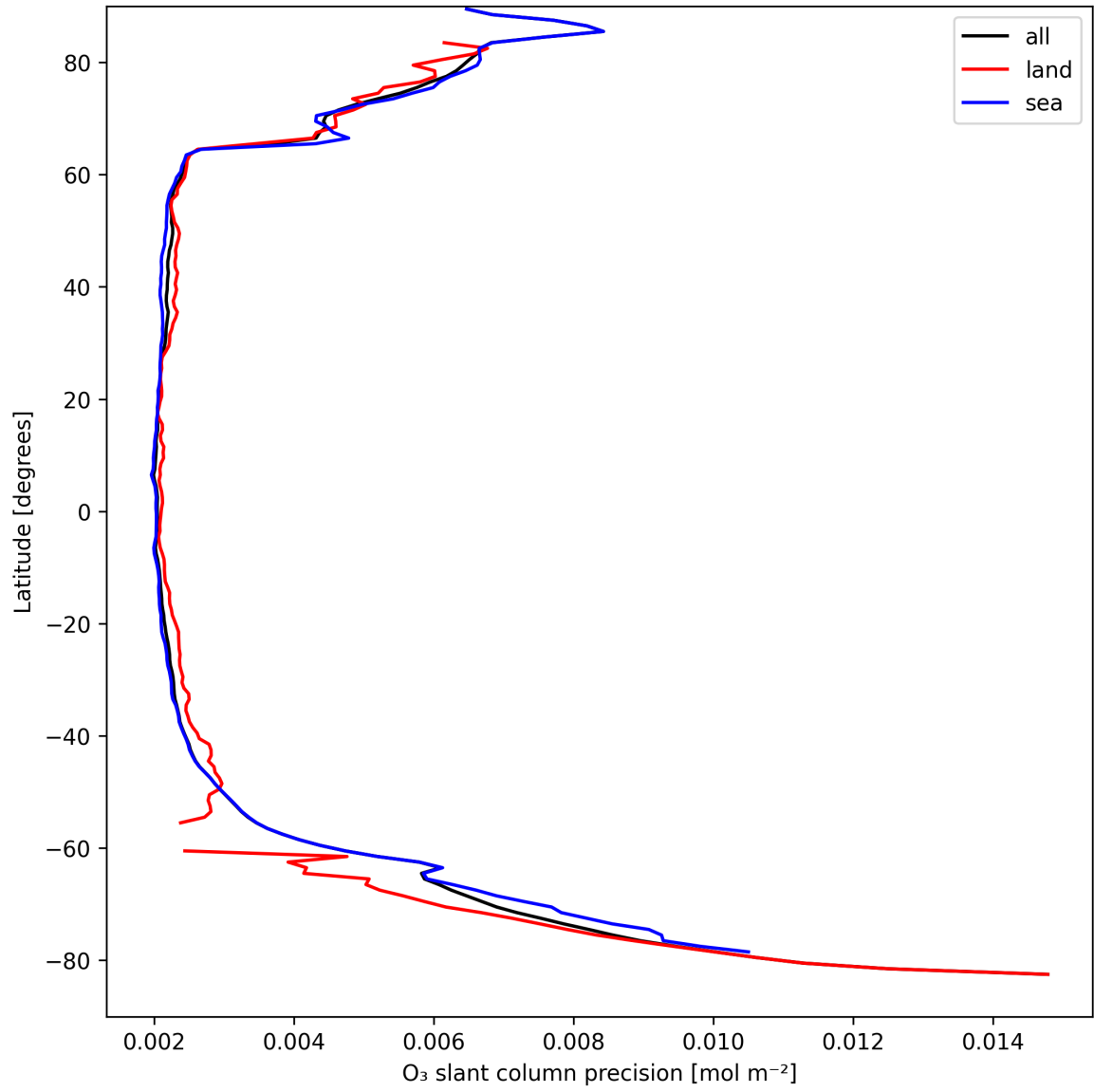
Figure 20: Zonal average of “O 3 slant column precision” for 2025-09-06 to 2025-09-07.
