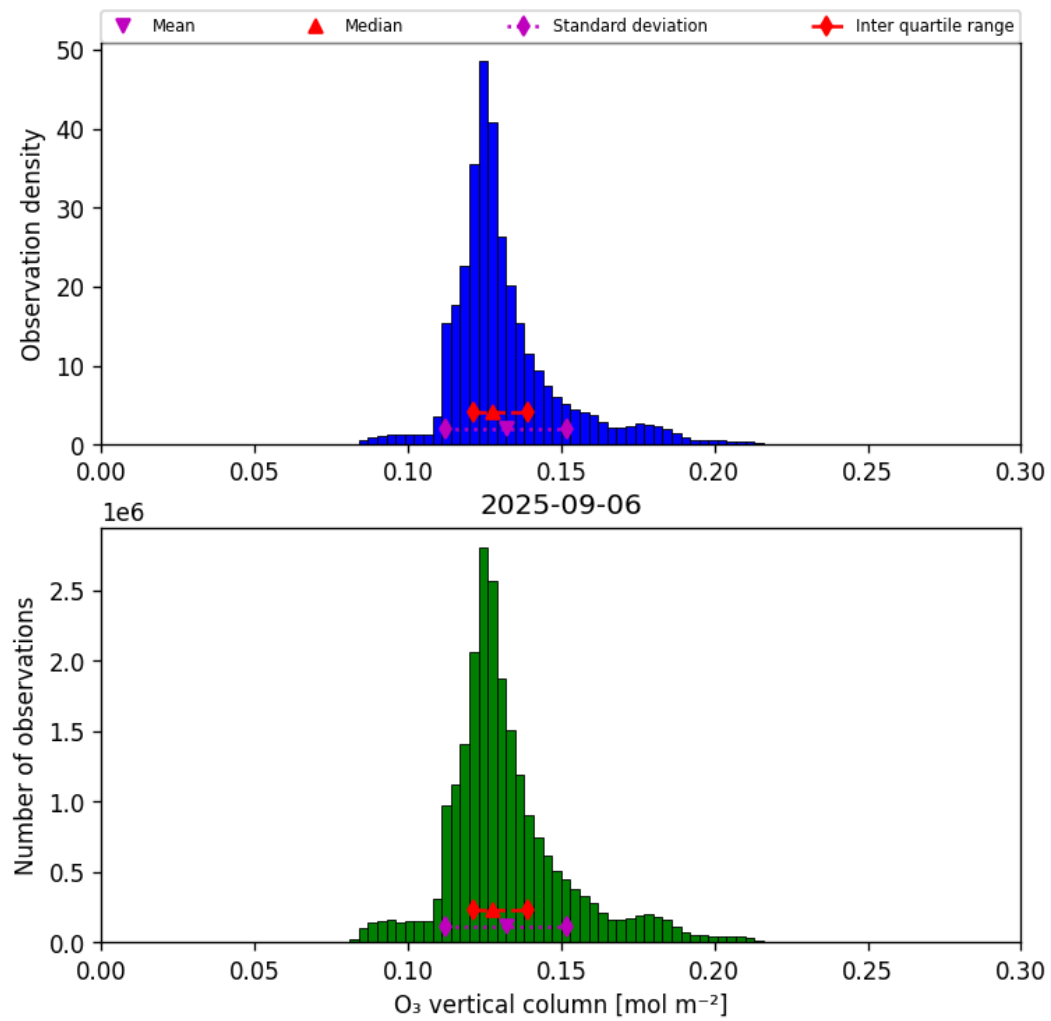
Figure 29: Histogram of “O 3 vertical column” for 2025-09-06 to 2025-09-07
