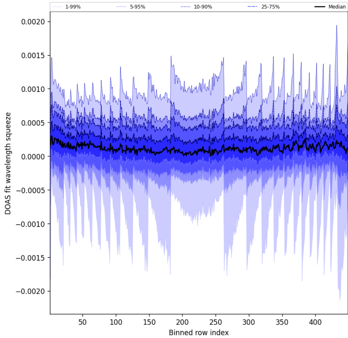
Figure 48: Along track statistics of “DOAS fit wavelength squeeze” for 2025-09-06 to 2025-09-07
