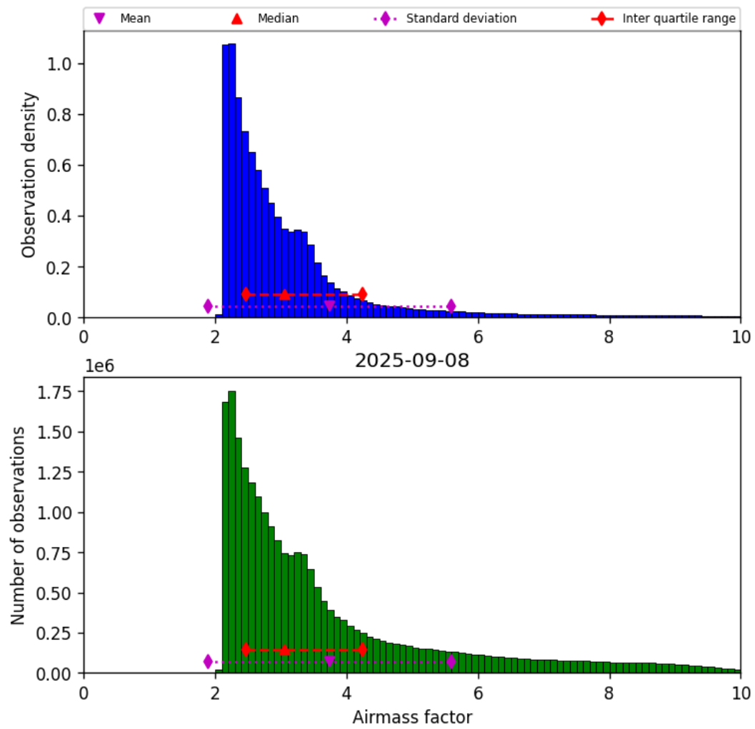
Figure 37: Histogram of “Airmass factor” for 2025-09-08 to 2025-09-08
