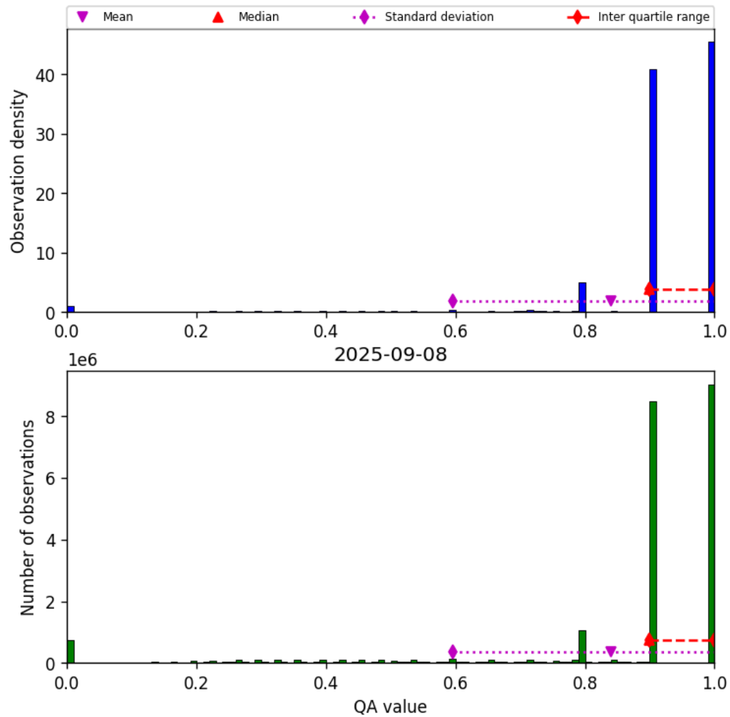
Figure 28: Histogram of “QA value” for 2025-09-08 to 2025-09-08
