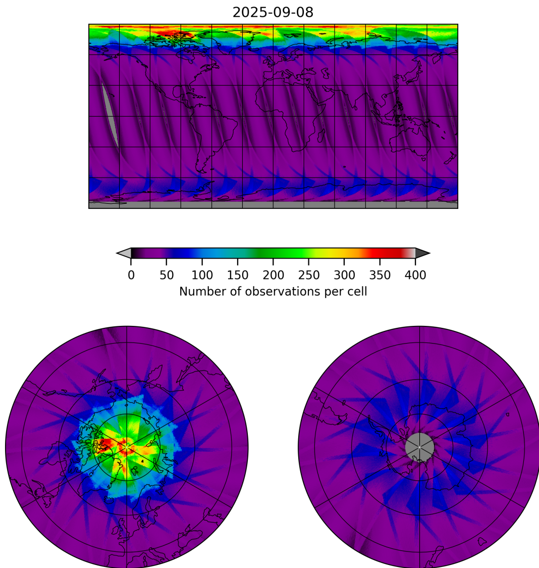
Figure 15: Map of the number of observations for 2025-09-08 to 2025-09-08
