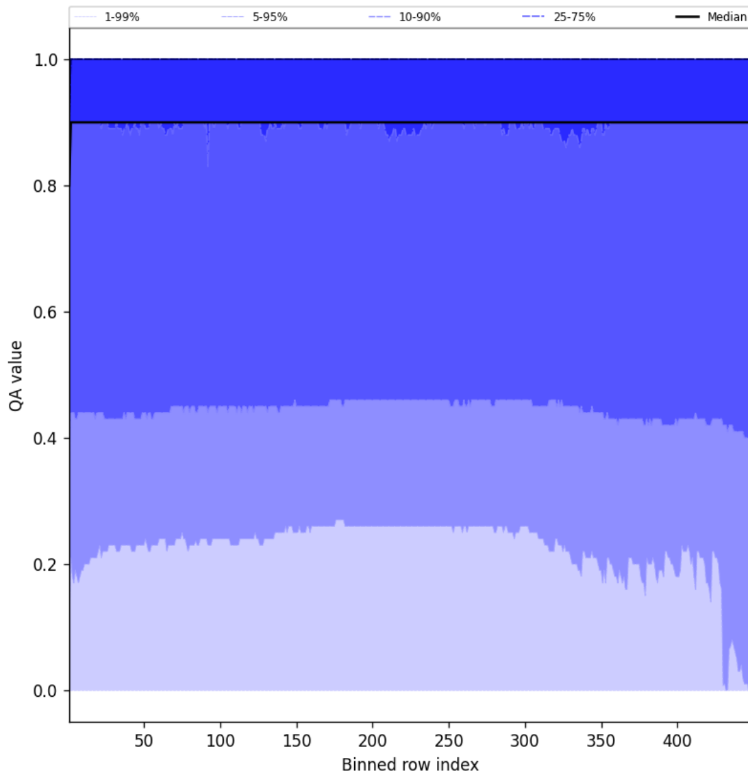
Figure 40: Along track statistics of “QA value” for 2025-09-08 to 2025-09-08
