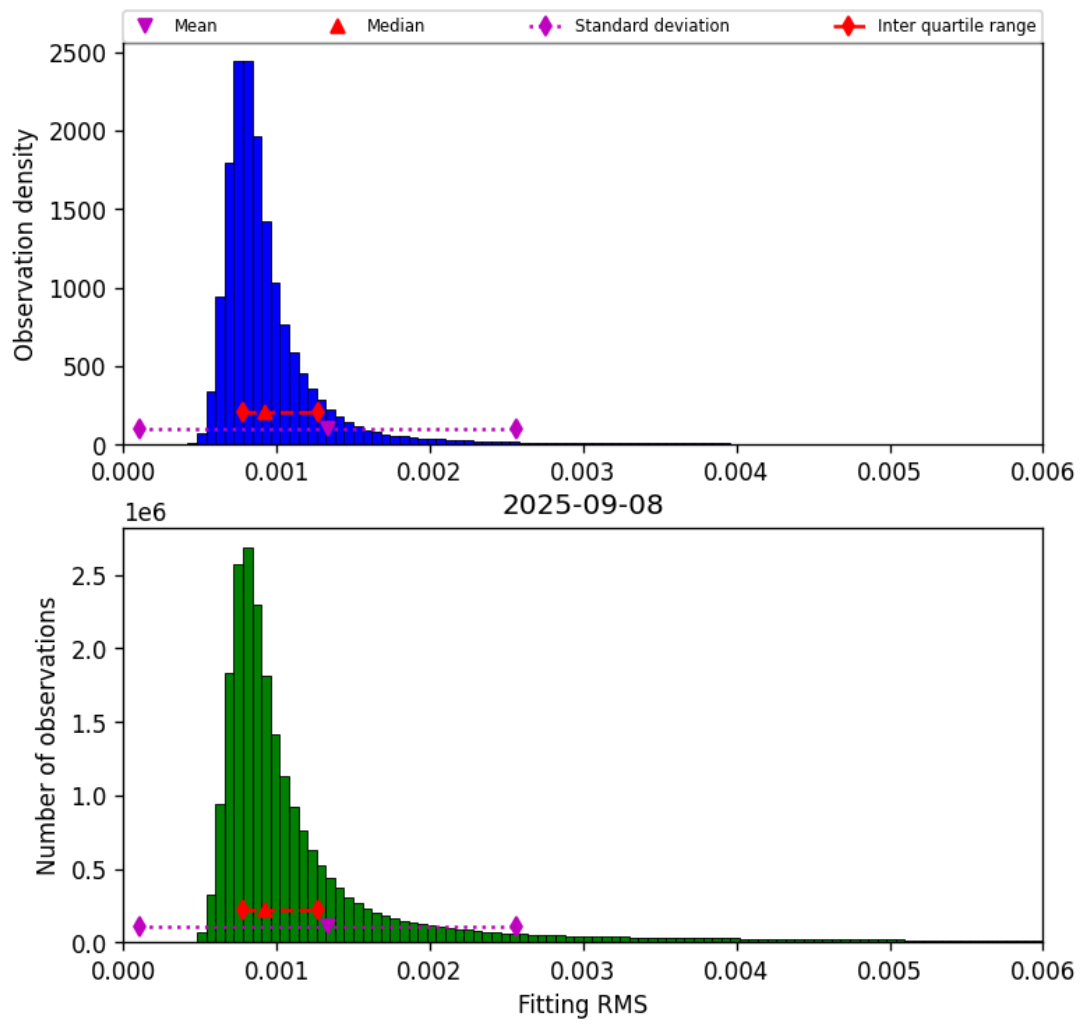
Figure 34: Histogram of “Fitting RMS” for 2025-09-08 to 2025-09-08
