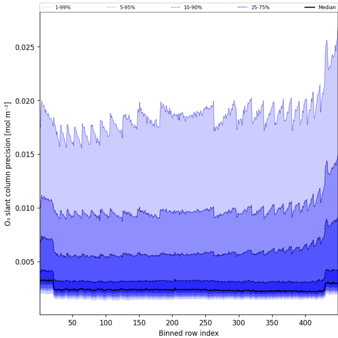
Figure 44: Along track statistics of “O 3 slant column precision” for 2025-09-08 to 2025-09-08
