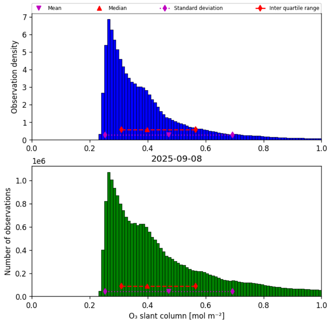
Figure 31: Histogram of “O 3 slant column” for 2025-09-08 to 2025-09-08
