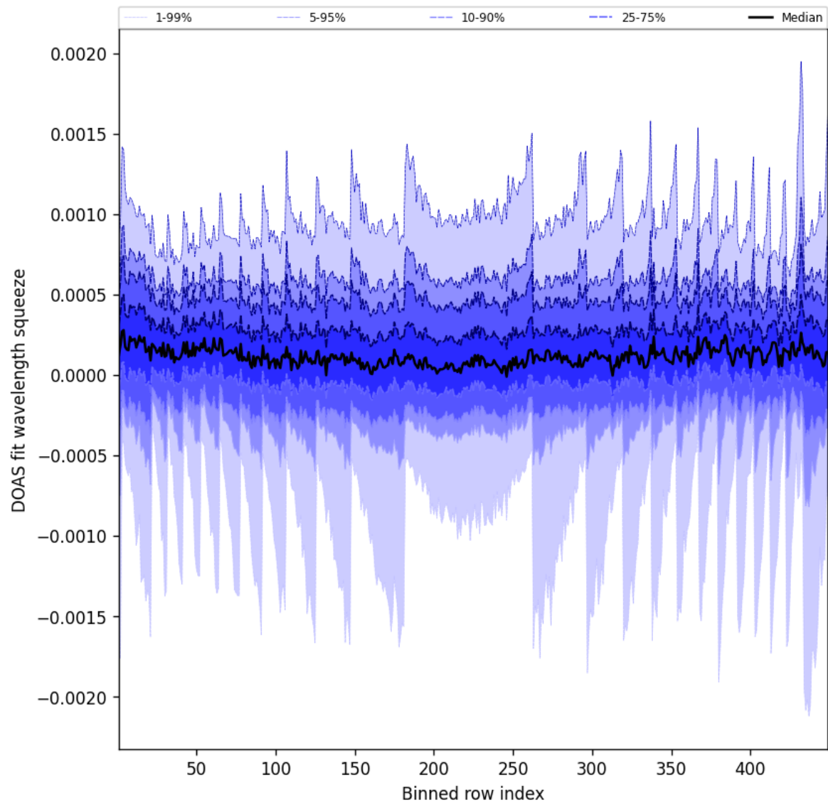
Figure 48: Along track statistics of “DOAS fit wavelength squeeze” for 2025-09-08 to 2025-09-08
