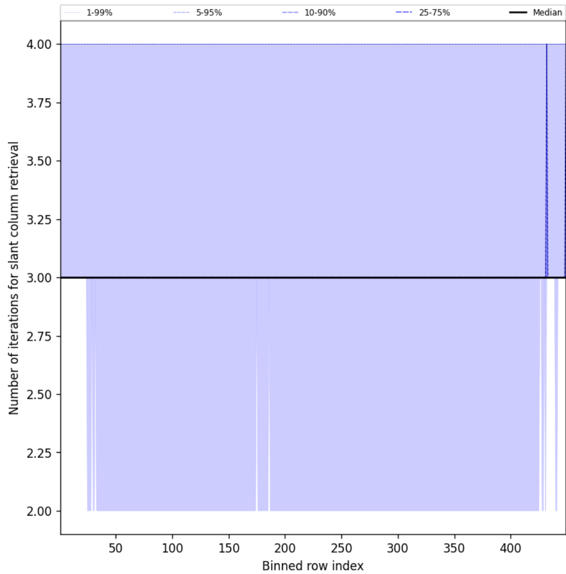
Figure 45: Along track statistics of “Number of iterations for slant column retrieval” for 2025-09-08 to 2025-09-08
