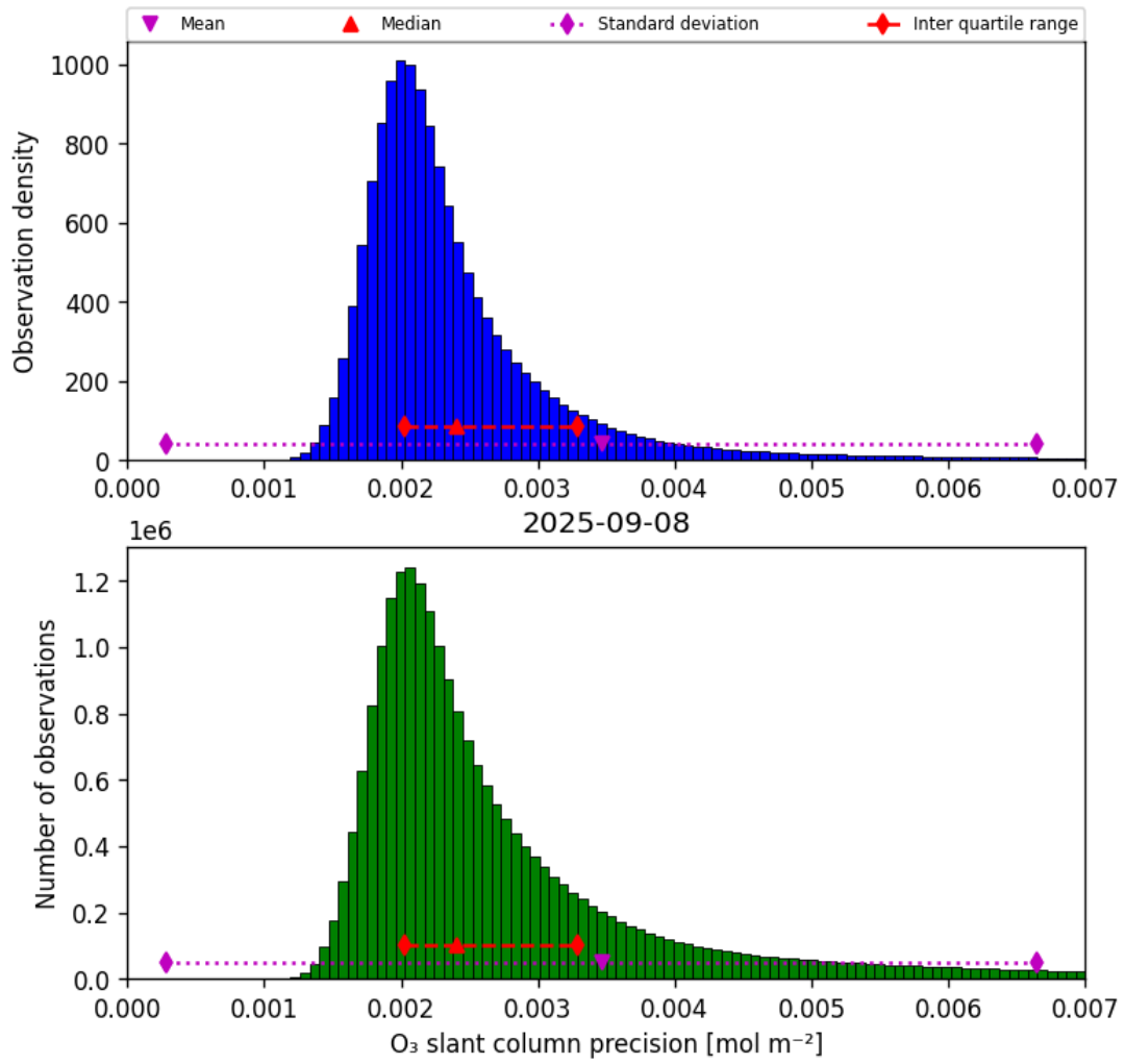
Figure 32: Histogram of “O 3 slant column precision” for 2025-09-08 to 2025-09-08
