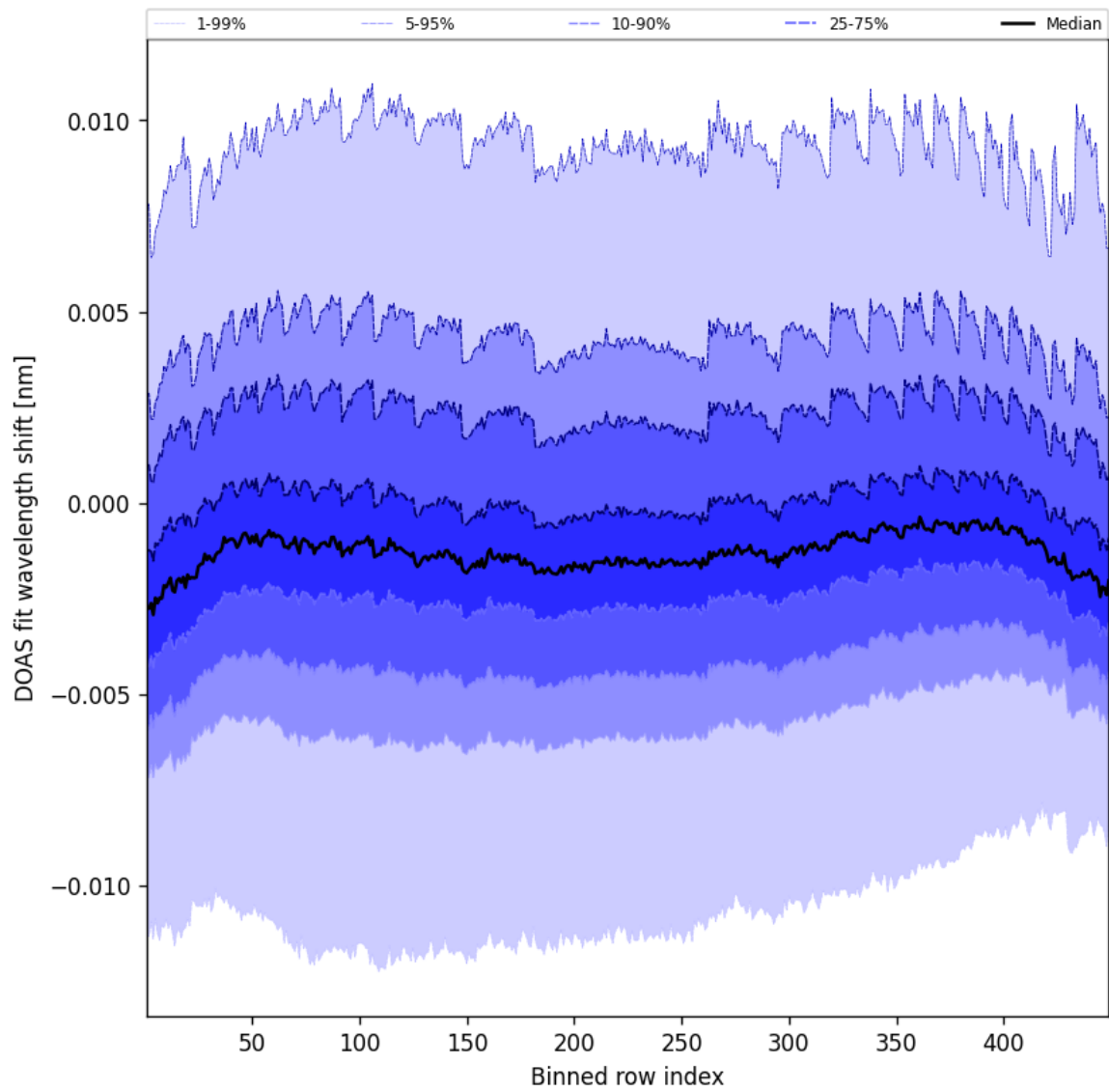
Figure 47: Along track statistics of “DOAS fit wavelength shift” for 2025-09-08 to 2025-09-08
