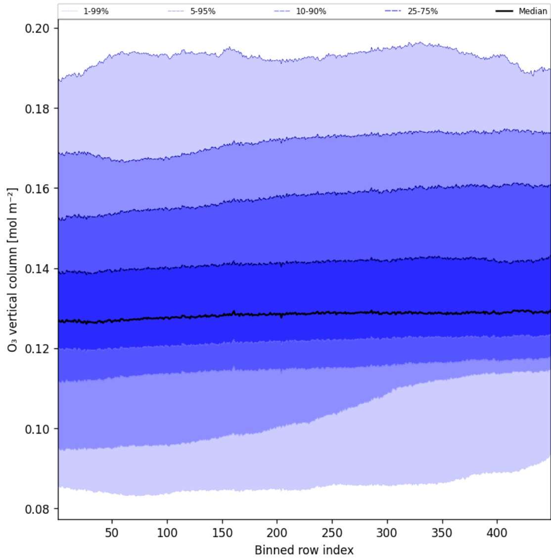
Figure 41: Along track statistics of “O 3 vertical column” for 2025-09-08 to 2025-09-08
