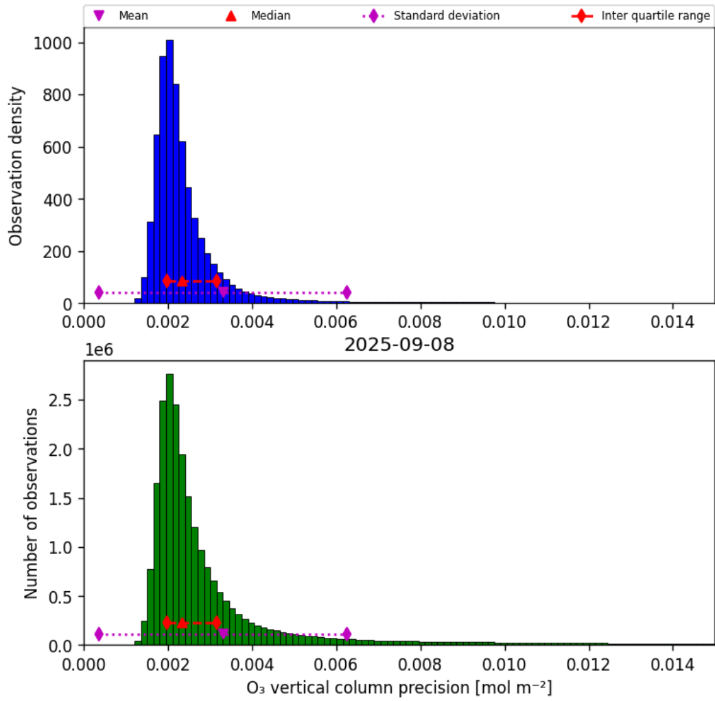
Figure 30: Histogram of “O 3 vertical column precision” for 2025-09-08 to 2025-09-08
