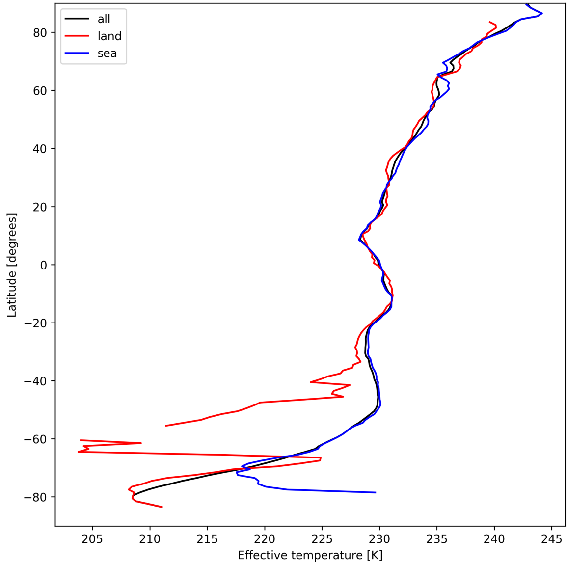
Figure 26: Zonal average of “Effective temperature” for 2025-09-08 to 2025-09-08.
