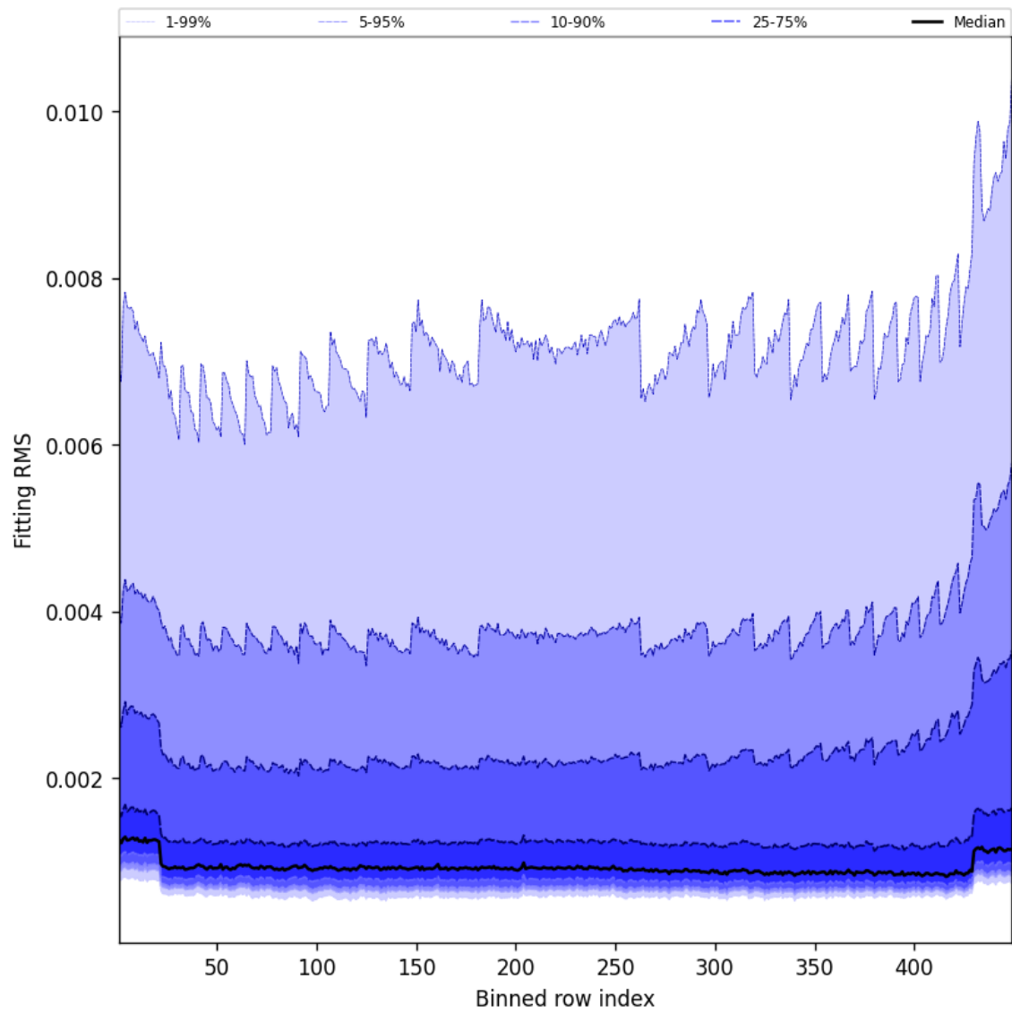
Figure 46: Along track statistics of “Fitting RMS” for 2025-09-08 to 2025-09-08
