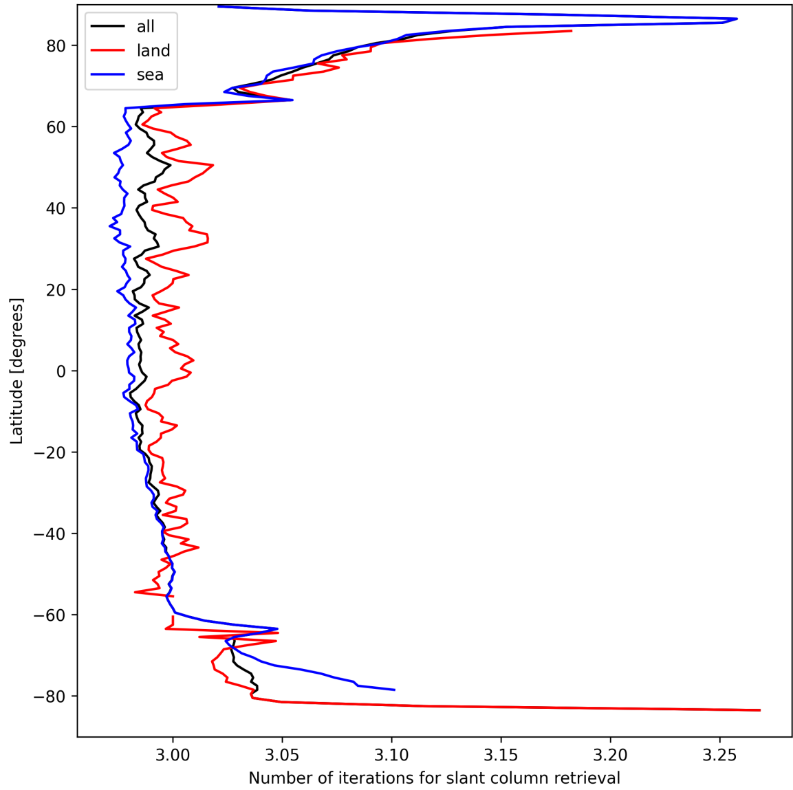
Figure 21: Zonal average of “Number of iterations for slant column retrieval” for 2025-09-08 to 2025-09-08.
