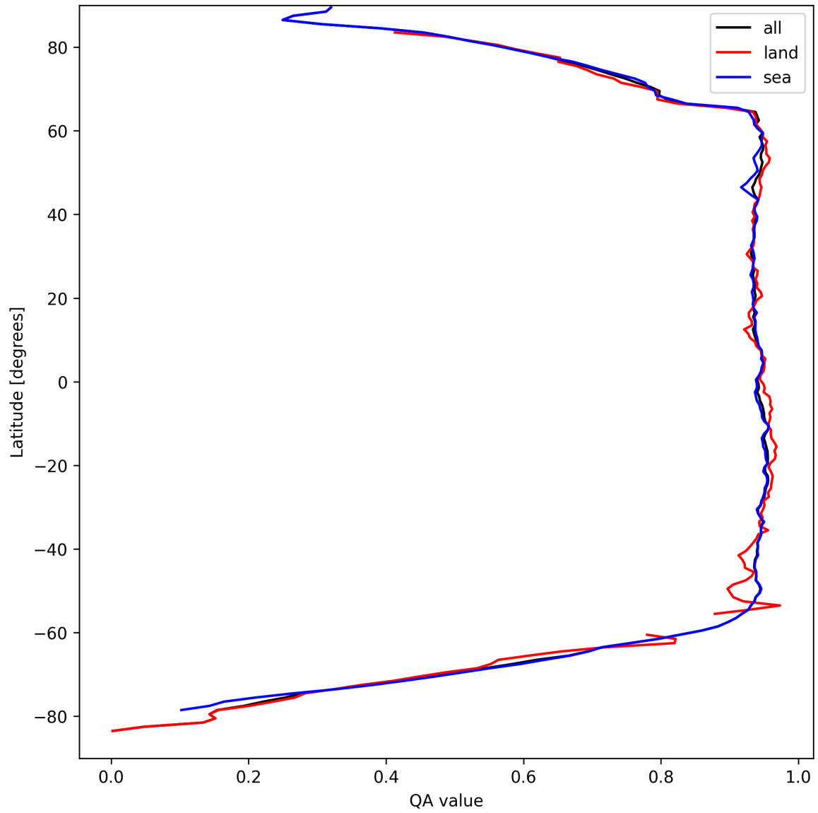
Figure 16: Zonal average of “QA value” for 2025-09-08 to 2025-09-08.
