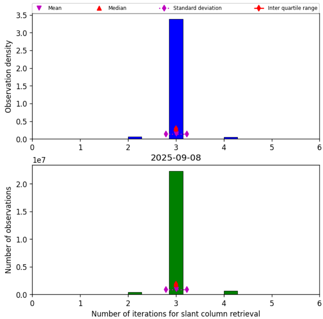
Figure 33: Histogram of “Number of iterations for slant column retrieval” for 2025-09-08 to 2025-09-08
