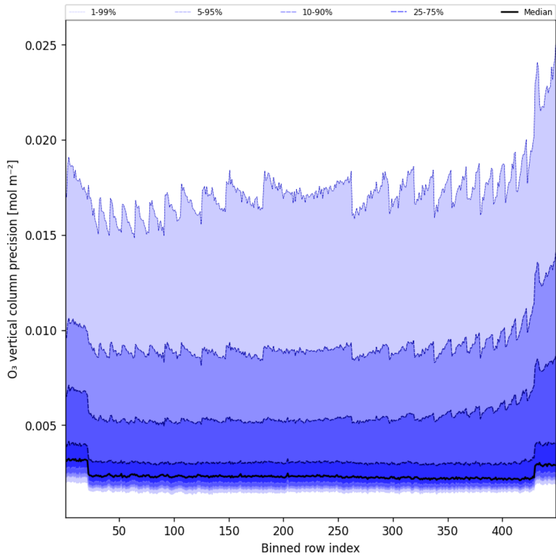
Figure 42: Along track statistics of “O 3 vertical column precision” for 2025-09-08 to 2025-09-08
