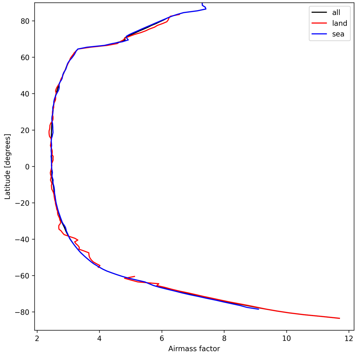
Figure 25: Zonal average of “Airmass factor” for 2025-09-08 to 2025-09-08.
