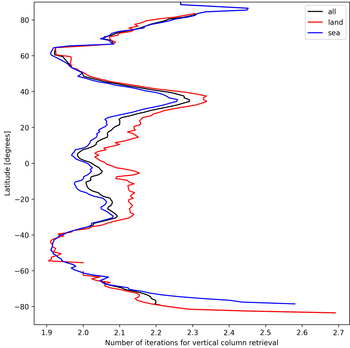
Figure 27: Zonal average of “Number of iterations for vertical column retrieval” for 2025-09-08 to 2025-09-08.
