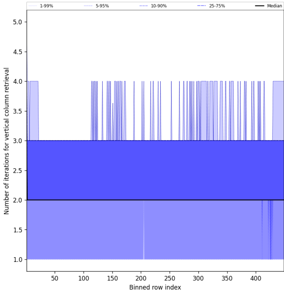
Figure 51: Along track statistics of “Number of iterations for vertical column retrieval” for 2025-09-08 to 2025-09-08
