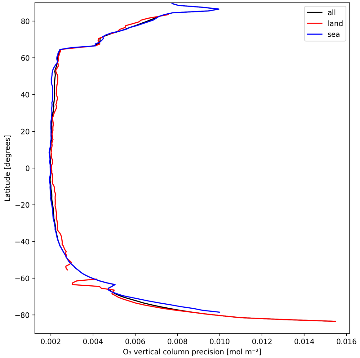
Figure 18: Zonal average of “O 3 vertical column precision” for 2025-09-08 to 2025-09-08.
