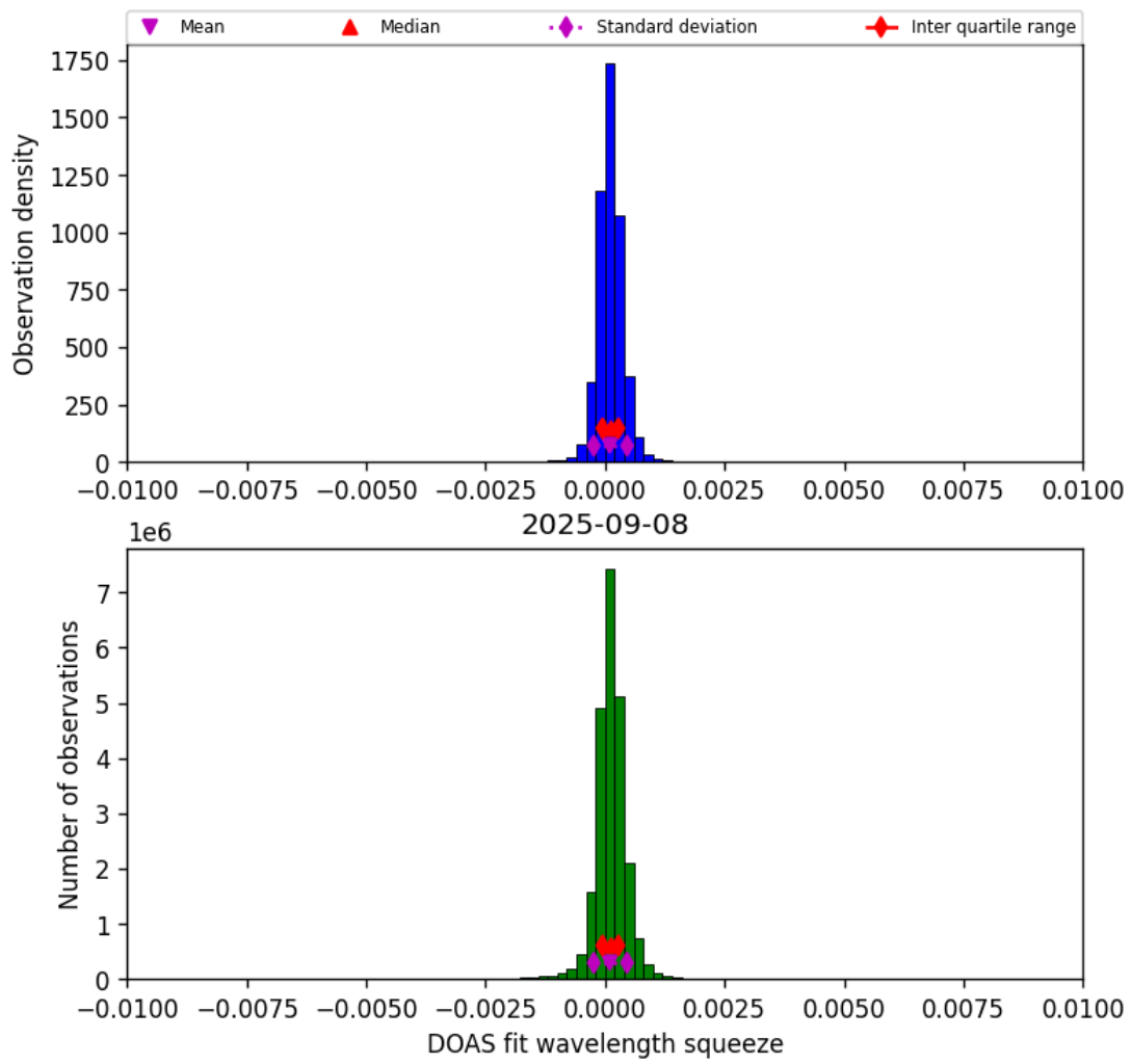
Figure 36: Histogram of “DOAS fit wavelength squeeze” for 2025-09-08 to 2025-09-08
