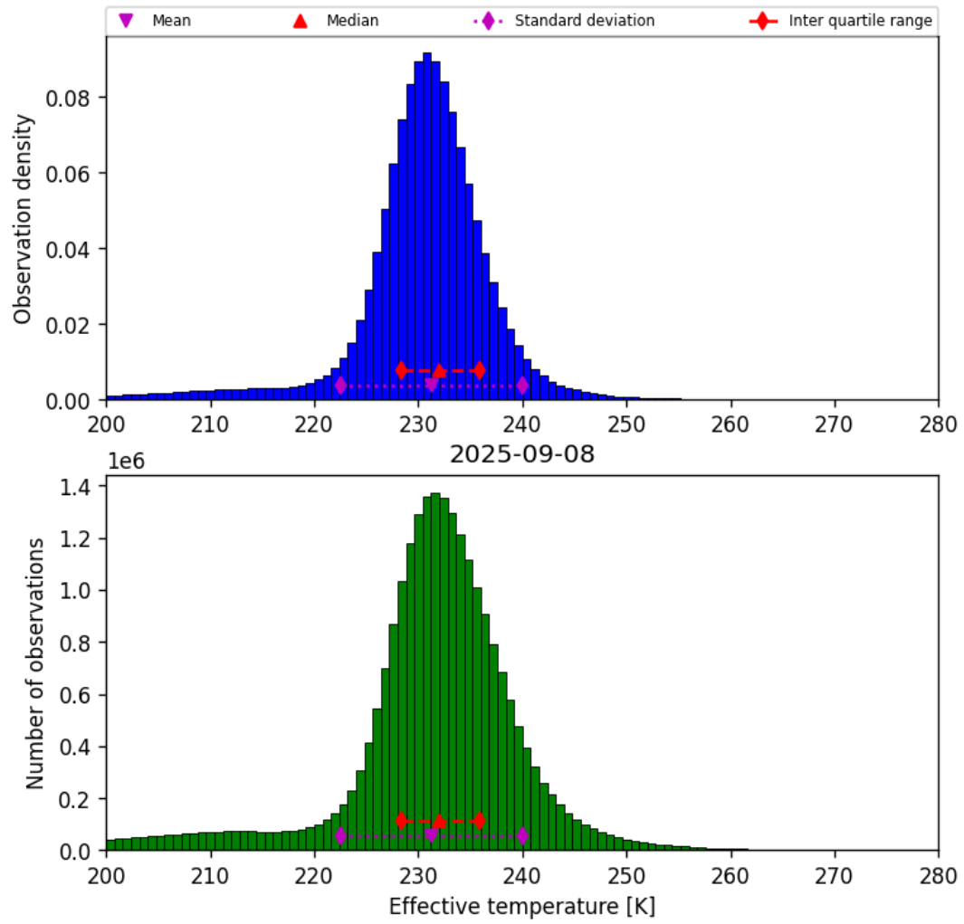
Figure 38: Histogram of “Effective temperature” for 2025-09-08 to 2025-09-08
