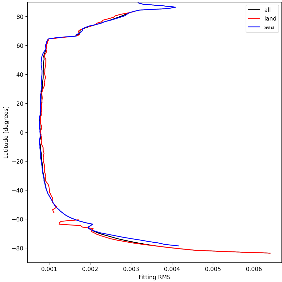
Figure 22: Zonal average of “Fitting RMS” for 2025-09-08 to 2025-09-08.
