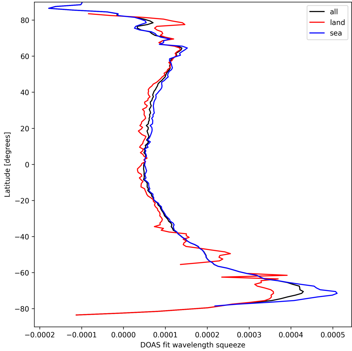
Figure 24: Zonal average of “DOAS fit wavelength squeeze” for 2025-09-08 to 2025-09-08.
