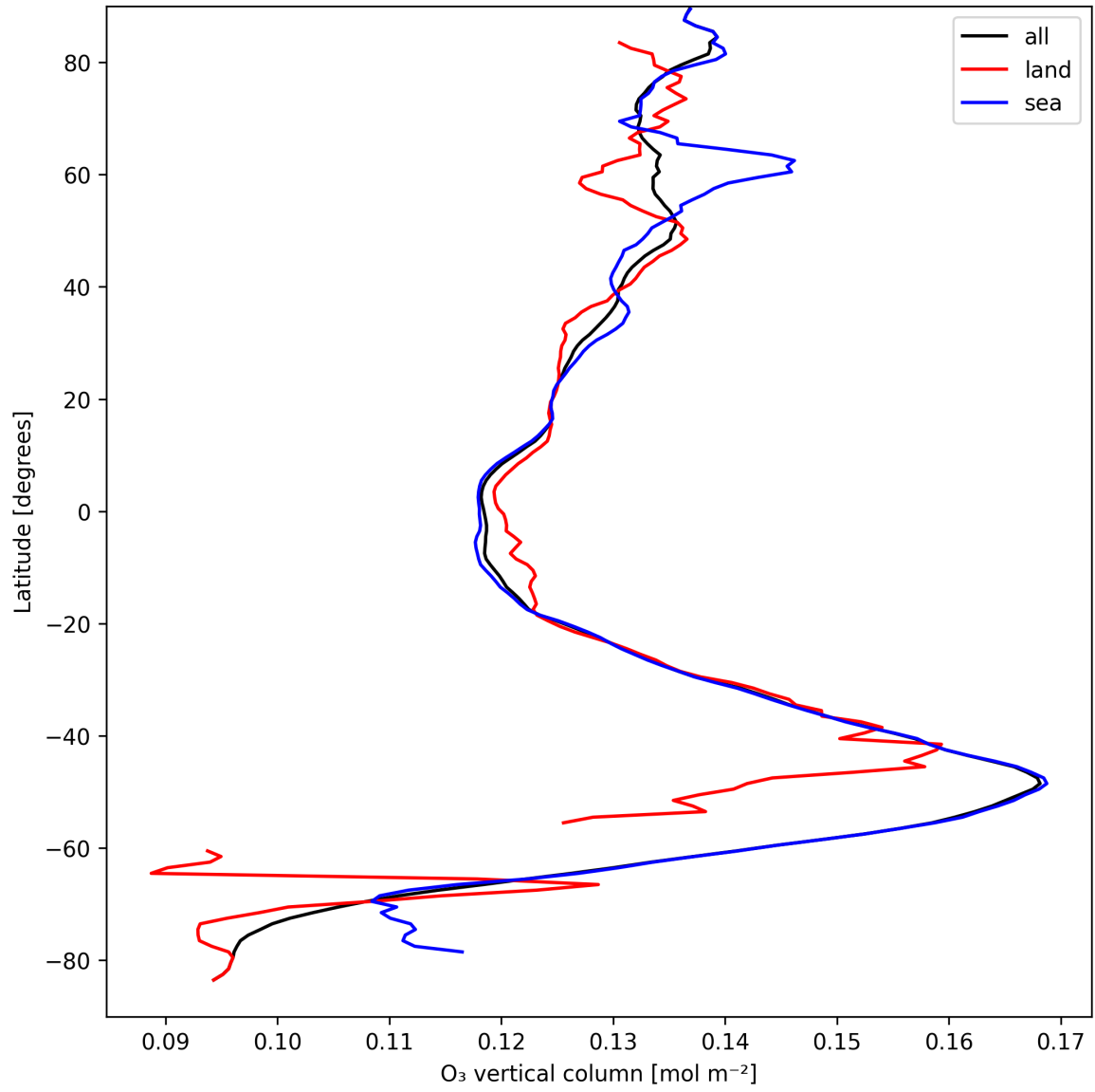
Figure 17: Zonal average of “O 3 vertical column” for 2025-09-08 to 2025-09-08.
