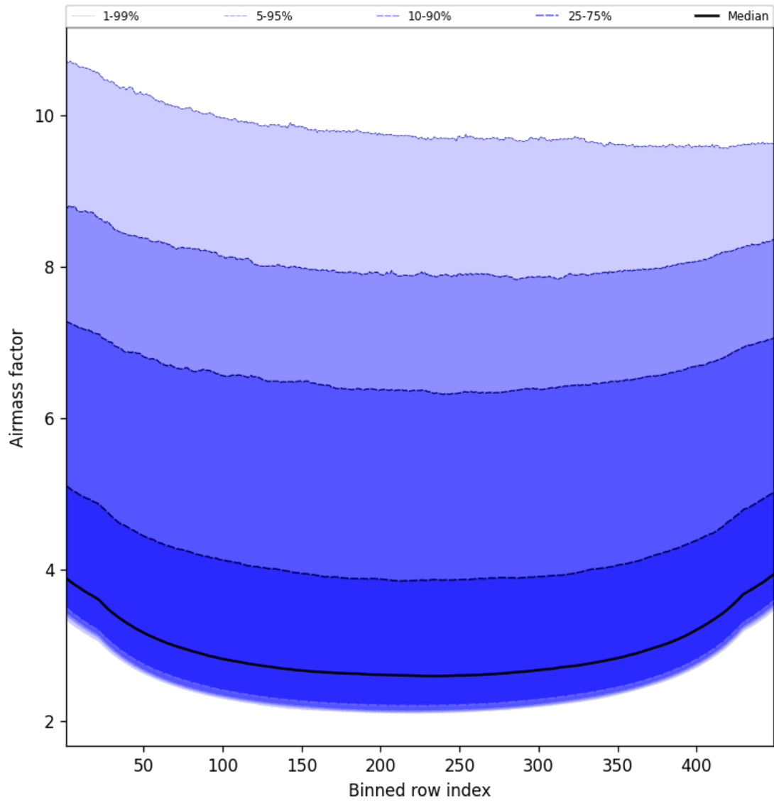
Figure 49: Along track statistics of “Airmass factor” for 2025-09-08 to 2025-09-08
