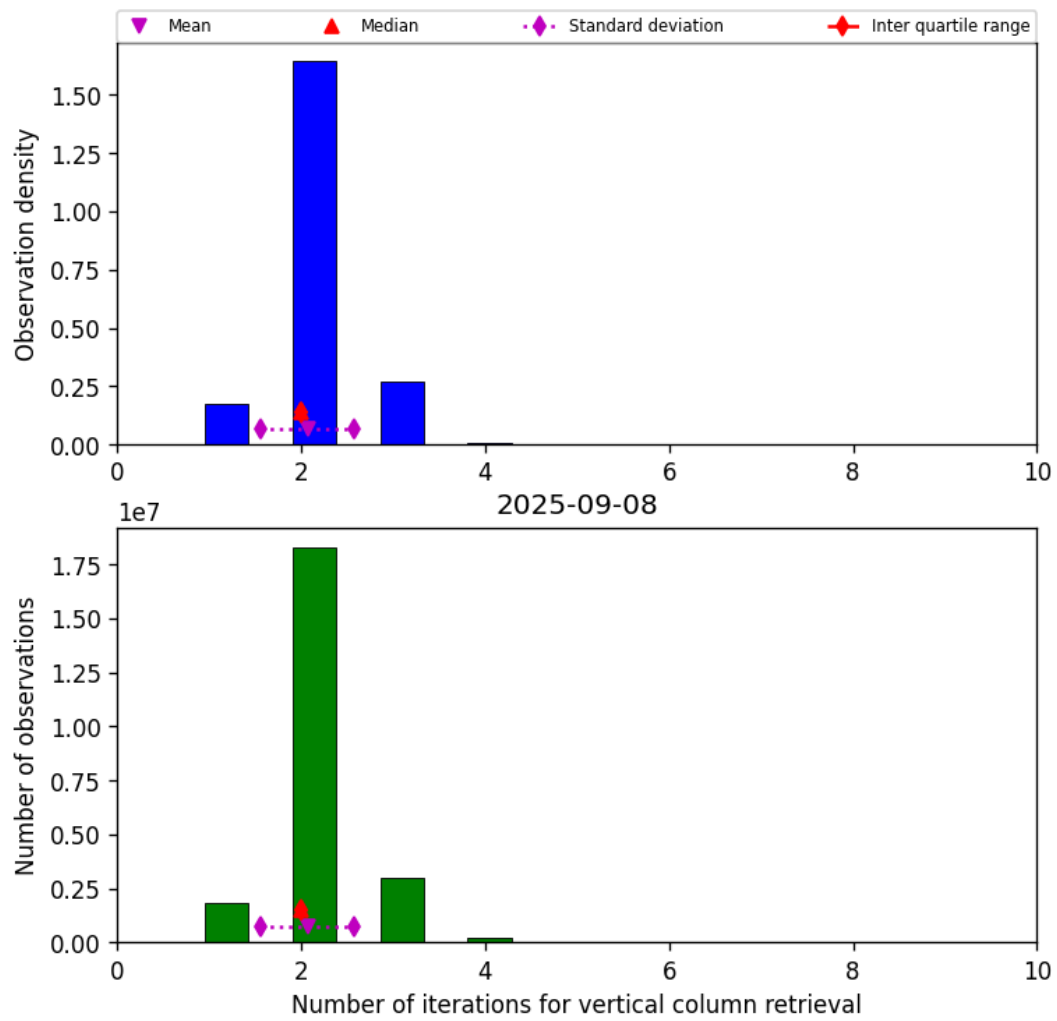
Figure 39: Histogram of “Number of iterations for vertical column retrieval” for 2025-09-08 to 2025-09-08
