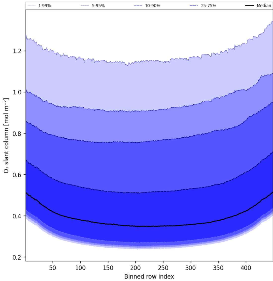
Figure 43: Along track statistics of “O 3 slant column” for 2025-09-08 to 2025-09-08
