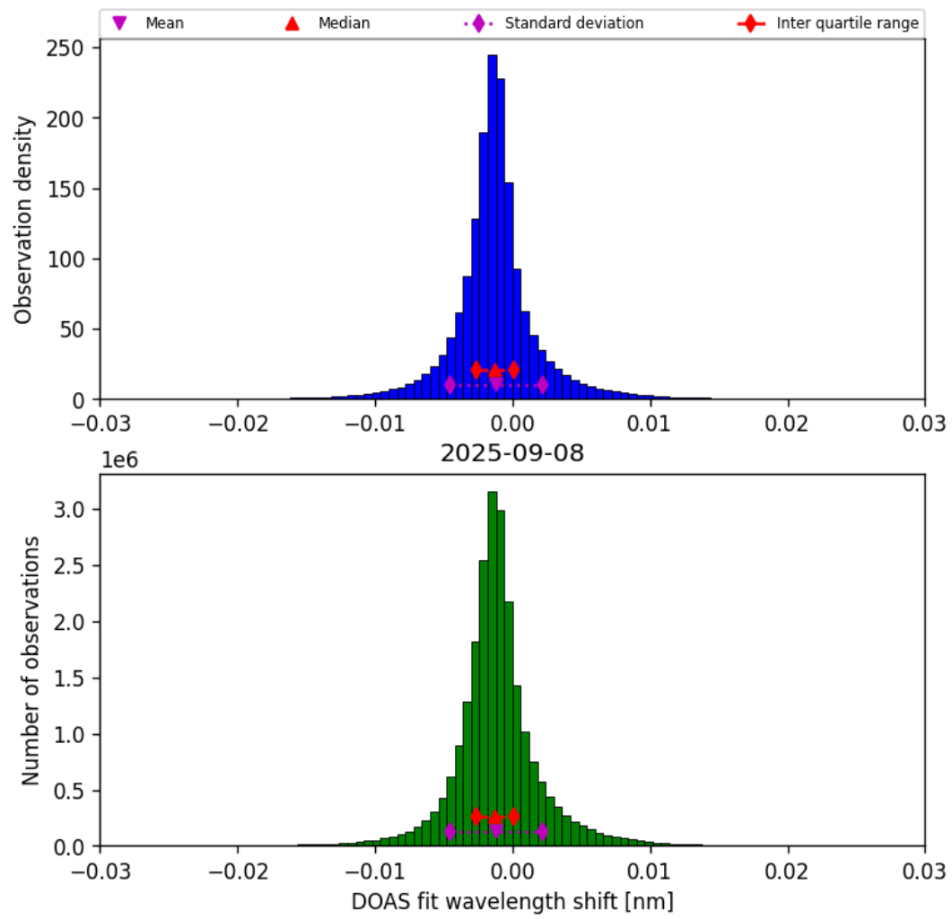
Figure 35: Histogram of “DOAS fit wavelength shift” for 2025-09-08 to 2025-09-08
