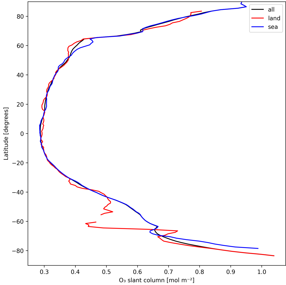
Figure 19: Zonal average of “O 3 slant column” for 2025-09-08 to 2025-09-08.
