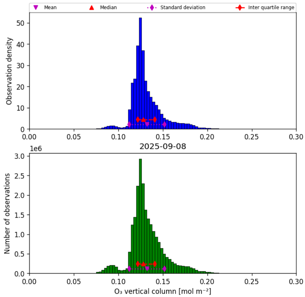
Figure 29: Histogram of “O 3 vertical column” for 2025-09-08 to 2025-09-08
