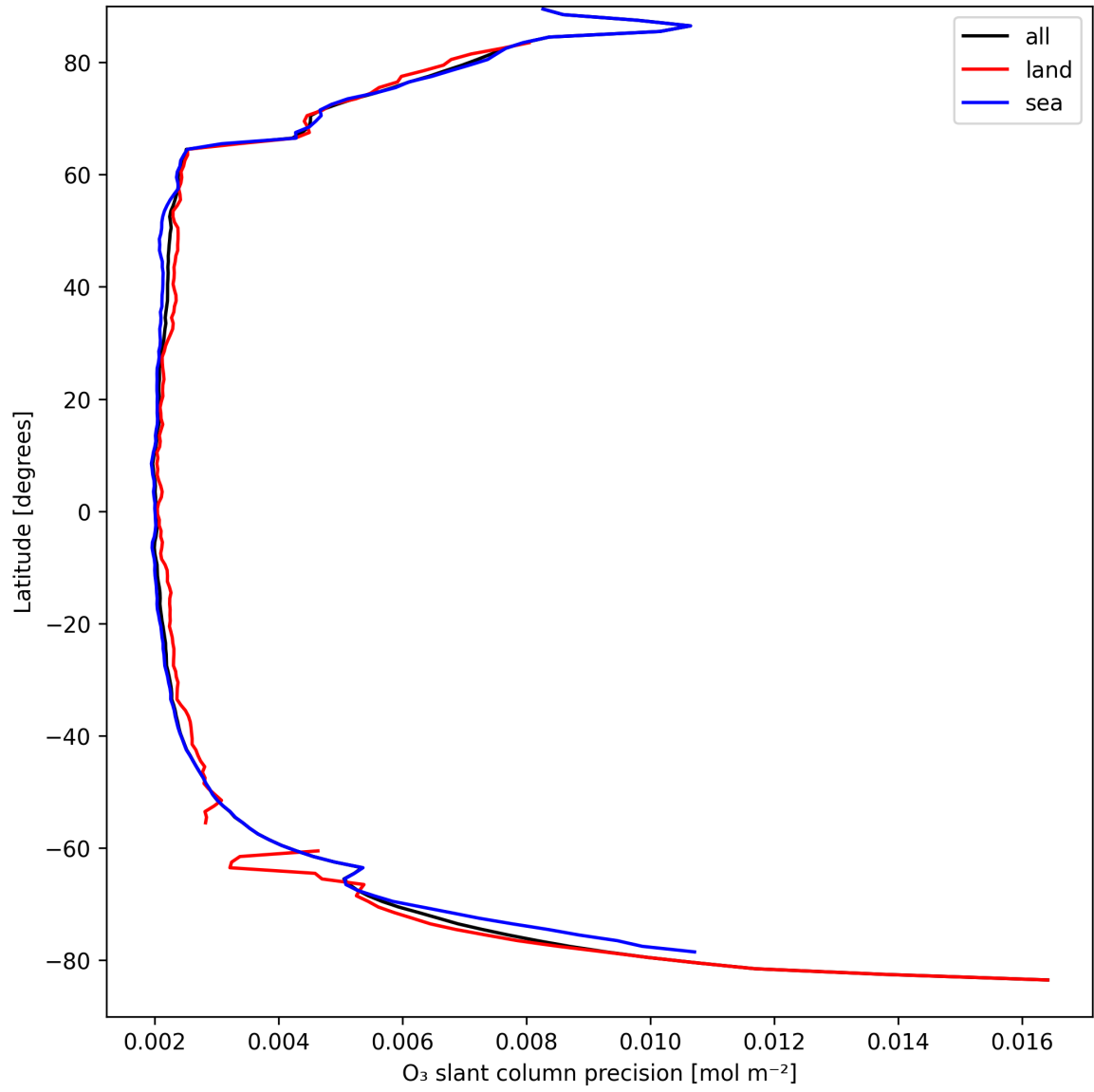
Figure 20: Zonal average of “O 3 slant column precision” for 2025-09-08 to 2025-09-08.
