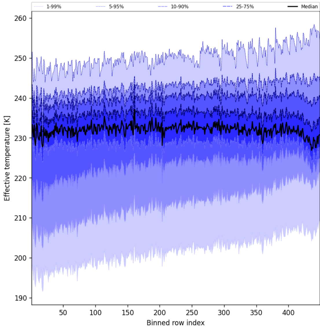
Figure 50: Along track statistics of “Effective temperature” for 2025-09-08 to 2025-09-08
