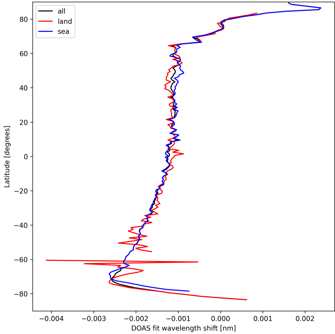
Figure 23: Zonal average of “DOAS fit wavelength shift” for 2025-09-08 to 2025-09-08.
