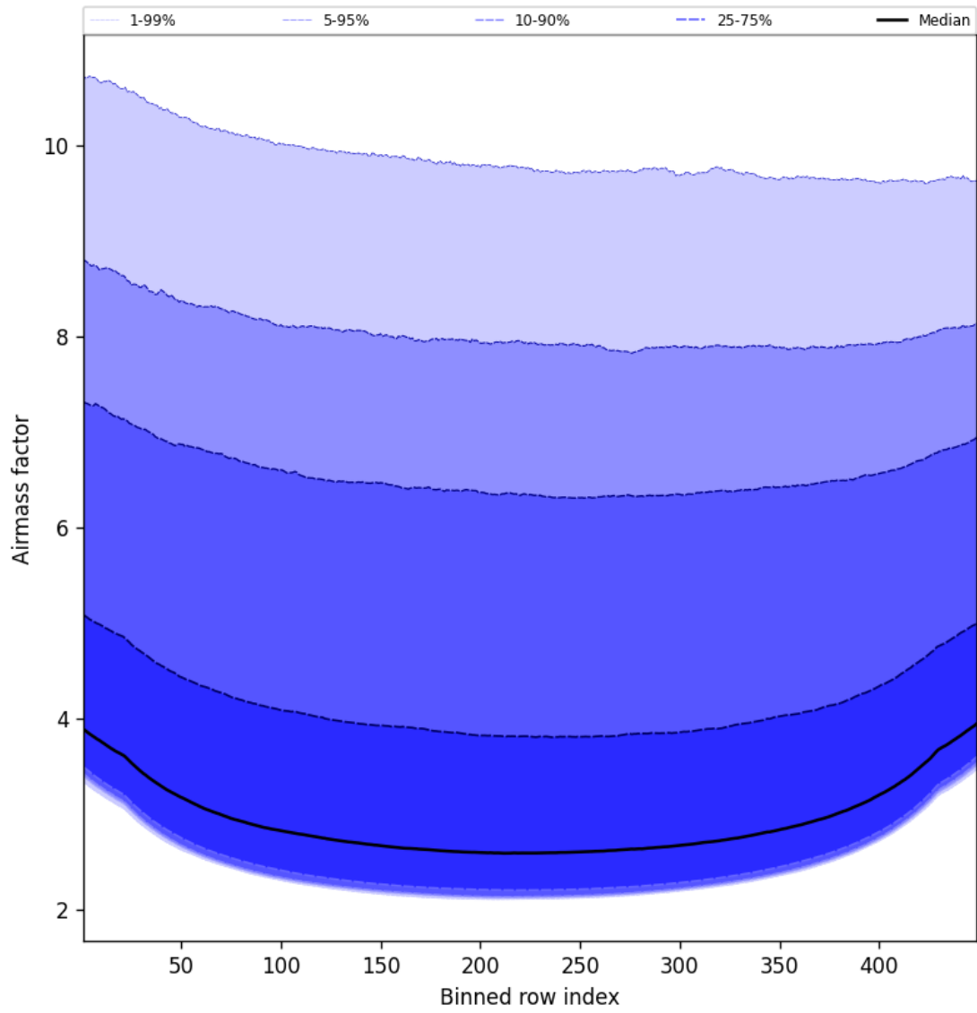
Figure 49: Along track statistics of “Airmass factor” for 2025-09-10 to 2025-09-11
