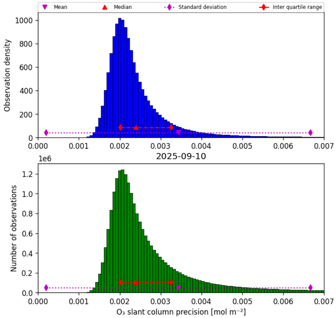
Figure 32: Histogram of “O 3 slant column precision” for 2025-09-10 to 2025-09-11
