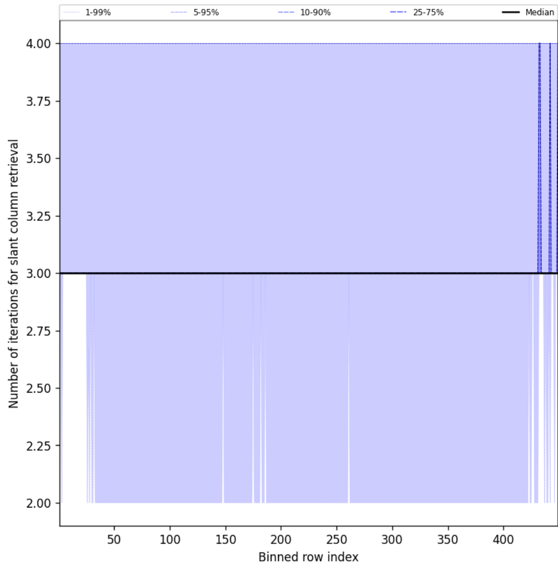
Figure 45: Along track statistics of “Number of iterations for slant column retrieval” for 2025-09-10 to 2025-09-11
