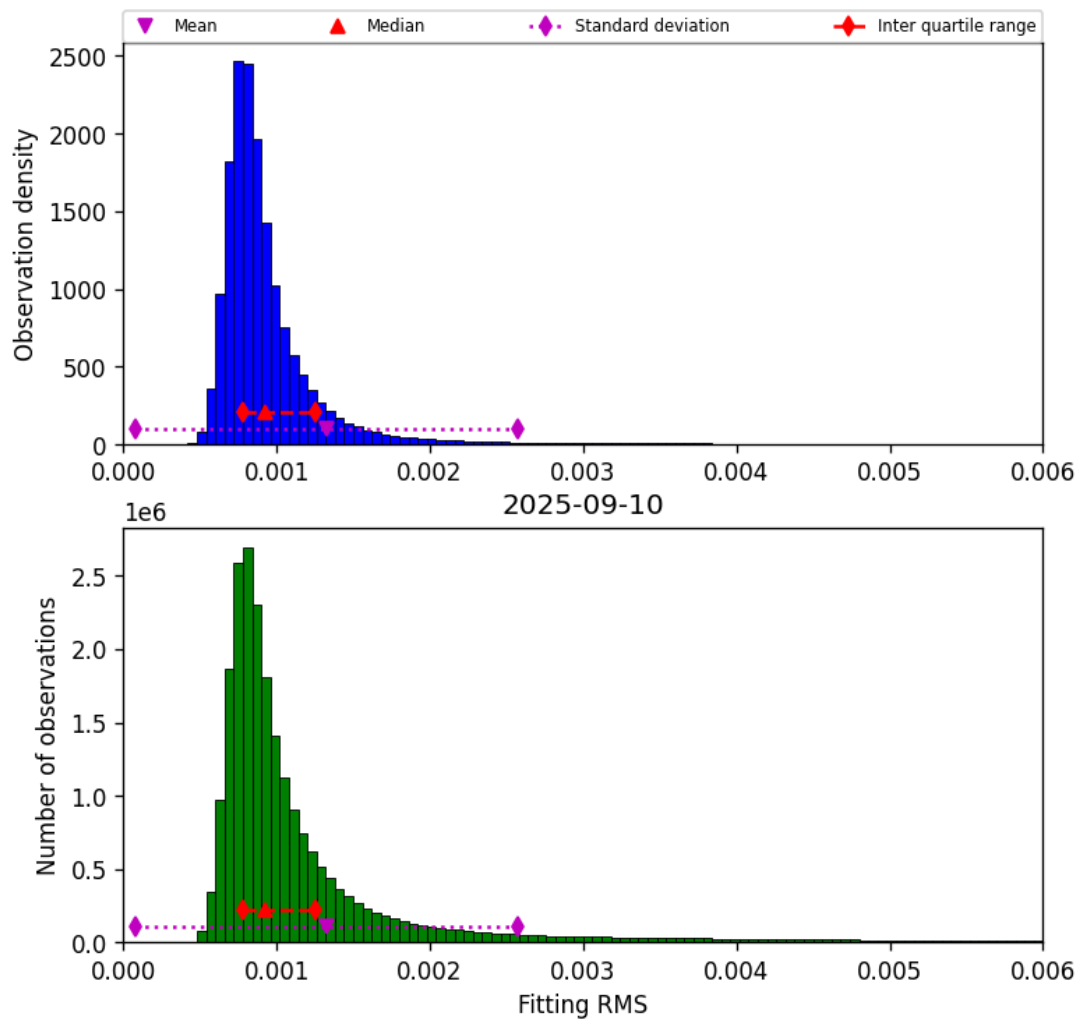
Figure 34: Histogram of “Fitting RMS” for 2025-09-10 to 2025-09-11
