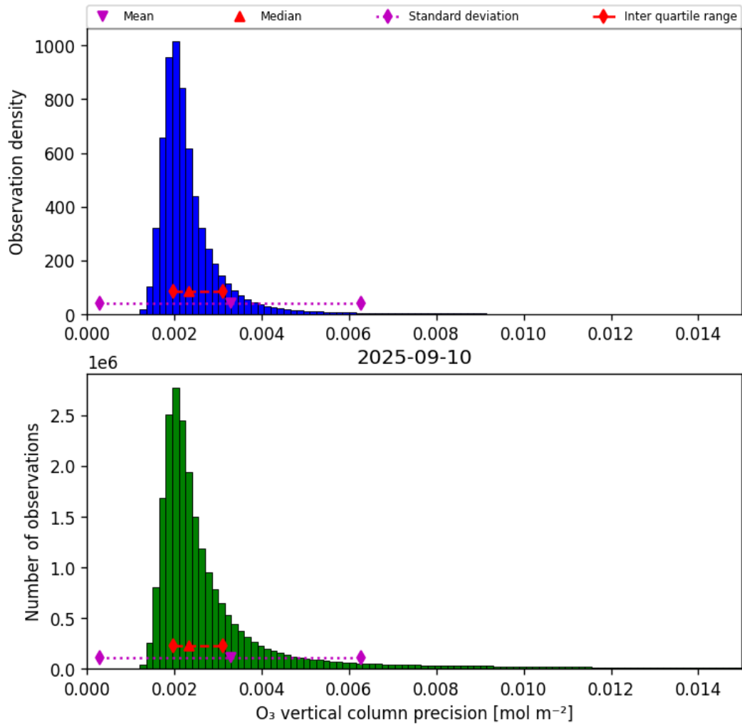
Figure 30: Histogram of “O 3 vertical column precision” for 2025-09-10 to 2025-09-11
