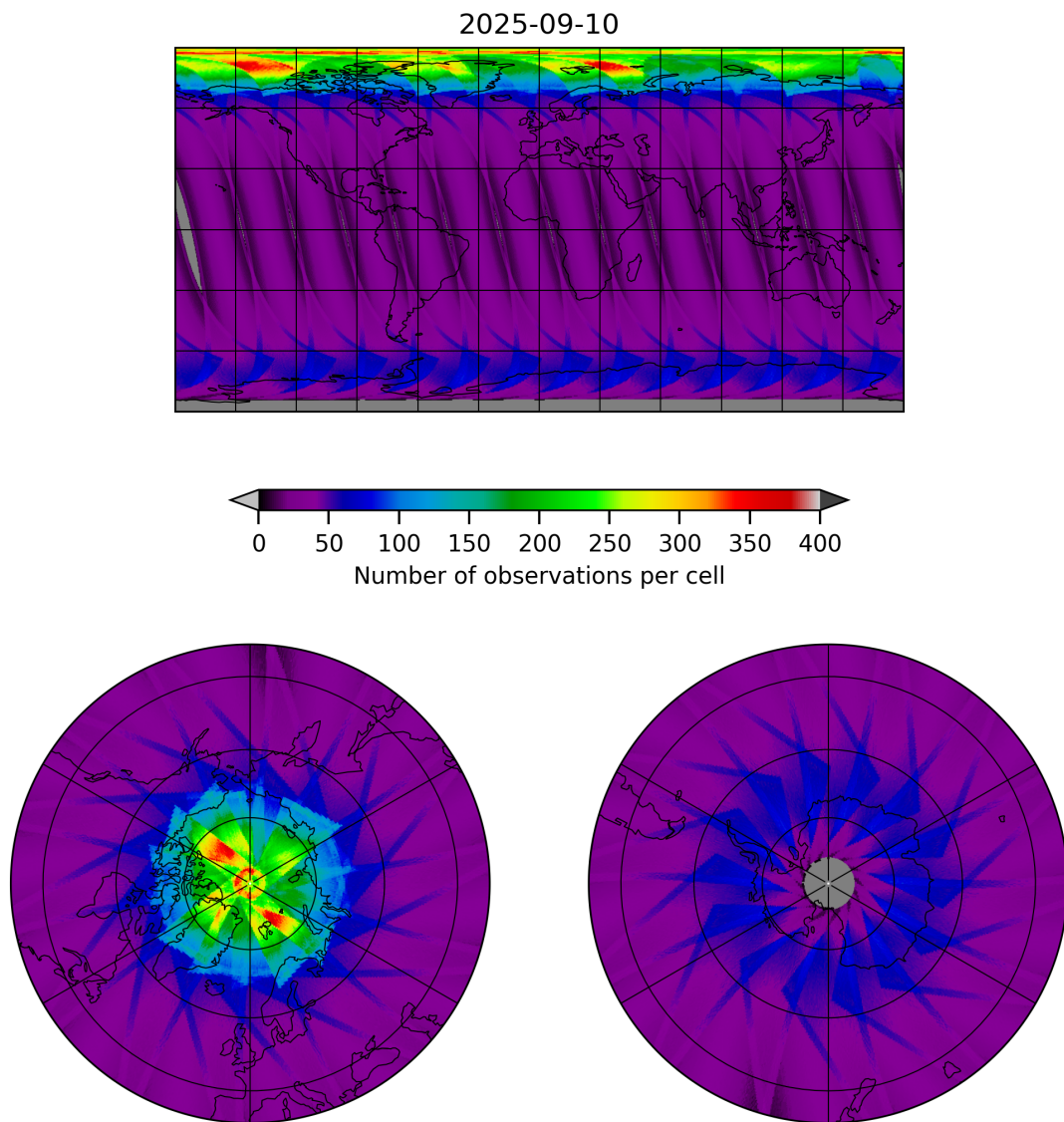
Figure 15: Map of the number of observations for 2025-09-10 to 2025-09-11
