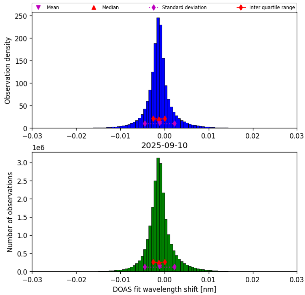
Figure 35: Histogram of “DOAS fit wavelength shift” for 2025-09-10 to 2025-09-11
