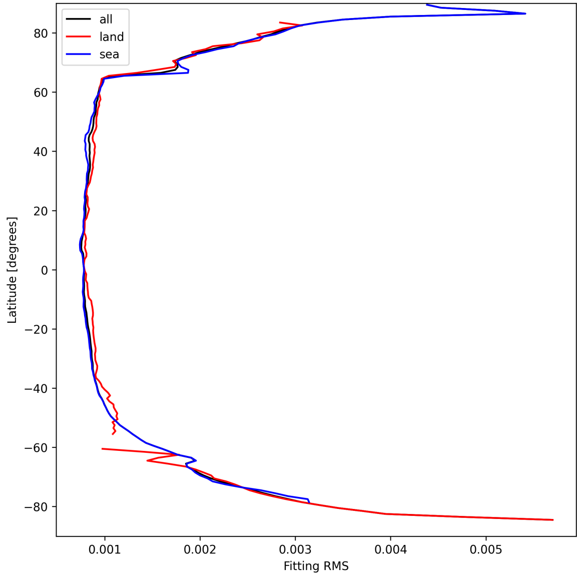
Figure 22: Zonal average of “Fitting RMS” for 2025-09-10 to 2025-09-11.
