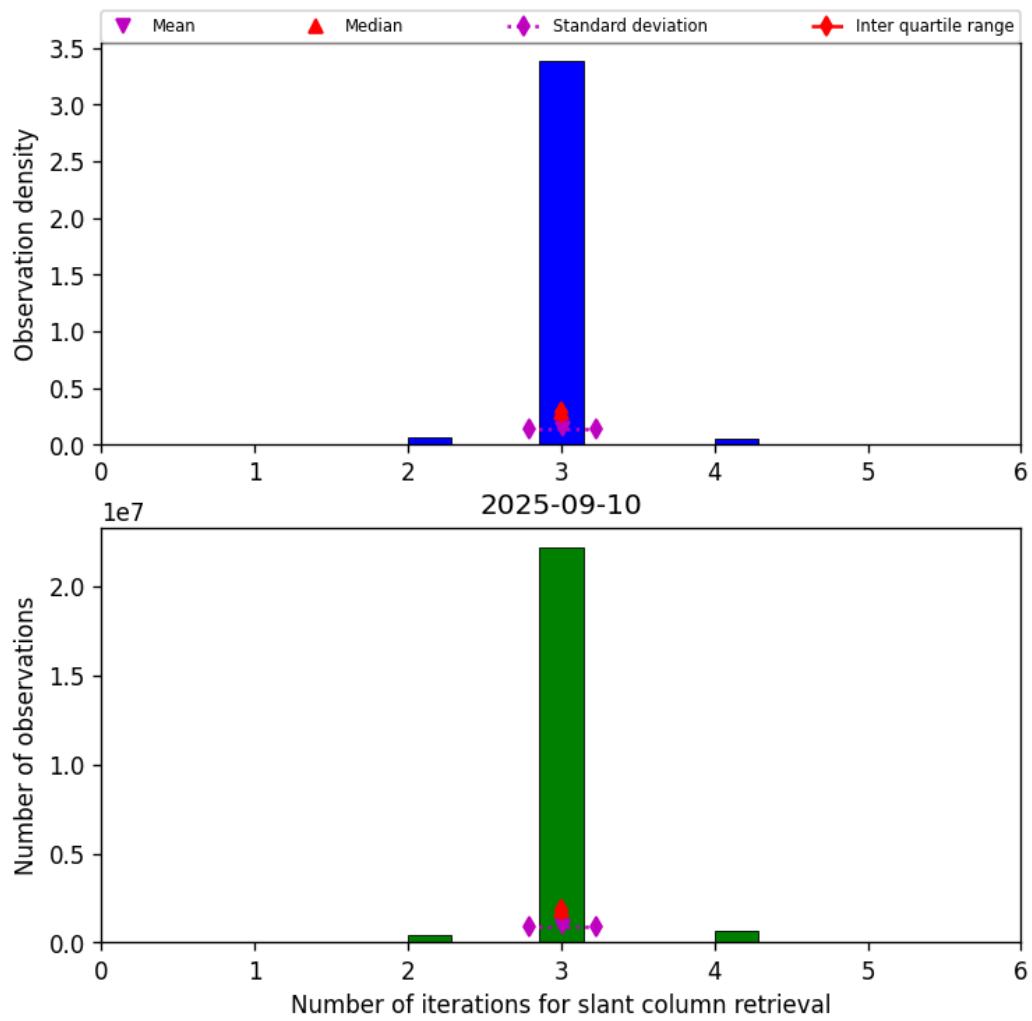
Figure 33: Histogram of “Number of iterations for slant column retrieval” for 2025-09-10 to 2025-09-11
