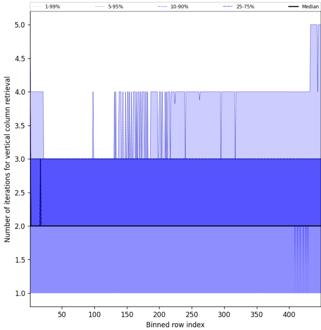
Figure 51: Along track statistics of “Number of iterations for vertical column retrieval” for 2025-09-10 to 2025-09-11
