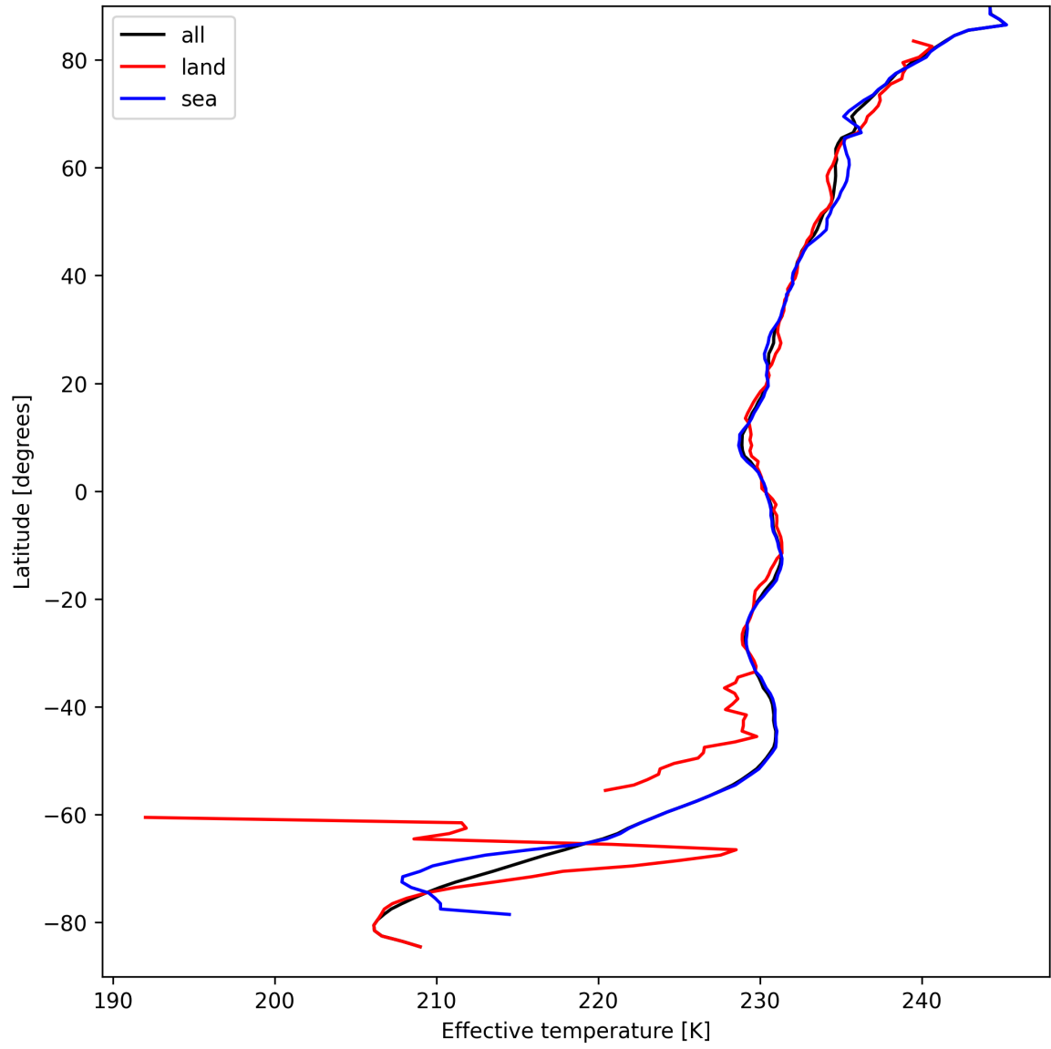
Figure 26: Zonal average of "Effective temperature" for 2025-09-10 to 2025-09-11.
