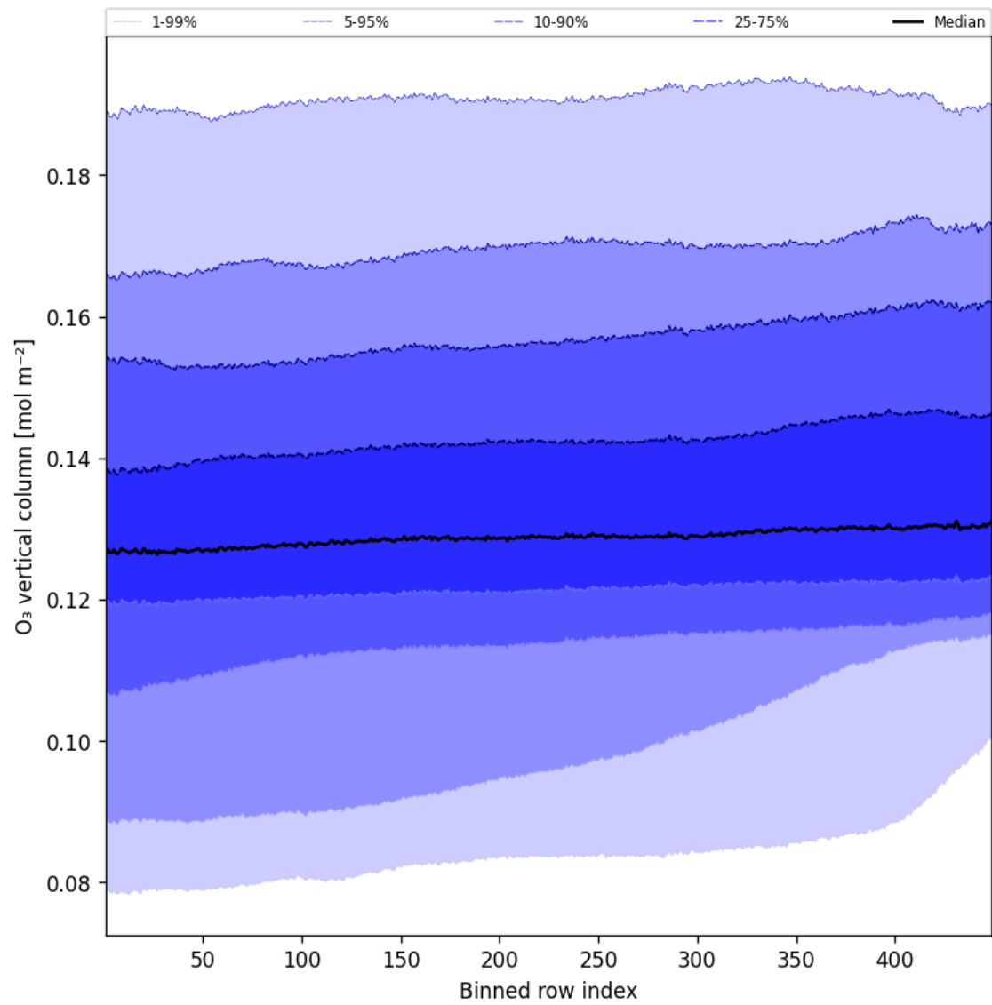
Figure 41: Along track statistics of “O 3 vertical column” for 2025-09-10 to 2025-09-11
