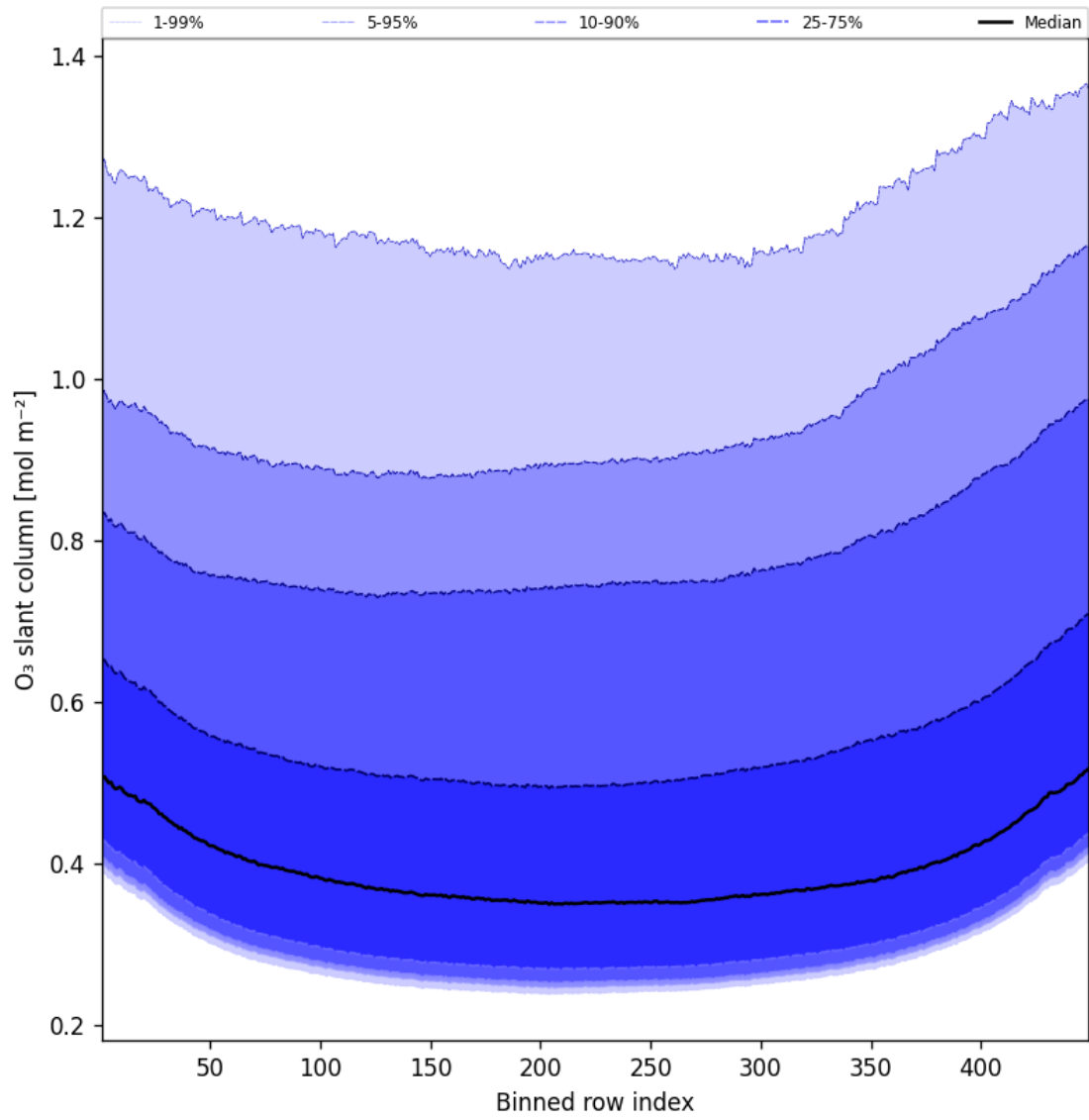
Figure 43: Along track statistics of “O 3 slant column” for 2025-09-10 to 2025-09-11
