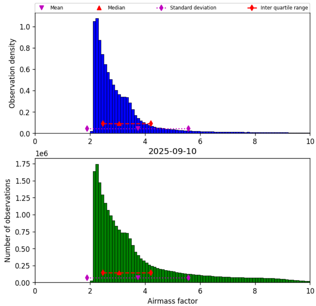
Figure 37: Histogram of “Airmass factor” for 2025-09-10 to 2025-09-11
