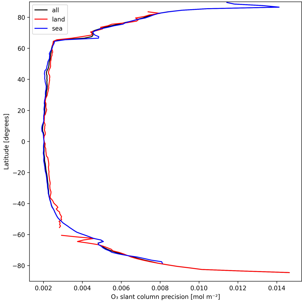
Figure 20: Zonal average of "O 3 slant column precision" for 2025-09-10 to 2025-09-11.
