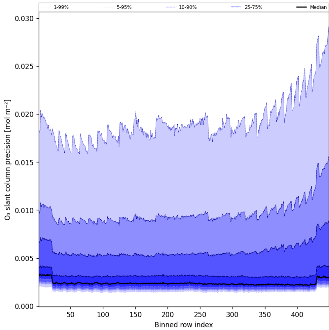
Figure 44: Along track statistics of “O 3 slant column precision” for 2025-09-10 to 2025-09-11
