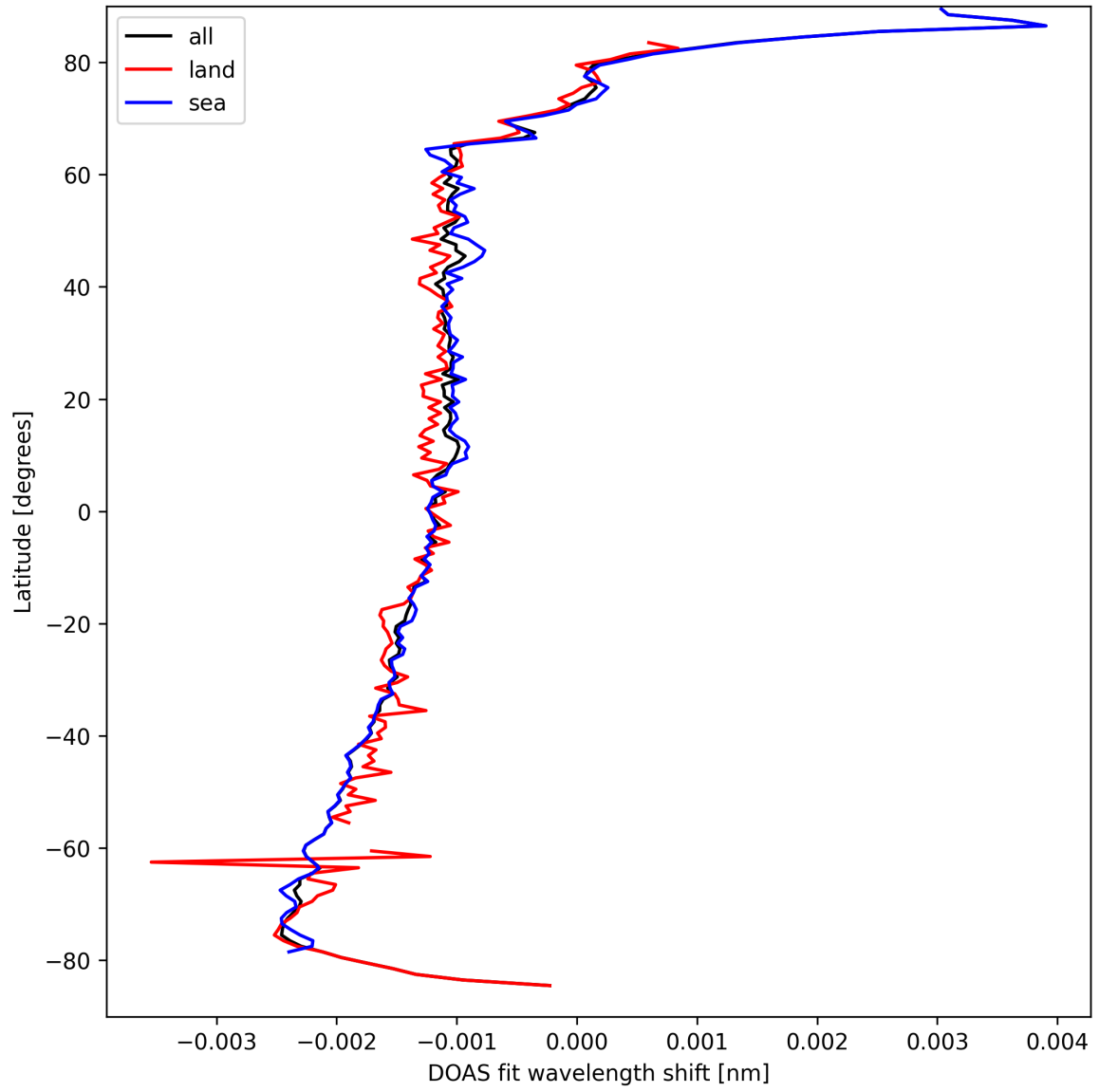
Figure 23: Zonal average of “DOAS fit wavelength shift” for 2025-09-10 to 2025-09-11.
