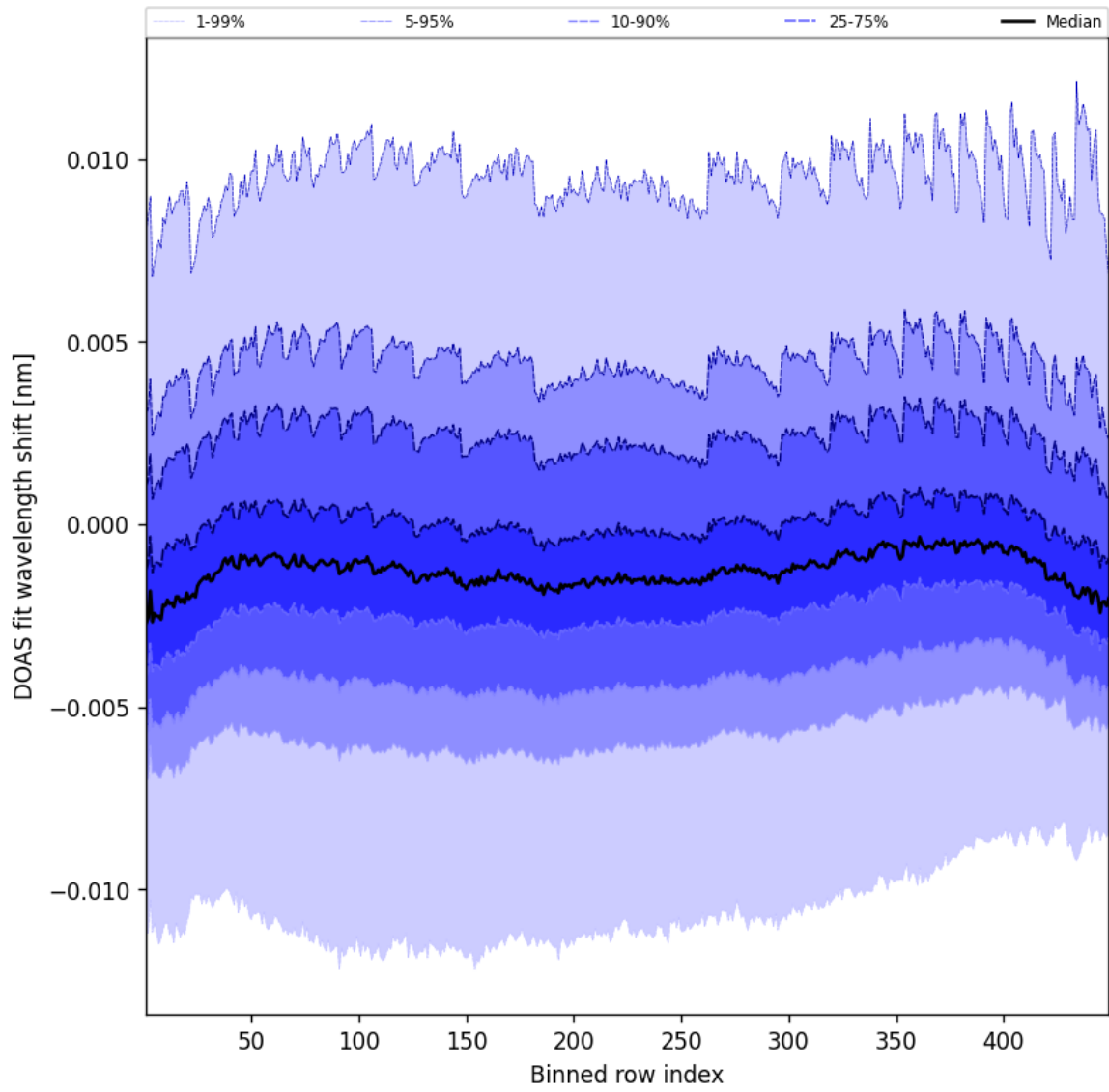
Figure 47: Along track statistics of “DOAS fit wavelength shift” for 2025-09-10 to 2025-09-11
