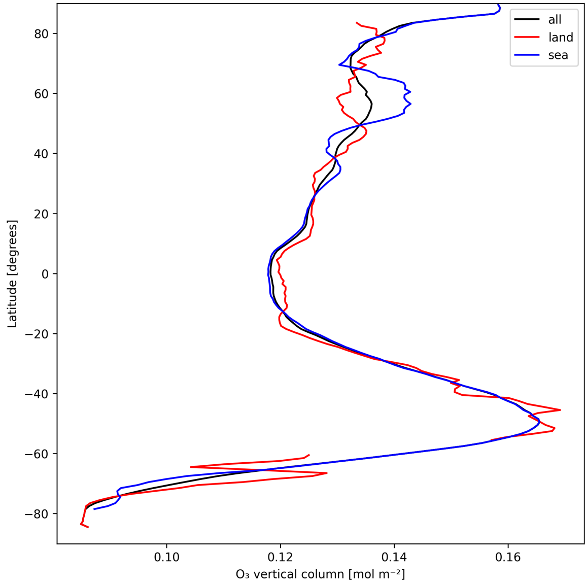
Figure 17: Zonal average of “O 3 vertical column” for 2025-09-10 to 2025-09-11.
