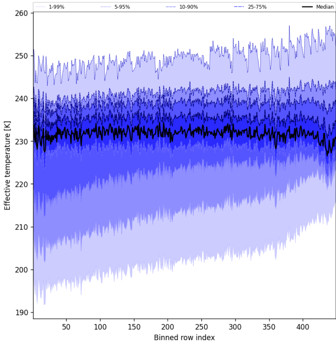
Figure 50: Along track statistics of “Effective temperature” for 2025-09-10 to 2025-09-11
