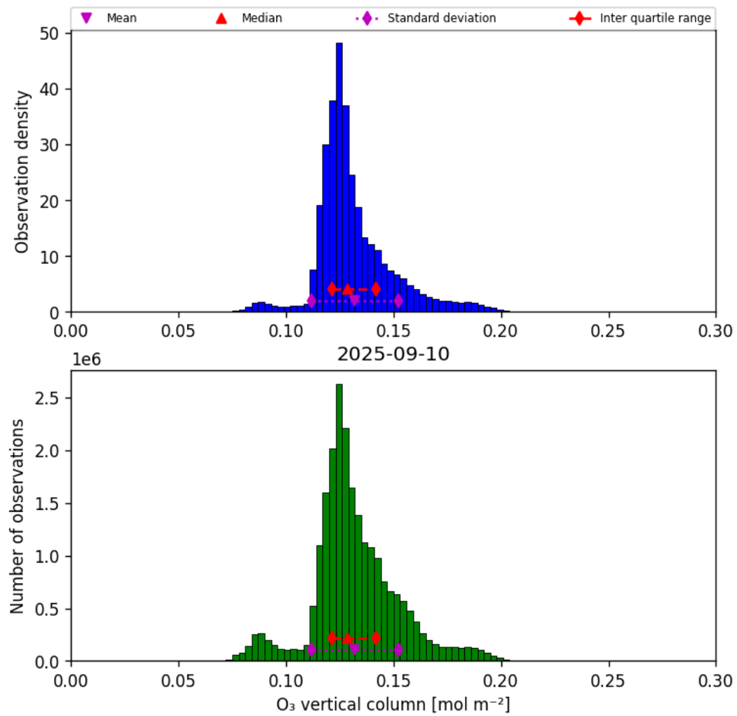
Figure 29: Histogram of “O 3 vertical column” for 2025-09-10 to 2025-09-11
