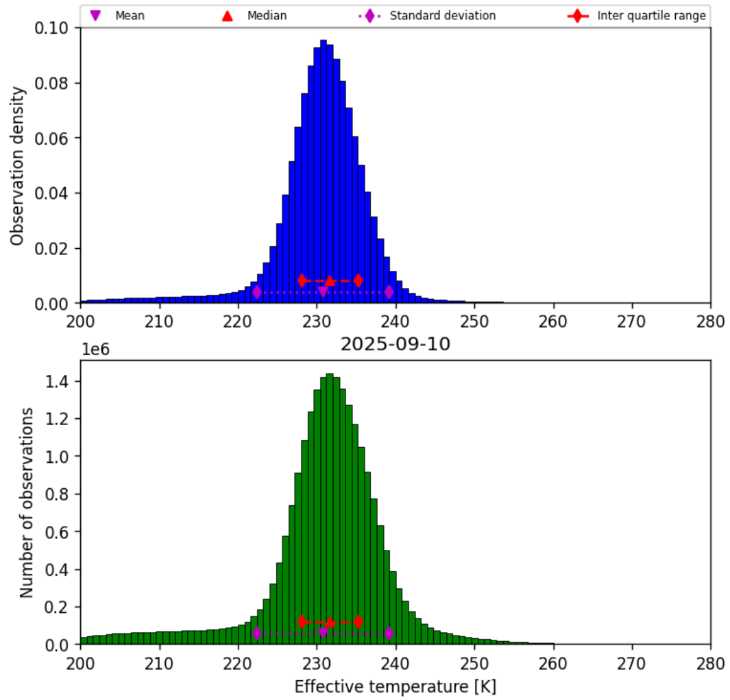
Figure 38: Histogram of “Effective temperature” for 2025-09-10 to 2025-09-11
