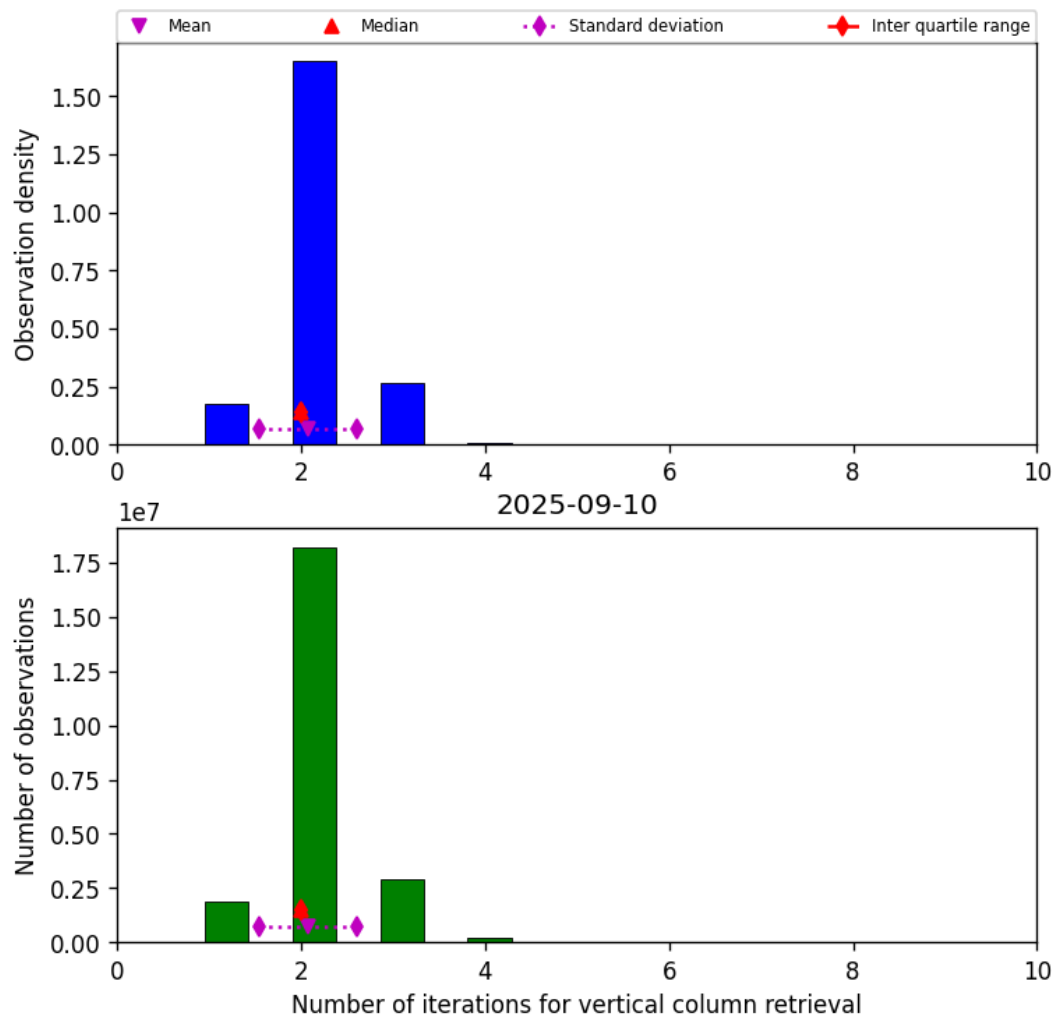
Figure 39: Histogram of “Number of iterations for vertical column retrieval” for 2025-09-10 to 2025-09-11
