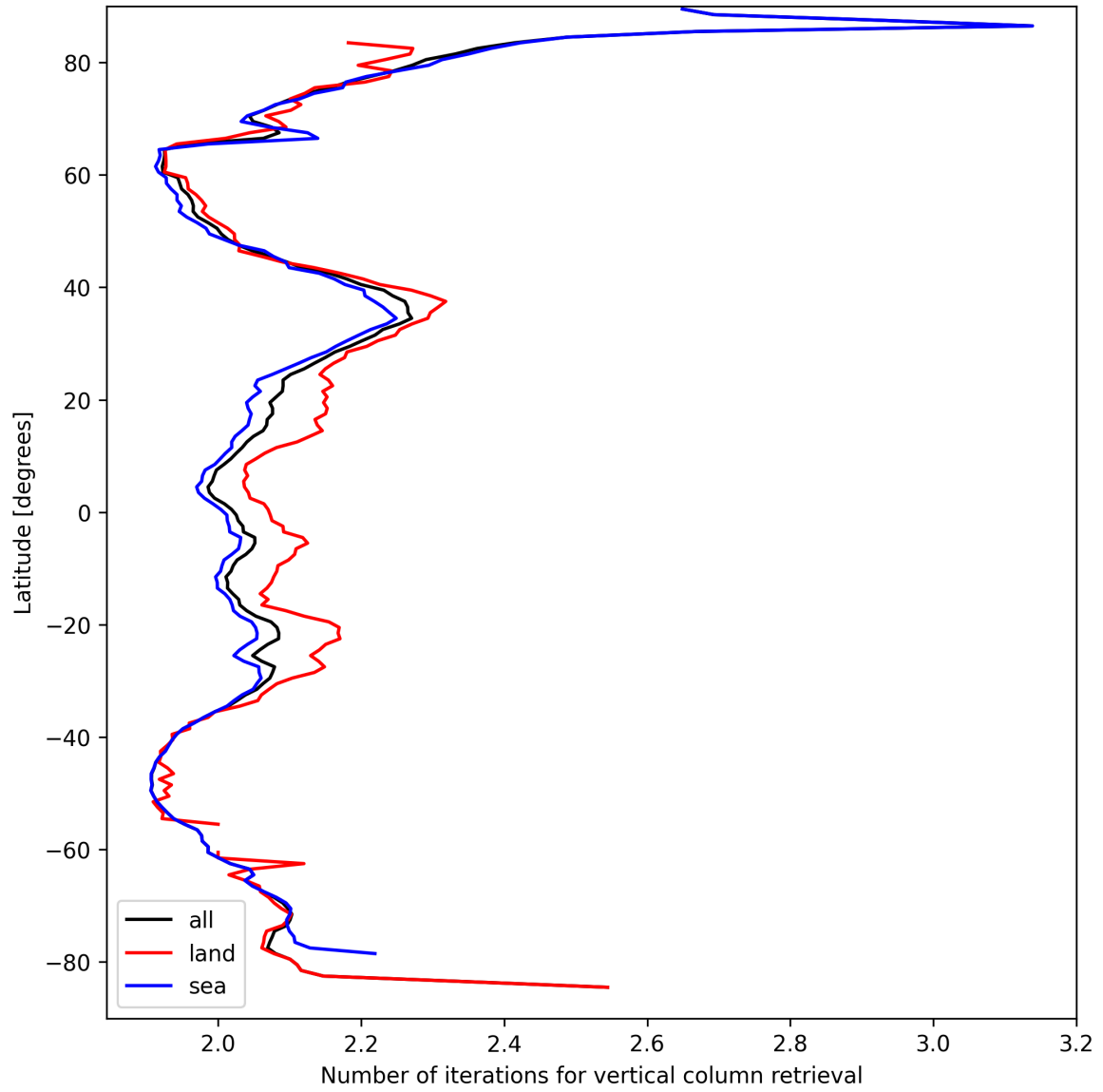
Figure 27: Zonal average of “Number of iterations for vertical column retrieval” for 2025-09-10 to 2025-09-11.
