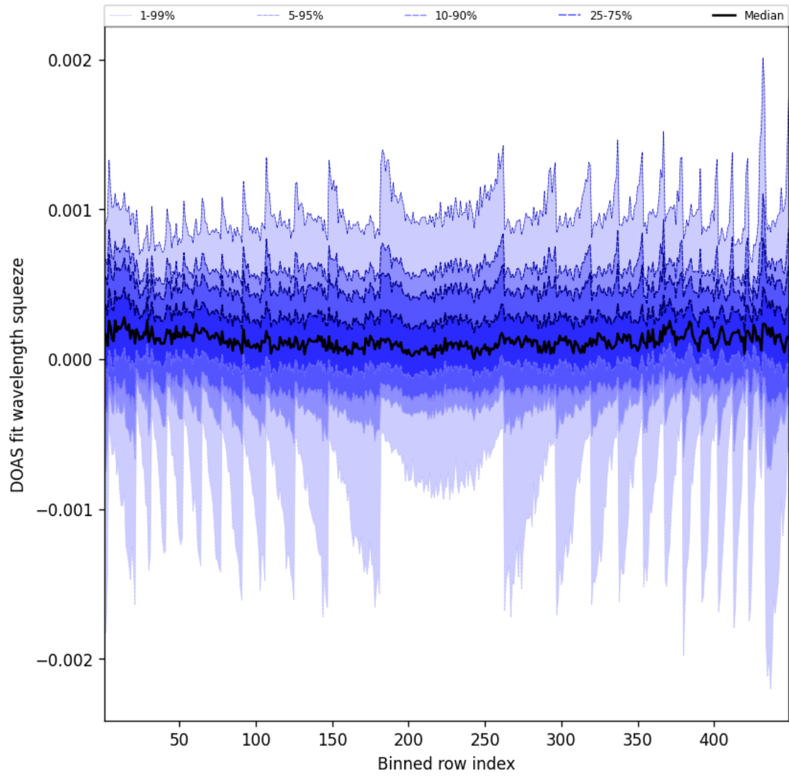
Figure 48: Along track statistics of “DOAS fit wavelength squeeze” for 2025-09-10 to 2025-09-11
