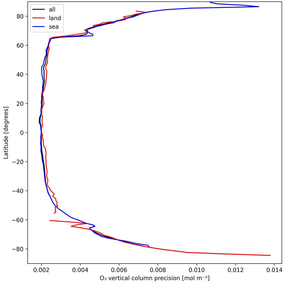
Figure 18: Zonal average of "O 3 vertical column precision" for 2025-09-10 to 2025-09-11.
