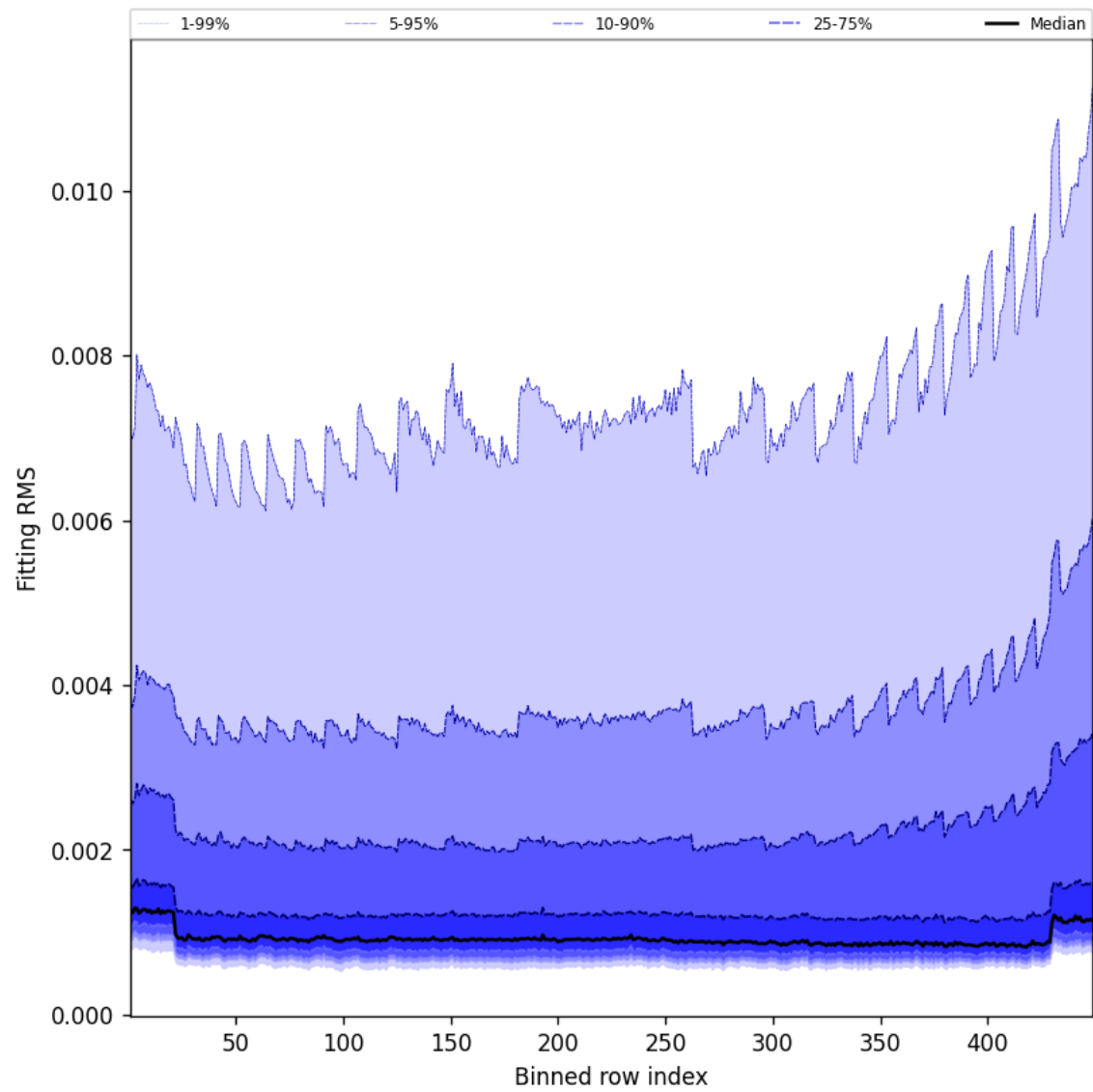
Figure 46: Along track statistics of “Fitting RMS” for 2025-09-10 to 2025-09-11
