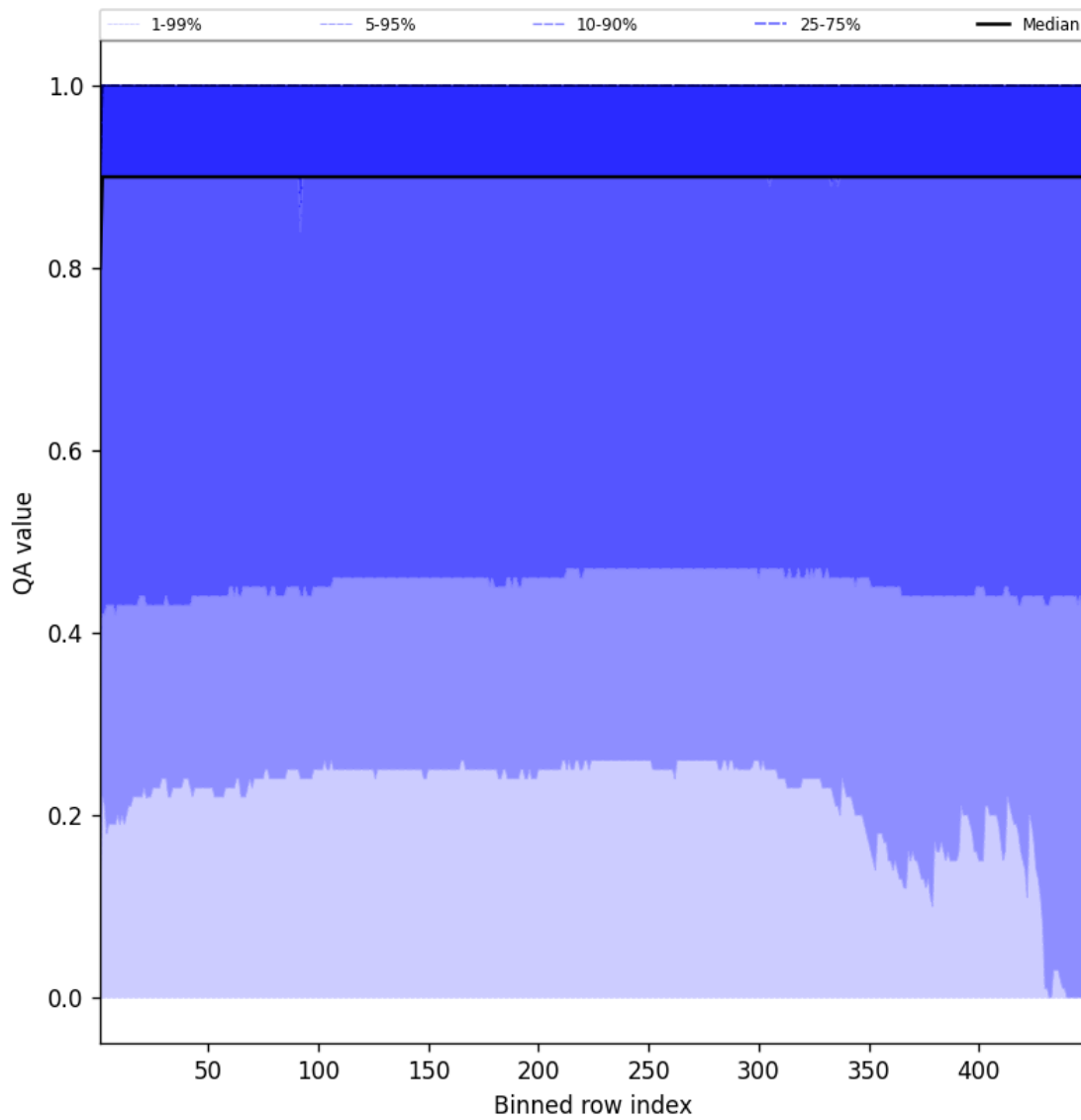
Figure 40: Along track statistics of “QA value” for 2025-09-10 to 2025-09-11
