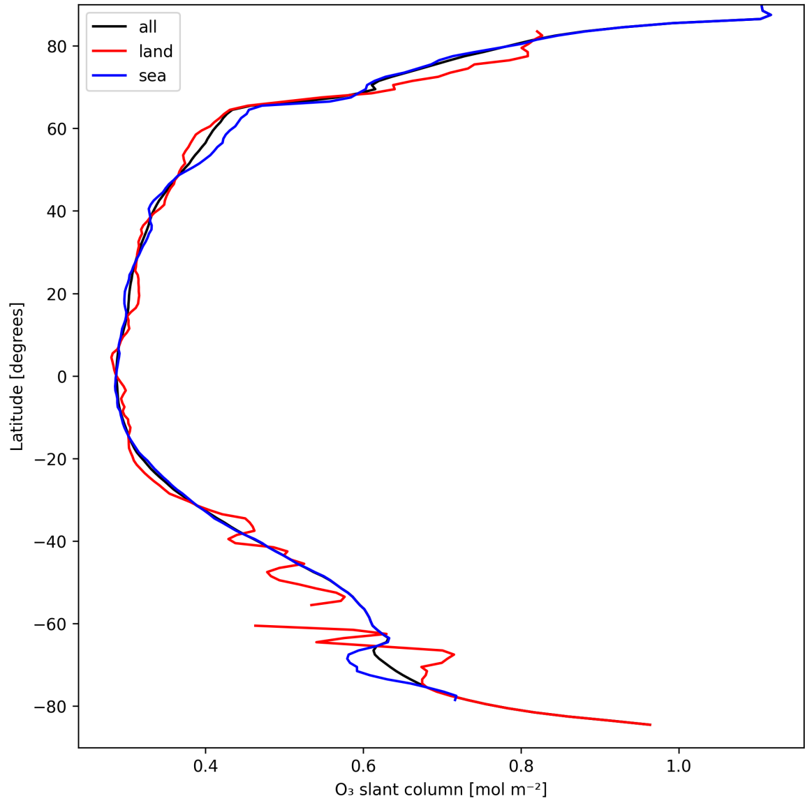
Figure 19: Zonal average of “O 3 slant column” for 2025-09-10 to 2025-09-11.
