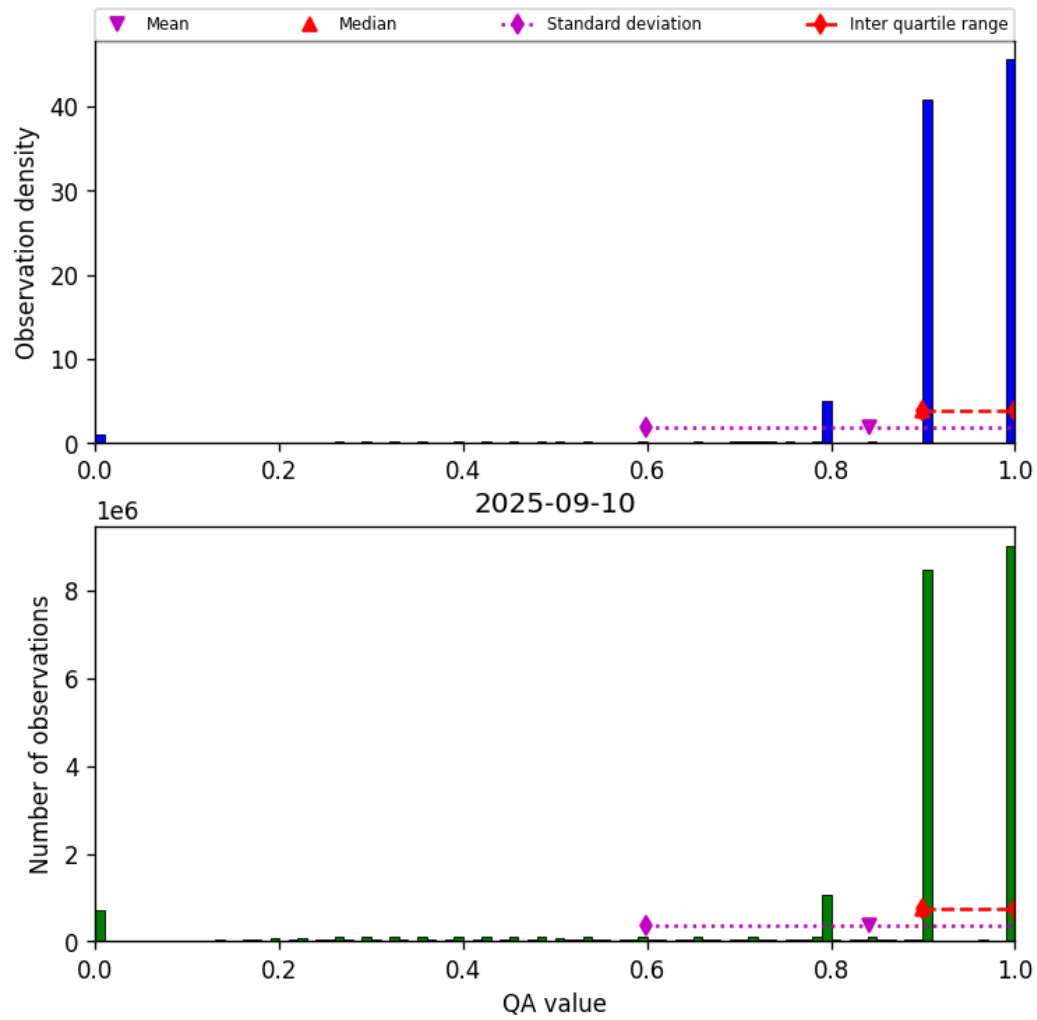
Figure 28: Histogram of “QA value” for 2025-09-10 to 2025-09-11
