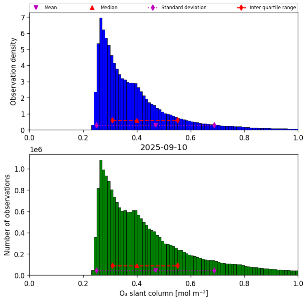
Figure 31: Histogram of “O 3 slant column” for 2025-09-10 to 2025-09-11
