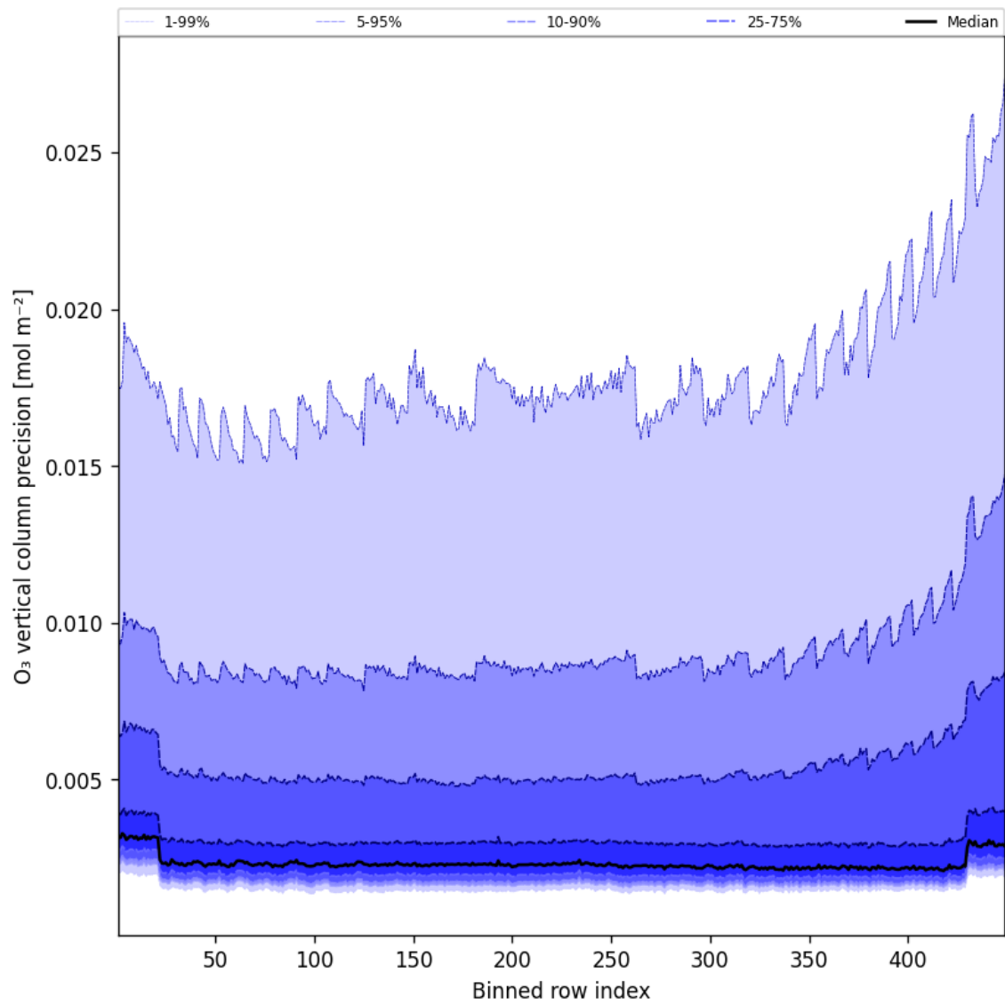
Figure 42: Along track statistics of “O 3 vertical column precision” for 2025-09-10 to 2025-09-11
