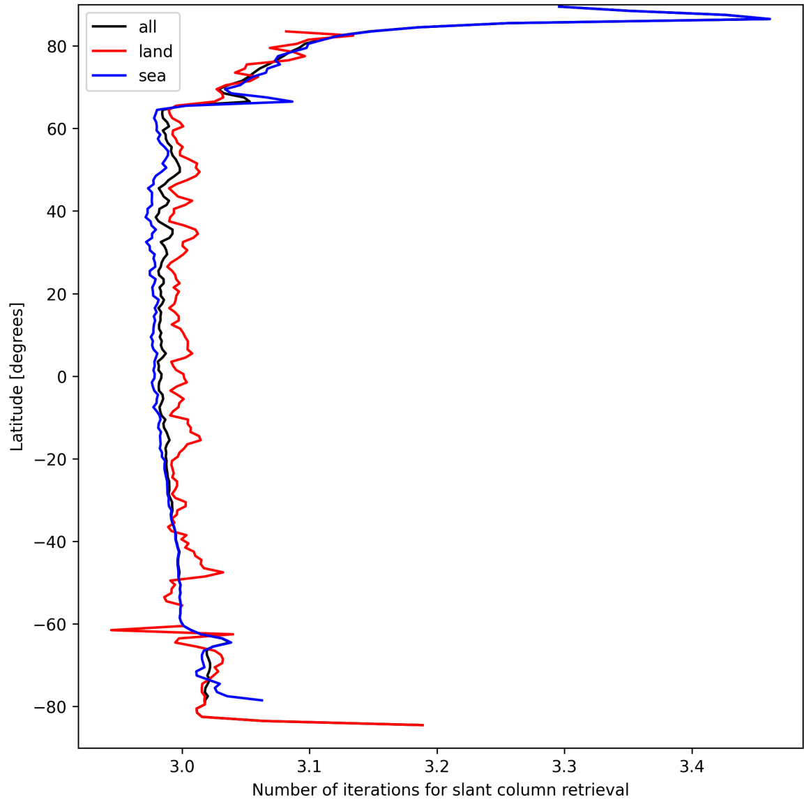
Figure 21: Zonal average of “Number of iterations for slant column retrieval” for 2025-09-10 to 2025-09-11.
