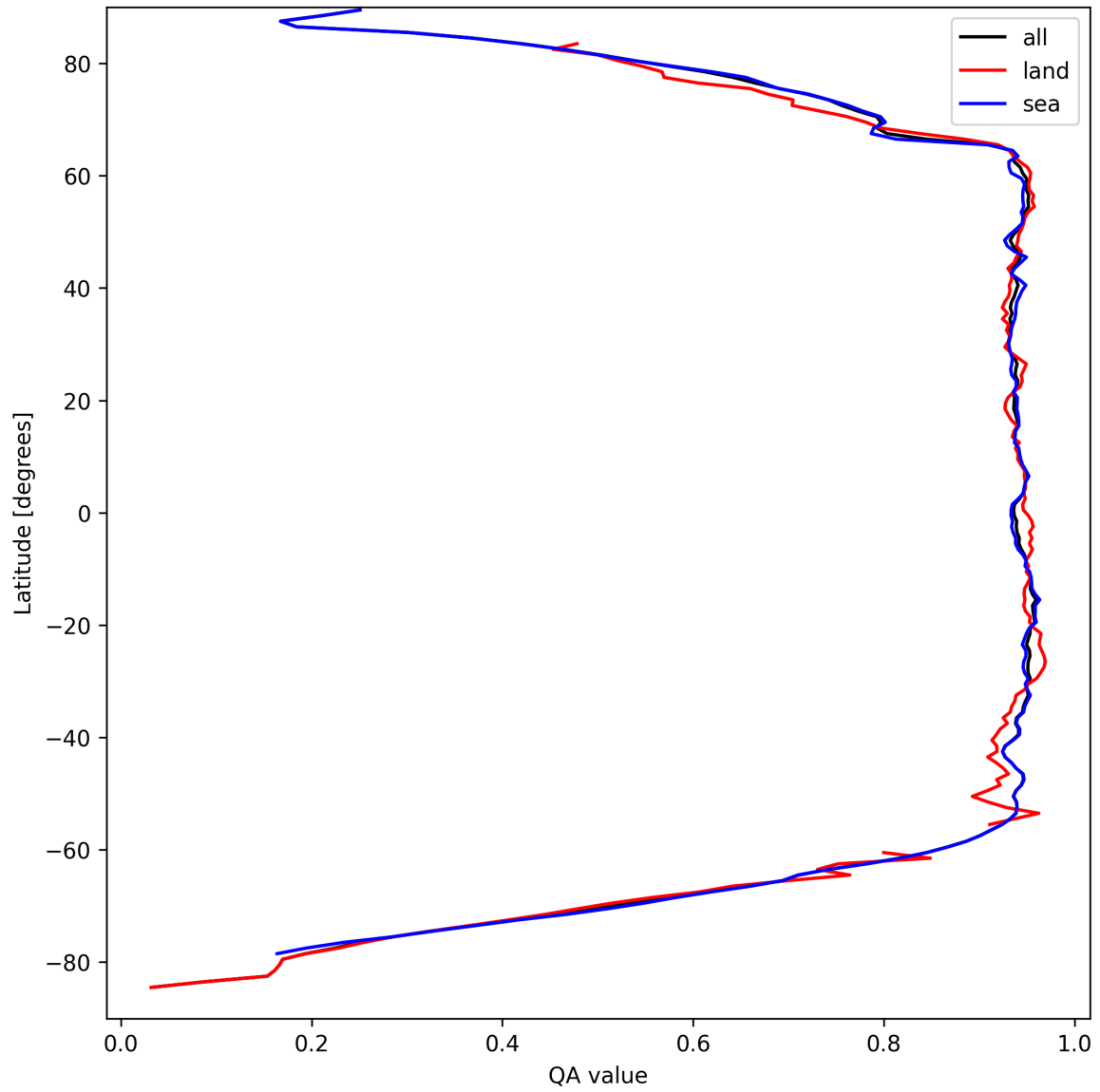
Figure 16: Zonal average of “QA value” for 2025-09-10 to 2025-09-11.
