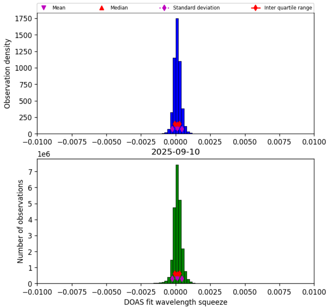
Figure 36: Histogram of “DOAS fit wavelength squeeze” for 2025-09-10 to 2025-09-11
