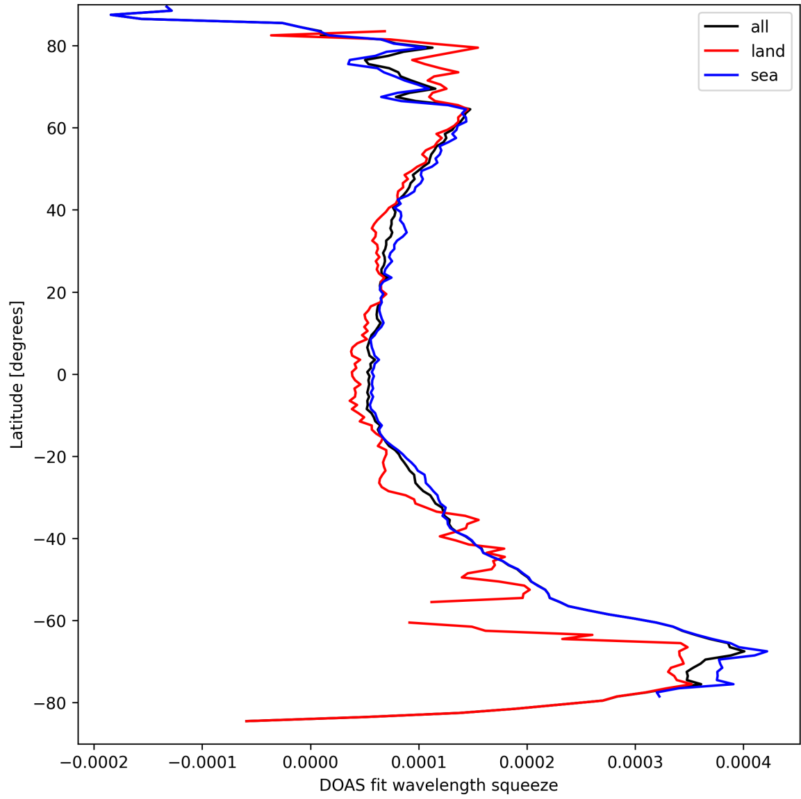
Figure 24: Zonal average of "DOAS fit wavelength squeeze" for 2025-09-10 to 2025-09-11.
