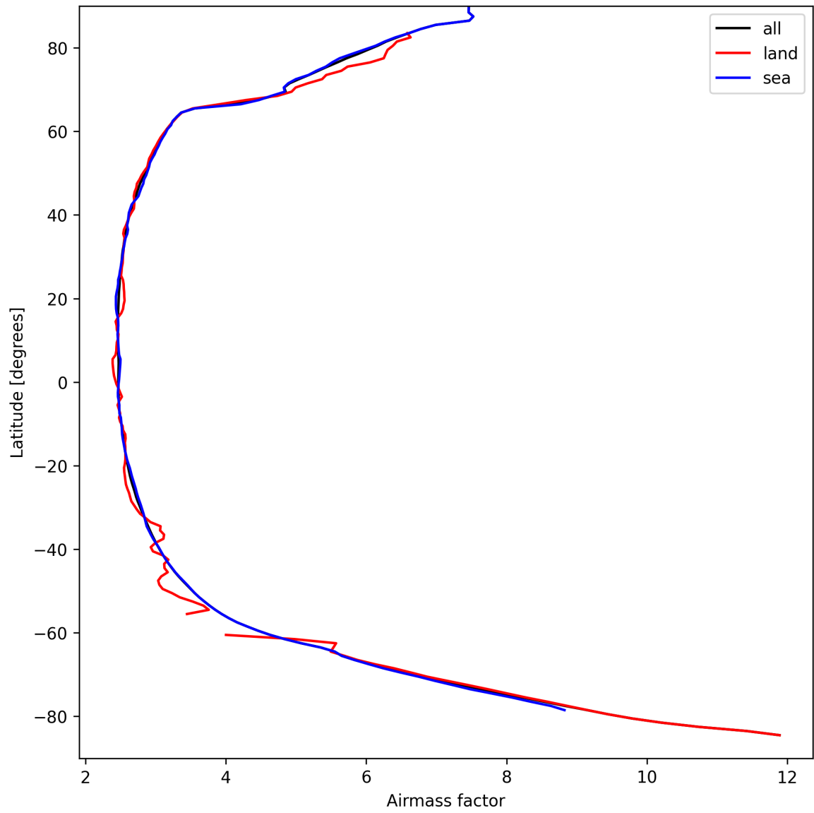
Figure 25: Zonal average of “Airmass factor” for 2025-09-10 to 2025-09-11.
