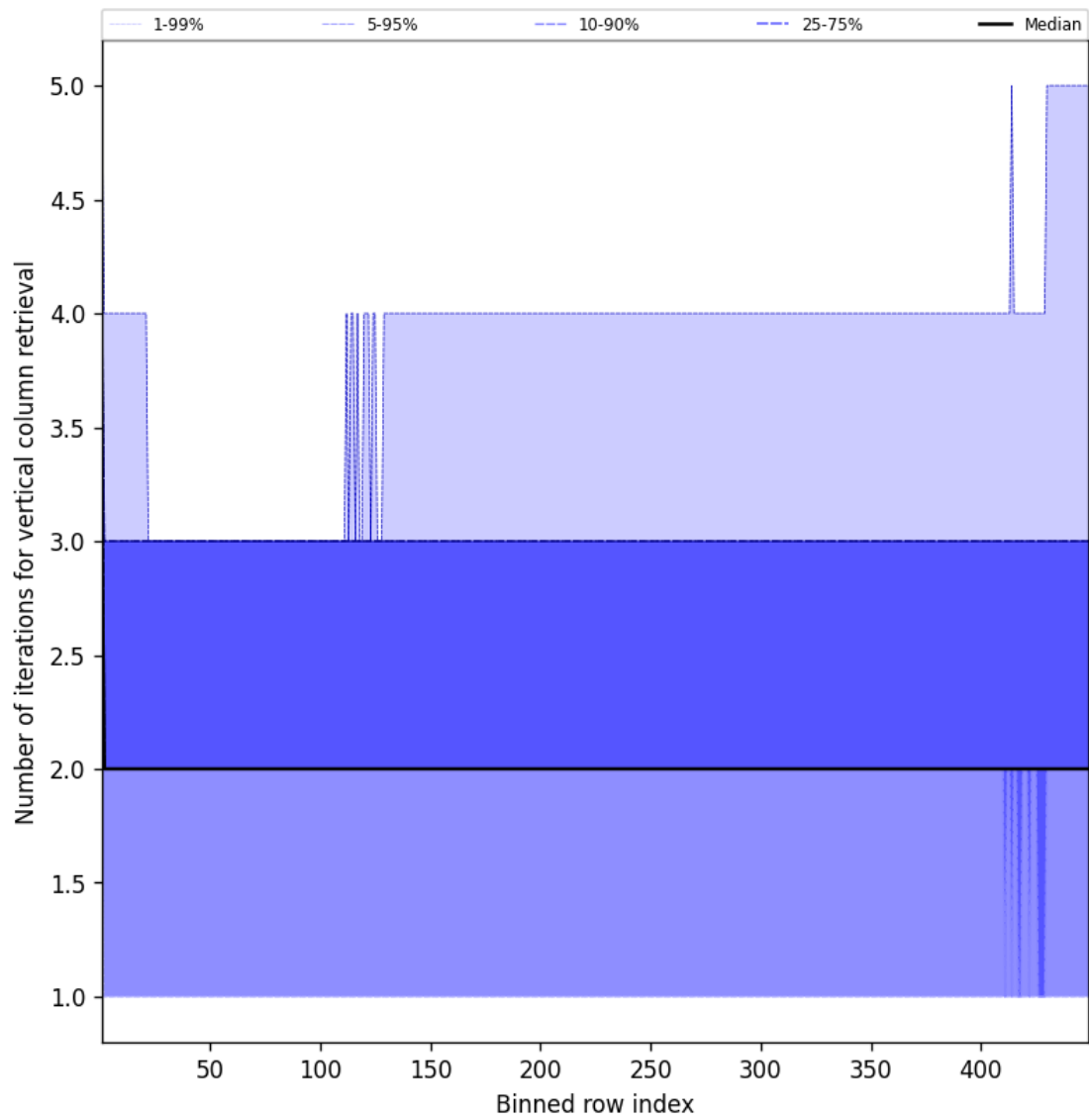
Figure 51: Along track statistics of “Number of iterations for vertical column retrieval” for 2025-09-11 to 2025-09-12
