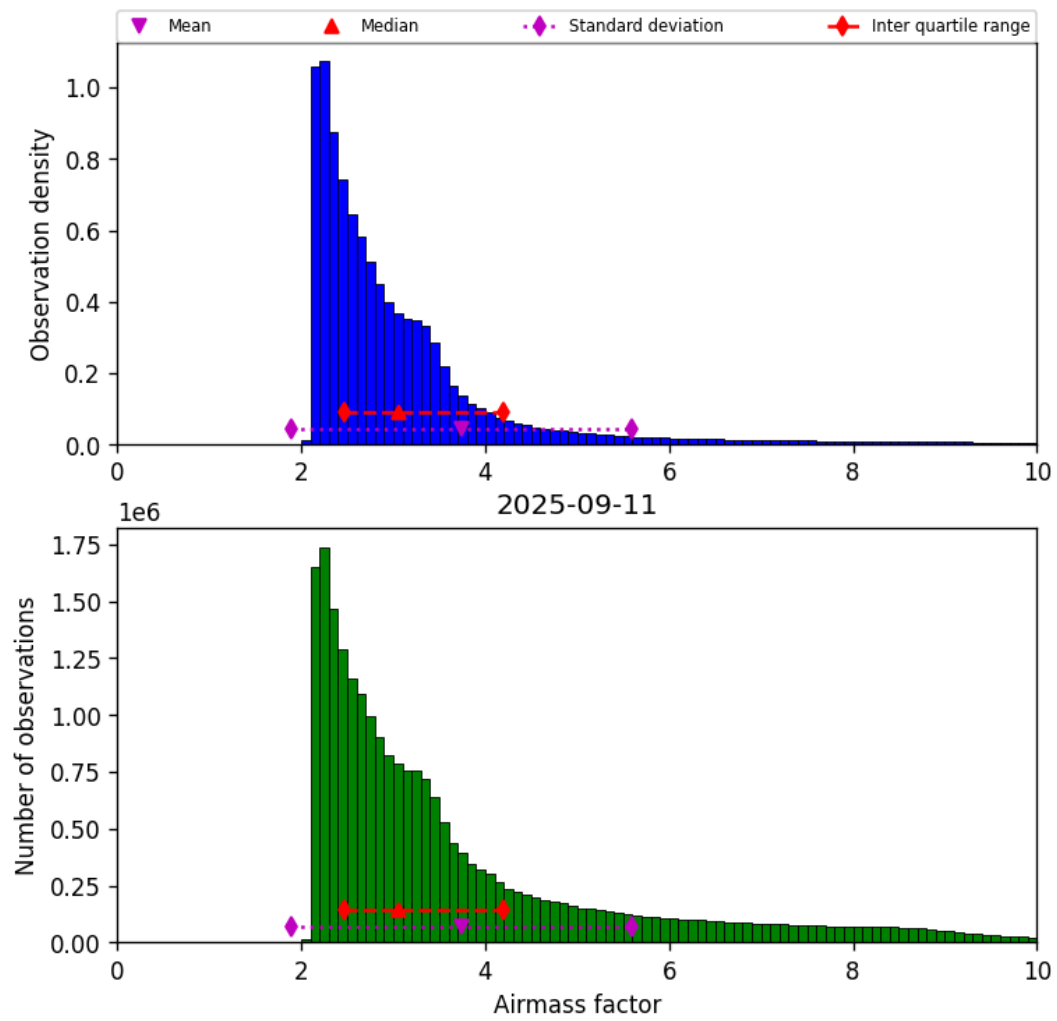
Figure 37: Histogram of “Airmass factor” for 2025-09-11 to 2025-09-12
