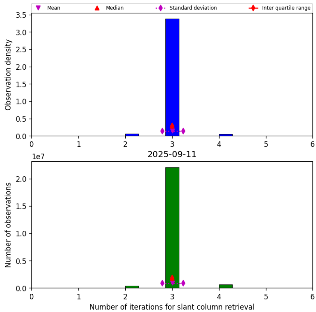
Figure 33: Histogram of “Number of iterations for slant column retrieval” for 2025-09-11 to 2025-09-12
