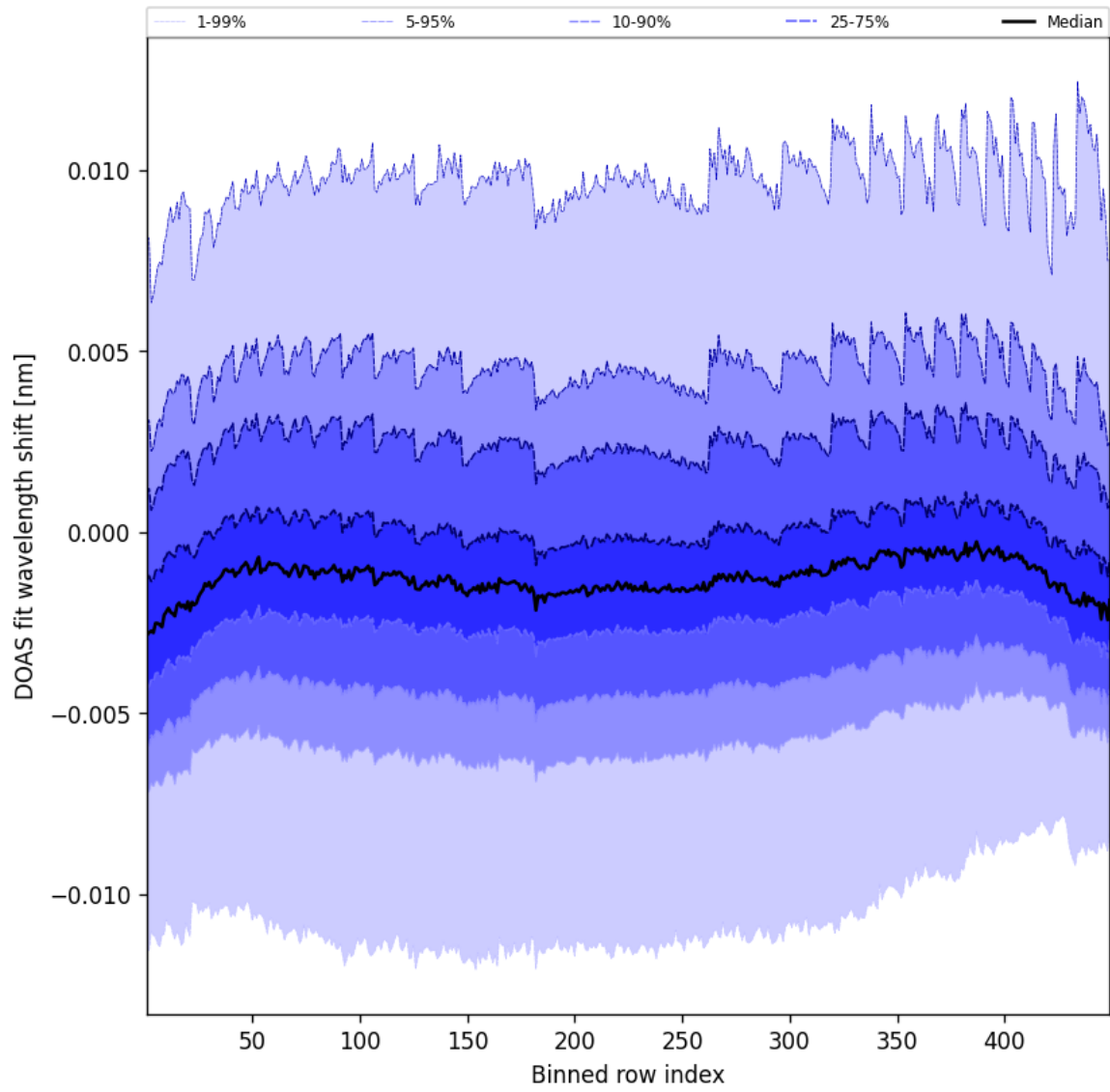
Figure 47: Along track statistics of “DOAS fit wavelength shift” for 2025-09-11 to 2025-09-12
