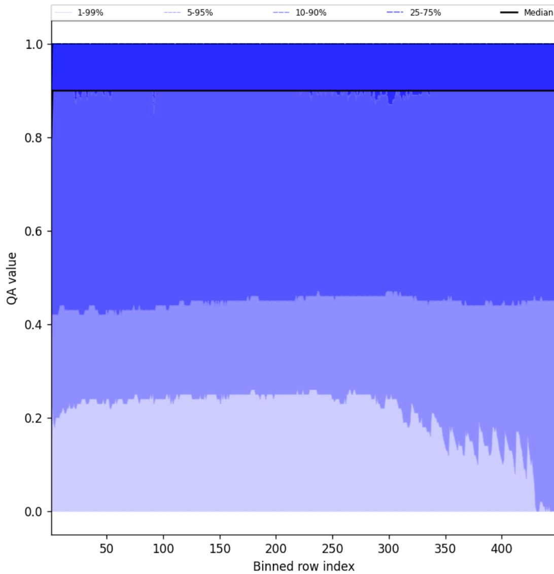
Figure 40: Along track statistics of “QA value” for 2025-09-11 to 2025-09-12
