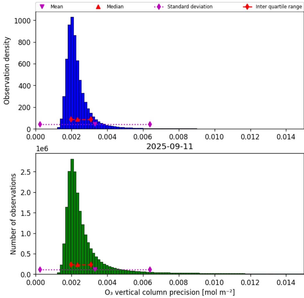
Figure 30: Histogram of “O 3 vertical column precision” for 2025-09-11 to 2025-09-12
