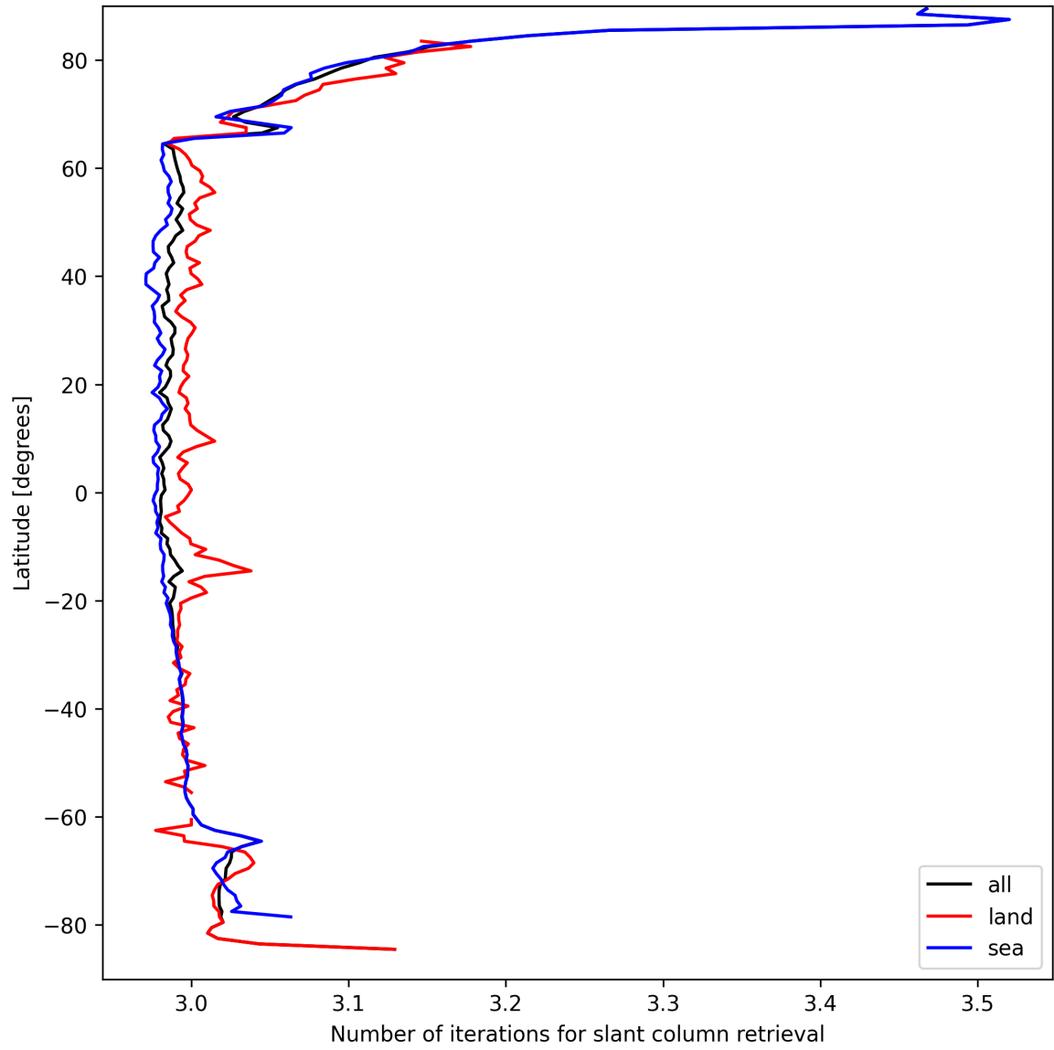
Figure 21: Zonal average of “Number of iterations for slant column retrieval” for 2025-09-11 to 2025-09-12.
