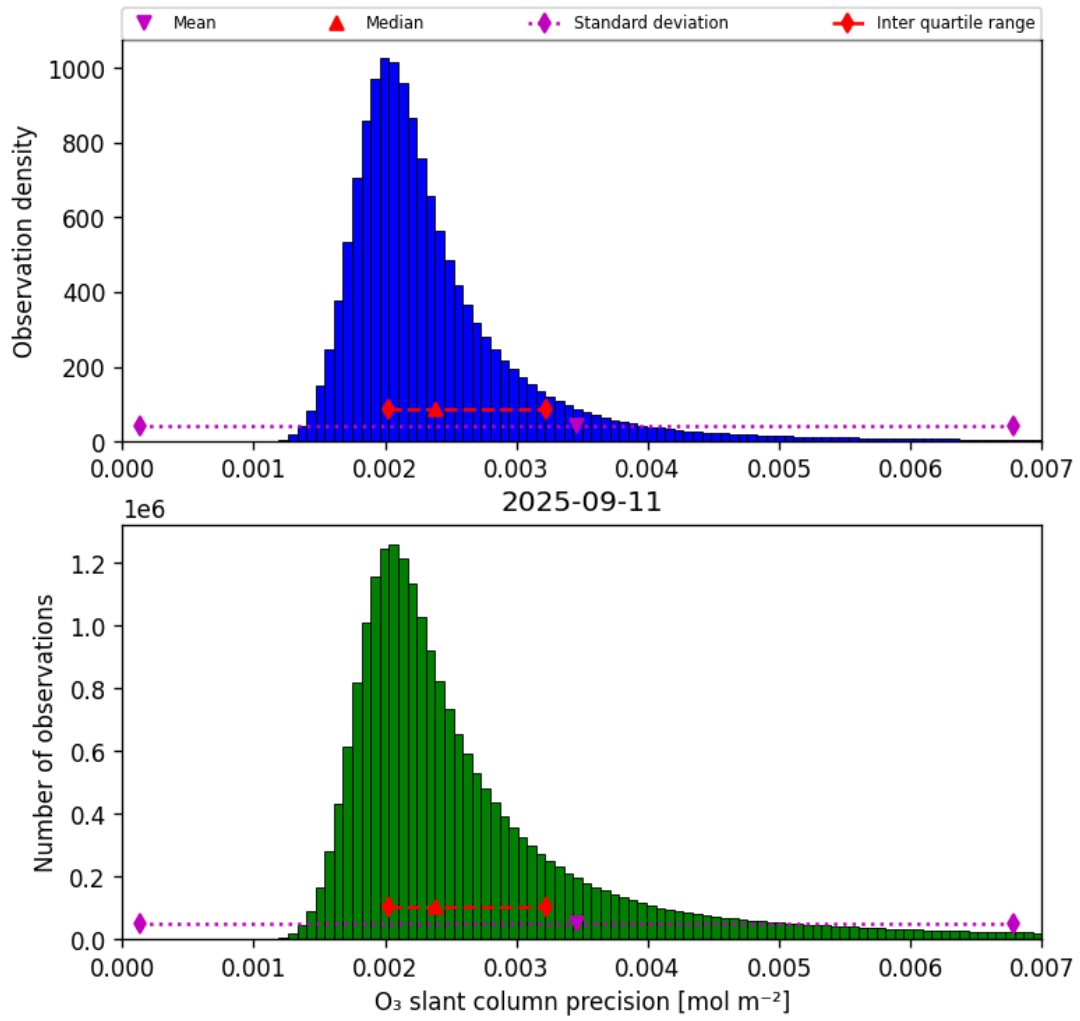
Figure 32: Histogram of “O 3 slant column precision” for 2025-09-11 to 2025-09-12
