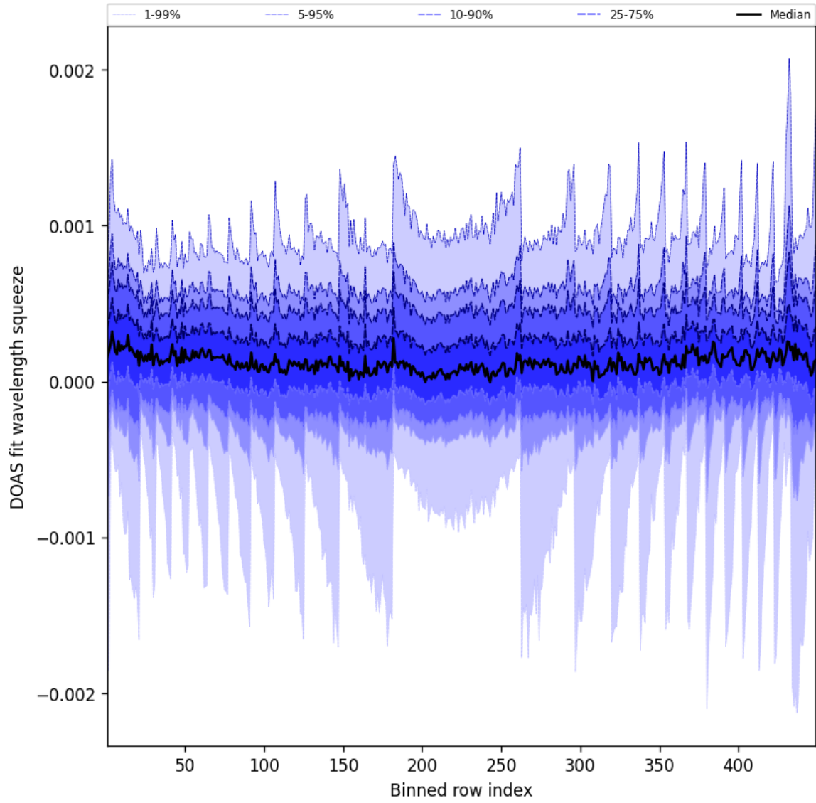
Figure 48: Along track statistics of “DOAS fit wavelength squeeze” for 2025-09-11 to 2025-09-12
