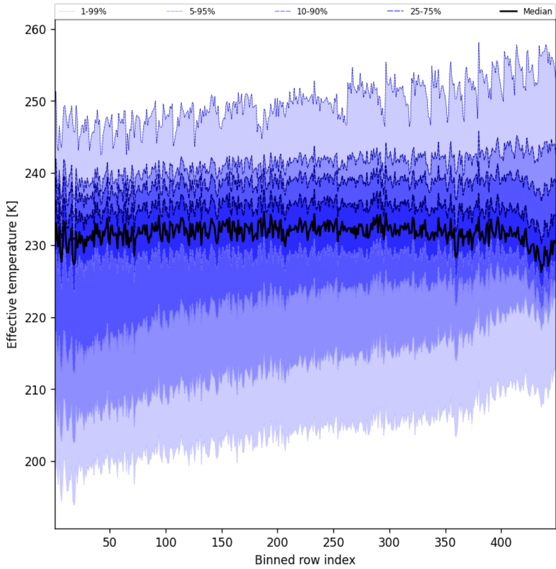
Figure 50: Along track statistics of “Effective temperature” for 2025-09-11 to 2025-09-12
