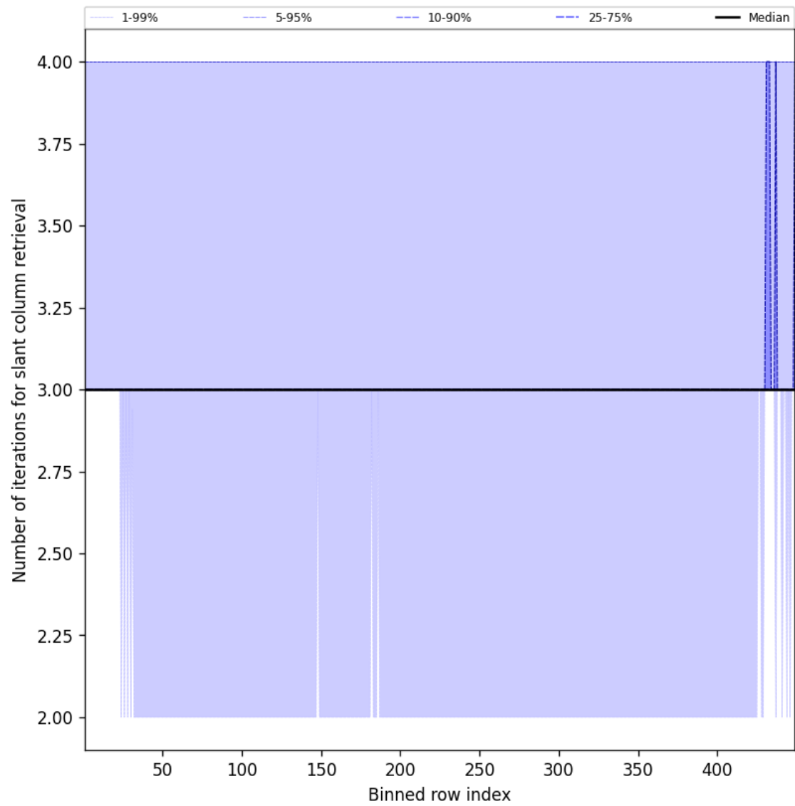
Figure 45: Along track statistics of “Number of iterations for slant column retrieval” for 2025-09-11 to 2025-09-12
