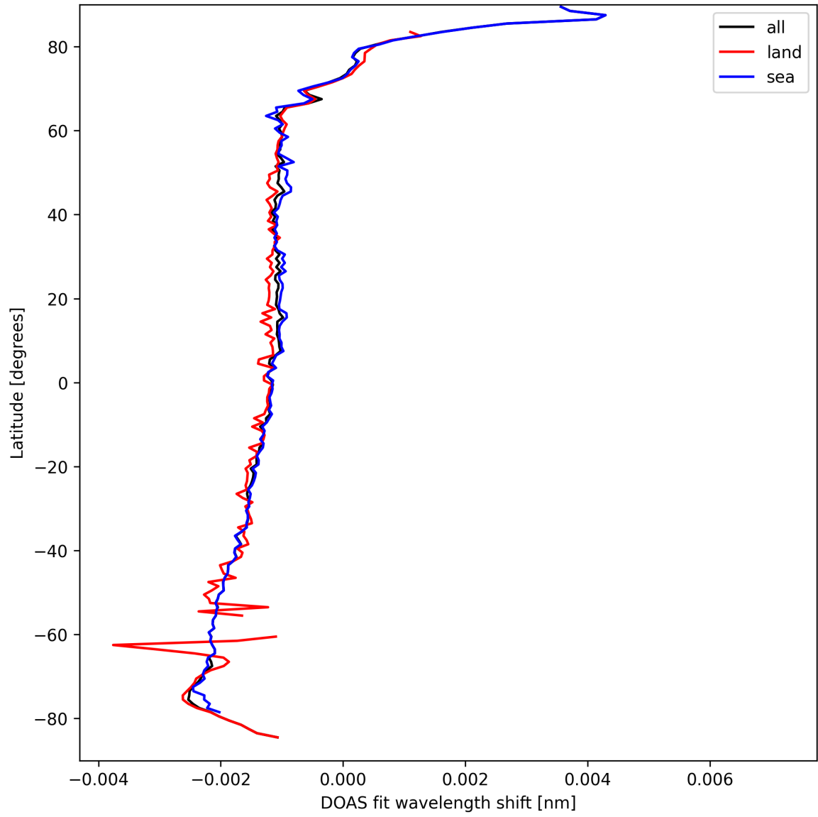
Figure 23: Zonal average of “DOAS fit wavelength shift” for 2025-09-11 to 2025-09-12.
