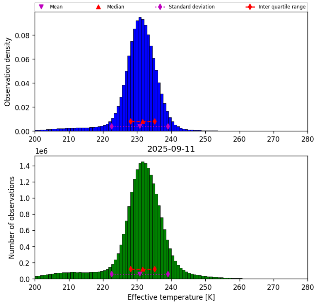
Figure 38: Histogram of “Effective temperature” for 2025-09-11 to 2025-09-12
