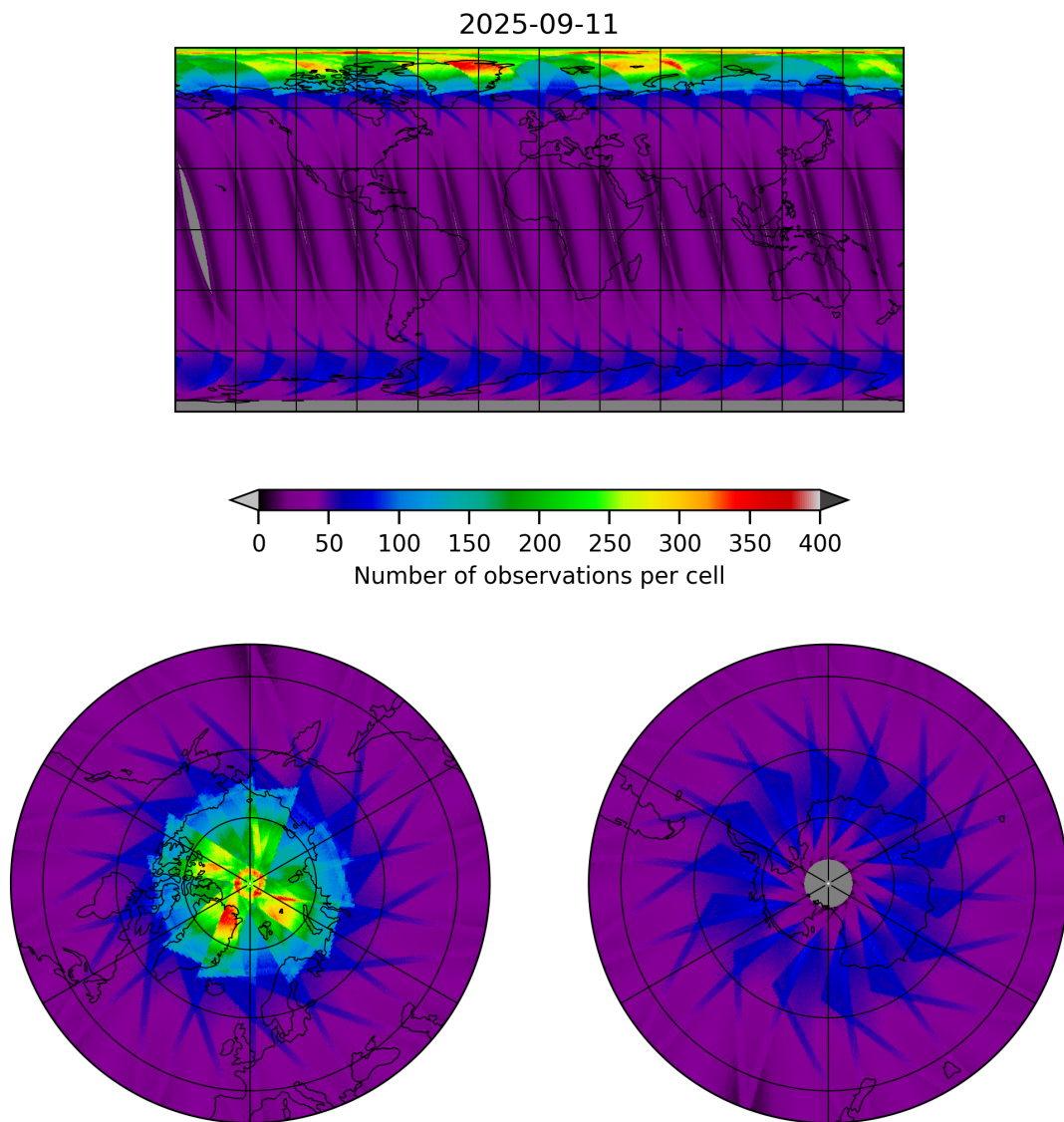
Figure 15: Map of the number of observations for 2025-09-11 to 2025-09-12
