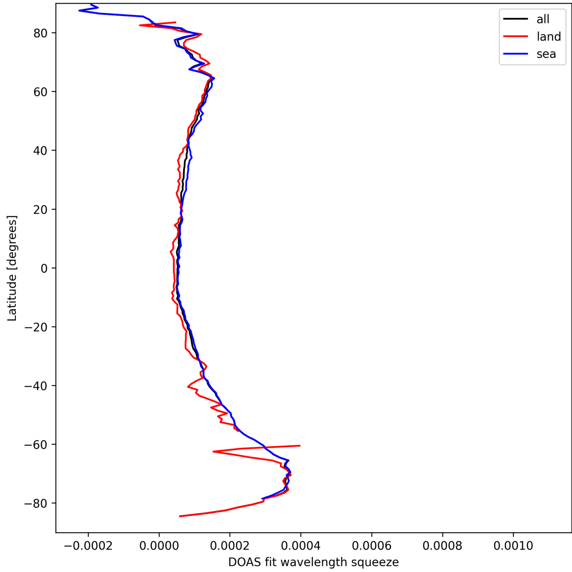
Figure 24: Zonal average of “DOAS fit wavelength squeeze” for 2025-09-11 to 2025-09-12.
