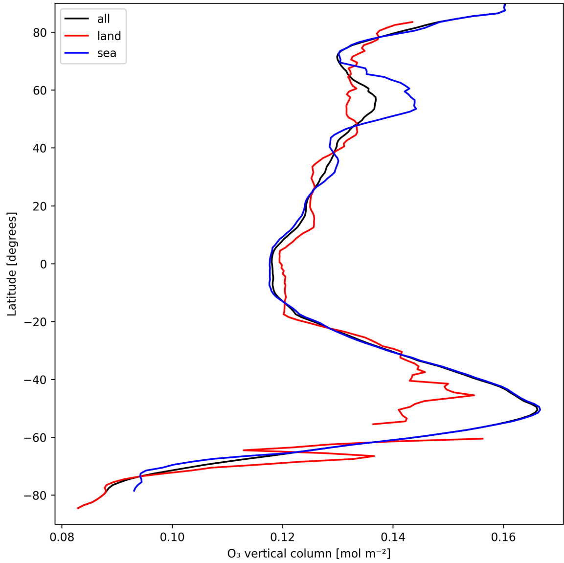
Figure 17: Zonal average of “O 3 vertical column” for 2025-09-11 to 2025-09-12.
