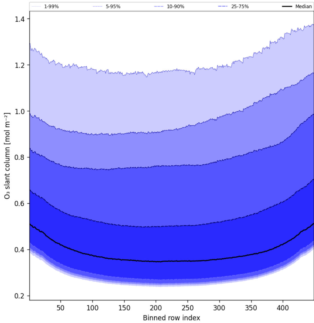
Figure 43: Along track statistics of “O 3 slant column” for 2025-09-11 to 2025-09-12
