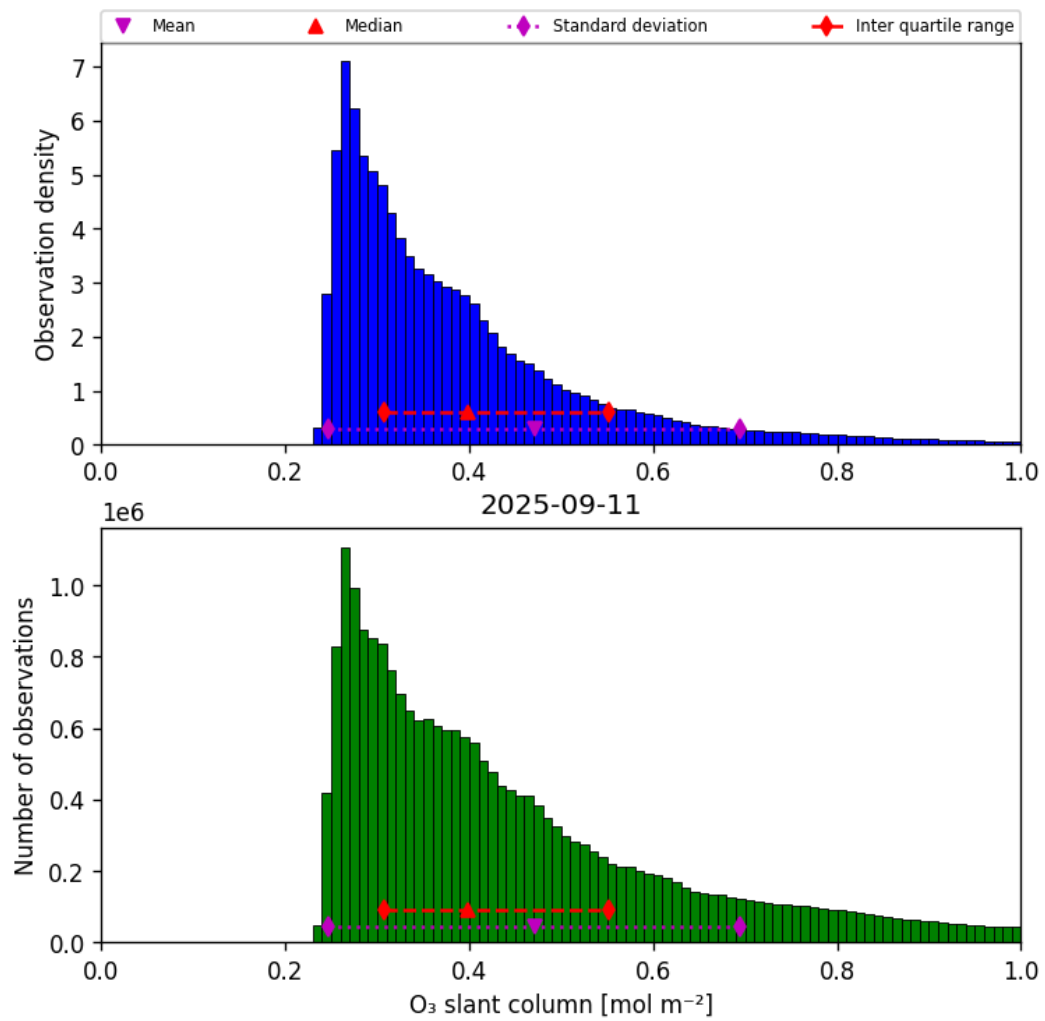
Figure 31: Histogram of “O 3 slant column” for 2025-09-11 to 2025-09-12
