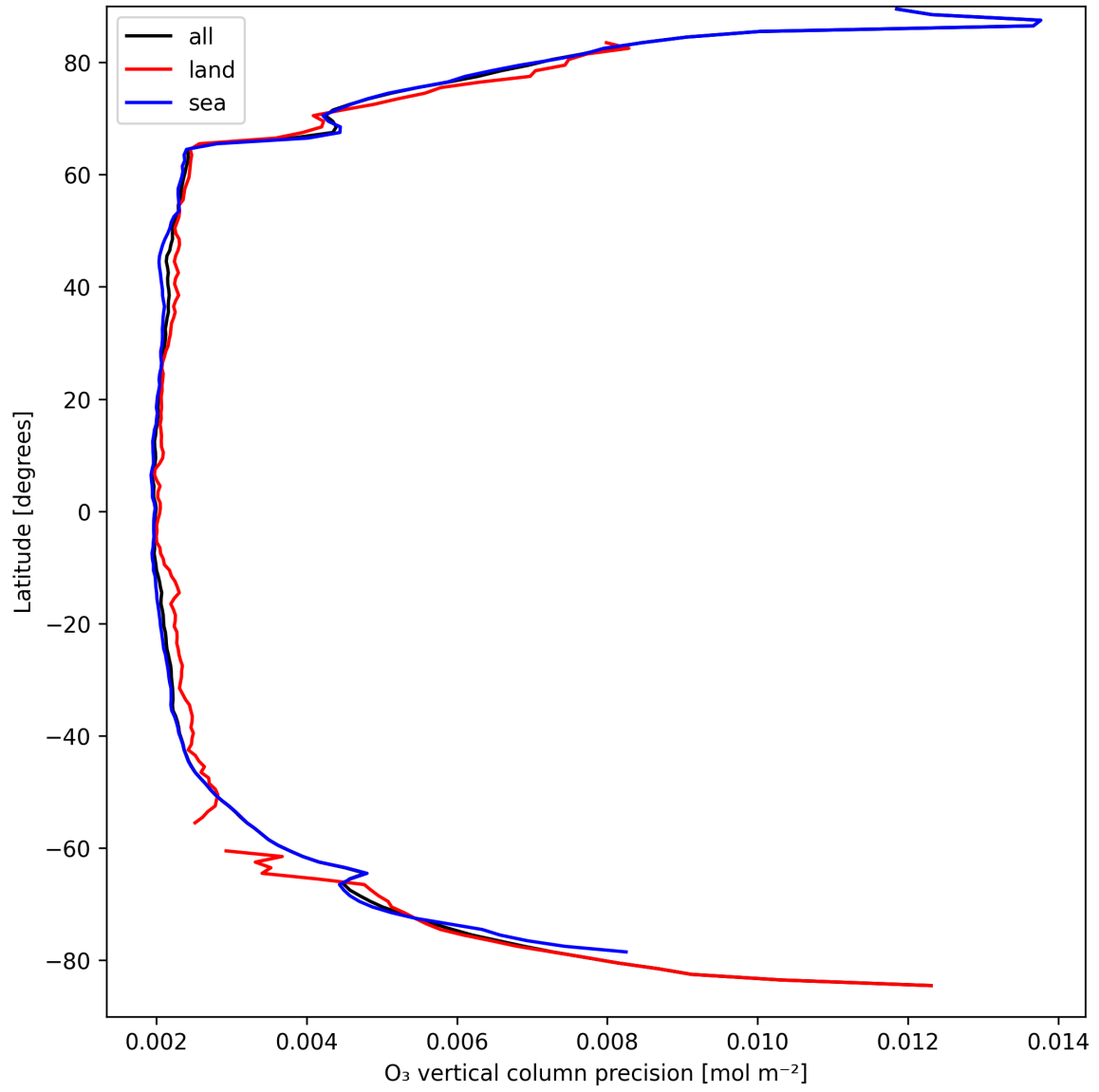
Figure 18: Zonal average of “O 3 vertical column precision” for 2025-09-11 to 2025-09-12.
