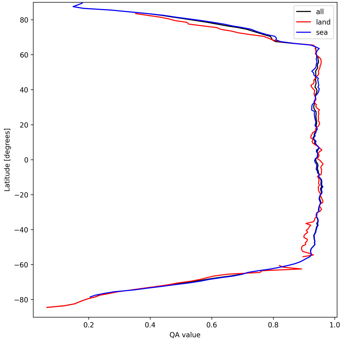
Figure 16: Zonal average of “QA value” for 2025-09-11 to 2025-09-12.
