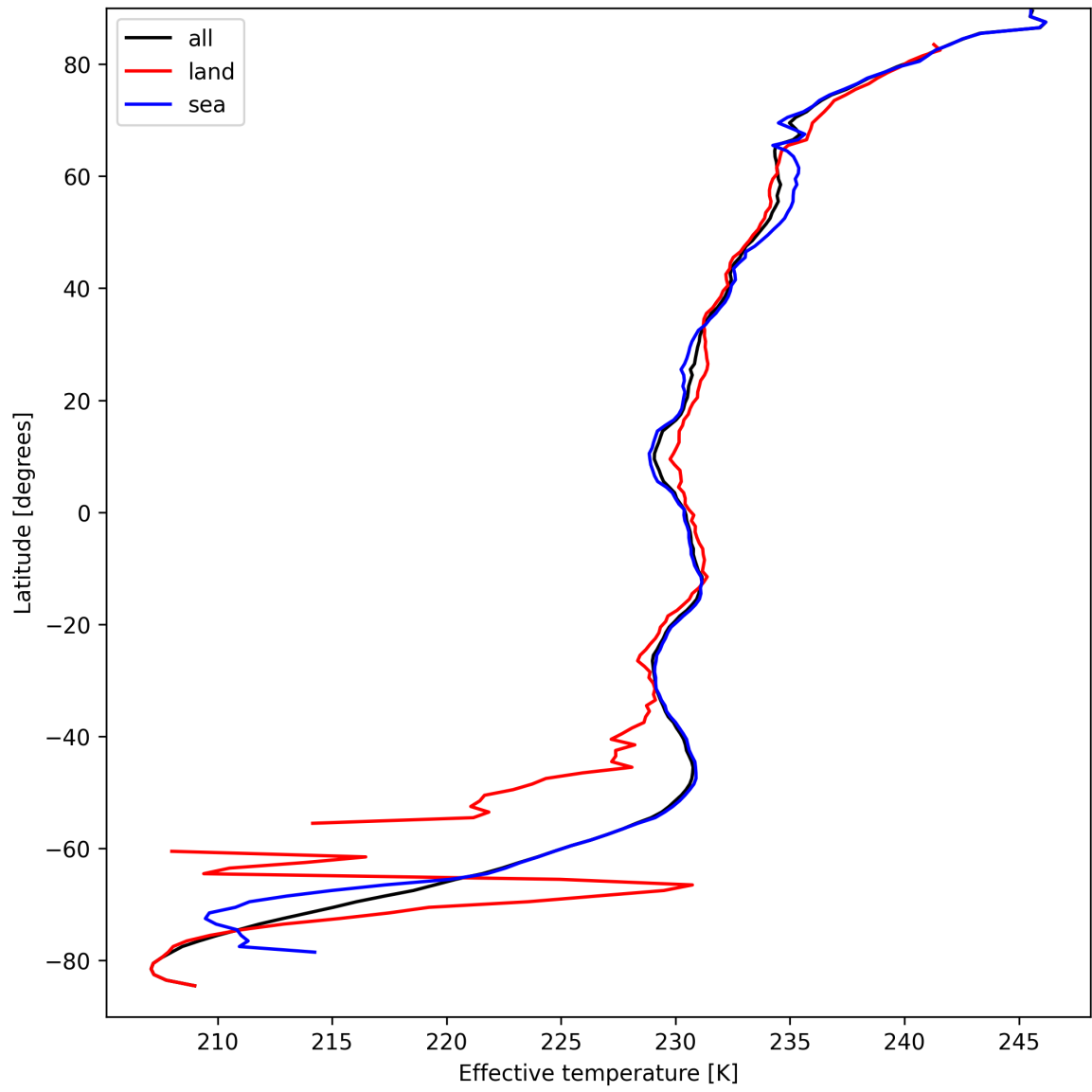
Figure 26: Zonal average of "Effective temperature" for 2025-09-11 to 2025-09-12.
