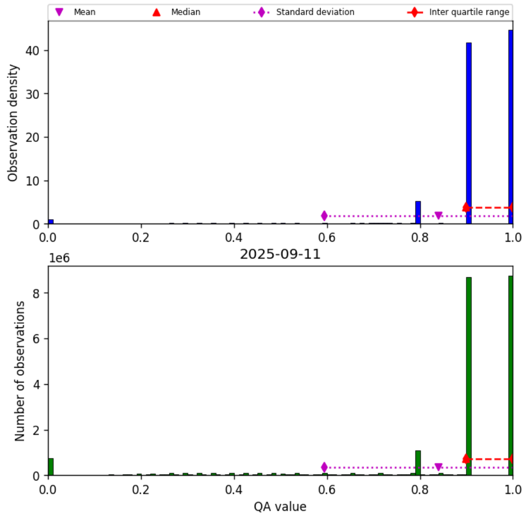
Figure 28: Histogram of “QA value” for 2025-09-11 to 2025-09-12
