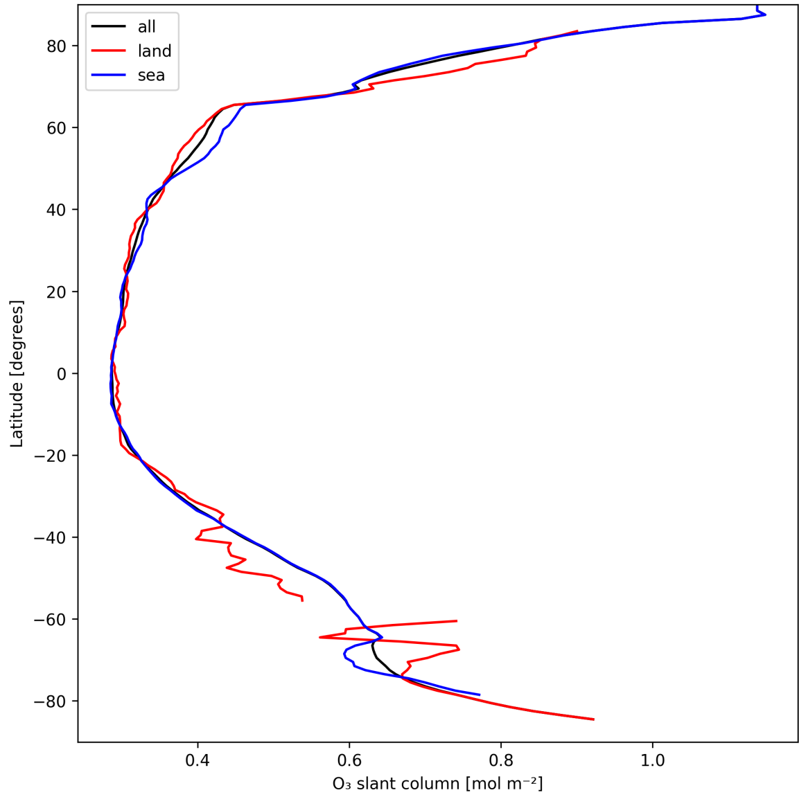
Figure 19: Zonal average of “O 3 slant column” for 2025-09-11 to 2025-09-12.
