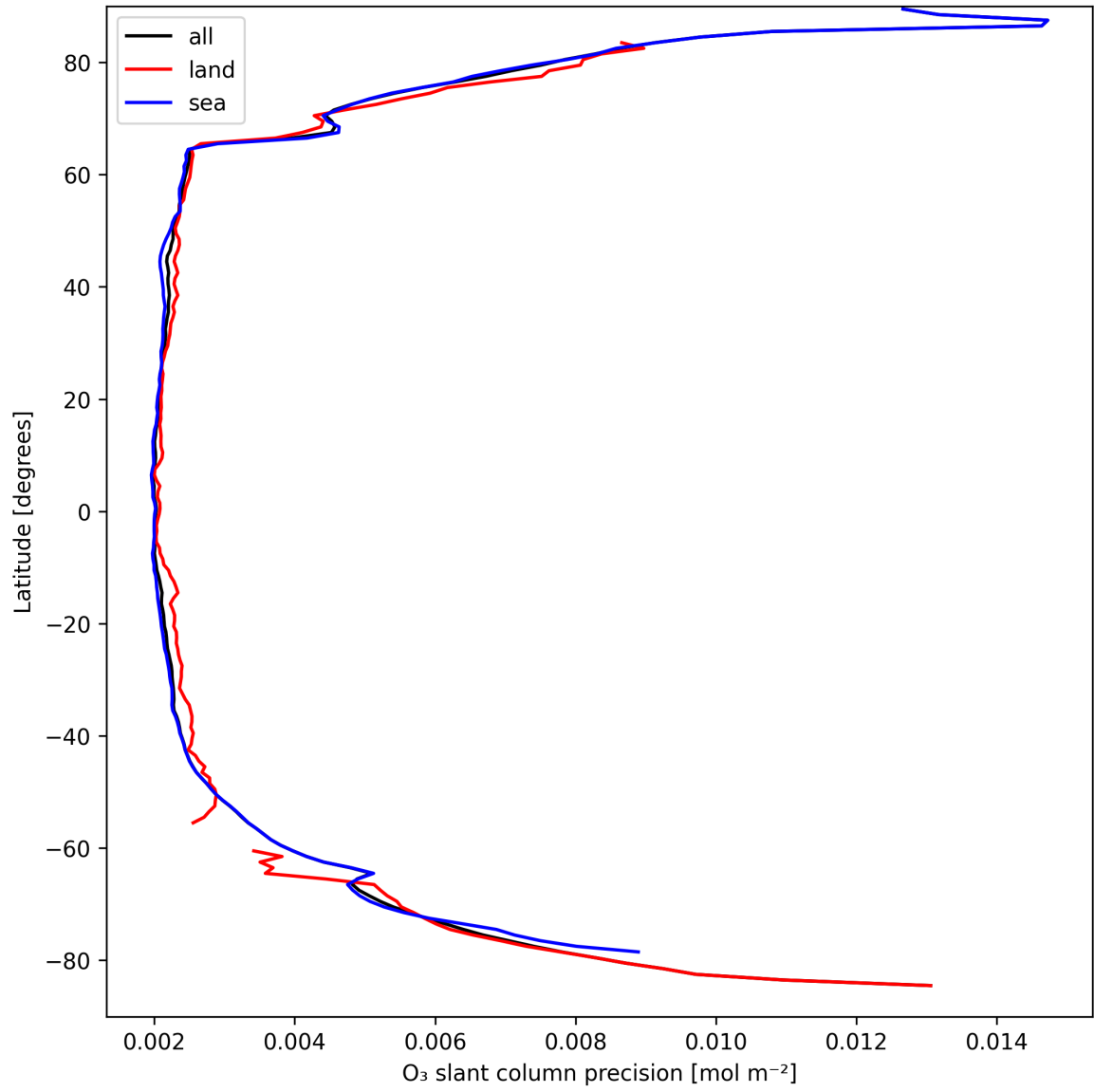
Figure 20: Zonal average of “O 3 slant column precision” for 2025-09-11 to 2025-09-12.
