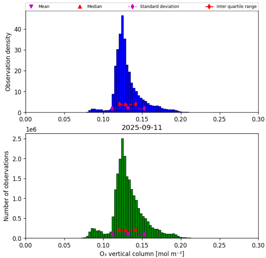
Figure 29: Histogram of “O 3 vertical column” for 2025-09-11 to 2025-09-12
