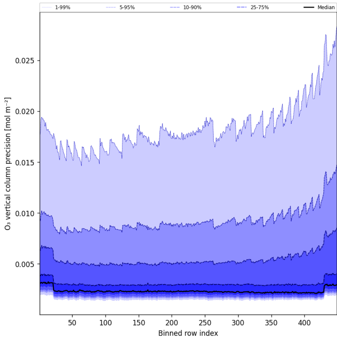
Figure 42: Along track statistics of “O 3 vertical column precision” for 2025-09-11 to 2025-09-12
