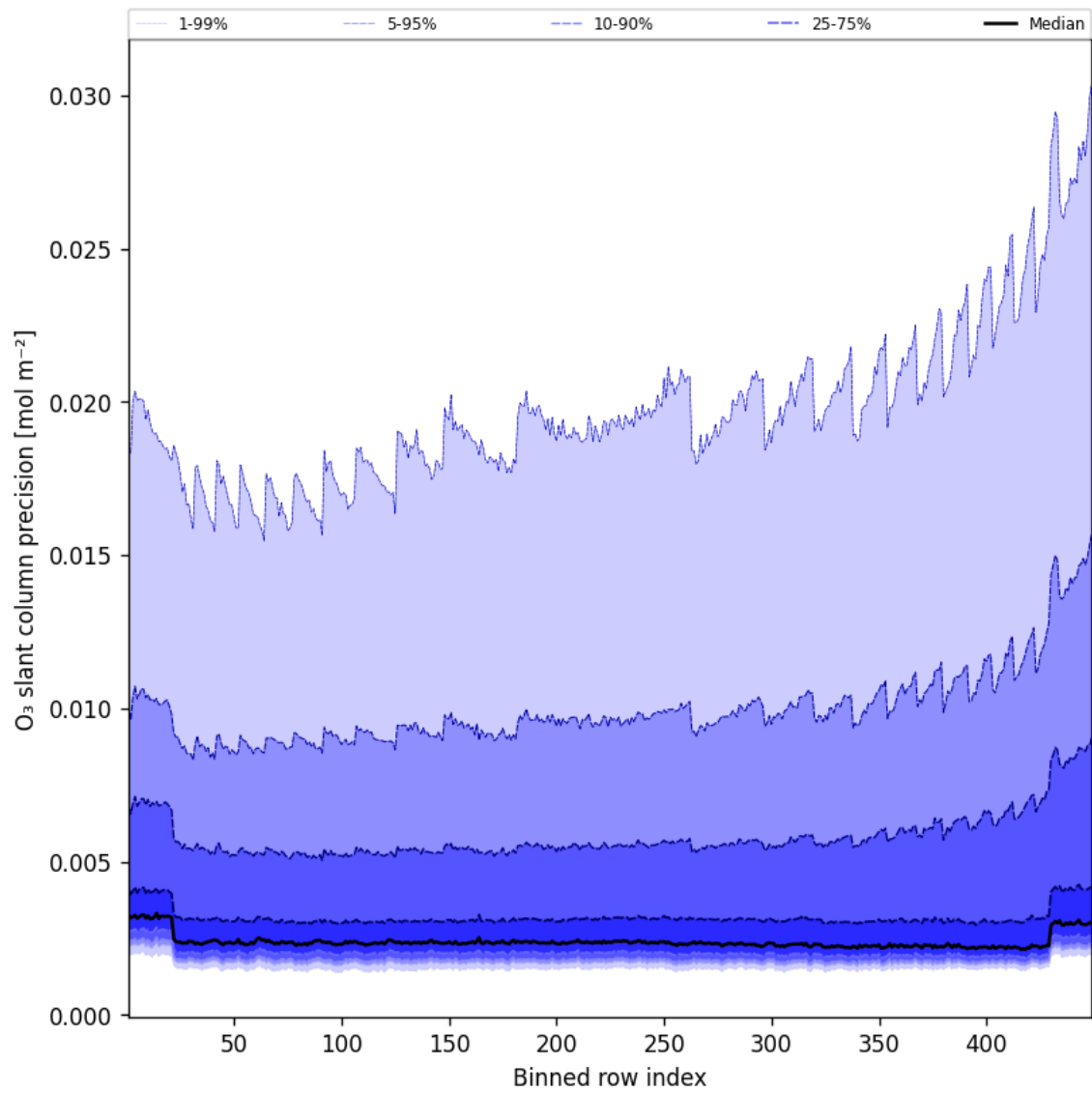
Figure 44: Along track statistics of “O 3 slant column precision” for 2025-09-11 to 2025-09-12
