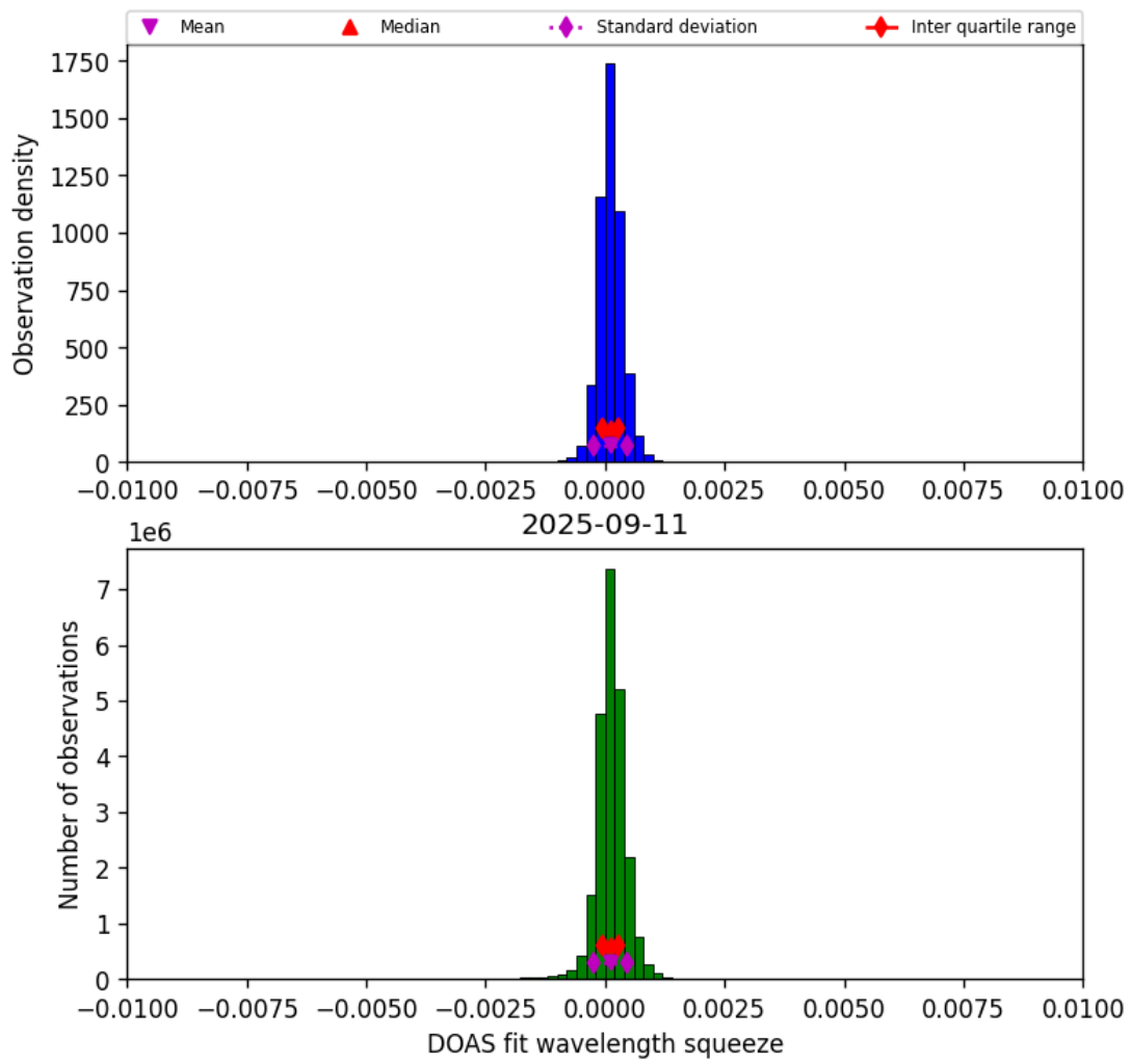
Figure 36: Histogram of “DOAS fit wavelength squeeze” for 2025-09-11 to 2025-09-12
