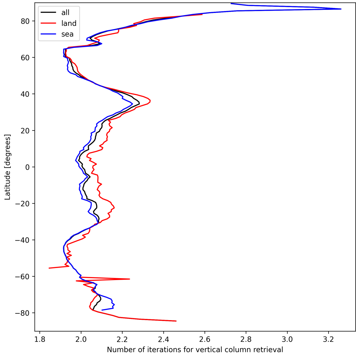
Figure 27: Zonal average of “Number of iterations for vertical column retrieval” for 2025-09-11 to 2025-09-12.
