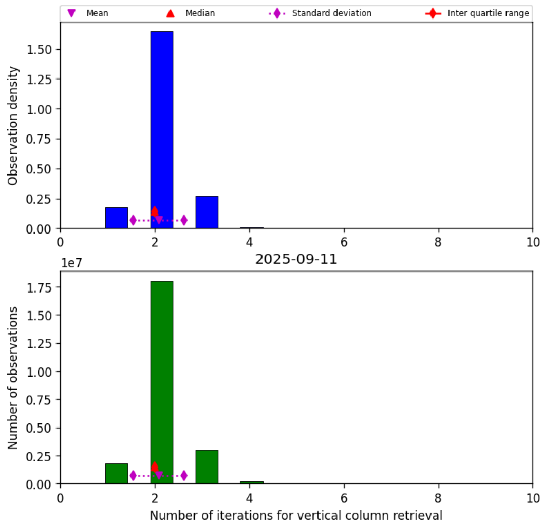
Figure 39: Histogram of “Number of iterations for vertical column retrieval” for 2025-09-11 to 2025-09-12
