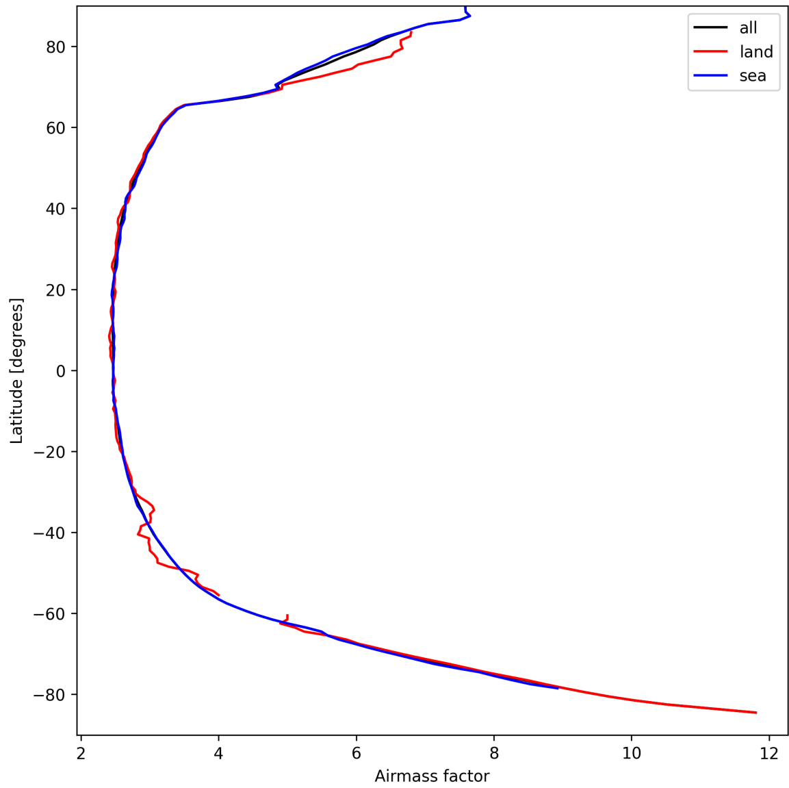
Figure 25: Zonal average of “Airmass factor” for 2025-09-11 to 2025-09-12.
