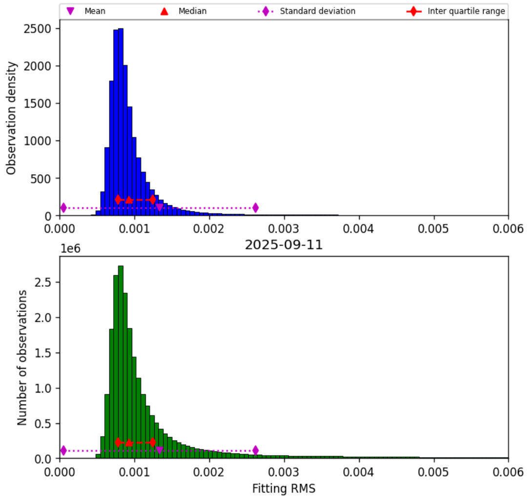
Figure 34: Histogram of “Fitting RMS” for 2025-09-11 to 2025-09-12
