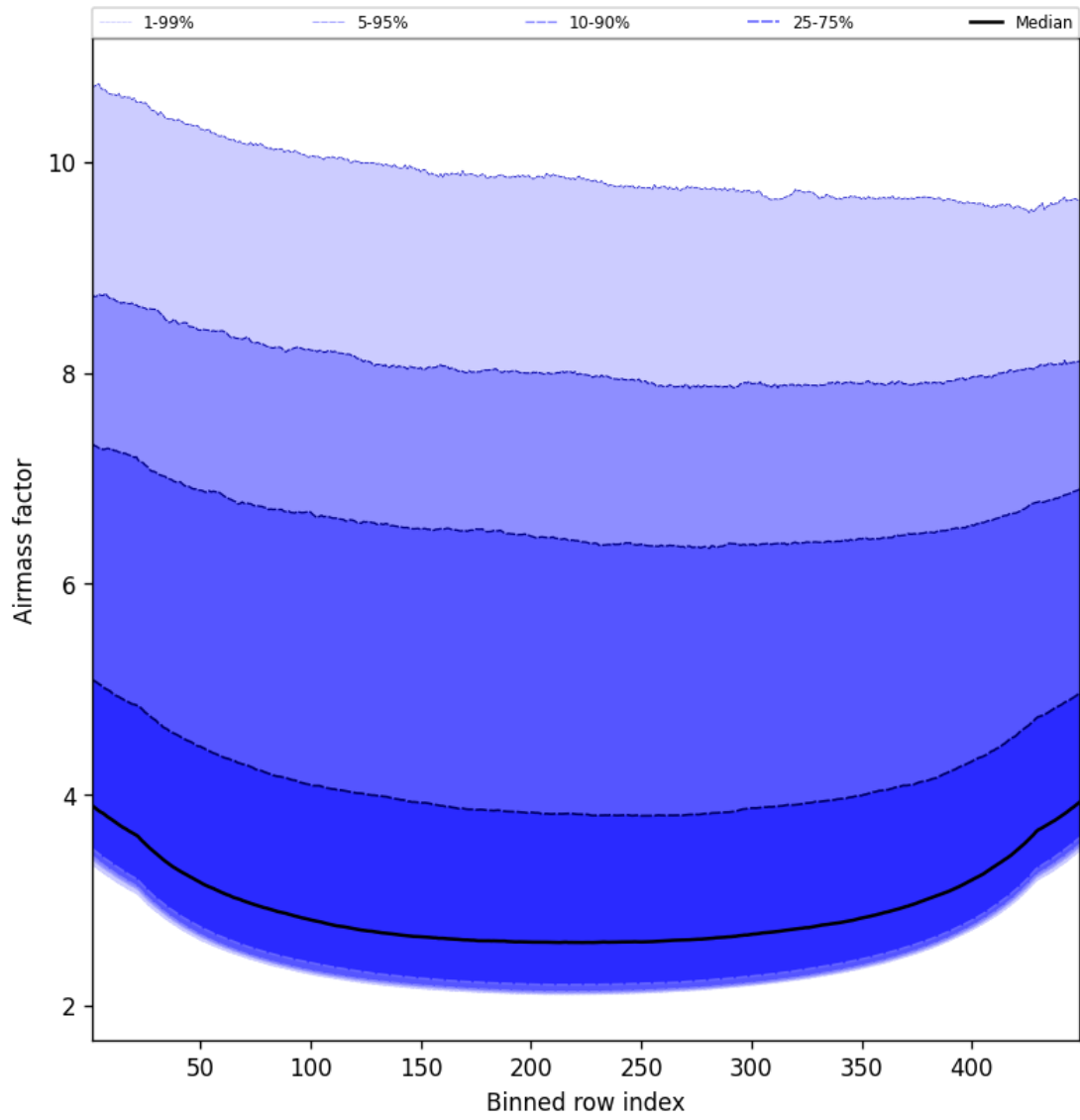
Figure 49: Along track statistics of “Airmass factor” for 2025-09-11 to 2025-09-12
