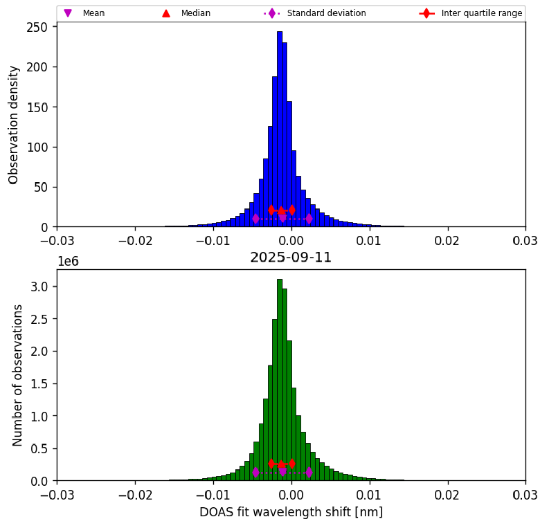
Figure 35: Histogram of “DOAS fit wavelength shift” for 2025-09-11 to 2025-09-12
