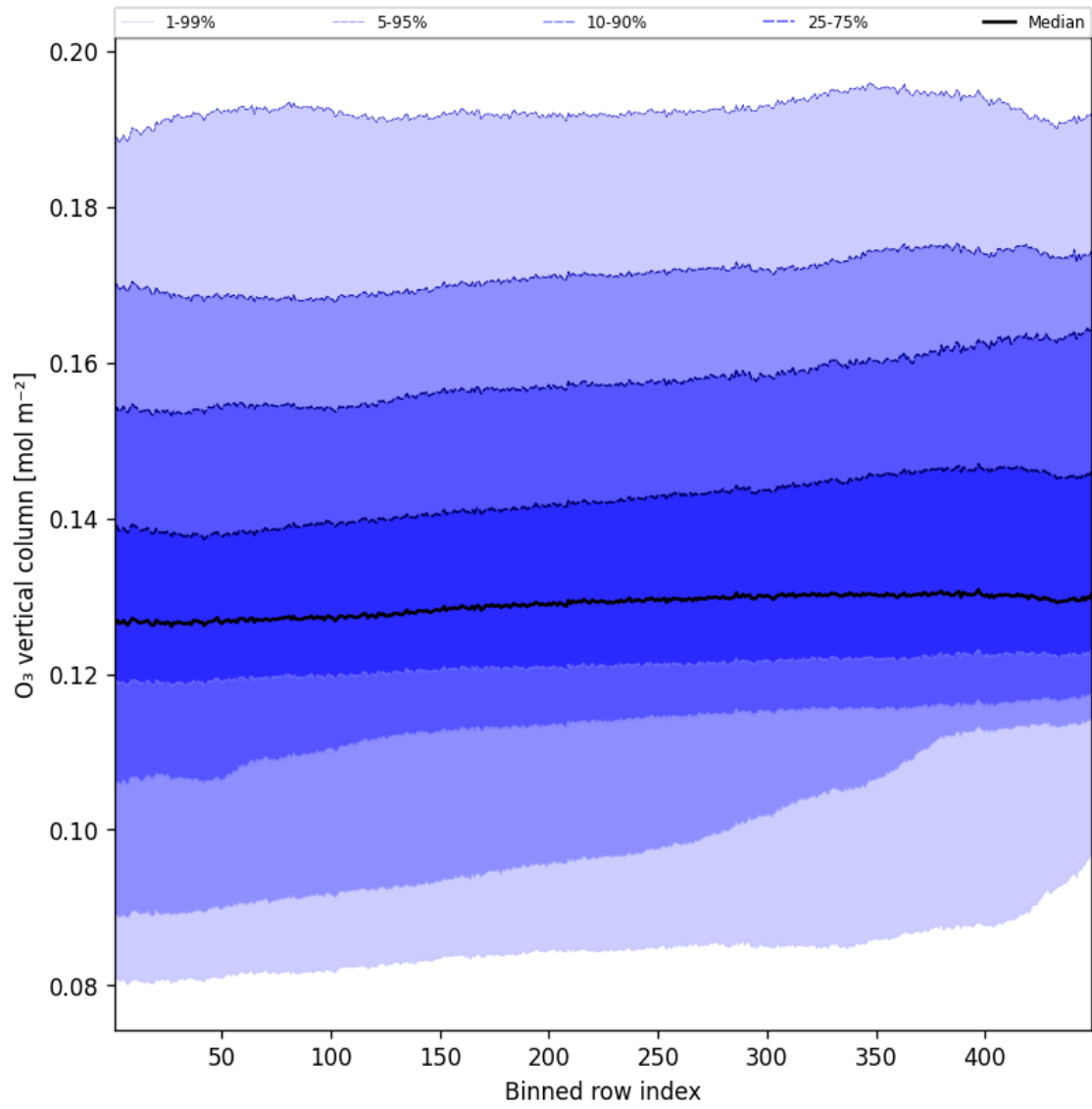
Figure 41: Along track statistics of “O 3 vertical column” for 2025-09-11 to 2025-09-12
