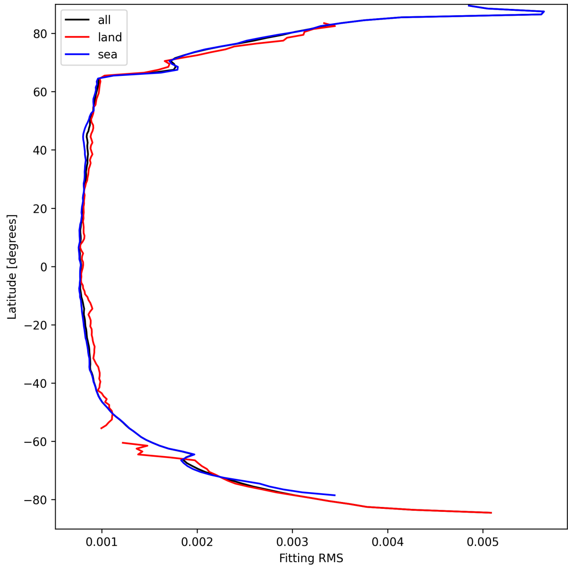
Figure 22: Zonal average of “Fitting RMS” for 2025-09-11 to 2025-09-12.
