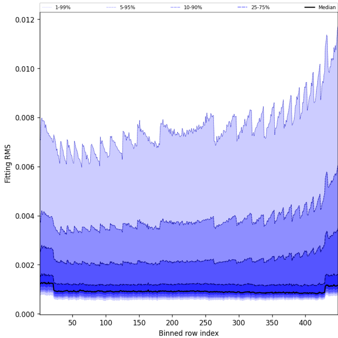
Figure 46: Along track statistics of “Fitting RMS” for 2025-09-11 to 2025-09-12
