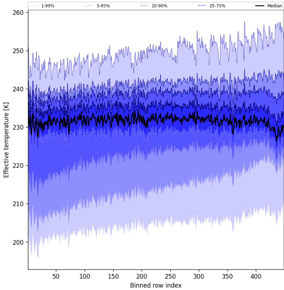
Figure 50: Along track statistics of “Effective temperature” for 2025-09-12 to 2025-09-13
