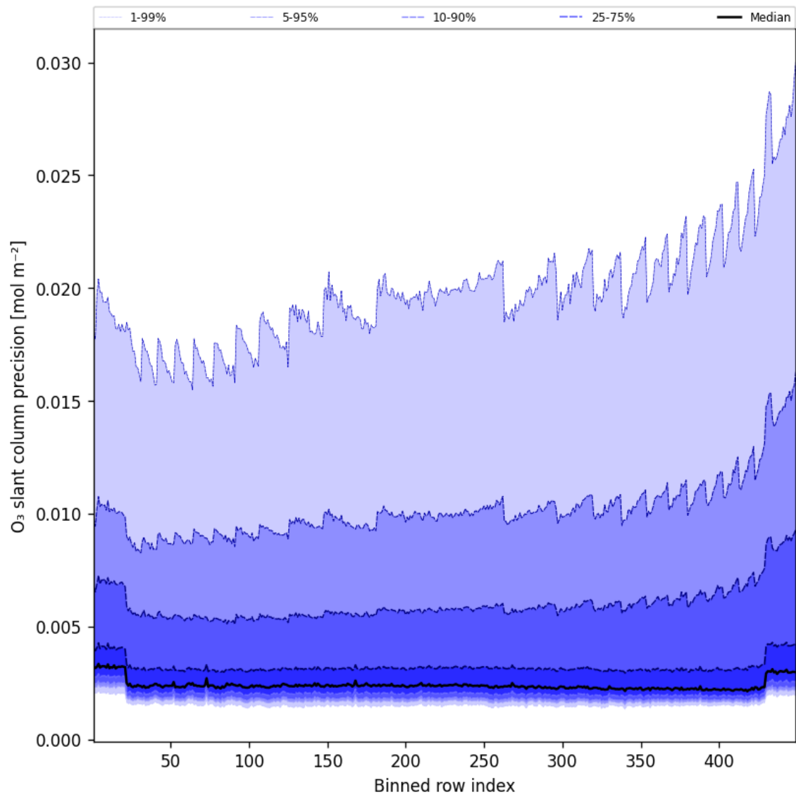
Figure 44: Along track statistics of “O 3 slant column precision” for 2025-09-12 to 2025-09-13
