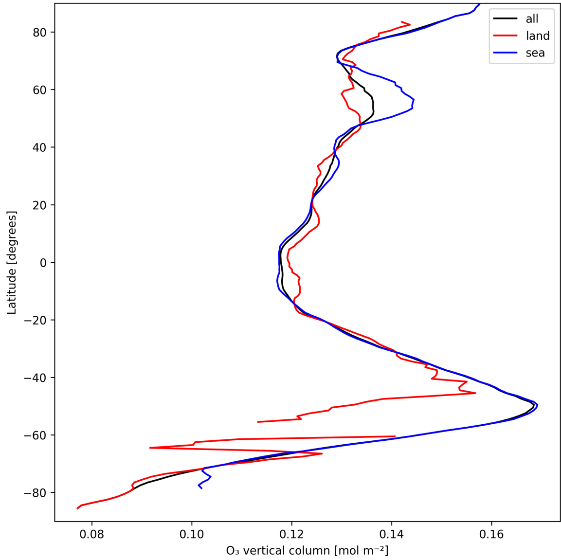
Figure 17: Zonal average of “O 3 vertical column” for 2025-09-12 to 2025-09-13.
