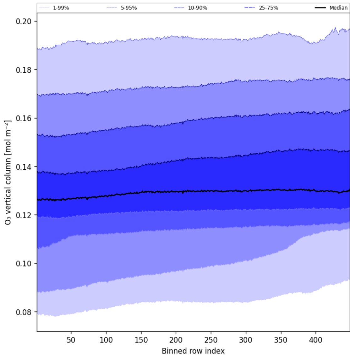
Figure 41: Along track statistics of “O 3 vertical column” for 2025-09-12 to 2025-09-13
