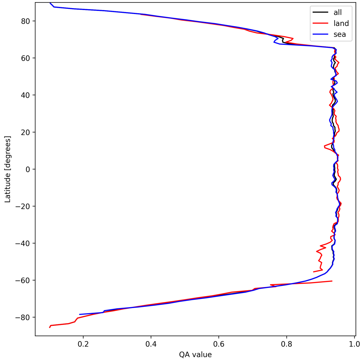
Figure 16: Zonal average of “QA value” for 2025-09-12 to 2025-09-13.
