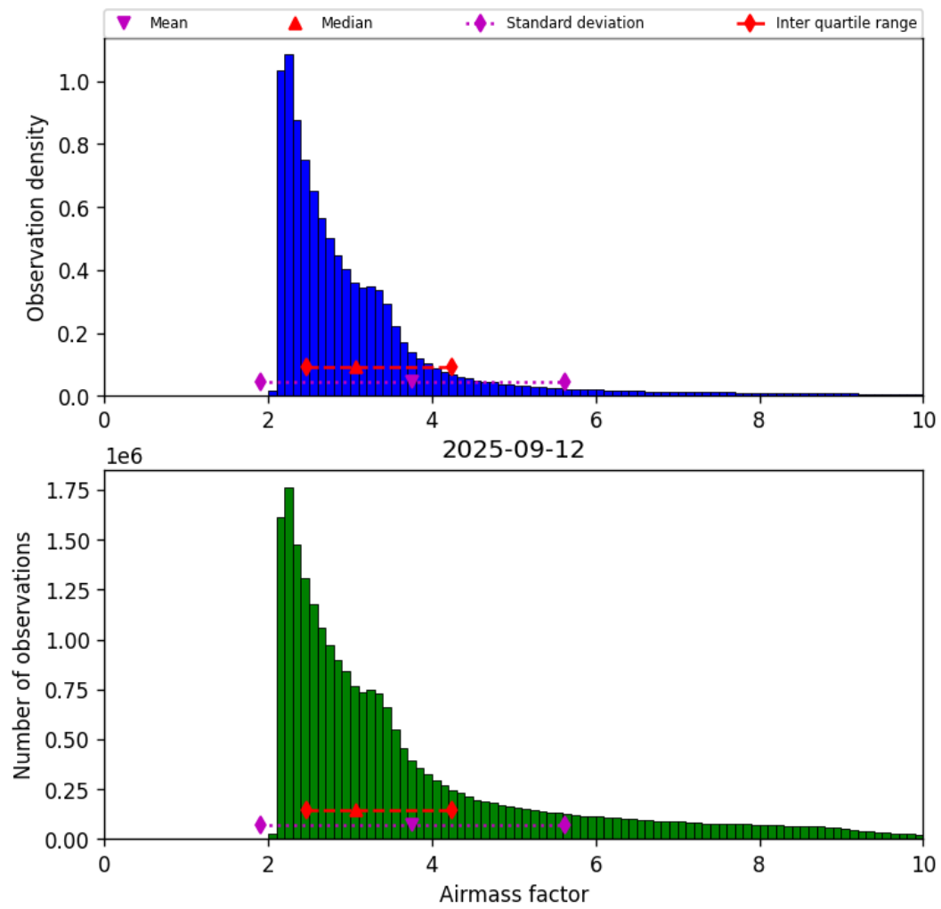
Figure 37: Histogram of “Airmass factor” for 2025-09-12 to 2025-09-13
