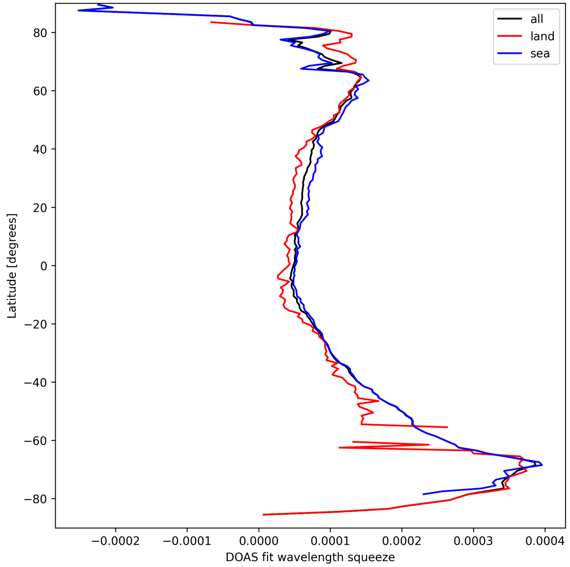
Figure 24: Zonal average of "DOAS fit wavelength squeeze" for 2025-09-12 to 2025-09-13.
