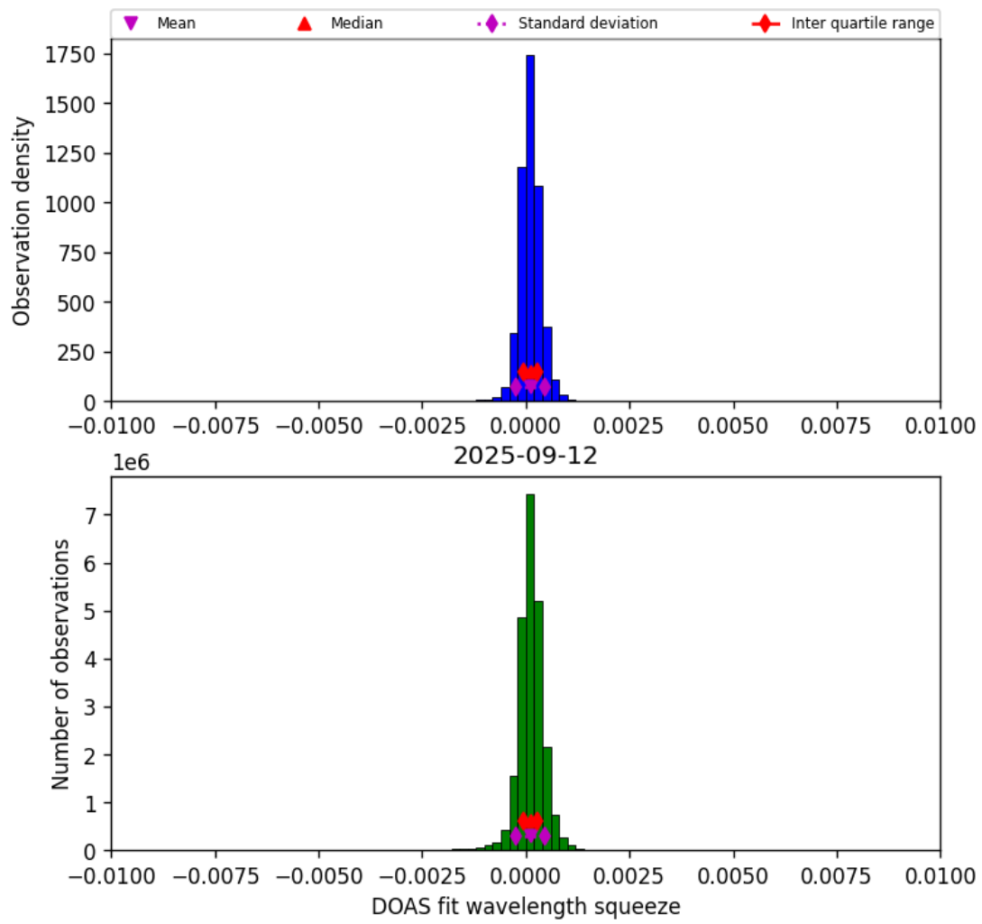
Figure 36: Histogram of “DOAS fit wavelength squeeze” for 2025-09-12 to 2025-09-13
