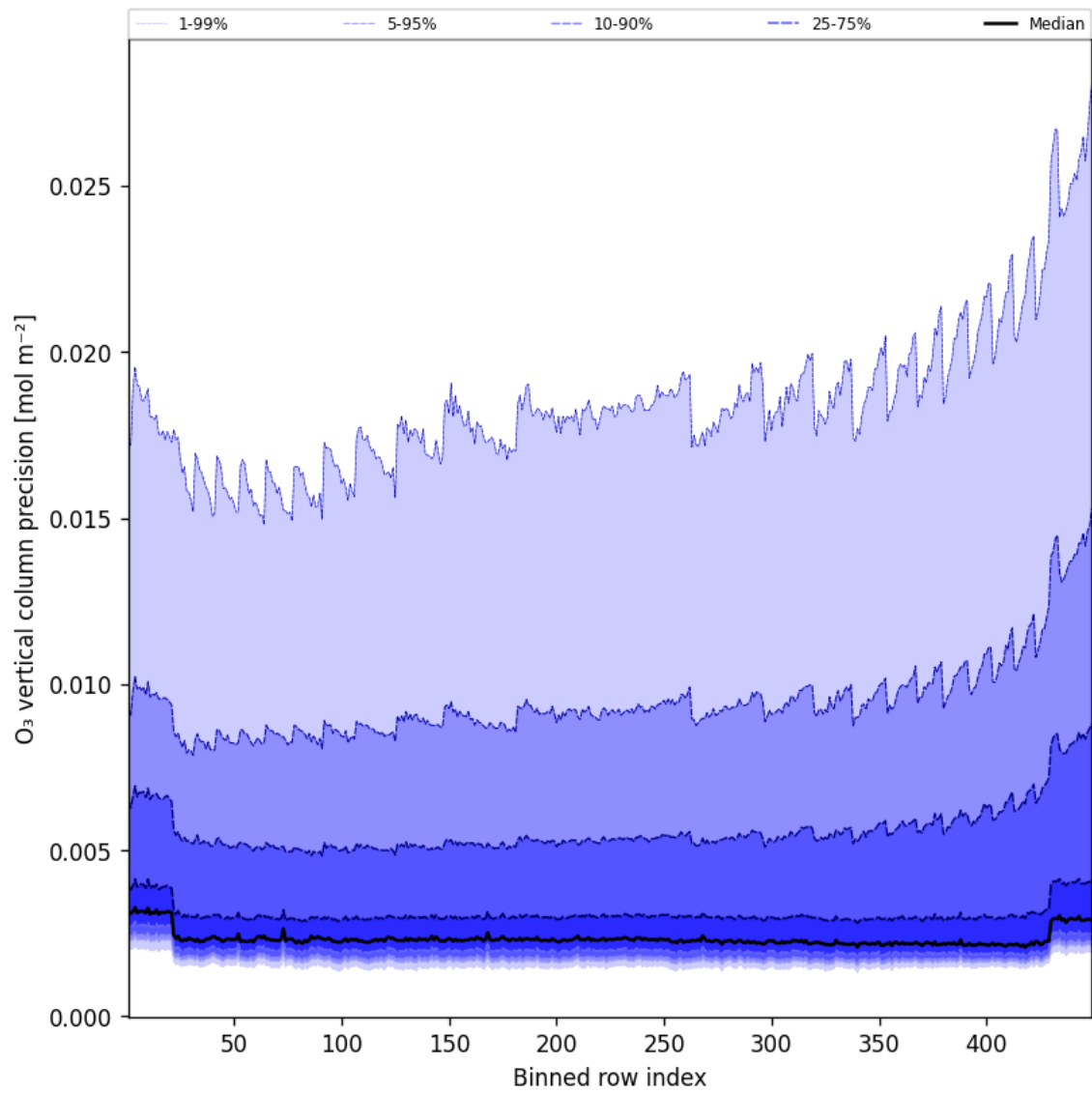
Figure 42: Along track statistics of “O 3 vertical column precision” for 2025-09-12 to 2025-09-13
