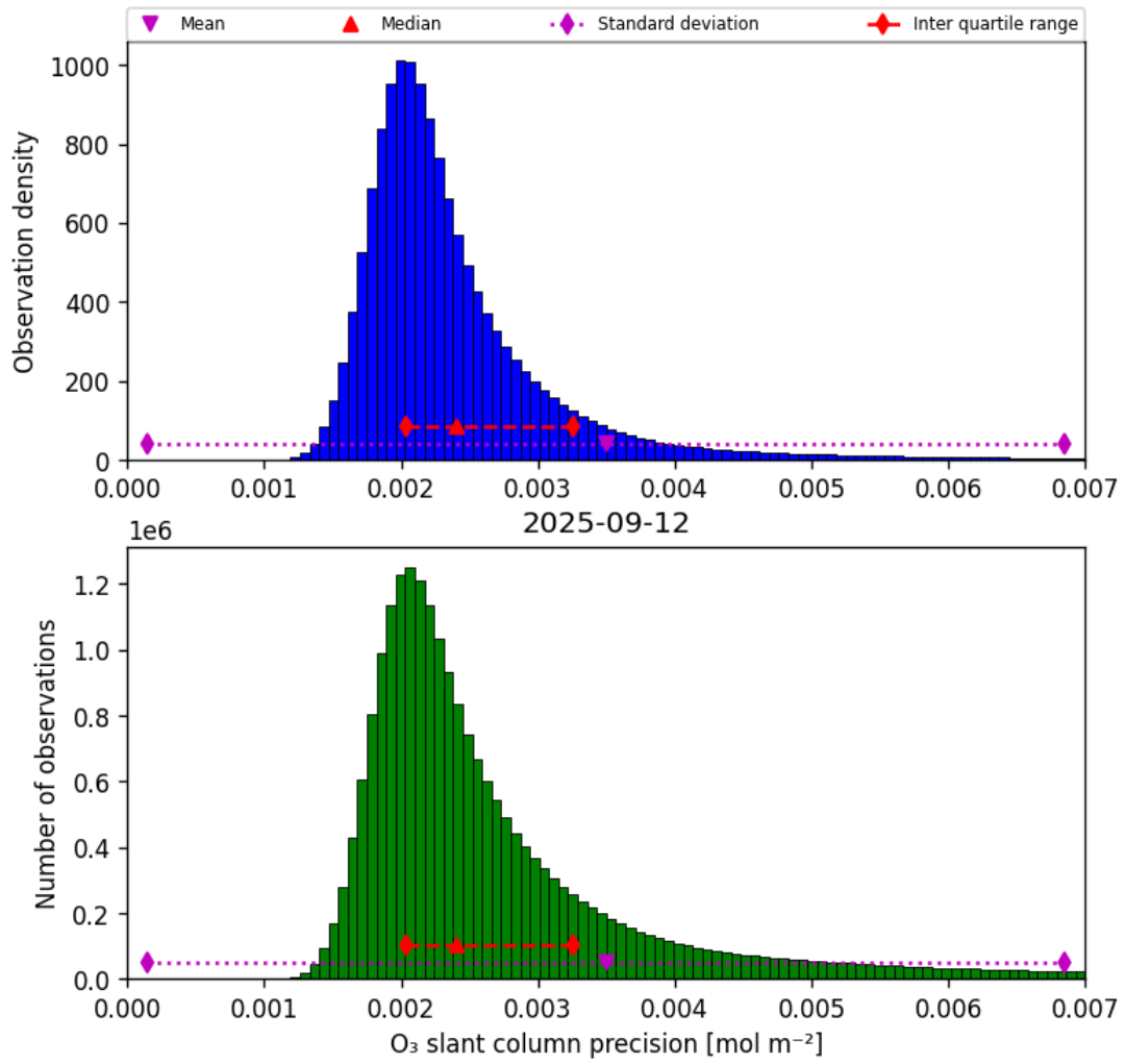
Figure 32: Histogram of “O 3 slant column precision” for 2025-09-12 to 2025-09-13
