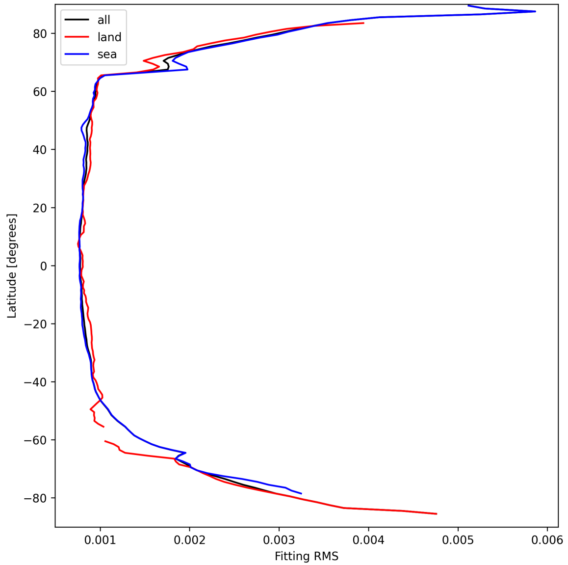
Figure 22: Zonal average of “Fitting RMS” for 2025-09-12 to 2025-09-13.
