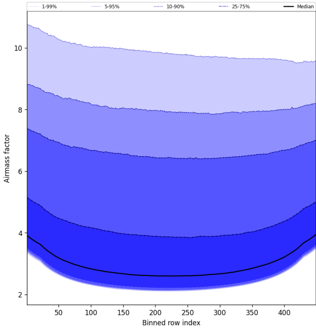
Figure 49: Along track statistics of “Airmass factor” for 2025-09-12 to 2025-09-13
