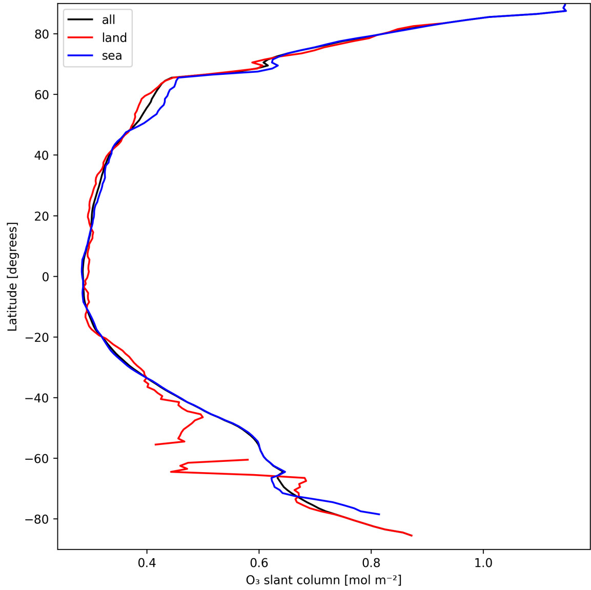
Figure 19: Zonal average of “O 3 slant column” for 2025-09-12 to 2025-09-13.
