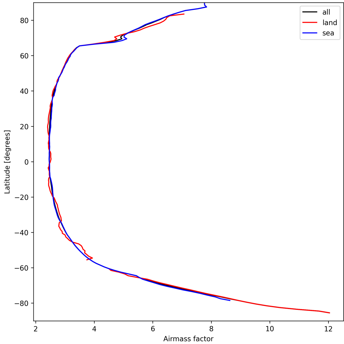
Figure 25: Zonal average of “Airmass factor” for 2025-09-12 to 2025-09-13.
