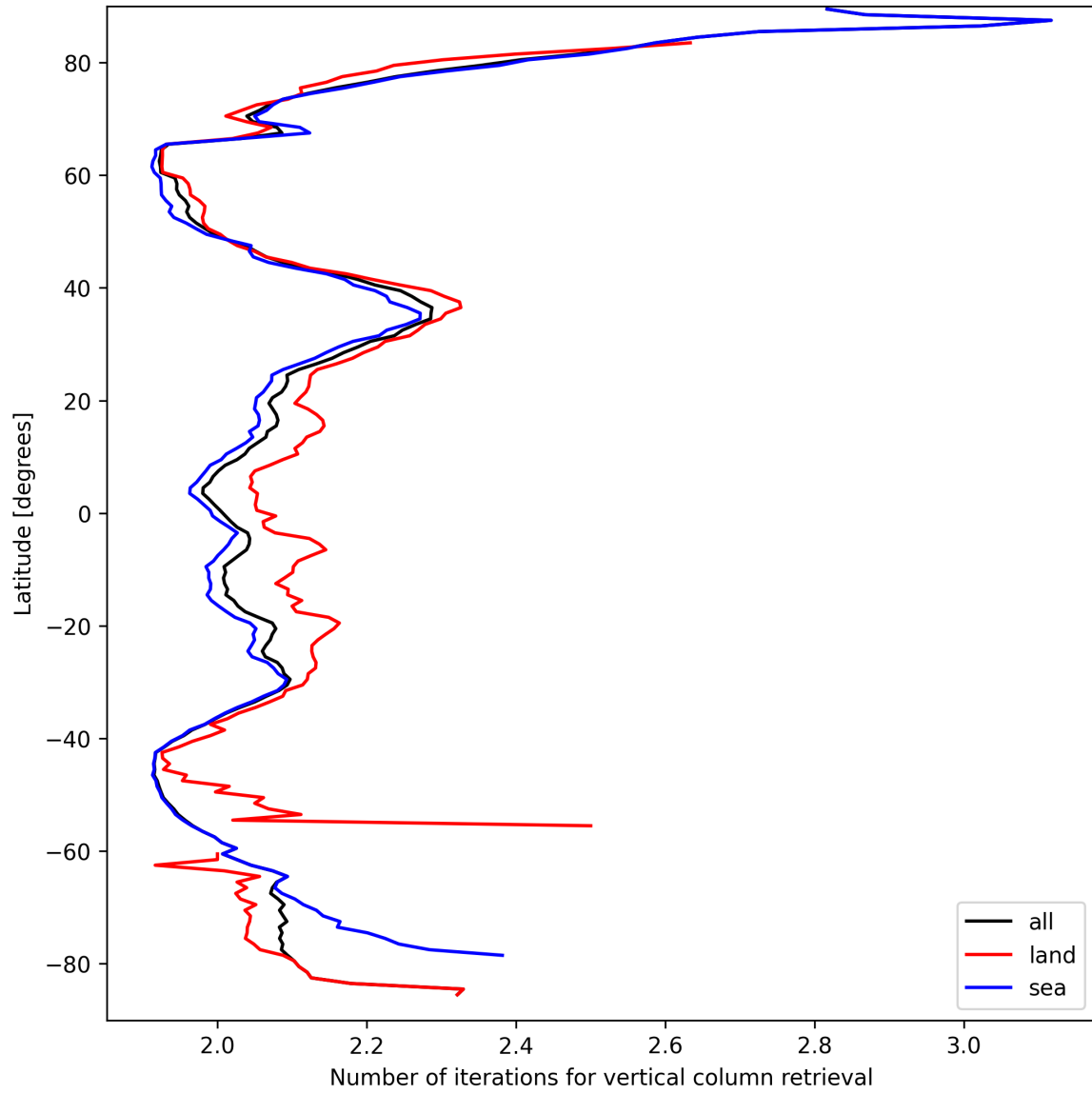
Figure 27: Zonal average of “Number of iterations for vertical column retrieval” for 2025-09-12 to 2025-09-13.
