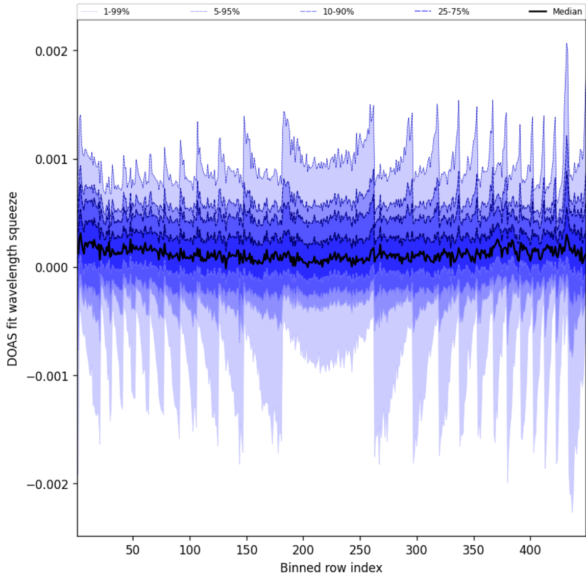
Figure 48: Along track statistics of “DOAS fit wavelength squeeze” for 2025-09-12 to 2025-09-13
