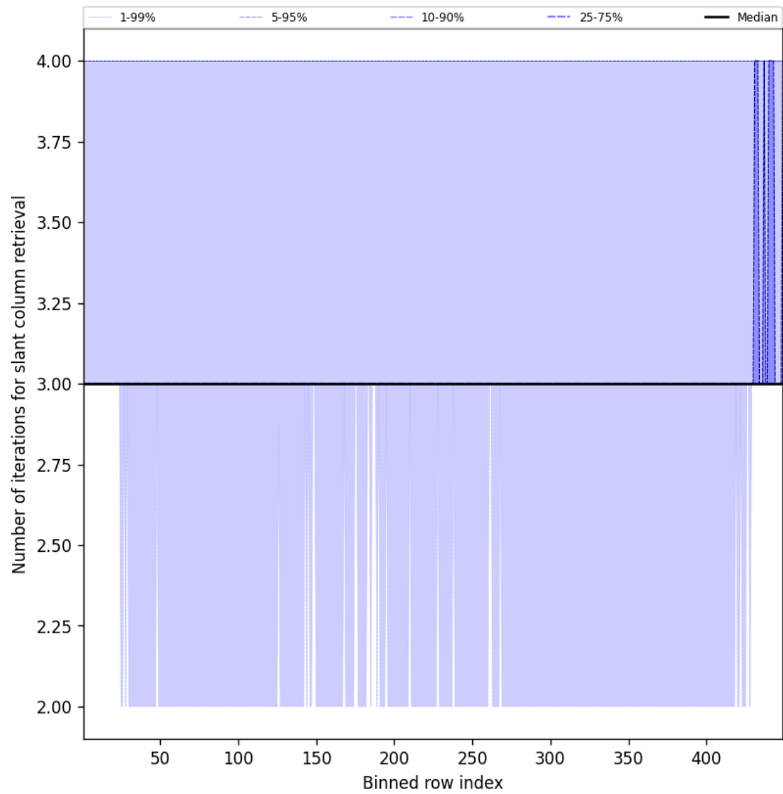
Figure 45: Along track statistics of “Number of iterations for slant column retrieval” for 2025-09-12 to 2025-09-13
