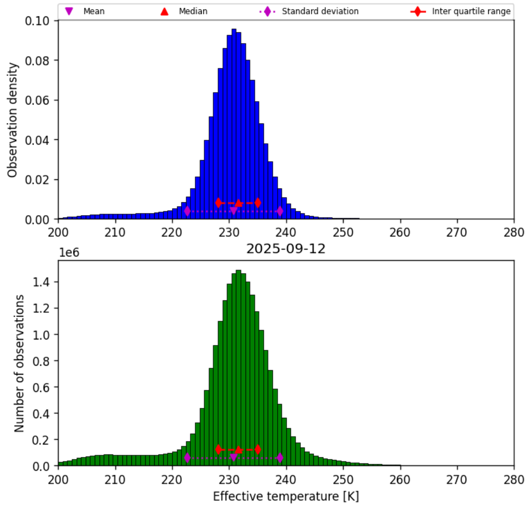
Figure 38: Histogram of “Effective temperature” for 2025-09-12 to 2025-09-13
