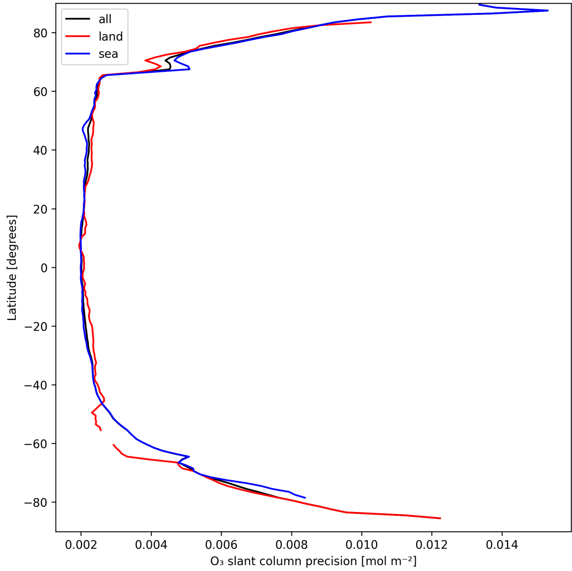
Figure 20: Zonal average of “O 3 slant column precision” for 2025-09-12 to 2025-09-13.
