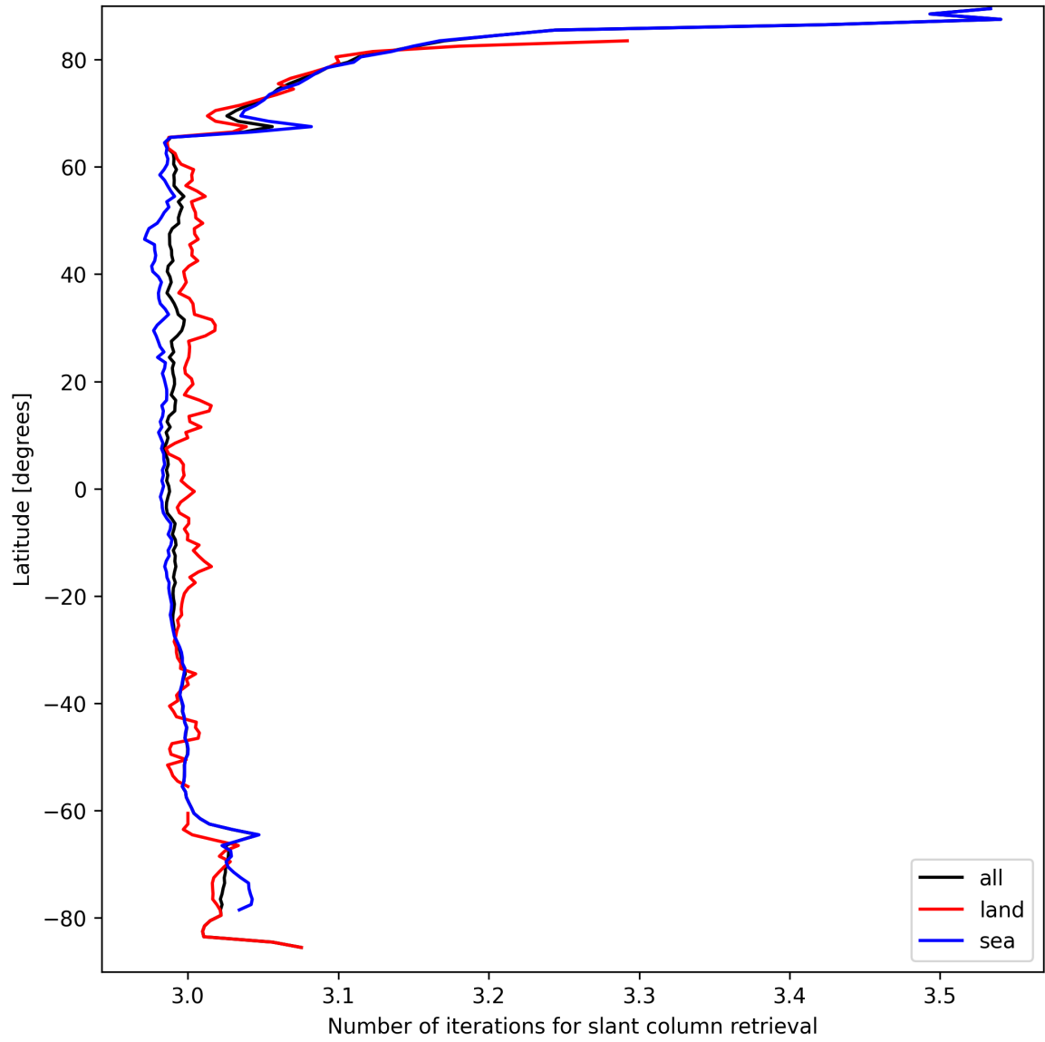
Figure 21: Zonal average of “Number of iterations for slant column retrieval” for 2025-09-12 to 2025-09-13.
