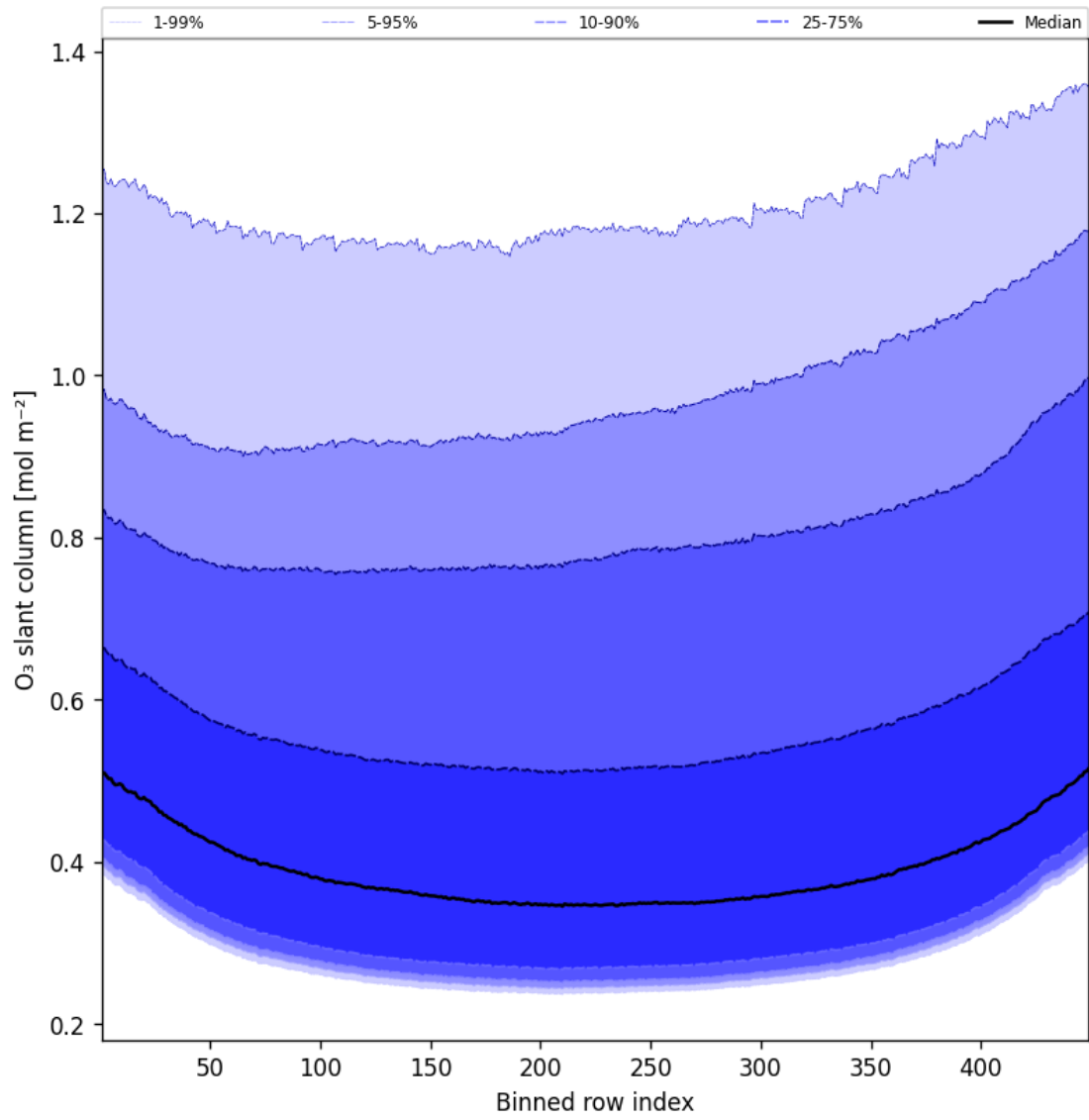
Figure 43: Along track statistics of “O 3 slant column” for 2025-09-12 to 2025-09-13
