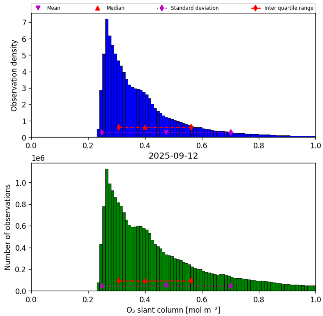
Figure 31: Histogram of “O 3 slant column” for 2025-09-12 to 2025-09-13
