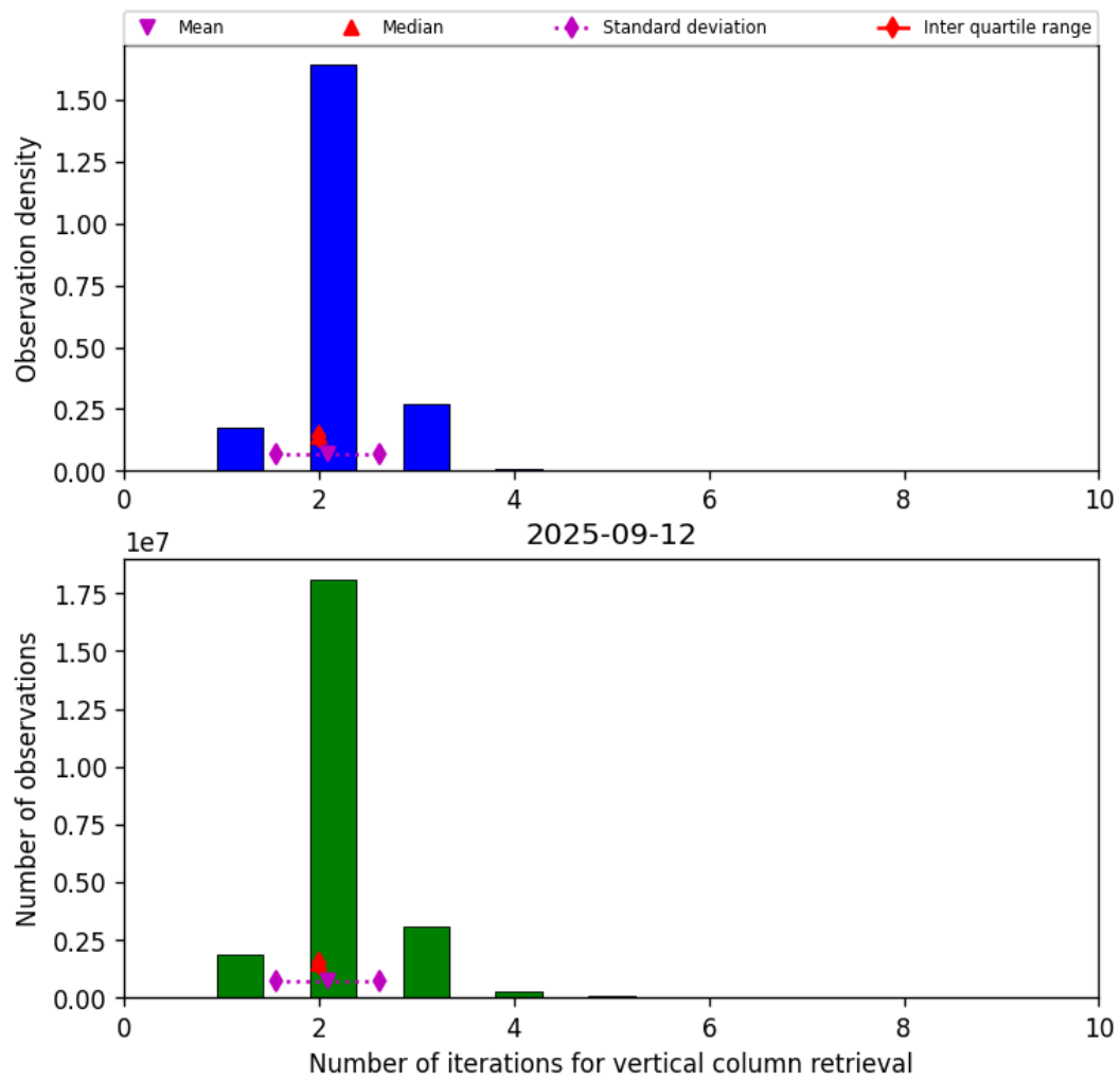
Figure 39: Histogram of “Number of iterations for vertical column retrieval” for 2025-09-12 to 2025-09-13
