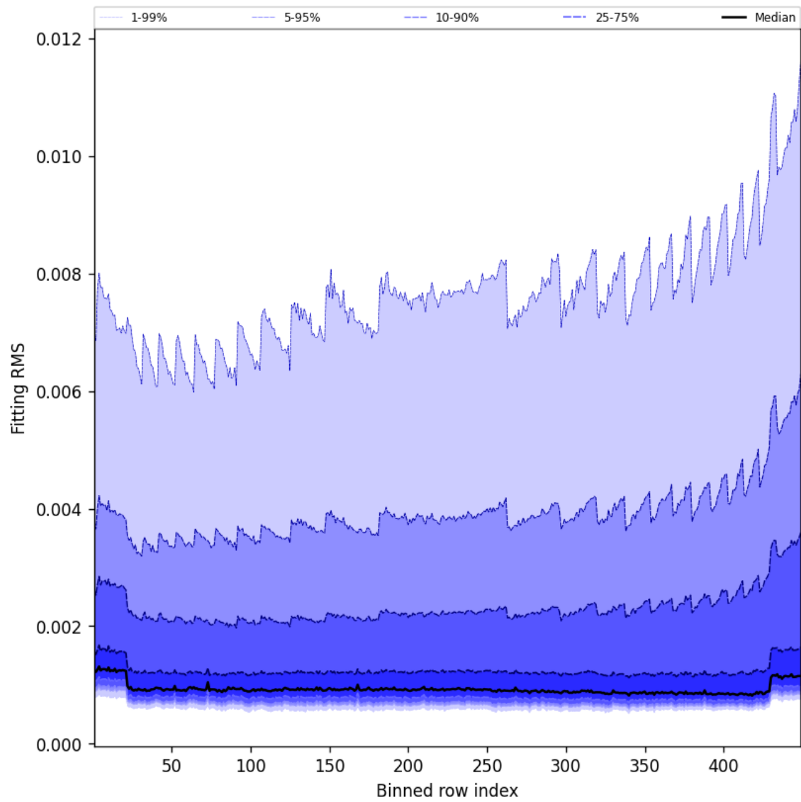
Figure 46: Along track statistics of “Fitting RMS” for 2025-09-12 to 2025-09-13
