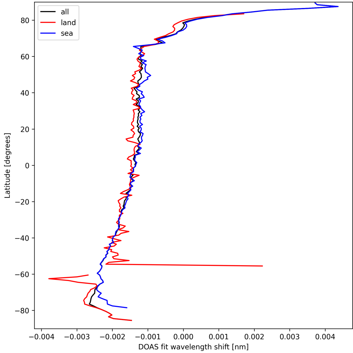
Figure 23: Zonal average of "DOAS fit wavelength shift" for 2025-09-12 to 2025-09-13.
