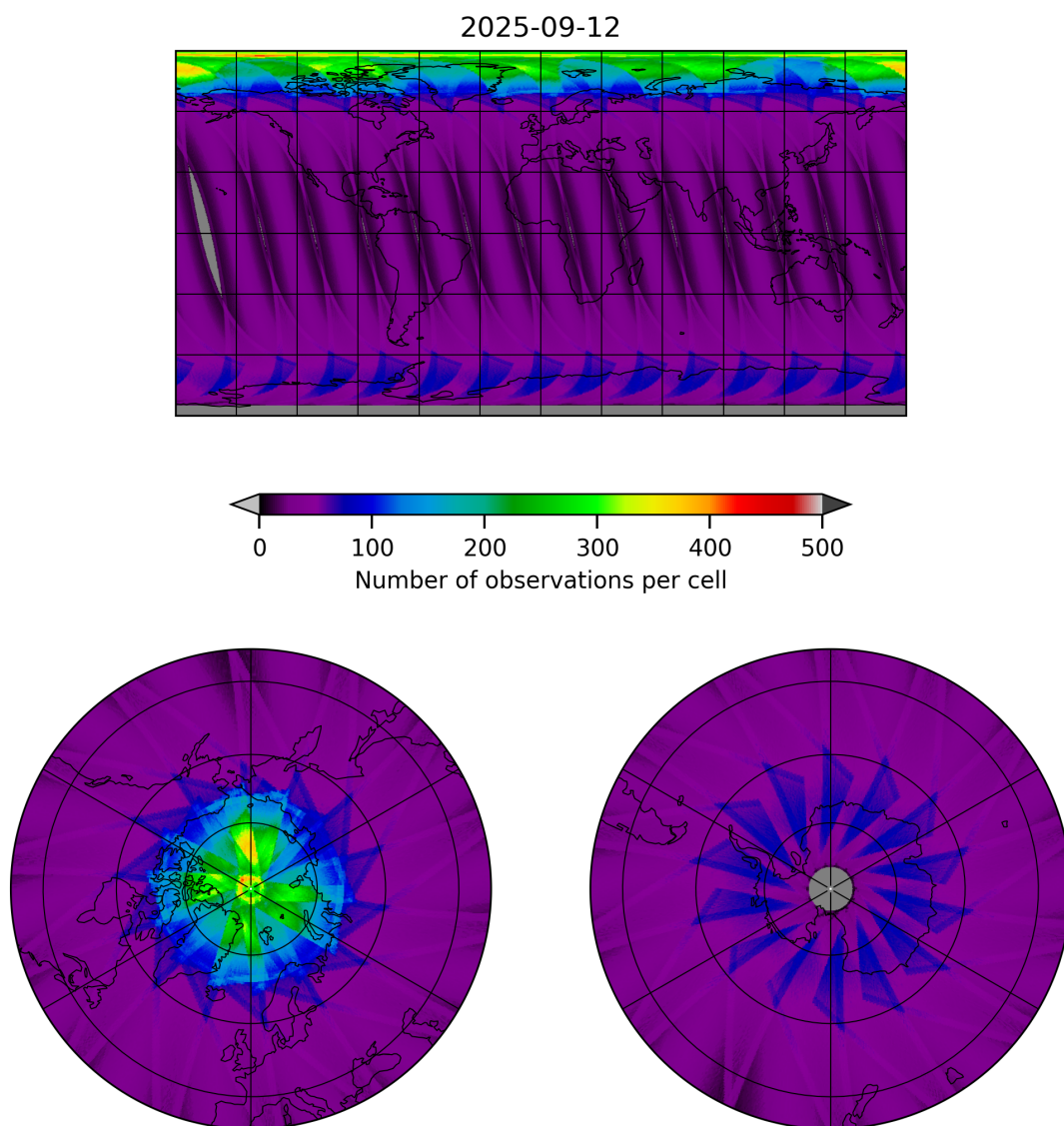
Figure 15: Map of the number of observations for 2025-09-12 to 2025-09-13
