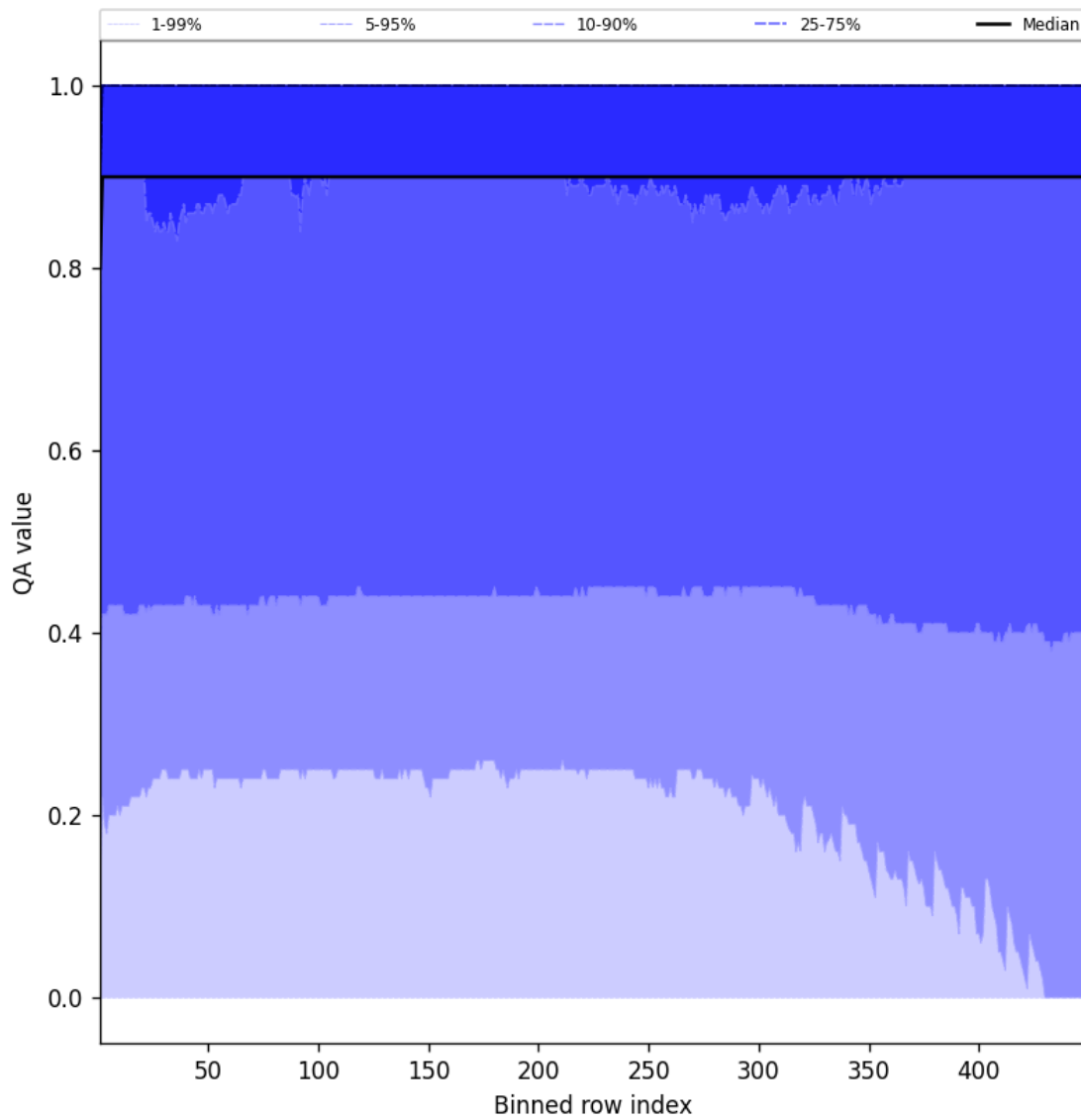
Figure 40: Along track statistics of “QA value” for 2025-09-12 to 2025-09-13
