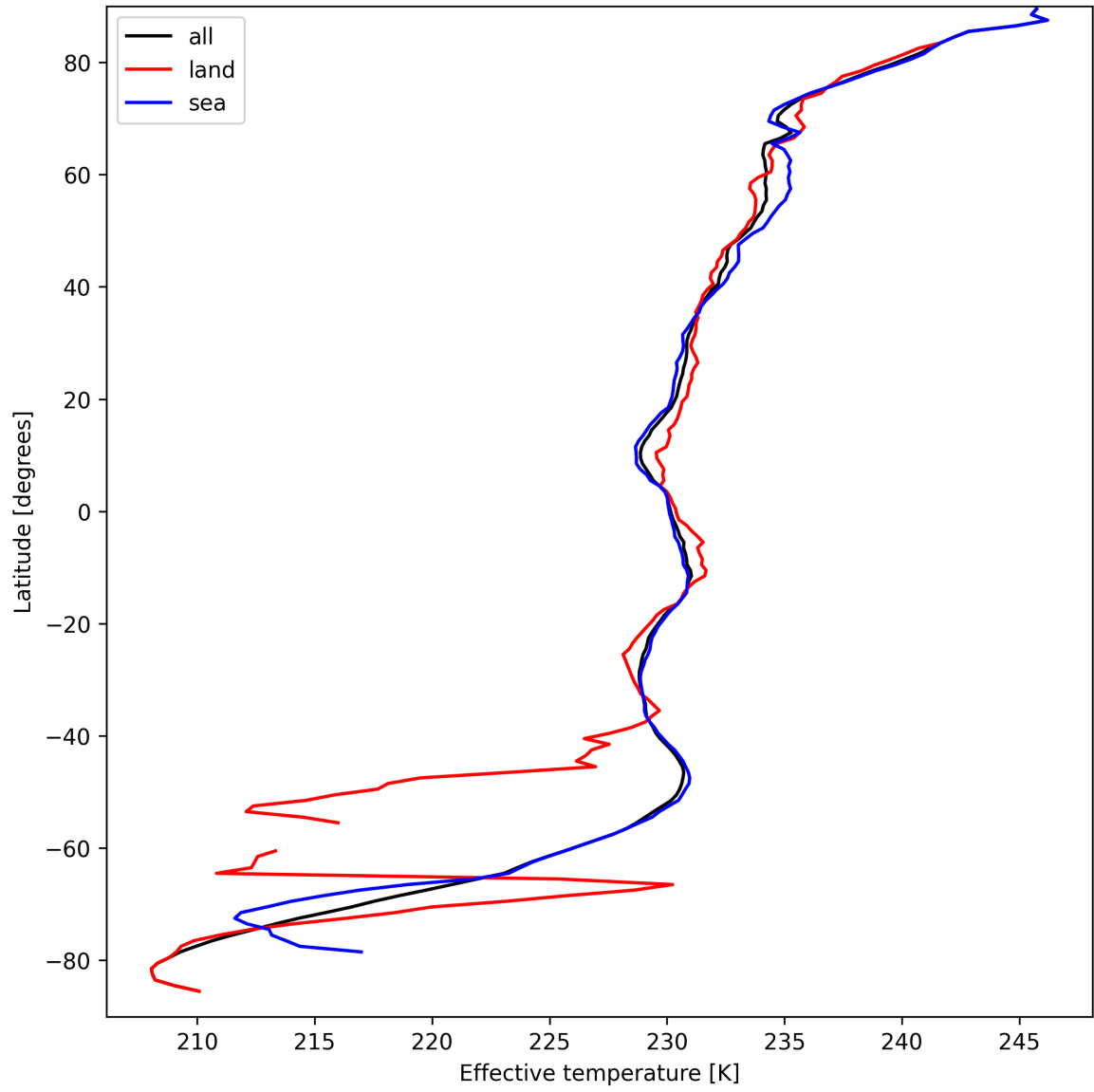
Figure 26: Zonal average of “Effective temperature” for 2025-09-12 to 2025-09-13.
