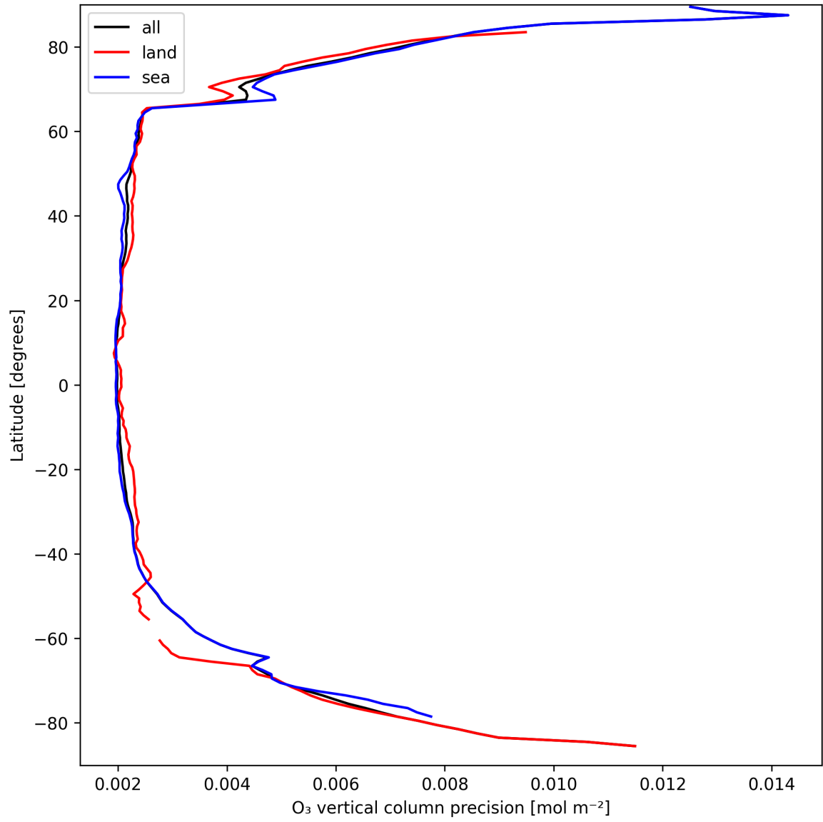
Figure 18: Zonal average of “O 3 vertical column precision” for 2025-09-12 to 2025-09-13.
