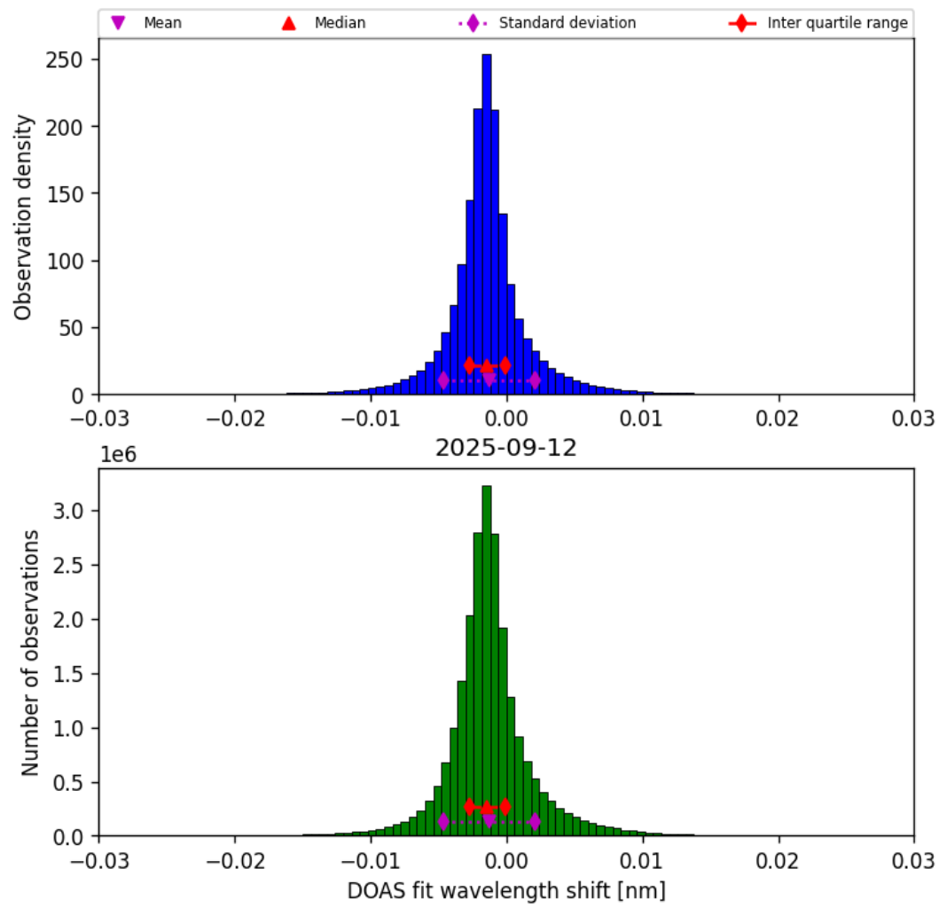
Figure 35: Histogram of “DOAS fit wavelength shift” for 2025-09-12 to 2025-09-13
