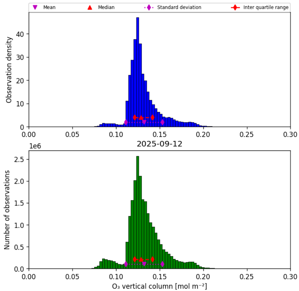
Figure 29: Histogram of “O 3 vertical column” for 2025-09-12 to 2025-09-13
