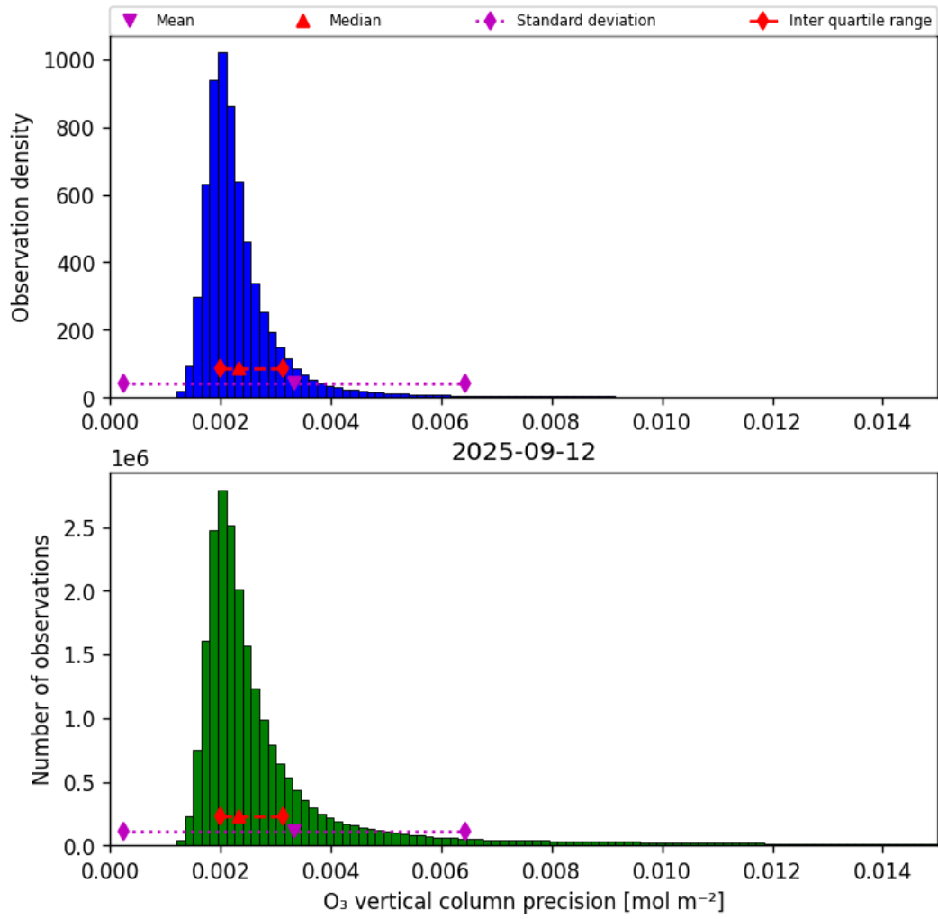
Figure 30: Histogram of “O 3 vertical column precision” for 2025-09-12 to 2025-09-13
