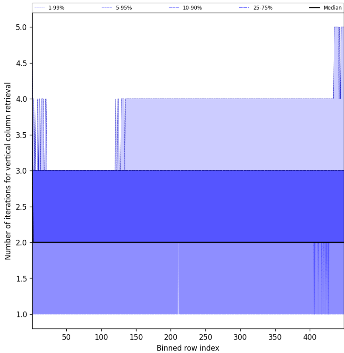
Figure 51: Along track statistics of “Number of iterations for vertical column retrieval” for 2025-09-12 to 2025-09-13
