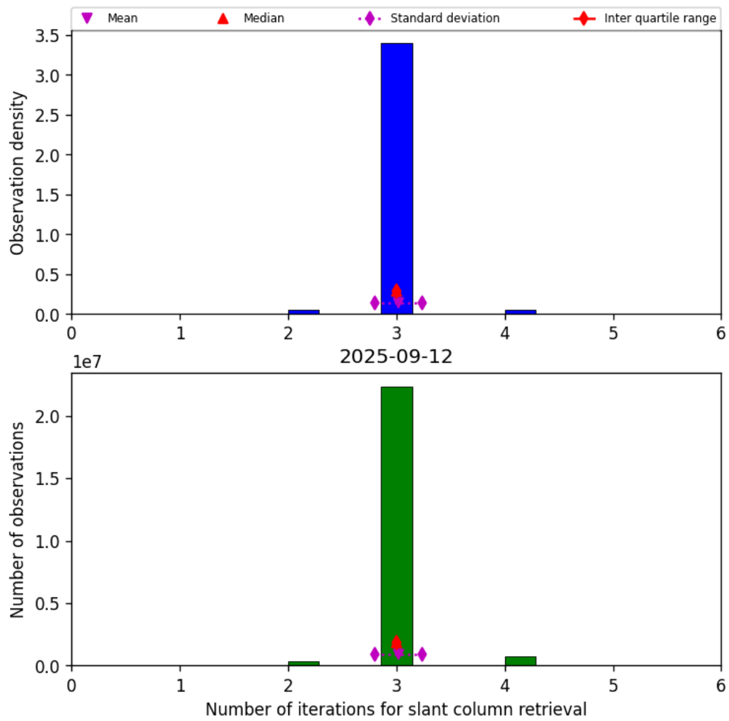
Figure 33: Histogram of “Number of iterations for slant column retrieval” for 2025-09-12 to 2025-09-13
