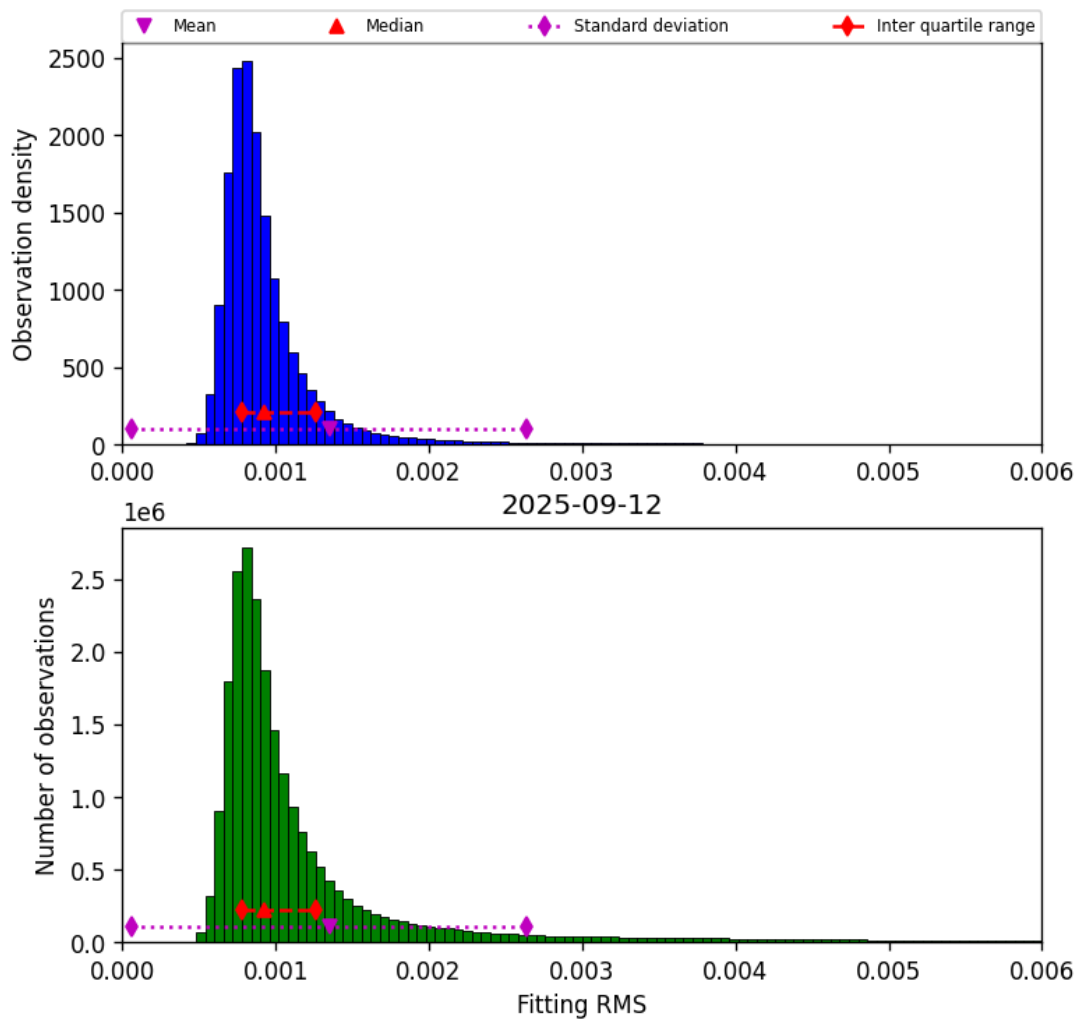
Figure 34: Histogram of “Fitting RMS” for 2025-09-12 to 2025-09-13
