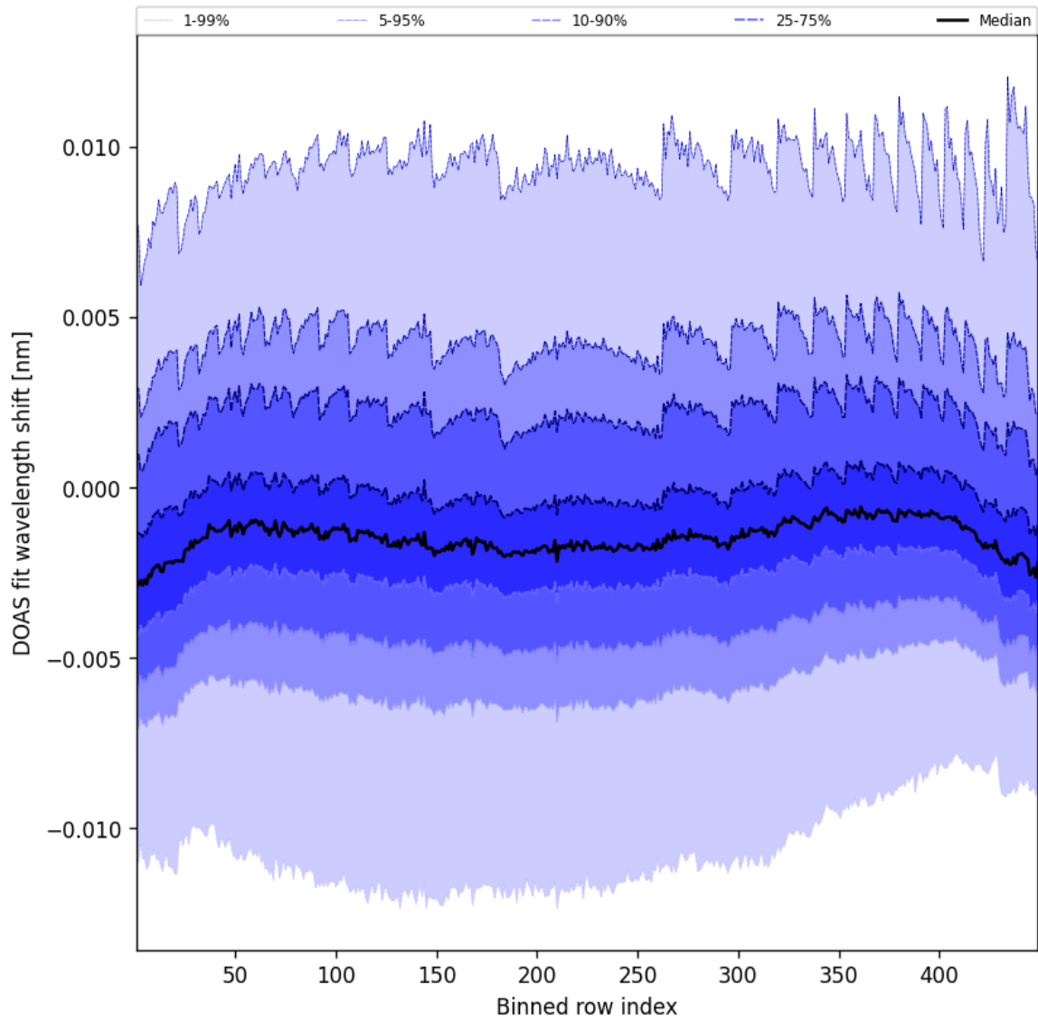
Figure 47: Along track statistics of “DOAS fit wavelength shift” for 2025-09-12 to 2025-09-13
