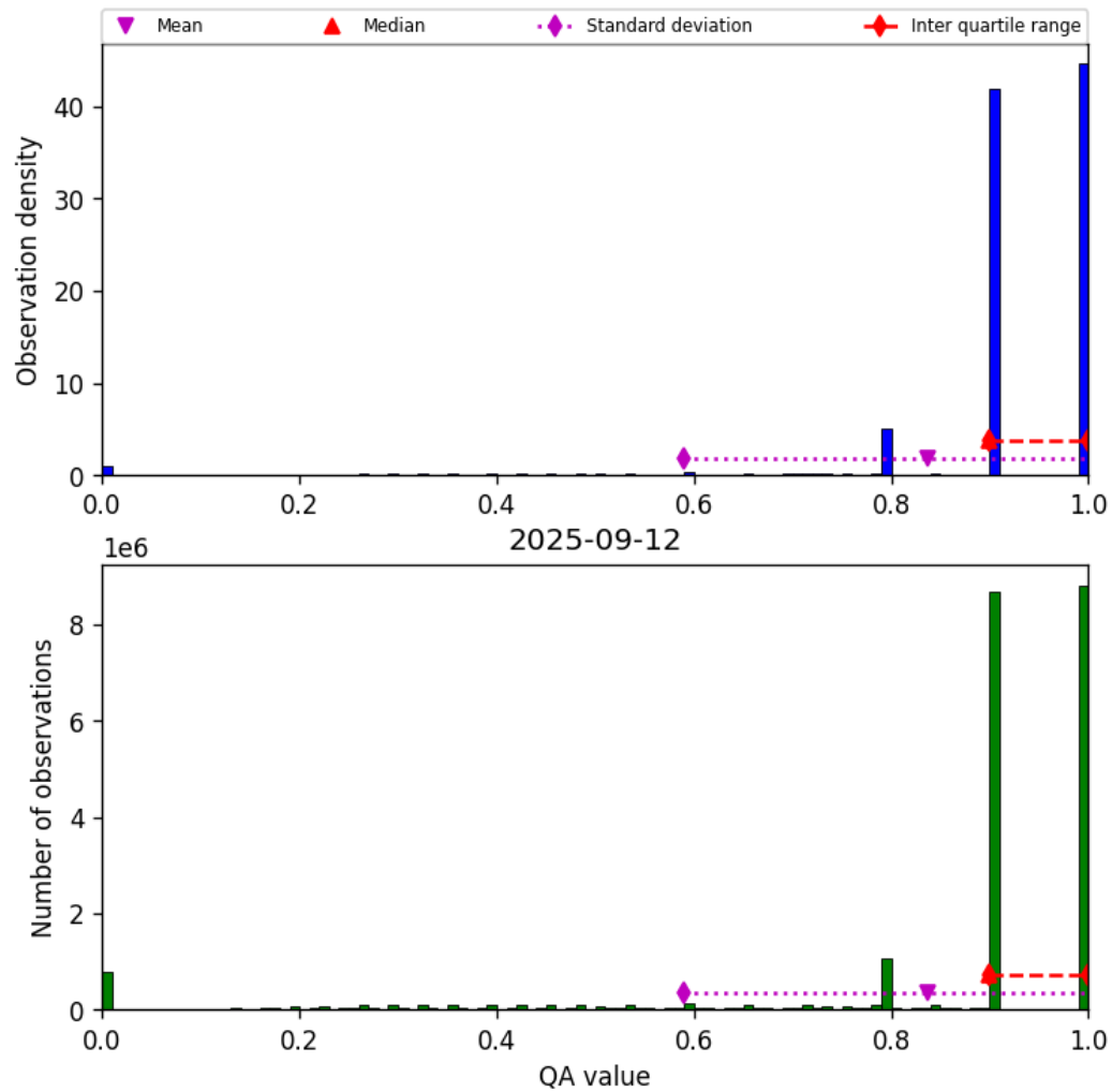
Figure 28: Histogram of “QA value” for 2025-09-12 to 2025-09-13
