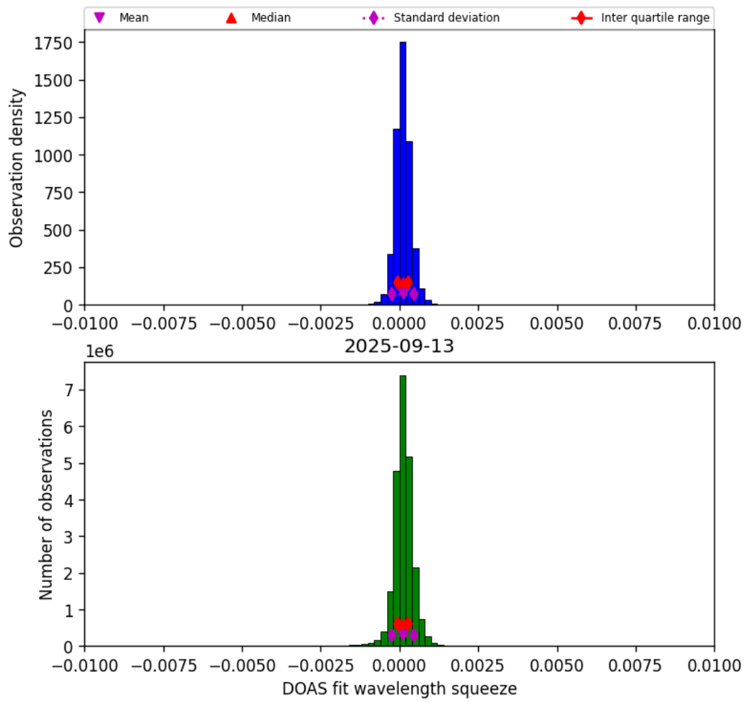
Figure 36: Histogram of “DOAS fit wavelength squeeze” for 2025-09-13 to 2025-09-13
