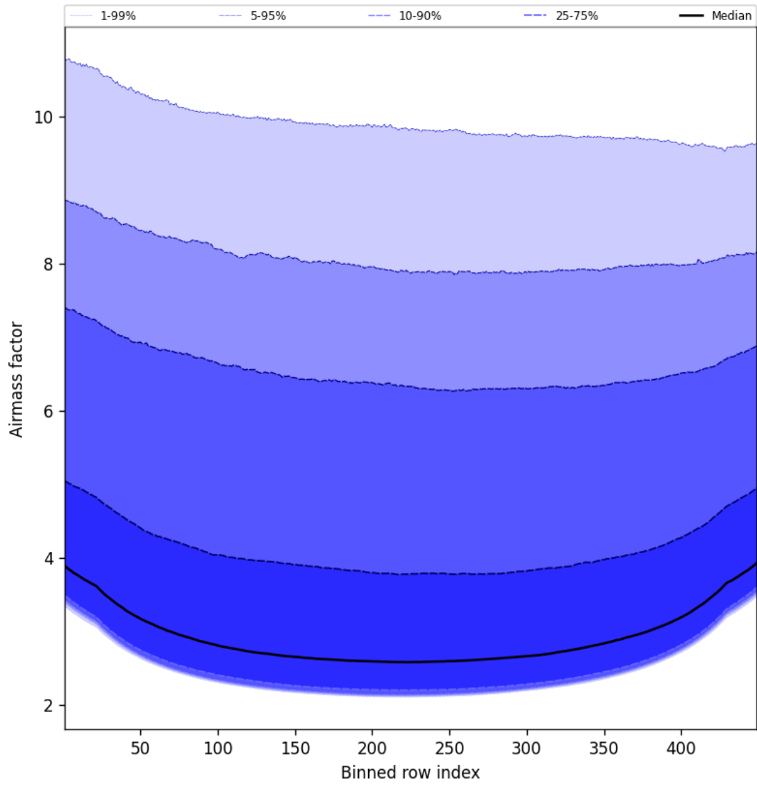
Figure 49: Along track statistics of “Airmass factor” for 2025-09-13 to 2025-09-13
