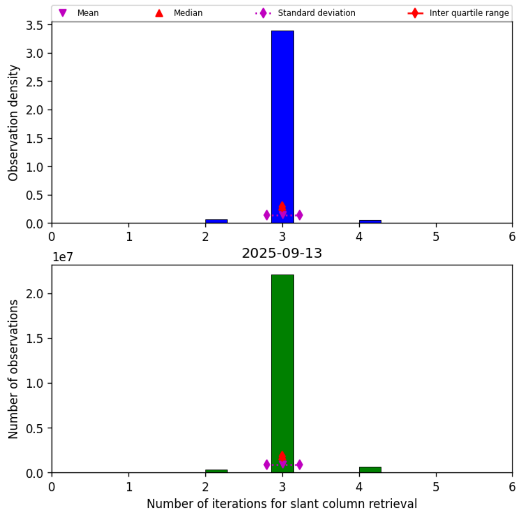
Figure 33: Histogram of "Number of iterations for slant column retrieval" for 2025-09-13 to 2025-09-13
