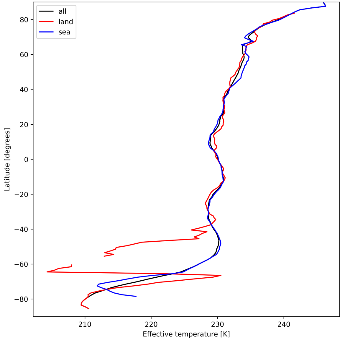
Figure 26: Zonal average of “Effective temperature” for 2025-09-13 to 2025-09-13.
