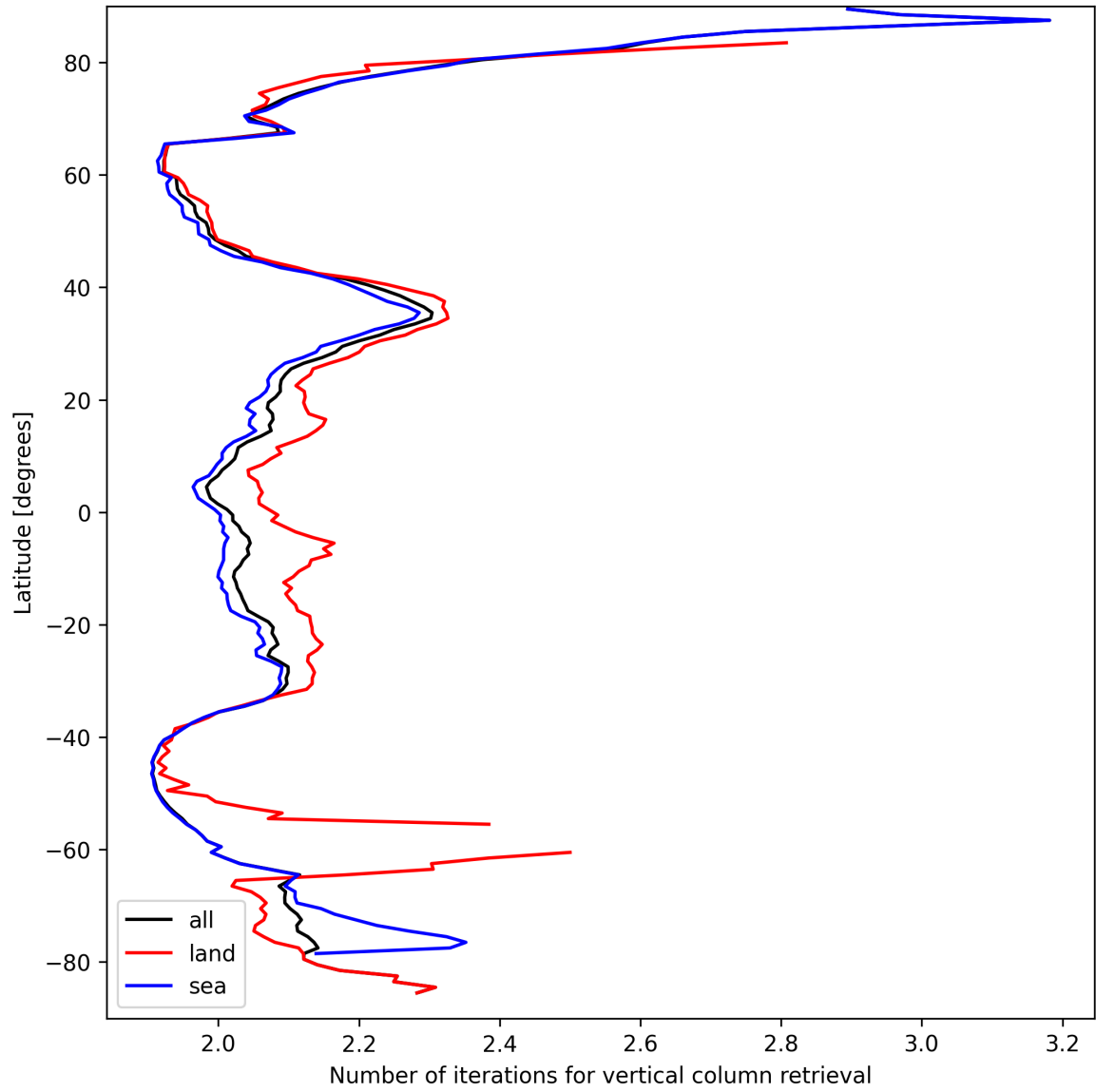
Figure 27: Zonal average of “Number of iterations for vertical column retrieval” for 2025-09-13 to 2025-09-13.
