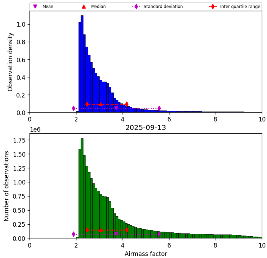
Figure 37: Histogram of “Airmass factor” for 2025-09-13 to 2025-09-13
