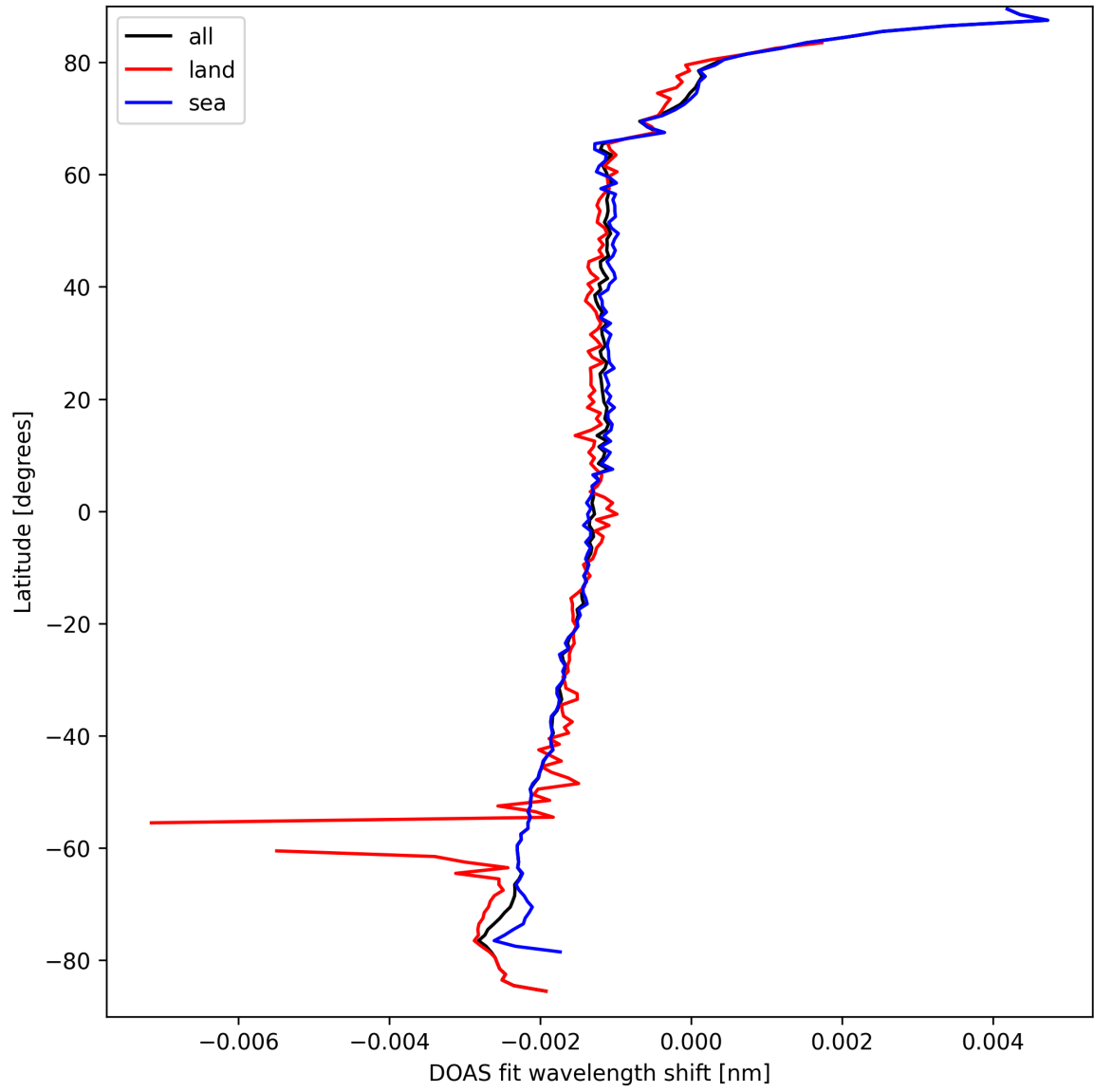
Figure 23: Zonal average of "DOAS fit wavelength shift" for 2025-09-13 to 2025-09-13.
