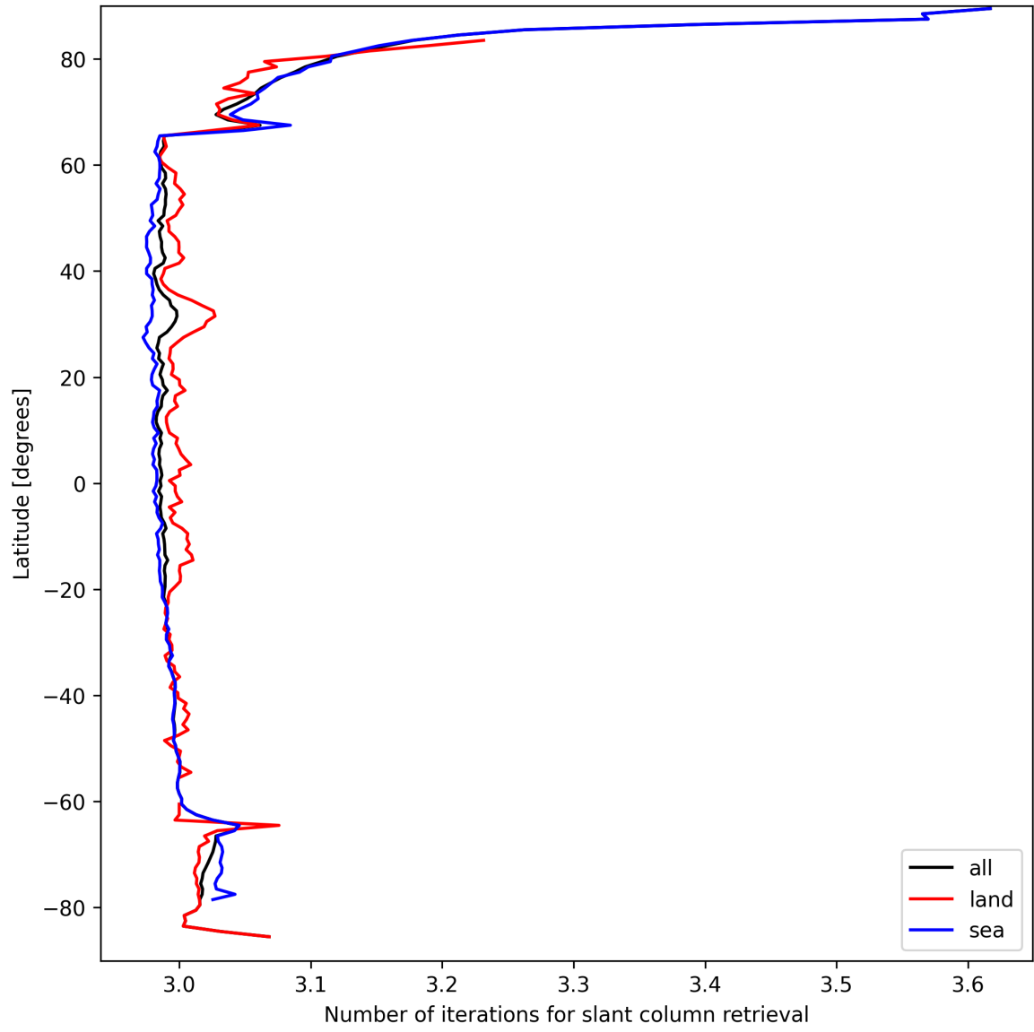
Figure 21: Zonal average of “Number of iterations for slant column retrieval” for 2025-09-13 to 2025-09-13.
