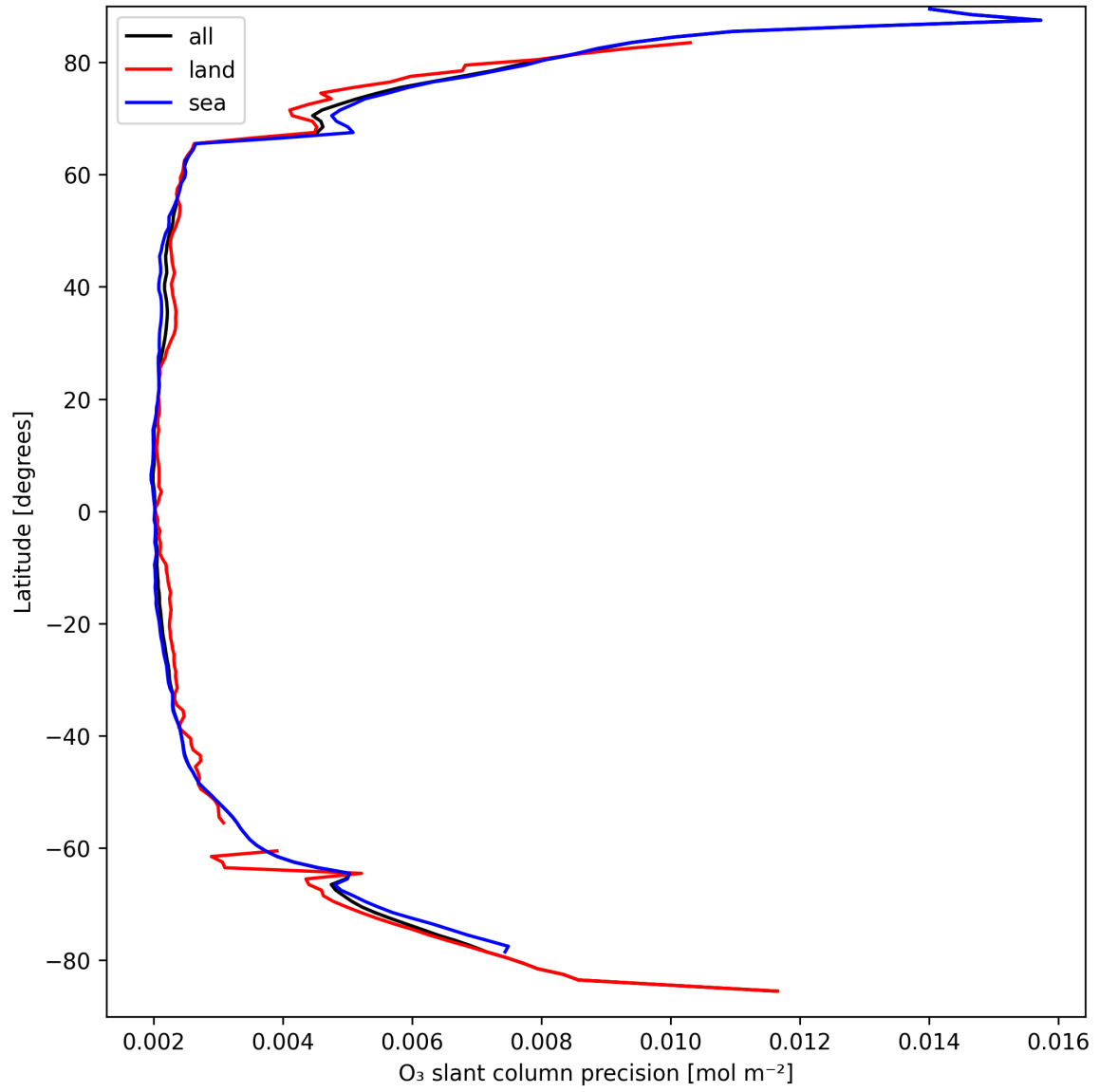
Figure 20: Zonal average of “O 3 slant column precision” for 2025-09-13 to 2025-09-13.
