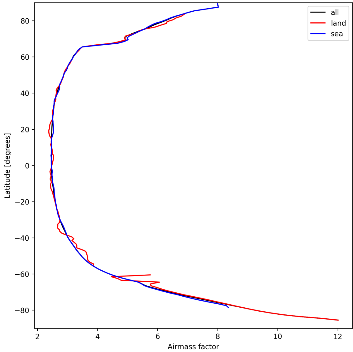
Figure 25: Zonal average of “Airmass factor” for 2025-09-13 to 2025-09-13.
