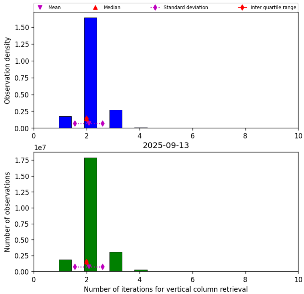
Figure 39: Histogram of “Number of iterations for vertical column retrieval” for 2025-09-13 to 2025-09-13
