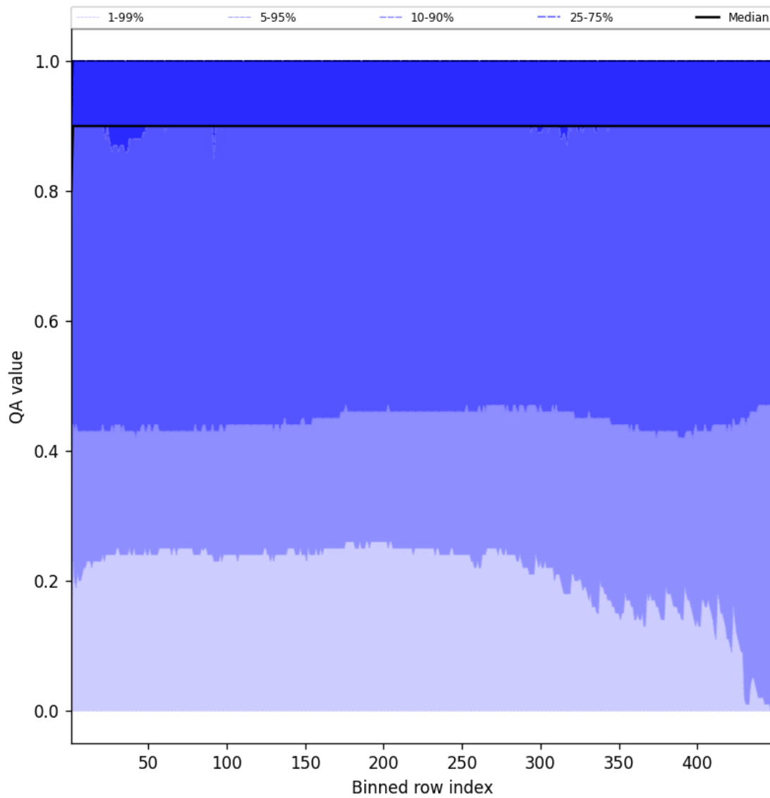
Figure 40: Along track statistics of “QA value” for 2025-09-13 to 2025-09-13
