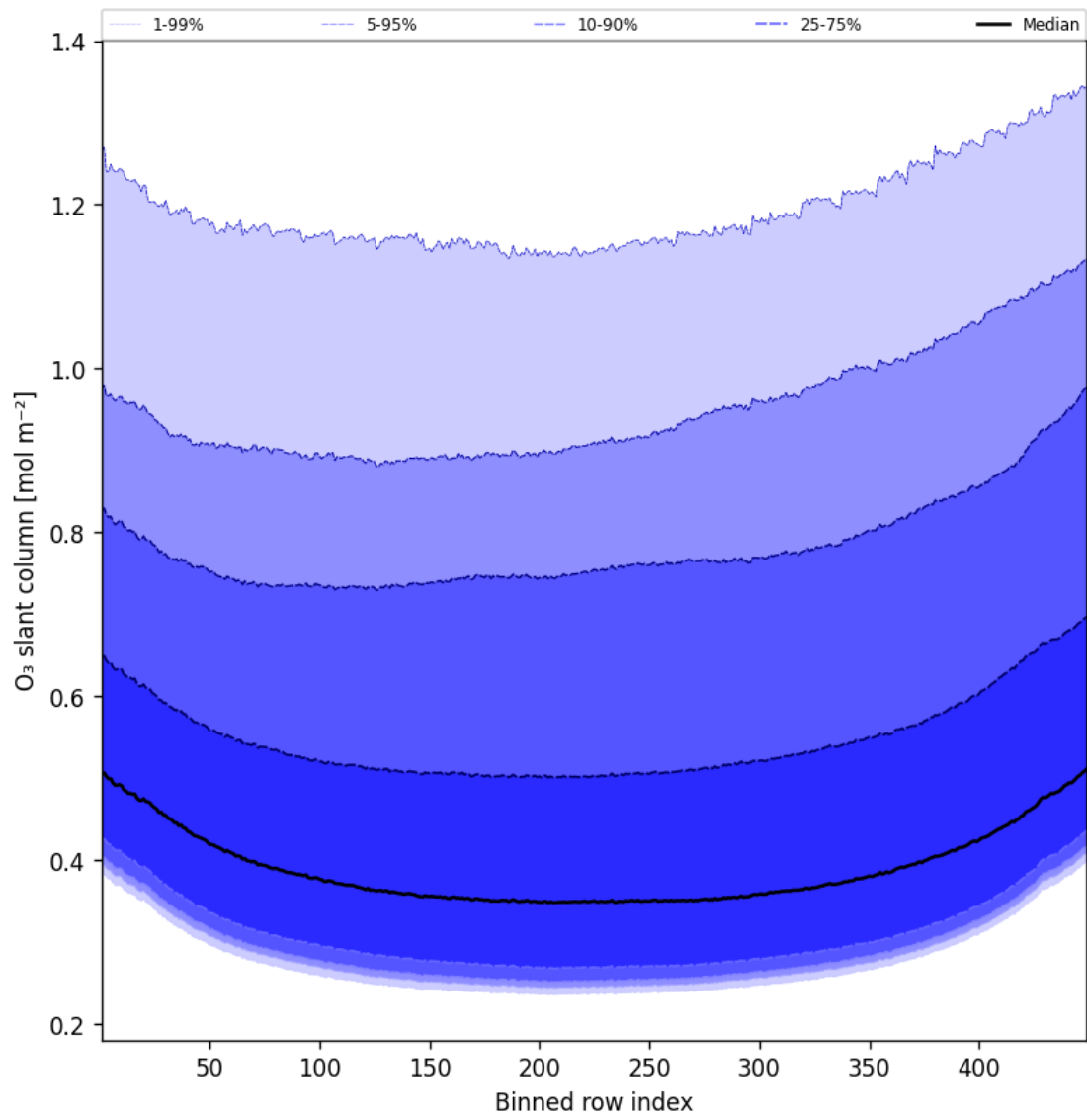
Figure 43: Along track statistics of “O 3 slant column” for 2025-09-13 to 2025-09-13
