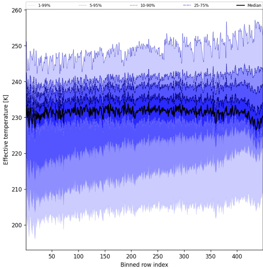
Figure 50: Along track statistics of “Effective temperature” for 2025-09-13 to 2025-09-13
