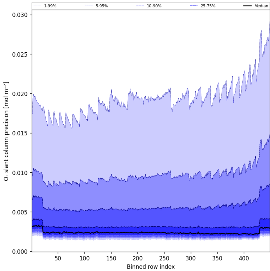
Figure 44: Along track statistics of “O 3 slant column precision” for 2025-09-13 to 2025-09-13
