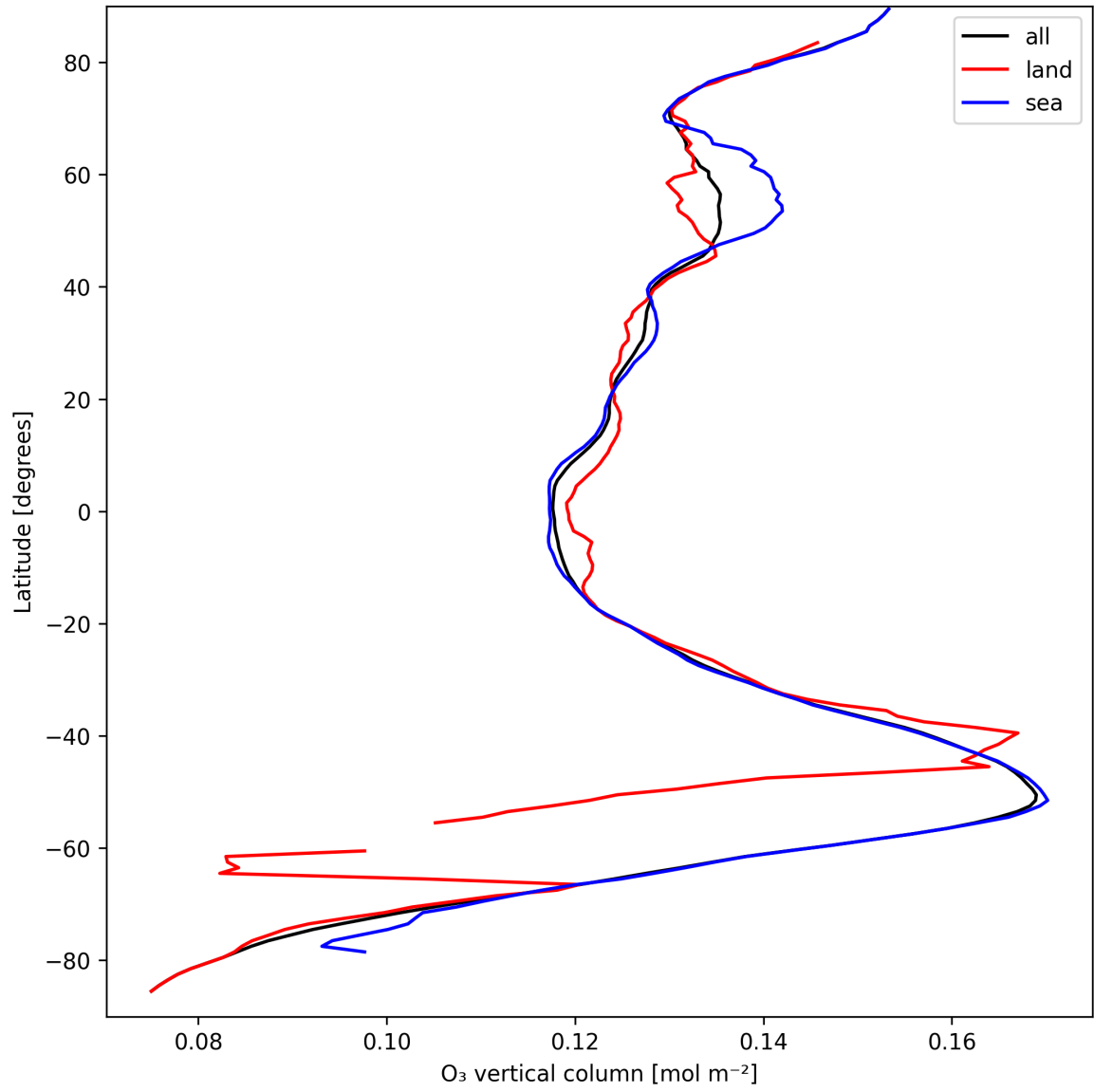
Figure 17: Zonal average of “O 3 vertical column” for 2025-09-13 to 2025-09-13.
