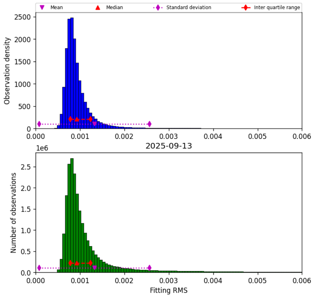
Figure 34: Histogram of “Fitting RMS” for 2025-09-13 to 2025-09-13
