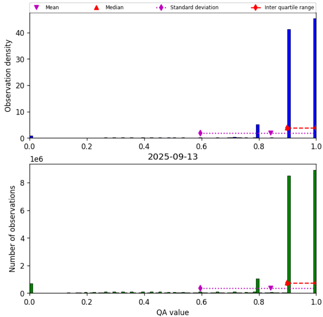
Figure 28: Histogram of “QA value” for 2025-09-13 to 2025-09-13
