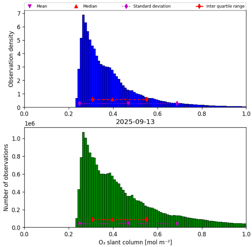
Figure 31: Histogram of “O 3 slant column” for 2025-09-13 to 2025-09-13
