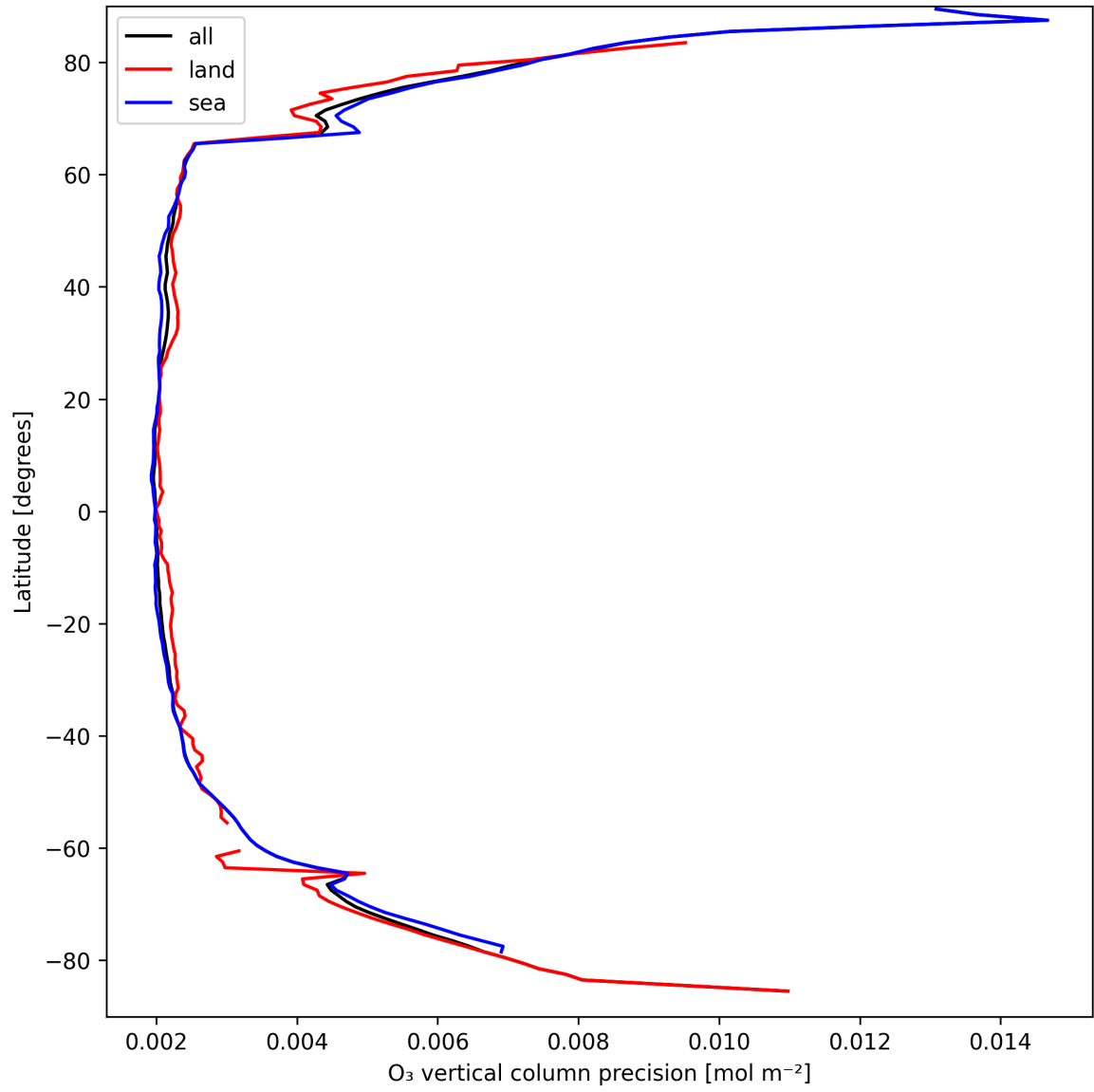
Figure 18: Zonal average of “O 3 vertical column precision” for 2025-09-13 to 2025-09-13.
