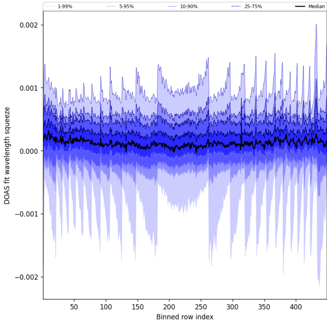
Figure 48: Along track statistics of “DOAS fit wavelength squeeze” for 2025-09-13 to 2025-09-13
