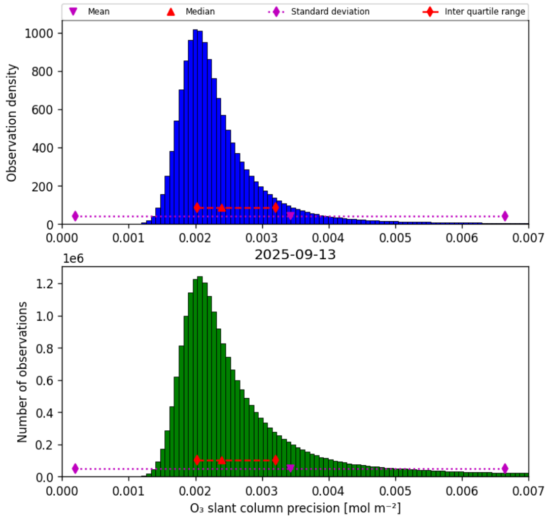
Figure 32: Histogram of “O 3 slant column precision” for 2025-09-13 to 2025-09-13
