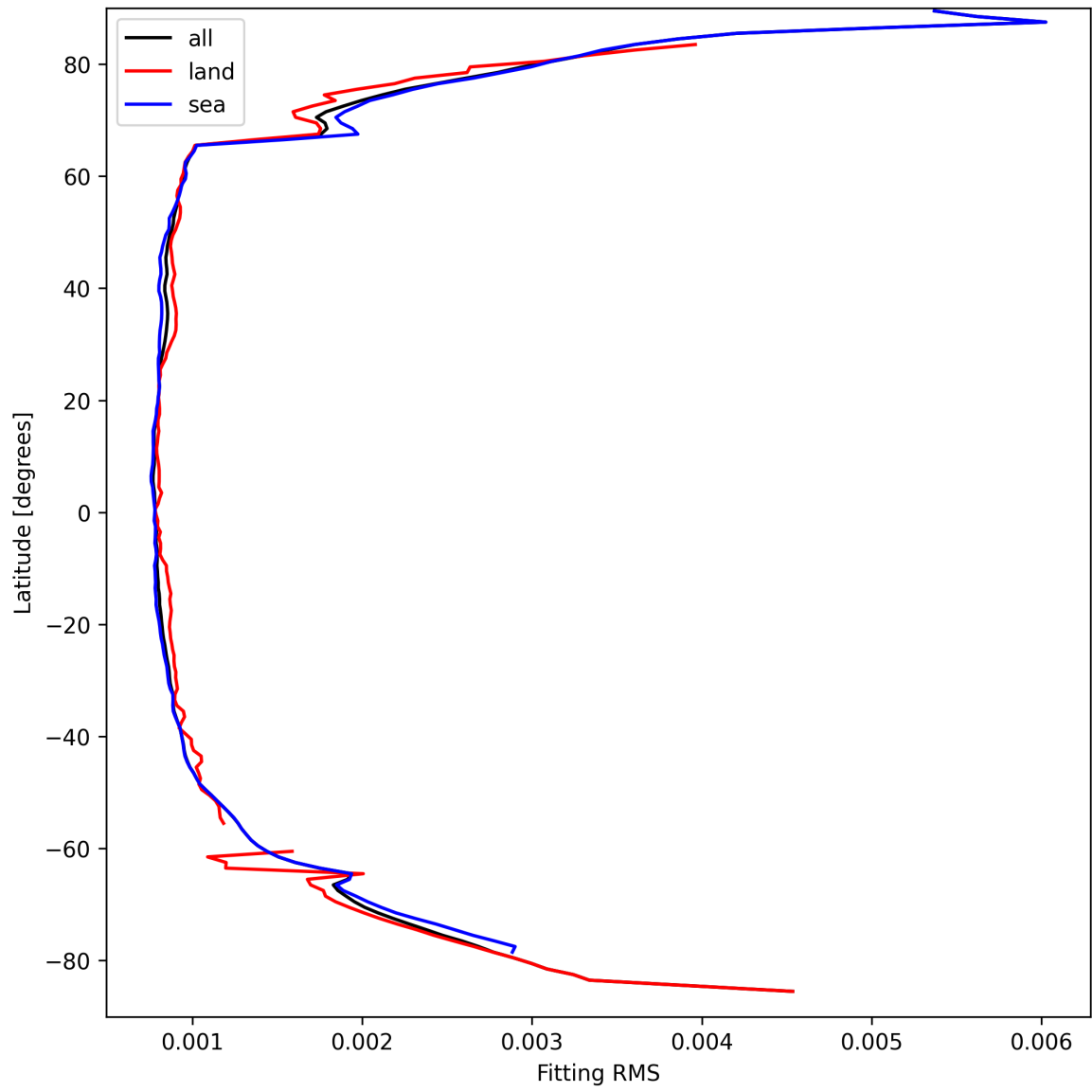
Figure 22: Zonal average of “Fitting RMS” for 2025-09-13 to 2025-09-13.
