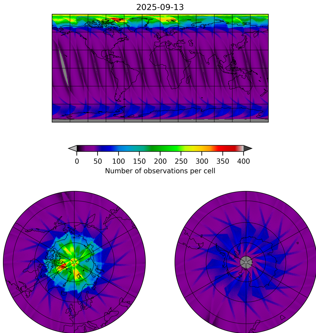
Figure 15: Map of the number of observations for 2025-09-13 to 2025-09-13
