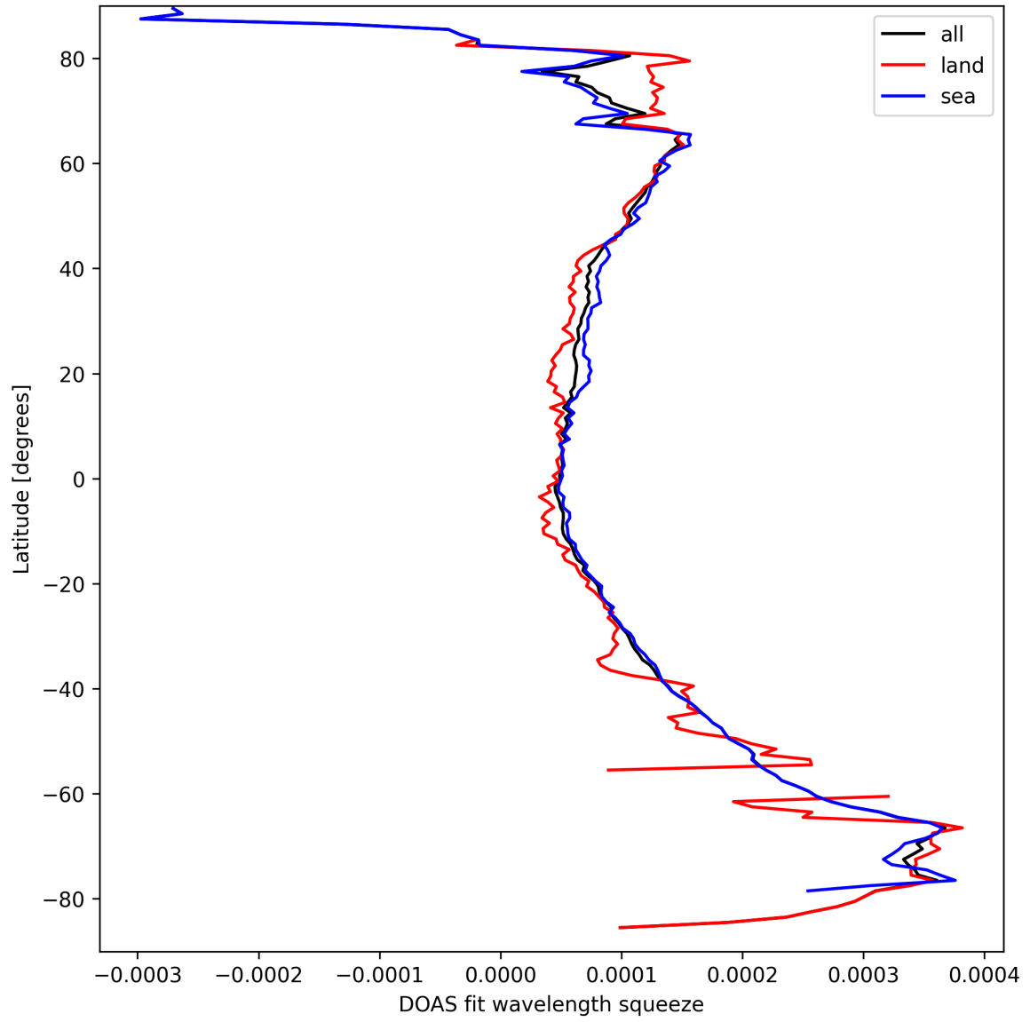
Figure 24: Zonal average of “DOAS fit wavelength squeeze” for 2025-09-13 to 2025-09-13.
