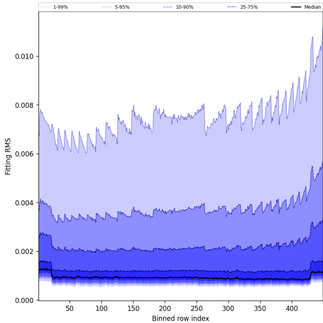
Figure 46: Along track statistics of “Fitting RMS” for 2025-09-13 to 2025-09-13
