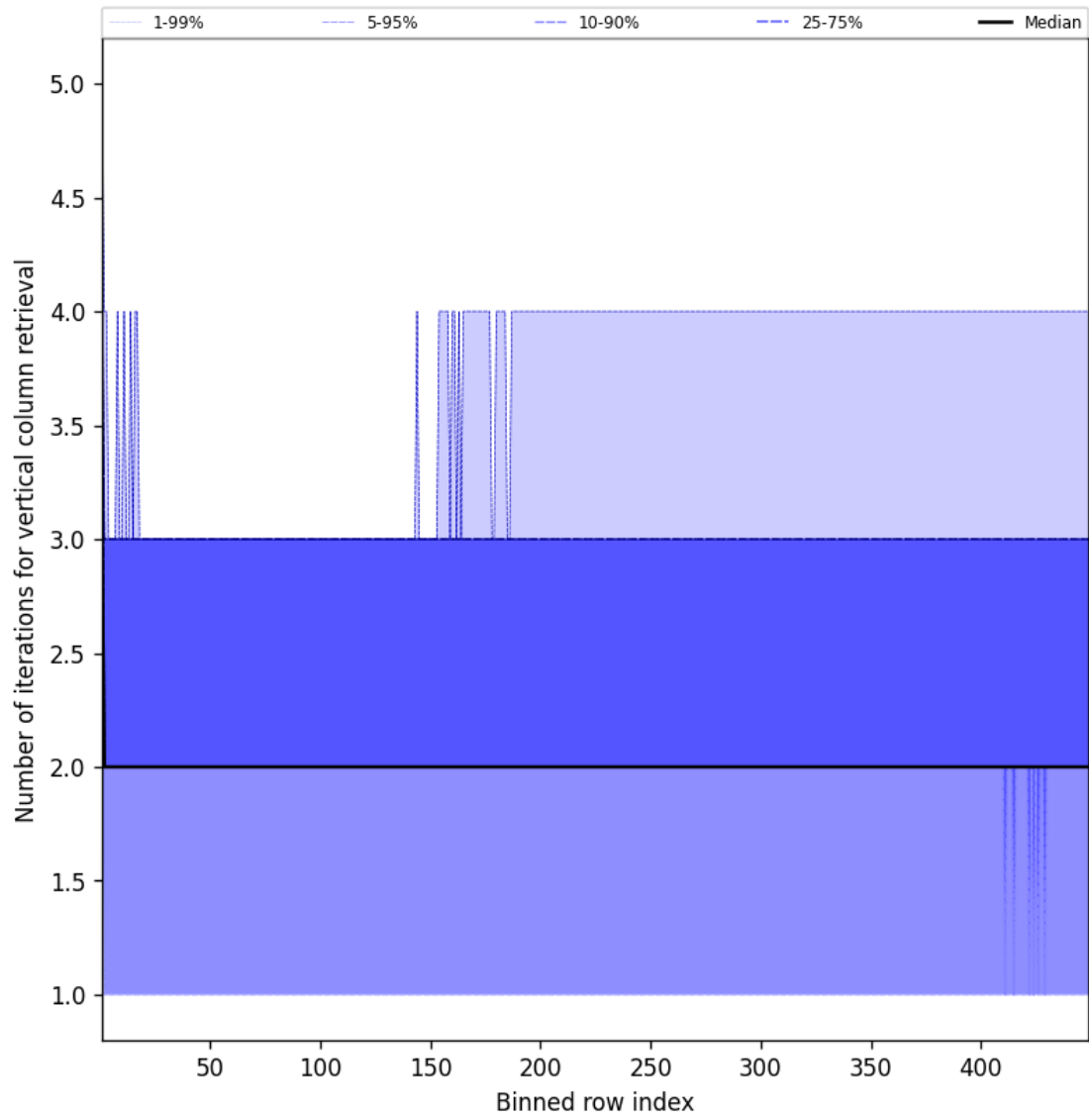
Figure 51: Along track statistics of “Number of iterations for vertical column retrieval” for 2025-09-13 to 2025-09-13
