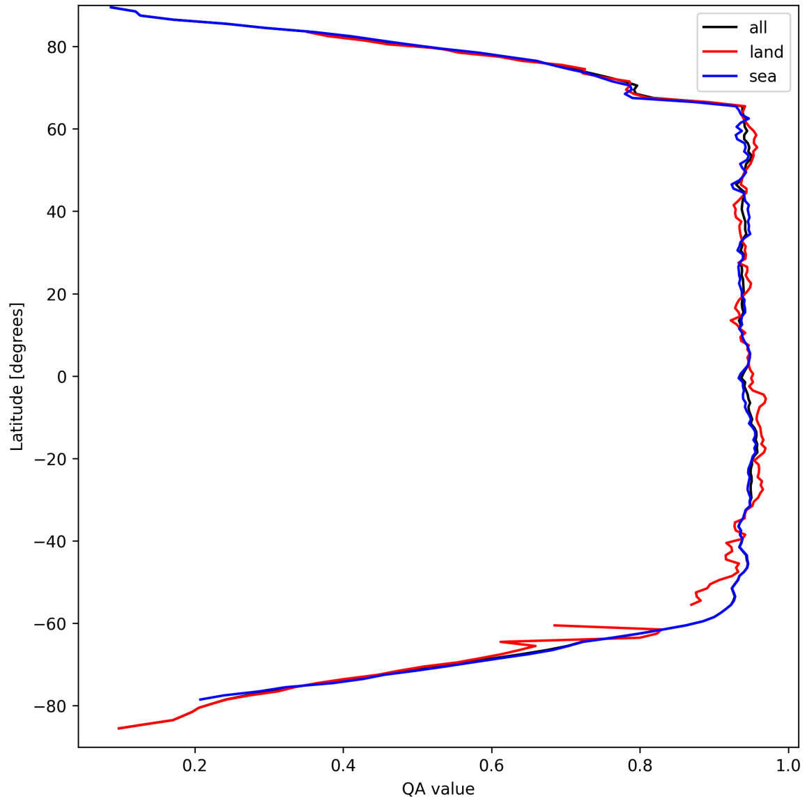
Figure 16: Zonal average of “QA value” for 2025-09-13 to 2025-09-13.
