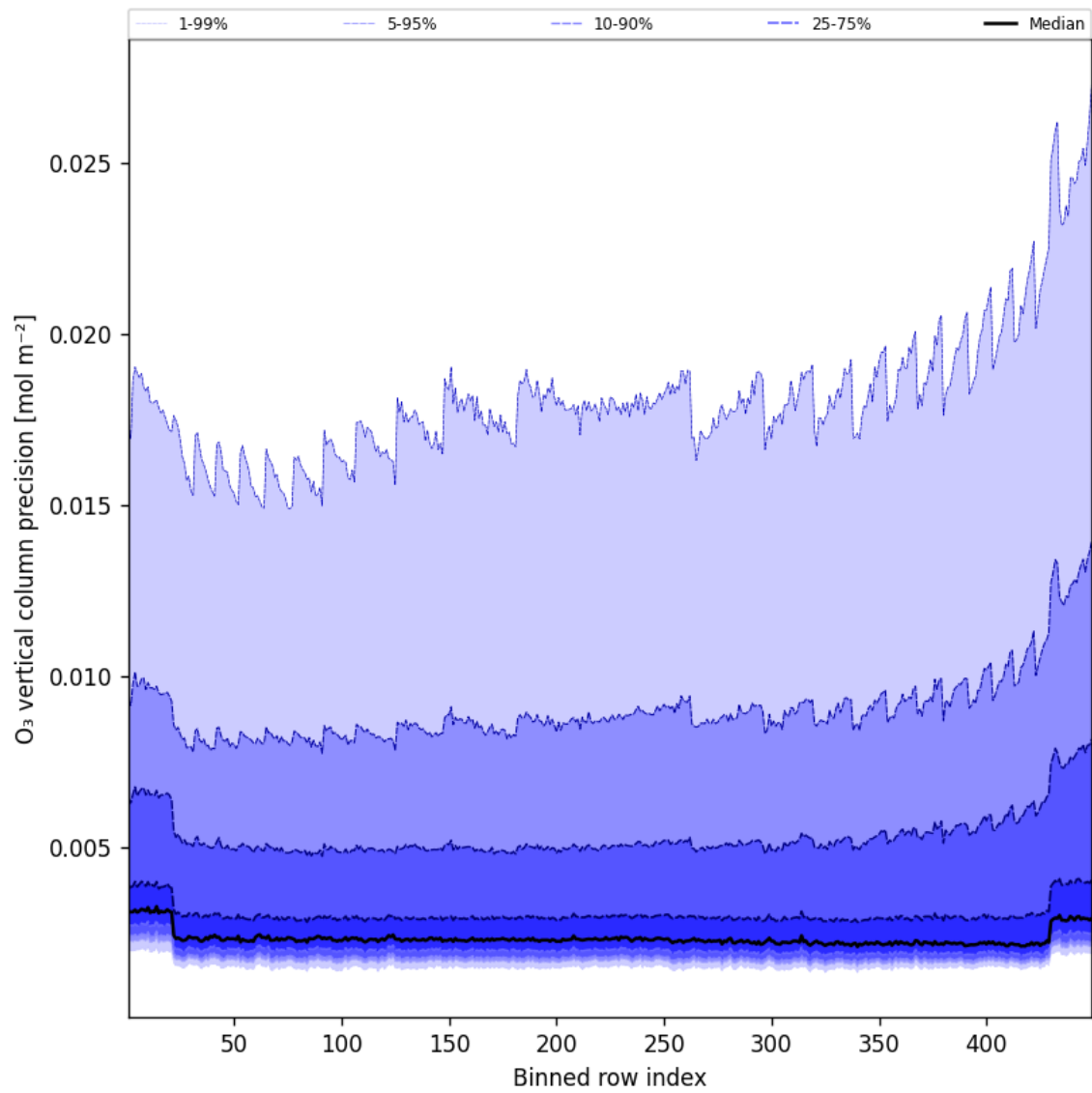
Figure 42: Along track statistics of “O 3 vertical column precision” for 2025-09-13 to 2025-09-13
