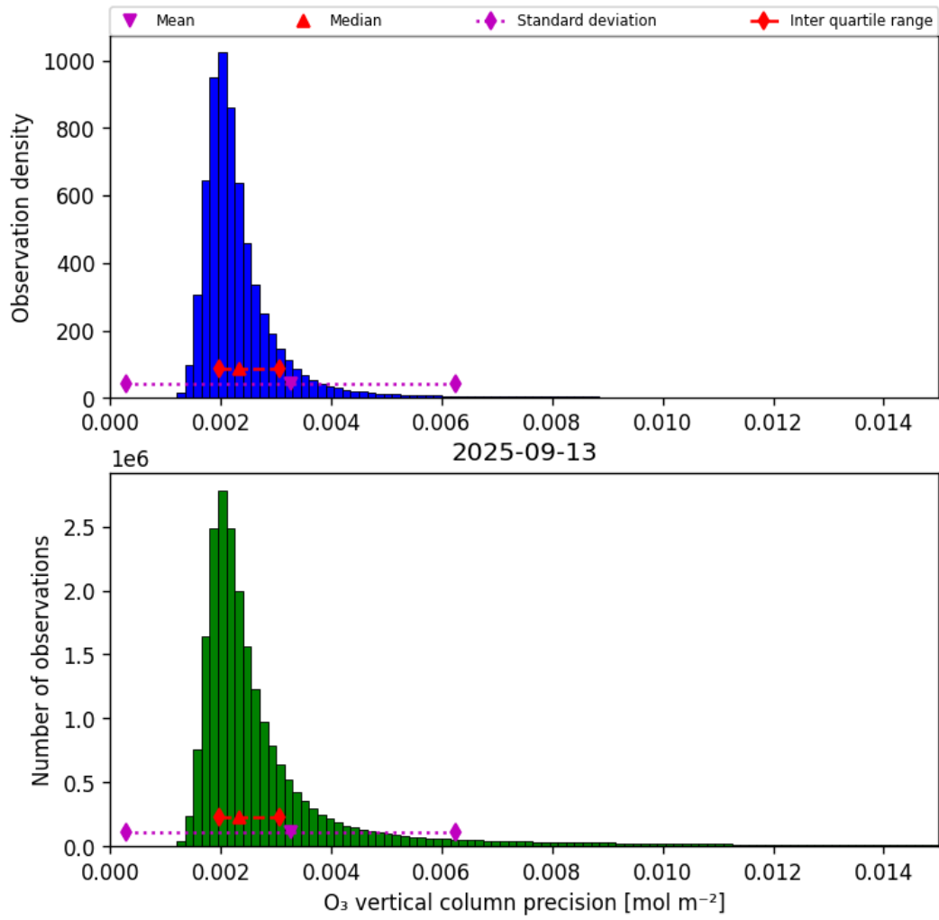
Figure 30: Histogram of “O 3 vertical column precision” for 2025-09-13 to 2025-09-13
