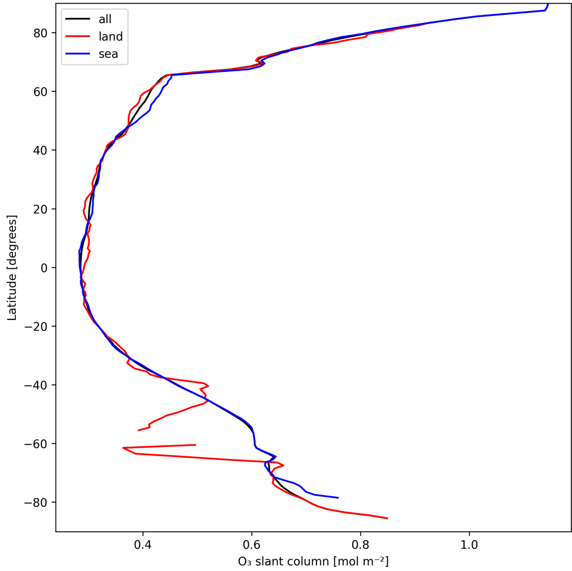
Figure 19: Zonal average of “O 3 slant column” for 2025-09-13 to 2025-09-13.
