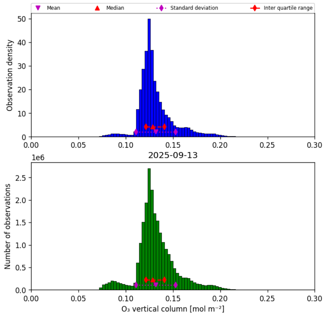
Figure 29: Histogram of “O 3 vertical column” for 2025-09-13 to 2025-09-13
