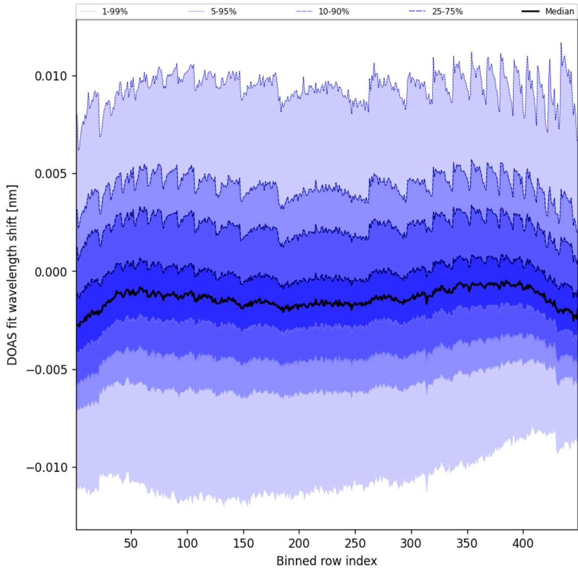
Figure 47: Along track statistics of “DOAS fit wavelength shift” for 2025-09-13 to 2025-09-13
