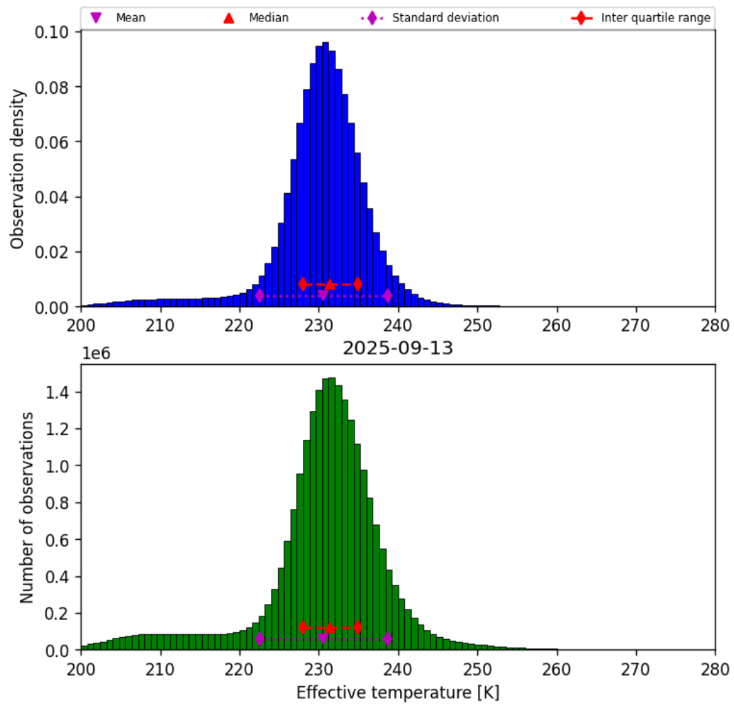
Figure 38: Histogram of “Effective temperature” for 2025-09-13 to 2025-09-13
