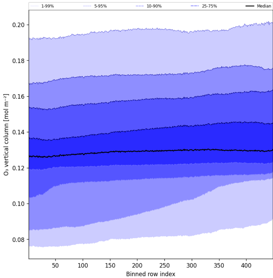
Figure 41: Along track statistics of “O 3 vertical column” for 2025-09-13 to 2025-09-13
