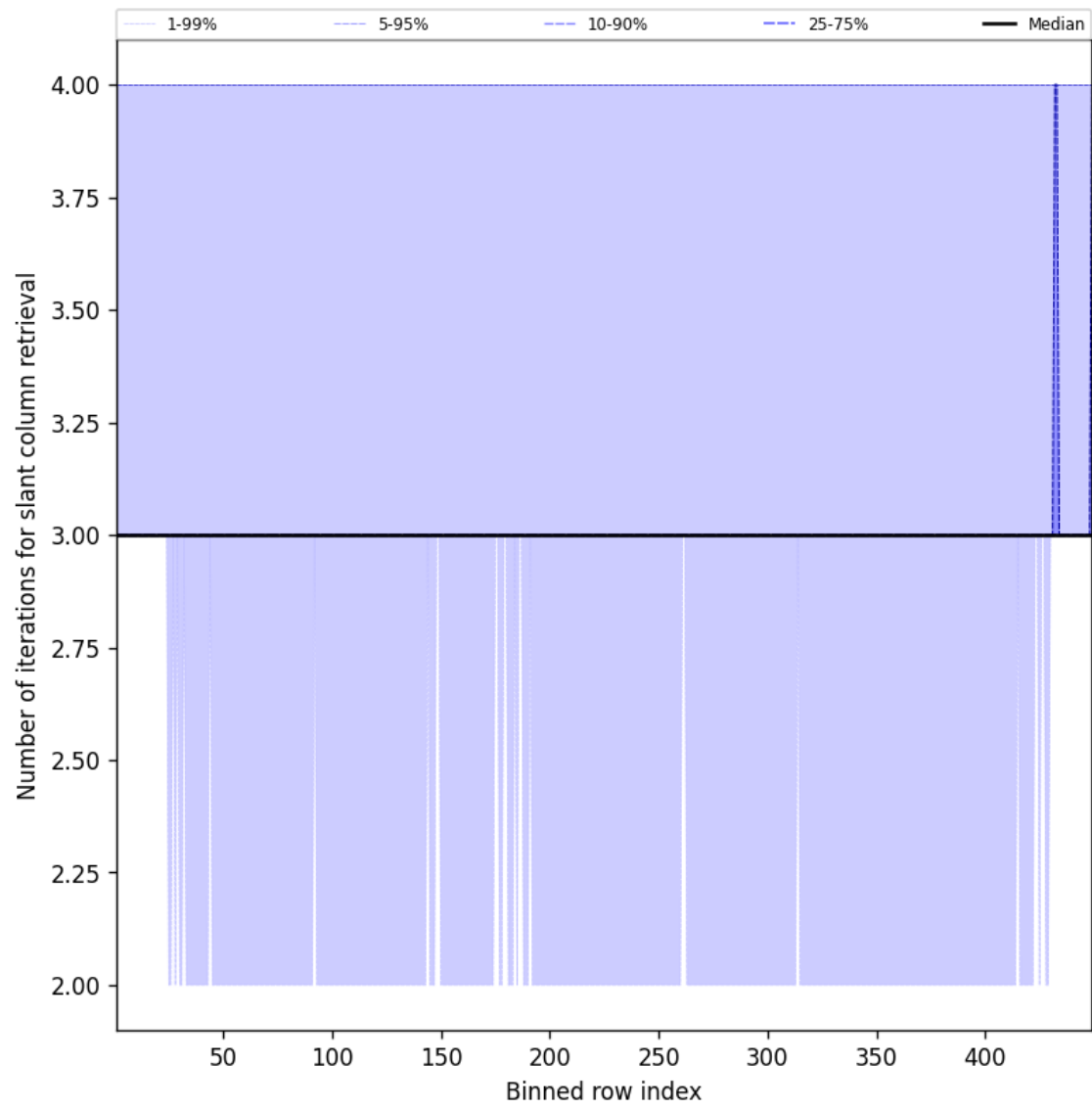
Figure 45: Along track statistics of “Number of iterations for slant column retrieval” for 2025-09-13 to 2025-09-13
