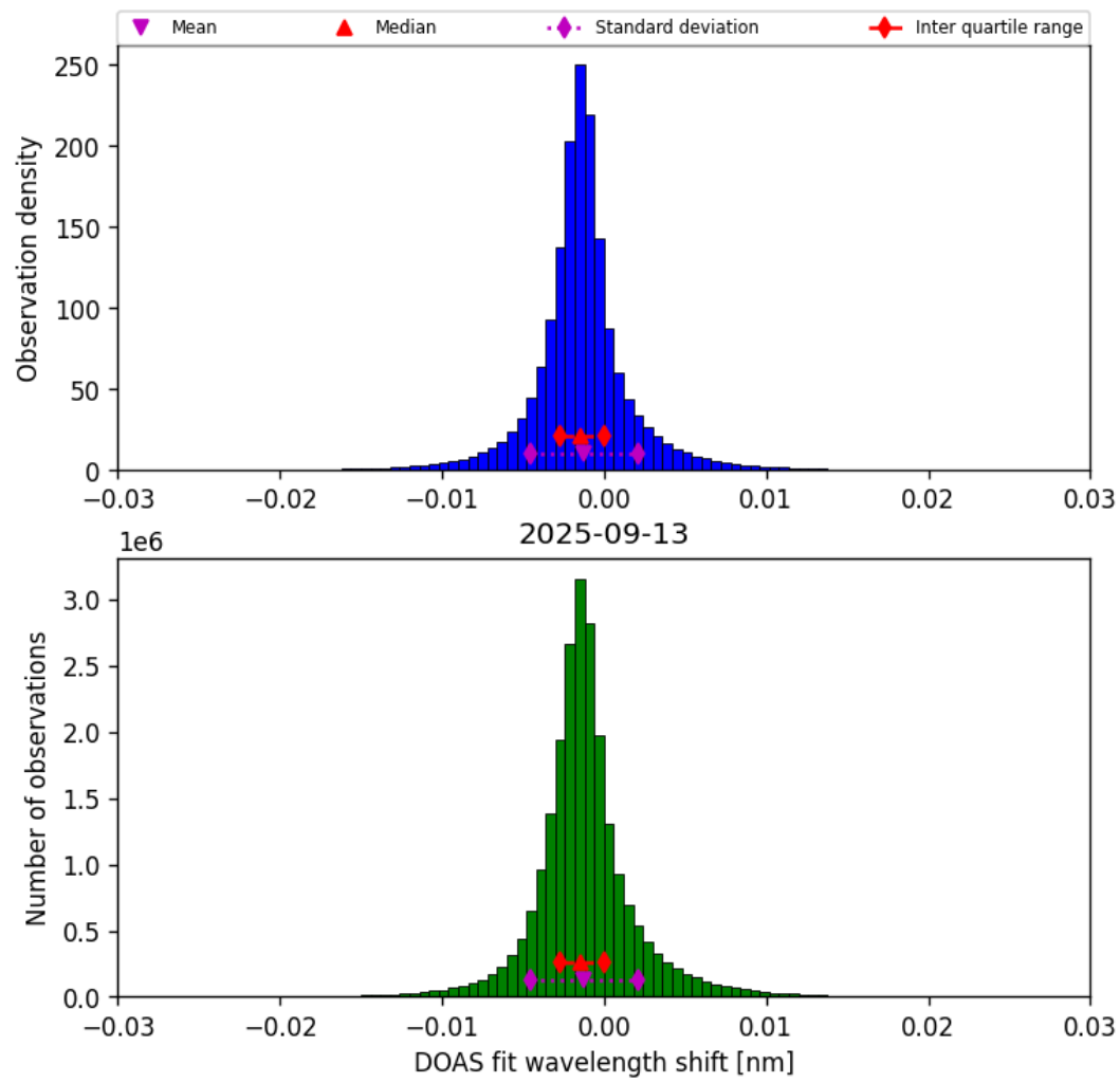
Figure 35: Histogram of “DOAS fit wavelength shift” for 2025-09-13 to 2025-09-13
