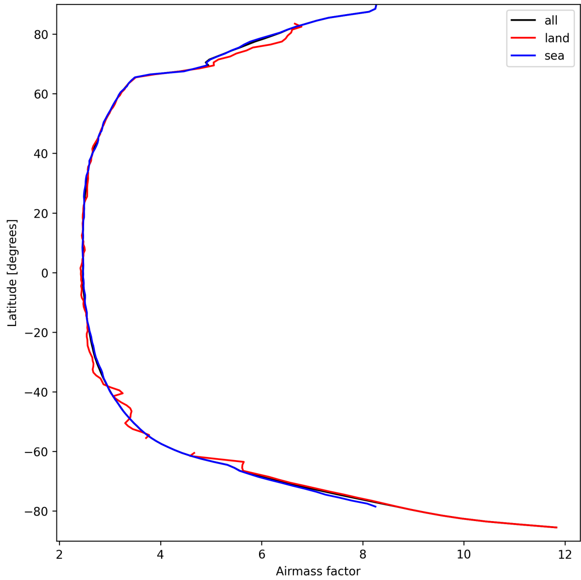
Figure 25: Zonal average of “Airmass factor” for 2025-09-14 to 2025-09-15.
