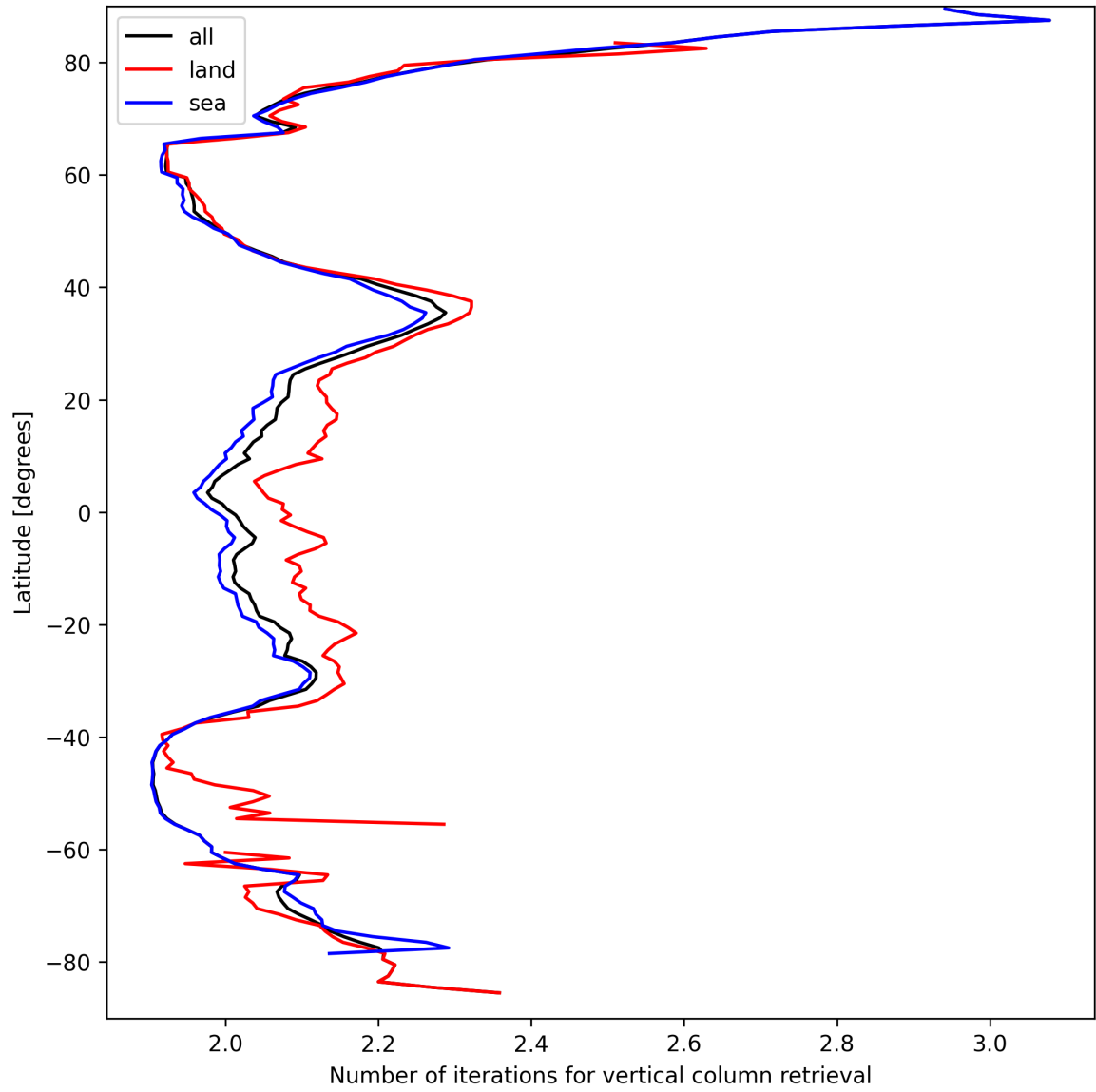
Figure 27: Zonal average of “Number of iterations for vertical column retrieval” for 2025-09-14 to 2025-09-15.
