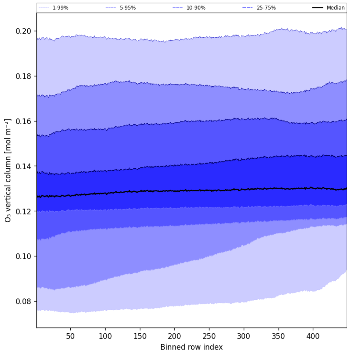
Figure 41: Along track statistics of “O 3 vertical column” for 2025-09-14 to 2025-09-15
