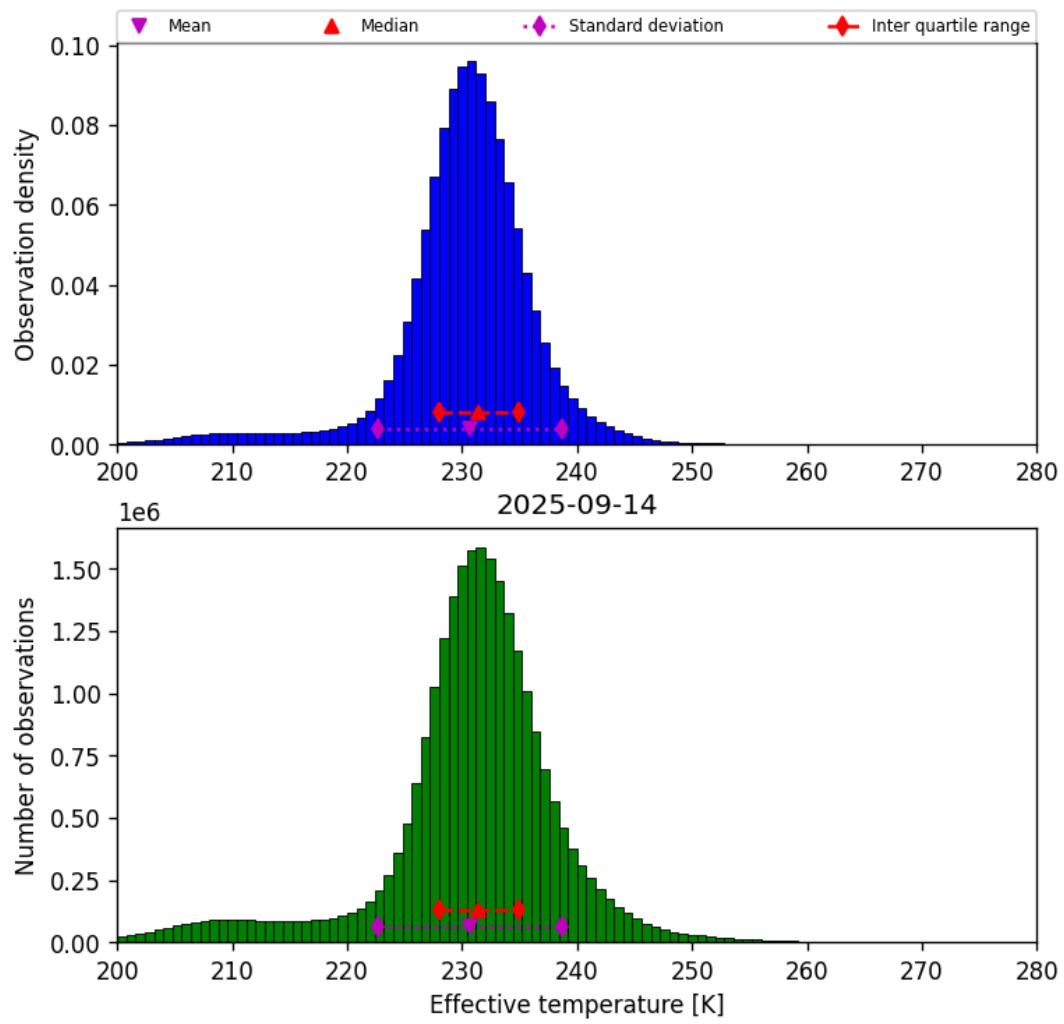
Figure 38: Histogram of “Effective temperature” for 2025-09-14 to 2025-09-15
