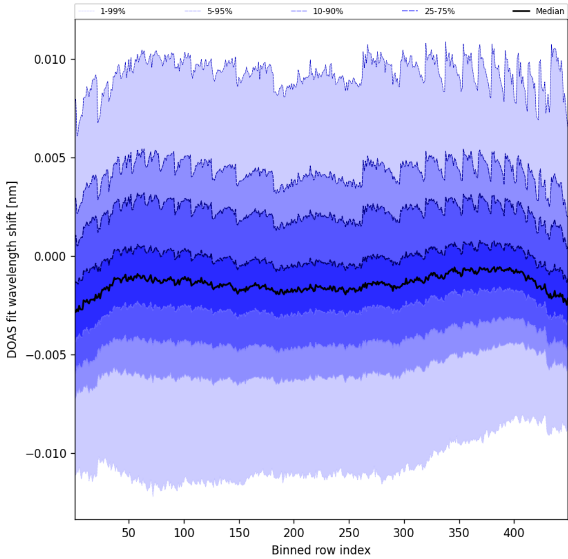
Figure 47: Along track statistics of “DOAS fit wavelength shift” for 2025-09-14 to 2025-09-15
