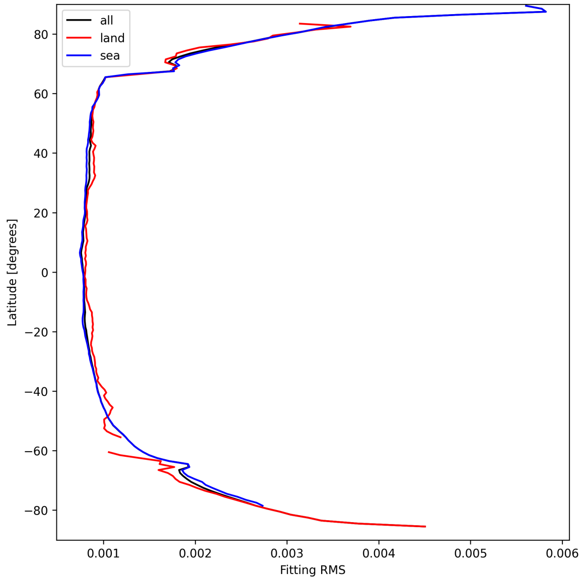
Figure 22: Zonal average of “Fitting RMS” for 2025-09-14 to 2025-09-15.
