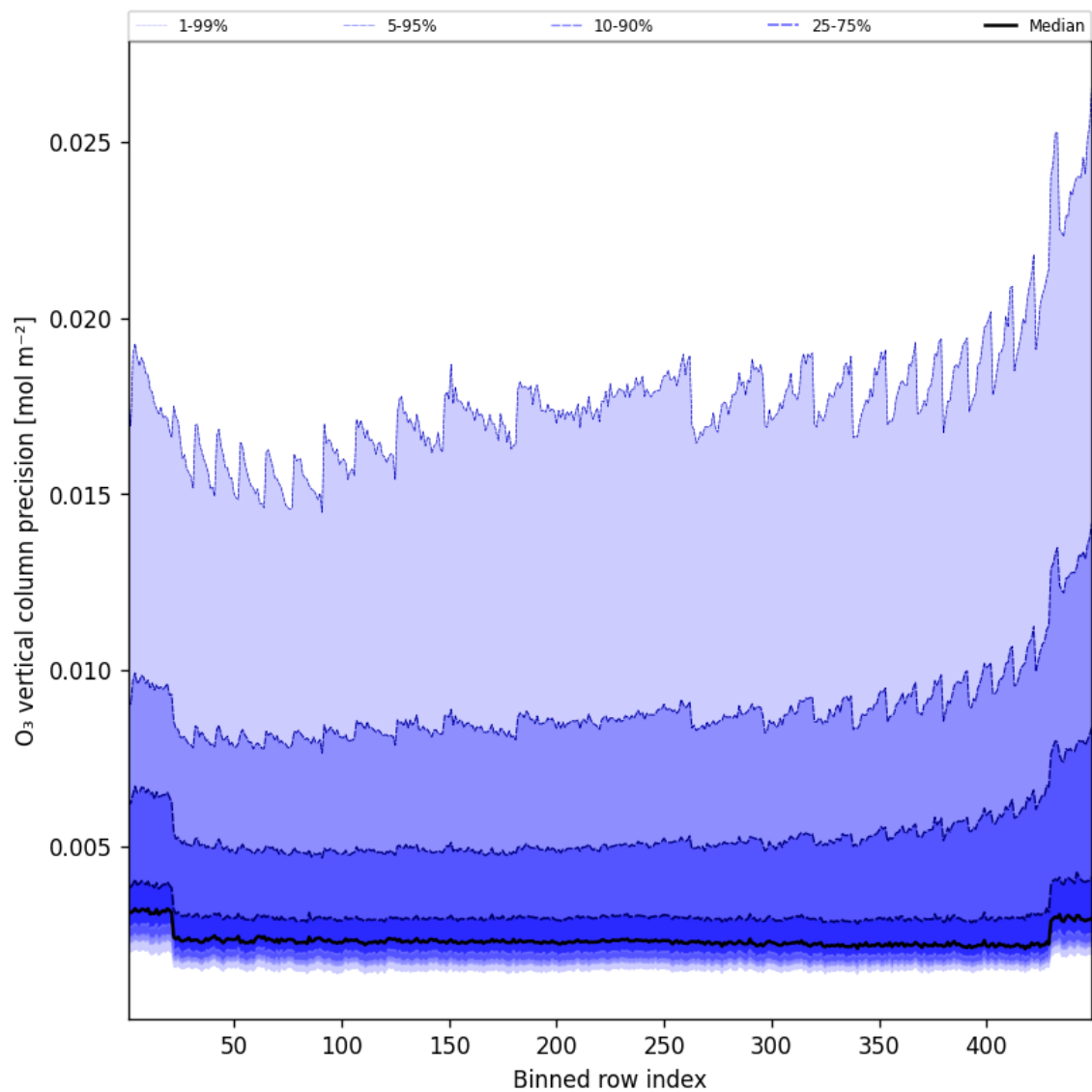
Figure 42: Along track statistics of “O 3 vertical column precision” for 2025-09-14 to 2025-09-15
