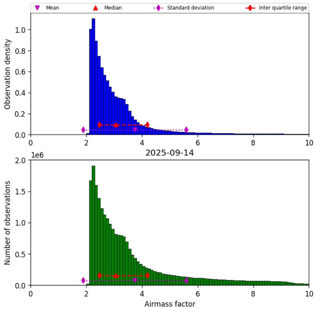
Figure 37: Histogram of “Airmass factor” for 2025-09-14 to 2025-09-15
