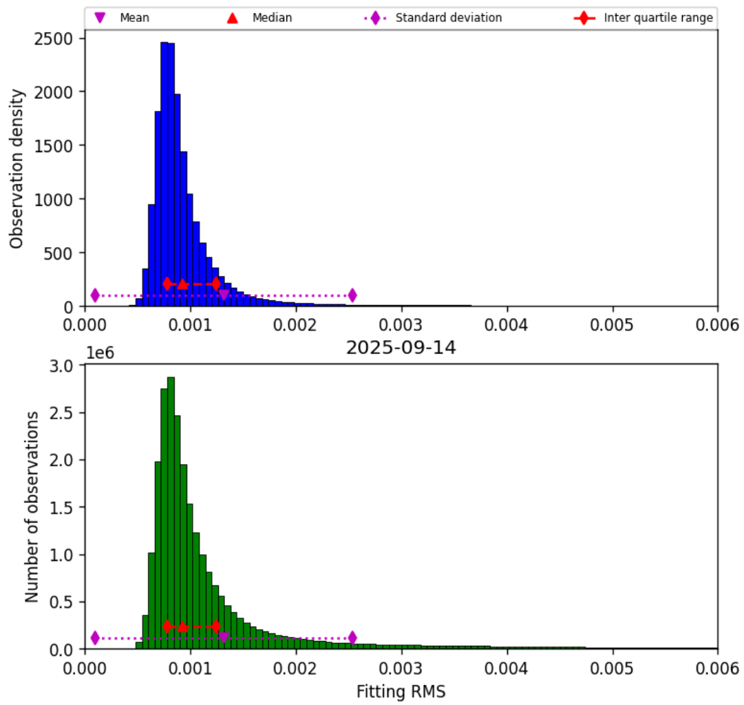
Figure 34: Histogram of “Fitting RMS” for 2025-09-14 to 2025-09-15
