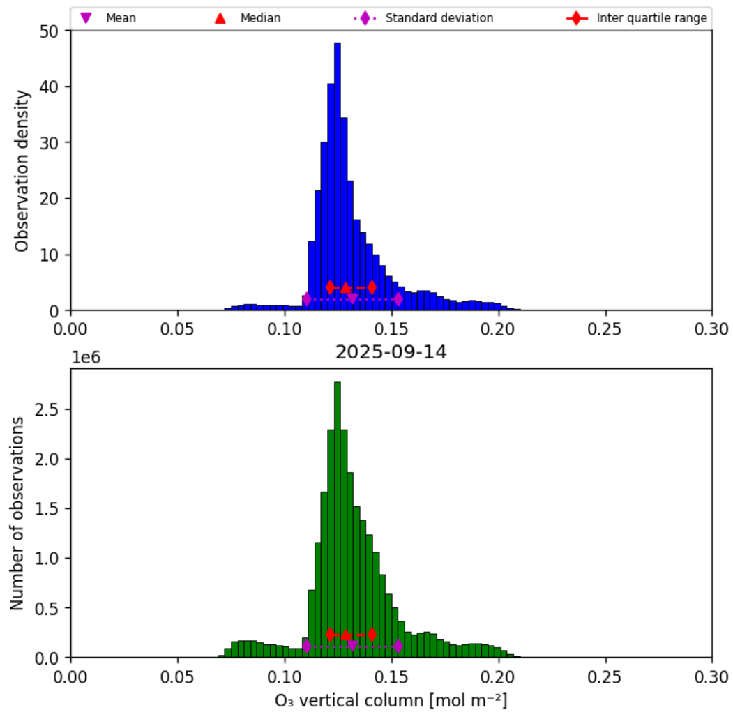
Figure 29: Histogram of “O 3 vertical column” for 2025-09-14 to 2025-09-15
