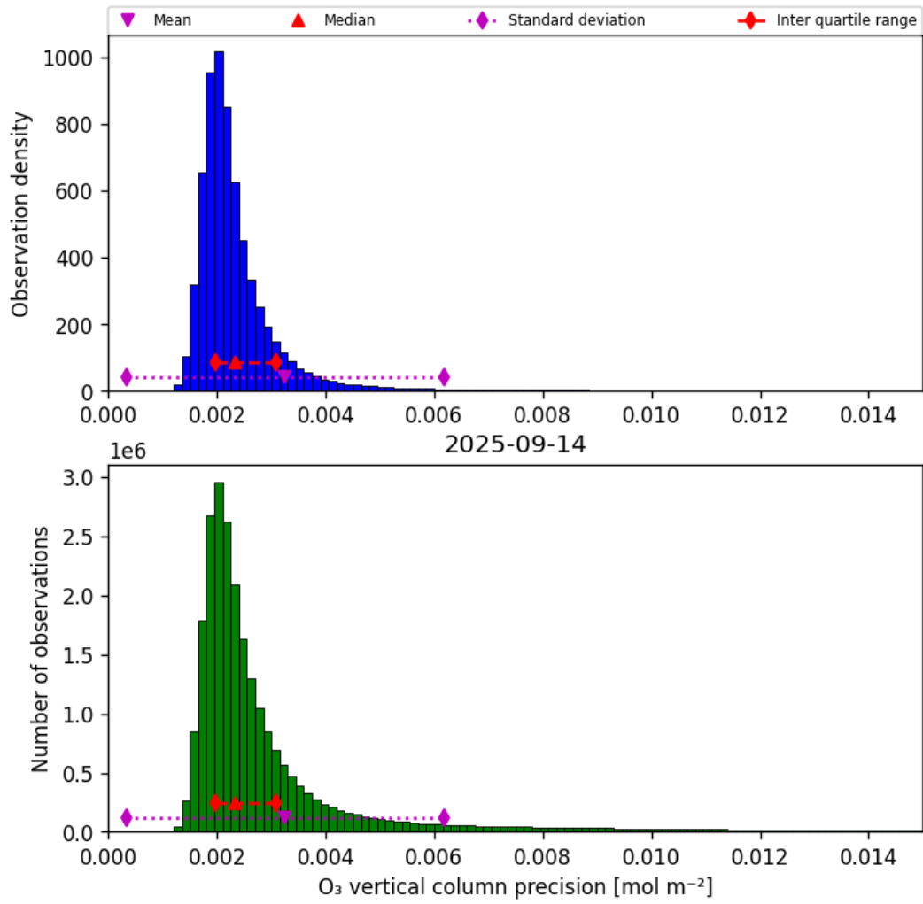
Figure 30: Histogram of “O 3 vertical column precision” for 2025-09-14 to 2025-09-15
