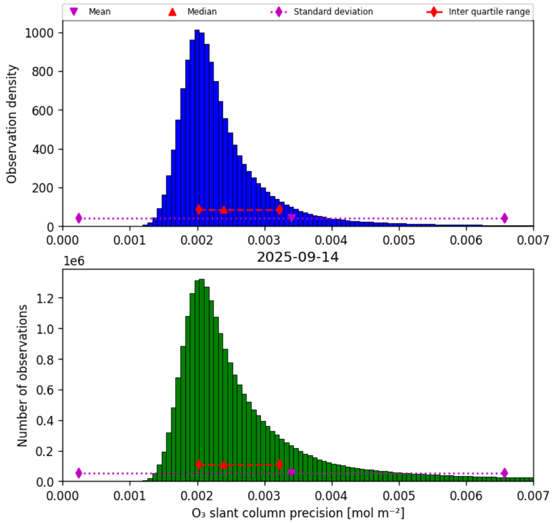
Figure 32: Histogram of “O 3 slant column precision” for 2025-09-14 to 2025-09-15
