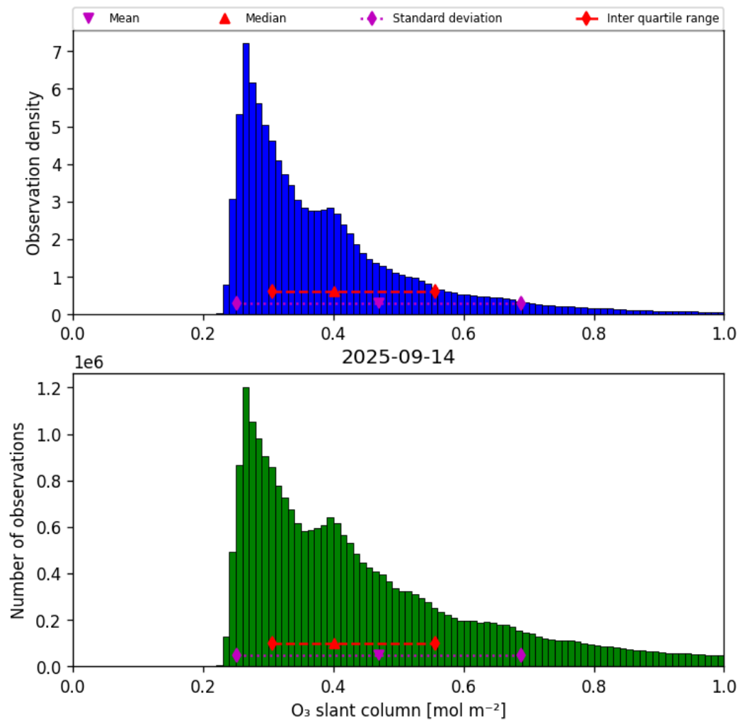
Figure 31: Histogram of “O 3 slant column” for 2025-09-14 to 2025-09-15
