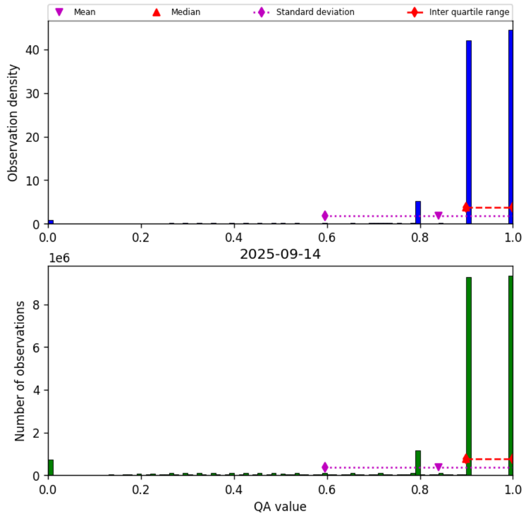
Figure 28: Histogram of “QA value” for 2025-09-14 to 2025-09-15
