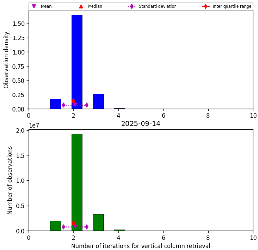
Figure 39: Histogram of “Number of iterations for vertical column retrieval” for 2025-09-14 to 2025-09-15
