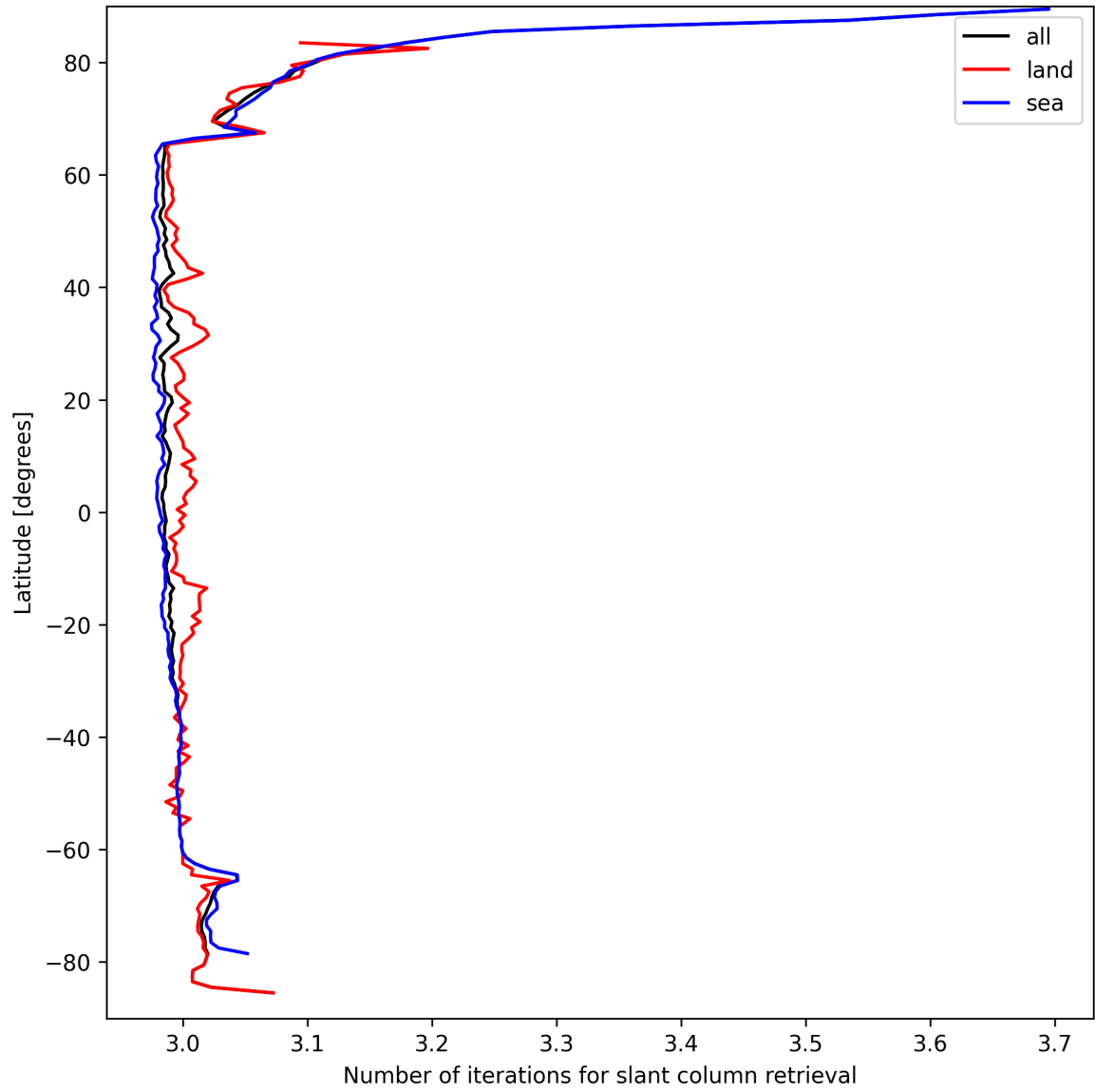
Figure 21: Zonal average of “Number of iterations for slant column retrieval” for 2025-09-14 to 2025-09-15.
