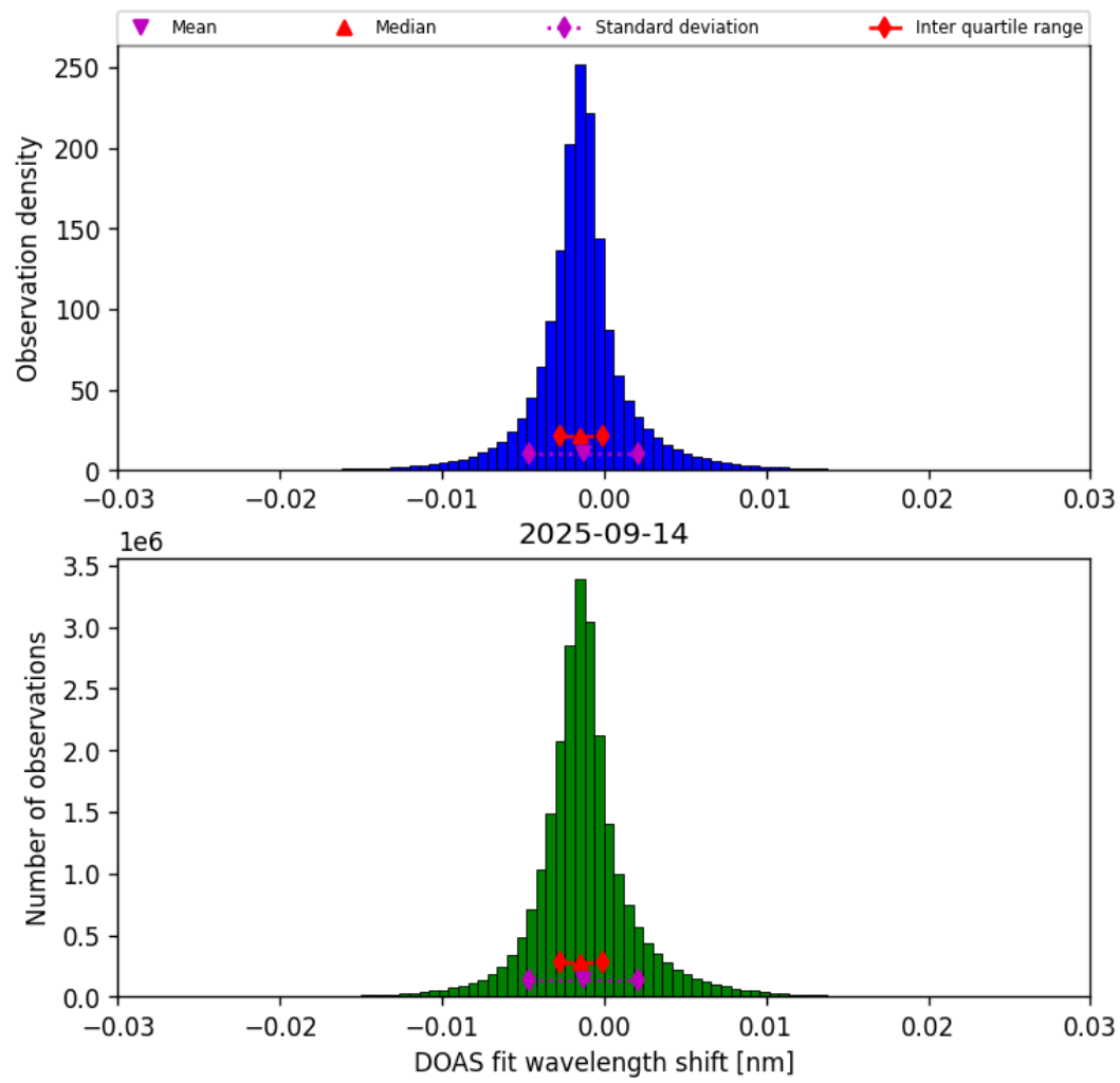
Figure 35: Histogram of “DOAS fit wavelength shift” for 2025-09-14 to 2025-09-15
