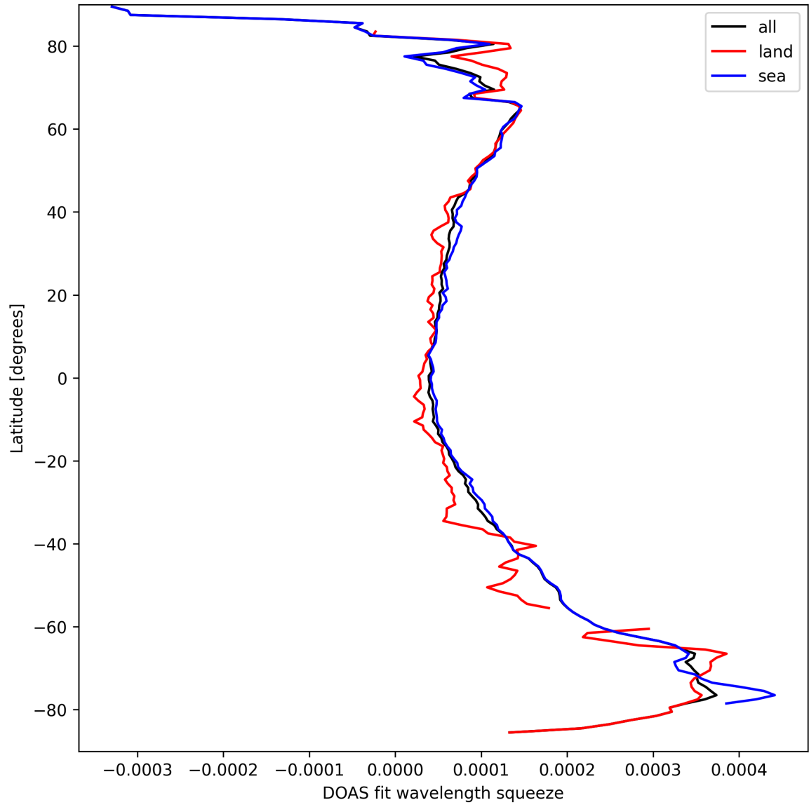
Figure 24: Zonal average of “DOAS fit wavelength squeeze” for 2025-09-14 to 2025-09-15.
