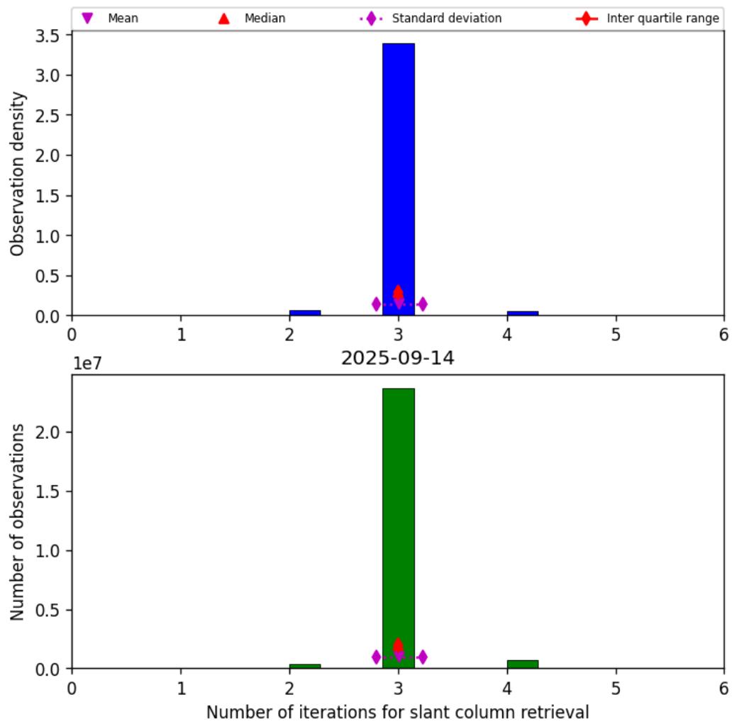
Figure 33: Histogram of “Number of iterations for slant column retrieval” for 2025-09-14 to 2025-09-15
