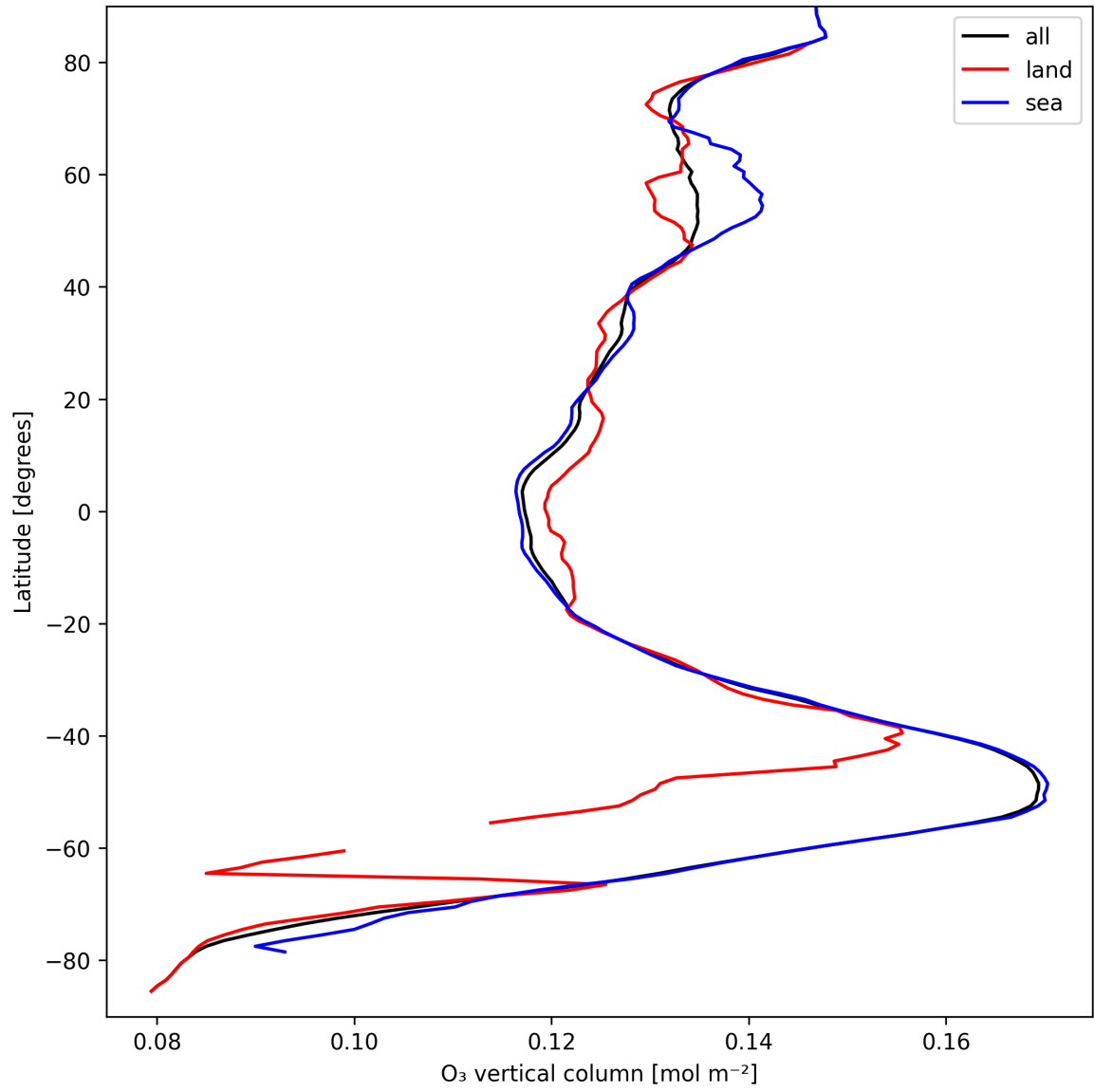
Figure 17: Zonal average of “O 3 vertical column” for 2025-09-14 to 2025-09-15.
