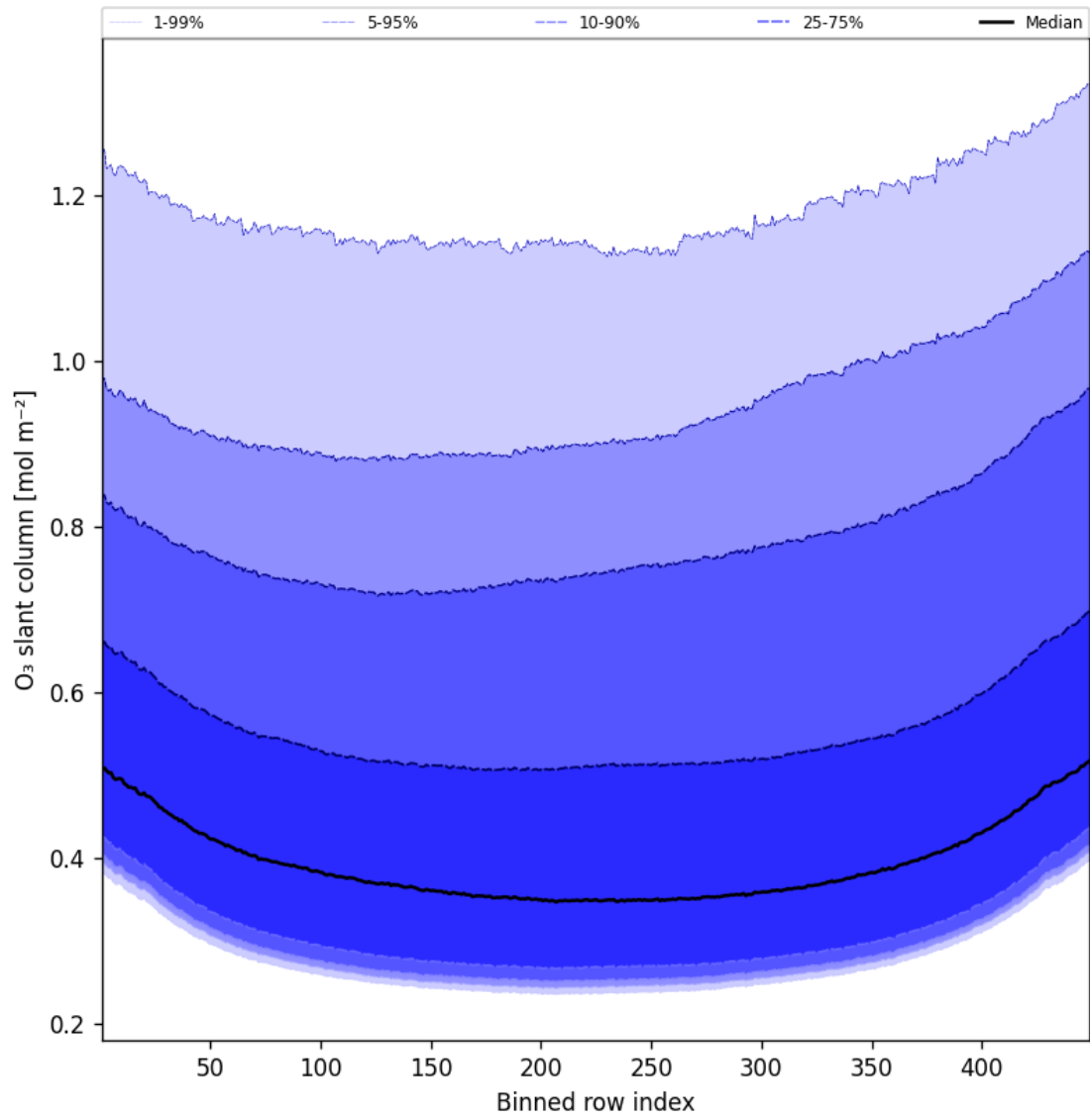
Figure 43: Along track statistics of “O 3 slant column” for 2025-09-14 to 2025-09-15
