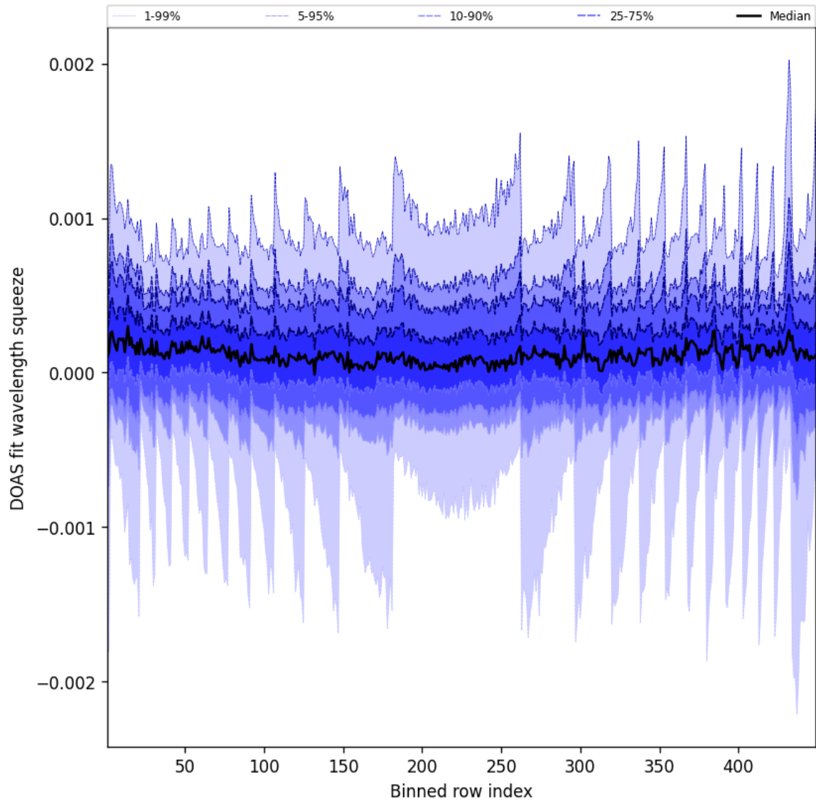
Figure 48: Along track statistics of “DOAS fit wavelength squeeze” for 2025-09-14 to 2025-09-15
