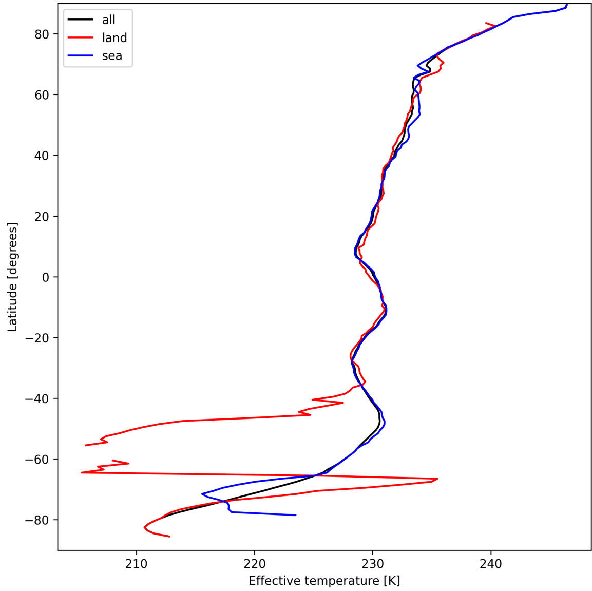
Figure 26: Zonal average of “Effective temperature” for 2025-09-14 to 2025-09-15.
