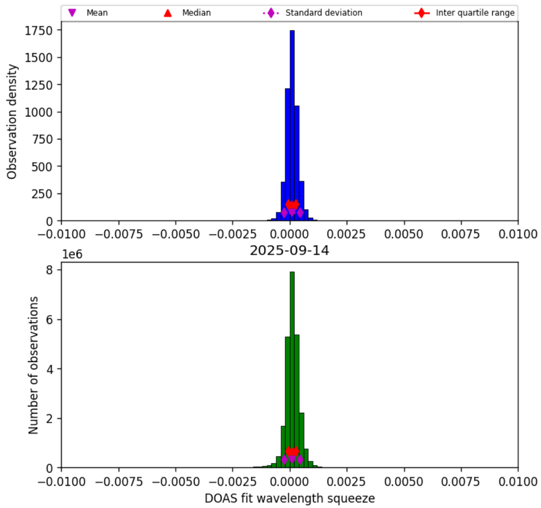
Figure 36: Histogram of “DOAS fit wavelength squeeze” for 2025-09-14 to 2025-09-15
