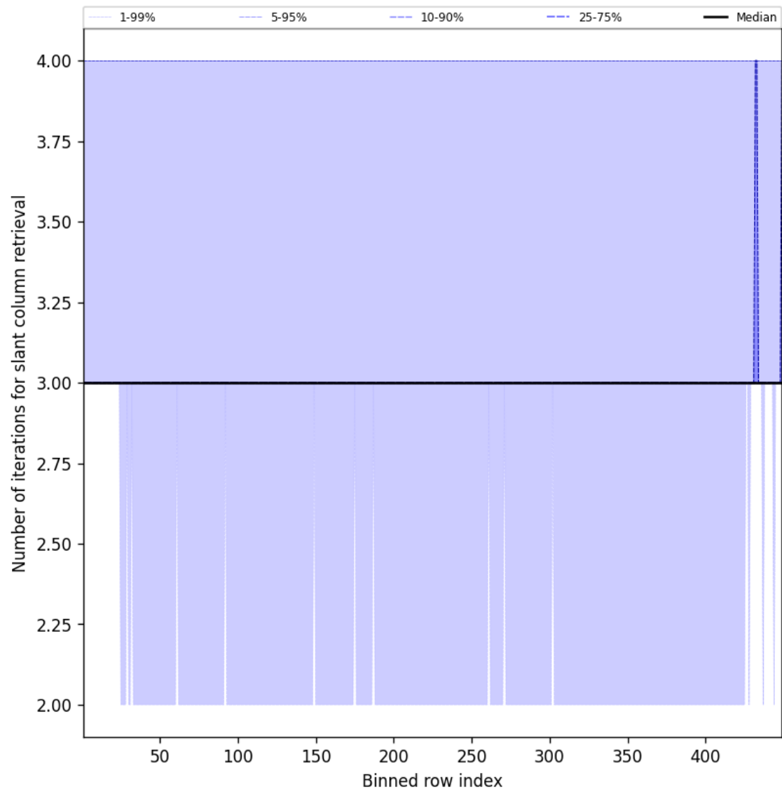
Figure 45: Along track statistics of “Number of iterations for slant column retrieval” for 2025-09-14 to 2025-09-15
