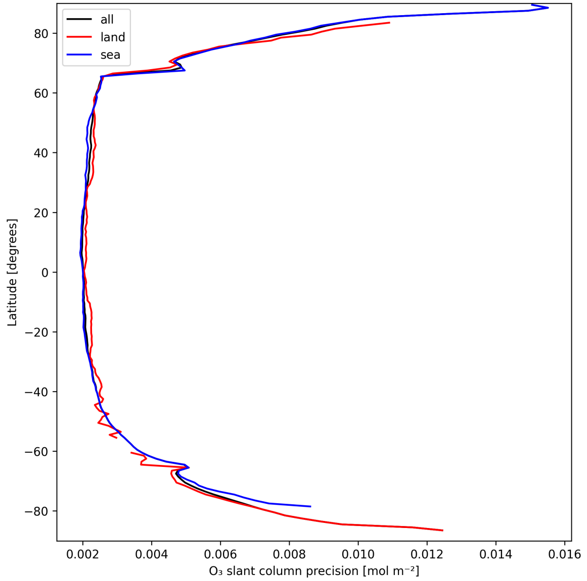
Figure 20: Zonal average of “O 3 slant column precision” for 2025-09-15 to 2025-09-16.
