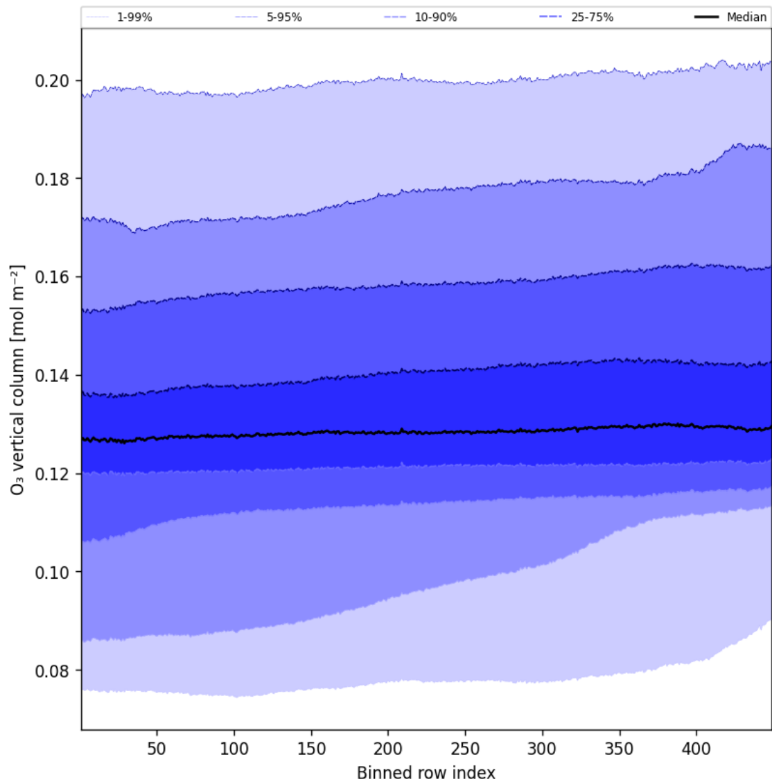
Figure 41: Along track statistics of “O 3 vertical column” for 2025-09-15 to 2025-09-16
