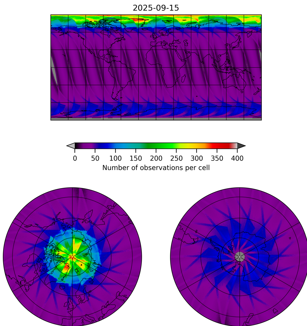
Figure 15: Map of the number of observations for 2025-09-15 to 2025-09-16
