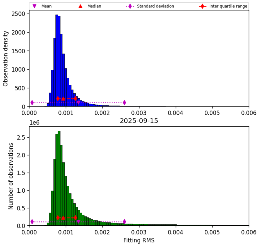
Figure 34: Histogram of “Fitting RMS” for 2025-09-15 to 2025-09-16
