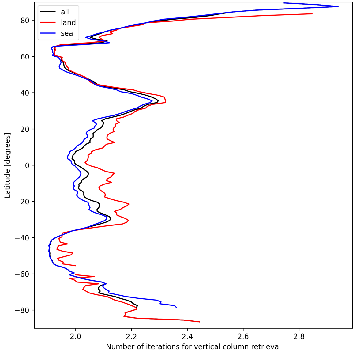
Figure 27: Zonal average of “Number of iterations for vertical column retrieval” for 2025-09-15 to 2025-09-16.
