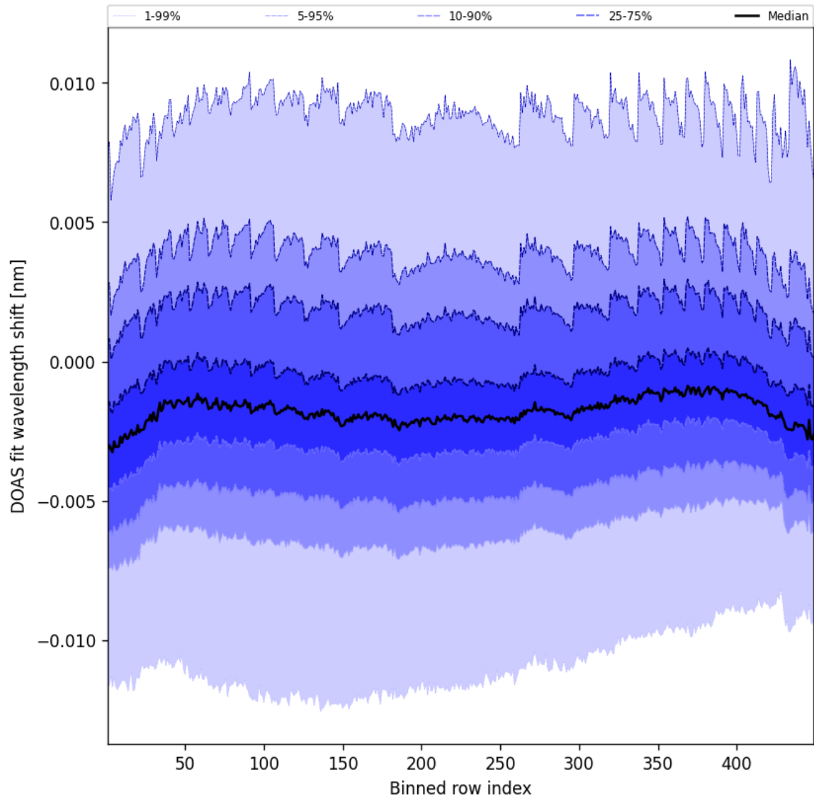
Figure 47: Along track statistics of “DOAS fit wavelength shift” for 2025-09-15 to 2025-09-16
