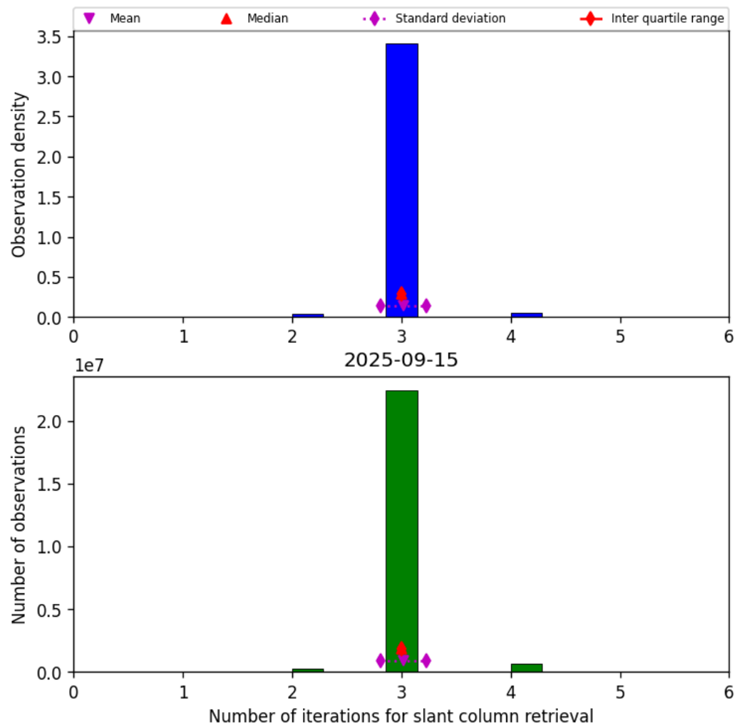
Figure 33: Histogram of “Number of iterations for slant column retrieval” for 2025-09-15 to 2025-09-16
