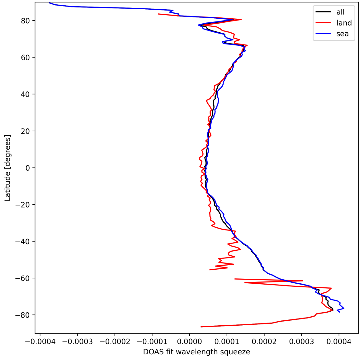
Figure 24: Zonal average of “DOAS fit wavelength squeeze” for 2025-09-15 to 2025-09-16.
