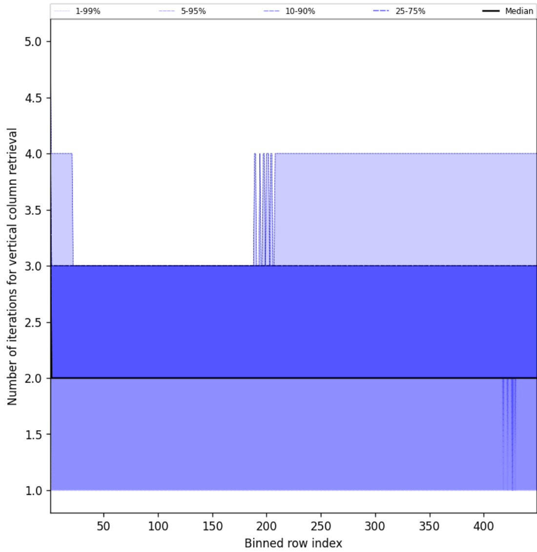
Figure 51: Along track statistics of “Number of iterations for vertical column retrieval” for 2025-09-15 to 2025-09-16
