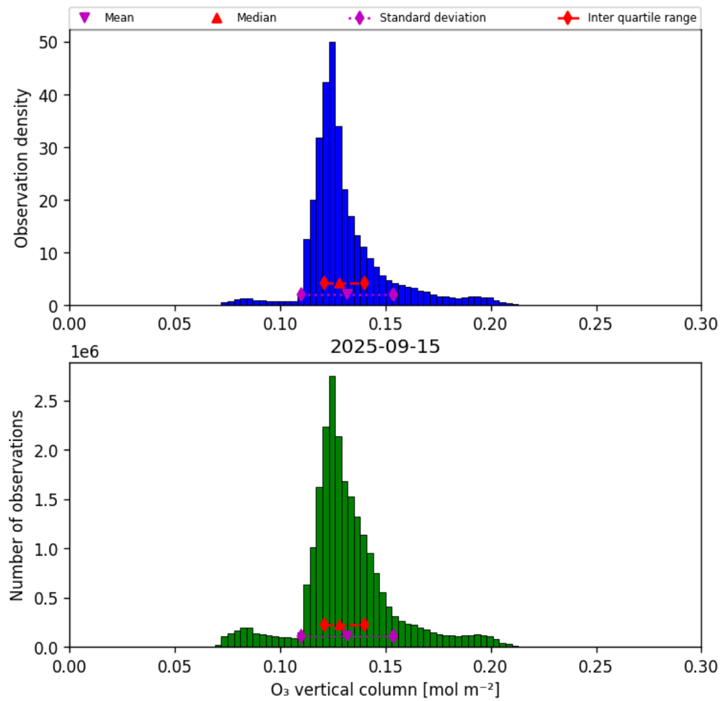
Figure 29: Histogram of “O 3 vertical column” for 2025-09-15 to 2025-09-16
