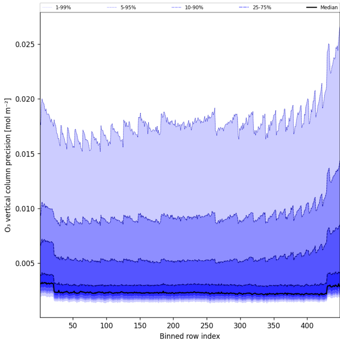
Figure 42: Along track statistics of “O 3 vertical column precision” for 2025-09-15 to 2025-09-16
