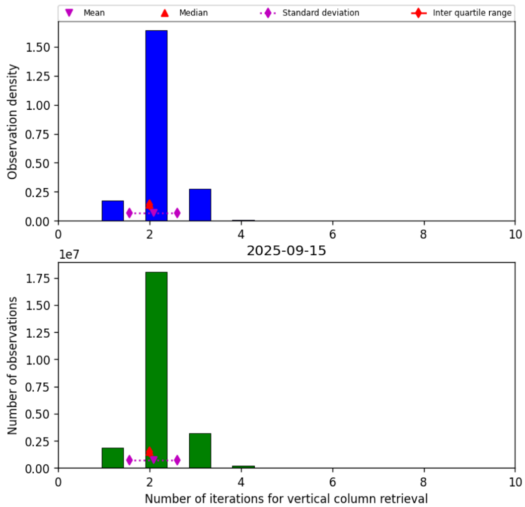
Figure 39: Histogram of “Number of iterations for vertical column retrieval” for 2025-09-15 to 2025-09-16
