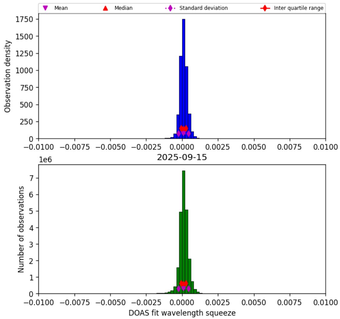
Figure 36: Histogram of “DOAS fit wavelength squeeze” for 2025-09-15 to 2025-09-16
