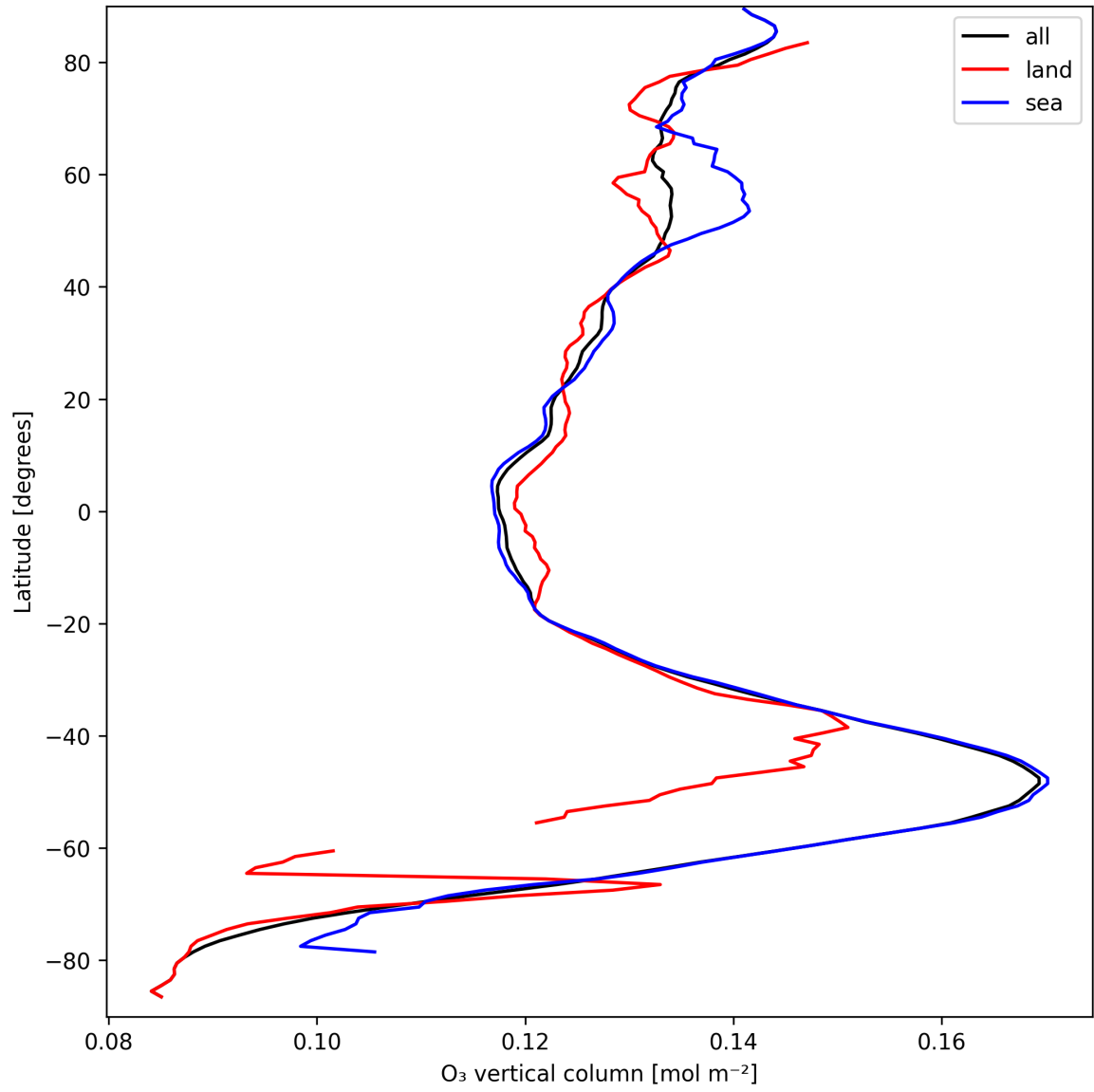
Figure 17: Zonal average of “O 3 vertical column” for 2025-09-15 to 2025-09-16.
