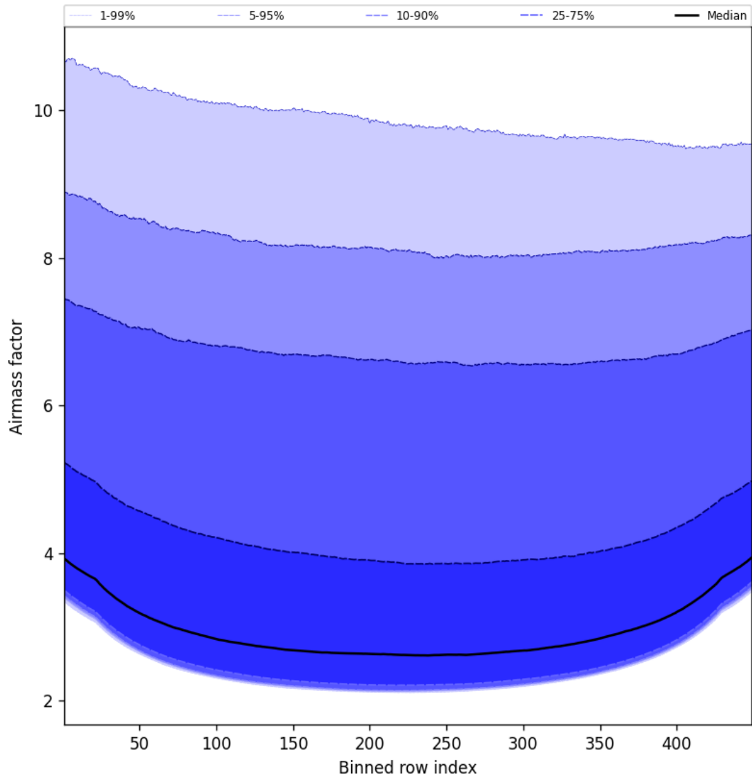
Figure 49: Along track statistics of “Airmass factor” for 2025-09-15 to 2025-09-16
