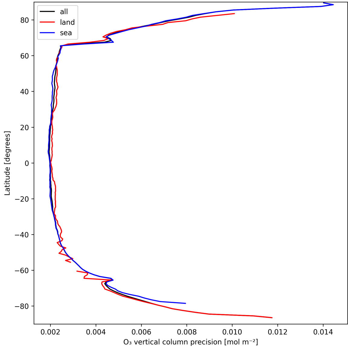
Figure 18: Zonal average of “O 3 vertical column precision” for 2025-09-15 to 2025-09-16.
