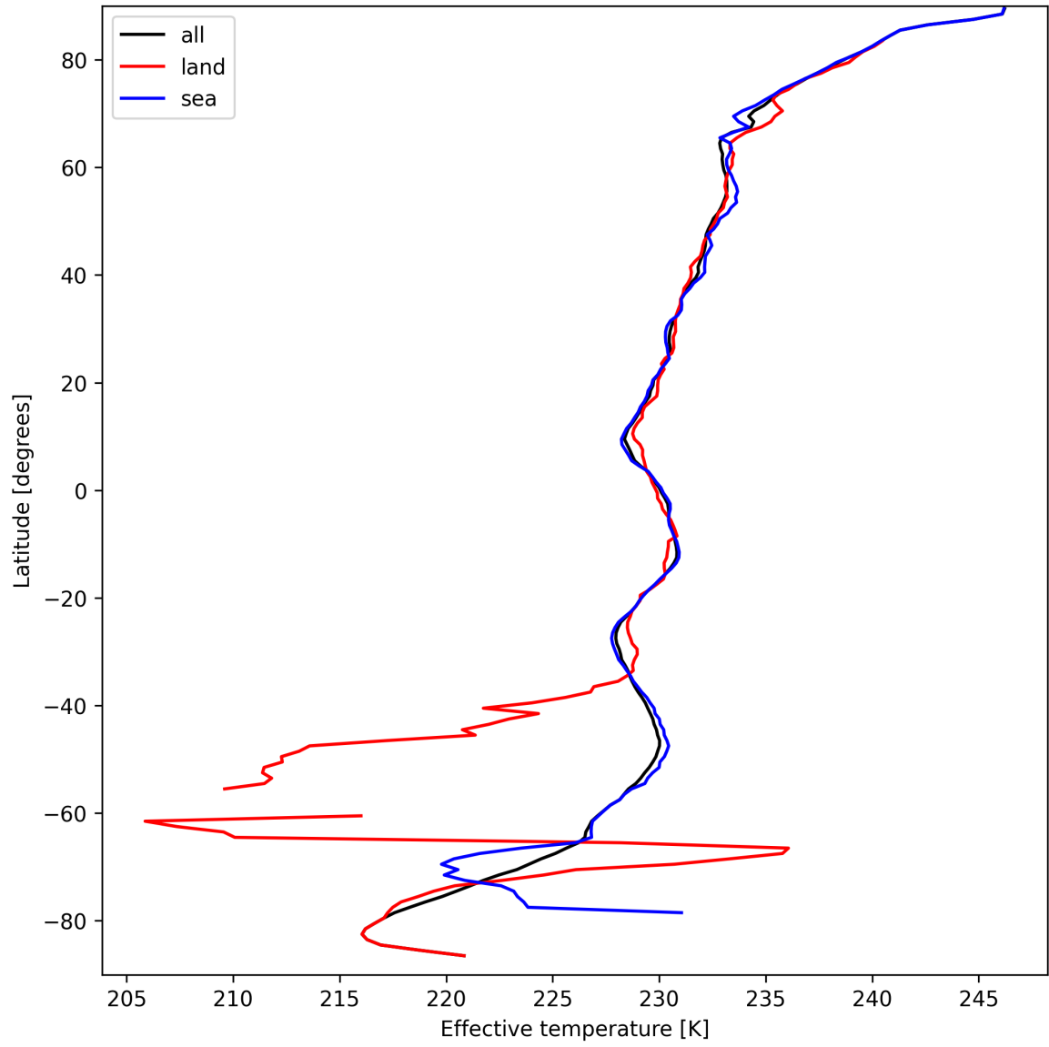
Figure 26: Zonal average of “Effective temperature” for 2025-09-15 to 2025-09-16.
