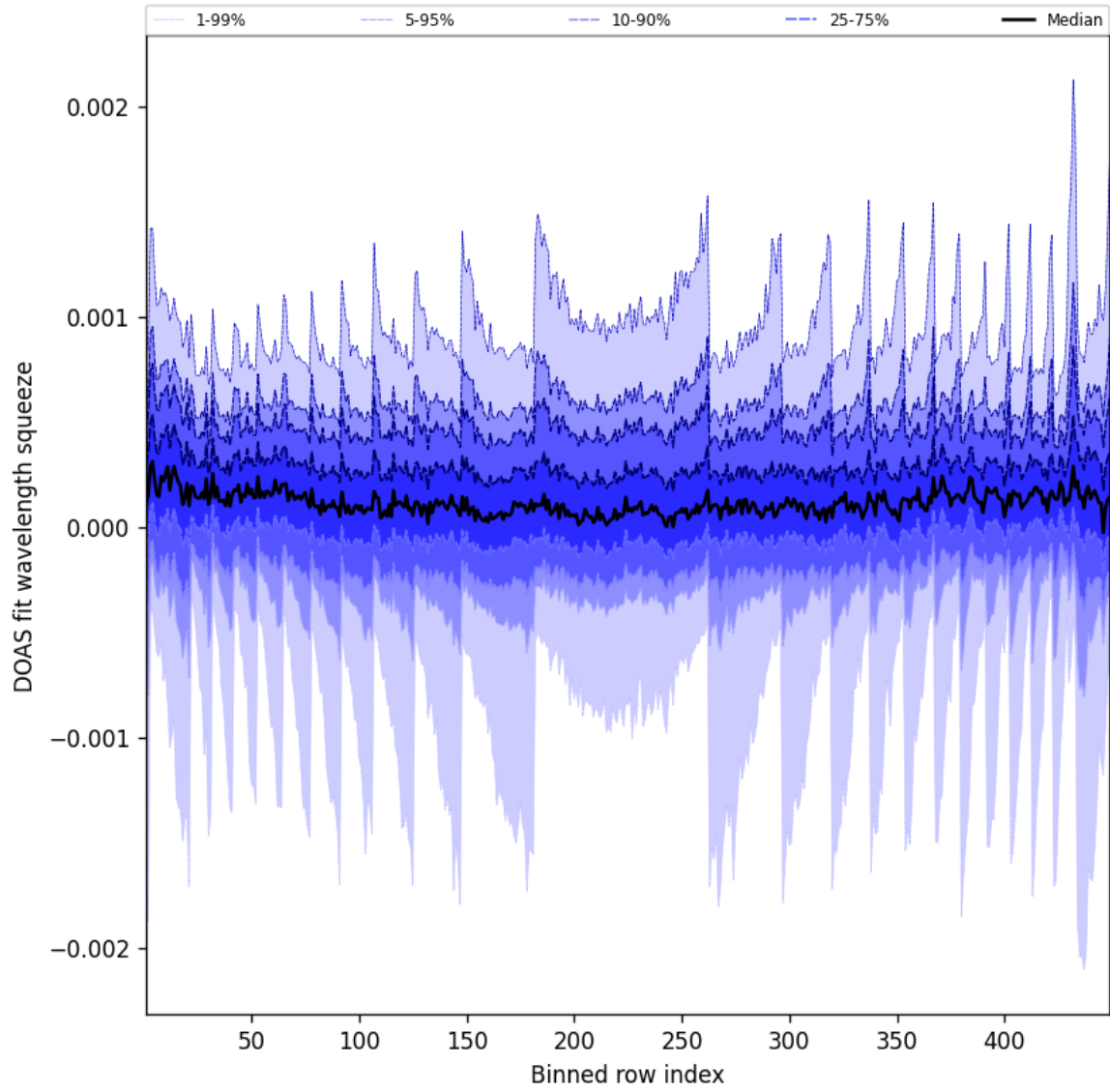
Figure 48: Along track statistics of “DOAS fit wavelength squeeze” for 2025-09-15 to 2025-09-16
