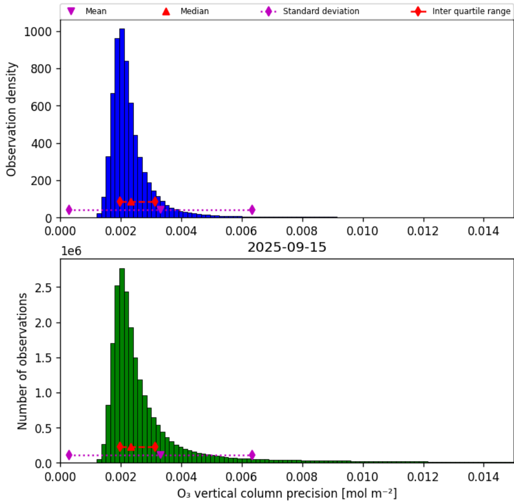
Figure 30: Histogram of “O 3 vertical column precision” for 2025-09-15 to 2025-09-16
