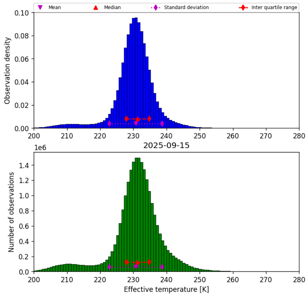
Figure 38: Histogram of “Effective temperature” for 2025-09-15 to 2025-09-16
