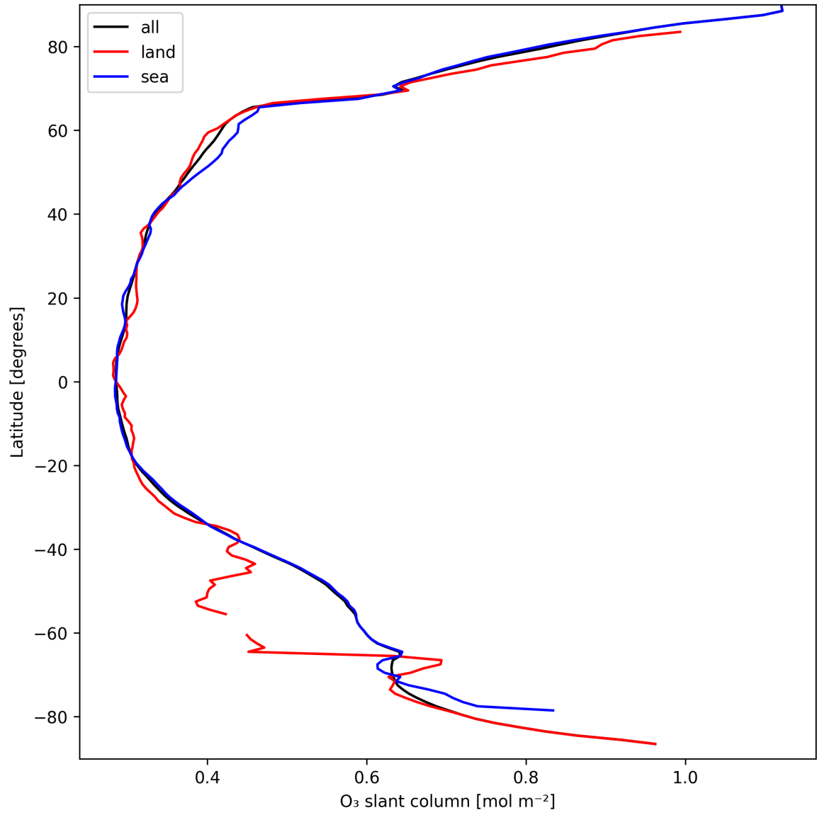
Figure 19: Zonal average of “O 3 slant column” for 2025-09-15 to 2025-09-16.
