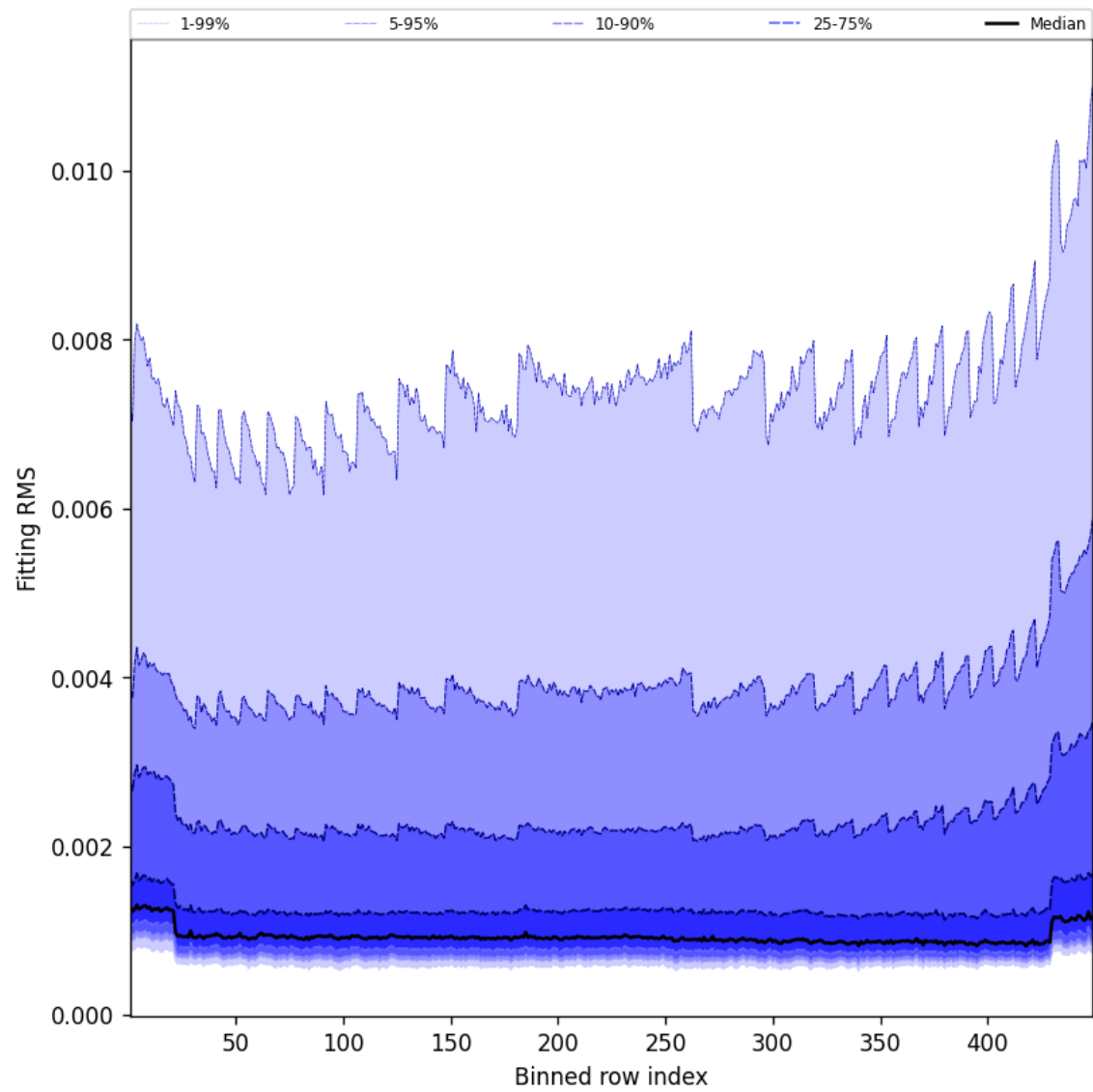
Figure 46: Along track statistics of “Fitting RMS” for 2025-09-15 to 2025-09-16
