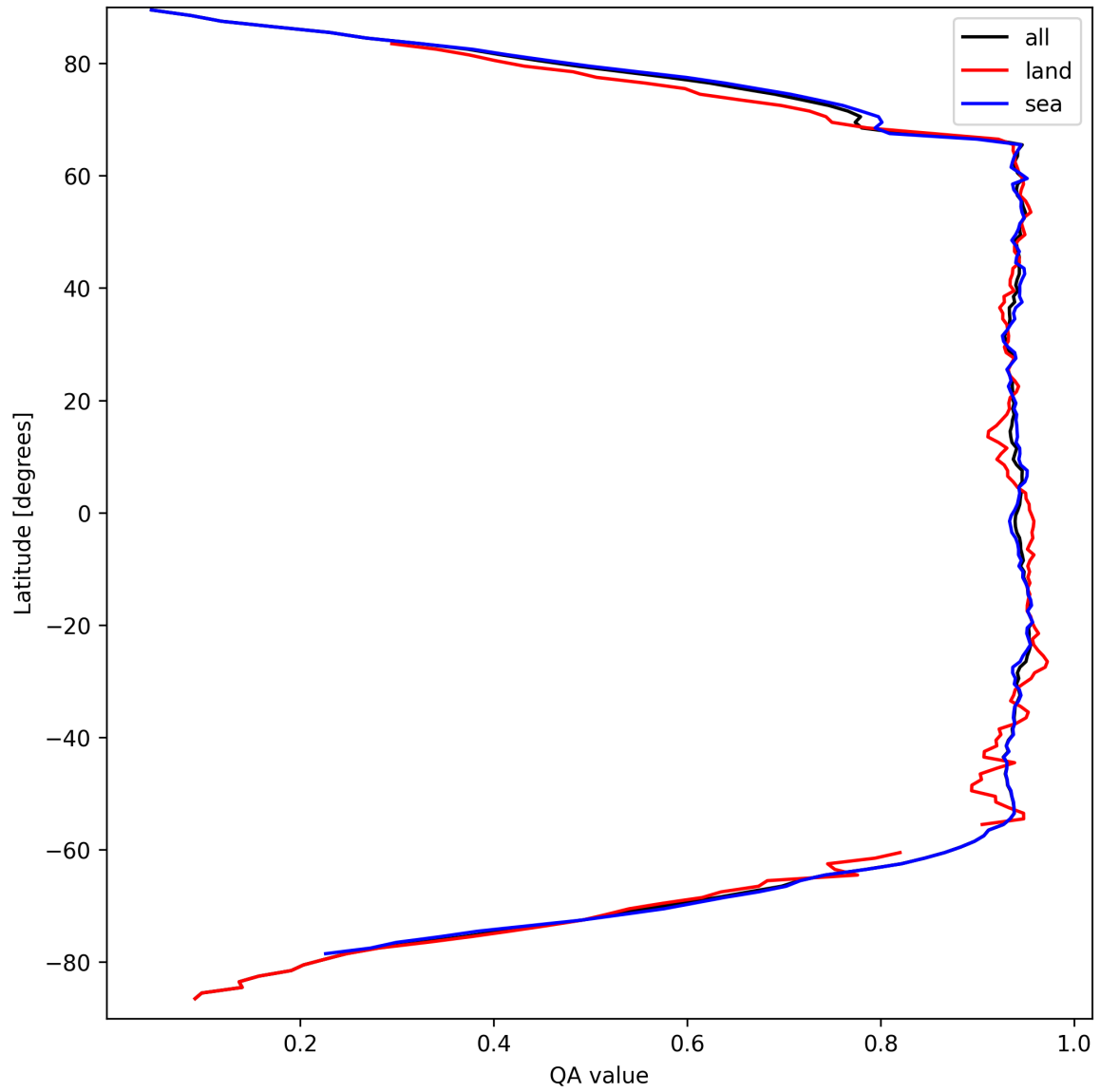
Figure 16: Zonal average of “QA value” for 2025-09-15 to 2025-09-16.
