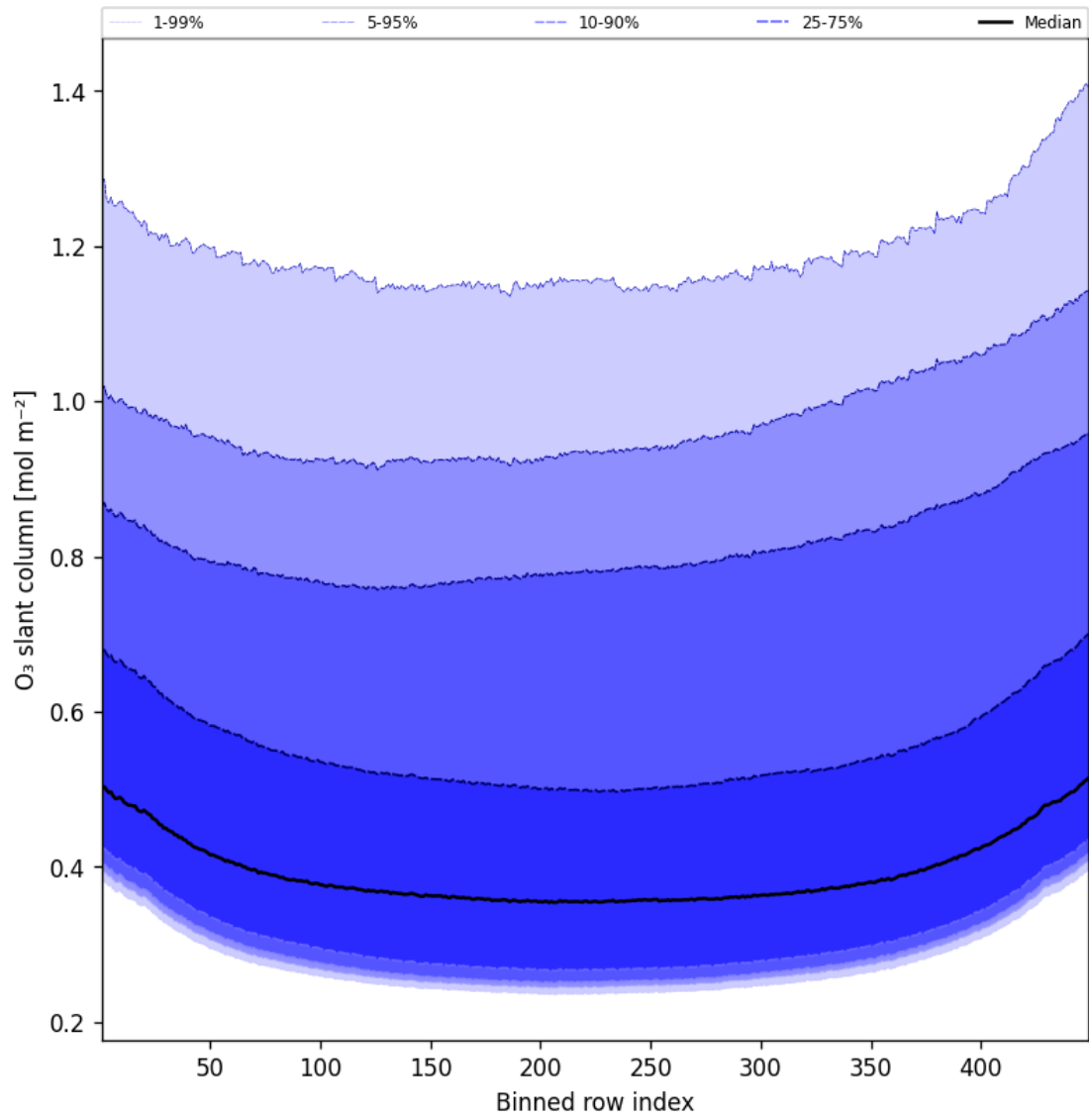
Figure 43: Along track statistics of “O 3 slant column” for 2025-09-15 to 2025-09-16
