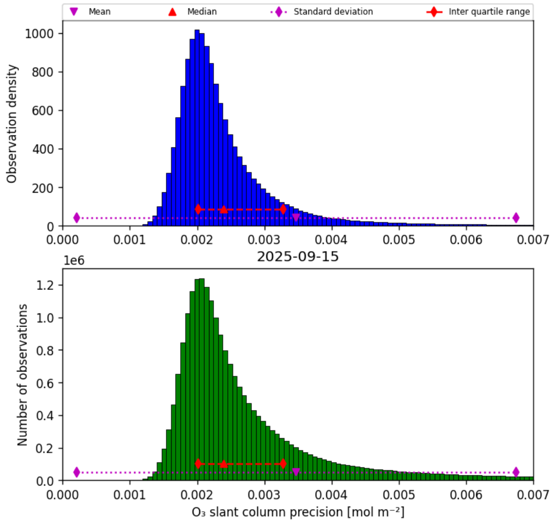
Figure 32: Histogram of “O 3 slant column precision” for 2025-09-15 to 2025-09-16
