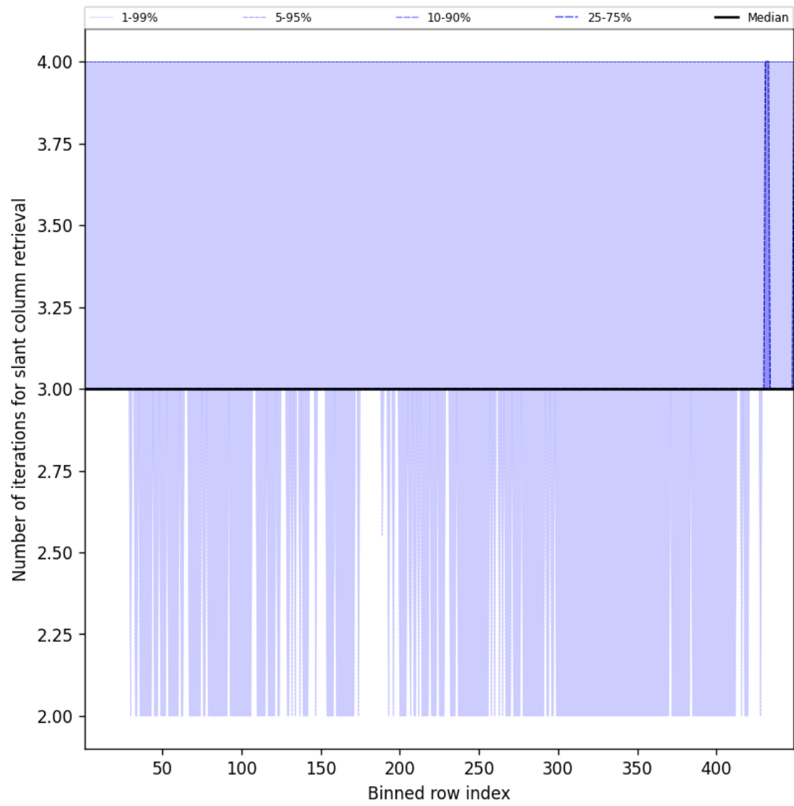
Figure 45: Along track statistics of “Number of iterations for slant column retrieval” for 2025-09-15 to 2025-09-16
