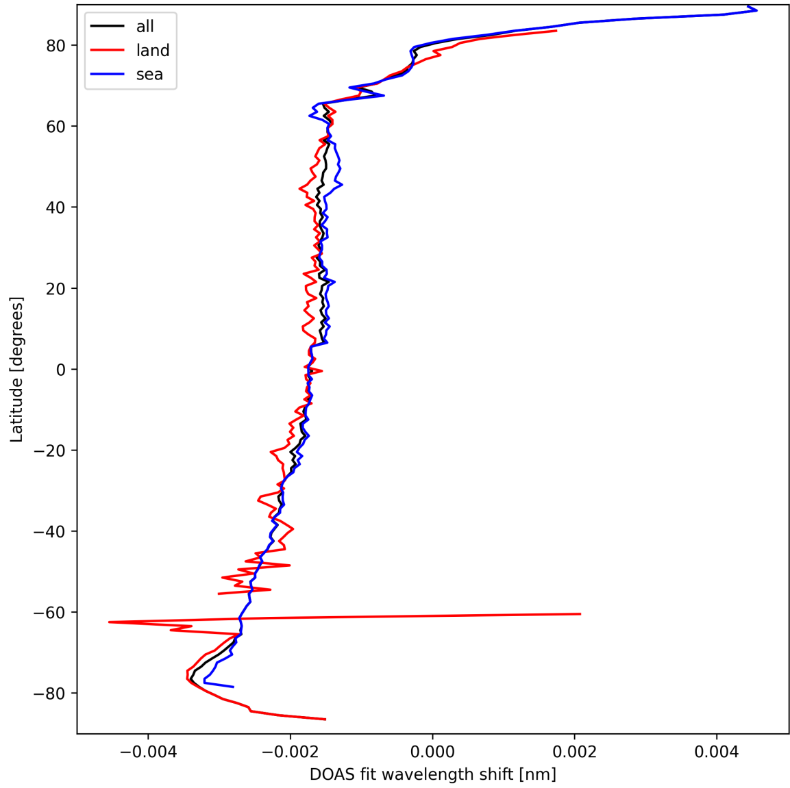
Figure 23: Zonal average of "DOAS fit wavelength shift" for 2025-09-15 to 2025-09-16.
