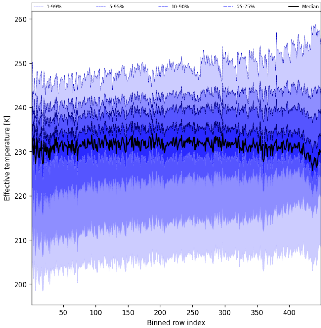
Figure 50: Along track statistics of “Effective temperature” for 2025-09-15 to 2025-09-16
