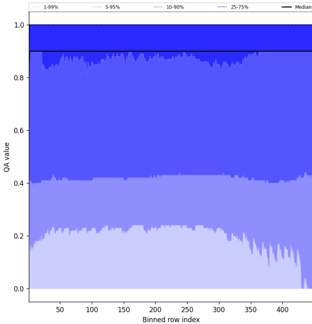
Figure 40: Along track statistics of “QA value” for 2025-09-15 to 2025-09-16
