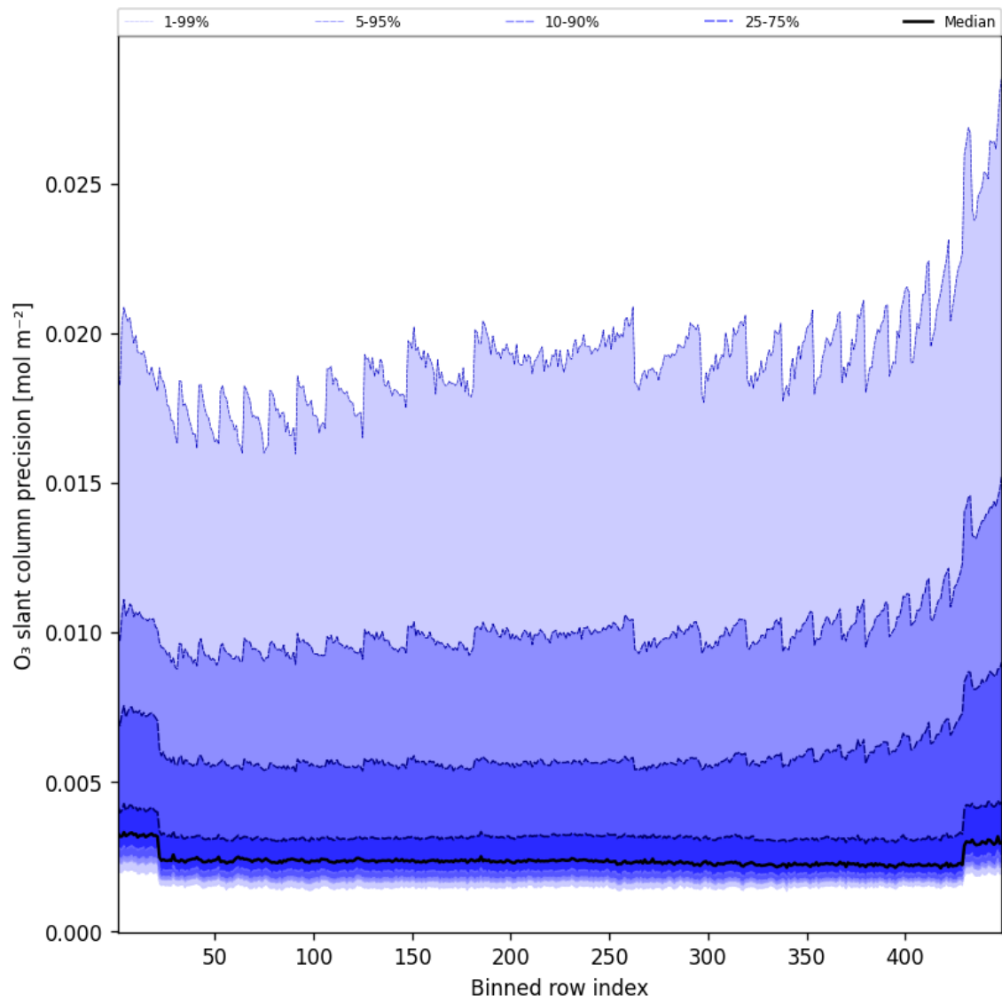
Figure 44: Along track statistics of “O 3 slant column precision” for 2025-09-15 to 2025-09-16
