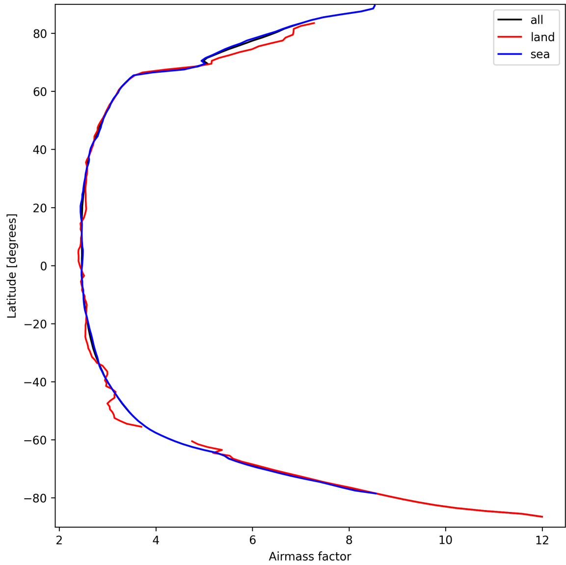
Figure 25: Zonal average of “Airmass factor” for 2025-09-15 to 2025-09-16.
