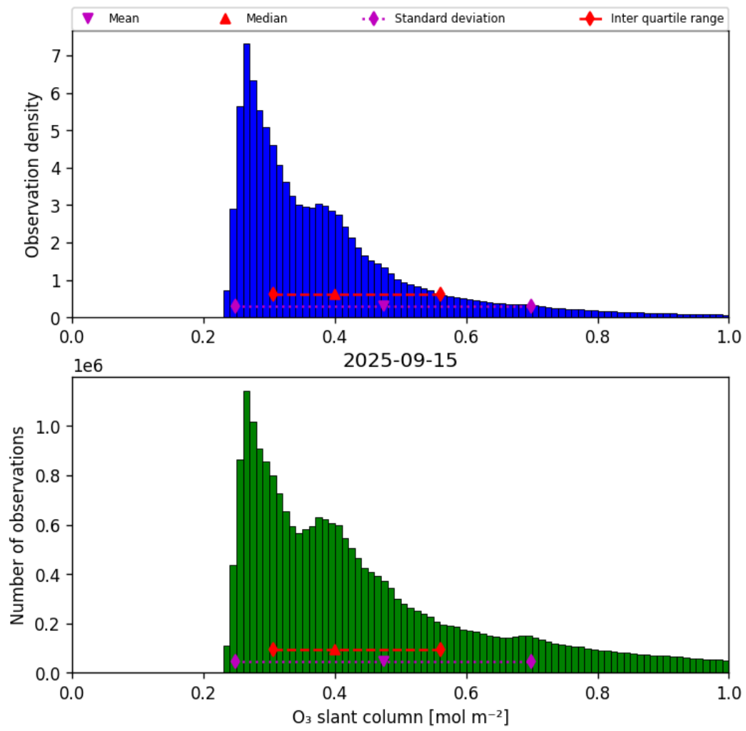
Figure 31: Histogram of “O 3 slant column” for 2025-09-15 to 2025-09-16
