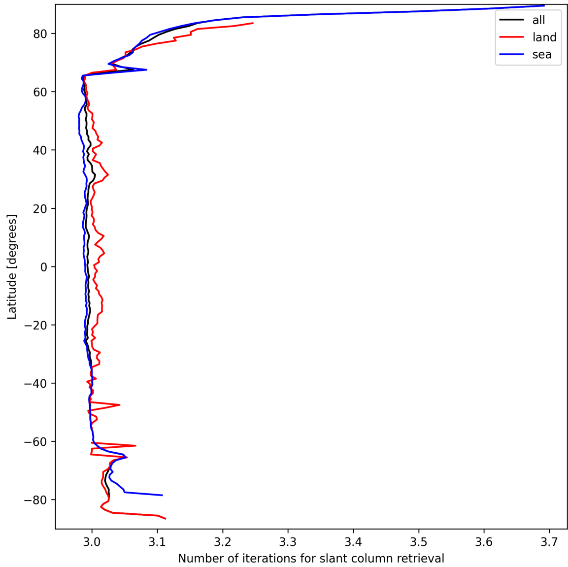
Figure 21: Zonal average of “Number of iterations for slant column retrieval” for 2025-09-15 to 2025-09-16.
