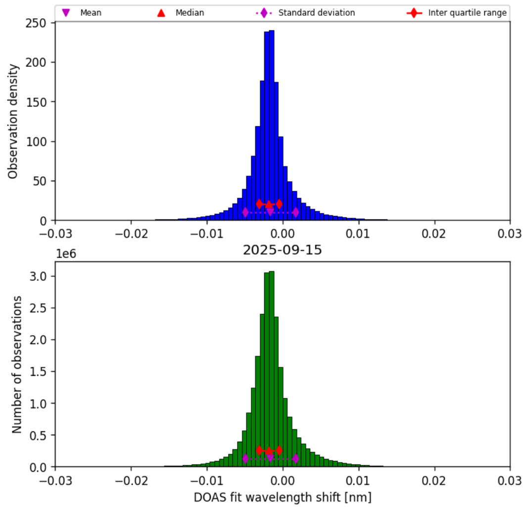
Figure 35: Histogram of “DOAS fit wavelength shift” for 2025-09-15 to 2025-09-16
