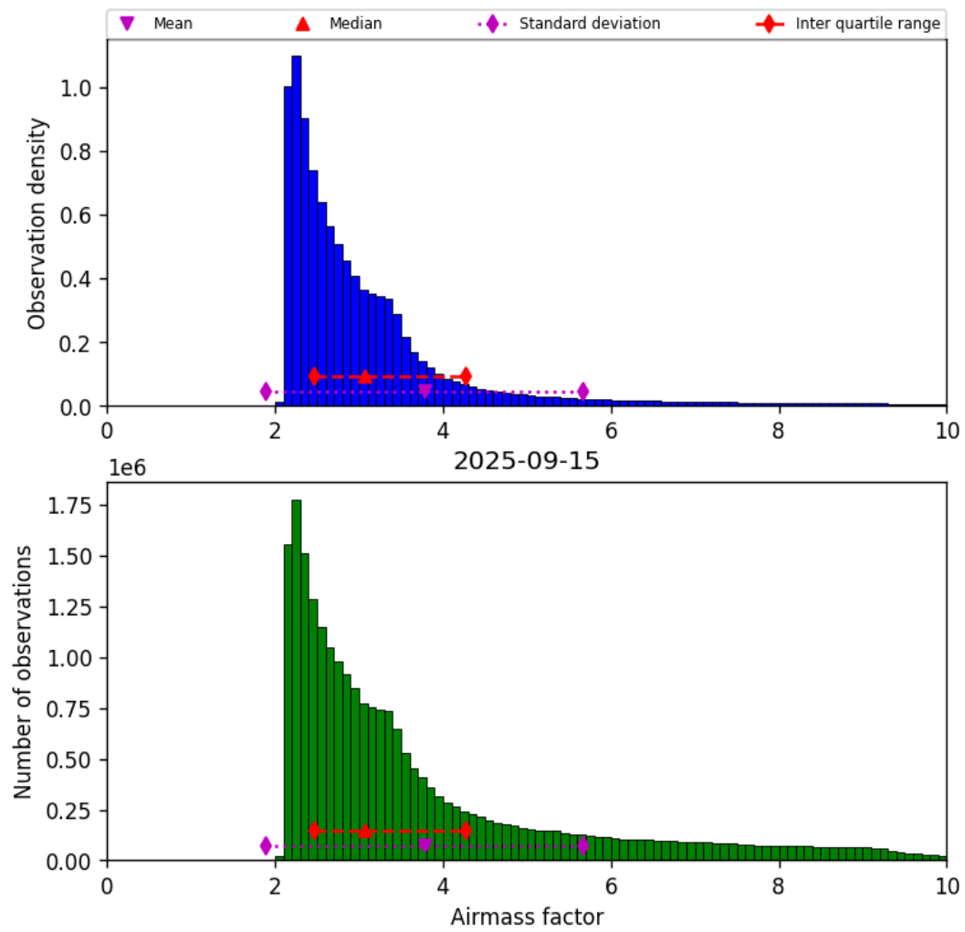
Figure 37: Histogram of “Airmass factor” for 2025-09-15 to 2025-09-16
