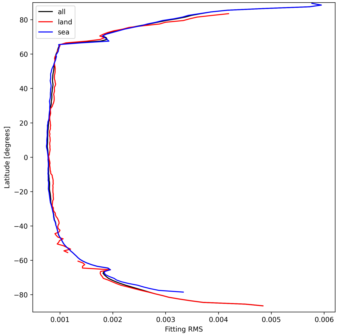
Figure 22: Zonal average of “Fitting RMS” for 2025-09-15 to 2025-09-16.
