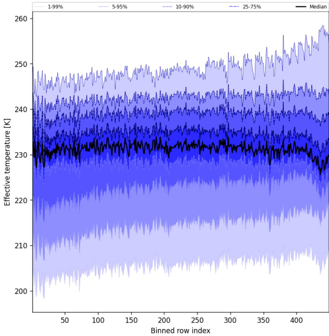
Figure 50: Along track statistics of “Effective temperature” for 2025-09-16 to 2025-09-17
