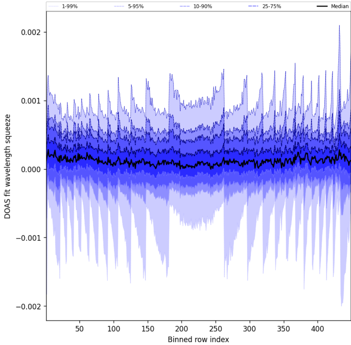
Figure 48: Along track statistics of “DOAS fit wavelength squeeze” for 2025-09-16 to 2025-09-17
