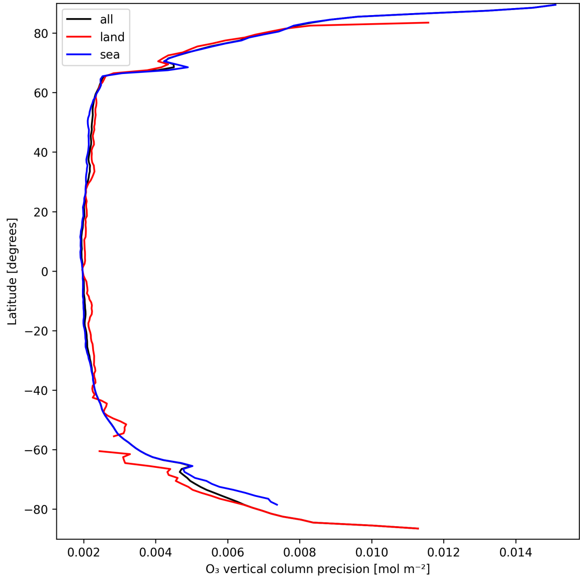
Figure 18: Zonal average of "O 3 vertical column precision" for 2025-09-16 to 2025-09-17.
