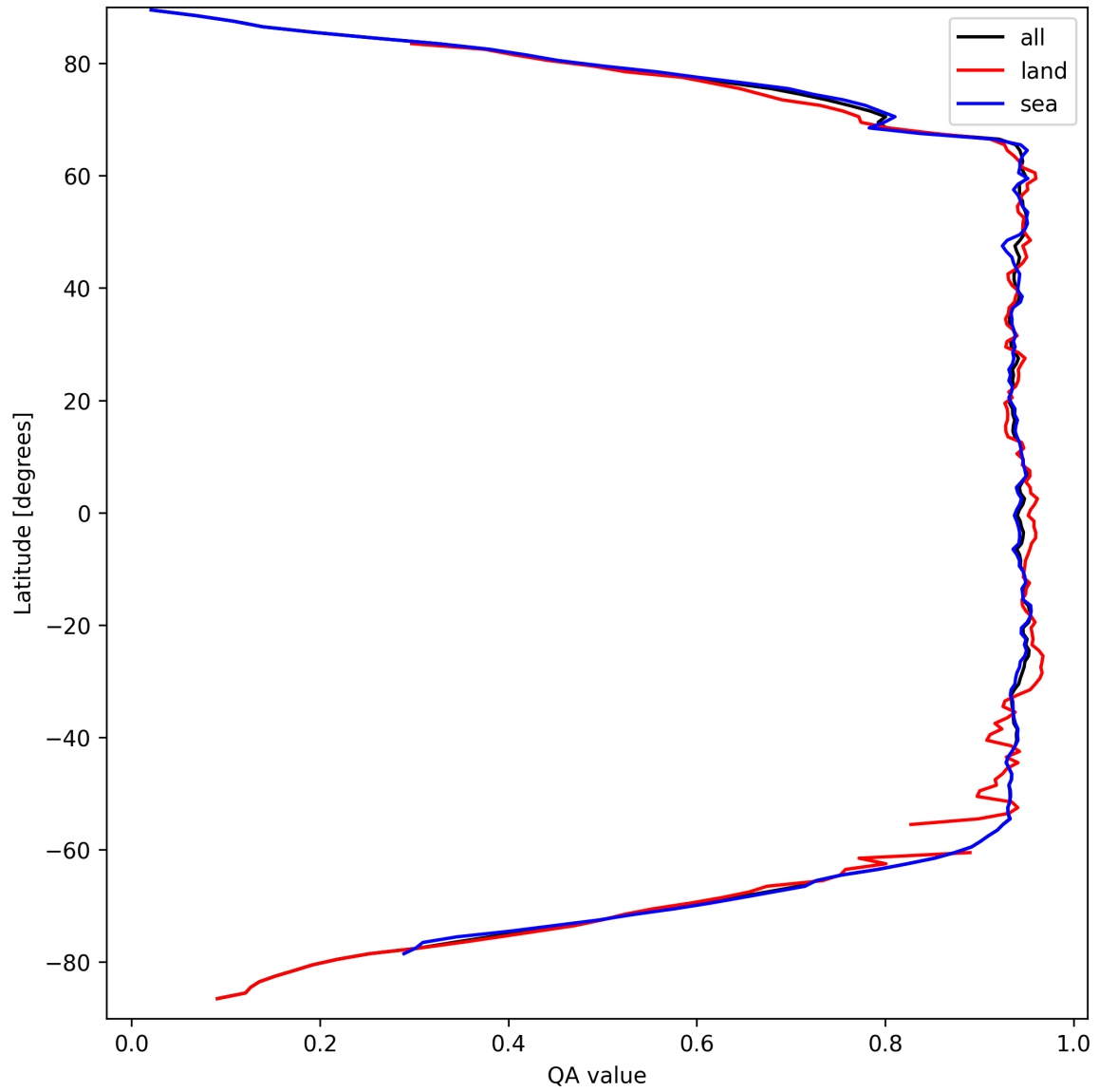
Figure 16: Zonal average of “QA value” for 2025-09-16 to 2025-09-17.
