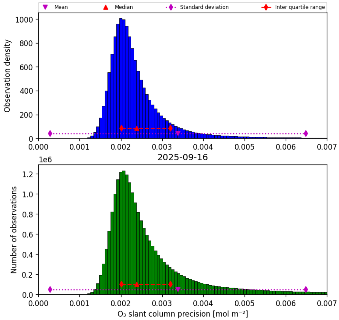
Figure 32: Histogram of “O 3 slant column precision” for 2025-09-16 to 2025-09-17
