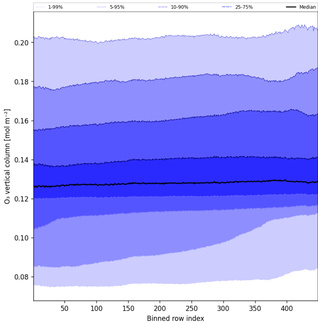
Figure 41: Along track statistics of “O 3 vertical column” for 2025-09-16 to 2025-09-17
