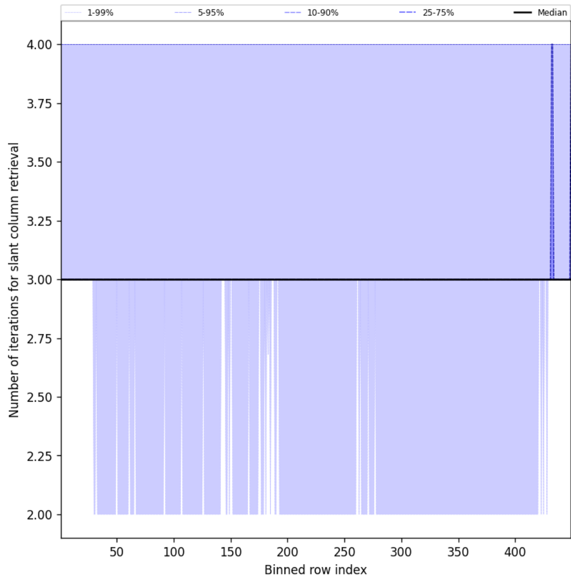
Figure 45: Along track statistics of “Number of iterations for slant column retrieval” for 2025-09-16 to 2025-09-17
