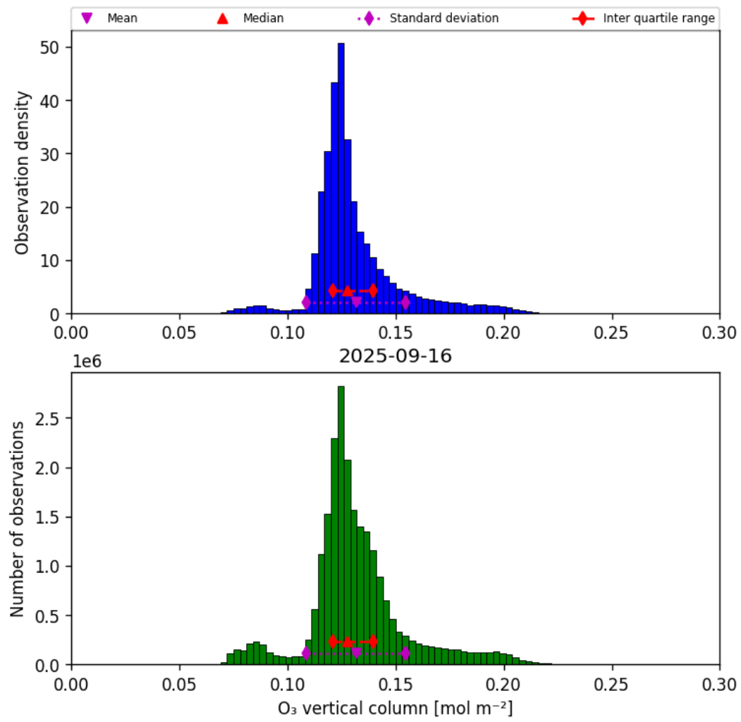
Figure 29: Histogram of “O 3 vertical column” for 2025-09-16 to 2025-09-17
