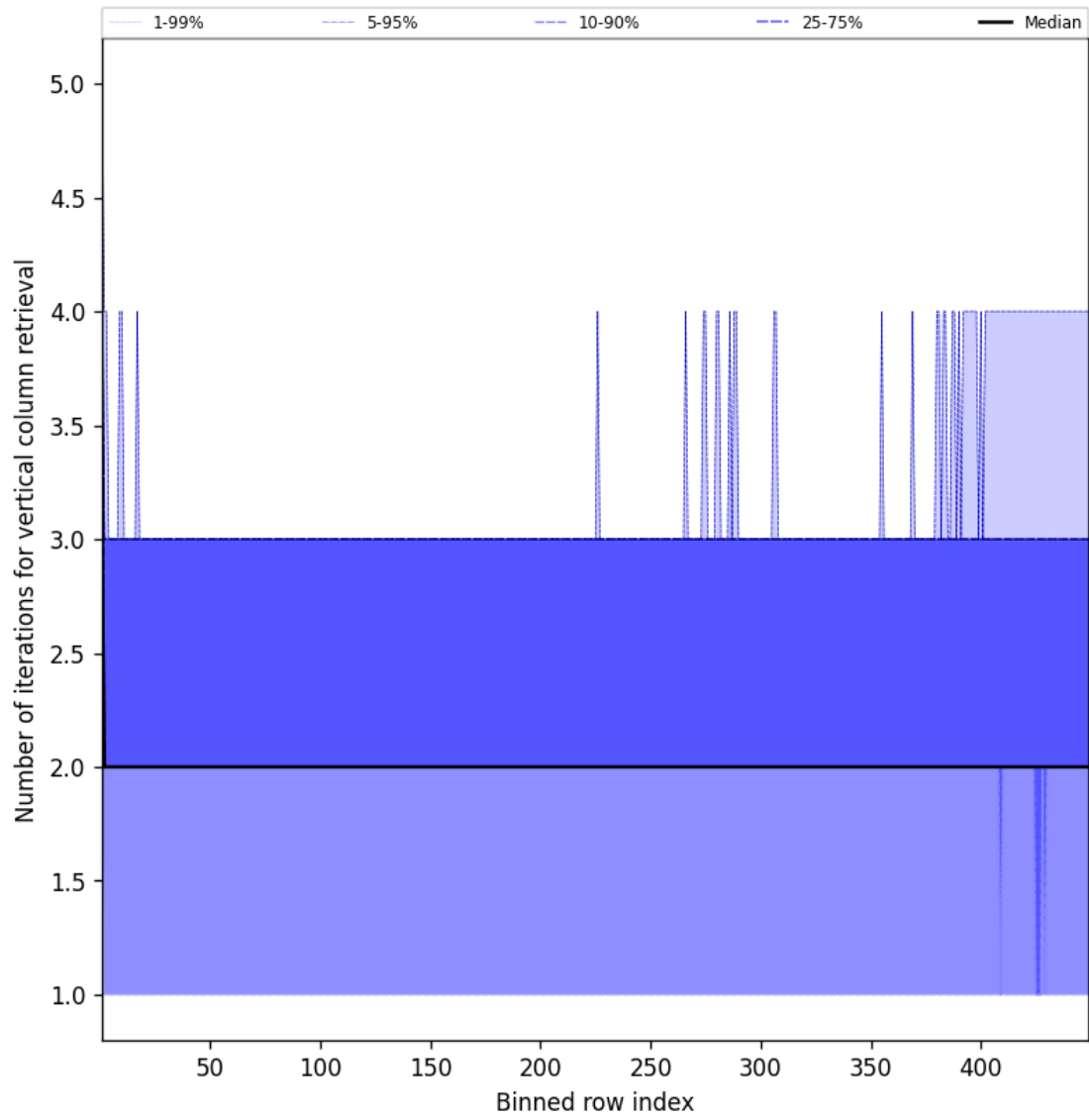
Figure 51: Along track statistics of “Number of iterations for vertical column retrieval” for 2025-09-16 to 2025-09-17
