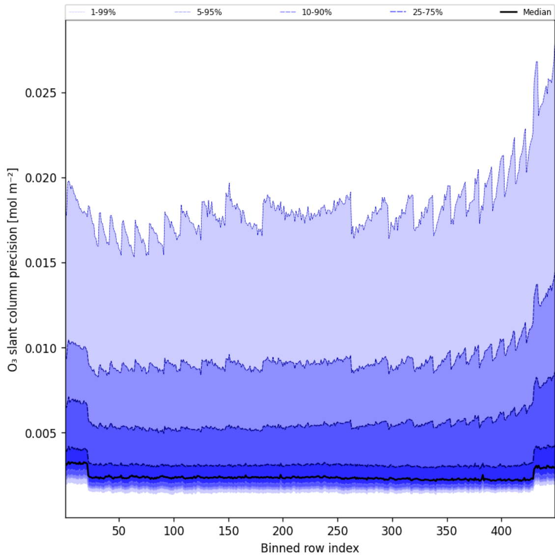
Figure 44: Along track statistics of “O 3 slant column precision” for 2025-09-16 to 2025-09-17
