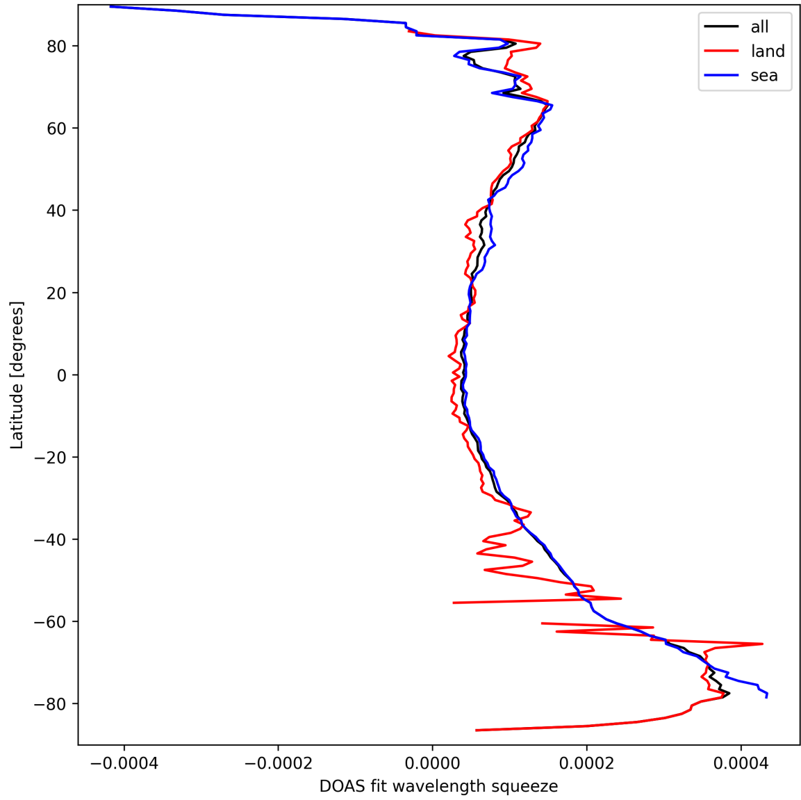
Figure 24: Zonal average of "DOAS fit wavelength squeeze" for 2025-09-16 to 2025-09-17.
