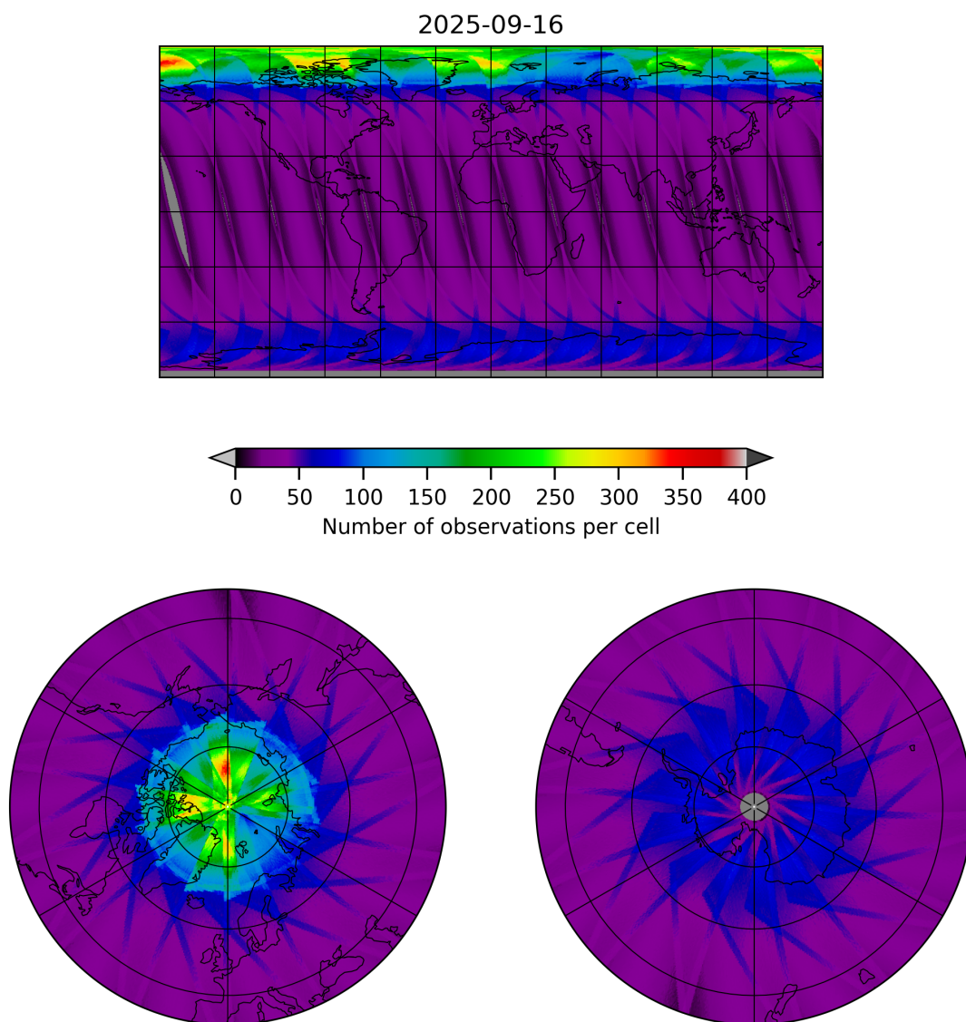
Figure 15: Map of the number of observations for 2025-09-16 to 2025-09-17
