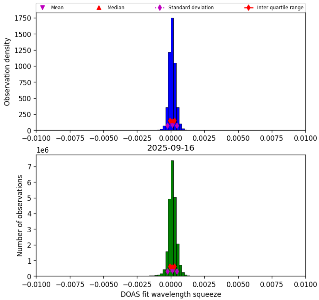
Figure 36: Histogram of “DOAS fit wavelength squeeze” for 2025-09-16 to 2025-09-17
