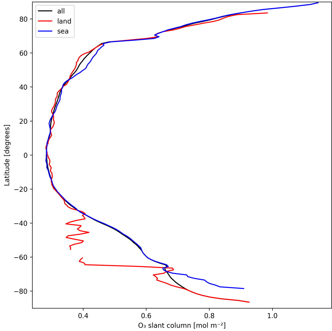
Figure 19: Zonal average of “O 3 slant column” for 2025-09-16 to 2025-09-17.
