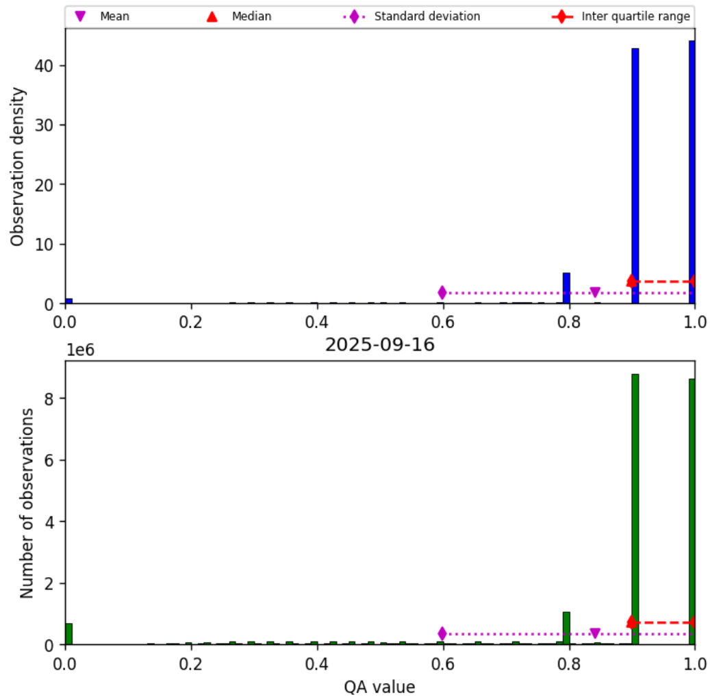
Figure 28: Histogram of “QA value” for 2025-09-16 to 2025-09-17
