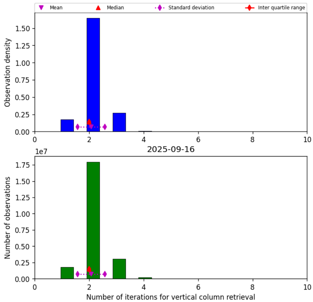
Figure 39: Histogram of “Number of iterations for vertical column retrieval” for 2025-09-16 to 2025-09-17
