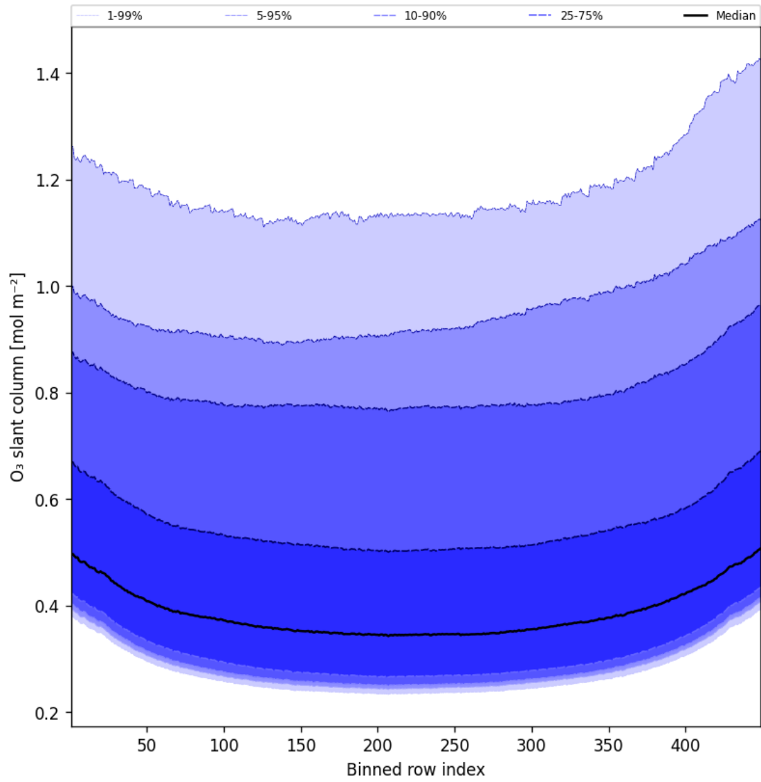
Figure 43: Along track statistics of “O 3 slant column” for 2025-09-16 to 2025-09-17
