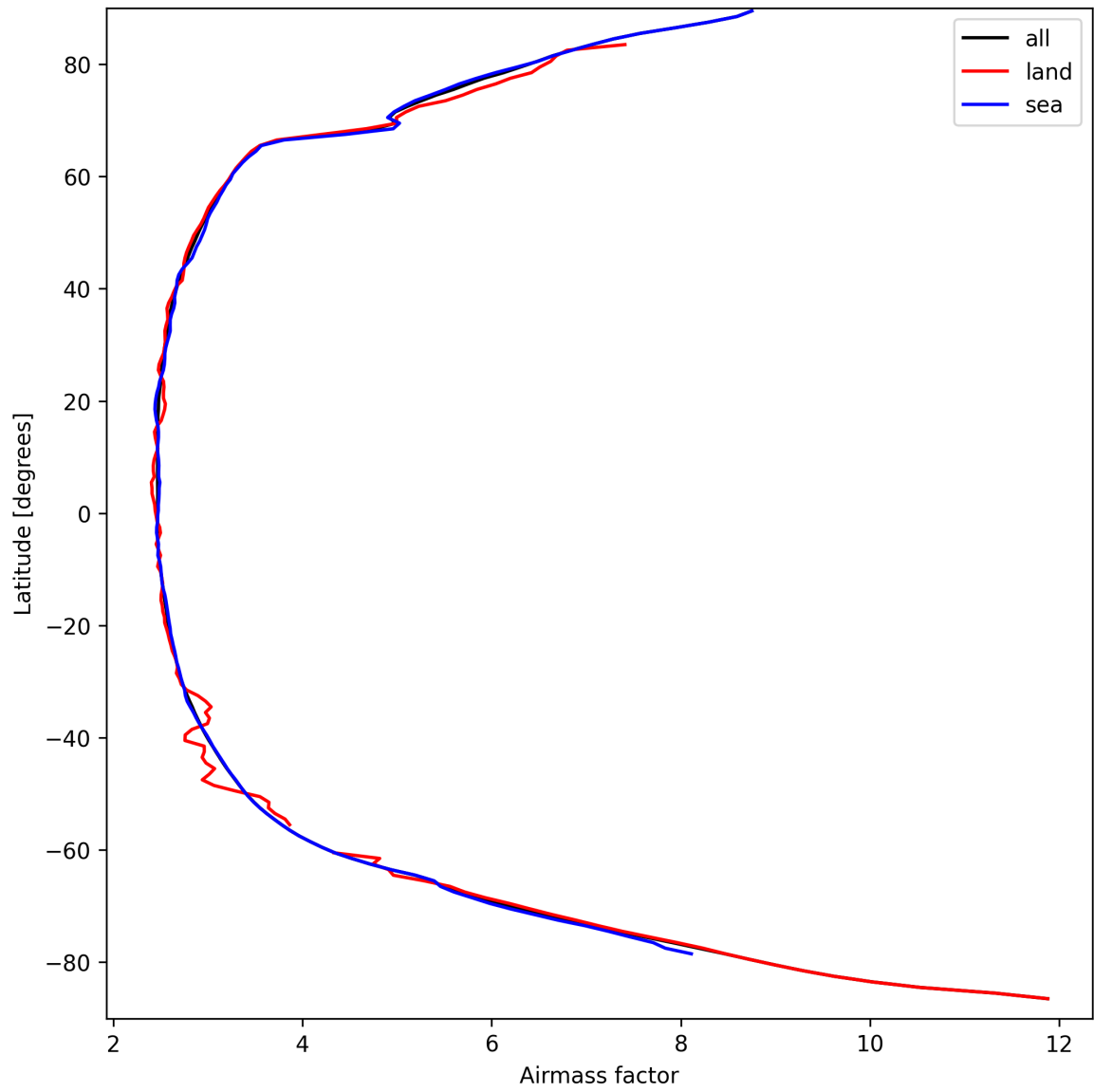
Figure 25: Zonal average of “Airmass factor” for 2025-09-16 to 2025-09-17.
