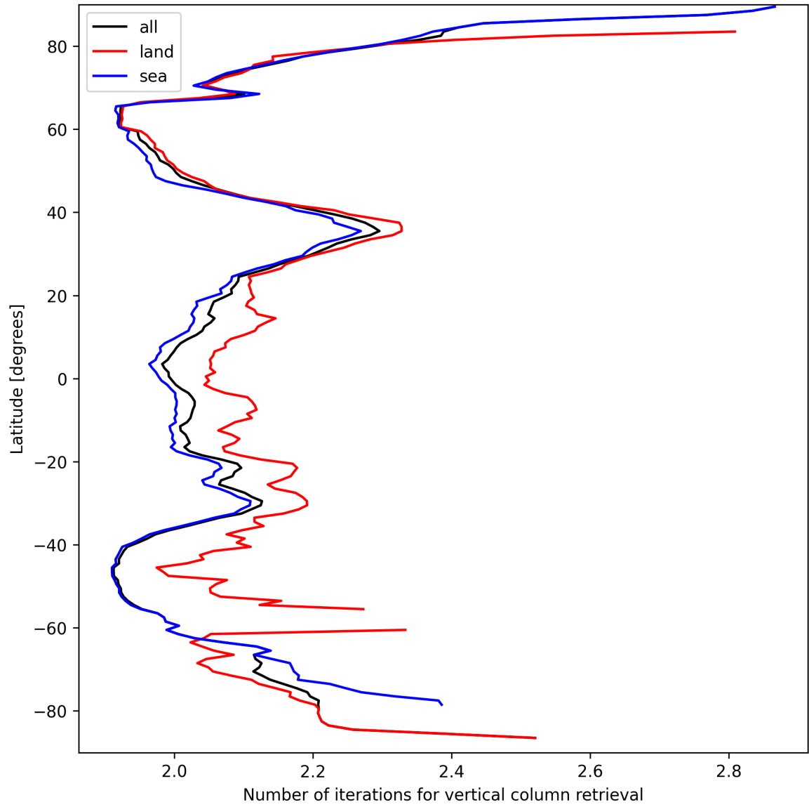
Figure 27: Zonal average of “Number of iterations for vertical column retrieval” for 2025-09-16 to 2025-09-17.
