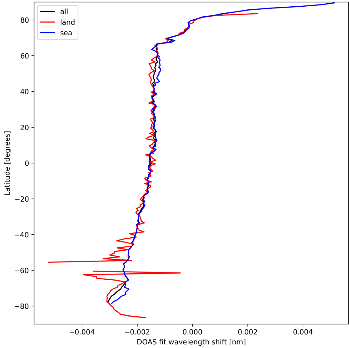
Figure 23: Zonal average of “DOAS fit wavelength shift” for 2025-09-16 to 2025-09-17.
