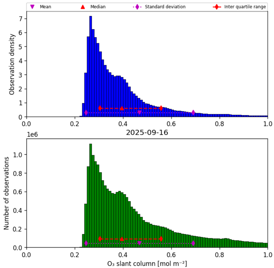
Figure 31: Histogram of “O 3 slant column” for 2025-09-16 to 2025-09-17
