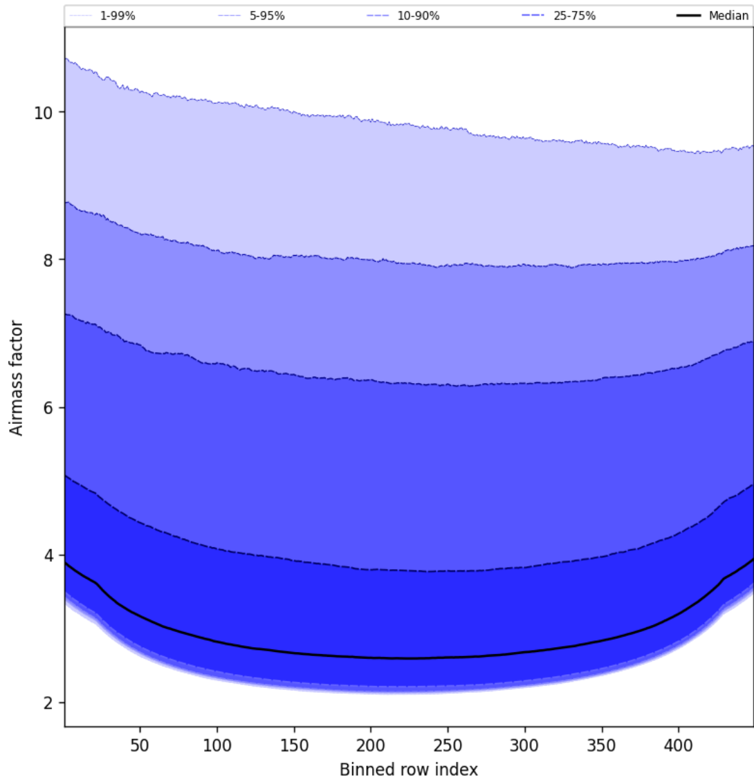
Figure 49: Along track statistics of “Airmass factor” for 2025-09-16 to 2025-09-17
