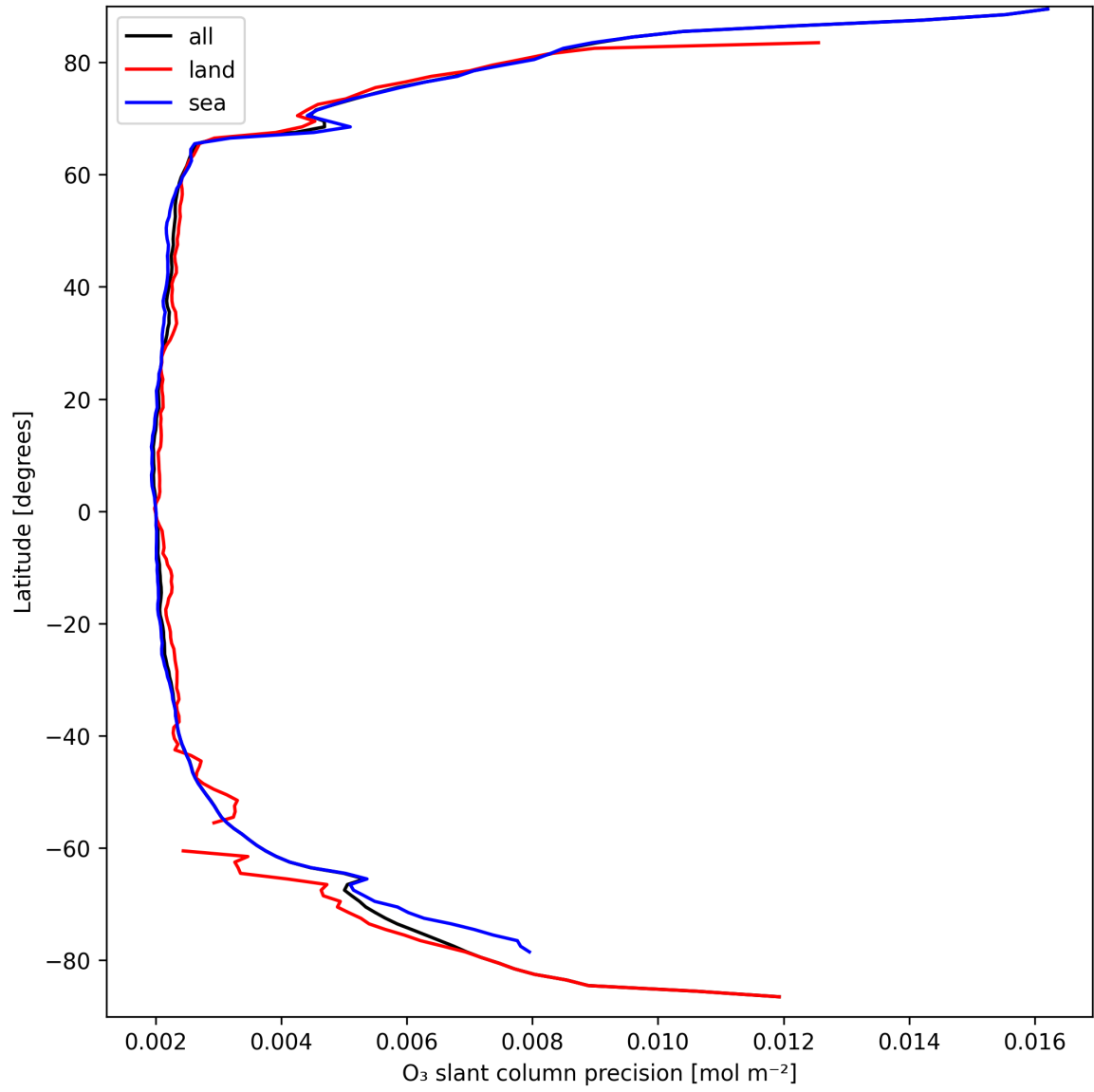
Figure 20: Zonal average of "O 3 slant column precision" for 2025-09-16 to 2025-09-17.
