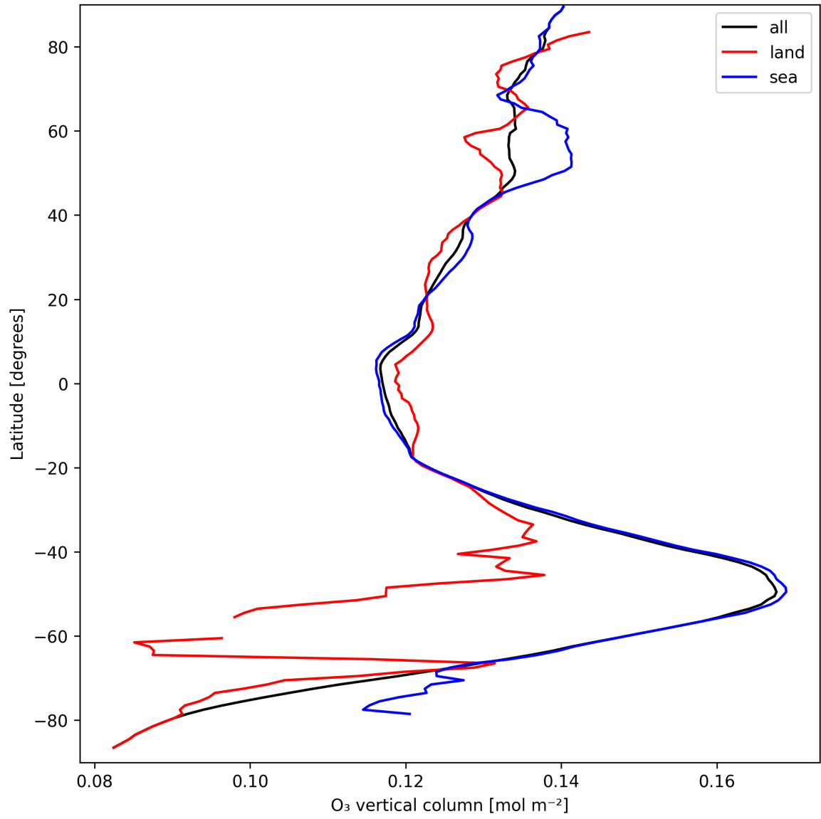
Figure 17: Zonal average of “O 3 vertical column” for 2025-09-16 to 2025-09-17.
