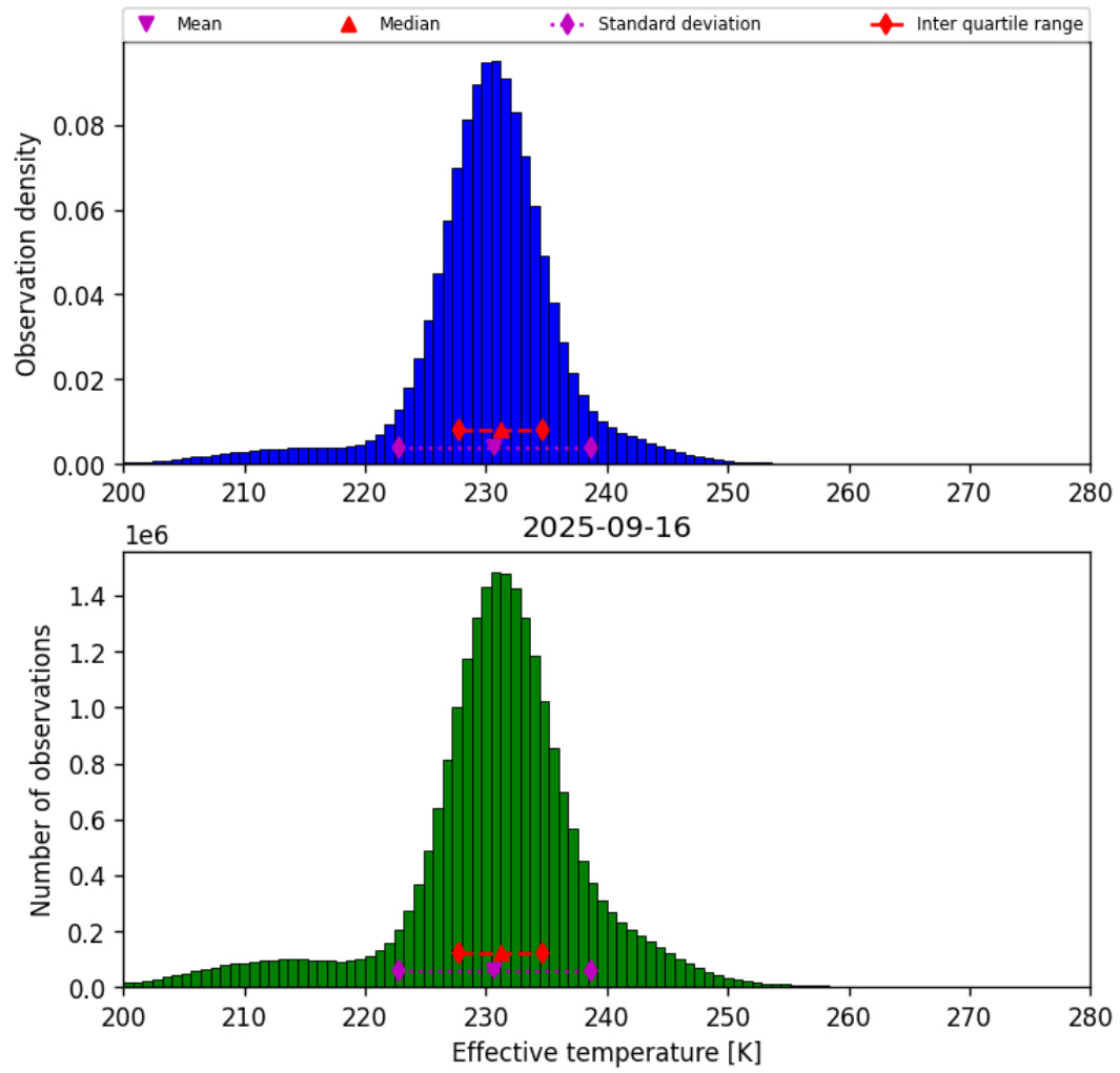
Figure 38: Histogram of “Effective temperature” for 2025-09-16 to 2025-09-17
