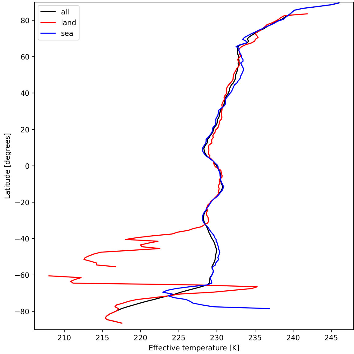
Figure 26: Zonal average of "Effective temperature" for 2025-09-16 to 2025-09-17.
