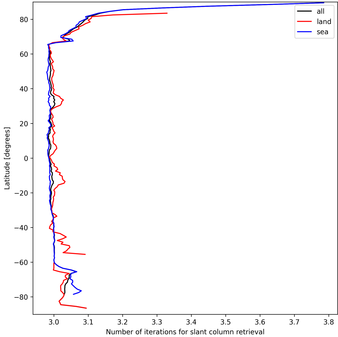
Figure 21: Zonal average of “Number of iterations for slant column retrieval” for 2025-09-16 to 2025-09-17.
