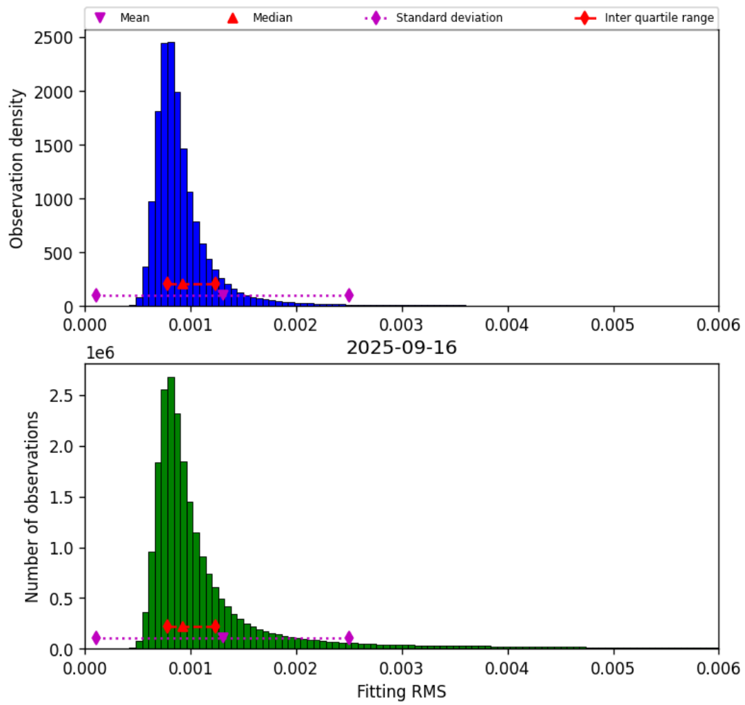
Figure 34: Histogram of “Fitting RMS” for 2025-09-16 to 2025-09-17
