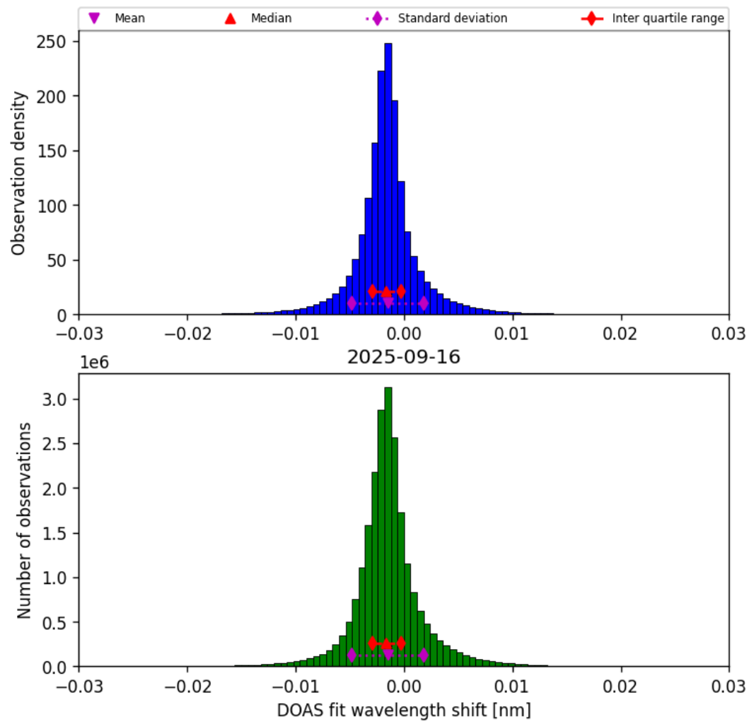
Figure 35: Histogram of “DOAS fit wavelength shift” for 2025-09-16 to 2025-09-17
