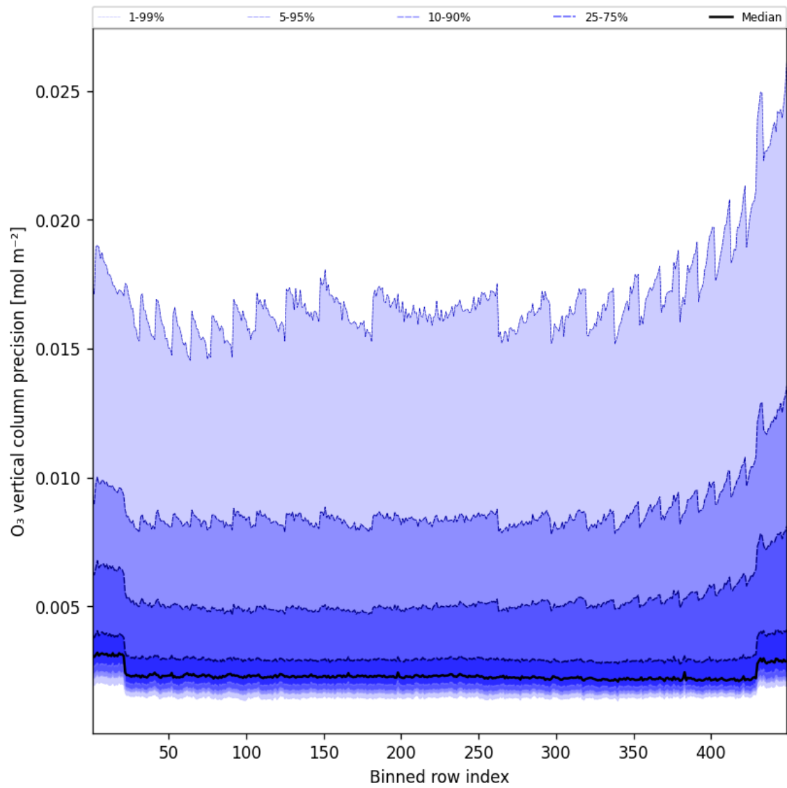
Figure 42: Along track statistics of “O 3 vertical column precision” for 2025-09-16 to 2025-09-17
