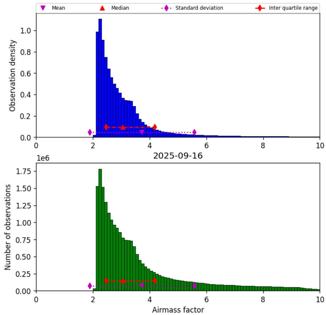
Figure 37: Histogram of “Airmass factor” for 2025-09-16 to 2025-09-17
