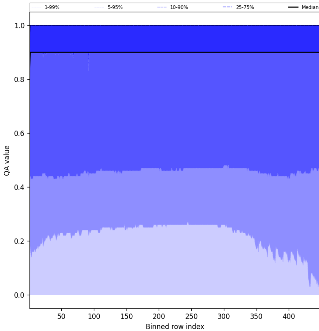
Figure 40: Along track statistics of “QA value” for 2025-09-16 to 2025-09-17
