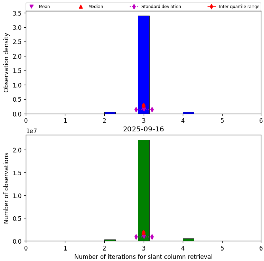
Figure 33: Histogram of “Number of iterations for slant column retrieval” for 2025-09-16 to 2025-09-17
