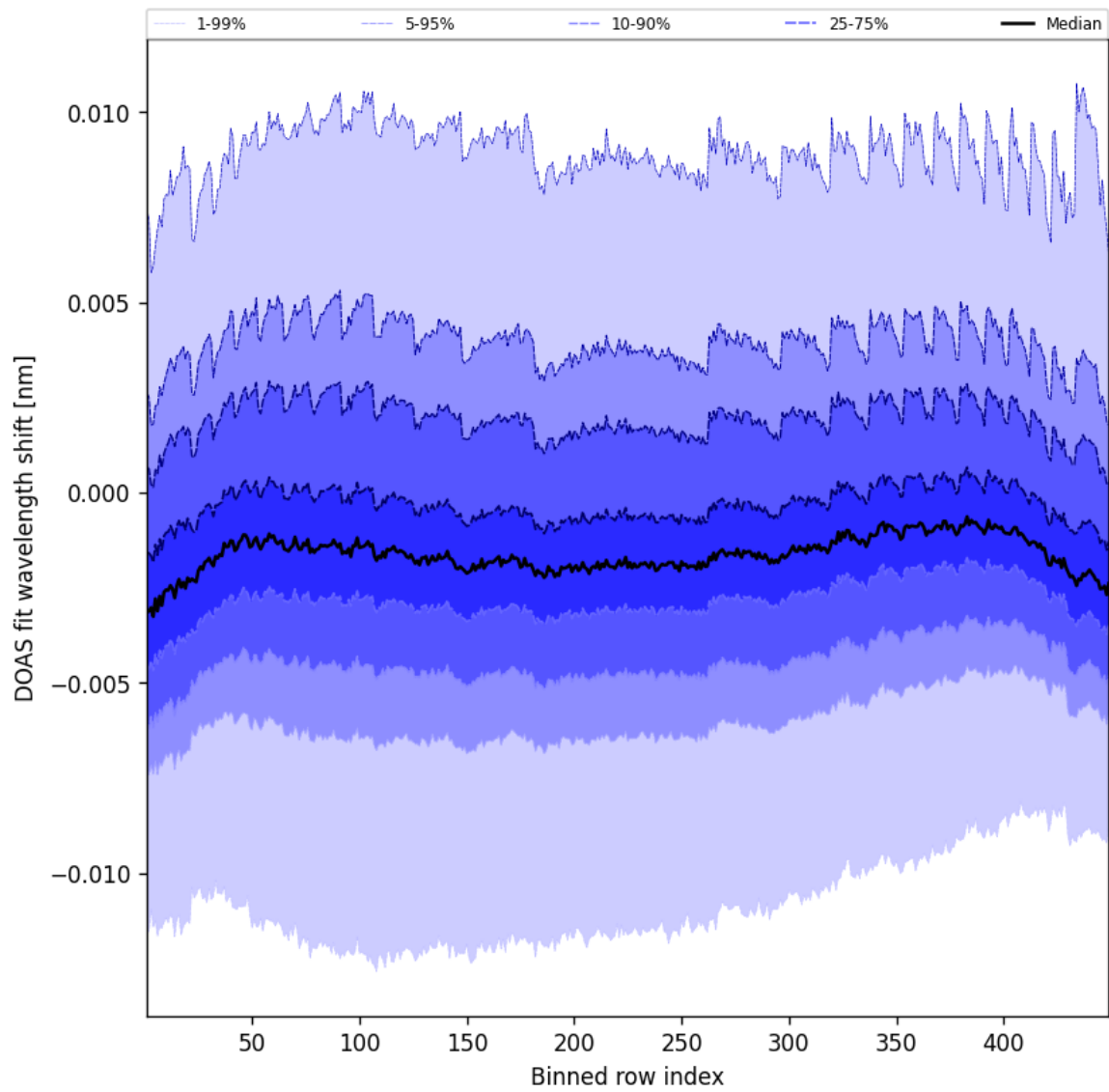
Figure 47: Along track statistics of “DOAS fit wavelength shift” for 2025-09-16 to 2025-09-17
