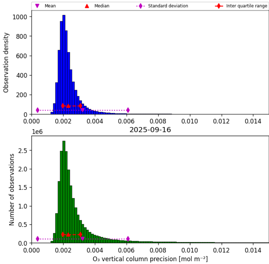
Figure 30: Histogram of “O 3 vertical column precision” for 2025-09-16 to 2025-09-17
