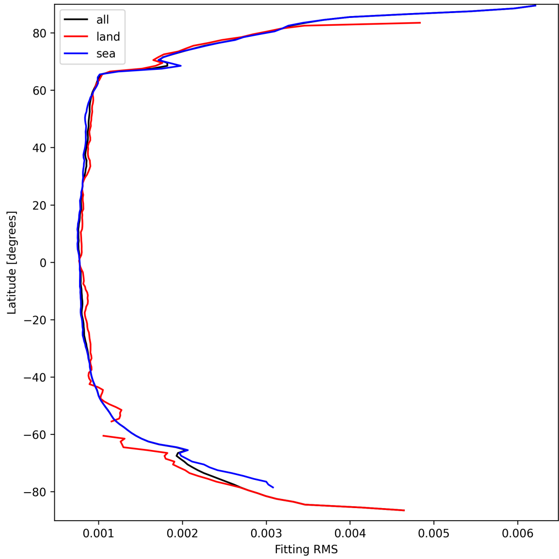
Figure 22: Zonal average of “Fitting RMS” for 2025-09-16 to 2025-09-17.
