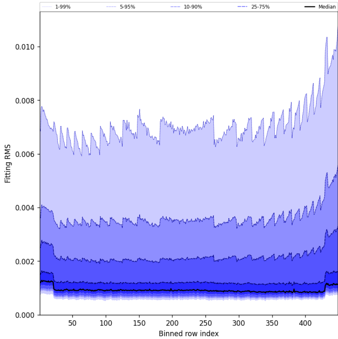
Figure 46: Along track statistics of “Fitting RMS” for 2025-09-16 to 2025-09-17
