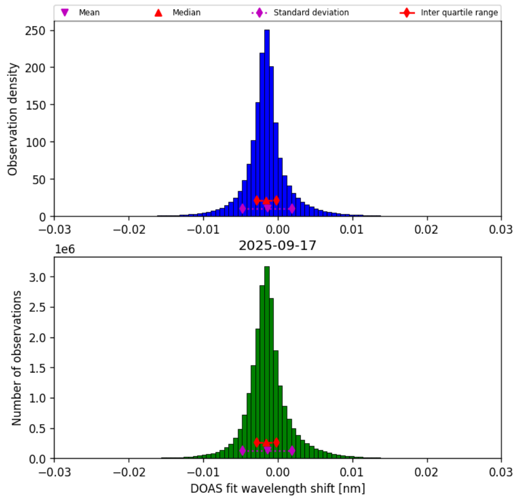
Figure 35: Histogram of “DOAS fit wavelength shift” for 2025-09-17 to 2025-09-18
