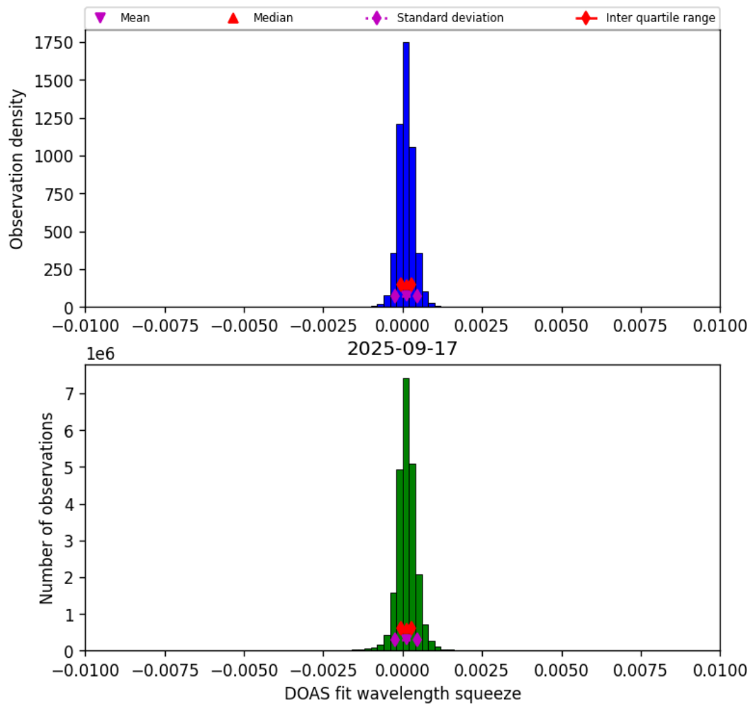
Figure 36: Histogram of “DOAS fit wavelength squeeze” for 2025-09-17 to 2025-09-18
