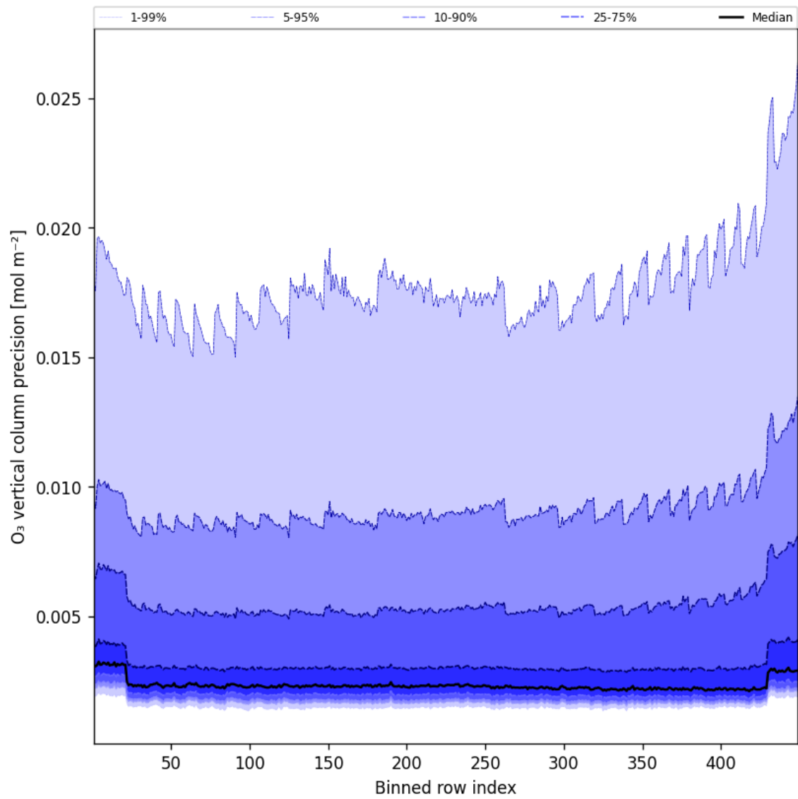
Figure 42: Along track statistics of “O 3 vertical column precision” for 2025-09-17 to 2025-09-18
