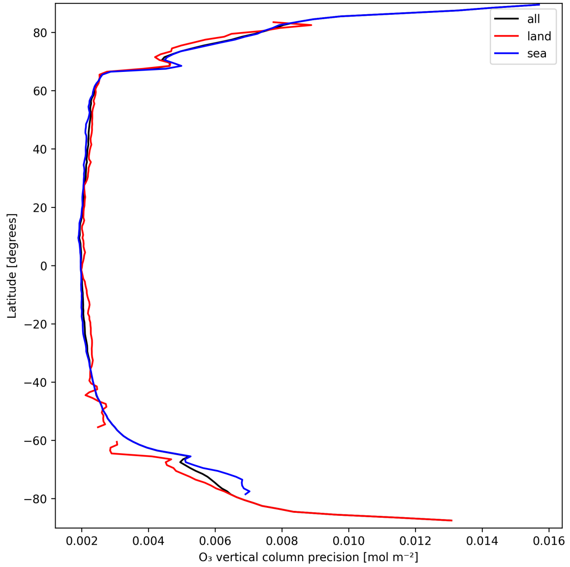
Figure 18: Zonal average of “O 3 vertical column precision” for 2025-09-17 to 2025-09-18.
