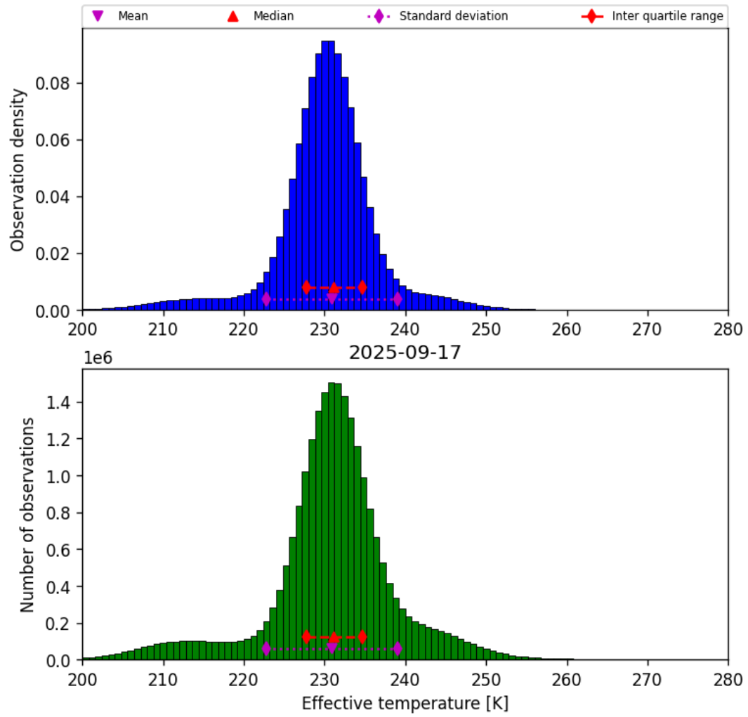
Figure 38: Histogram of “Effective temperature” for 2025-09-17 to 2025-09-18
