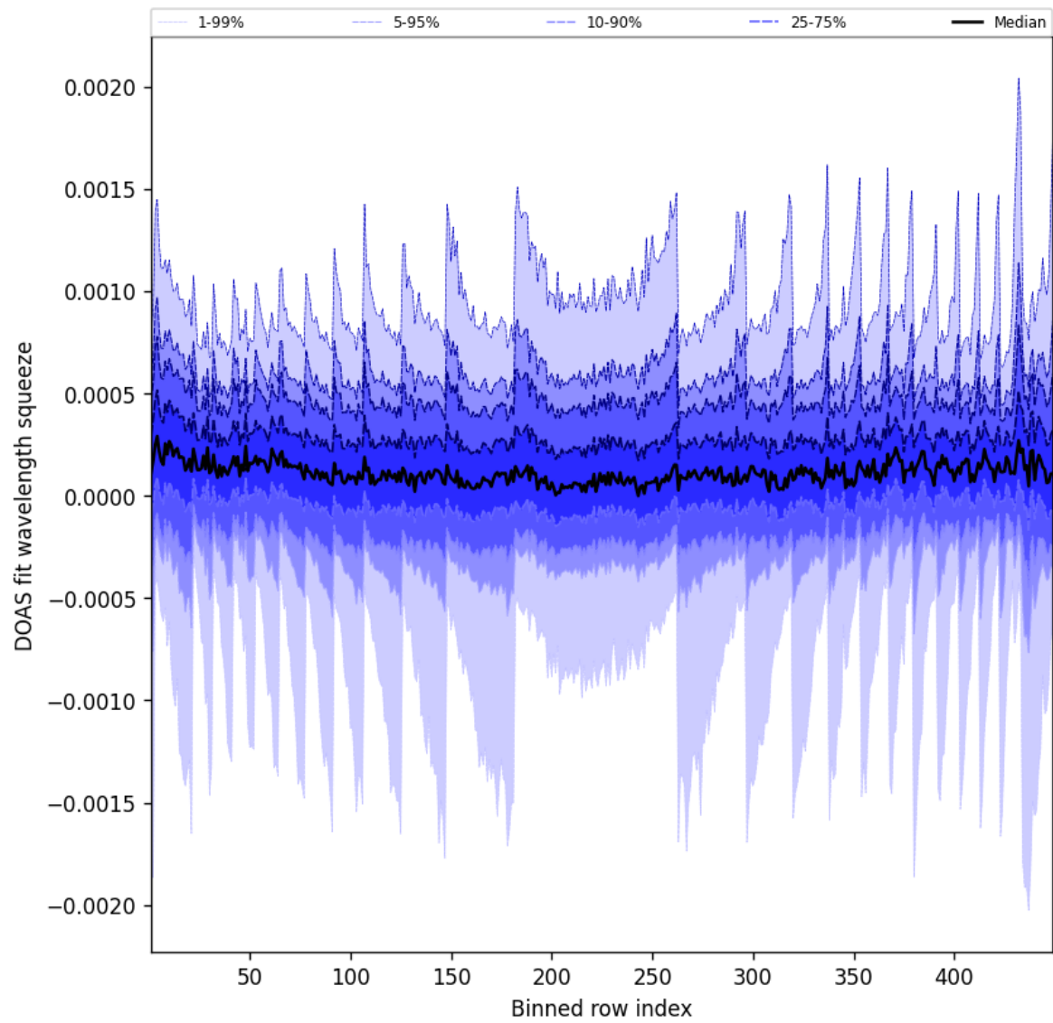
Figure 48: Along track statistics of “DOAS fit wavelength squeeze” for 2025-09-17 to 2025-09-18
