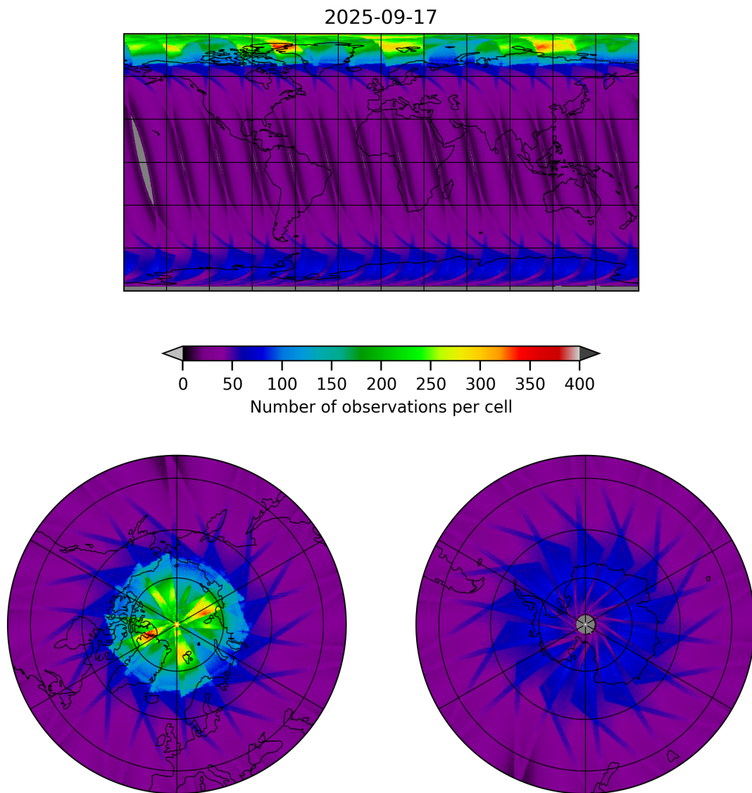
Figure 15: Map of the number of observations for 2025-09-17 to 2025-09-18
