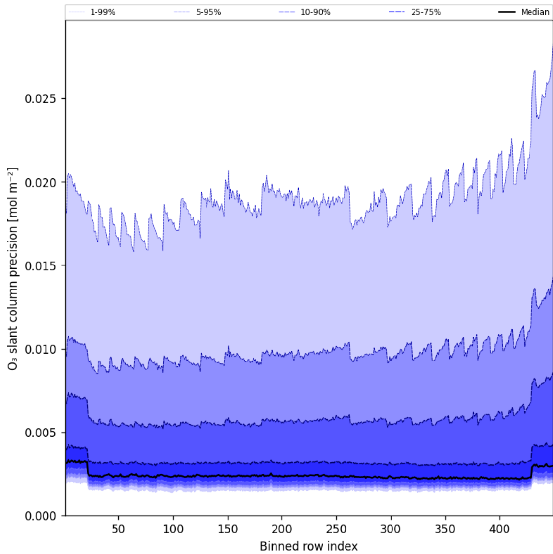
Figure 44: Along track statistics of “O 3 slant column precision” for 2025-09-17 to 2025-09-18
