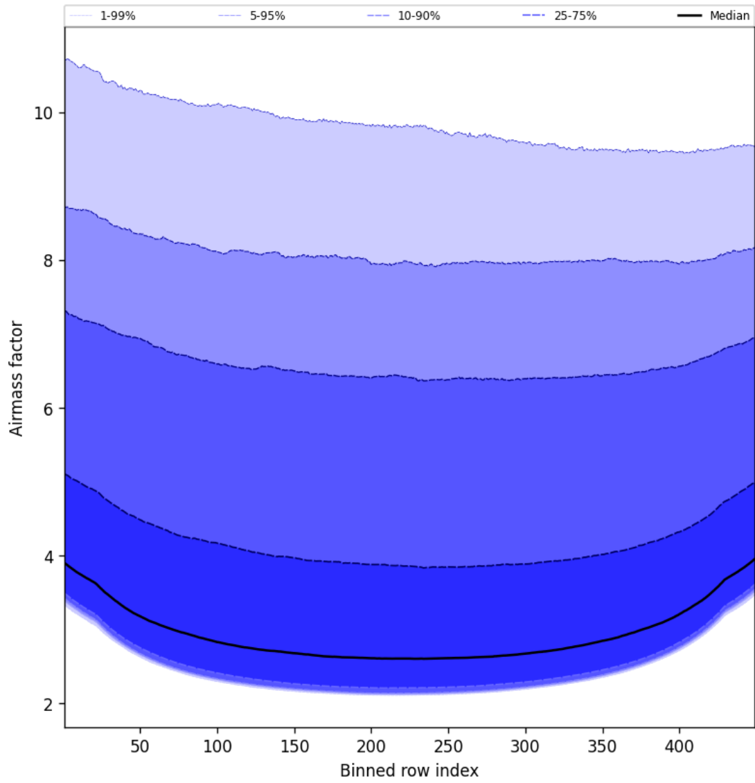
Figure 49: Along track statistics of “Airmass factor” for 2025-09-17 to 2025-09-18
