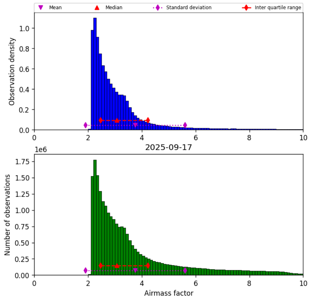
Figure 37: Histogram of “Airmass factor” for 2025-09-17 to 2025-09-18
