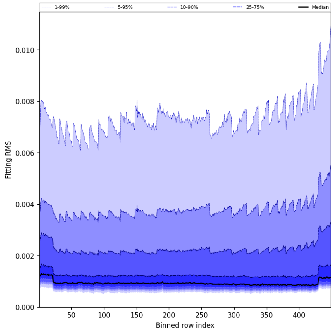
Figure 46: Along track statistics of “Fitting RMS” for 2025-09-17 to 2025-09-18
