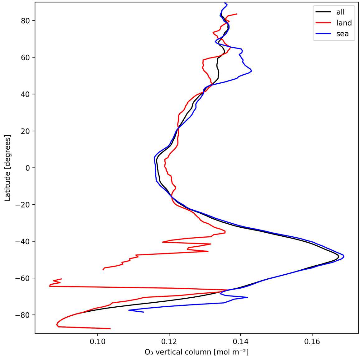
Figure 17: Zonal average of “O 3 vertical column” for 2025-09-17 to 2025-09-18.
