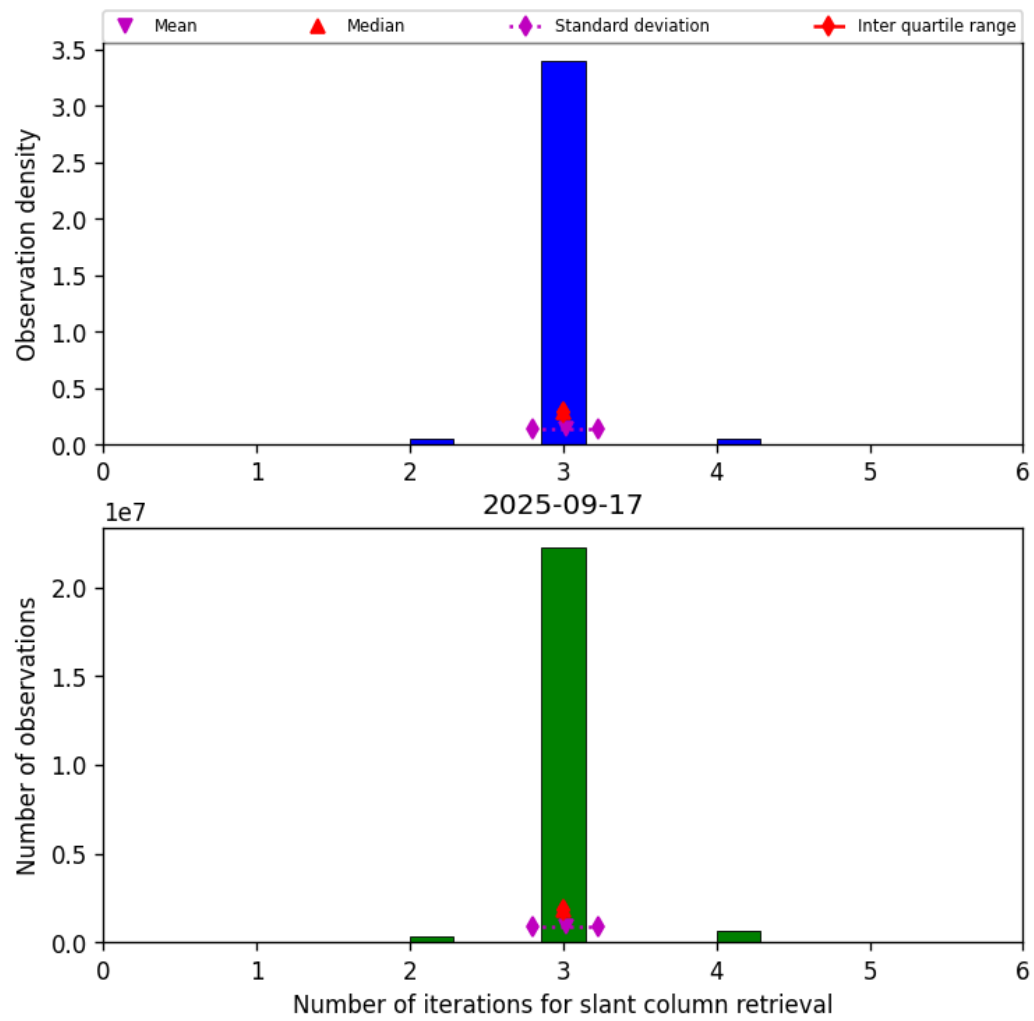
Figure 33: Histogram of “Number of iterations for slant column retrieval” for 2025-09-17 to 2025-09-18
