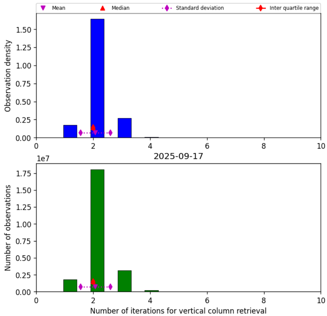
Figure 39: Histogram of “Number of iterations for vertical column retrieval” for 2025-09-17 to 2025-09-18
