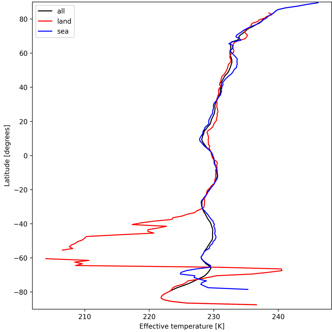
Figure 26: Zonal average of "Effective temperature" for 2025-09-17 to 2025-09-18.
