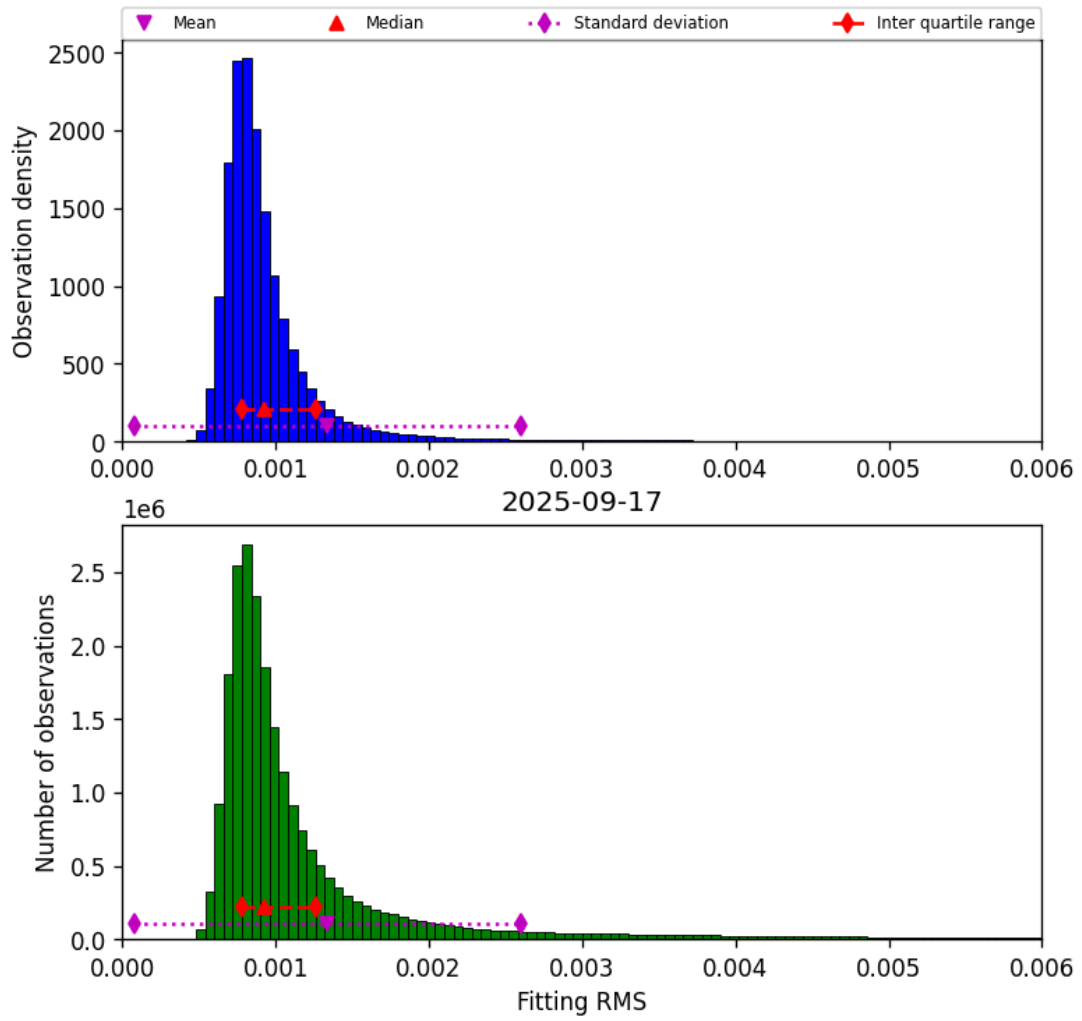
Figure 34: Histogram of “Fitting RMS” for 2025-09-17 to 2025-09-18
