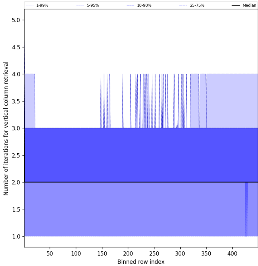
Figure 51: Along track statistics of “Number of iterations for vertical column retrieval” for 2025-09-17 to 2025-09-18
