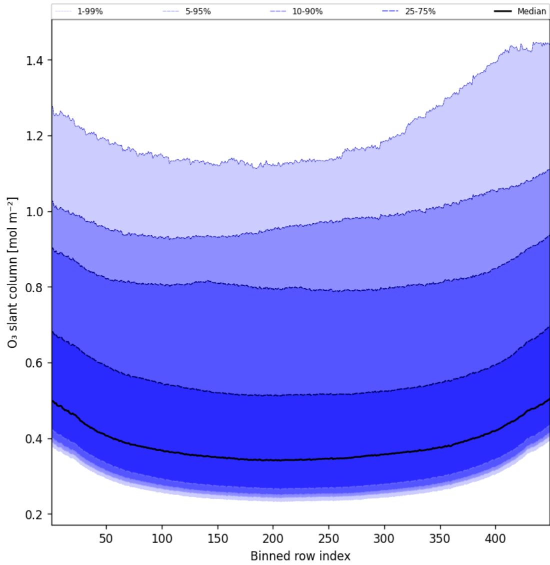
Figure 43: Along track statistics of “O 3 slant column” for 2025-09-17 to 2025-09-18
