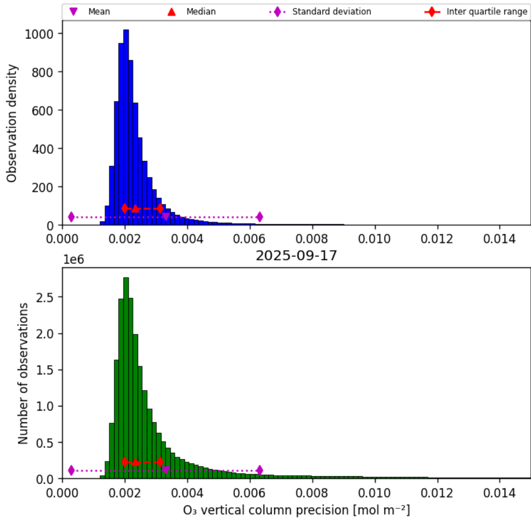
Figure 30: Histogram of “O 3 vertical column precision” for 2025-09-17 to 2025-09-18
