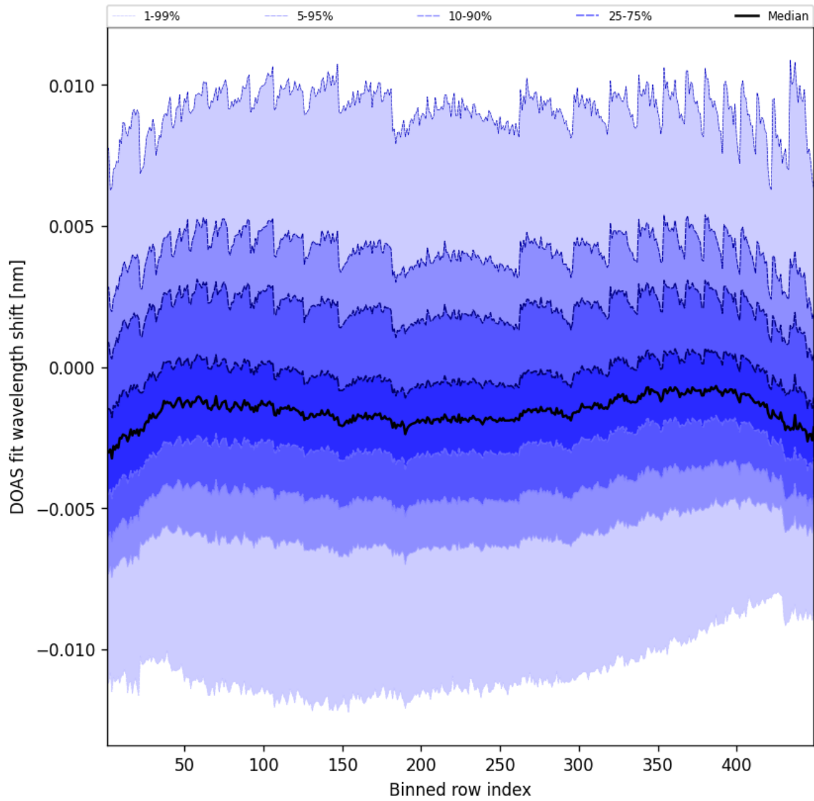
Figure 47: Along track statistics of “DOAS fit wavelength shift” for 2025-09-17 to 2025-09-18
