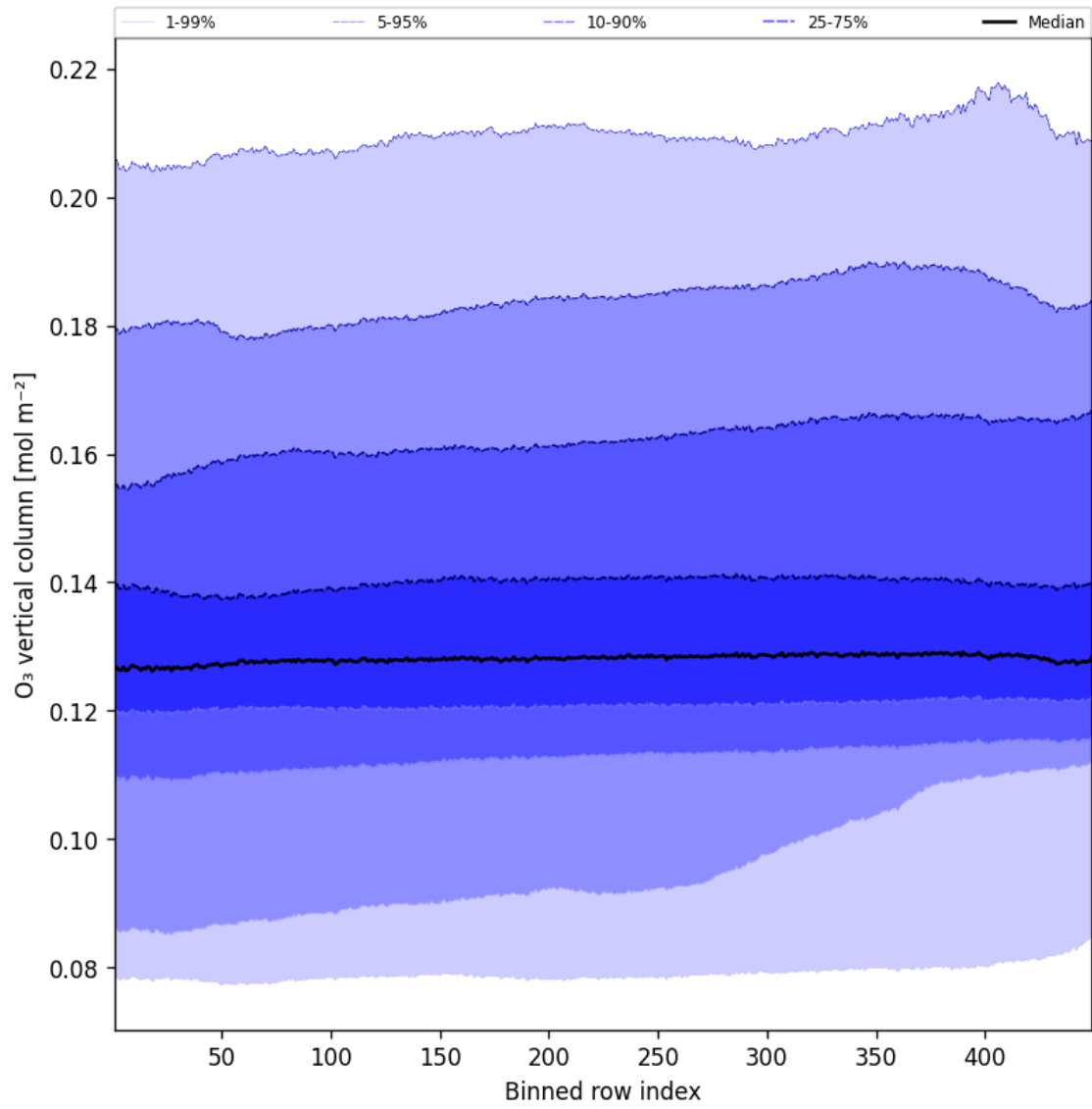
Figure 41: Along track statistics of “O 3 vertical column” for 2025-09-17 to 2025-09-18
