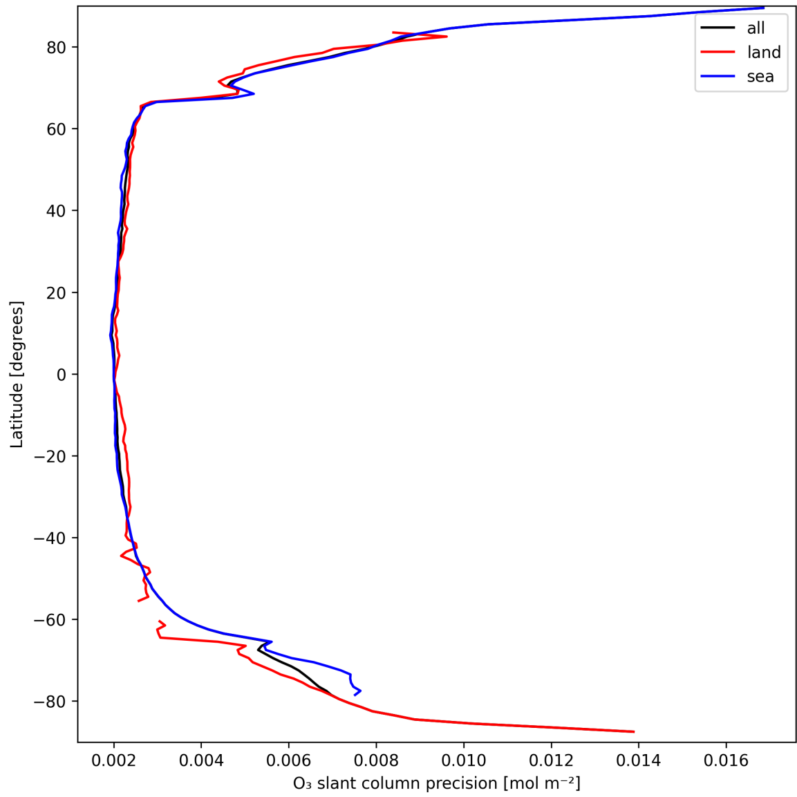
Figure 20: Zonal average of “O 3 slant column precision” for 2025-09-17 to 2025-09-18.
