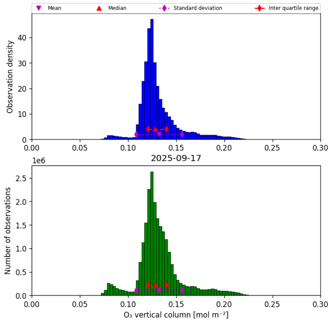
Figure 29: Histogram of “O 3 vertical column” for 2025-09-17 to 2025-09-18
