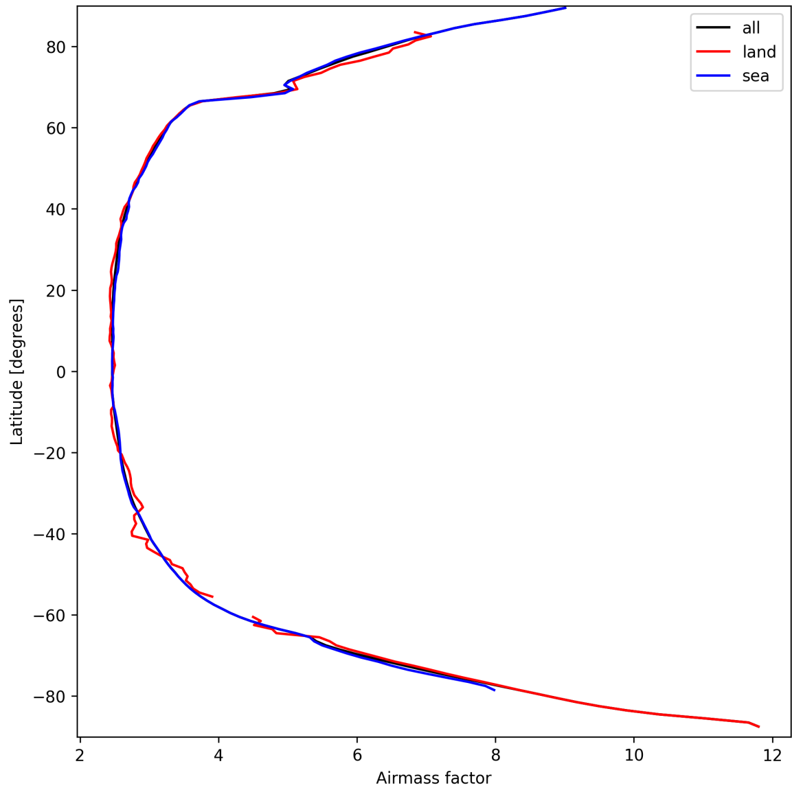
Figure 25: Zonal average of “Airmass factor” for 2025-09-17 to 2025-09-18.
