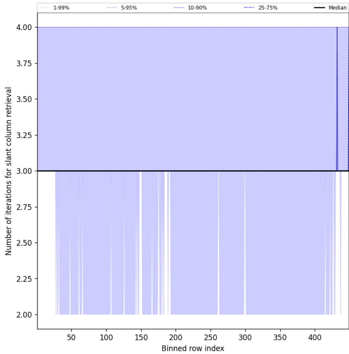
Figure 45: Along track statistics of “Number of iterations for slant column retrieval” for 2025-09-17 to 2025-09-18
