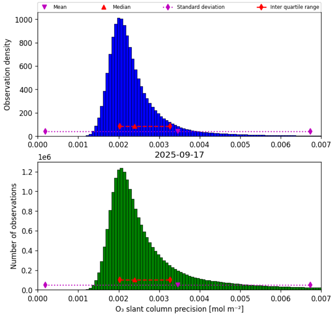
Figure 32: Histogram of “O 3 slant column precision” for 2025-09-17 to 2025-09-18
