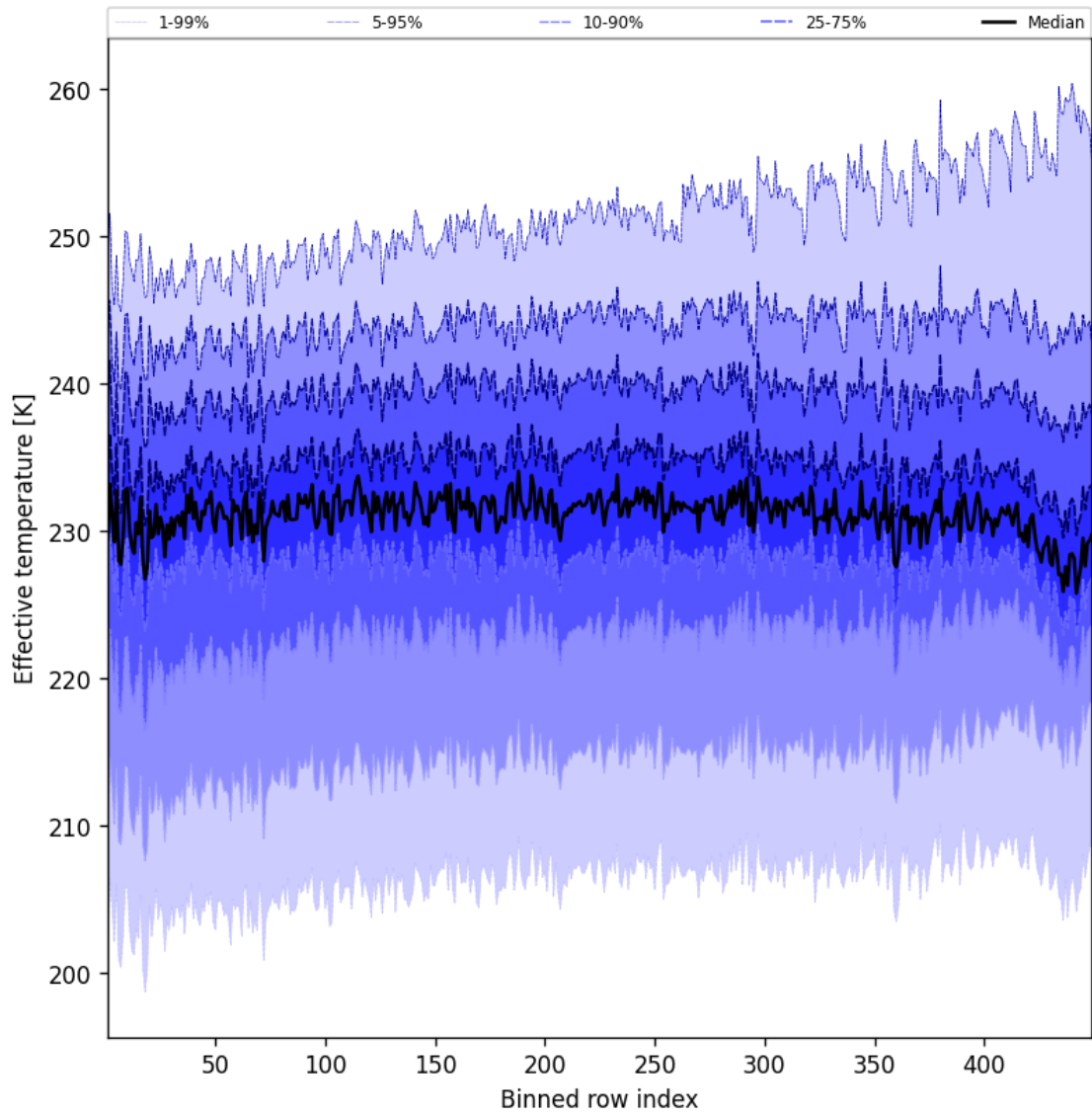
Figure 50: Along track statistics of “Effective temperature” for 2025-09-17 to 2025-09-18
