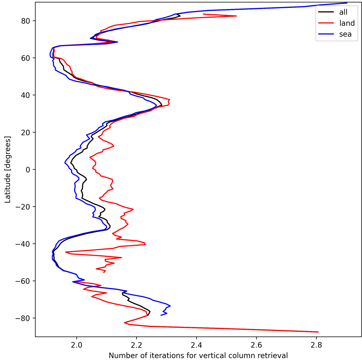
Figure 27: Zonal average of “Number of iterations for vertical column retrieval” for 2025-09-17 to 2025-09-18.
