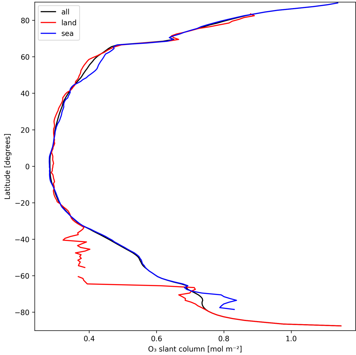
Figure 19: Zonal average of “O 3 slant column” for 2025-09-17 to 2025-09-18.
