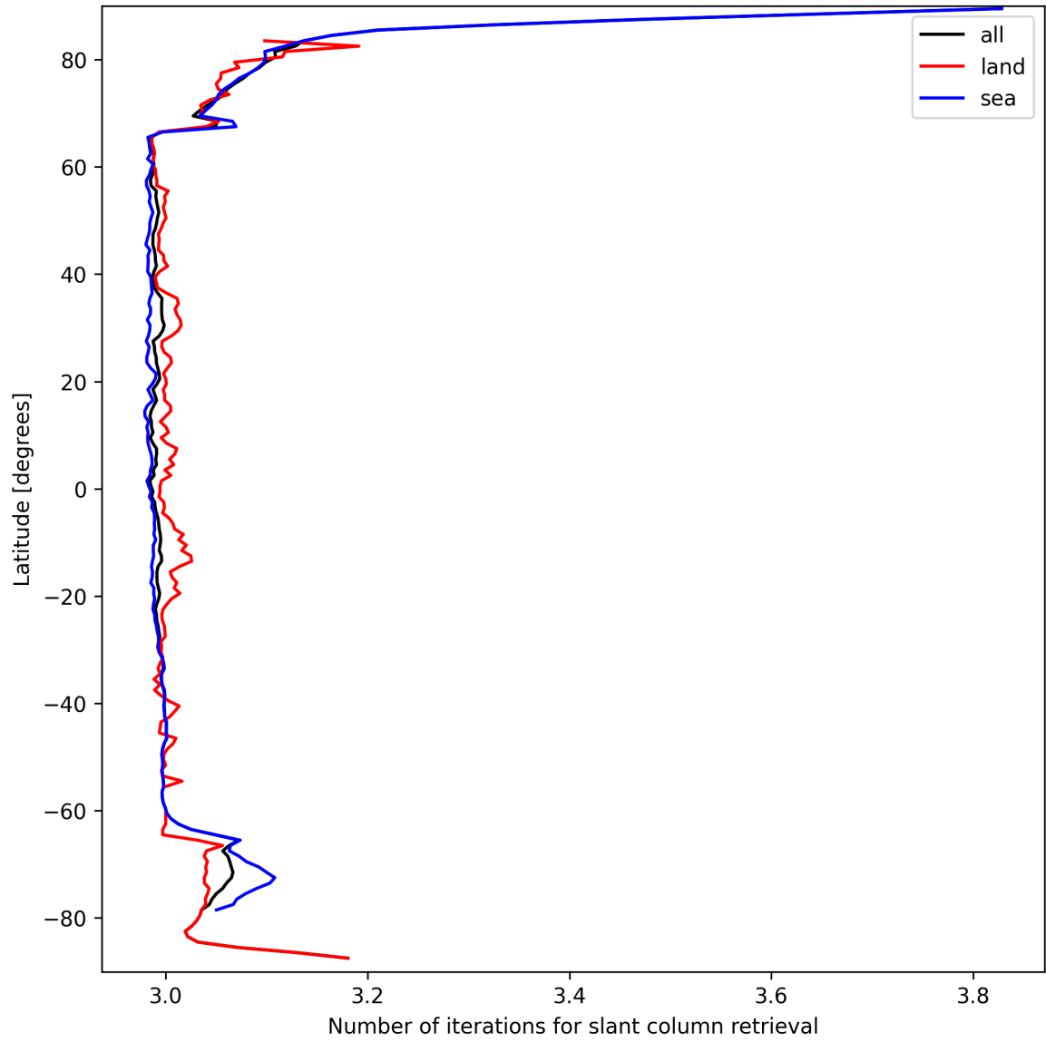
Figure 21: Zonal average of “Number of iterations for slant column retrieval” for 2025-09-17 to 2025-09-18.
