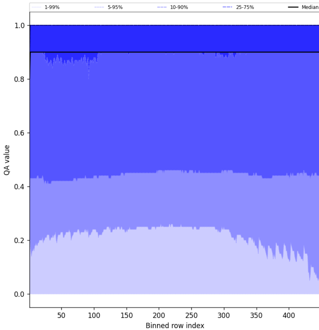
Figure 40: Along track statistics of “QA value” for 2025-09-17 to 2025-09-18
