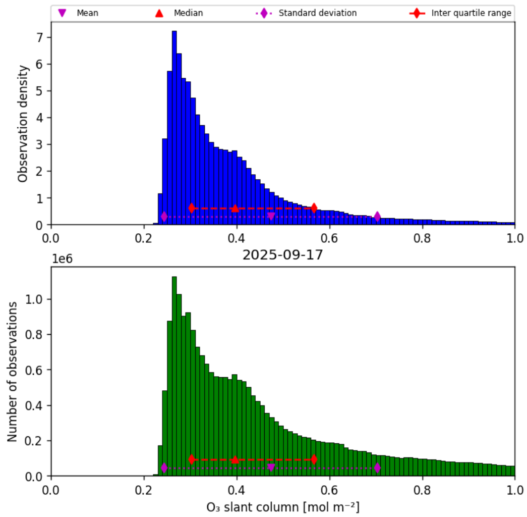
Figure 31: Histogram of “O 3 slant column” for 2025-09-17 to 2025-09-18
