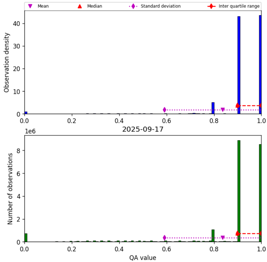
Figure 28: Histogram of “QA value” for 2025-09-17 to 2025-09-18
