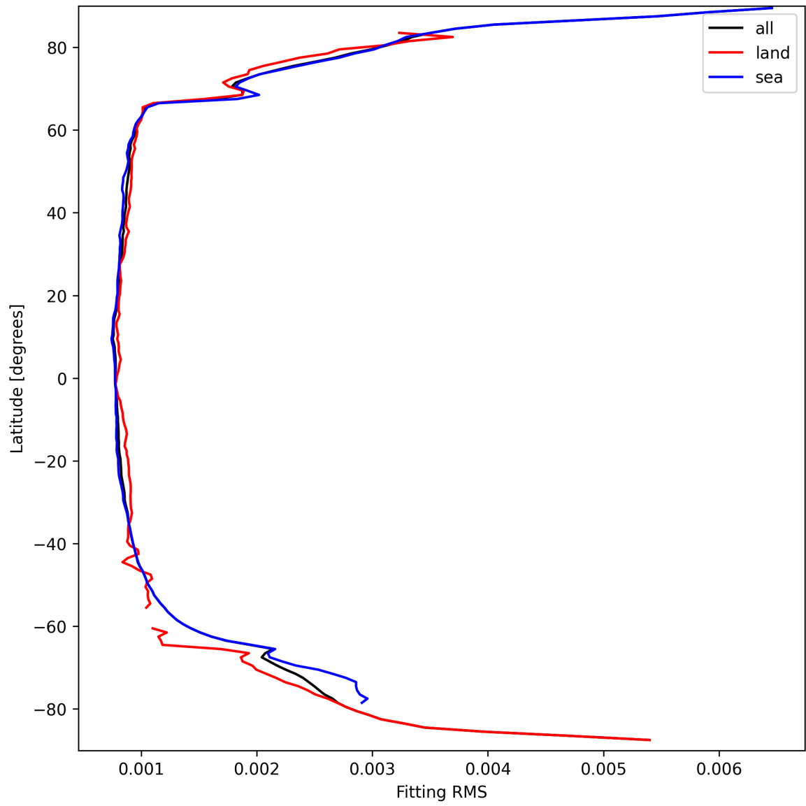
Figure 22: Zonal average of “Fitting RMS” for 2025-09-17 to 2025-09-18.
