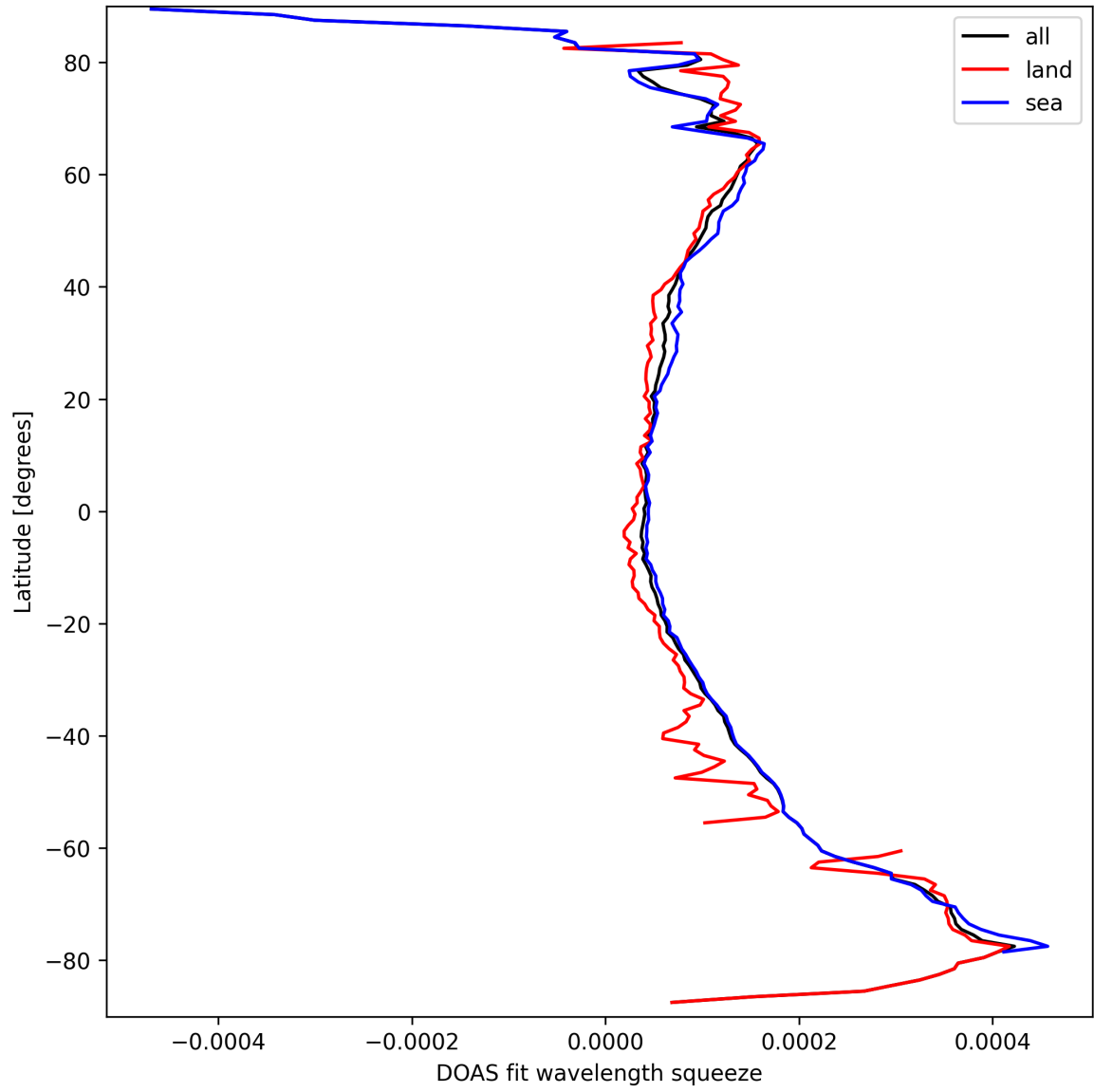
Figure 24: Zonal average of “DOAS fit wavelength squeeze” for 2025-09-17 to 2025-09-18.
