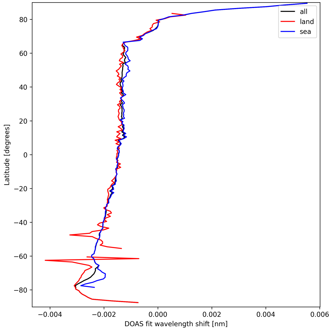
Figure 23: Zonal average of “DOAS fit wavelength shift” for 2025-09-17 to 2025-09-18.
