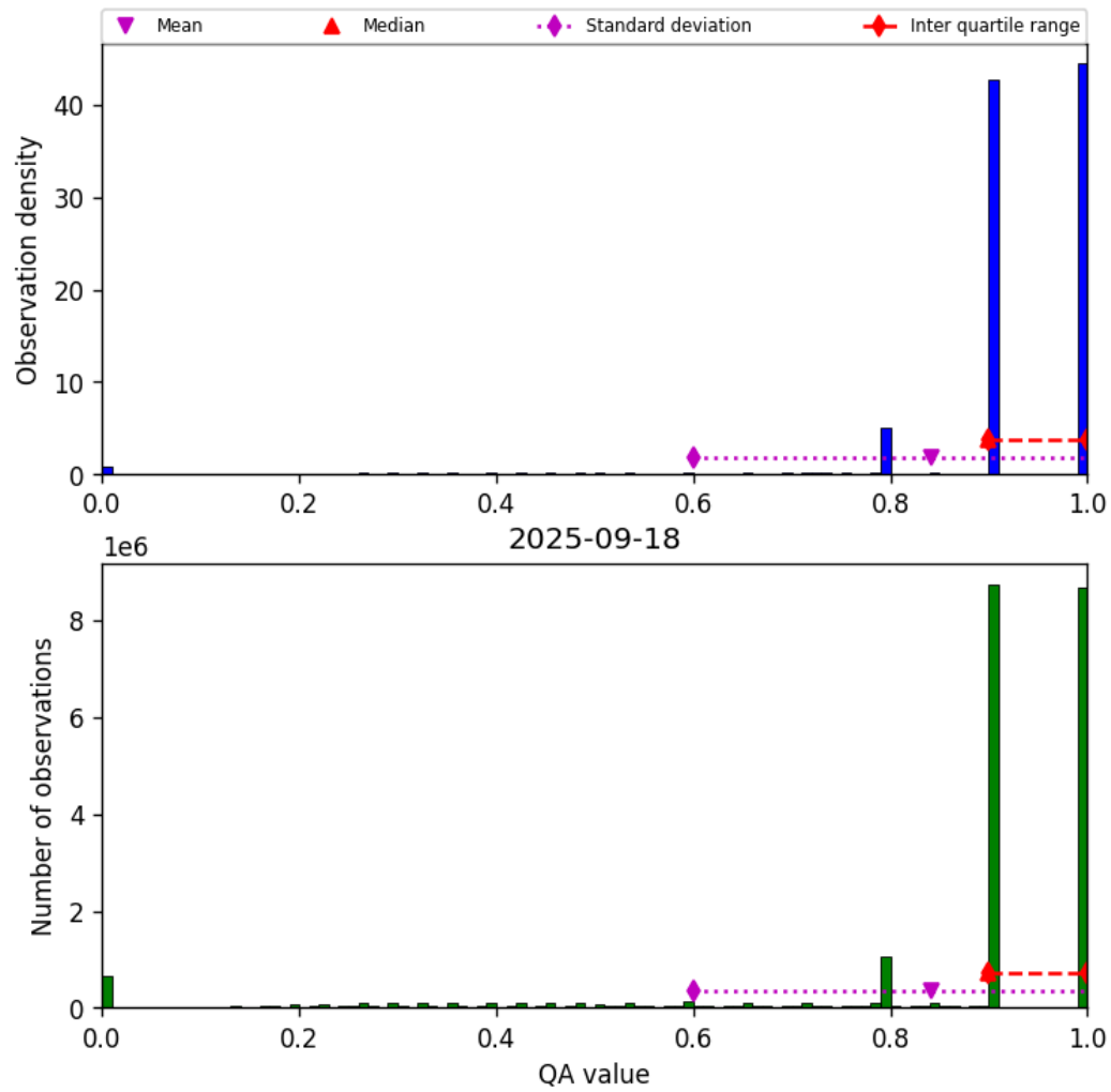
Figure 28: Histogram of “QA value” for 2025-09-18 to 2025-09-18
