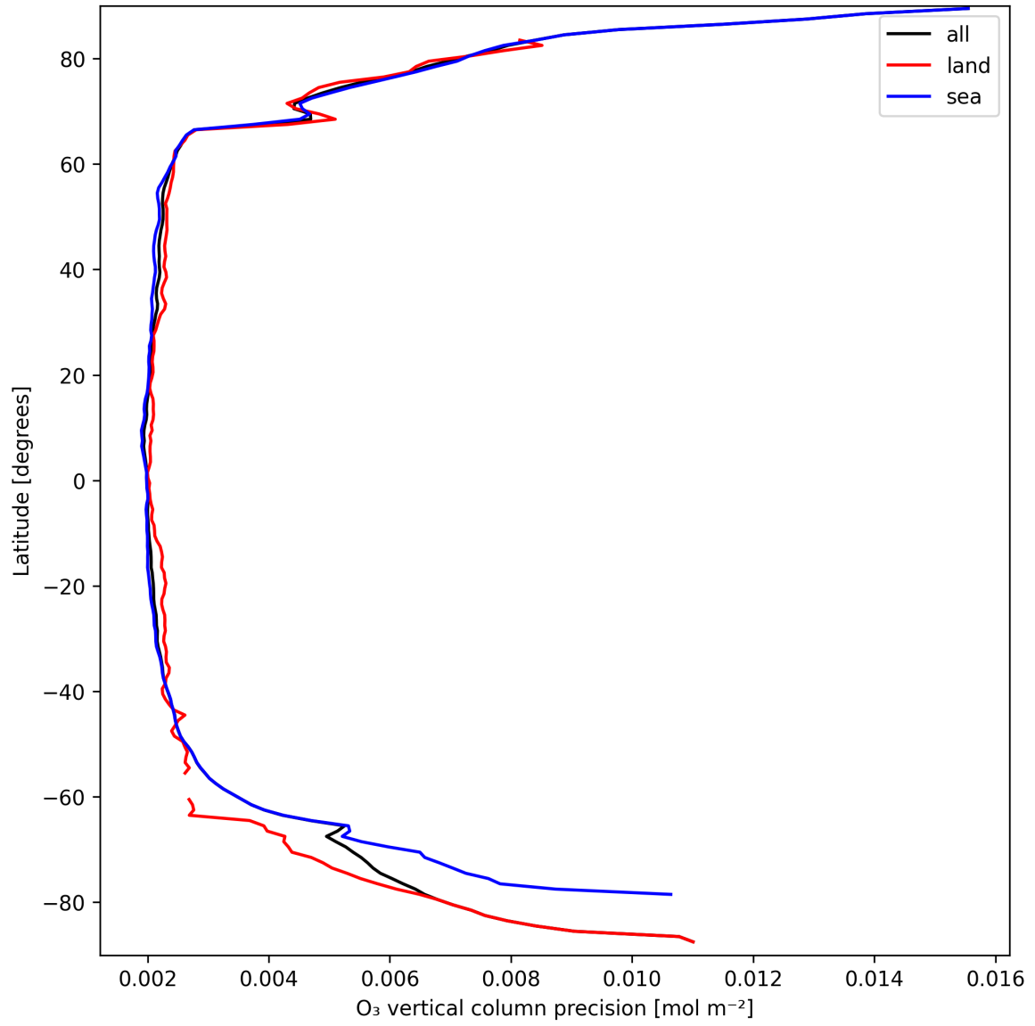
Figure 18: Zonal average of “O 3 vertical column precision” for 2025-09-18 to 2025-09-18.
