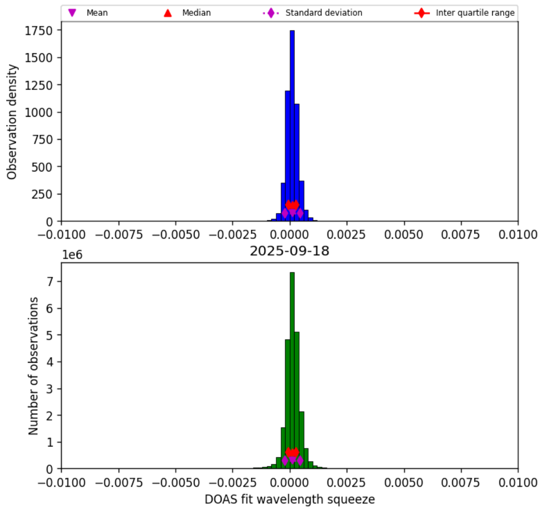
Figure 36: Histogram of “DOAS fit wavelength squeeze” for 2025-09-18 to 2025-09-18
