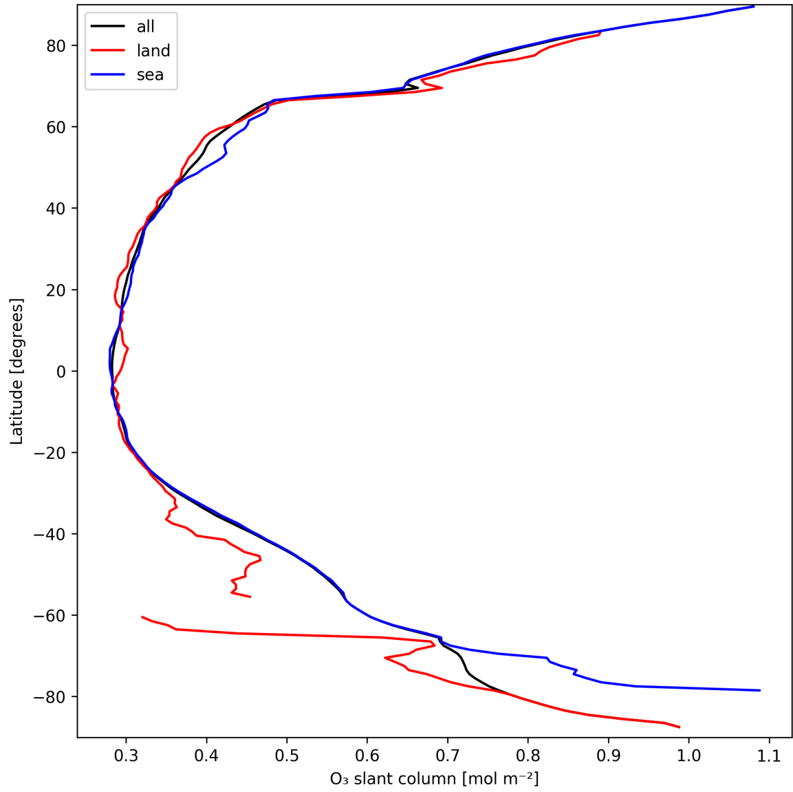
Figure 19: Zonal average of “O 3 slant column” for 2025-09-18 to 2025-09-18.
