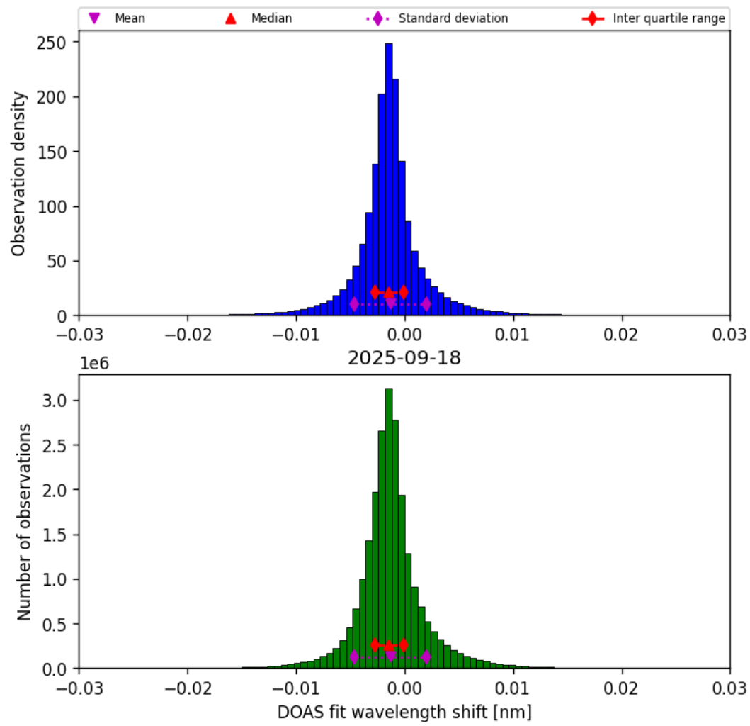
Figure 35: Histogram of “DOAS fit wavelength shift” for 2025-09-18 to 2025-09-18
