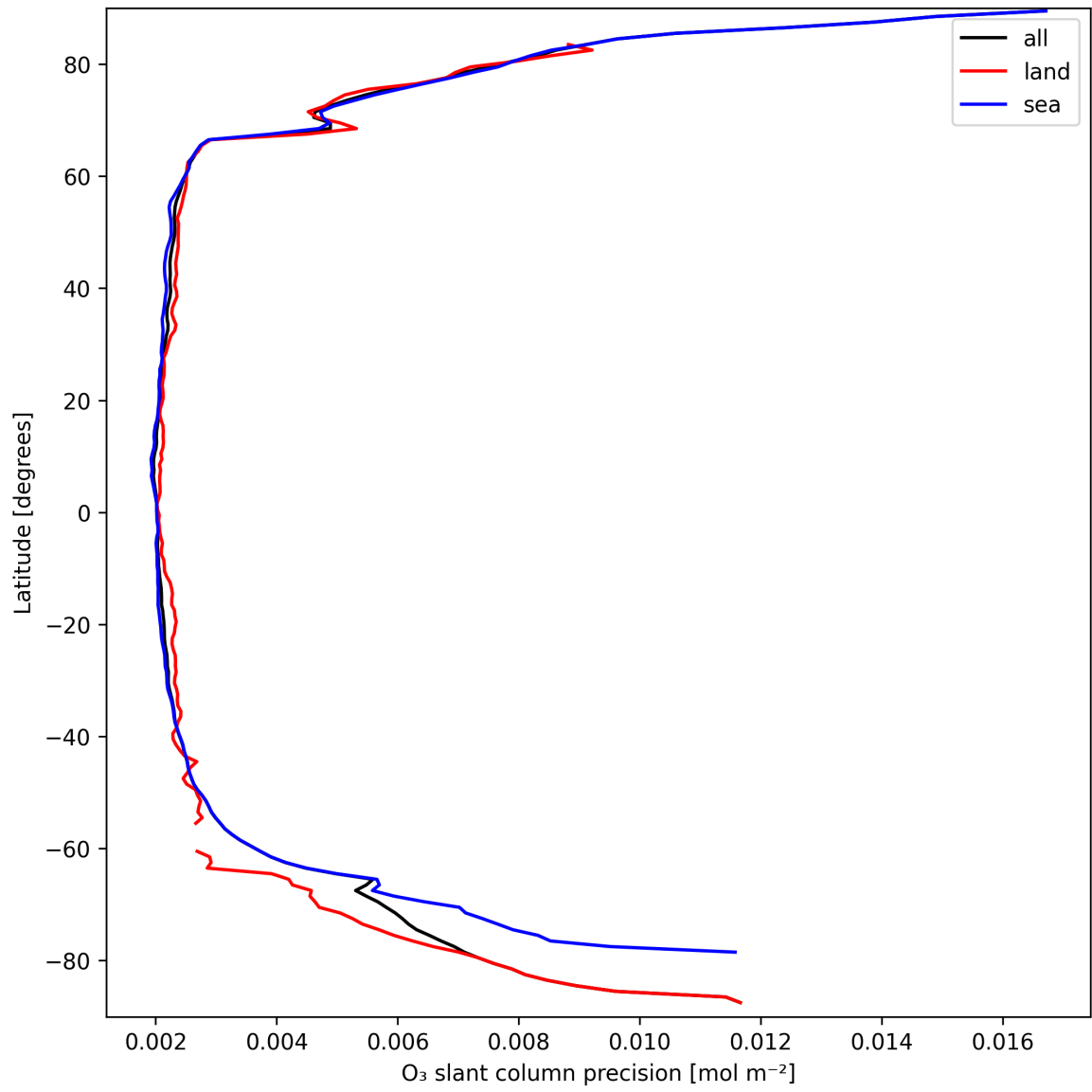
Figure 20: Zonal average of “O 3 slant column precision” for 2025-09-18 to 2025-09-18.
