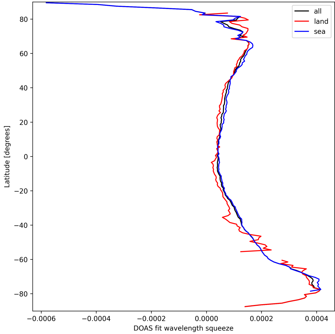
Figure 24: Zonal average of “DOAS fit wavelength squeeze” for 2025-09-18 to 2025-09-18.
