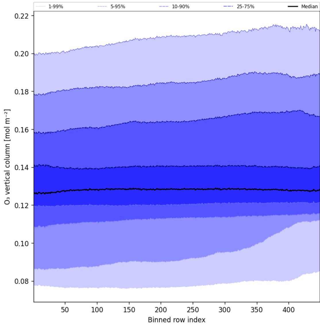
Figure 41: Along track statistics of “O 3 vertical column” for 2025-09-18 to 2025-09-18
