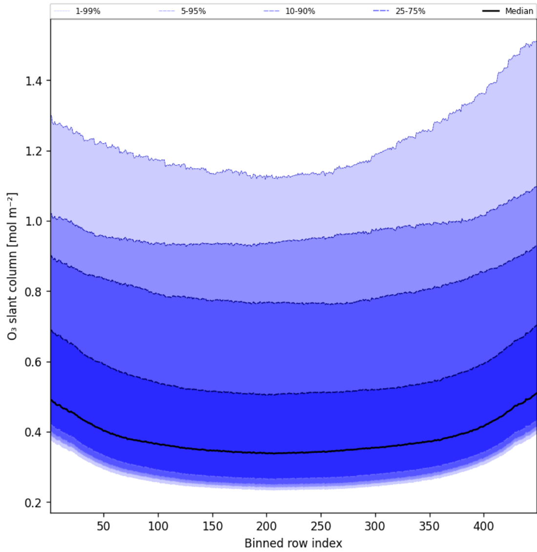
Figure 43: Along track statistics of “O 3 slant column” for 2025-09-18 to 2025-09-18
