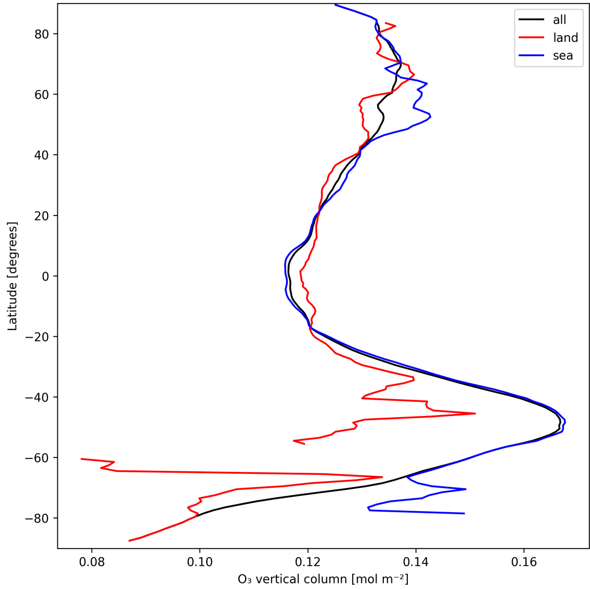
Figure 17: Zonal average of “O 3 vertical column” for 2025-09-18 to 2025-09-18.
