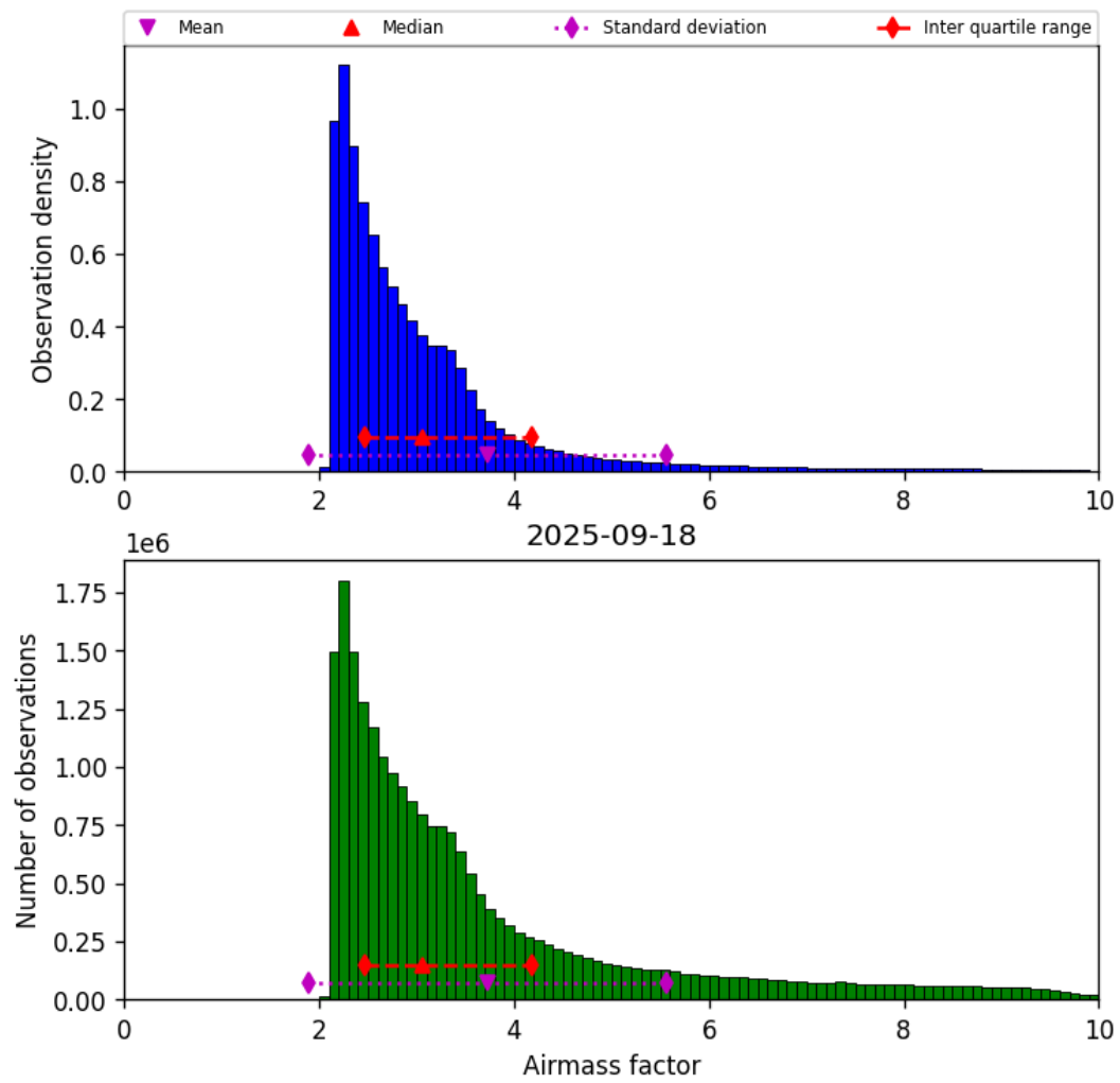
Figure 37: Histogram of “Airmass factor” for 2025-09-18 to 2025-09-18
