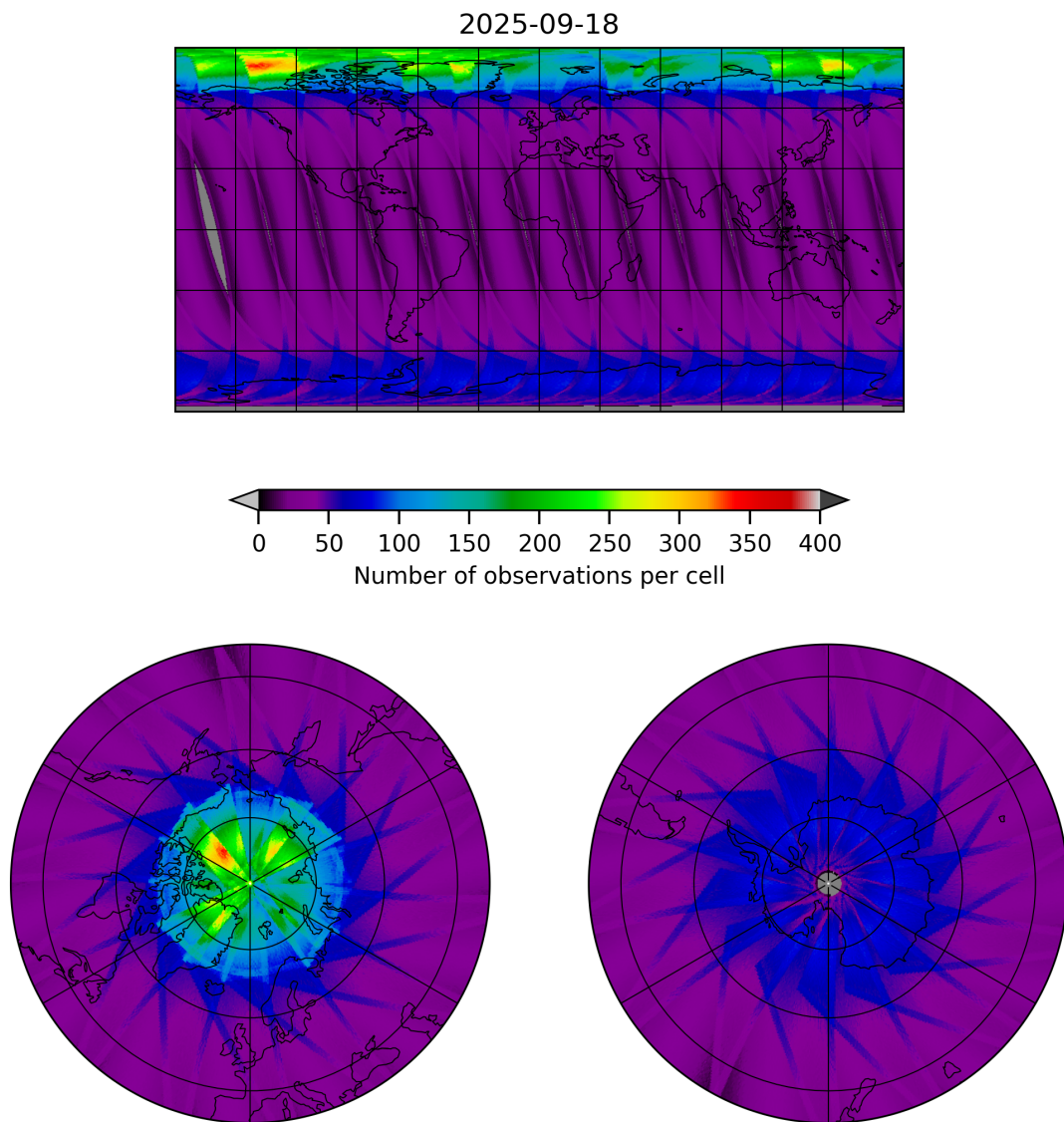
Figure 15: Map of the number of observations for 2025-09-18 to 2025-09-18
