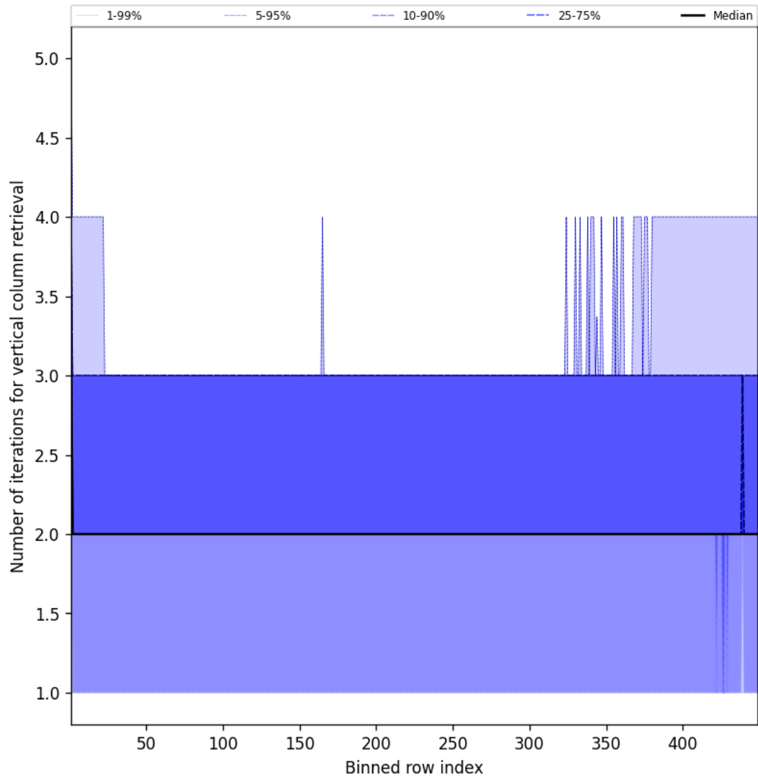
Figure 51: Along track statistics of “Number of iterations for vertical column retrieval” for 2025-09-18 to 2025-09-18
