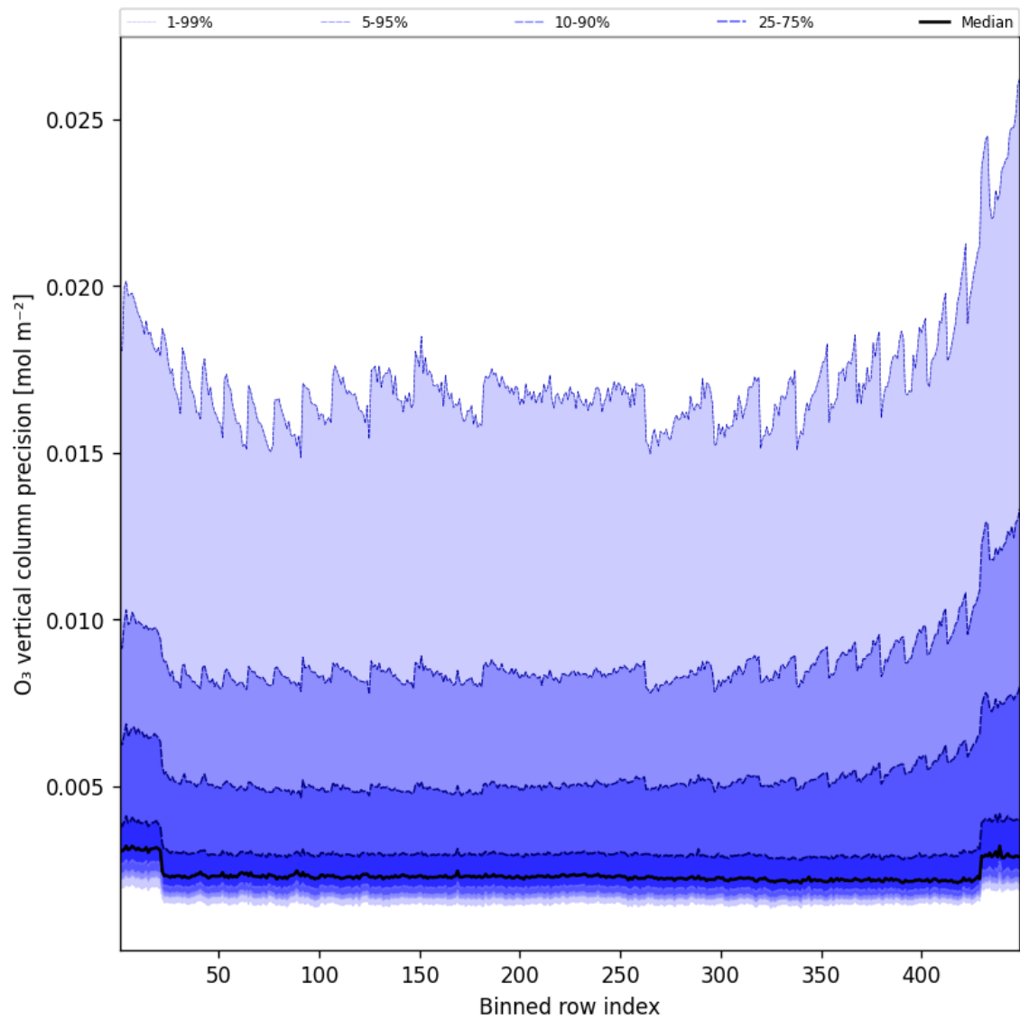
Figure 42: Along track statistics of “O 3 vertical column precision” for 2025-09-18 to 2025-09-18
