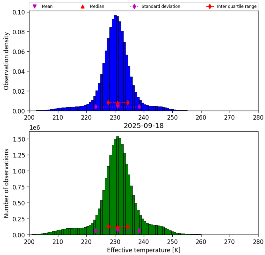
Figure 38: Histogram of “Effective temperature” for 2025-09-18 to 2025-09-18
