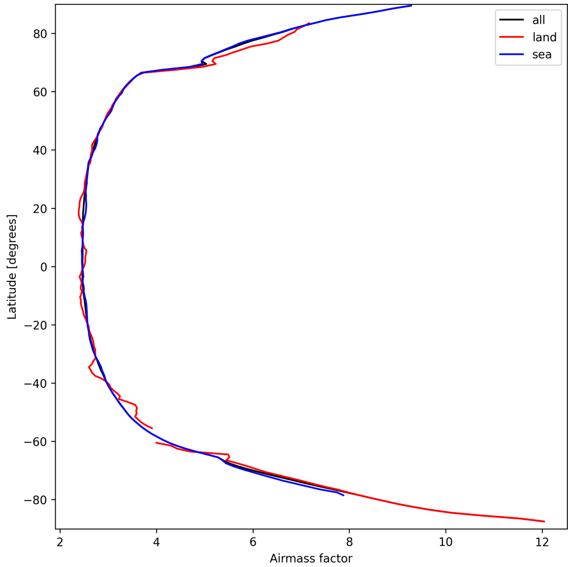
Figure 25: Zonal average of “Airmass factor” for 2025-09-18 to 2025-09-18.
