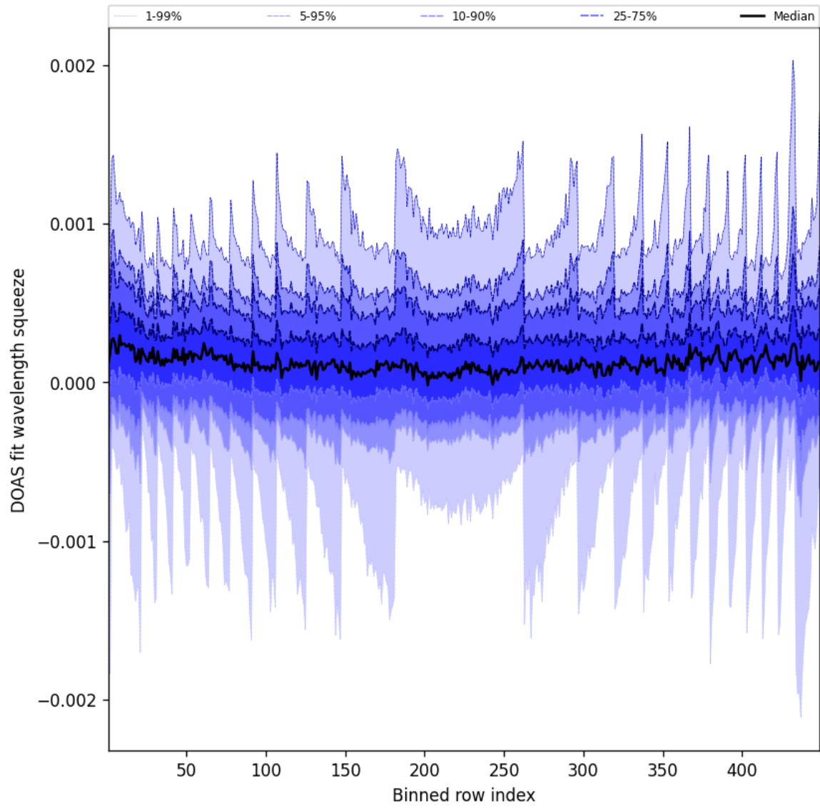
Figure 48: Along track statistics of “DOAS fit wavelength squeeze” for 2025-09-18 to 2025-09-18
