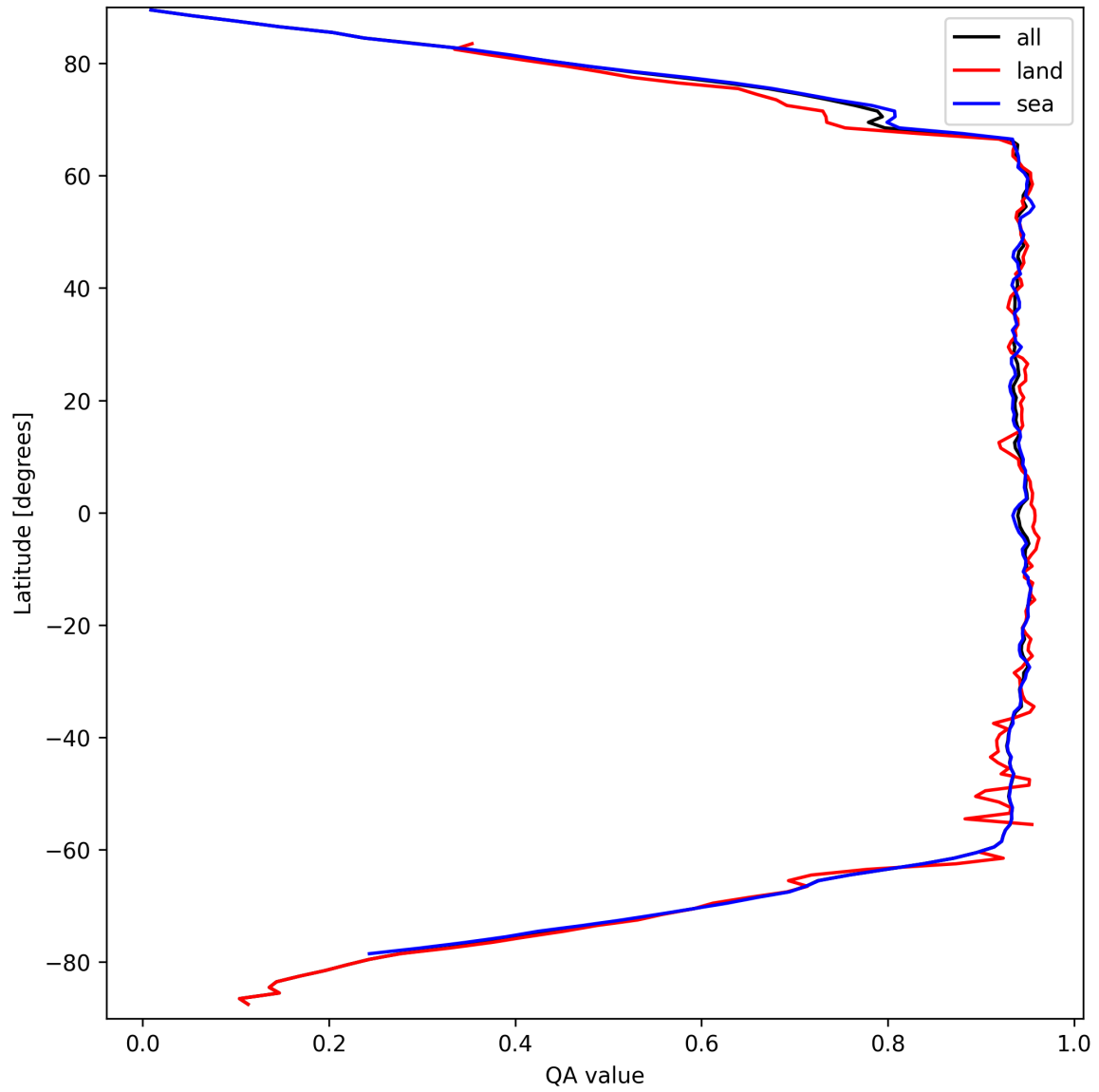
Figure 16: Zonal average of “QA value” for 2025-09-18 to 2025-09-18.
