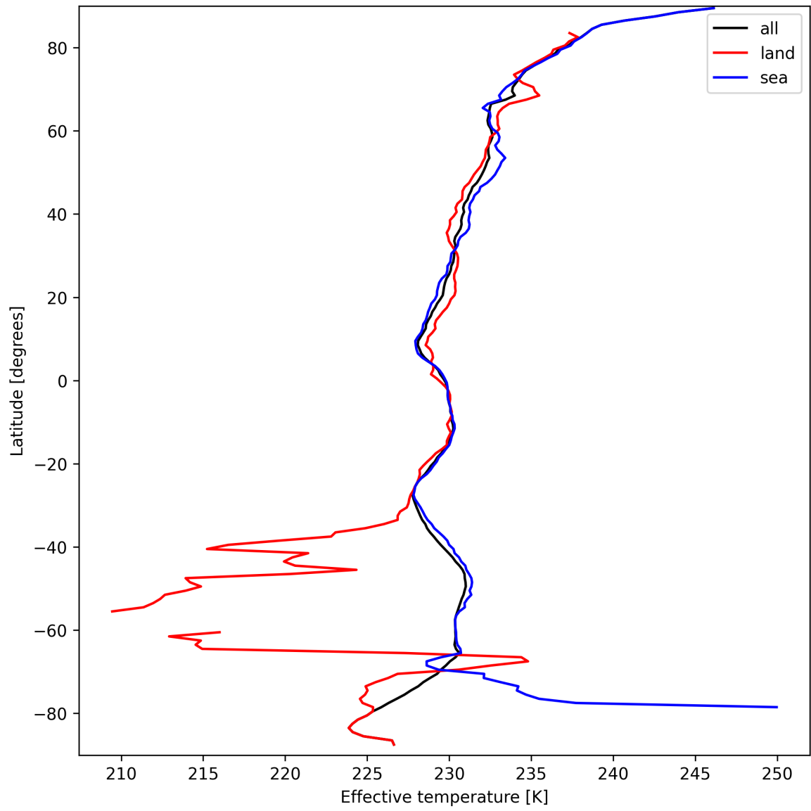
Figure 26: Zonal average of "Effective temperature" for 2025-09-18 to 2025-09-18.
