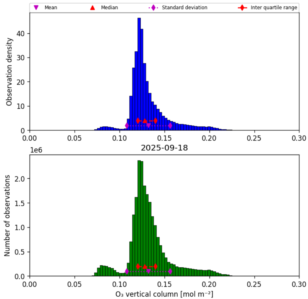
Figure 29: Histogram of “O 3 vertical column” for 2025-09-18 to 2025-09-18
