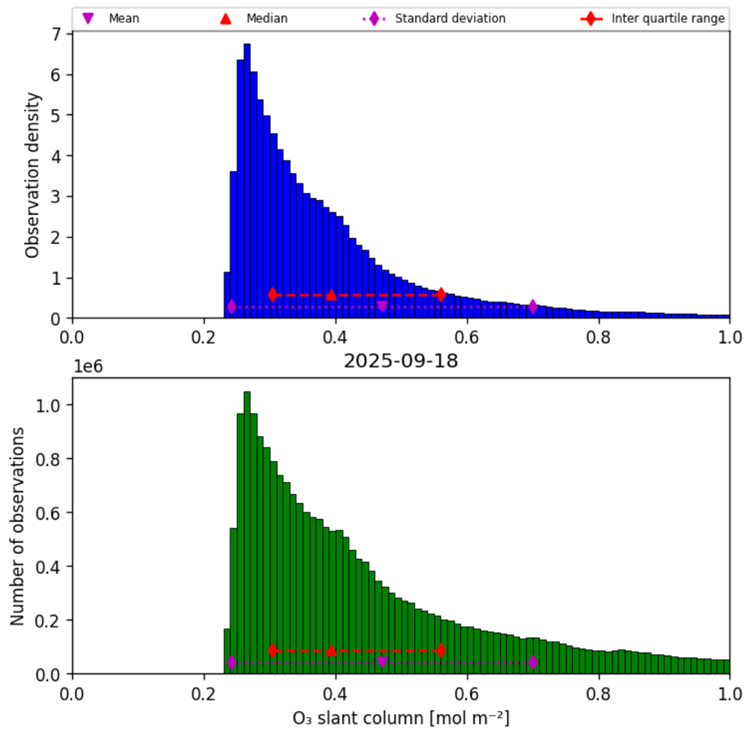
Figure 31: Histogram of “O 3 slant column” for 2025-09-18 to 2025-09-18
