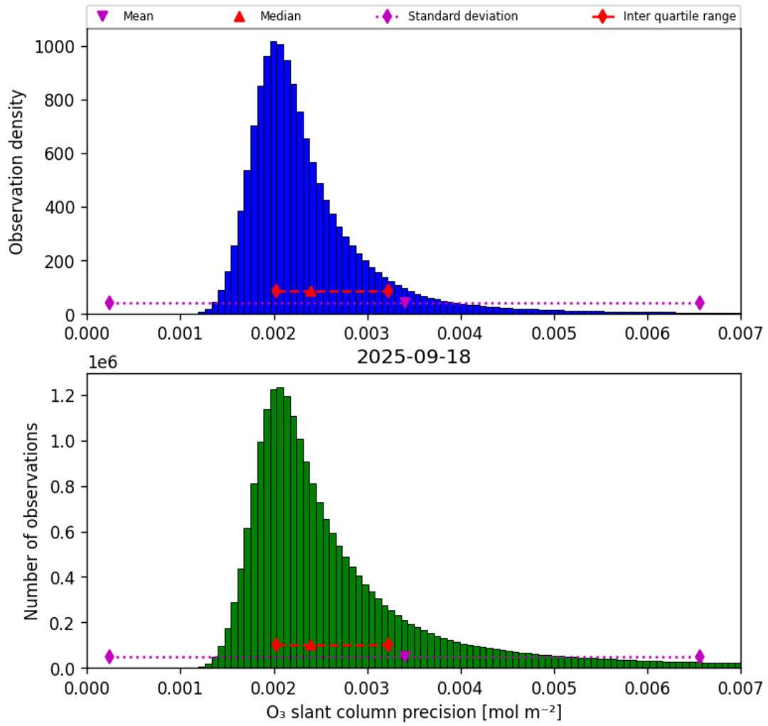
Figure 32: Histogram of “O 3 slant column precision” for 2025-09-18 to 2025-09-18
