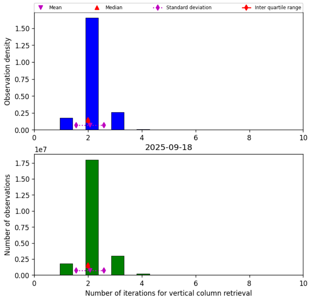
Figure 39: Histogram of “Number of iterations for vertical column retrieval” for 2025-09-18 to 2025-09-18
