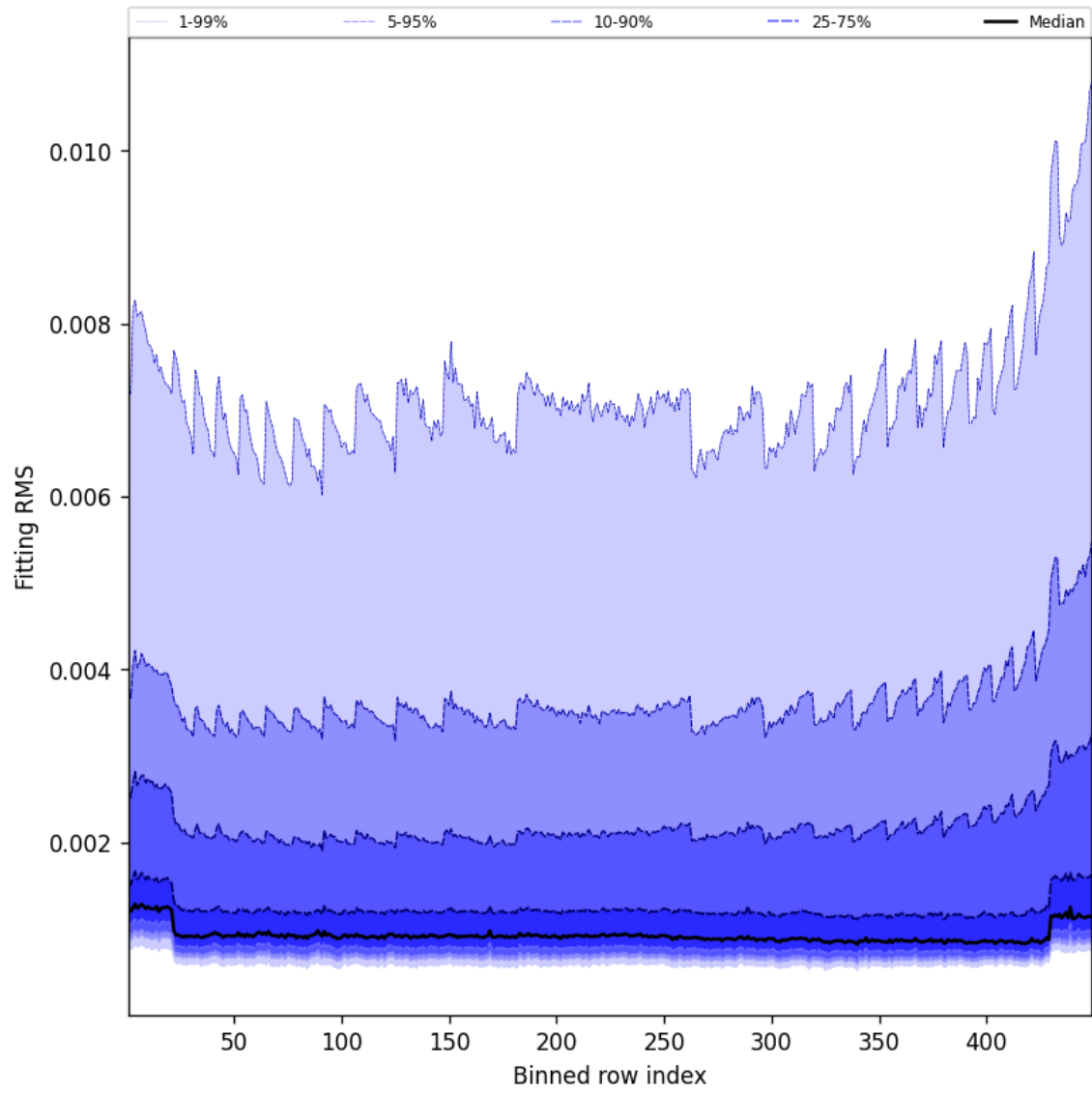
Figure 46: Along track statistics of “Fitting RMS” for 2025-09-18 to 2025-09-18
