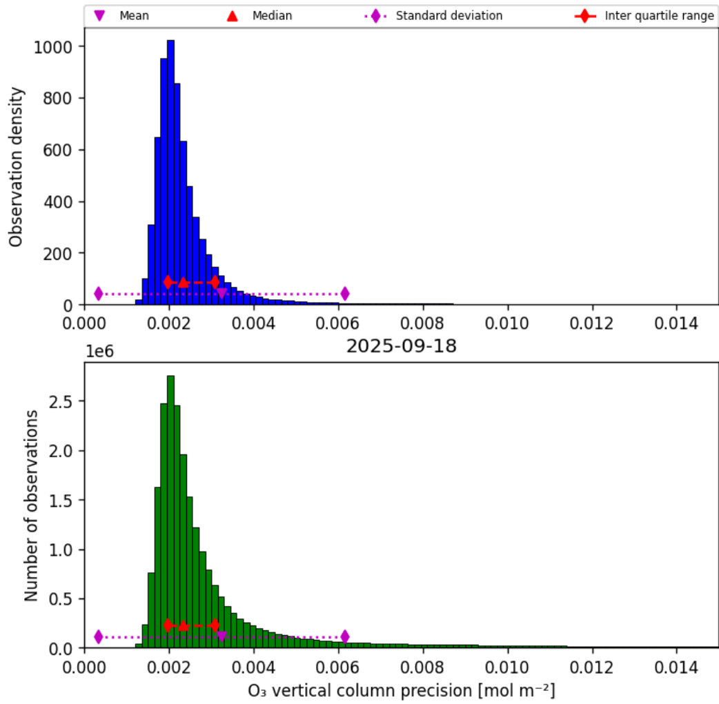
Figure 30: Histogram of “O 3 vertical column precision” for 2025-09-18 to 2025-09-18
