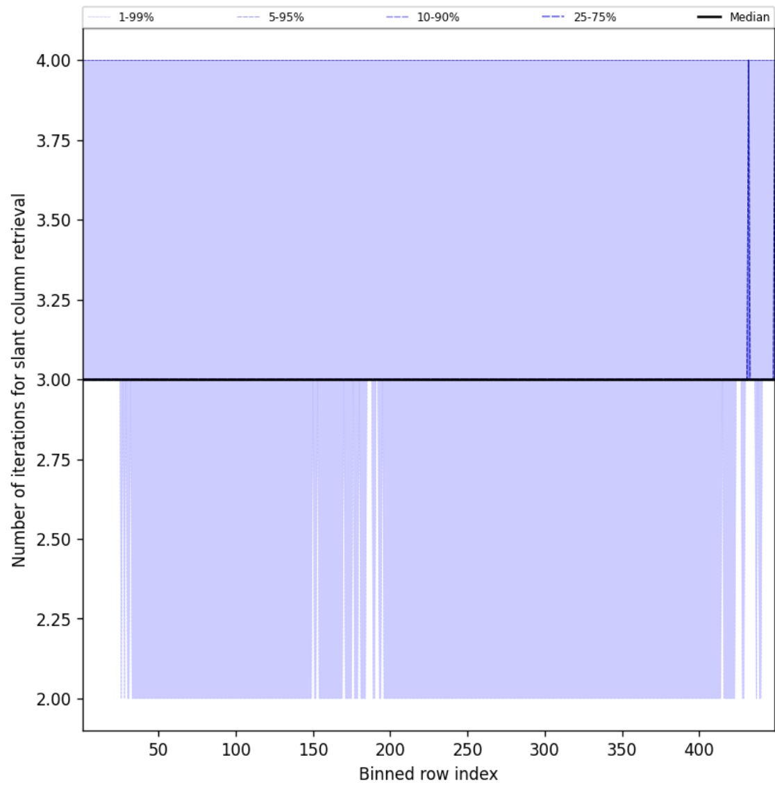
Figure 45: Along track statistics of “Number of iterations for slant column retrieval” for 2025-09-18 to 2025-09-18
