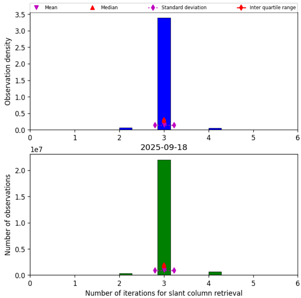
Figure 33: Histogram of "Number of iterations for slant column retrieval" for 2025-09-18 to 2025-09-18
