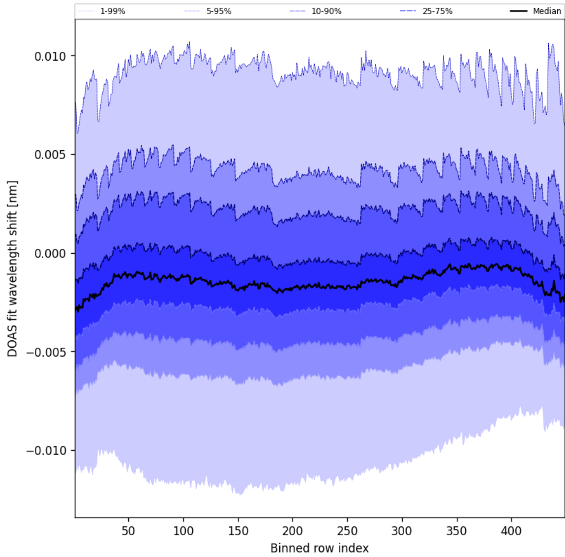
Figure 47: Along track statistics of “DOAS fit wavelength shift” for 2025-09-18 to 2025-09-18
