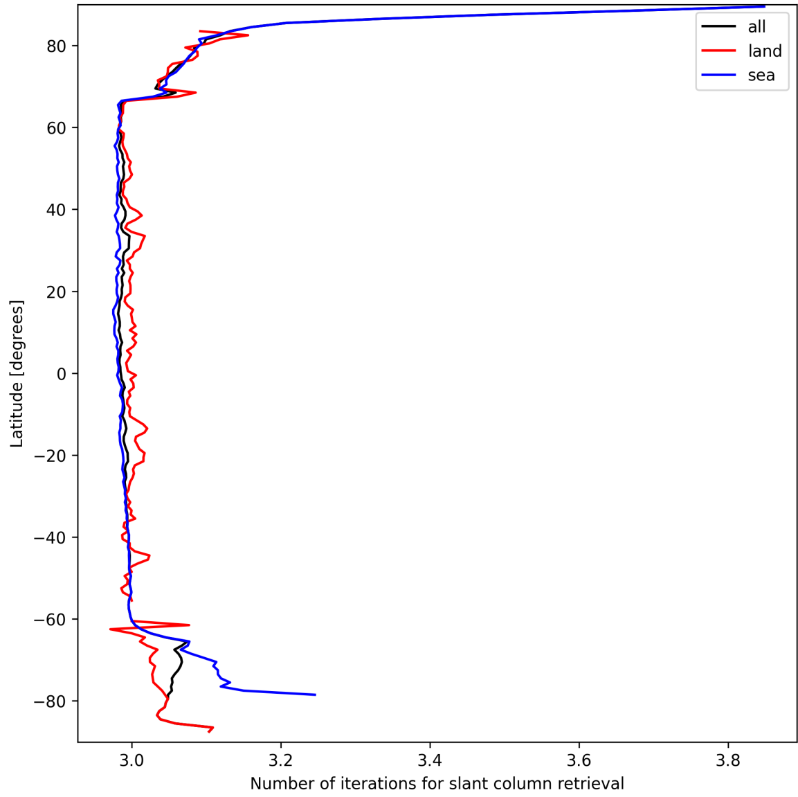
Figure 21: Zonal average of “Number of iterations for slant column retrieval” for 2025-09-18 to 2025-09-18.
