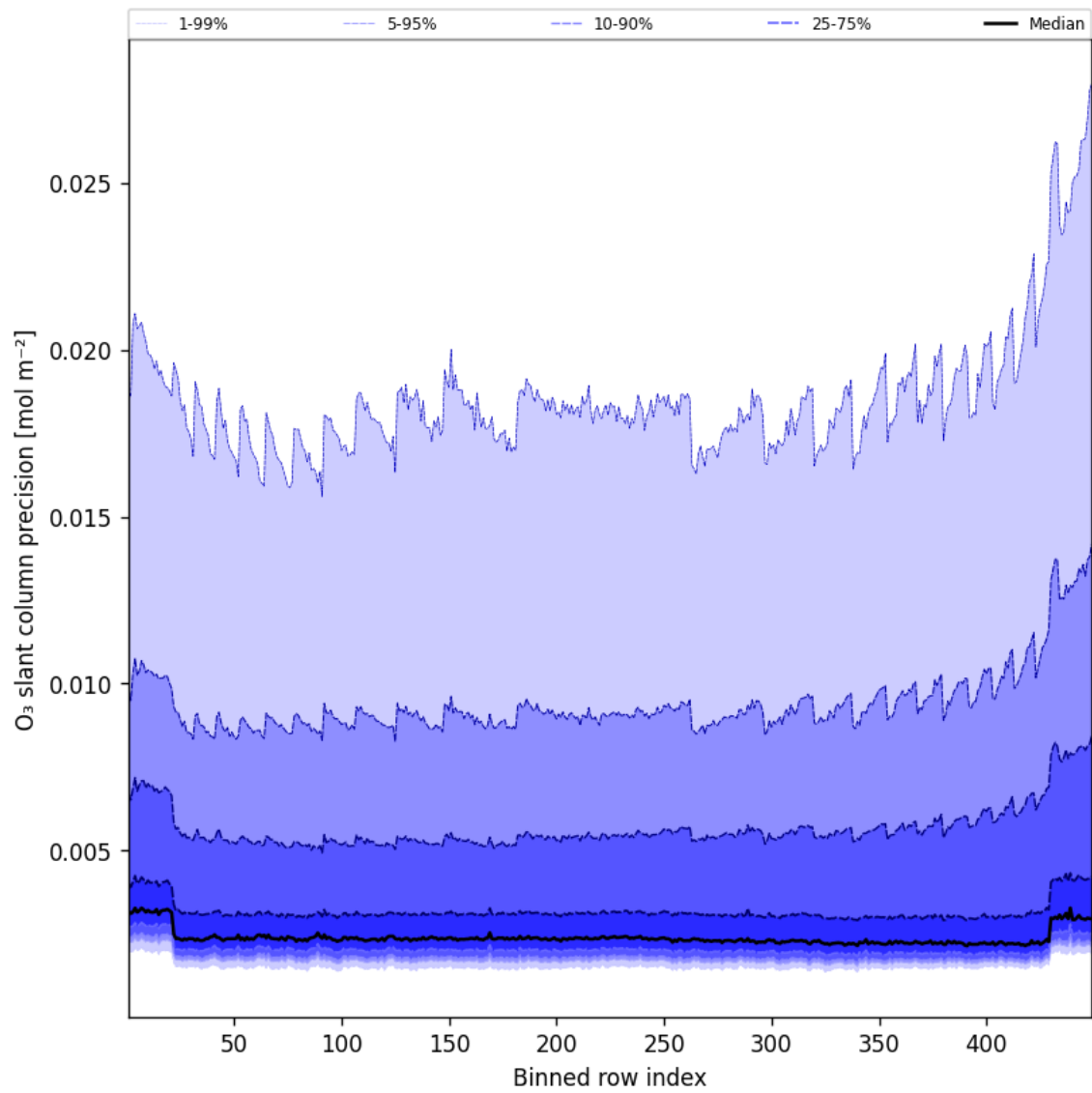
Figure 44: Along track statistics of “O 3 slant column precision” for 2025-09-18 to 2025-09-18
