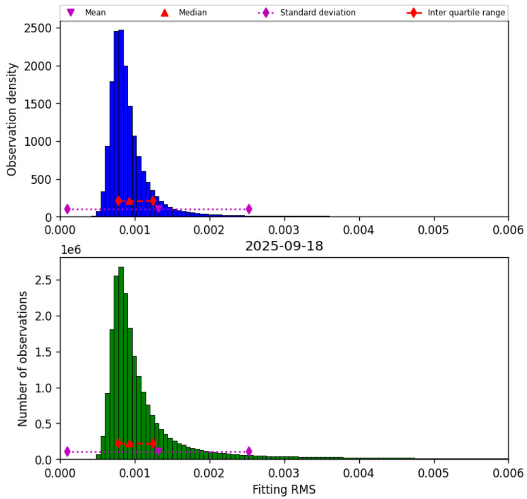
Figure 34: Histogram of “Fitting RMS” for 2025-09-18 to 2025-09-18
