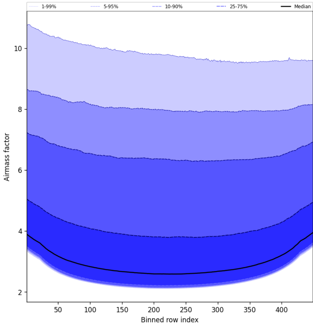
Figure 49: Along track statistics of “Airmass factor” for 2025-09-18 to 2025-09-18
