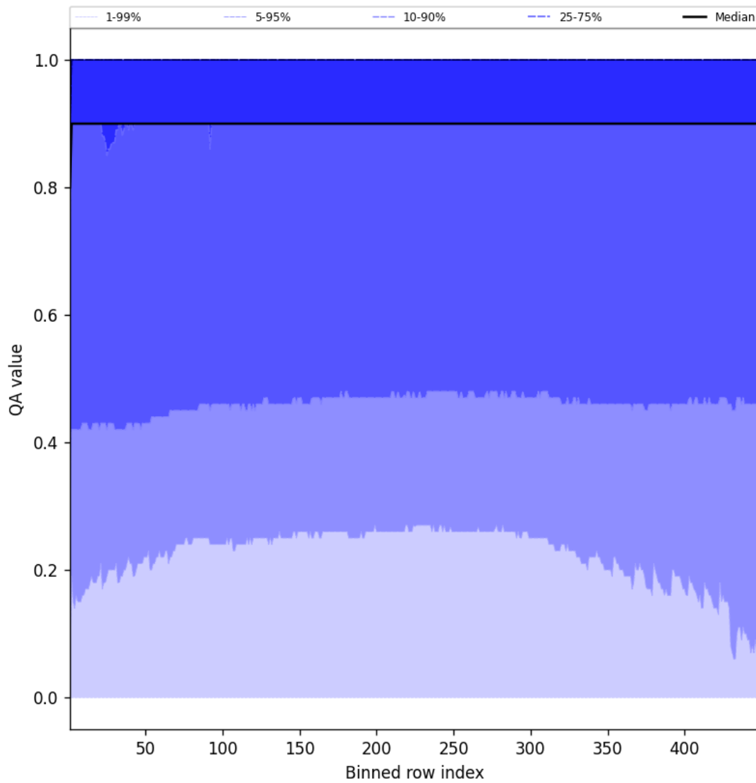
Figure 40: Along track statistics of “QA value” for 2025-09-18 to 2025-09-18
