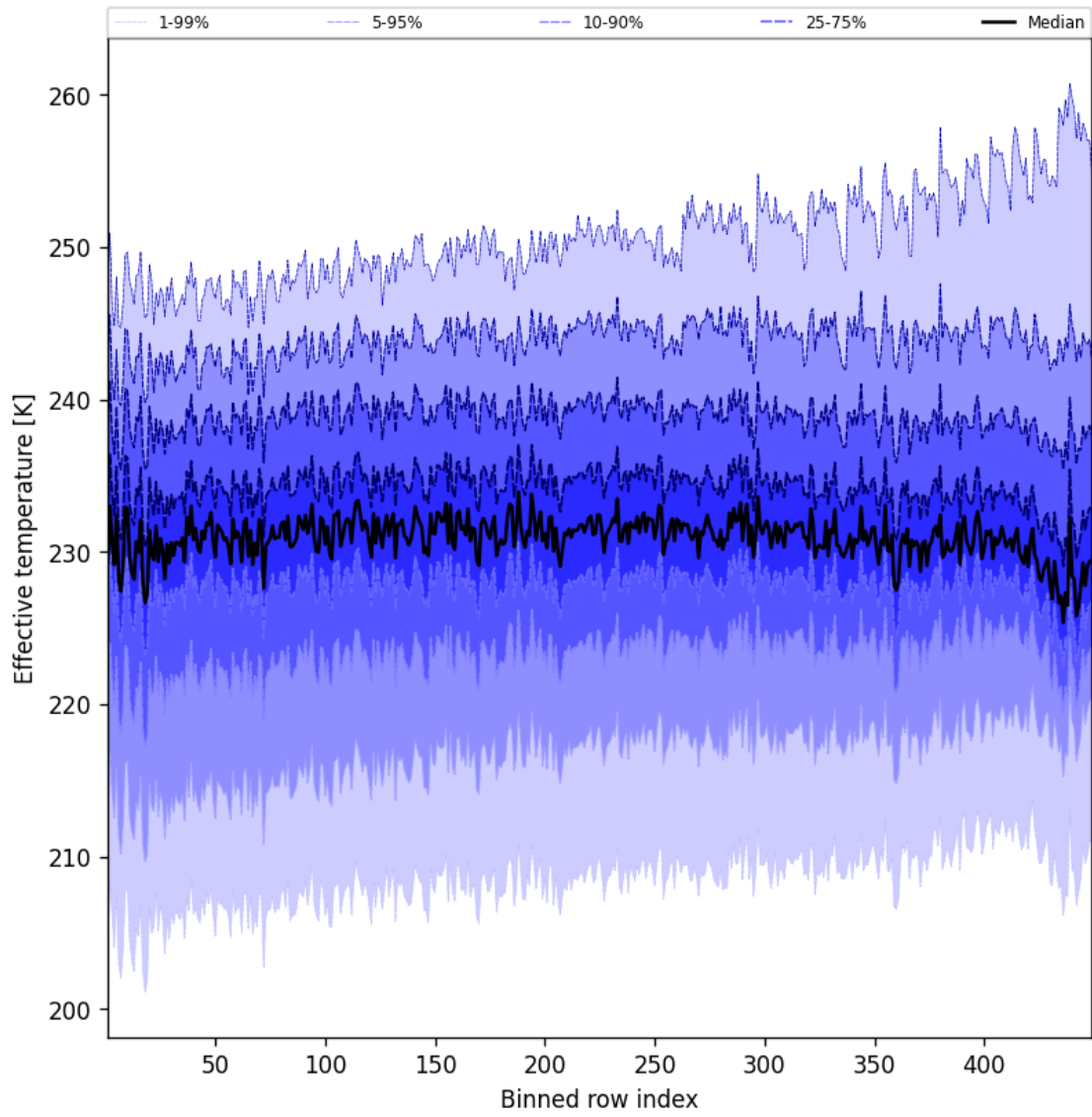
Figure 50: Along track statistics of “Effective temperature” for 2025-09-18 to 2025-09-18
