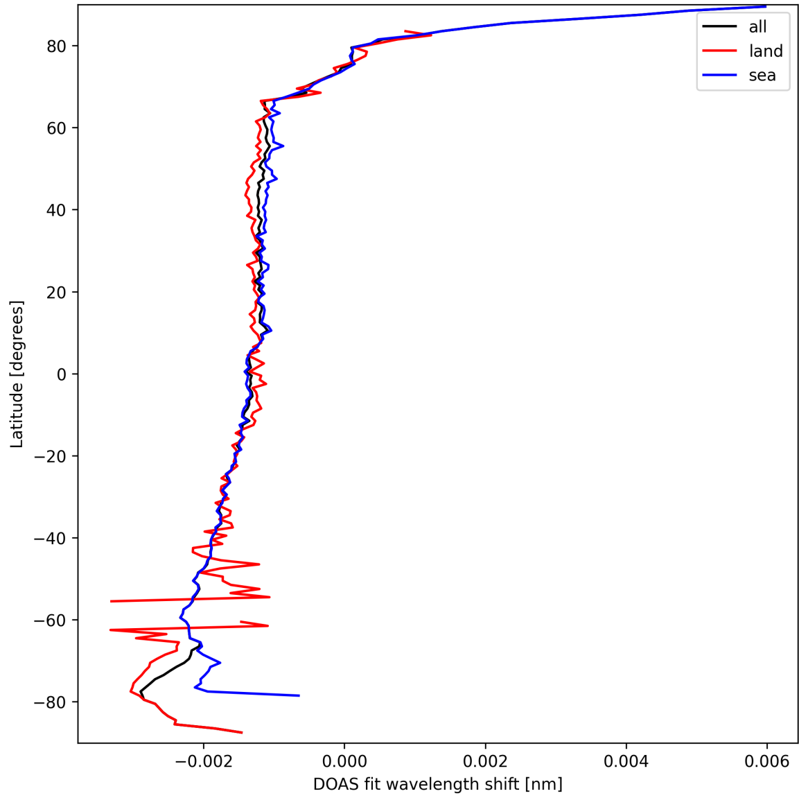
Figure 23: Zonal average of “DOAS fit wavelength shift” for 2025-09-18 to 2025-09-18.
