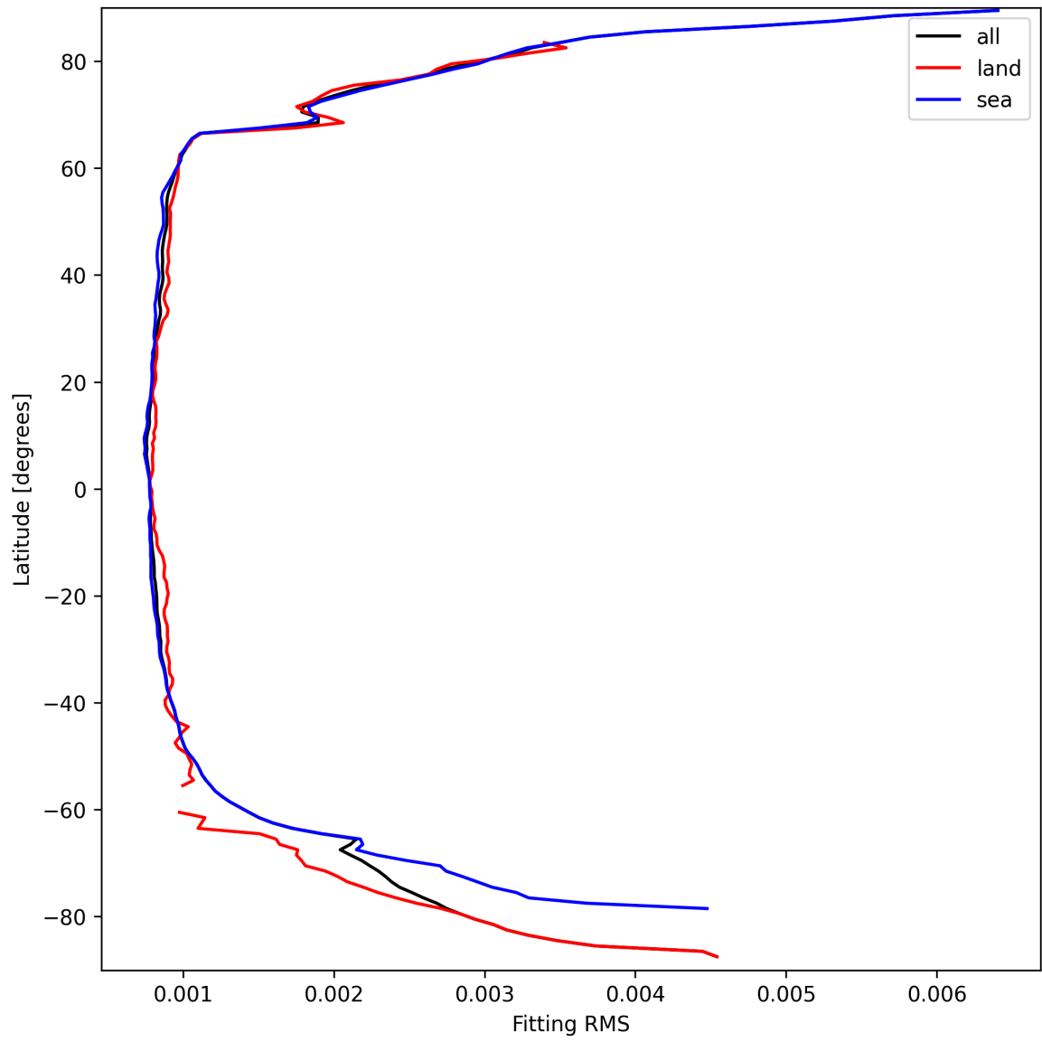
Figure 22: Zonal average of “Fitting RMS” for 2025-09-18 to 2025-09-18.
