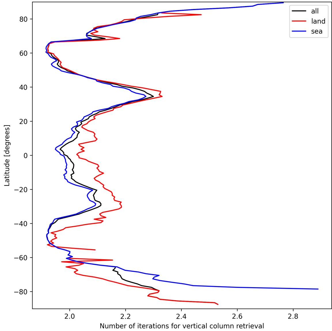
Figure 27: Zonal average of “Number of iterations for vertical column retrieval” for 2025-09-18 to 2025-09-18.
