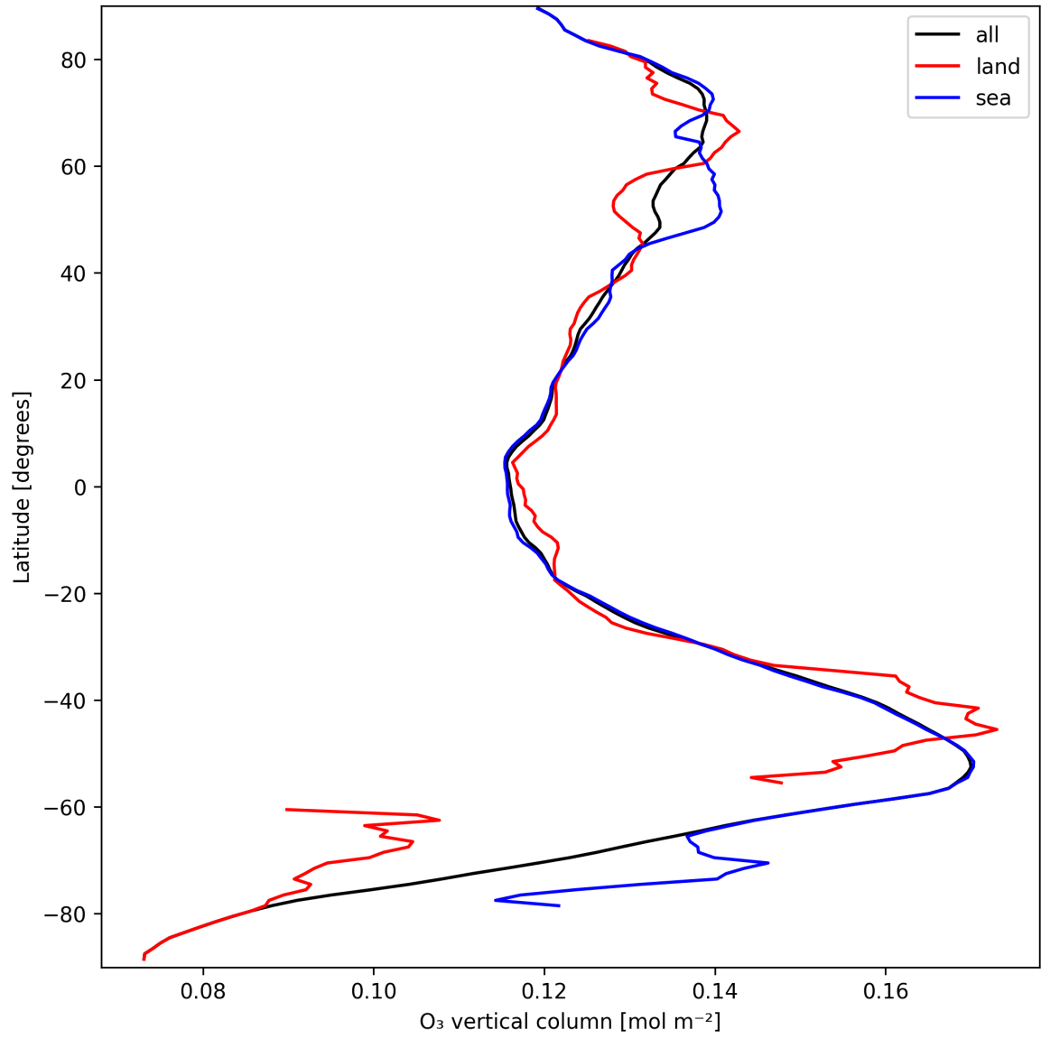
Figure 17: Zonal average of “O 3 vertical column” for 2025-09-20 to 2025-09-21.
