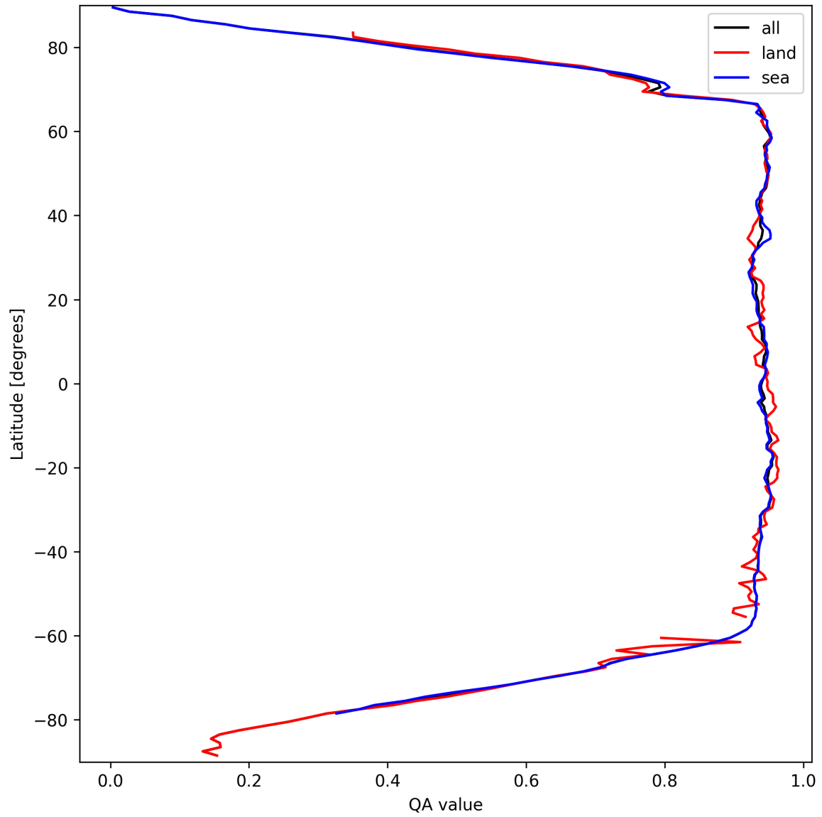
Figure 16: Zonal average of “QA value” for 2025-09-20 to 2025-09-21.
