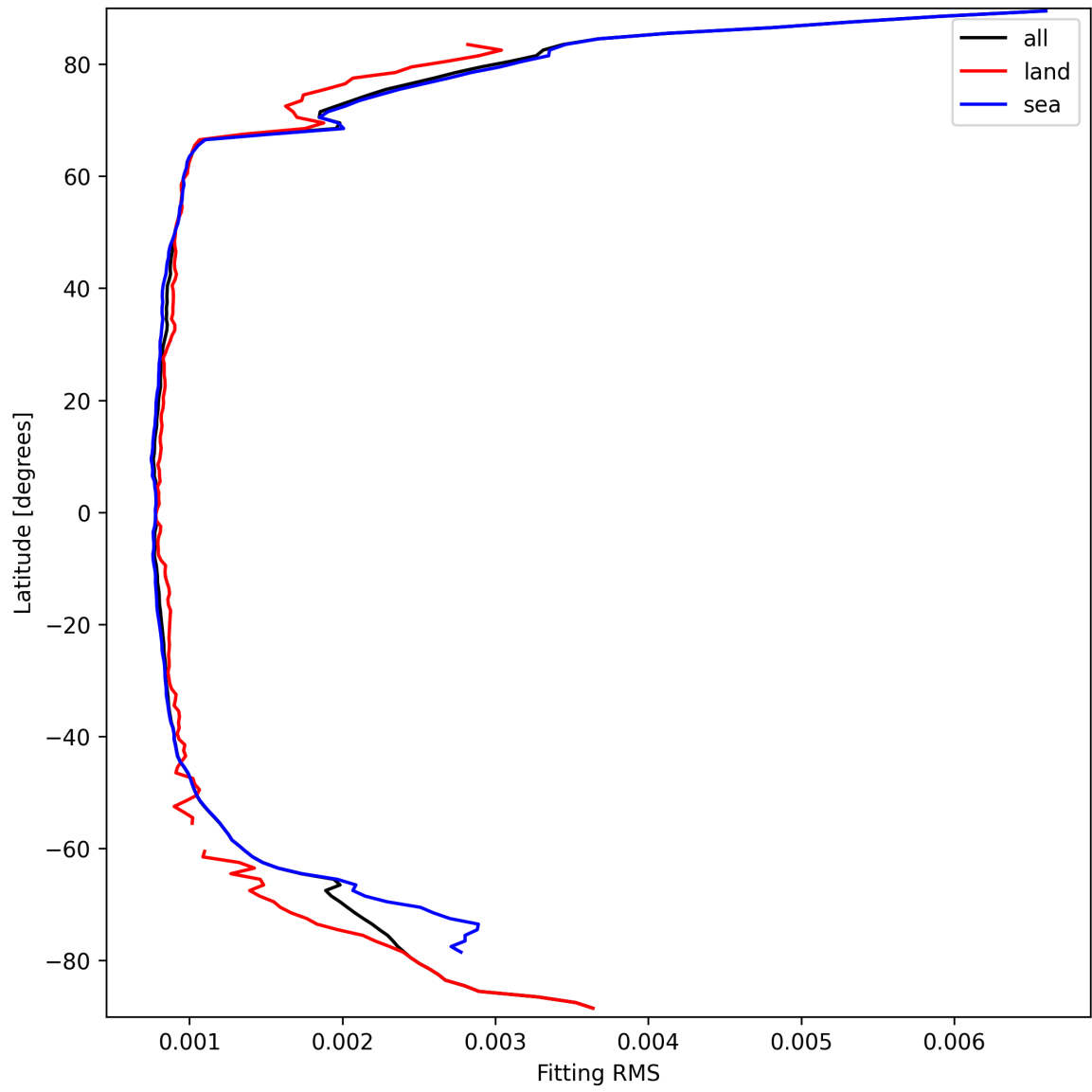
Figure 22: Zonal average of “Fitting RMS” for 2025-09-20 to 2025-09-21.
