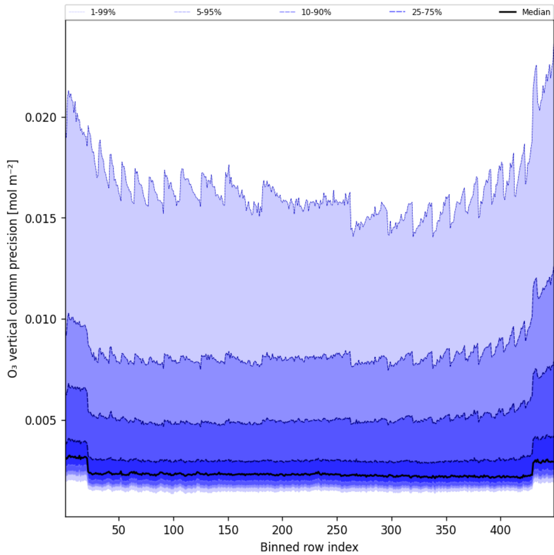
Figure 42: Along track statistics of “O 3 vertical column precision” for 2025-09-20 to 2025-09-21
