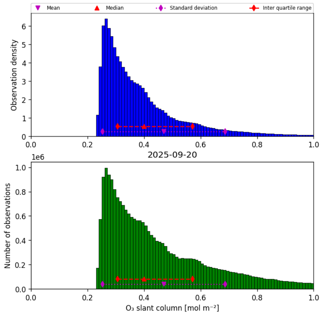
Figure 31: Histogram of “O 3 slant column” for 2025-09-20 to 2025-09-21
