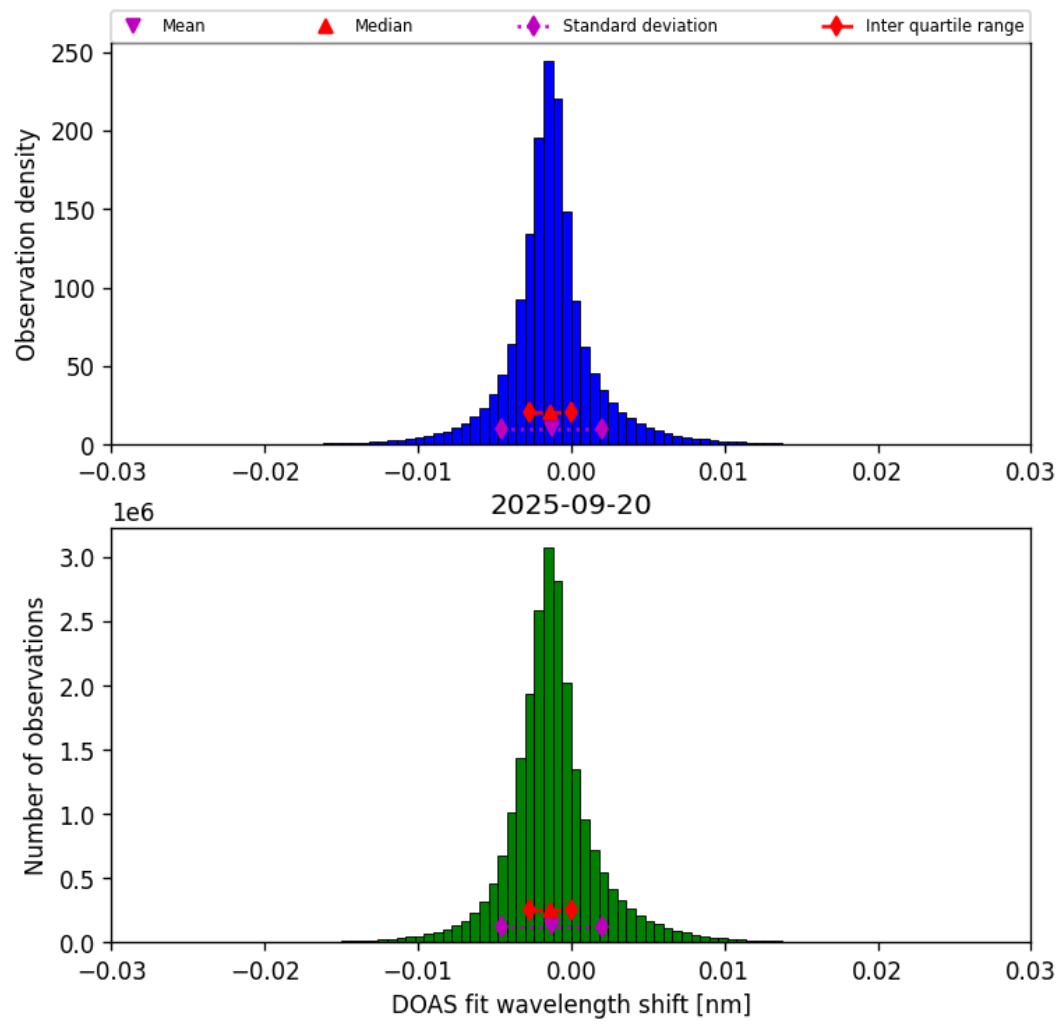
Figure 35: Histogram of “DOAS fit wavelength shift” for 2025-09-20 to 2025-09-21
