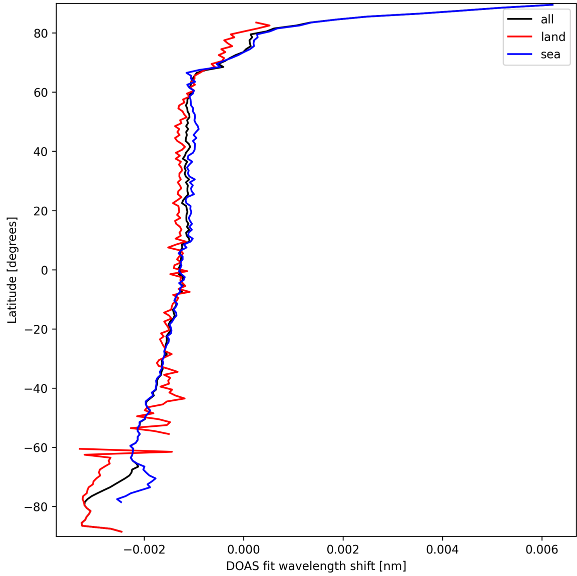
Figure 23: Zonal average of “DOAS fit wavelength shift” for 2025-09-20 to 2025-09-21.
