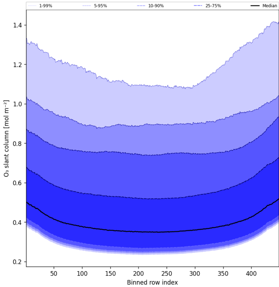
Figure 43: Along track statistics of “O 3 slant column” for 2025-09-20 to 2025-09-21
