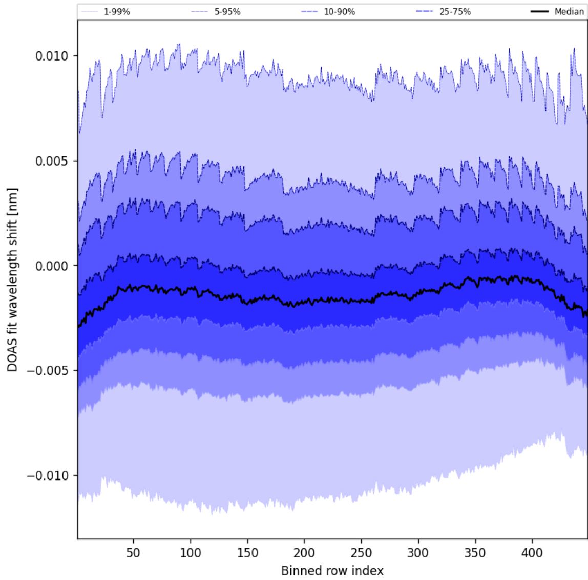
Figure 47: Along track statistics of “DOAS fit wavelength shift” for 2025-09-20 to 2025-09-21
