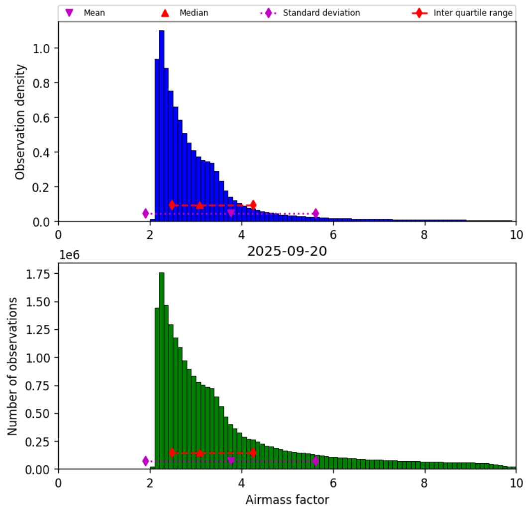
Figure 37: Histogram of “Airmass factor” for 2025-09-20 to 2025-09-21
