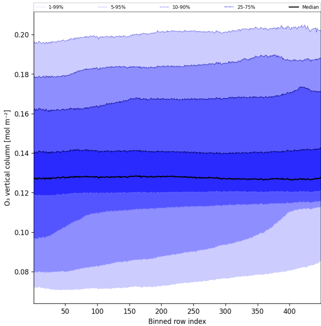
Figure 41: Along track statistics of “O 3 vertical column” for 2025-09-20 to 2025-09-21
