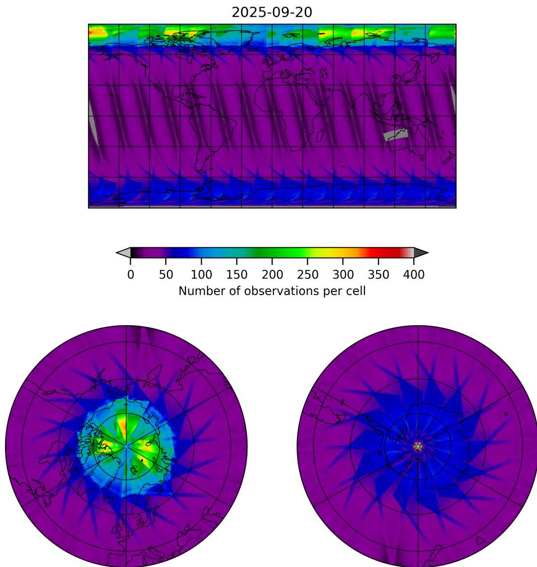
Figure 15: Map of the number of observations for 2025-09-20 to 2025-09-21
