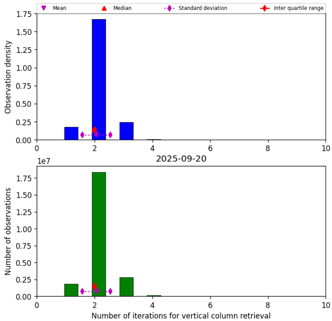
Figure 39: Histogram of “Number of iterations for vertical column retrieval” for 2025-09-20 to 2025-09-21
