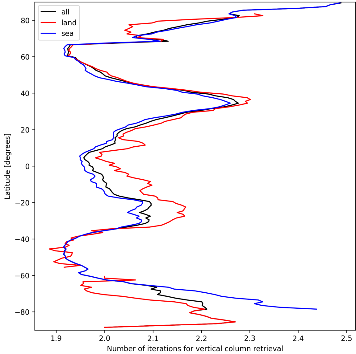
Figure 27: Zonal average of “Number of iterations for vertical column retrieval” for 2025-09-20 to 2025-09-21.
