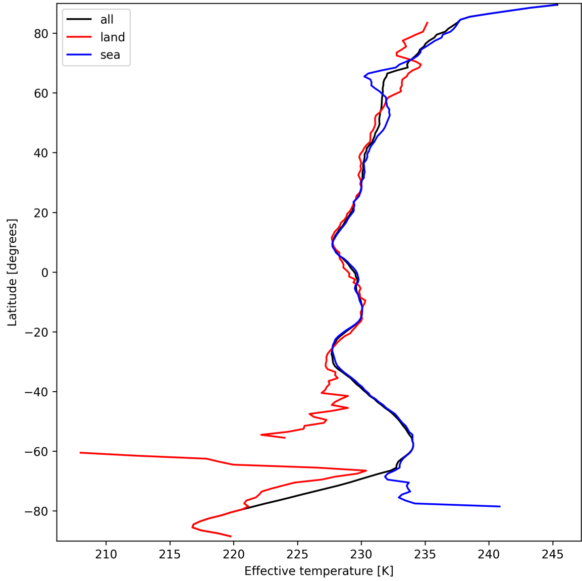
Figure 26: Zonal average of "Effective temperature" for 2025-09-20 to 2025-09-21.
