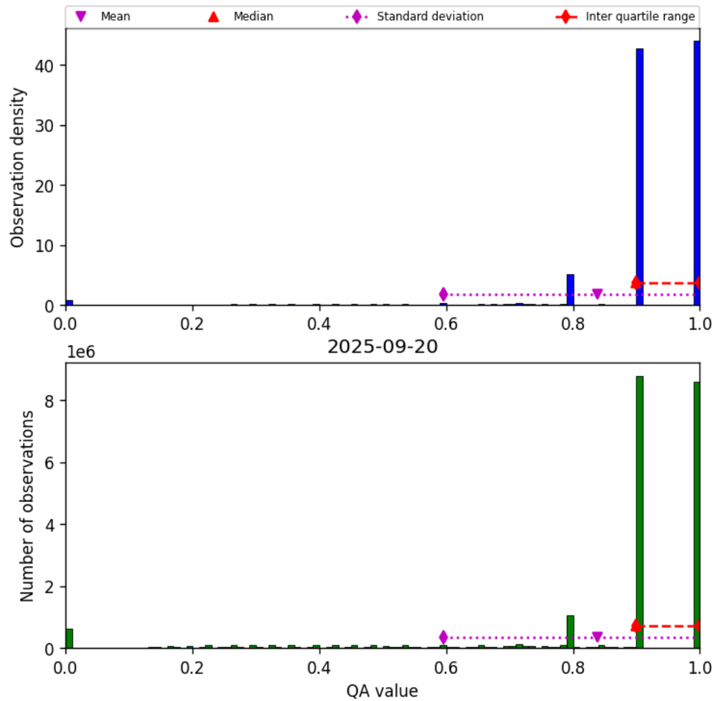
Figure 28: Histogram of “QA value” for 2025-09-20 to 2025-09-21
