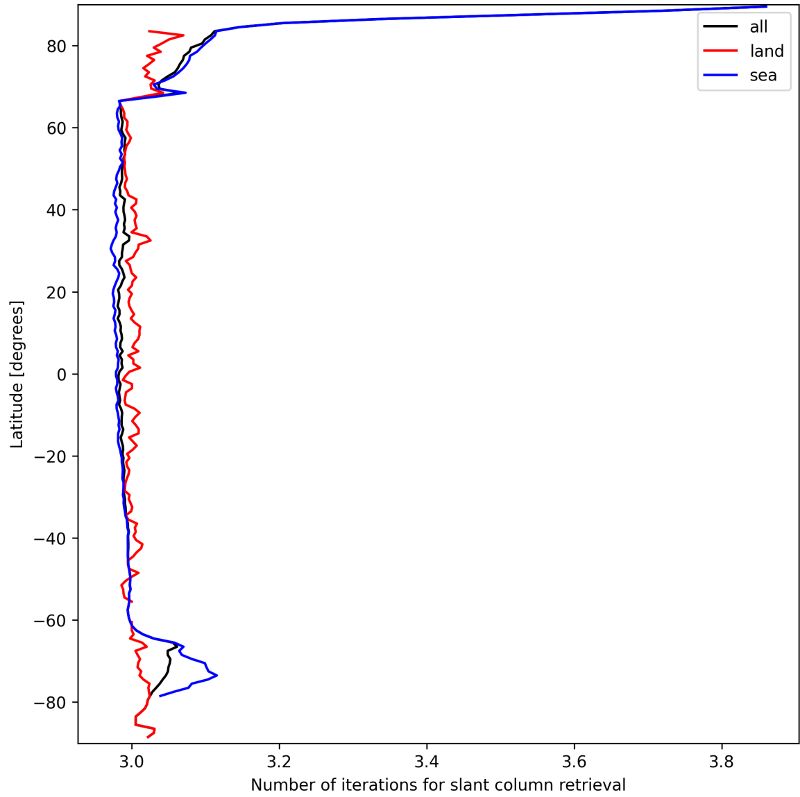
Figure 21: Zonal average of “Number of iterations for slant column retrieval” for 2025-09-20 to 2025-09-21.
