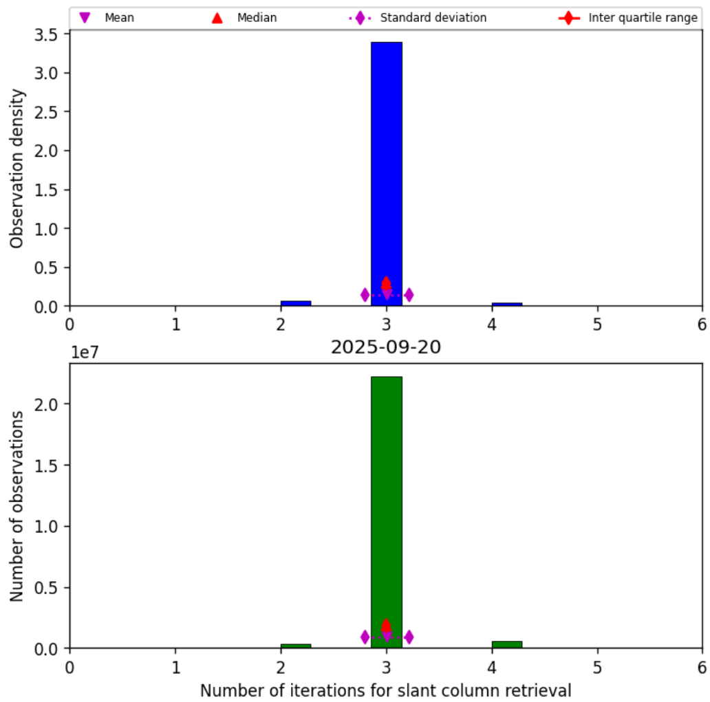
Figure 33: Histogram of “Number of iterations for slant column retrieval” for 2025-09-20 to 2025-09-21
