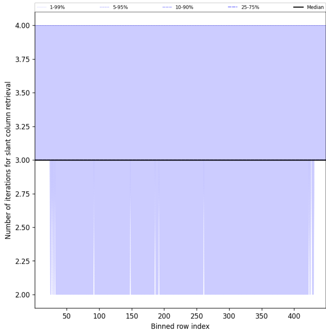
Figure 45: Along track statistics of “Number of iterations for slant column retrieval” for 2025-09-20 to 2025-09-21
