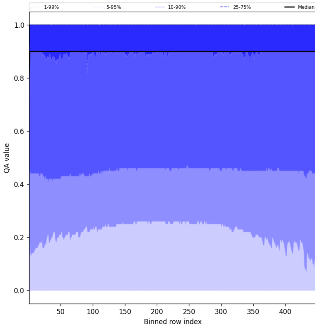
Figure 40: Along track statistics of “QA value” for 2025-09-20 to 2025-09-21
