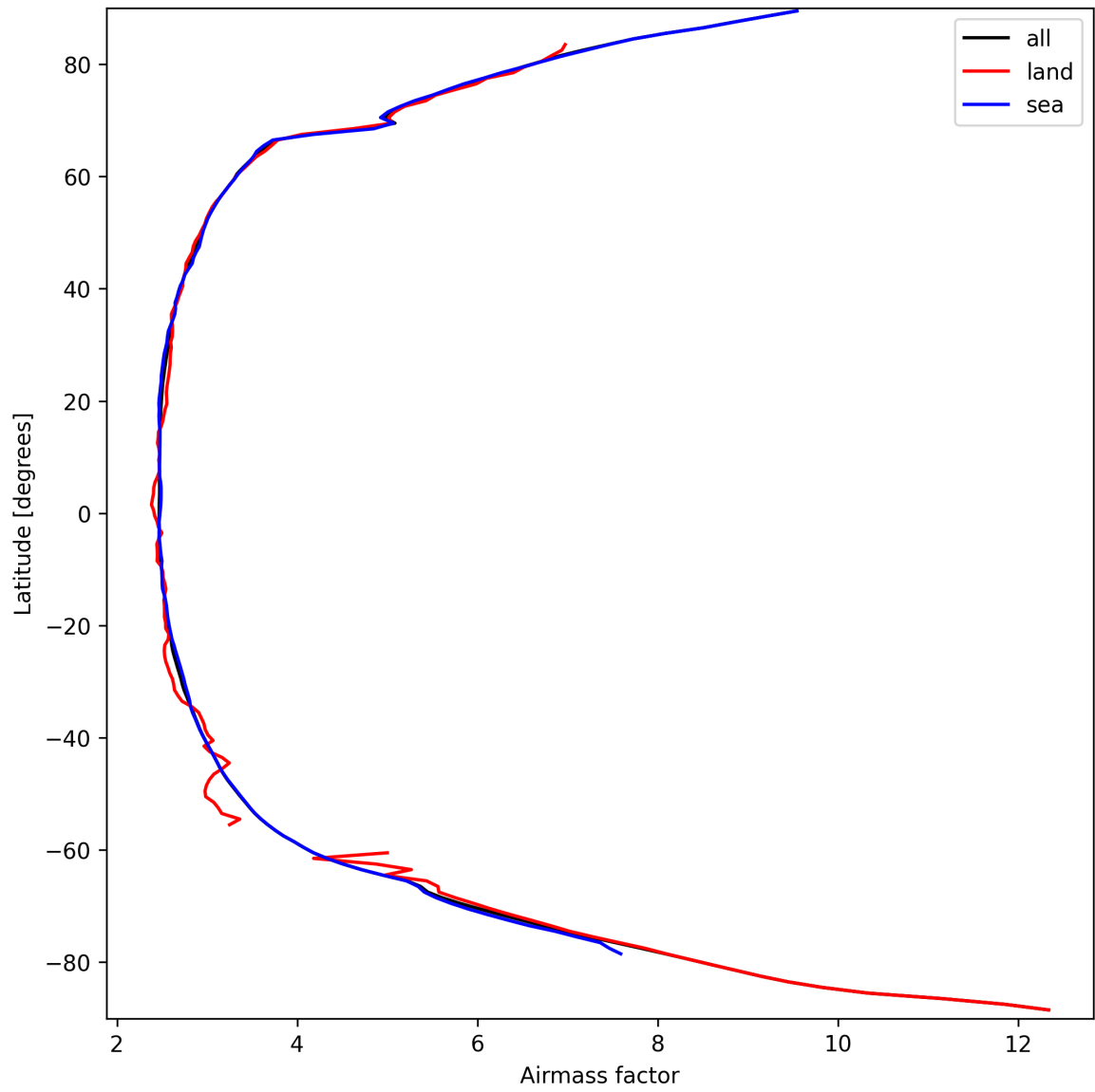
Figure 25: Zonal average of “Airmass factor” for 2025-09-20 to 2025-09-21.
