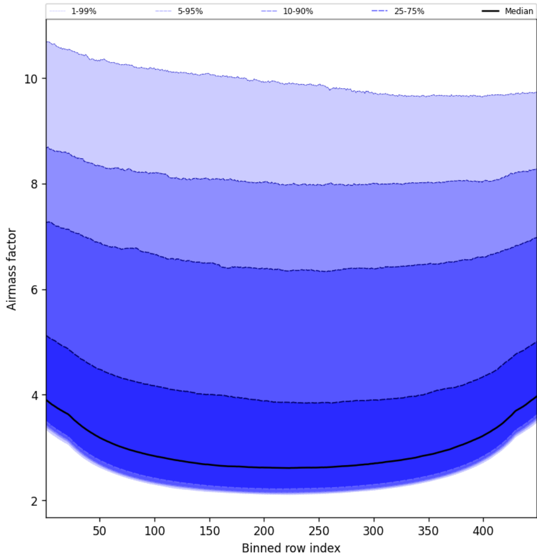
Figure 49: Along track statistics of “Airmass factor” for 2025-09-20 to 2025-09-21
