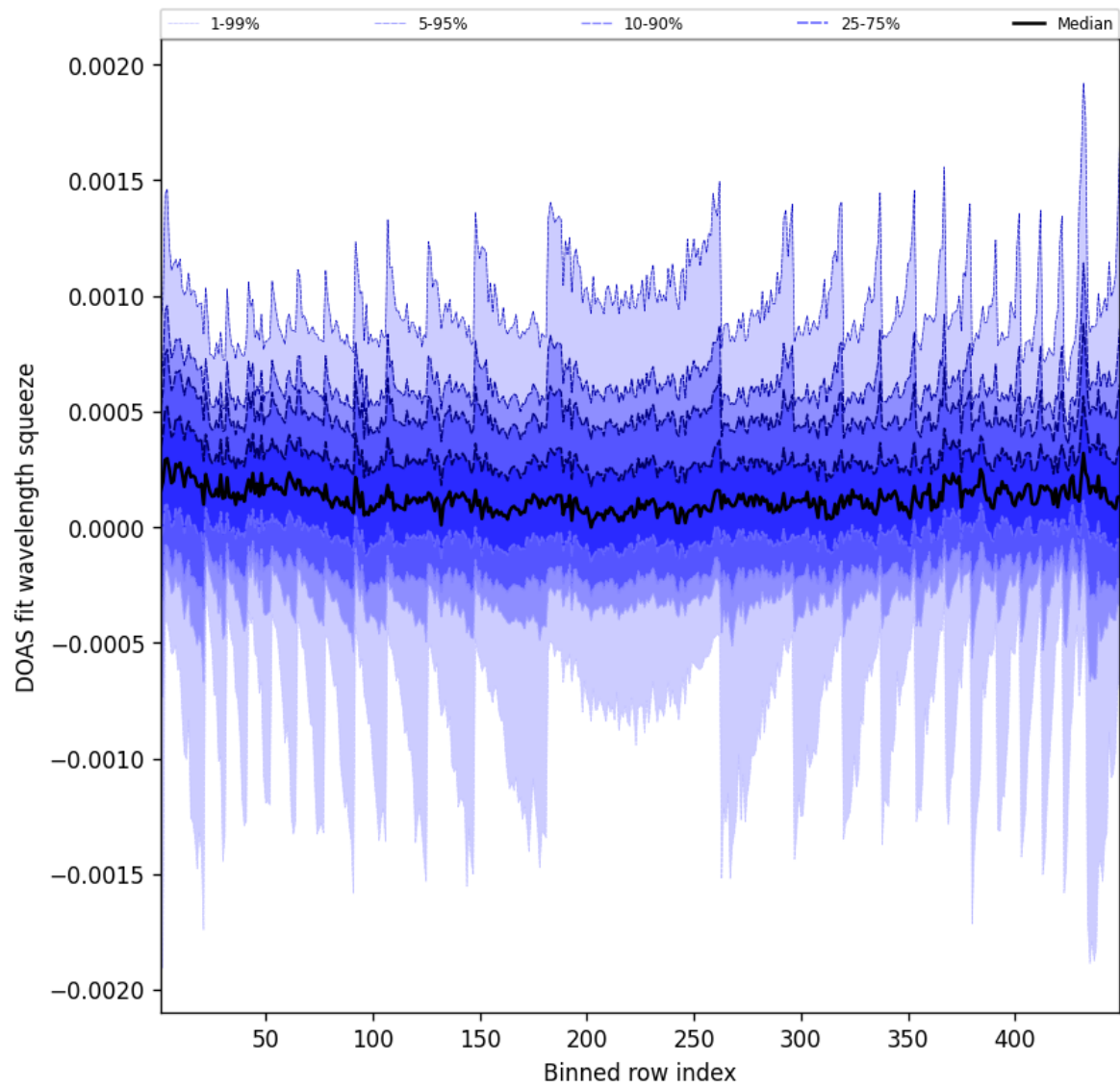
Figure 48: Along track statistics of “DOAS fit wavelength squeeze” for 2025-09-20 to 2025-09-21
