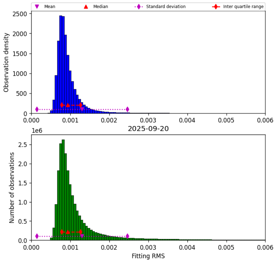
Figure 34: Histogram of “Fitting RMS” for 2025-09-20 to 2025-09-21
