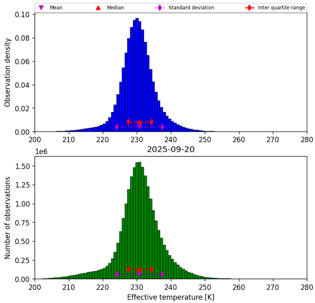
Figure 38: Histogram of “Effective temperature” for 2025-09-20 to 2025-09-21
