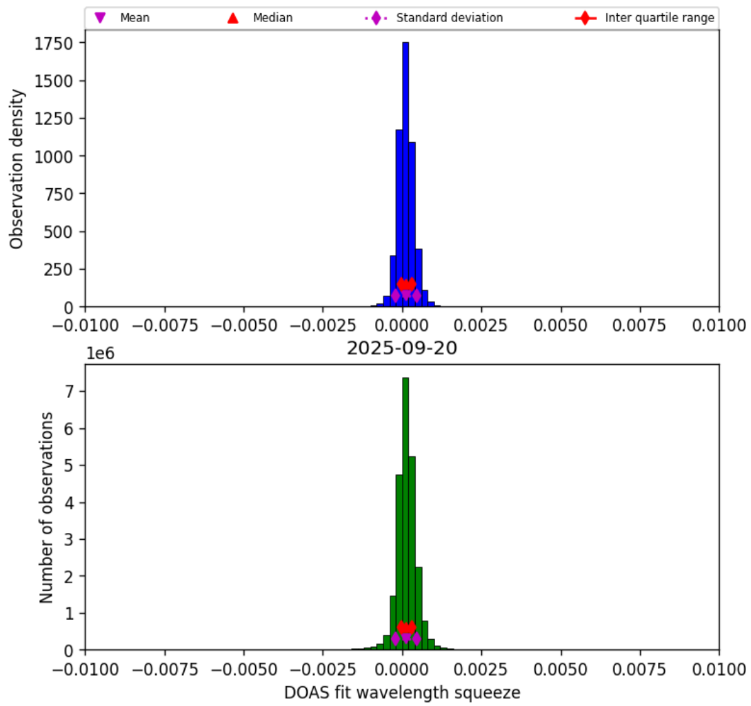
Figure 36: Histogram of “DOAS fit wavelength squeeze” for 2025-09-20 to 2025-09-21
