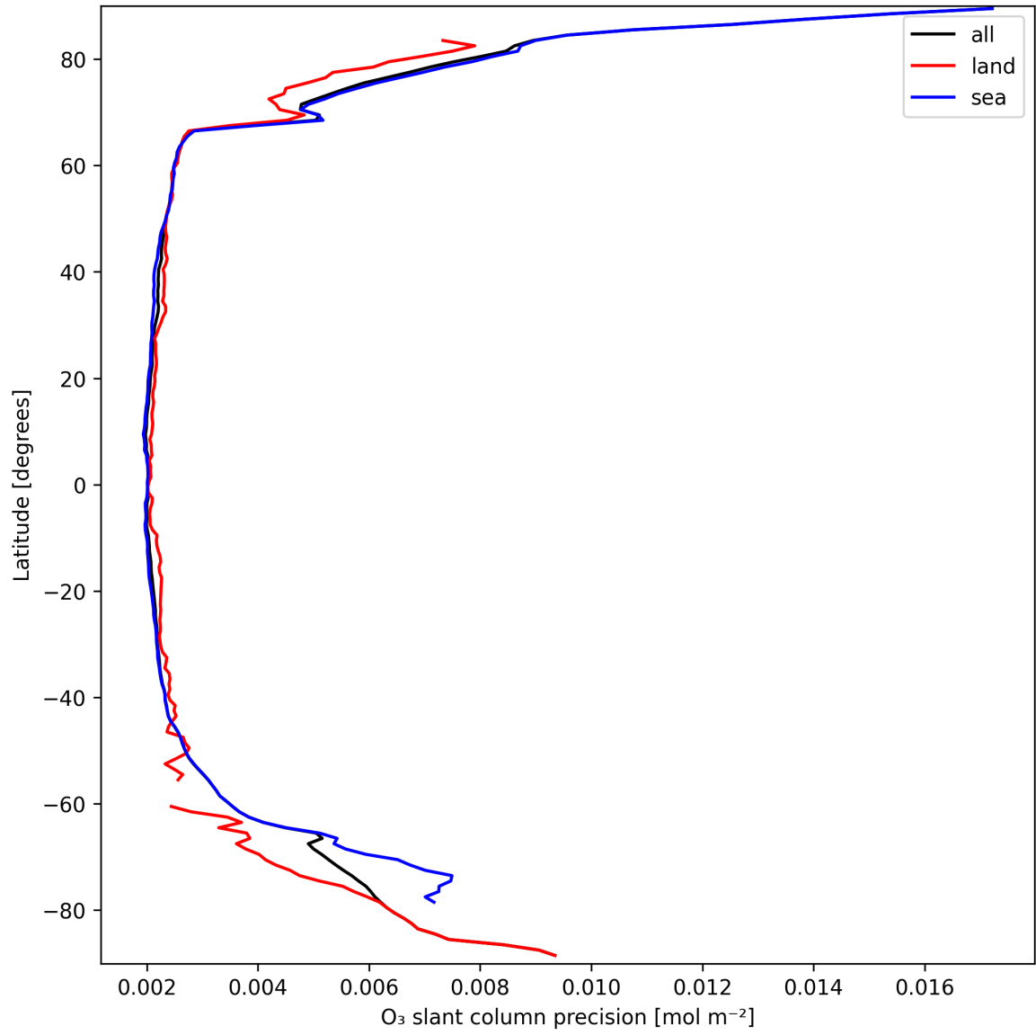
Figure 20: Zonal average of "O 3 slant column precision" for 2025-09-20 to 2025-09-21.
