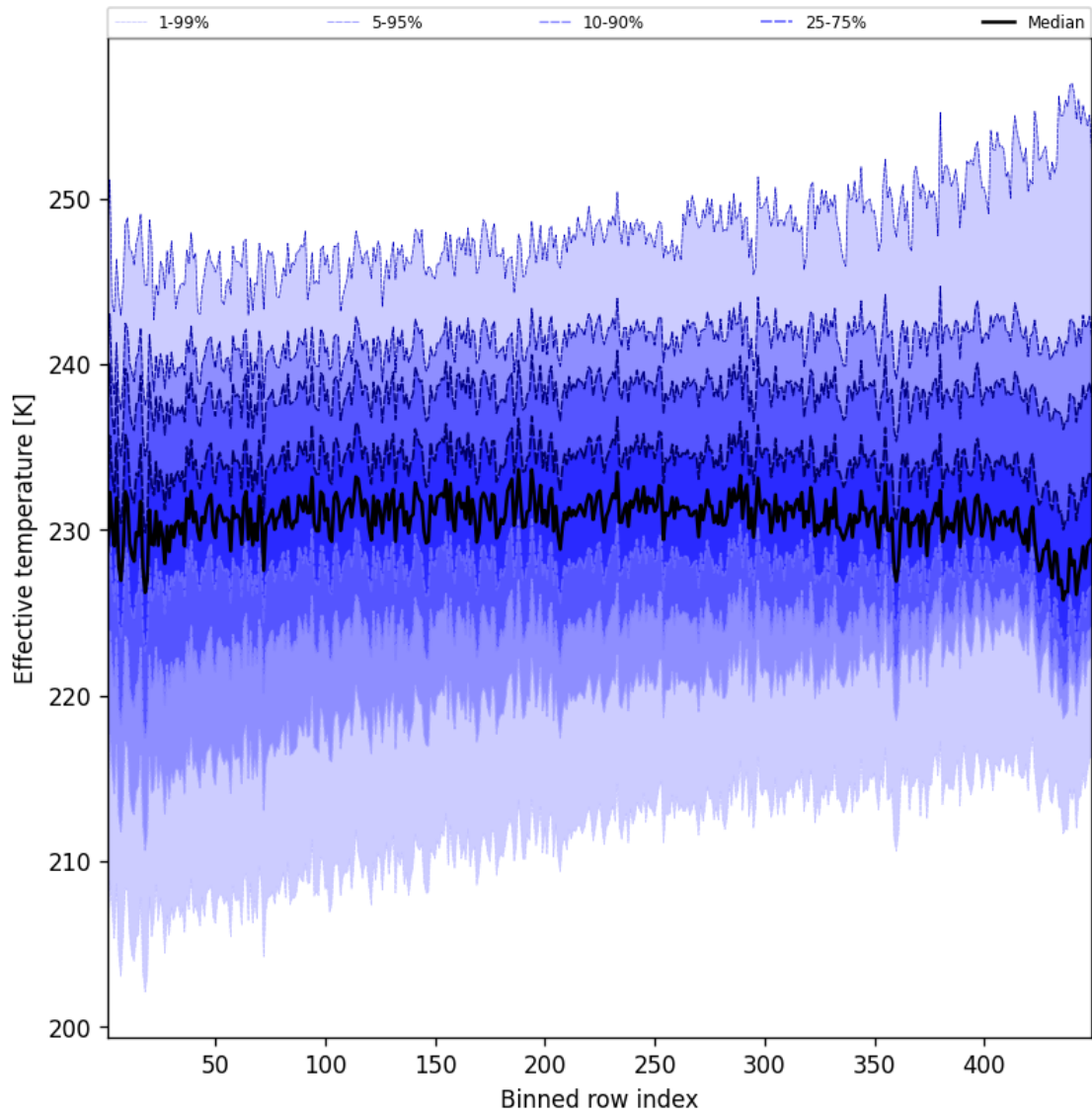
Figure 50: Along track statistics of “Effective temperature” for 2025-09-20 to 2025-09-21
