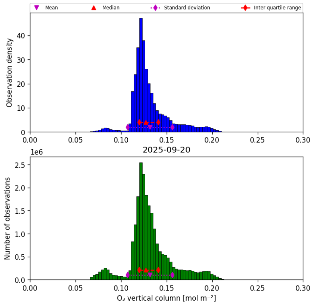
Figure 29: Histogram of “O 3 vertical column” for 2025-09-20 to 2025-09-21
