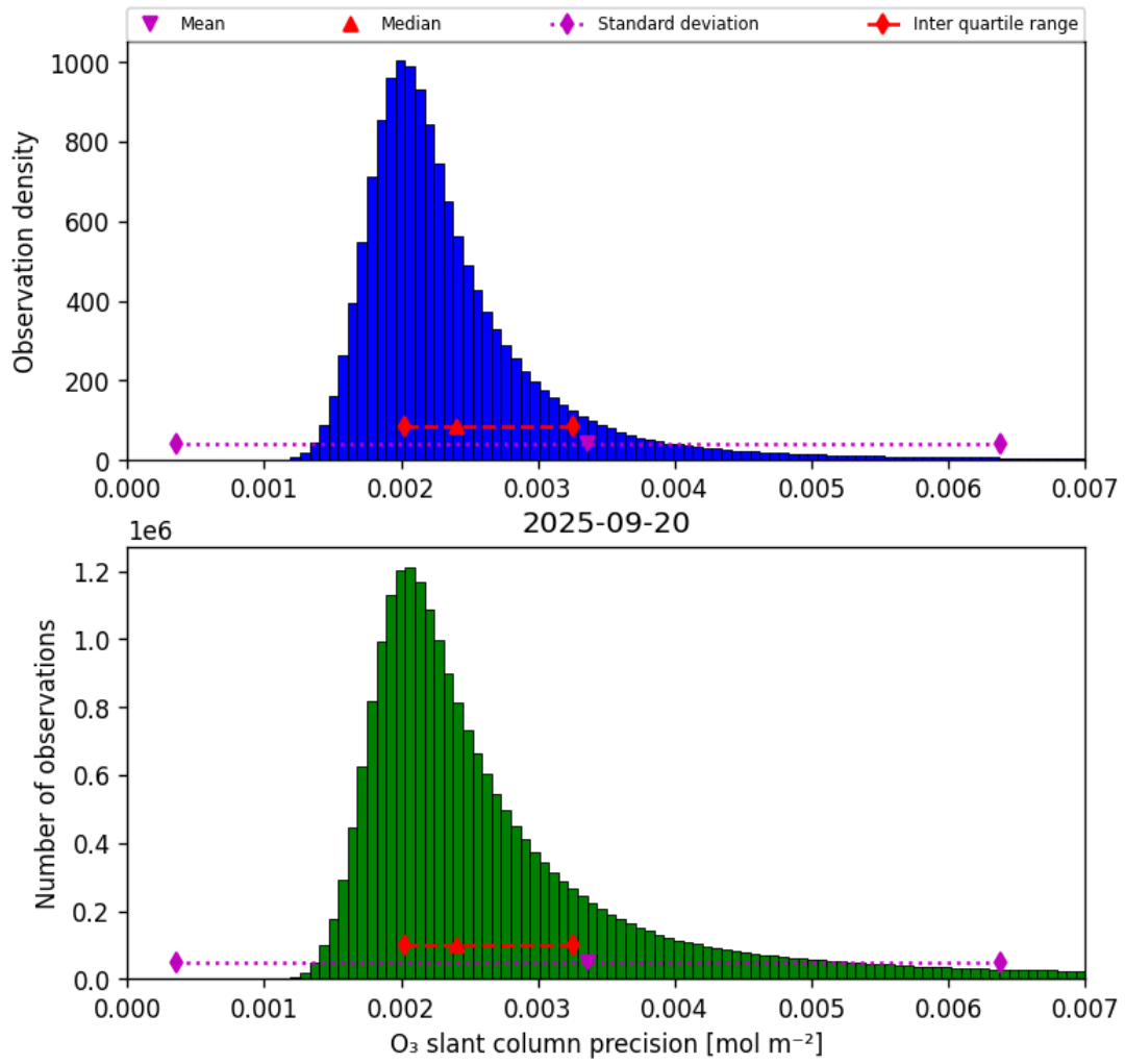
Figure 32: Histogram of “O 3 slant column precision” for 2025-09-20 to 2025-09-21
