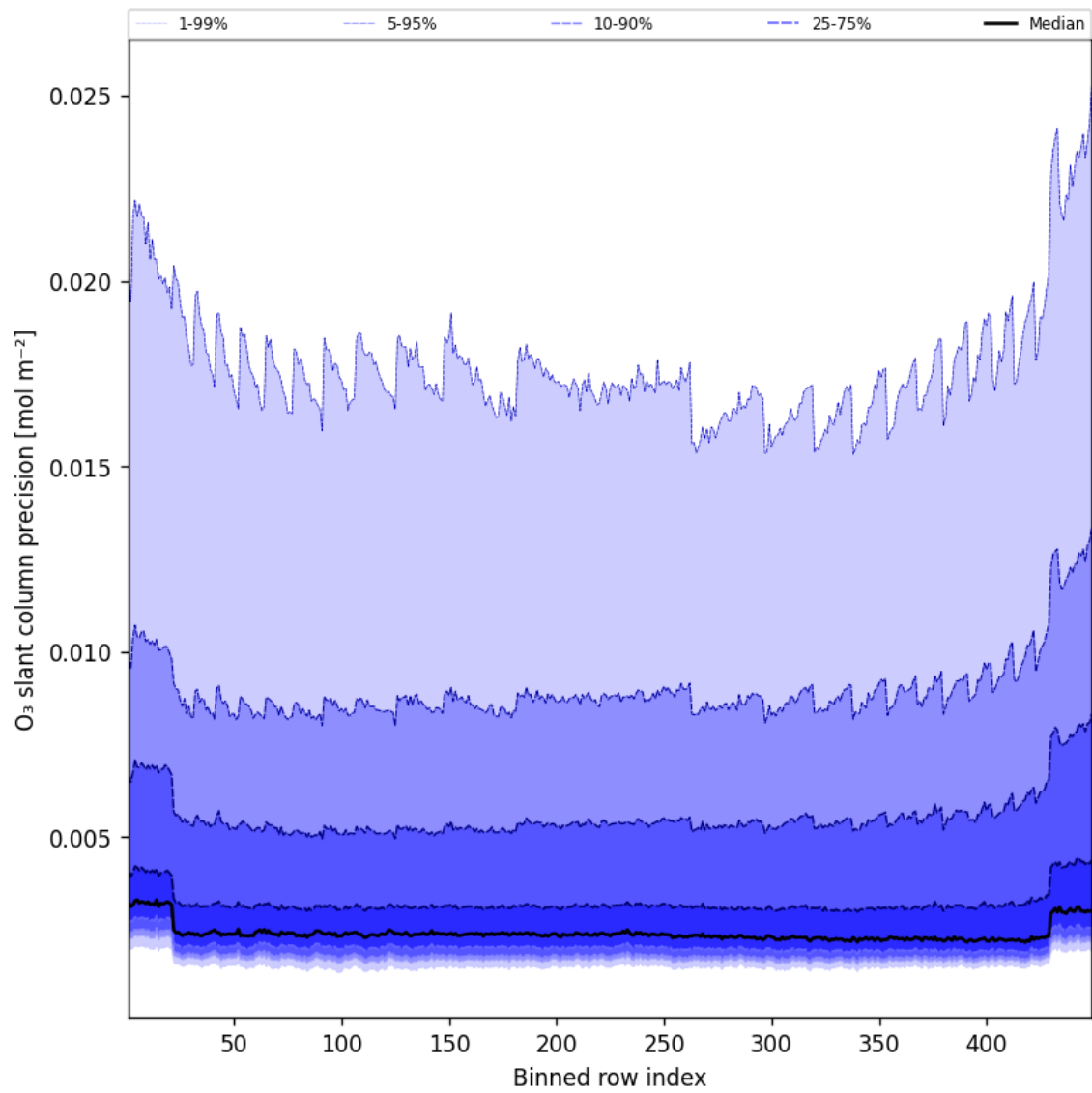
Figure 44: Along track statistics of “O 3 slant column precision” for 2025-09-20 to 2025-09-21
