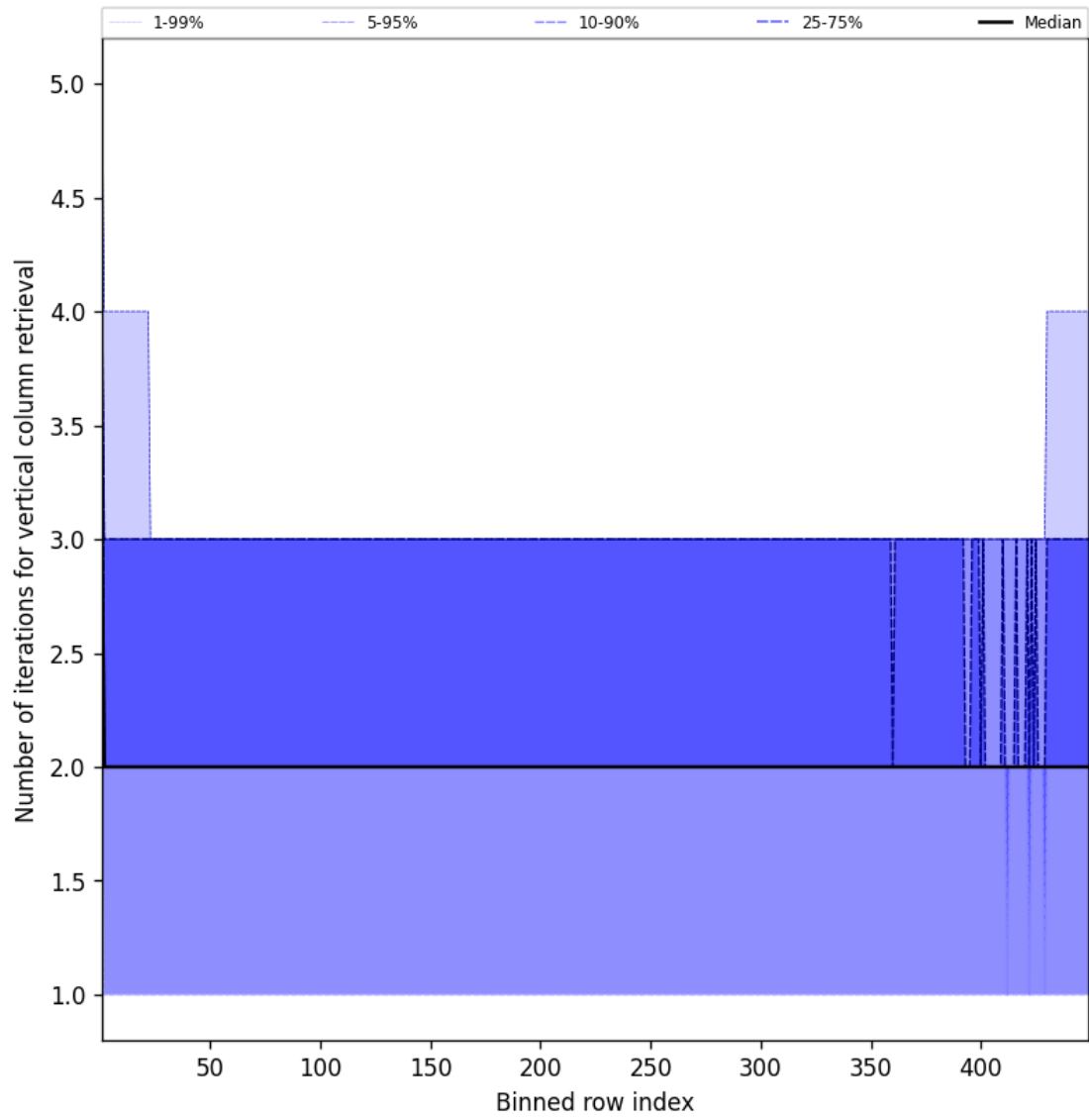
Figure 51: Along track statistics of “Number of iterations for vertical column retrieval” for 2025-09-20 to 2025-09-21
