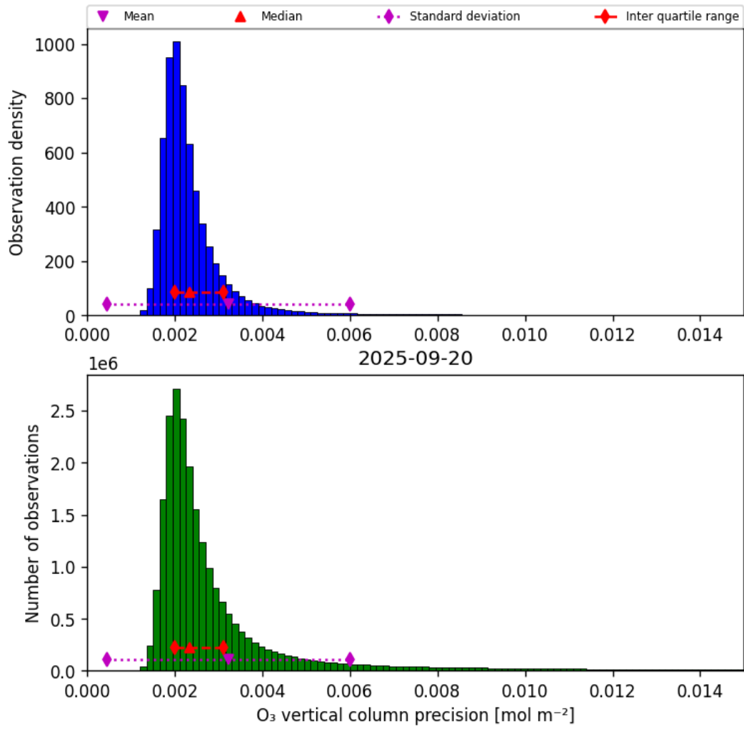
Figure 30: Histogram of “O 3 vertical column precision” for 2025-09-20 to 2025-09-21
