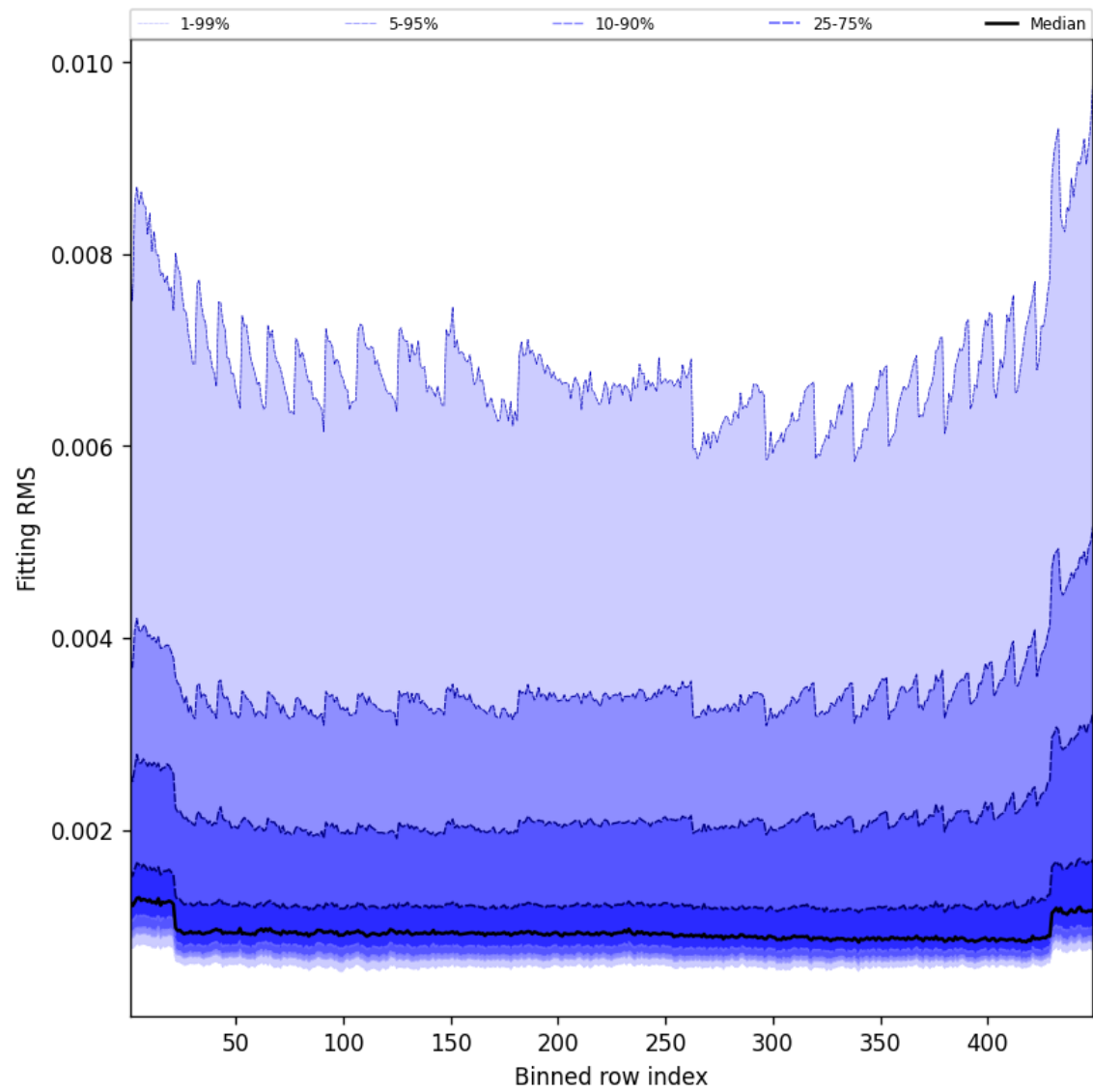
Figure 46: Along track statistics of “Fitting RMS” for 2025-09-20 to 2025-09-21
