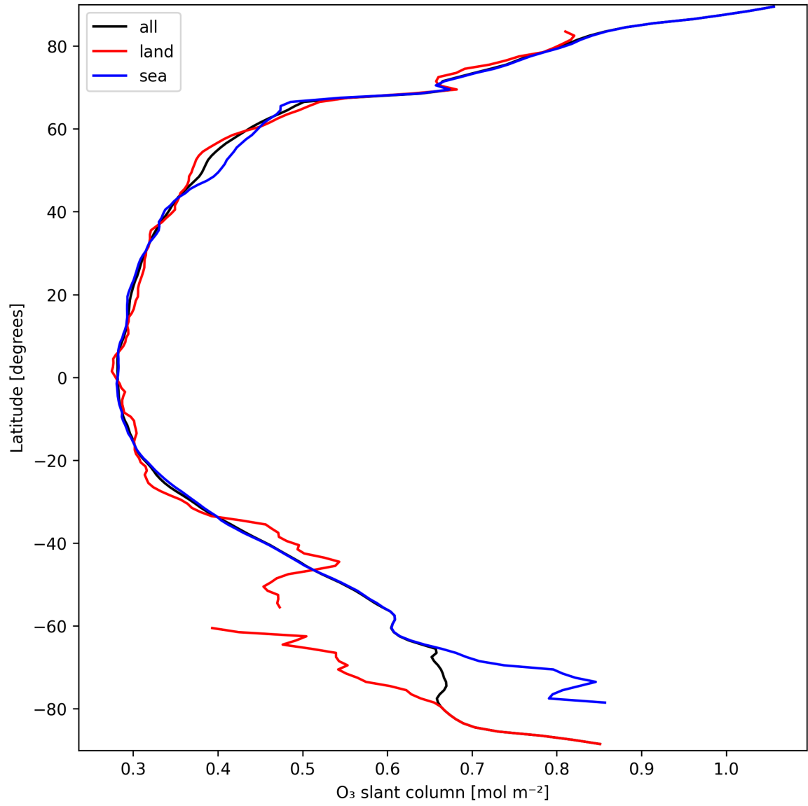
Figure 19: Zonal average of “O 3 slant column” for 2025-09-20 to 2025-09-21.
