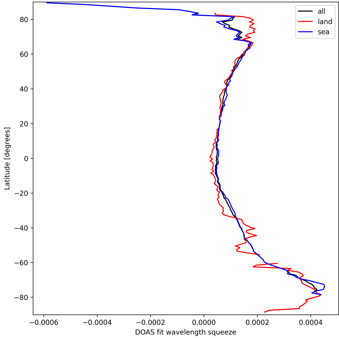
Figure 24: Zonal average of “DOAS fit wavelength squeeze” for 2025-09-20 to 2025-09-21.
