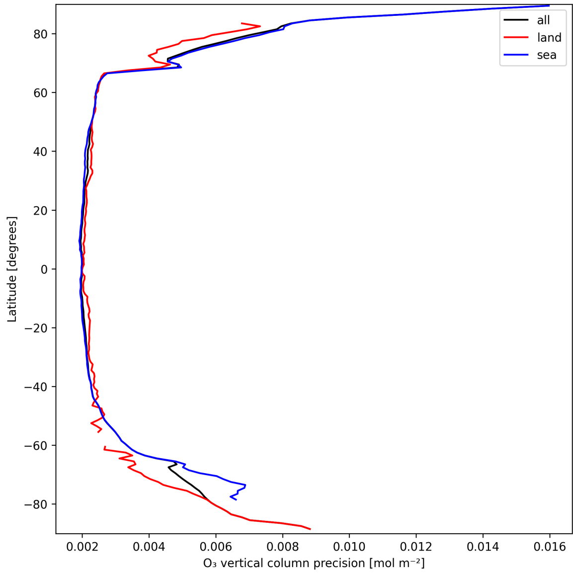
Figure 18: Zonal average of “O 3 vertical column precision” for 2025-09-20 to 2025-09-21.
